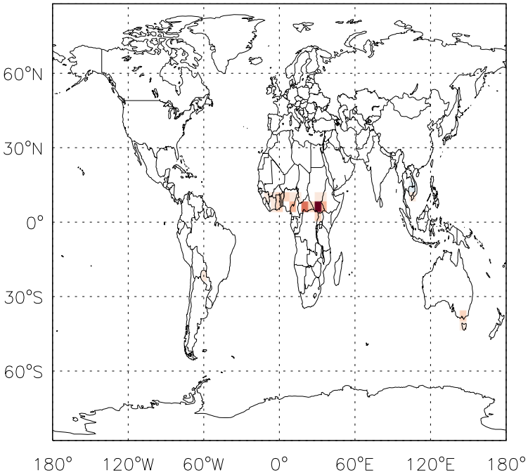
v11-01f-merra2-Run0 - v11-01d-Run1 CH 2 O biomass emissions for Jan
