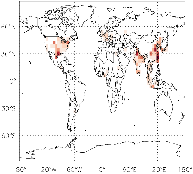
v11-01f-merra2-Run0 - v11-01d-Run1 CH 2 O anthro+biofuel emissions for Jan
