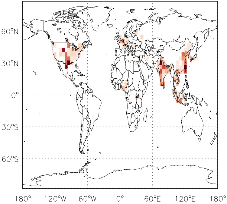
v11-01f-merra2-Run0 - v11-01d-Run1 CH 2 O anthro+biofuel emissions for Oct
