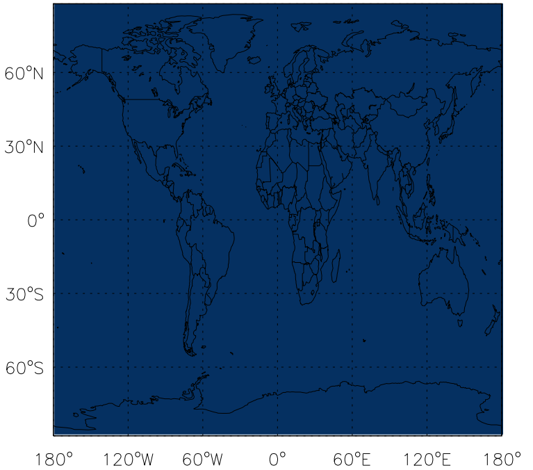
v11-01f-merra2-Run0 - v11-01f-geosp-Run0 CH 2 O biomass emissions for Oct
