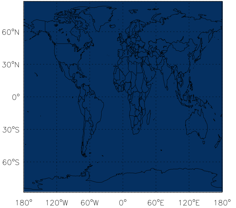
v11-01f-merra2-Run0 - v11-01f-geosp-Run0 CH 2 O anthro+biofuel emissions for Oct
