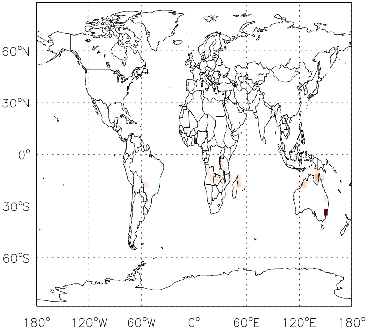
v11-01f-merra2-Run0 - v11-01d-Run1 CH 2 O biomass emissions for Oct
