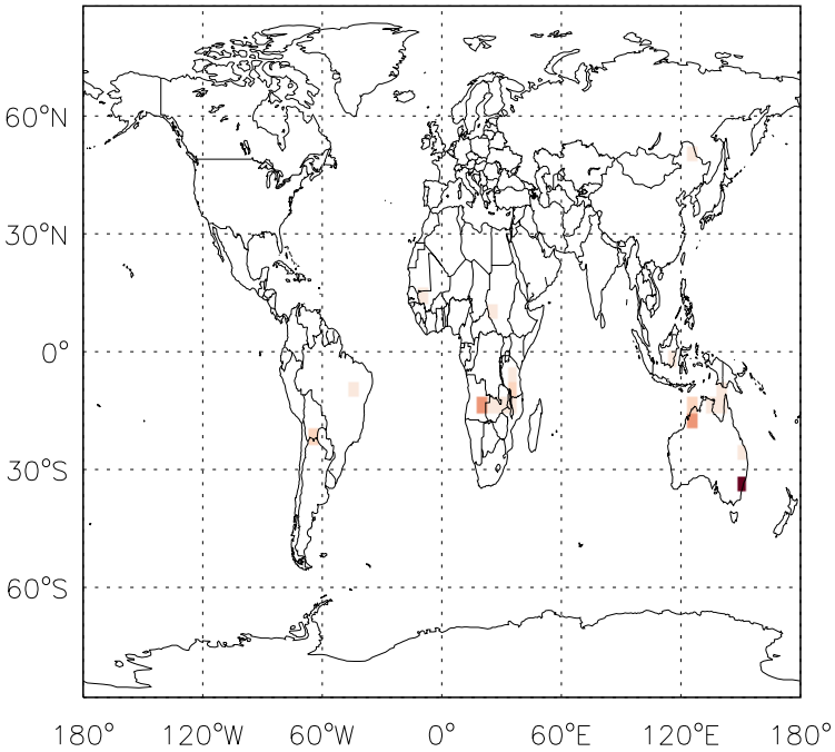
v11-01f-merra2-Run0 - v11-01d-Run1 CO biomass emissions for Oct
