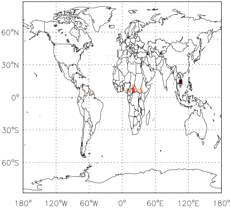
v11-01f-merra2-Run0 - v11-01d-Run1 PRPE biomass emissions for Jan
