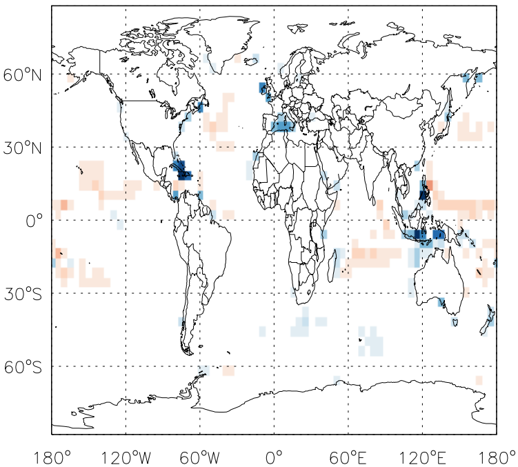
v11-01f-merra2-Run0 - v11-01d-Run1 Coarse-mode sea salt emissions for Jan
