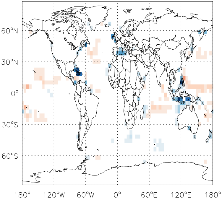
v11-01f-merra2-Run0 - v11-01d-Run1 Accum-mode sea salt emissions for Jan
