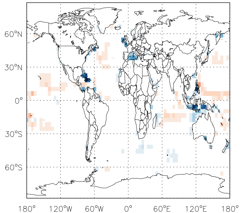
v11-01f-merra2-Run0 - v11-01f-geosp-Run0 Coarse-mode sea salt emissions for Jan
