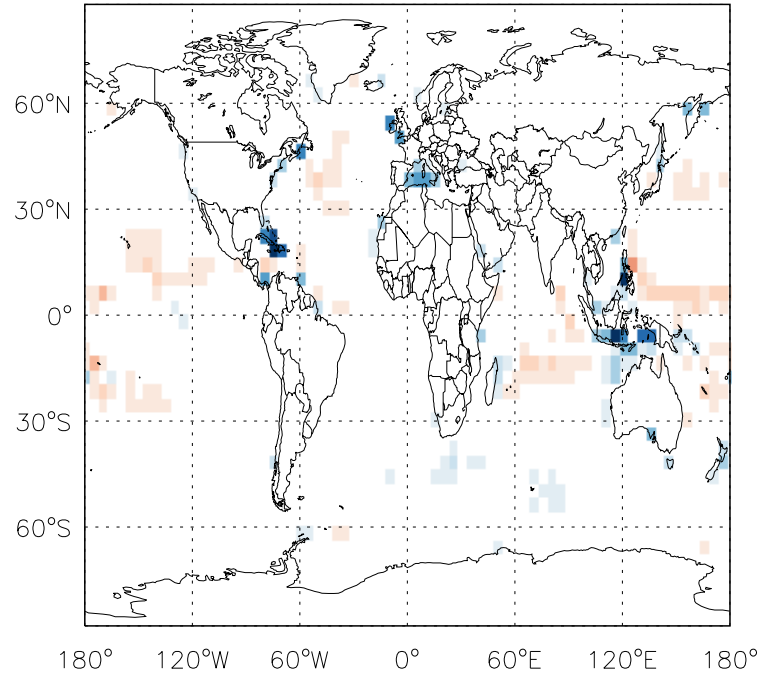
v11-01f-merra2-Run0 - v11-01f-geosp-Run0 Accum-mode sea salt emissions for Jan
