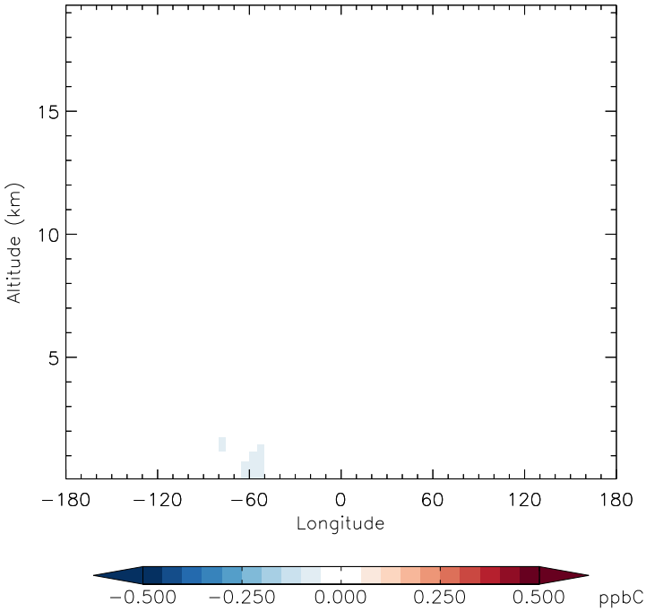
v11-01f-merra2-Run0 - v11-01f-geosfp-Run0 C2H6 - Diff along 15S for Apr
