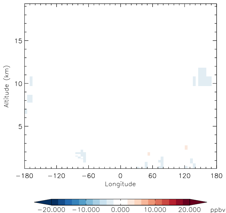
v11-01f-merra2-Run0 - v11-01f-geosfp-Run0 CO - Diff along 42N for Apr
