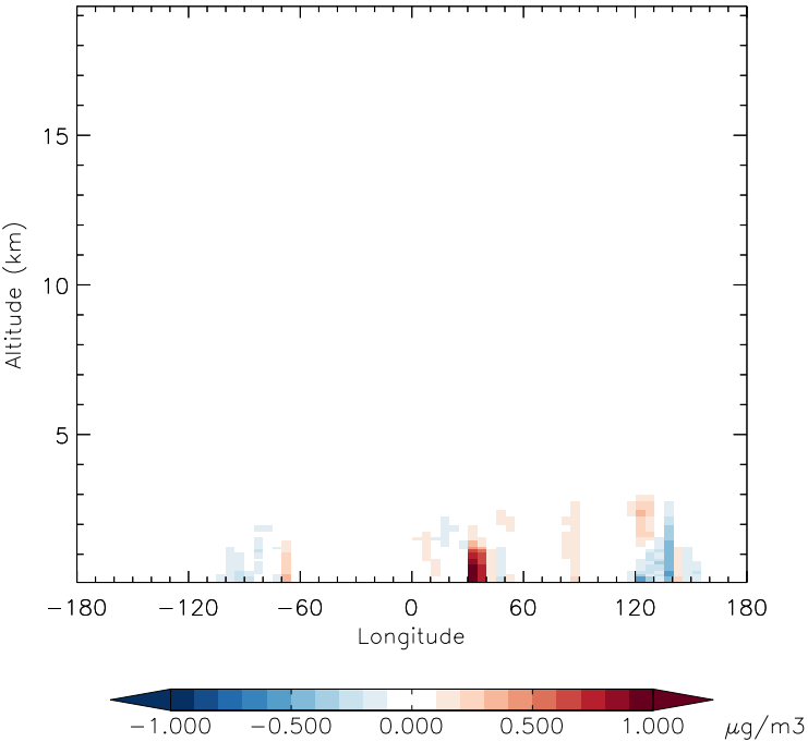
v11-01f-merra2-Run0 - v11-01d-Run1 NIT - Diff along 42N for Apr
