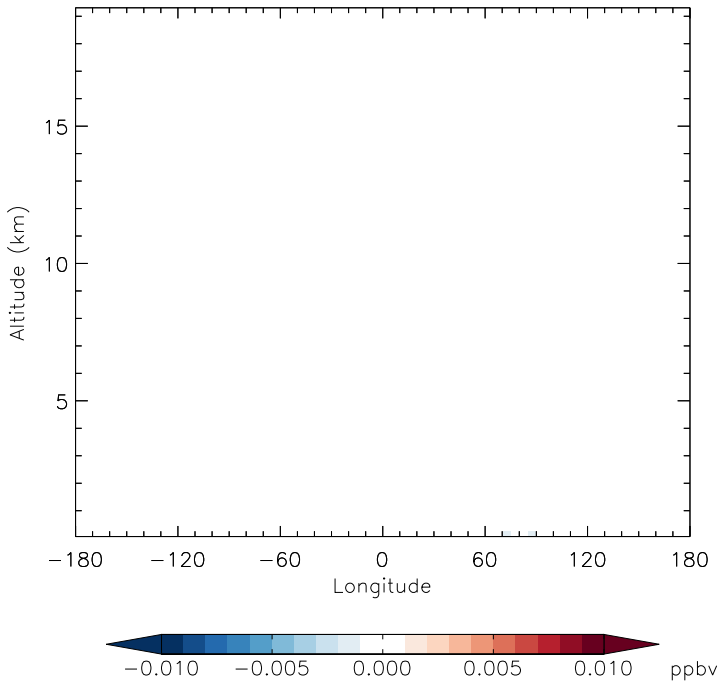
v11-01f-merra2-Run0 - v11-01d-Run1 NO3 - Diff along 42N for Apr
