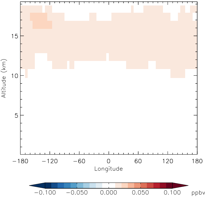
v11-01f-merra2-Run0 - v11-01f-geosfp-Run0 HCl - Diff along 42N for Apr
