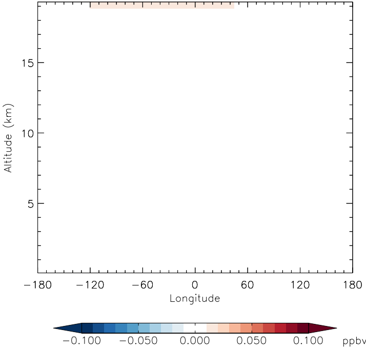
v11-01f-merra2-Run0 - v11-01d-Run1 CFC11 - Diff along 15S for Apr
