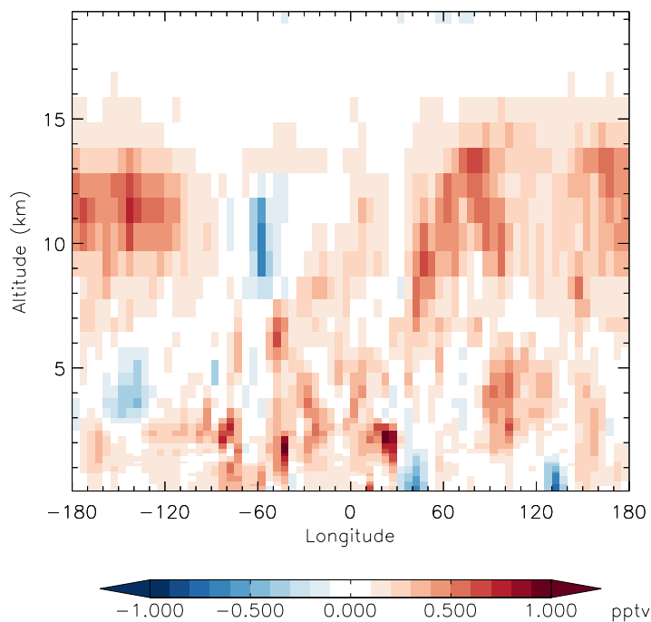
v11-01f-merra2-Run0 - v11-01d-Run1 HO2 - Diff along 15S for Apr
