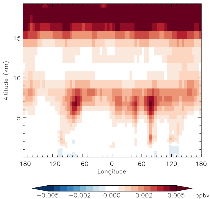
v11-01f-merra2-Run0 - v11-01d-Run1 HNO 4 - Diff along 42N for Apr
