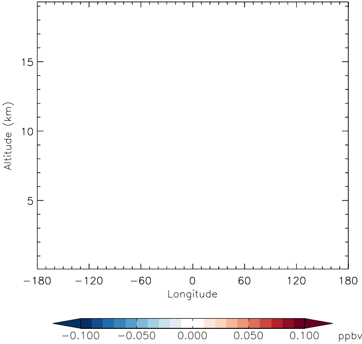
v11-01f-merra2-Run0 - v11-01d-Run1 BrCl - Diff along 42N for Apr
