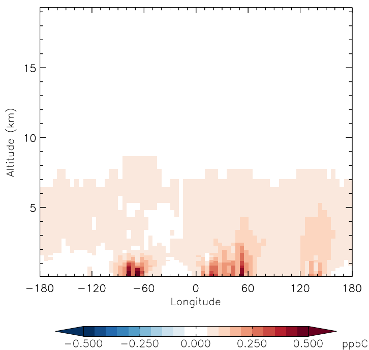
v11-01f-merra2-Run0 - v11-01d-Run1 ACET - Diff along 42N for Apr
