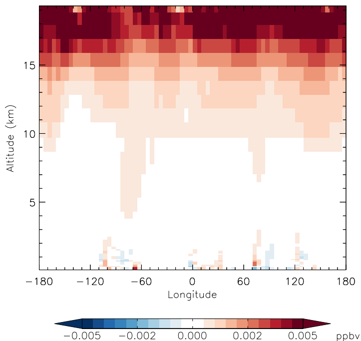
v11-01f-merra2-Run0 - v11-01f-geosfp-Run0 N2O5 - Diff along 42N for Apr
