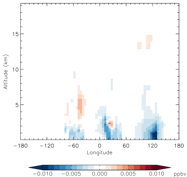
v11-01f-merra2-Run0 - v11-01d-Run1 R4N2 - Diff along 15S for Apr
