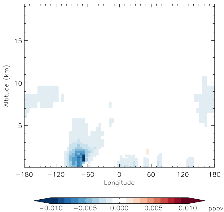
v11-01f-merra2-Run0 - v11-01d-Run1 R4N2 - Diff along 42N for Apr
