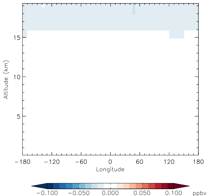
v11-01f-merra2-Run0 - v11-01f-geosfp-Run0 OCS - Diff along 42N for Apr
