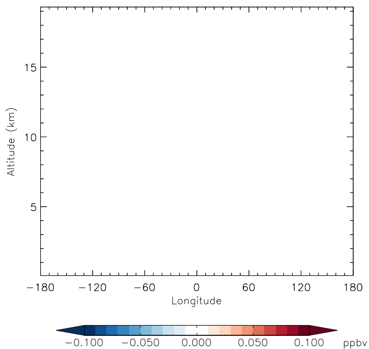
v11-01f-merra2-Run0 - v11-01f-geosfp-Run0 ISOPN - Diff along 15S for Apr
