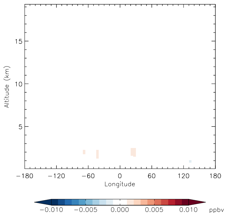
v11-01f-merra2-Run0 - v11-01f-geosfp-Run0 PMN - Diff along 15S for Apr
