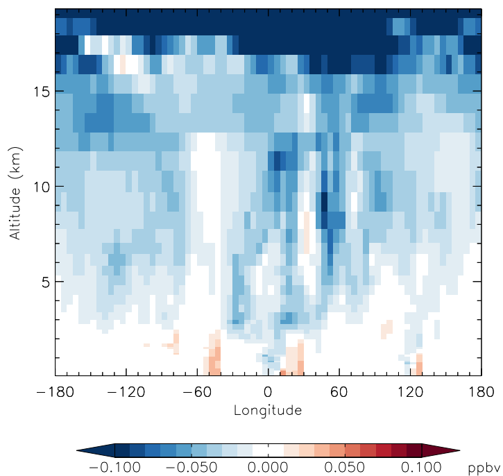
v11-01f-merra2-Run0 - v11-01d-Run1 HNO 3 - Diff along 15S for Apr
