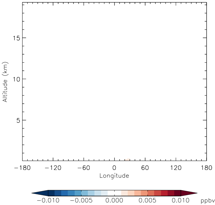
v11-01f-merra2-Run0 - v11-01f-geosfp-Run0 NO3 - Diff along 15S for Apr
