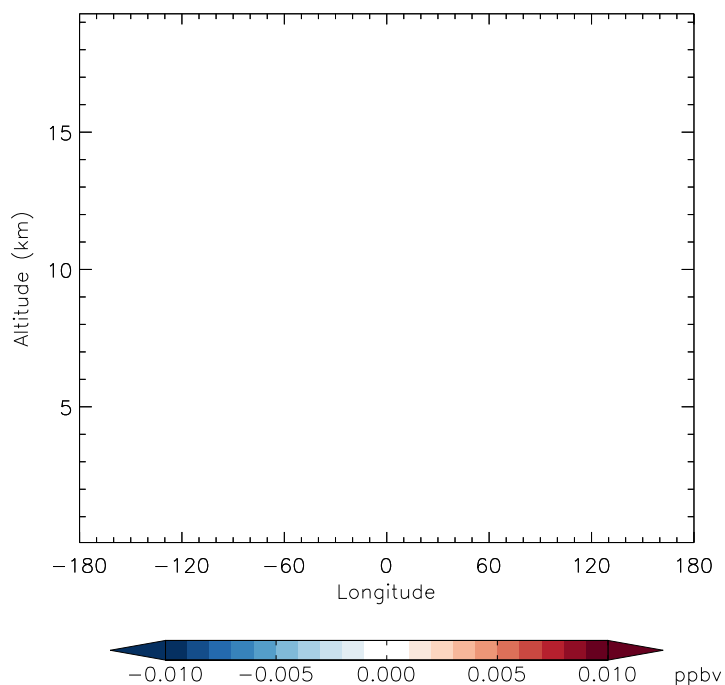
v11-01f-merra2-Run0 - v11-01f-geosfp-Run0 BrNO2 - Diff along 15S for Apr
