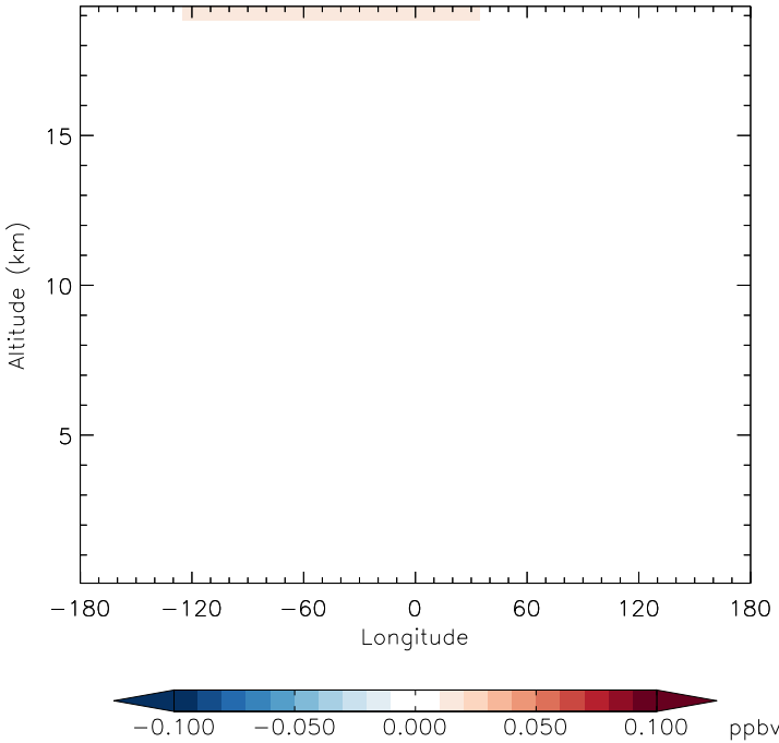
v11-01f-merra2-Run0 - v11-01d-Run1 CFC12 - Diff along 15S for Apr
