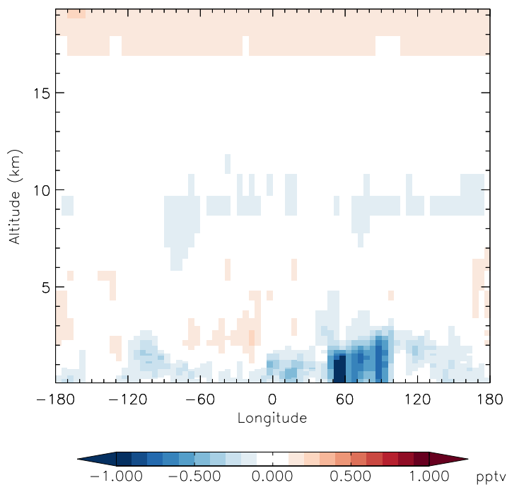
v11-01f-merra2-Run0 - v11-01d-Run1 HO2 - Diff along 42N for Apr
