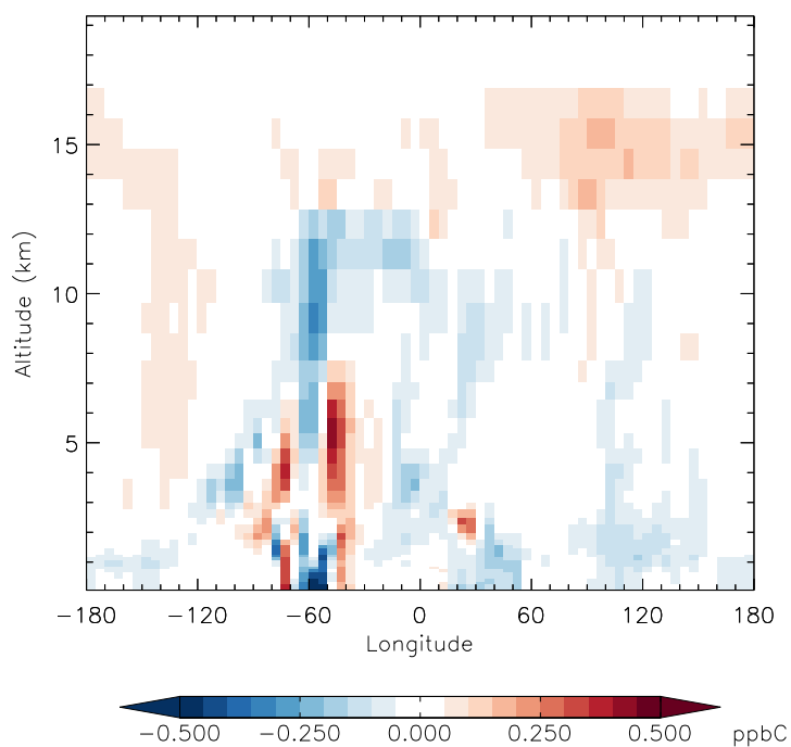
v11-01f-merra2-Run0 - v11-01d-Run1 ACET - Diff along 15S for Apr
