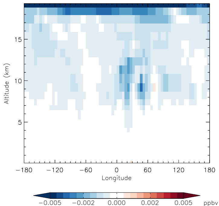
v11-01f-merra2-Run0 - v11-01f-geosfp-Run0 N2O5 - Diff along 15S for Apr
