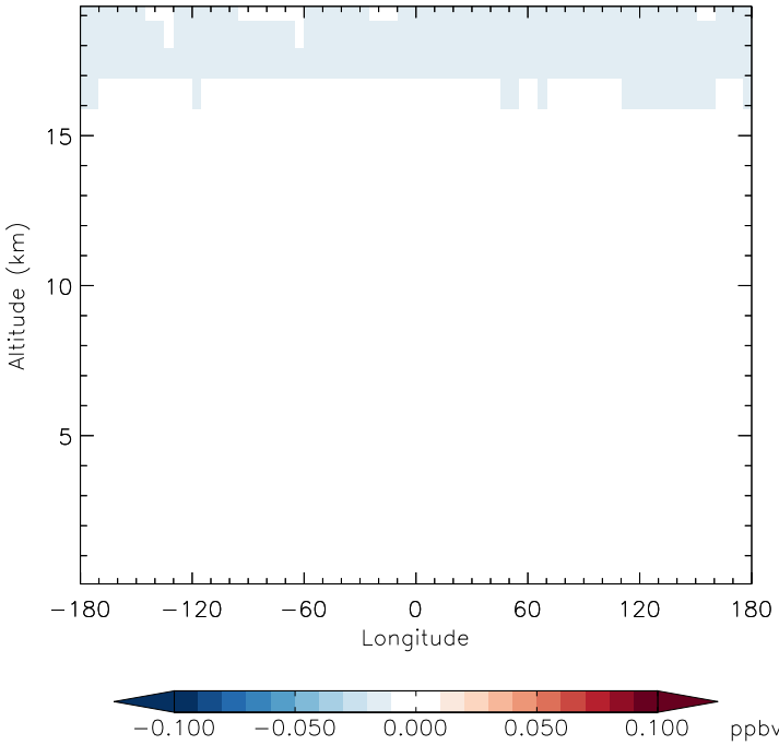
v11-01f-merra2-Run0 - v11-01f-geosfp-Run0 CFC12 - Diff along 42N for Apr
