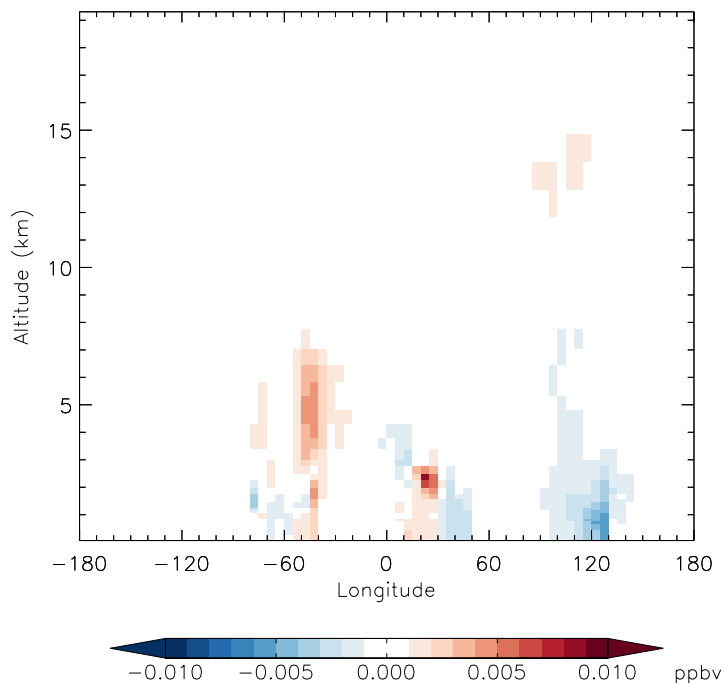
v11-01f-merra2-Run0 - v11-01f-geosfp-Run0 R4N2 - Diff along 15S for Apr
