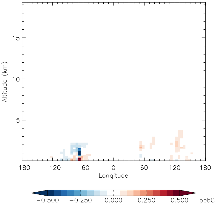
v11-01f-merra2-Run0 - v11-01f-geosfp-Run0 ALK4 - Diff along 42N for Apr
