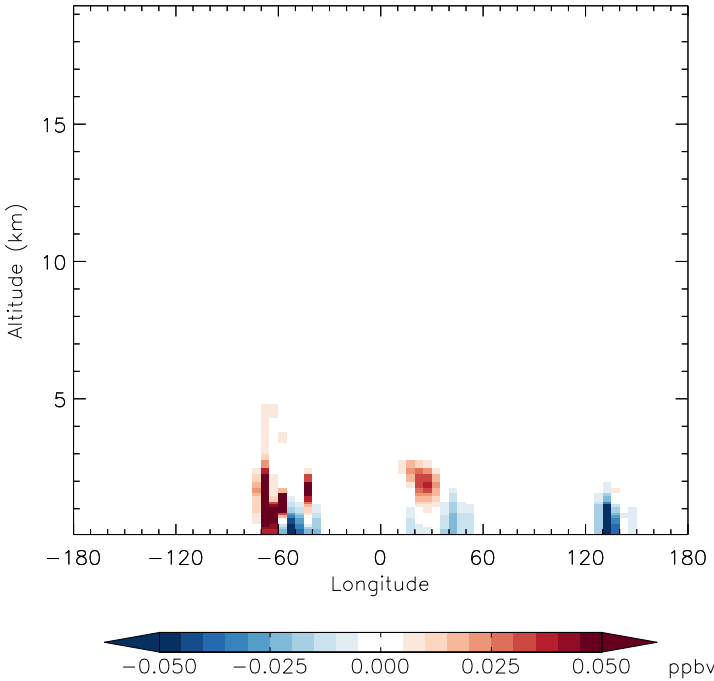
v11-01f-merra2-Run0 - v11-01d-Run1 MVK - Diff along 15S for Apr
