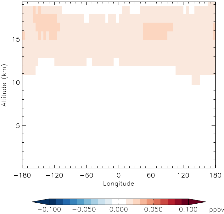
v11-01f-merra2-Run0 - v11-01d-Run1 HCl - Diff along 42N for Apr
