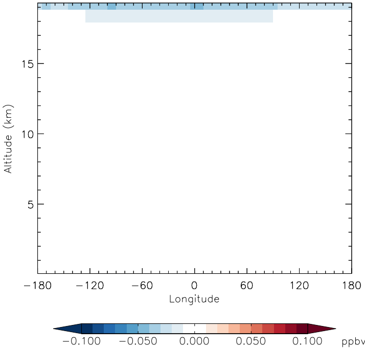
v11-01f-merra2-Run0 - v11-01f-geosfp-Run0 CINO3 - Diff along 15S for Apr
