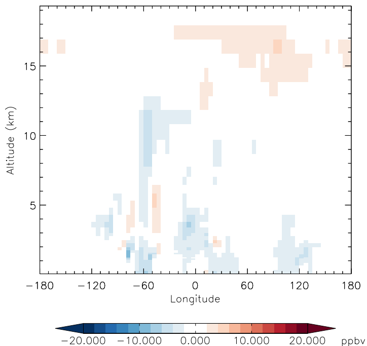
v11-01f-merra2-Run0 - v11-01f-geosfp-Run0 CO - Diff along 15S for Apr
