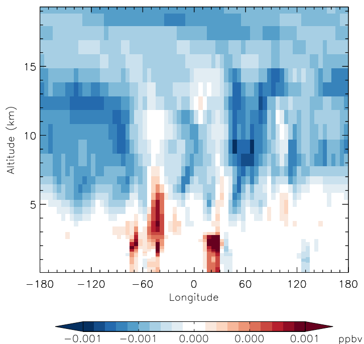
v11-01f-merra2-Run0 - v11-01f-geosfp-Run0 PPN - Diff along 15S for Apr
