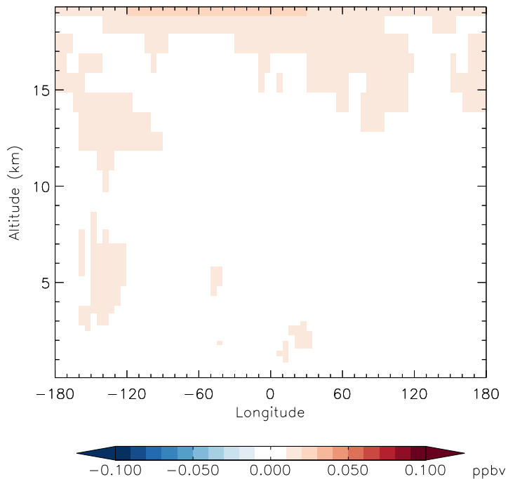
v11-01f-merra2-Run0 - v11-01d-Run1 CH 3 Cl - Diff along 15S for Apr
