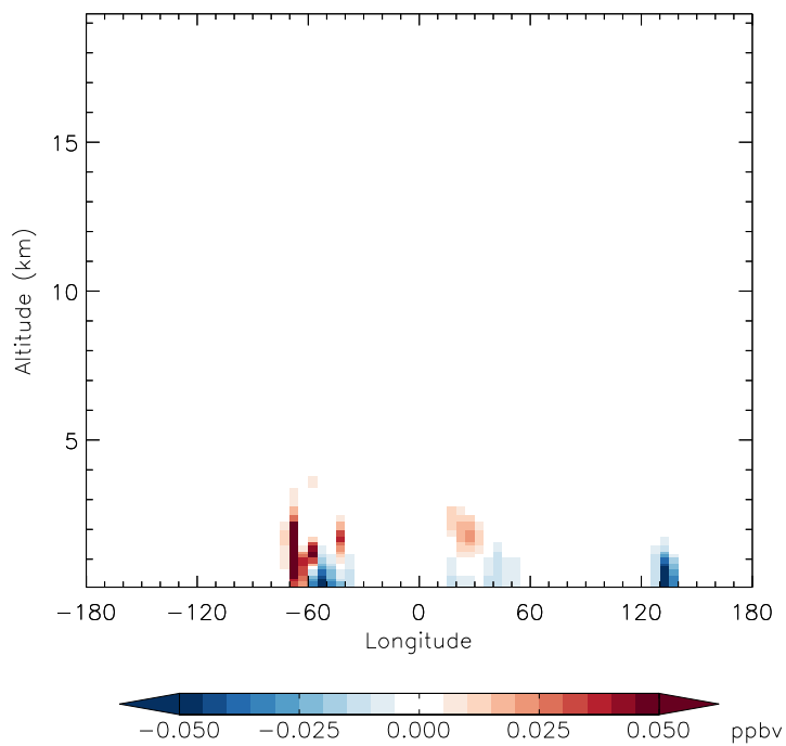
v11-01f-merra2-Run0 - v11-01d-Run1 MACR - Diff along 15S for Apr
