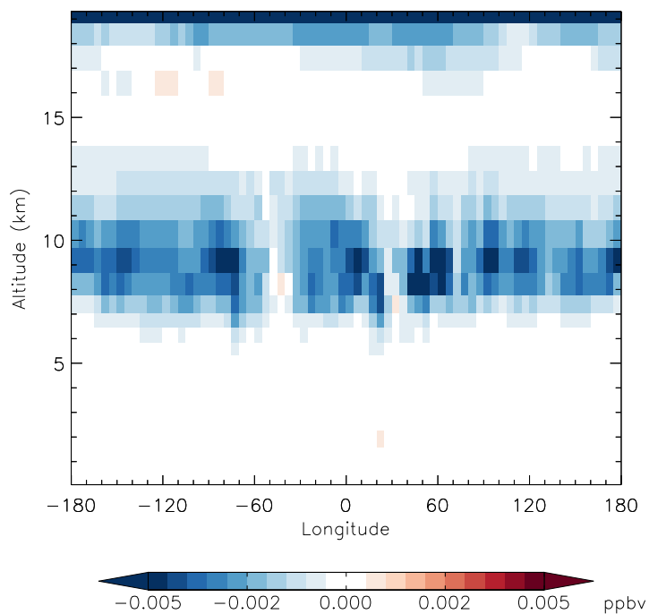
v11-01f-merra2-Run0 - v11-01d-Run1 HNO 4 - Diff along 15S for Apr
