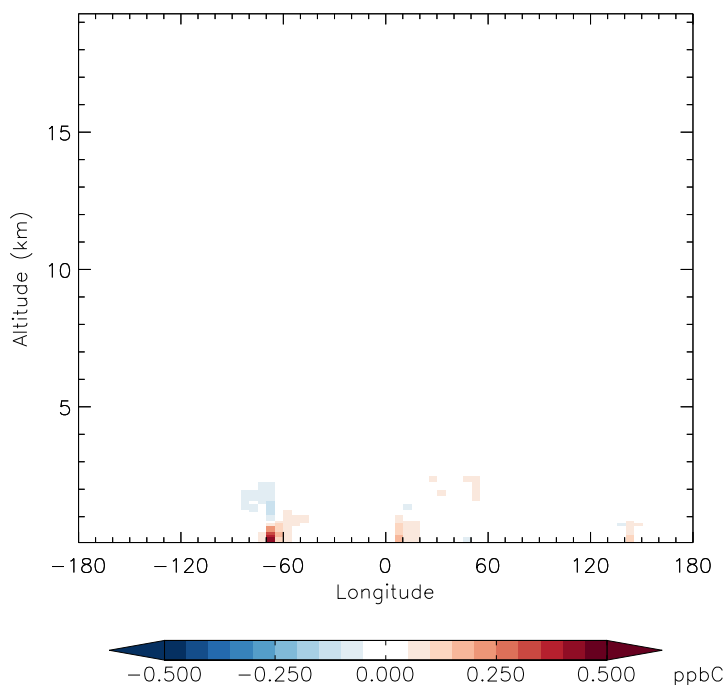
v11-01f-merra2-Run0 - v11-01f-geosfp-Run0 ACET - Diff along 42N for Apr
