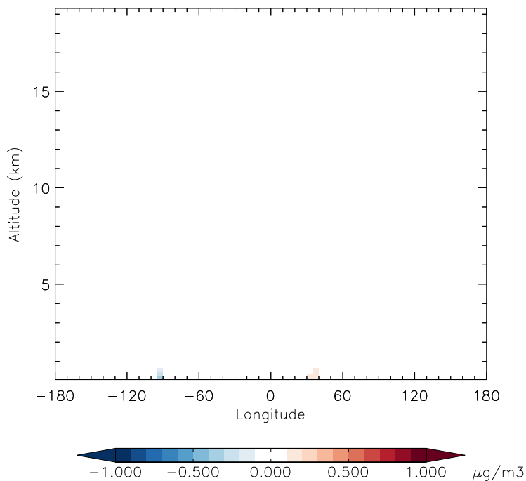
v11-01f-merra2-Run0 - v11-01f-geosfp-Run0 NH3 - Diff along 42N for Apr
