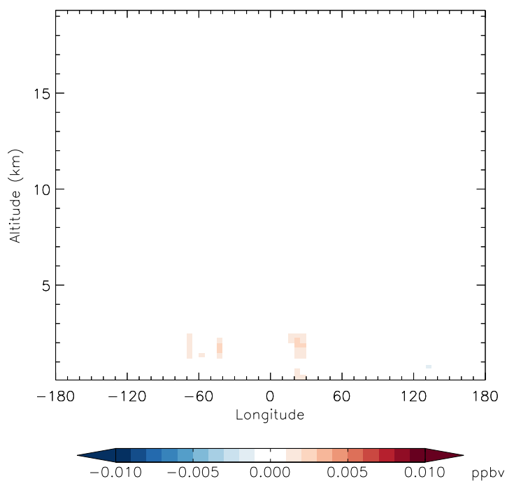
v11-01f-merra2-Run0 - v11-01d-Run1 PMN - Diff along 15S for Apr
