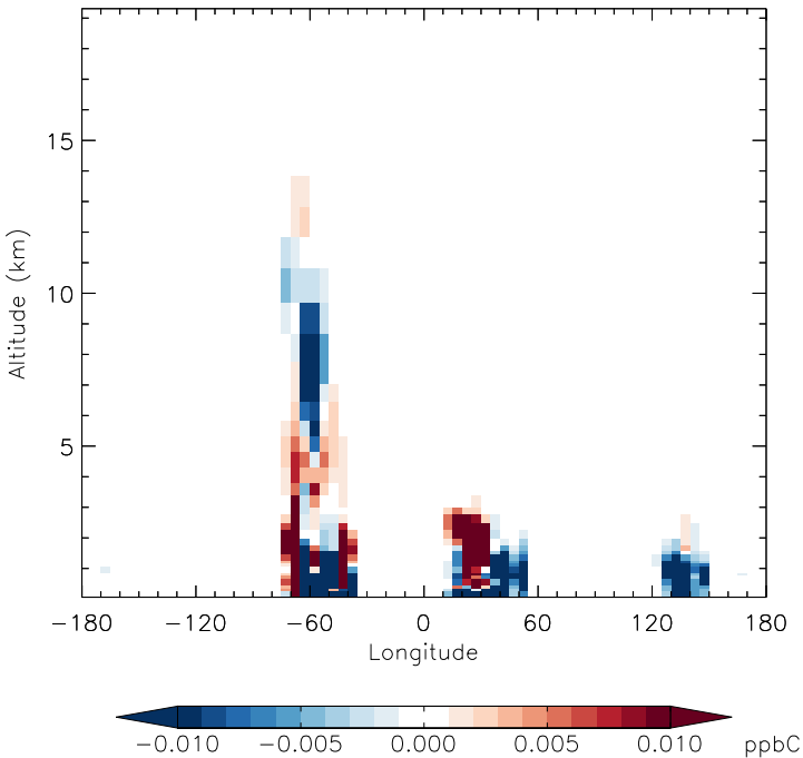
v11-01f-merra2-Run0 - v11-01d-Run1 PRPE - Diff along 15S for Apr
