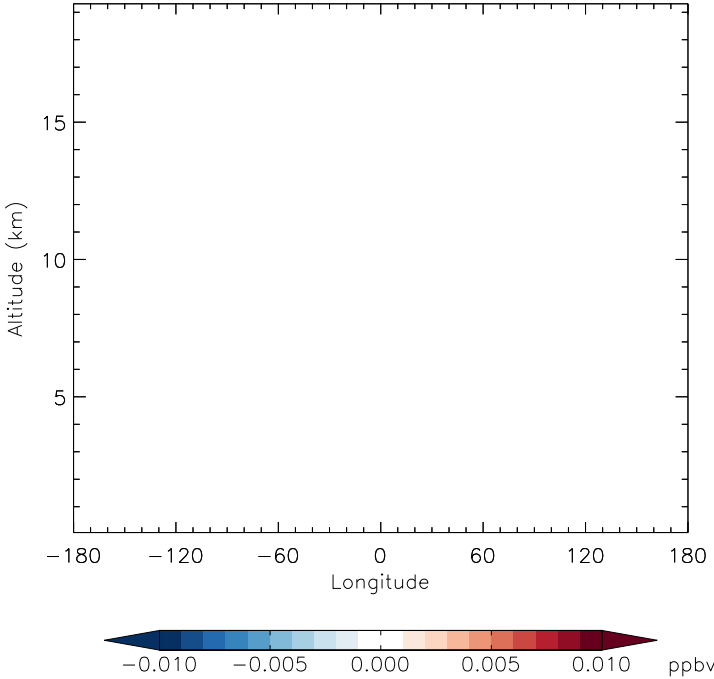
v11-01f-merra2-Run0 - v11-01d-Run1 CHBr3 - Diff along 15S for Apr
