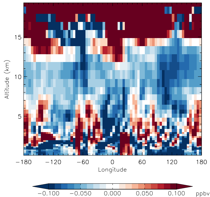
v11-01f-merra2-Run0 - v11-01d-Run1 N2O - Diff along 15S for Apr
