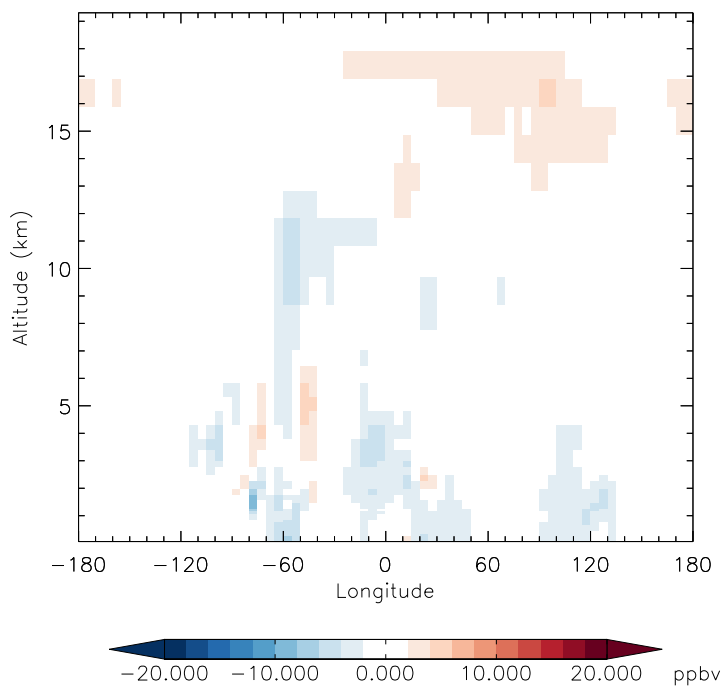
v11-01f-merra2-Run0 - v11-01d-Run1 CO - Diff along 15S for Apr
