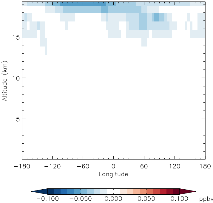
v11-01f-merra2-Run0 - v11-01d-Run1 HCl - Diff along 15S for Apr
