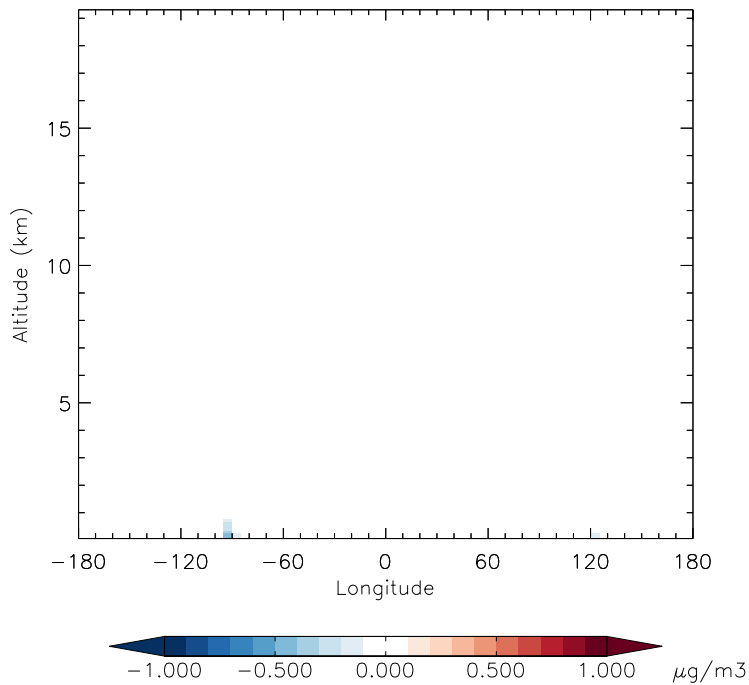
v11-01f-merra2-Run0 - v11-01d-Run1 NH3 - Diff along 42N for Apr
