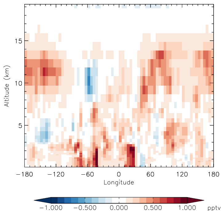
v11-01f-merra2-Run0 - v11-01f-geosfp-Run0 HO2 - Diff along 15S for Apr
