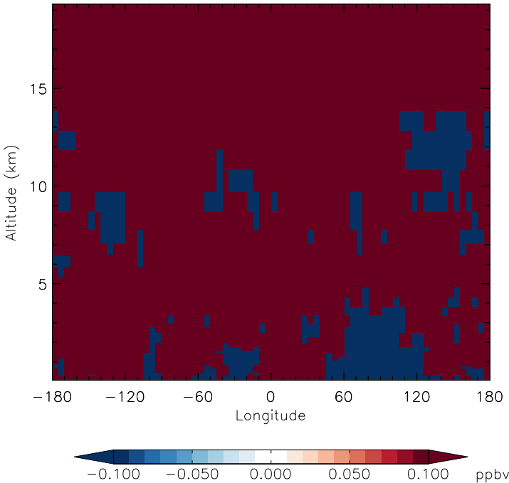
v11-01f-merra2-Run0 - v11-01f-geosfp-Run0 H2O - Diff along 42N for Apr
