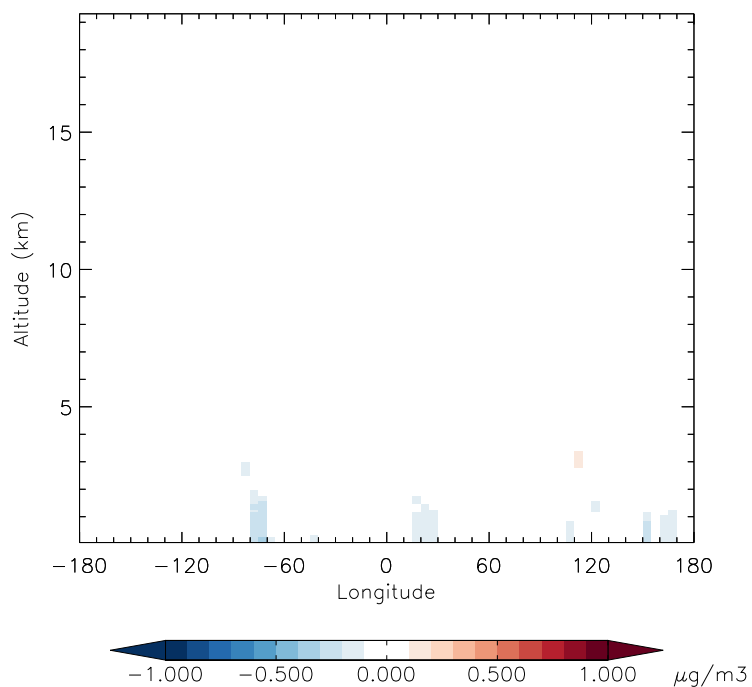
v11-01f-merra2-Run0 - v11-01f-geosfp-Run0 S04 - Diff along 15S for Apr
