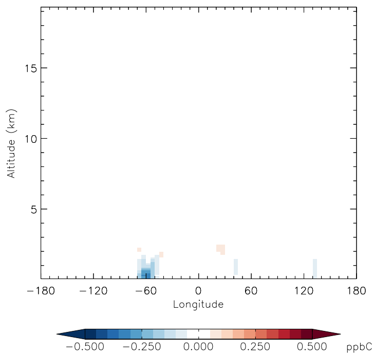
v11-01f-merra2-Run0 - v11-01f-geosfp-Run0 ALD2 - Diff along 15S for Apr
