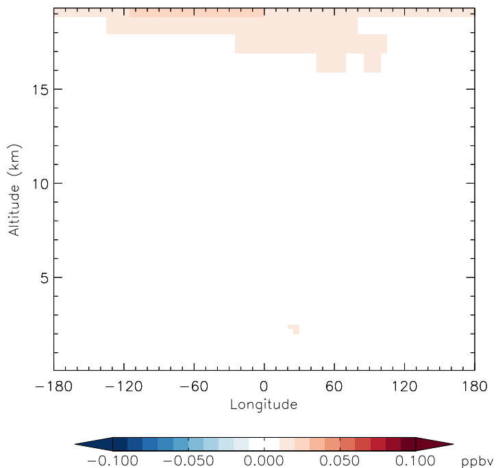
v11-01f-merra2-Run0 - v11-01f-geosfp-Run0 CH 3 Cl - Diff along 15S for Apr
