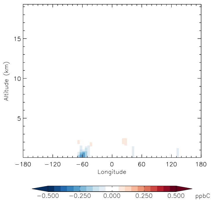
v11-01f-merra2-Run0 - v11-01d-Run1 ALD2 - Diff along 15S for Apr
