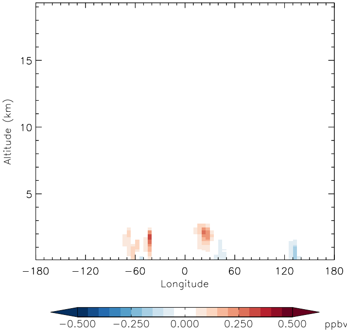
v11-01f-merra2-Run0 - v11-01d-Run1 CH2O - Diff along 15S for Apr
