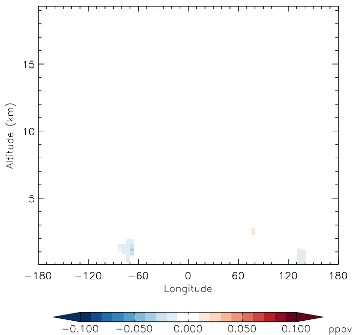
v11-01f-merra2-Run0 - v11-01d-Run1 PAN - Diff along 42N for Apr
