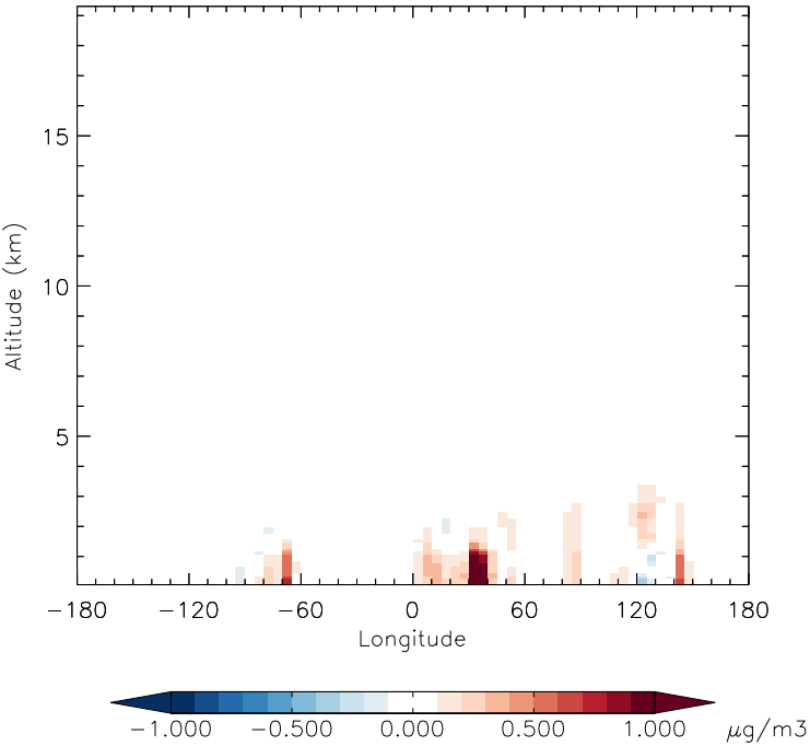
v11-01f-merra2-Run0 - v11-01f-geosfp-Run0 NIT - Diff along 42N for Apr
