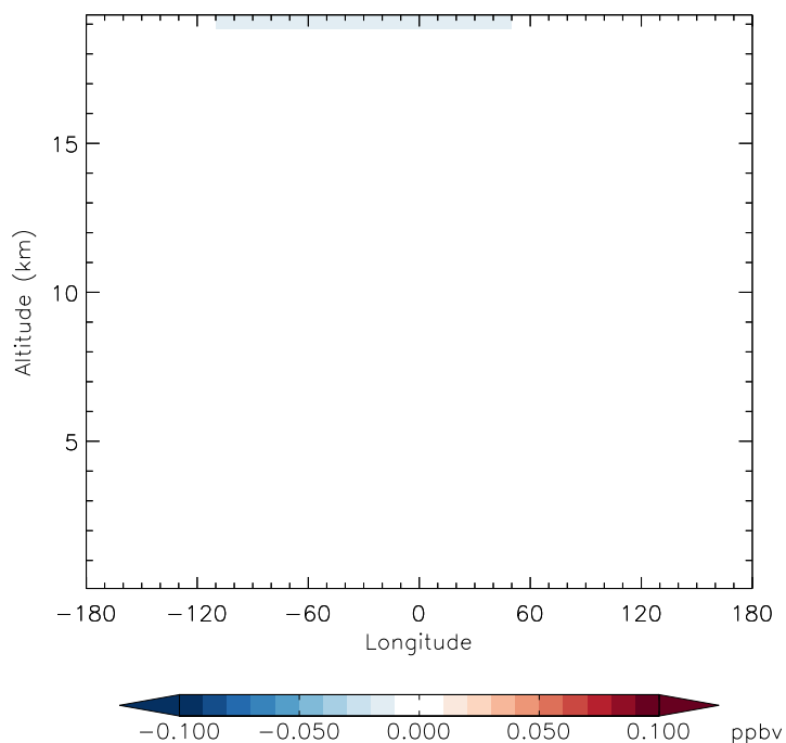
v11-01f-merra2-Run0 - v11-01f-geosfp-Run0 MPN - Diff along 15S for Apr
