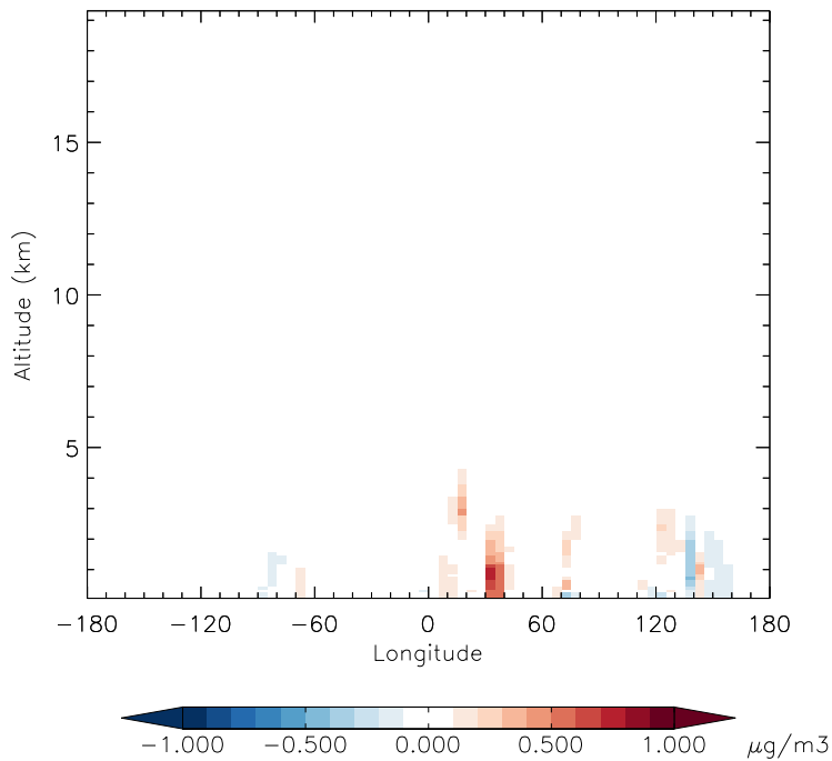
v11-01f-merra2-Run0 - v11-01d-Run1 SO 2 - Diff along 42N for Apr
