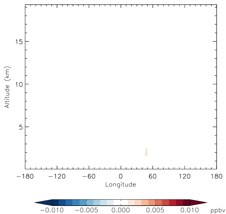
v11-01f-merra2-Run0 - v11-01d-Run1 IEPOX - Diff along 42N for Apr
