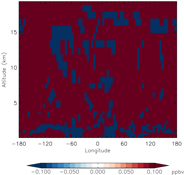
v11-01f-merra2-Run0 - v11-01f-geosfp-Run0 H2O - Diff along 15S for Apr
