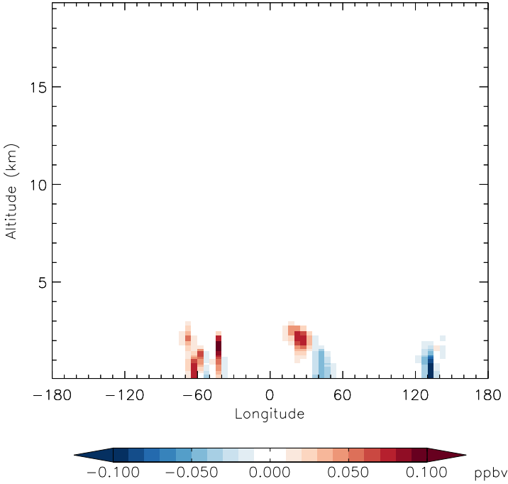
v11-01f-merra2-Run0 - v11-01d-Run1 GLYC - Diff along 15S for Apr
