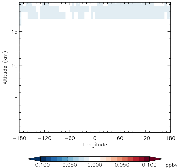
v11-01f-merra2-Run0 - v11-01d-Run1 CH 3 Cl - Diff along 42N for Apr
