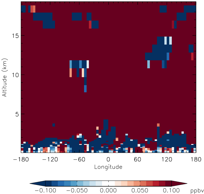
v11-01f-merra2-Run0 - v11-01f-geosfp-Run0 CH4 - Diff along 15S for Apr
