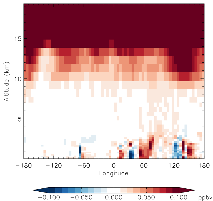
v11-01f-merra2-Run0 - v11-01d-Run1 HNO 3 - Diff along 42N for Apr
