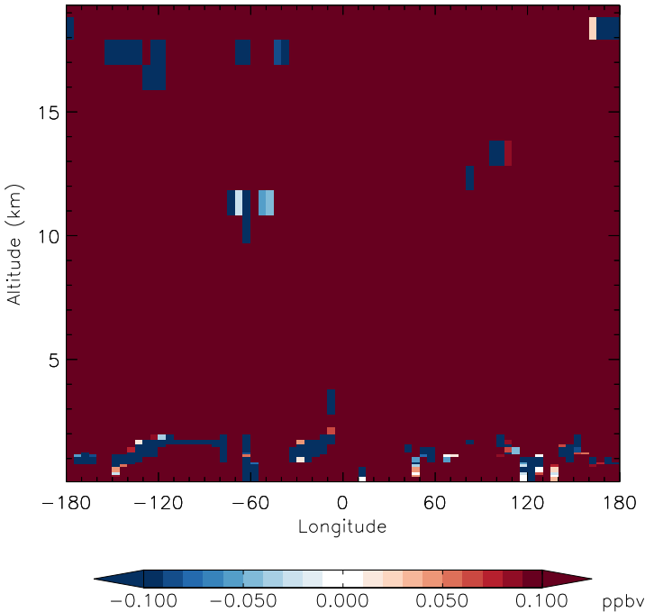
v11-01f-merra2-Run0 - v11-01d-Run1 CH4 - Diff along 15S for Apr
