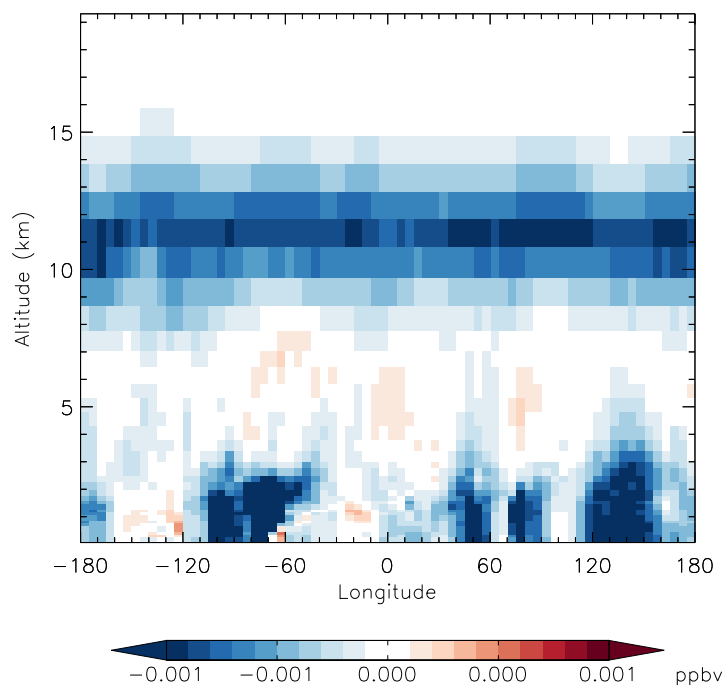
v11-01f-merra2-Run0 - v11-01f-geosfp-Run0 PPN - Diff along 42N for Apr
