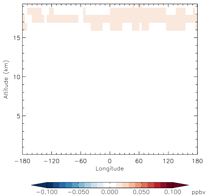
v11-01f-merra2-Run0 - v11-01f-geosfp-Run0 MPN - Diff along 42N for Apr
