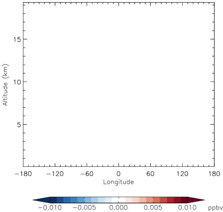
v11-01f-merra2-Run0 - v11-01d-Run1 NO3 - Diff along 15S for Apr
