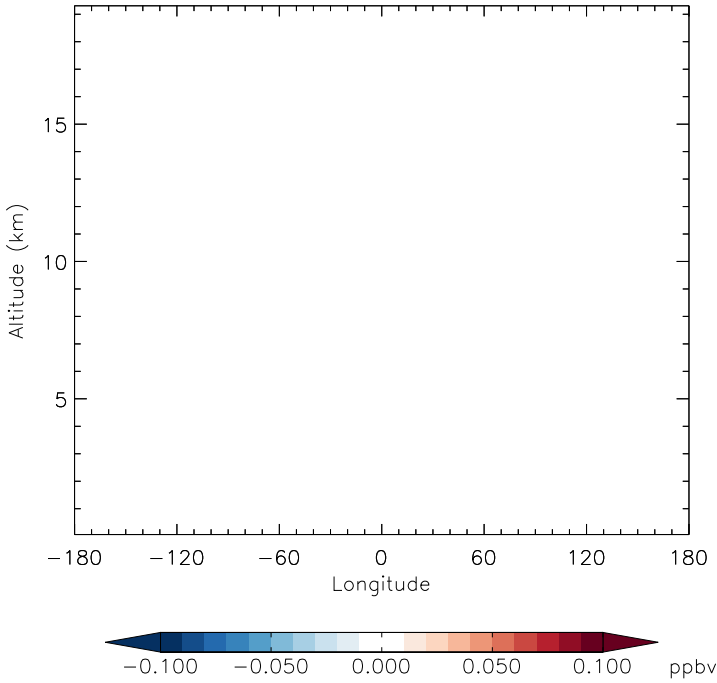
v11-01f-merra2-Run0 - v11-01d-Run1 CH3CCI3 - Diff along 15S for Apr
