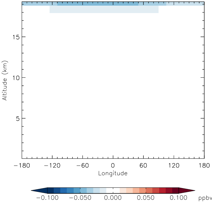
v11-01f-merra2-Run0 - v11-01d-Run1 CINO3 - Diff along 15S for Apr
