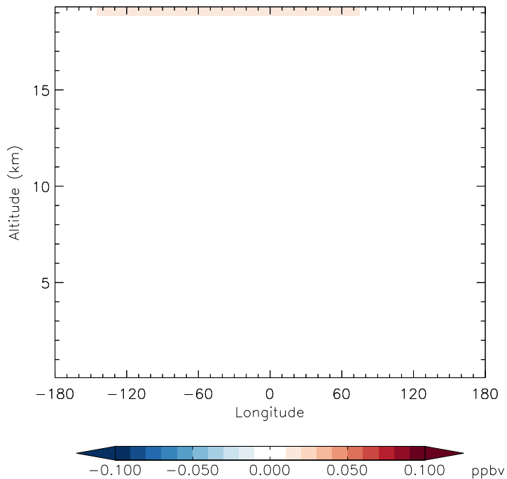
v11-01f-merra2-Run0 - v11-01d-Run1 OCS - Diff along 15S for Apr
