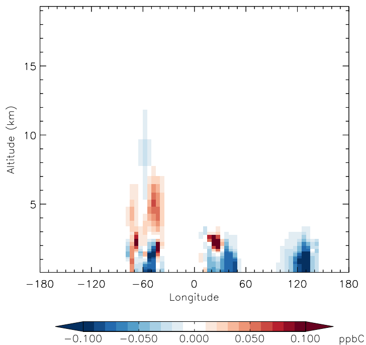
v11-01f-merra2-Run0 - v11-01d-Run1 MEK - Diff along 15S for Apr
