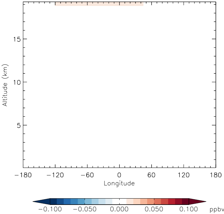
v11-01f-merra2-Run0 - v11-01f-geosfp-Run0 CFC11 - Diff along 15S for Apr
