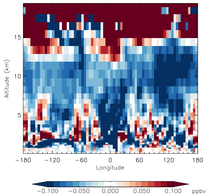
v11-01f-merra2-Run0 - v11-01f-geosfp-Run0 N2O - Diff along 15S for Apr
