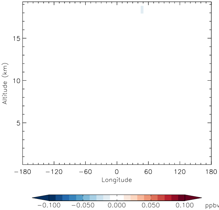
v11-01f-merra2-Run0 - v11-01f-geosfp-Run0 CFC11 - Diff along 42N for Apr
