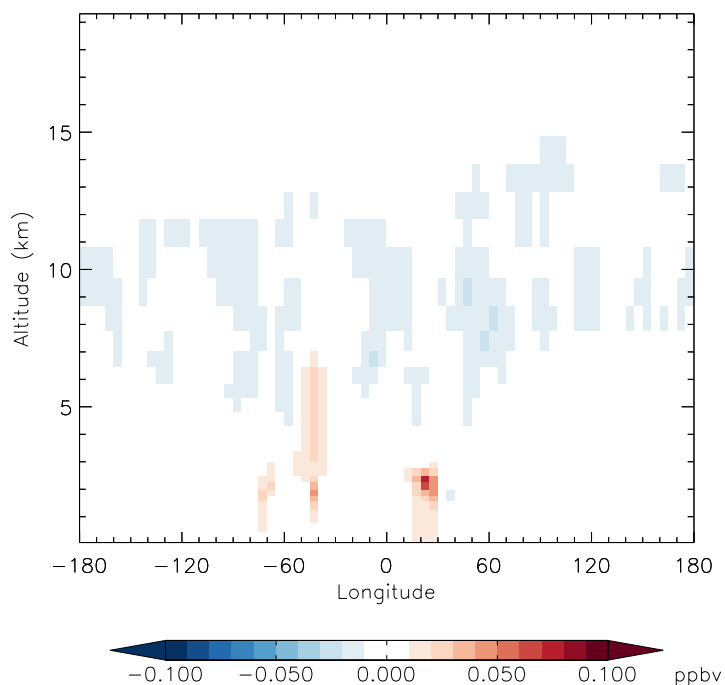
v11-01f-merra2-Run0 - v11-01f-geosfp-Run0 PAN - Diff along 15S for Apr
