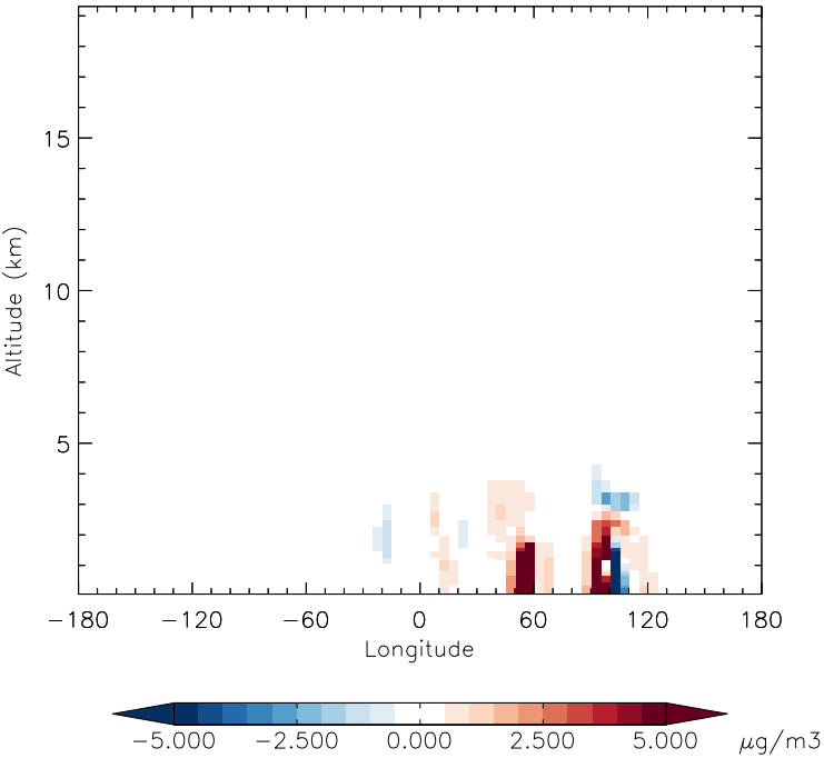
v11-01f-merra2-Run0 - v11-01f-geosfp-Run0 DST2 - Diff along 42N for Apr
