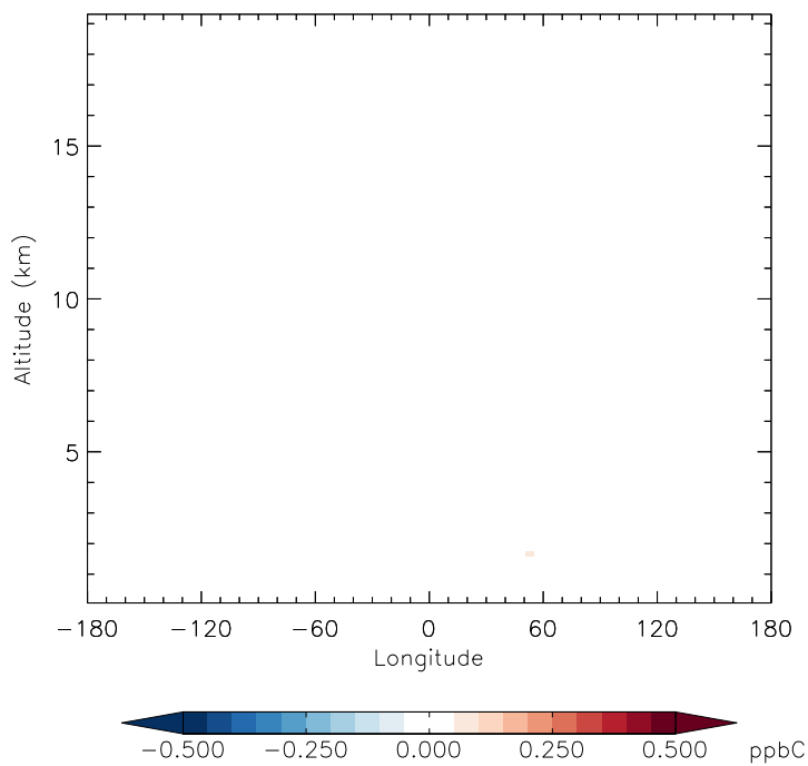
v11-01f-merra2-Run0 - v11-01d-Run1 C3H8 - Diff along 42N for Apr
