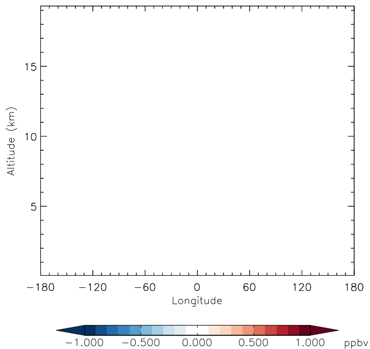
v11-01f-merra2-Run0 - v11-01f-geosfp-Run0 NO2 - Diff along 15S for Apr
