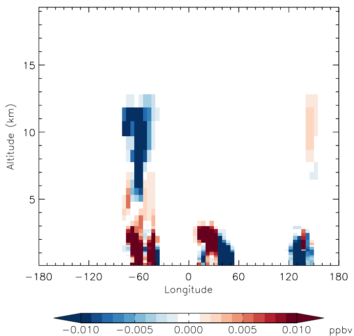
v11-01f-merra2-Run0 - v11-01d-Run1 IEPOX - Diff along 15S for Apr
