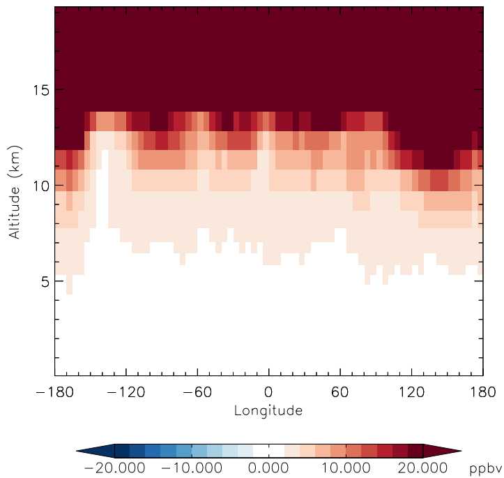
v11-01f-merra2-Run0 - v11-01d-Run1 O3 - Diff along 42N for Apr
