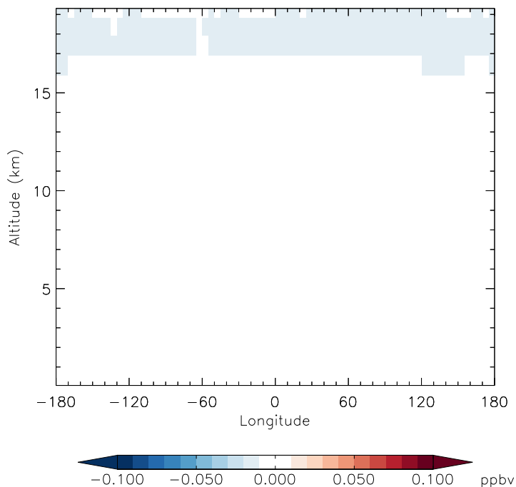
v11-01f-merra2-Run0 - v11-01f-geosfp-Run0 CH 3 Cl - Diff along 42N for Apr
