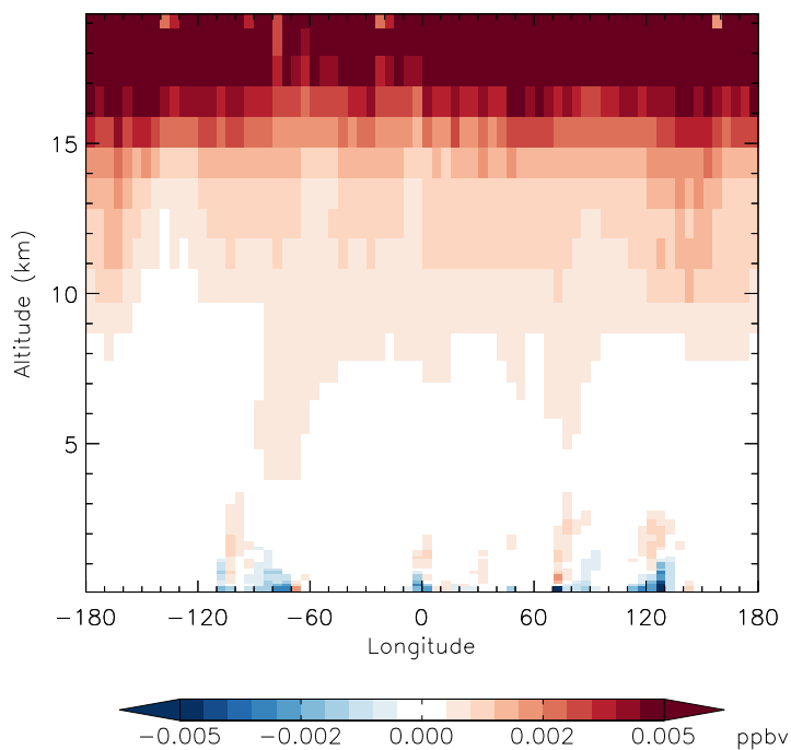
v11-01f-merra2-Run0 - v11-01d-Run1 N2O5 - Diff along 42N for Apr
