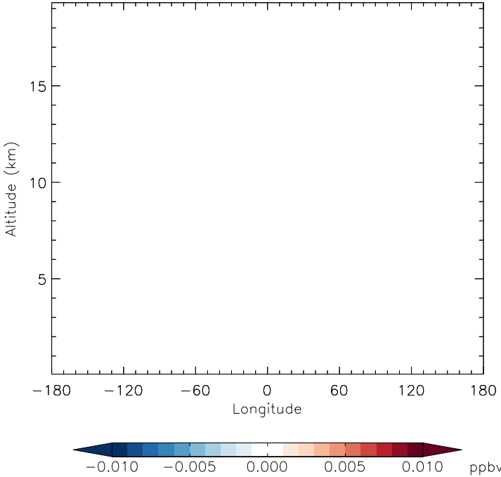
v11-01f-merra2-Run0 - v11-01d-Run1 HBr - Diff along 42N for Apr
