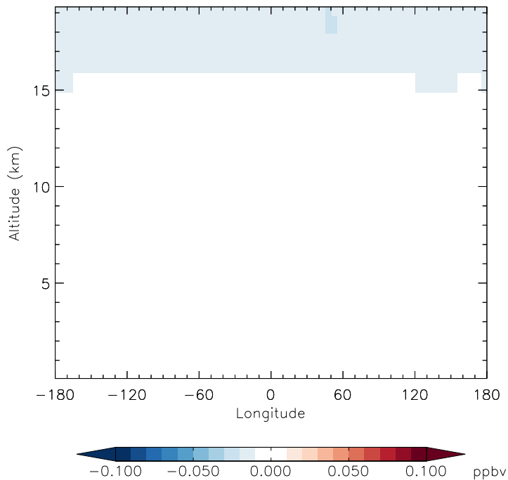
v11-01f-merra2-Run0 - v11-01d-Run1 OCS - Diff along 42N for Apr
