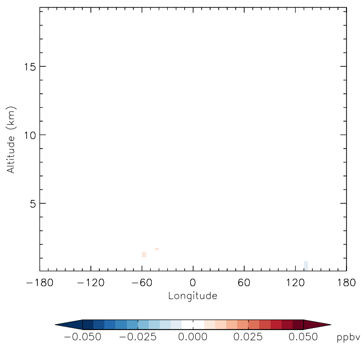
v11-01f-merra2-Run0 - v11-01d-Run1 RCHO - Diff along 15S for Apr
