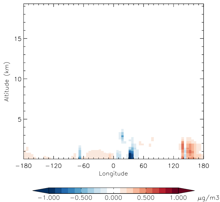
v11-01f-merra2-Run0 - v11-01d-Run1 S04 - Diff along 42N for Apr
