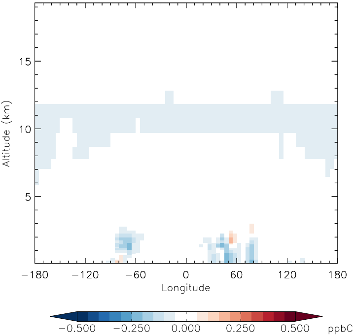
v11-01f-merra2-Run0 - v11-01f-geosfp-Run0 C2H6 - Diff along 42N for Apr
