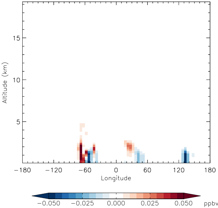
v11-01f-merra2-Run0 - v11-01f-geosfp-Run0 MVK - Diff along 15S for Apr
