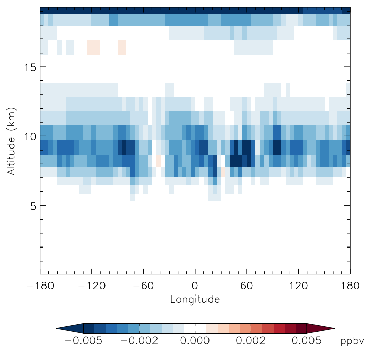
v11-01f-merra2-Run0 - v11-01f-geosfp-Run0 HNO 4 - Diff along 15S for Apr
