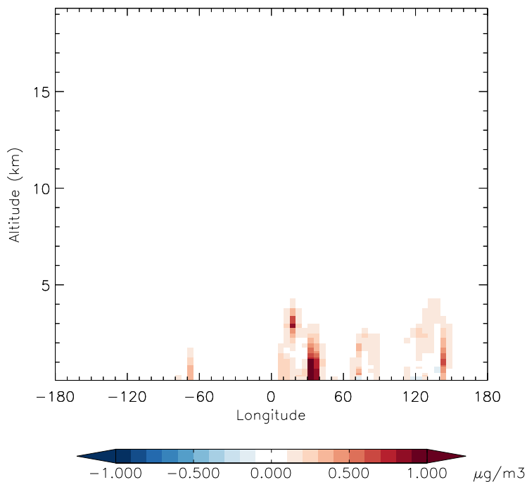
v11-01f-merra2-Run0 - v11-01f-geosfp-Run0 SO 2 - Diff along 42N for Apr
