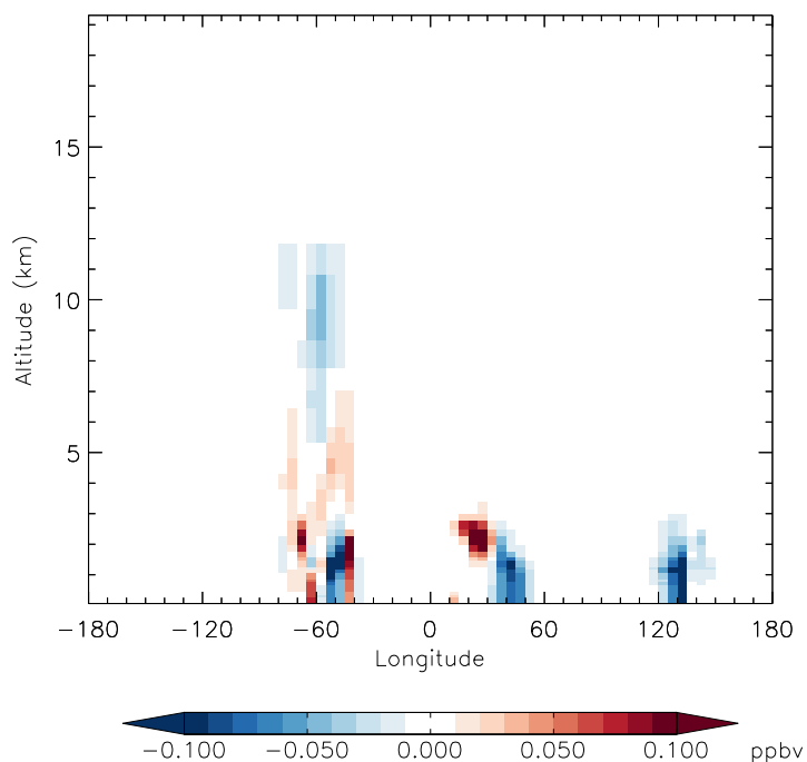
v11-01f-merra2-Run0 - v11-01f-geosfp-Run0 HAC - Diff along 15S for Apr
