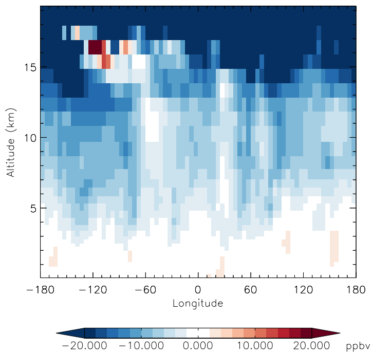
v11-01f-merra2-Run0 - v11-01f-geosfp-Run0 O3 - Diff along 15S for Apr
