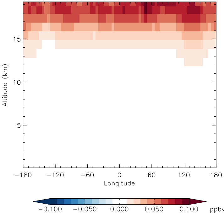
v11-01f-merra2-Run0 - v11-01f-geosfp-Run0 CINO3 - Diff along 42N for Apr
