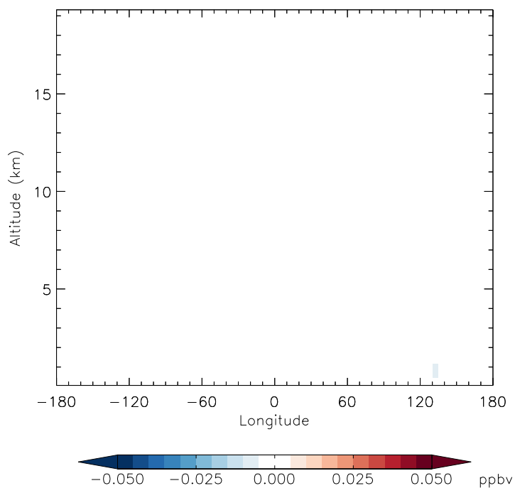
v11-01f-merra2-Run0 - v11-01f-geosfp-Run0 RCHO - Diff along 15S for Apr
