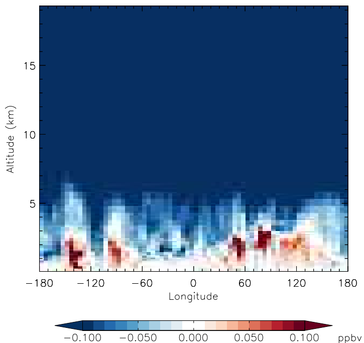
v11-01f-merra2-Run0 - v11-01f-geosfp-Run0 N2O - Diff along 42N for Apr
