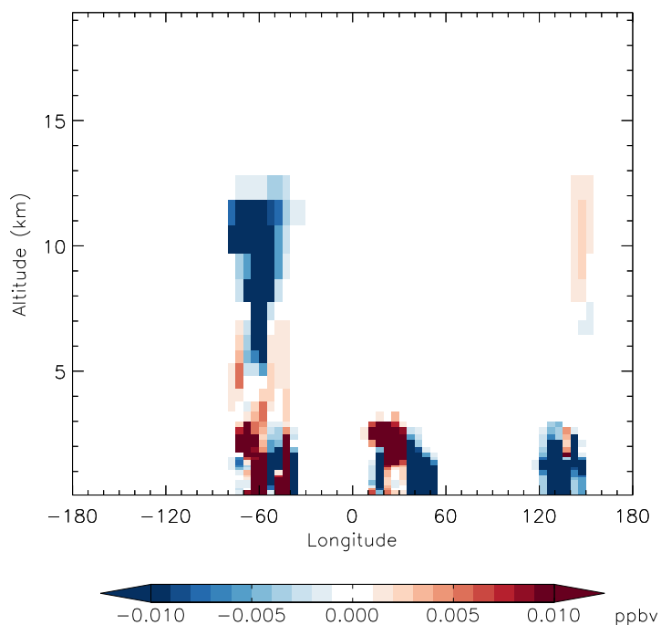
v11-01f-merra2-Run0 - v11-01f-geosfp-Run0 IEPOX - Diff along 15S for Apr
