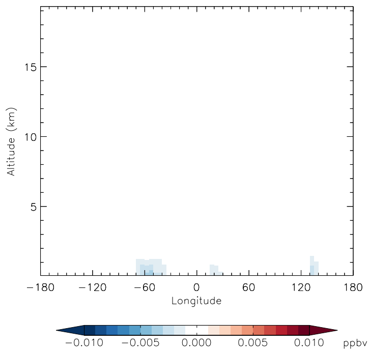
v11-01f-merra2-Run0 - v11-01d-Run1 MOBA - Diff along 15S for Apr
