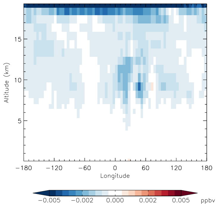
v11-01f-merra2-Run0 - v11-01d-Run1 N2O5 - Diff along 15S for Apr
