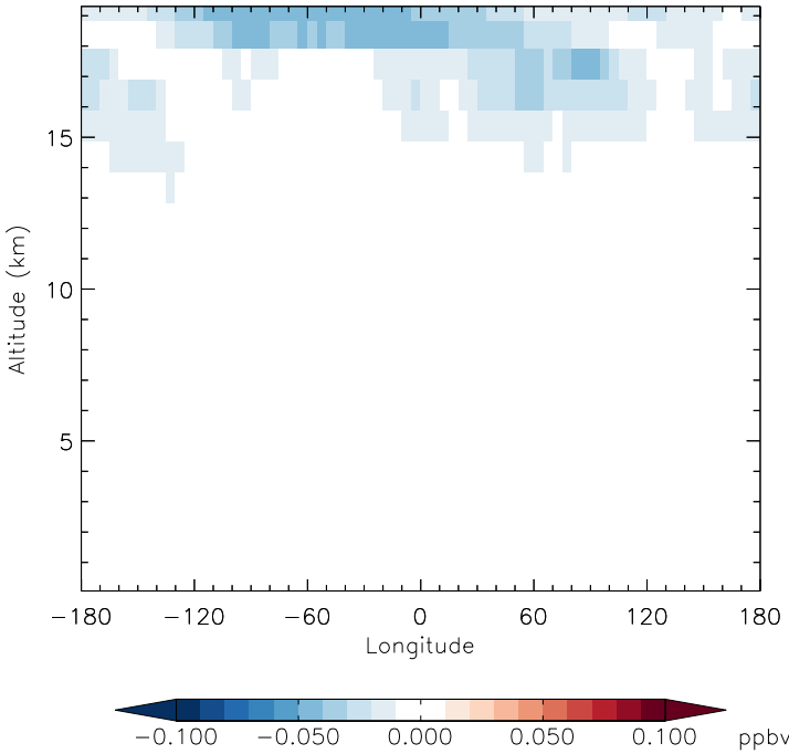
v11-01f-merra2-Run0 - v11-01f-geosfp-Run0 HCl - Diff along 15S for Apr
