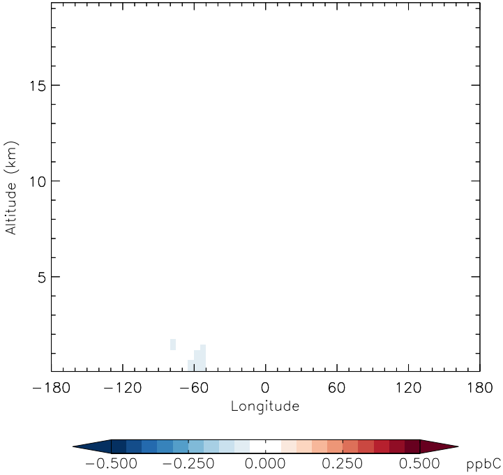
v11-01f-merra2-Run0 - v11-01d-Run1 C2H6 - Diff along 15S for Apr
