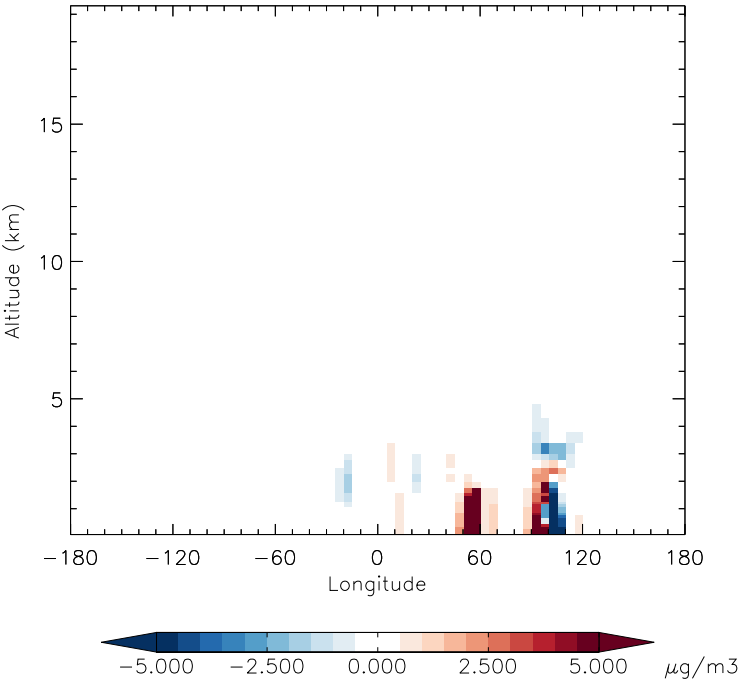
v11-01f-merra2-Run0 - v11-01d-Run1 DST2 - Diff along 42N for Apr
