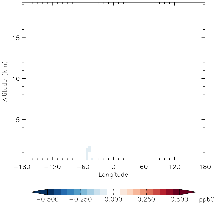
v11-01f-merra2-Run0 - v11-01f-geosfp-Run0 ALK4 - Diff along 15S for Apr
