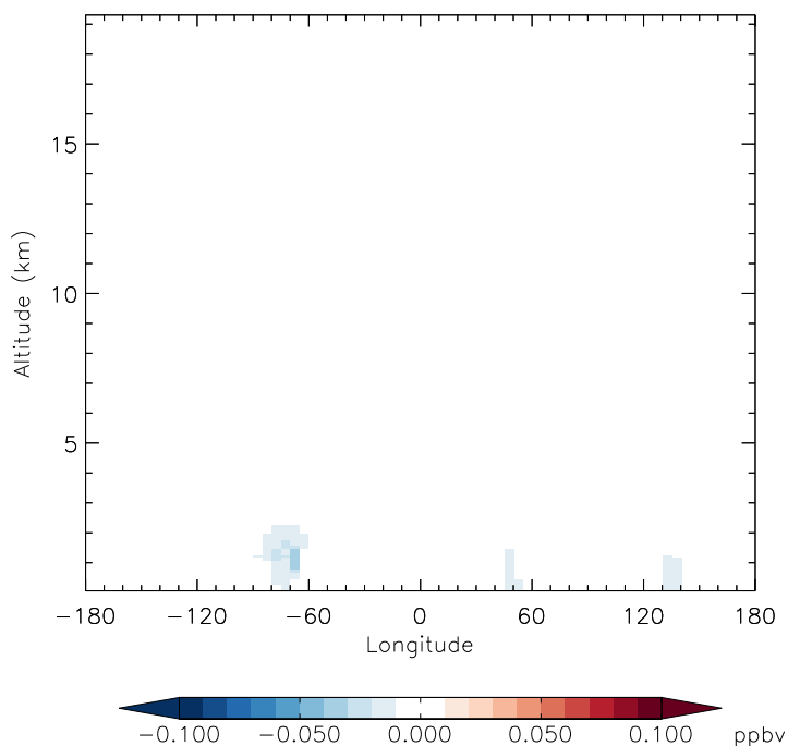
v11-01f-merra2-Run0 - v11-01f-geosfp-Run0 PAN - Diff along 42N for Apr
