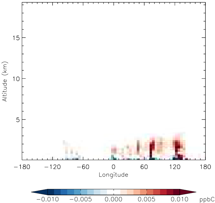
v11-01f-merra2-Run0 - v11-01d-Run1 PRPE - Diff along 42N for Apr
