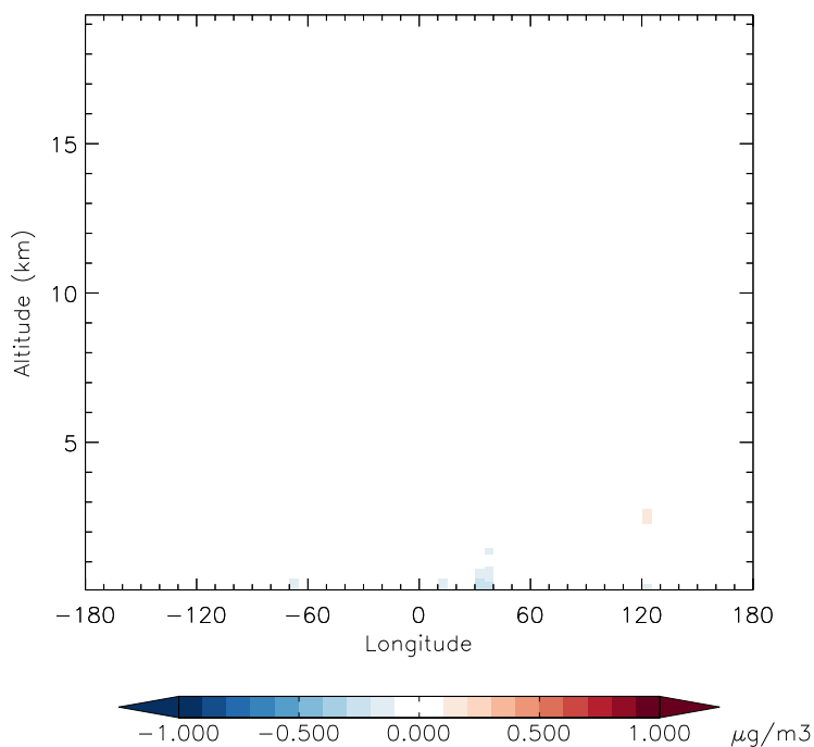
v11-01f-merra2-Run0 - v11-01f-geosfp-Run0 NH4 - Diff along 42N for Apr
