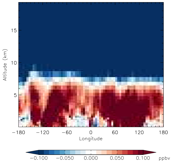
v11-01f-merra2-Run0 - v11-01d-Run1 N2O - Diff along 42N for Apr
