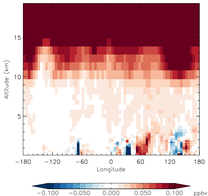
v11-01f-merra2-Run0 - v11-01f-geosfp-Run0 HNO 3 - Diff along 42N for Apr
