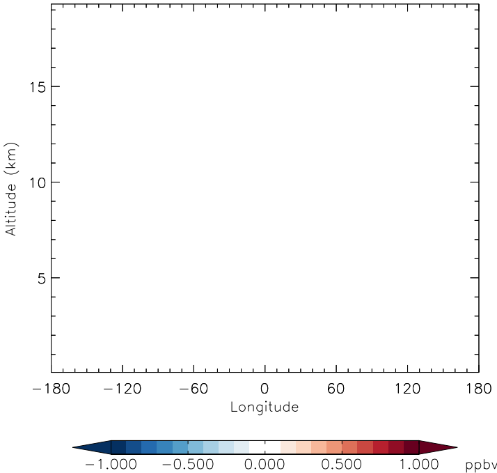
v11-01f-merra2-Run0 - v11-01f-geosfp-Run0 HNO2 - Diff along 15S for Apr
