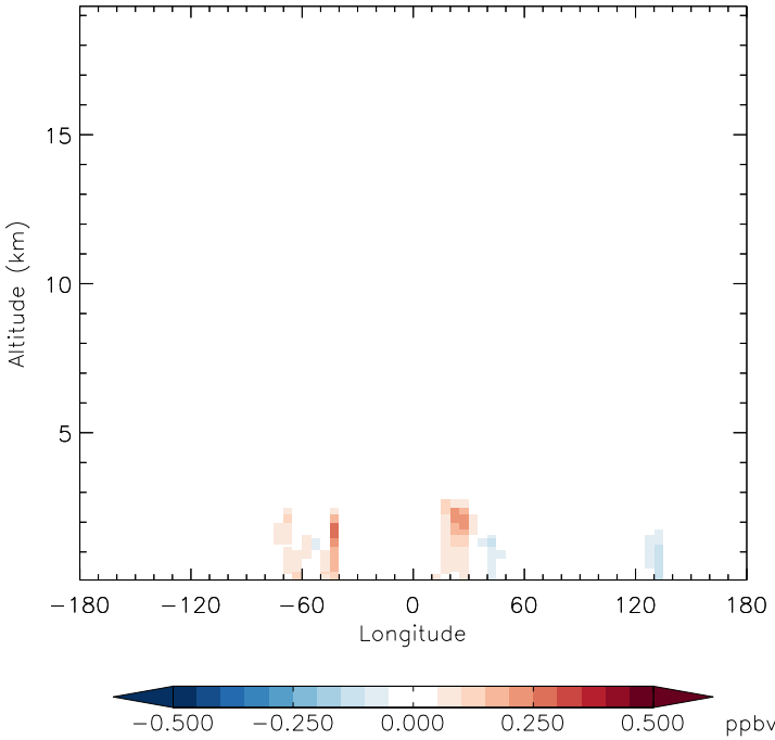
v11-01f-merra2-Run0 - v11-01f-geosfp-Run0 CH2O - Diff along 15S for Apr
