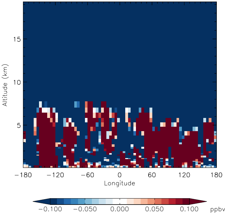
v11-01f-merra2-Run0 - v11-01f-geosfp-Run0 CH4 - Diff along 42N for Apr
