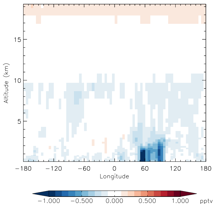
v11-01f-merra2-Run0 - v11-01f-geosfp-Run0 HO2 - Diff along 42N for Apr
