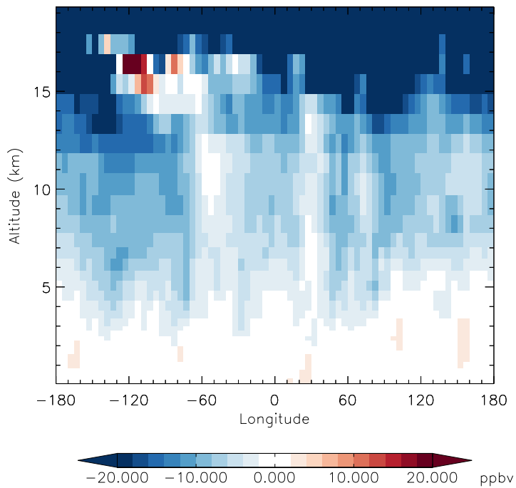
v11-01f-merra2-Run0 - v11-01d-Run1 O3 - Diff along 15S for Apr
