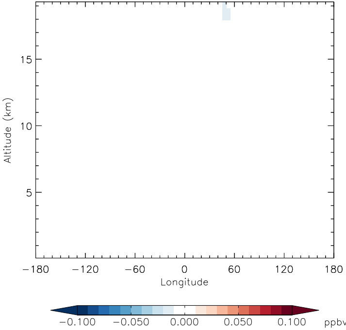
v11-01f-merra2-Run0 - v11-01d-Run1 CFC11 - Diff along 42N for Apr
