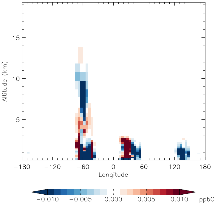
v11-01f-merra2-Run0 - v11-01f-geosfp-Run0 PRPE - Diff along 15S for Apr
