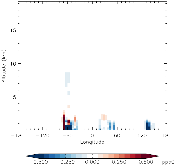
v11-01f-merra2-Run0 - v11-01f-geosfp-Run0 ISOP - Diff along 15S for Apr
