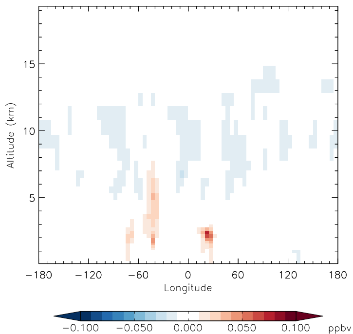
v11-01f-merra2-Run0 - v11-01d-Run1 PAN - Diff along 15S for Apr
