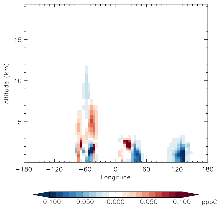
v11-01f-merra2-Run0 - v11-01f-geosfp-Run0 MEK - Diff along 15S for Apr
