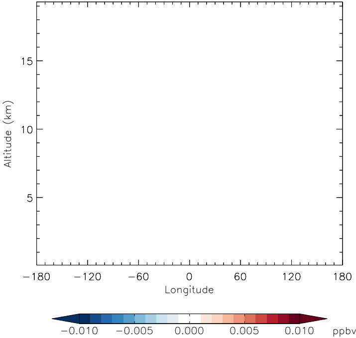
v11-01f-merra2-Run0 - v11-01d-Run1 CHBr3 - Diff along 42N for Apr
