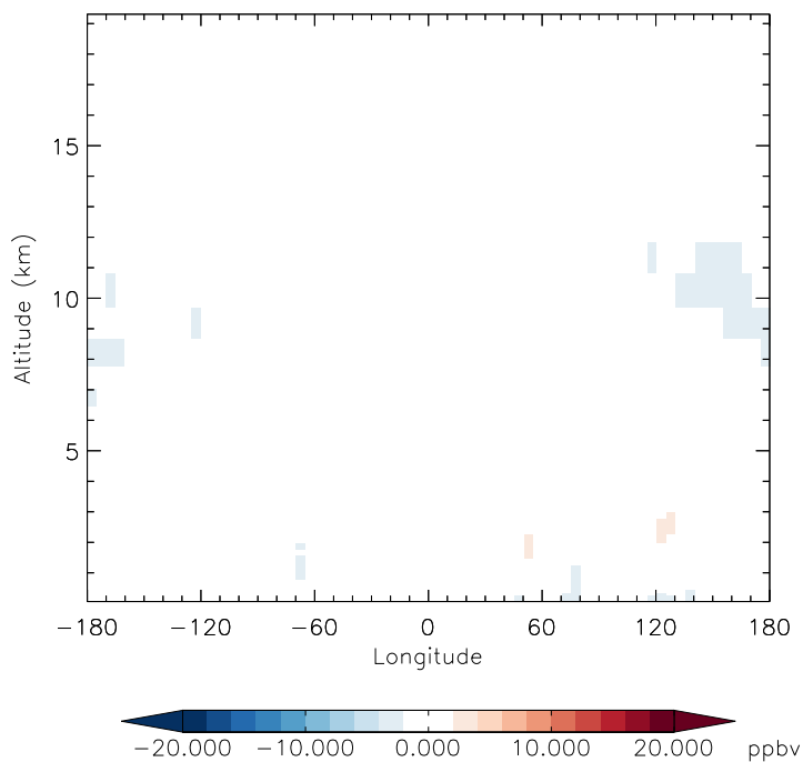
v11-01f-merra2-Run0 - v11-01d-Run1 CO - Diff along 42N for Apr
