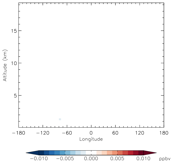
v11-01f-merra2-Run0 - v11-01f-geosfp-Run0 MMN - Diff along 42N for Apr
