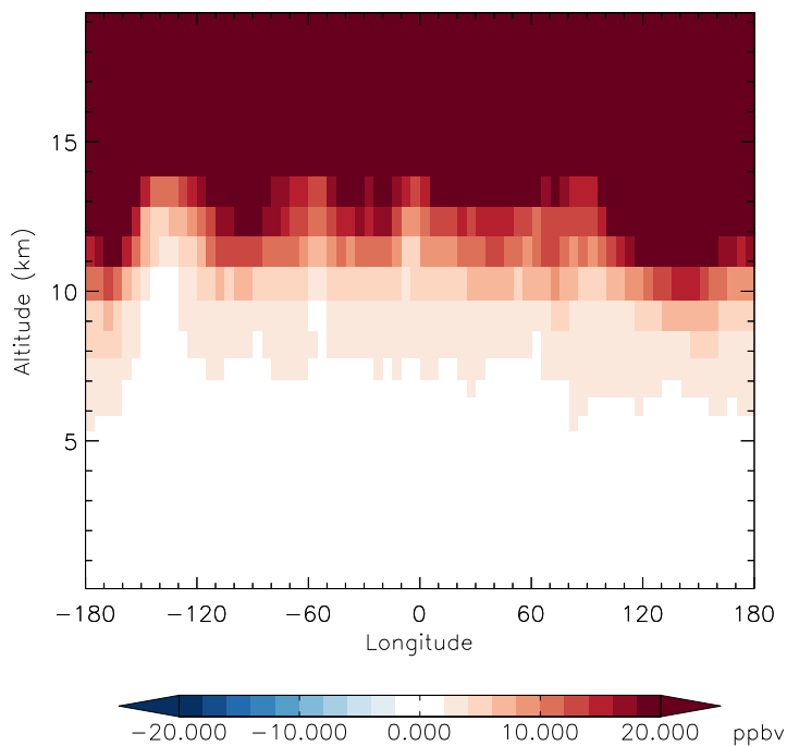
v11-01f-merra2-Run0 - v11-01f-geosfp-Run0 O3 - Diff along 42N for Apr
