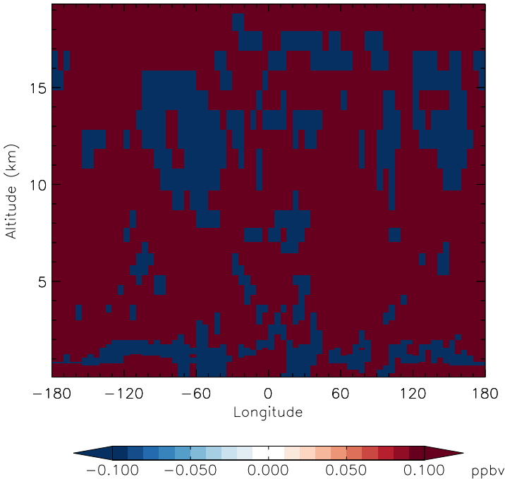
v11-01f-merra2-Run0 - v11-01d-Run1 H2O - Diff along 15S for Apr
