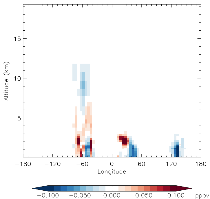
v11-01f-merra2-Run0 - v11-01d-Run1 HAC - Diff along 15S for Apr
