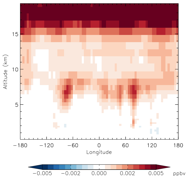
v11-01f-merra2-Run0 - v11-01f-geosfp-Run0 HNO 4 - Diff along 42N for Apr
