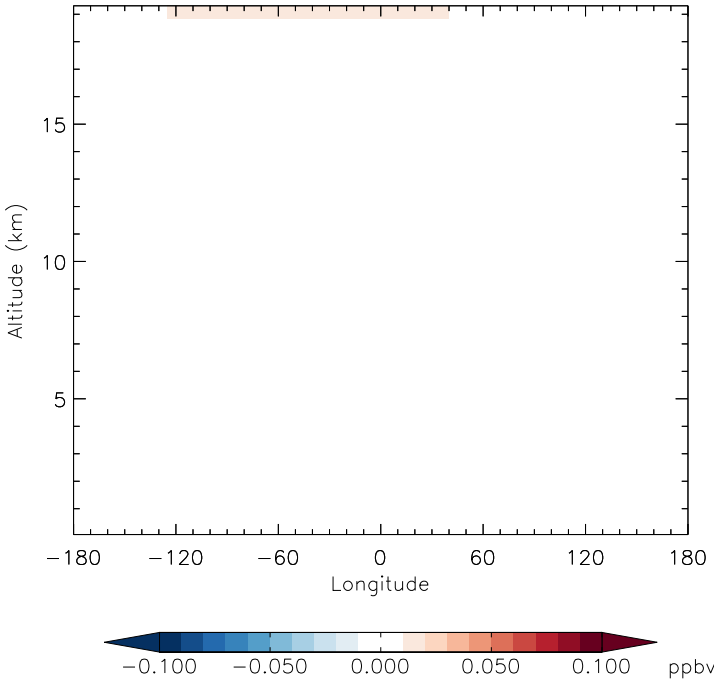
v11-01f-merra2-Run0 - v11-01f-geosfp-Run0 CFC12 - Diff along 15S for Apr
