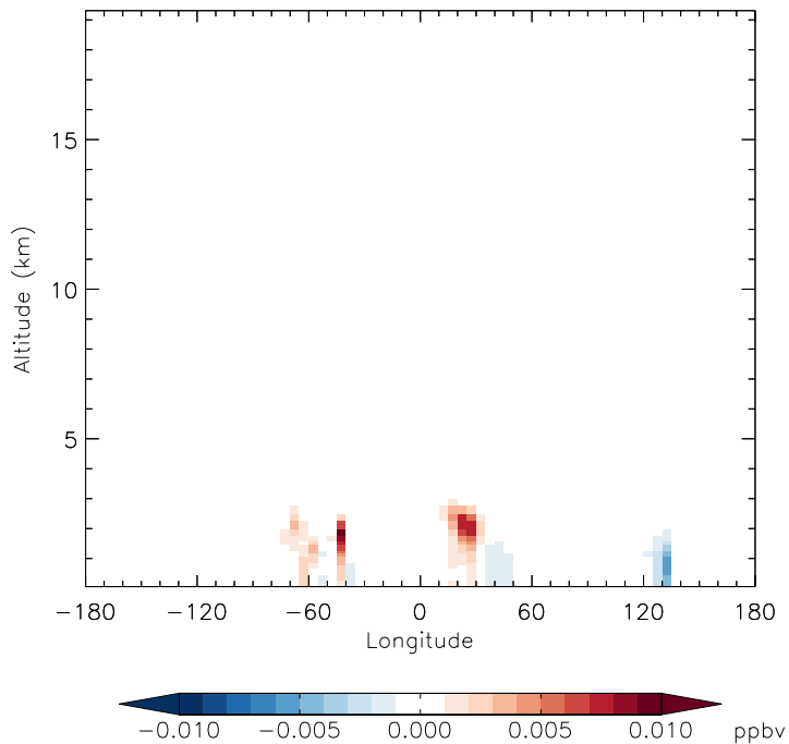
v11-01f-merra2-Run0 - v11-01d-Run1 MMN - Diff along 15S for Apr
