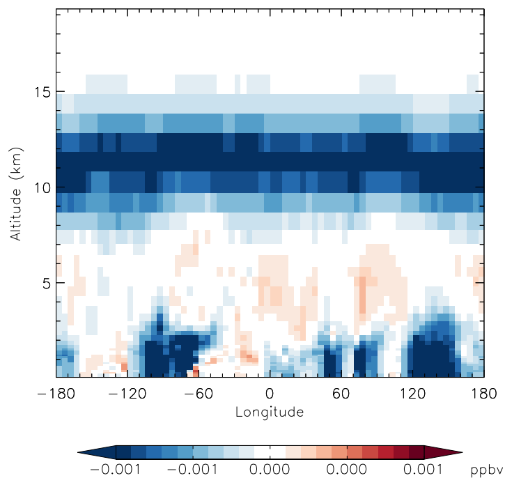
v11-01f-merra2-Run0 - v11-01d-Run1 PPN - Diff along 42N for Apr
