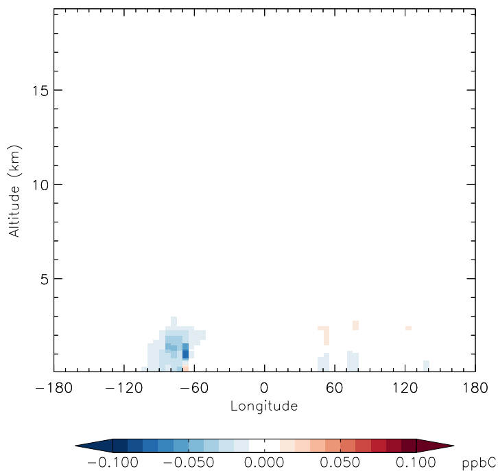
v11-01f-merra2-Run0 - v11-01d-Run1 MEK - Diff along 42N for Apr
