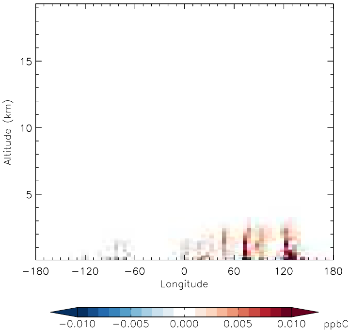
v11-01f-merra2-Run0 - v11-01f-geosfp-Run0 PRPE - Diff along 42N for Apr
