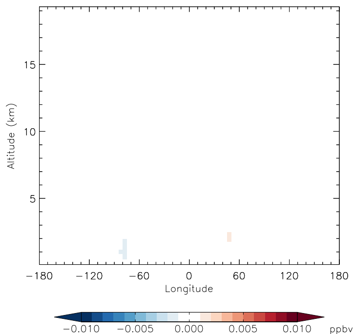
v11-01f-merra2-Run0 - v11-01f-geosfp-Run0 IEPOX - Diff along 42N for Apr
