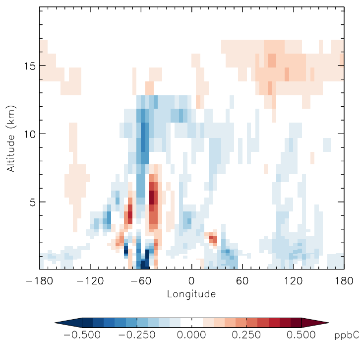
v11-01f-merra2-Run0 - v11-01f-geosfp-Run0 ACET - Diff along 15S for Apr
