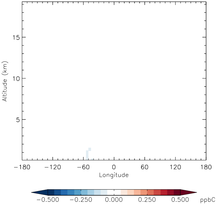
v11-01f-merra2-Run0 - v11-01d-Run1 ALK4 - Diff along 15S for Apr
