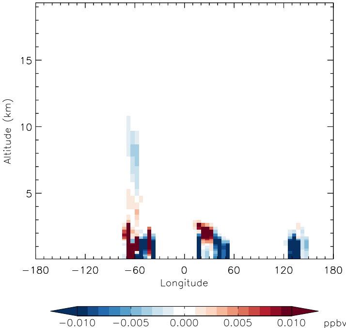
v11-01f-merra2-Run0 - v11-01f-geosfp-Run0 RIP - Diff along 15S for Apr
