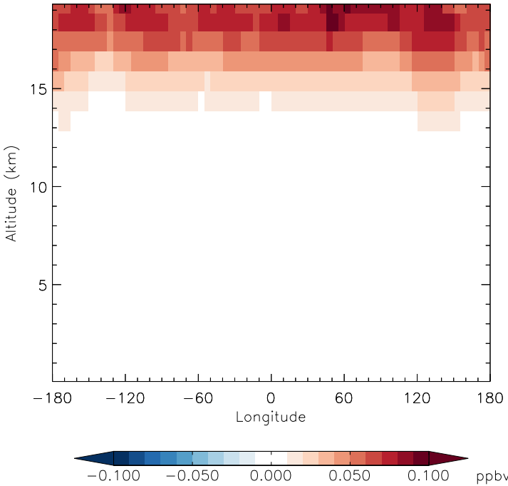
v11-01f-merra2-Run0 - v11-01d-Run1 CINO3 - Diff along 42N for Apr
