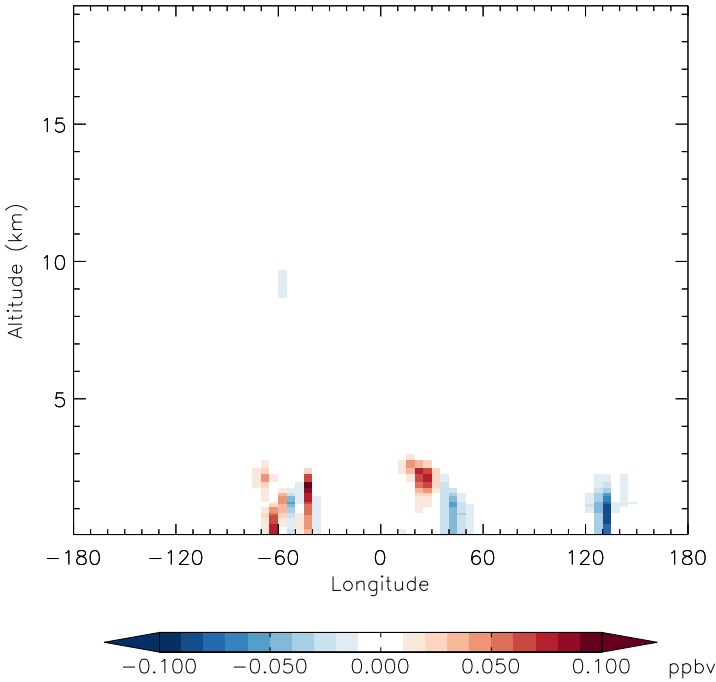
v11-01f-merra2-Run0 - v11-01f-geosfp-Run0 GLYC - Diff along 15S for Apr
