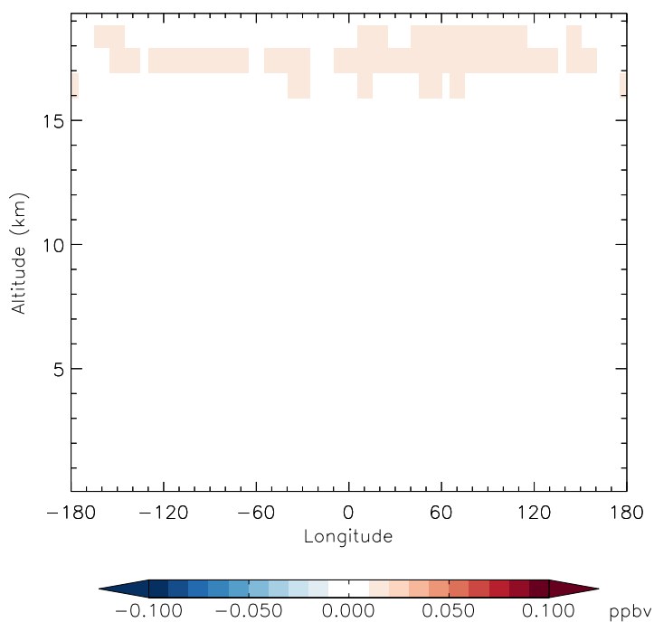
v11-01f-merra2-Run0 - v11-01d-Run1 MPN - Diff along 42N for Apr
