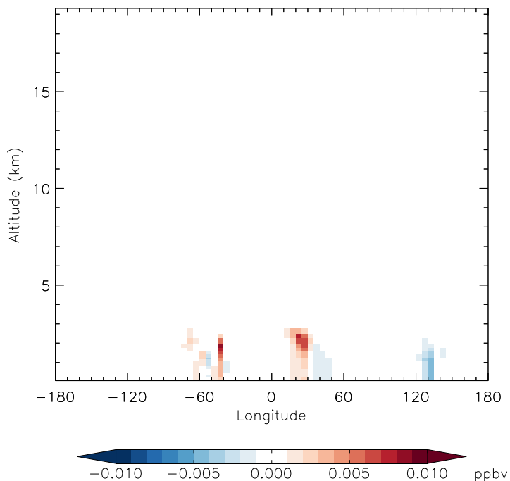
v11-01f-merra2-Run0 - v11-01f-geosfp-Run0 MMN - Diff along 15S for Apr
