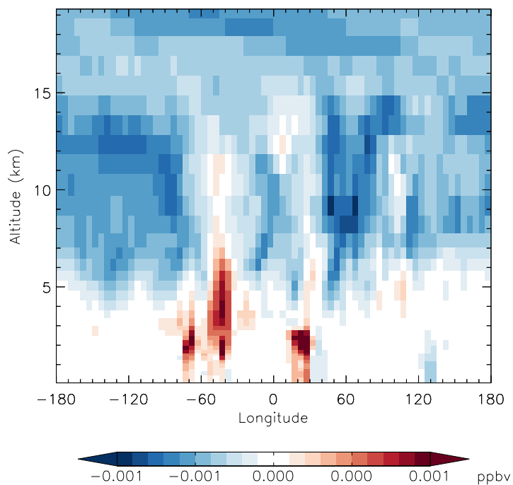
v11-01f-merra2-Run0 - v11-01d-Run1 PPN - Diff along 15S for Apr
