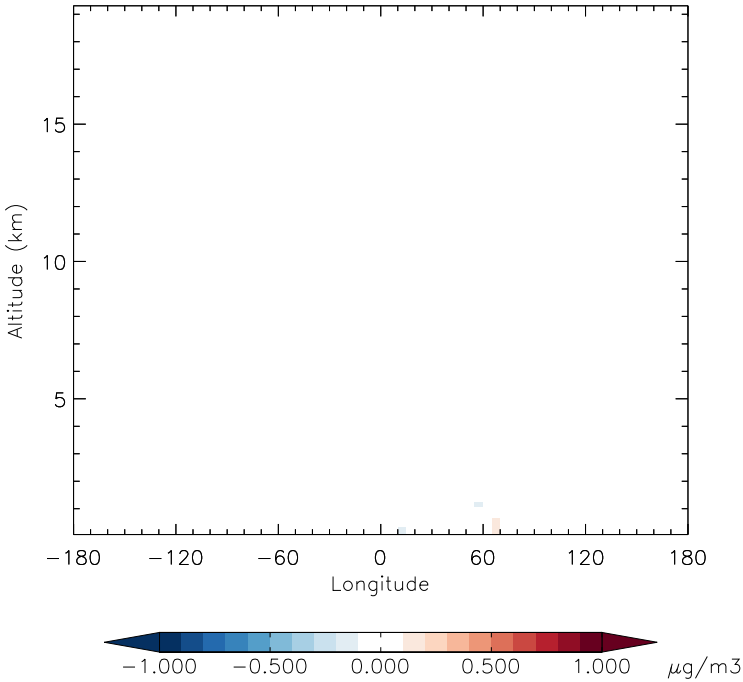
v11-01f-merra2-Run0 - v11-01f-geosfp-Run0 SALA - Diff along 15S for Apr
