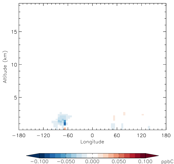
v11-01f-merra2-Run0 - v11-01f-geosfp-Run0 MEK - Diff along 42N for Apr
