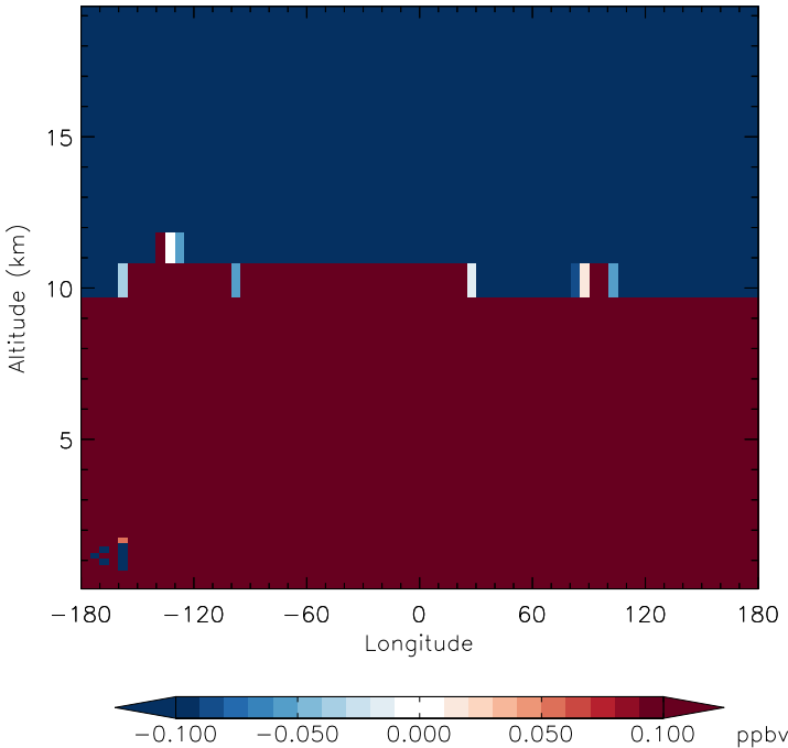
v11-01f-merra2-Run0 - v11-01d-Run1 CH4 - Diff along 42N for Apr
