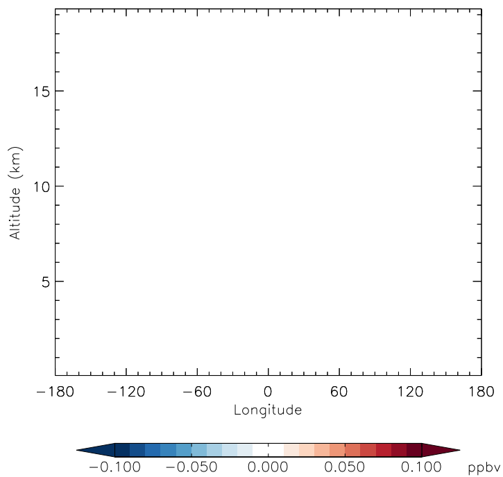
v11-01f-merra2-Run0 - v11-01d-Run1 ISOPN - Diff along 15S for Apr
