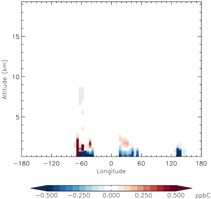
v11-01f-merra2-Run0 - v11-01d-Run1 ISOP - Diff along 15S for Apr
