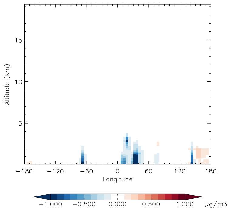
v11-01f-merra2-Run0 - v11-01f-geosfp-Run0 S04 - Diff along 42N for Apr
