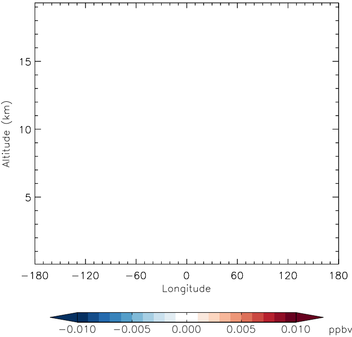
v11-01f-merra2-Run0 - v11-01f-geosfp-Run0 Br2 - Diff along 42N for Apr
