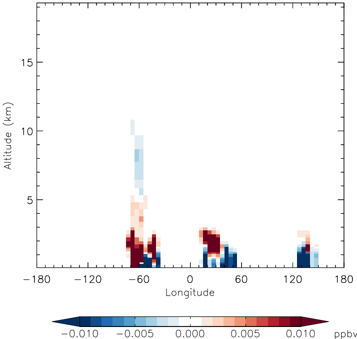
v11-01f-merra2-Run0 - v11-01d-Run1 RIP - Diff along 15S for Apr
