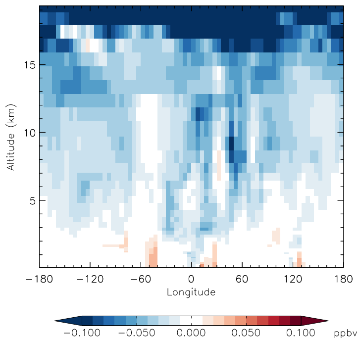
v11-01f-merra2-Run0 - v11-01f-geosfp-Run0 HNO 3 - Diff along 15S for Apr
