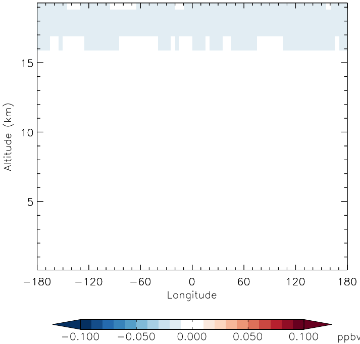
v11-01f-merra2-Run0 - v11-01d-Run1 CFC12 - Diff along 42N for Apr
