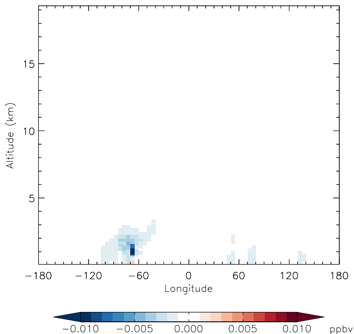
v11-01f-merra2-Run0 - v11-01f-geosfp-Run0 R4N2 - Diff along 42N for Apr
