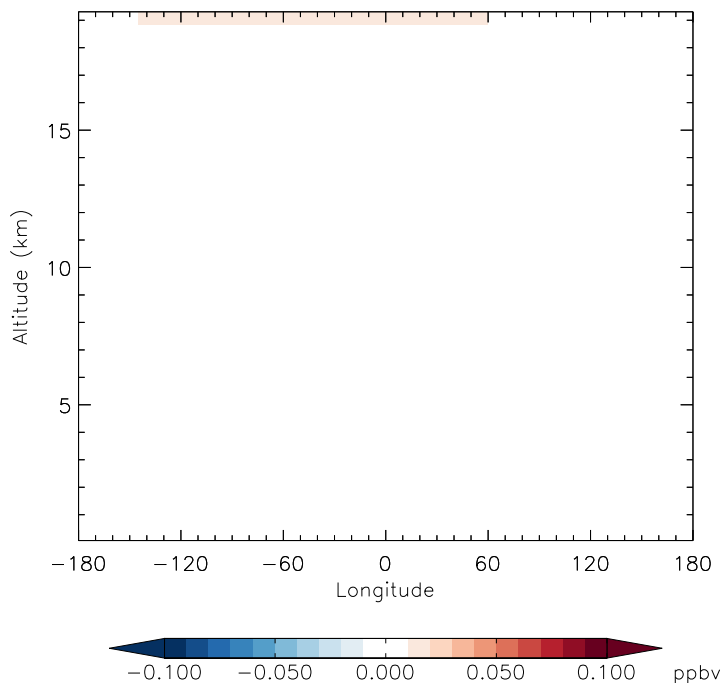
v11-01f-merra2-Run0 - v11-01f-geosfp-Run0 OCS - Diff along 15S for Apr
