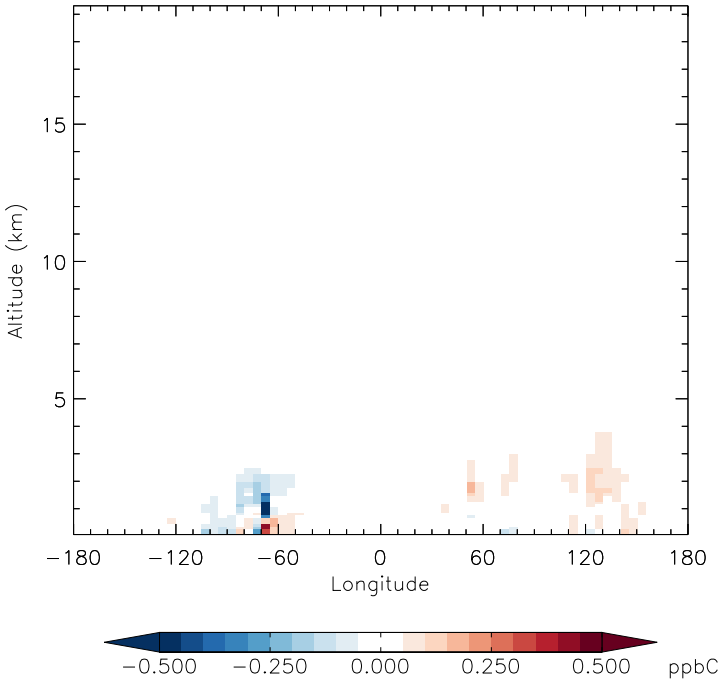
v11-01f-merra2-Run0 - v11-01d-Run1 ALK4 - Diff along 42N for Apr
