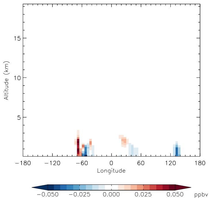
v11-01f-merra2-Run0 - v11-01f-geosfp-Run0 MACR - Diff along 15S for Apr
