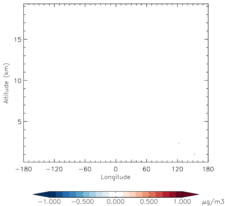
v11-01f-merra2-Run0 - v11-01d-Run1 NH4 - Diff along 42N for Apr
