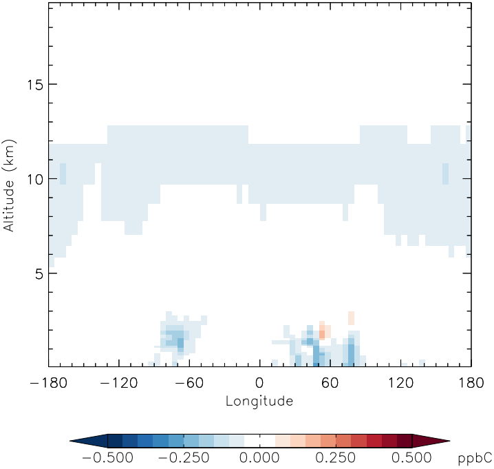
v11-01f-merra2-Run0 - v11-01d-Run1 C2H6 - Diff along 42N for Apr
