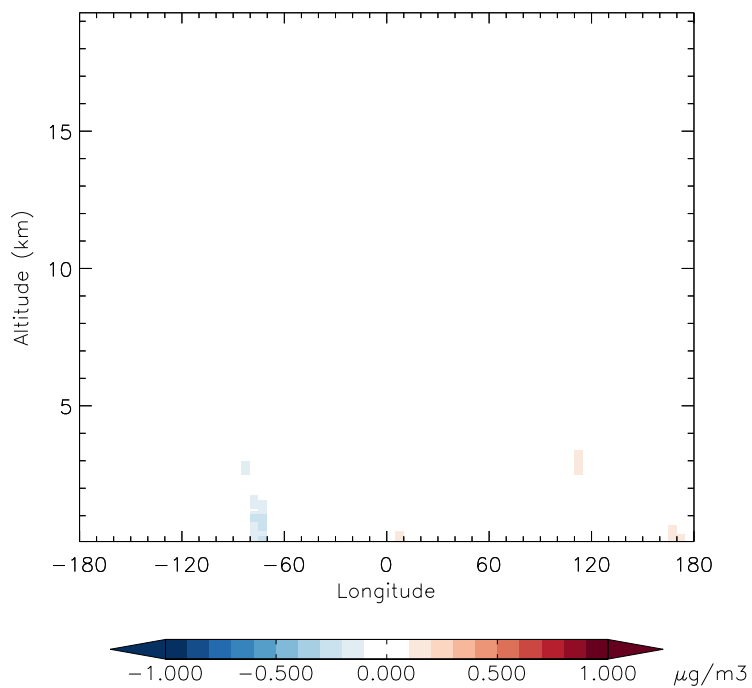
v11-01f-merra2-Run0 - v11-01d-Run1 S04 - Diff along 15S for Apr
