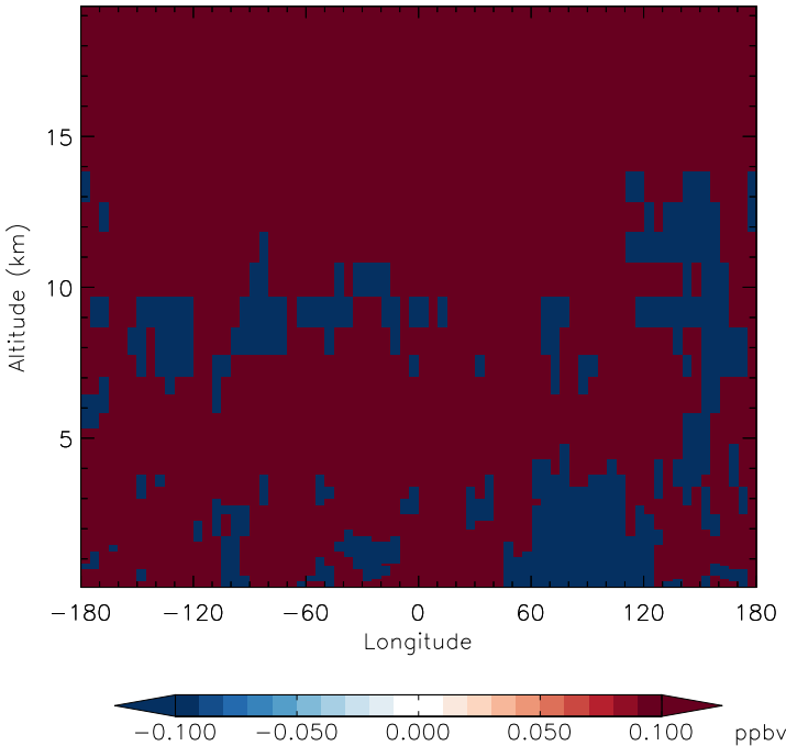
v11-01f-merra2-Run0 - v11-01d-Run1 H2O - Diff along 42N for Apr
