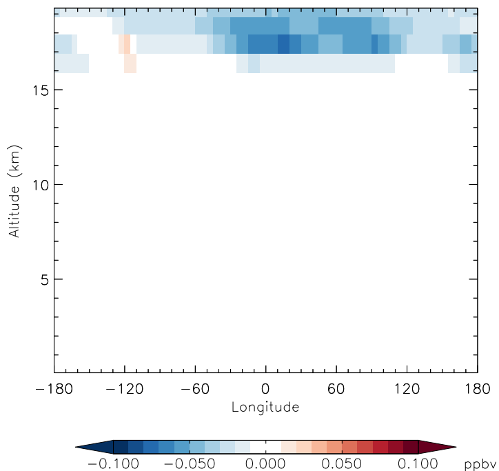
v11-01f-merra2-Run0 - v11-01f-geosfp-Run0 CINO3 - Diff along 15S for Jan
