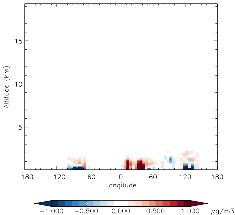
v11-01f-merra2-Run0 - v11-01f-geosfp-Run0 NIT - Diff along 42N for Jan
