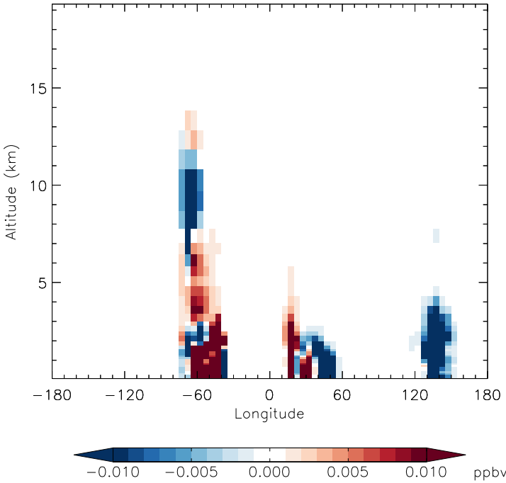
v11-01f-merra2-Run0 - v11-01f-geosfp-Run0 IEPOX - Diff along 15S for Jan
