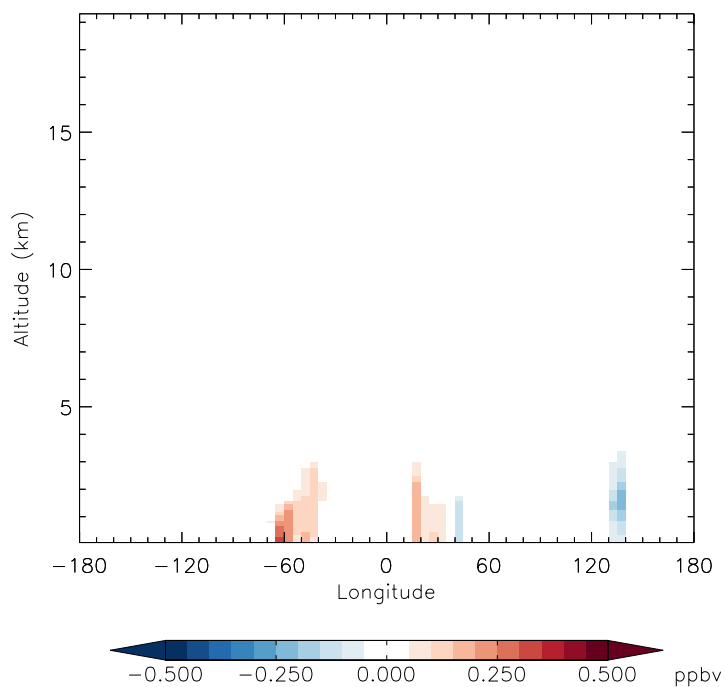
v11-01f-merra2-Run0 - v11-01f-geosfp-Run0 CH 2 O - Diff along 15S for Jan
