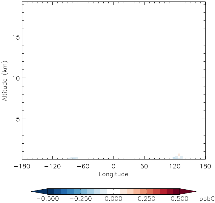
v11-01f-merra2-Run0 - v11-01d-Run1 ALD2 - Diff along 42N for Jan
