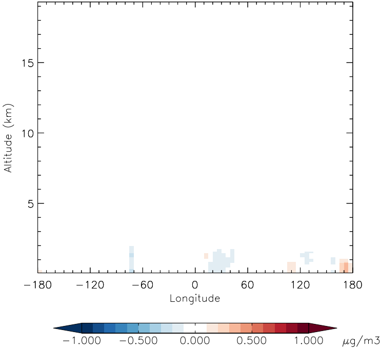
v11-01f-merra2-Run0 - v11-01d-Run1 S04 - Diff along 15S for Jan
