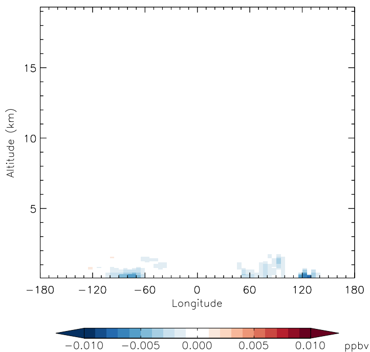
v11-01f-merra2-Run0 - v11-01f-geosfp-Run0 R4N2 - Diff along 42N for Jan
