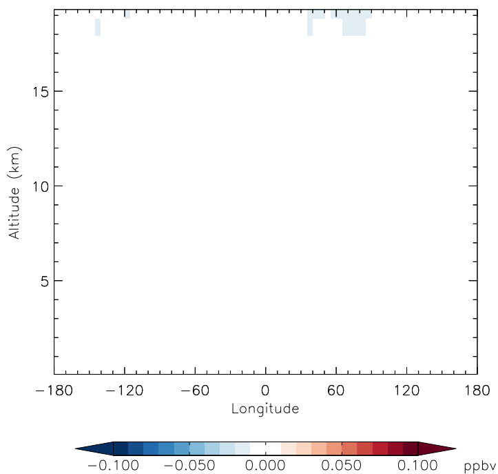
v11-01f-merra2-Run0 - v11-01f-geosfp-Run0 CH3Cl - Diff along 42N for Jan
