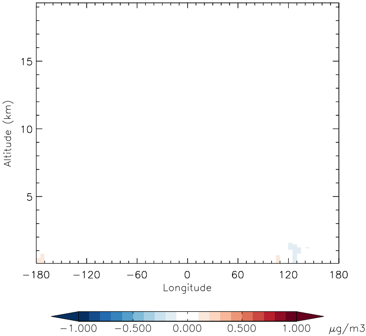
v11-01f-merra2-Run0 - v11-01f-geosfp-Run0 SALA - Diff along 15S for Jan
