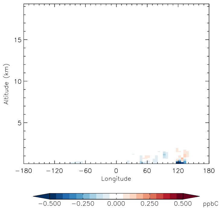
v11-01f-merra2-Run0 - v11-01d-Run1 C3H8 - Diff along 42N for Jan
