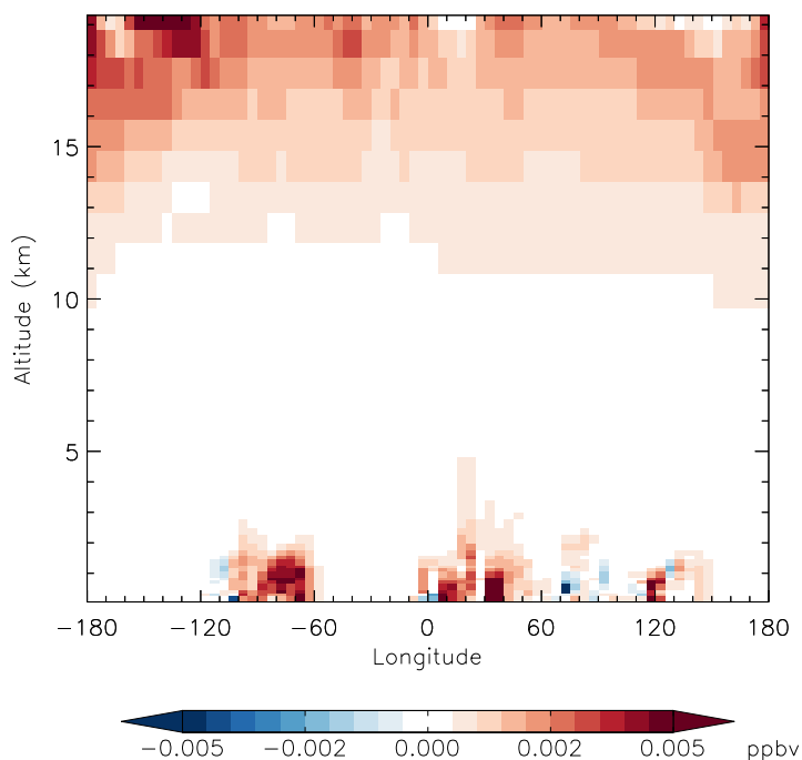
v11-01f-merra2-Run0 - v11-01f-geosfp-Run0 N2O5 - Diff along 42N for Jan
