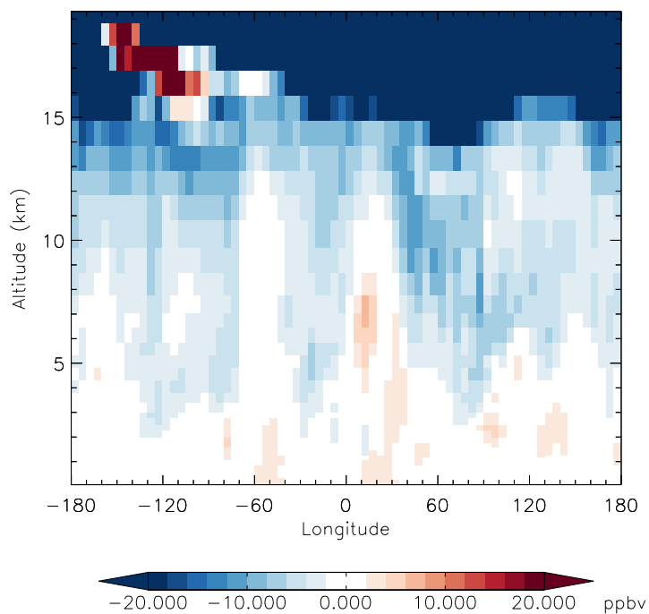
v11-01f-merra2-Run0 - v11-01d-Run1 O3 - Diff along 15S for Jan
