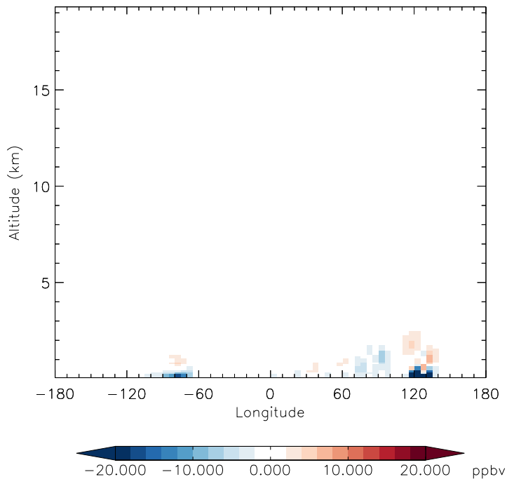
v11-01f-merra2-Run0 - v11-01d-Run1 CO - Diff along 42N for Jan
