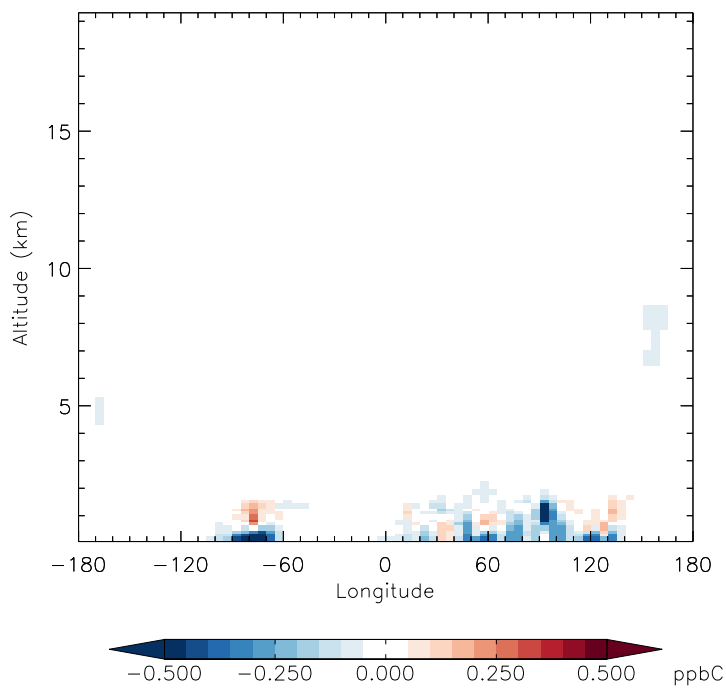
v11-01f-merra2-Run0 - v11-01d-Run1 C2H6 - Diff along 42N for Jan
