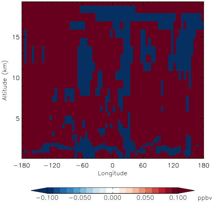
v11-01f-merra2-Run0 - v11-01d-Run1 H2O - Diff along 15S for Jan
