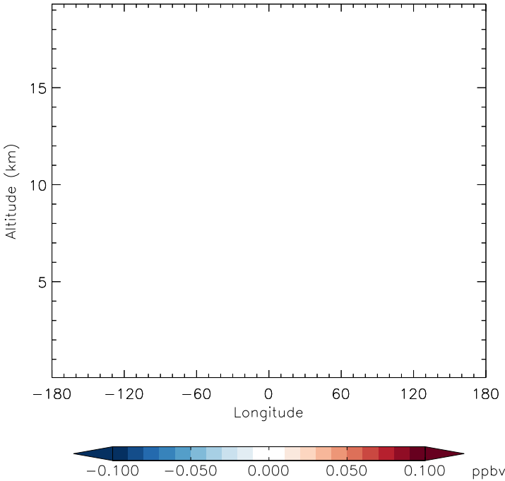
v11-01f-merra2-Run0 - v11-01d-Run1 H1301 - Diff along 42N for Jan
