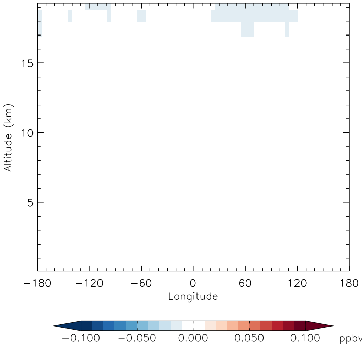
v11-01f-merra2-Run0 - v11-01f-geosfp-Run0 CFC12 - Diff along 42N for Jan
