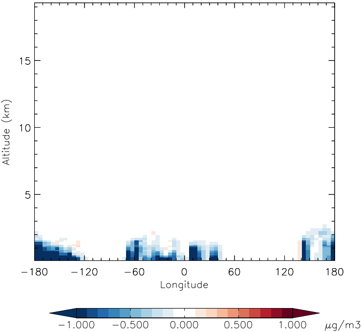
v11-01f-merra2-Run0 - v11-01d-Run1 SALC - Diff along 42N for Jan
