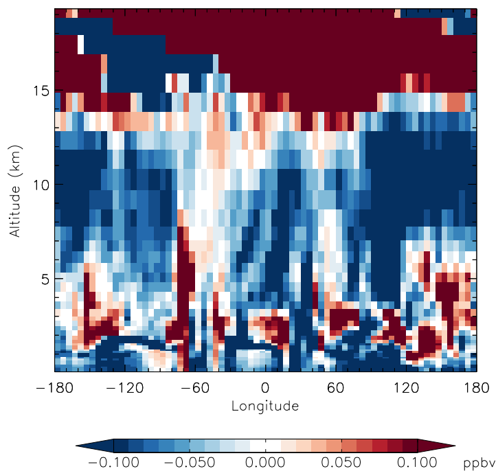
v11-01f-merra2-Run0 - v11-01d-Run1 N2O - Diff along 15S for Jan
