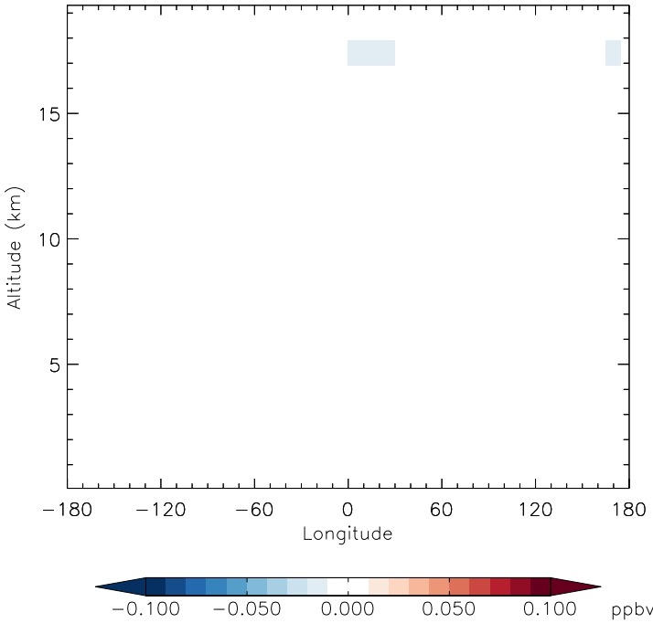
v11-01f-merra2-Run0 - v11-01f-geosfp-Run0 CIO - Diff along 15S for Jan
