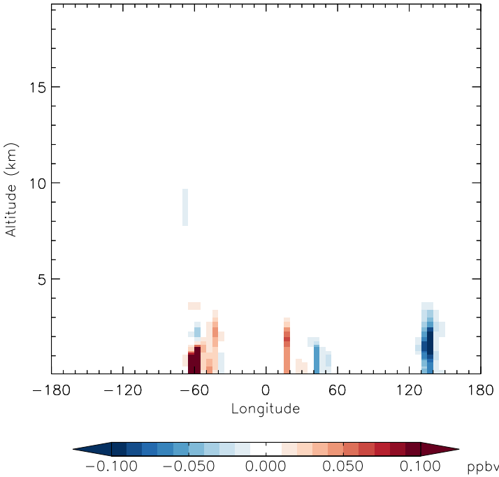
v11-01f-merra2-Run0 - v11-01f-geosfp-Run0 GLYC - Diff along 15S for Jan
