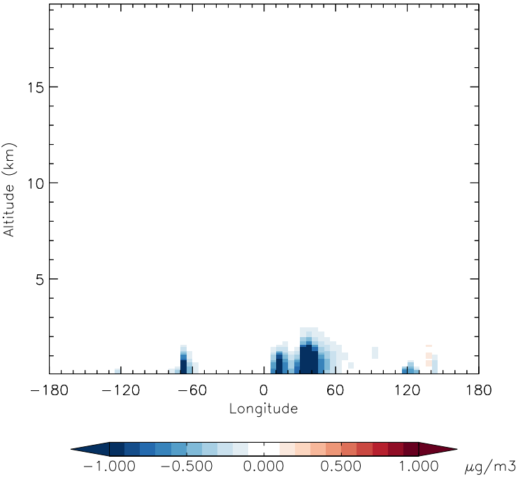
v11-01f-merra2-Run0 - v11-01f-geosfp-Run0 S04 - Diff along 42N for Jan
