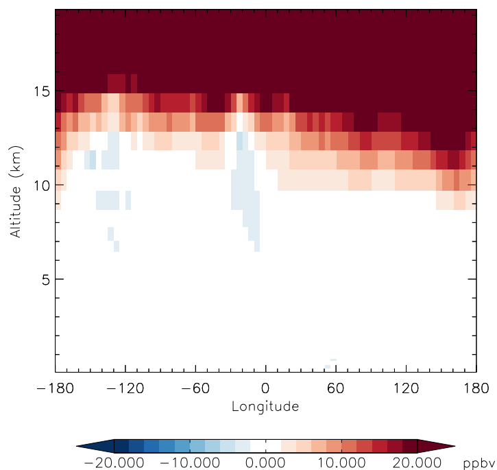
v11-01f-merra2-Run0 - v11-01f-geosfp-Run0 O3 - Diff along 42N for Jan
