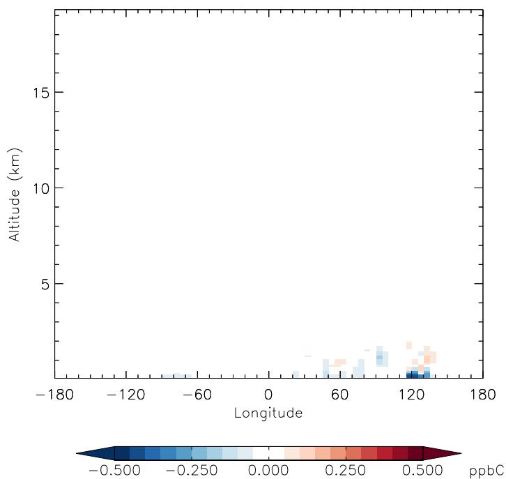
v11-01f-merra2-Run0 - v11-01f-geosfp-Run0 C3H8 - Diff along 42N for Jan
