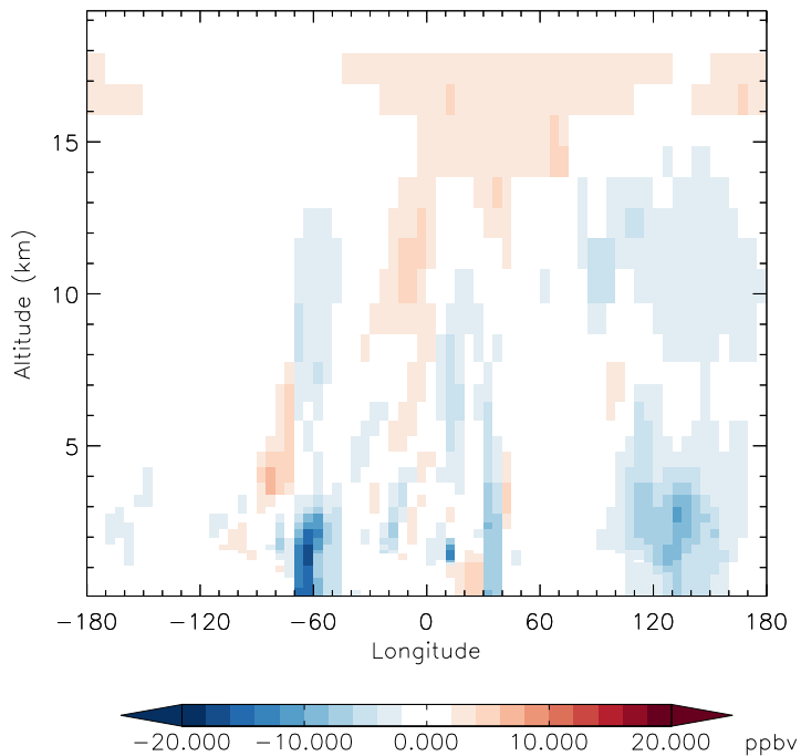
v11-01f-merra2-Run0 - v11-01d-Run1 CO - Diff along 15S for Jan
