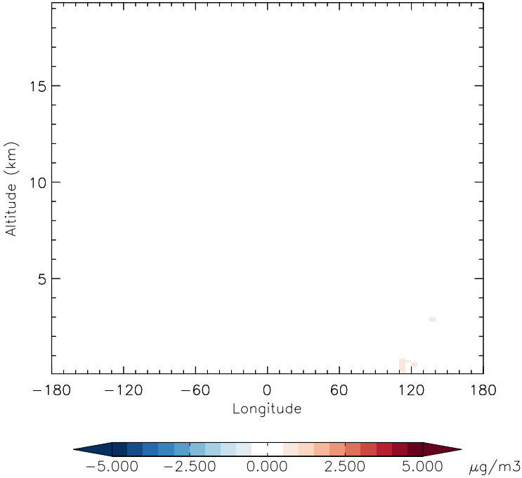
v11-01f-merra2-Run0 - v11-01d-Run1 DST1 - Diff along 15S for Jan
