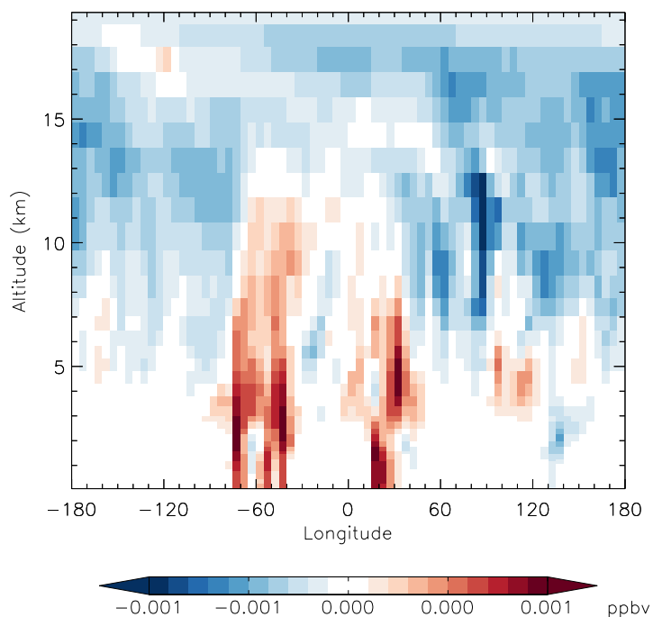
v11-01f-merra2-Run0 - v11-01f-geosfp-Run0 PPN - Diff along 15S for Jan
