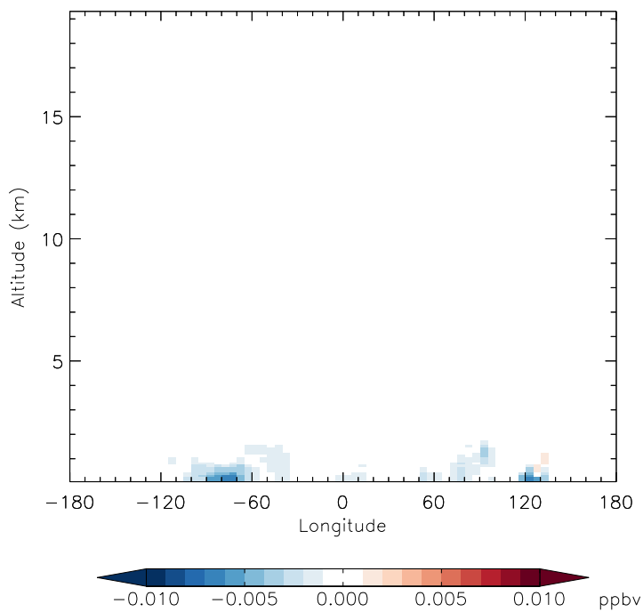
v11-01f-merra2-Run0 - v11-01d-Run1 R4N2 - Diff along 42N for Jan
