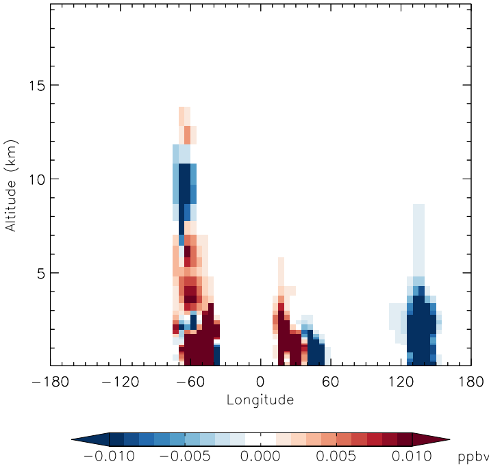
v11-01f-merra2-Run0 - v11-01d-Run1 IEPOX - Diff along 15S for Jan
