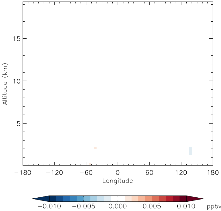
v11-01f-merra2-Run0 - v11-01f-geosfp-Run0 PMN - Diff along 15S for Jan
