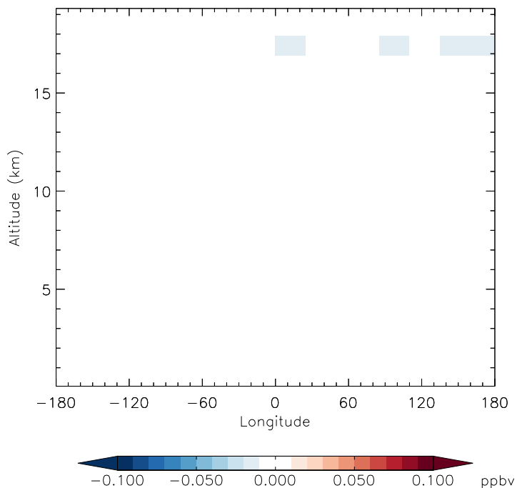
v11-01f-merra2-Run0 - v11-01f-geosfp-Run0 HOCl - Diff along 15S for Jan
