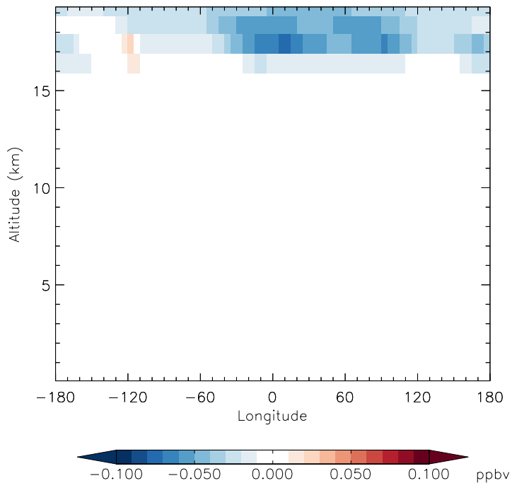
v11-01f-merra2-Run0 - v11-01d-Run1 CINO3 - Diff along 15S for Jan
