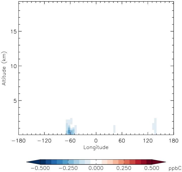
v11-01f-merra2-Run0 - v11-01f-geosfp-Run0 ALD2 - Diff along 15S for Jan
