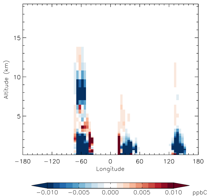
v11-01f-merra2-Run0 - v11-01f-geosfp-Run0 PRPE - Diff along 15S for Jan
