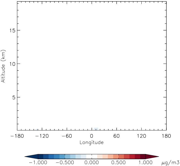
v11-01f-merra2-Run0 - v11-01d-Run1 SALA - Diff along 42N for Jan
