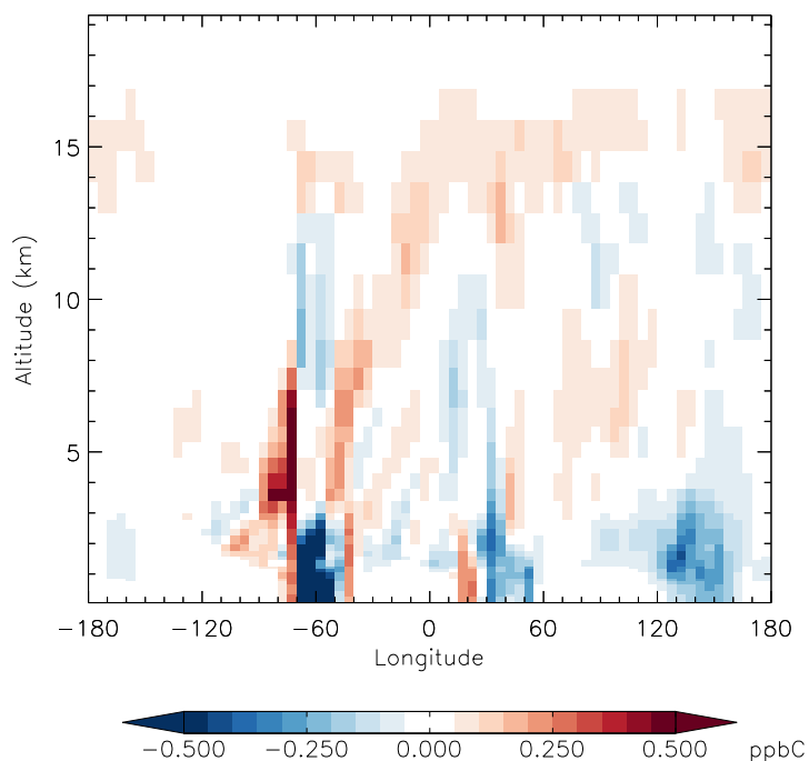
v11-01f-merra2-Run0 - v11-01f-geosfp-Run0 ACET - Diff along 15S for Jan
