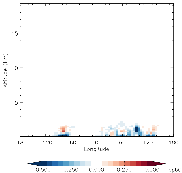
v11-01f-merra2-Run0 - v11-01f-geosfp-Run0 C2H6 - Diff along 42N for Jan
