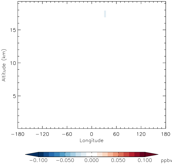
v11-01f-merra2-Run0 - v11-01f-geosfp-Run0 Cl2 - Diff along 15S for Jan
