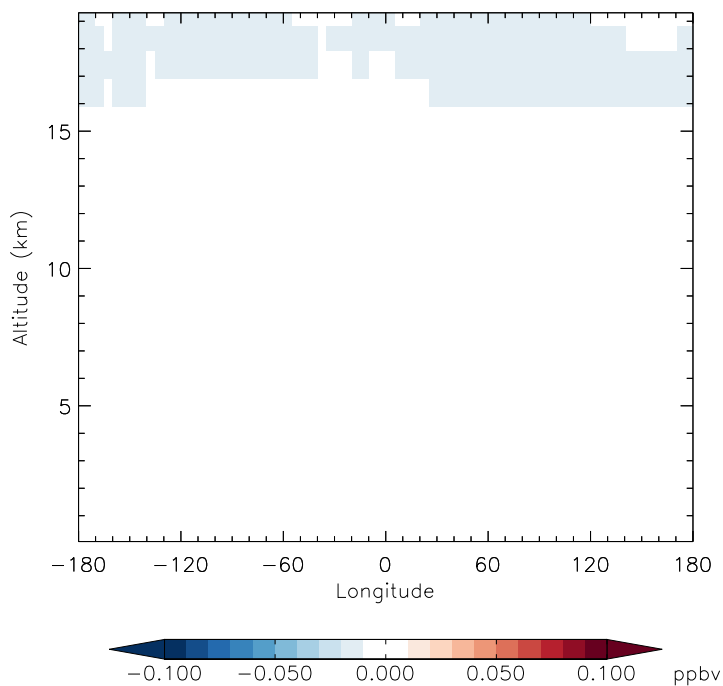
v11-01f-merra2-Run0 - v11-01d-Run1 OCS - Diff along 42N for Jan
