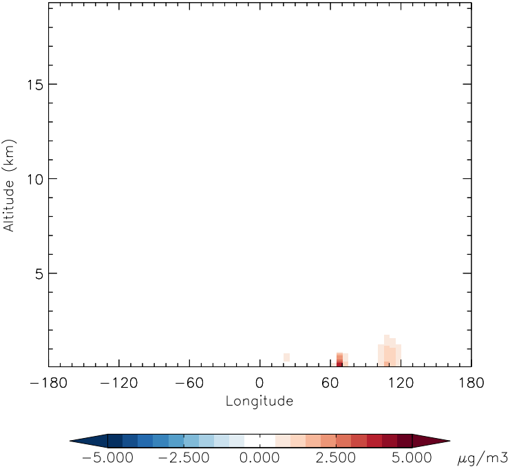
v11-01f-merra2-Run0 - v11-01d-Run1 DST4 - Diff along 42N for Jan
