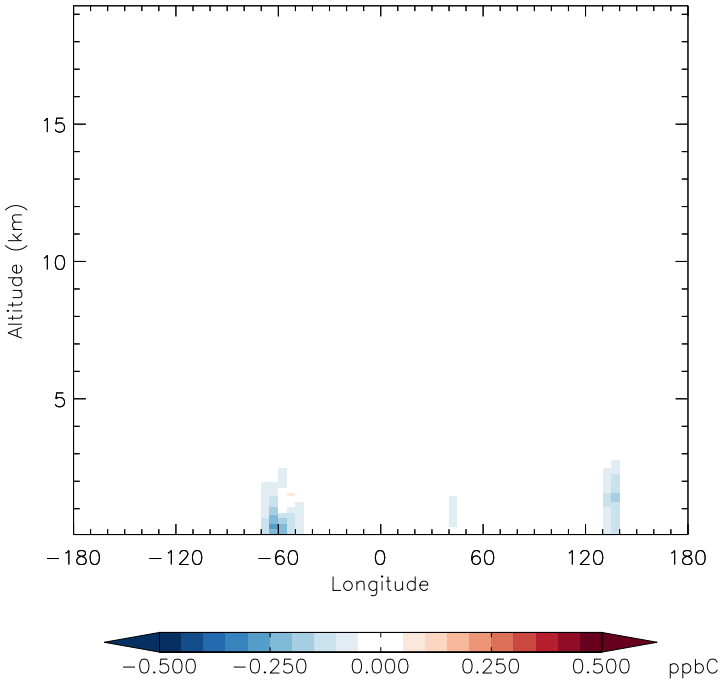
v11-01f-merra2-Run0 - v11-01d-Run1 ALD2 - Diff along 15S for Jan
