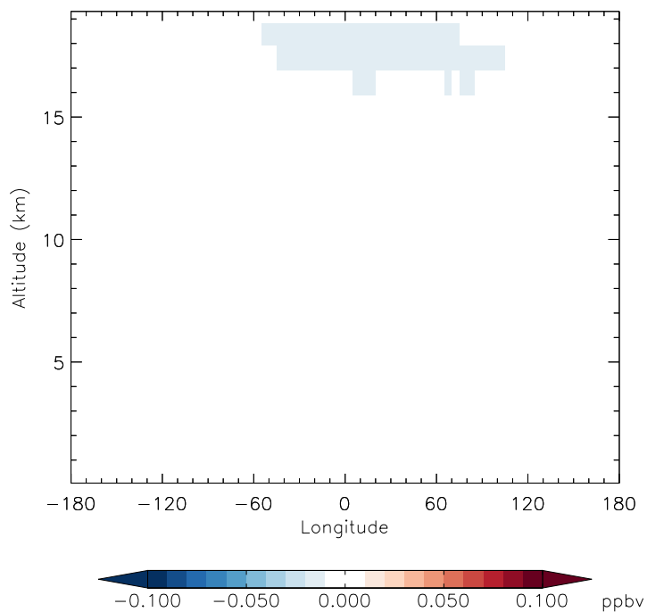
v11-01f-merra2-Run0 - v11-01d-Run1 MPN - Diff along 15S for Jan
