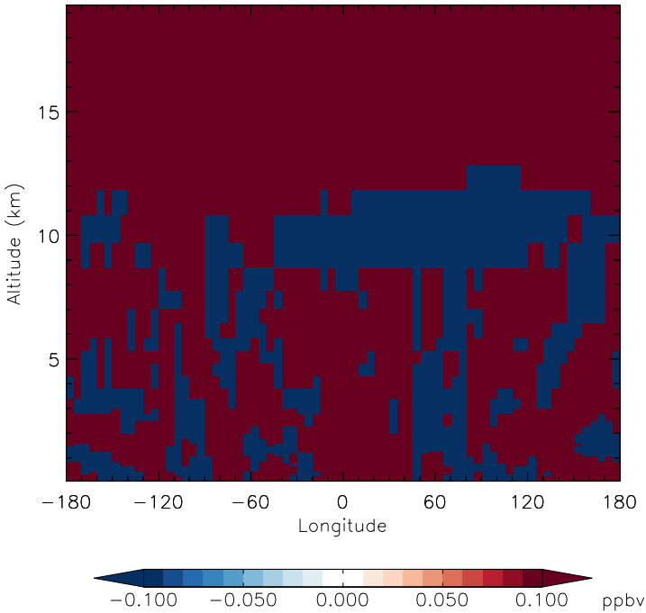
v11-01f-merra2-Run0 - v11-01d-Run1 H2O - Diff along 42N for Jan
