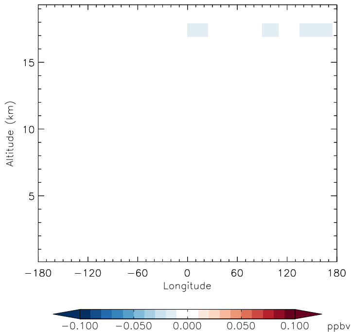
v11-01f-merra2-Run0 - v11-01d-Run1 HOCl - Diff along 15S for Jan
