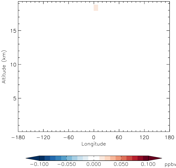
v11-01f-merra2-Run0 - v11-01f-geosfp-Run0 CFC12 - Diff along 15S for Jan
