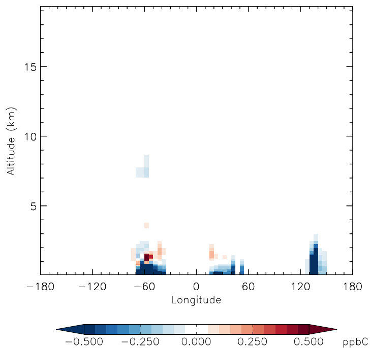
v11-01f-merra2-Run0 - v11-01d-Run1 ISOP - Diff along 15S for Jan
