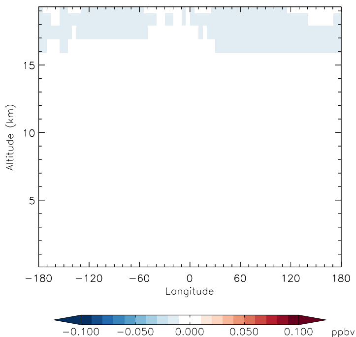
v11-01f-merra2-Run0 - v11-01f-geosfp-Run0 OCS - Diff along 42N for Jan
