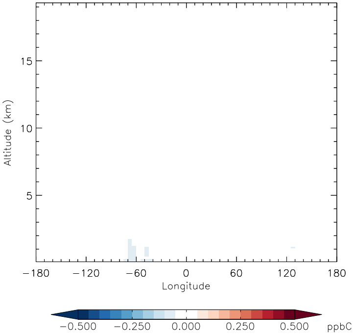
v11-01f-merra2-Run0 - v11-01f-geosfp-Run0 ALK4 - Diff along 15S for Jan
