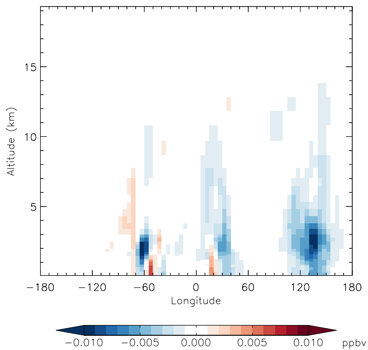
v11-01f-merra2-Run0 - v11-01d-Run1 R4N2 - Diff along 15S for Jan
