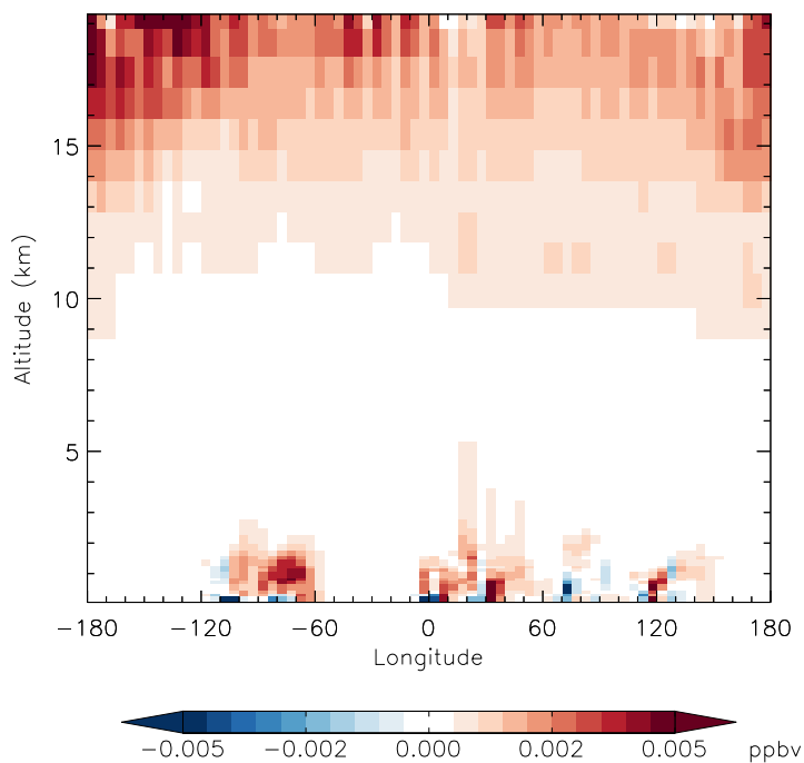
v11-01f-merra2-Run0 - v11-01d-Run1 N2O5 - Diff along 42N for Jan
