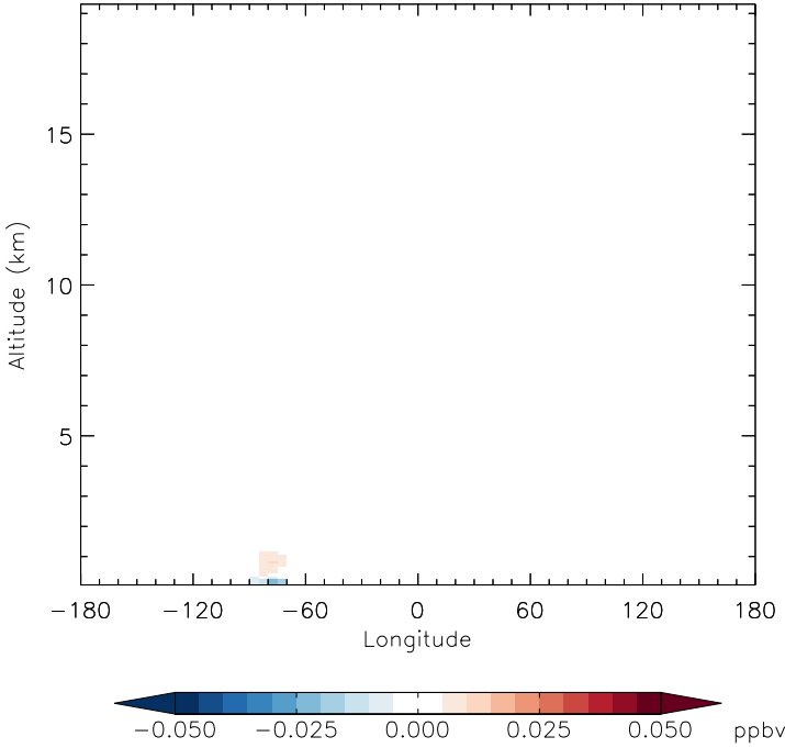
v11-01f-merra2-Run0 - v11-01d-Run1 RCHO - Diff along 42N for Jan
