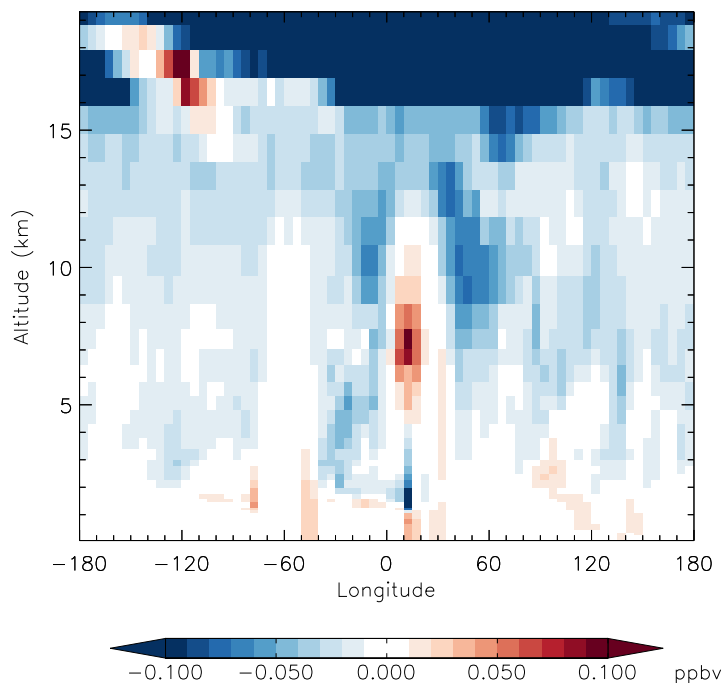
v11-01f-merra2-Run0 - v11-01f-geosfp-Run0 HNO 3 - Diff along 15S for Jan
