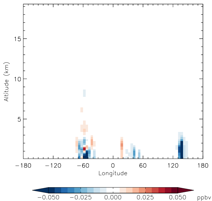
v11-01f-merra2-Run0 - v11-01f-geosfp-Run0 MVK - Diff along 15S for Jan
