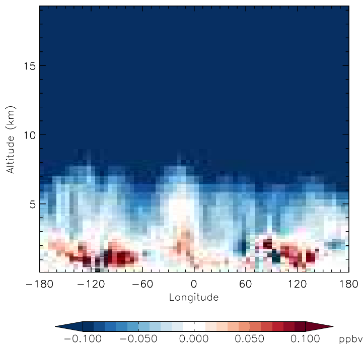
v11-01f-merra2-Run0 - v11-01f-geosfp-Run0 N2O - Diff along 42N for Jan
