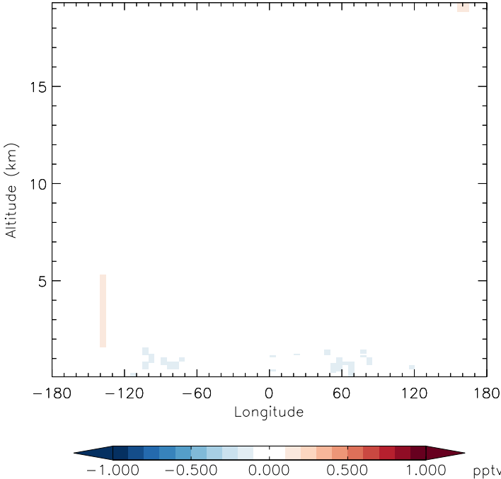
v11-01f-merra2-Run0 - v11-01d-Run1 HO2 - Diff along 42N for Jan
