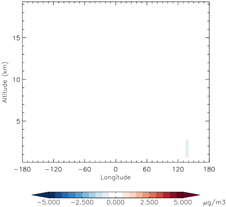
v11-01f-merra2-Run0 - v11-01f-geosfp-Run0 DST4 - Diff along 15S for Jan
