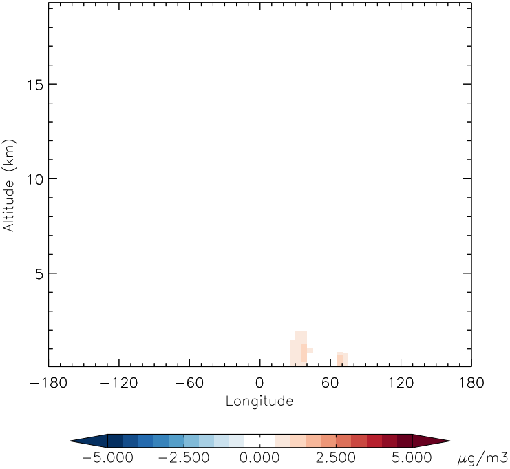
v11-01f-merra2-Run0 - v11-01d-Run1 DST1 - Diff along 42N for Jan
