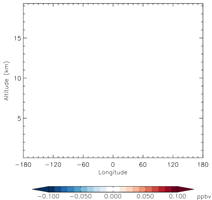
v11-01f-merra2-Run0 - v11-01f-geosfp-Run0 ClO 0 - Diff along 15S for Jan
