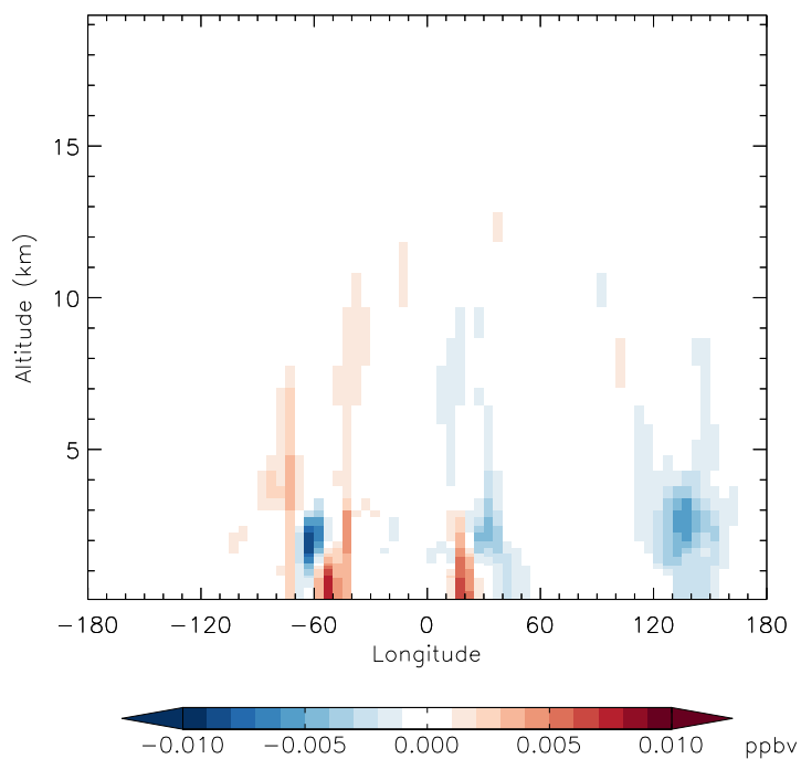
v11-01f-merra2-Run0 - v11-01f-geosfp-Run0 R4N2 - Diff along 15S for Jan
