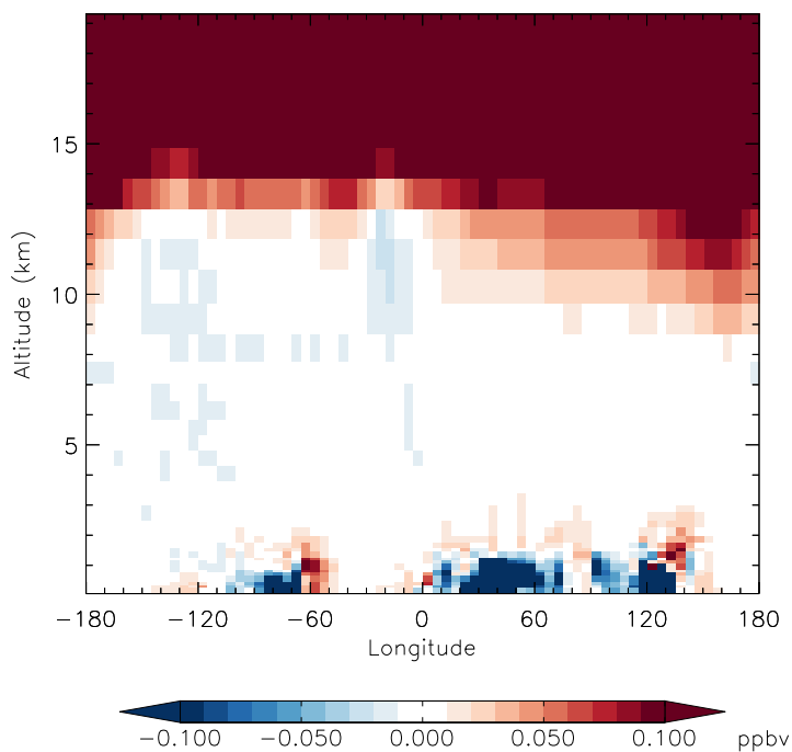
v11-01f-merra2-Run0 - v11-01d-Run1 HNO 3 - Diff along 42N for Jan
