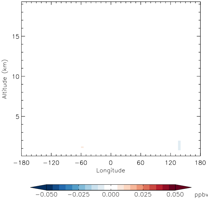
v11-01f-merra2-Run0 - v11-01f-geosfp-Run0 RCHO - Diff along 15S for Jan
