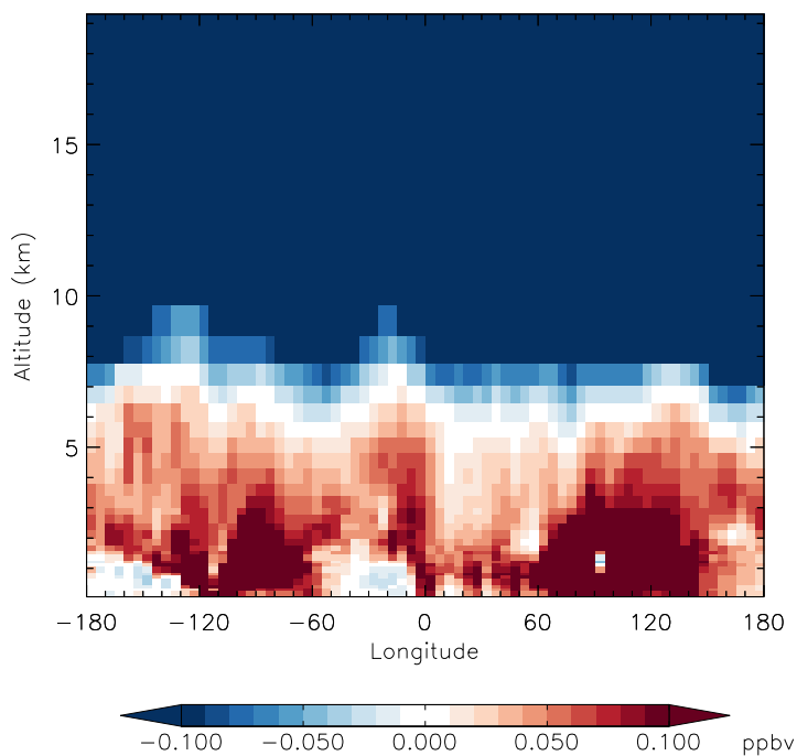
v11-01f-merra2-Run0 - v11-01d-Run1 N2O - Diff along 42N for Jan
