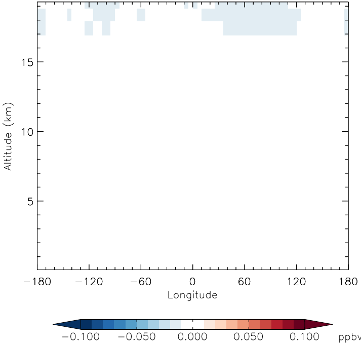
v11-01f-merra2-Run0 - v11-01d-Run1 CFC12 - Diff along 42N for Jan
