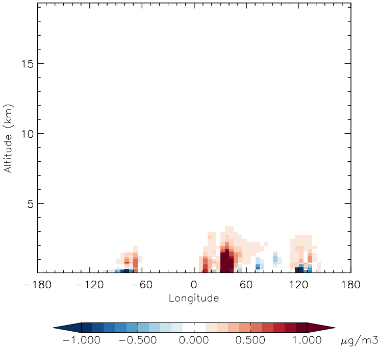
v11-01f-merra2-Run0 - v11-01f-geosfp-Run0 SO2 - Diff along 42N for Jan
