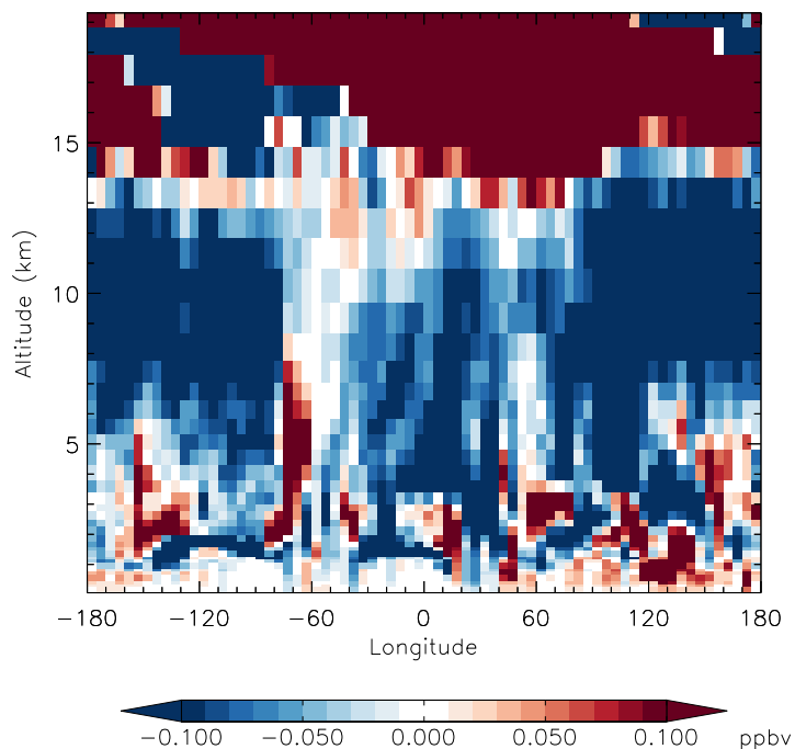
v11-01f-merra2-Run0 - v11-01f-geosfp-Run0 N2O - Diff along 15S for Jan
