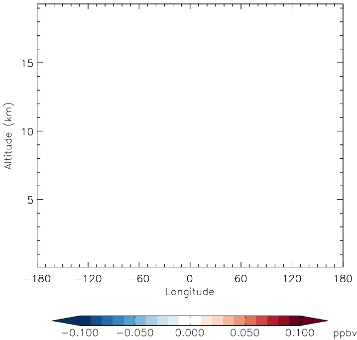
v11-01f-merra2-Run0 - v11-01d-Run1 H1211 - Diff along 15S for Jan
