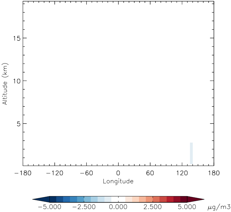
v11-01f-merra2-Run0 - v11-01d-Run1 DST4 - Diff along 15S for Jan
