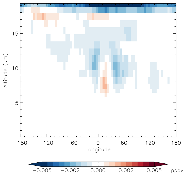
v11-01f-merra2-Run0 - v11-01f-geosfp-Run0 N2O5 - Diff along 15S for Jan
