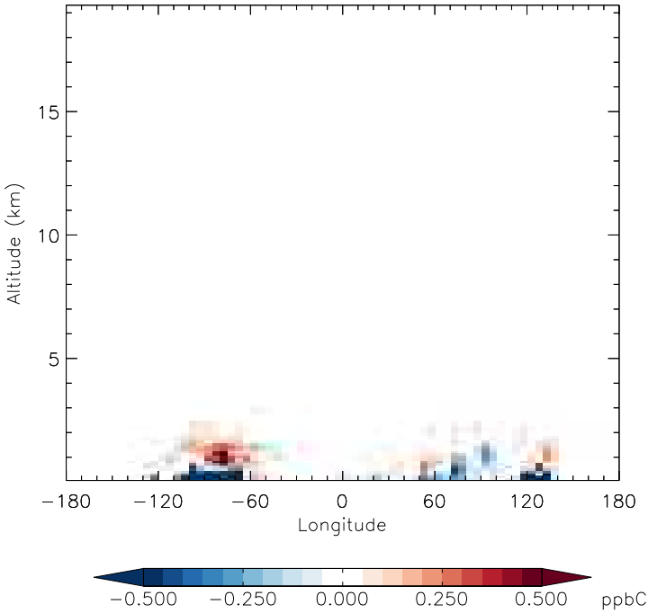
v11-01f-merra2-Run0 - v11-01f-geosfp-Run0 ALK4 - Diff along 42N for Jan
