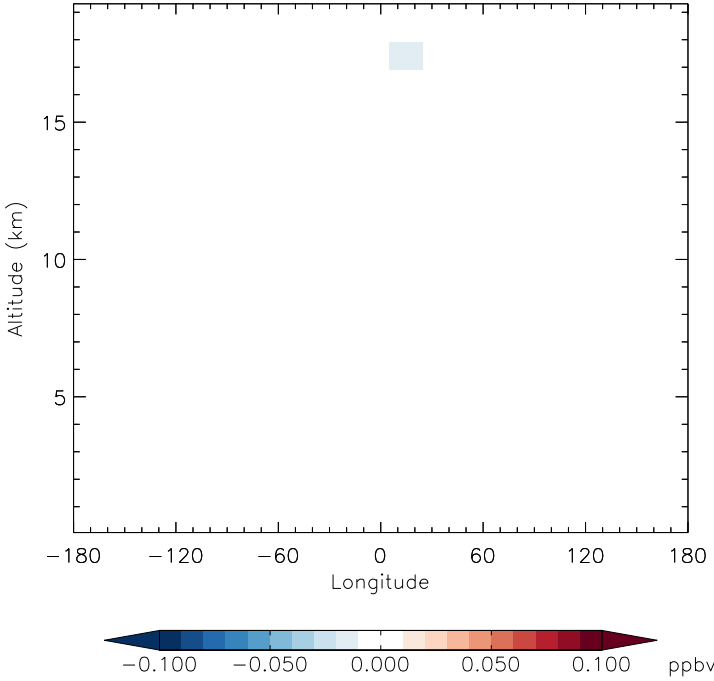
v11-01f-merra2-Run0 - v11-01d-Run1 CIO - Diff along 15S for Jan
