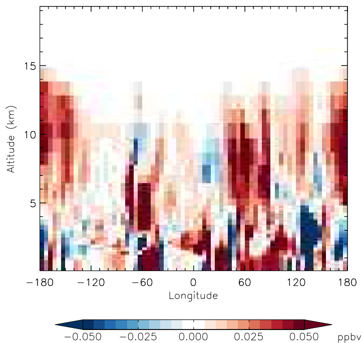
v11-01f-merra2-Run0 - v11-01d-Run1 MP - Diff along 15S for Jan
