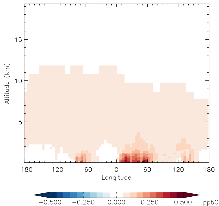
v11-01f-merra2-Run0 - v11-01d-Run1 ACET - Diff along 42N for Jan
