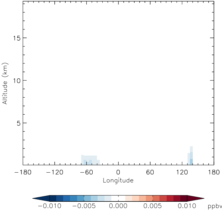
v11-01f-merra2-Run0 - v11-01d-Run1 MOBA - Diff along 15S for Jan
