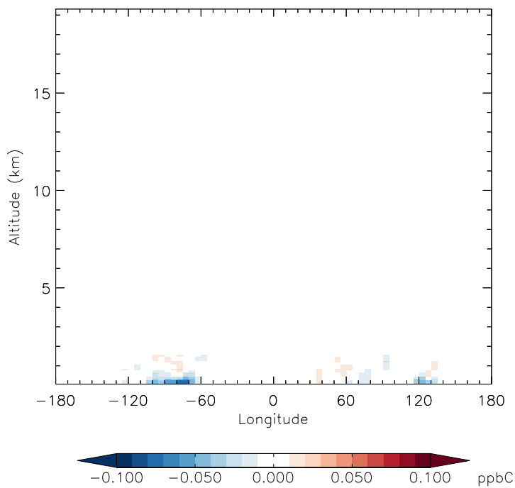
v11-01f-merra2-Run0 - v11-01d-Run1 MEK - Diff along 42N for Jan
