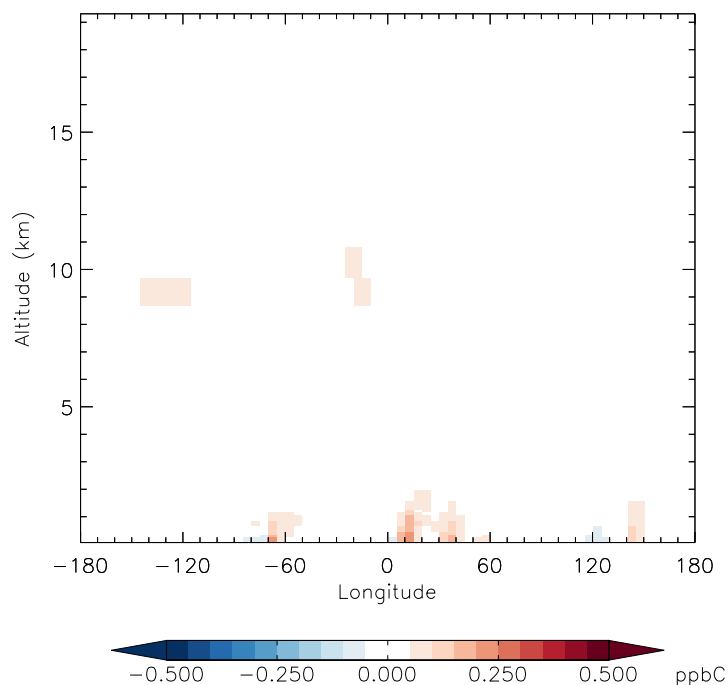
v11-01f-merra2-Run0 - v11-01f-geosfp-Run0 ACET - Diff along 42N for Jan
