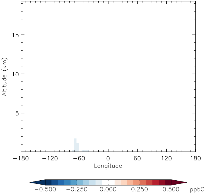
v11-01f-merra2-Run0 - v11-01d-Run1 ALK4 - Diff along 15S for Jan
