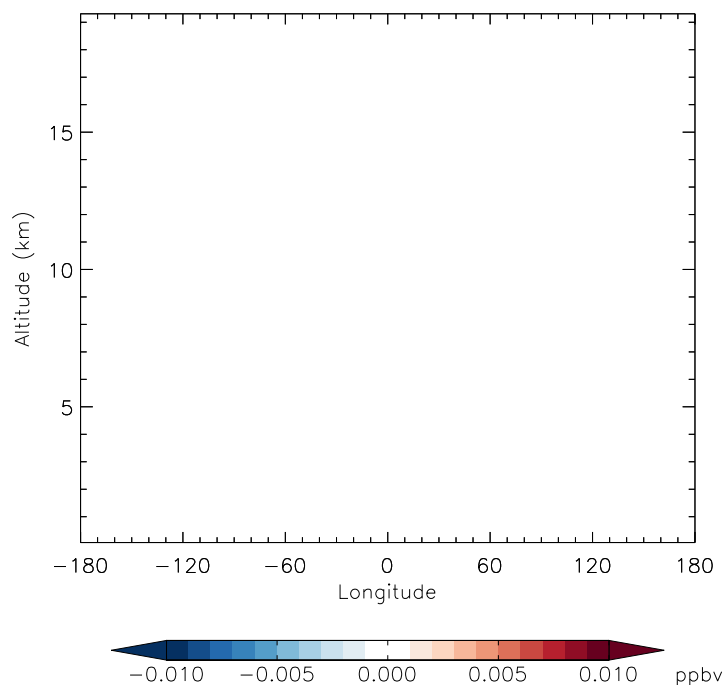
v11-01f-merra2-Run0 - v11-01f-geosfp-Run0 BrO - Diff along 42N for Jan
