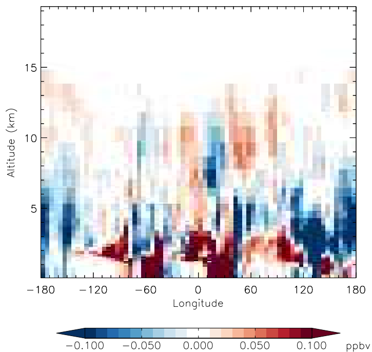
v11-01f-merra2-Run0 - v11-01d-Run1 H2O2 - Diff along 15S for Jan
