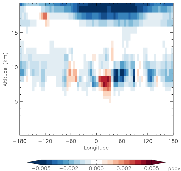
v11-01f-merra2-Run0 - v11-01f-geosfp-Run0 HNO 4 - Diff along 15S for Jan
