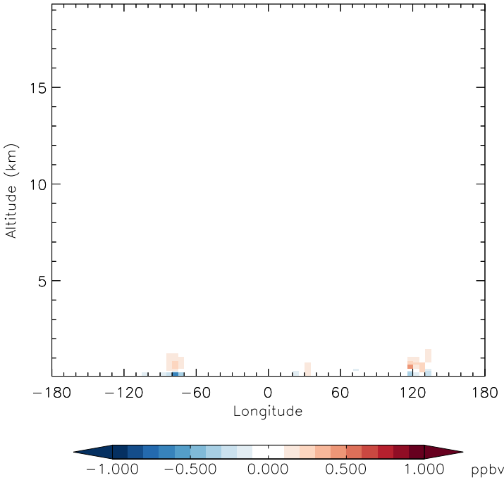
v11-01f-merra2-Run0 - v11-01f-geosfp-Run0 NO2 - Diff along 42N for Jan
