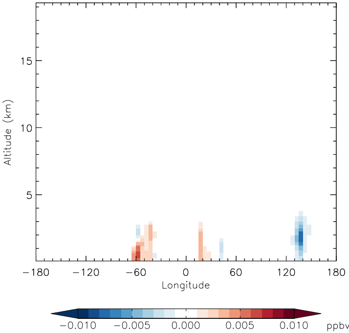
v11-01f-merra2-Run0 - v11-01f-geosfp-Run0 MMN - Diff along 15S for Jan
