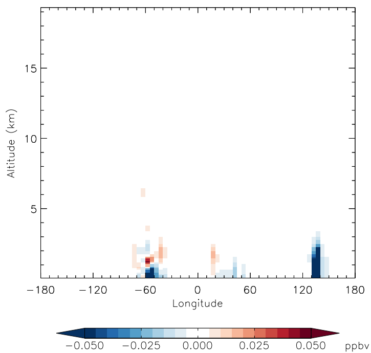
v11-01f-merra2-Run0 - v11-01d-Run1 MACR - Diff along 15S for Jan
