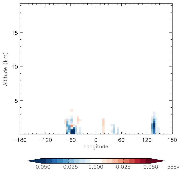
v11-01f-merra2-Run0 - v11-01f-geosfp-Run0 MACR - Diff along 15S for Jan
