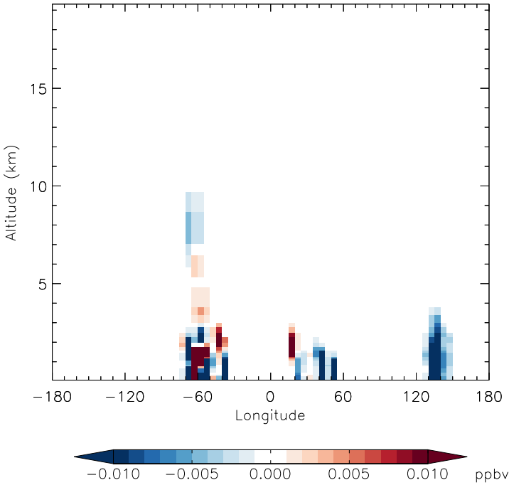
v11-01f-merra2-Run0 - v11-01f-geosfp-Run0 RIP - Diff along 15S for Jan
