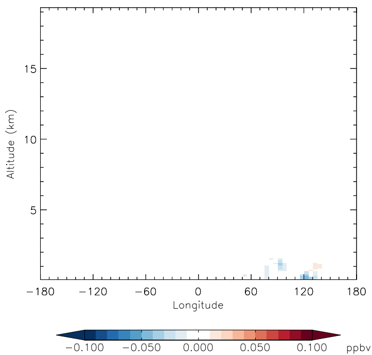
v11-01f-merra2-Run0 - v11-01d-Run1 PAN - Diff along 42N for Jan
