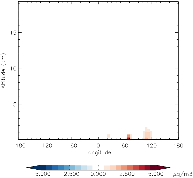
v11-01f-merra2-Run0 - v11-01f-geosfp-Run0 DST4 - Diff along 42N for Jan
