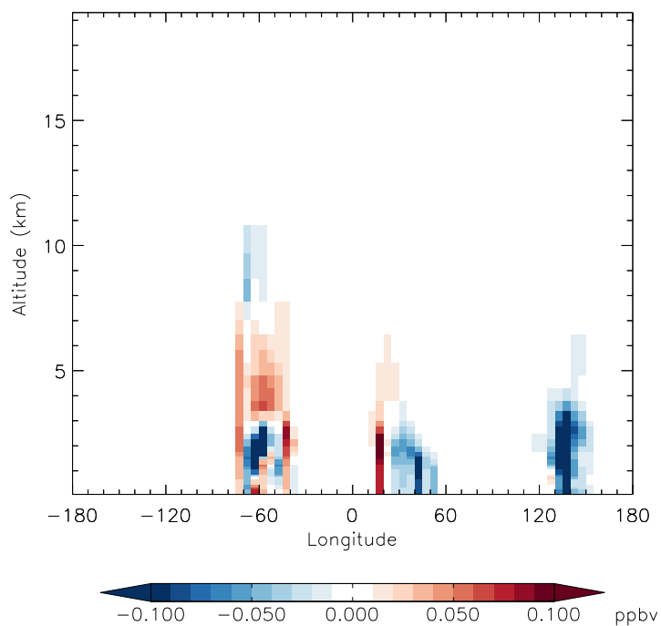
v11-01f-merra2-Run0 - v11-01f-geosfp-Run0 HAC - Diff along 15S for Jan
