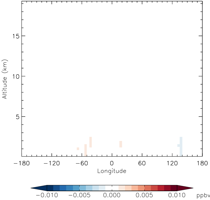
v11-01f-merra2-Run0 - v11-01d-Run1 PMN - Diff along 15S for Jan
