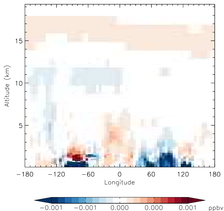
v11-01f-merra2-Run0 - v11-01f-geosfp-Run0 PPN - Diff along 42N for Jan
