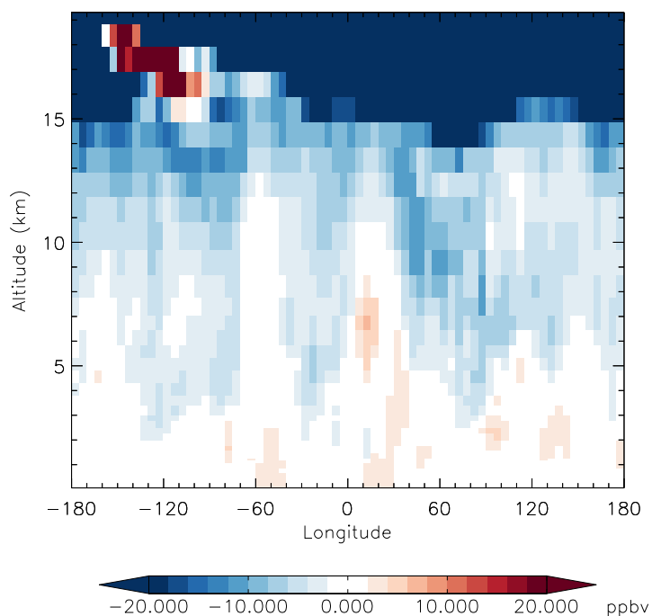
v11-01f-merra2-Run0 - v11-01f-geosfp-Run0 O3 - Diff along 15S for Jan
