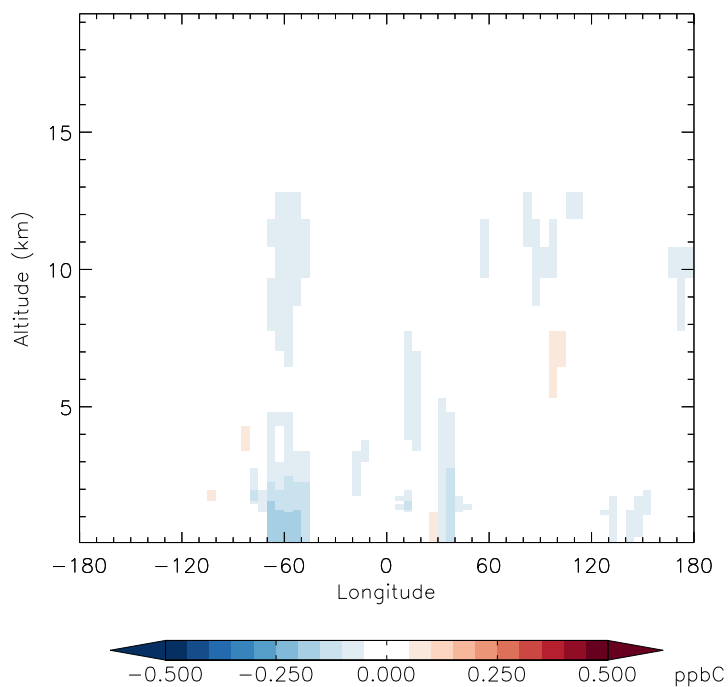
v11-01f-merra2-Run0 - v11-01f-geosfp-Run0 C2H6 - Diff along 15S for Jan
