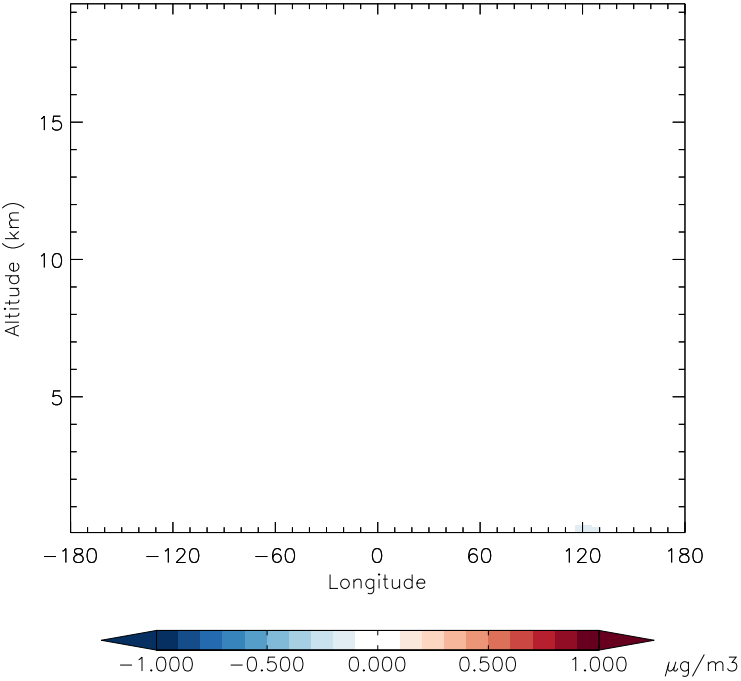
v11-01f-merra2-Run0 - v11-01d-Run1 BCPI - Diff along 42N for Jan
