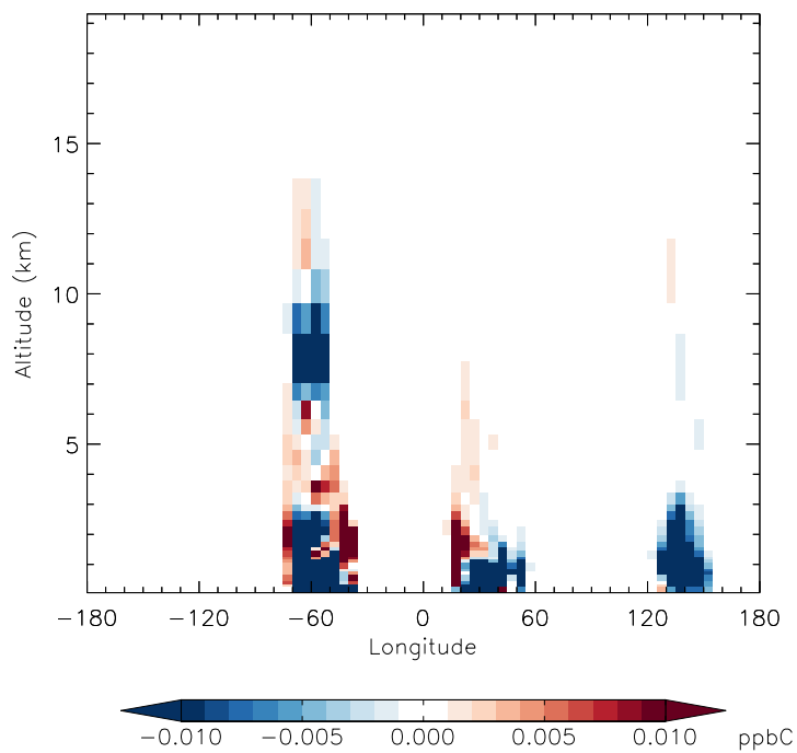
v11-01f-merra2-Run0 - v11-01d-Run1 PRPE - Diff along 15S for Jan
