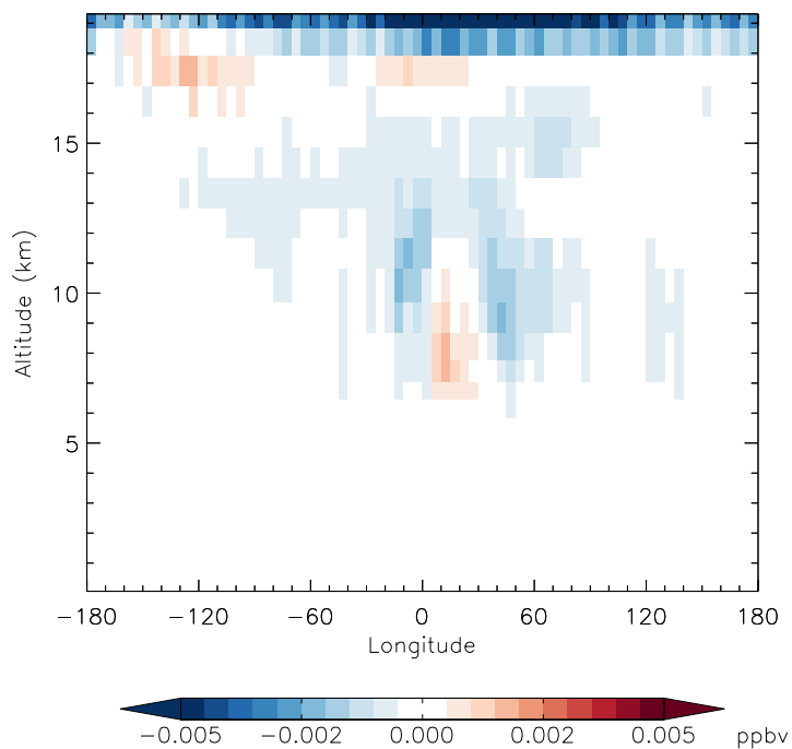
v11-01f-merra2-Run0 - v11-01d-Run1 N2O5 - Diff along 15S for Jan
