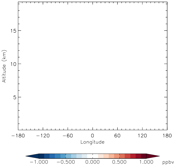
v11-01f-merra2-Run0 - v11-01f-geosfp-Run0 HNO2 - Diff along 15S for Jan
