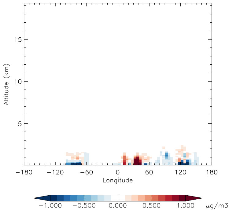
v11-01f-merra2-Run0 - v11-01d-Run1 NIT - Diff along 42N for Jan
