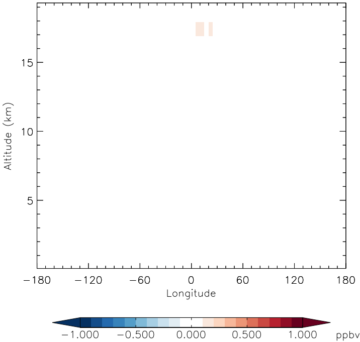
v11-01f-merra2-Run0 - v11-01d-Run1 NO2 - Diff along 15S for Jan
