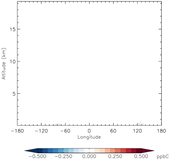
v11-01f-merra2-Run0 - v11-01f-geosfp-Run0 ALD2 - Diff along 42N for Jan
