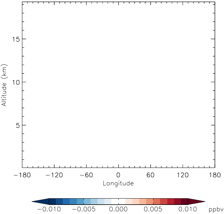
v11-01f-merra2-Run0 - v11-01f-geosfp-Run0 Br - Diff along 42N for Jan
