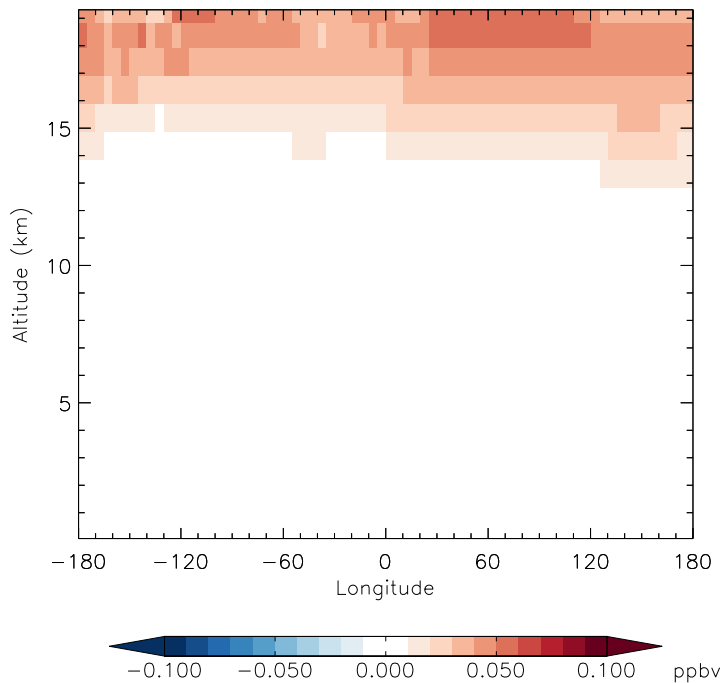
v11-01f-merra2-Run0 - v11-01d-Run1 CINO3 - Diff along 42N for Jan
