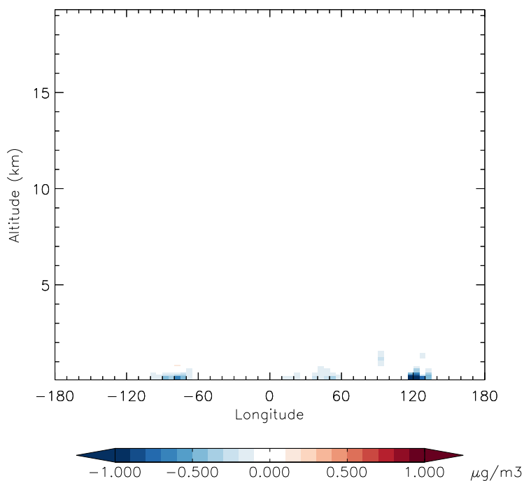
v11-01f-merra2-Run0 - v11-01f-geosfp-Run0 NH4 - Diff along 42N for Jan
