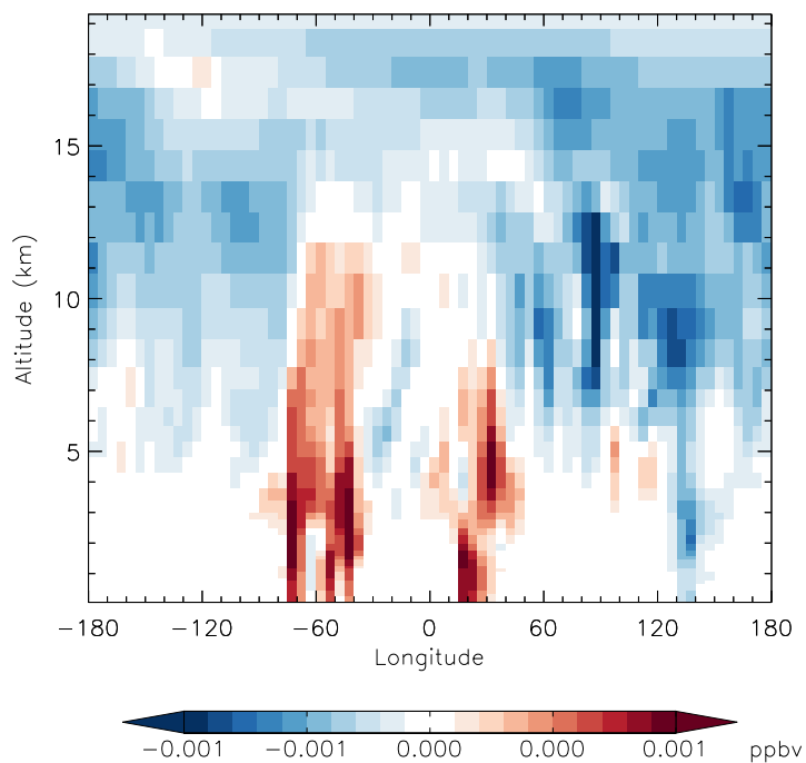
v11-01f-merra2-Run0 - v11-01d-Run1 PPN - Diff along 15S for Jan
