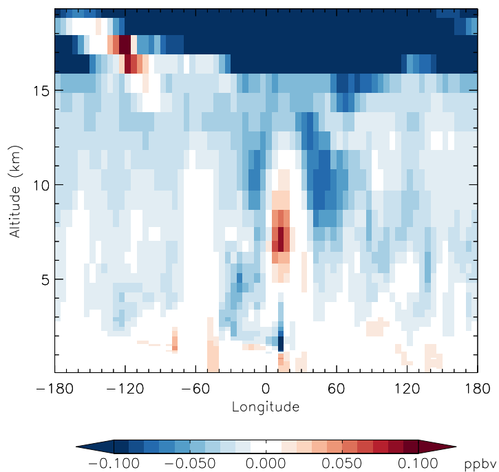
v11-01f-merra2-Run0 - v11-01d-Run1 HNO 3 - Diff along 15S for Jan
