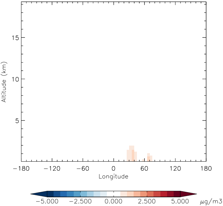
v11-01f-merra2-Run0 - v11-01f-geosfp-Run0 DST1 - Diff along 42N for Jan
