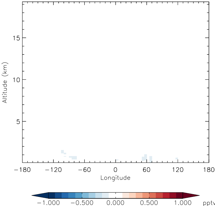
v11-01f-merra2-Run0 - v11-01f-geosfp-Run0 HO2 - Diff along 42N for Jan
