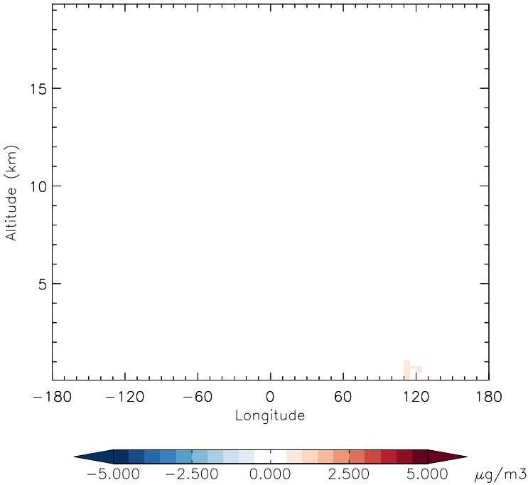
v11-01f-merra2-Run0 - v11-01f-geosfp-Run0 DST1 - Diff along 15S for Jan
