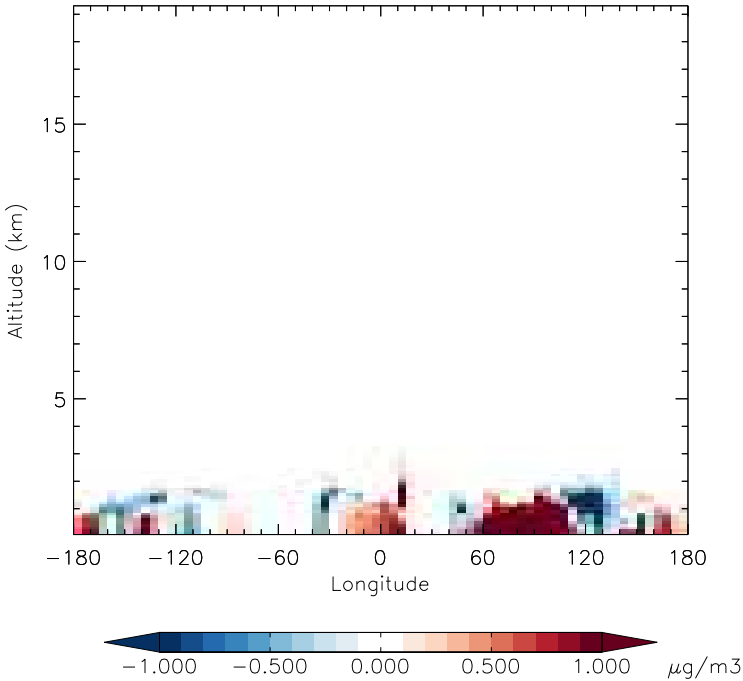
v11-01f-merra2-Run0 - v11-01d-Run1 SALC - Diff along 15S for Jan
