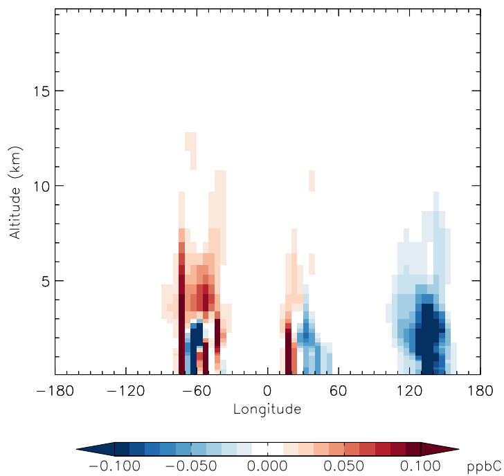
v11-01f-merra2-Run0 - v11-01d-Run1 MEK - Diff along 15S for Jan
