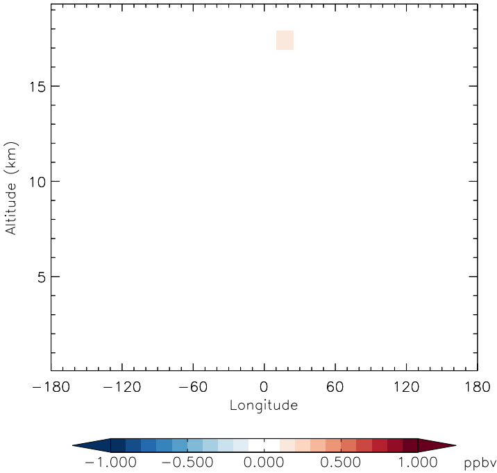
v11-01f-merra2-Run0 - v11-01f-geosfp-Run0 NO2 - Diff along 15S for Jan
