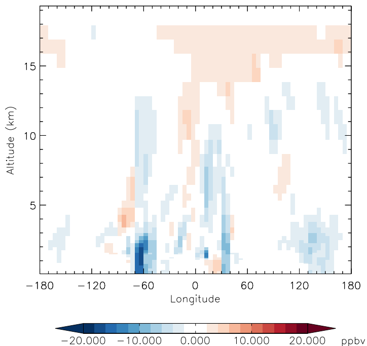
v11-01f-merra2-Run0 - v11-01f-geosfp-Run0 CO - Diff along 15S for Jan
