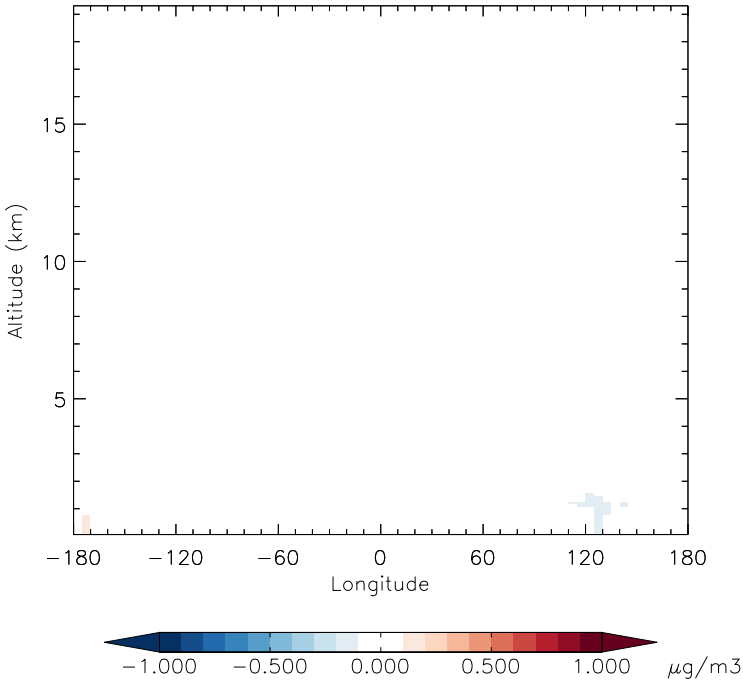
v11-01f-merra2-Run0 - v11-01d-Run1 SALA - Diff along 15S for Jan
