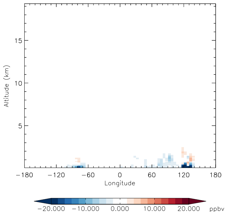
v11-01f-merra2-Run0 - v11-01f-geosfp-Run0 CO - Diff along 42N for Jan
