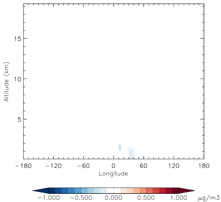
v11-01f-merra2-Run0 - v11-01d-Run1 OCPI - Diff along 15S for Jan
