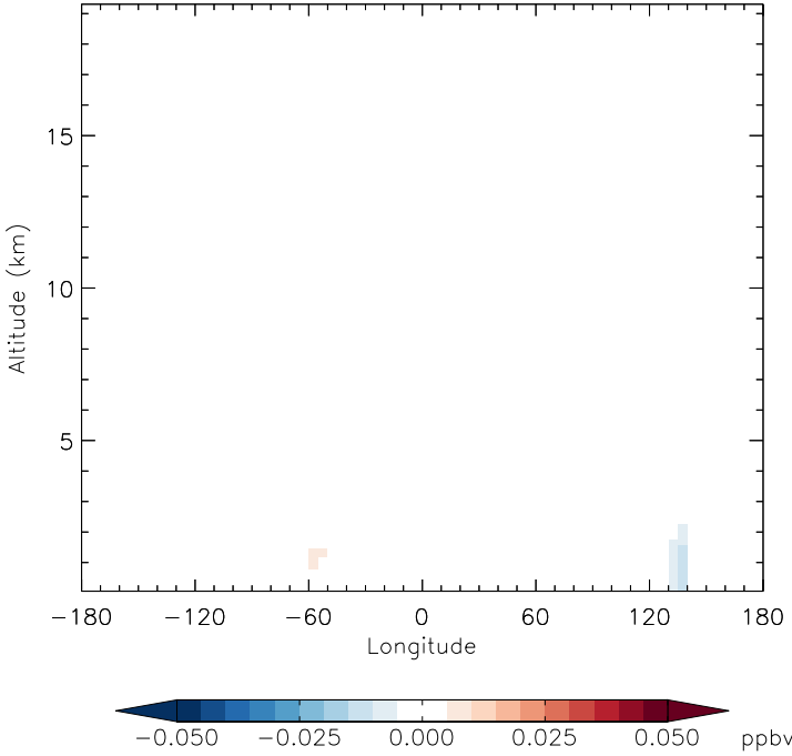
v11-01f-merra2-Run0 - v11-01d-Run1 RCHO - Diff along 15S for Jan
