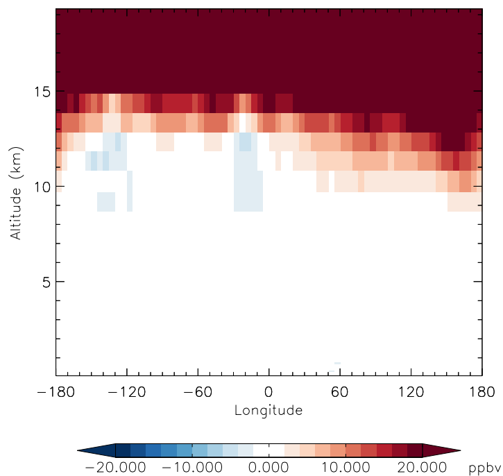
v11-01f-merra2-Run0 - v11-01d-Run1 O3 - Diff along 42N for Jan
