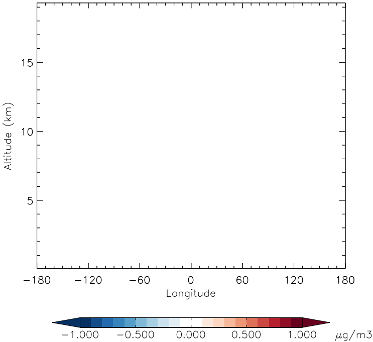
v11-01f-merra2-Run0 - v11-01d-Run1 BCPO - Diff along 15S for Jan
