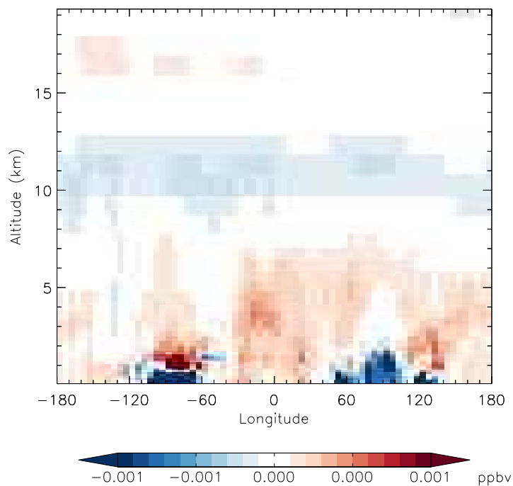
v11-01f-merra2-Run0 - v11-01d-Run1 PPN - Diff along 42N for Jan
