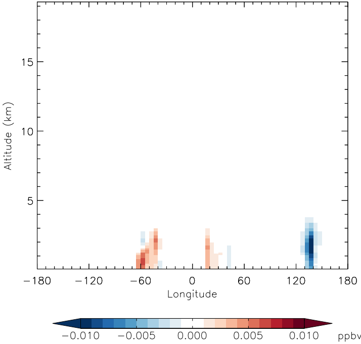
v11-01f-merra2-Run0 - v11-01d-Run1 MMN - Diff along 15S for Jan
