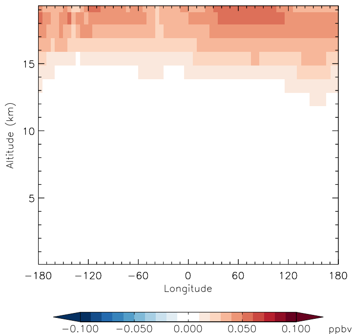
v11-01f-merra2-Run0 - v11-01f-geosfp-Run0 CINO3 - Diff along 42N for Jan
