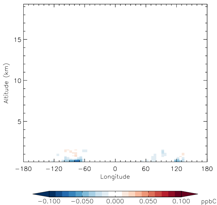
v11-01f-merra2-Run0 - v11-01f-geosfp-Run0 MEK - Diff along 42N for Jan
