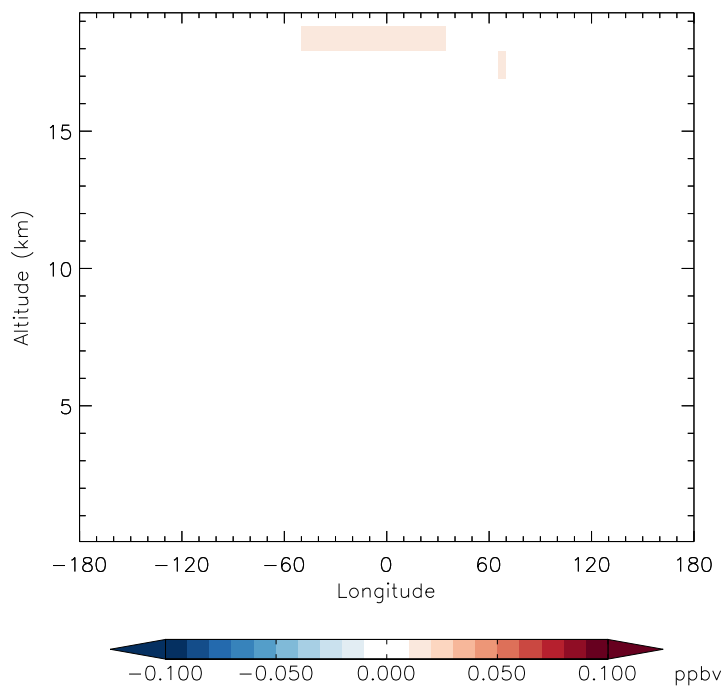
v11-01f-merra2-Run0 - v11-01d-Run1 OCS - Diff along 15S for Jan
