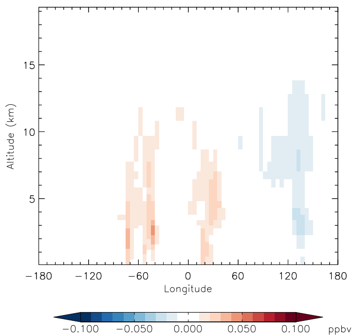
v11-01f-merra2-Run0 - v11-01d-Run1 PAN - Diff along 15S for Jan
