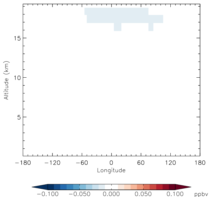
v11-01f-merra2-Run0 - v11-01f-geosfp-Run0 MPN - Diff along 15S for Jan
