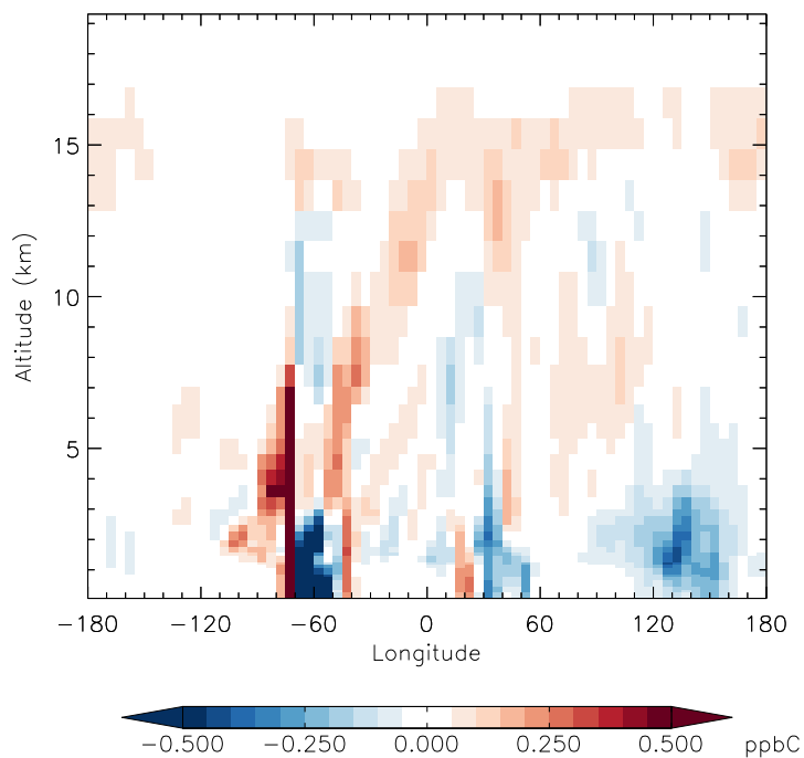
v11-01f-merra2-Run0 - v11-01d-Run1 ACET - Diff along 15S for Jan
