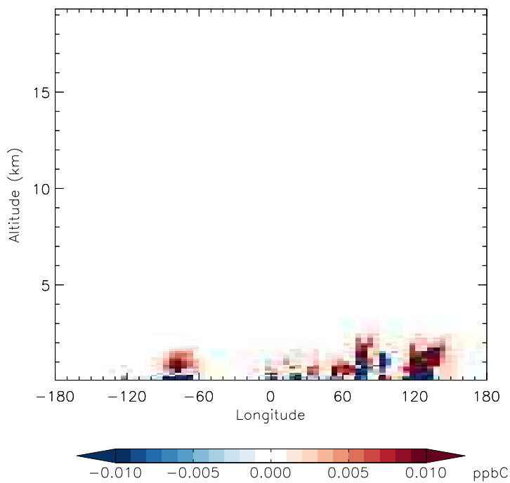
v11-01f-merra2-Run0 - v11-01d-Run1 PRPE - Diff along 42N for Jan
