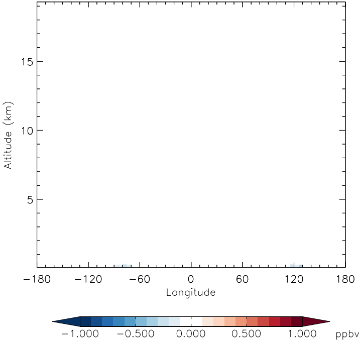
v11-01f-merra2-Run0 - v11-01d-Run1 NO - Diff along 42N for Jan
