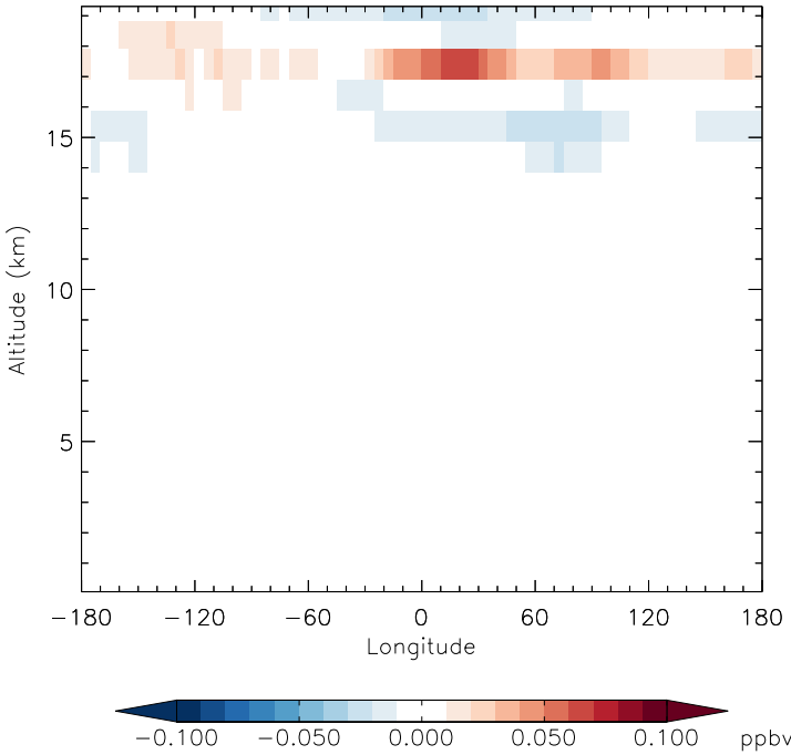
v11-01f-merra2-Run0 - v11-01f-geosfp-Run0 HCl - Diff along 15S for Jan
