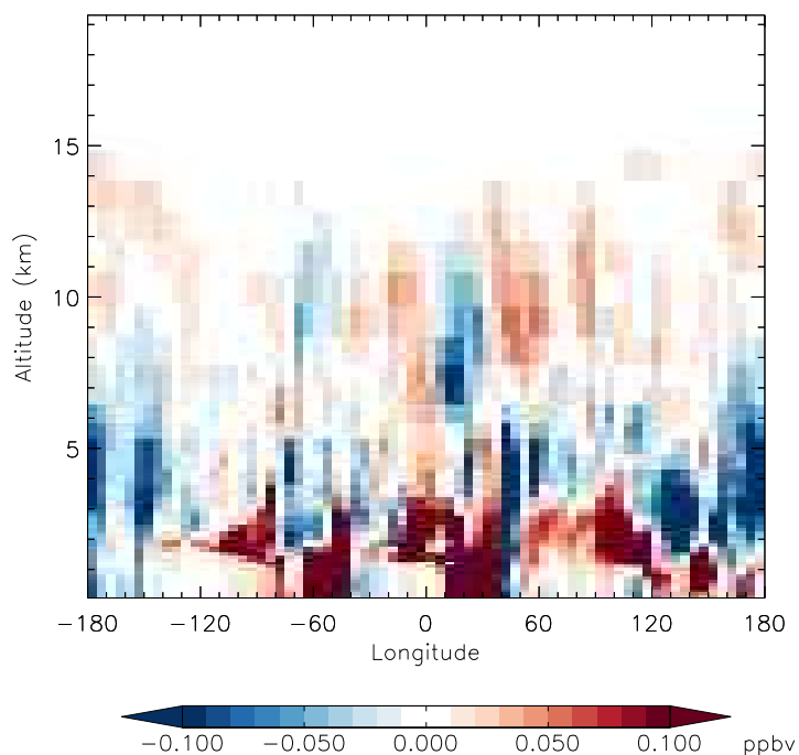
v11-01f-merra2-Run0 - v11-01f-geosfp-Run0 H2O2 - Diff along 15S for Jan
