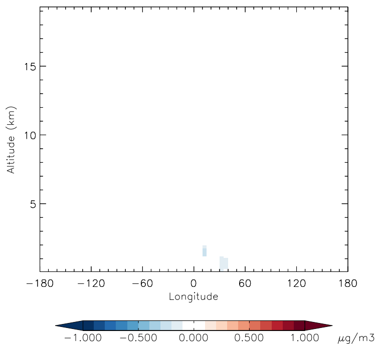
v11-01f-merra2-Run0 - v11-01f-geosfp-Run0 OCPI - Diff along 15S for Jan
