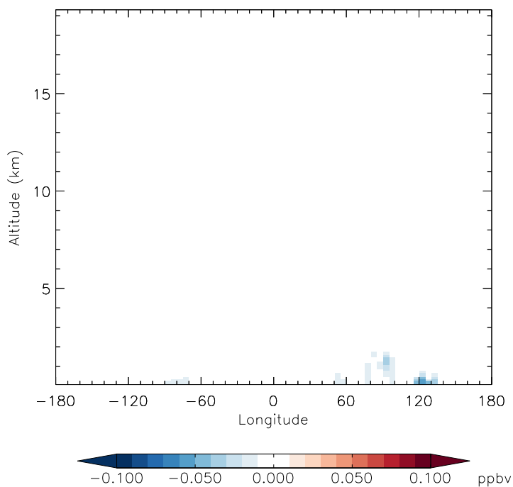
v11-01f-merra2-Run0 - v11-01f-geosfp-Run0 PAN - Diff along 42N for Jan
