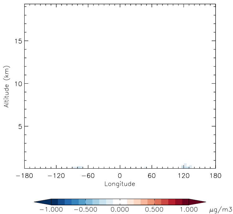
v11-01f-merra2-Run0 - v11-01d-Run1 OCPI - Diff along 42N for Jan
