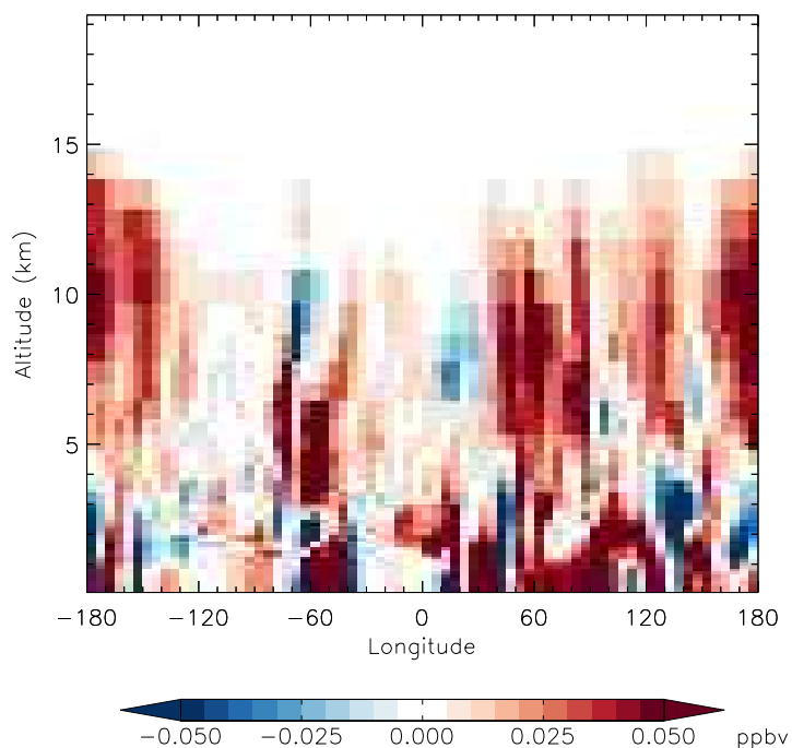
v11-01f-merra2-Run0 - v11-01f-geosfp-Run0 MP - Diff along 15S for Jan
