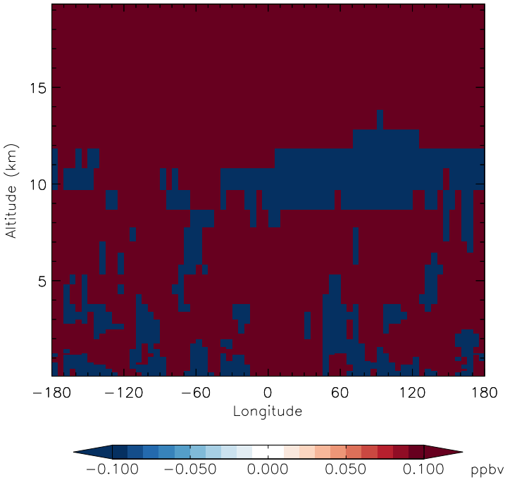
v11-01f-merra2-Run0 - v11-01f-geosfp-Run0 H2O - Diff along 42N for Jan
