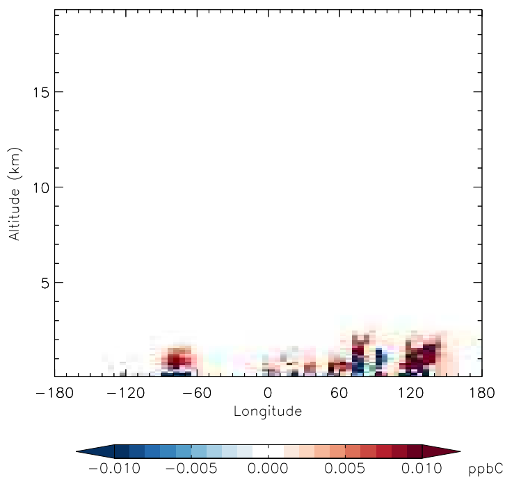
v11-01f-merra2-Run0 - v11-01f-geosfp-Run0 PRPE - Diff along 42N for Jan
