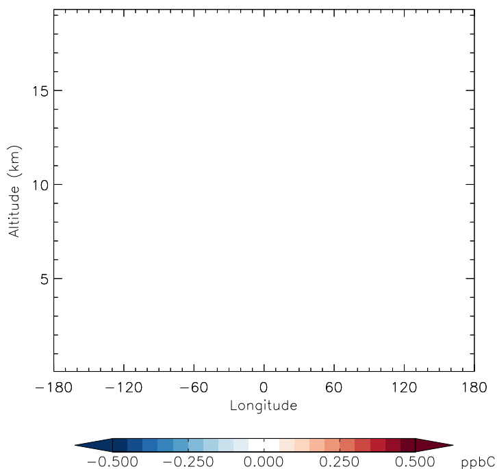
v11-01f-merra2-Run0 - v11-01f-geosfp-Run0 ISOP - Diff along 42N for Jan
