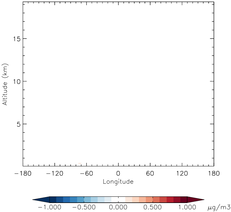
v11-01f-merra2-Run0 - v11-01f-geosfp-Run0 SO2 - Diff along 15S for Jan
