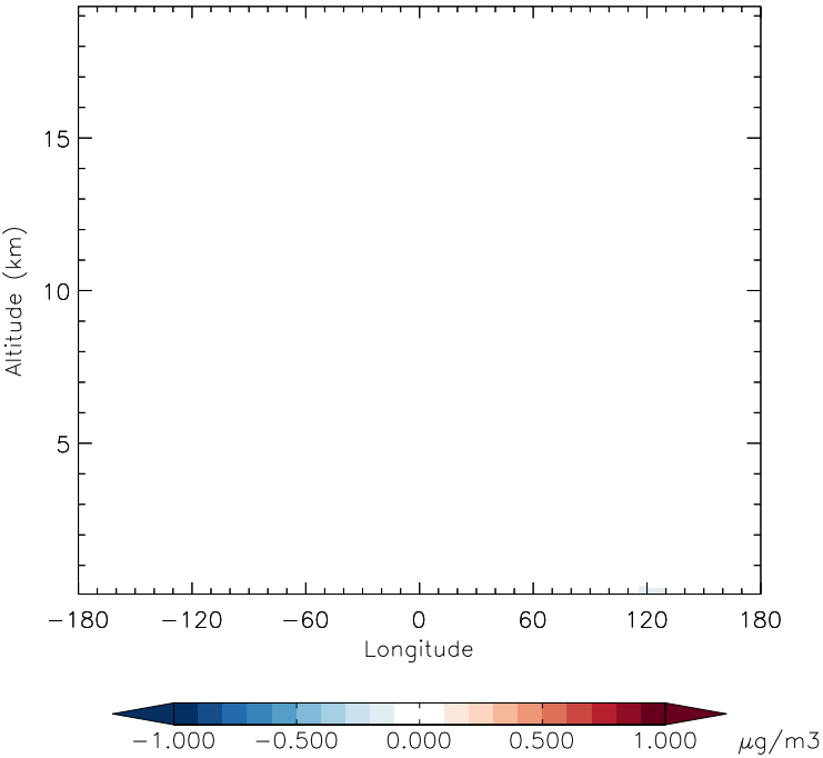
v11-01f-merra2-Run0 - v11-01f-geosfp-Run0 BCPI - Diff along 42N for Jan
