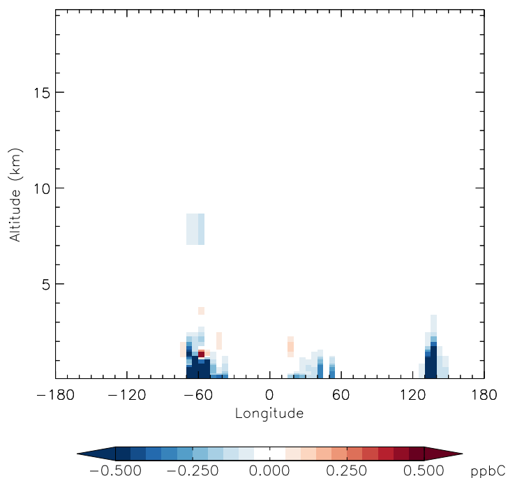
v11-01f-merra2-Run0 - v11-01f-geosfp-Run0 ISOP - Diff along 15S for Jan
