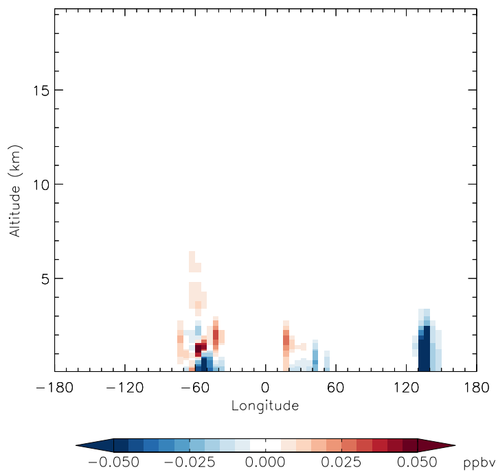
v11-01f-merra2-Run0 - v11-01d-Run1 MVK - Diff along 15S for Jan
