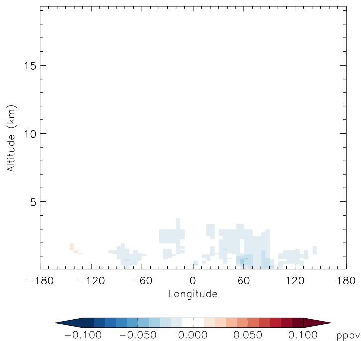
v11-01f-merra2-Run0 - v11-01d-Run1 H2O2 - Diff along 42N for Jan
