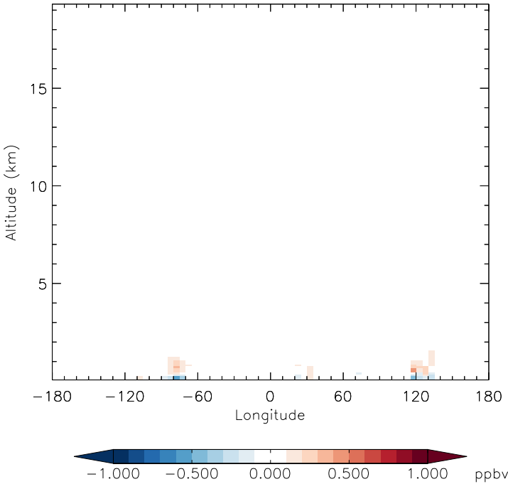
v11-01f-merra2-Run0 - v11-01d-Run1 NO2 - Diff along 42N for Jan
