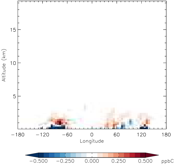
v11-01f-merra2-Run0 - v11-01d-Run1 ALK4 - Diff along 42N for Jan
