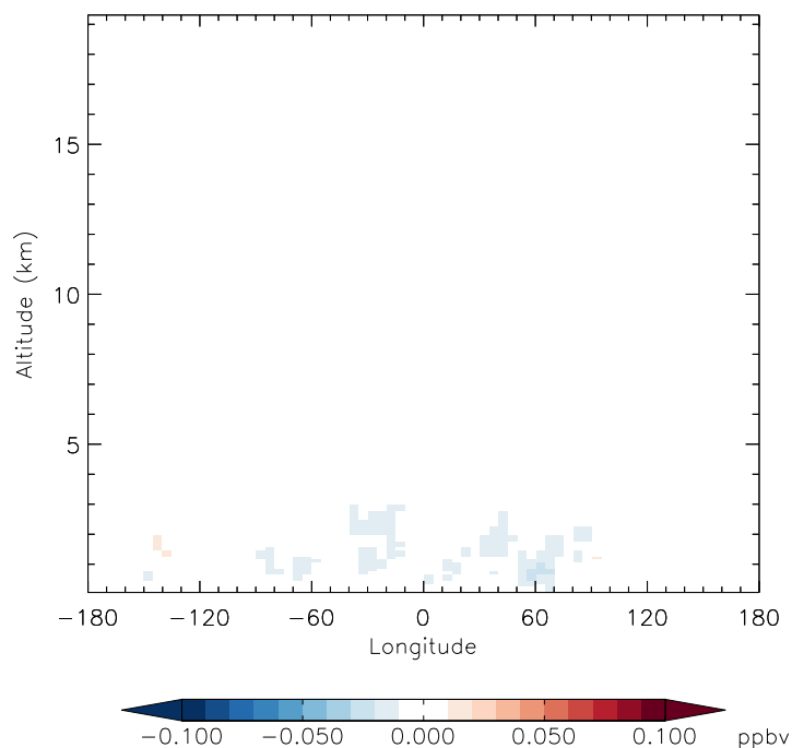
v11-01f-merra2-Run0 - v11-01f-geosfp-Run0 H2O2 - Diff along 42N for Jan
