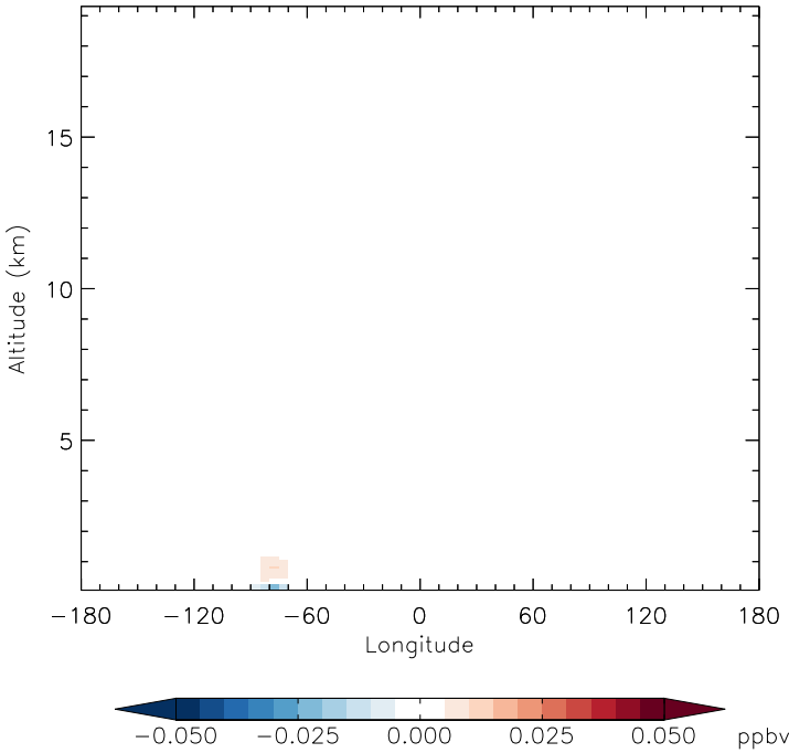
v11-01f-merra2-Run0 - v11-01f-geosfp-Run0 RCHO - Diff along 42N for Jan
