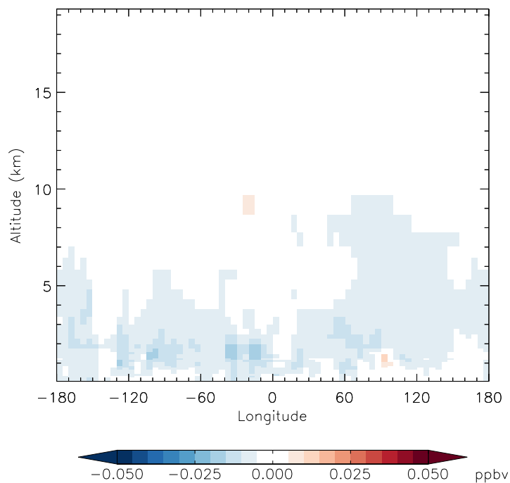
v11-01f-merra2-Run0 - v11-01d-Run1 MP - Diff along 42N for Jan
