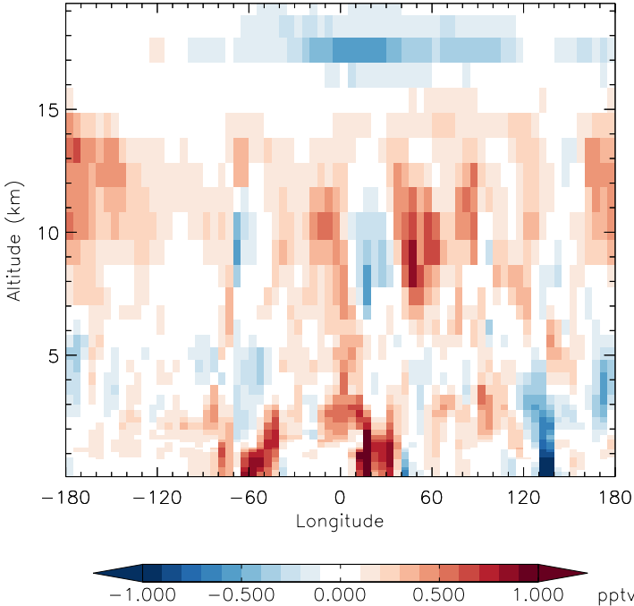
v11-01f-merra2-Run0 - v11-01d-Run1 HO2 - Diff along 15S for Jan
