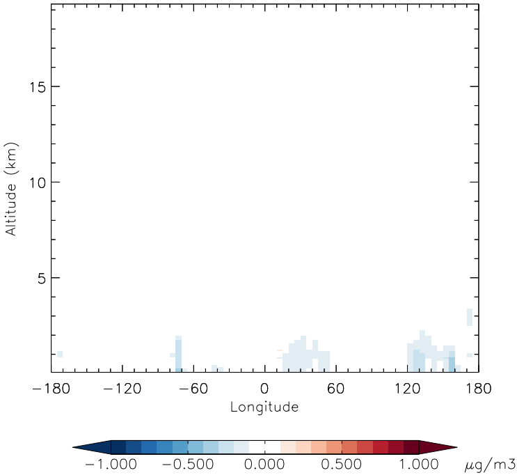
v11-01f-merra2-Run0 - v11-01f-geosfp-Run0 S04 - Diff along 15S for Jan
