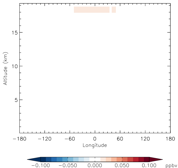
v11-01f-merra2-Run0 - v11-01f-geosfp-Run0 OCS - Diff along 15S for Jan
