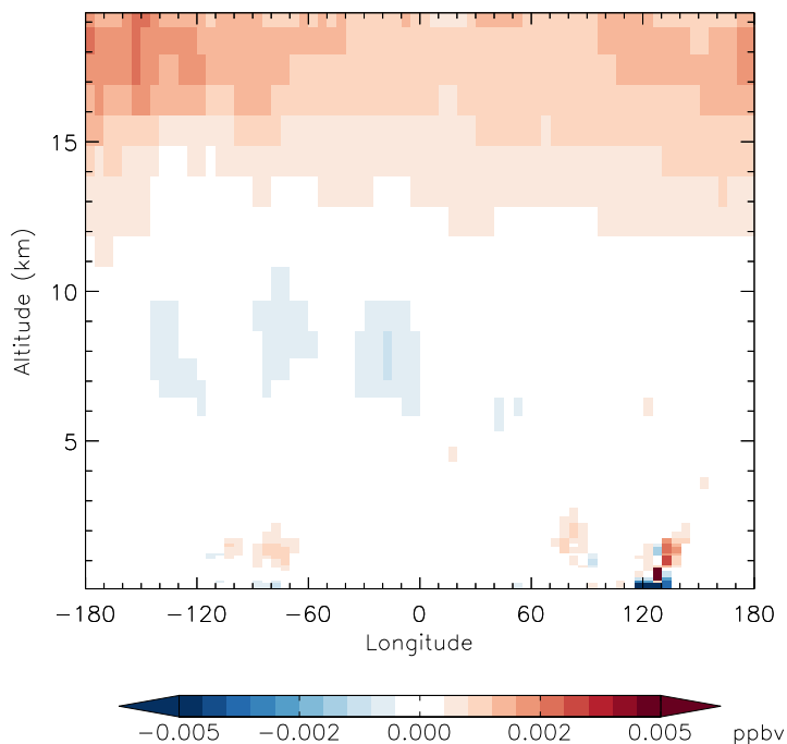
v11-01f-merra2-Run0 - v11-01f-geosfp-Run0 HNO 4 - Diff along 42N for Jan
