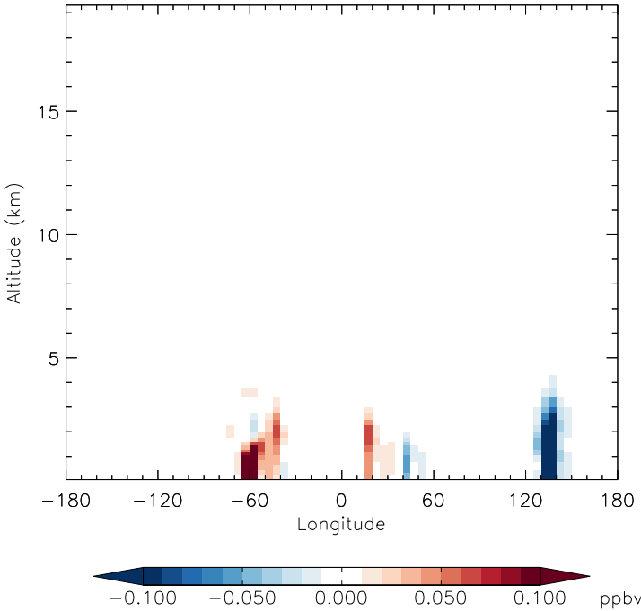
v11-01f-merra2-Run0 - v11-01d-Run1 GLYC - Diff along 15S for Jan
