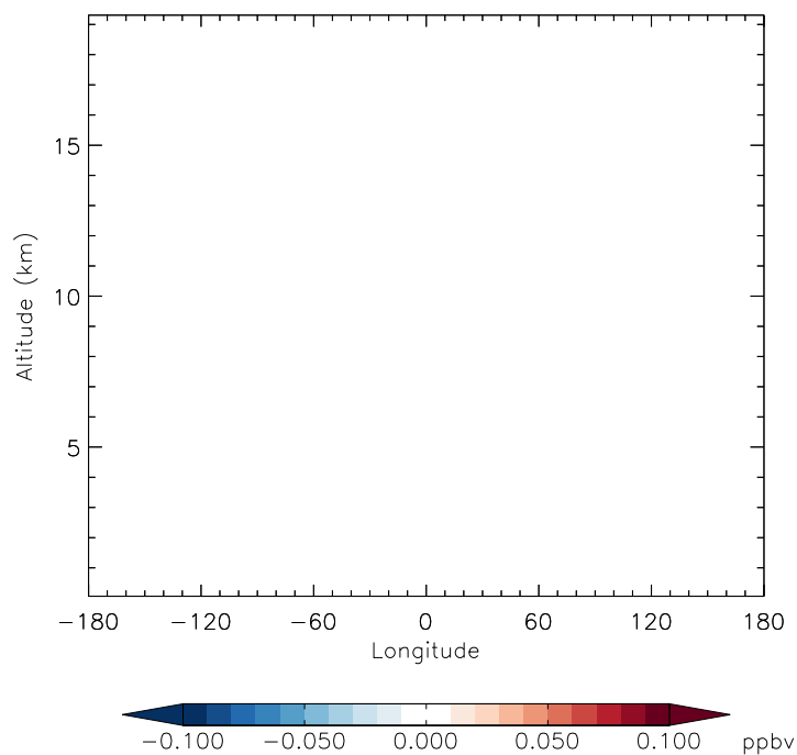
v11-01f-merra2-Run0 - v11-01f-geosfp-Run0 OCIO - Diff along 42N for Jan
