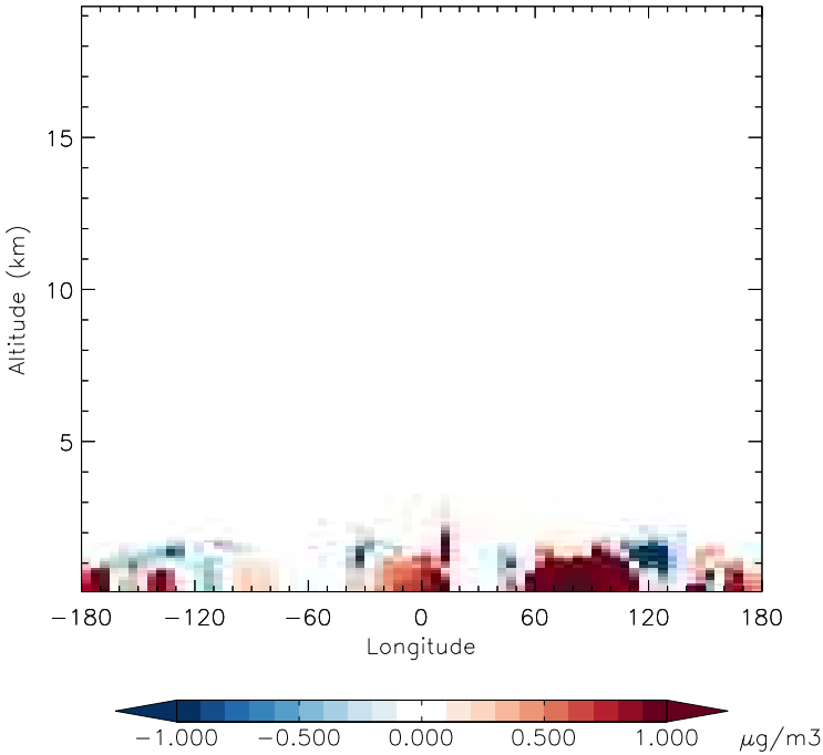
v11-01f-merra2-Run0 - v11-01f-geosfp-Run0 SALC - Diff along 15S for Jan
