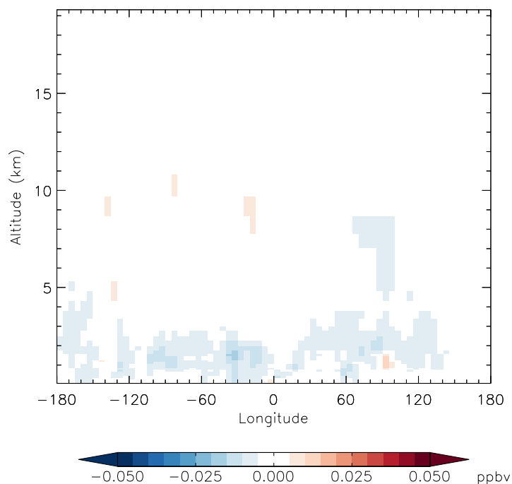
v11-01f-merra2-Run0 - v11-01f-geosfp-Run0 MP - Diff along 42N for Jan
