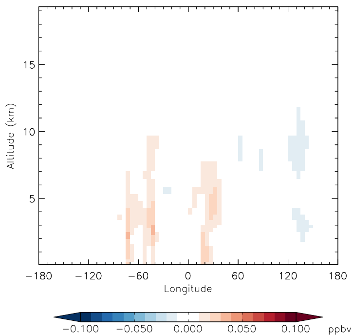
v11-01f-merra2-Run0 - v11-01f-geosfp-Run0 PAN - Diff along 15S for Jan
