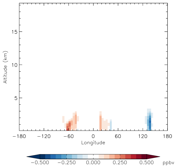
v11-01f-merra2-Run0 - v11-01d-Run1 CH 2 O - Diff along 15S for Jan
