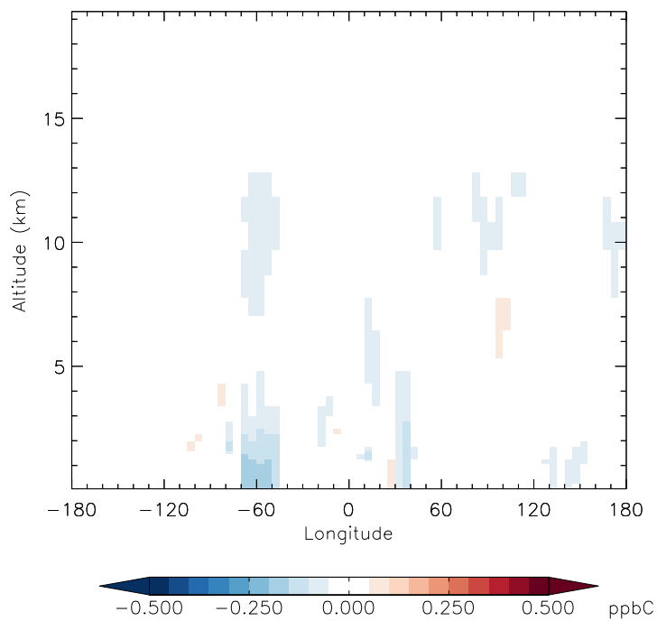
v11-01f-merra2-Run0 - v11-01d-Run1 C2H6 - Diff along 15S for Jan
