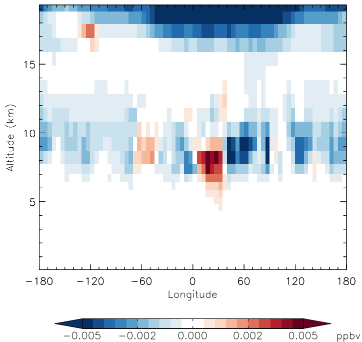
v11-01f-merra2-Run0 - v11-01d-Run1 HNO 4 - Diff along 15S for Jan
