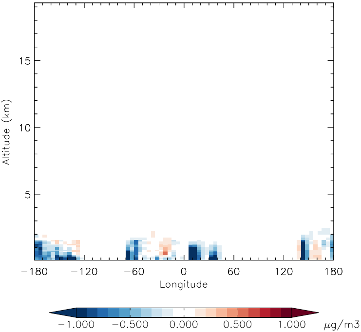
v11-01f-merra2-Run0 - v11-01f-geosfp-Run0 SALC - Diff along 42N for Jan
