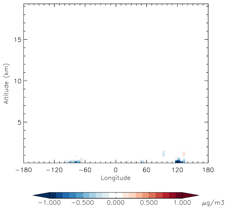
v11-01f-merra2-Run0 - v11-01d-Run1 NH4 - Diff along 42N for Jan
