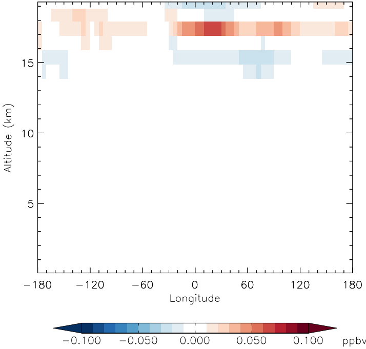
v11-01f-merra2-Run0 - v11-01d-Run1 HCl - Diff along 15S for Jan
