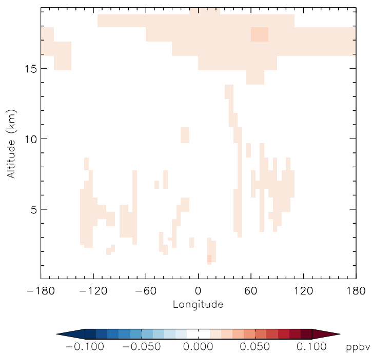
v11-01f-merra2-Run0 - v11-01d-Run1 CH3Cl - Diff along 15S for Jan
