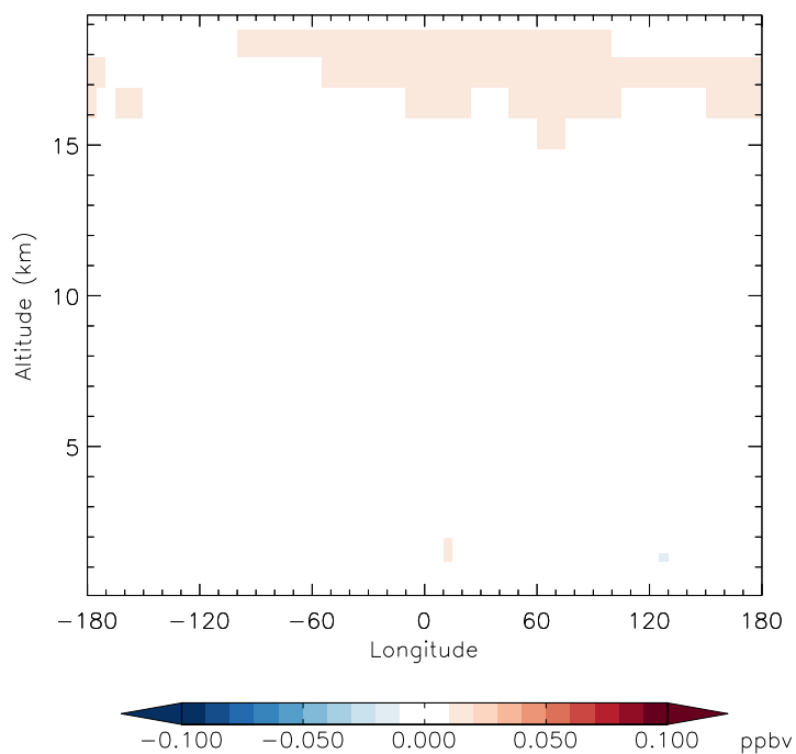
v11-01f-merra2-Run0 - v11-01f-geosfp-Run0 CH3Cl - Diff along 15S for Jan
