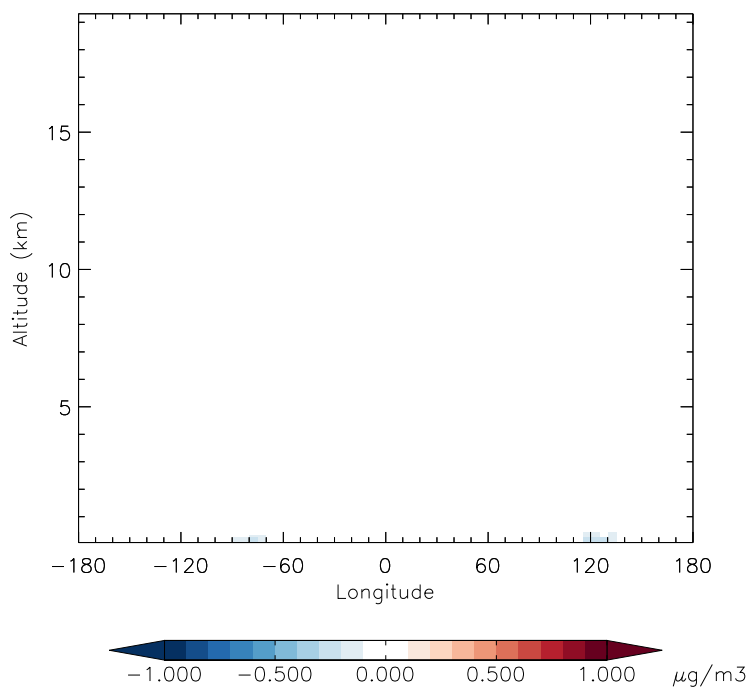
v11-01f-merra2-Run0 - v11-01f-geosfp-Run0 OCPI - Diff along 42N for Jan
