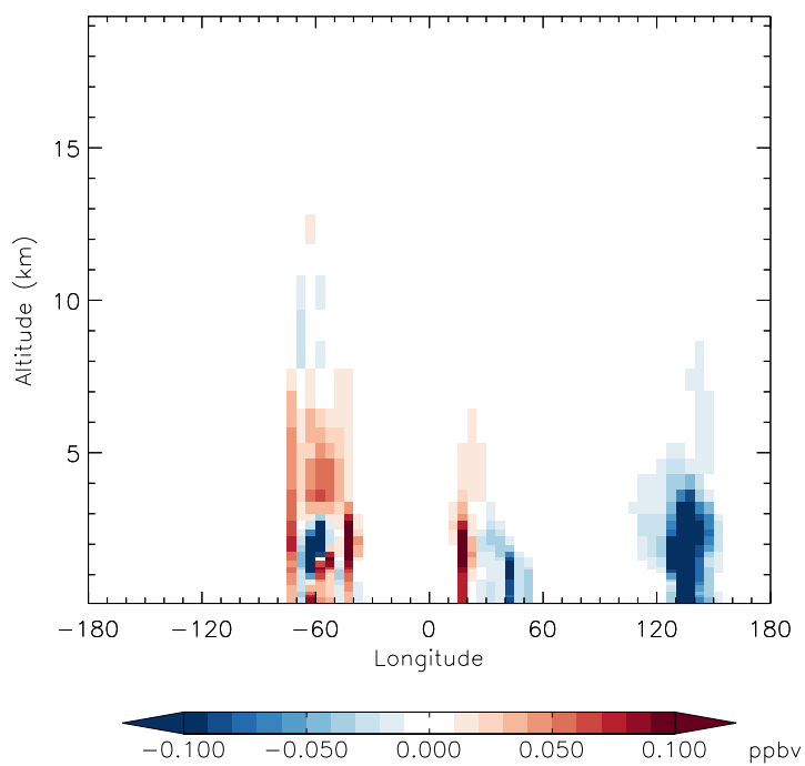
v11-01f-merra2-Run0 - v11-01d-Run1 HAC - Diff along 15S for Jan
