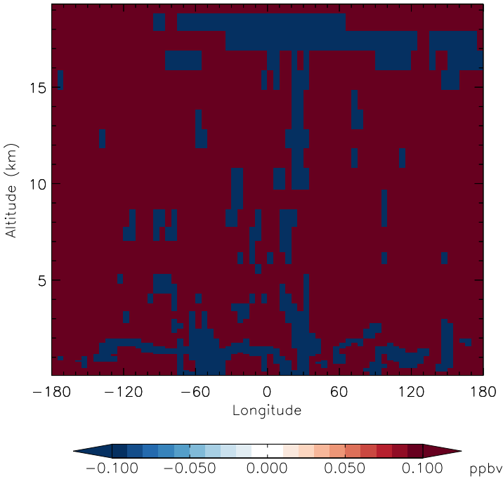
v11-01f-merra2-Run0 - v11-01f-geosfp-Run0 H2O - Diff along 15S for Jan
