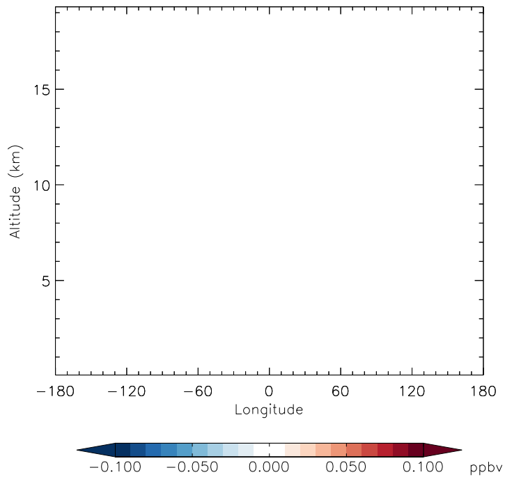
v11-01f-merra2-Run0 - v11-01d-Run1 ClO 0 - Diff along 15S for Jan
