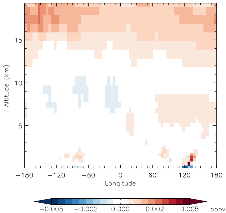
v11-01f-merra2-Run0 - v11-01d-Run1 HNO 4 - Diff along 42N for Jan
