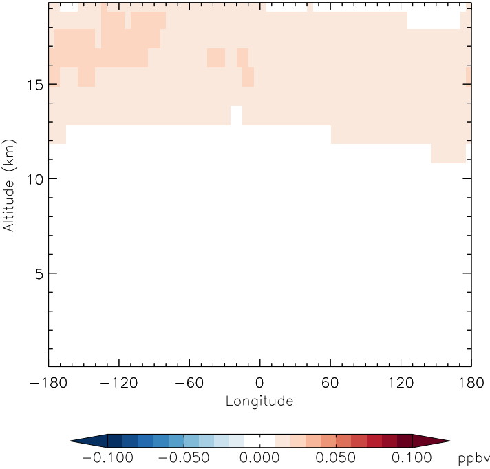
v11-01f-merra2-Run0 - v11-01d-Run1 HCl - Diff along 42N for Jan
