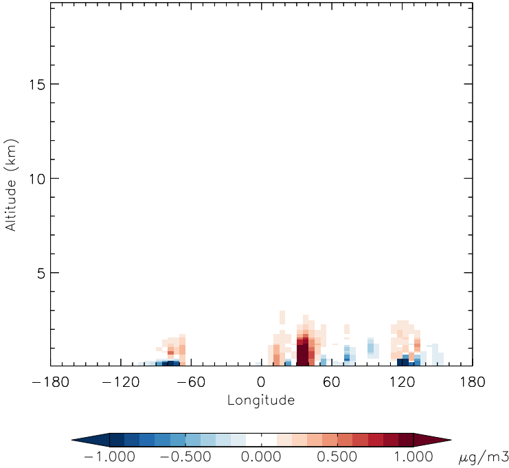
v11-01f-merra2-Run0 - v11-01d-Run1 SO2 - Diff along 42N for Jan
