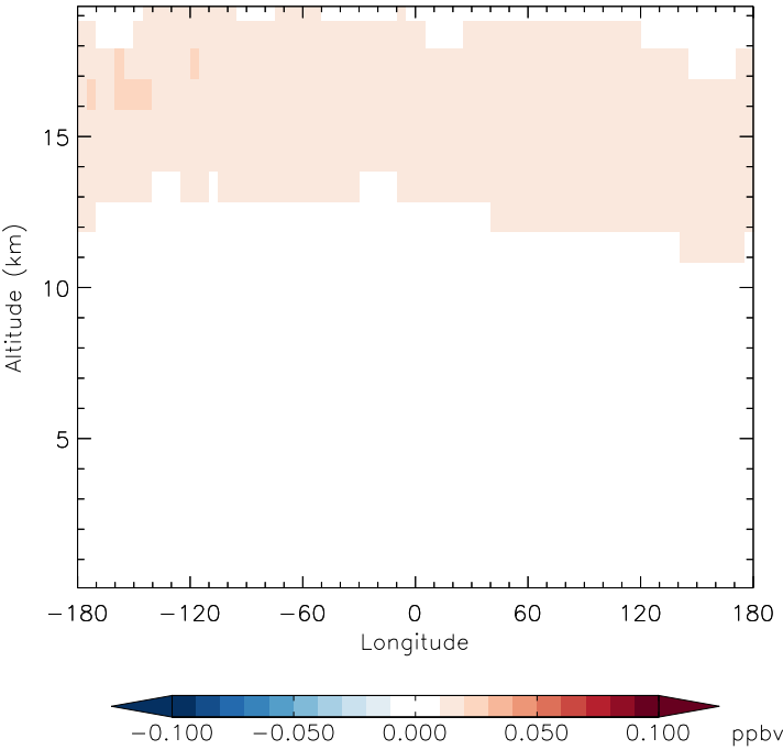
v11-01f-merra2-Run0 - v11-01f-geosfp-Run0 HCl - Diff along 42N for Jan
