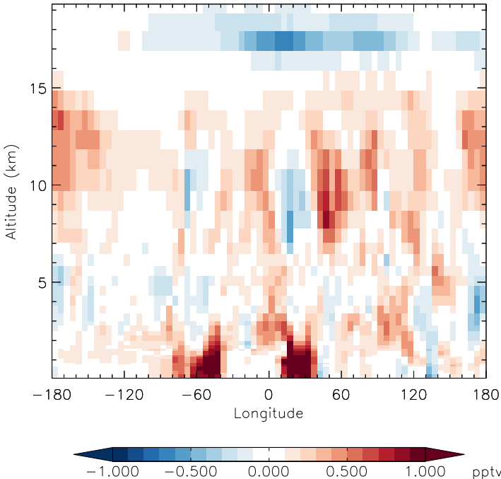
v11-01f-merra2-Run0 - v11-01f-geosfp-Run0 HO2 - Diff along 15S for Jan
