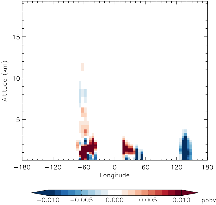
v11-01f-merra2-Run0 - v11-01d-Run1 RIP - Diff along 15S for Jan
