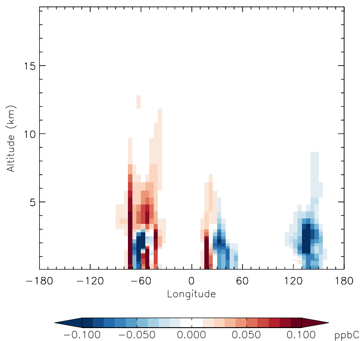
v11-01f-merra2-Run0 - v11-01f-geosfp-Run0 MEK - Diff along 15S for Jan
