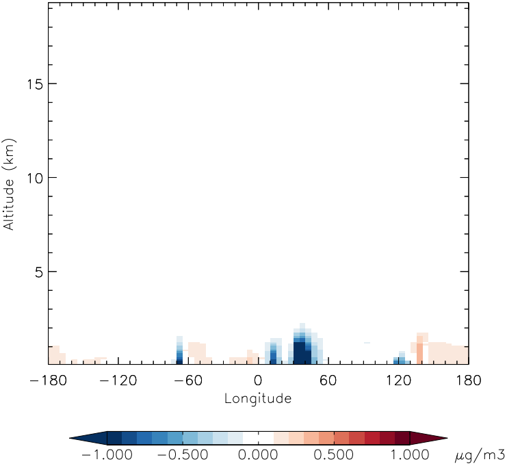
v11-01f-merra2-Run0 - v11-01d-Run1 S04 - Diff along 42N for Jan
