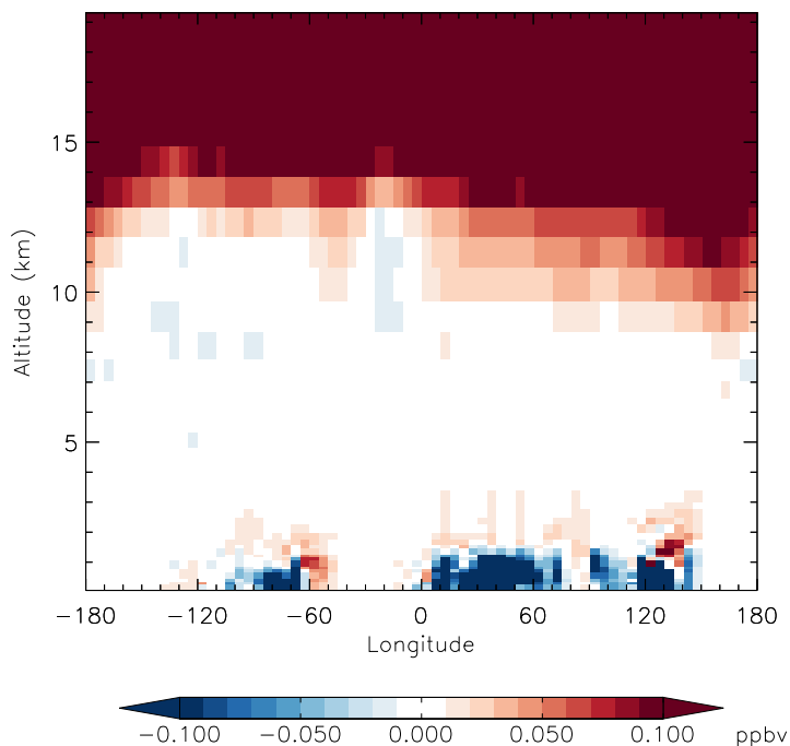
v11-01f-merra2-Run0 - v11-01f-geosfp-Run0 HNO 3 - Diff along 42N for Jan
