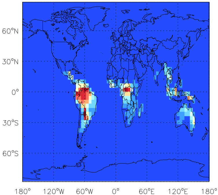
ACET from MONOT emissions for Jan
