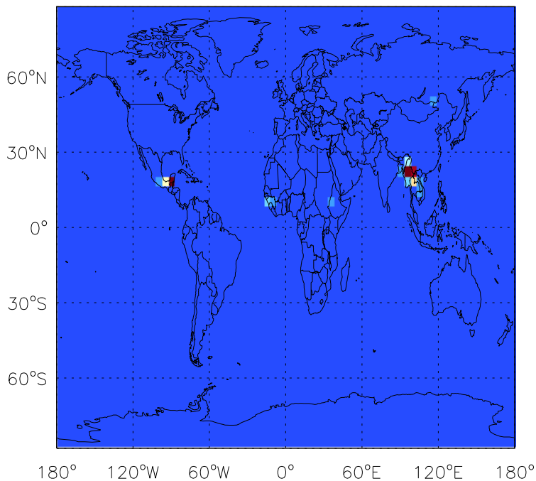
C3H8 biomass emissions for Apr
