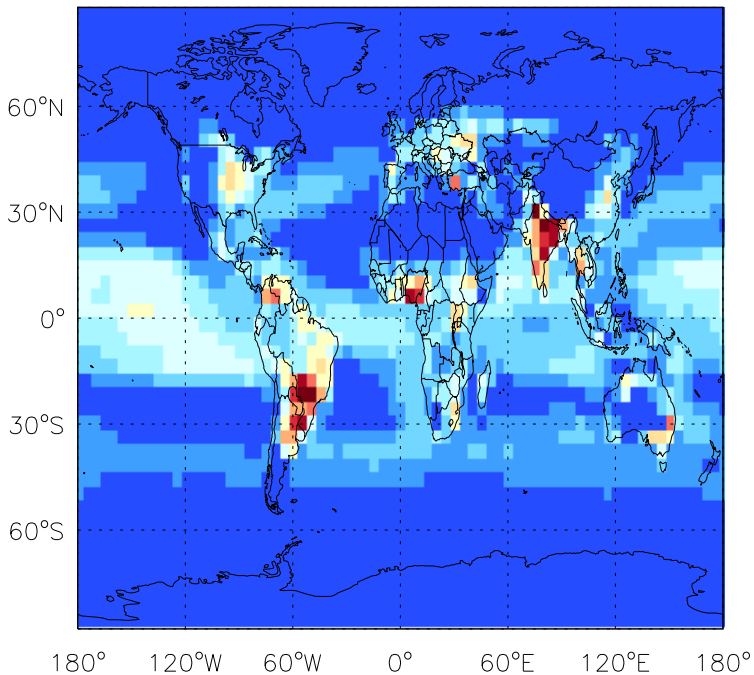
NH3 natural src emissions for Jan
