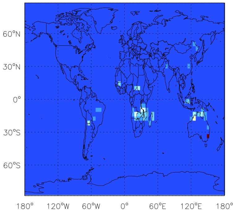
NH 3 biomass emissions for Oct
