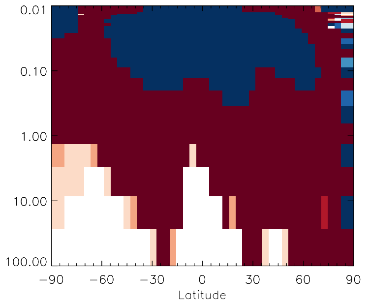
v11-01g-Run0 / v11-01f-geosfp-Run0 ISOP - Strat zonal mean % diff for Apr
