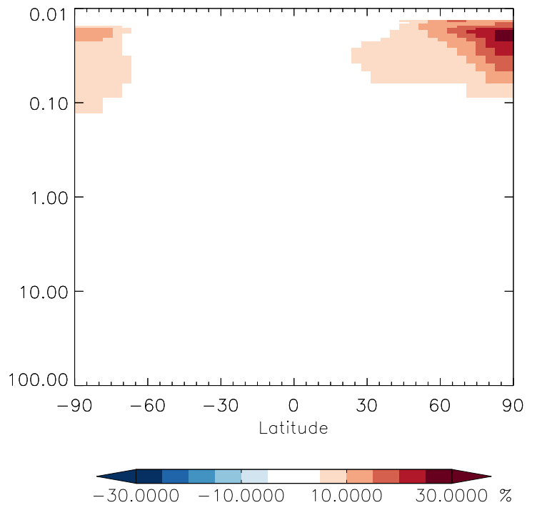
v11-01g-Run0 / v11-01f-geosfp-Run0 H2O2 - Strat zonal mean % diff for Apr
