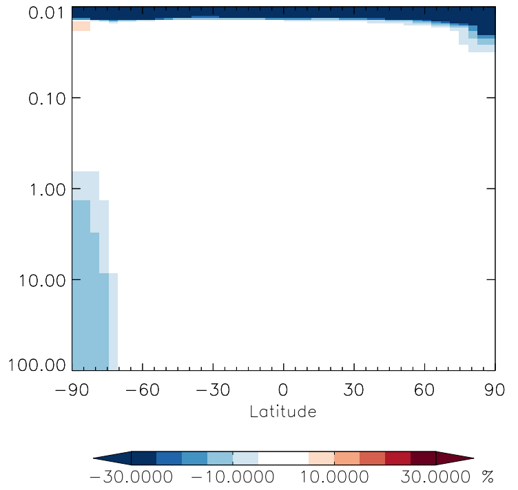
v11-01g-Run0 / v11-01d-Run1 NO 3 - Strat zonal mean % diff for Apr
