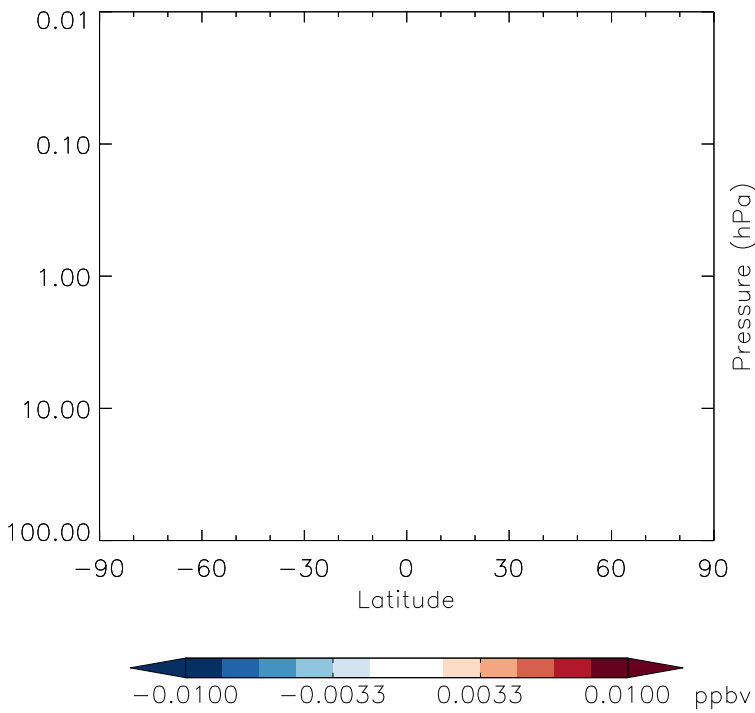
v11-01g-Run0 - v11-01f-geosfp-Run0 MACRN - Strat zonal mean abs diff for Apr
