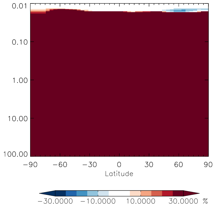
v11-01g-Run0 / v11-01f-geosfp-Run0 MVKN - Strat zonal mean % diff for Apr
