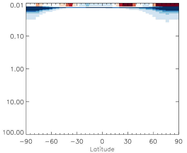
v11-01g-Run0 / v11-01d-Run1 N2O5 - Strat zonal mean % diff for Apr
