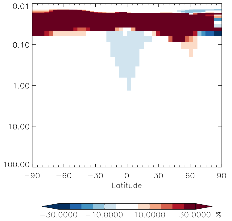
v11-01g-Run0 / v11-01f-geosfp-Run0 IEPOX - Strat zonal mean % diff for Apr
