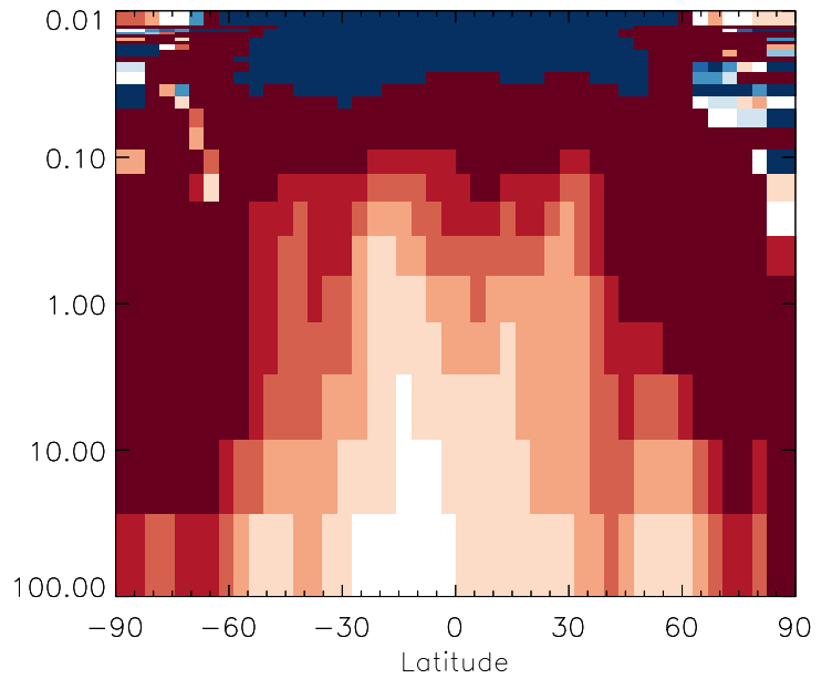
v11-01g-Run0 / v11-01d-Run1 OCPO - Strat zonal mean % diff for Apr
