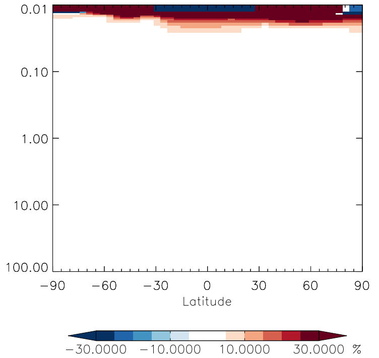
v11-01g-Run0 / v11-01d-Run1 H2402 - Strat zonal mean % diff for Apr
