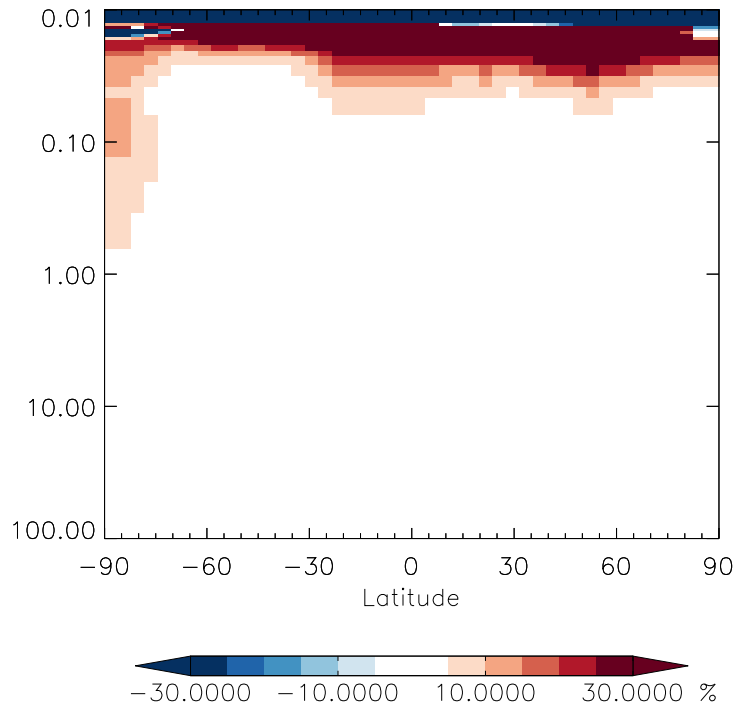
v11-01g-Run0 / v11-01d-Run1 CHBr3 - Strat zonal mean % diff for Apr
