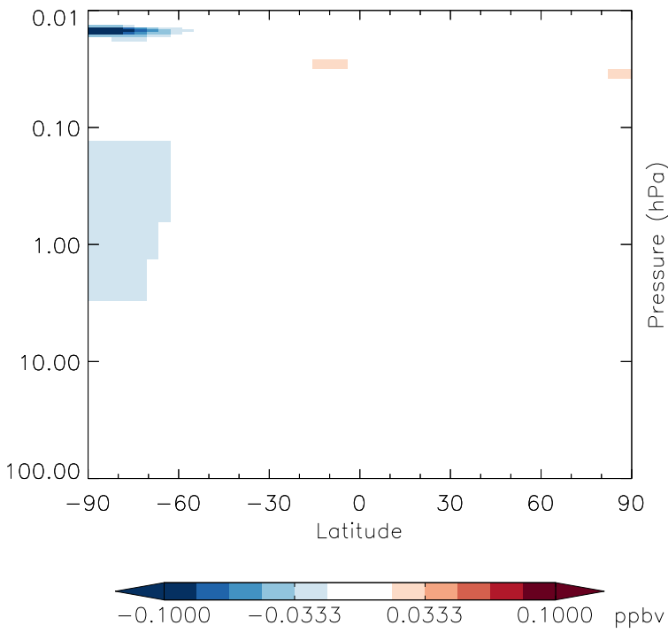
v11-01g-Run0 - v11-01f-geosfp-Run0 ClNO 3 - Strat zonal mean abs diff for Apr
