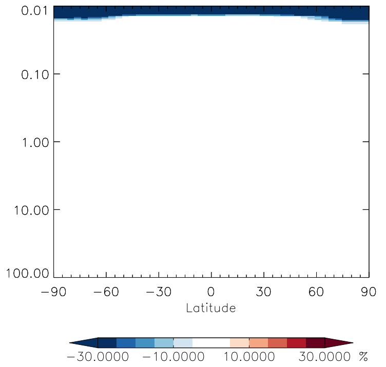
v11-01g-Run0 / v11-01f-geosfp-Run0 ClNO 3 - Strat zonal mean % diff for Apr
