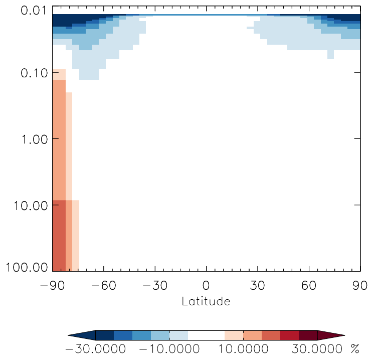
v11-01g-Run0 / v11-01f-geosfp-Run0 HN02 - Strat zonal mean % diff for Apr
