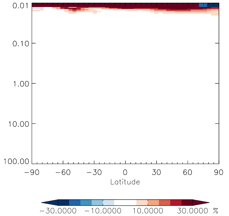
v11-01g-Run0 / v11-01d-Run1 CH 3 CCl 3 - Strat zonal mean % diff for Apr
