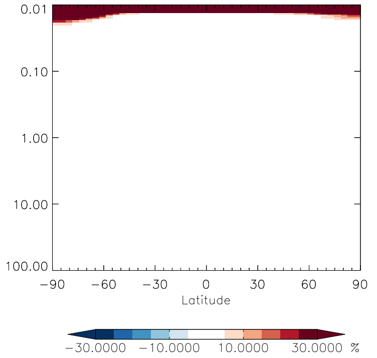
v11-01g-Run0 / v11-01f-geosfp-Run0 N2O - Strat zonal mean % diff for Apr
