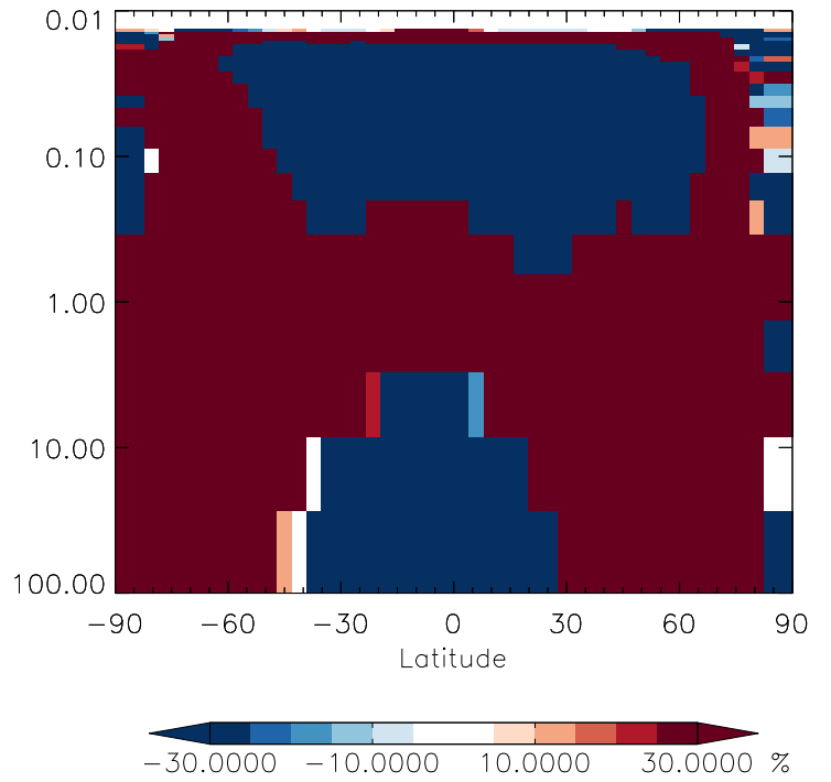
v11-01g-Run0 / v11-01d-Run1 ISOPND - Strat zonal mean % diff for Apr
