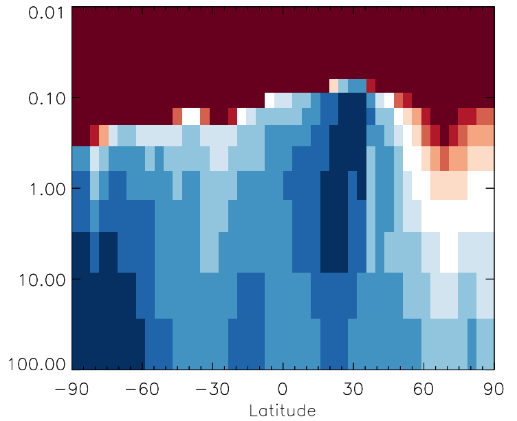
v11-01g-Run0 / v11-01d-Run1 DST4 - Strat zonal mean % diff for Apr
