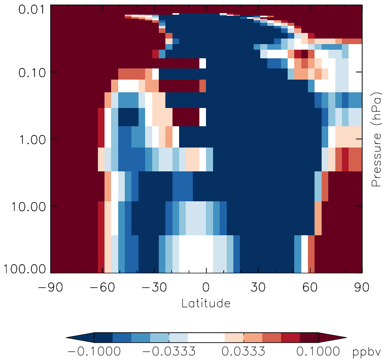
v11-01g-Run0 - v11-01d-Run1 N2O - Strat zonal mean abs diff for Apr
