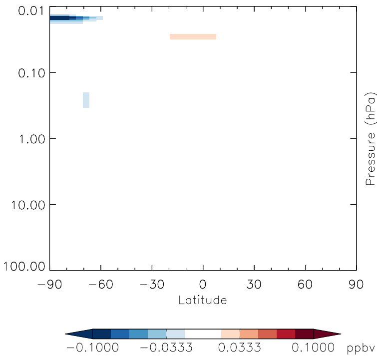
v11-01g-Run0 - v11-01d-Run1 ClNO 3 - Strat zonal mean abs diff for Apr
