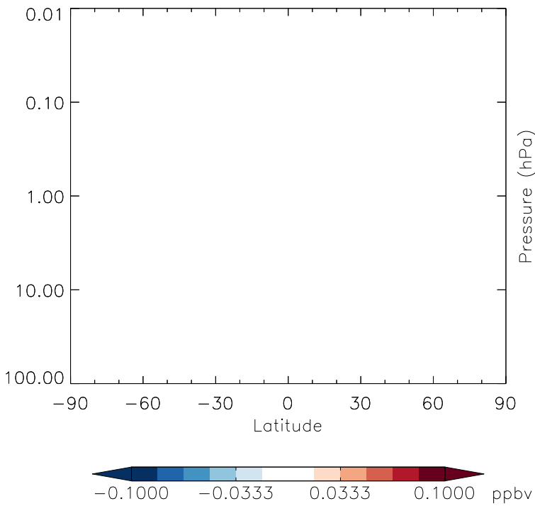
v11-01g-Run0 - v11-01f-geosfp-Run0 CFC11 - Strat zonal mean abs diff for Apr
