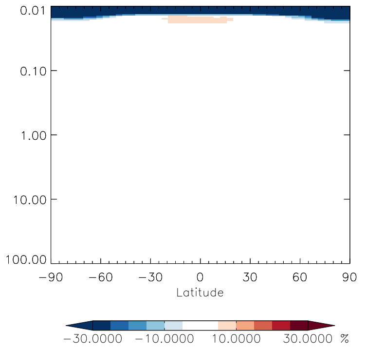
v11-01g-Run0 / v11-01d-Run1 ClNO 3 - Strat zonal mean % diff for Apr
