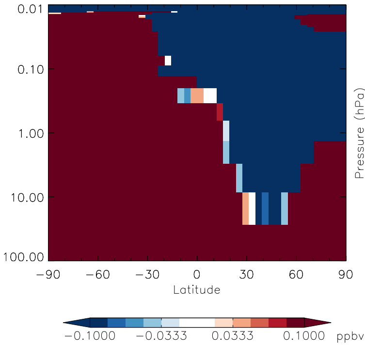
v11-01g-Run0 - v11-01d-Run1 CH4 - Strat zonal mean abs diff for Apr
