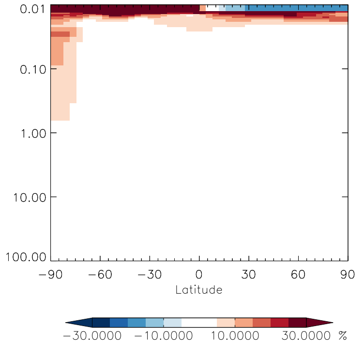
v11-01g-Run0 / v11-01d-Run1 C3H8 - Strat zonal mean % diff for Apr
