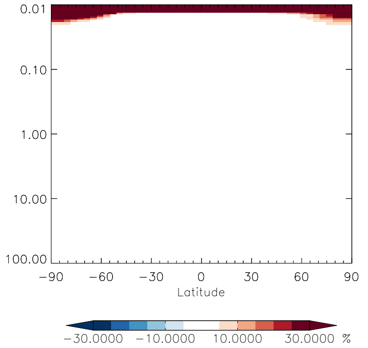
v11-01g-Run0 / v11-01d-Run1 N2O - Strat zonal mean % diff for Apr
