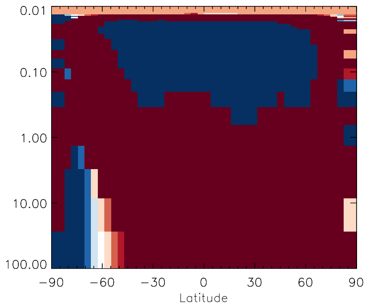
v11-01g-Run0 / v11-01d-Run1 ISOPNB - Strat zonal mean % diff for Apr
