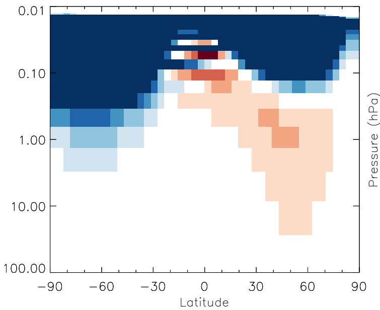
v11-01g-Run0 - v11-01d-Run1 N2O5 - Strat zonal mean abs diff for Apr
