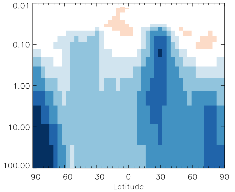
v11-01g-Run0 / v11-01d-Run1 DST3 - Strat zonal mean % diff for Apr
