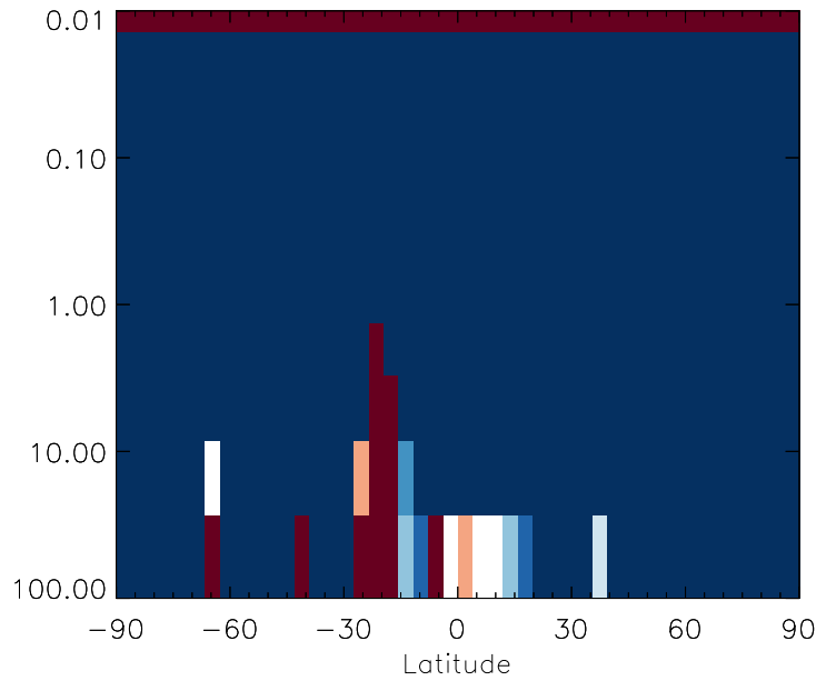
v11-01g-Run0 / v11-01d-Run1 SO4s - Strat zonal mean % diff for Apr
