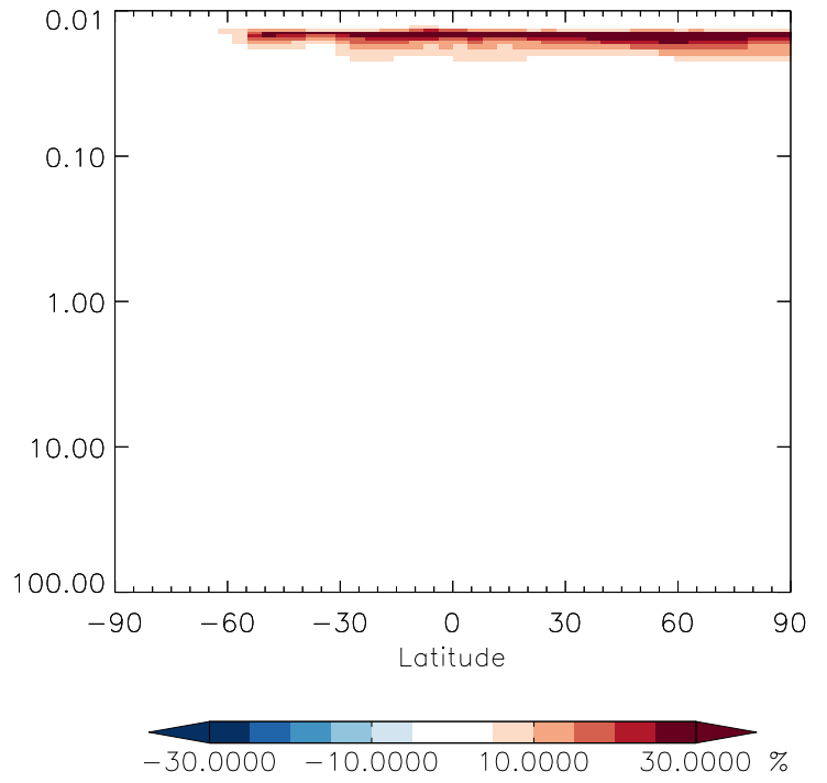
v11-01g-Run0 / v11-01d-Run1 CH3Br - Strat zonal mean % diff for Apr
