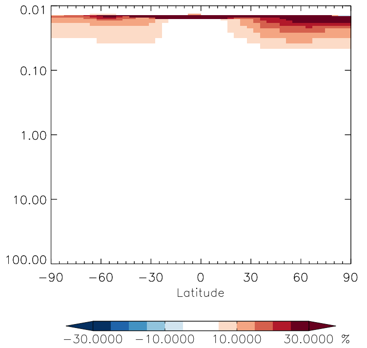
v11-01g-Run0 / v11-01f-geosfp-Run0 CH 2 Br 2 - Strat zonal mean % diff for Apr
