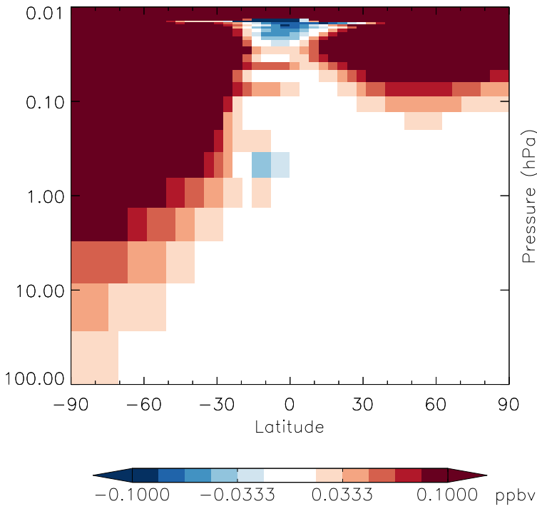
v11-01g-Run0 - v11-01f-geosfp-Run0 N2O - Strat zonal mean abs diff for Apr
