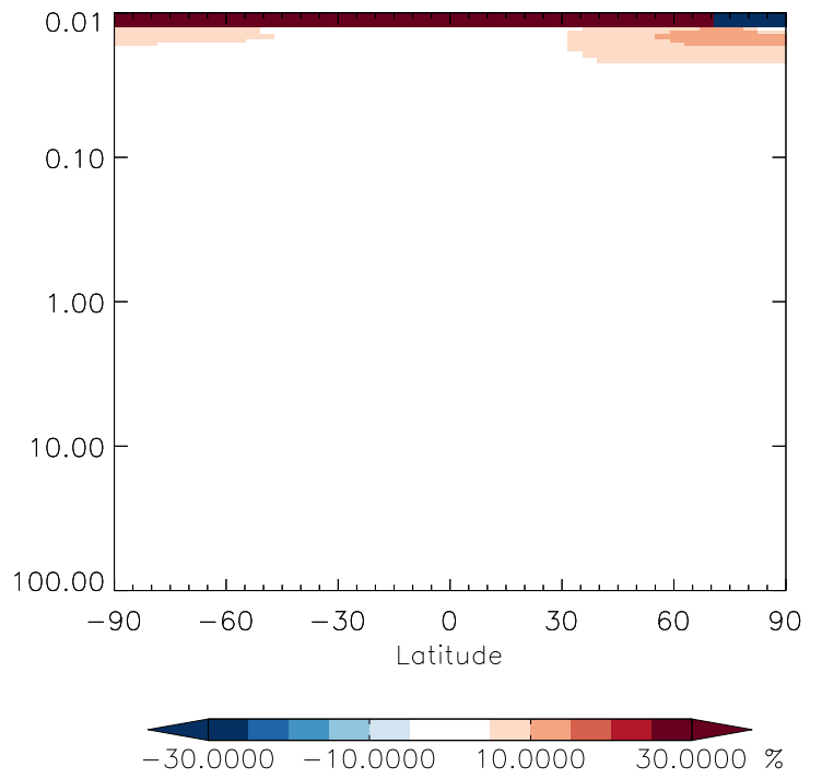
v11-01g-Run0 / v11-01f-geosfp-Run0 CH 3 CCl 3 - Strat zonal mean % diff for Apr
