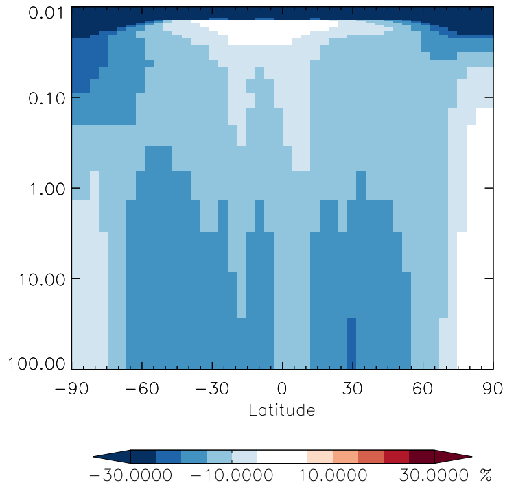
v11-01g-Run0 / v11-01d-Run1 BrNO2 - Strat zonal mean % diff for Apr
