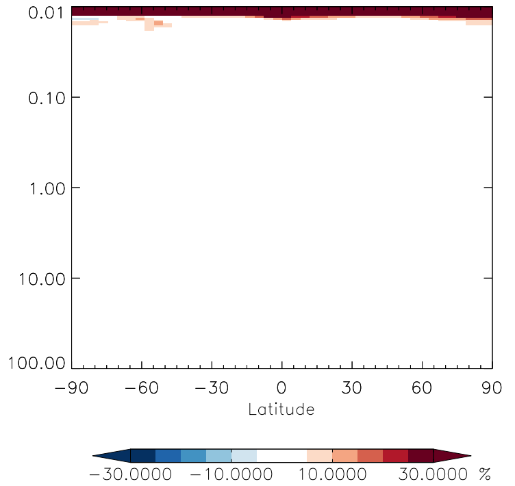
v11-01g-Run0 / v11-01d-Run1 CFC11 - Strat zonal mean % diff for Apr
