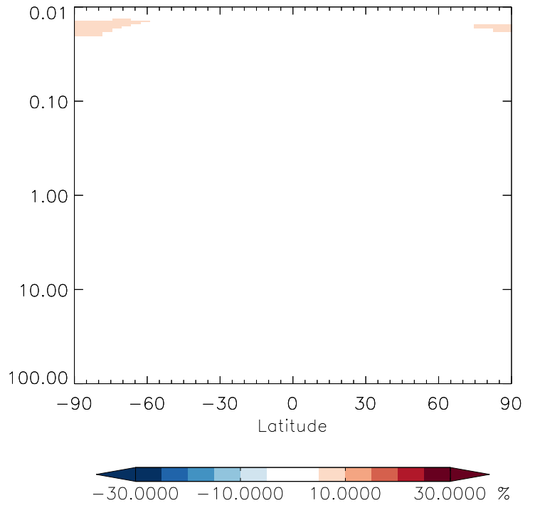
v11-01g-Run0 / v11-01f-geosfp-Run0 O3 - Strat zonal mean % diff for Apr
