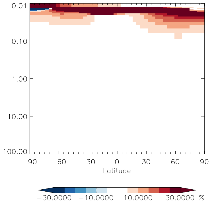
v11-01g-Run0 / v11-01f-geosfp-Run0 CHBr3 - Strat zonal mean % diff for Apr
