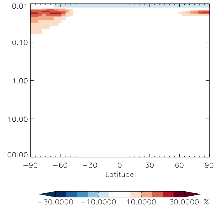
v11-01g-Run0 / v11-01d-Run1 C2H6 - Strat zonal mean % diff for Apr
