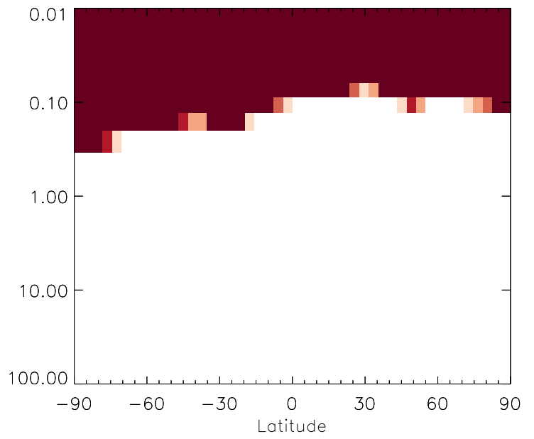
v11-01g-Run0 / v11-01f-geosfp-Run0 DST4 - Strat zonal mean % diff for Apr
