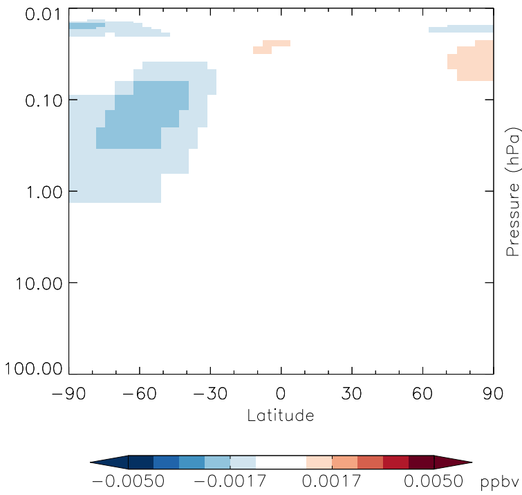
v11-01g-Run0 - v11-01f-geosfp-Run0 HN04 - Strat zonal mean abs diff for Apr
