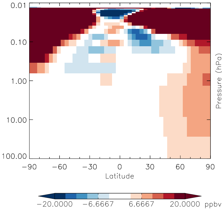
v11-01g-Run0 - v11-01f-geosfp-Run0 O3 - Strat zonal mean abs diff for Apr
