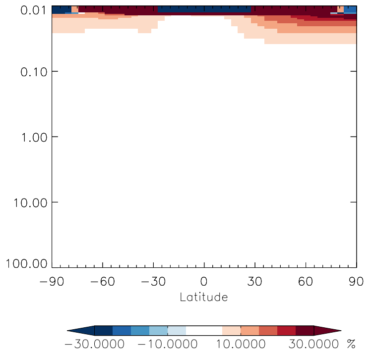
v11-01g-Run0 / v11-01f-geosfp-Run0 H1211 - Strat zonal mean % diff for Apr
