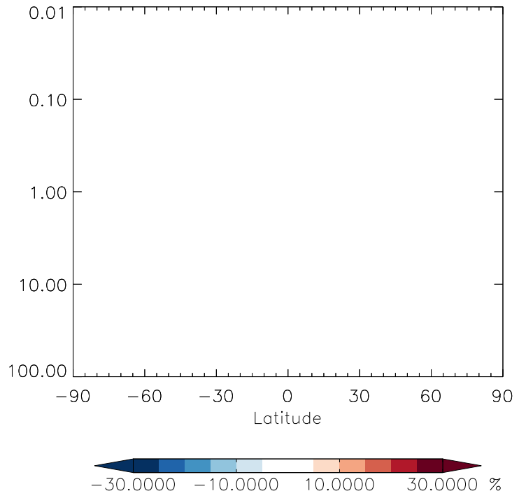
v11-01g-Run0 / v11-01d-Run1 CH4 - Strat zonal mean % diff for Apr
