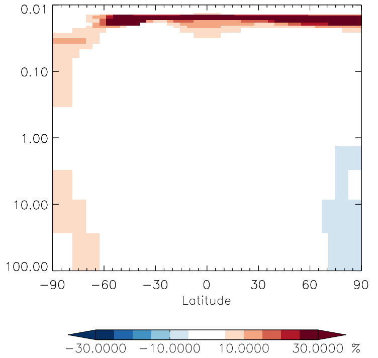
v11-01g-Run0 / v11-01d-Run1 MEK - Strat zonal mean % diff for Apr
