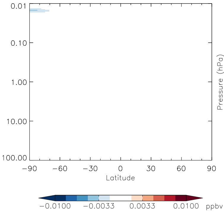
v11-01g-Run0 - v11-01f-geosfp-Run0 BrNO 3 - Strat zonal mean abs diff for Apr
