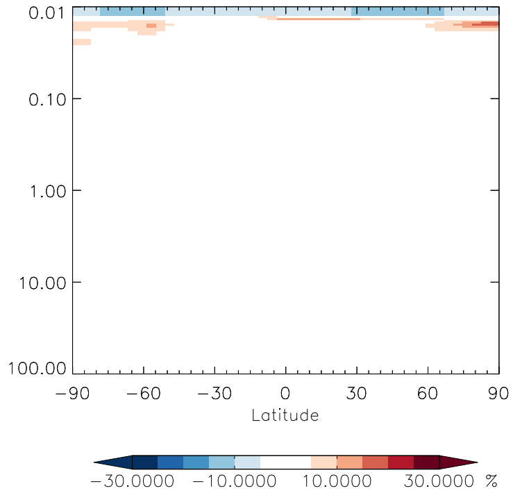
v11-01g-Run0 / v11-01d-Run1 H1301 - Strat zonal mean % diff for Apr
