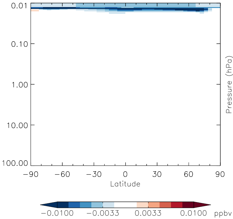
v11-01g-Run0 - v11-01d-Run1 NO 3 - Strat zonal mean abs diff for Apr
