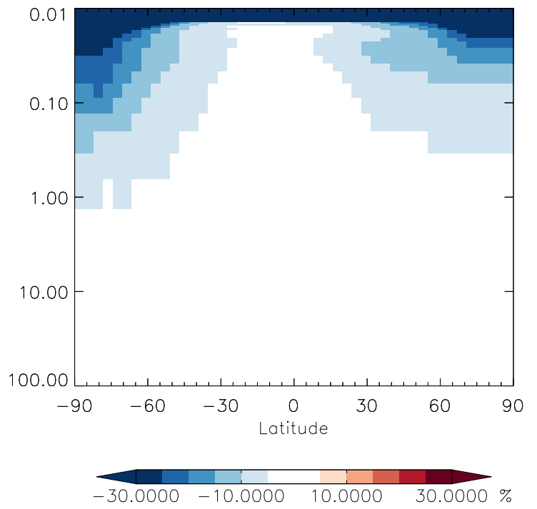
v11-01g-Run0 / v11-01f-geosfp-Run0 BrNO2 - Strat zonal mean % diff for Apr
