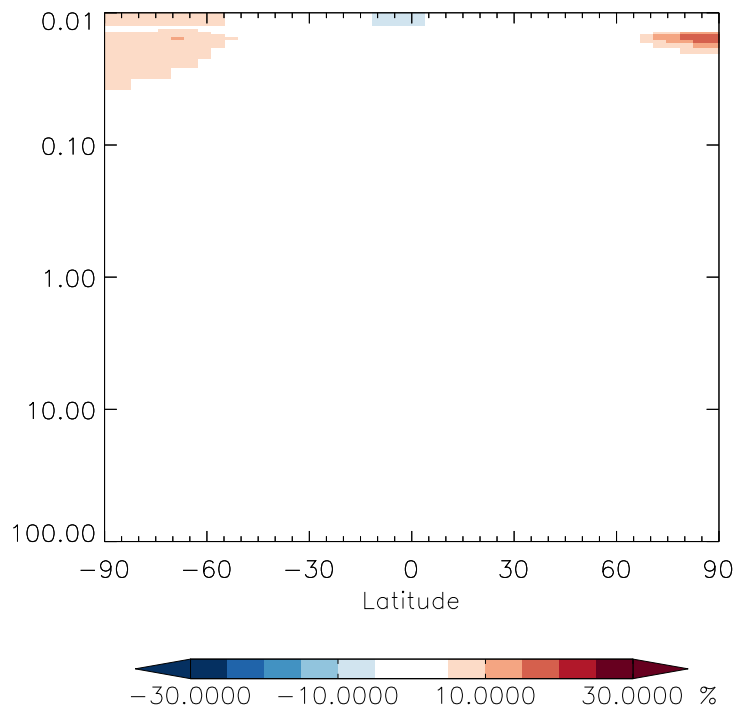
v11-01g-Run0 / v11-01d-Run1 CH3Cl - Strat zonal mean % diff for Apr
