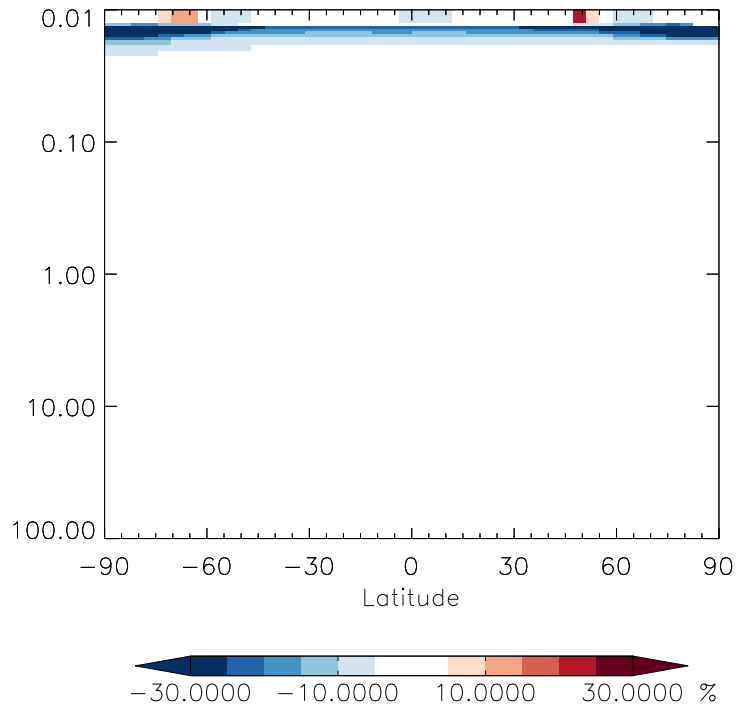
v11-01g-Run0 / v11-01d-Run1 HN04 - Strat zonal mean % diff for Apr
