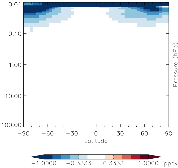
v11-01g-Run0 - v11-01f-geosfp-Run0 NO 2 - Strat zonal mean abs diff for Apr
