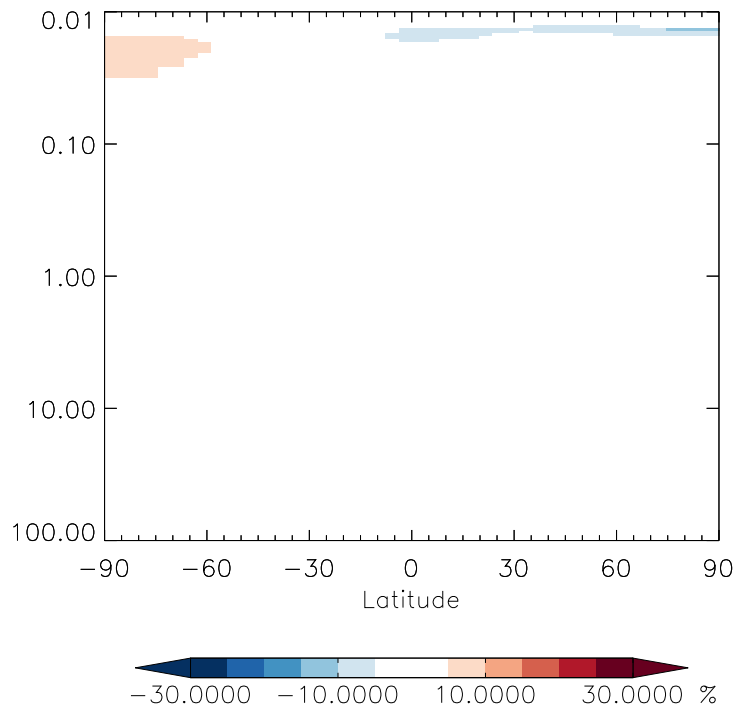
v11-01g-Run0 / v11-01f-geosfp-Run0 C2H6 - Strat zonal mean % diff for Apr
