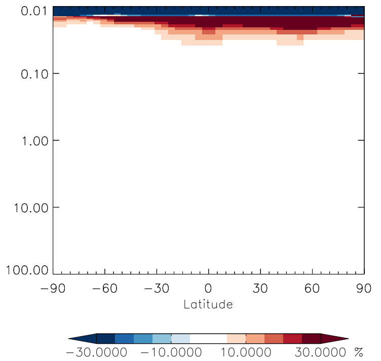
v11-01g-Run0 / v11-01d-Run1 CH 2 Br 2 - Strat zonal mean % diff for Apr
