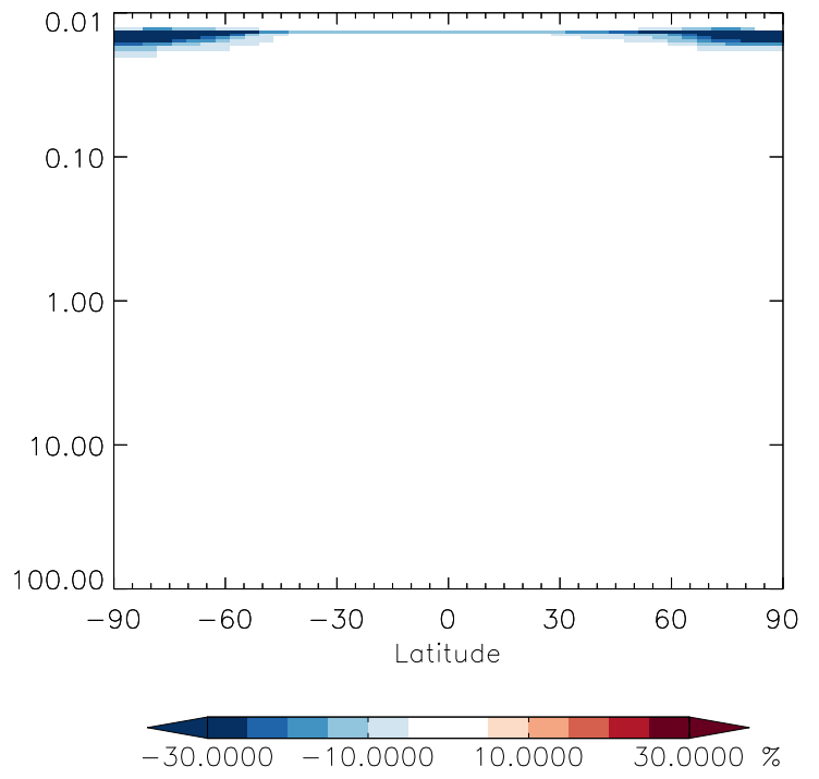
v11-01g-Run0 / v11-01f-geosfp-Run0 HN04 - Strat zonal mean % diff for Apr
