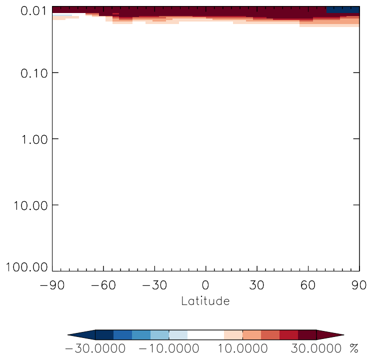
v11-01g-Run0 / v11-01d-Run1 CCI4 - Strat zonal mean % diff for Apr
