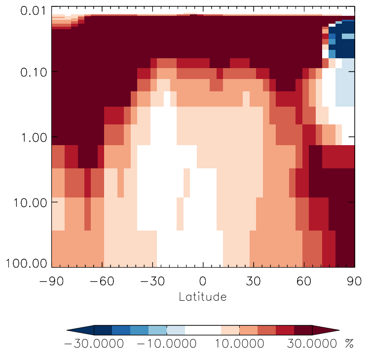
v11-01g-Run0 / v11-01d-Run1 IEPOX - Strat zonal mean % diff for Apr
