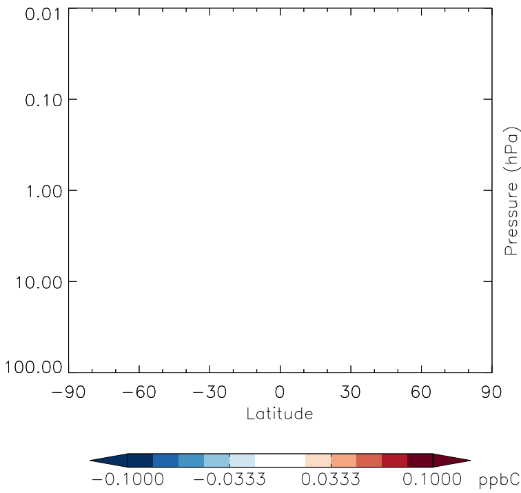
v11-01g-Run0 - v11-01f-geosfp-Run0 MEK - Strat zonal mean abs diff for Apr
