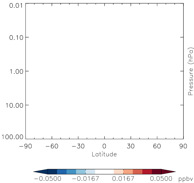
v11-01g-Run0 - v11-01d-Run1 MACR - Strat zonal mean abs diff for Apr
