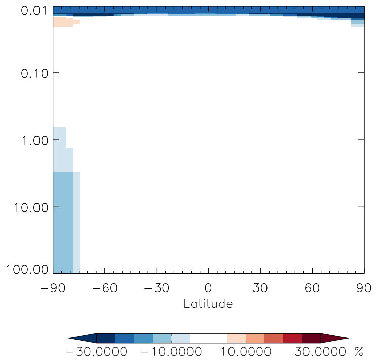
v11-01g-Run0 / v11-01f-geosfp-Run0 NO 3 - Strat zonal mean % diff for Apr
