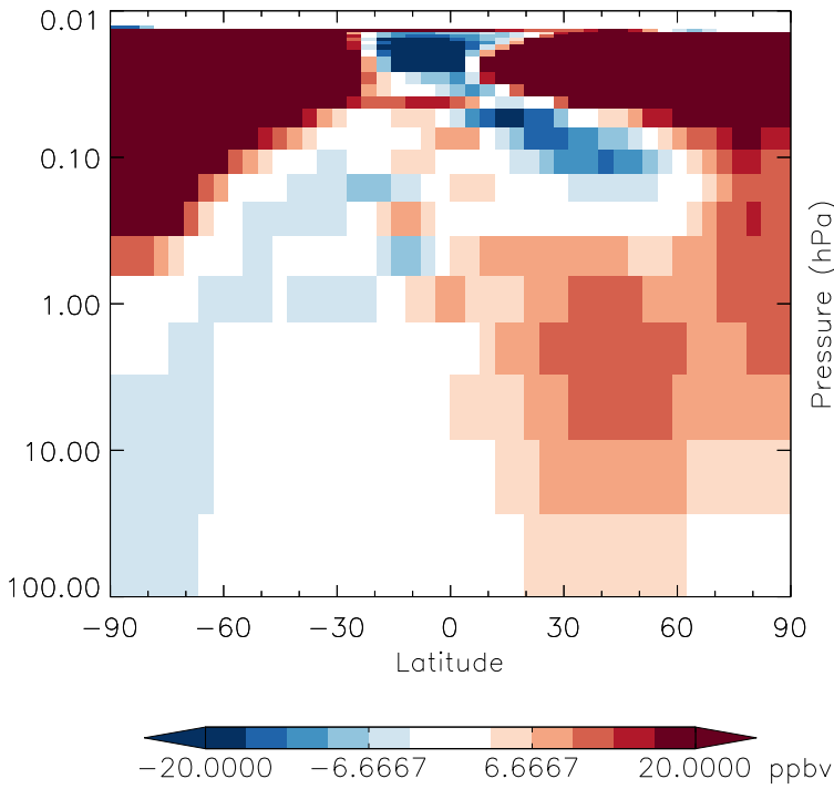
v11-01g-Run0 - v11-01d-Run1 O3 - Strat zonal mean abs diff for Apr
