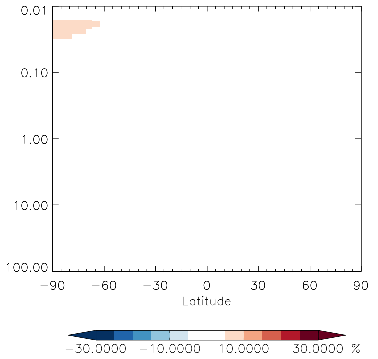
v11-01g-Run0 / v11-01f-geosfp-Run0 CH3Cl - Strat zonal mean % diff for Apr
