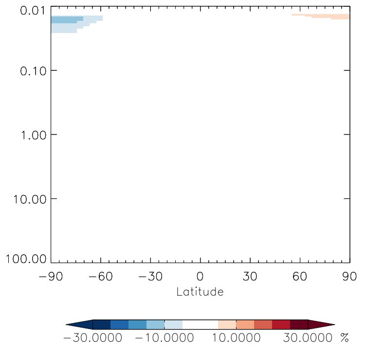
v11-01g-Run0 / v11-01d-Run1 CH2O - Strat zonal mean % diff for Apr
