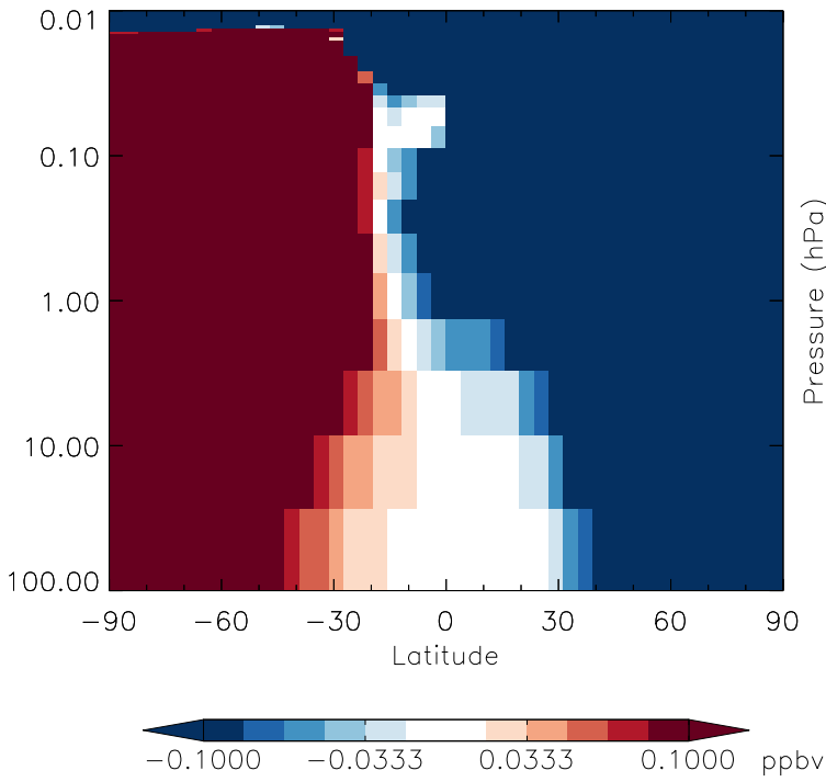
v11-01g-Run0 - v11-01f-geosfp-Run0 CH4 - Strat zonal mean abs diff for Apr
