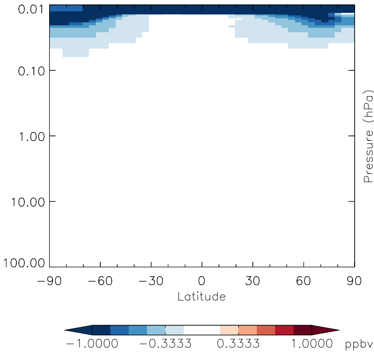
v11-01g-Run0 - v11-01d-Run1 NO 2 - Strat zonal mean abs diff for Apr
