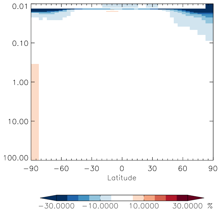
v11-01g-Run0 / v11-01d-Run1 BrNO 3 - Strat zonal mean % diff for Apr
