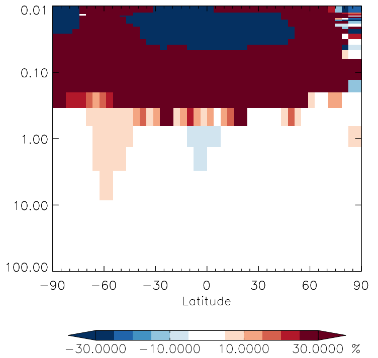
v11-01g-Run0 / v11-01f-geosfp-Run0 MACR - Strat zonal mean % diff for Apr
