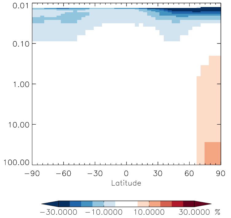
v11-01g-Run0 / v11-01d-Run1 HN02 - Strat zonal mean % diff for Jan
