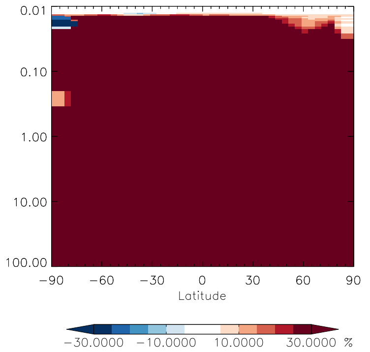
v11-01g-Run0 / v11-01d-Run1 MVKN - Strat zonal mean % diff for Jan
