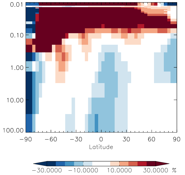
v11-01g-Run0 / v11-01d-Run1 GLYC - Strat zonal mean % diff for Jan
