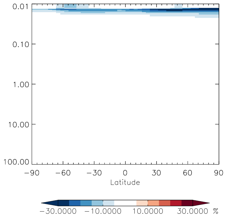
v11-01g-Run0 / v11-01d-Run1 HN04 - Strat zonal mean % diff for Jan
