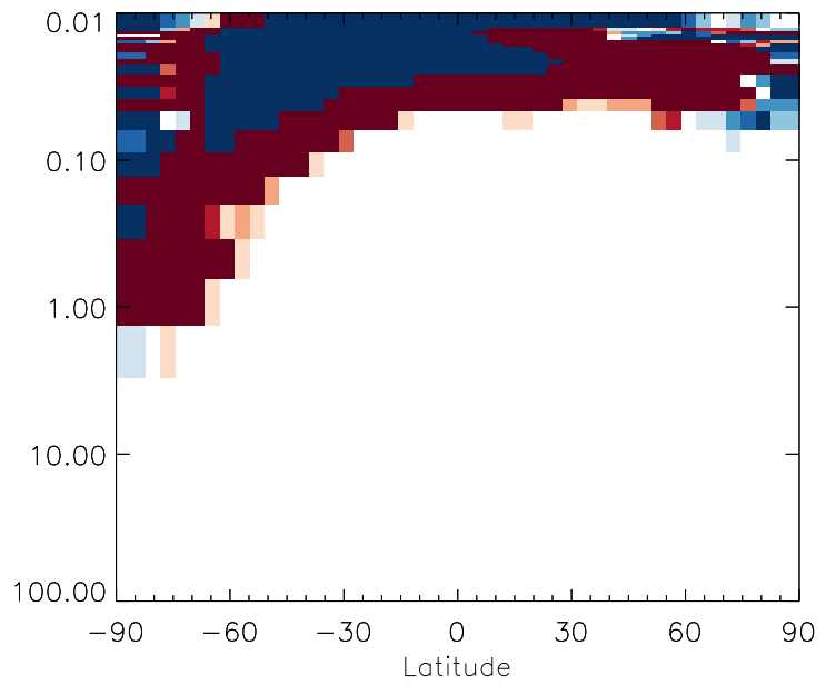
v11-01g-Run0 / v11-01f-geosfp-Run0 OCPO - Strat zonal mean % diff for Jan
