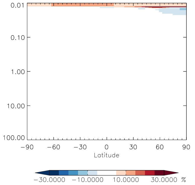
v11-01g-Run0 / v11-01f-geosfp-Run0 MPN - Strat zonal mean % diff for Jan
