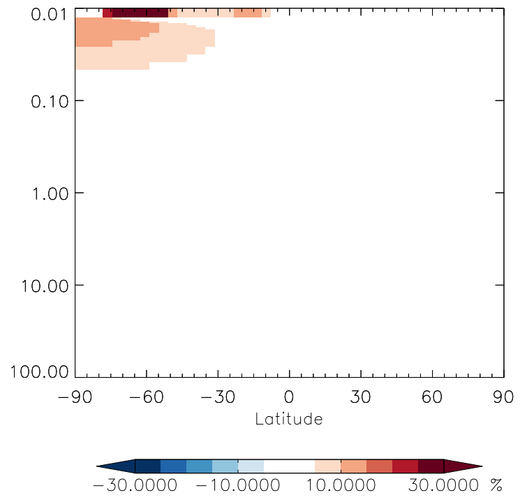
v11-01g-Run0 / v11-01f-geosfp-Run0 CFC11 - Strat zonal mean % diff for Jan
