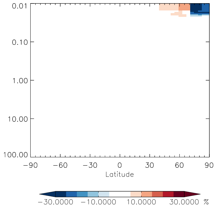
v11-01g-Run0 / v11-01f-geosfp-Run0 HO 2 - Strat zonal mean % diff for Jan
