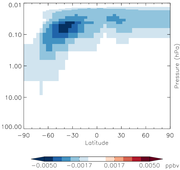
v11-01g-Run0 - v11-01d-Run1 HN04 - Strat zonal mean abs diff for Jan
