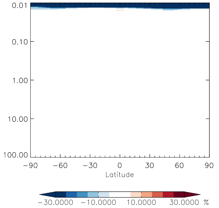
v11-01g-Run0 / v11-01d-Run1 CIN03 - Strat zonal mean % diff for Jan
