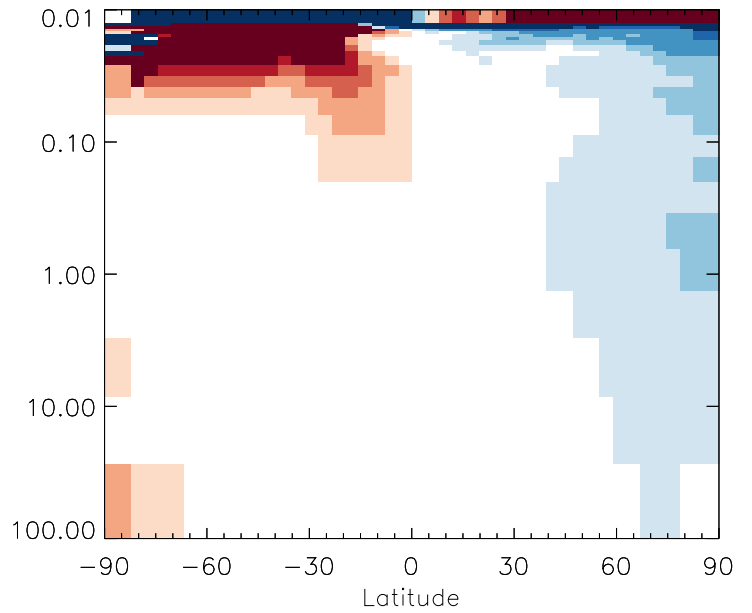
v11-01g-Run0 / v11-01d-Run1 ALK4 - Strat zonal mean % diff for Jan
