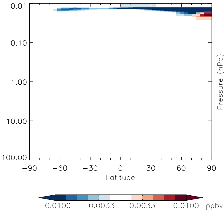
v11-01g-Run0 - v11-01f-geosfp-Run0 NO3 - Strat zonal mean abs diff for Jan
