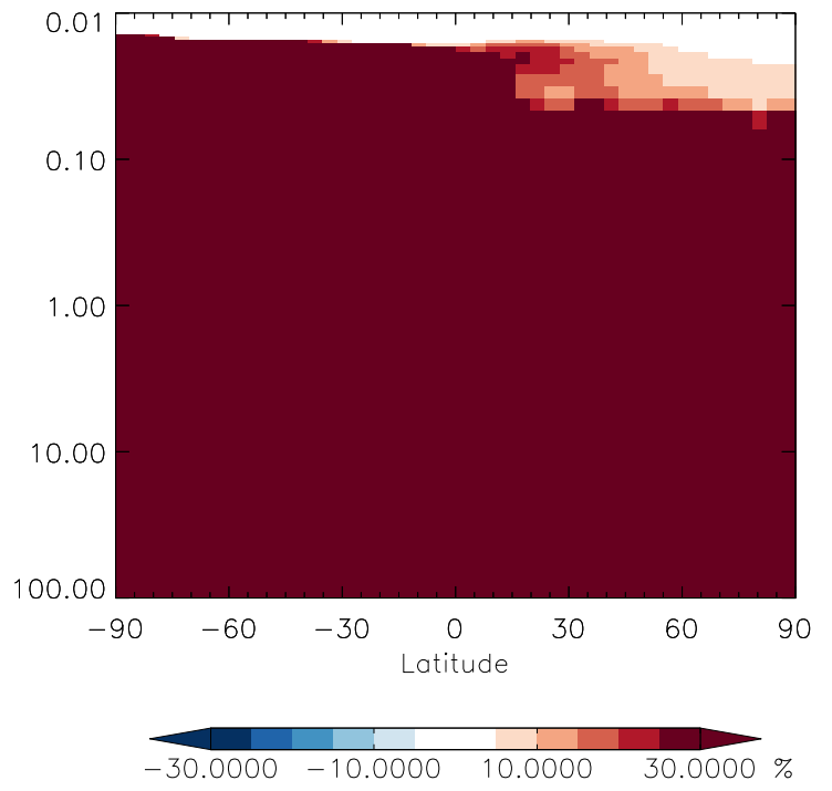
v11-01g-Run0 / v11-01f-geosfp-Run0 MVKN - Strat zonal mean % diff for Jan
