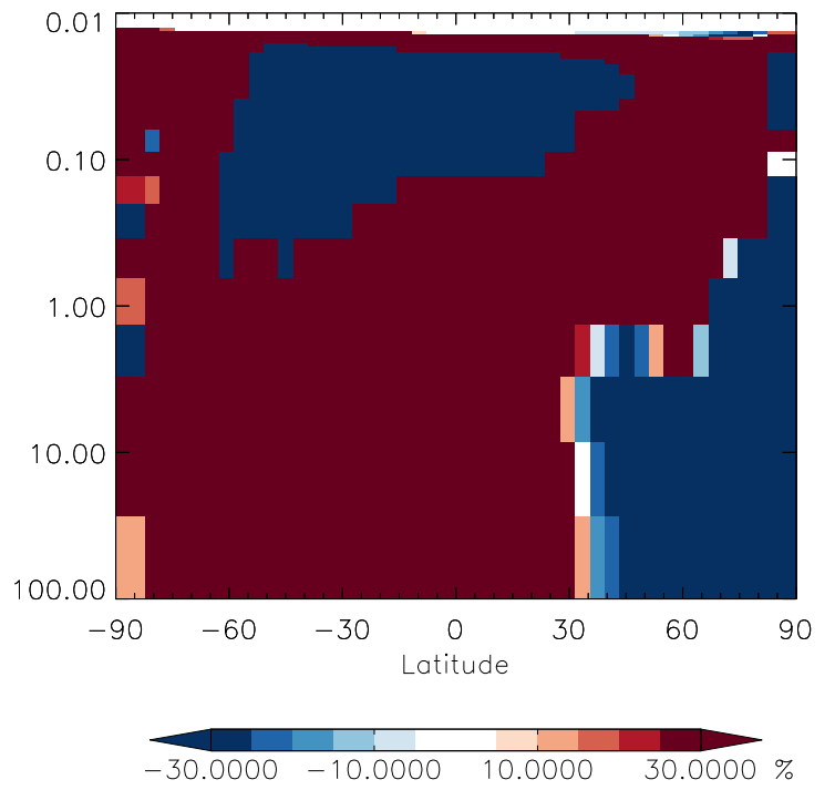
v11-01g-Run0 / v11-01f-geosfp-Run0 ISOPNB - Strat zonal mean % diff for Jan
