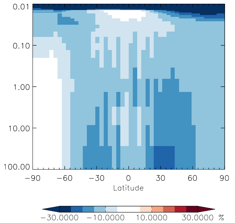
v11-01g-Run0 / v11-01d-Run1 BrNO2 - Strat zonal mean % diff for Jan
