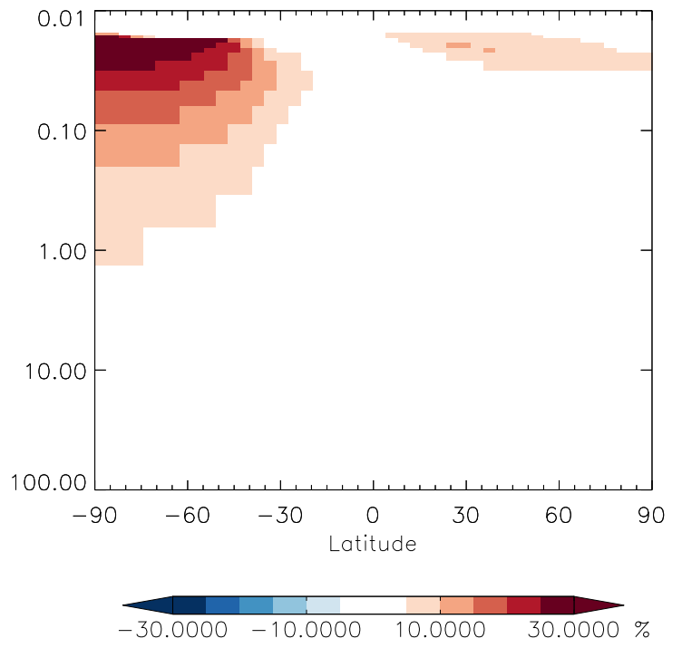
v11-01g-Run0 / v11-01f-geosfp-Run0 R4N2 - Strat zonal mean % diff for Jan
