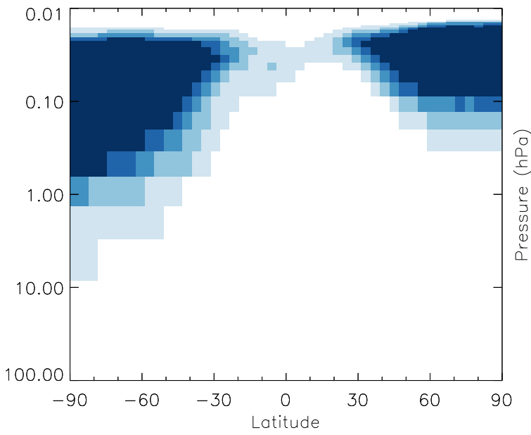
v11-01g-Run0 - v11-01f-geosfp-Run0 HN03 - Strat zonal mean abs diff for Jan
