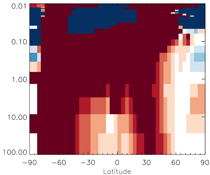
v11-01g-Run0 / v11-01d-Run1 MVK - Strat zonal mean % diff for Jan
