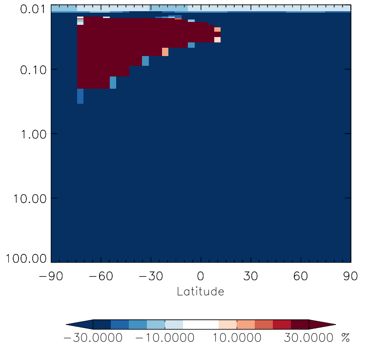
v11-01g-Run0 / v11-01d-Run1 MACRN - Strat zonal mean % diff for Jan
