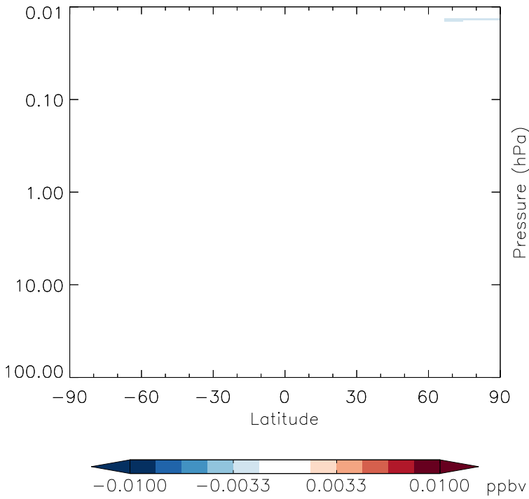
v11-01g-Run0 - v11-01d-Run1 BrNO3 - Strat zonal mean abs diff for Jan
