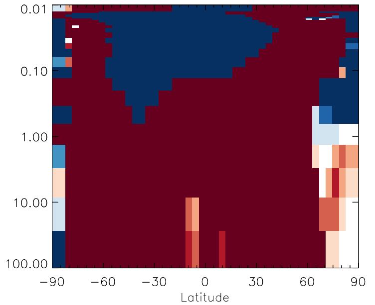
v11-01g-Run0 / v11-01d-Run1 ISOP - Strat zonal mean % diff for Jan
