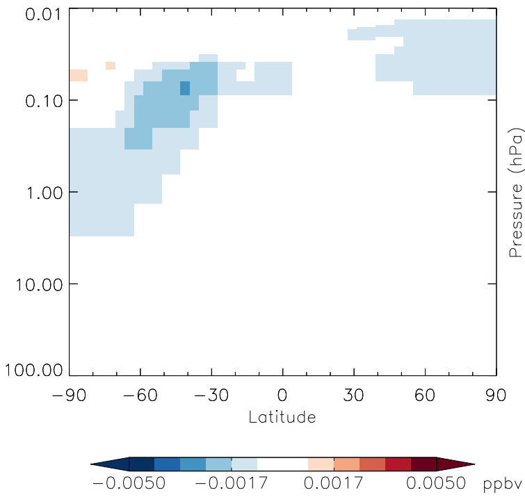
v11-01g-Run0 - v11-01f-geosfp-Run0 HN04 - Strat zonal mean abs diff for Jan
