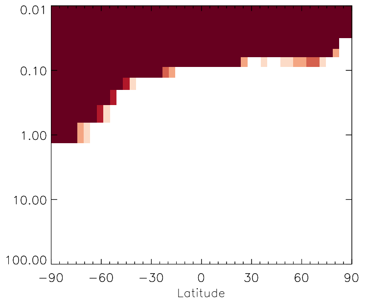
v11-01g-Run0 / v11-01f-geosfp-Run0 DST4 - Strat zonal mean % diff for Jan
