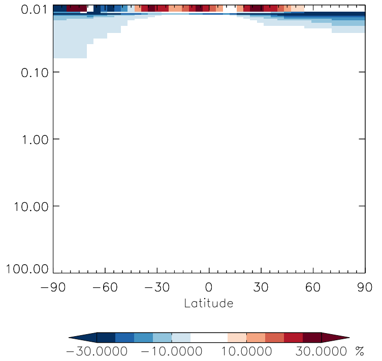
v11-01g-Run0 / v11-01d-Run1 N2O5 - Strat zonal mean % diff for Jan
