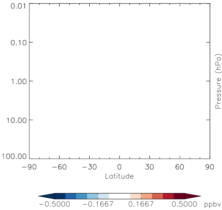
v11-01g-Run0 - v11-01f-geosfp-Run0 CH2O - Strat zonal mean abs diff for Jan
