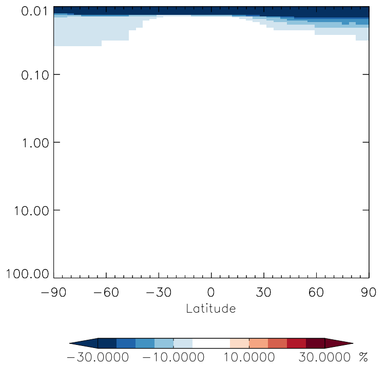
v11-01g-Run0 / v11-01d-Run1 NO 2 - Strat zonal mean % diff for Jan
