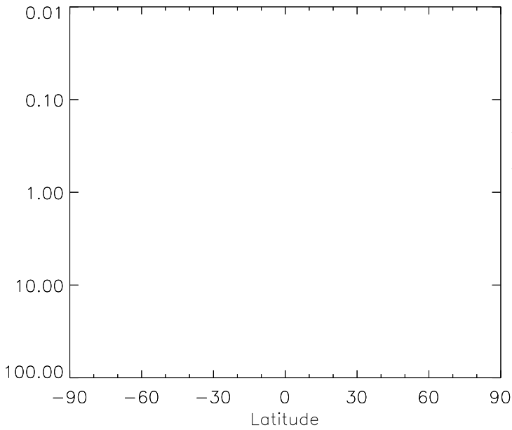
v11-01g-Run0 - v11-01d-Run1 ALK4 - Strat zonal mean abs diff for Jan
