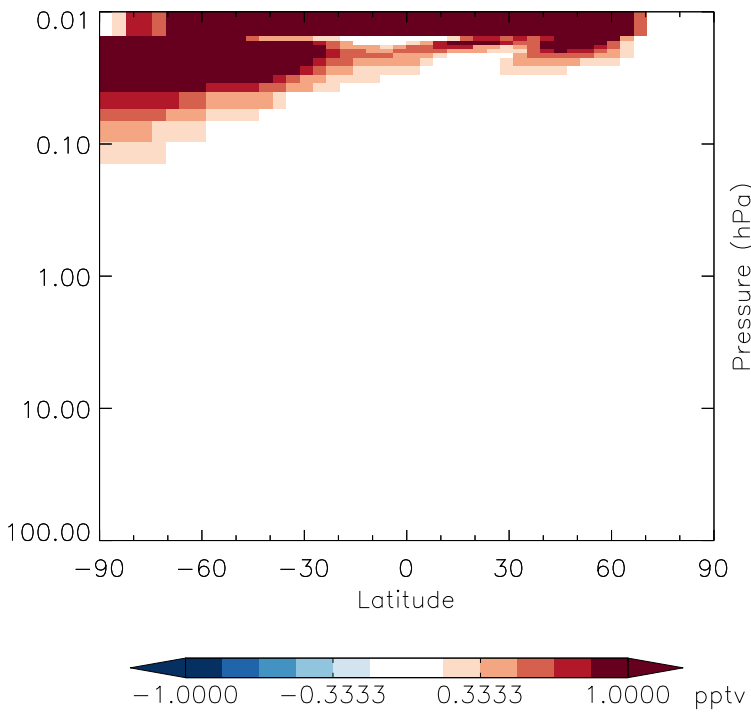
v11-01g-Run0 - v11-01f-geosfp-Run0 HO 2 - Strat zonal mean abs diff for Jan
