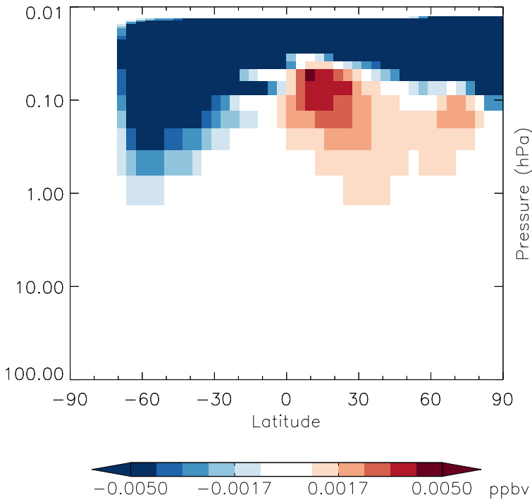
v11-01g-Run0 - v11-01d-Run1 N2O5 - Strat zonal mean abs diff for Jan
