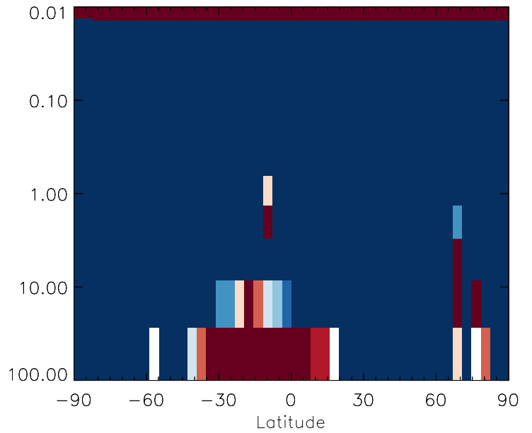
v11-01g-Run0 / v11-01d-Run1 SO4s - Strat zonal mean % diff for Jan
