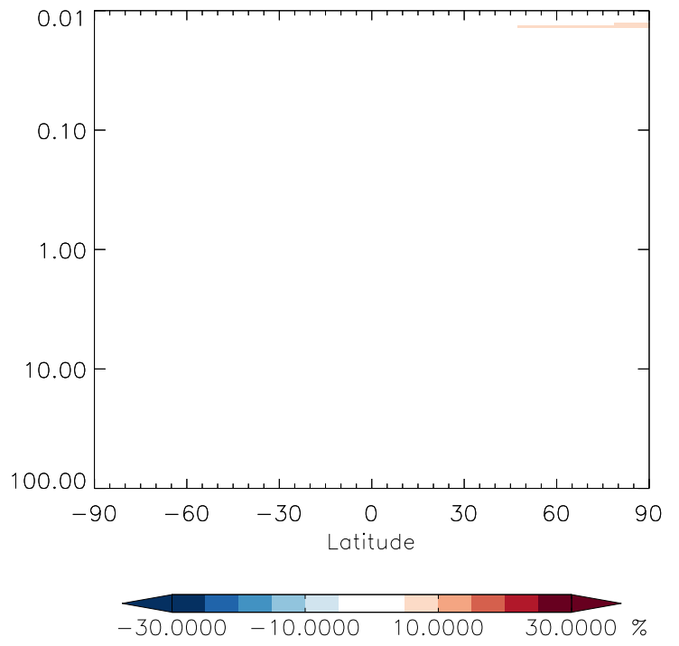
v11-01g-Run0 / v11-01f-geosfp-Run0 CH2O - Strat zonal mean % diff for Jan
