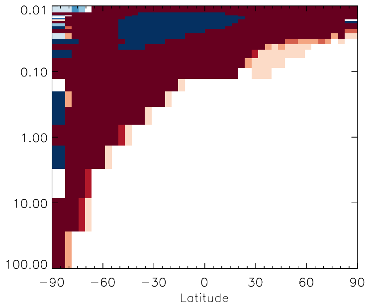
v11-01g-Run0 / v11-01f-geosfp-Run0 PRPE - Strat zonal mean % diff for Jan
