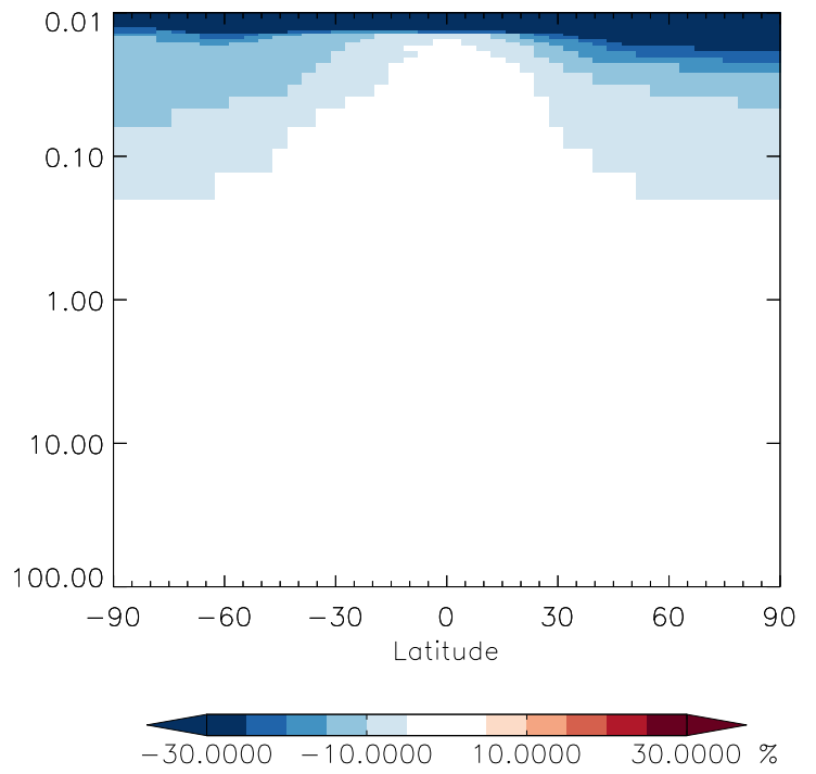
v11-01g-Run0 / v11-01f-geosfp-Run0 BrNO2 - Strat zonal mean % diff for Jan
