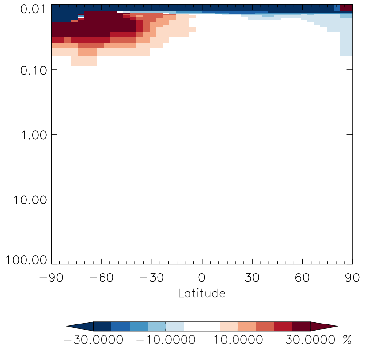
v11-01g-Run0 / v11-01d-Run1 C3H8 - Strat zonal mean % diff for Jan
