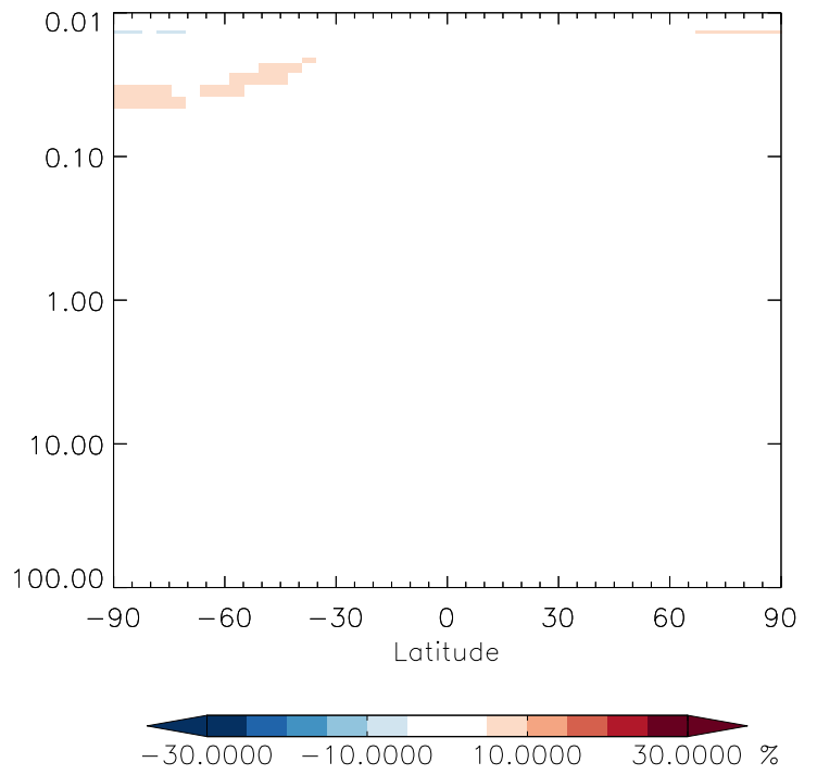
v11-01g-Run0 / v11-01f-geosfp-Run0 ALD2 - Strat zonal mean % diff for Jan
