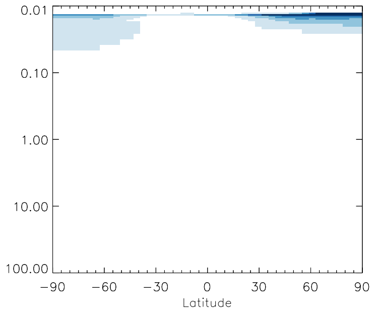
v11-01g-Run0 / v11-01f-geosfp-Run0 HN03 - Strat zonal mean % diff for Jan
