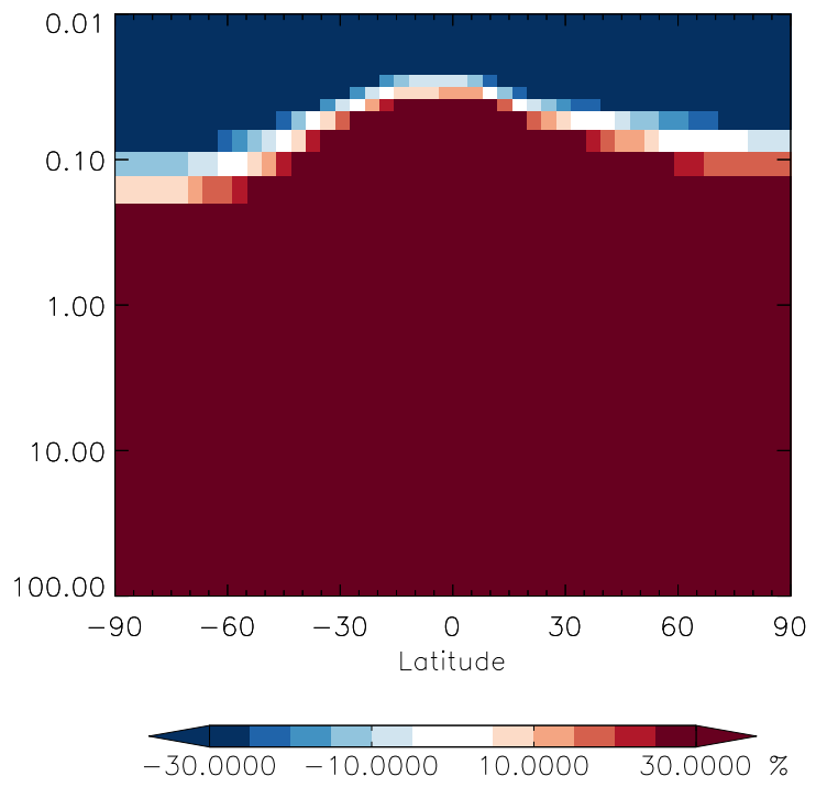
v11-01g-Run0 / v11-01d-Run1 CFC113 - Strat zonal mean % diff for Jan
