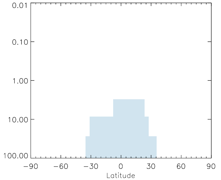
v11-01g-Run0 / v11-01d-Run1 NH4 - Strat zonal mean % diff for Jan
