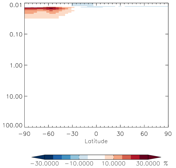
v11-01g-Run0 / v11-01d-Run1 H1301 - Strat zonal mean % diff for Jan
