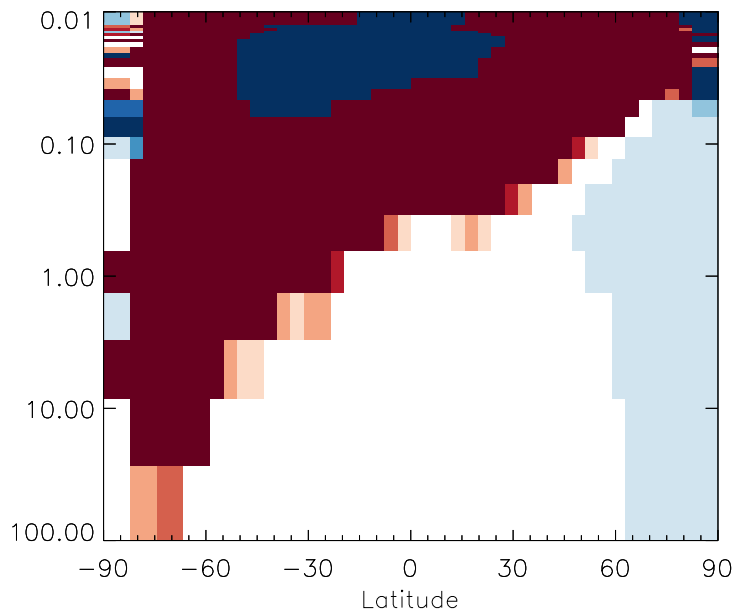
v11-01g-Run0 / v11-01f-geosp-Run0 MVK - Strat zonal mean % diff for Jan
