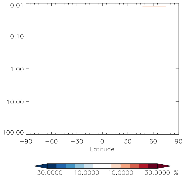
v11-01g-Run0 / v11-01d-Run1 CFC12 - Strat zonal mean % diff for Jan
