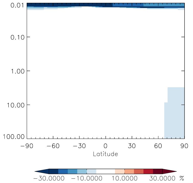
v11-01g-Run0 / v11-01f-geosfp-Run0 NO3 - Strat zonal mean % diff for Jan
