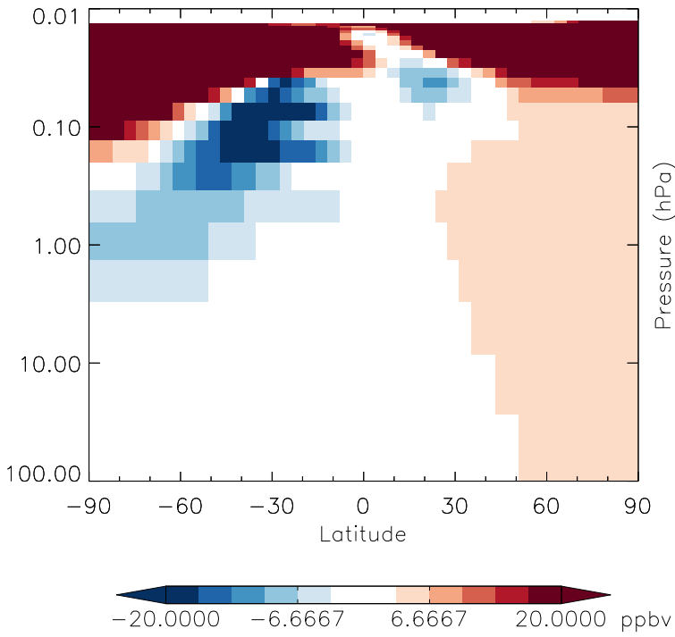
v11-01g-Run0 - v11-01f-geosfp-Run0 O3 - Strat zonal mean abs diff for Jan
