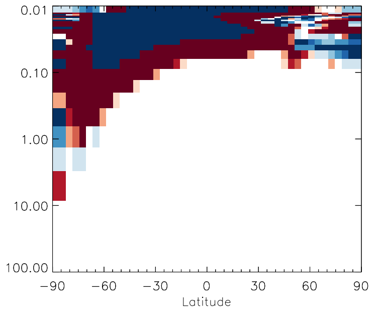
v11-01g-Run0 / v11-01f-geosfp-Run0 BCPO - Strat zonal mean % diff for Jan
