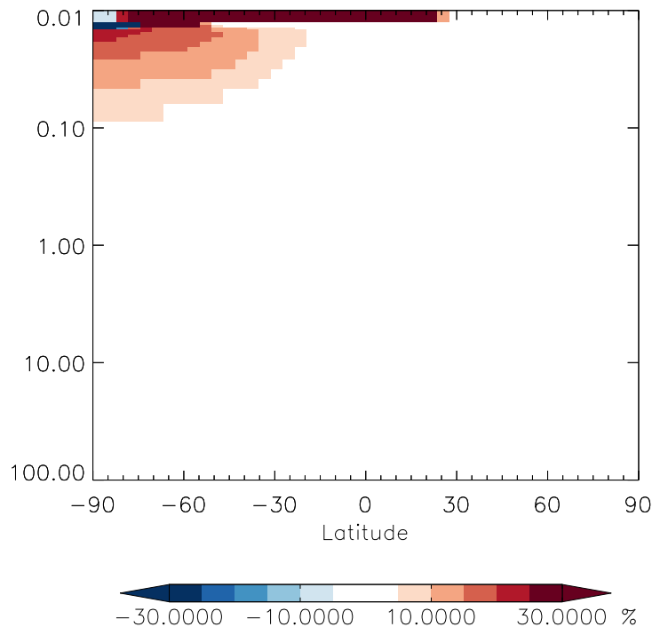
v11-01g-Run0 / v11-01f-geosfp-Run0 CCI4 - Strat zonal mean % diff for Jan
