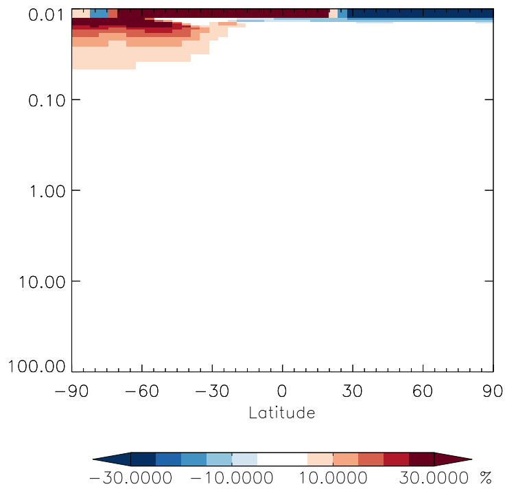
v11-01g-Run0 / v11-01d-Run1 CH 3 CCl 3 - Strat zonal mean % diff for Jan
