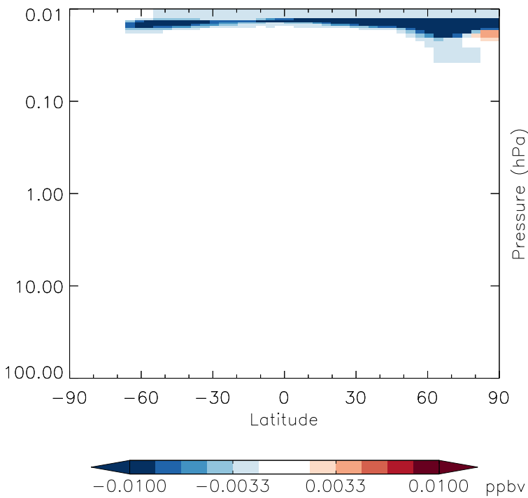
v11-01g-Run0 - v11-01d-Run1 NO3 - Strat zonal mean abs diff for Jan
