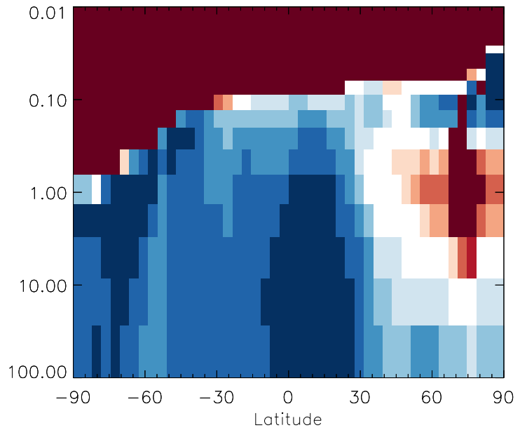
v11-01g-Run0 / v11-01d-Run1 DST4 - Strat zonal mean % diff for Jan
