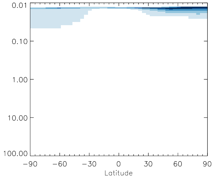
v11-01g-Run0 / v11-01d-Run1 HN03 - Strat zonal mean % diff for Jan
