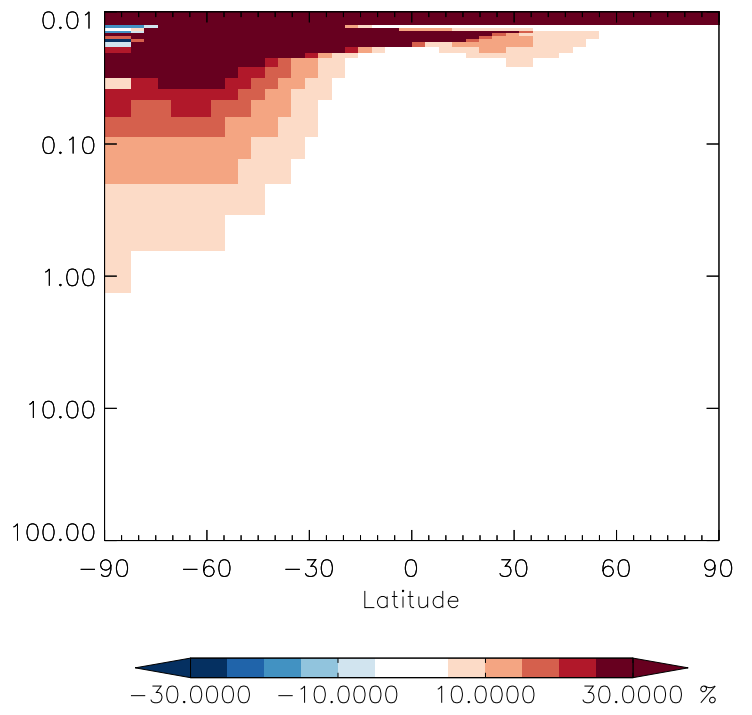
v11-01g-Run0 / v11-01f-geosfp-Run0 CHBr3 - Strat zonal mean % diff for Jan
