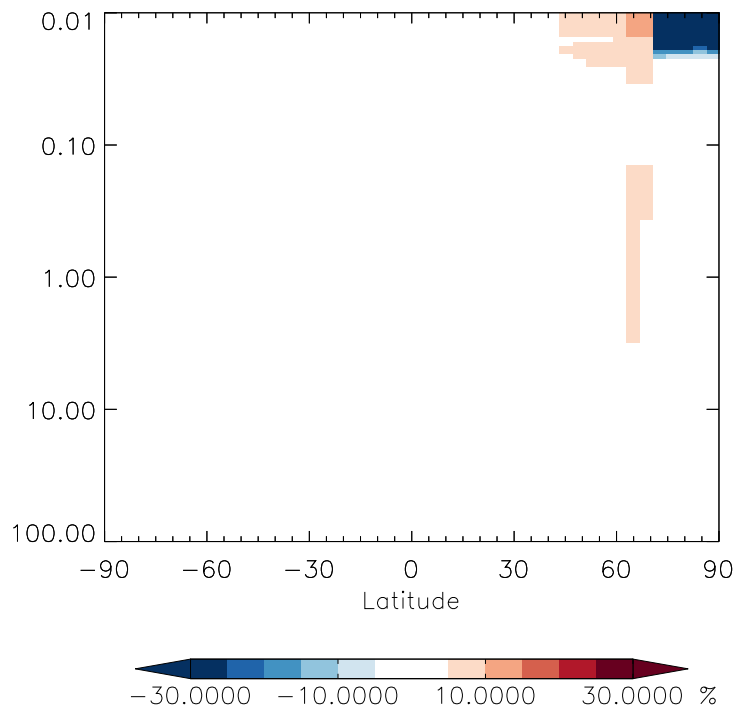
v11-01g-Run0 / v11-01d-Run1 HO 2 - Strat zonal mean % diff for Jan
