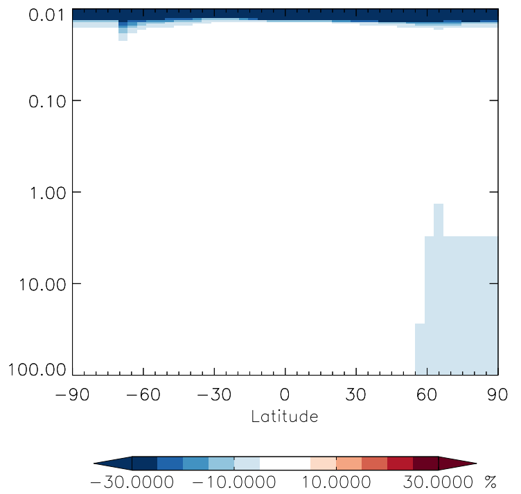
v11-01g-Run0 / v11-01d-Run1 NO3 - Strat zonal mean % diff for Jan
