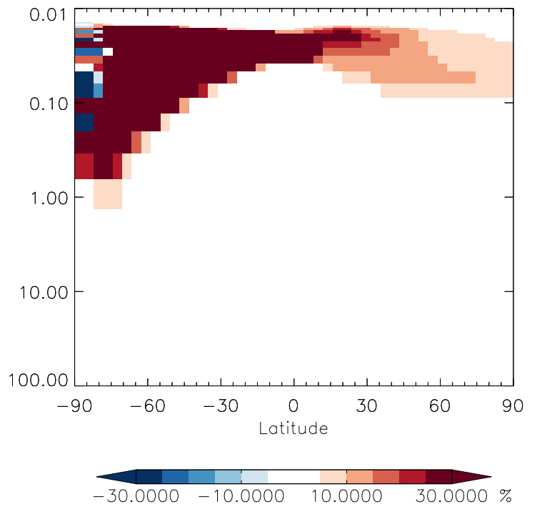
v11-01g-Run0 / v11-01f-geosfp-Run0 IEPOX - Strat zonal mean % diff for Jan
