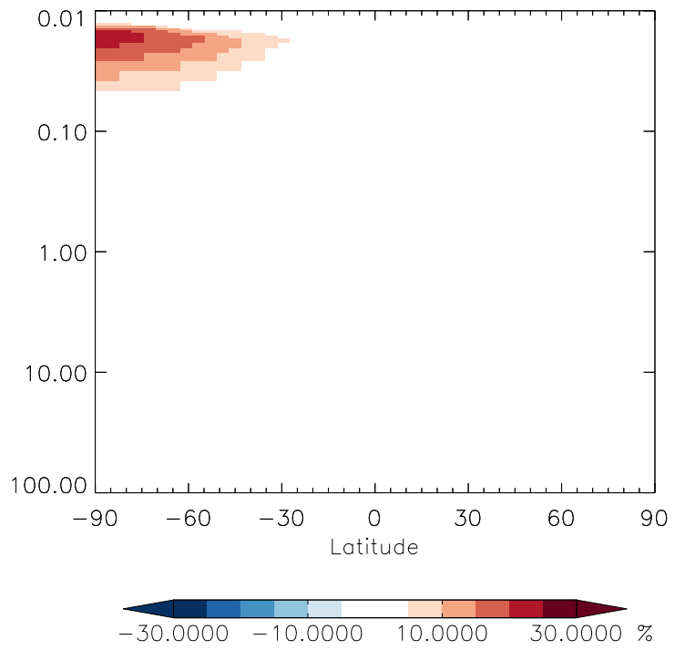
v11-01g-Run0 / v11-01f-geosfp-Run0 C2H6 - Strat zonal mean % diff for Jan
