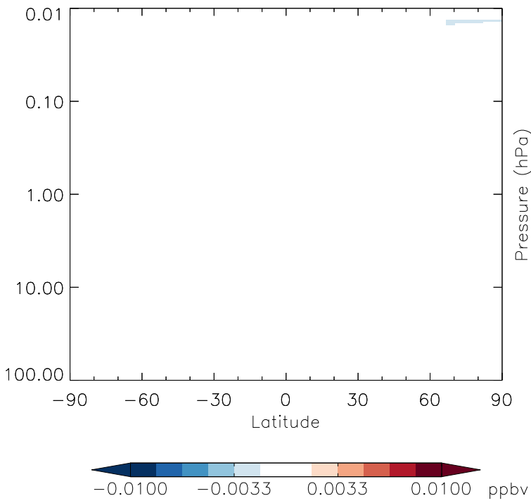
v11-01g-Run0 - v11-01f-geosfp-Run0 BrNO3 - Strat zonal mean abs diff for Jan
