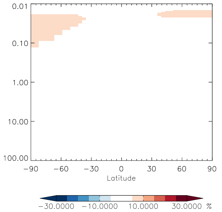
v11-01g-Run0 / v11-01d-Run1 H2O2 - Strat zonal mean % diff for Jan
