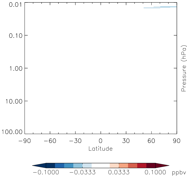
v11-01g-Run0 - v11-01d-Run1 CIN03 - Strat zonal mean abs diff for Jan
