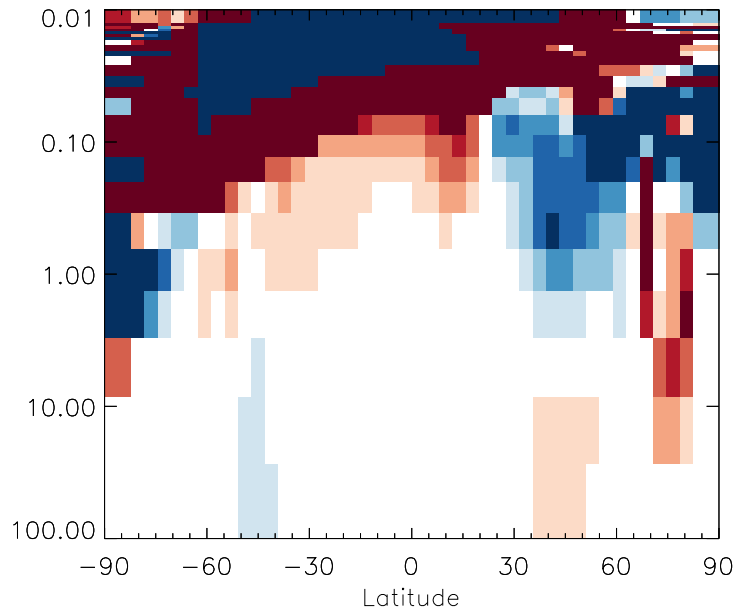
v11-01g-Run0 / v11-01d-Run1 BCPO - Strat zonal mean % diff for Jan
