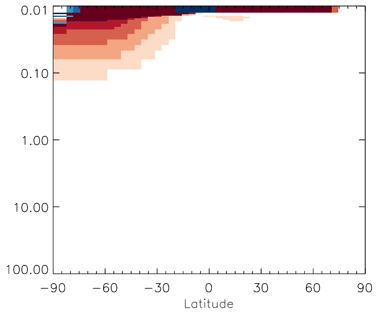
v11-01g-Run0 / v11-01f-geosfp-Run0 H2402 - Strat zonal mean % diff for Jan
