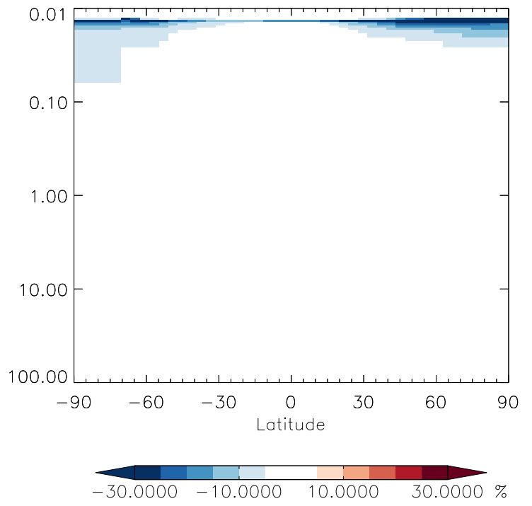
v11-01g-Run0 / v11-01f-geosfp-Run0 N2O5 - Strat zonal mean % diff for Jan
