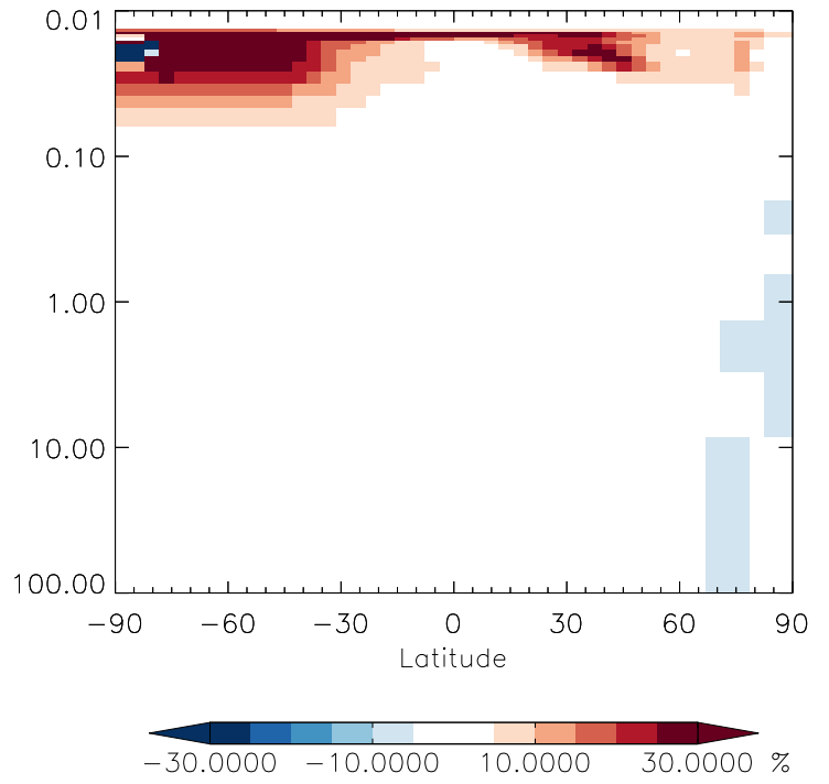
v11-01g-Run0 / v11-01d-Run1 RCHO - Strat zonal mean % diff for Jan
