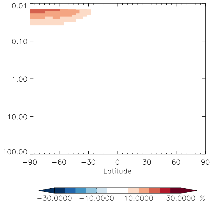
v11-01g-Run0 / v11-01f-geosfp-Run0 H1301 - Strat zonal mean % diff for Jan
