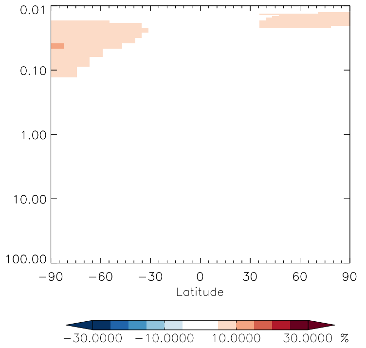
v11-01g-Run0 / v11-01f-geosfp-Run0 H2O2 - Strat zonal mean % diff for Jan
