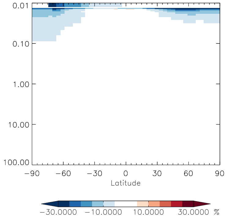
v11-01g-Run0 / v11-01d-Run1 BrNO3 - Strat zonal mean % diff for Jan
