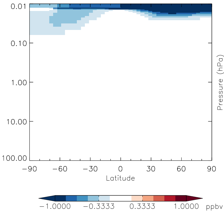
v11-01g-Run0 - v11-01d-Run1 NO 2 - Strat zonal mean abs diff for Jan
