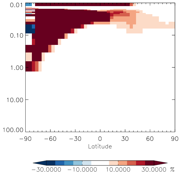
v11-01g-Run0 / v11-01f-geosfp-Run0 GLYC - Strat zonal mean % diff for Jan
