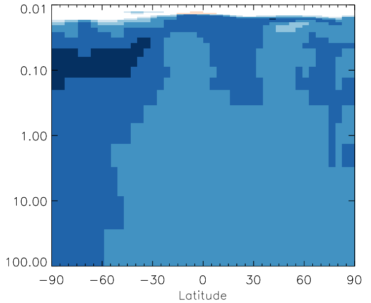
v11-01g-Run0 / v11-01d-Run1 DST1 - Strat zonal mean % diff for Jan
