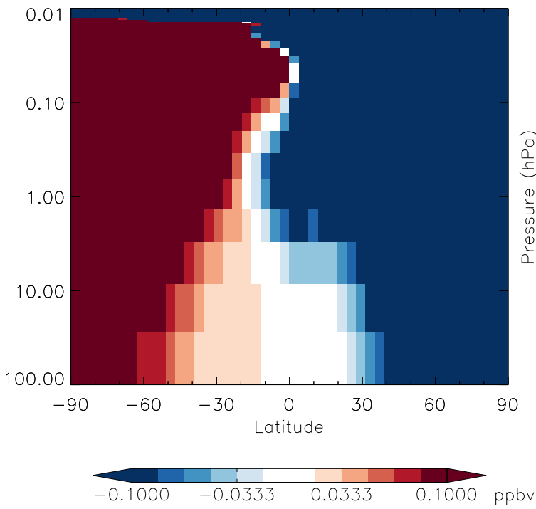
v11-01g-Run0 - v11-01f-geosfp-Run0 CH4 - Strat zonal mean abs diff for Jan
