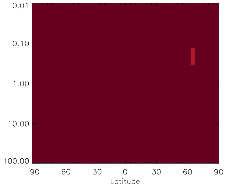
v11-01g-Run0 / v11-01d-Run1 NITs - Strat zonal mean % diff for Jan
