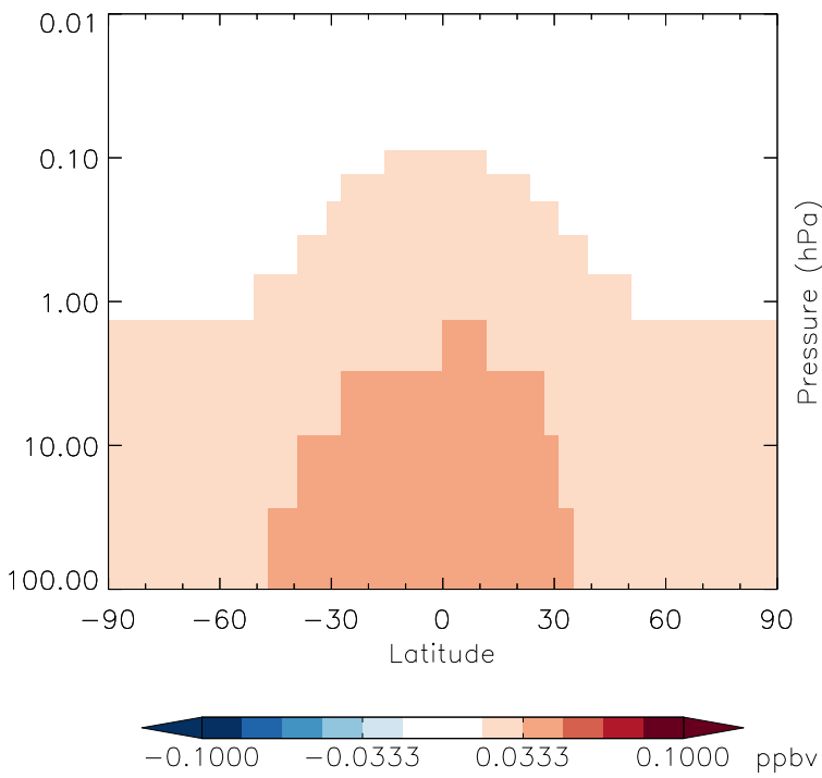
v11-01g-Run0 - v11-01d-Run1 CFC113 - Strat zonal mean abs diff for Jan
