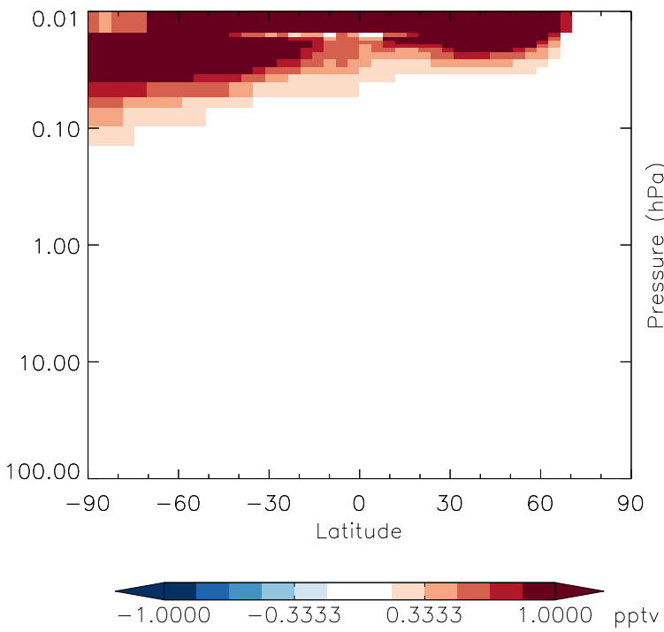
v11-01g-Run0 - v11-01d-Run1 HO 2 - Strat zonal mean abs diff for Jan
