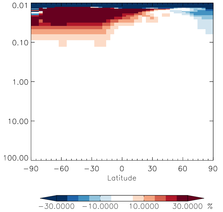
v11-01g-Run0 / v11-01d-Run1 CHBr3 - Strat zonal mean % diff for Jan
