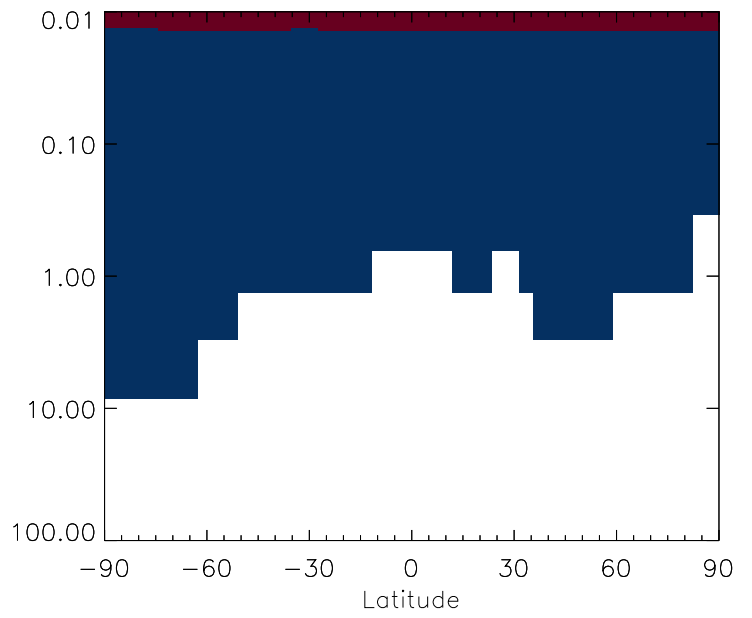
v11-01g-Run0 / v11-01f-geosfp-Run0 SO4s - Strat zonal mean % diff for Jan
