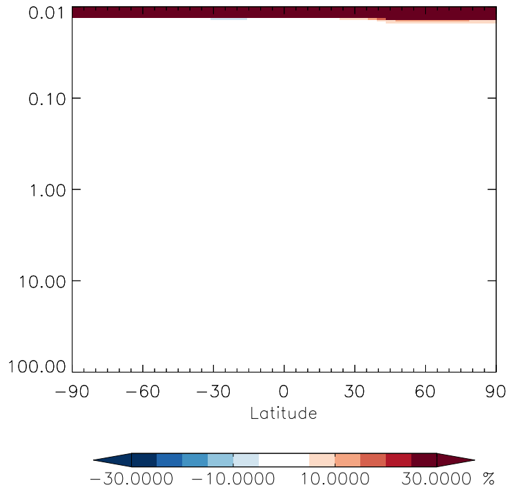
v11-01g-Run0 / v11-01d-Run1 N2O - Strat zonal mean % diff for Jan
