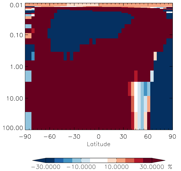
v11-01g-Run0 / v11-01d-Run1 ISOPNB - Strat zonal mean % diff for Jan
