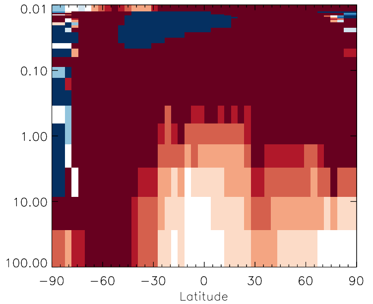
v11-01g-Run0 / v11-01d-Run1 PRPE - Strat zonal mean % diff for Jan
