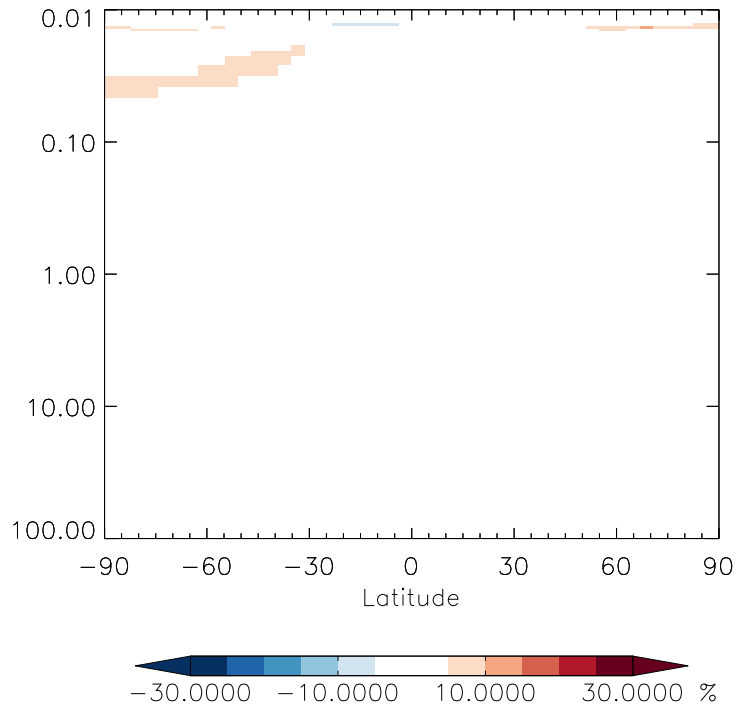
v11-01g-Run0 / v11-01d-Run1 ALD2 - Strat zonal mean % diff for Jan
