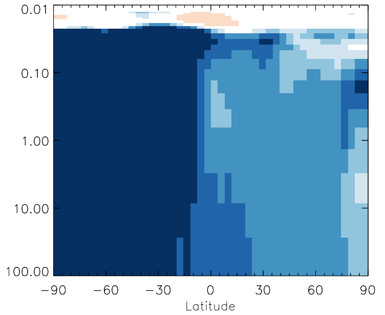
v11-01g-Run0 / v11-01d-Run1 DST2 - Strat zonal mean % diff for Jan
