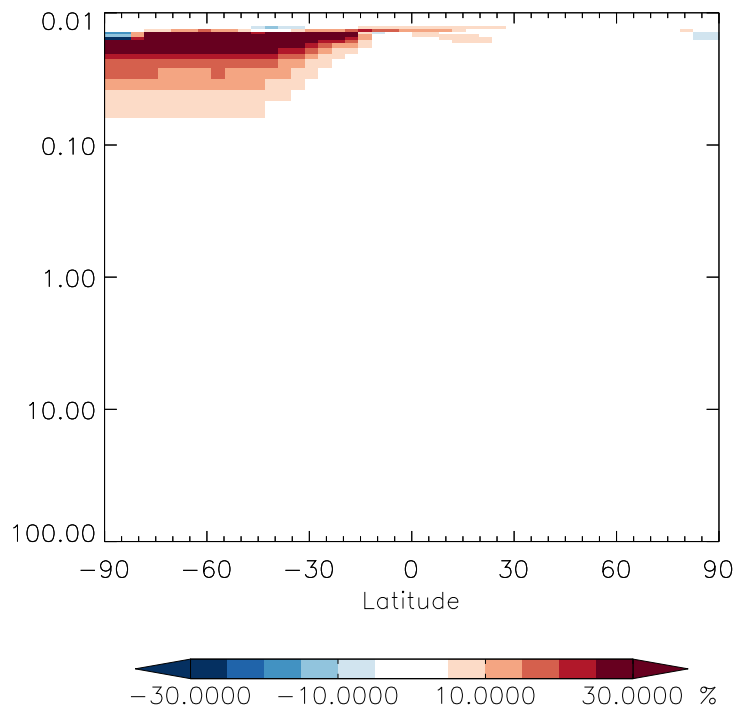
v11-01g-Run0 / v11-01d-Run1 CH3Br - Strat zonal mean % diff for Jan
