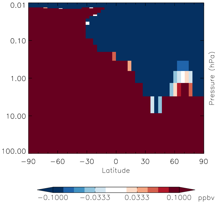
v11-01g-Run0 - v11-01d-Run1 CH4 - Strat zonal mean abs diff for Jan
