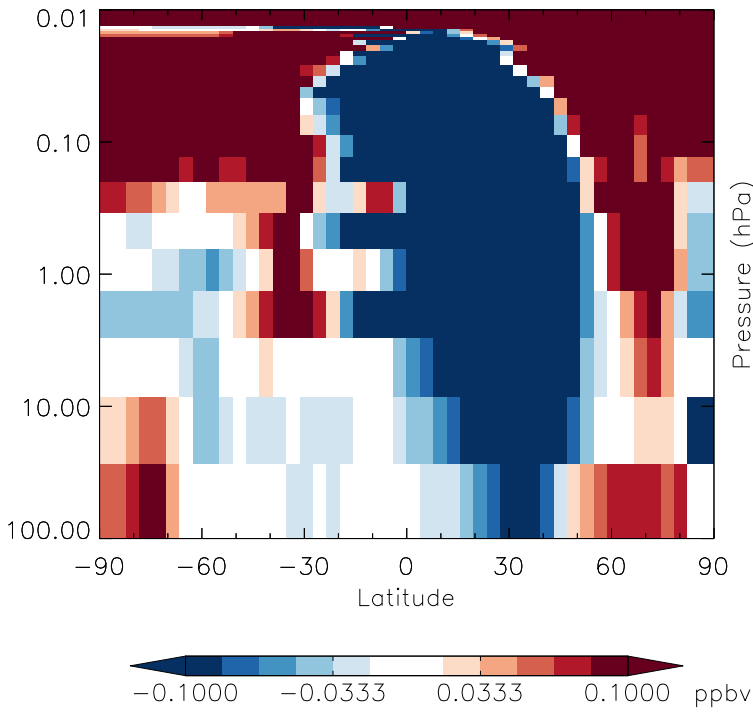
v11-01g-Run0 - v11-01d-Run1 N2O - Strat zonal mean abs diff for Jan
