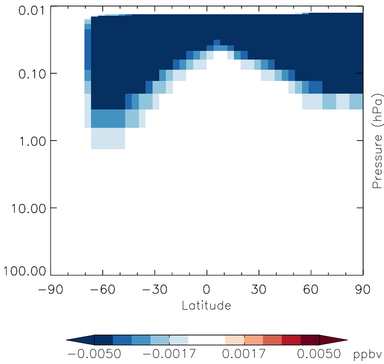
v11-01g-Run0 - v11-01f-geosfp-Run0 N2O5 - Strat zonal mean abs diff for Jan
