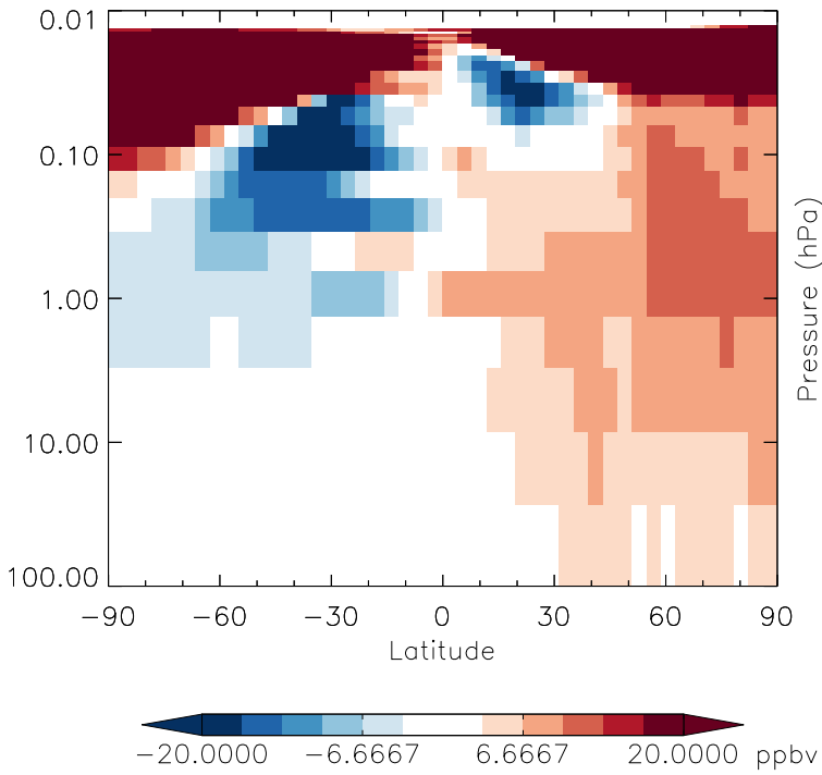
v11-01g-Run0 - v11-01d-Run1 O3 - Strat zonal mean abs diff for Jan
