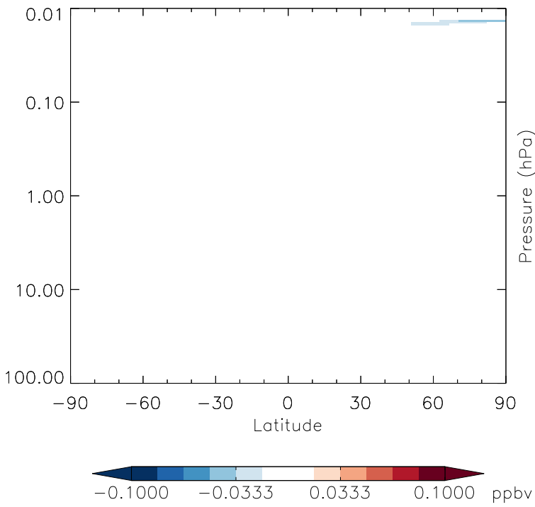
v11-01g-Run0 - v11-01f-geosfp-Run0 CIN03 - Strat zonal mean abs diff for Jan
