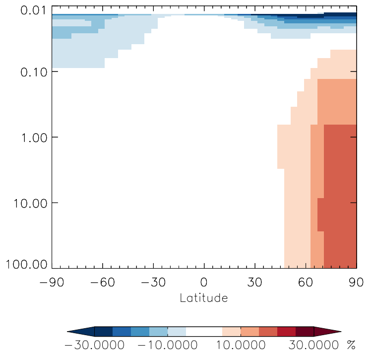
v11-01g-Run0 / v11-01f-geosfp-Run0 HN02 - Strat zonal mean % diff for Jan
