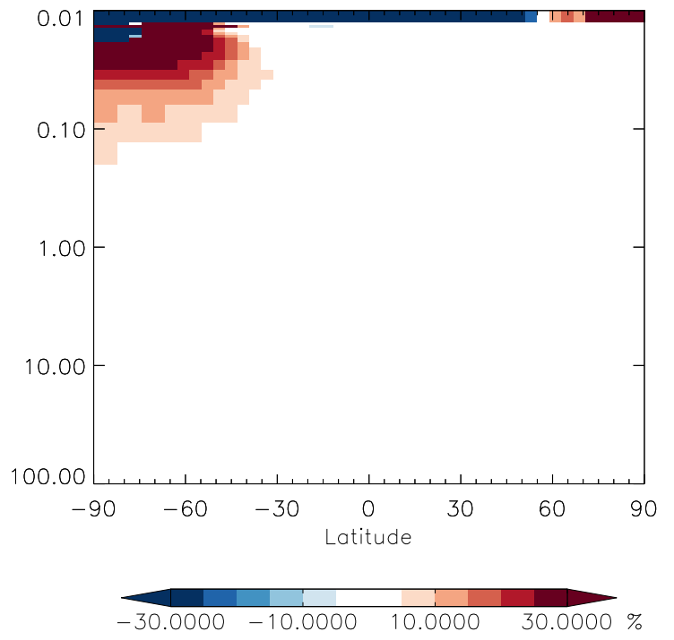
v11-01g-Run0 / v11-01f-geosfp-Run0 C3H8 - Strat zonal mean % diff for Jan
