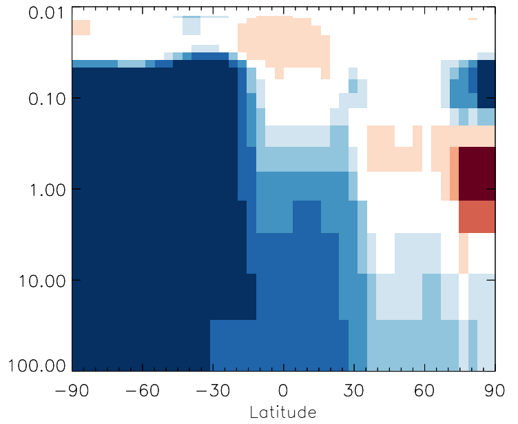
v11-01g-Run0 / v11-01d-Run1 DST3 - Strat zonal mean % diff for Jan
