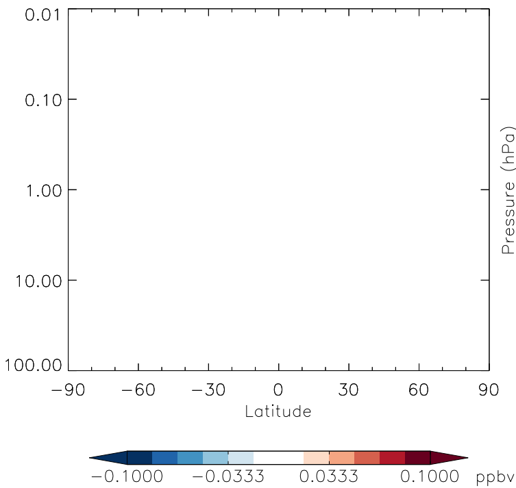
v11-01g-Run0 - v11-01d-Run1 ISOPNB - Strat zonal mean abs diff for Jan
