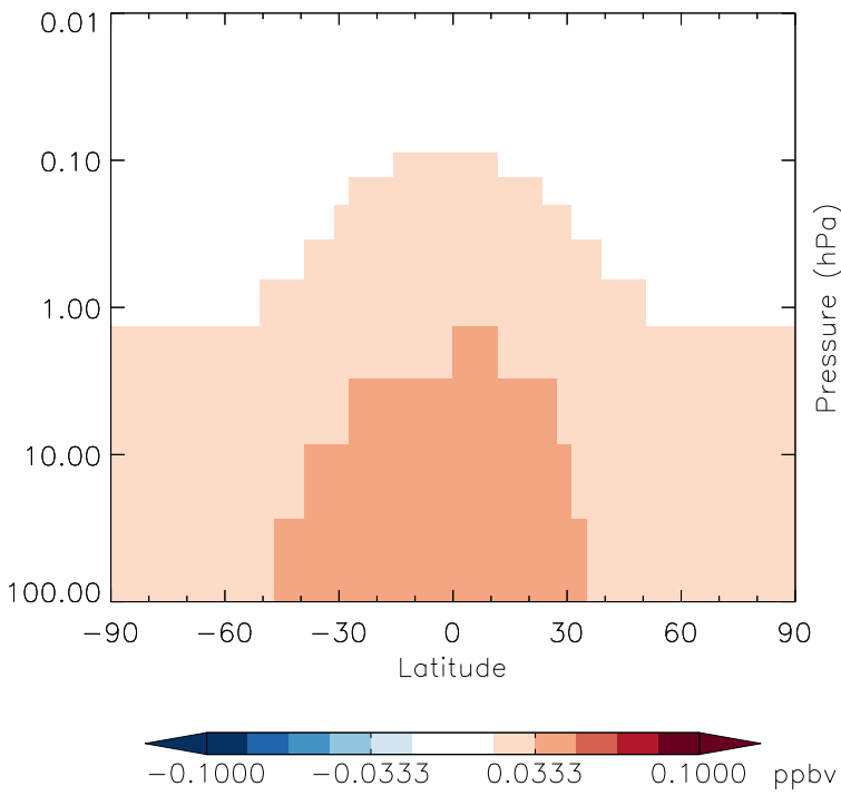
v11-01g-Run0 - v11-01f-geosfp-Run0 CFC113 - Strat zonal mean abs diff for Jan
