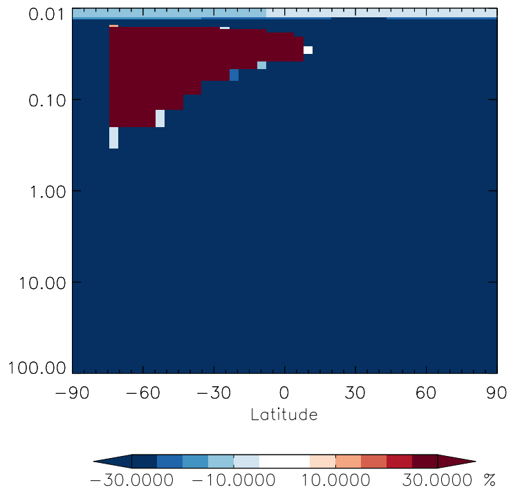
v11-01g-Run0 / v11-01f-geosfp-Run0 MACRN - Strat zonal mean % diff for Jan
