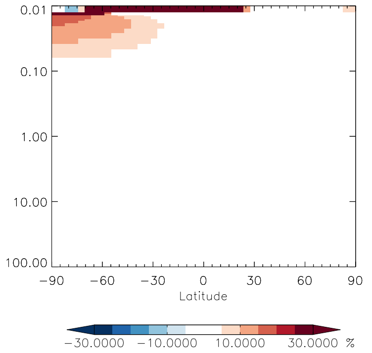
v11-01g-Run0 / v11-01f-geosfp-Run0 CH 3 CCl 3 - Strat zonal mean % diff for Jan
