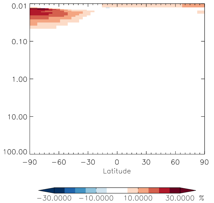
v11-01g-Run0 / v11-01d-Run1 C2H6 - Strat zonal mean % diff for Jan
