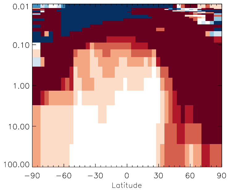
v11-01g-Run0 / v11-01d-Run1 OCPO - Strat zonal mean % diff for Jan
