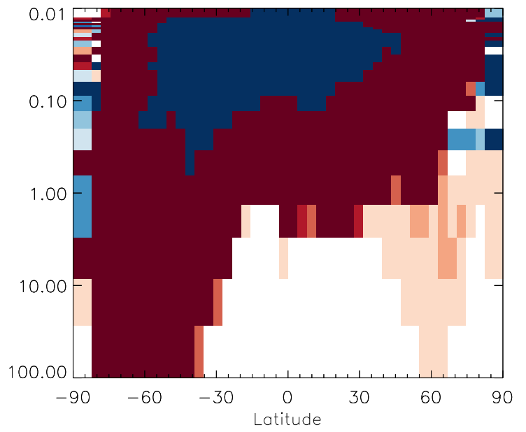
v11-01g-Run0 / v11-01f-geosfp-Run0 ISOP - Strat zonal mean % diff for Jan
