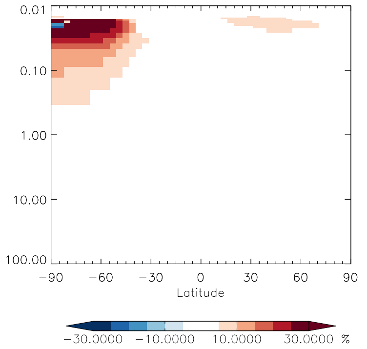
v11-01g-Run0 / v11-01f-geosfp-Run0 RCHO - Strat zonal mean % diff for Jan
