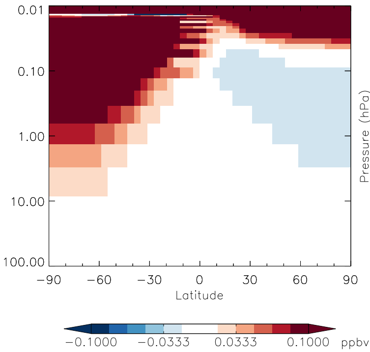
v11-01g-Run0 - v11-01f-geosfp-Run0 N2O - Strat zonal mean abs diff for Jan
