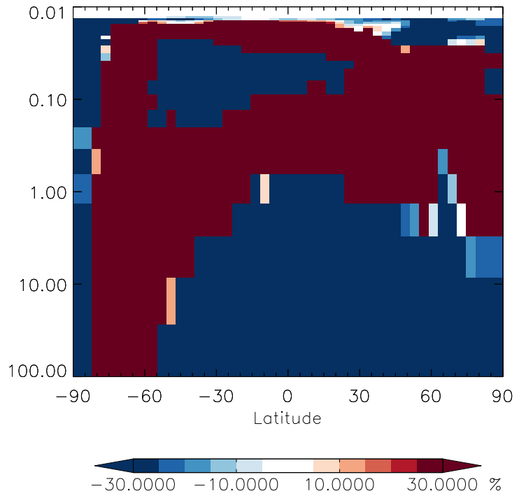
v11-01g-Run0 / v11-01d-Run1 MOBA - Strat zonal mean % diff for Jan
