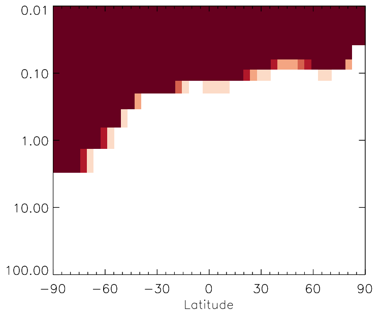
v11-01g-Run0 / v11-01f-geosfp-Run0 NITs - Strat zonal mean % diff for Jan
