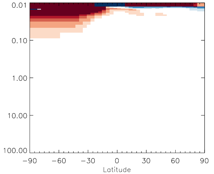
v11-01g-Run0 / v11-01d-Run1 H2402 - Strat zonal mean % diff for Jan
