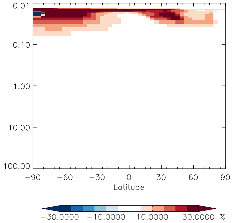
v11-01g-Run0 / v11-01d-Run1 R4N2 - Strat zonal mean % diff for Jan
