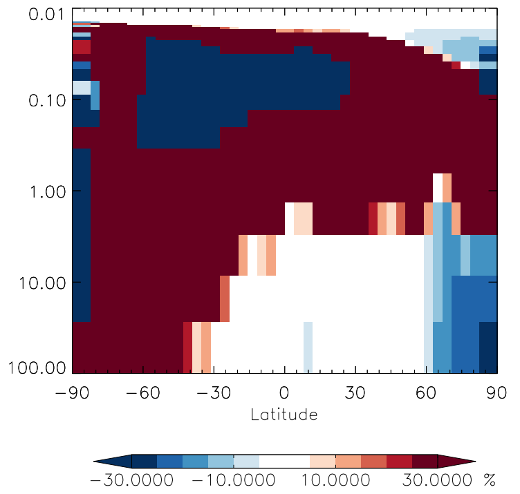
v11-01g-Run0 / v11-01f-geosfp-Run0 MOBA - Strat zonal mean % diff for Jan
