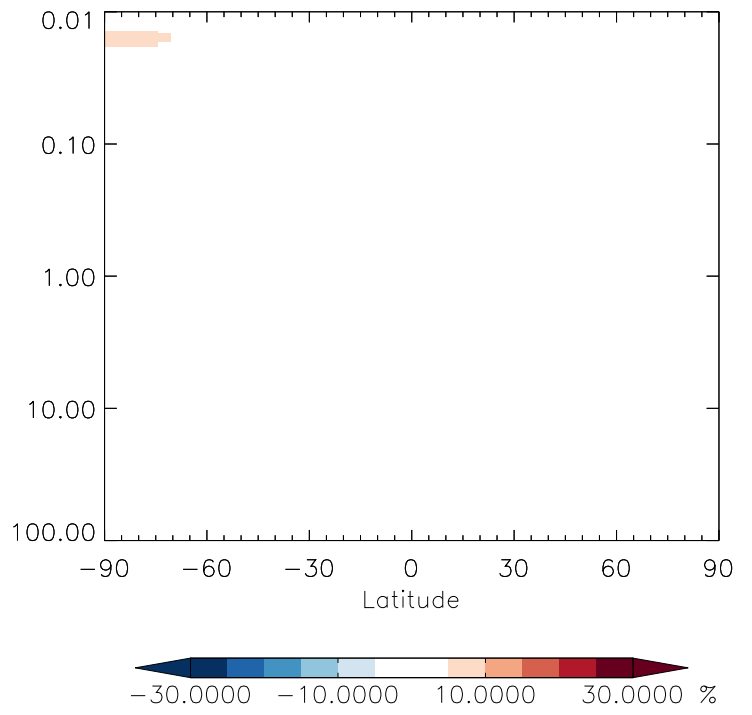
v11-01g-Run0 / v11-01f-geosfp-Run0 CH3Cl - Strat zonal mean % diff for Jan
