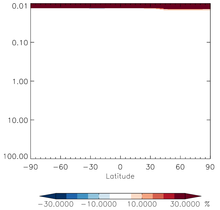
v11-01g-Run0 / v11-01f-geosfp-Run0 N2O - Strat zonal mean % diff for Jan
