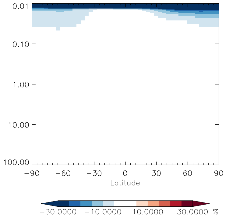
v11-01g-Run0 / v11-01f-geosfp-Run0 NO 2 - Strat zonal mean % diff for Jan
