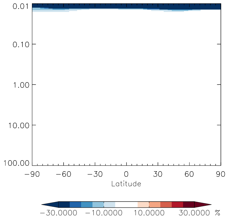
v11-01g-Run0 / v11-01f-geosfp-Run0 CIN03 - Strat zonal mean % diff for Jan
