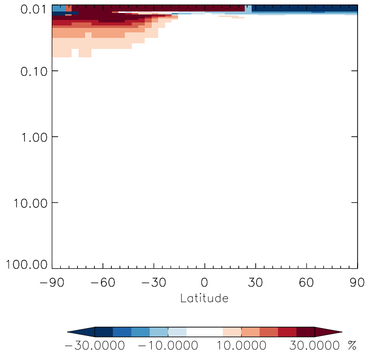
v11-01g-Run0 / v11-01d-Run1 CCI4 - Strat zonal mean % diff for Jan
