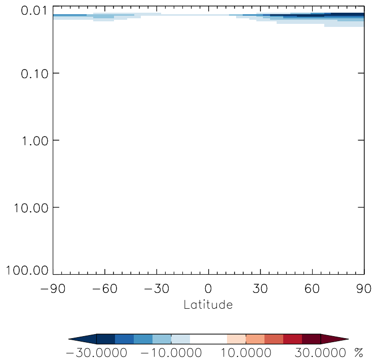
v11-01g-Run0 / v11-01f-geosfp-Run0 HN04 - Strat zonal mean % diff for Jan
