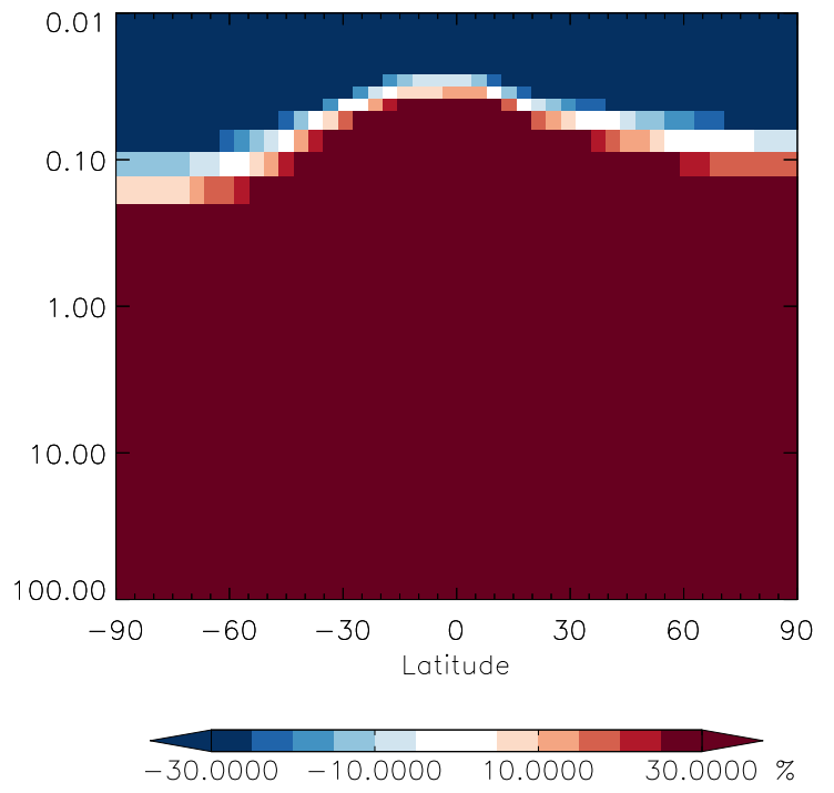
v11-01g-Run0 / v11-01f-geosfp-Run0 CFC113 - Strat zonal mean % diff for Jan
