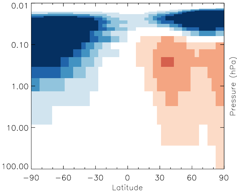
v11-01g-Run0 - v11-01d-Run1 HN03 - Strat zonal mean abs diff for Jan
