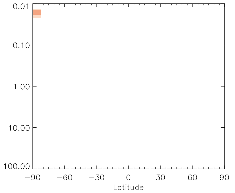
v11-01g-Run0 / v11-01f-geosfp-Run0 DST3 - Strat zonal mean % diff for Jan
