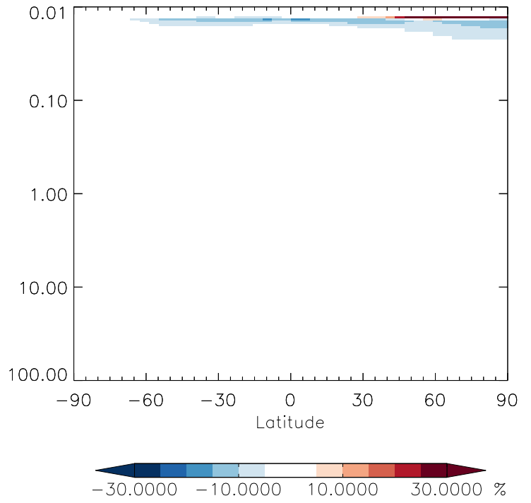
v11-01g-Run0 / v11-01d-Run1 MPN - Strat zonal mean % diff for Jan
