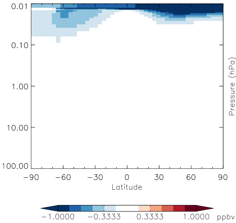
v11-01g-Run0 - v11-01f-geosfp-Run0 NO 2 - Strat zonal mean abs diff for Jan
