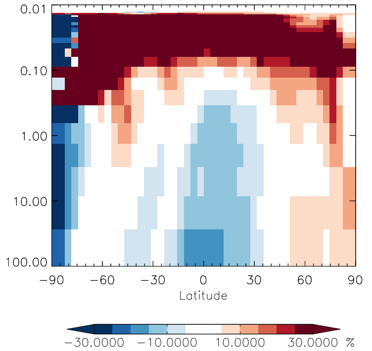
v11-01g-Run0 / v11-01d-Run1 IEPOX - Strat zonal mean % diff for Jan
