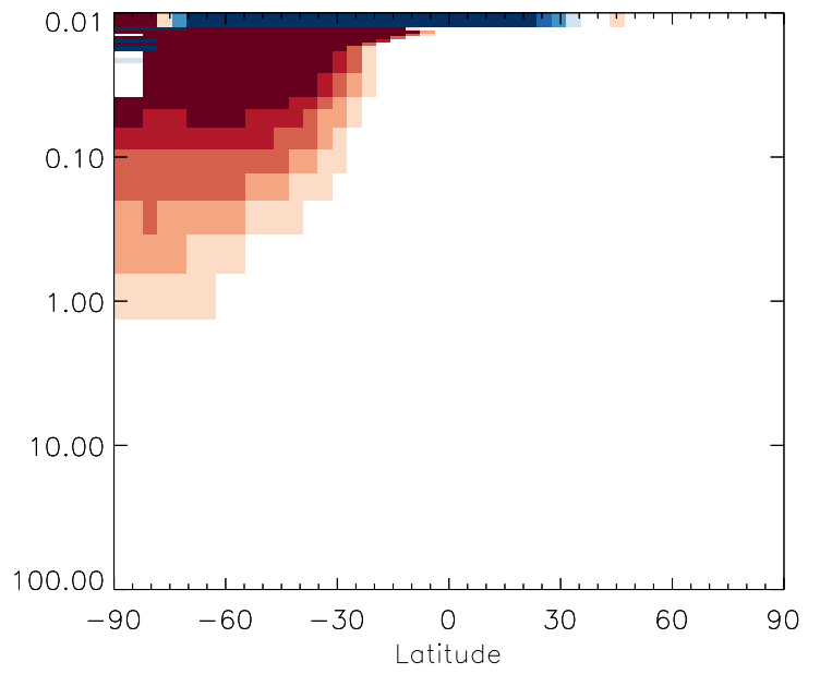
v11-01g-Run0 / v11-01f-geosfp-Run0 ALK4 - Strat zonal mean % diff for Jan
