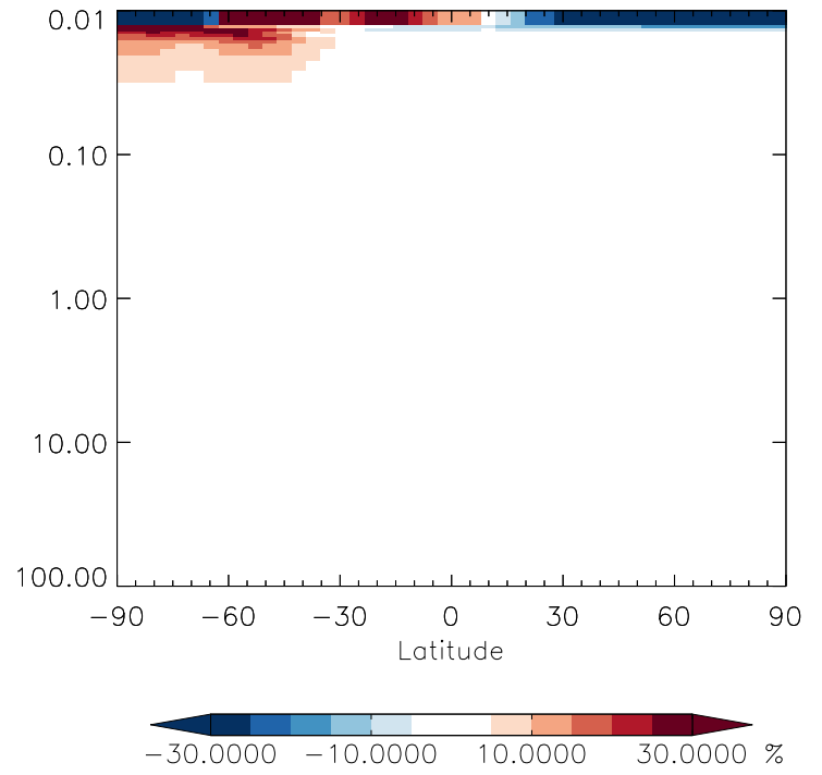
v11-01g-Run0 / v11-01d-Run1 CFC11 - Strat zonal mean % diff for Jan
