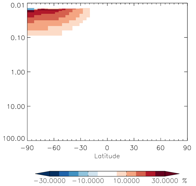
v11-01g-Run0 / v11-01f-geosfp-Run0 CH3Br - Strat zonal mean % diff for Jan
