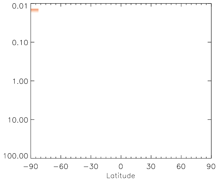
v11-01g-Run0 / v11-01f-geosfp-Run0 DST2 - Strat zonal mean % diff for Jan
