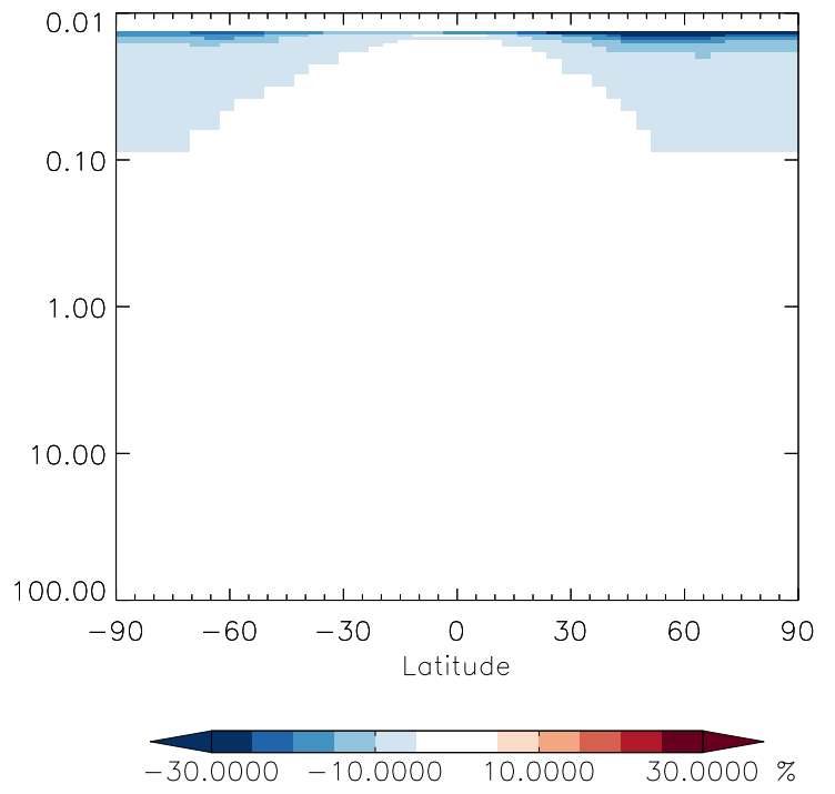
v11-01g-Run0 / v11-01f-geosfp-Run0 BrNO3 - Strat zonal mean % diff for Jan
