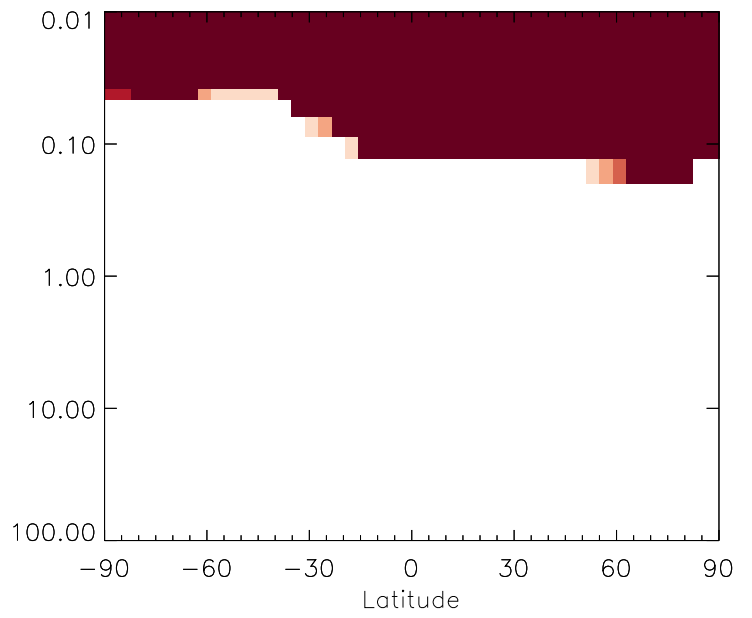
v11-01g-Run0 / v11-01f-geosp-Run0 DST4 - Strat zonal mean % diff for Oct
