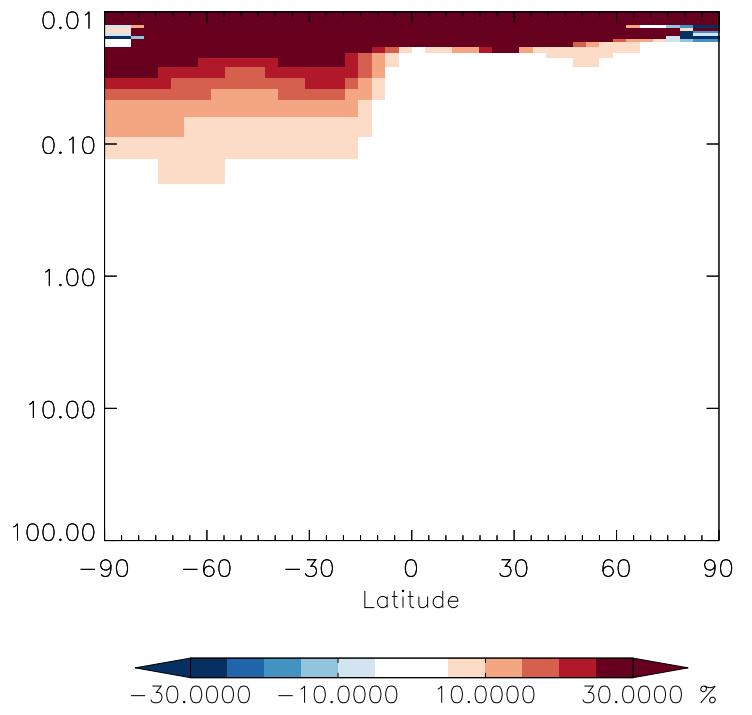
v11-01g-Run0 / v11-01f-geosp-Run0 CHBr3 - Strat zonal mean % diff for Oct
