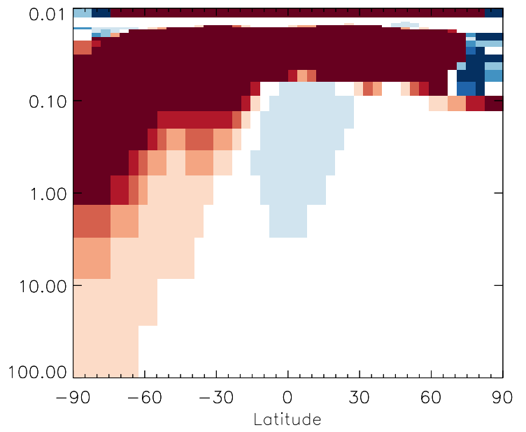
v11-01g-Run0 / v11-01f-geosfp-Run0 GLYC - Strat zonal mean % diff for Oct
