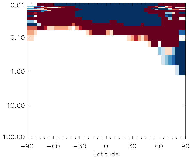
v11-01g-Run0 / v11-01f-geosfp-Run0 BCPO - Strat zonal mean % diff for Oct
