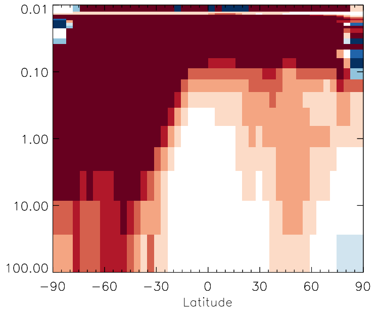
v11-01g-Run0 / v11-01d-Run1 GLYC - Strat zonal mean % diff for Oct
