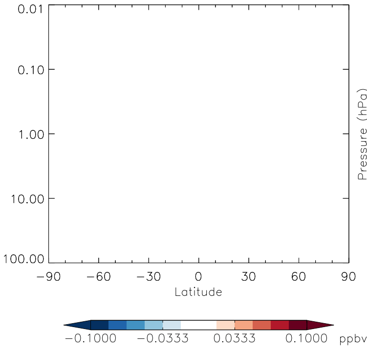
v11-01g-Run0 - v11-01d-Run1 CFC12 - Strat zonal mean abs diff for Oct
