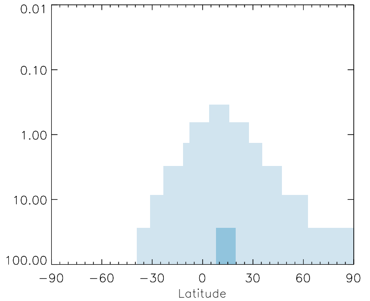
v11-01g-Run0 / v11-01d-Run1 NH4 - Strat zonal mean % diff for Oct
