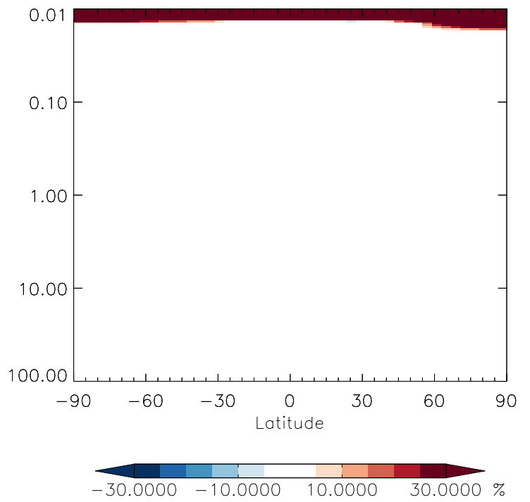
v11-01g-Run0 / v11-01d-Run1 N2O - Strat zonal mean % diff for Oct
