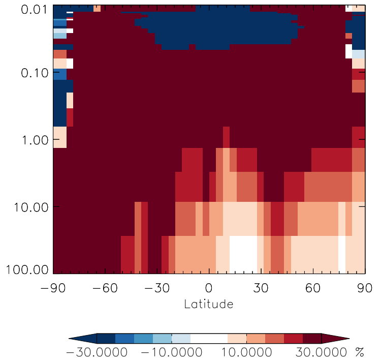
v11-01g-Run0 / v11-01d-Run1 MACR - Strat zonal mean % diff for Oct
