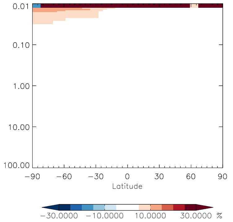
v11-01g-Run0 / v11-01f-geosfp-Run0 CH 3 CCl 3 - Strat zonal mean % diff for Oct
