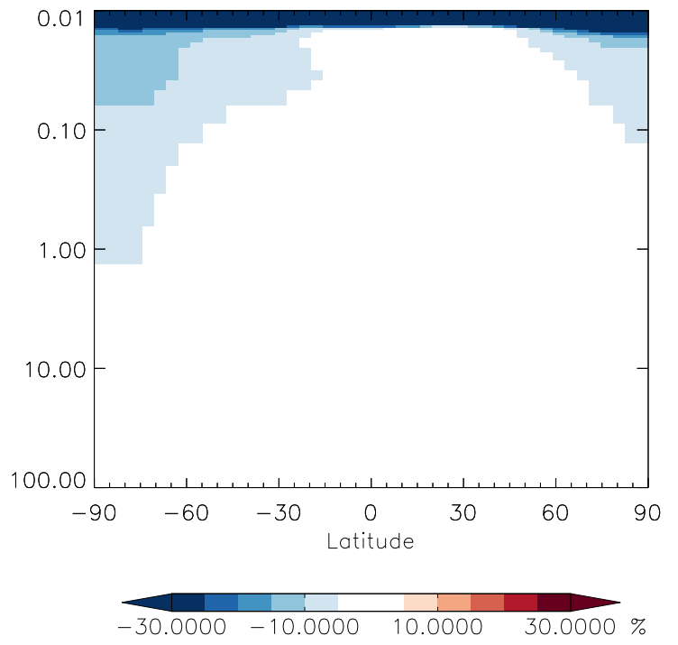
v11-01g-Run0 / v11-01f-geosfp-Run0 NO 2 - Strat zonal mean % diff for Oct
