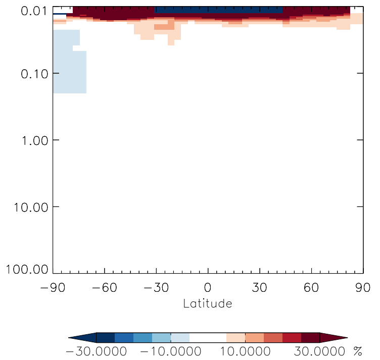
v11-01g-Run0 / v11-01d-Run1 H2402 - Strat zonal mean % diff for Oct
