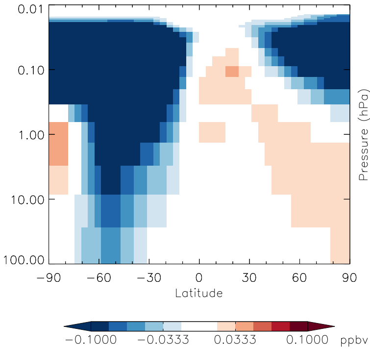
v11-01g-Run0 - v11-01d-Run1 HN03 - Strat zonal mean abs diff for Oct
