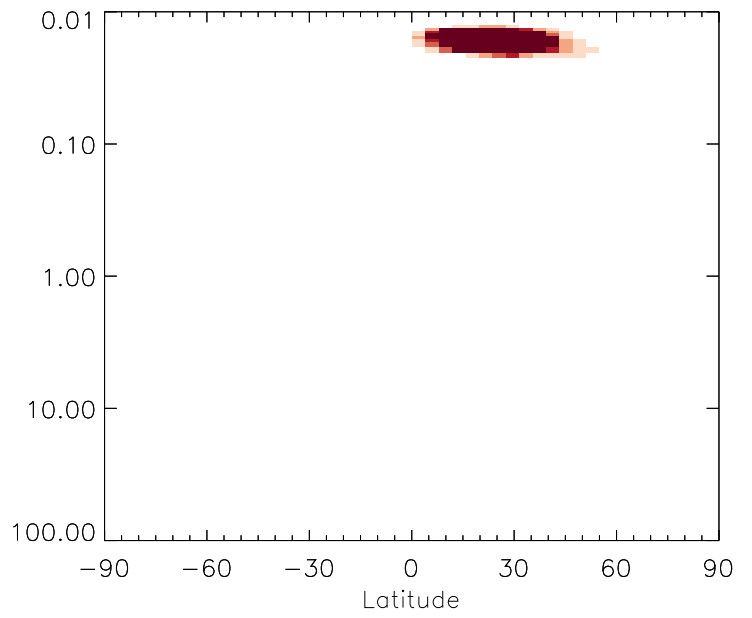
v11-01g-Run0 / v11-01f-geosfp-Run0 DST2 - Strat zonal mean % diff for Oct
