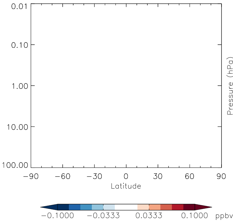
v11-01g-Run0 - v11-01f-geosfp-Run0 CFC11 - Strat zonal mean abs diff for Oct
