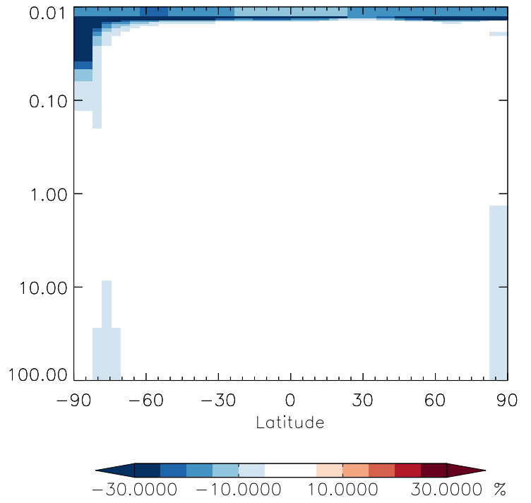
v11-01g-Run0 / v11-01d-Run1 NO3 - Strat zonal mean % diff for Oct
