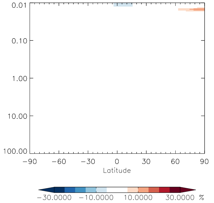
v11-01g-Run0 / v11-01d-Run1 CH3Cl - Strat zonal mean % diff for Oct
