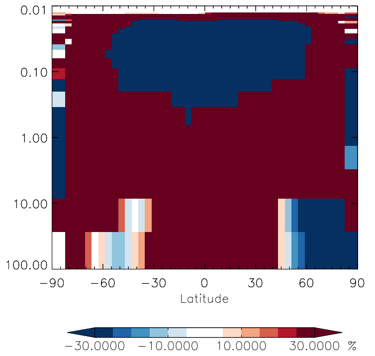
v11-01g-Run0 / v11-01f-geosfp-Run0 ISOPNB - Strat zonal mean % diff for Oct
