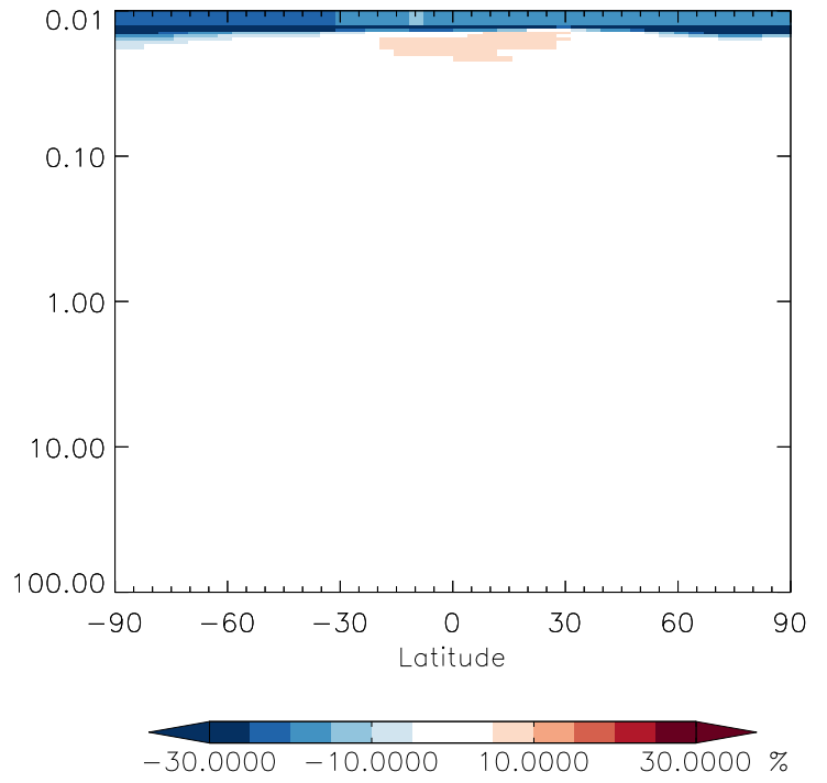
v11-01g-Run0 / v11-01d-Run1 ClNO 3 - Strat zonal mean % diff for Oct
