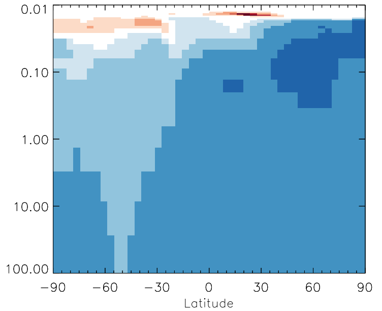
v11-01g-Run0 / v11-01d-Run1 DST1 - Strat zonal mean % diff for Oct
