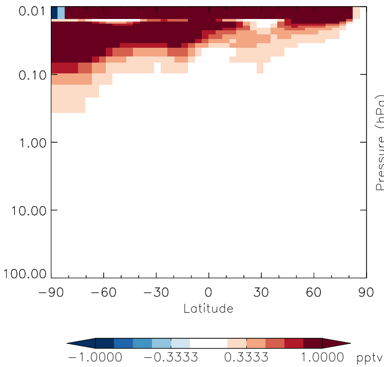
v11-01g-Run0 - v11-01d-Run1 HO2 - Strat zonal mean abs diff for Oct
