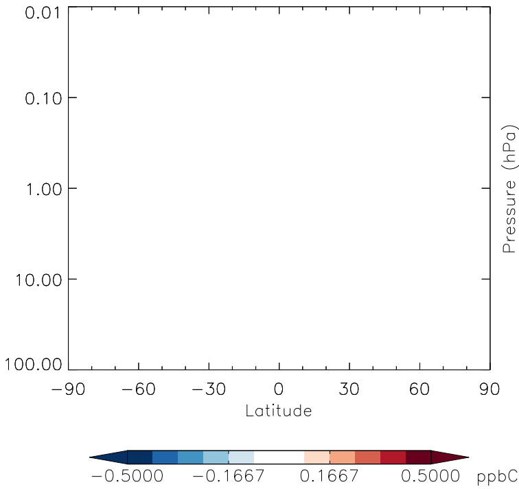
v11-01g-Run0 - v11-01d-Run1 C3H8 - Strat zonal mean abs diff for Oct
