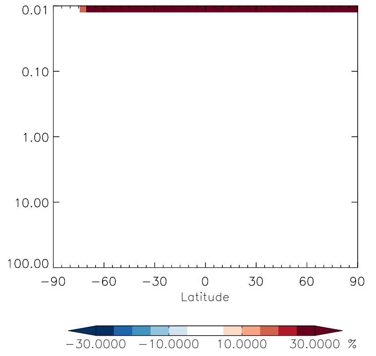
v11-01g-Run0 / v11-01f-geosfp-Run0 CFC11 - Strat zonal mean % diff for Oct
