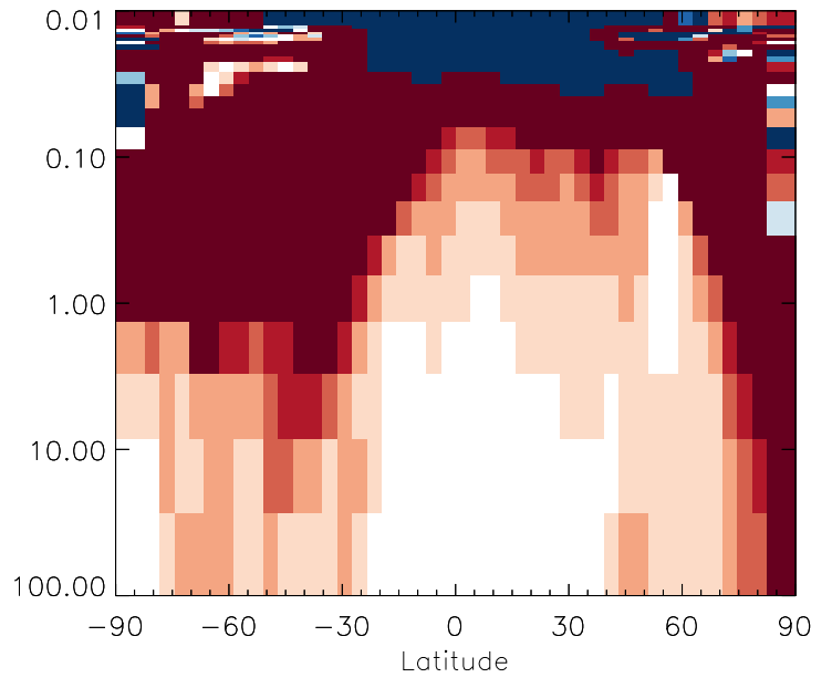
v11-01g-Run0 / v11-01d-Run1 OCPO - Strat zonal mean % diff for Oct
