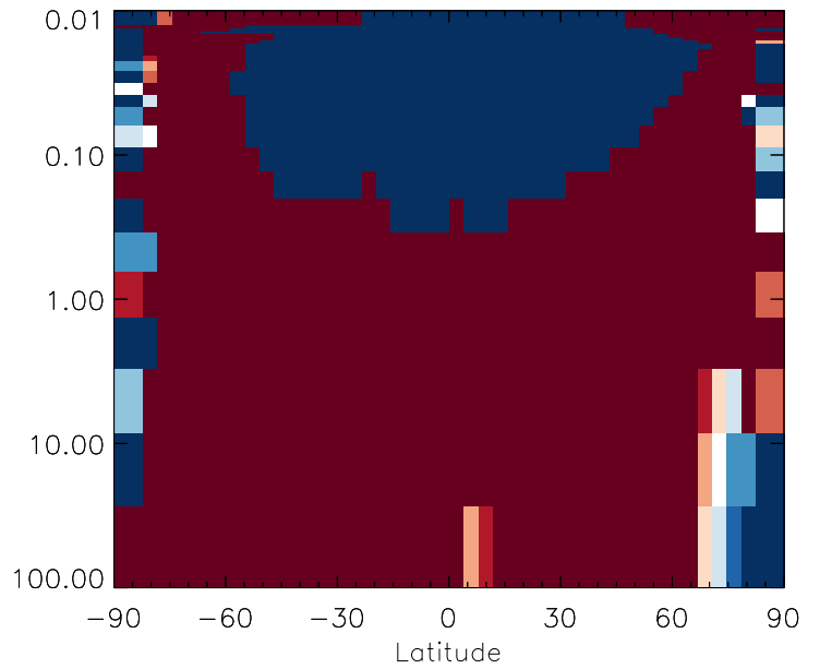
v11-01g-Run0 / v11-01d-Run1 ISOP - Strat zonal mean % diff for Oct
