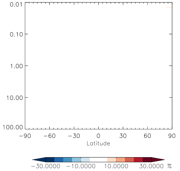
v11-01g-Run0 / v11-01f-geosp-Run0 O3 - Strat zonal mean % diff for Oct
