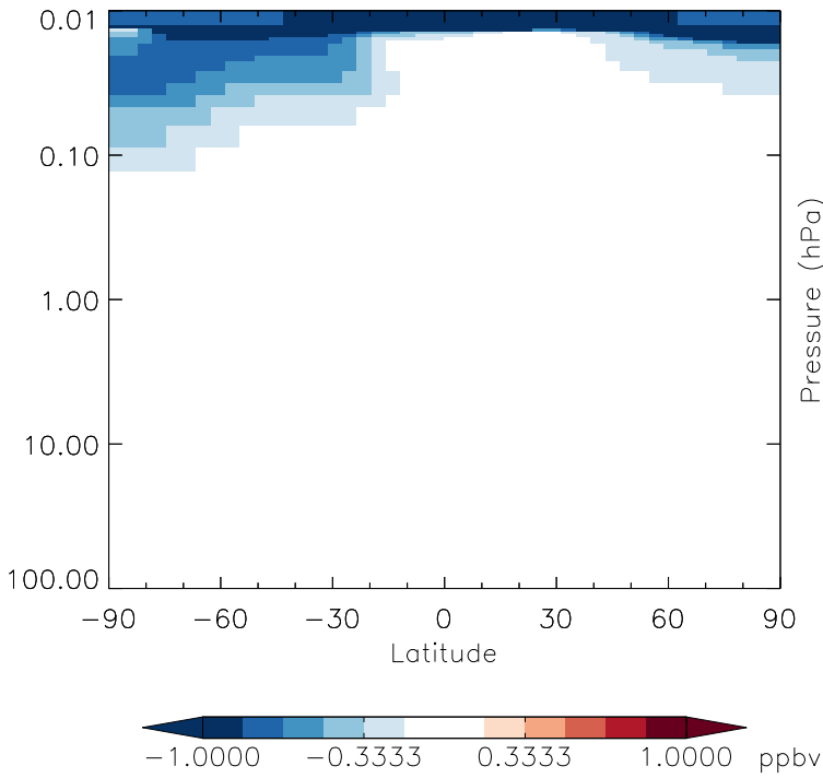
v11-01g-Run0 - v11-01d-Run1 NO 2 - Strat zonal mean abs diff for Oct
