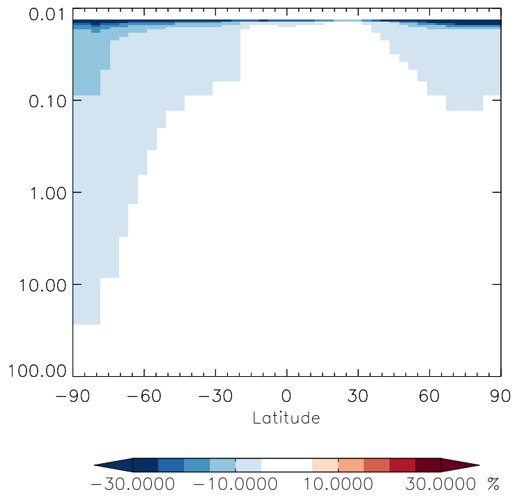
v11-01g-Run0 / v11-01f-geosfp-Run0 BrNO3 - Strat zonal mean % diff for Oct
