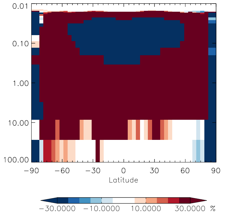
v11-01g-Run0 / v11-01f-geosfp-Run0 MOBA - Strat zonal mean % diff for Oct
