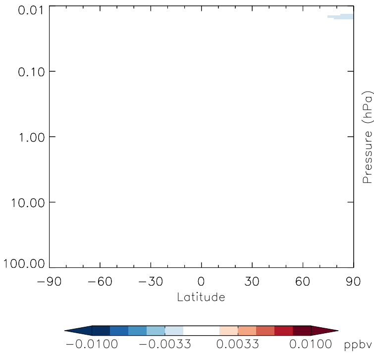
v11-01g-Run0 - v11-01f-geosfp-Run0 BrNO3 - Strat zonal mean abs diff for Oct
