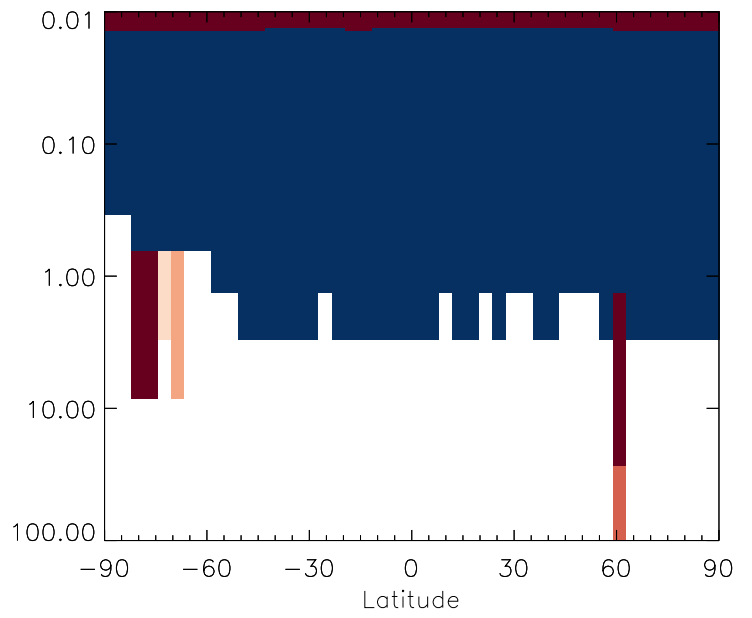
v11-01g-Run0 / v11-01f-geosfp-Run0 SO4s - Strat zonal mean % diff for Oct
