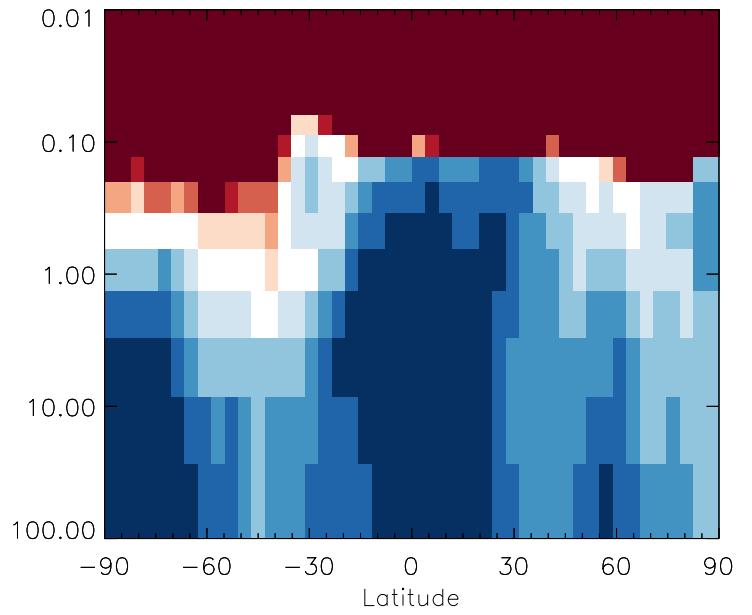
v11-01g-Run0 / v11-01d-Run1 DST4 - Strat zonal mean % diff for Oct
