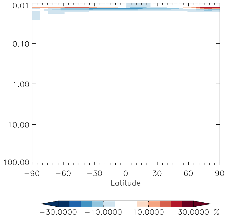
v11-01g-Run0 / v11-01d-Run1 MPN - Strat zonal mean % diff for Oct
