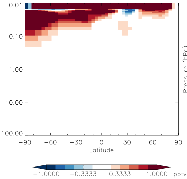
v11-01g-Run0 - v11-01f-geosfp-Run0 HO2 - Strat zonal mean abs diff for Oct
