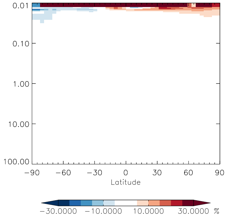
v11-01g-Run0 / v11-01d-Run1 CH 3 CCl 3 - Strat zonal mean % diff for Oct
