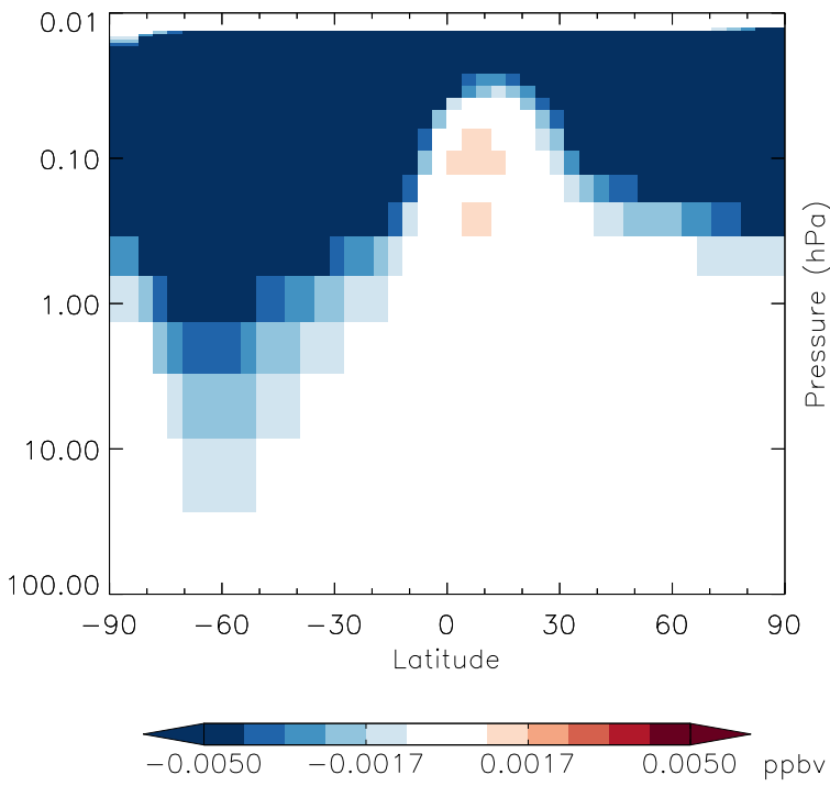
v11-01g-Run0 - v11-01f-geosfp-Run0 N2O5 - Strat zonal mean abs diff for Oct
