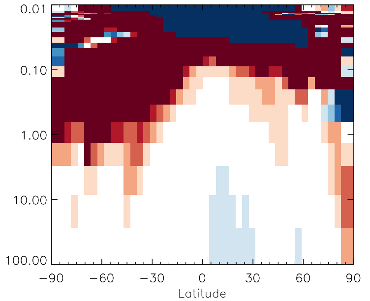
v11-01g-Run0 / v11-01d-Run1 BCPO - Strat zonal mean % diff for Oct
