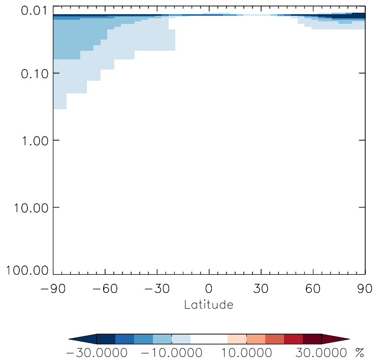
v11-01g-Run0 / v11-01f-geosfp-Run0 HN03 - Strat zonal mean % diff for Oct
