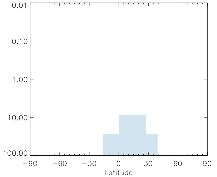
v11-01g-Run0 / v11-01d-Run1 OCPI - Strat zonal mean % diff for Oct
