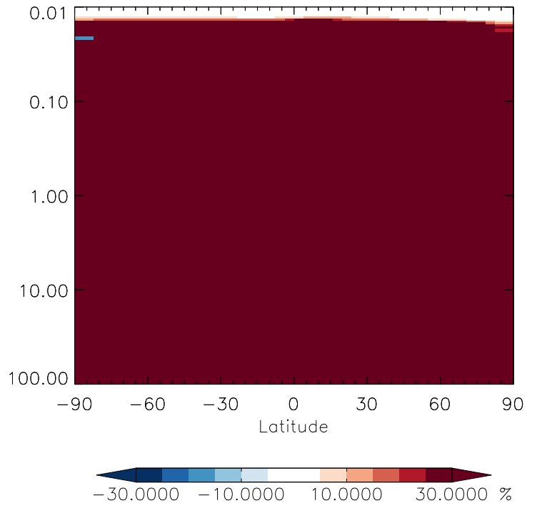
v11-01g-Run0 / v11-01d-Run1 MVKN - Strat zonal mean % diff for Oct
