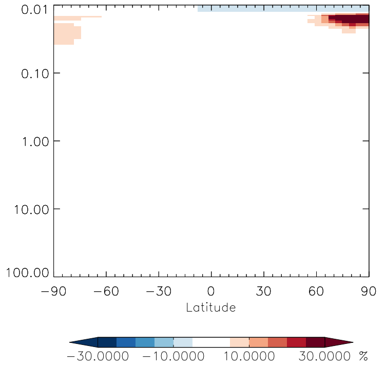
v11-01g-Run0 / v11-01d-Run1 C2H6 - Strat zonal mean % diff for Oct
