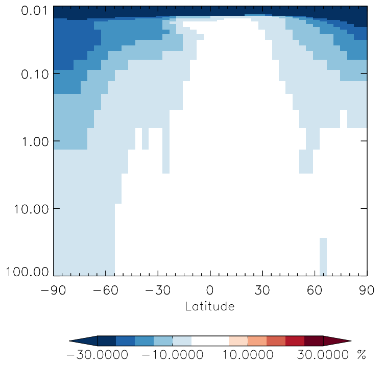
v11-01g-Run0 / v11-01f-geosfp-Run0 BrNO 2 - Strat zonal mean % diff for Oct
