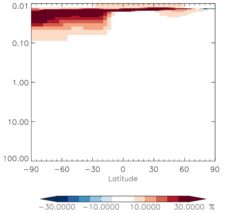
v11-01g-Run0 / v11-01f-geosfp-Run0 CH 2 Br 2 - Strat zonal mean % diff for Oct
