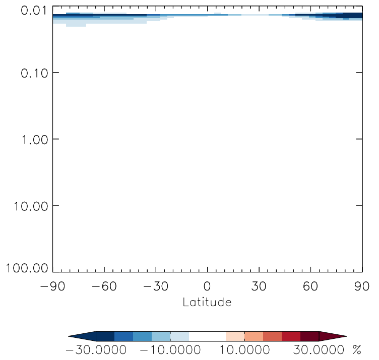
v11-01g-Run0 / v11-01f-geosfp-Run0 HN04 - Strat zonal mean % diff for Oct
