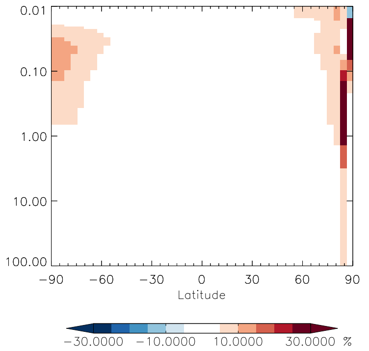
v11-01g-Run0 / v11-01d-Run1 HO2 - Strat zonal mean % diff for Oct
