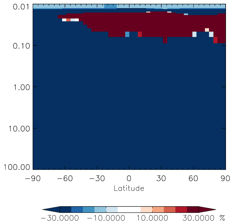
v11-01g-Run0 / v11-01d-Run1 MACRN - Strat zonal mean % diff for Oct
