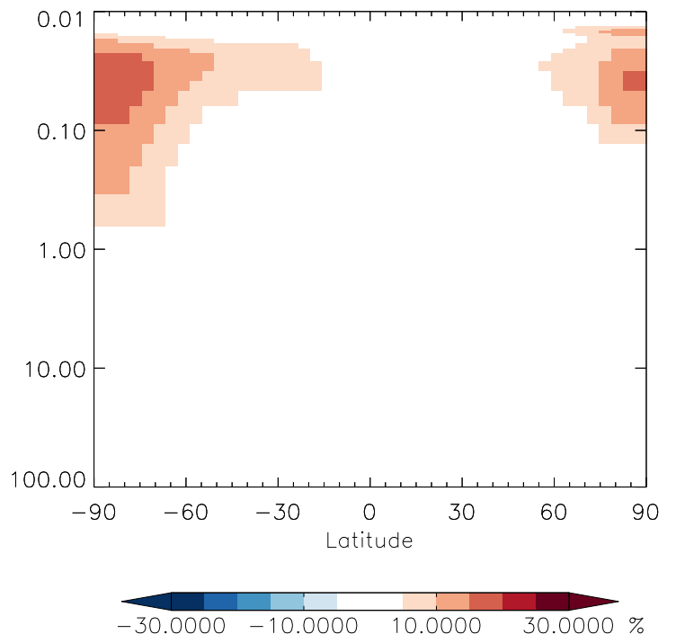
v11-01g-Run0 / v11-01d-Run1 H2O2 - Strat zonal mean % diff for Oct
