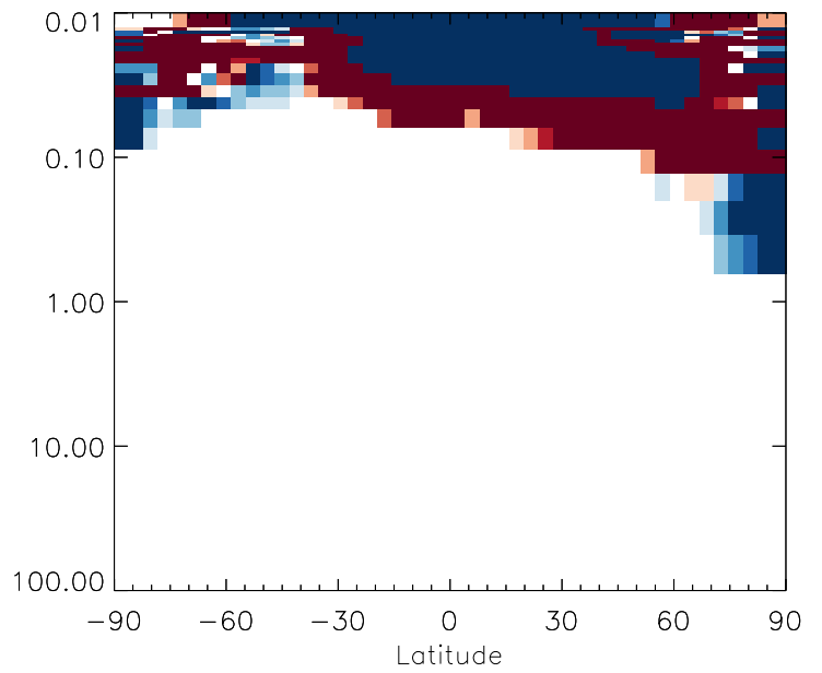
v11-01g-Run0 / v11-01f-geosfp-Run0 OCPO - Strat zonal mean % diff for Oct
