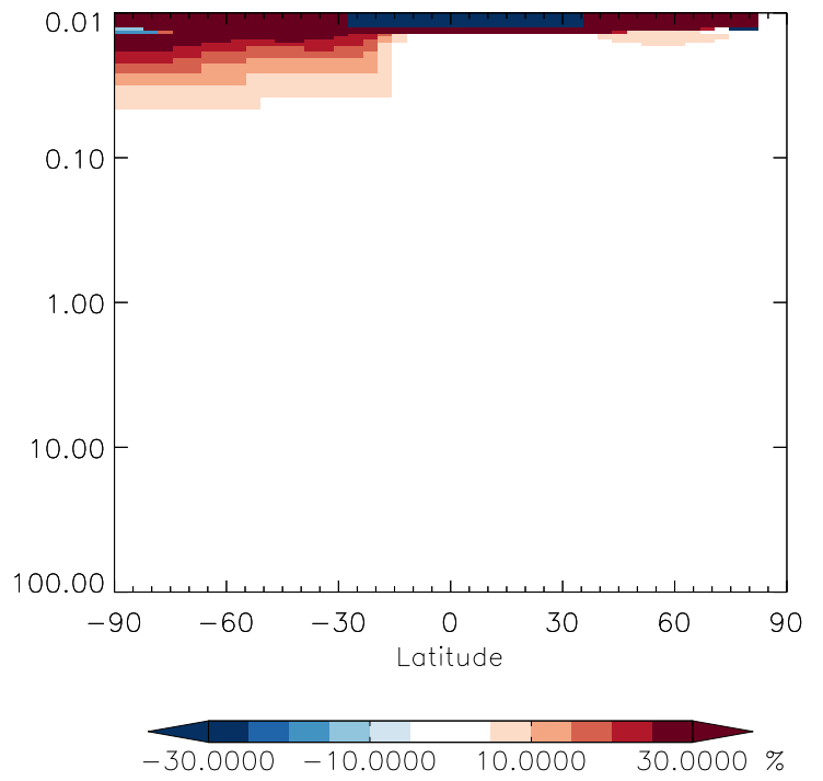
v11-01g-Run0 / v11-01f-geosfp-Run0 H2402 - Strat zonal mean % diff for Oct
