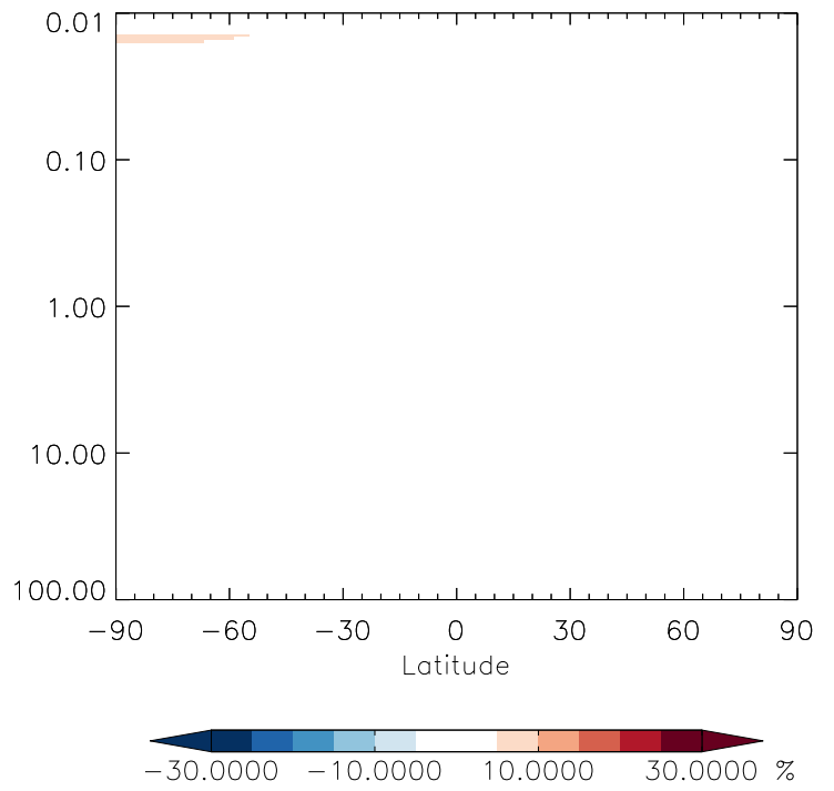
v11-01g-Run0 / v11-01f-geosfp-Run0 H1301 - Strat zonal mean % diff for Oct
