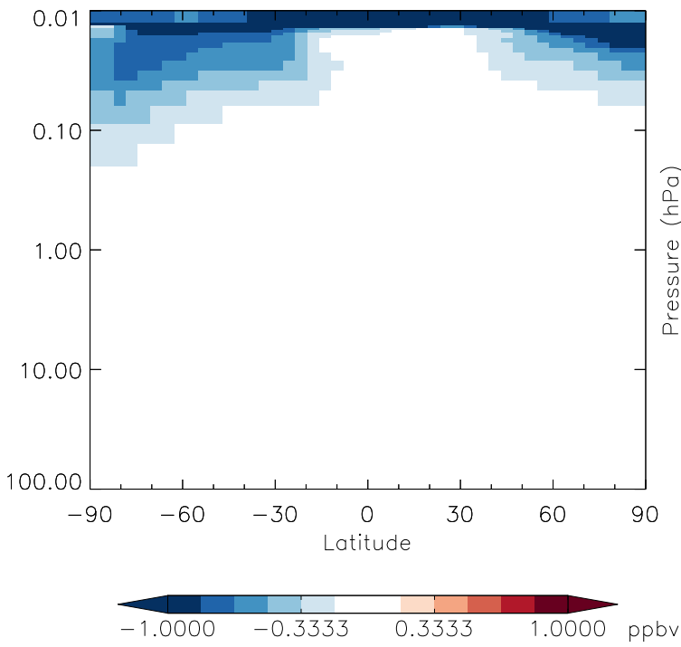
v11-01g-Run0 - v11-01f-geosfp-Run0 NO 2 - Strat zonal mean abs diff for Oct
