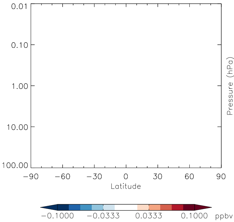
v11-01g-Run0 - v11-01f-geosfp-Run0 H2O2 - Strat zonal mean abs diff for Oct
