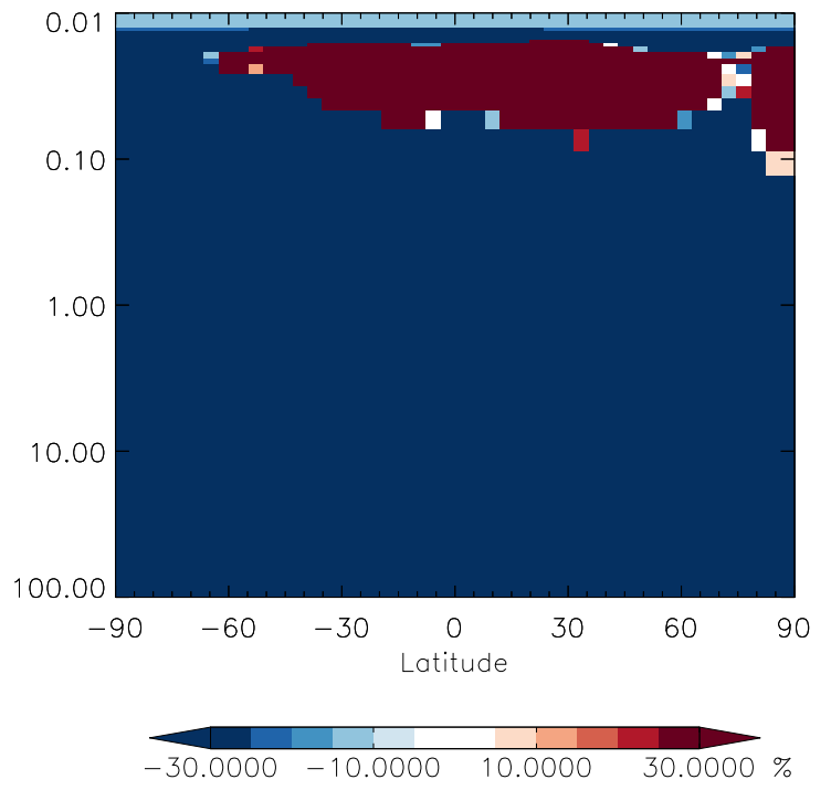
v11-01g-Run0 / v11-01f-geosfp-Run0 MACRN - Strat zonal mean % diff for Oct
