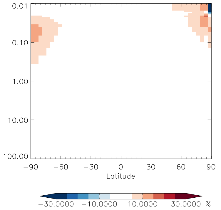
v11-01g-Run0 / v11-01f-geosfp-Run0 HO2 - Strat zonal mean % diff for Oct
