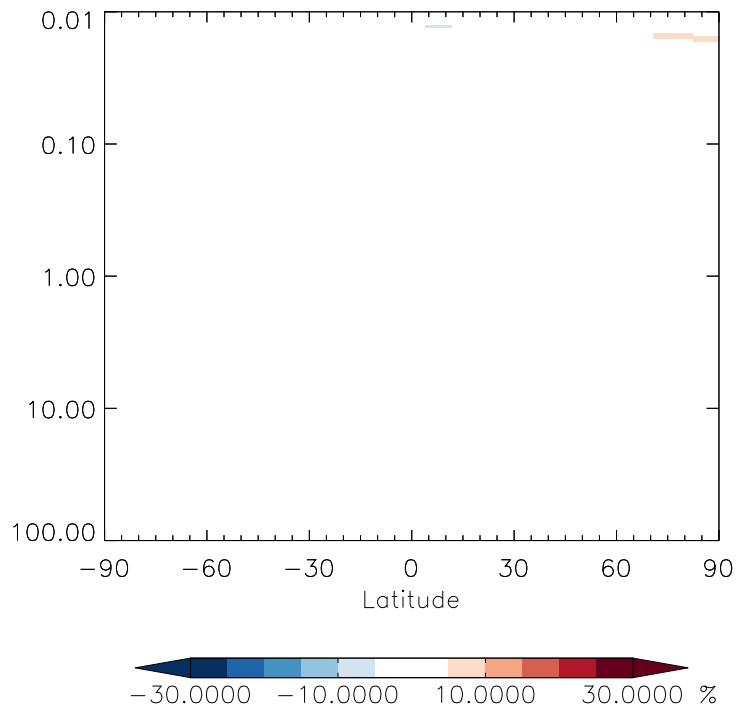
v11-01g-Run0 / v11-01f-geosfp-Run0 ALD2 - Strat zonal mean % diff for Oct
