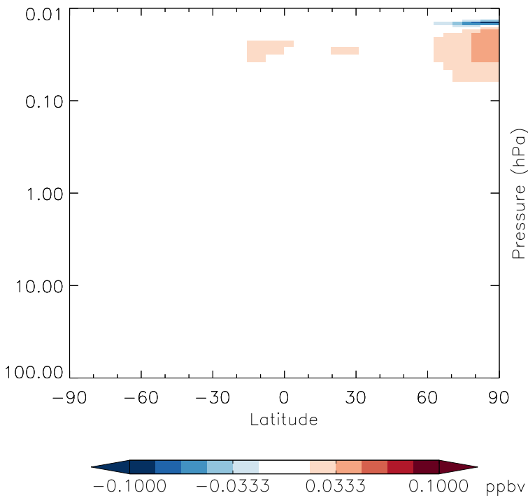
v11-01g-Run0 - v11-01f-geosfp-Run0 ClNO 3 - Strat zonal mean abs diff for Oct
