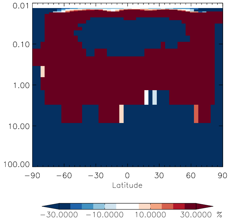
v11-01g-Run0 / v11-01d-Run1 MOBA - Strat zonal mean % diff for Oct
