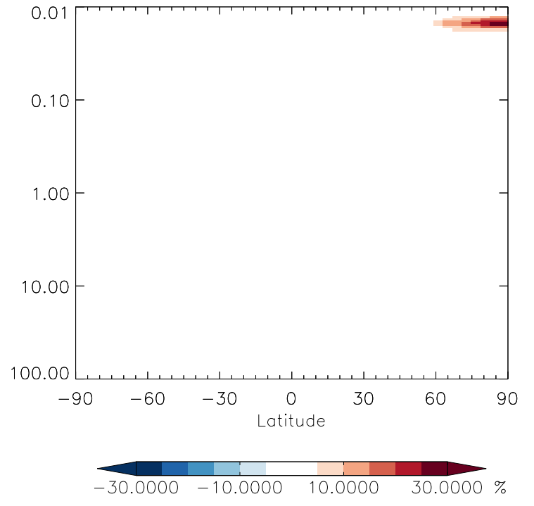
v11-01g-Run0 / v11-01d-Run1 CFC12 - Strat zonal mean % diff for Oct
