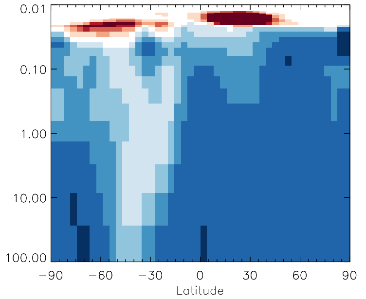
v11-01g-Run0 / v11-01d-Run1 DST2 - Strat zonal mean % diff for Oct
