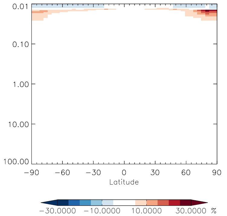
v11-01g-Run0 / v11-01d-Run1 H1301 - Strat zonal mean % diff for Oct
