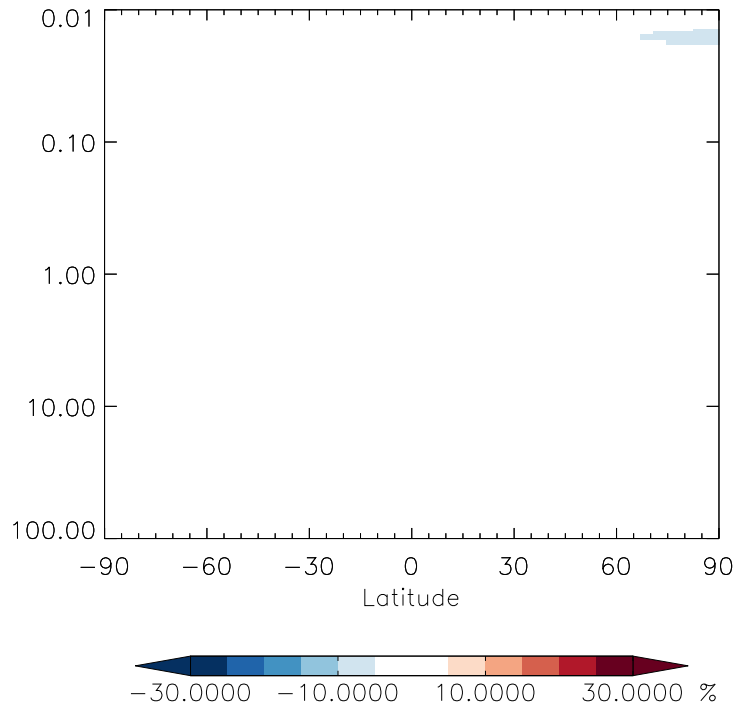
v11-01g-Run0 / v11-01d-Run1 CH2O - Strat zonal mean % diff for Oct
