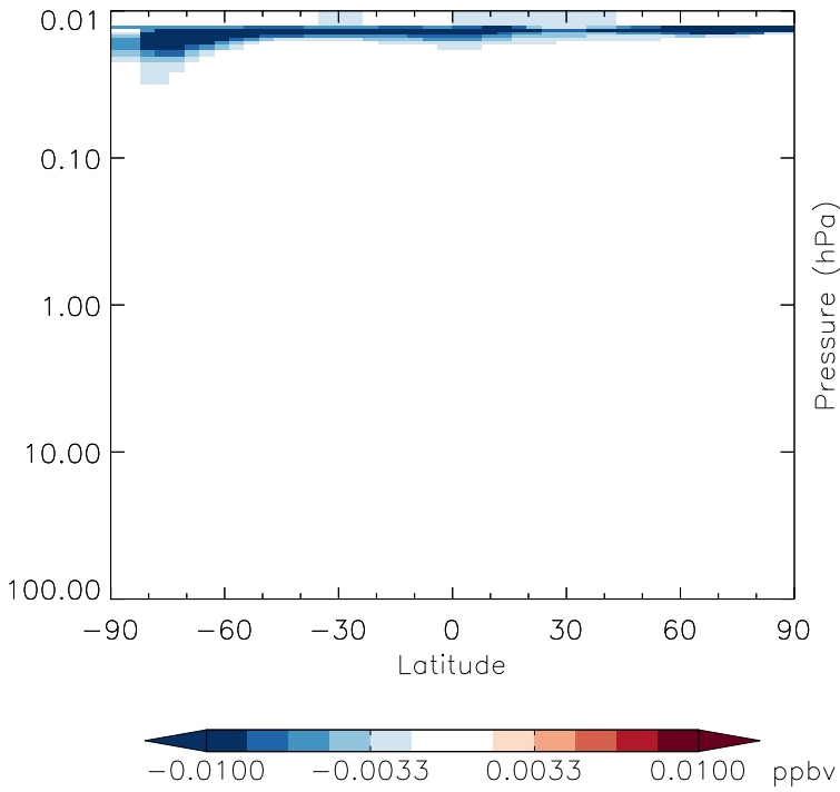
v11-01g-Run0 - v11-01d-Run1 NO3 - Strat zonal mean abs diff for Oct
