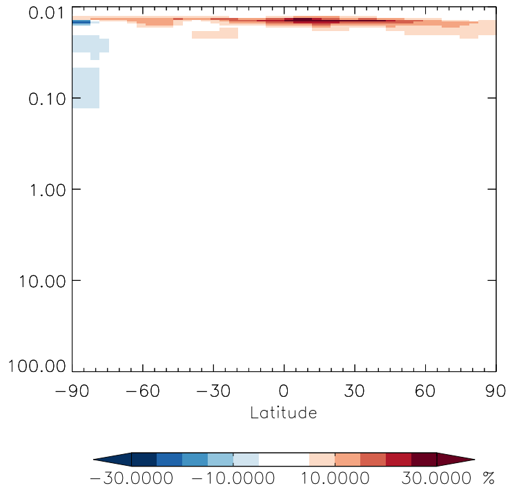
v11-01g-Run0 / v11-01d-Run1 CH3Br - Strat zonal mean % diff for Oct
