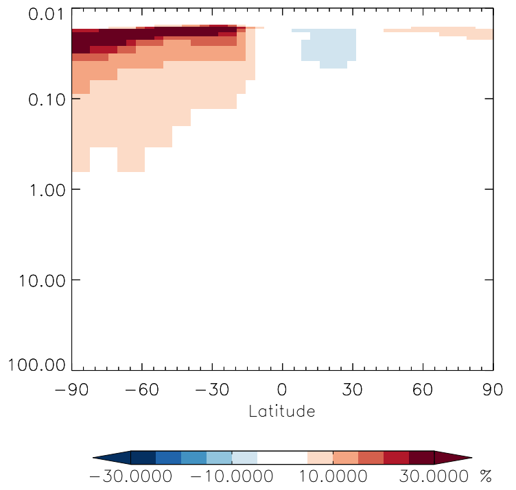
v11-01g-Run0 / v11-01f-geosfp-Run0 MEK - Strat zonal mean % diff for Oct
