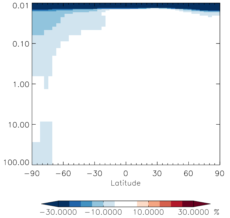
v11-01g-Run0 / v11-01d-Run1 NO 2 - Strat zonal mean % diff for Oct
