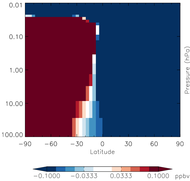
v11-01g-Run0 - v11-01f-geosfp-Run0 CH4 - Strat zonal mean abs diff for Oct
