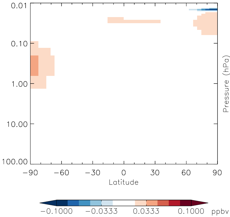
v11-01g-Run0 - v11-01d-Run1 ClNO 3 - Strat zonal mean abs diff for Oct
