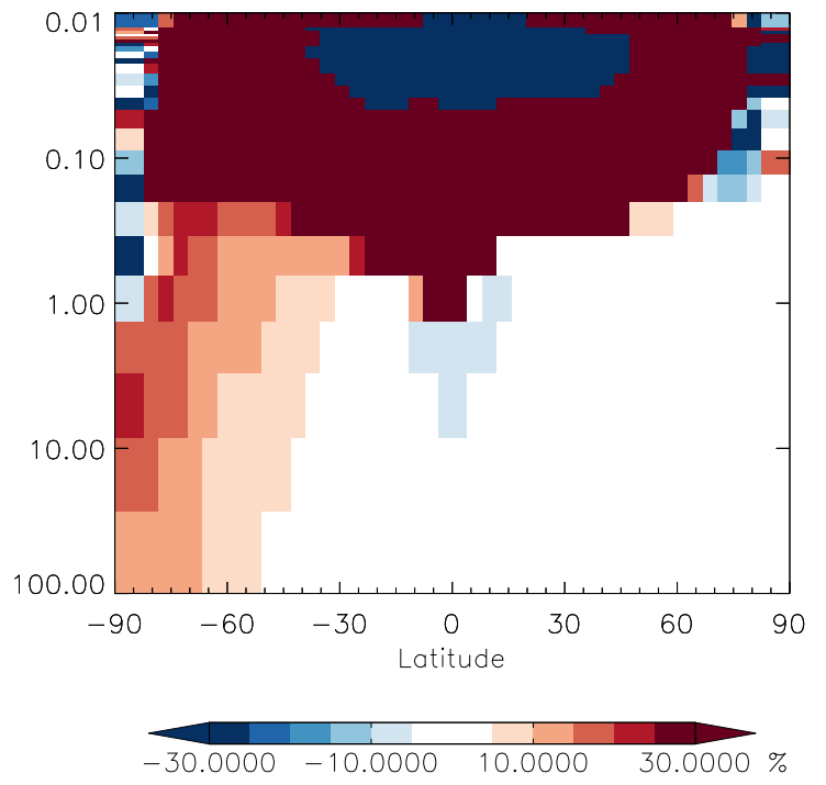
v11-01g-Run0 / v11-01f-geosfp-Run0 MACR - Strat zonal mean % diff for Oct
