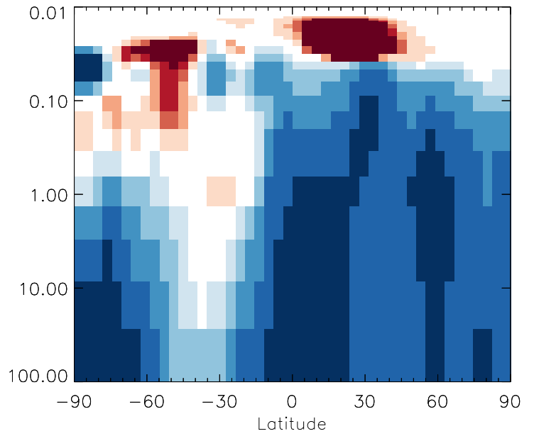
v11-01g-Run0 / v11-01d-Run1 DST3 - Strat zonal mean % diff for Oct
