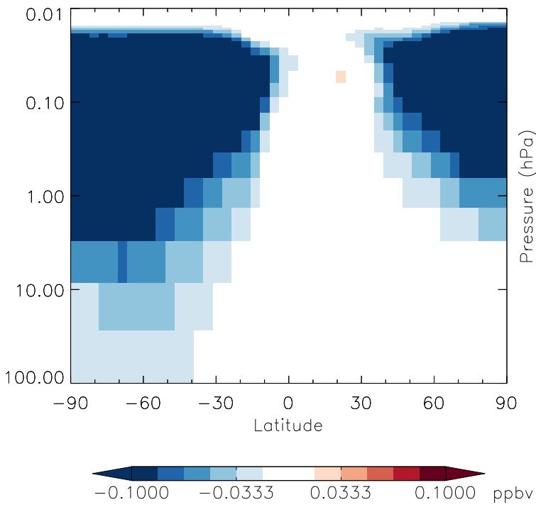
v11-01g-Run0 - v11-01f-geosfp-Run0 HN03 - Strat zonal mean abs diff for Oct
