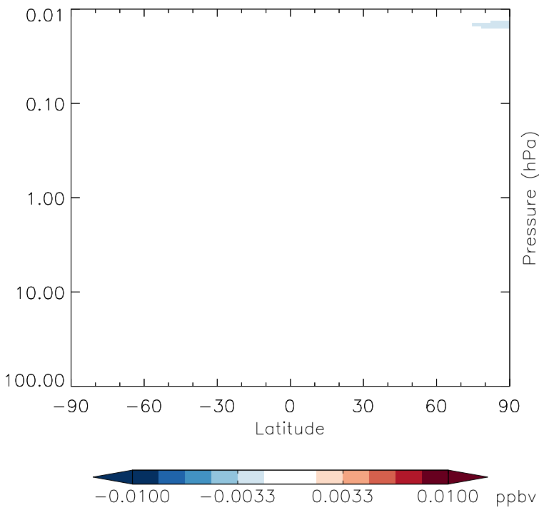
v11-01g-Run0 - v11-01d-Run1 BrNO3 - Strat zonal mean abs diff for Oct
