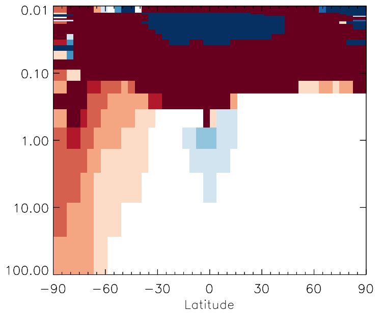
v11-01g-Run0 / v11-01f-geosfp-Run0 PRPE - Strat zonal mean % diff for Oct
