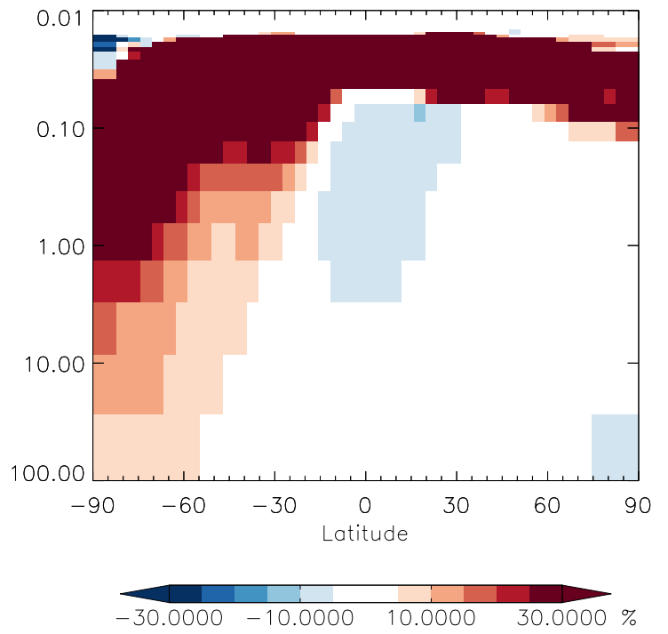
v11-01g-Run0 / v11-01f-geosfp-Run0 IEPOX - Strat zonal mean % diff for Oct
