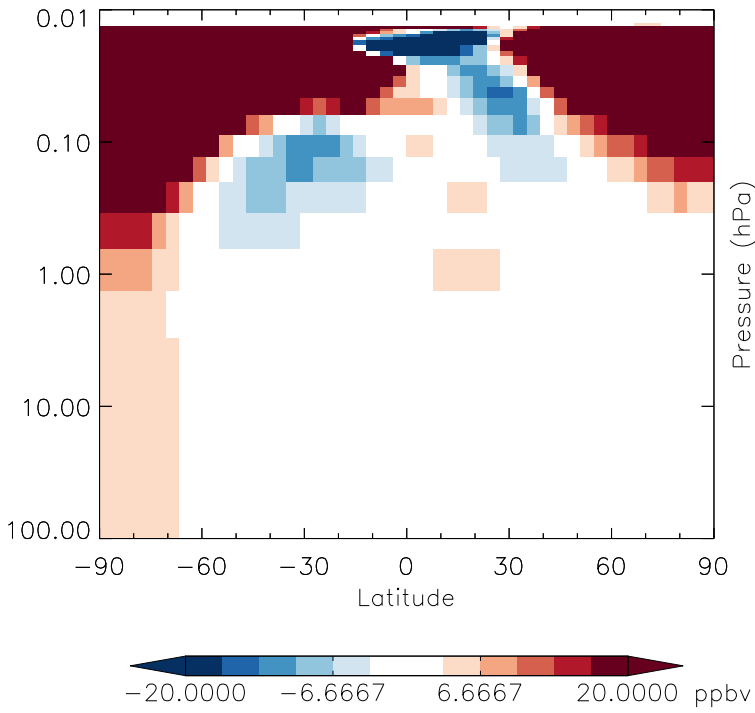
v11-01g-Run0 - v11-01f-geosp-Run0 O3 - Strat zonal mean abs diff for Oct
