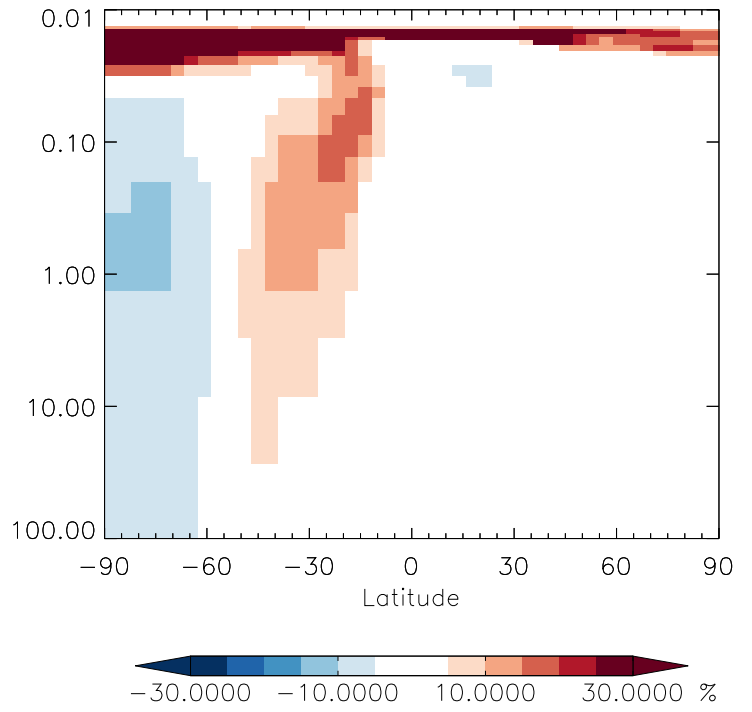
v11-01g-Run0 / v11-01d-Run1 R4N2 - Strat zonal mean % diff for Oct
