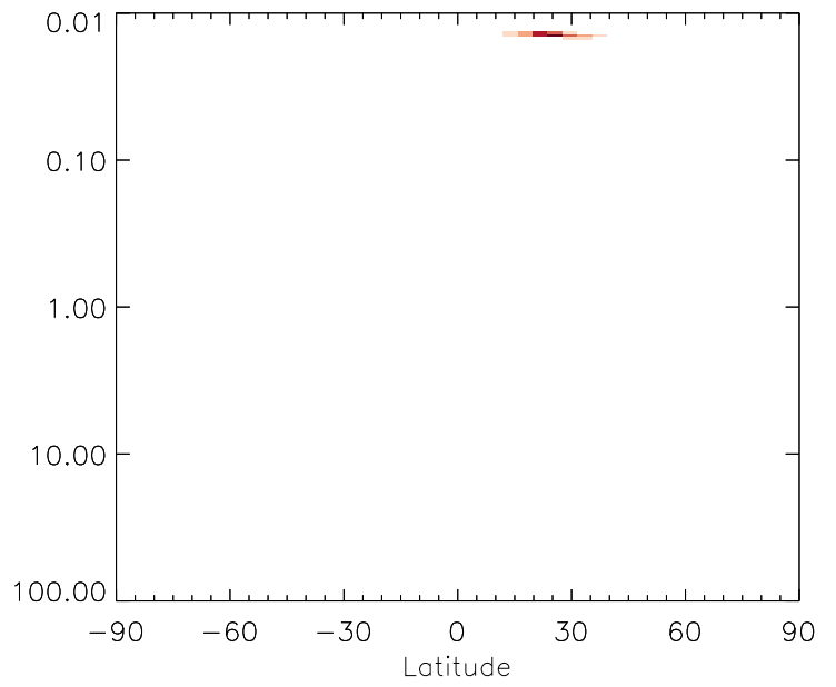
v11-01g-Run0 / v11-01f-geosfp-Run0 DST1 - Strat zonal mean % diff for Oct
