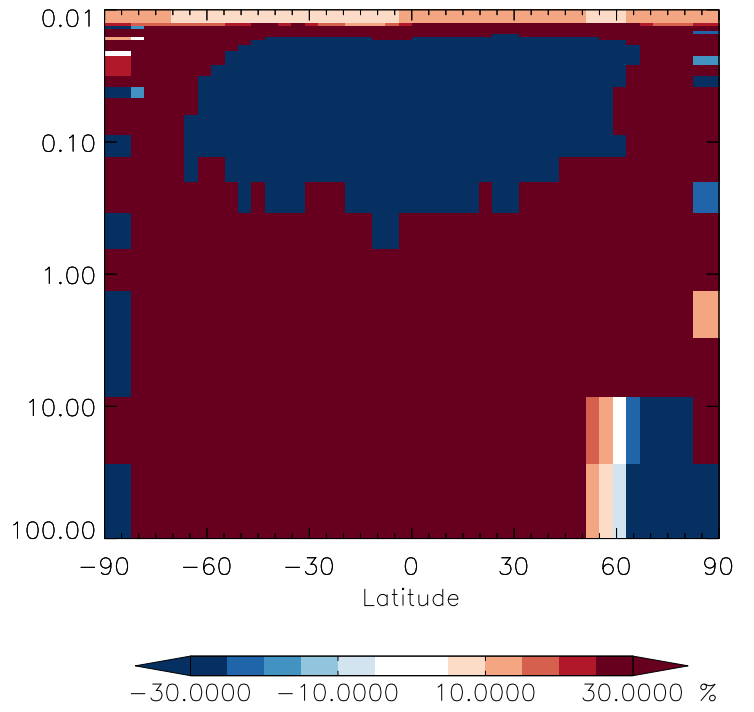
v11-01g-Run0 / v11-01d-Run1 ISOPNB - Strat zonal mean % diff for Oct
