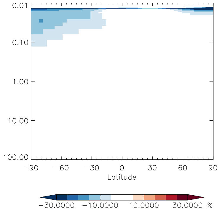
v11-01g-Run0 / v11-01d-Run1 HN03 - Strat zonal mean % diff for Oct
