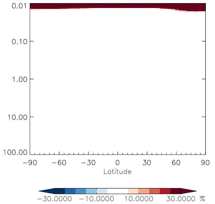
v11-01g-Run0 / v11-01f-geosp-Run0 N2O - Strat zonal mean % diff for Oct
