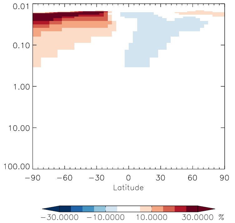
v11-01g-Run0 / v11-01f-geosfp-Run0 RCHO - Strat zonal mean % diff for Oct
