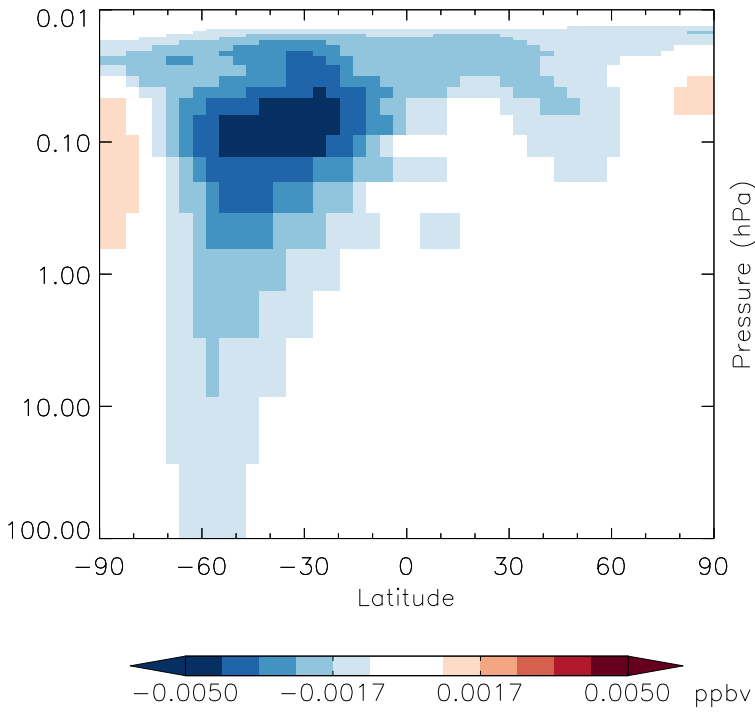
v11-01g-Run0 - v11-01d-Run1 HN04 - Strat zonal mean abs diff for Oct
