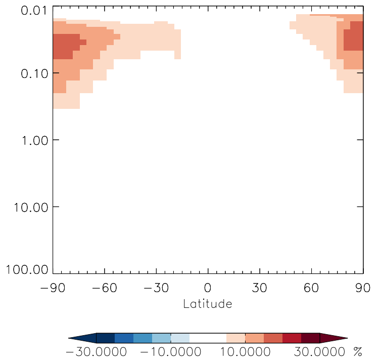
v11-01g-Run0 / v11-01f-geosfp-Run0 H2O2 - Strat zonal mean % diff for Oct
