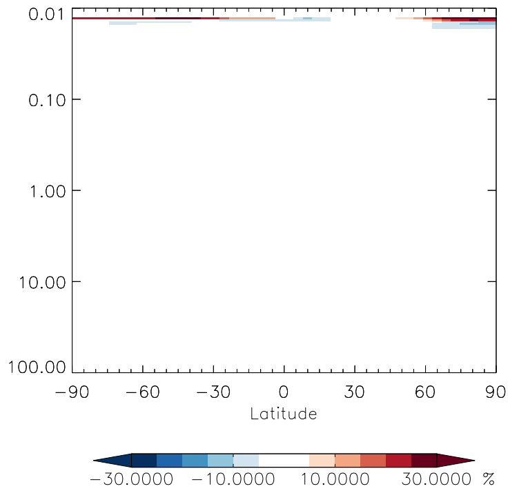
v11-01g-Run0 / v11-01f-geosfp-Run0 MPN - Strat zonal mean % diff for Oct
