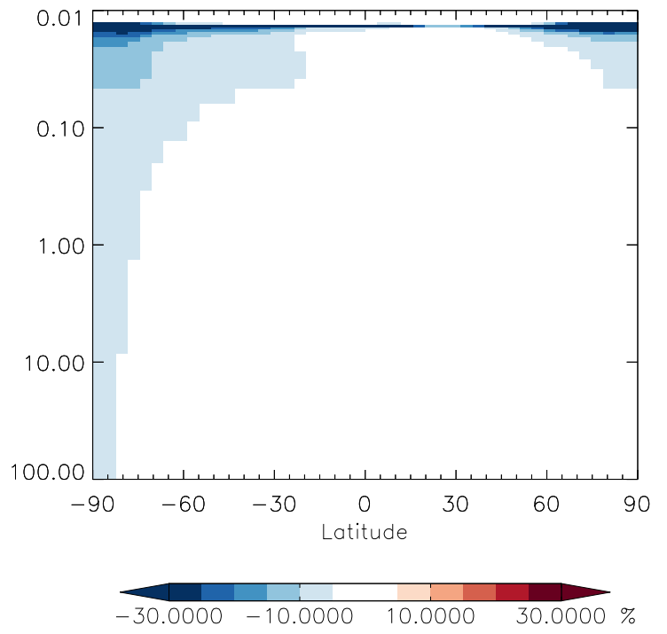
v11-01g-Run0 / v11-01f-geosfp-Run0 N2O5 - Strat zonal mean % diff for Oct
