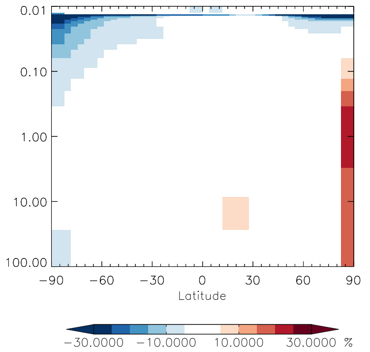
v11-01g-Run0 / v11-01d-Run1 BrNO3 - Strat zonal mean % diff for Oct
