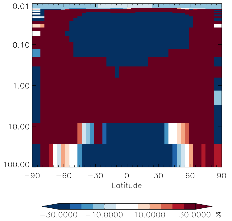
v11-01g-Run0 / v11-01f-geosfp-Run0 ISOPND - Strat zonal mean % diff for Oct
