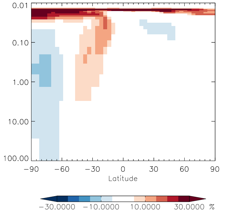
v11-01g-Run0 / v11-01d-Run1 RCHO - Strat zonal mean % diff for Oct
