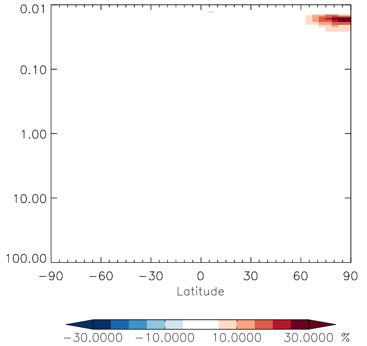
v11-01g-Run0 / v11-01d-Run1 ALD2 - Strat zonal mean % diff for Oct
