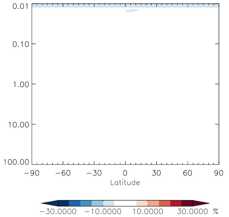
v11-01g-Run0 / v11-01f-geosfp-Run0 C2H6 - Strat zonal mean % diff for Oct
