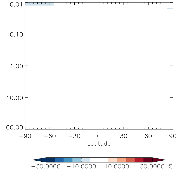
v11-01g-Run0 / v11-01d-Run1 CH4 - Strat zonal mean % diff for Oct
