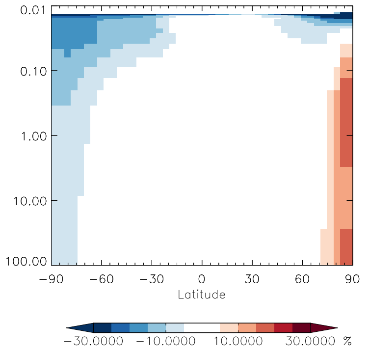
v11-01g-Run0 / v11-01f-geosfp-Run0 HN02 - Strat zonal mean % diff for Oct
