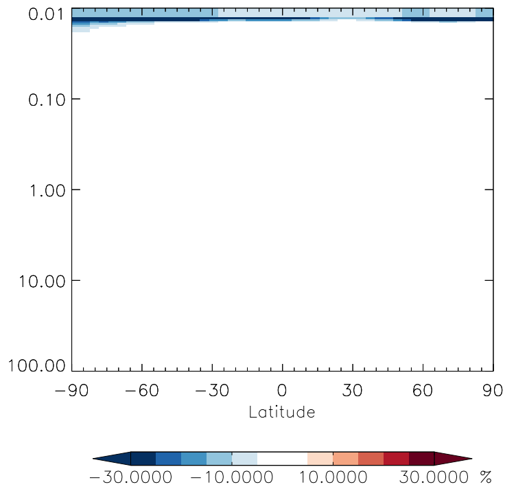
v11-01g-Run0 / v11-01f-geosfp-Run0 NO3 - Strat zonal mean % diff for Oct
