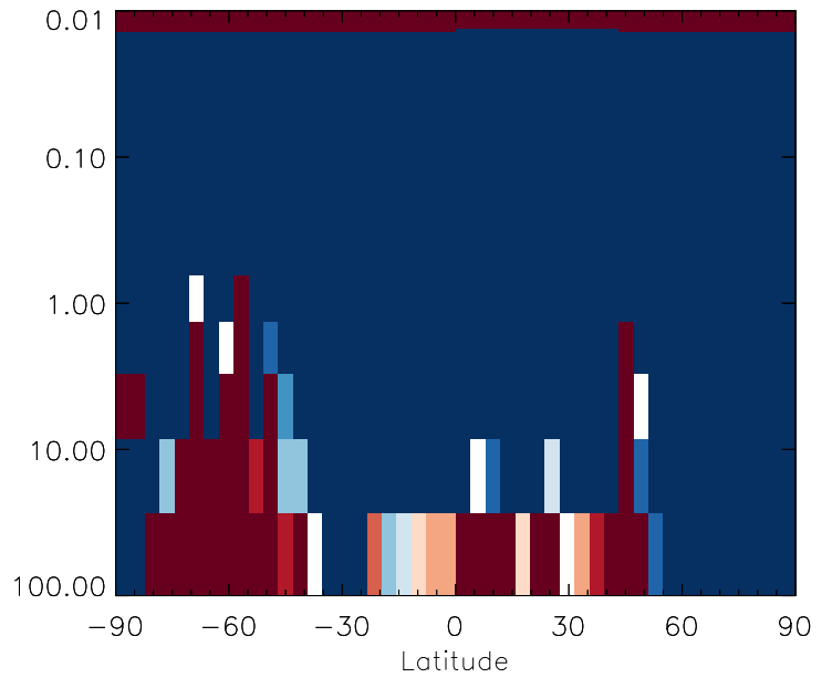
v11-01g-Run0 / v11-01d-Run1 SO4s - Strat zonal mean % diff for Oct
