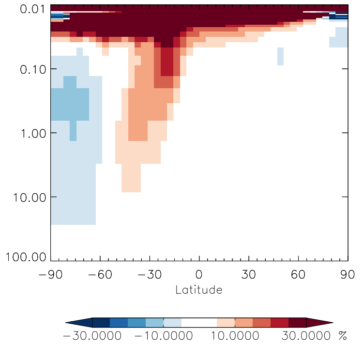
v11-01g-Run0 / v11-01d-Run1 CHBr3 - Strat zonal mean % diff for Oct
