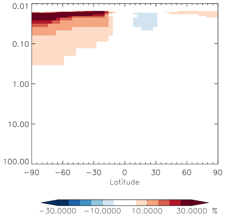
v11-01g-Run0 / v11-01f-geosfp-Run0 R4N2 - Strat zonal mean % diff for Oct
