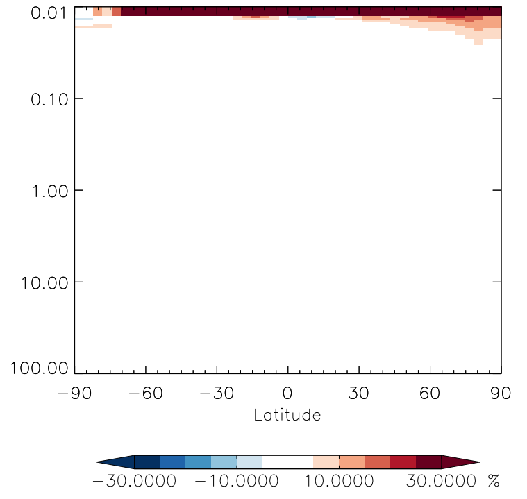
v11-01g-Run0 / v11-01d-Run1 CFC11 - Strat zonal mean % diff for Oct
