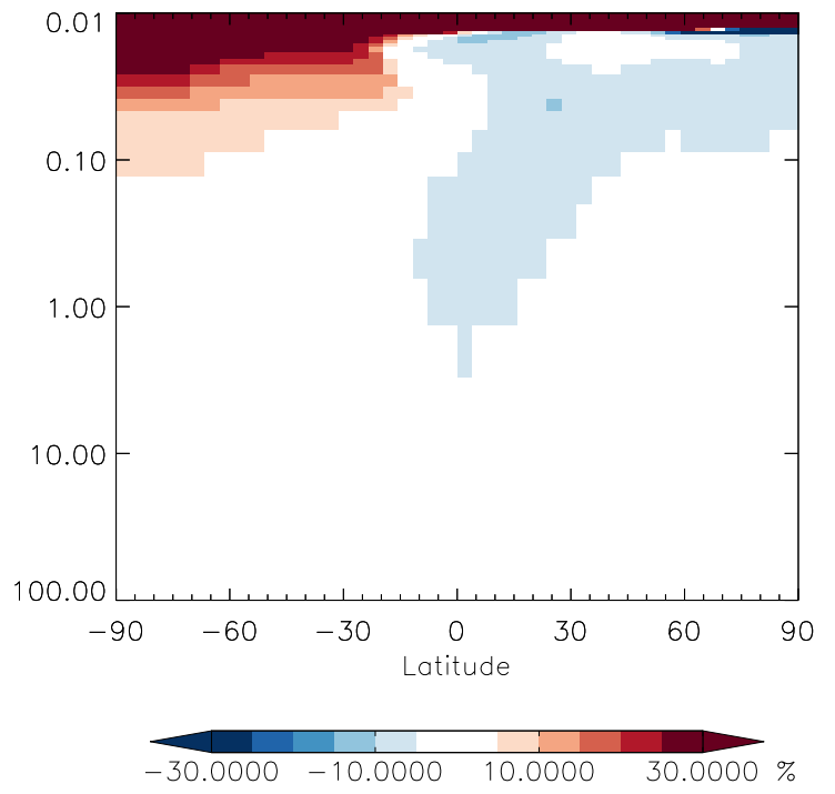
v11-01g-Run0 / v11-01f-geosfp-Run0 C3H8 - Strat zonal mean % diff for Oct
