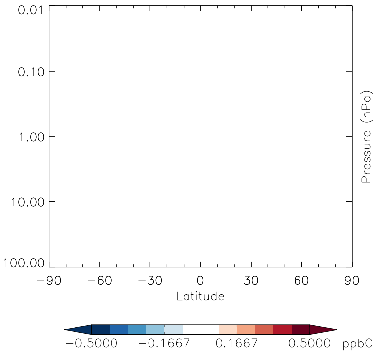
v11-01g-Run0 - v11-01f-geosfp-Run0 C2H6 - Strat zonal mean abs diff for Oct
