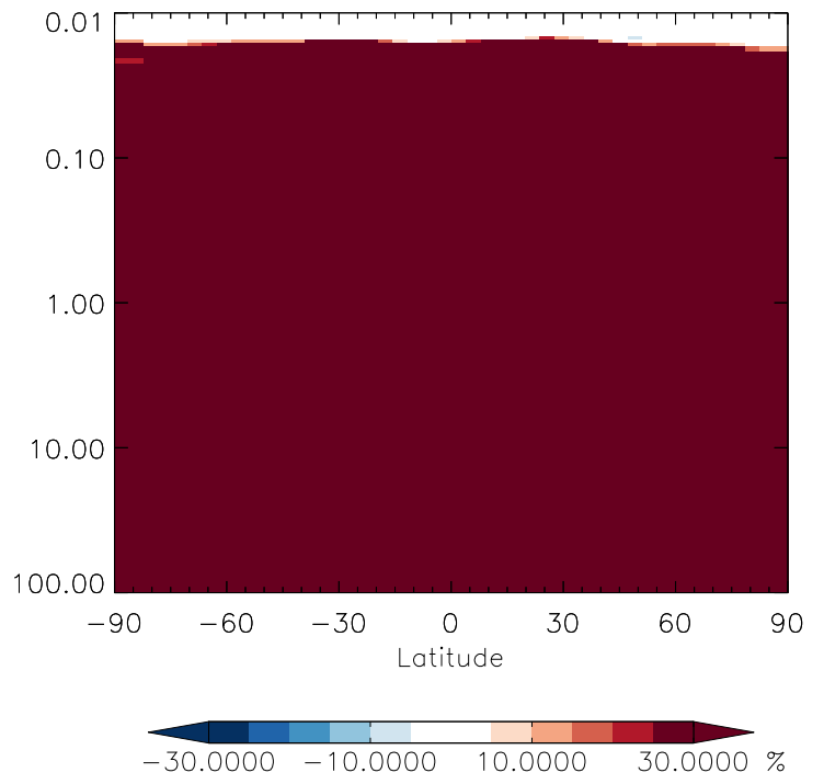
v11-01g-Run0 / v11-01f-geosfp-Run0 MVKN - Strat zonal mean % diff for Oct
