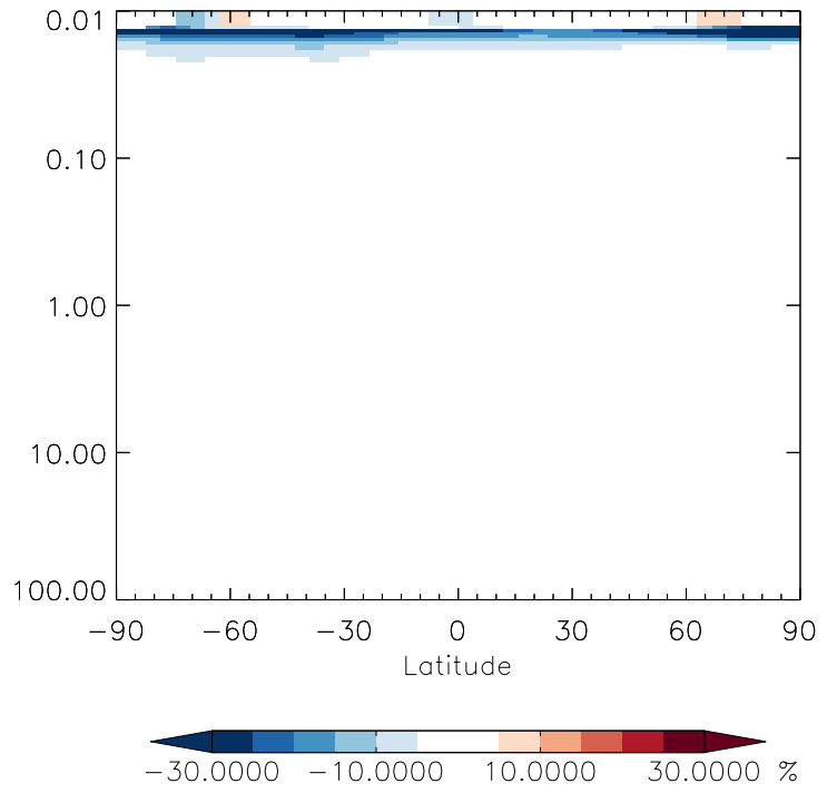
v11-01g-Run0 / v11-01d-Run1 HN04 - Strat zonal mean % diff for Oct
