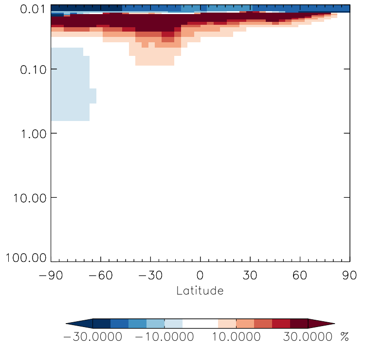
v11-01g-Run0 / v11-01d-Run1 CH 2 Br 2 - Strat zonal mean % diff for Oct
