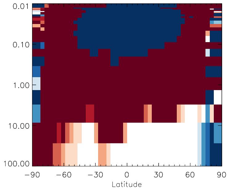
v11-01g-Run0 / v11-01f-geosfp-Run0 ISOP - Strat zonal mean % diff for Oct
