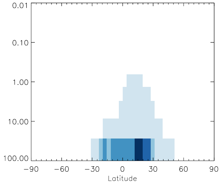
v11-01g-Run0 / v11-01d-Run1 NH3 - Strat zonal mean % diff for Oct
