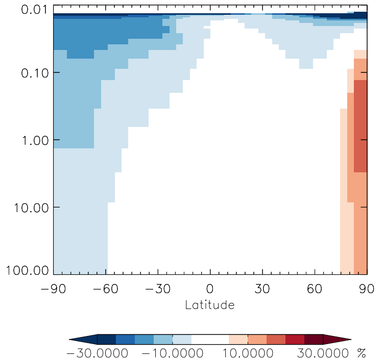
v11-01g-Run0 / v11-01d-Run1 HN02 - Strat zonal mean % diff for Oct
