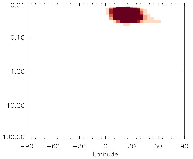
v11-01g-Run0 / v11-01f-geosfp-Run0 DST3 - Strat zonal mean % diff for Oct
