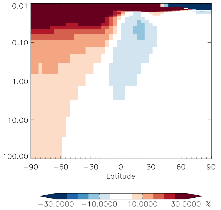
v11-01g-Run0 / v11-01f-geosfp-Run0 ALK4 - Strat zonal mean % diff for Oct
