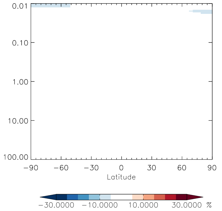
v11-01g-Run0 / v11-01f-geosfp-Run0 CH4 - Strat zonal mean % diff for Oct
