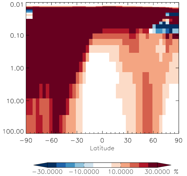
v11-01g-Run0 / v11-01d-Run1 IEPOX - Strat zonal mean % diff for Oct
