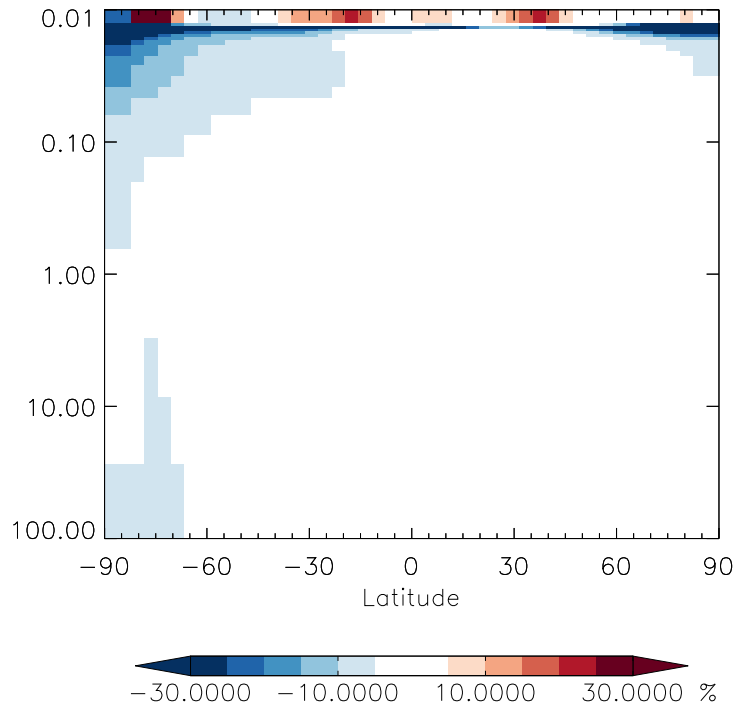
v11-01g-Run0 / v11-01d-Run1 N2O5 - Strat zonal mean % diff for Oct
