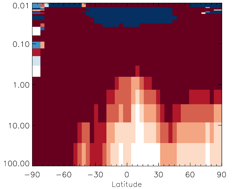
v11-01g-Run0 / v11-01d-Run1 PRPE - Strat zonal mean % diff for Oct
