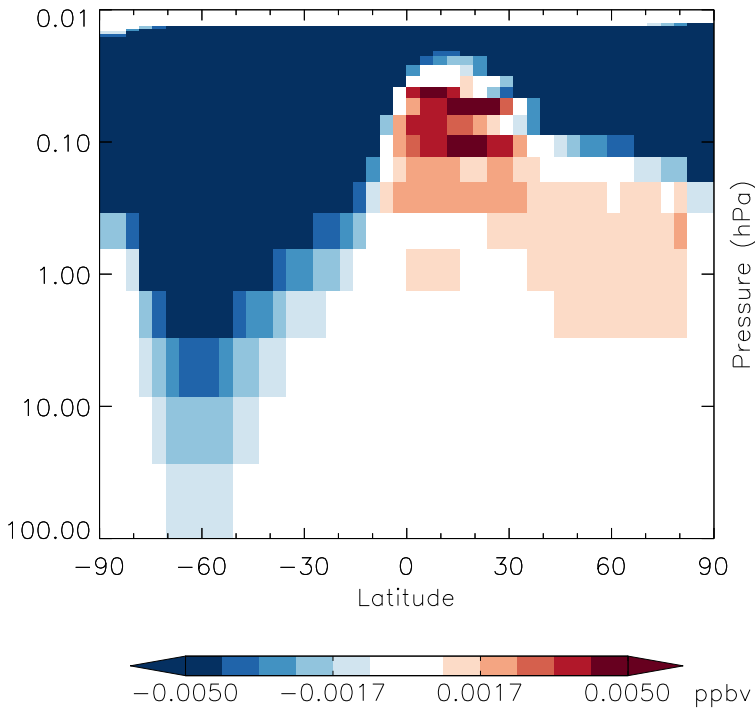
v11-01g-Run0 - v11-01d-Run1 N2O5 - Strat zonal mean abs diff for Oct
