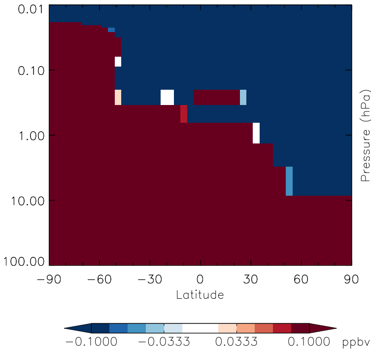
v11-01g-Run0 - v11-01d-Run1 CH4 - Strat zonal mean abs diff for Oct
