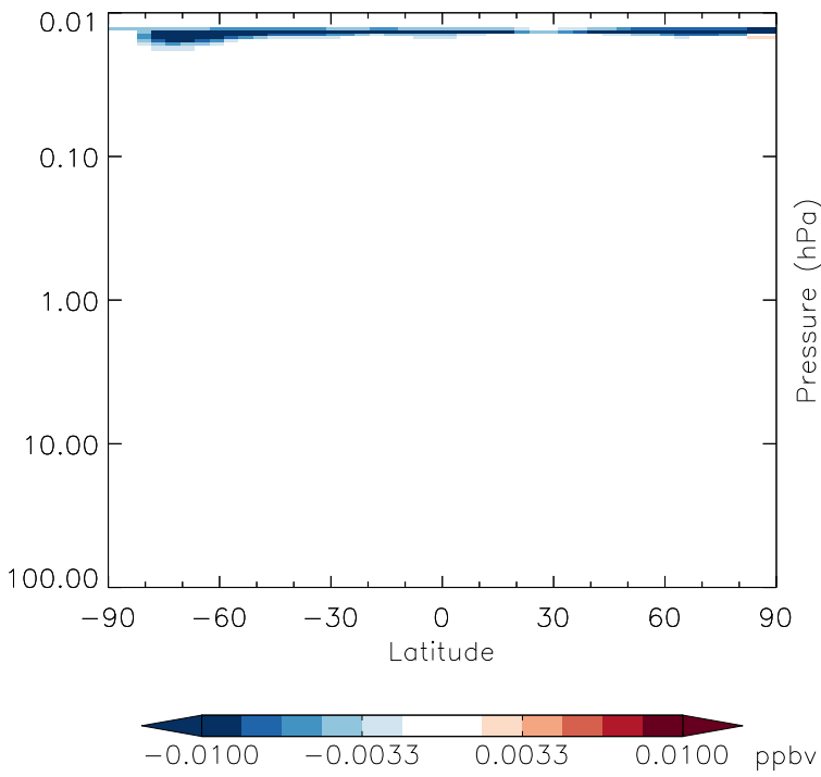
v11-01g-Run0 - v11-01f-geosfp-Run0 NO3 - Strat zonal mean abs diff for Oct
