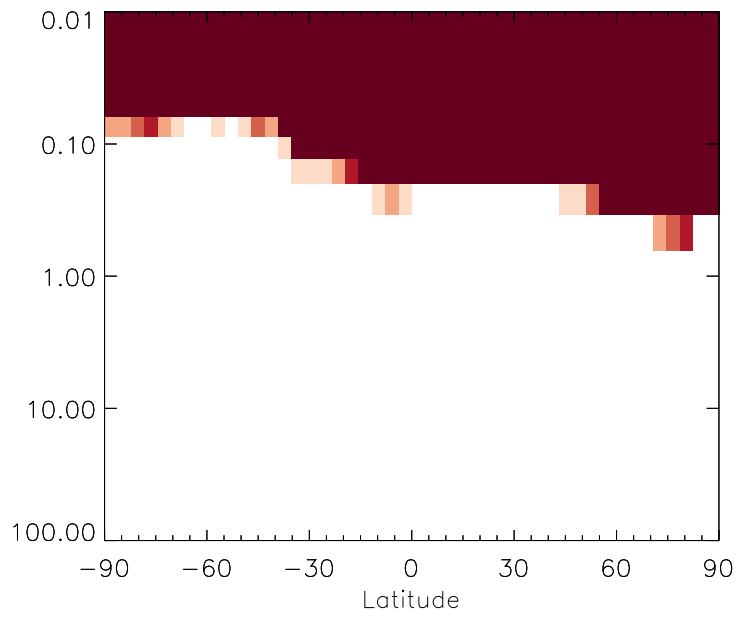
v11-01g-Run0 / v11-01f-geosfp-Run0 NITs - Strat zonal mean % diff for Oct
