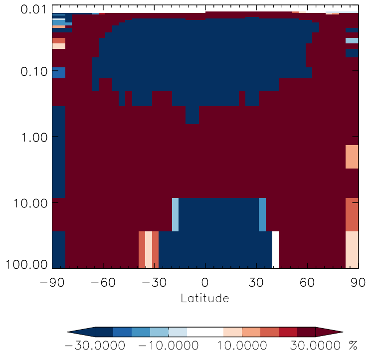
v11-01g-Run0 / v11-01d-Run1 ISOPND - Strat zonal mean % diff for Oct
