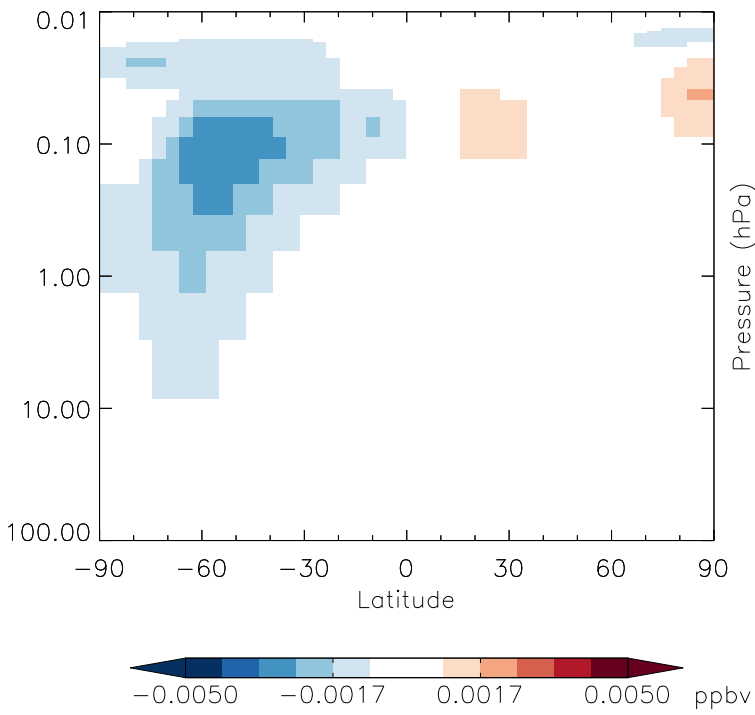
v11-01g-Run0 - v11-01f-geosfp-Run0 HN04 - Strat zonal mean abs diff for Oct
