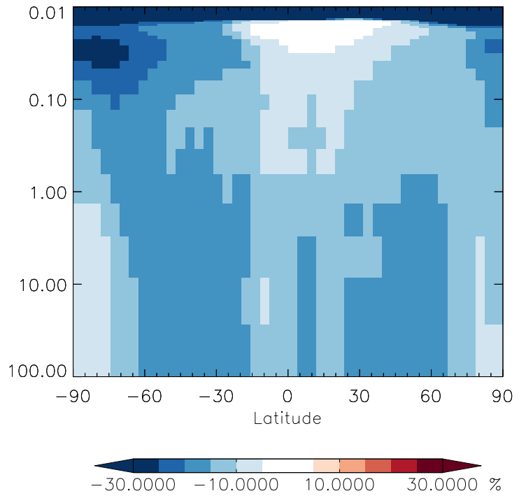
v11-01g-Run0 / v11-01d-Run1 BrNO 2 - Strat zonal mean % diff for Oct
