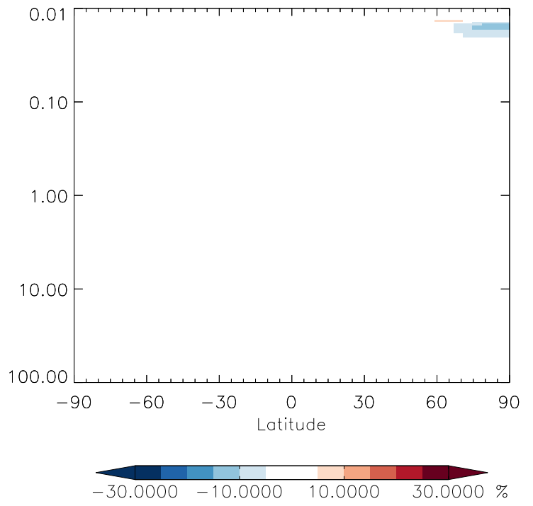
v11-01g-Run0 / v11-01f-geosfp-Run0 CH2O - Strat zonal mean % diff for Oct
