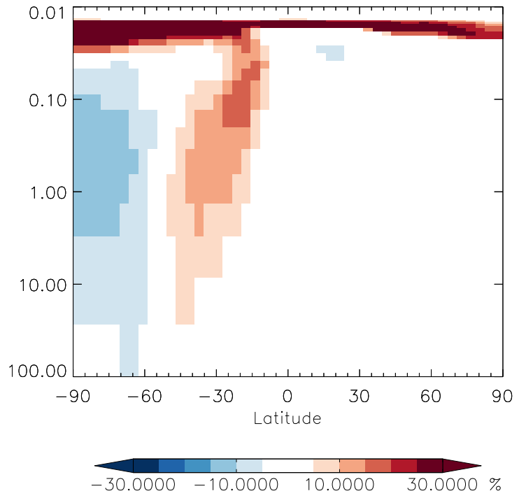
v11-01g-Run0 / v11-01d-Run1 MEK - Strat zonal mean % diff for Oct
