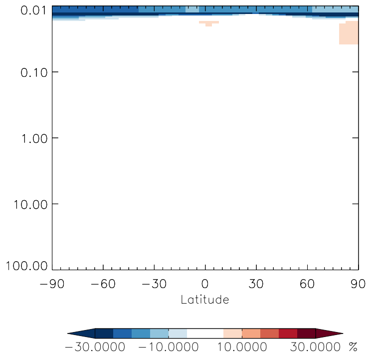
v11-01g-Run0 / v11-01f-geosfp-Run0 ClNO 3 - Strat zonal mean % diff for Oct
