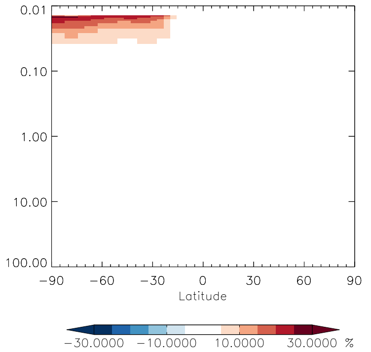
v11-01g-Run0 / v11-01f-geosfp-Run0 CH3Br - Strat zonal mean % diff for Oct
