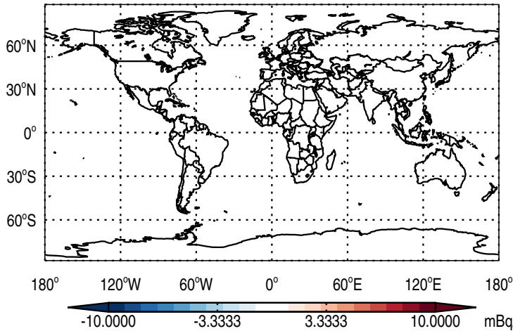
Abs Diff @ Surface - Pb
