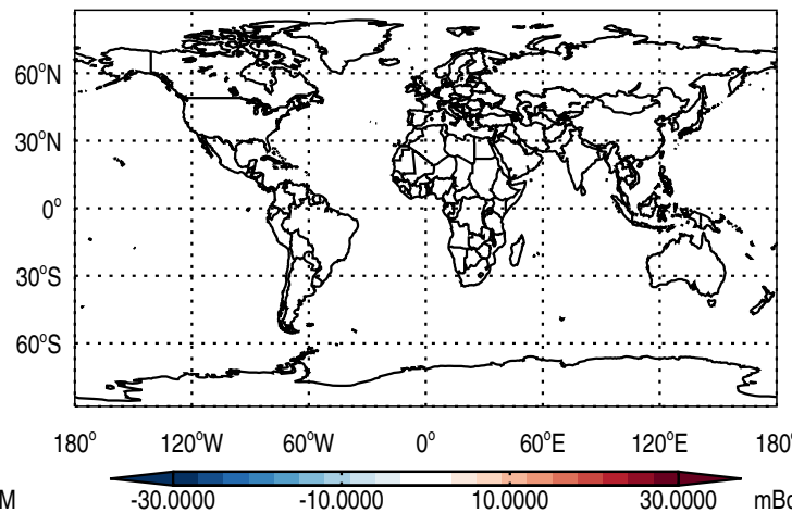
Abs Diff @ 500 hPa - Be7
