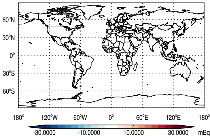
Abs Diff @ Surface - Be7
