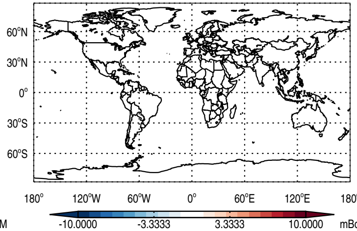
Abs Diff @ 500 hPa - Pb
