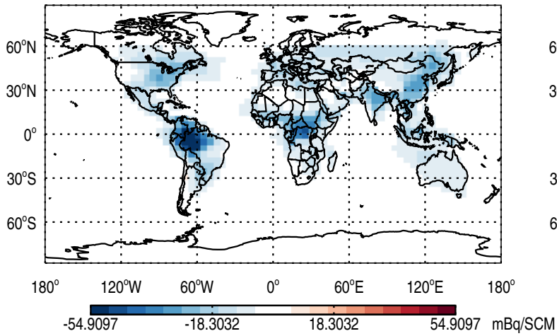
Abs Diff @ Surface - Rn
