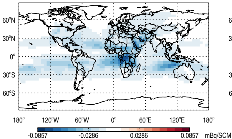
Abs Diff @ Surface - Be7
