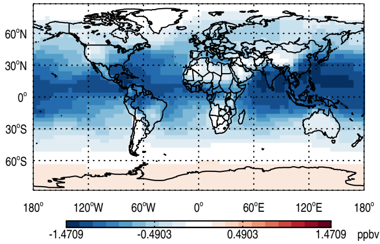
Abs Diff @ Surface - PASV
