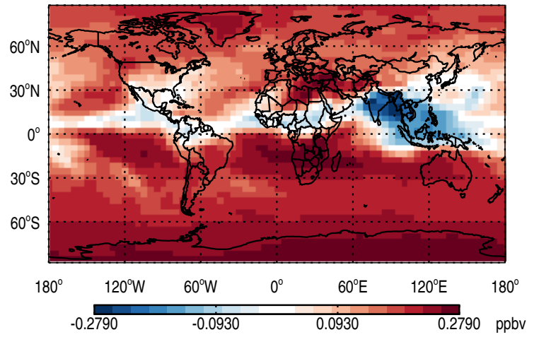
Abs Diff @ 500 hPa - PASV
