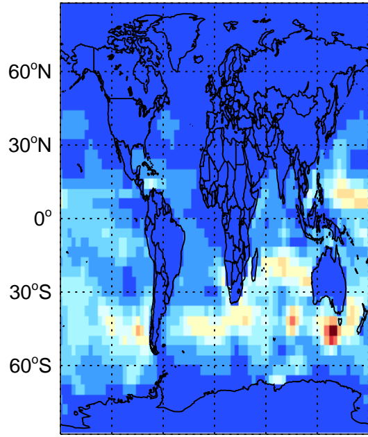
DMS biogenic emissions for Jan
