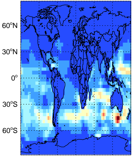
DMS biogenic emissions for Jan
