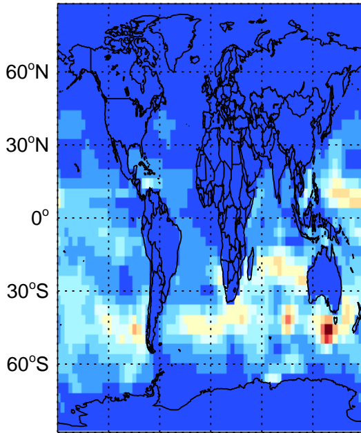
DMS biogenic emissions for Jan
