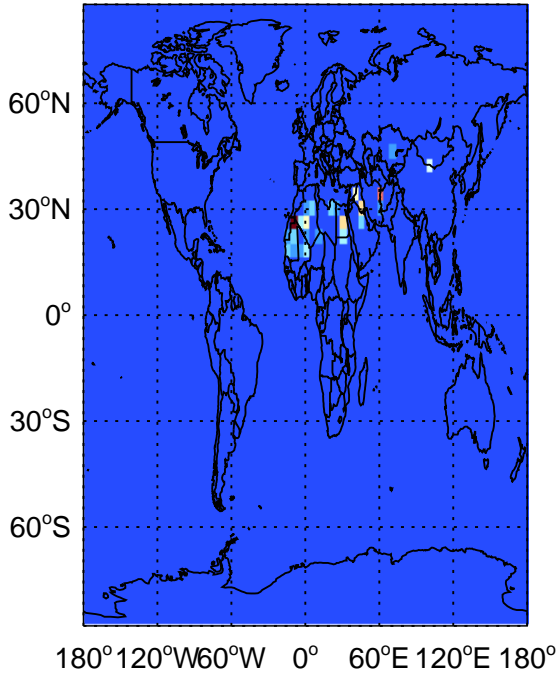
DST4 emissions for Jul
