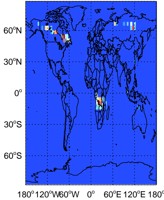
MEK biomass emissions for Jul
