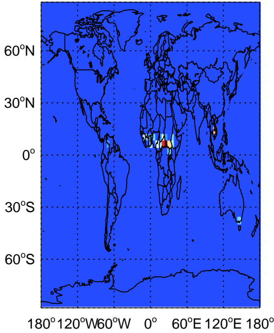
OC biomass emissions for Jan
