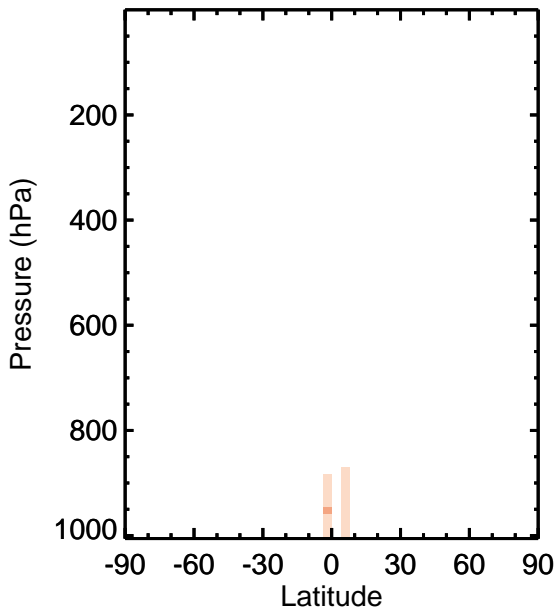
v11-01k-Run0 - v11-01g-Run0 MVK - Zonal mean abs diff for Apr
