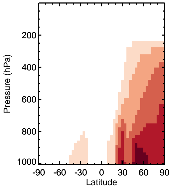
v11-01k-Run0 - v11-01g-Run0 C3H8 - Zonal mean abs diff for Apr
