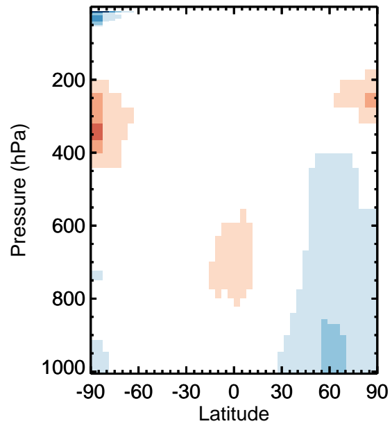
v11-01k-Run0 / v11-01g-Run0 CIO - Zonal mean % diff for Apr
