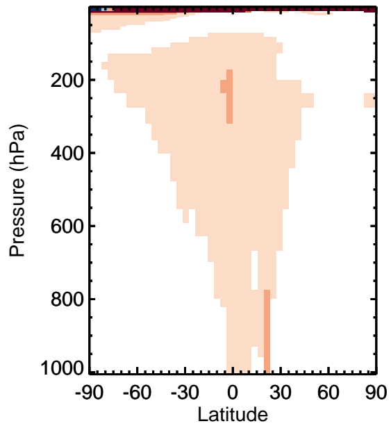
v11-01k-Run0 - v11-01f-geosfp-Run0 / v11-01k-Run0 / v11-01f-geosfp-Run0 ALK4 - Zonal mean abs diff for Apr ALK4 - Zonal mean % diff for Apr
