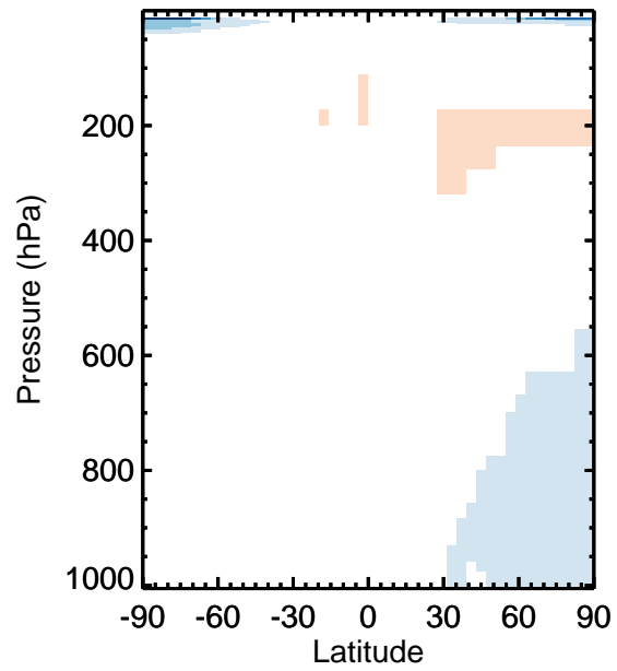
v11-01k-Run0 / v11-01g-Run0 MP - Zonal mean % diff for Apr
