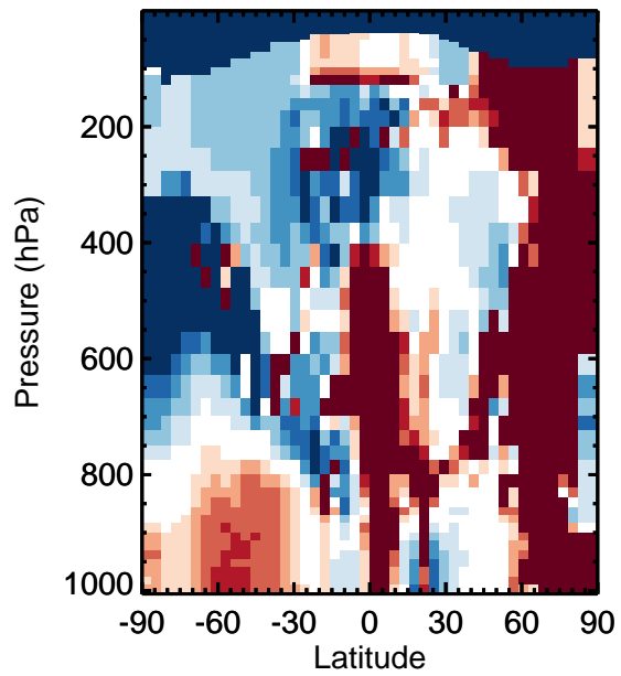
v11-01k-Run0 - v11-01f-geosfp-Run0 / v11-01k-Run0 / v11-01f-geosfp-Run0 NIT - Zonal mean abs diff for Apr NIT - Zonal mean % diff for Apr
