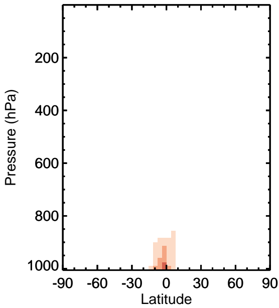
v11-01k-Run0 - v11-01g-Run0 ISOP - Zonal mean abs diff for Apr
