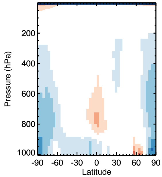
v11-01k-Run0 / v11-01g-Run0 NO 2 - Zonal mean % diff for Apr
