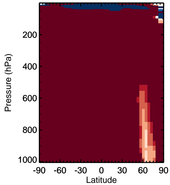
v11-01k-Run0 - v11-01f-geosfp-Run0 / v11-01k-Run0 / v11-01f-geosfp-Run0 ISOP - Zonal mean abs diff for Apr ISOP - Zonal mean % diff for Apr
