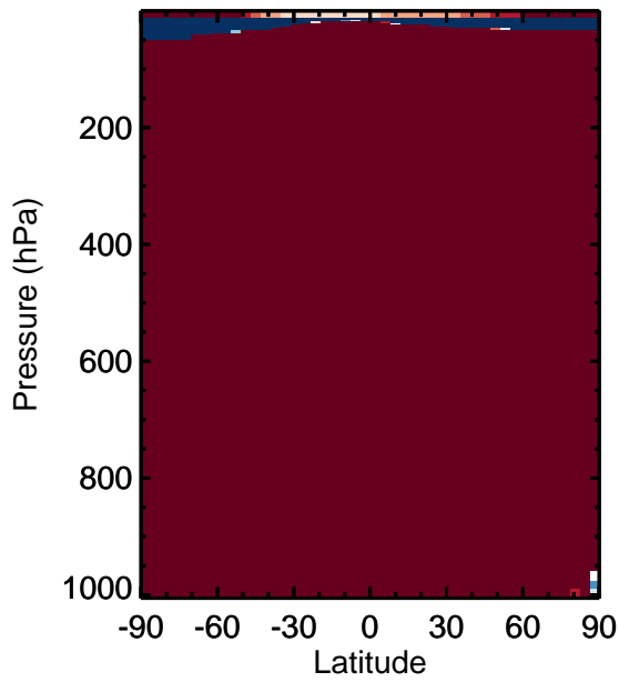
v11-01k-Run0 - v11-01g-Run0 CH4 - Zonal mean abs diff for Apr
