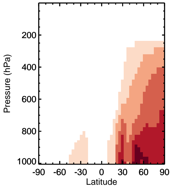
v11-01k-Run0 - v11-01f-geosfp-Run0 / v11-01k-Run0 / v11-01f-geosfp-Run0 C3H8 - Zonal mean abs diff for Apr C3H8 - Zonal mean % diff for Apr
