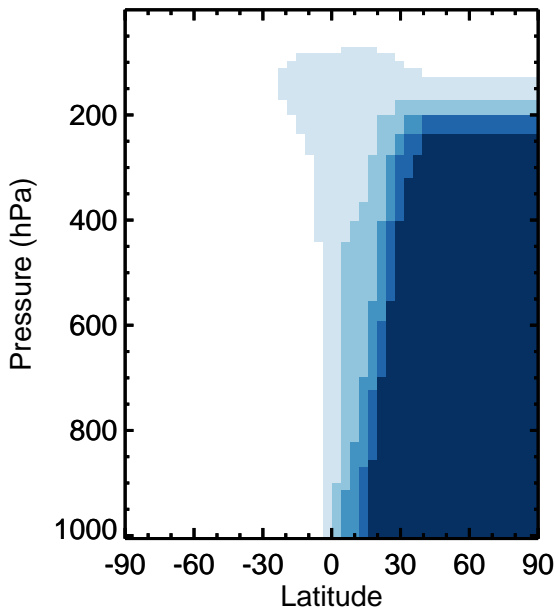
v11-01k-Run0 - v11-01f-geosfp-Run0 / v11-01k-Run0 / v11-01f-geosfp-Run0 C2H6 - Zonal mean abs diff for Apr C2H6 - Zonal mean % diff for Apr
