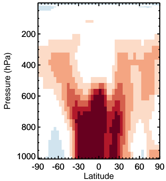
v11-01k-Run0 - v11-01f-geosfp-Run0 / v11-01k-Run0 / v11-01f-geosfp-Run0 BrCl - Zonal mean abs diff for Apr BrCl - Zonal mean % diff for Apr
