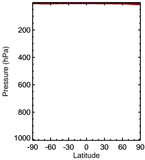
v11-01k-Run0 - v11-01g-Run0 NO - Zonal mean abs diff for Apr
