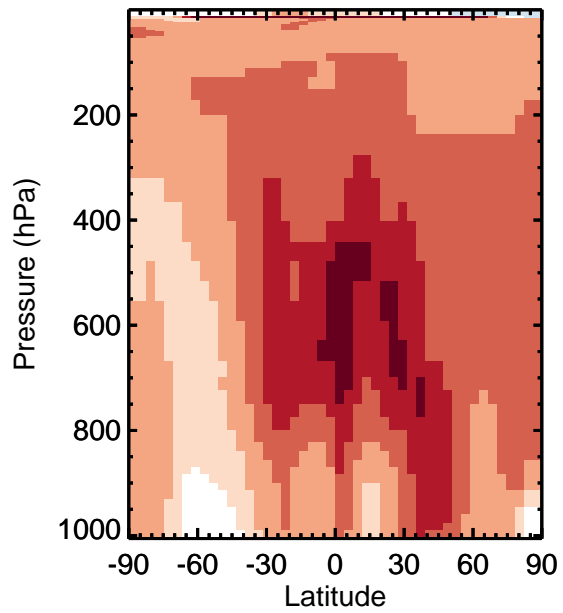
v11-01k-Run0 - v11-01f-geosfp-Run0 / v11-01k-Run0 / v11-01f-geosfp-Run0 SALC - Zonal mean abs diff for Apr SALC - Zonal mean % diff for Apr
