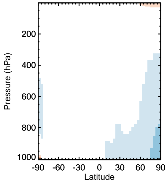
v11-01k-Run0 - v11-01f-geosfp-Run0 / v11-01k-Run0 / v11-01f-geosfp-Run0 HO2 - Zonal mean abs diff for Apr HO2 - Zonal mean % diff for Apr
