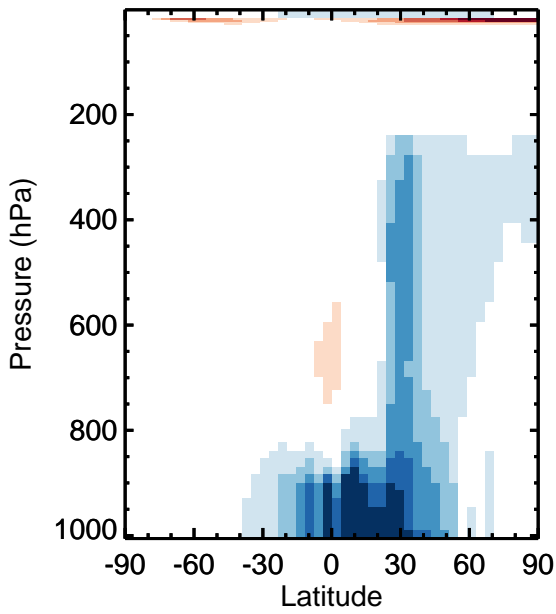
v11-01k-Run0 - v11-01g-Run0 OH - Zonal mean abs diff for Apr
