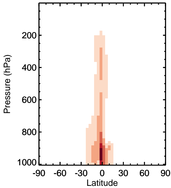
v11-01k-Run0 - v11-01f-geosfp-Run0 / v11-01k-Run0 / v11-01f-geosfp-Run0 MAP - Zonal mean abs diff for Apr MAP - Zonal mean % diff for Apr
