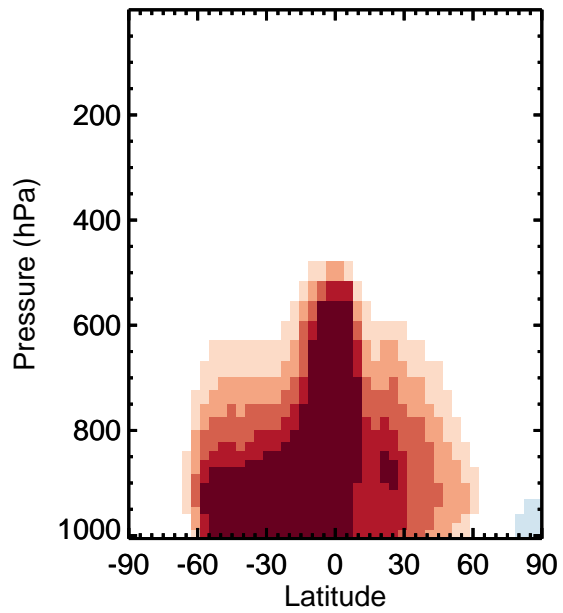
v11-01k-Run0 - v11-01f-geosfp-Run0 / v11-01k-Run0 / v11-01f-geosfp-Run0 HCl - Zonal mean abs diff for Apr HCl - Zonal mean % diff for Apr
