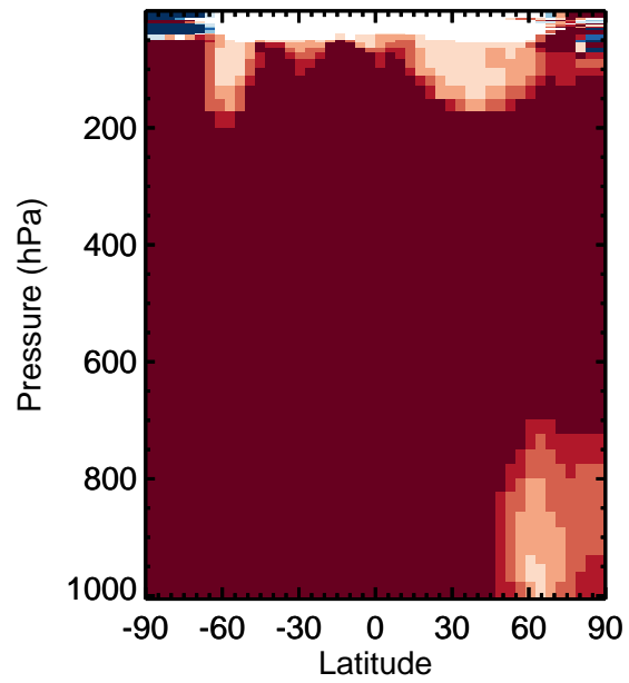
v11-01k-Run0 / v11-01g-Run0 MVK - Zonal mean % diff for Apr
