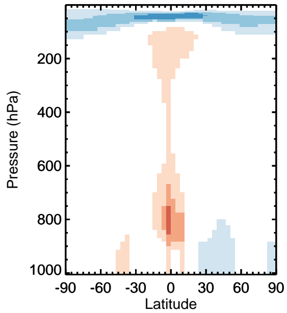
v11-01k-Run0 / v11-01g-Run0 PAN - Zonal mean % diff for Apr
