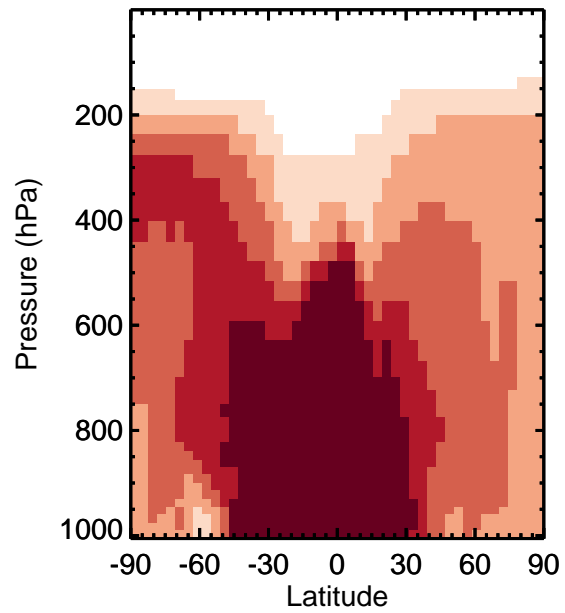
v11-01k-Run0 - v11-01f-geosfp-Run0 / v11-01k-Run0 / v11-01f-geosfp-Run0 NH4 - Zonal mean abs diff for Apr NH4 - Zonal mean % diff for Apr
