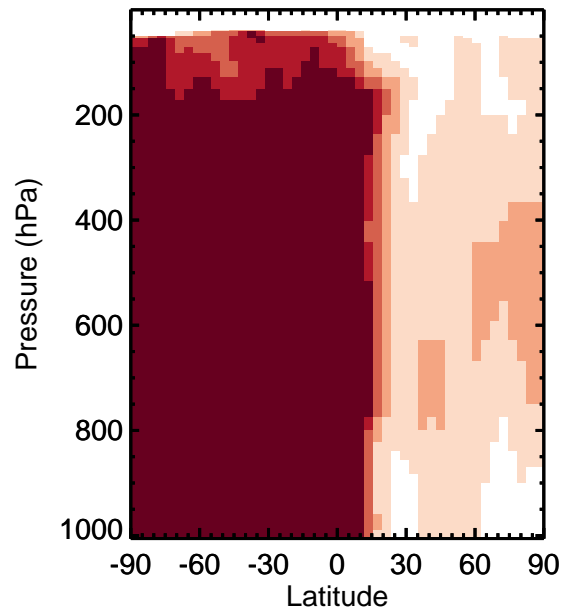
v11-01k-Run0 / v11-01g-Run0 NITs - Zonal mean % diff for Apr
