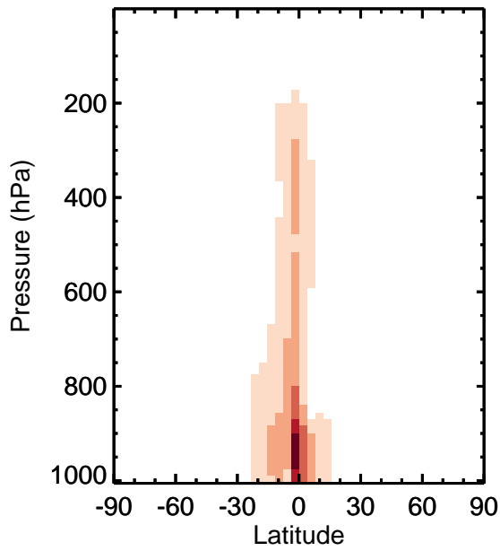
v11-01k-Run0 - v11-01g-Run0 MAP - Zonal mean abs diff for Apr
