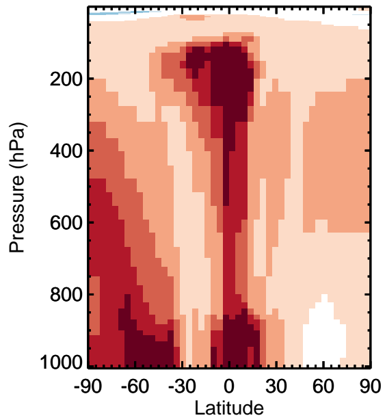
v11-01k-Run0 / v11-01g-Run0 HAC - Zonal mean % diff for Apr
