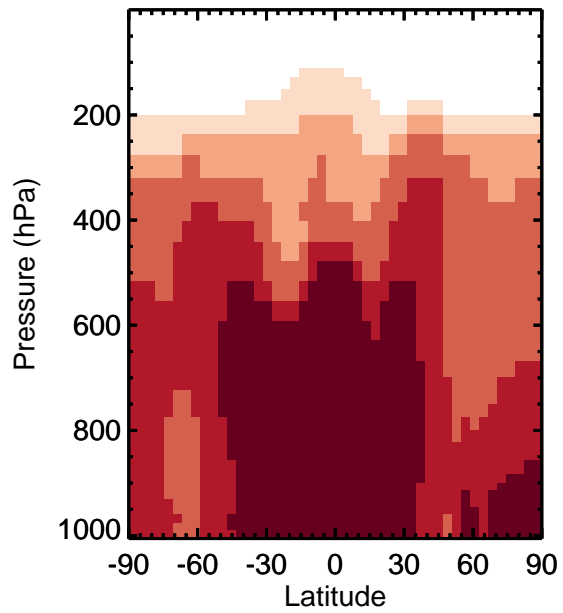
v11-01k-Run0 - v11-01f-geosfp-Run0 / v11-01k-Run0 / v11-01f-geosfp-Run0 SO4 - Zonal mean abs diff for Apr SO4 - Zonal mean % diff for Apr
