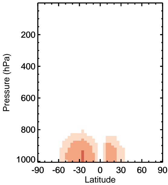
v11-01k-Run0 - v11-01g-Run0 SALC - Zonal mean abs diff for Apr
