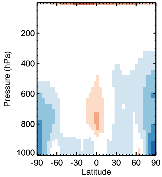
v11-01k-Run0 / v11-01g-Run0 MPN - Zonal mean % diff for Apr
