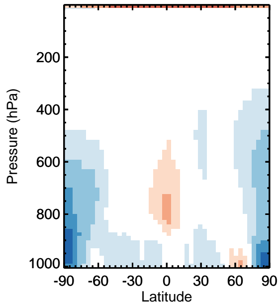
v11-01k-Run0 - v11-01f-geosfp-Run0 / v11-01k-Run0 / v11-01f-geosfp-Run0 MPN - Zonal mean abs diff for Apr MPN - Zonal mean % diff for Apr
