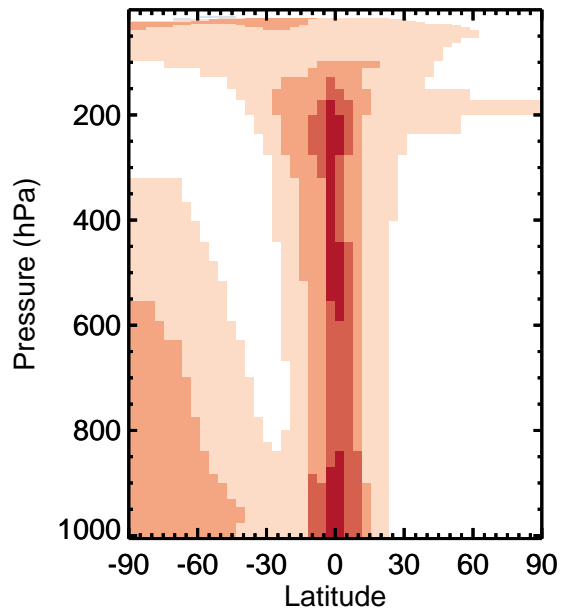
v11-01k-Run0 / v11-01g-Run0 MEK - Zonal mean % diff for Apr
