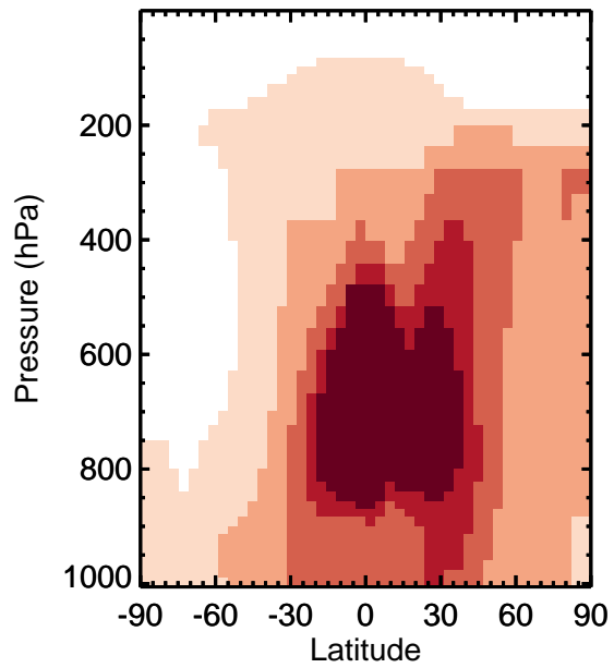
v11-01k-Run0 - v11-01f-geosfp-Run0 / v11-01k-Run0 / v11-01f-geosfp-Run0 MSA - Zonal mean abs diff for Apr MSA - Zonal mean % diff for Apr
