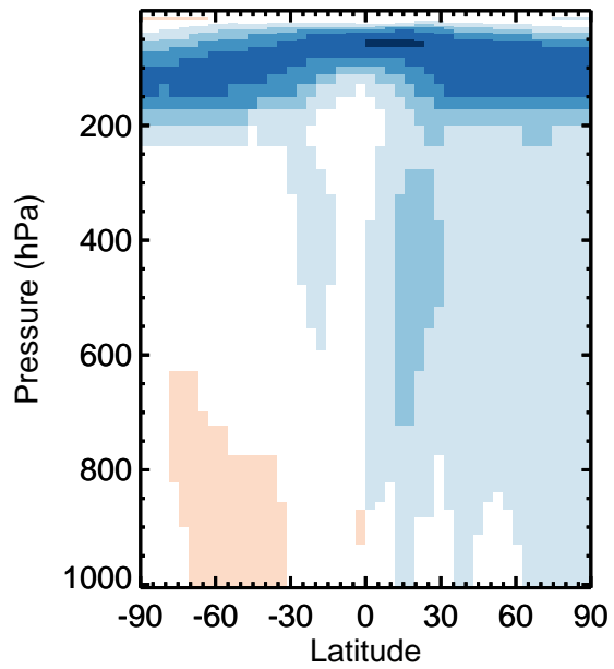
v11-01k-Run0 - v11-01f-geosfp-Run0 / v11-01k-Run0 / v11-01f-geosfp-Run0 ALD2 - Zonal mean abs diff for Apr ALD2 - Zonal mean % diff for Apr
