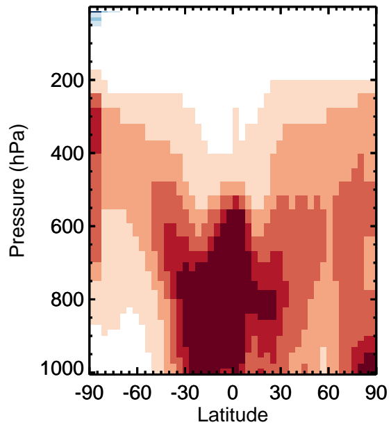
v11-01k-Run0 / v11-01g-Run0 BrO - Zonal mean % diff for Apr
