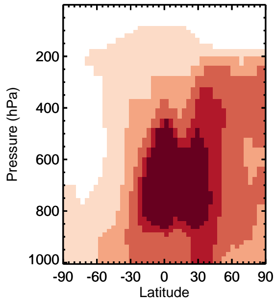
v11-01k-Run0 / v11-01g-Run0 MSA - Zonal mean % diff for Apr
