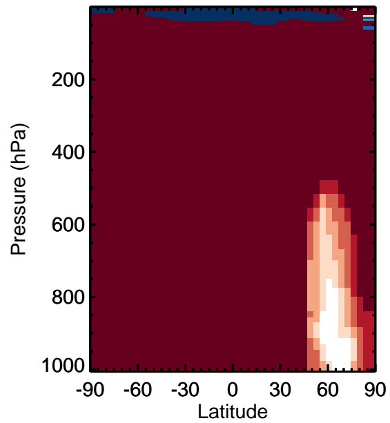
v11-01k-Run0 - v11-01f-geosfp-Run0 / v11-01k-Run0 / v11-01f-geosfp-Run0 RIP - Zonal mean abs diff for Apr RIP - Zonal mean % diff for Apr
