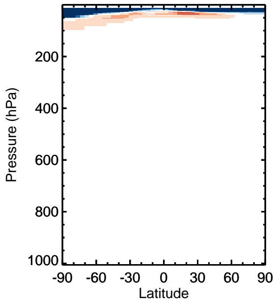
v11-01k-Run0 - v11-01g-Run0 O3 - Zonal mean abs diff for Apr
