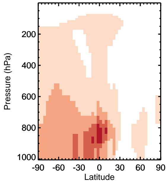
v11-01k-Run0 - v11-01f-geosfp-Run0 / v11-01k-Run0 / v11-01f-geosfp-Run0 PPN - Zonal mean abs diff for Apr PPN - Zonal mean % diff for Apr
