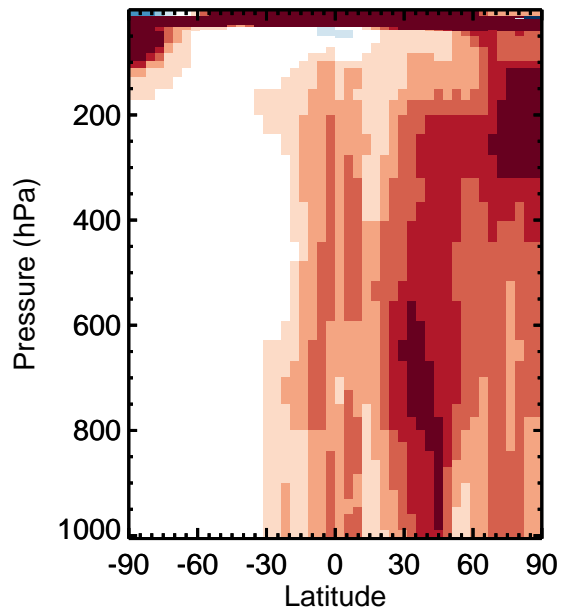
v11-01k-Run0 - v11-01f-geosfp-Run0 / v11-01k-Run0 / v11-01f-geosfp-Run0 DMS - Zonal mean abs diff for Apr DMS - Zonal mean % diff for Apr
