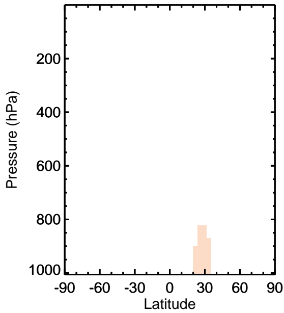
v11-01k-Run0 - v11-01g-Run0 NH4 - Zonal mean abs diff for Apr
