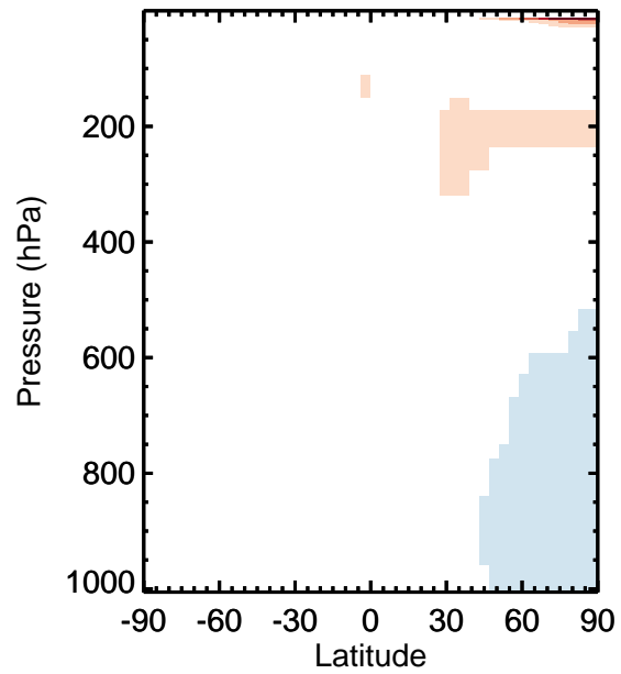
v11-01k-Run0 - v11-01f-geosfp-Run0 / v11-01k-Run0 / v11-01f-geosfp-Run0 MP - Zonal mean abs diff for Apr MP - Zonal mean % diff for Apr
