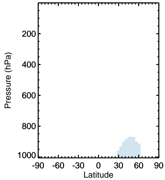
v11-01k-Run0 / v11-01g-Run0 O3 - Zonal mean % diff for Apr
