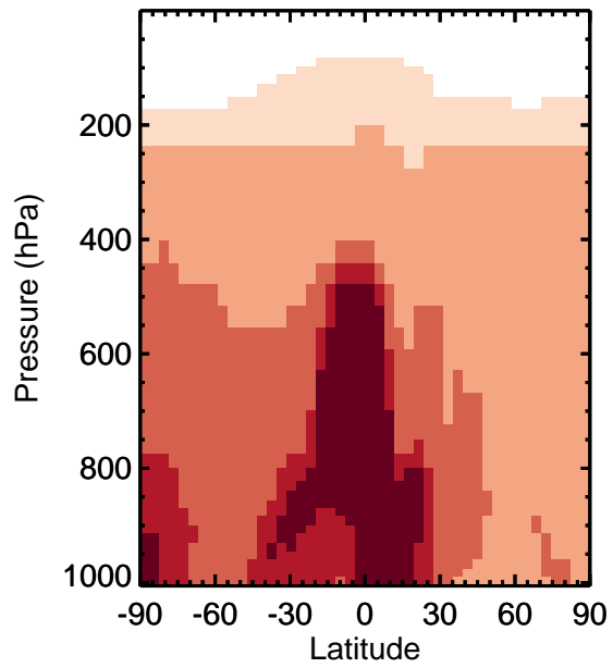
v11-01k-Run0 / v11-01g-Run0 BCPI - Zonal mean % diff for Apr
