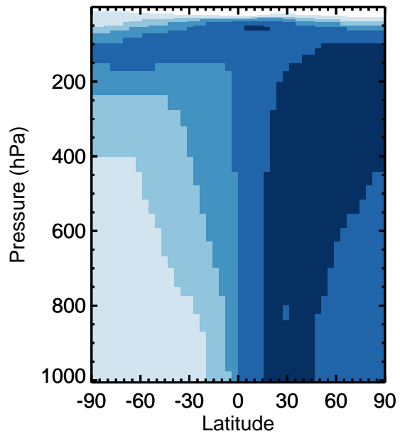
v11-01k-Run0 / v11-01g-Run0 C2H6 - Zonal mean % diff for Apr
