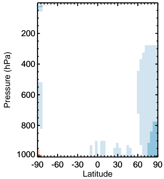
v11-01k-Run0 / v11-01g-Run0 OH - Zonal mean % diff for Apr
