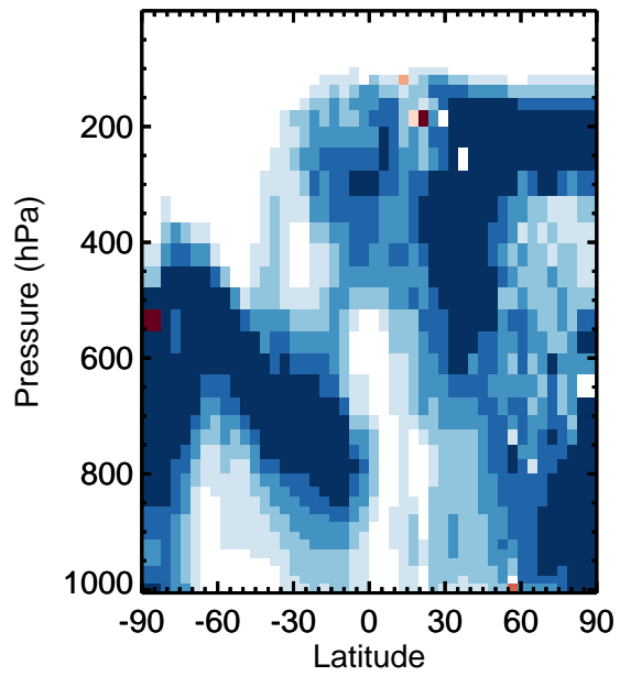
v11-01k-Run0 / v11-01g-Run0 NH3 - Zonal mean % diff for Apr
