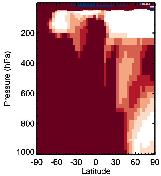
v11-01k-Run0 - v11-01f-geosfp-Run0 / v11-01k-Run0 / v11-01f-geosfp-Run0 PMN - Zonal mean abs diff for Apr PMN - Zonal mean % diff for Apr
