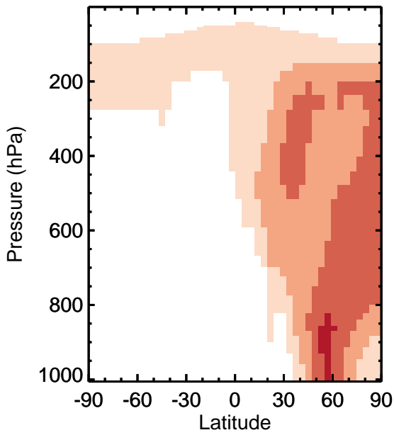
v11-01k-Run0 - v11-01g-Run0 PPN - Zonal mean abs diff for Apr
