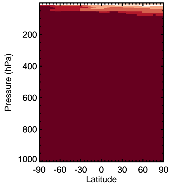
v11-01k-Run0 / v11-01g-Run0 C3H8 - Zonal mean % diff for Apr
