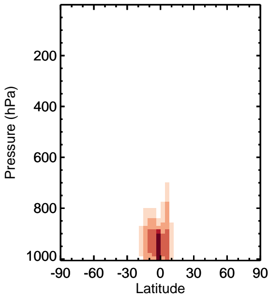
v11-01k-Run0 - v11-01g-Run0 RIP - Zonal mean abs diff for Apr
