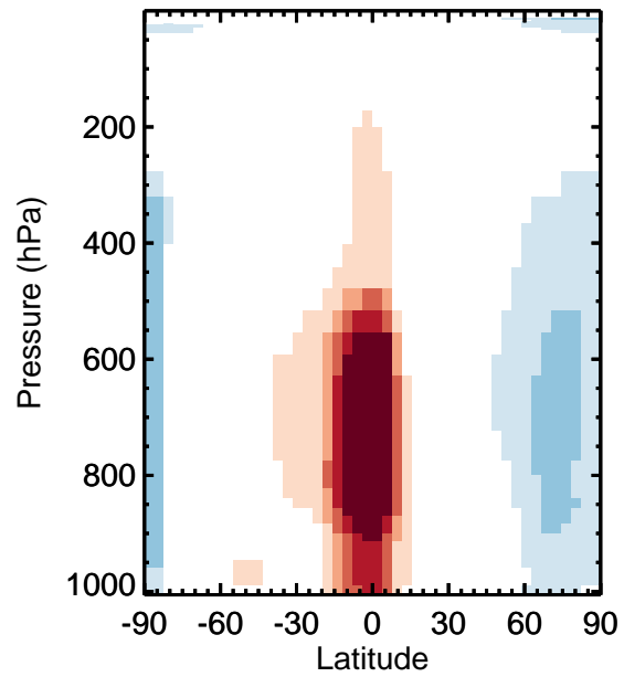
v11-01k-Run0 - v11-01f-geosfp-Run0 / v11-01k-Run0 / v11-01f-geosfp-Run0 HBr - Zonal mean abs diff for Apr HBr - Zonal mean % diff for Apr
