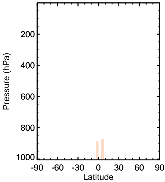
v11-01k-Run0 - v11-01f-geosfp-Run0 / v11-01k-Run0 / v11-01f-geosfp-Run0 MVK - Zonal mean abs diff for Apr MVK - Zonal mean % diff for Apr
