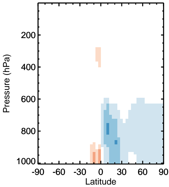
v11-01k-Run0 - v11-01g-Run0 MP - Zonal mean abs diff for Apr
