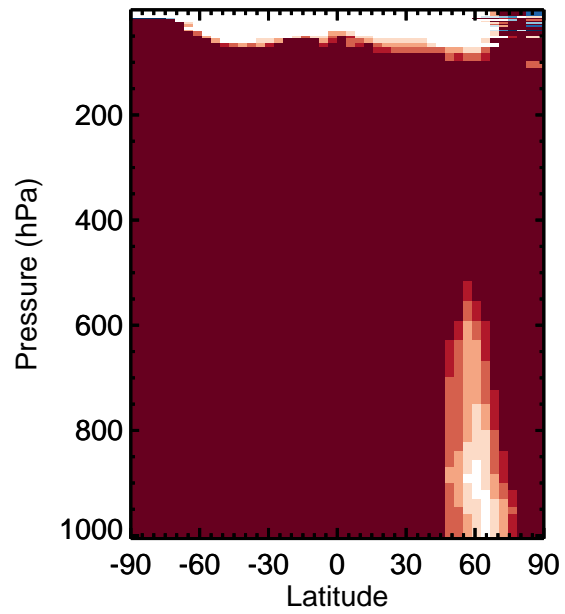
v11-01k-Run0 / v11-01g-Run0 RIP - Zonal mean % diff for Apr
