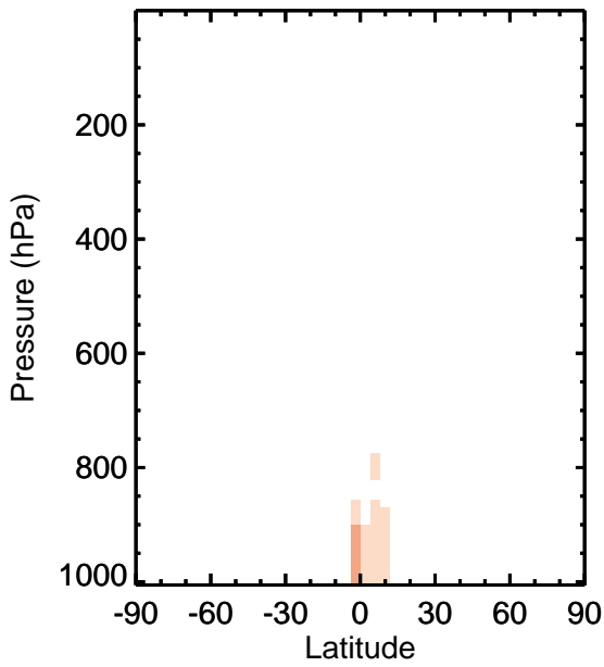
v11-01k-Run0 - v11-01g-Run0 HAC - Zonal mean abs diff for Apr
