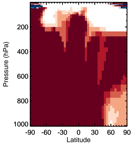
v11-01k-Run0 / v11-01g-Run0 PMN - Zonal mean % diff for Apr
