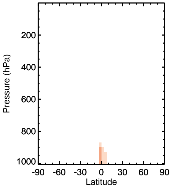
v11-01k-Run0 - v11-01f-geosfp-Run0 / v11-01k-Run0 / v11-01f-geosfp-Run0 MEK - Zonal mean abs diff for Apr MEK - Zonal mean % diff for Apr
