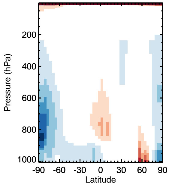
v11-01k-Run0 / v11-01g-Run0 NO - Zonal mean % diff for Apr
