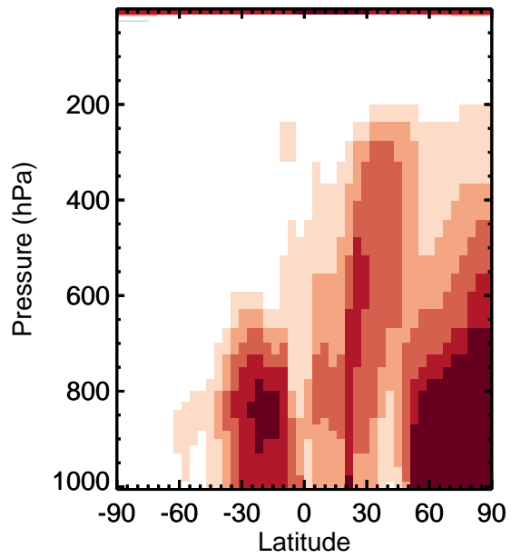
v11-01k-Run0 / v11-01g-Run0 SO 2 - Zonal mean % diff for Apr
