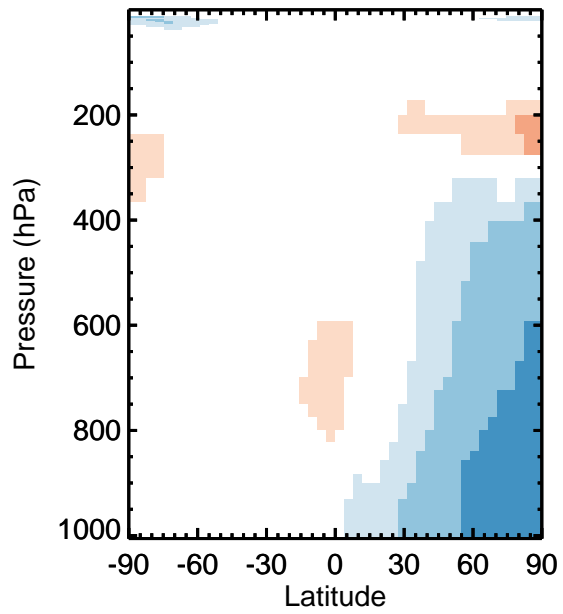
v11-01k-Run0 / v11-01g-Run0 HOCl - Zonal mean % diff for Apr
