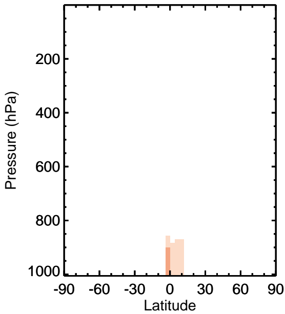
v11-01k-Run0 - v11-01f-geosfp-Run0 / v11-01k-Run0 / v11-01f-geosfp-Run0 HAC - Zonal mean abs diff for Apr HAC - Zonal mean % diff for Apr
