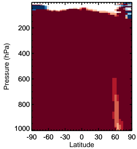
v11-01k-Run0 / v11-01g-Run0 ISOP - Zonal mean % diff for Apr
