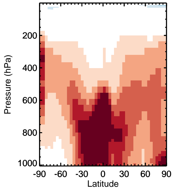
v11-01k-Run0 - v11-01f-geosfp-Run0 / v11-01k-Run0 / v11-01f-geosfp-Run0 BrO - Zonal mean abs diff for Apr BrO - Zonal mean % diff for Apr
