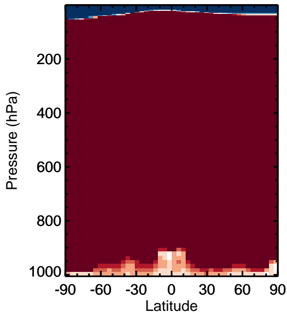
v11-01k-Run0 - v11-01g-Run0 N2O - Zonal mean abs diff for Apr
