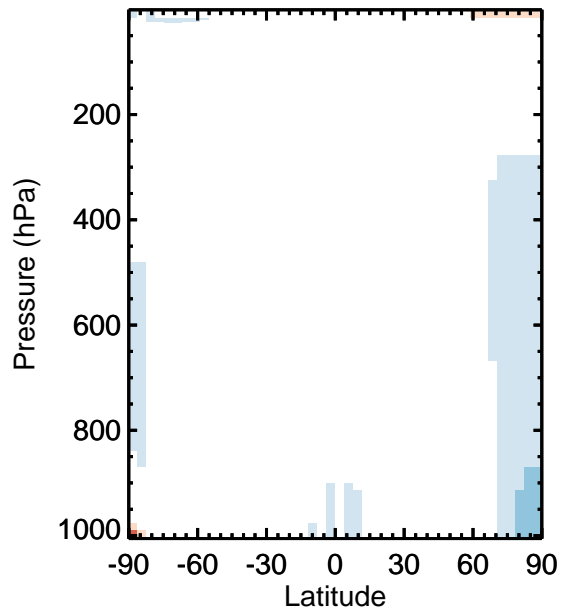
v11-01k-Run0 - v11-01f-geosfp-Run0 / v11-01k-Run0 / v11-01f-geosfp-Run0 OH - Zonal mean abs diff for Apr OH - Zonal mean % diff for Apr
