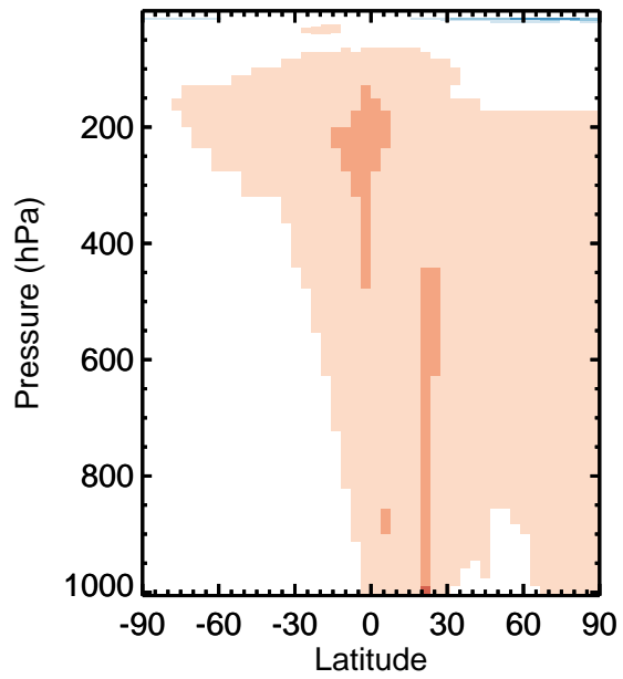
v11-01k-Run0 / v11-01g-Run0 ALK4 - Zonal mean % diff for Apr
