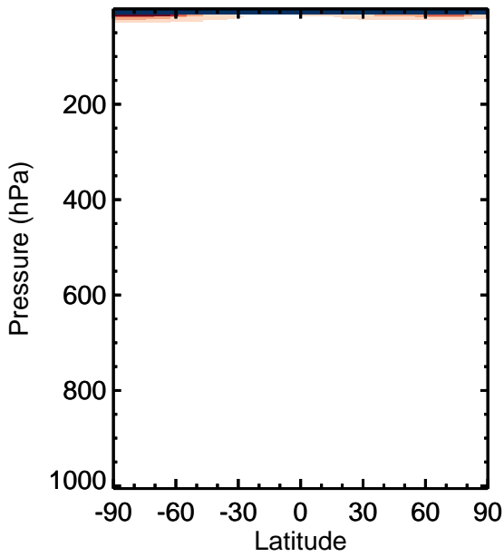
v11-01k-Run0 - v11-01g-Run0 NO 2 - Zonal mean abs diff for Apr
