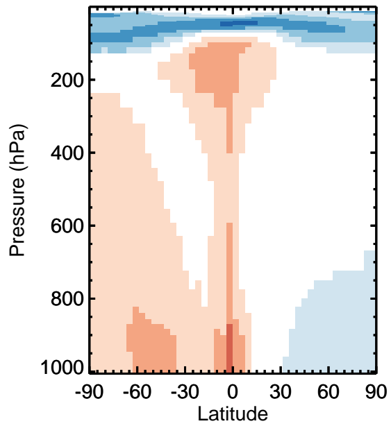
v11-01k-Run0 / v11-01g-Run0 MAP - Zonal mean % diff for Apr
