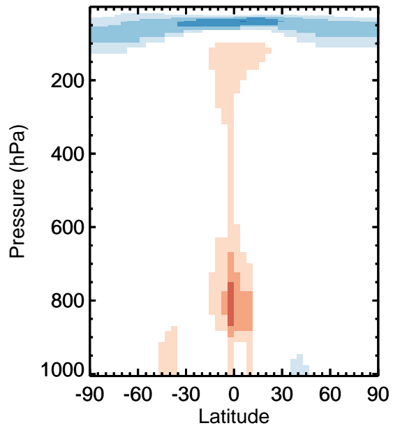
v11-01k-Run0 - v11-01f-geosfp-Run0 / v11-01k-Run0 / v11-01f-geosfp-Run0 PAN - Zonal mean abs diff for Apr PAN - Zonal mean % diff for Apr
