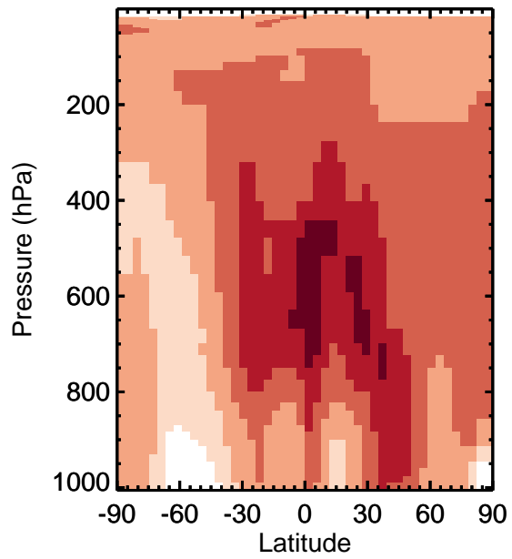
v11-01k-Run0 / v11-01g-Run0 SALC - Zonal mean % diff for Apr
