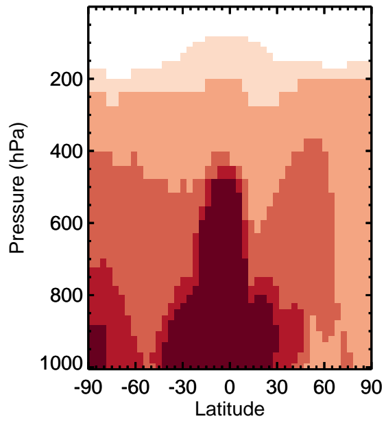
v11-01k-Run0 / v11-01g-Run0 OCPI - Zonal mean % diff for Apr
