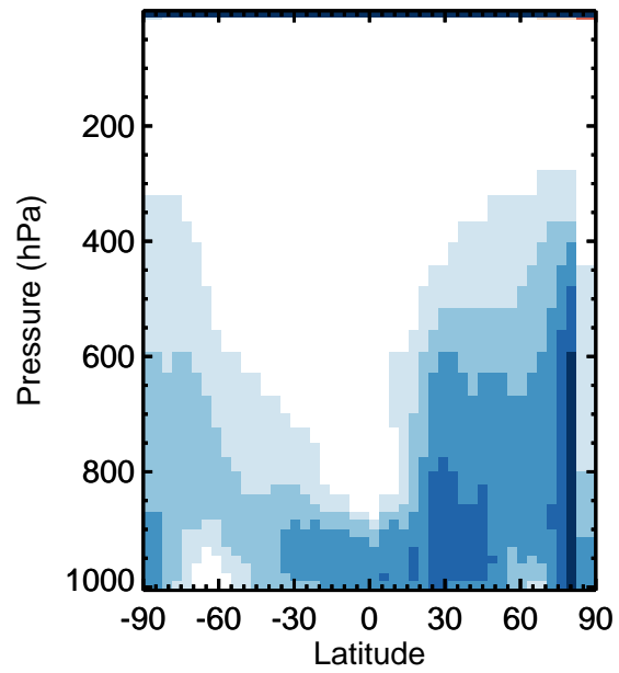
v11-01k-Run0 / v11-01g-Run0 NO3 - Zonal mean % diff for Apr
