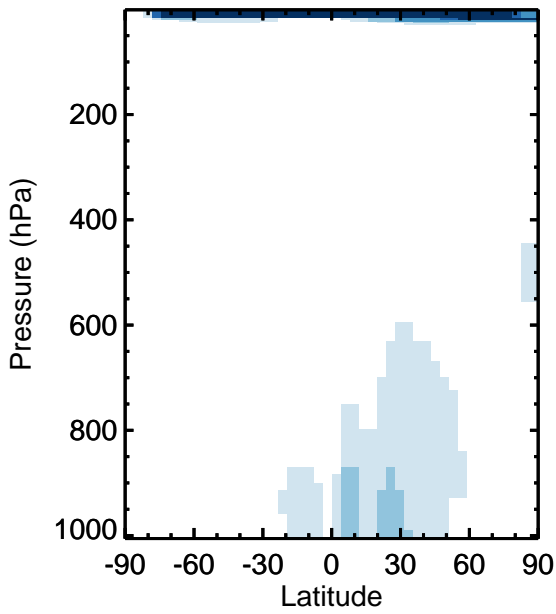
v11-01k-Run0 - v11-01g-Run0 HO2 - Zonal mean abs diff for Apr
