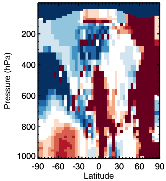
v11-01k-Run0 / v11-01g-Run0 NIT - Zonal mean % diff for Apr
