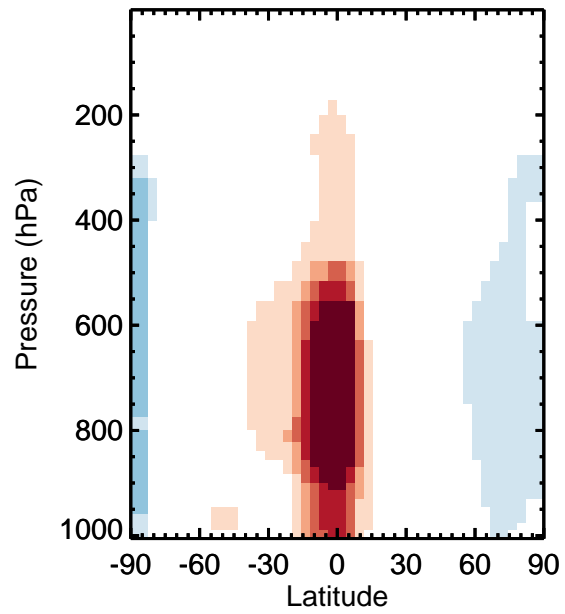
v11-01k-Run0 / v11-01g-Run0 HBr - Zonal mean % diff for Apr
