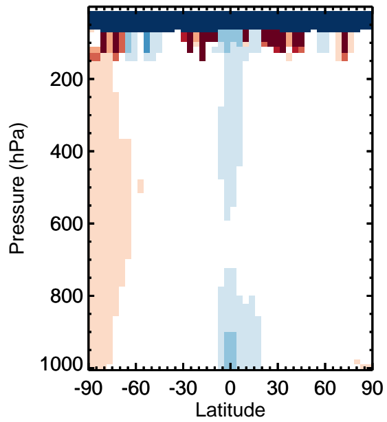
v11-01k-Run0 / v11-01g-Run0 SO 4 s - Zonal mean % diff for Apr
