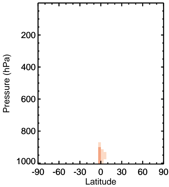
v11-01k-Run0 - v11-01g-Run0 MEK - Zonal mean abs diff for Apr
