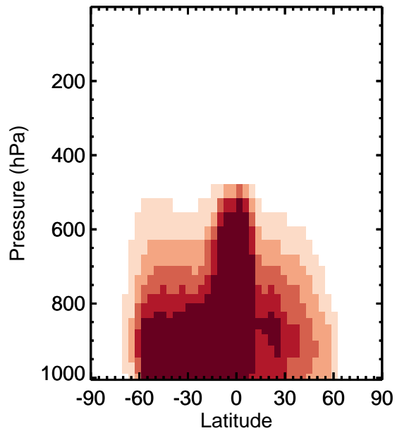
v11-01k-Run0 / v11-01g-Run0 HCl - Zonal mean % diff for Apr
