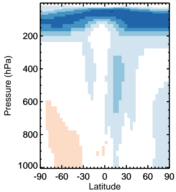
v11-01k-Run0 / v11-01g-Run0 ALD2 - Zonal mean % diff for Apr
