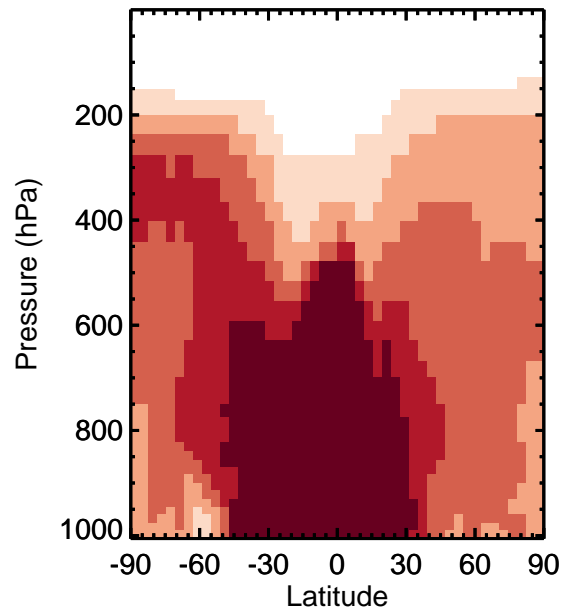
v11-01k-Run0 / v11-01g-Run0 NH4 - Zonal mean % diff for Apr
