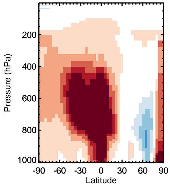
v11-01k-Run0 / v11-01g-Run0 Br2 - Zonal mean % diff for Apr
