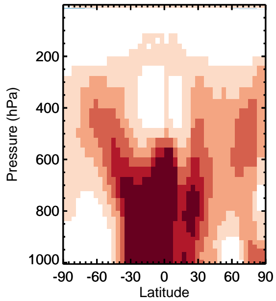
v11-01k-Run0 / v11-01g-Run0 BrCl - Zonal mean % diff for Apr
