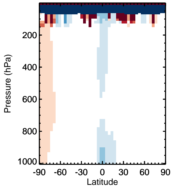
v11-01k-Run0 - v11-01f-geosfp-Run0 / v11-01k-Run0 / v11-01f-geosfp-Run0 SO 4 s - Zonal mean abs diff for Apr SO 4 s - Zonal mean % diff for Apr
