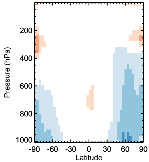
v11-01k-Run0 - v11-01f-geosfp-Run0 / v11-01k-Run0 / v11-01f-geosfp-Run0 CIO - Zonal mean abs diff for Apr CIO - Zonal mean % diff for Apr
