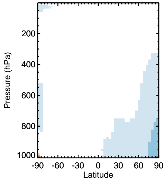
v11-01k-Run0 / v11-01g-Run0 HO2 - Zonal mean % diff for Apr
