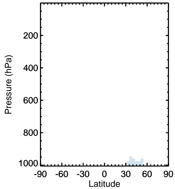
v11-01k-Run0 - v11-01f-geosfp-Run0 / v11-01k-Run0 / v11-01f-geosfp-Run0 O3 - Zonal mean abs diff for Apr O3 - Zonal mean % diff for Apr
