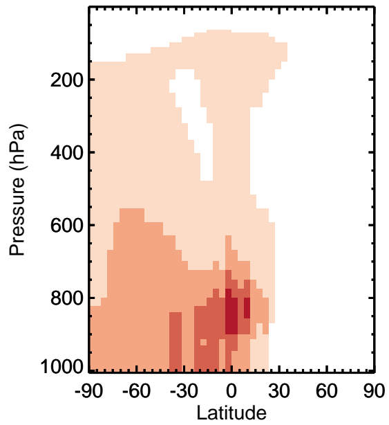
v11-01k-Run0 / v11-01g-Run0 PPN - Zonal mean % diff for Apr
