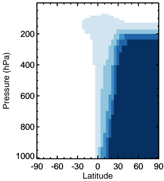
v11-01k-Run0 - v11-01g-Run0 C2H6 - Zonal mean abs diff for Apr
