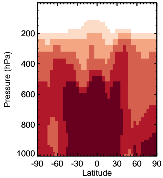
v11-01k-Run0 / v11-01g-Run0 SO4 - Zonal mean % diff for Apr
