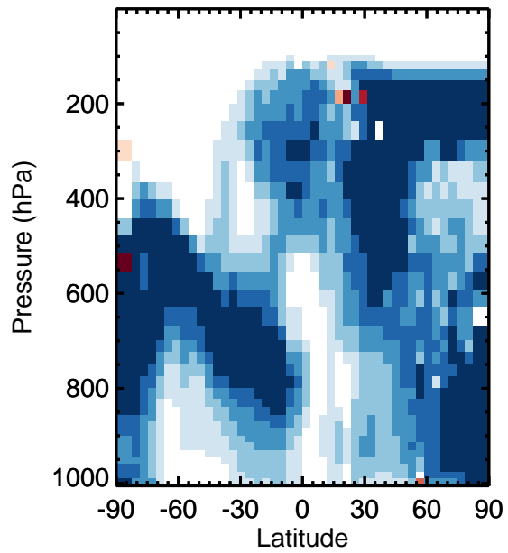
v11-01k-Run0 - v11-01f-geosfp-Run0 / v11-01k-Run0 / v11-01f-geosfp-Run0 NH3 - Zonal mean abs diff for Apr NH3 - Zonal mean % diff for Apr
