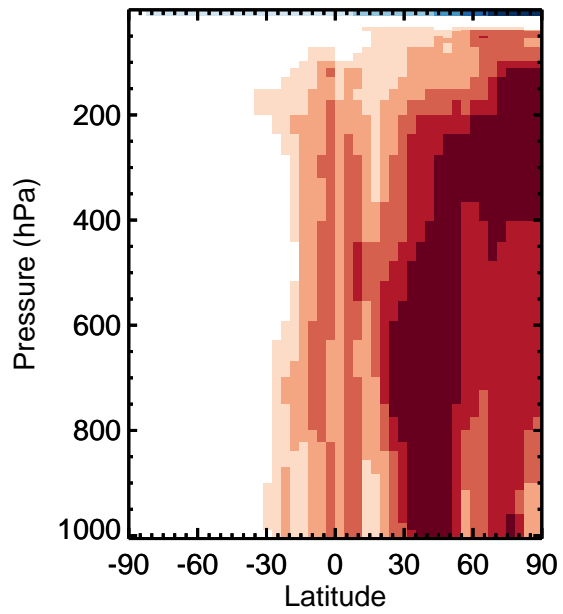
v11-01k-Run0 / v11-01g-Run0 DMS - Zonal mean % diff for Apr
