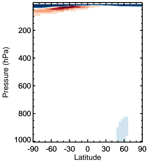
v11-01k-Run0 - v11-01g-Run0 O3 - Zonal mean abs diff for Jan
