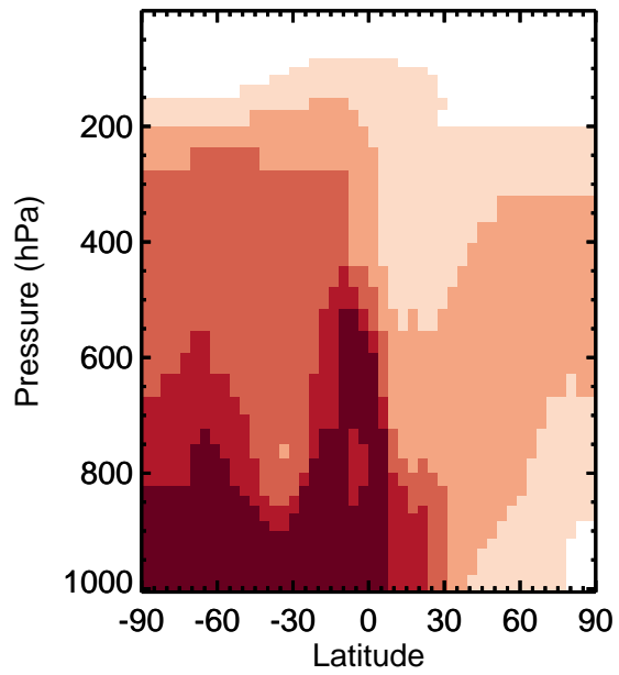
v11-01k-Run0 / v11-01g-Run0 BCPI - Zonal mean % diff for Jan
