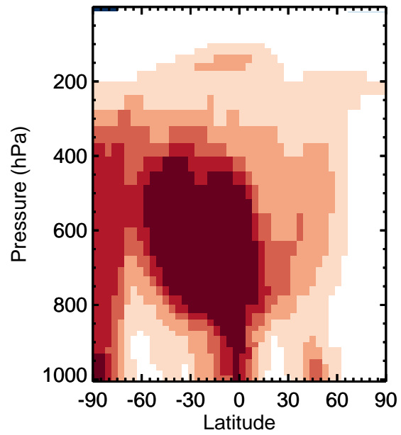
v11-01k-Run0 / v11-01g-Run0 Br2 - Zonal mean % diff for Jan
