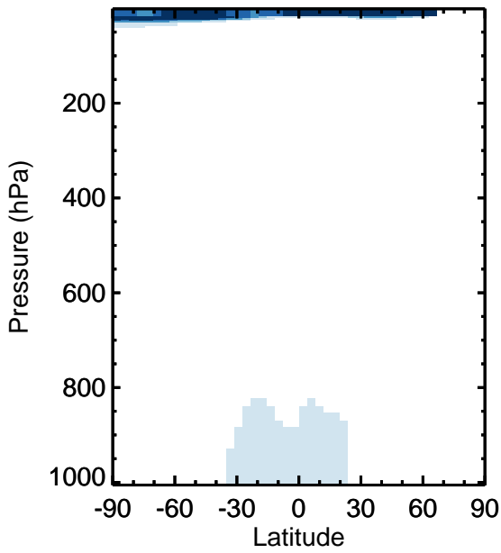
v11-01k-Run0 - v11-01g-Run0 HO2 - Zonal mean abs diff for Jan
