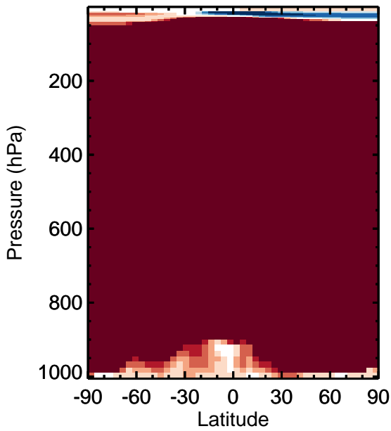
v11-01k-Run0 - v11-01f-geosfp-Run0 / v11-01k-Run0 / v11-01f-geosfp-Run0 N2O - Zonal mean abs diff for Jan N2O - Zonal mean % diff for Jan
