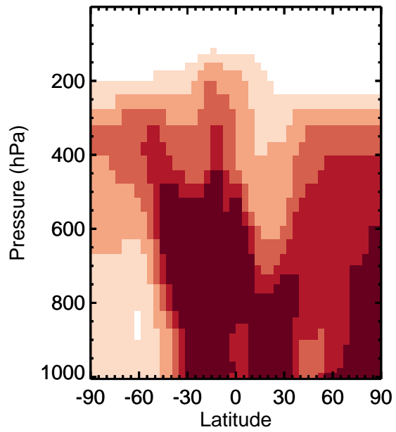
v11-01k-Run0 / v11-01g-Run0 SO4 - Zonal mean % diff for Jan
