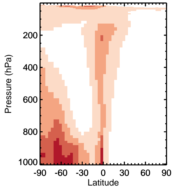
v11-01k-Run0 / v11-01g-Run0 MEK - Zonal mean % diff for Jan
