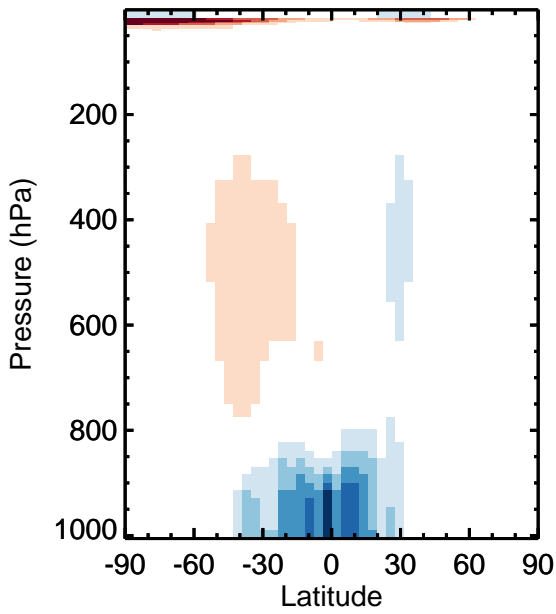
v11-01k-Run0 - v11-01g-Run0 OH - Zonal mean abs diff for Jan
