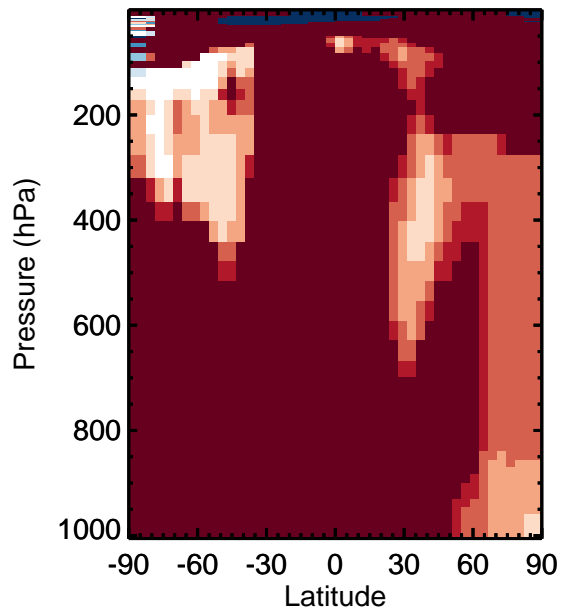
v11-01k-Run0 - v11-01f-geosfp-Run0 / v11-01k-Run0 / v11-01f-geosfp-Run0 MVK - Zonal mean abs diff for Jan MVK - Zonal mean % diff for Jan
