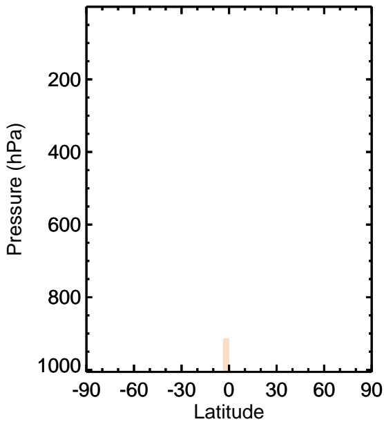
v11-01k-Run0 - v11-01g-Run0 MVK - Zonal mean abs diff for Jan
