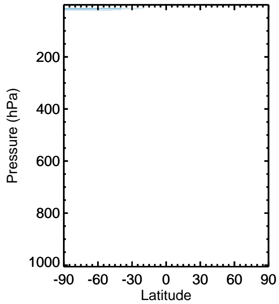
v11-01k-Run0 / v11-01g-Run0 OCS - Zonal mean % diff for Jan
