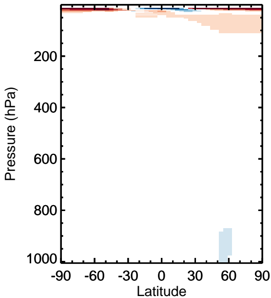
v11-01k-Run0 - v11-01f-geosfp-Run0 / v11-01k-Run0 / v11-01f-geosfp-Run0 O3 - Zonal mean abs diff for Jan O3 - Zonal mean % diff for Jan
