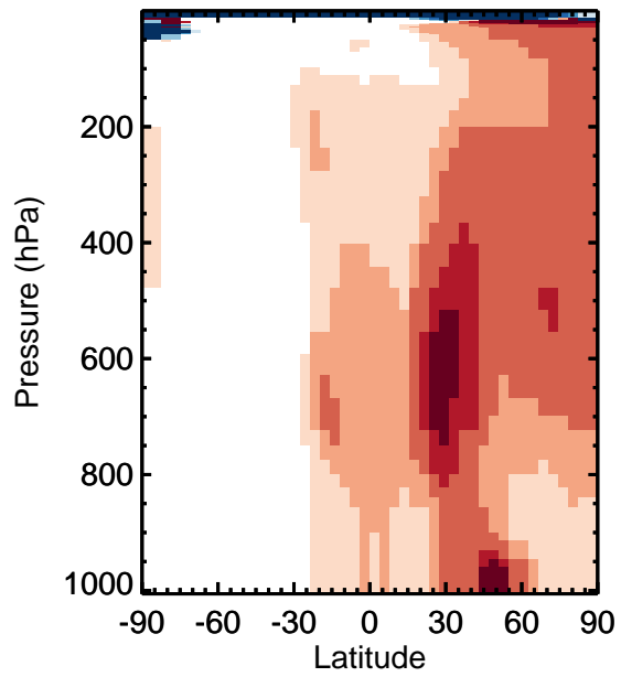
v11-01k-Run0 / v11-01g-Run0 DMS - Zonal mean % diff for Jan
