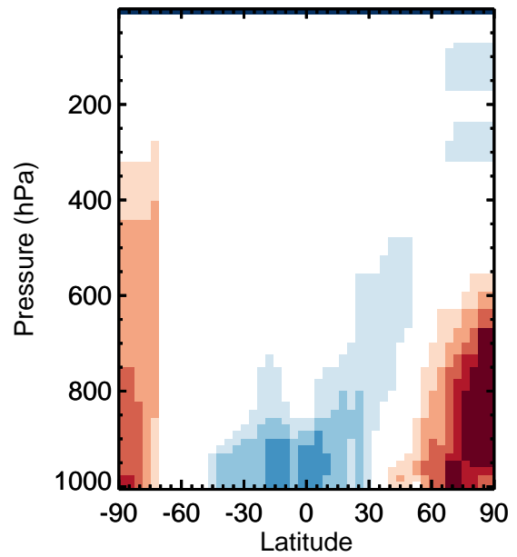
v11-01k-Run0 - v11-01f-geosfp-Run0 / v11-01k-Run0 / v11-01f-geosfp-Run0 NO3 - Zonal mean abs diff for Jan NO3 - Zonal mean % diff for Jan
