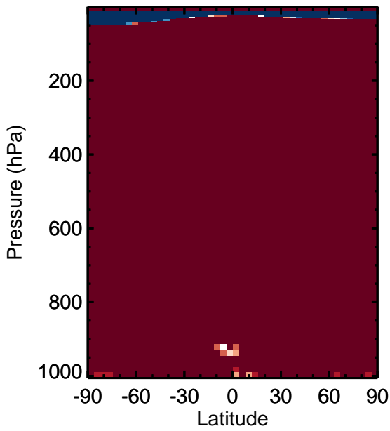
v11-01k-Run0 - v11-01g-Run0 CH4 - Zonal mean abs diff for Jan
