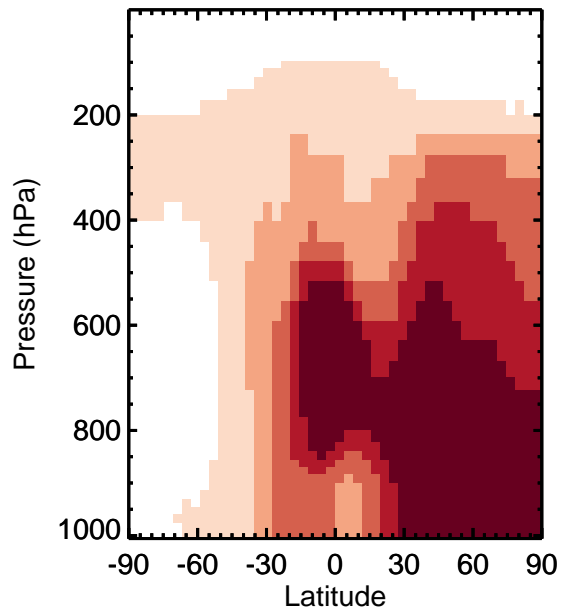
v11-01k-Run0 / v11-01g-Run0 MSA - Zonal mean % diff for Jan
