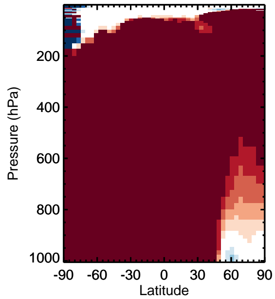
v11-01k-Run0 / v11-01g-Run0 RIP - Zonal mean % diff for Jan
