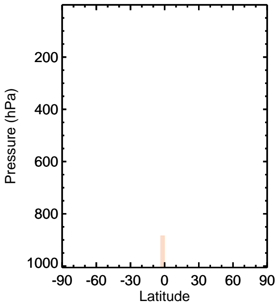
v11-01k-Run0 - v11-01g-Run0 HAC - Zonal mean abs diff for Jan
