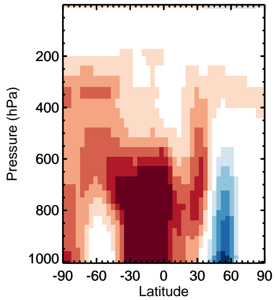
v11-01k-Run0 / v11-01g-Run0 BrCl - Zonal mean % diff for Jan
