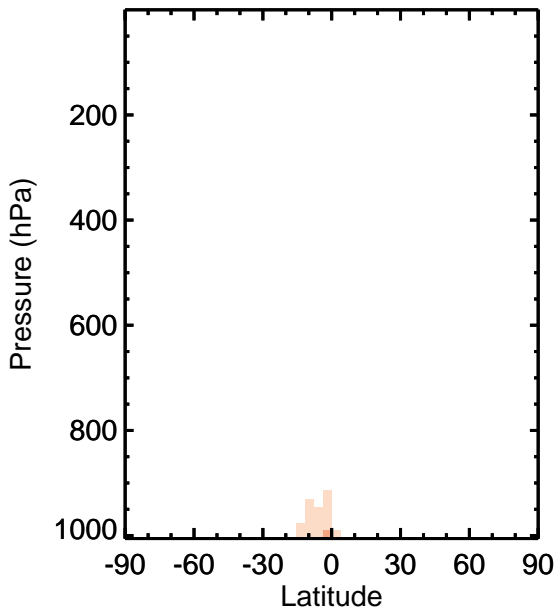
v11-01k-Run0 - v11-01g-Run0 ISOP - Zonal mean abs diff for Jan
