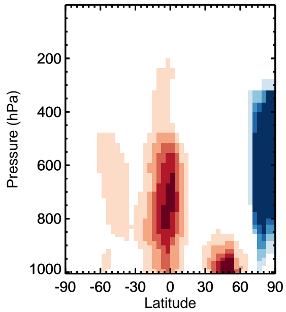
v11-01k-Run0 / v11-01g-Run0 HBr - Zonal mean % diff for Jan
