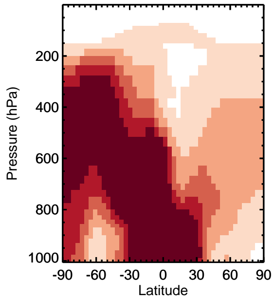
v11-01k-Run0 / v11-01g-Run0 NH4 - Zonal mean % diff for Jan
