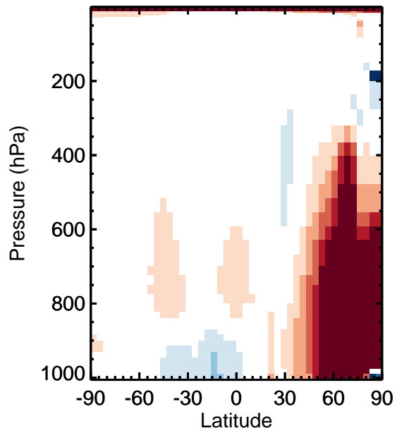
v11-01k-Run0 / v11-01g-Run0 NO - Zonal mean % diff for Jan
