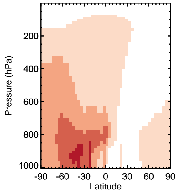
v11-01k-Run0 / v11-01g-Run0 PPN - Zonal mean % diff for Jan
