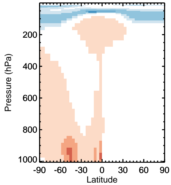
v11-01k-Run0 / v11-01g-Run0 MAP - Zonal mean % diff for Jan
