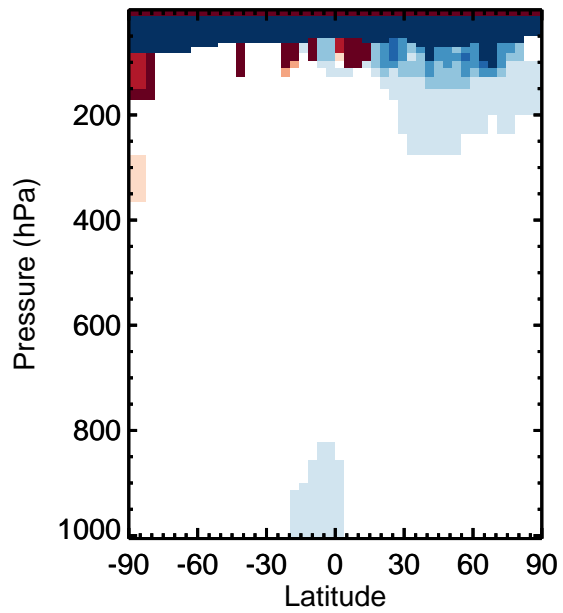
v11-01k-Run0 - v11-01f-geosfp-Run0 / v11-01k-Run0 / v11-01f-geosfp-Run0 SO 4 s - Zonal mean abs diff for Jan SO 4 s - Zonal mean % diff for Jan
