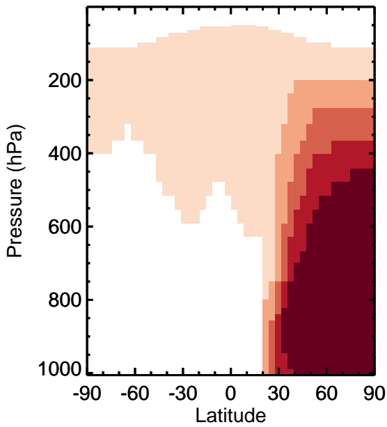
v11-01k-Run0 - v11-01f-geosfp-Run0 / v11-01k-Run0 / v11-01f-geosfp-Run0 PPN - Zonal mean abs diff for Jan PPN - Zonal mean % diff for Jan
