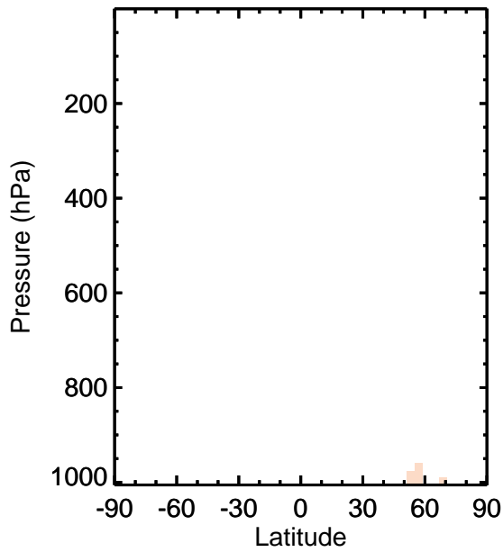
v11-01k-Run0 - v11-01f-geosfp-Run0 / v11-01k-Run0 / v11-01f-geosfp-Run0 SO2 - Zonal mean abs diff for Jan SO2 - Zonal mean % diff for Jan
