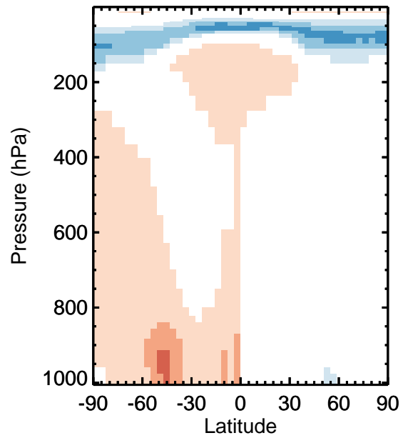
v11-01k-Run0 - v11-01f-geosfp-Run0 / v11-01k-Run0 / v11-01f-geosfp-Run0 MAP - Zonal mean abs diff for Jan MAP - Zonal mean % diff for Jan
