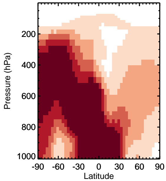
v11-01k-Run0 - v11-01f-geosfp-Run0 / v11-01k-Run0 / v11-01f-geosfp-Run0 NH4 - Zonal mean abs diff for Jan NH4 - Zonal mean % diff for Jan
