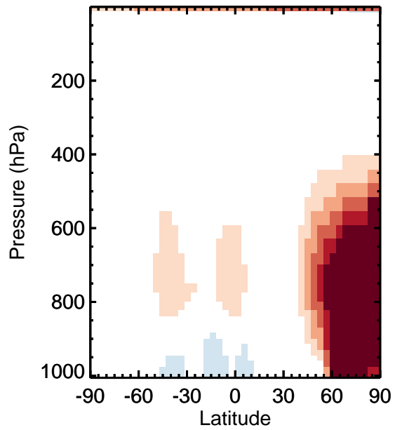
v11-01k-Run0 - v11-01f-geosfp-Run0 / v11-01k-Run0 / v11-01f-geosfp-Run0 MPN - Zonal mean abs diff for Jan MPN - Zonal mean % diff for Jan
