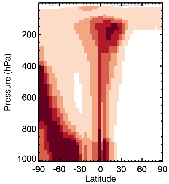
v11-01k-Run0 / v11-01g-Run0 HAC - Zonal mean % diff for Jan
