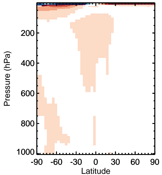
v11-01k-Run0 - v11-01f-geosfp-Run0 / v11-01k-Run0 / v11-01f-geosfp-Run0 ALK4 - Zonal mean abs diff for Jan ALK4 - Zonal mean % diff for Jan
