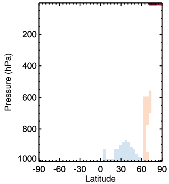
v11-01k-Run0 / v11-01g-Run0 HO2 - Zonal mean % diff for Jan
