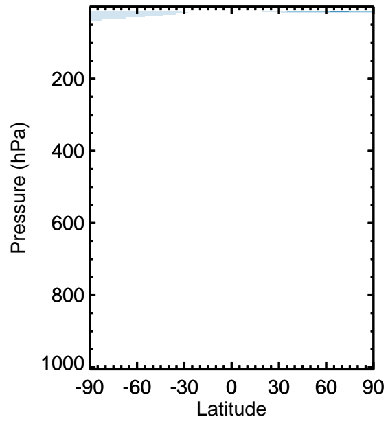
v11-01k-Run0 / v11-01g-Run0 MP - Zonal mean % diff for Jan
