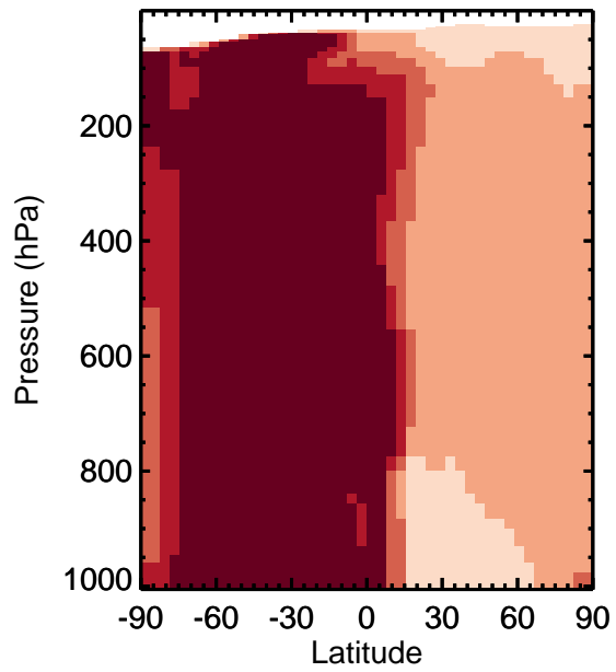
v11-01k-Run0 / v11-01g-Run0 NITs - Zonal mean % diff for Jan
