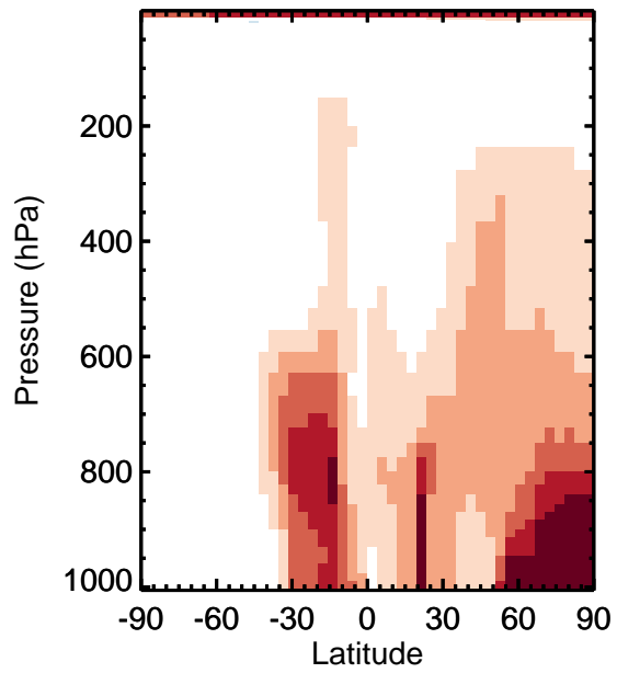
v11-01k-Run0 / v11-01g-Run0 SO2 - Zonal mean % diff for Jan
