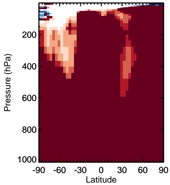
v11-01k-Run0 / v11-01g-Run0 MVK - Zonal mean % diff for Jan
