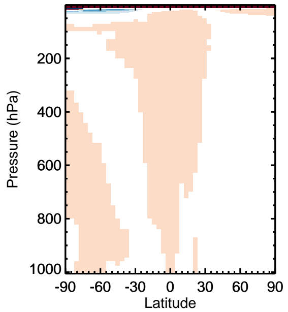
v11-01k-Run0 / v11-01g-Run0 ALK4 - Zonal mean % diff for Jan
