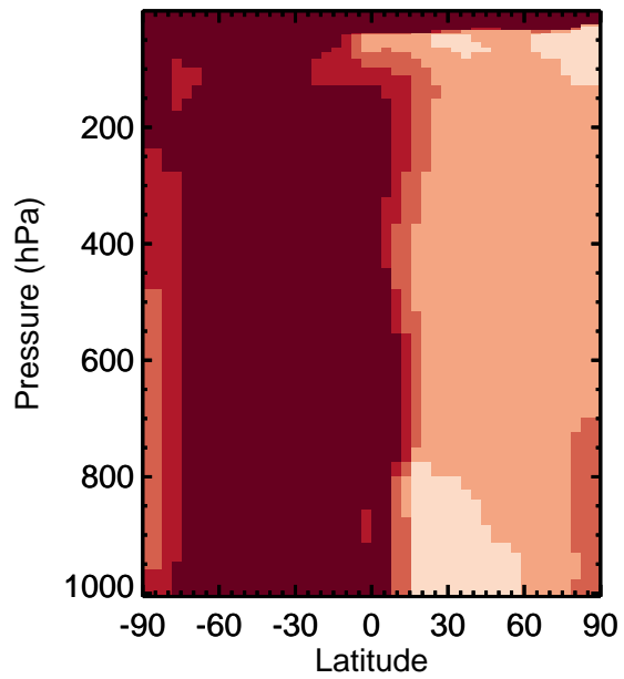
v11-01k-Run0 - v11-01f-geosfp-Run0 / v11-01k-Run0 / v11-01f-geosfp-Run0 NITs - Zonal mean abs diff for Jan NITs - Zonal mean % diff for Jan
