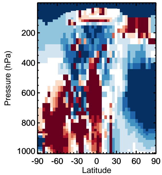
v11-01k-Run0 - v11-01f-geosfp-Run0 / v11-01k-Run0 / v11-01f-geosfp-Run0 NIT - Zonal mean abs diff for Jan NIT - Zonal mean % diff for Jan
