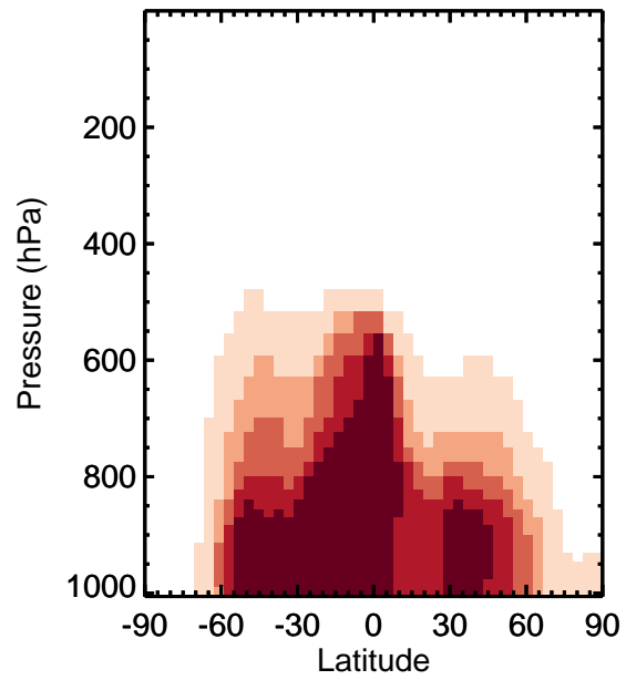
v11-01k-Run0 / v11-01g-Run0 HCl - Zonal mean % diff for Jan
