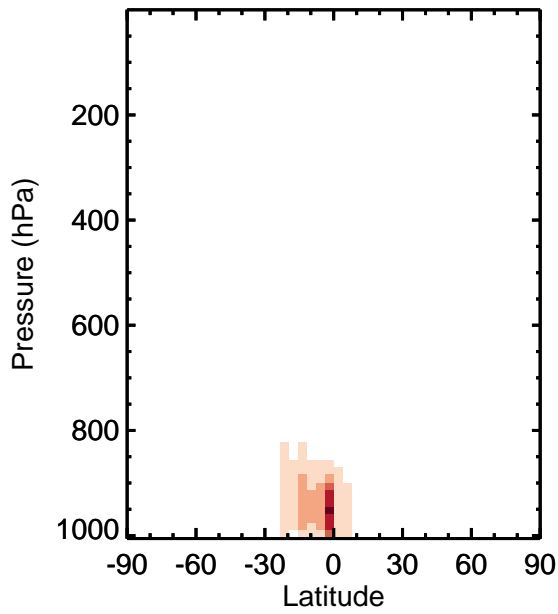
v11-01k-Run0 - v11-01g-Run0 RIP - Zonal mean abs diff for Jan
