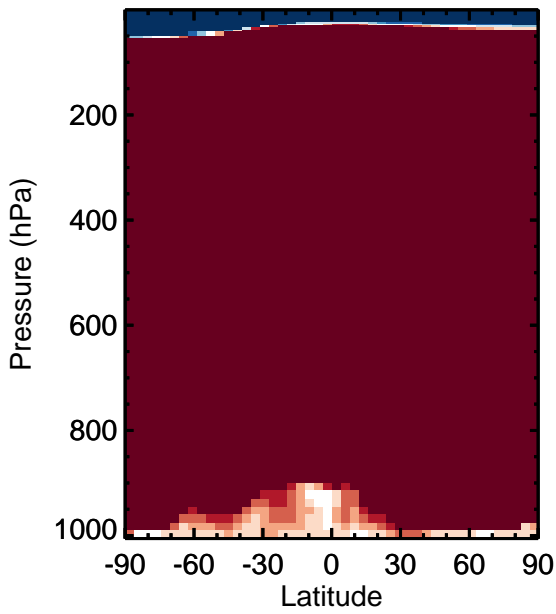
v11-01k-Run0 - v11-01g-Run0 N2O - Zonal mean abs diff for Jan
