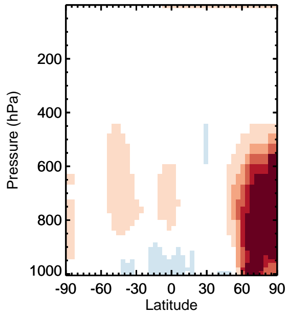
v11-01k-Run0 / v11-01g-Run0 MPN - Zonal mean % diff for Jan
