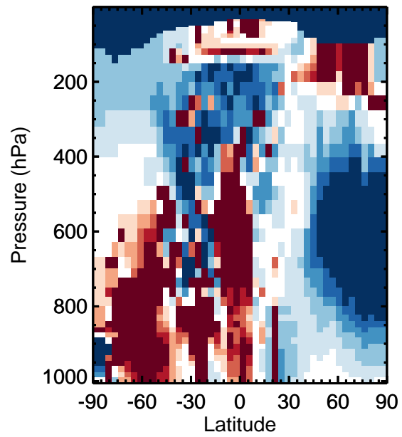
v11-01k-Run0 / v11-01g-Run0 NIT - Zonal mean % diff for Jan
