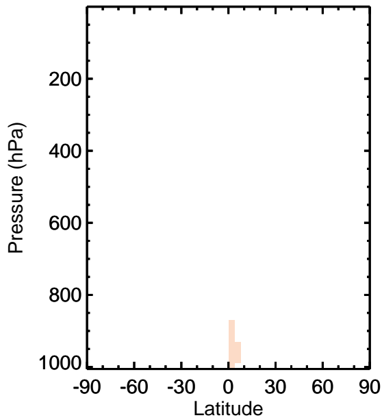
v11-01k-Run0 - v11-01f-geosfp-Run0 / v11-01k-Run0 / v11-01f-geosfp-Run0 OCPI - Zonal mean abs diff for Jan OCPI - Zonal mean % diff for Jan
