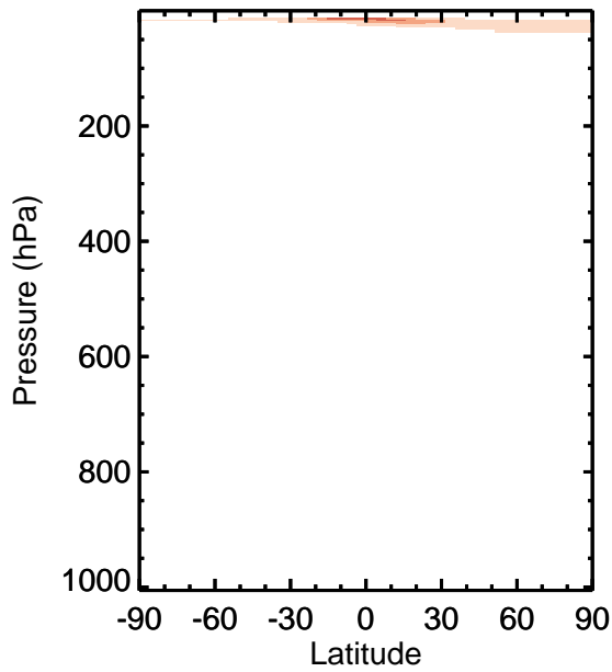
v11-01k-Run0 - v11-01f-geosfp-Run0 / v11-01k-Run0 / v11-01f-geosfp-Run0 HCl - Zonal mean abs diff for Jan HCl - Zonal mean % diff for Jan
