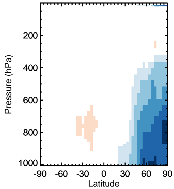
v11-01k-Run0 / v11-01g-Run0 CIO - Zonal mean % diff for Jan
