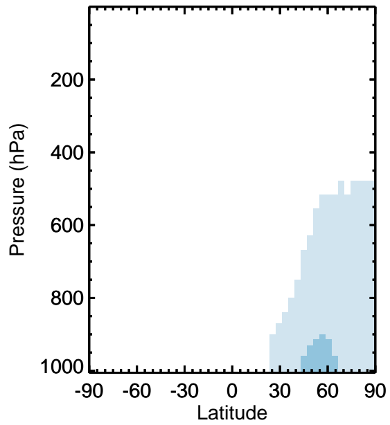
v11-01k-Run0 / v11-01g-Run0 O3 - Zonal mean % diff for Jan
