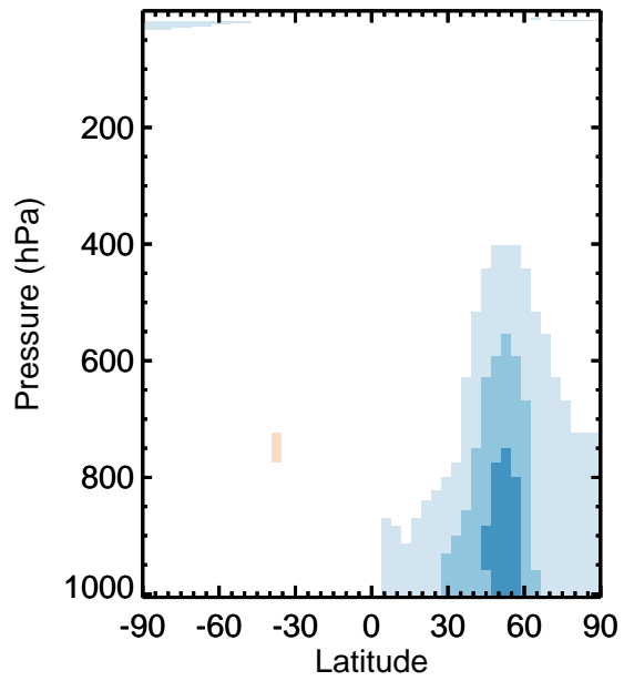
v11-01k-Run0 / v11-01g-Run0 HOCl - Zonal mean % diff for Jan
