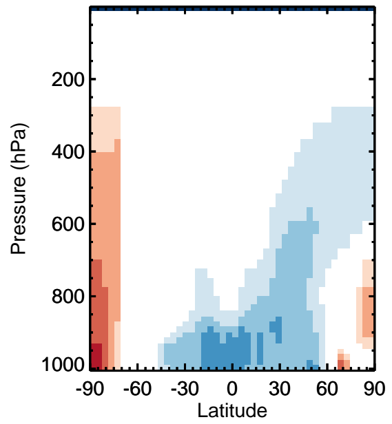
v11-01k-Run0 / v11-01g-Run0 NO3 - Zonal mean % diff for Jan
