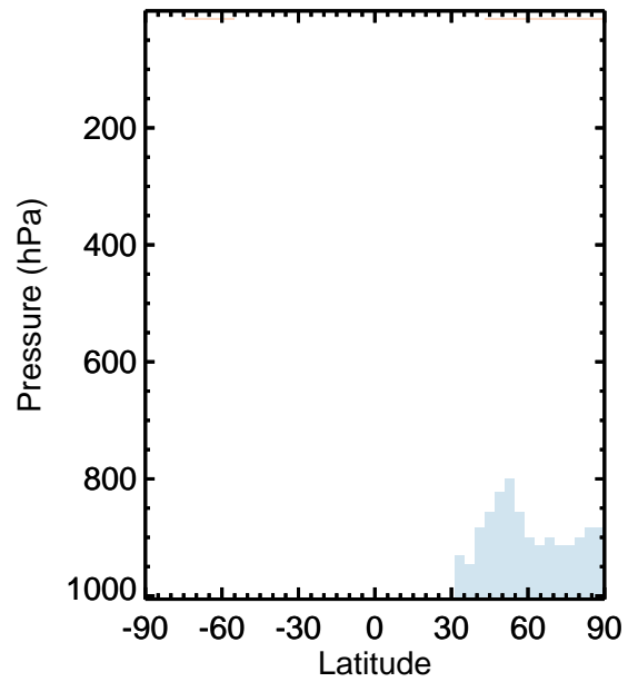
v11-01k-Run0 - v11-01f-geosfp-Run0 / v11-01k-Run0 / v11-01f-geosfp-Run0 MP - Zonal mean abs diff for Jan MP - Zonal mean % diff for Jan
