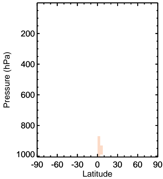
v11-01k-Run0 - v11-01g-Run0 OCPI - Zonal mean abs diff for Jan
