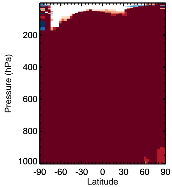
v11-01k-Run0 / v11-01g-Run0 ISOP - Zonal mean % diff for Jan
