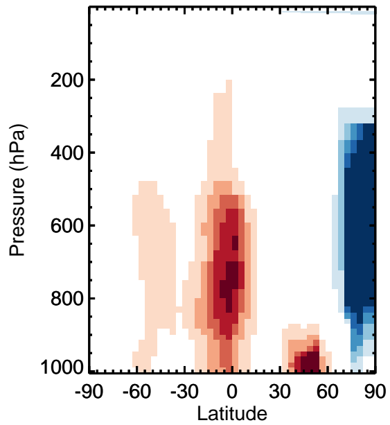
v11-01k-Run0 - v11-01f-geosfp-Run0 / v11-01k-Run0 / v11-01f-geosfp-Run0 HBr - Zonal mean abs diff for Jan HBr - Zonal mean % diff for Jan
