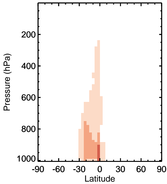
v11-01k-Run0 - v11-01g-Run0 MAP - Zonal mean abs diff for Jan
