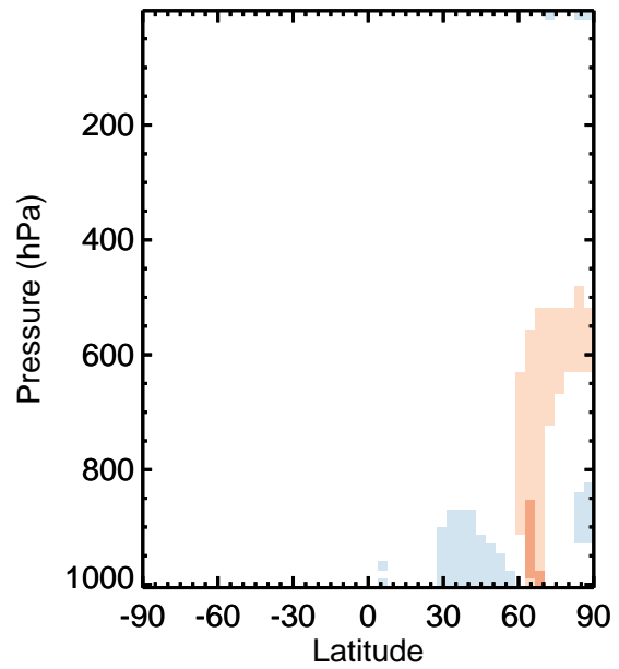
v11-01k-Run0 - v11-01f-geosfp-Run0 / v11-01k-Run0 / v11-01f-geosfp-Run0 HO2 - Zonal mean abs diff for Jan HO2 - Zonal mean % diff for Jan
