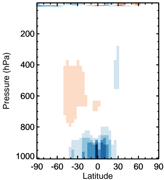
v11-01k-Run0 - v11-01f-geosp-Run0 / v11-01k-Run0 / v11-01f-geosp-Run0 OH - Zonal mean abs diff for Jan OH - Zonal mean % diff for Jan
