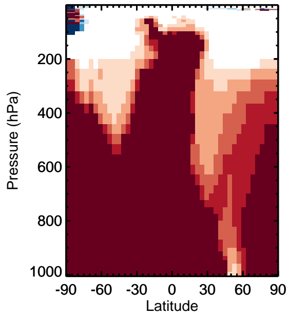
v11-01k-Run0 / v11-01g-Run0 PMN - Zonal mean % diff for Jan
