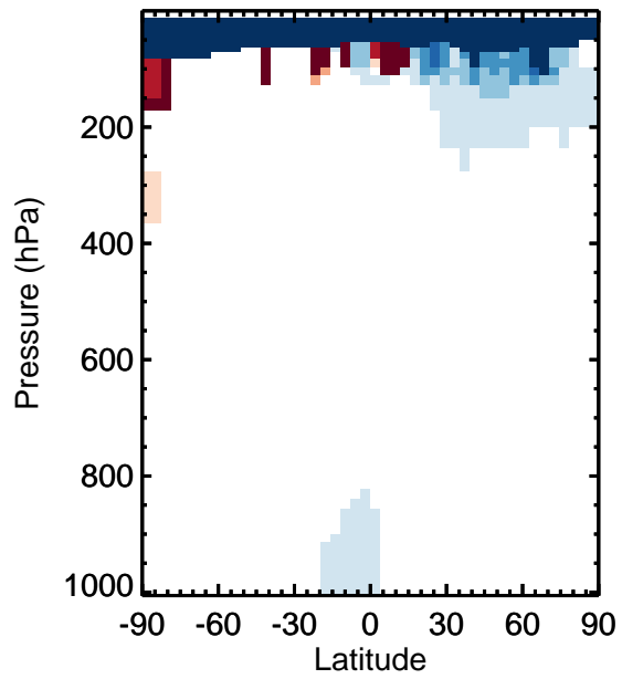
v11-01k-Run0 / v11-01g-Run0 SO 4 s - Zonal mean % diff for Jan
