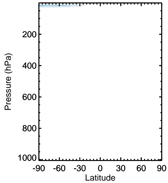
v11-01k-Run0 / v11-01g-Run0 CCI4 - Zonal mean % diff for Jan
