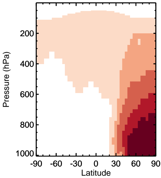
v11-01k-Run0 - v11-01g-Run0 PPN - Zonal mean abs diff for Jan
