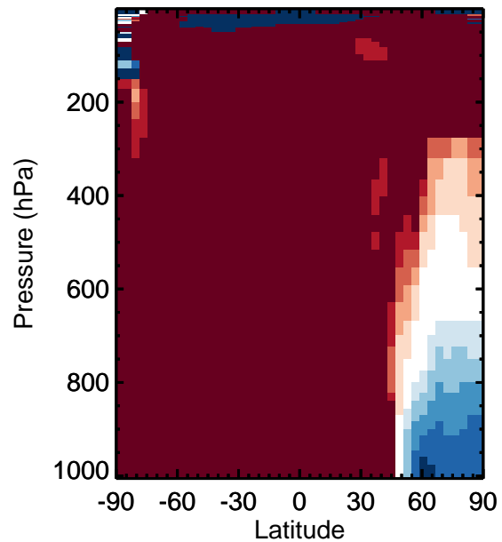
v11-01k-Run0 - v11-01f-geosfp-Run0 / v11-01k-Run0 / v11-01f-geosfp-Run0 RIP - Zonal mean abs diff for Jan RIP - Zonal mean % diff for Jan
