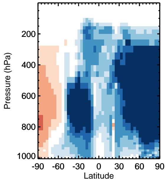
v11-01k-Run0 / v11-01g-Run0 NH3 - Zonal mean % diff for Jan
