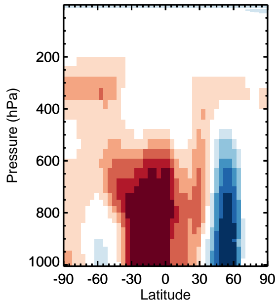
v11-01k-Run0 - v11-01f-geosfp-Run0 / v11-01k-Run0 / v11-01f-geosfp-Run0 BrCl - Zonal mean abs diff for Jan BrCl - Zonal mean % diff for Jan
