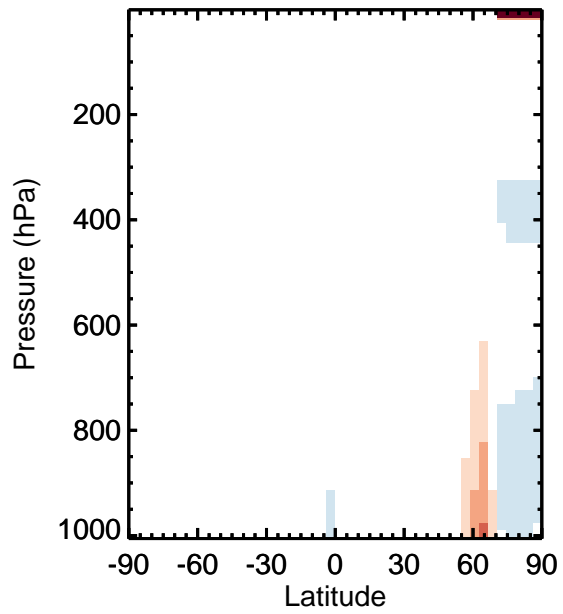
v11-01k-Run0 / v11-01g-Run0 OH - Zonal mean % diff for Jan
