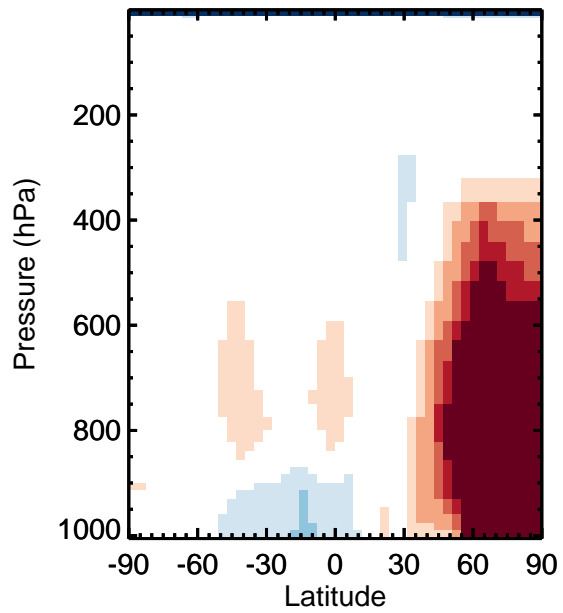
v11-01k-Run0 - v11-01f-geosfp-Run0 / v11-01k-Run0 / v11-01f-geosfp-Run0 NO 2 - Zonal mean abs diff for Jan NO 2 - Zonal mean % diff for Jan
