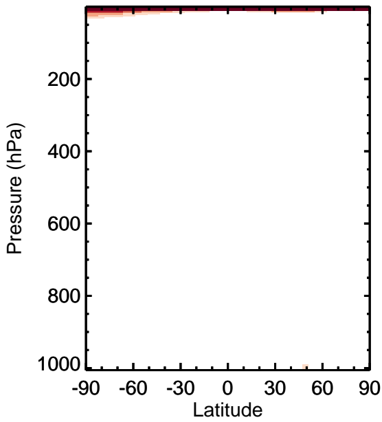
v11-01k-Run0 - v11-01g-Run0 NO - Zonal mean abs diff for Jan
