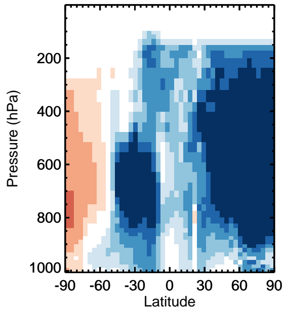
v11-01k-Run0 - v11-01f-geosfp-Run0 / v11-01k-Run0 / v11-01f-geosfp-Run0 NH3 - Zonal mean abs diff for Jan NH3 - Zonal mean % diff for Jan
