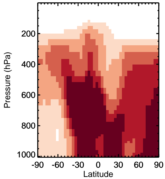
v11-01k-Run0 - v11-01f-geosfp-Run0 / v11-01k-Run0 / v11-01f-geosfp-Run0 SO4 - Zonal mean abs diff for Jan SO4 - Zonal mean % diff for Jan
