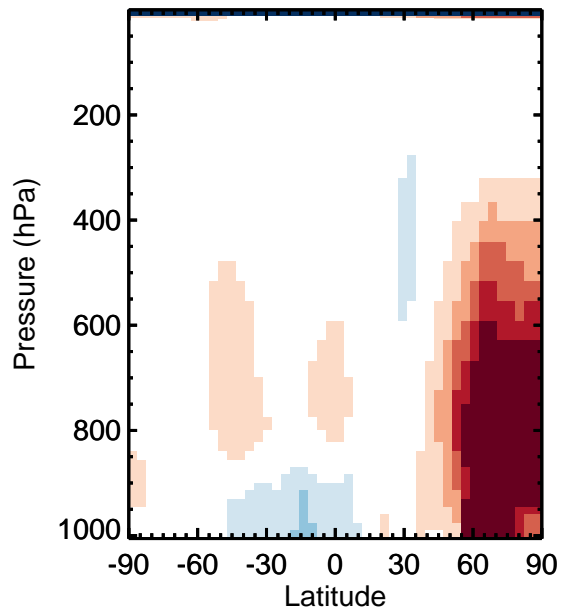
v11-01k-Run0 / v11-01g-Run0 NO 2 - Zonal mean % diff for Jan
