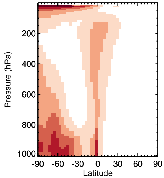
v11-01k-Run0 - v11-01f-geosfp-Run0 / v11-01k-Run0 / v11-01f-geosfp-Run0 MEK - Zonal mean abs diff for Jan MEK - Zonal mean % diff for Jan
