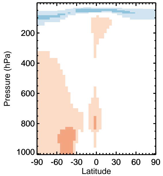
v11-01k-Run0 - v11-01f-geosfp-Run0 / v11-01k-Run0 / v11-01f-geosfp-Run0 PAN - Zonal mean abs diff for Jan PAN - Zonal mean % diff for Jan
