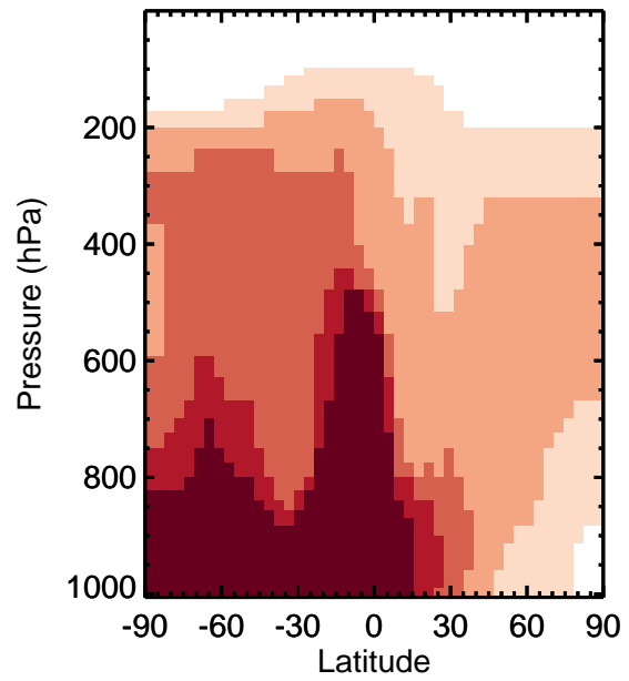
v11-01k-Run0 / v11-01g-Run0 OCPI - Zonal mean % diff for Jan
