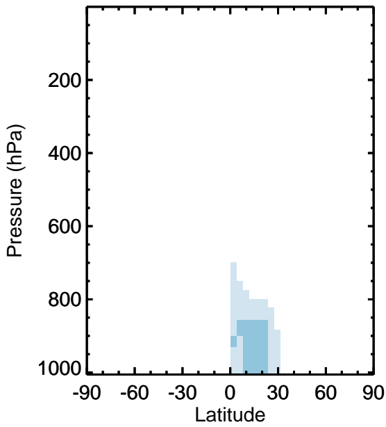
v11-01k-Run0 - v11-01g-Run0 MP - Zonal mean abs diff for Jan
