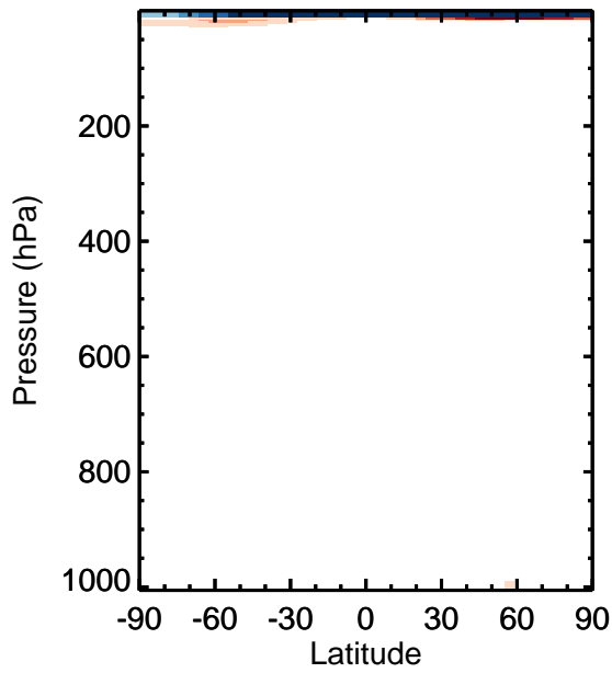
v11-01k-Run0 - v11-01g-Run0 NO 2 - Zonal mean abs diff for Jan
