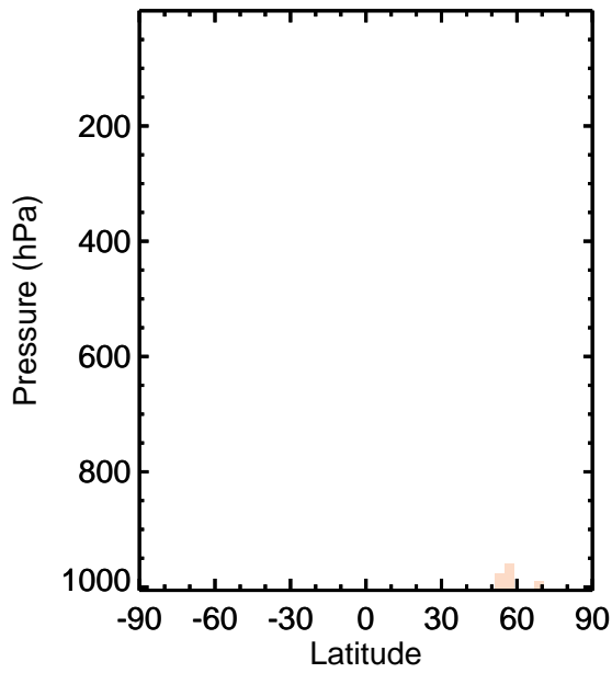
v11-01k-Run0 - v11-01g-Run0 SO2 - Zonal mean abs diff for Jan
