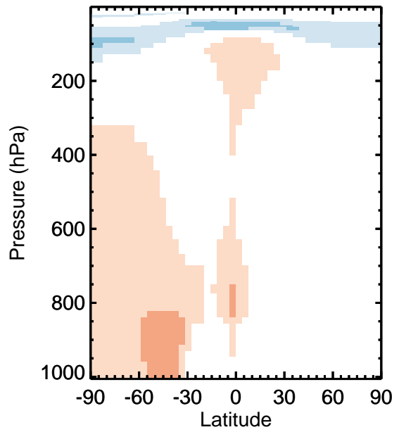
v11-01k-Run0 / v11-01g-Run0 PAN - Zonal mean % diff for Jan
