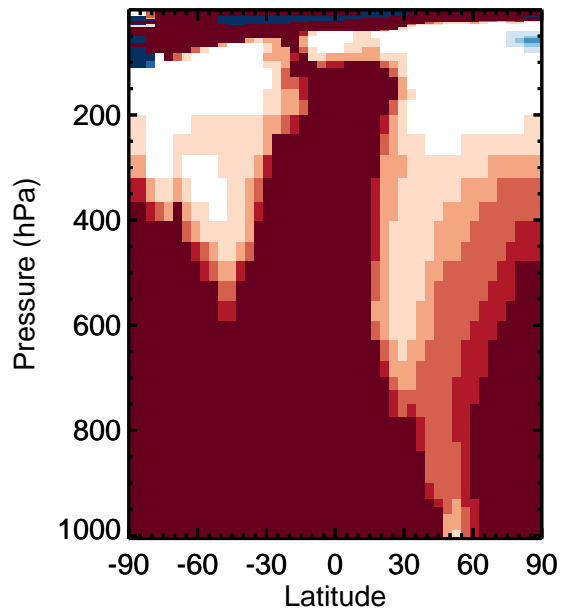
v11-01k-Run0 - v11-01f-geosfp-Run0 / v11-01k-Run0 / v11-01f-geosfp-Run0 PMN - Zonal mean abs diff for Jan PMN - Zonal mean % diff for Jan
