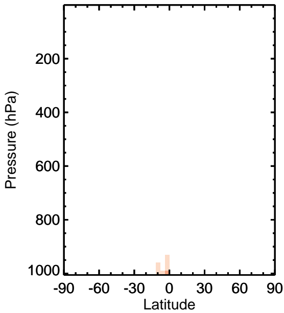
v11-01k-Run0 - v11-01f-geosfp-Run0 / v11-01k-Run0 / v11-01f-geosfp-Run0 ISOP - Zonal mean abs diff for Jan ISOP - Zonal mean % diff for Jan
