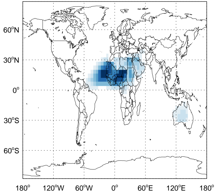
v11-02a - v11-01k-Run0 SALC: Column AOD diff for Jan
