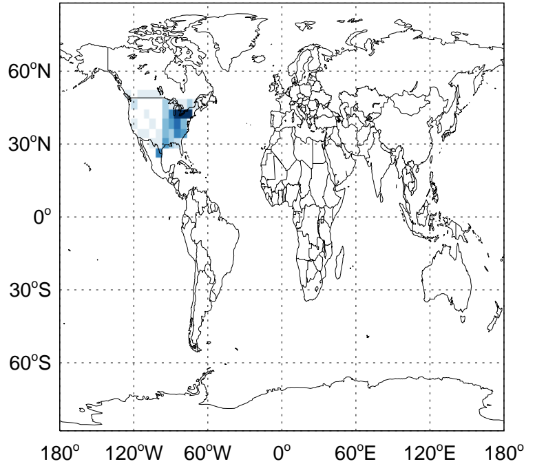
PRPE column anth+biof emissions for Jul
