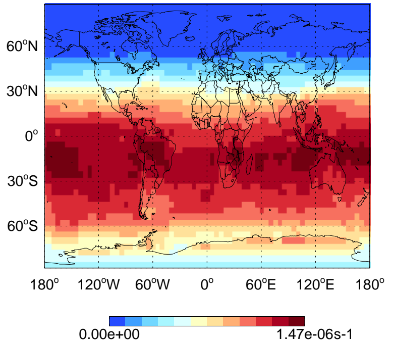
JHNO3 - J-Value @ 500 hPa for Jan
