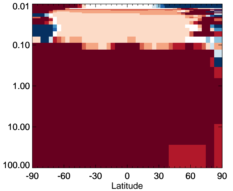
PRPE - Strat zonal mean % diff for Apr
