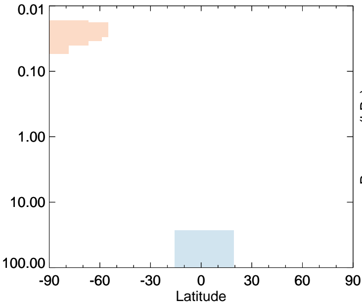
OH - Strat zonal mean abs diff for Jan
