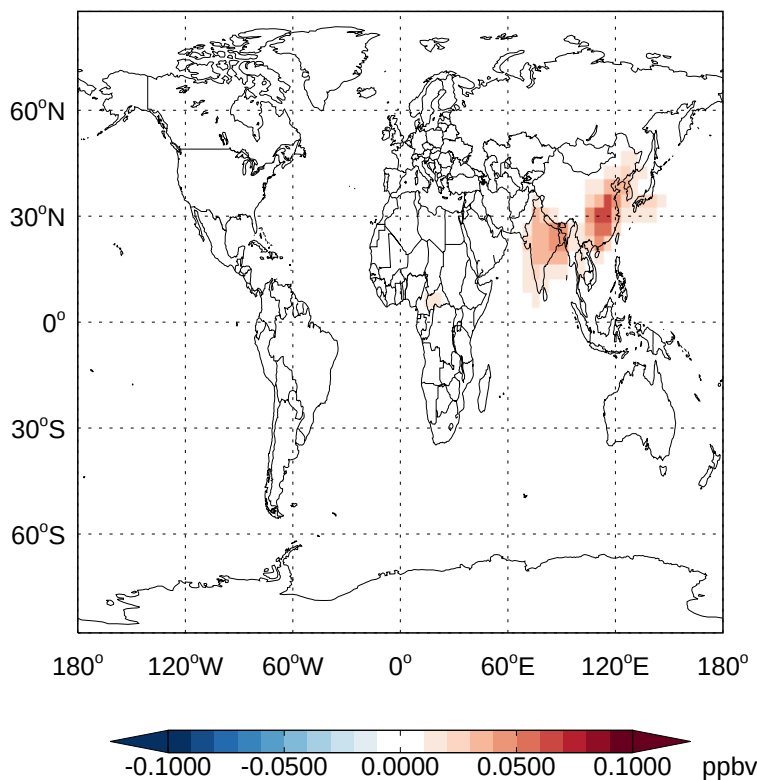
v11-02a - v11-01k-Run0 ASOG3 - Diff @ Surface for Jan
