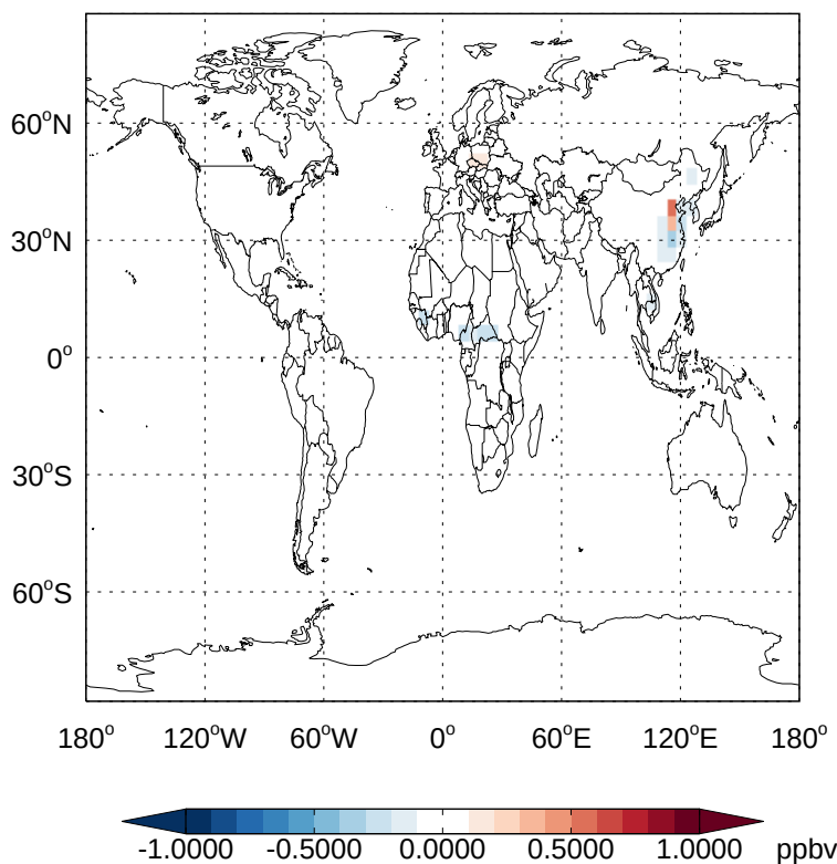
v11-02a - v11-01k-Run0 HNO 2 - Diff @ Surface for Jan
