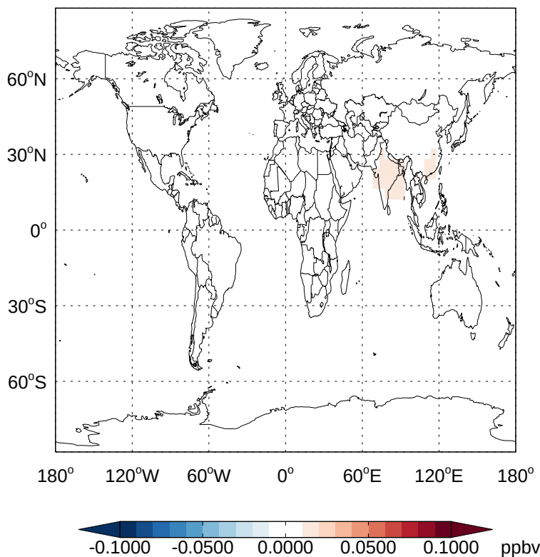
v11-02a - v11-01k-Run0 ASOG2 - Diff @ Surface for Jan
