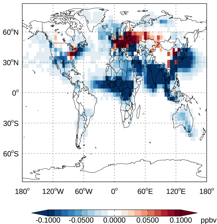
v11-02a - v11-01k-Run0 HNO 3 - Diff @ Surface for Jan
