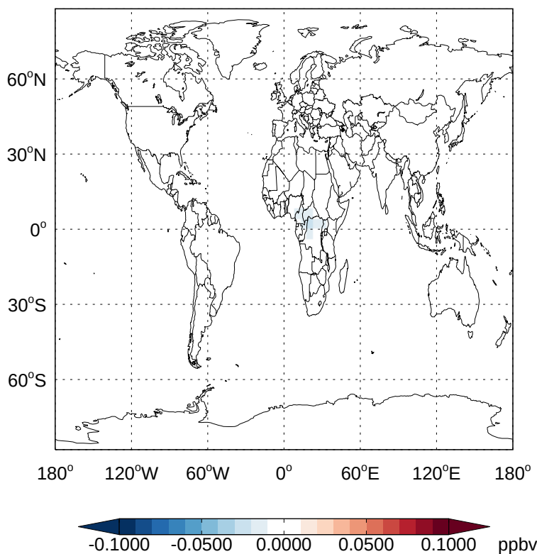
v11-02a - v11-01k-Run0 ISOA2 - Diff @ Surface for Jan
