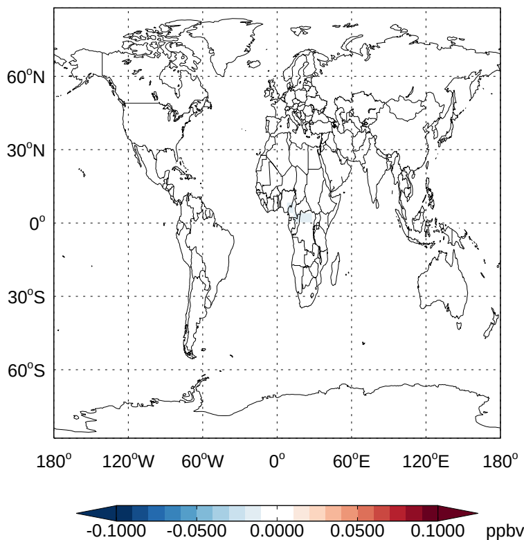
v11-02a - v11-01k-Run0 PROPNN - Diff @ Surface for Jan
