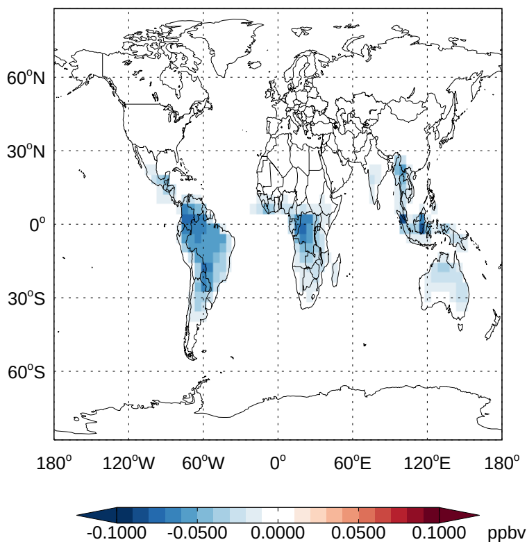
v11-02a - v11-01k-Run0 TSOG2 - Diff @ Surface for Jan
