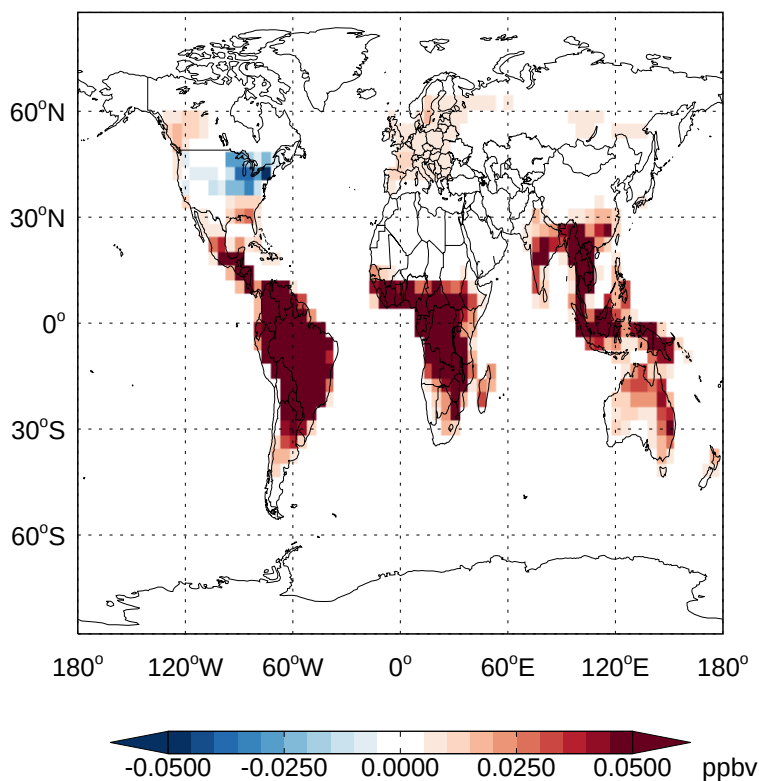
v11-02a - v11-01k-Run0 RCHO - Diff @ Surface for Jan
