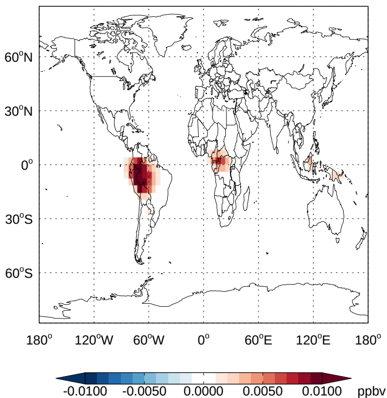
v11-02a - v11-01k-Run0 IEPOX- Diff @ 500 hPa for Jan
