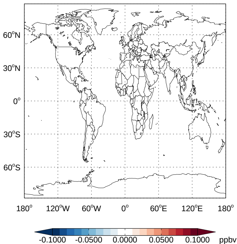
v11-02a - v11-01k-Run0 HCFC142b - Diff @ Surface for Jan
