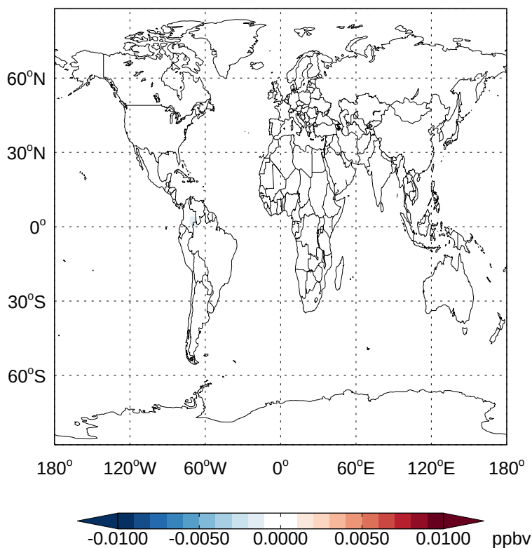
v11-02a - v11-01k-Run0 MOBA - Diff @ Surface for Jan
