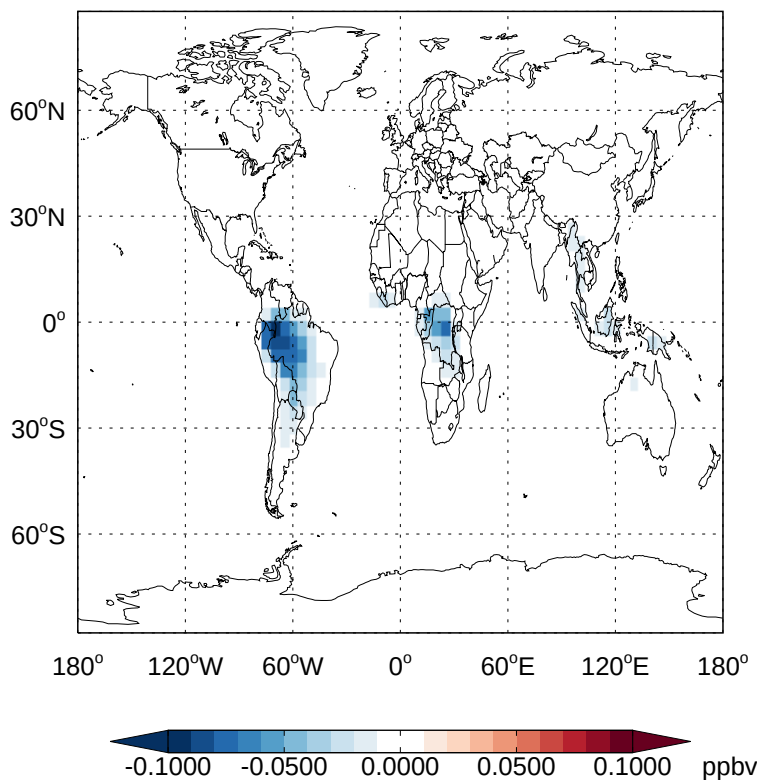
v11-02a - v11-01k-Run0 TSOA0 - Diff @ Surface for Jan
