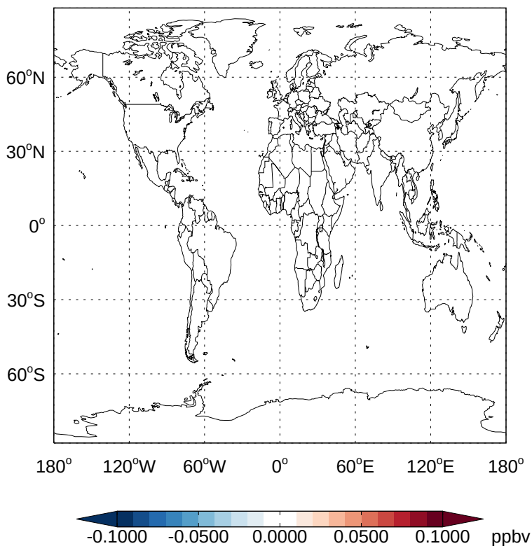
v11-02a - v11-01k-Run0 ISOPNB- Diff @ 500 hPa for Jan
