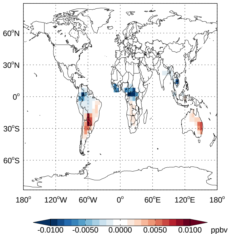
v11-02a - v11-01k-Run0 MVKN - Diff @ Surface for Jan
