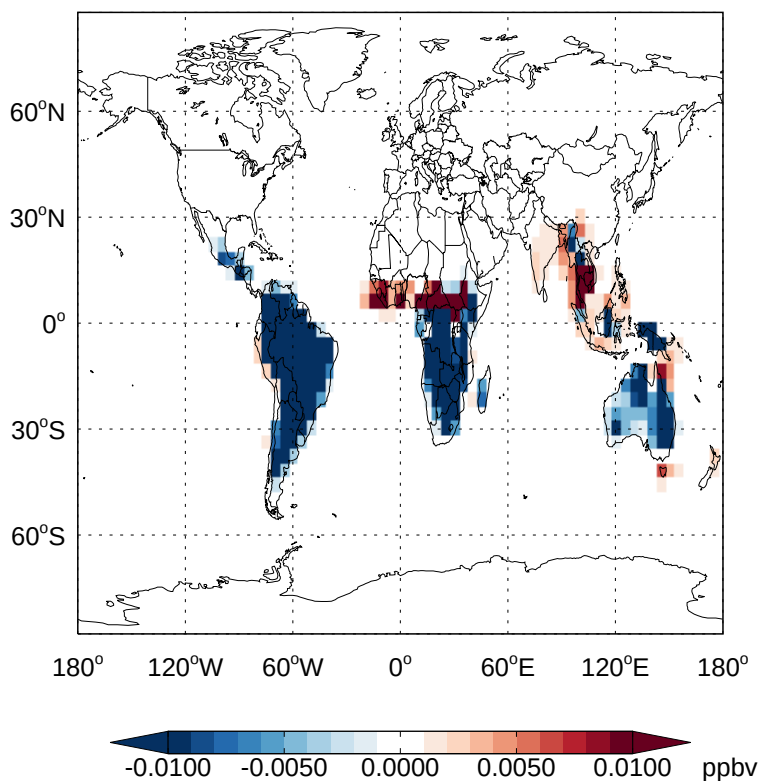
v11-02a - v11-01k-Run0 IEPOX - Diff @ Surface for Jan
