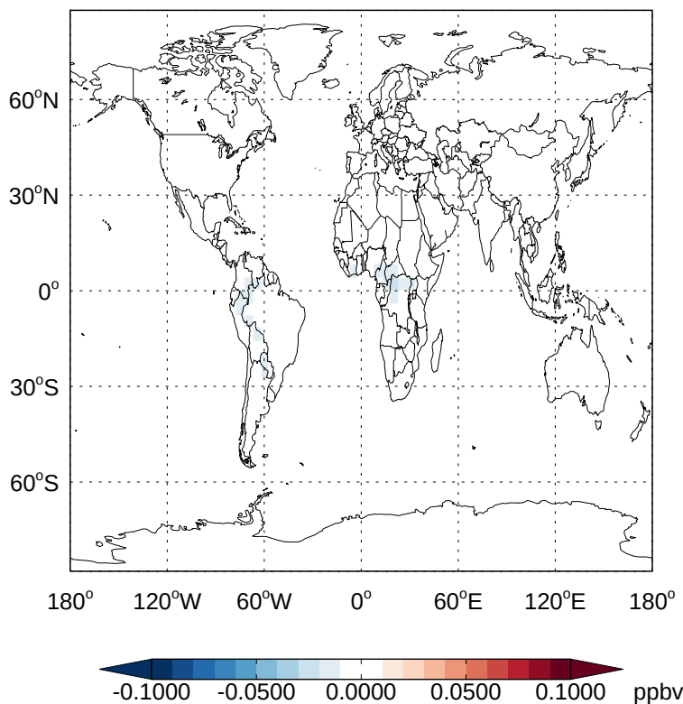
v11-02a - v11-01k-Run0 ISOG3 - Diff @ Surface for Jan
