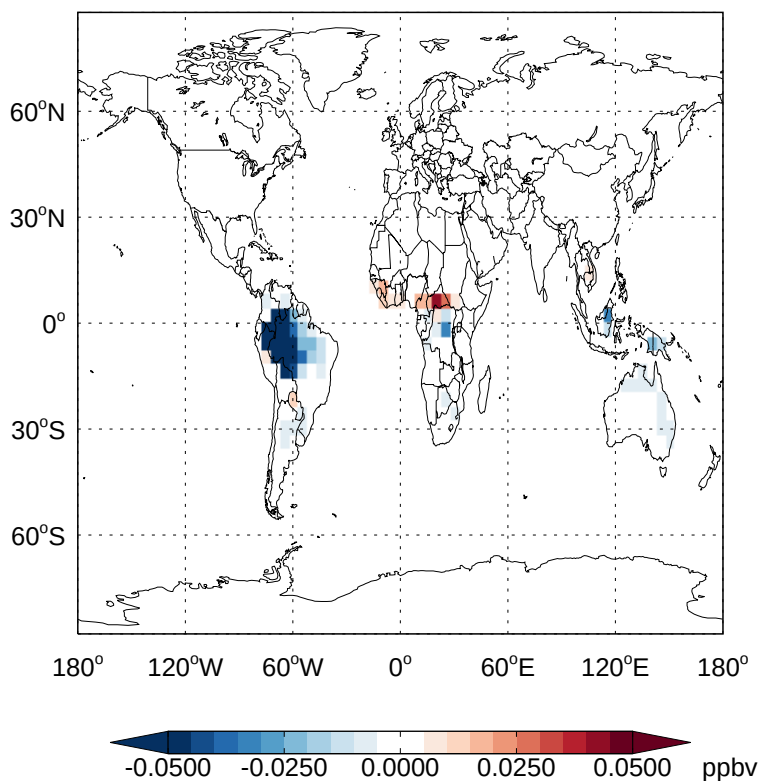
v11-02a - v11-01k-Run0 MACR - Diff @ Surface for Jan
