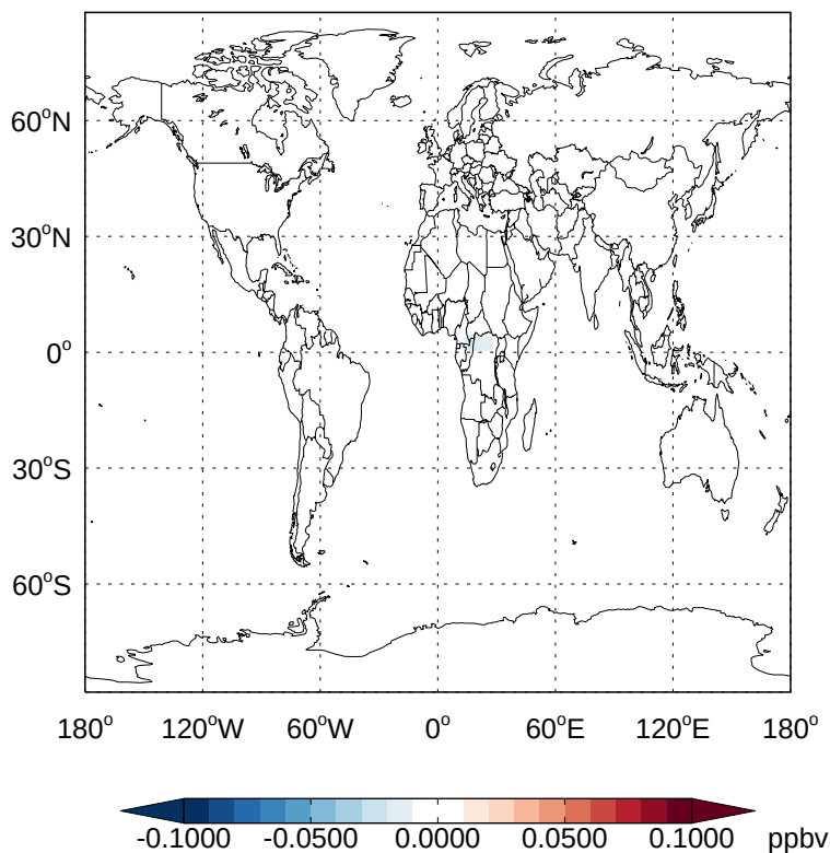
v11-02a - v11-01k-Run0 ISOA3 - Diff @ Surface for Jan
