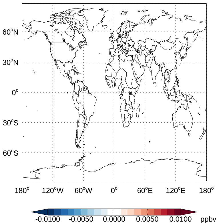
v11-02a - v11-01k-Run0 CH 2 Br 2 - Diff @ 500 hPa for Jan
