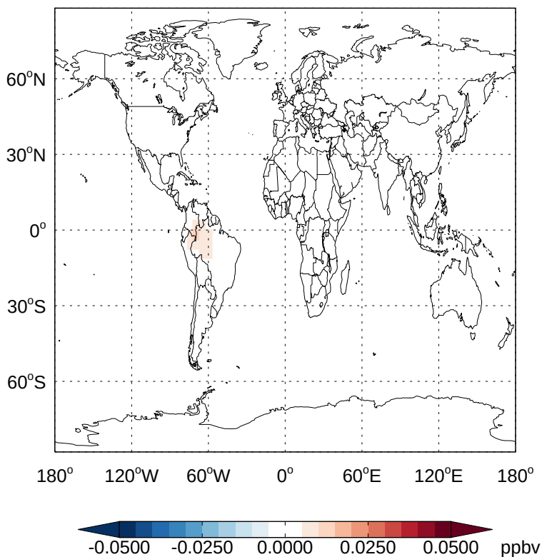
v11-02a - v11-01k-Run0 RCHO- Diff @ 500 hPa for Jan
