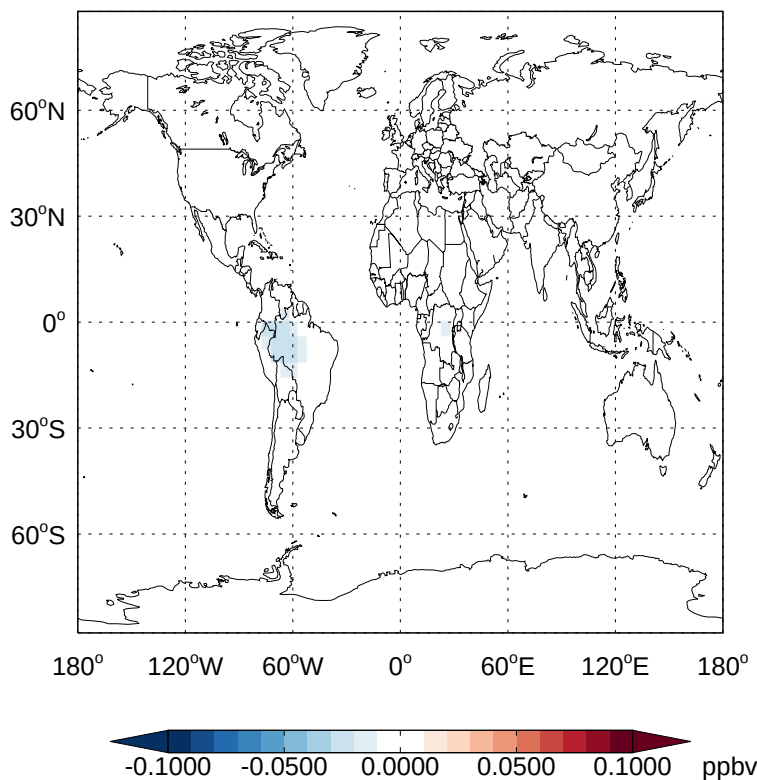
v11-02a - v11-01k-Run0 TSOA1 - Diff @ Surface for Jan
