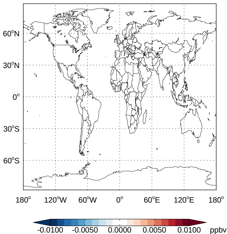
v11-02a - v11-01k-Run0 CH 2 Br 2 - Diff @ Surface for Jan
