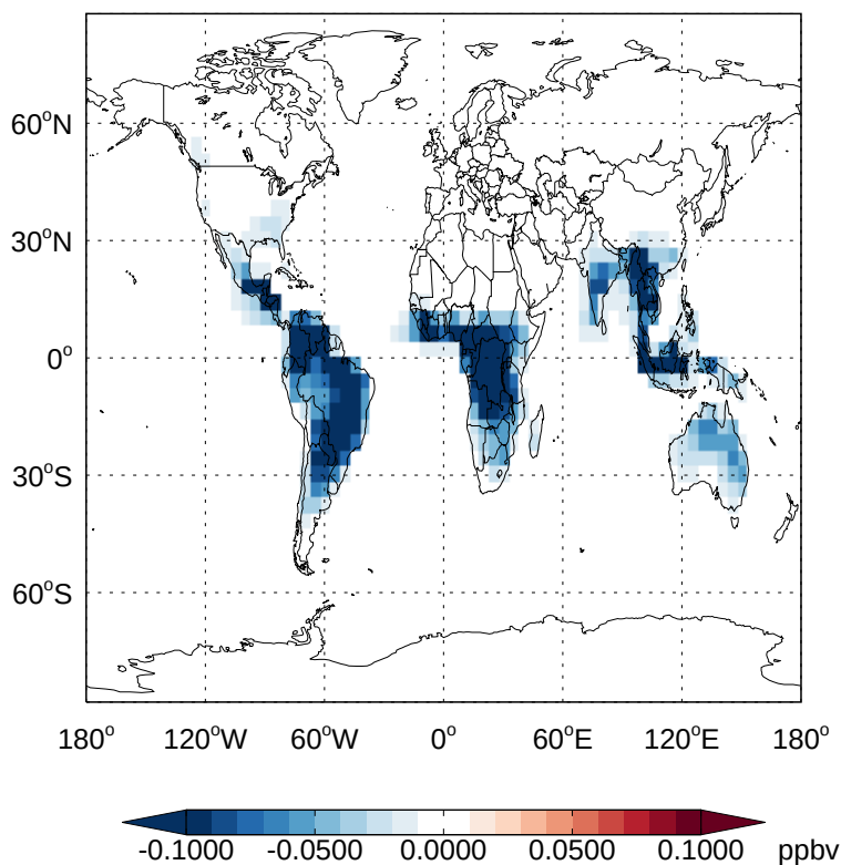
v11-02a - v11-01k-Run0 TSOG3 - Diff @ Surface for Jan
