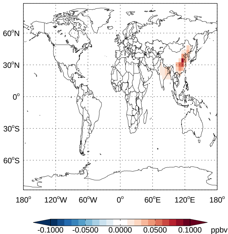
v11-02a - v11-01k-Run0 ASOA2 - Diff @ Surface for Jan
