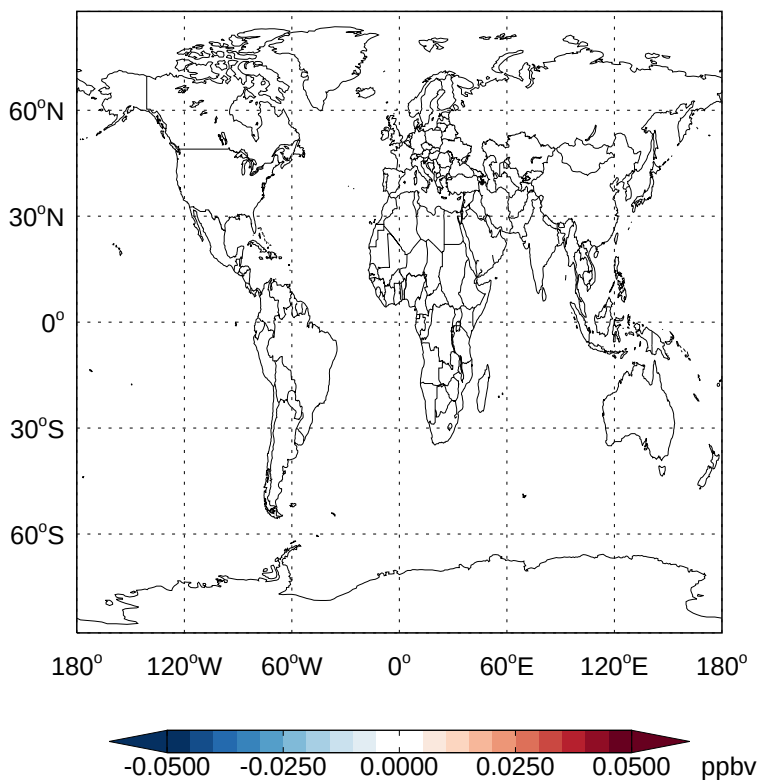
v11-02a - v11-01k-Run0 MACR - Diff @ 500 hPa for Jan
