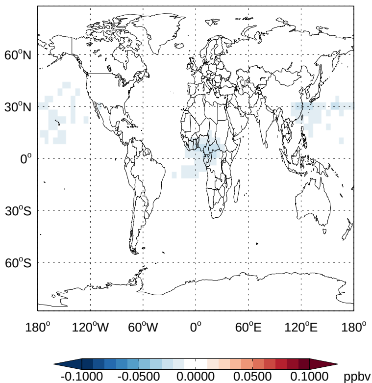
v11-02a - v11-01k-Run0 HNO 3 - Diff @ 500 hPa for Jan
