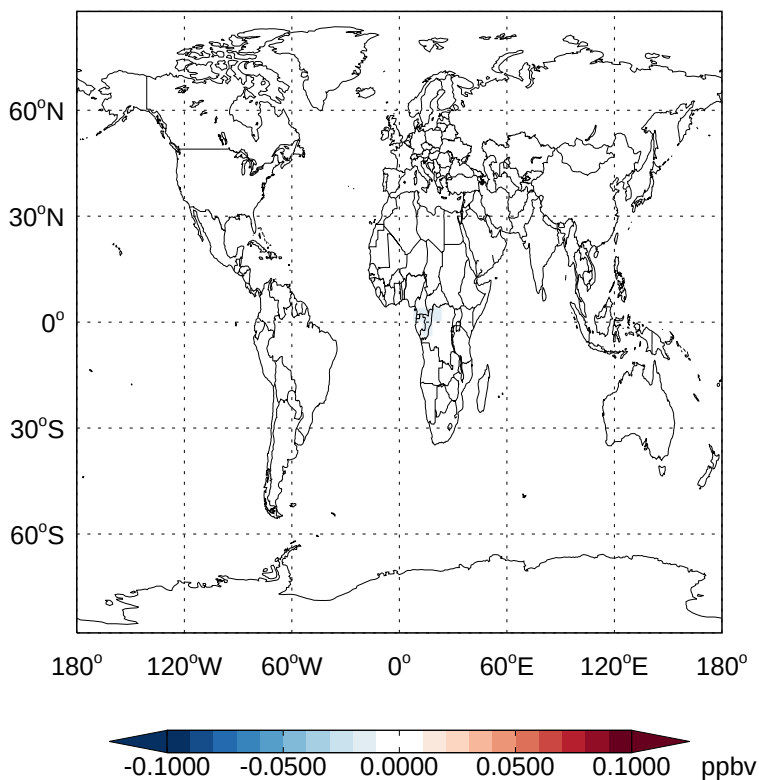
v11-02a - v11-01k-Run0 TSOG3- Diff @ 500 hPa for Jan
