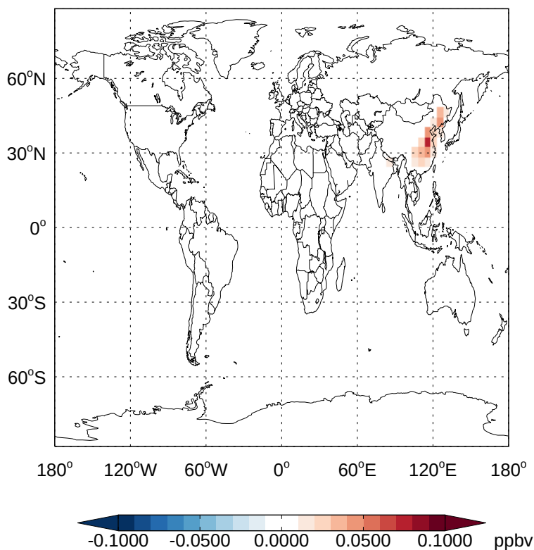
v11-02a - v11-01k-Run0 ASOA3 - Diff @ Surface for Jan
