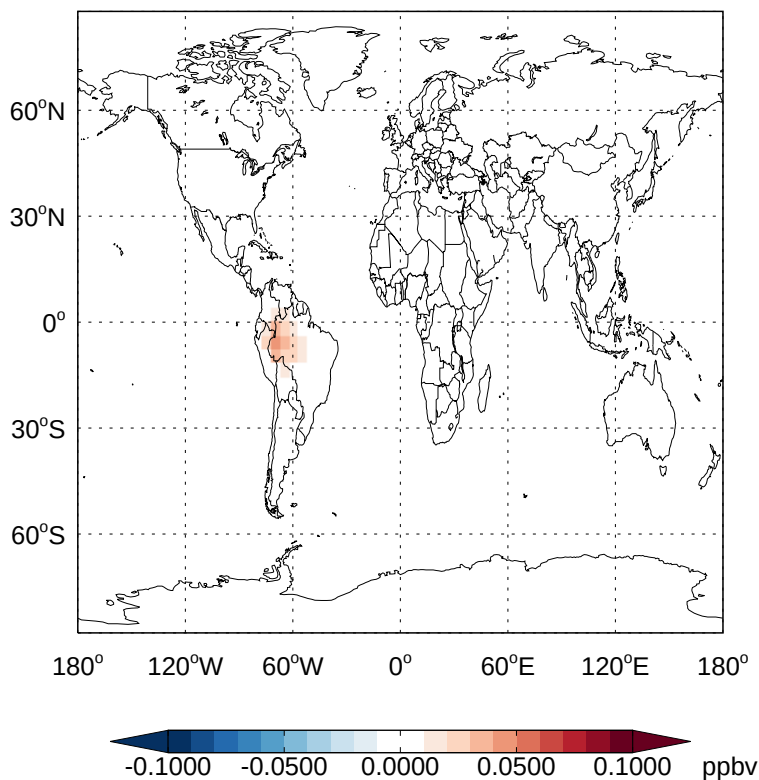
v11-02a - v11-01k-Run0 MTPO - Diff @ Surface for Jan
