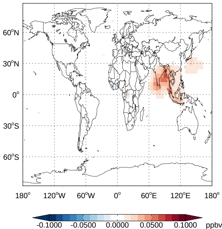
v11-02a - v11-01k-Run0 ASOAN - Diff @ Surface for Jan
