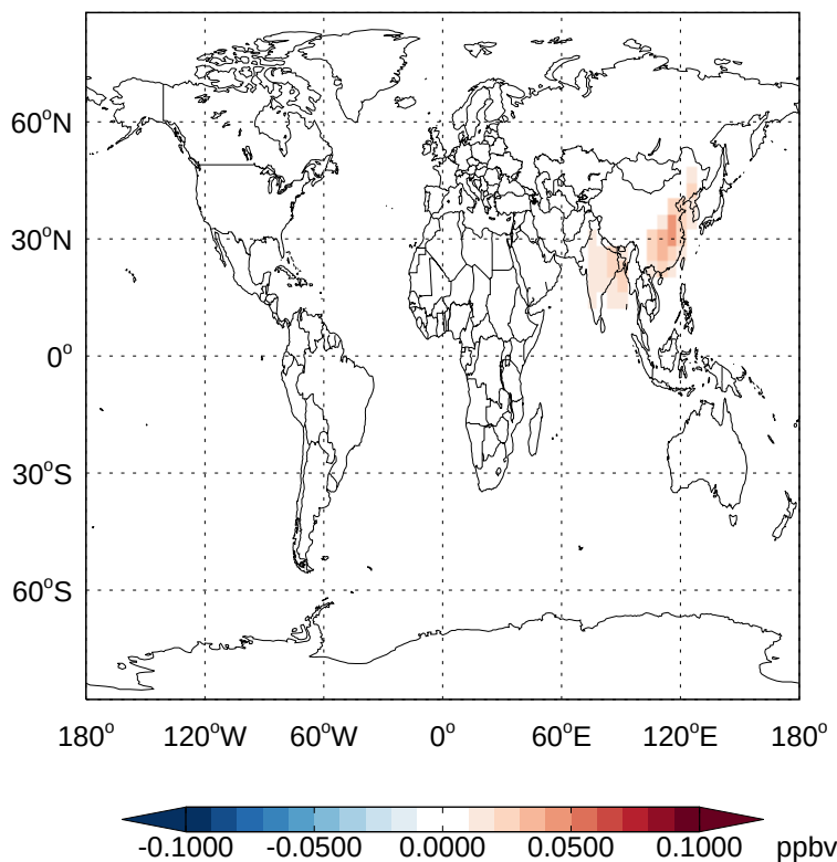
v11-02a - v11-01k-Run0 ASOA1 - Diff @ Surface for Jan
