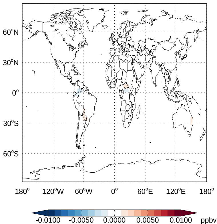
v11-02a - v11-01k-Run0 MACRN - Diff @ Surface for Jan
