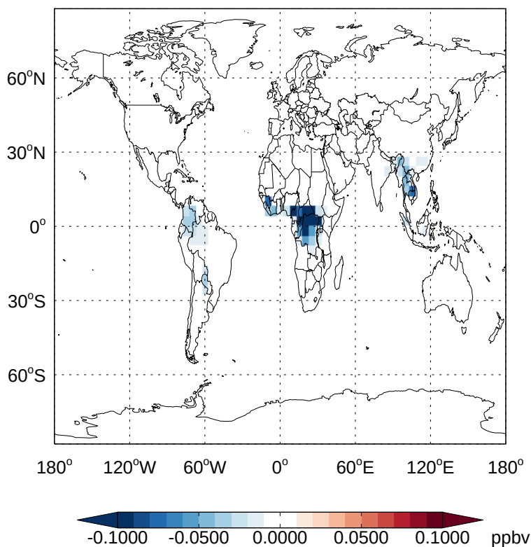
v11-02a - v11-01k-Run0 TSOA3 - Diff @ Surface for Jan
