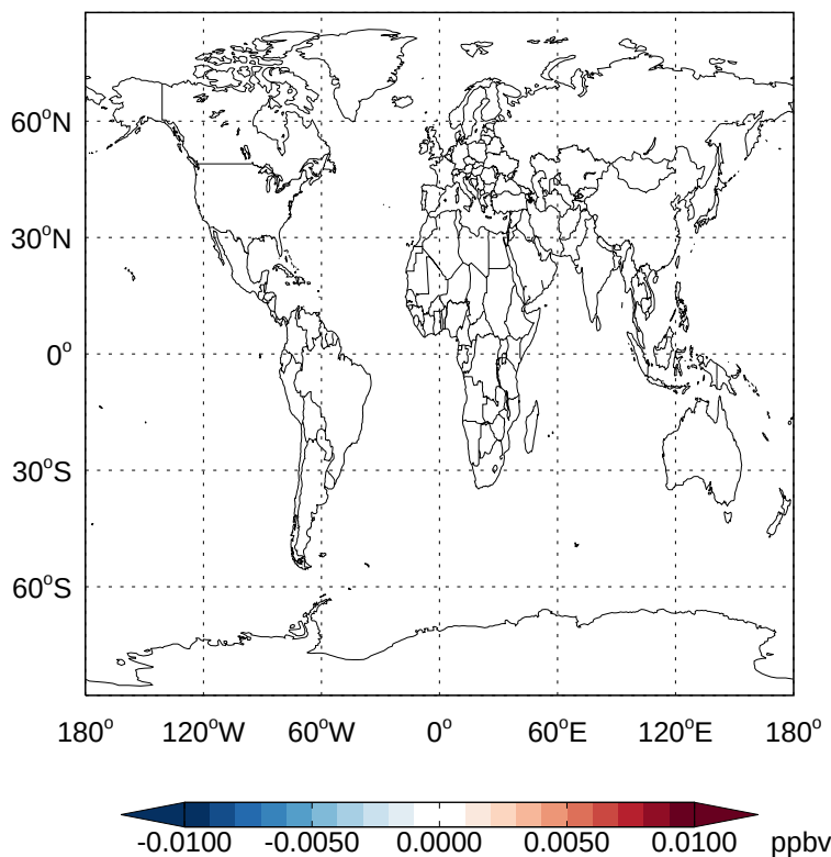
v11-02a - v11-01k-Run0 CHBr3 - Diff @ Surface for Jan
