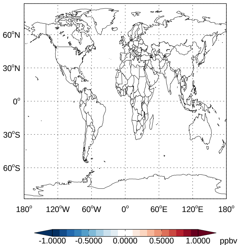
v11-02a - v11-01k-Run0 HNO 2 - Diff @ 500 hPa for Jan
