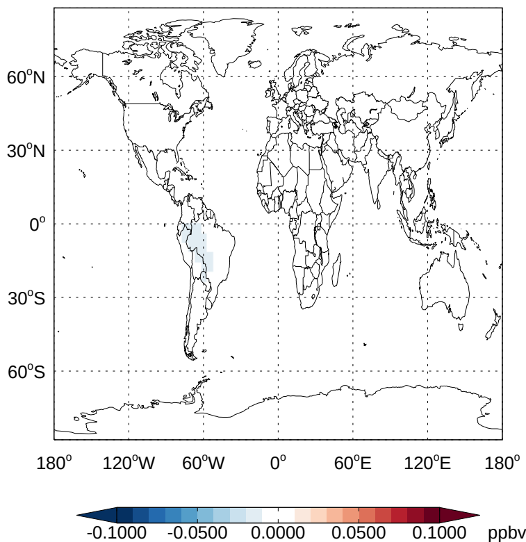
v11-02a - v11-01k-Run0 ISOA1 - Diff @ Surface for Jan
