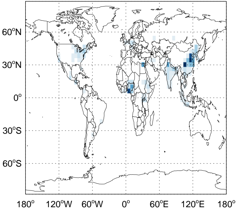
ALD2 column anth+biof emissions for Jan
