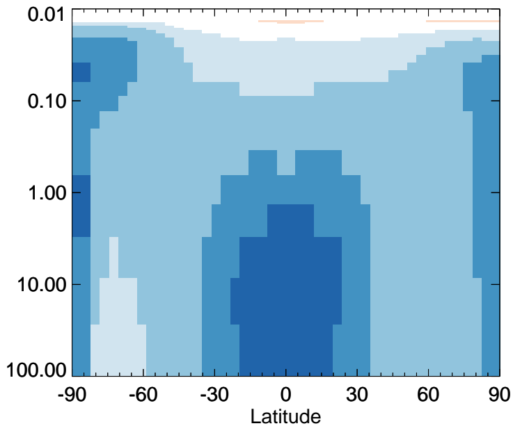
Cl2O2 - Strat zonal mean % diff for Apr
