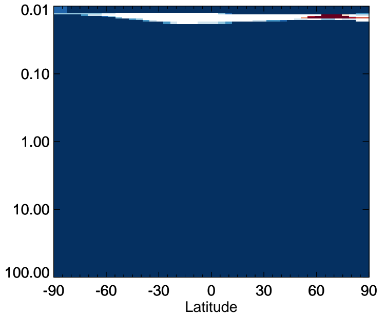
CHBr3 - Strat zonal mean % diff for Apr
