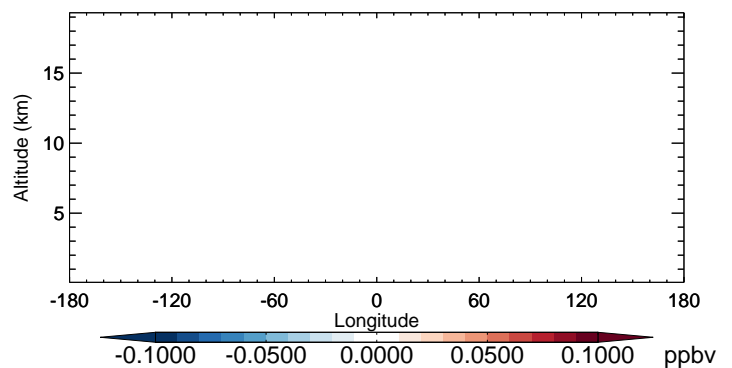
v11-02b-HP - v11-02a ASOA1 - Diff along 42N for Oct
