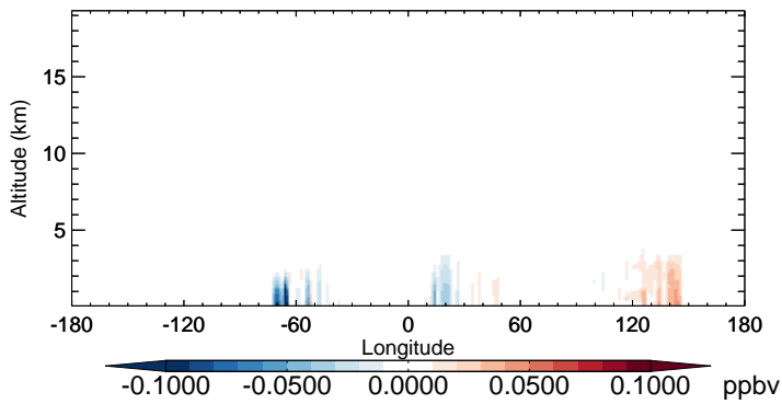
v11-02b-HP - v11-02a TSOG2 - Diff along 15S for Oct
