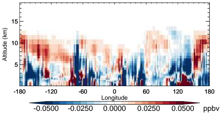
v11-02b-HP - v11-02a MP - Diff along 15S for Oct
