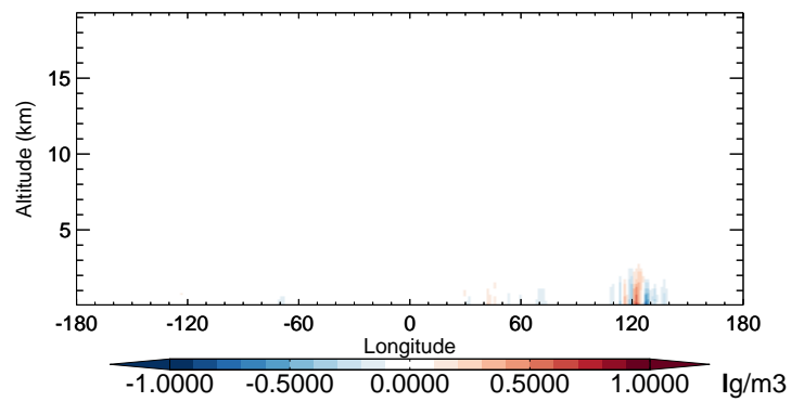
v11-02b-HP - v11-02a OCPI - Diff along 42N for Oct
