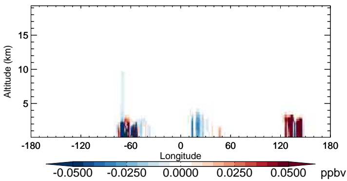
v11-02b-HP - v11-02a MACR - Diff along 15S for Oct
