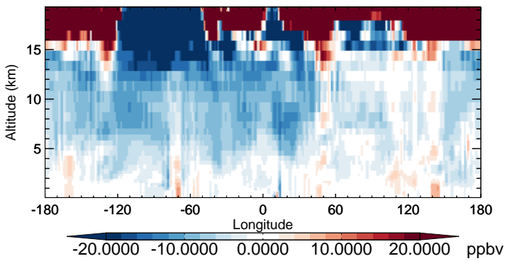
v11-02b-HP - v11-02a O3 - Diff along 15S for Oct
