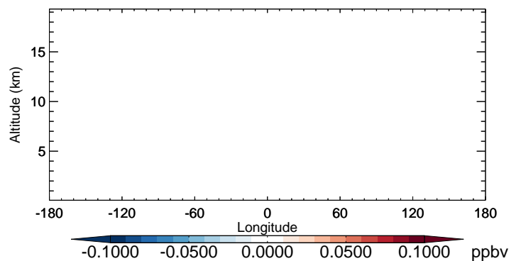
v11-02b-HP - v11-02a TSOA3 - Diff along 42N for Oct
