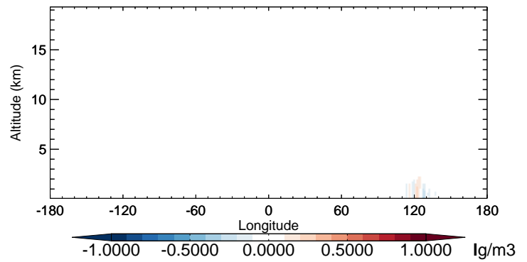
v11-02b-HP - v11-02a BCPI - Diff along 42N for Oct
