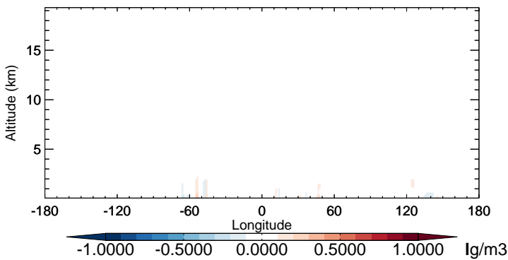
v11-02b-HP - v11-02a NH 3 - Diff along 15S for Oct
