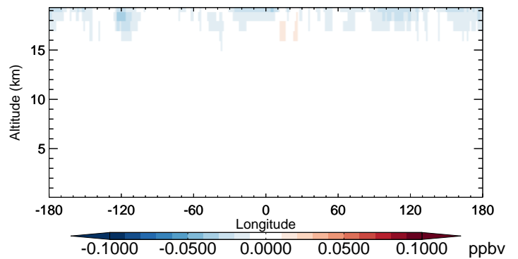
v11-02b-HP - v11-02a CH3Cl - Diff along 42N for Oct
