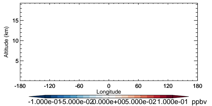
v11-02b-HP - v11-02a H1301 - Diff along 42N for Oct
