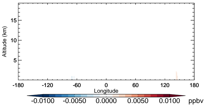
v11-02b-HP - v11-02a MOBA - Diff along 15S for Oct
