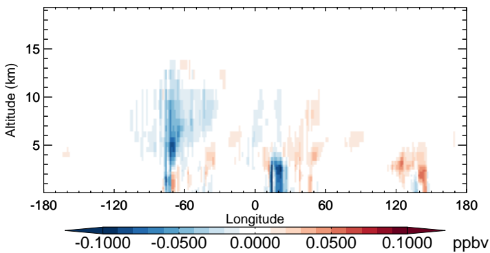
v11-02b-HP - v11-02a PAN - Diff along 15S for Oct
