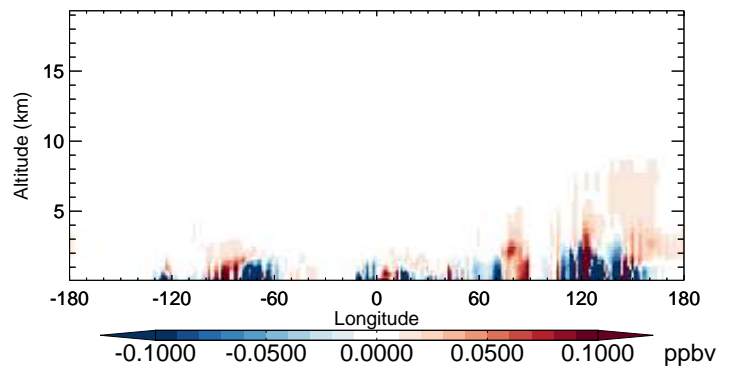
v11-02b-HP - v11-02a TOLU - Diff along 42N for Oct
