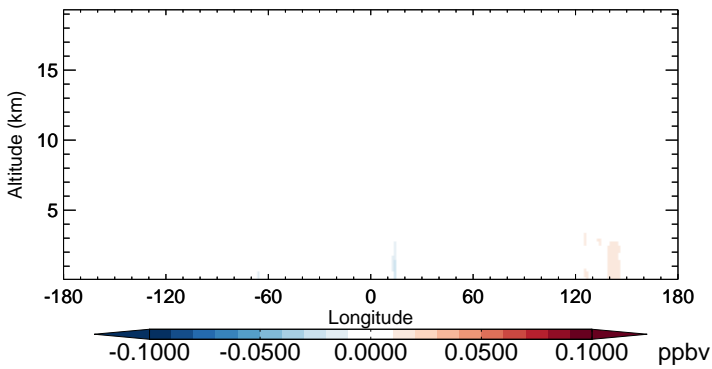
v11-02b-HP - v11-02a PROPNN - Diff along 15S for Oct
