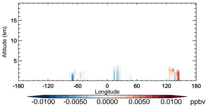
v11-02b-HP - v11-02a PMN - Diff along 15S for Oct
