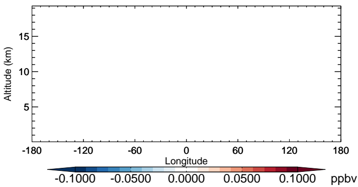
v11-02b-HP - v11-02a MTPO - Diff along 15S for Oct
