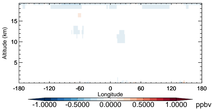
v11-02b-HP - v11-02a NO2 - Diff along 15S for Oct
