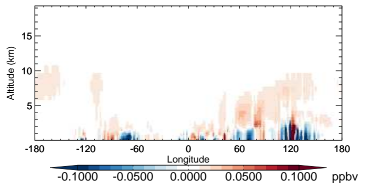
v11-02b-HP - v11-02a BENZ - Diff along 42N for Oct
