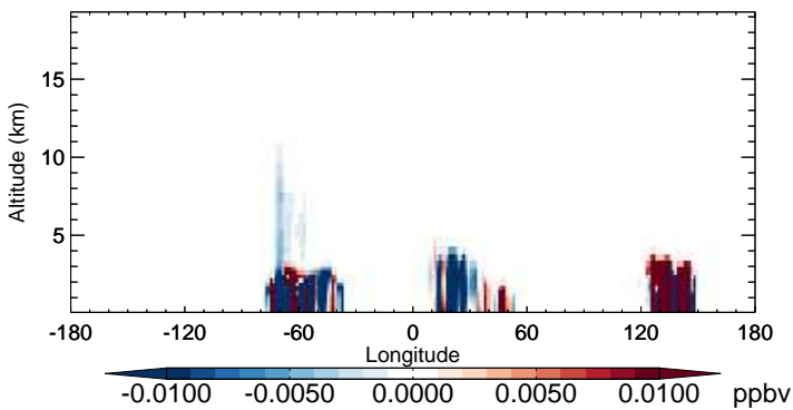
v11-02b-HP - v11-02a RIP - Diff along 15S for Oct
