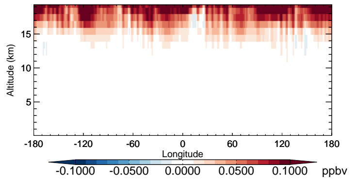
v11-02b-HP - v11-02a HCl - Diff along 42N for Oct
