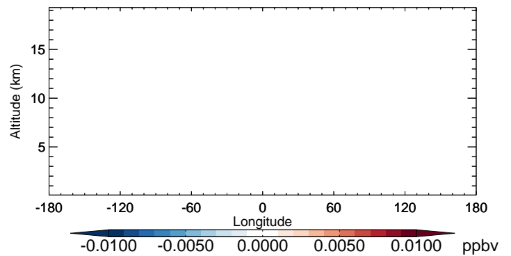
v11-02b-HP - v11-02a MOBA - Diff along 42N for Oct
