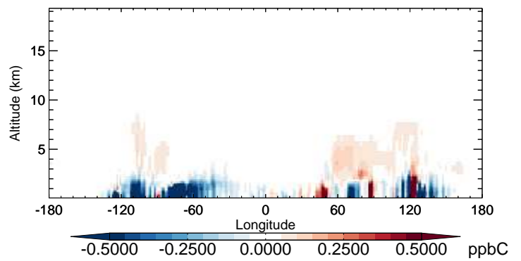
v11-02b-HP - v11-02a ALK4 - Diff along 42N for Oct
