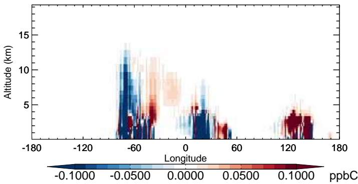
v11-02b-HP - v11-02a MEK - Diff along 15S for Oct
