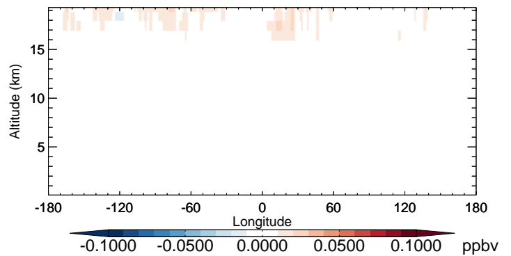
v11-02b-HP - v11-02a CFC12 - Diff along 42N for Oct
