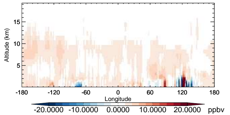
v11-02b-HP - v11-02a CO - Diff along 42N for Oct
