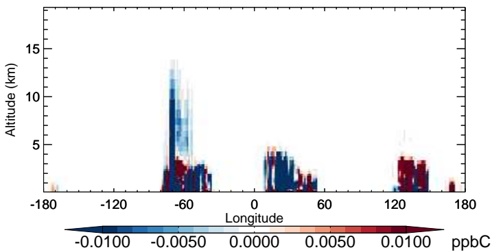
v11-02b-HP - v11-02a PRPE - Diff along 15S for Oct
