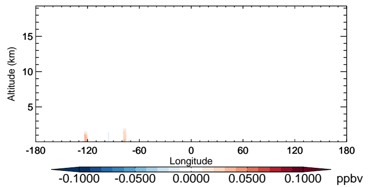
v11-02b-HP - v11-02a TSOG3 - Diff along 42N for Oct
