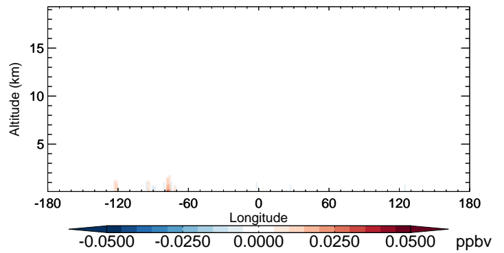
v11-02b-HP - v11-02a MVK - Diff along 42N for Oct
