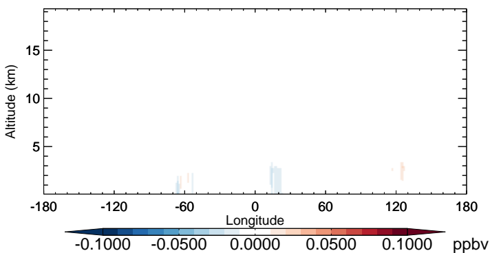
v11-02b-HP - v11-02a TSOA3 - Diff along 15S for Oct
