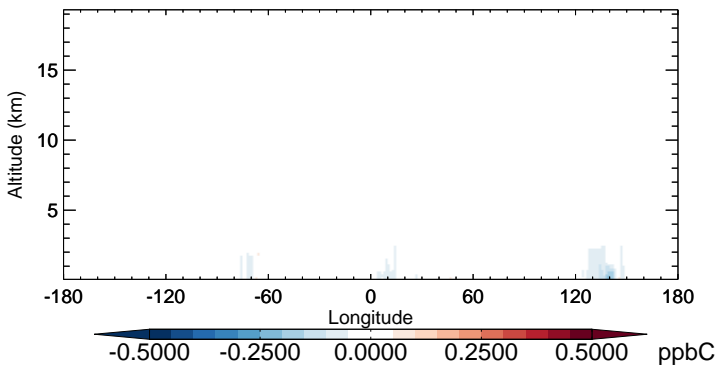
v11-02b-HP - v11-02a C3H8 - Diff along 15S for Oct
