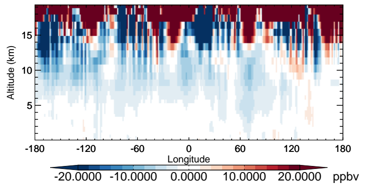
v11-02b-HP - v11-02a O3 - Diff along 42N for Oct
