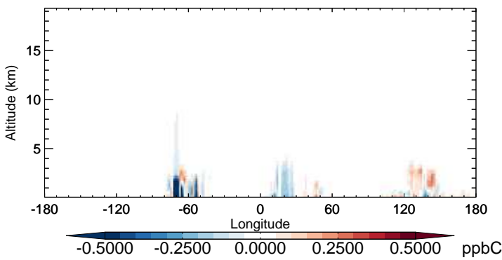
v11-02b-HP - v11-02a ALD2 - Diff along 15S for Oct
