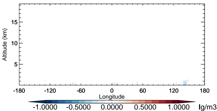
v11-02b-HP - v11-02a SALA - Diff along 15S for Oct
