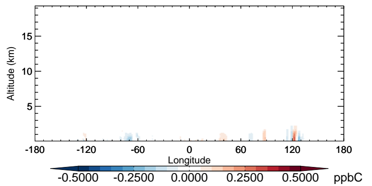
v11-02b-HP - v11-02a ALD2 - Diff along 42N for Oct
