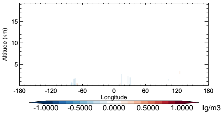
v11-02b-HP - v11-02a NH4 - Diff along 15S for Oct
