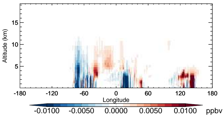
v11-02b-HP - v11-02a R4N2 - Diff along 15S for Oct
