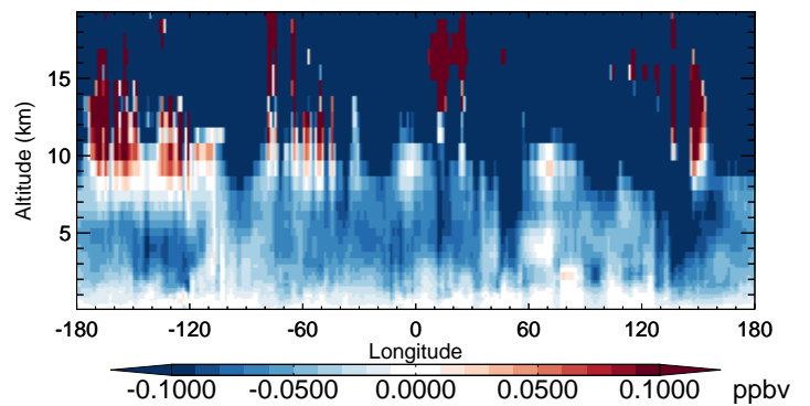
v11-02b-HP - v11-02a N 2 O - Diff along 42N for Oct
