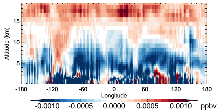
v11-02b-HP - v11-02a PPN - Diff along 42N for Oct
