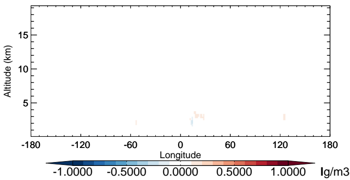
v11-02b-HP - v11-02a NIT - Diff along 15S for Oct
