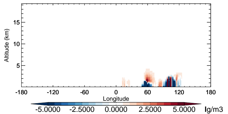
v11-02b-HP - v11-02a DST4 - Diff along 42N for Oct
