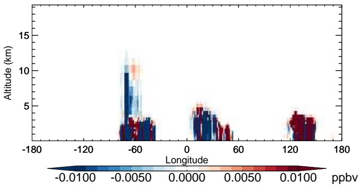
v11-02b-HP - v11-02a IEPOX - Diff along 15S for Oct
