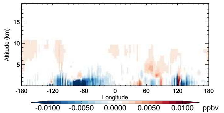
v11-02b-HP - v11-02a R4N2 - Diff along 42N for Oct
