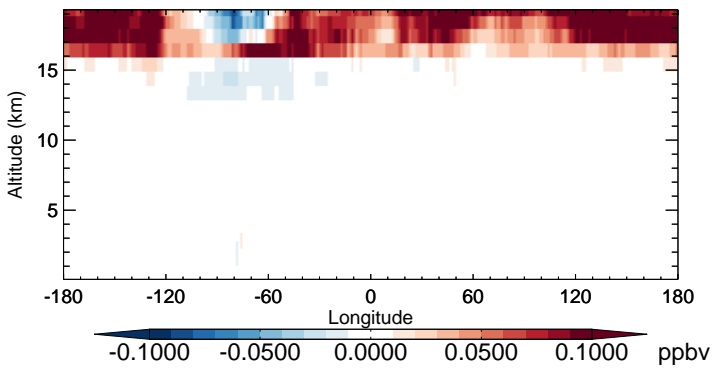
v11-02b-HP - v11-02a HCl - Diff along 15S for Oct
