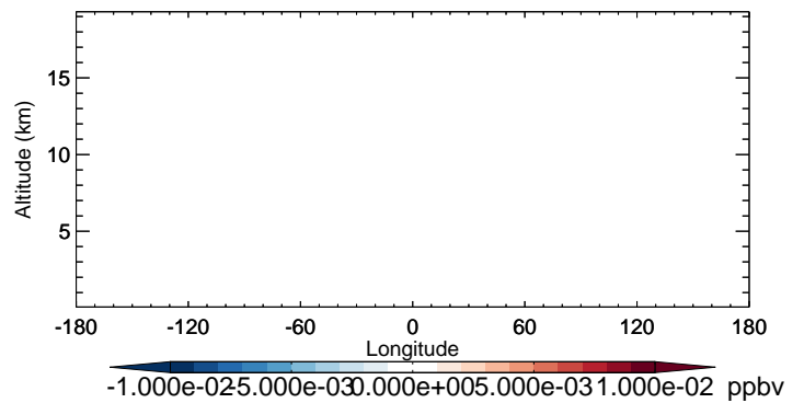
v11-02b-HP - v11-02a Br - Diff along 42N for Oct
