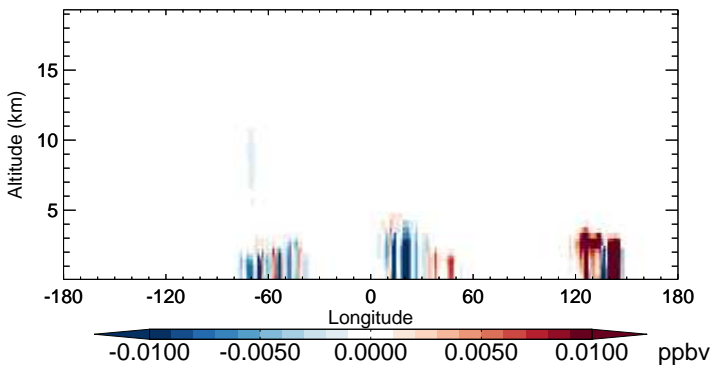
v11-02b-HP - v11-02a MVKN - Diff along 15S for Oct
