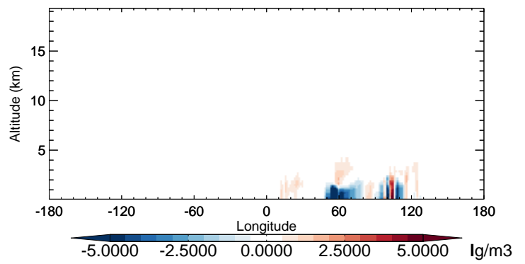
v11-02b-HP - v11-02a DST1 - Diff along 42N for Oct
