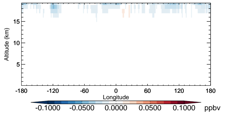
v11-02b-HP - v11-02a OCS - Diff along 42N for Oct
