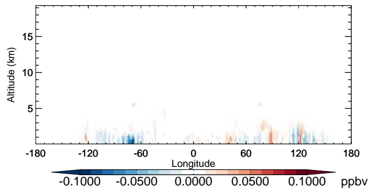
v11-02b-HP - v11-02a PAN - Diff along 42N for Oct
