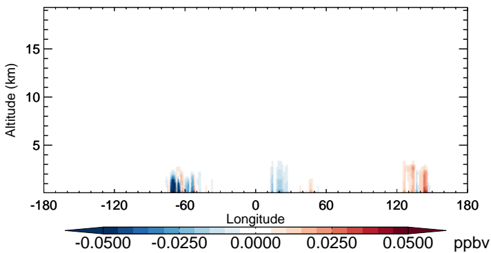
v11-02b-HP - v11-02a RCHO - Diff along 15S for Oct
