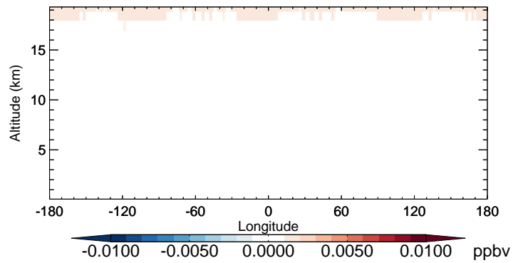
v11-02b-HP - v11-02a BrO - Diff along 42N for Oct
