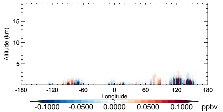
v11-02b-HP - v11-02a XYLE - Diff along 42N for Oct
