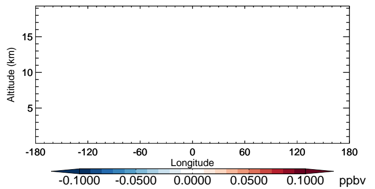
v11-02b-HP - v11-02a CCl4 - Diff along 42N for Oct
