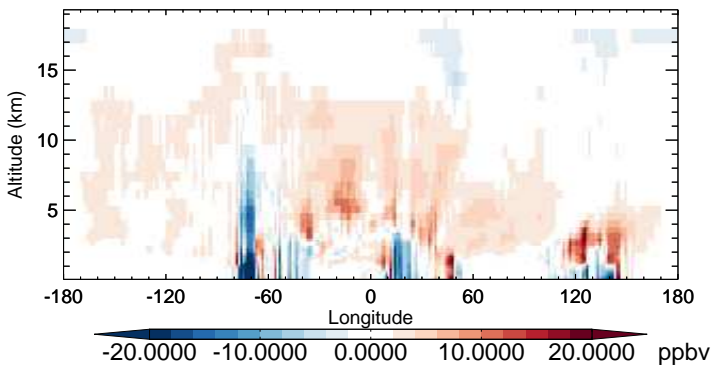
v11-02b-HP - v11-02a CO - Diff along 15S for Oct
