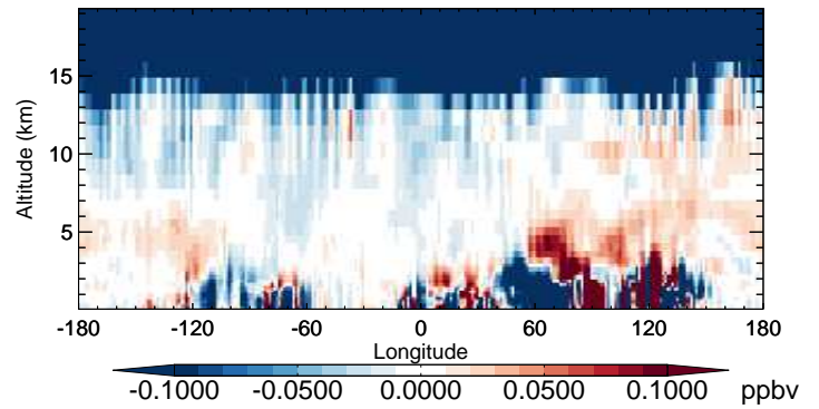
v11-02b-HP - v11-02a HNO 3 - Diff along 42N for Oct
