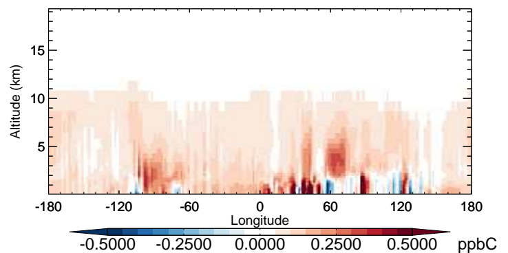
v11-02b-HP - v11-02a C2H6 - Diff along 42N for Oct
