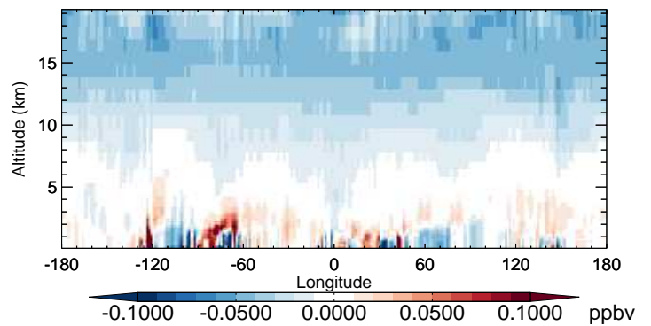
v11-02b-HP - v11-02a EOH - Diff along 42N for Oct
