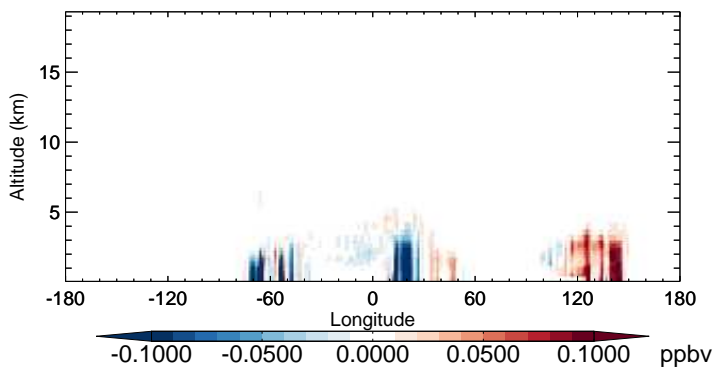
v11-02b-HP - v11-02a TSOG3 - Diff along 15S for Oct
