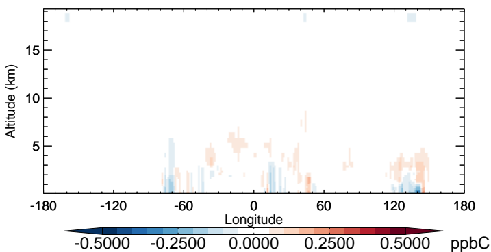
v11-02b-HP - v11-02a C2H6 - Diff along 15S for Oct
