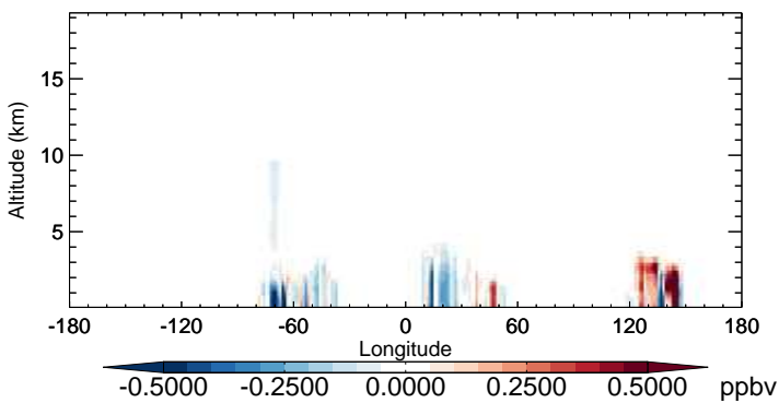
v11-02b-HP - v11-02a CH2O - Diff along 15S for Oct
