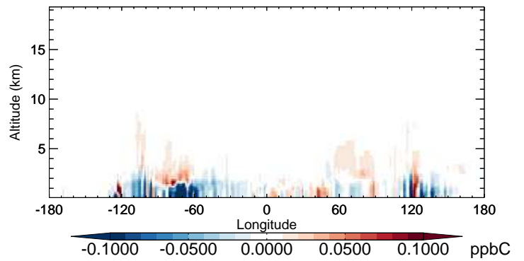
v11-02b-HP - v11-02a MEK - Diff along 42N for Oct
