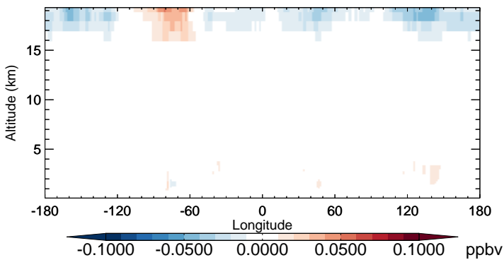
v11-02b-HP - v11-02a CH3Cl - Diff along 15S for Oct
