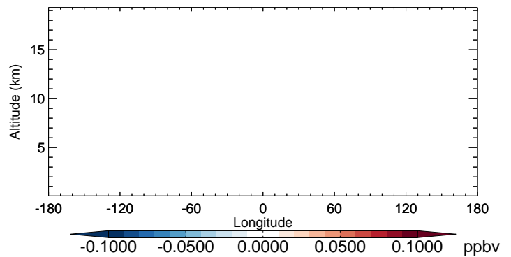
v11-02b-HP - v11-02a ISOA2 - Diff along 42N for Oct
