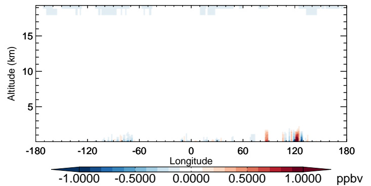
v11-02b-HP - v11-02a NO2 - Diff along 42N for Oct
