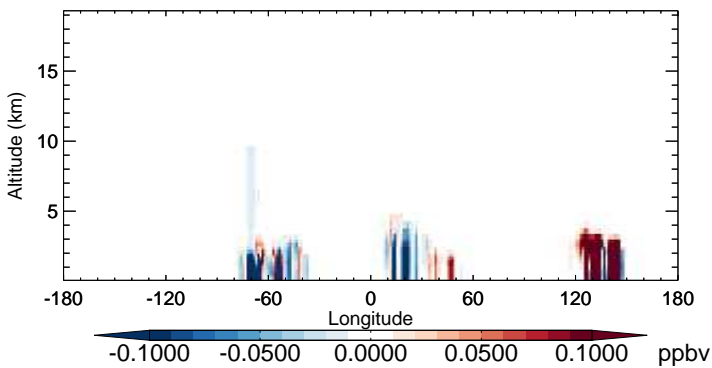
v11-02b-HP - v11-02a GLYC - Diff along 15S for Oct
