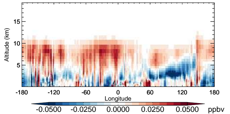
v11-02b-HP - v11-02a MP - Diff along 42N for Oct
