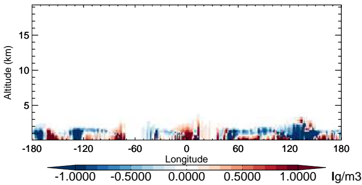
v11-02b-HP - v11-02a SALC - Diff along 15S for Oct
