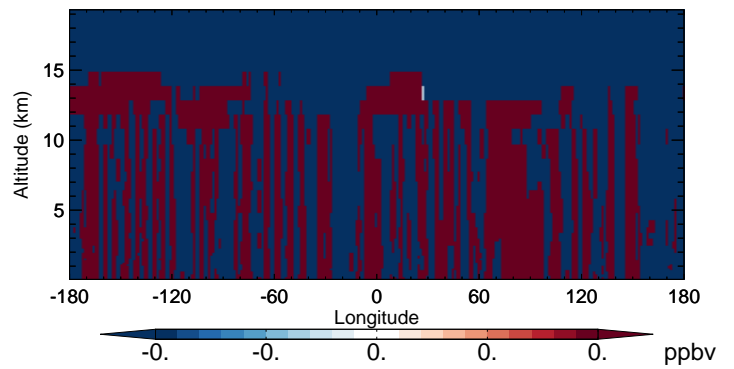
v11-02b-HP - v11-02a H 2 O - Diff along 42N for Oct
