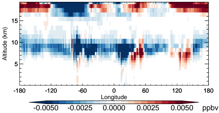
v11-02b-HP - v11-02a HNO4 - Diff along 15S for Oct
