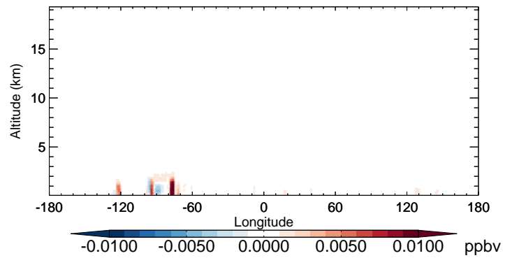
v11-02b-HP - v11-02a IEPOX - Diff along 42N for Oct
