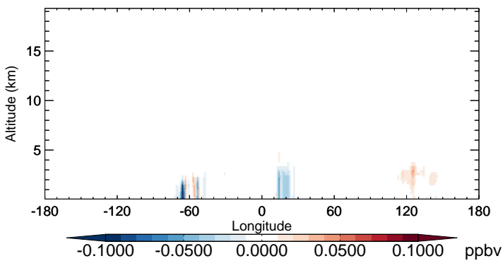
v11-02b-HP - v11-02a TSOA2 - Diff along 15S for Oct
