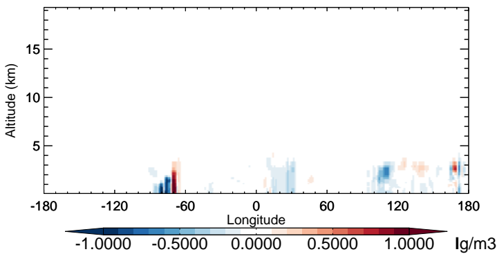
v11-02b-HP - v11-02a SO 4 - Diff along 15S for Oct
