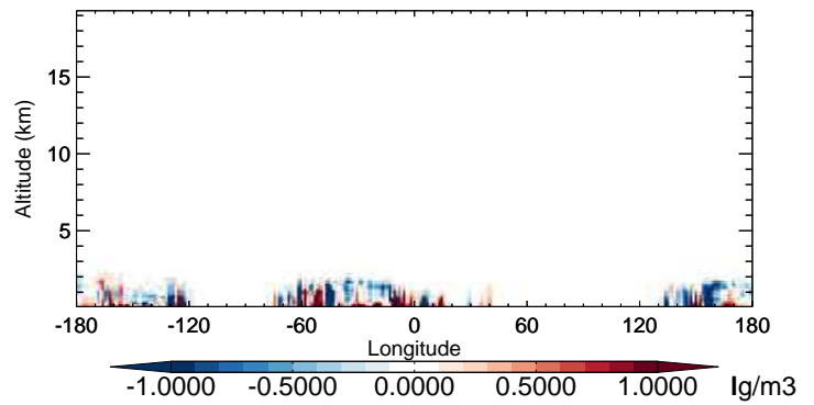
v11-02b-HP - v11-02a SALC - Diff along 42N for Oct
