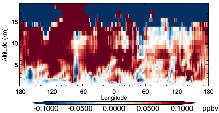
v11-02b-HP - v11-02a N 2 O - Diff along 15S for Oct
