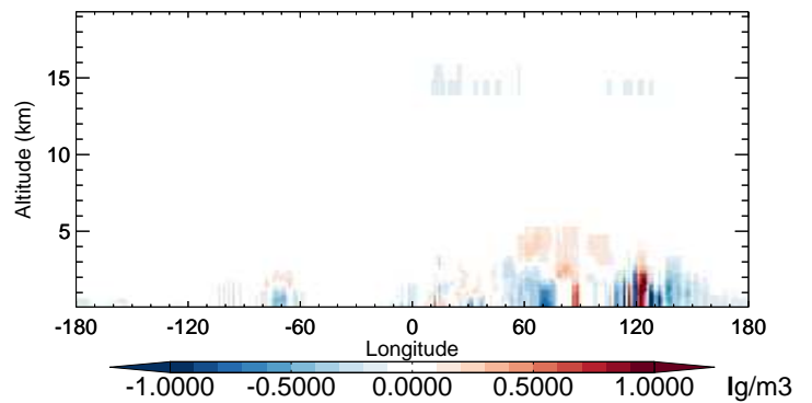
v11-02b-HP - v11-02a SO 4 - Diff along 42N for Oct
