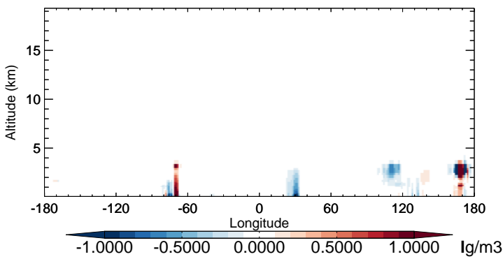
v11-02b-HP - v11-02a SO 2 - Diff along 15S for Oct
