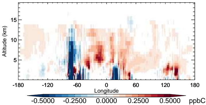
v11-02b-HP - v11-02a ACET - Diff along 15S for Oct
