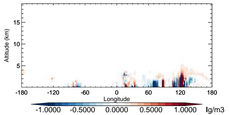
v11-02b-HP - v11-02a SO 2 - Diff along 42N for Oct
