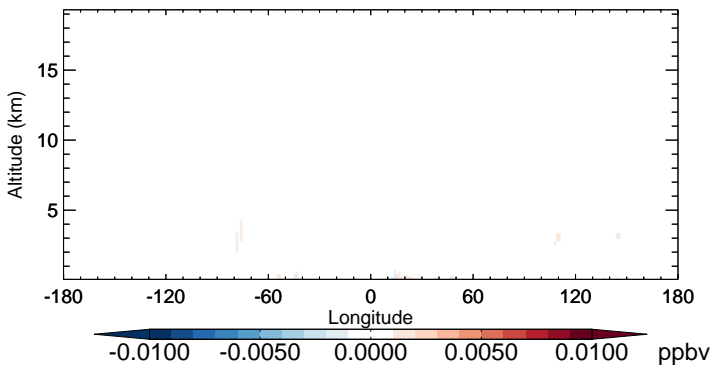
v11-02b-HP - v11-02a NO 3 - Diff along 15S for Oct
