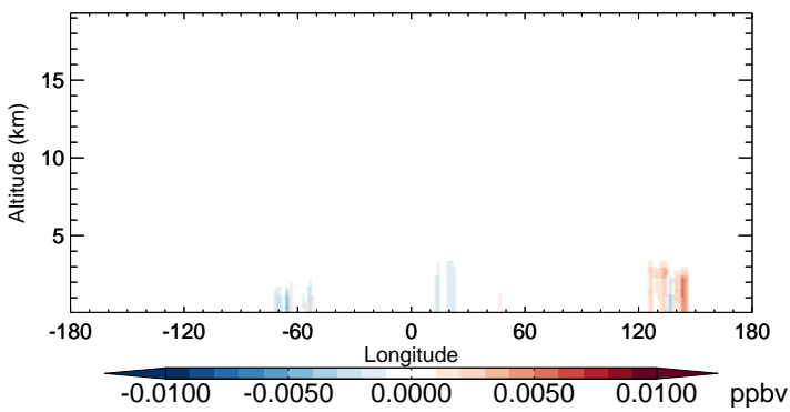
v11-02b-HP - v11-02a MACRN - Diff along 15S for Oct
