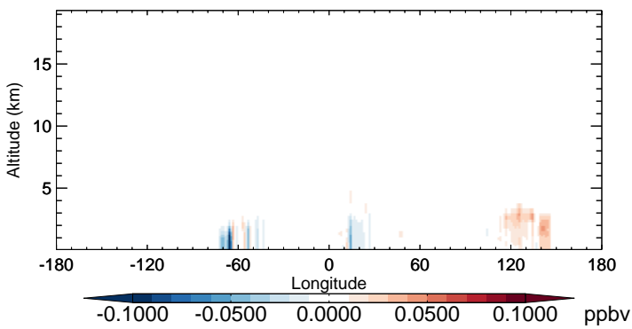
v11-02b-HP - v11-02a ISOA1 - Diff along 15S for Oct
