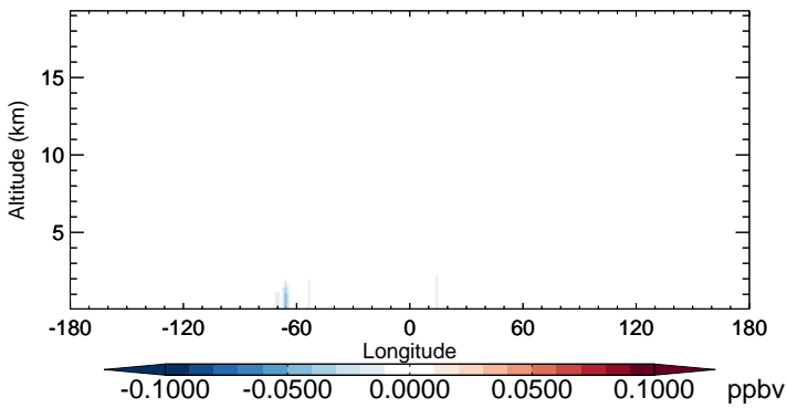
v11-02b-HP - v11-02a TSOA1 - Diff along 15S for Oct
