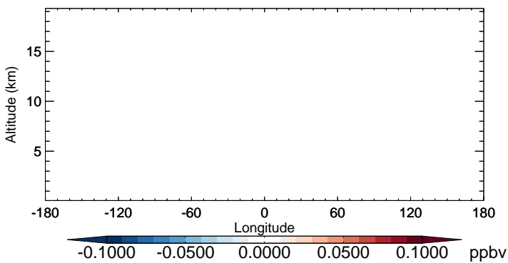
v11-02b-HP - v11-02a ISOPNB - Diff along 15S for Oct
