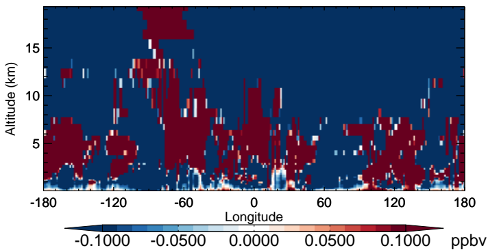
v11-02b-HP - v11-02a CH4 - Diff along 15S for Oct
