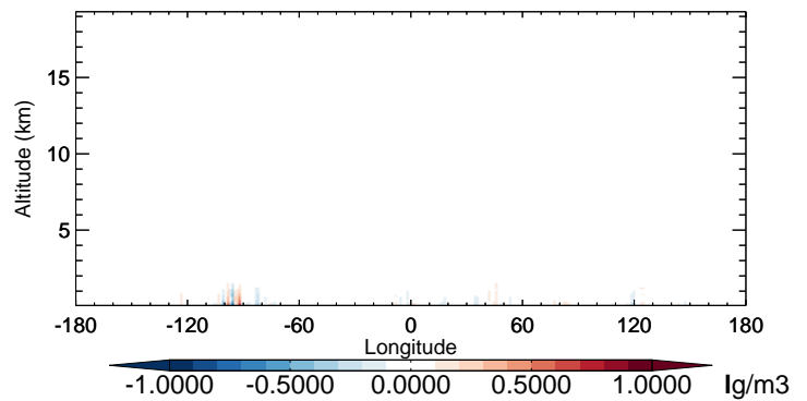
v11-02b-HP - v11-02a NH 3 - Diff along 42N for Oct
