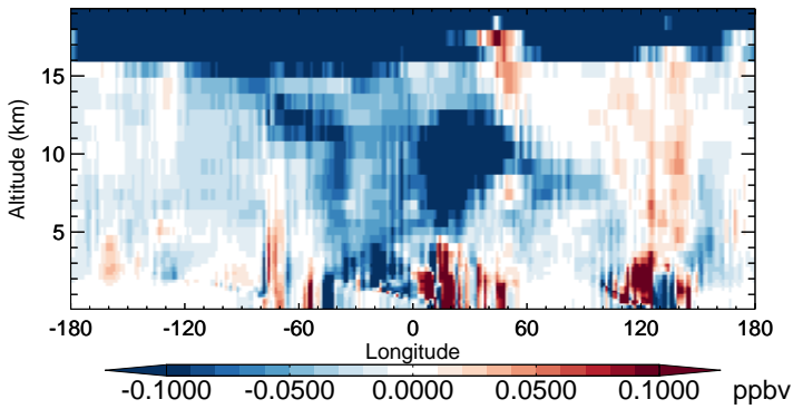
v11-02b-HP - v11-02a HNO 3 - Diff along 15S for Oct
