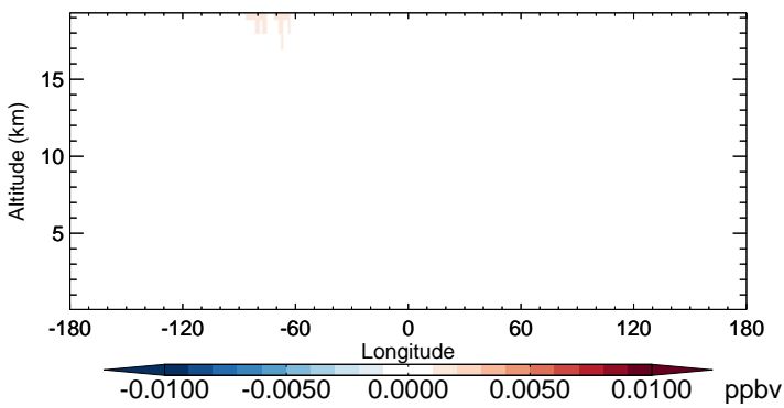
v11-02b-HP - v11-02a CH 3 Br - Diff along 15S for Oct
