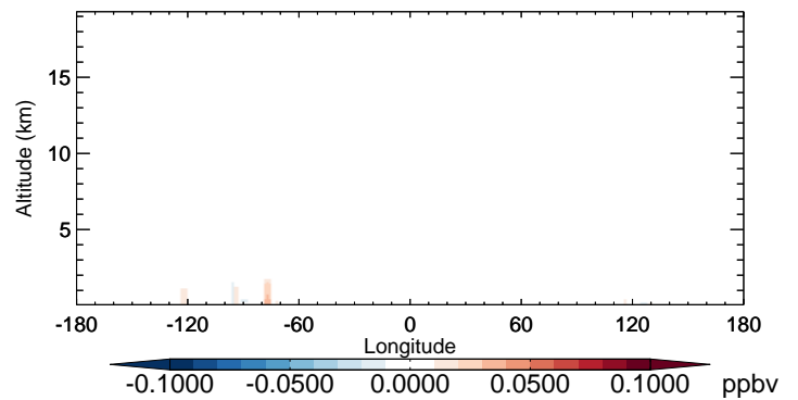
v11-02b-HP - v11-02a GLYC - Diff along 42N for Oct
