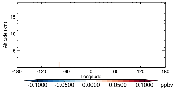
v11-02b-HP - v11-02a ISOG3 - Diff along 42N for Oct
