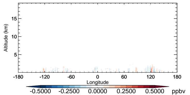
v11-02b-HP - v11-02a CH2O - Diff along 42N for Oct
