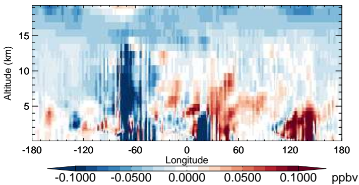
v11-02b-HP - v11-02a EOH - Diff along 15S for Oct
