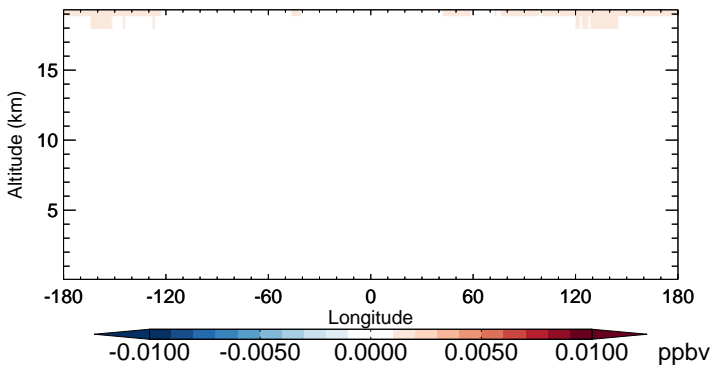
v11-02b-HP - v11-02a BrO - Diff along 15S for Oct
