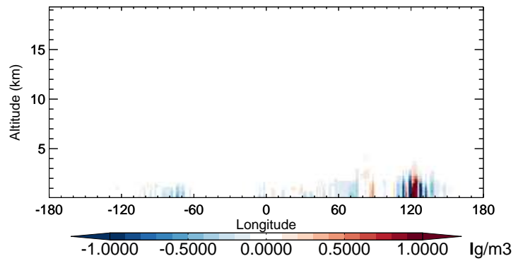
v11-02b-HP - v11-02a NH4 - Diff along 42N for Oct
