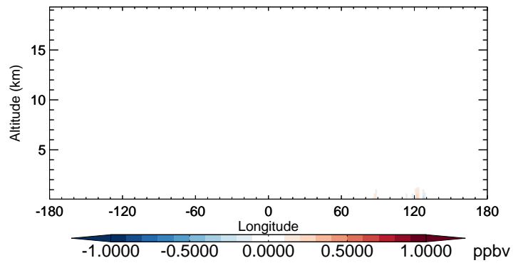
v11-02b-HP - v11-02a NO - Diff along 42N for Oct
