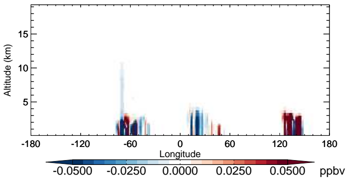
v11-02b-HP - v11-02a MVK - Diff along 15S for Oct
