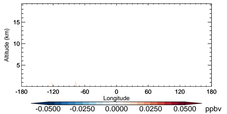
v11-02b-HP - v11-02a MACR - Diff along 42N for Oct
