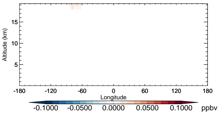
v11-02b-HP - v11-02a CCl4 - Diff along 15S for Oct
