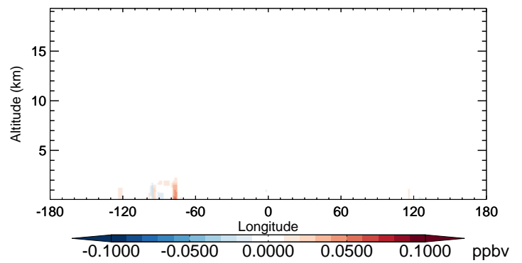
v11-02b-HP - v11-02a HAC - Diff along 42N for Oct
