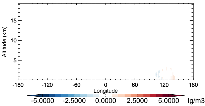
v11-02b-HP - v11-02a DST1 - Diff along 15S for Oct
