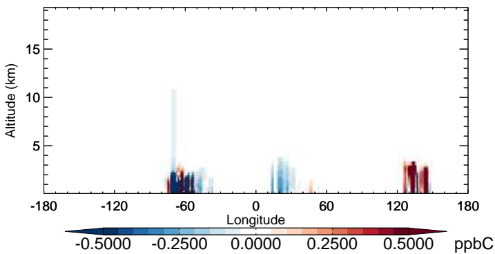
v11-02b-HP - v11-02a ISOP - Diff along 15S for Oct
