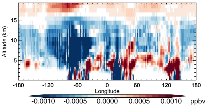
v11-02b-HP - v11-02a PPN - Diff along 15S for Oct
