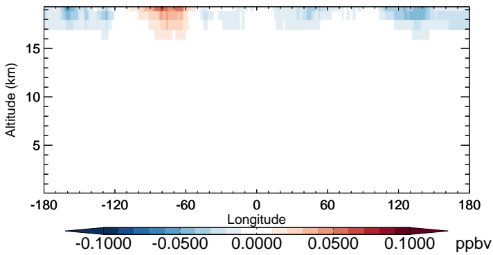
v11-02b-HP - v11-02a OCS - Diff along 15S for Oct
