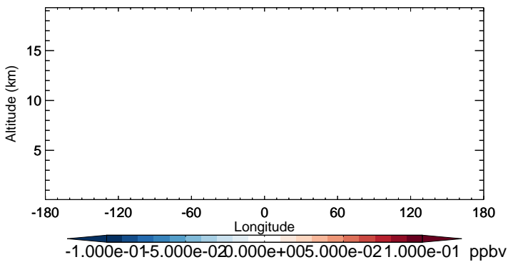
v11-02b-HP - v11-02a ClONO2 - Diff along 15S for Oct
