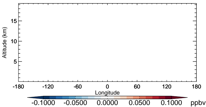
v11-02b-HP - v11-02a ASOAN - Diff along 15S for Oct
