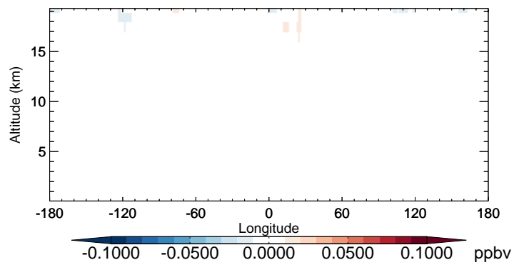
v11-02b-HP - v11-02a CFC11 - Diff along 42N for Oct
