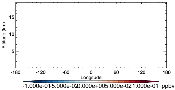
v11-02b-HP - v11-02a ClOO - Diff along 15S for Oct
