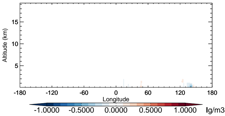
v11-02b-HP - v11-02a OCPO - Diff along 15S for Oct
