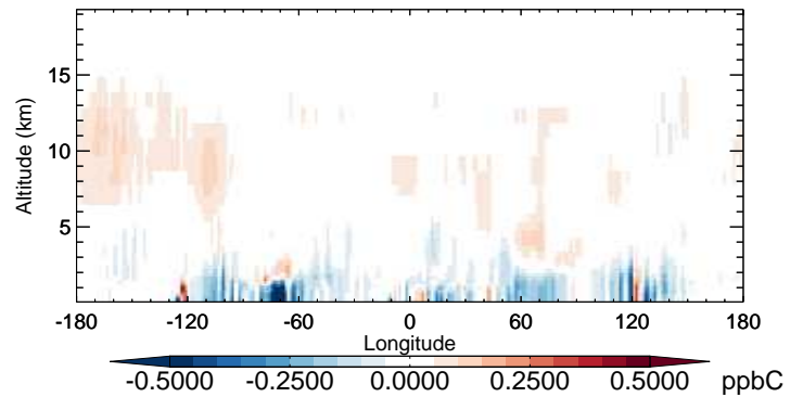
v11-02b-HP - v11-02a ACET - Diff along 42N for Oct
