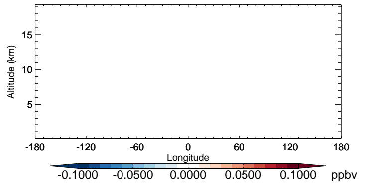
v11-02b-HP - v11-02a PROPNN - Diff along 42N for Oct
