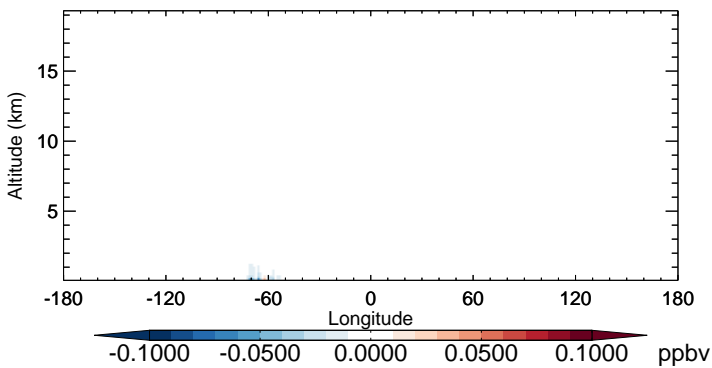
v11-02b-HP - v11-02a MTPA - Diff along 15S for Oct
