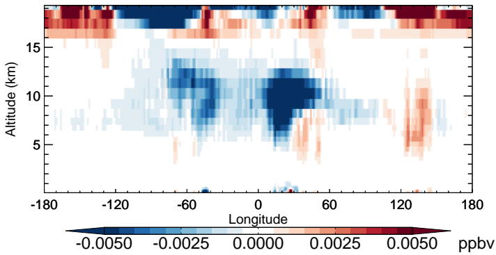
v11-02b-HP - v11-02a N2O5 - Diff along 15S for Oct
