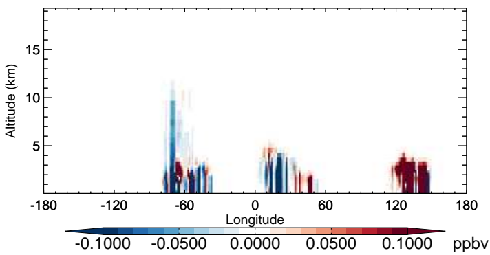
v11-02b-HP - v11-02a HAC - Diff along 15S for Oct
