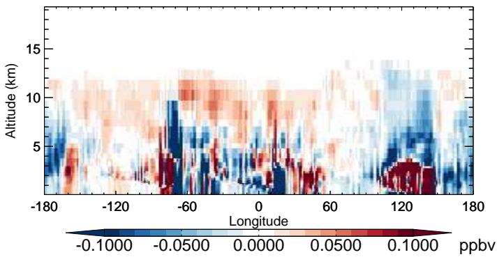
v11-02b-HP - v11-02a H 2 O 2 - Diff along 15S for Oct
