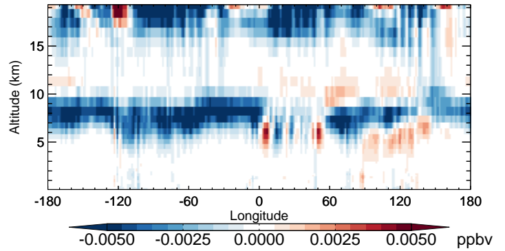
v11-02b-HP - v11-02a HNO4 - Diff along 42N for Oct
