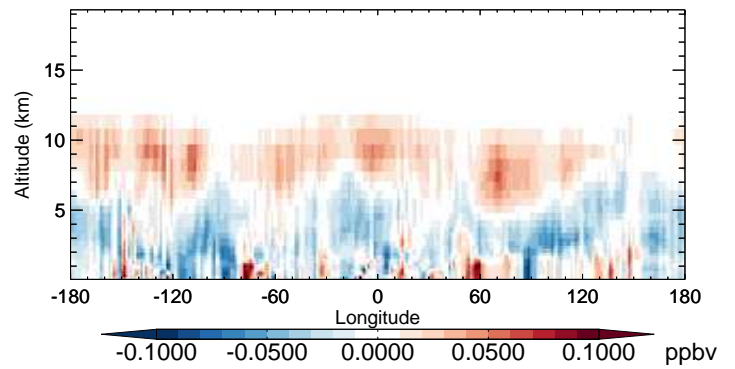
v11-02b-HP - v11-02a H 2 O 2 - Diff along 42N for Oct
