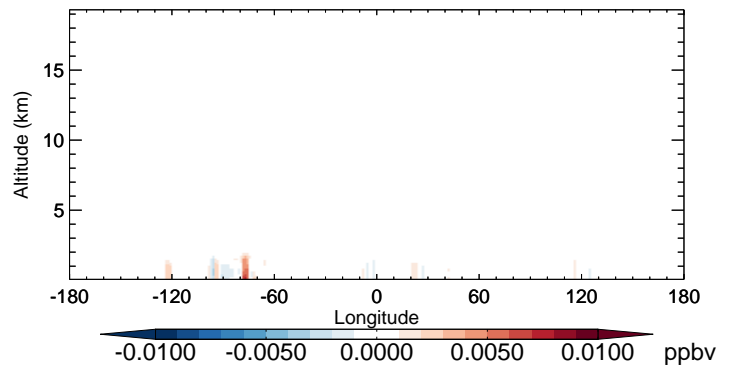
v11-02b-HP - v11-02a MVKN - Diff along 42N for Oct
