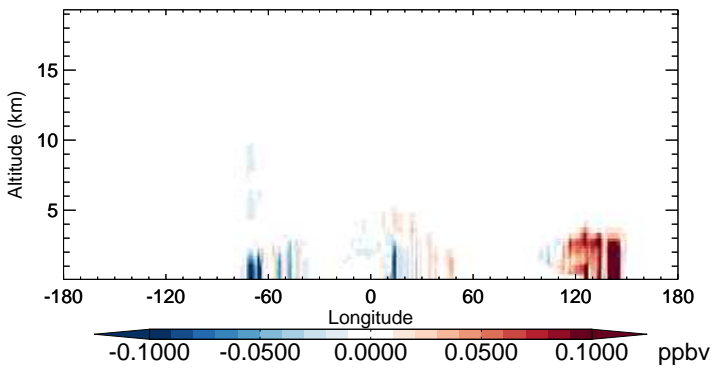
v11-02b-HP - v11-02a ISOG3 - Diff along 15S for Oct
