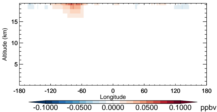
v11-02b-HP - v11-02a CFC12 - Diff along 15S for Oct
