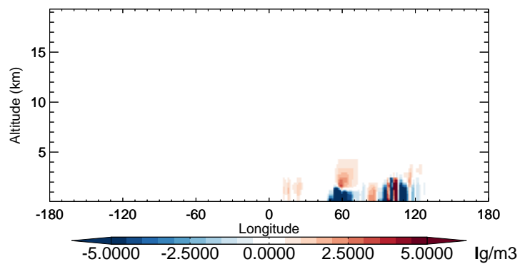
v11-02b-HP - v11-02a DST2 - Diff along 42N for Oct
