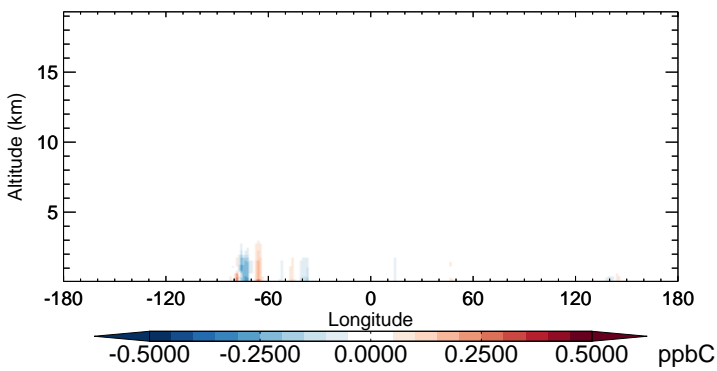
v11-02b-HP - v11-02a ALK4 - Diff along 15S for Oct
