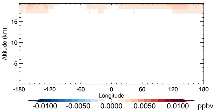
v11-02b-HP - v11-02a BrNO 3 - Diff along 15S for Oct
