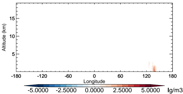
v11-02b-HP - v11-02a DST4 - Diff along 15S for Oct
