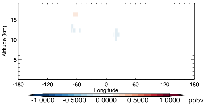
v11-02b-HP - v11-02a NO - Diff along 15S for Oct
