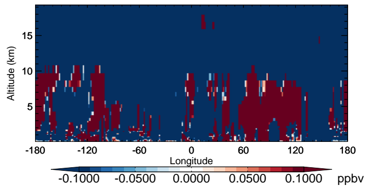
v11-02b-HP - v11-02a CH4 - Diff along 42N for Oct
