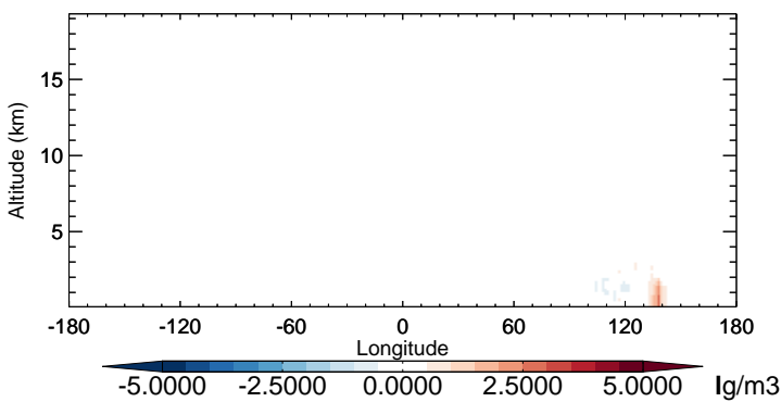
v11-02b-HP - v11-02a DST2 - Diff along 15S for Oct
