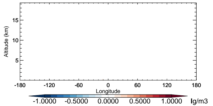
v11-02b-HP - v11-02a DMS - Diff along 42N for Oct
