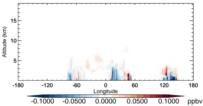
v11-02b-HP - v11-02a BENZ - Diff along 15S for Oct
