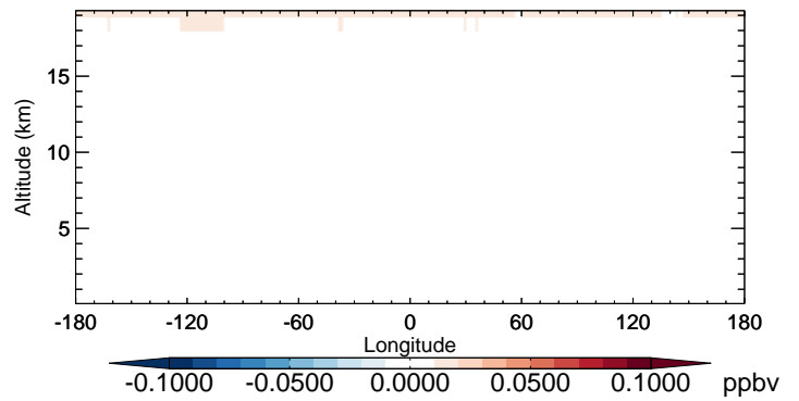
v11-02b-HP - v11-02a CFC115 - Diff along 42N for Oct
