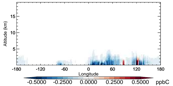
v11-02b-HP - v11-02a C3H8 - Diff along 42N for Oct
