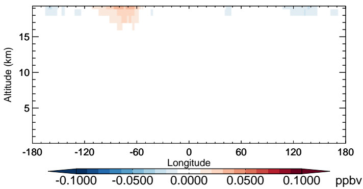
v11-02b-HP - v11-02a CFC11 - Diff along 15S for Oct
