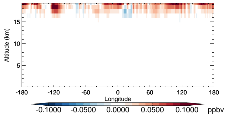
v11-02b-HP - v11-02a ClONO2 - Diff along 42N for Oct
