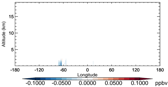
v11-02b-HP - v11-02a TSOA0 - Diff along 15S for Oct
