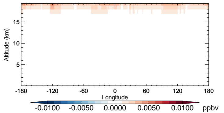
v11-02b-HP - v11-02a BrNO 3 - Diff along 42N for Oct
