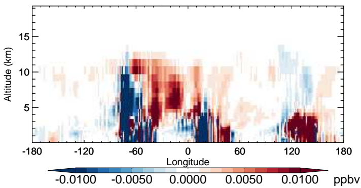
v11-02b-HP - v11-02a MAP - Diff along 15S for Oct
