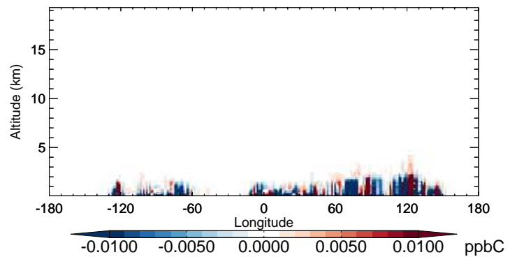
v11-02b-HP - v11-02a PRPE - Diff along 42N for Oct
