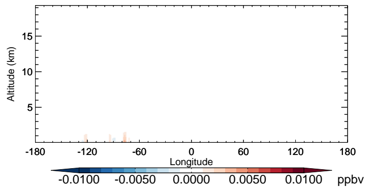
v11-02b-HP - v11-02a RIP - Diff along 42N for Oct
