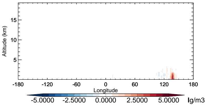
v11-02b-HP - v11-02a DST3 - Diff along 15S for Oct
