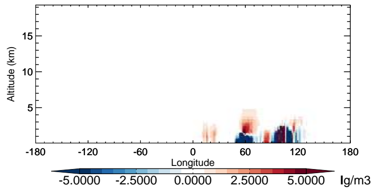
v11-02b-HP - v11-02a DST3 - Diff along 42N for Oct
