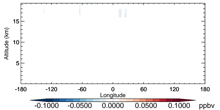
v11-02b-HP - v11-02a MPN - Diff along 42N for Oct
