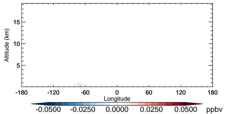
v11-02b-HP - v11-02a RCHO - Diff along 42N for Oct
