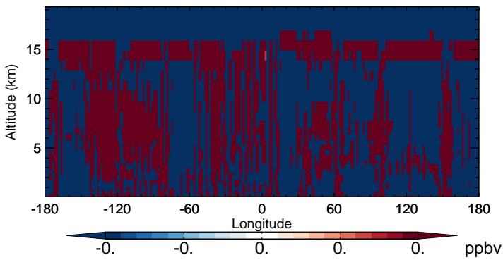
v11-02b-HP - v11-02a H 2 O - Diff along 15S for Oct
