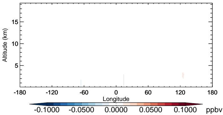
v11-02b-HP - v11-02a ISOA3 - Diff along 15S for Oct
