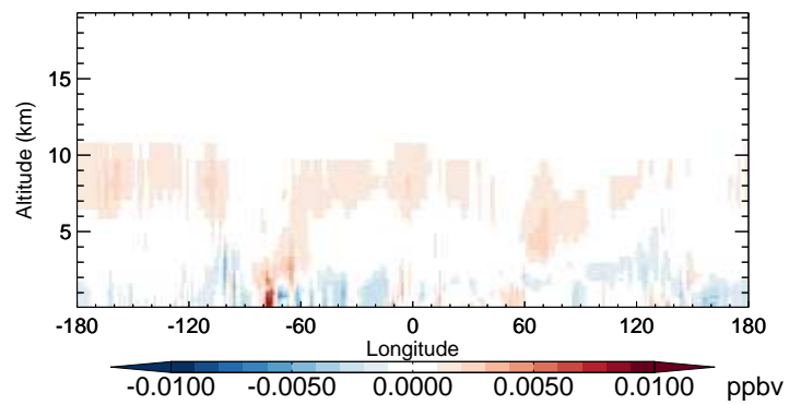
v11-02b-HP - v11-02a MAP - Diff along 42N for Oct
