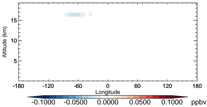
v11-02b-HP - v11-02a HOCl - Diff along 15S for Oct
