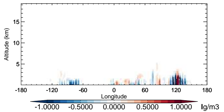
v11-02b-HP - v11-02a NIT - Diff along 42N for Oct
