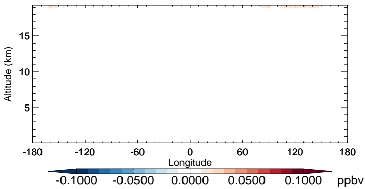
v11-02b-HP - v11-02a CFC115 - Diff along 15S for Oct
