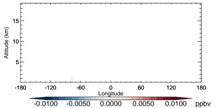
v11-02b-HP - v11-02a PMN - Diff along 42N for Oct
