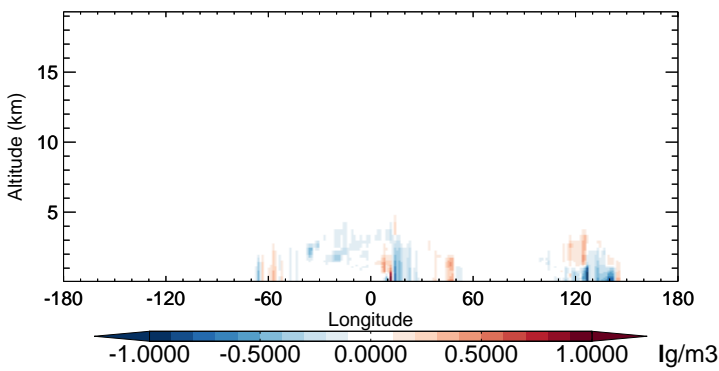
v11-02b-HP - v11-02a OCPI - Diff along 15S for Oct
