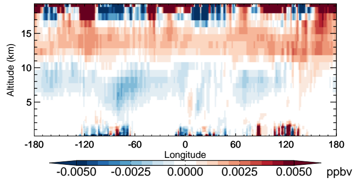
v11-02b-HP - v11-02a N2O5 - Diff along 42N for Oct
