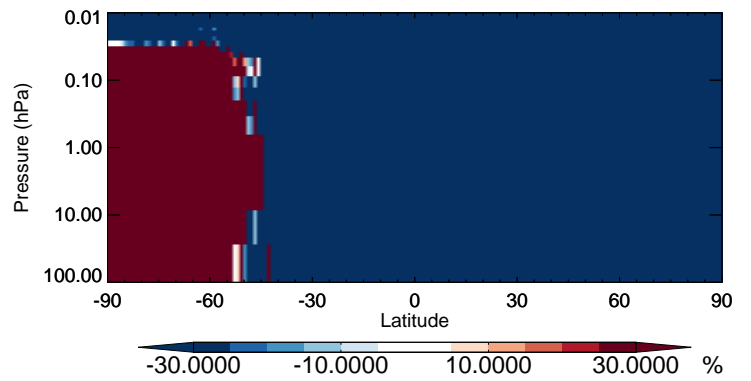
v11-02b-HP / v11-02a ClONO2 - Strat zonal mean % diff for Jul
