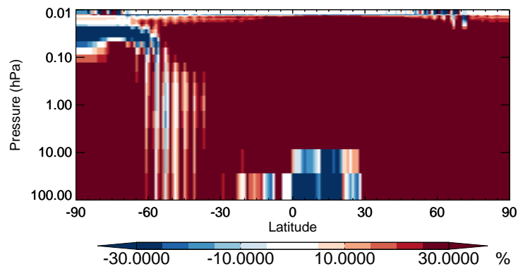
v11-02b-HP / v11-02a OCIO - Strat zonal mean % diff for Jul
