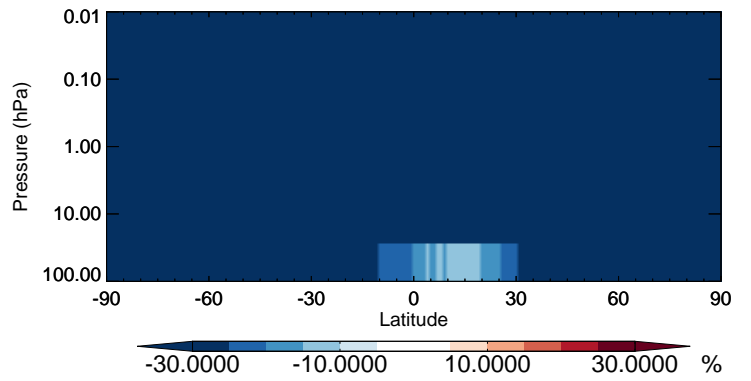
v11-02b-HP / v11-02a BCPI - Strat zonal mean % diff for Jul
