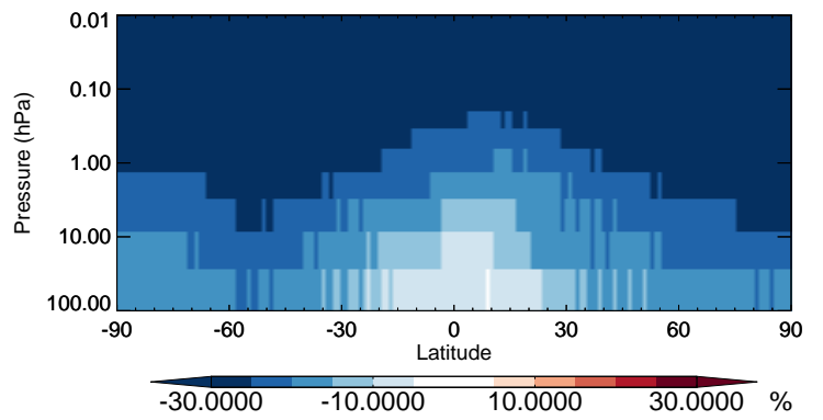
v11-02b-HP / v11-02a MSA - Strat zonal mean % diff for Jul
