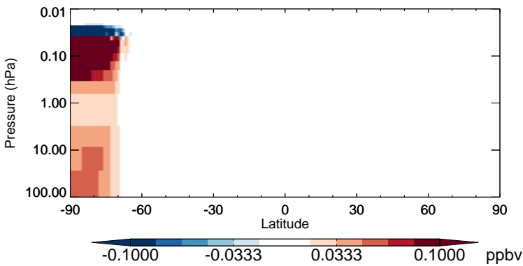
v11-02b-HP - v11-02a Cl2 - Strat zonal mean abs diff for Jul
