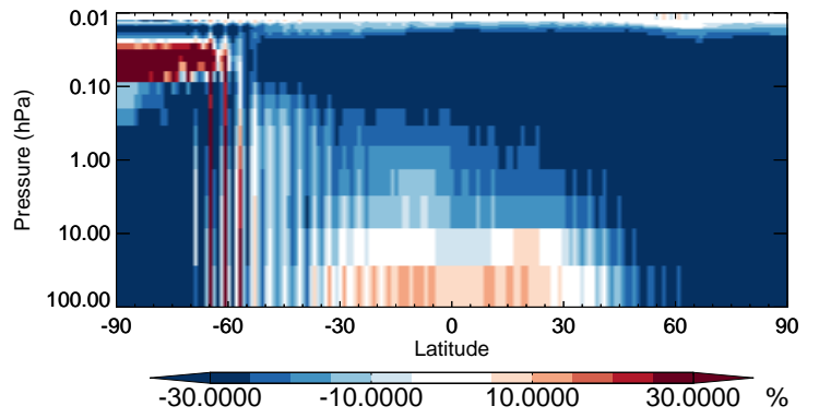
v11-02b-HP / v11-02a HNO 2 - Strat zonal mean % diff for Jul
