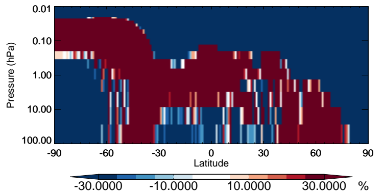
v11-02b-HP / v11-02a ISOP - Strat zonal mean % diff for Jul
