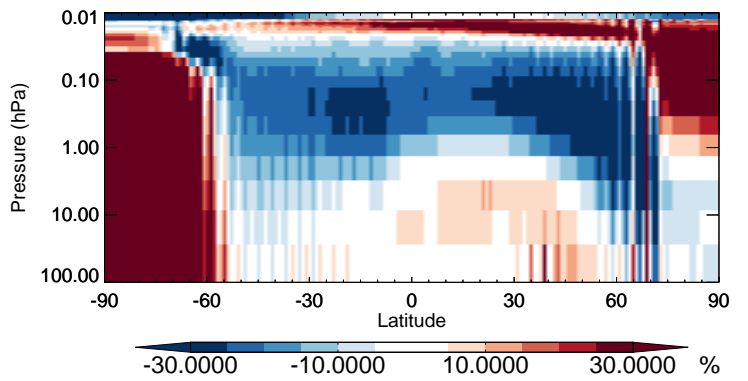
v11-02b-HP / v11-02a BrCl - Strat zonal mean % diff for Jul
