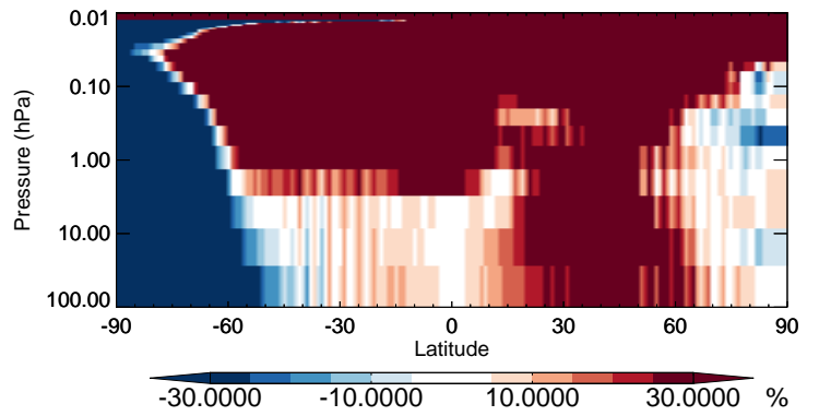
v11-02b-HP / v11-02a C3H8 - Strat zonal mean % diff for Jul
