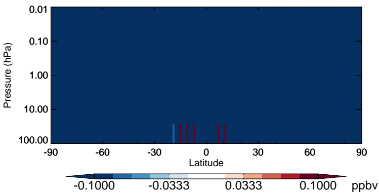
v11-02b-HP - v11-02a H 2 O - Strat zonal mean abs diff for Jul
