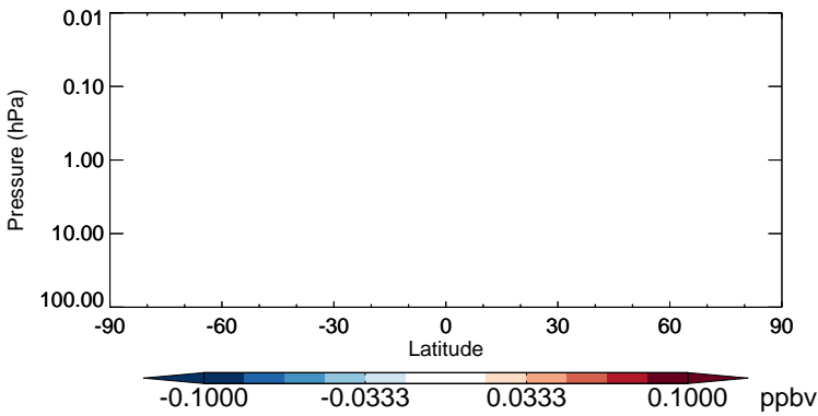
v11-02b-HP - v11-02a ClOO - Strat zonal mean abs diff for Jul
