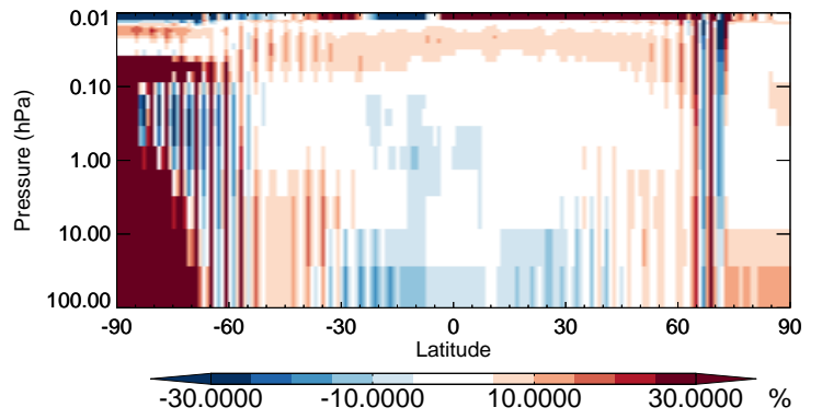
v11-02b-HP / v11-02a NO 3 - Strat zonal mean % diff for Jul
