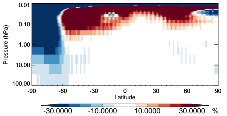
v11-02b-HP / v11-02a OCS - Strat zonal mean % diff for Jul
