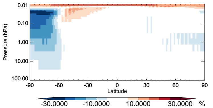
v11-02b-HP / v11-02a CH4 - Strat zonal mean % diff for Jul
