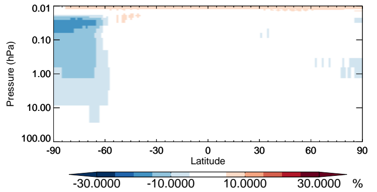
v11-02b-HP / v11-02a HCFC22 - Strat zonal mean % diff for Jul
