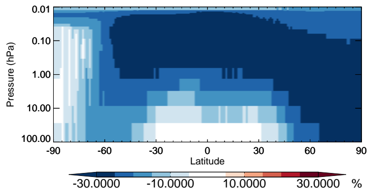
v11-02b-HP / v11-02a H 2 O - Strat zonal mean % diff for Jul
