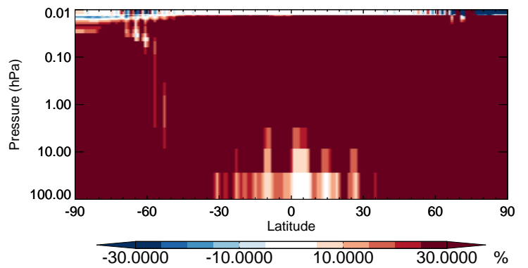
v11-02b-HP / v11-02a Br2 - Strat zonal mean % diff for Jul
