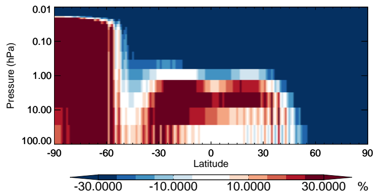
v11-02b-HP / v11-02a ISOG1 - Strat zonal mean % diff for Jul
