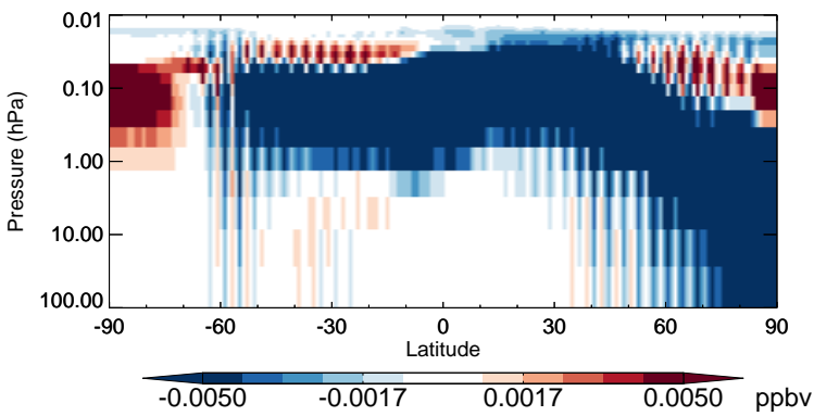
v11-02b-HP - v11-02a HNO4 - Strat zonal mean abs diff for Jul
