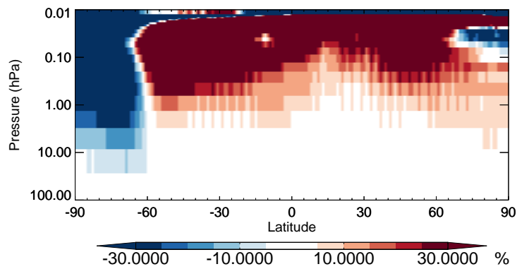
v11-02b-HP / v11-02a CCl4 - Strat zonal mean % diff for Jul
