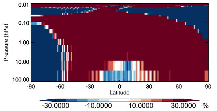
v11-02b-HP / v11-02a MVKN - Strat zonal mean % diff for Jul
