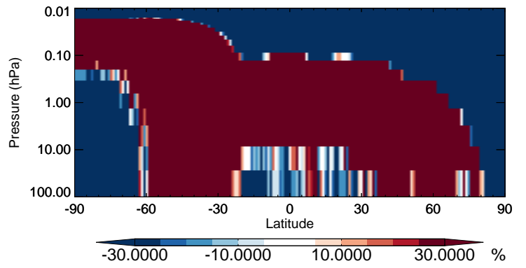
v11-02b-HP / v11-02a MVK - Strat zonal mean % diff for Jul
