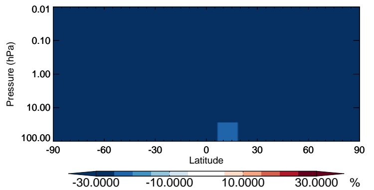
v11-02b-HP / v11-02a ASOA3 - Strat zonal mean % diff for Jul
