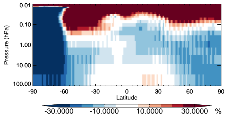
v11-02b-HP / v11-02a C2H6 - Strat zonal mean % diff for Jul
