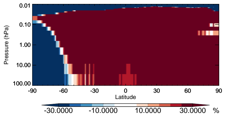
v11-02b-HP / v11-02a BENZ - Strat zonal mean % diff for Jul
