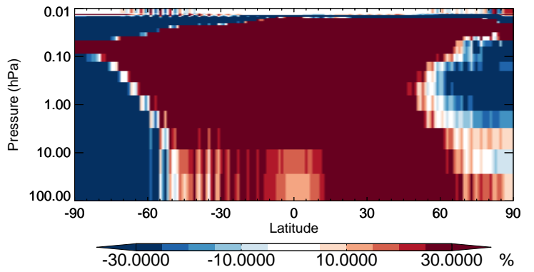
v11-02b-HP / v11-02a MEK - Strat zonal mean % diff for Jul
