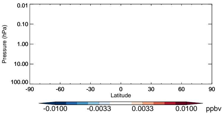
v11-02b-HP - v11-02a Br2 - Strat zonal mean abs diff for Jul
