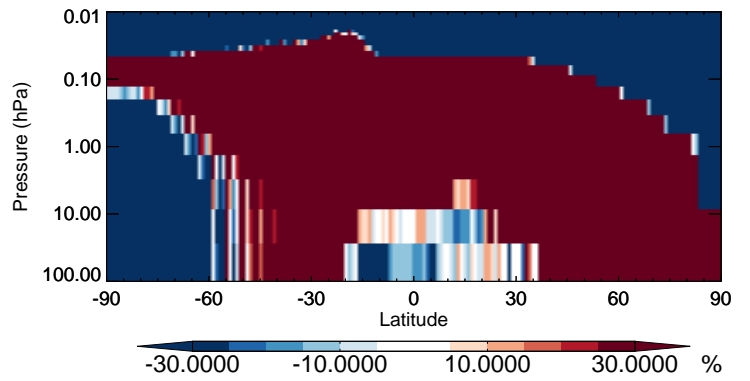
v11-02b-HP / v11-02a XYLE - Strat zonal mean % diff for Jul
