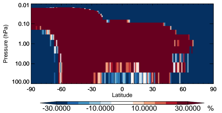
v11-02b-HP / v11-02a PRPE - Strat zonal mean % diff for Jul
