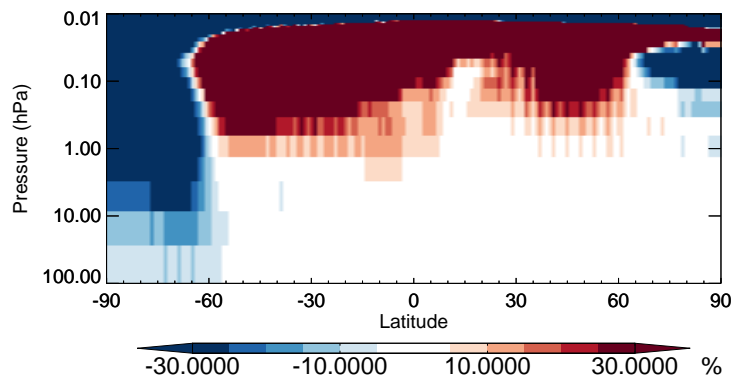
v11-02b-HP / v11-02a H1211 - Strat zonal mean % diff for Jul
