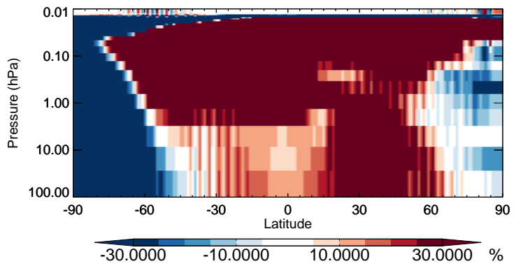
v11-02b-HP / v11-02a RCHO - Strat zonal mean % diff for Jul
