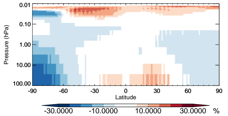
v11-02b-HP / v11-02a CO - Strat zonal mean % diff for Jul
