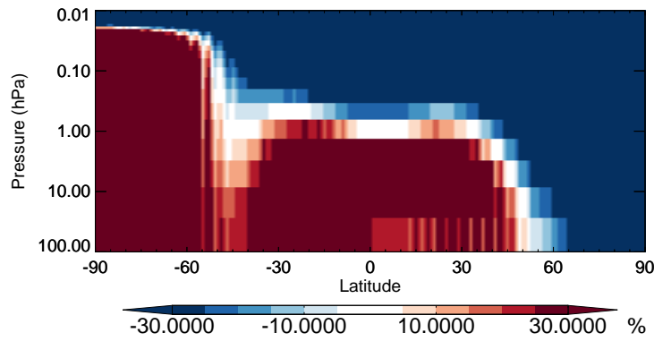
v11-02b-HP / v11-02a ASOG1 - Strat zonal mean % diff for Jul
