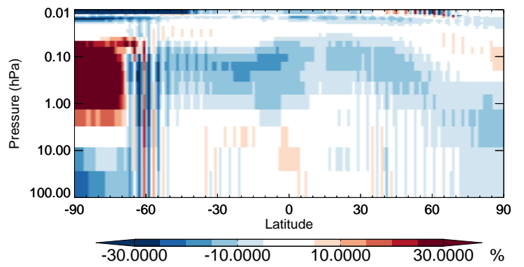
v11-02b-HP / v11-02a HNO4 - Strat zonal mean % diff for Jul
