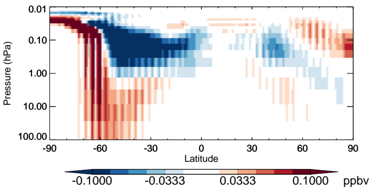
v11-02b-HP - v11-02a ClONO2 - Strat zonal mean abs diff for Jul
