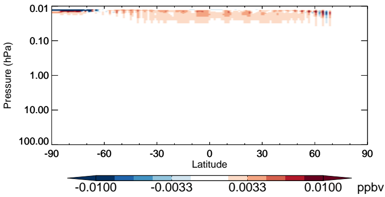
v11-02b-HP - v11-02a NO 3 - Strat zonal mean abs diff for Jul
