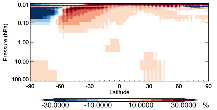
v11-02b-HP / v11-02a PPN - Strat zonal mean % diff for Jul
