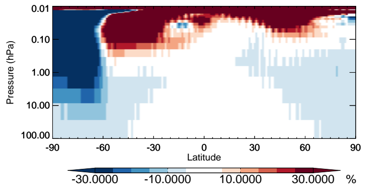
v11-02b-HP / v11-02a H1301 - Strat zonal mean % diff for Jul
