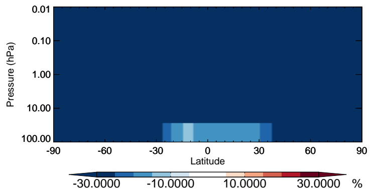
v11-02b-HP / v11-02a ASOAN - Strat zonal mean % diff for Jul
