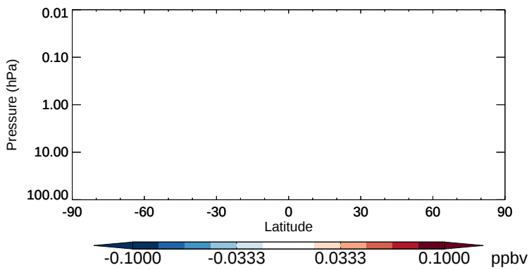
v11-02b-HP - v11-02a ISOA1 - Strat zonal mean abs diff for Oct
