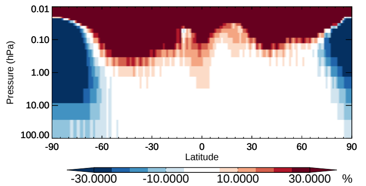
v11-02b-HP / v11-02a CH 3 Br - Strat zonal mean % diff for Oct
