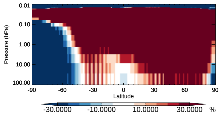
v11-02b-HP / v11-02a BENZ - Strat zonal mean % diff for Oct
