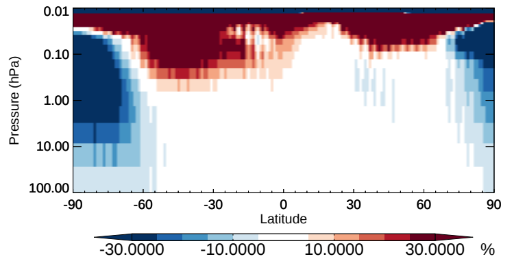
v11-02b-HP / v11-02a OCS - Strat zonal mean % diff for Oct
