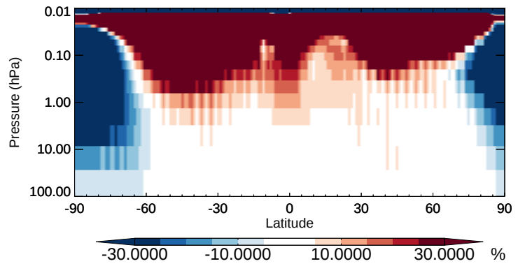
v11-02b-HP / v11-02a H2402 - Strat zonal mean % diff for Oct
