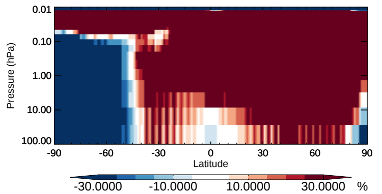
v11-02b-HP / v11-02a ALK4 - Strat zonal mean % diff for Oct
