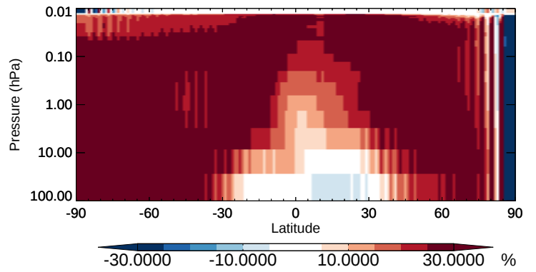
v11-02b-HP / v11-02a BrO - Strat zonal mean % diff for Oct
