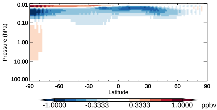
v11-02b-HP - v11-02a NO - Strat zonal mean abs diff for Oct
