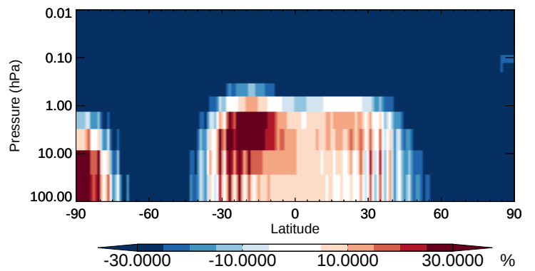
v11-02b-HP / v11-02a ISOG1 - Strat zonal mean % diff for Oct
