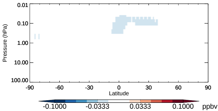
v11-02b-HP - v11-02a MPN - Strat zonal mean abs diff for Oct
