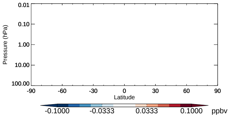
v11-02b-HP - v11-02a TSOA0 - Strat zonal mean abs diff for Oct
