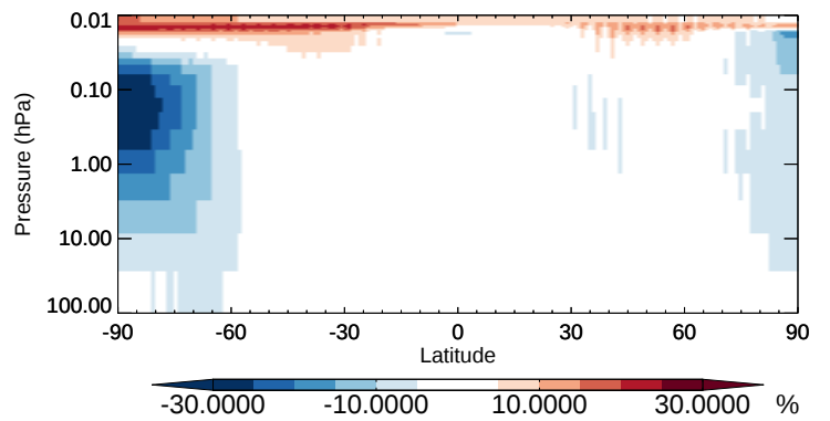
v11-02b-HP / v11-02a CH4 - Strat zonal mean % diff for Oct
