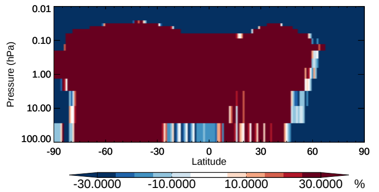
v11-02b-HP / v11-02a PRPE - Strat zonal mean % diff for Oct
