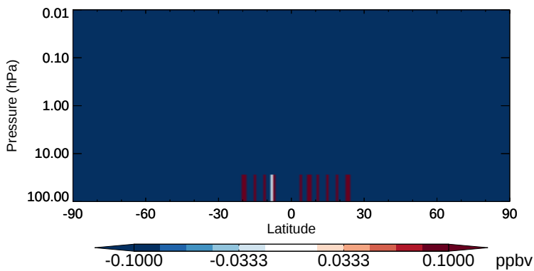
v11-02b-HP - v11-02a H 2 O - Strat zonal mean abs diff for Oct
