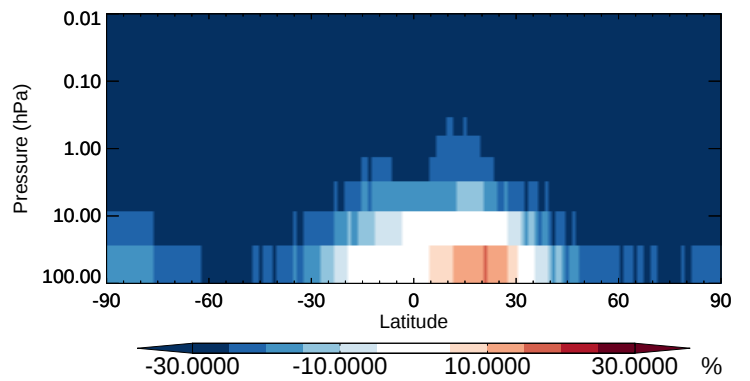
v11-02b-HP / v11-02a MSA - Strat zonal mean % diff for Oct
