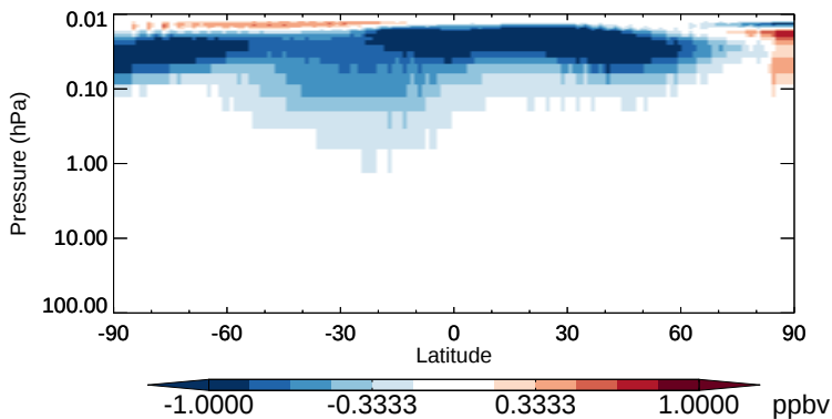
v11-02b-HP - v11-02a NO2 - Strat zonal mean abs diff for Oct
