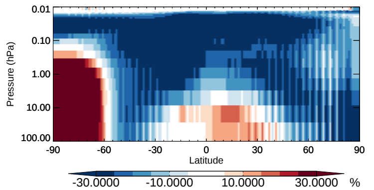
v11-02b-HP / v11-02a HNO 2 - Strat zonal mean % diff for Oct
