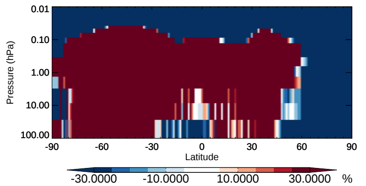
v11-02b-HP / v11-02a MACR - Strat zonal mean % diff for Oct
