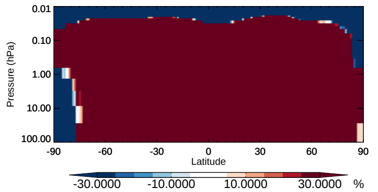
v11-02b-HP / v11-02a BCPO - Strat zonal mean % diff for Oct
