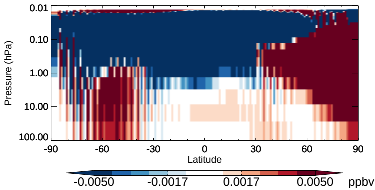
v11-02b-HP - v11-02a N2O5 - Strat zonal mean abs diff for Oct
