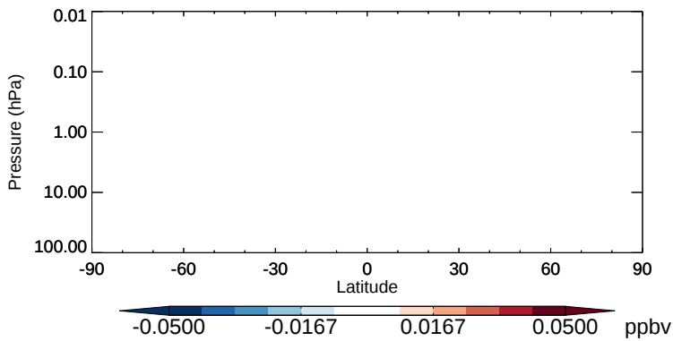
v11-02b-HP - v11-02a RCHO - Strat zonal mean abs diff for Oct
