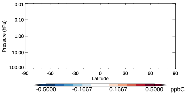
v11-02b-HP - v11-02a ALK4 - Strat zonal mean abs diff for Oct
