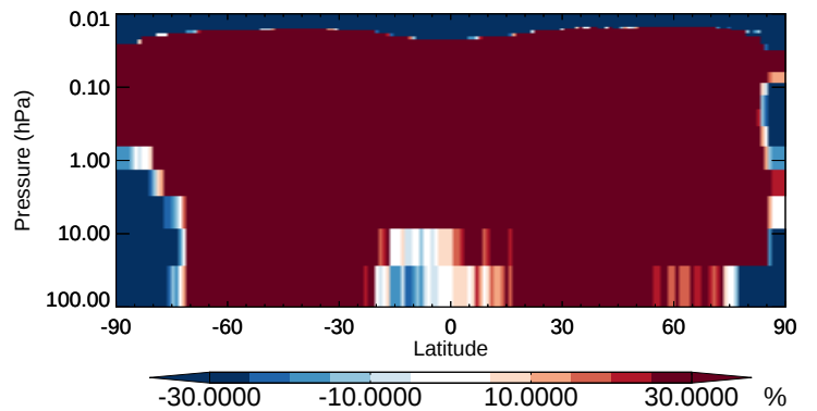
v11-02b-HP / v11-02a TOLU - Strat zonal mean % diff for Oct
