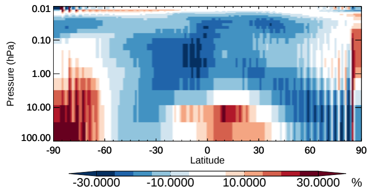
v11-02b-HP / v11-02a NO2 - Strat zonal mean % diff for Oct
