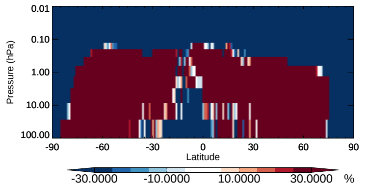
v11-02b-HP / v11-02a ISOP - Strat zonal mean % diff for Oct
