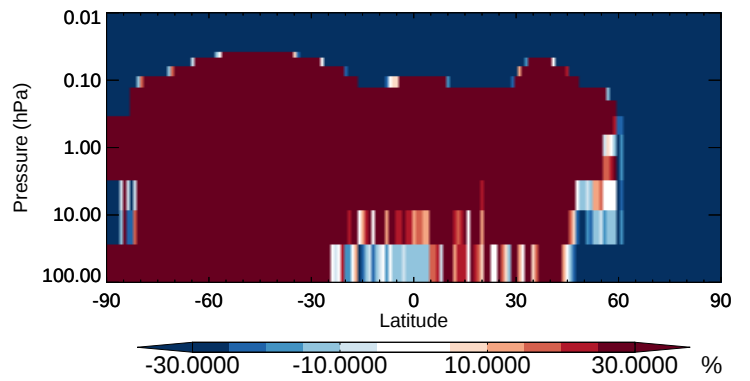
v11-02b-HP / v11-02a PMN - Strat zonal mean % diff for Oct
