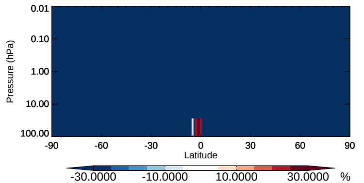
v11-02b-HP / v11-02a NH 3 - Strat zonal mean % diff for Oct
