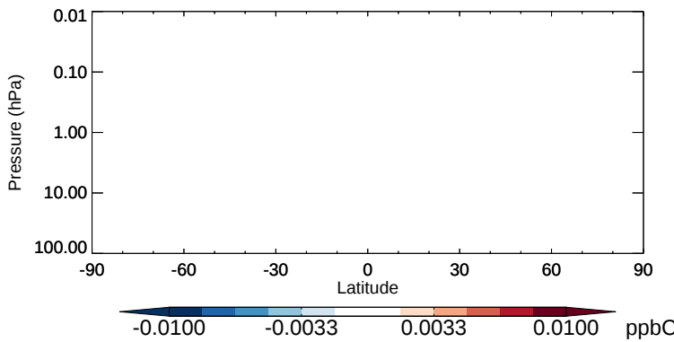
v11-02b-HP - v11-02a PRPE - Strat zonal mean abs diff for Oct
