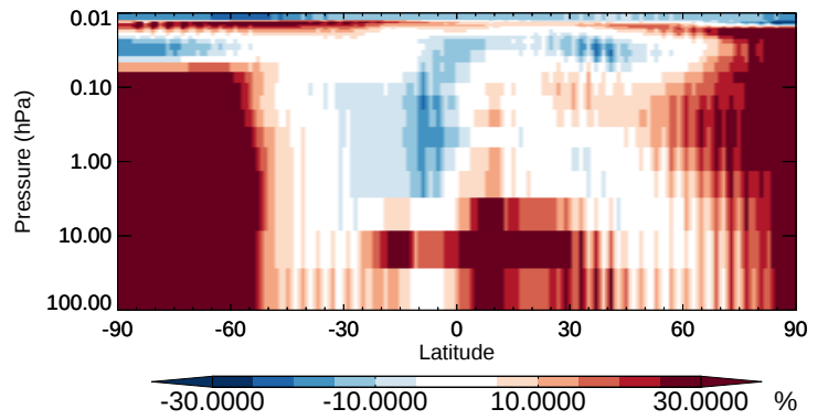
v11-02b-HP / v11-02a BrNO 2 - Strat zonal mean % diff for Oct
