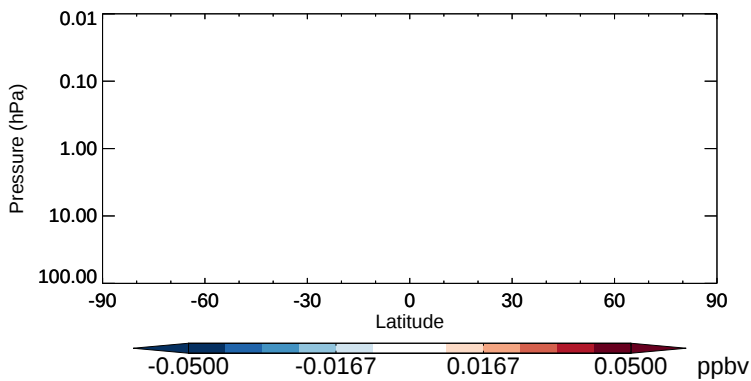
v11-02b-HP - v11-02a MACR - Strat zonal mean abs diff for Oct
