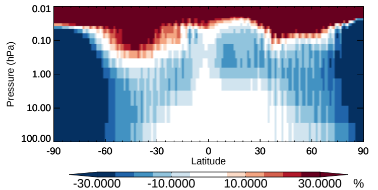
v11-02b-HP / v11-02a C2H6 - Strat zonal mean % diff for Oct
