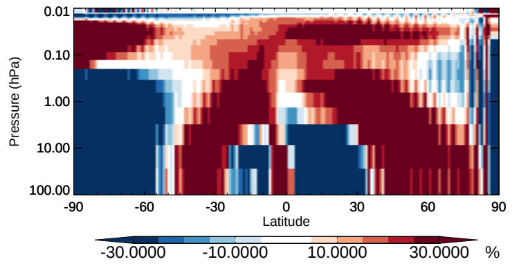
v11-02b-HP / v11-02a Cl 2 O 2 - Strat zonal mean % diff for Oct
