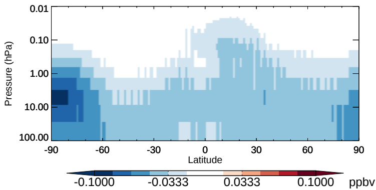
v11-02b-HP - v11-02a EOH - Strat zonal mean abs diff for Oct
