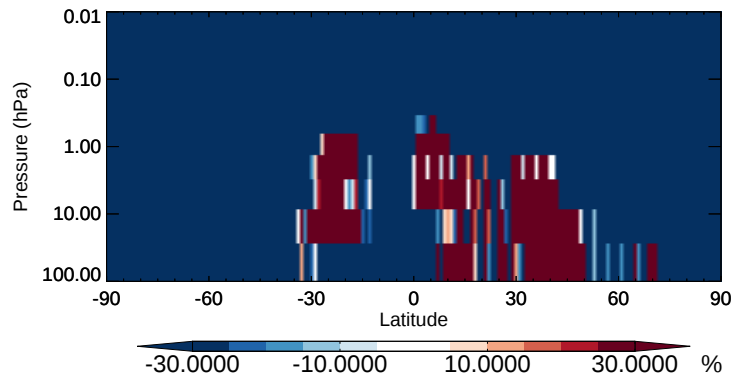
v11-02b-HP / v11-02a LIMO - Strat zonal mean % diff for Oct
