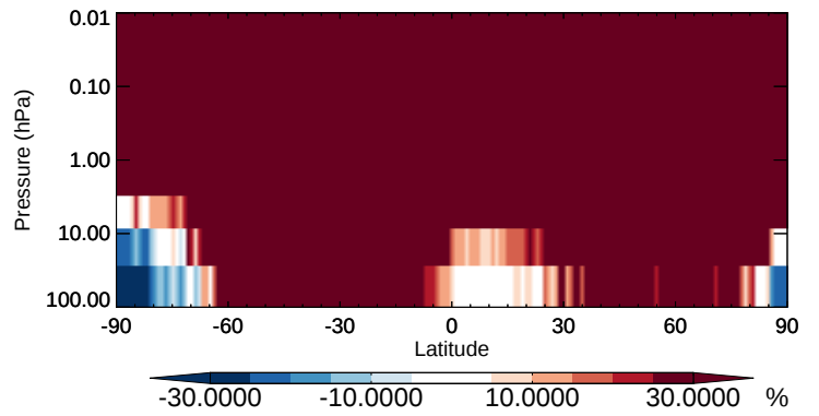
v11-02b-HP / v11-02a SALC - Strat zonal mean % diff for Oct
