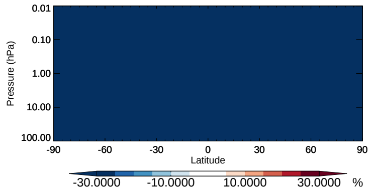
v11-02b-HP / v11-02a BCPI - Strat zonal mean % diff for Oct
