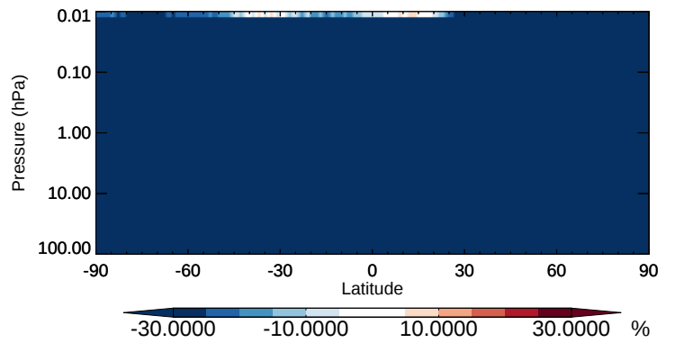
v11-02b-HP / v11-02a SO4 - Strat zonal mean % diff for Oct
