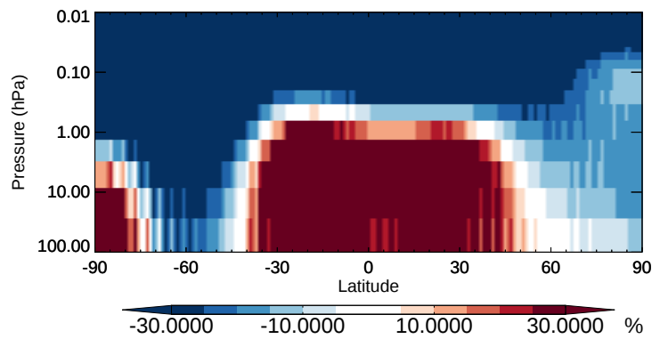
v11-02b-HP / v11-02a ASOG1 - Strat zonal mean % diff for Oct
