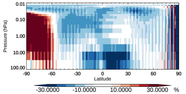
v11-02b-HP / v11-02a ClOO - Strat zonal mean % diff for Oct
