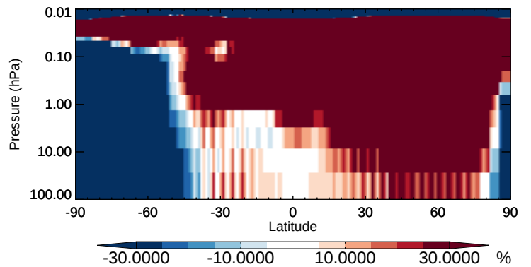
v11-02b-HP / v11-02a CHBr 3 - Strat zonal mean % diff for Oct
