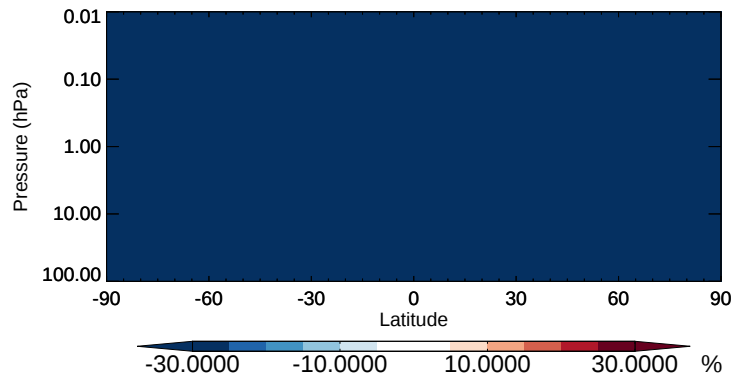
v11-02b-HP / v11-02a TSOA1 - Strat zonal mean % diff for Oct
