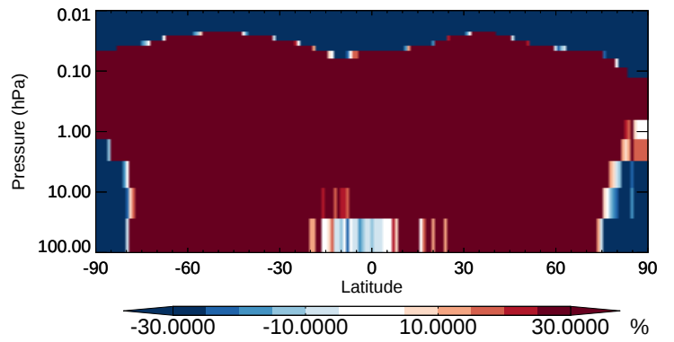
v11-02b-HP / v11-02a XYLE - Strat zonal mean % diff for Oct
