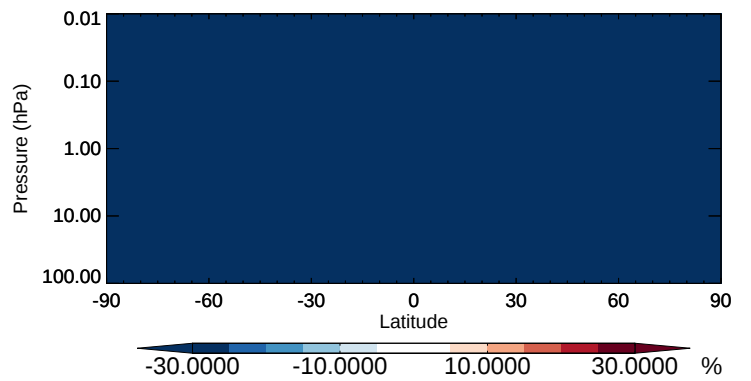
v11-02b-HP / v11-02a TSOA2 - Strat zonal mean % diff for Oct
