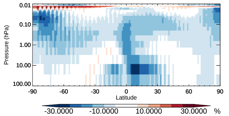
v11-02b-HP / v11-02a MPN - Strat zonal mean % diff for Oct
