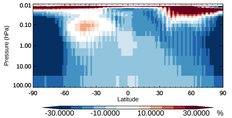
v11-02b-HP / v11-02a EOH - Strat zonal mean % diff for Oct
