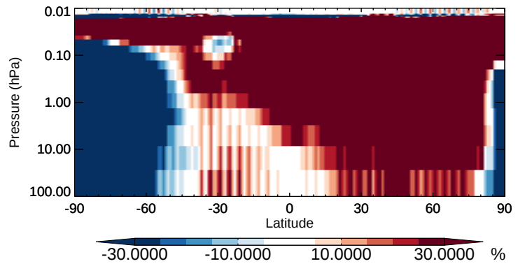
v11-02b-HP / v11-02a MEK - Strat zonal mean % diff for Oct
