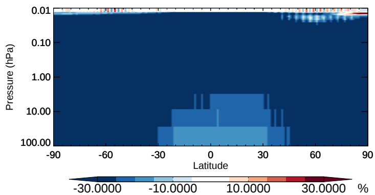
v11-02b-HP / v11-02a MGLY - Strat zonal mean % diff for Oct
