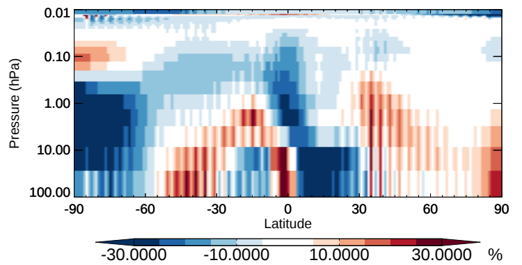
v11-02b-HP / v11-02a ClNO3 - Strat zonal mean % diff for Oct
