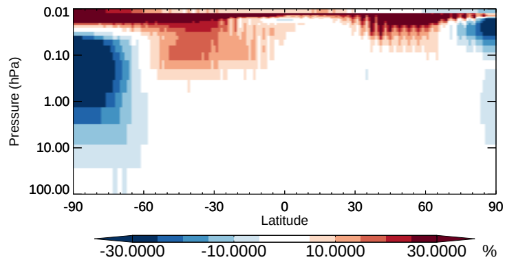
v11-02b-HP / v11-02a N 2 O - Strat zonal mean % diff for Oct
