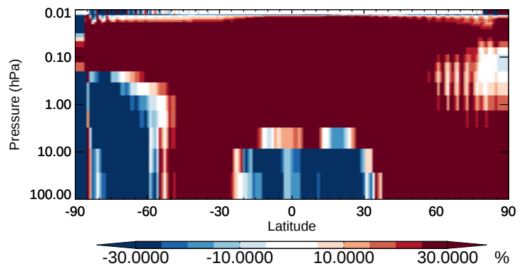
v11-02b-HP / v11-02a OCIO - Strat zonal mean % diff for Oct
