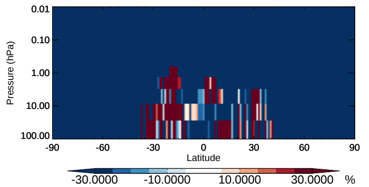
v11-02b-HP / v11-02a MTPO - Strat zonal mean % diff for Oct
