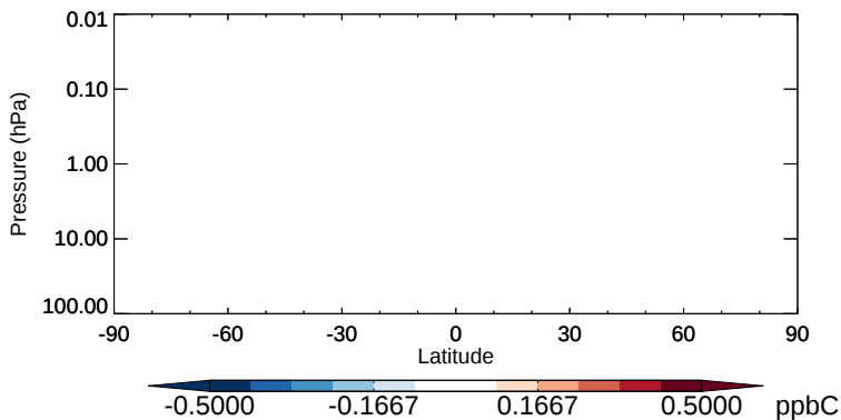
v11-02b-HP - v11-02a C2H6 - Strat zonal mean abs diff for Oct
