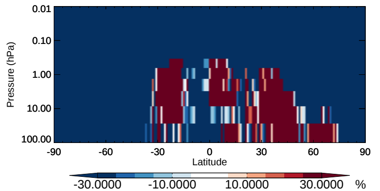
v11-02b-HP / v11-02a MTPA - Strat zonal mean % diff for Oct
