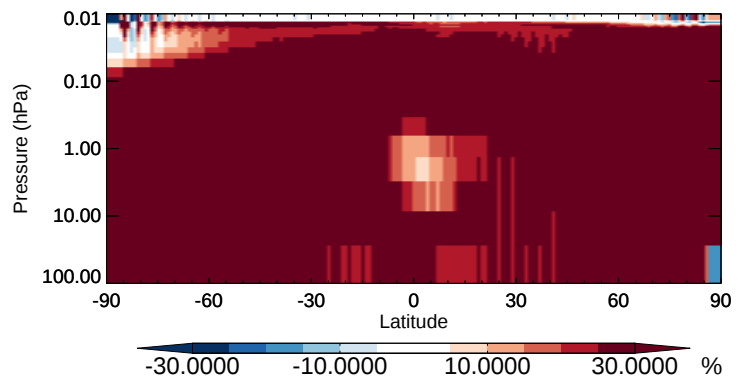
v11-02b-HP / v11-02a BrNO 3 - Strat zonal mean % diff for Oct
