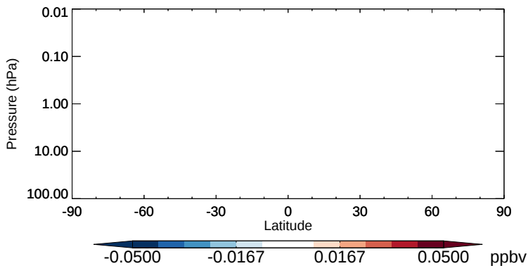
v11-02b-HP - v11-02a MP - Strat zonal mean abs diff for Oct
