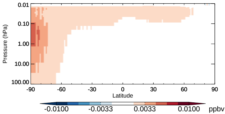
v11-02b-HP - v11-02a BrO - Strat zonal mean abs diff for Oct
