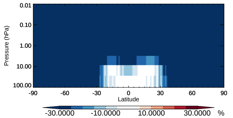
v11-02b-HP / v11-02a ASOG2 - Strat zonal mean % diff for Oct
