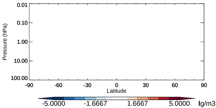
v11-02b-HP - v11-02a DST2 - Strat zonal mean abs diff for Oct
