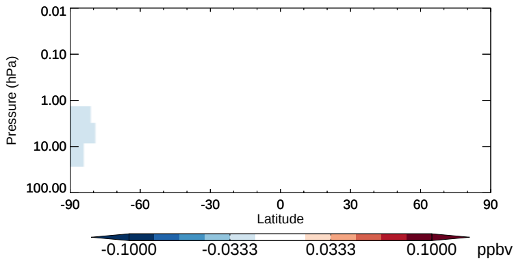
v11-02b-HP - v11-02a Cl 2 O 2 - Strat zonal mean abs diff for Oct
