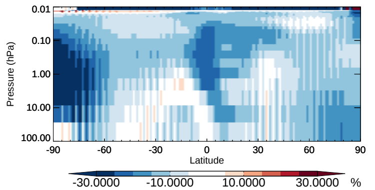
v11-02b-HP / v11-02a HNO4 - Strat zonal mean % diff for Oct
