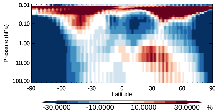
v11-02b-HP / v11-02a PAN - Strat zonal mean % diff for Oct
