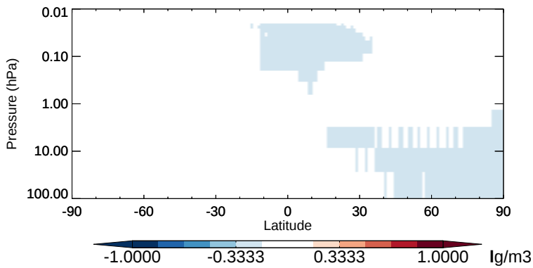
v11-02b-HP - v11-02a SO4 - Strat zonal mean abs diff for Oct
