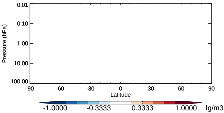
v11-02b-HP - v11-02a BCPI - Strat zonal mean abs diff for Oct
