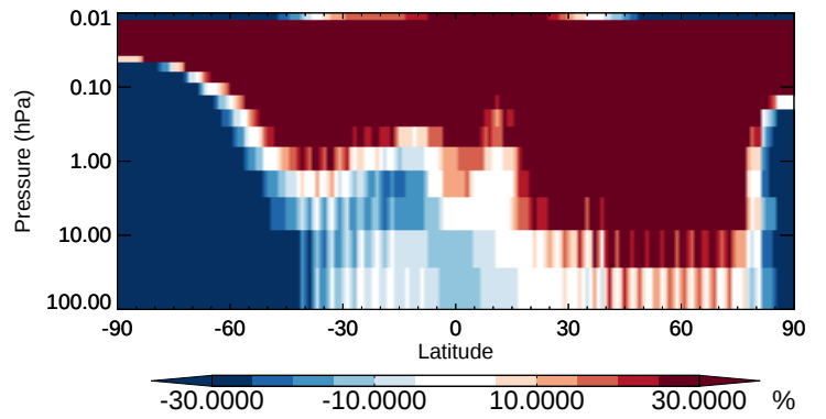
v11-02b-HP / v11-02a C3H8 - Strat zonal mean % diff for Oct
