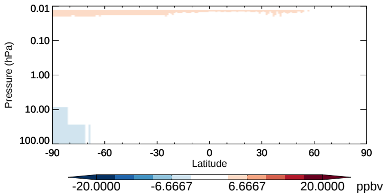
v11-02b-HP - v11-02a CO - Strat zonal mean abs diff for Oct
