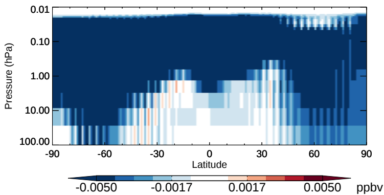
v11-02b-HP - v11-02a HNO4 - Strat zonal mean abs diff for Oct
