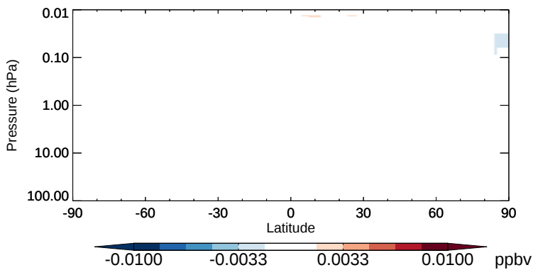
v11-02b-HP - v11-02a HOBr - Strat zonal mean abs diff for Oct
