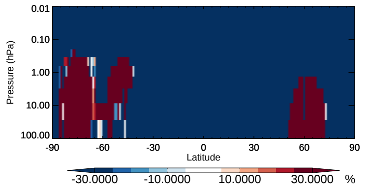
v11-02b-HP / v11-02a ClNO2 - Strat zonal mean % diff for Oct
