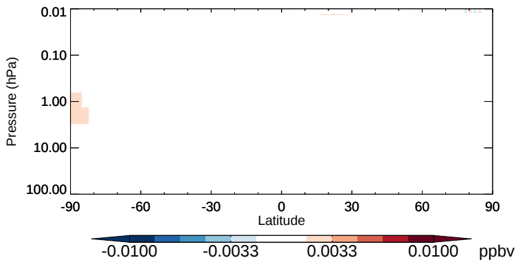
v11-02b-HP - v11-02a Br - Strat zonal mean abs diff for Oct
