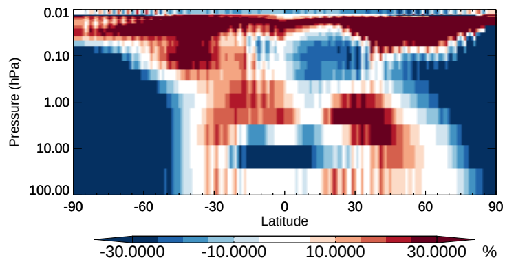
v11-02b-HP / v11-02a MAP - Strat zonal mean % diff for Oct
