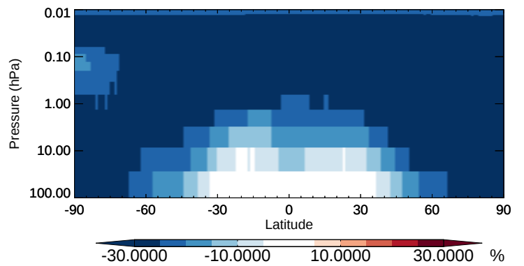
v11-02b-HP / v11-02a H 2 O - Strat zonal mean % diff for Oct
