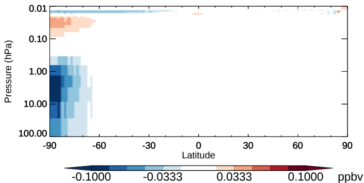
v11-02b-HP - v11-02a ClO - Strat zonal mean abs diff for Oct
