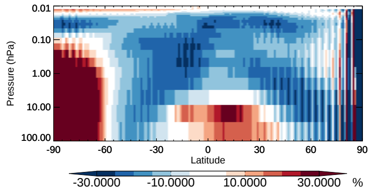
v11-02b-HP / v11-02a NO - Strat zonal mean % diff for Oct
