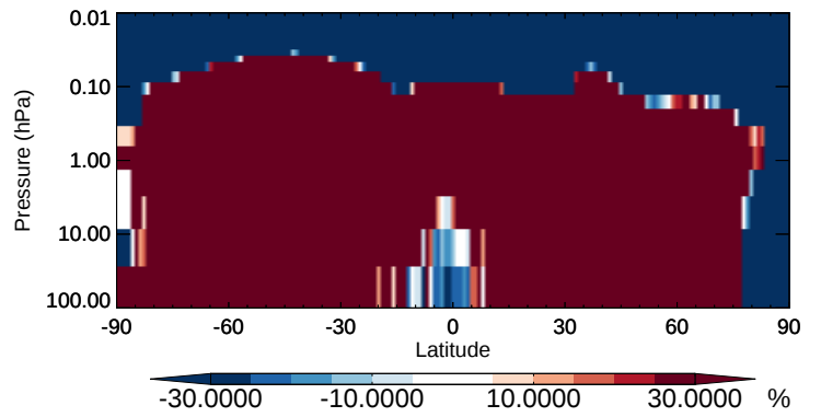
v11-02b-HP / v11-02a MVK - Strat zonal mean % diff for Oct
