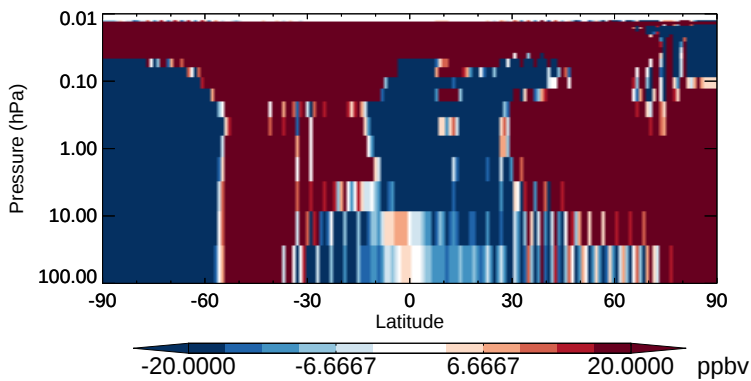
v11-02b-HP - v11-02a O3 - Strat zonal mean abs diff for Oct
