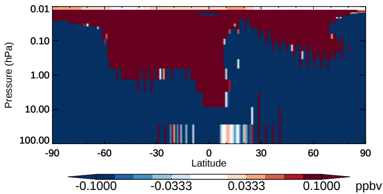
v11-02b-HP - v11-02a N 2 O - Strat zonal mean abs diff for Oct
