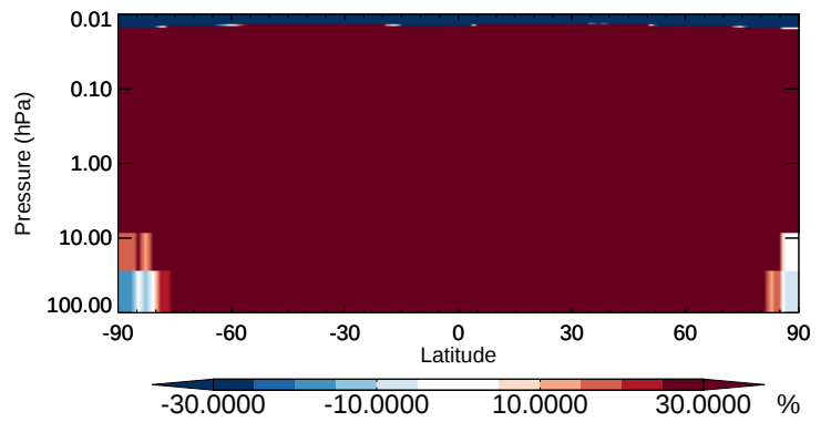
v11-02b-HP / v11-02a DST2 - Strat zonal mean % diff for Oct
