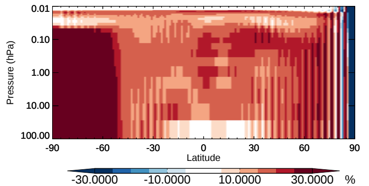
v11-02b-HP / v11-02a Br - Strat zonal mean % diff for Oct
