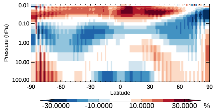
v11-02b-HP / v11-02a HOBr - Strat zonal mean % diff for Oct
