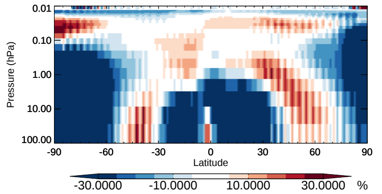
v11-02b-HP / v11-02a HOCl - Strat zonal mean % diff for Oct
