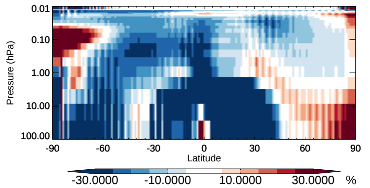
v11-02b-HP / v11-02a Cl2 - Strat zonal mean % diff for Oct
