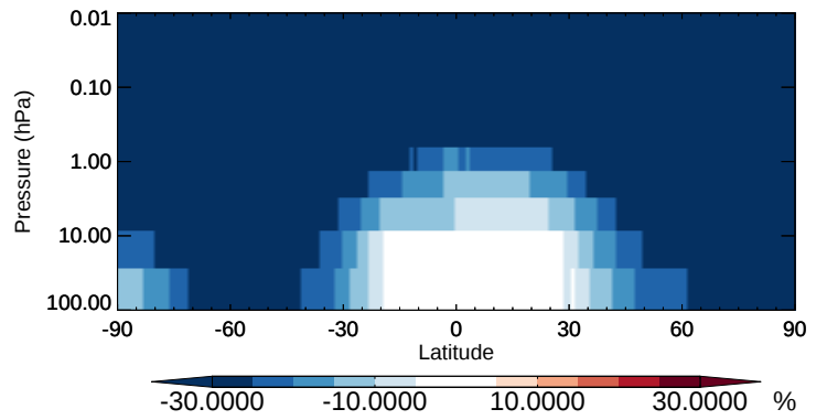
v11-02b-HP / v11-02a ASOG3 - Strat zonal mean % diff for Oct
