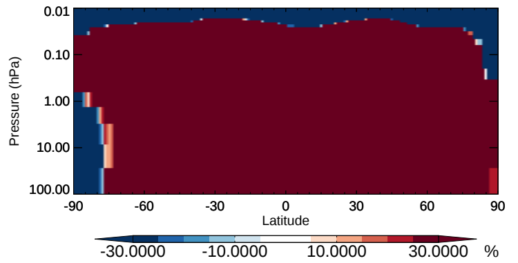
v11-02b-HP / v11-02a OCPO - Strat zonal mean % diff for Oct
