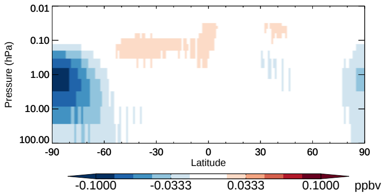
v11-02b-HP - v11-02a OCS - Strat zonal mean abs diff for Oct
