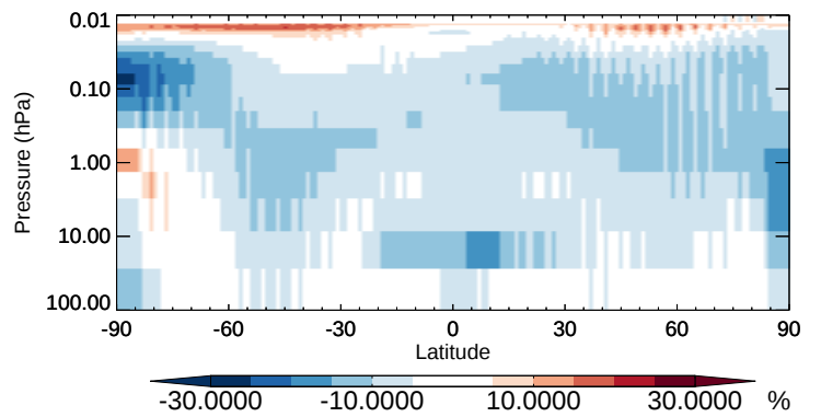
v11-02b-HP / v11-02a CH2O - Strat zonal mean % diff for Oct
