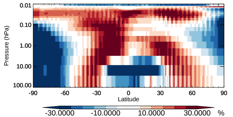
v11-02b-HP / v11-02a MP - Strat zonal mean % diff for Oct
