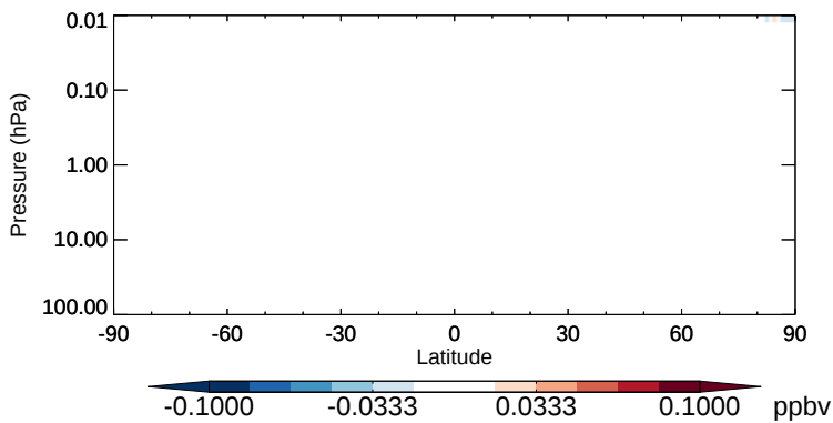
v11-02b-HP - v11-02a Cl - Strat zonal mean abs diff for Oct
