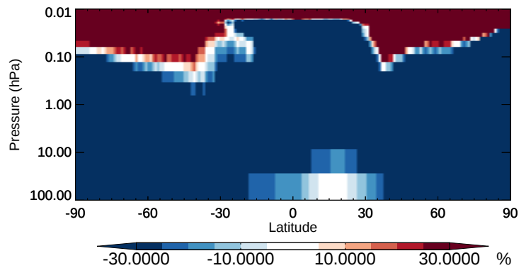
v11-02b-HP / v11-02a SALA - Strat zonal mean % diff for Oct
