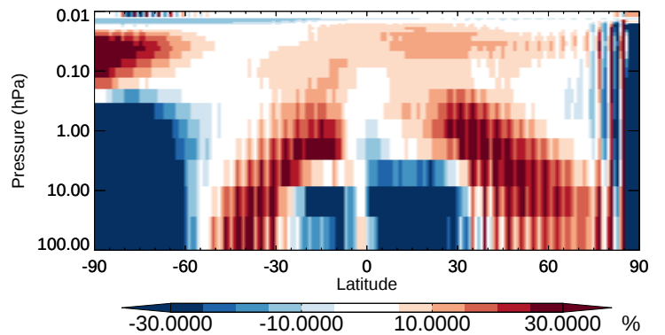
v11-02b-HP / v11-02a ClO - Strat zonal mean % diff for Oct
