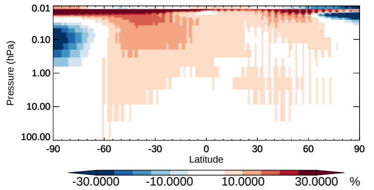
v11-02b-HP / v11-02a PPN - Strat zonal mean % diff for Oct
