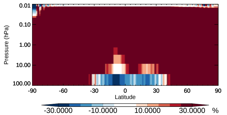
v11-02b-HP / v11-02a Br2 - Strat zonal mean % diff for Oct
