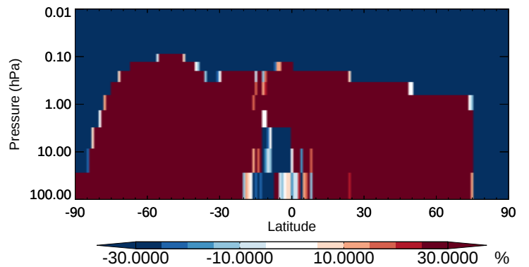
v11-02b-HP / v11-02a RIP - Strat zonal mean % diff for Oct
