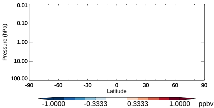
v11-02b-HP - v11-02a HNO 2 - Strat zonal mean abs diff for Oct
