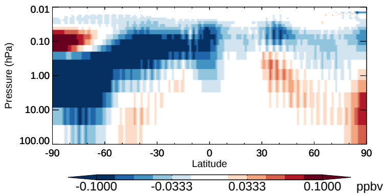
v11-02b-HP - v11-02a ClNO3 - Strat zonal mean abs diff for Oct
