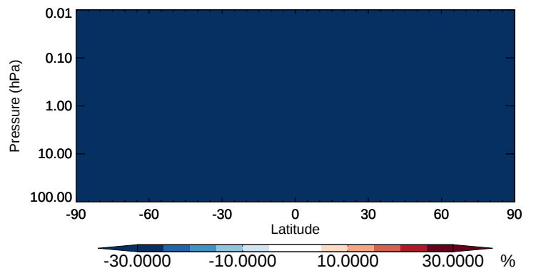
v11-02b-HP / v11-02a ISOA1 - Strat zonal mean % diff for Oct
