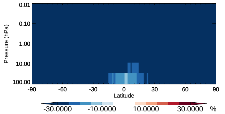
v11-02b-HP / v11-02a ISOG3 - Strat zonal mean % diff for Oct
