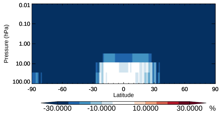
v11-02b-HP / v11-02a ISOG2 - Strat zonal mean % diff for Oct
