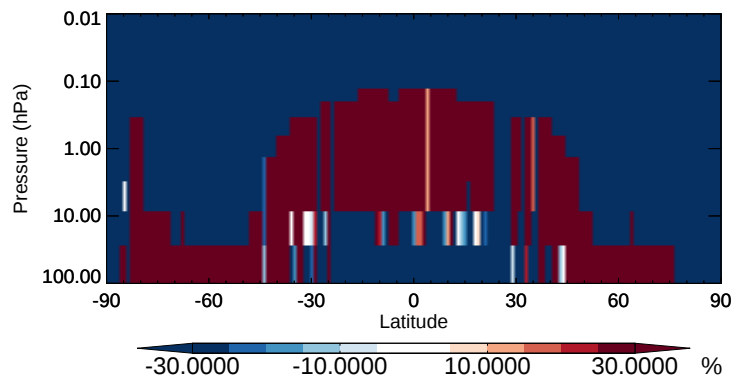
v11-02b-HP / v11-02a NIT - Strat zonal mean % diff for Oct
