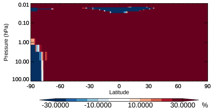
v11-02b-HP / v11-02a DMS - Strat zonal mean % diff for Oct
