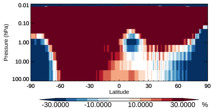
v11-02b-HP / v11-02a DST1 - Strat zonal mean % diff for Oct
