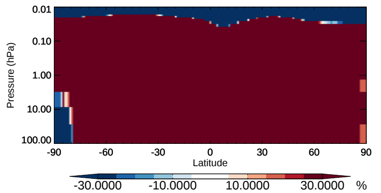
v11-02b-HP / v11-02a DST4 - Strat zonal mean % diff for Oct
