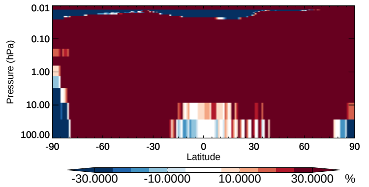
v11-02b-HP / v11-02a IEPOX - Strat zonal mean % diff for Oct
