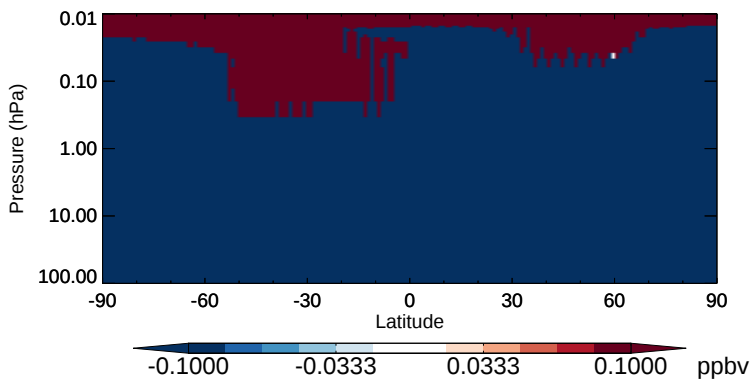
v11-02b-HP - v11-02a CH4 - Strat zonal mean abs diff for Oct
