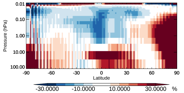
v11-02b-HP / v11-02a N2O5 - Strat zonal mean % diff for Oct
