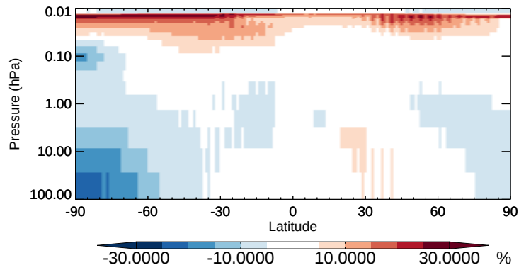
v11-02b-HP / v11-02a CO - Strat zonal mean % diff for Oct
