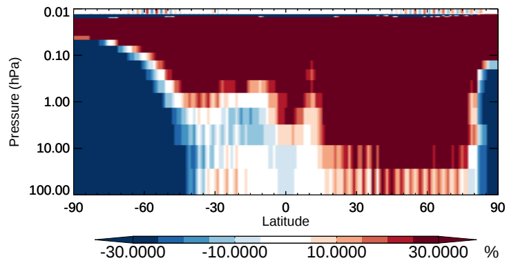
v11-02b-HP / v11-02a RCHO - Strat zonal mean % diff for Oct
