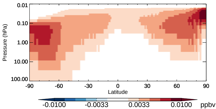
v11-02b-HP - v11-02a BrNO 3 - Strat zonal mean abs diff for Oct
