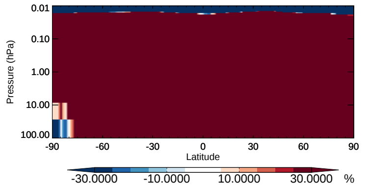
v11-02b-HP / v11-02a DST3 - Strat zonal mean % diff for Oct
