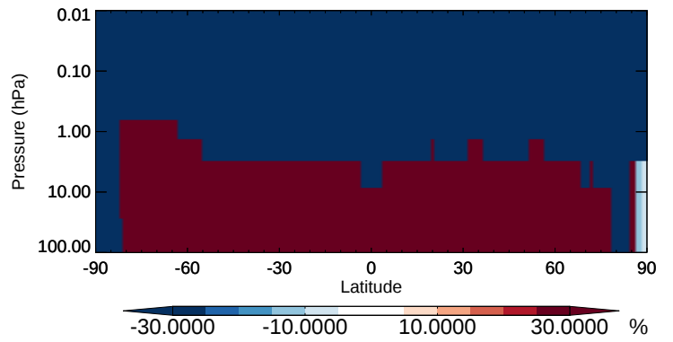
v11-02b-HP / v11-02a SO 4 s - Strat zonal mean % diff for Oct
