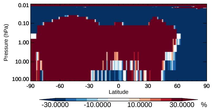
v11-02b-HP / v11-02a MACRN - Strat zonal mean % diff for Oct
