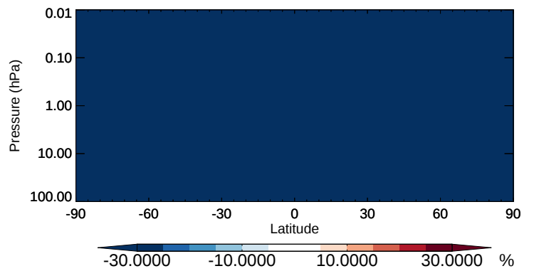
v11-02b-HP / v11-02a OCPI - Strat zonal mean % diff for Oct
