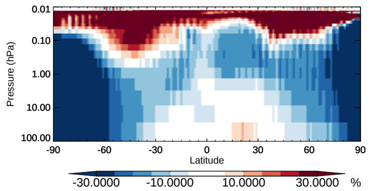
v11-02b-HP / v11-02a ALD2 - Strat zonal mean % diff for Oct
