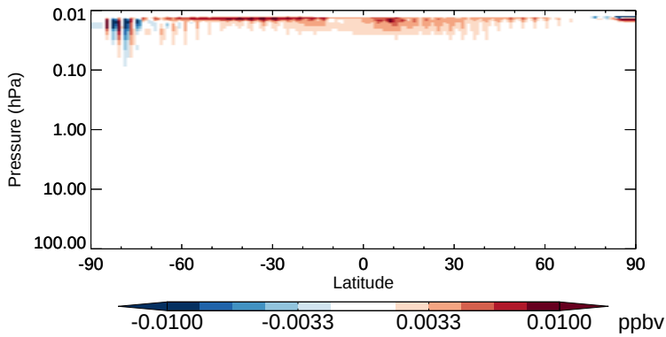
v11-02b-HP - v11-02a NO 3 - Strat zonal mean abs diff for Oct
