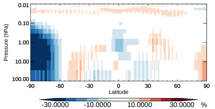
v11-02b-HP / v11-02a O3 - Strat zonal mean % diff for Oct
