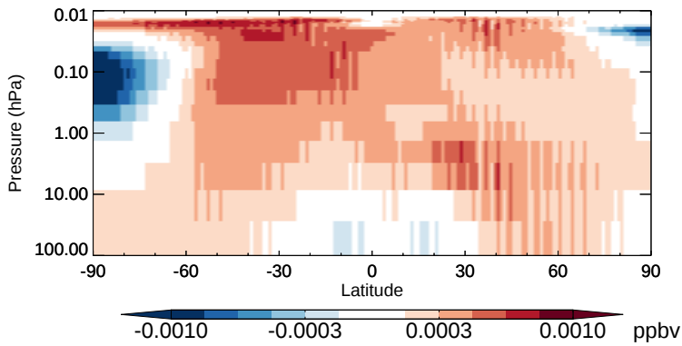
v11-02b-HP - v11-02a PPN - Strat zonal mean abs diff for Oct
