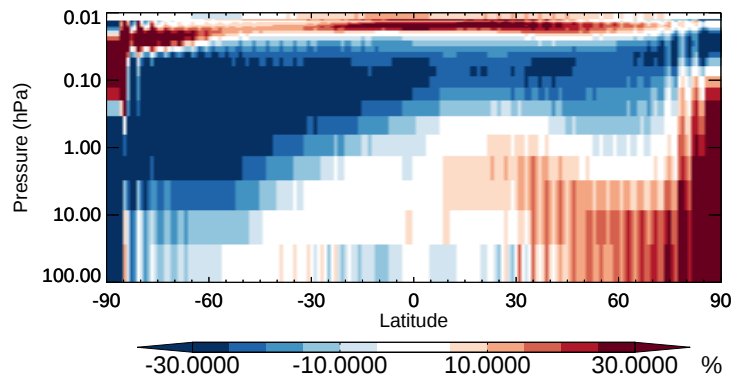
v11-02b-HP / v11-02a BrCl - Strat zonal mean % diff for Oct
