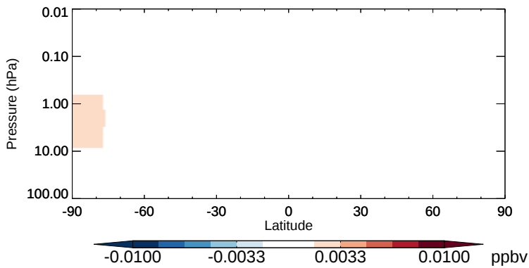
v11-02b-HP - v11-02a HBr - Strat zonal mean abs diff for Oct
