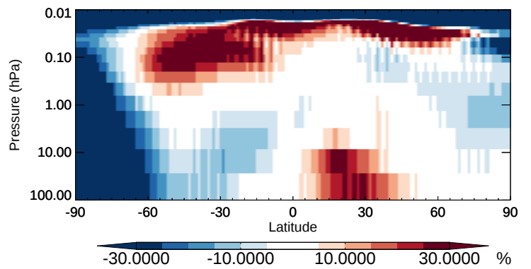
v11-02b-HP / v11-02a SO2 - Strat zonal mean % diff for Oct
