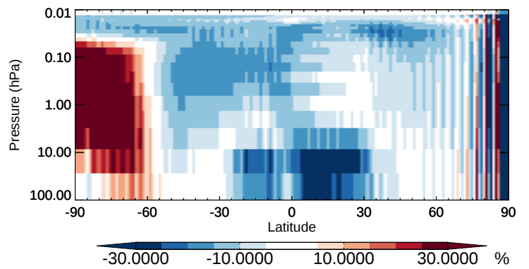
v11-02b-HP / v11-02a Cl - Strat zonal mean % diff for Oct
