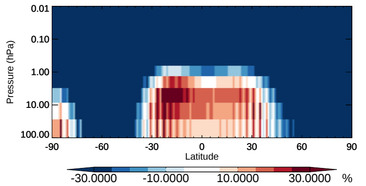
v11-02b-HP / v11-02a TSOG1 - Strat zonal mean % diff for Oct
