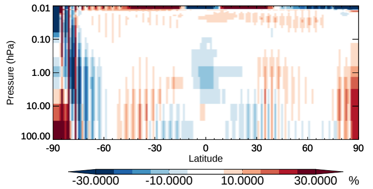
v11-02b-HP / v11-02a NO 3 - Strat zonal mean % diff for Oct
