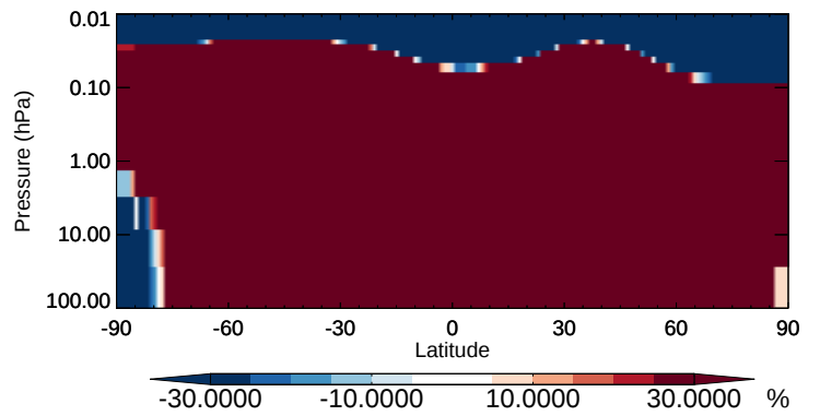
v11-02b-HP / v11-02a NITs - Strat zonal mean % diff for Oct
