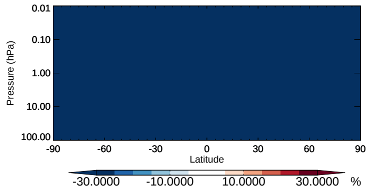
v11-02b-HP / v11-02a ASOAN - Strat zonal mean % diff for Oct
