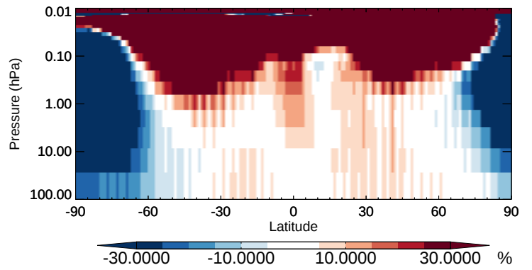
v11-02b-HP / v11-02a CH 2 Br 2 - Strat zonal mean % diff for Oct
