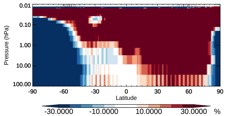
v11-02b-HP / v11-02a R4N2 - Strat zonal mean % diff for Oct
