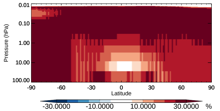
v11-02b-HP / v11-02a HBr - Strat zonal mean % diff for Oct
