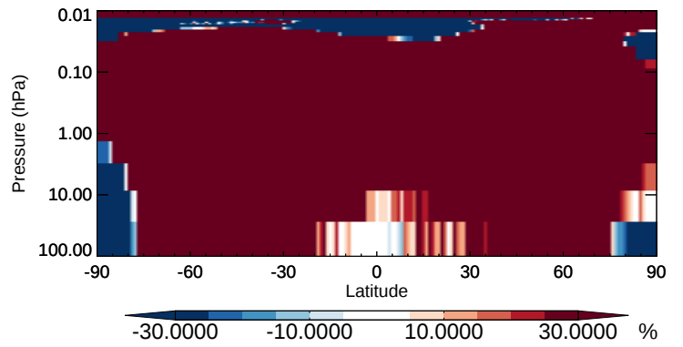
v11-02b-HP / v11-02a MVKN - Strat zonal mean % diff for Oct
