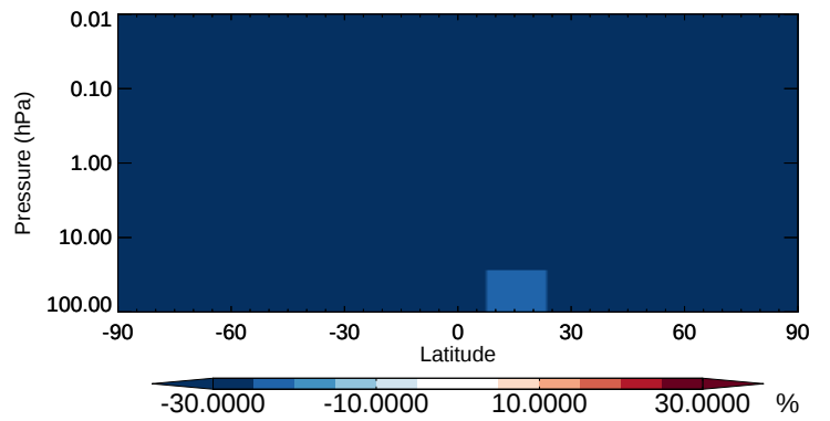
v11-02b-HP / v11-02a ASOA1 - Strat zonal mean % diff for Oct
