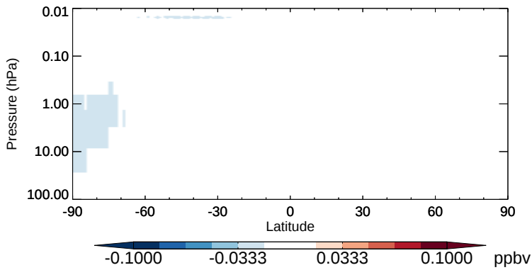
v11-02b-HP - v11-02a HOCl - Strat zonal mean abs diff for Oct
