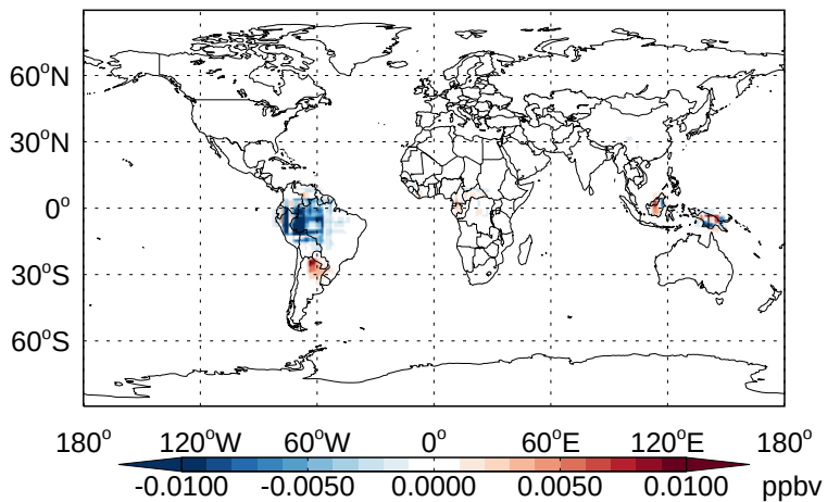
v11-02b-HP - v11-02a RIP- Diff @ 500 hPa for Apr
