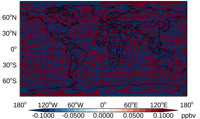
v11-02b-HP - v11-02a H 2 O- Diff @ 500 hPa for Apr
