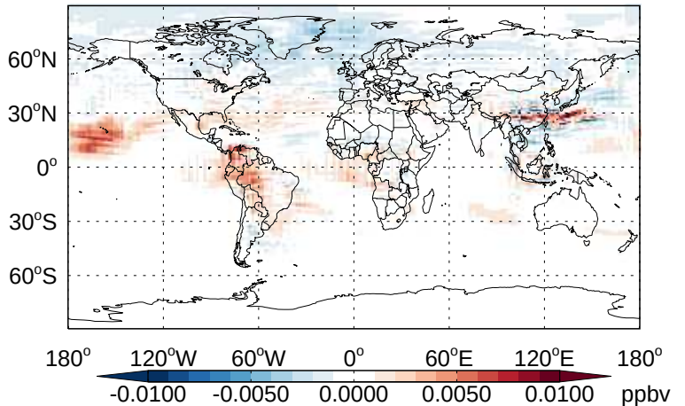
v11-02b-HP - v11-02a R4N2- Diff @ 500 hPa for Apr
