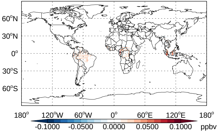
v11-02b-HP - v11-02a TSOA1 - Diff @ Surface for Apr
