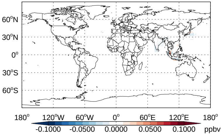
v11-02b-HP - v11-02a ASOAN - Diff @ Surface for Apr
