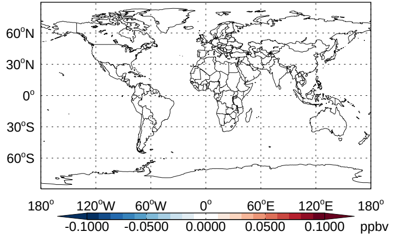
v11-02b-HP - v11-02a TSOA2- Diff @ 500 hPa for Apr
