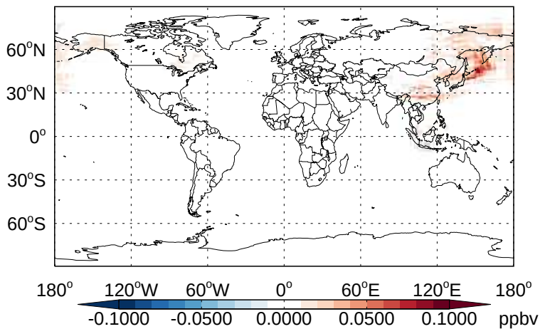
v11-02b-HP - v11-02a TOLU- Diff @ 500 hPa for Apr
