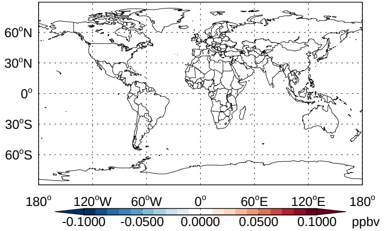
v11-02b-HP - v11-02a TSOG2- Diff @ 500 hPa for Apr
