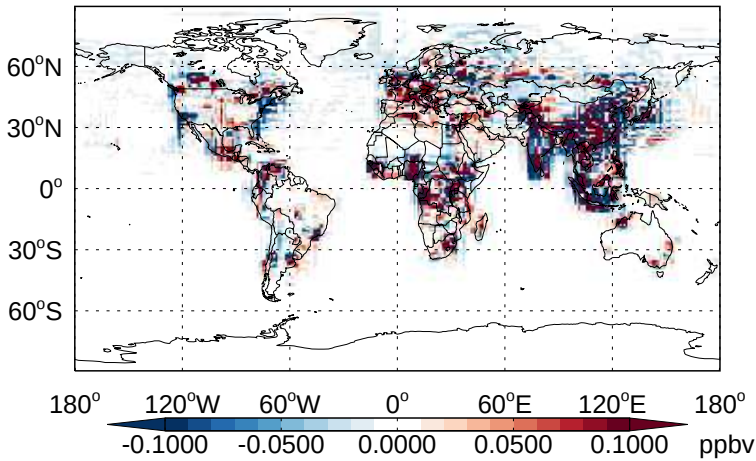
v11-02b-HP - v11-02a BENZ - Diff @ Surface for Apr
