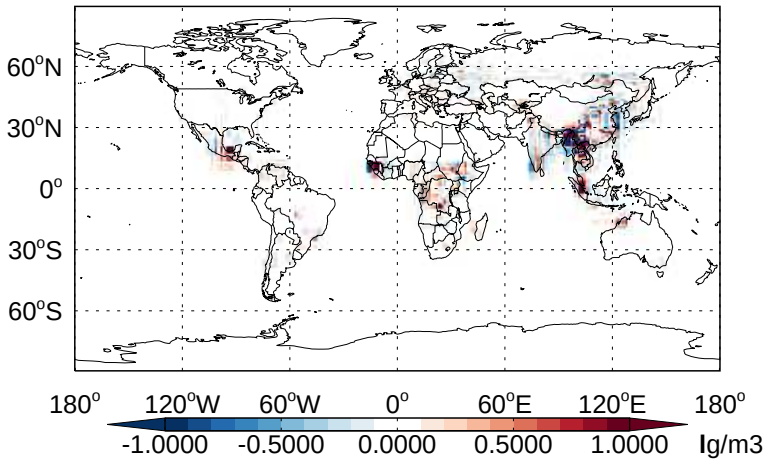
v11-02b-HP - v11-02a OCPI - Diff @ Surface for Apr
