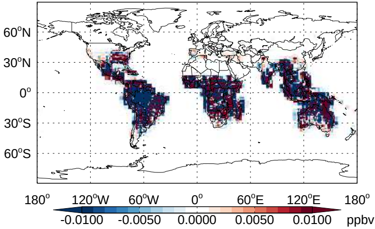
v11-02b-HP - v11-02a IEPOX - Diff @ Surface for Apr
