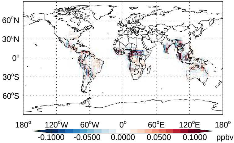
v11-02b-HP - v11-02a ISOG3 - Diff @ Surface for Apr
