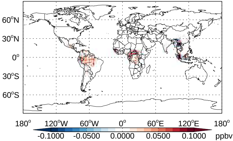
v11-02b-HP - v11-02a TSOA2 - Diff @ Surface for Apr
