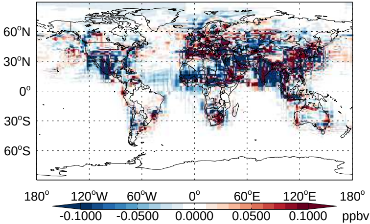
v11-02b-HP - v11-02a HNO 3 - Diff @ Surface for Apr
