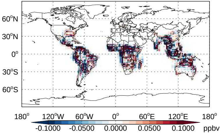
v11-02b-HP - v11-02a HAC - Diff @ Surface for Apr
