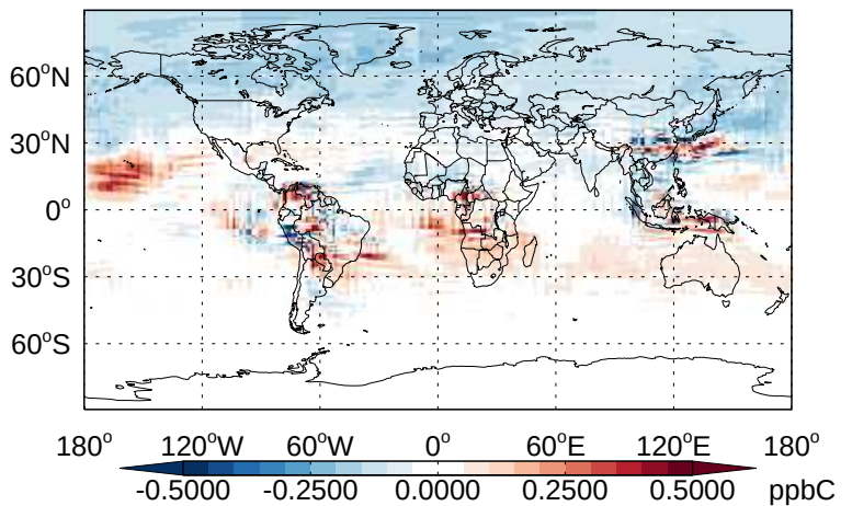
v11-02b-HP - v11-02a ACET- Diff @ 500 hPa for Apr
