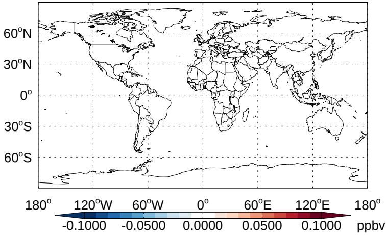
v11-02b-HP - v11-02a C1O0 - Diff @ Surface for Apr
