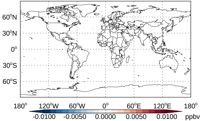
v11-02b-HP - v11-02a NO 3 - Diff @ 500 hPa for Apr
