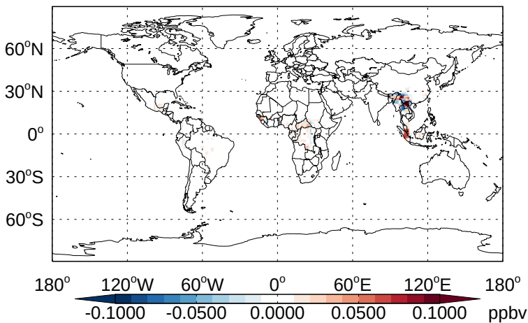
v11-02b-HP - v11-02a TSOA3 - Diff @ Surface for Apr
