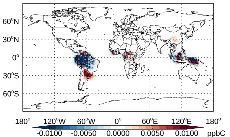
v11-02b-HP - v11-02a PRPE- Diff @ 500 hPa for Apr
