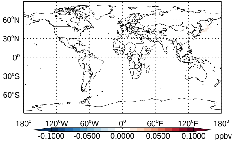
v11-02b-HP - v11-02a XYLE- Diff @ 500 hPa for Apr
