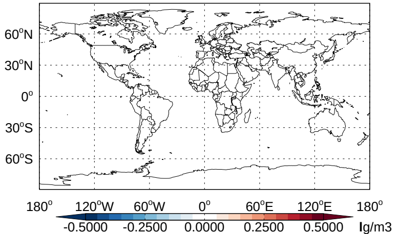
v11-02b-HP - v11-02a MSA- Diff @ 500 hPa for Apr
