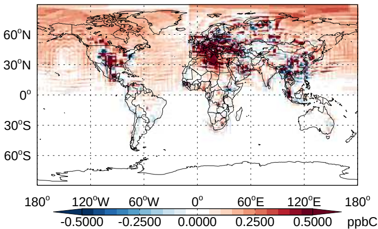
v11-02b-HP - v11-02a C2H6 - Diff @ Surface for Apr
