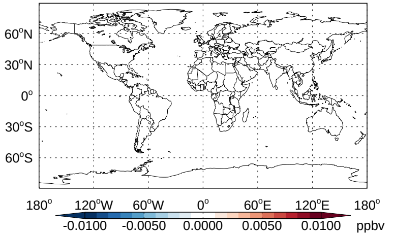
v11-02b-HP - v11-02a Br2- Diff @ 500 hPa for Apr
