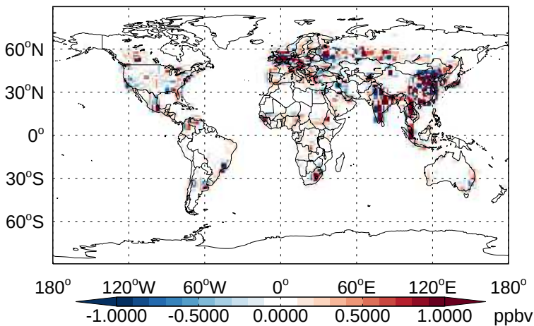
v11-02b-HP - v11-02a NO2 - Diff @ Surface for Apr
