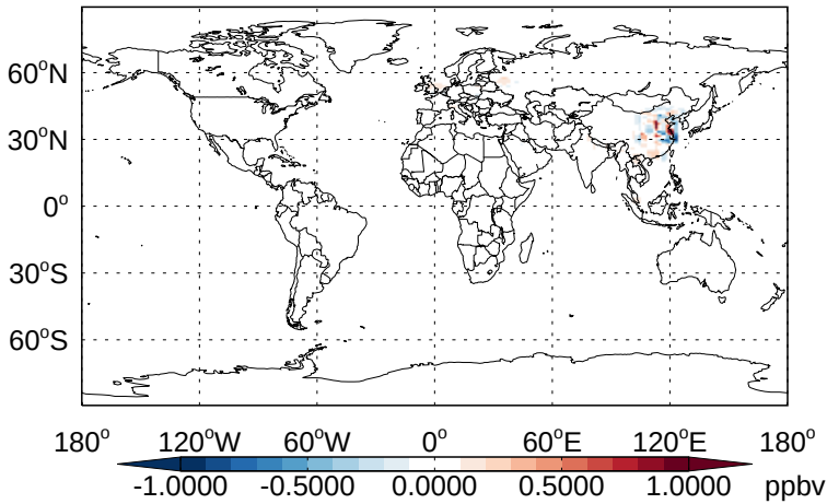
v11-02b-HP - v11-02a HNO 2 - Diff @ Surface for Apr
