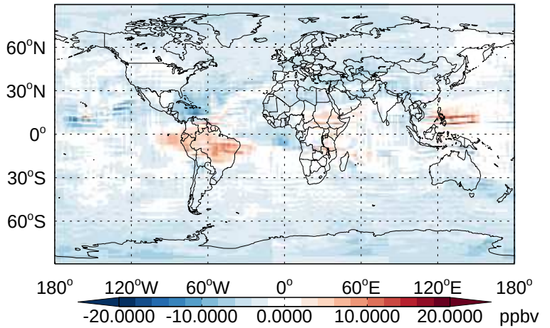
v11-02b-HP - v11-02a O3- Diff @ 500 hPa for Apr
