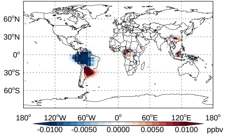
v11-02b-HP - v11-02a IEPOX- Diff @ 500 hPa for Apr
