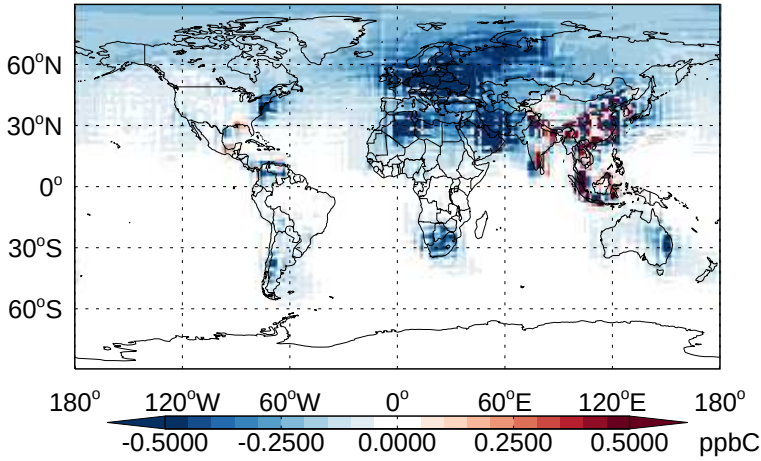
v11-02b-HP - v11-02a C3H8 - Diff @ Surface for Apr
