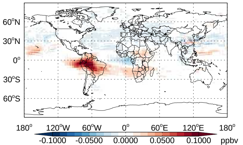
v11-02b-HP - v11-02a PAN- Diff @ 500 hPa for Apr
