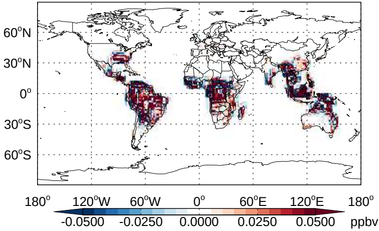
v11-02b-HP - v11-02a MVK - Diff @ Surface for Apr
