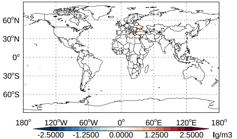
v11-02b-HP - v11-02a DST4- Diff @ 500 hPa for Apr
