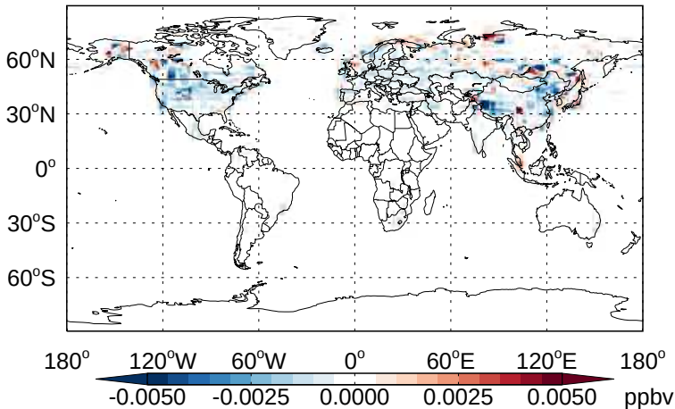
v11-02b-HP - v11-02a HNO4 - Diff @ Surface for Apr
