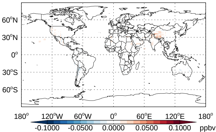
v11-02b-HP - v11-02a N 2 O - Diff @ Surface for Apr
