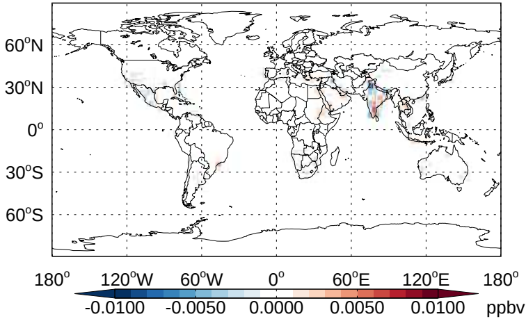
v11-02b-HP - v11-02a NO 3 - Diff @ Surface for Apr
