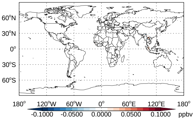
v11-02b-HP - v11-02a ISOA2 - Diff @ Surface for Apr
