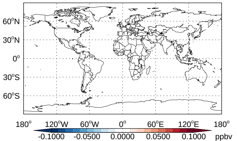
v11-02b-HP - v11-02a CH3Cl- Diff @ 500 hPa for Apr
