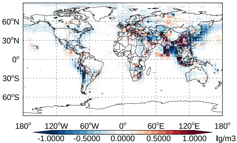
v11-02b-HP - v11-02a SO4 - Diff @ Surface for Apr
