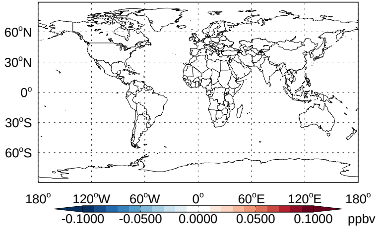
v11-02b-HP - v11-02a ClNO3- Diff @ 500 hPa for Apr
