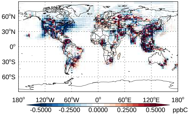
v11-02b-HP - v11-02a ALK4 - Diff @ Surface for Apr
