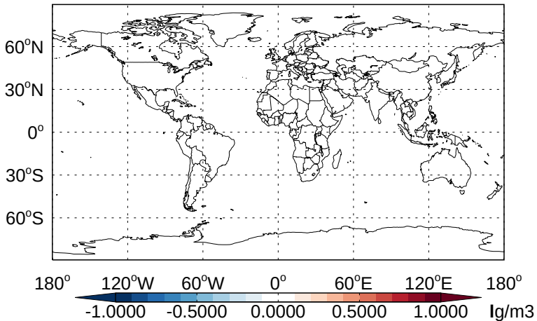
v11-02b-HP - v11-02a MSA - Diff @ Surface for Apr
