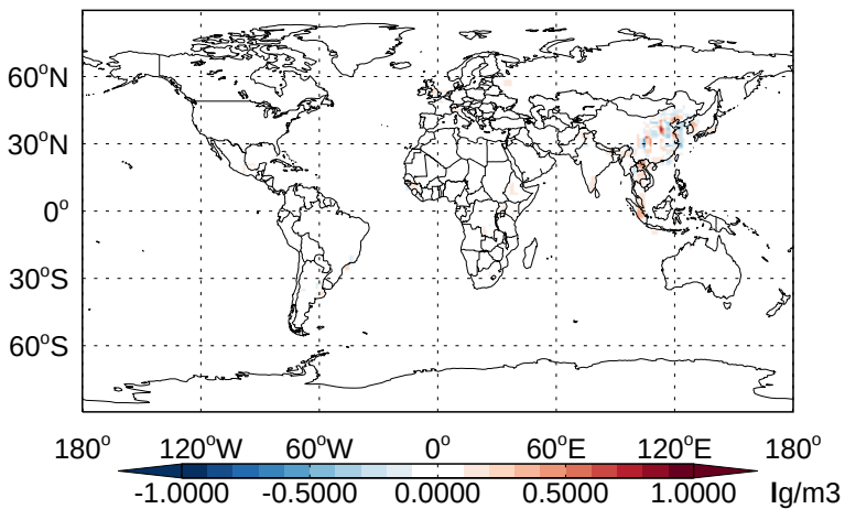
v11-02b-HP - v11-02a BCPO - Diff @ Surface for Apr
