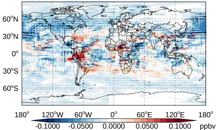
v11-02b-HP - v11-02a H 2 O 2 - Diff @ 500 hPa for Apr
