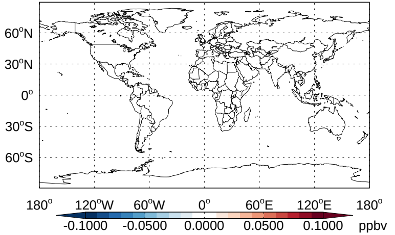
v11-02b-HP - v11-02a HOCl- Diff @ 500 hPa for Apr
