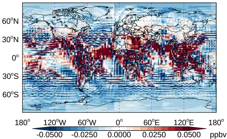
v11-02b-HP - v11-02a MP - Diff @ Surface for Apr
