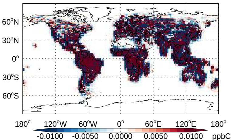
v11-02b-HP - v11-02a PRPE - Diff @ Surface for Apr
