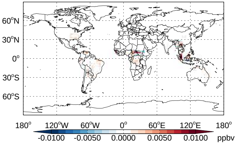
v11-02b-HP - v11-02a MACRN - Diff @ Surface for Apr
