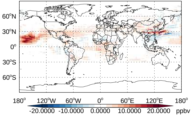
v11-02b-HP - v11-02a CO- Diff @ 500 hPa for Apr
