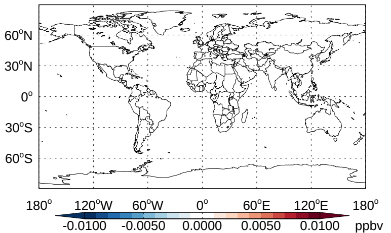
v11-02b-HP - v11-02a MOBA- Diff @ 500 hPa for Apr
