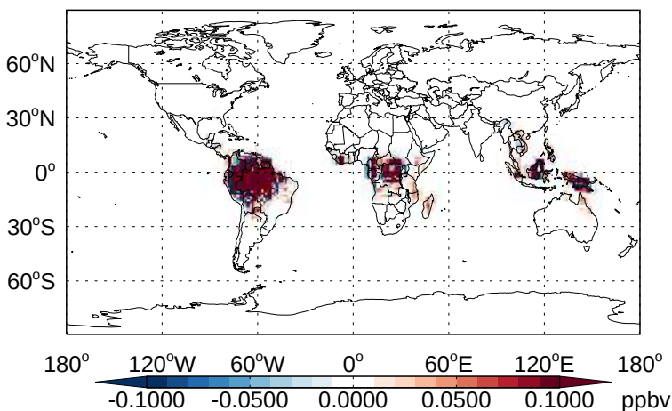
v11-02b-HP - v11-02a MTPA - Diff @ Surface for Apr
