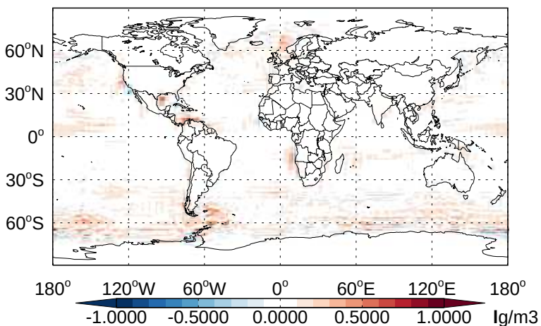
v11-02b-HP - v11-02a SALA - Diff @ Surface for Apr
