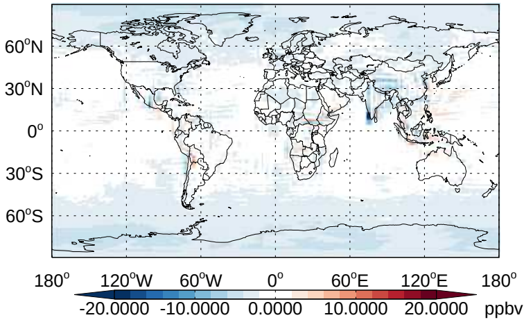
v11-02b-HP - v11-02a O3 - Diff @ Surface for Apr
