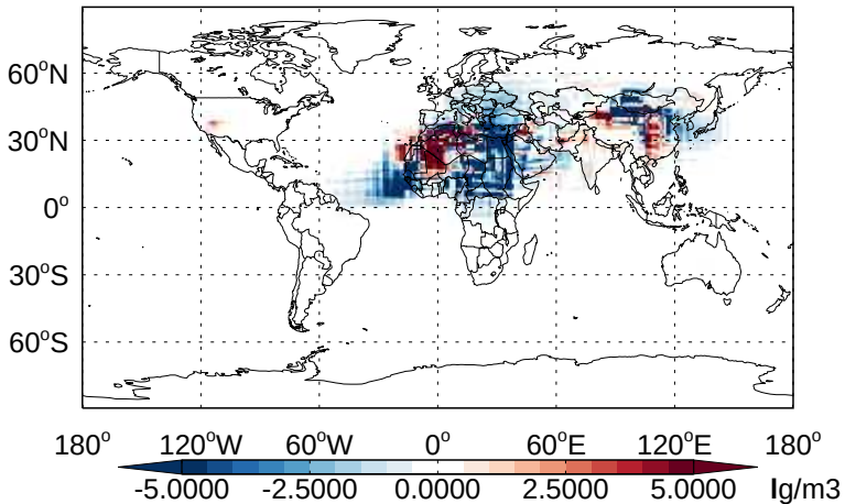
v11-02b-HP - v11-02a DST1 - Diff @ Surface for Apr
