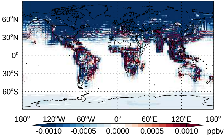
v11-02b-HP - v11-02a PPN - Diff @ Surface for Apr
