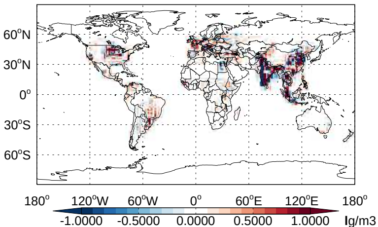
v11-02b-HP - v11-02a NH 3 - Diff @ Surface for Apr
