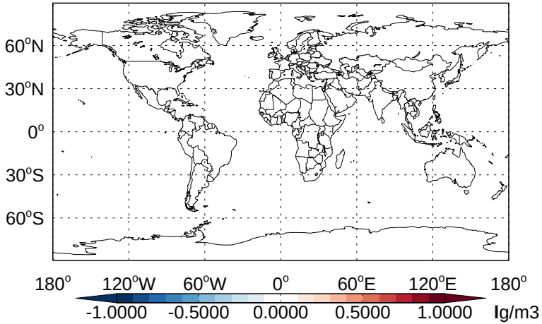
v11-02b-HP - v11-02a SO 4 s - Diff @ Surface for Apr
