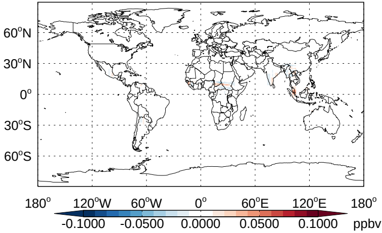
v11-02b-HP - v11-02a PROPNN - Diff @ Surface for Apr
