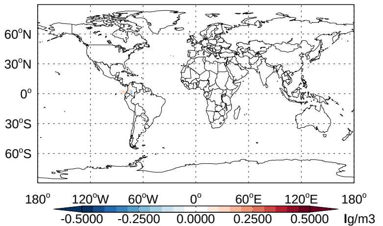
v11-02b-HP - v11-02a SO4- Diff @ 500 hPa for Apr
