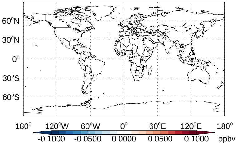
v11-02b-HP - v11-02a ASOA3 - Diff @ Surface for Apr
