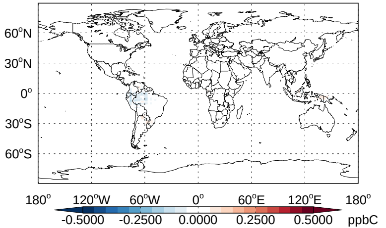
v11-02b-HP - v11-02a ALD2- Diff @ 500 hPa for Apr
