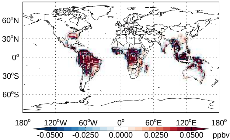
v11-02b-HP - v11-02a MACR - Diff @ Surface for Apr
