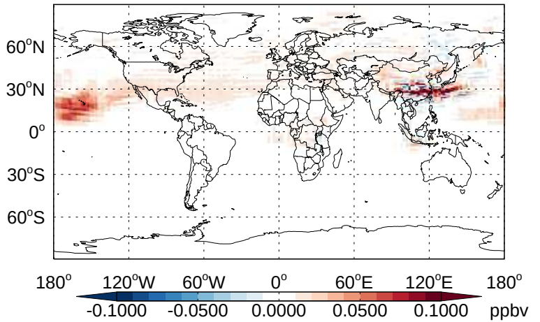
v11-02b-HP - v11-02a BENZ- Diff @ 500 hPa for Apr
