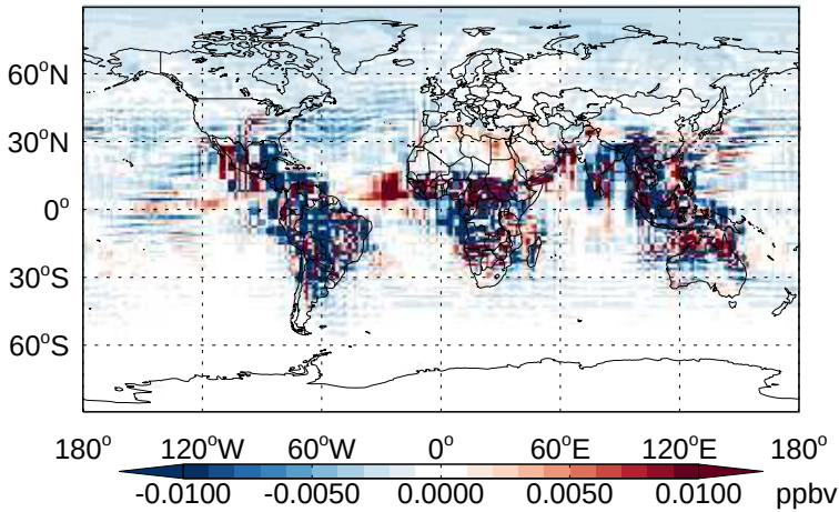
v11-02b-HP - v11-02a MAP - Diff @ Surface for Apr
