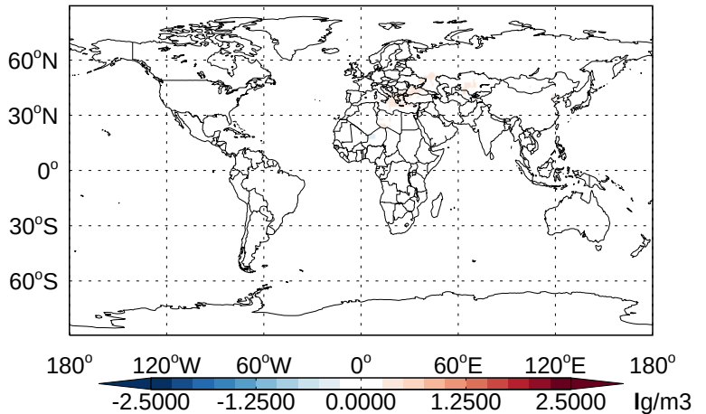
v11-02b-HP - v11-02a DST1- Diff @ 500 hPa for Apr
