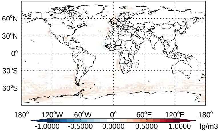
v11-02b-HP - v11-02a DMS - Diff @ Surface for Apr
