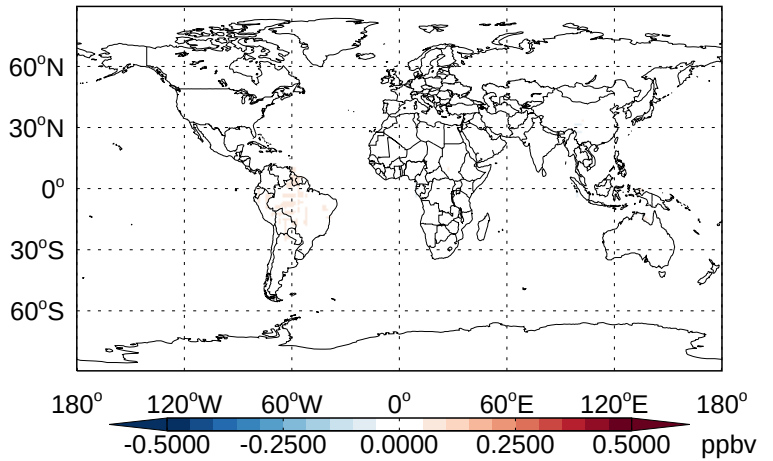
v11-02b-HP - v11-02a CH2O- Diff @ 500 hPa for Apr
