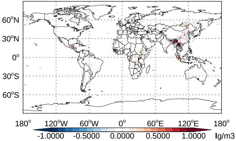
v11-02b-HP - v11-02a OCPO - Diff @ Surface for Apr
