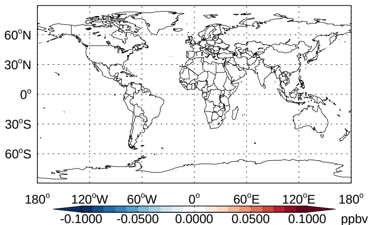
v11-02b-HP - v11-02a BrCl- Diff @ 500 hPa for Apr
