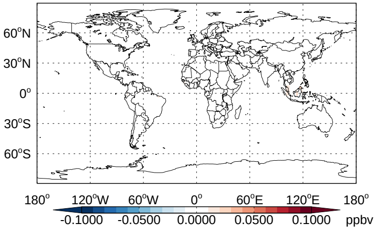
v11-02b-HP - v11-02a ISOPNB - Diff @ Surface for Apr
