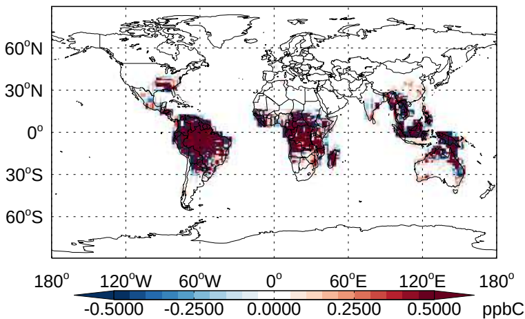
v11-02b-HP - v11-02a ISOP - Diff @ Surface for Apr
