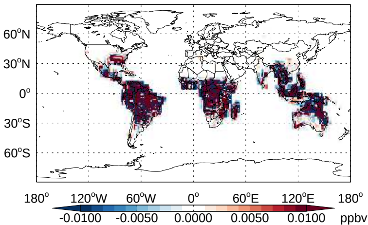
v11-02b-HP - v11-02a RIP - Diff @ Surface for Apr
