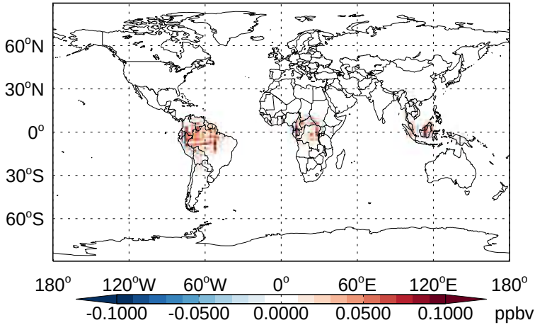
v11-02b-HP - v11-02a TSOA0 - Diff @ Surface for Apr
