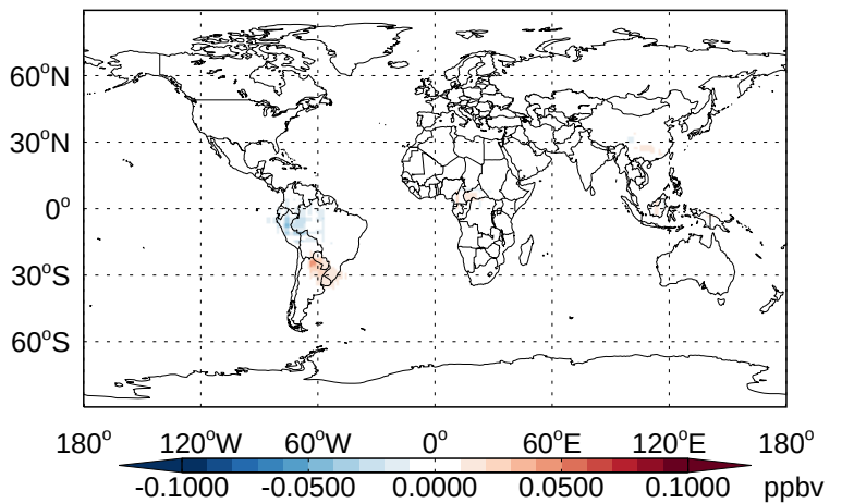
v11-02b-HP - v11-02a GLYC- Diff @ 500 hPa for Apr
