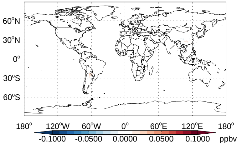
v11-02b-HP - v11-02a TSOG3- Diff @ 500 hPa for Apr
