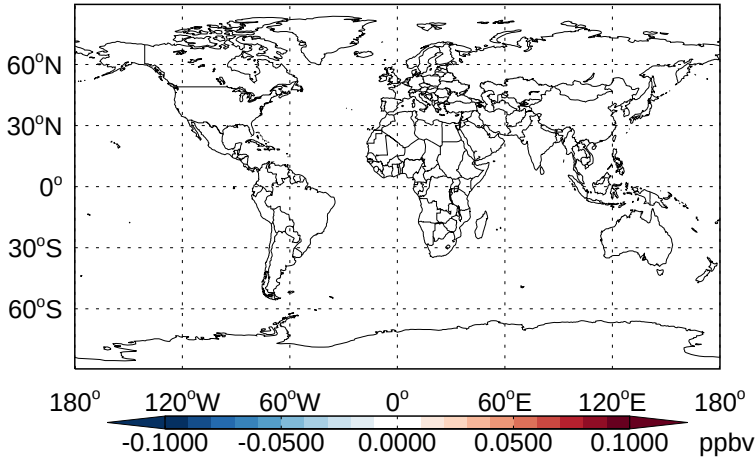
v11-02b-HP - v11-02a HCl - Diff @ Surface for Apr
