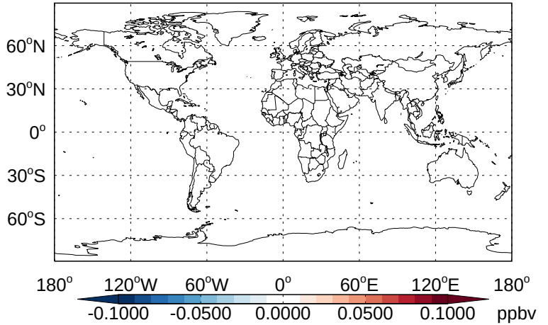
v11-02b-HP - v11-02a Cl 2 O 2 - Diff @ 500 hPa for Apr
