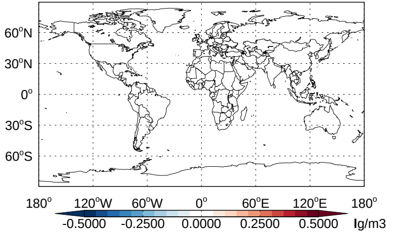
v11-02b-HP - v11-02a SO 4 s- Diff @ 500 hPa for Apr
