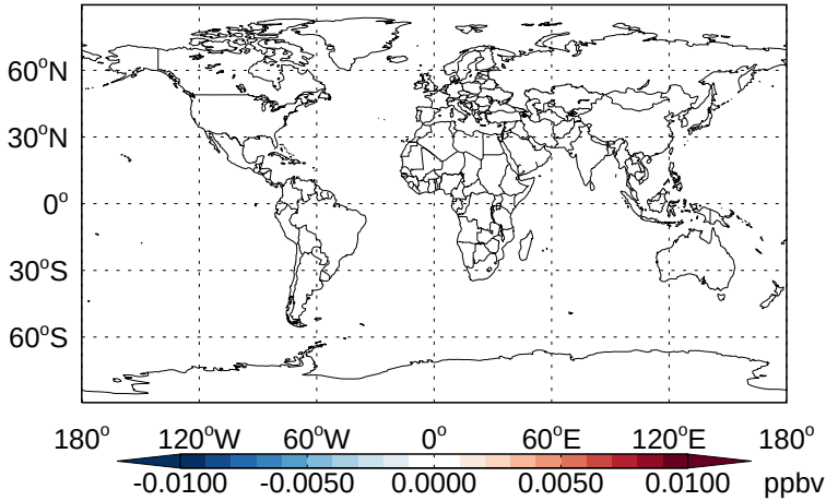
v11-02b-HP - v11-02a HOBr - Diff @ Surface for Apr
