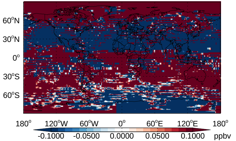
v11-02b-HP - v11-02a CH4- Diff @ 500 hPa for Apr
