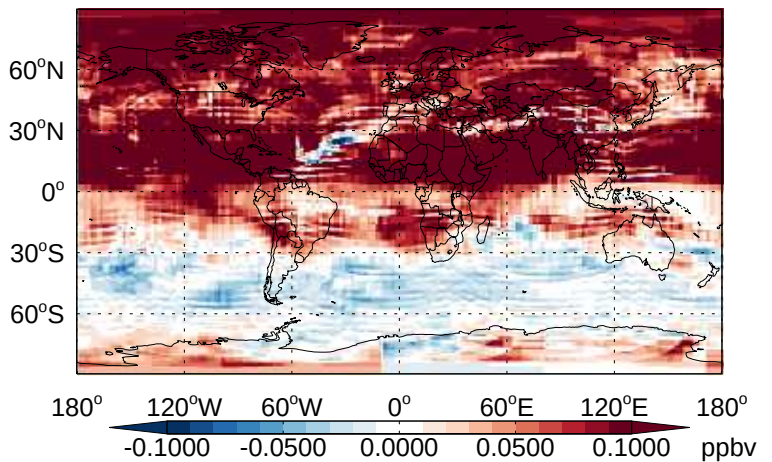
v11-02b-HP - v11-02a N 2 O- Diff @ 500 hPa for Apr
