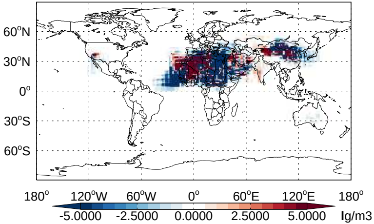
v11-02b-HP - v11-02a DST3 - Diff @ Surface for Apr
