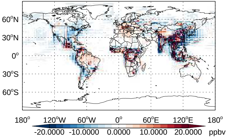
v11-02b-HP - v11-02a CO - Diff @ Surface for Apr
