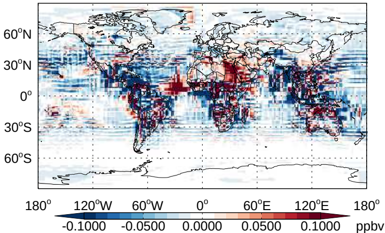
v11-02b-HP - v11-02a H 2 O 2 - Diff @ Surface for Apr
