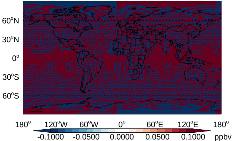
v11-02b-HP - v11-02a H 2 O - Diff @ Surface for Apr
