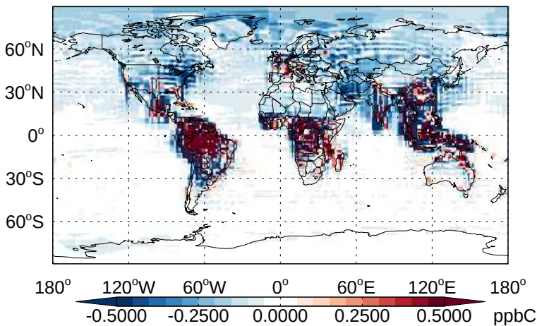
v11-02b-HP - v11-02a ACET - Diff @ Surface for Apr
