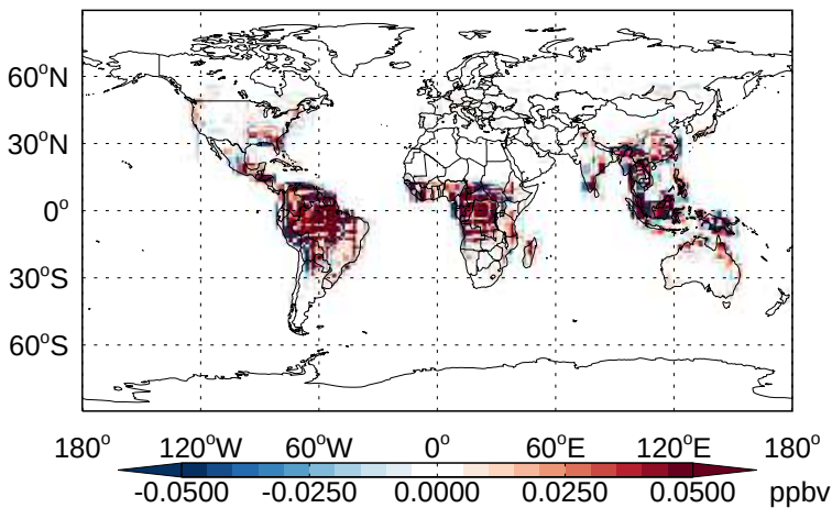
v11-02b-HP - v11-02a RCHO - Diff @ Surface for Apr
