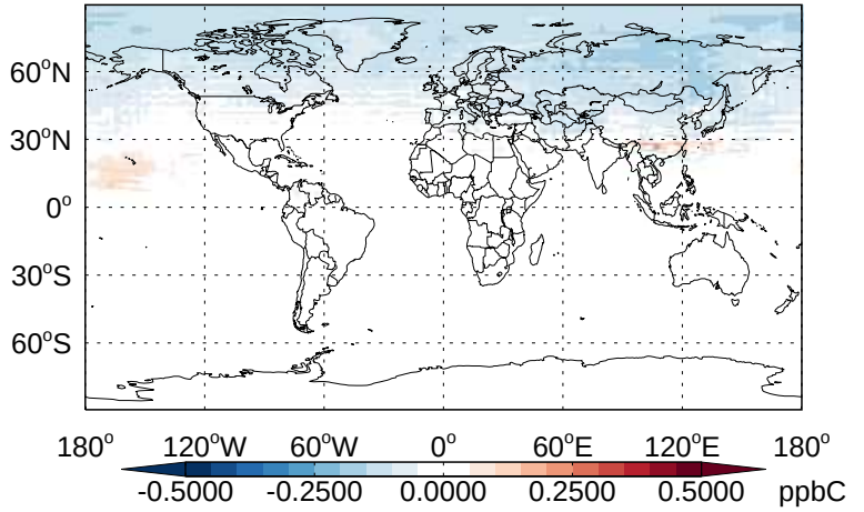
v11-02b-HP - v11-02a C3H8- Diff @ 500 hPa for Apr
