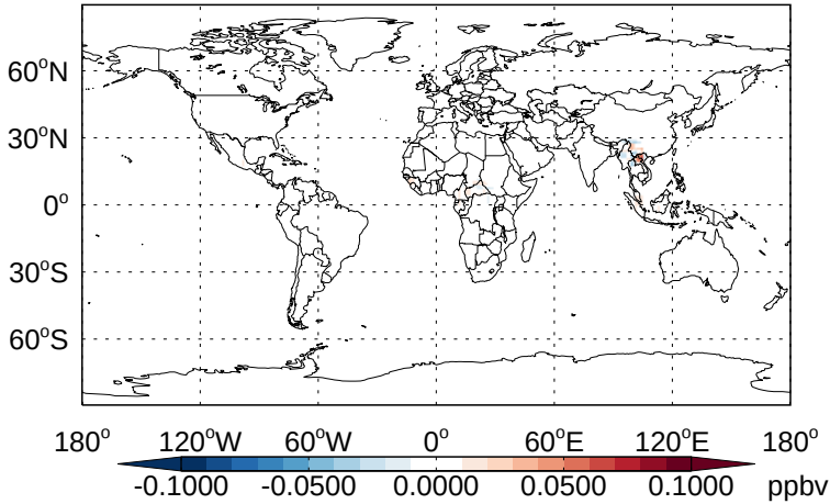
v11-02b-HP - v11-02a ISOA3 - Diff @ Surface for Apr
