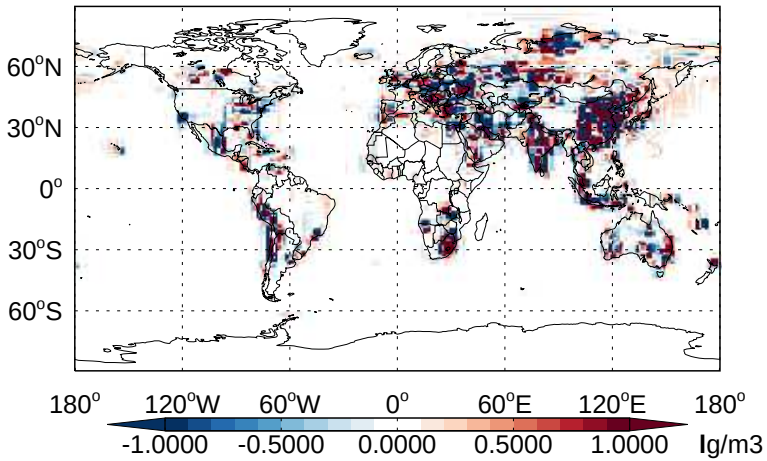
v11-02b-HP - v11-02a SO2 - Diff @ Surface for Apr
