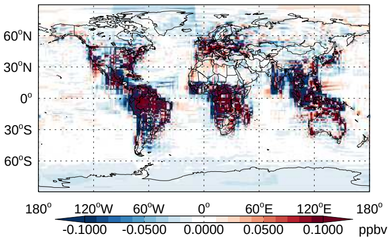
v11-02b-HP - v11-02a EOH - Diff @ Surface for Apr
