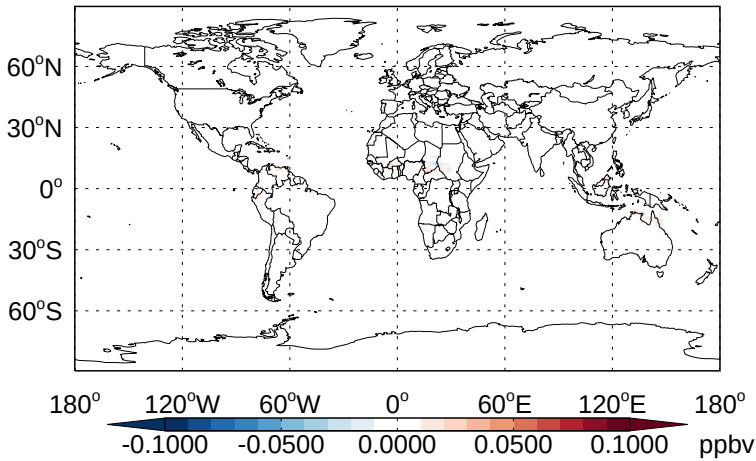
v11-02b-HP - v11-02a ISOG1 - Diff @ Surface for Apr
