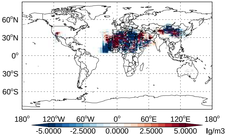
v11-02b-HP - v11-02a DST4 - Diff @ Surface for Apr
