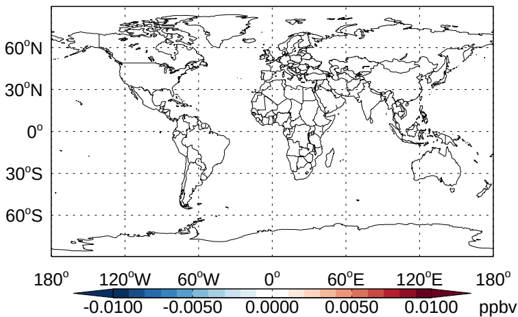
v11-02b-HP - v11-02a Br - Diff @ Surface for Apr
