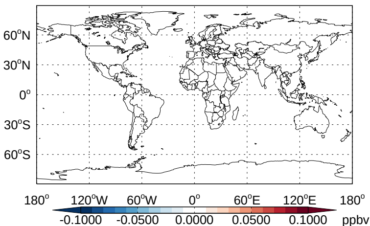
v11-02b-HP - v11-02a BrCl - Diff @ Surface for Apr
