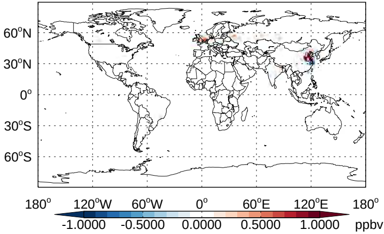
v11-02b-HP - v11-02a NO - Diff @ Surface for Apr
