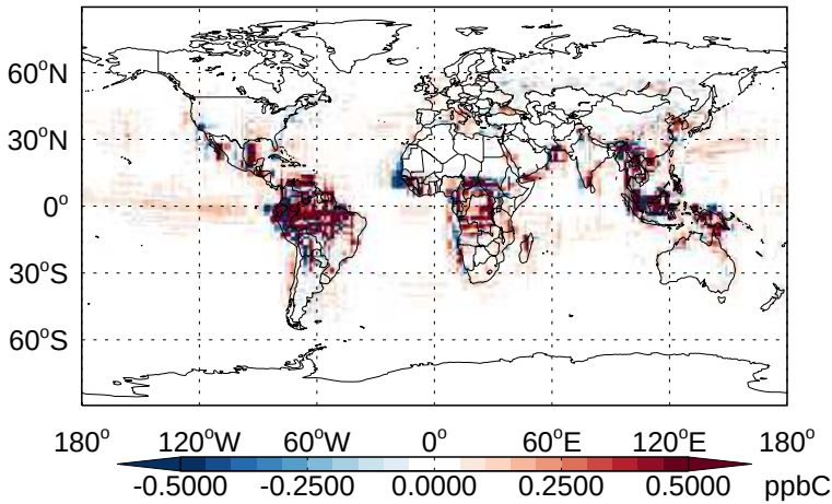
v11-02b-HP - v11-02a ALD2 - Diff @ Surface for Apr
