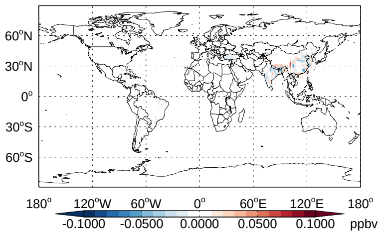
v11-02b-HP - v11-02a MGLY - Diff @ Surface for Apr
