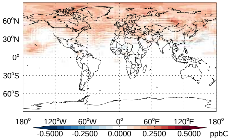
v11-02b-HP - v11-02a C2H6- Diff @ 500 hPa for Apr
