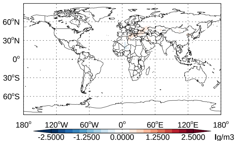
v11-02b-HP - v11-02a DST2- Diff @ 500 hPa for Apr
