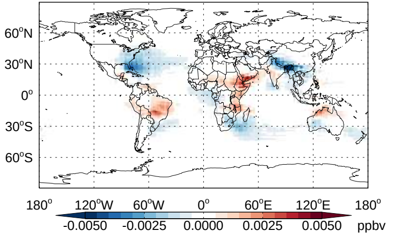
v11-02b-HP - v11-02a N2O5- Diff @ 500 hPa for Apr
