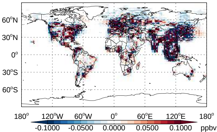
v11-02b-HP - v11-02a TOLU - Diff @ Surface for Apr
