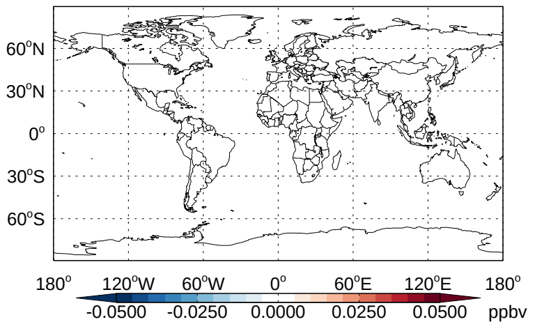
v11-02b-HP - v11-02a RCHO- Diff @ 500 hPa for Apr
