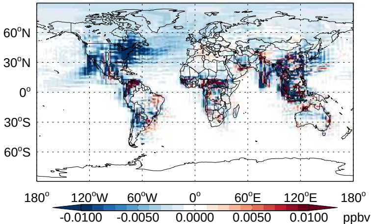
v11-02b-HP - v11-02a R4N2 - Diff @ Surface for Apr
