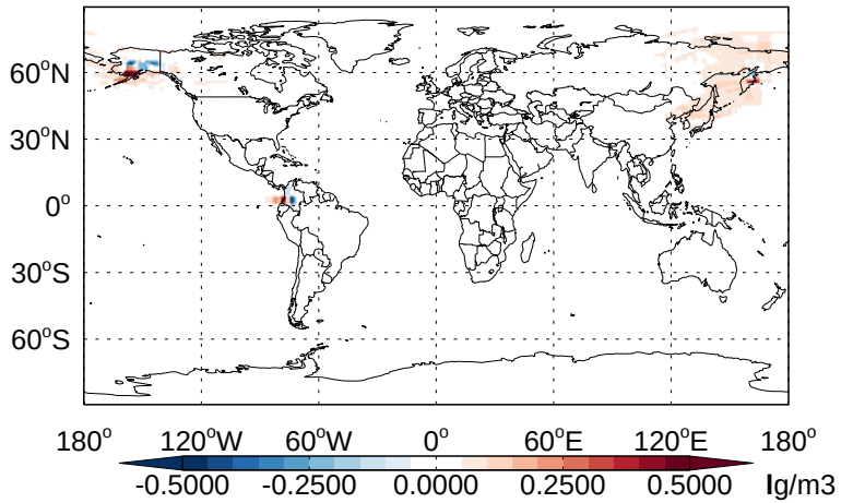
v11-02b-HP - v11-02a SO2- Diff @ 500 hPa for Apr
