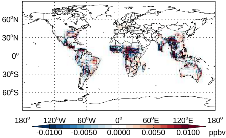
v11-02b-HP - v11-02a MVKN - Diff @ Surface for Apr
