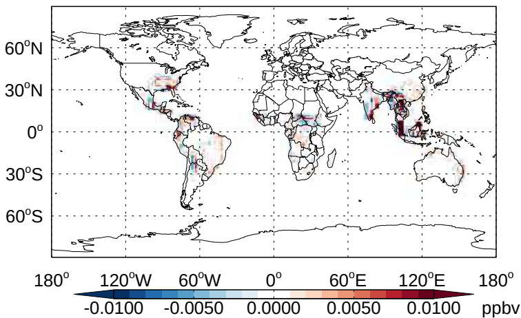
v11-02b-HP - v11-02a PMN - Diff @ Surface for Apr
