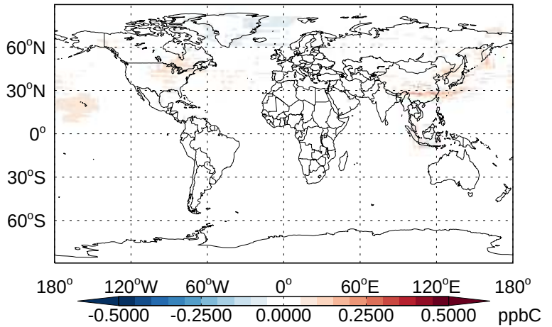
v11-02b-HP - v11-02a ALK4- Diff @ 500 hPa for Apr
