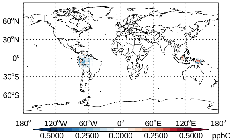
v11-02b-HP - v11-02a ISOP- Diff @ 500 hPa for Apr
