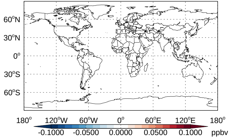
v11-02b-HP - v11-02a TSOA1- Diff @ 500 hPa for Apr
