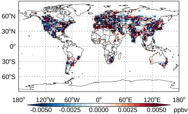
v11-02b-HP - v11-02a N2O5 - Diff @ Surface for Apr
