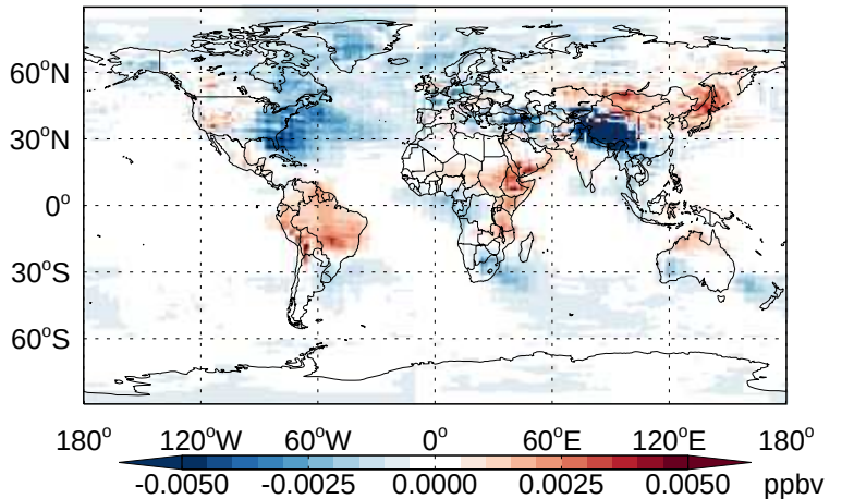
v11-02b-HP - v11-02a HNO4- Diff @ 500 hPa for Apr
