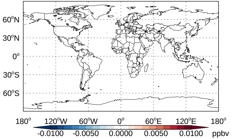
v11-02b-HP - v11-02a BrO- Diff @ 500 hPa for Apr
