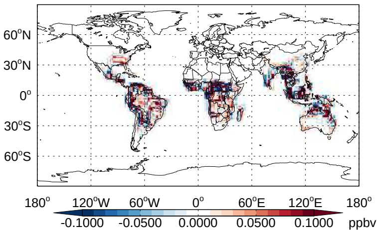
v11-02b-HP - v11-02a GLYC - Diff @ Surface for Apr
