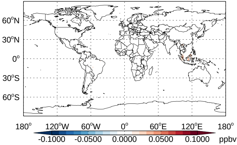
v11-02b-HP - v11-02a ISOPND - Diff @ Surface for Apr
