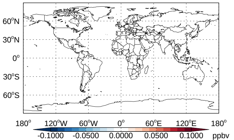
v11-02b-HP - v11-02a CFC114- Diff @ 500 hPa for Apr
