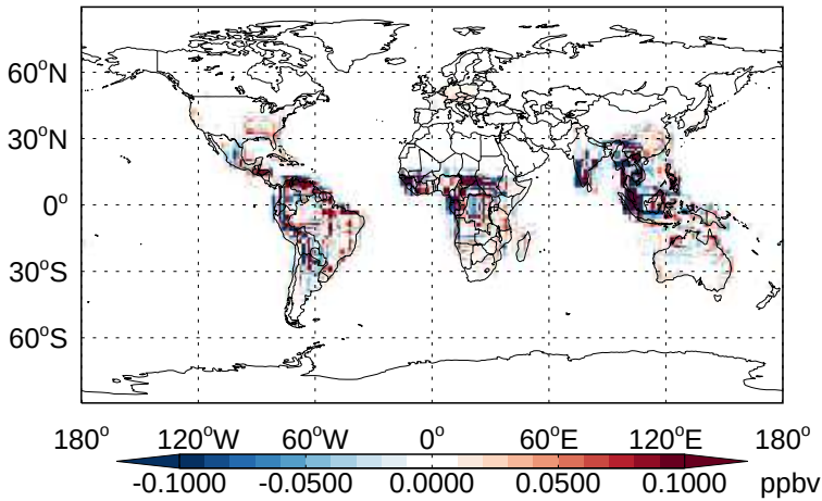
v11-02b-HP - v11-02a TSOG3 - Diff @ Surface for Apr
