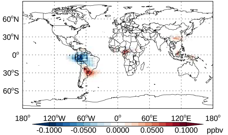
v11-02b-HP - v11-02a HAC- Diff @ 500 hPa for Apr
