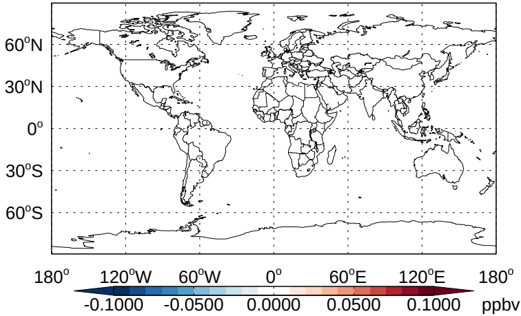
v11-02b-HP - v11-02a ASOA2 - Diff @ Surface for Apr
