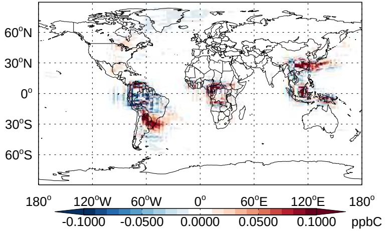
v11-02b-HP - v11-02a MEK- Diff @ 500 hPa for Apr
