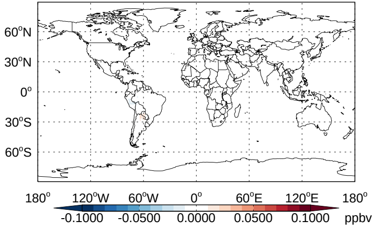
v11-02b-HP - v11-02a ISOG3- Diff @ 500 hPa for Apr
