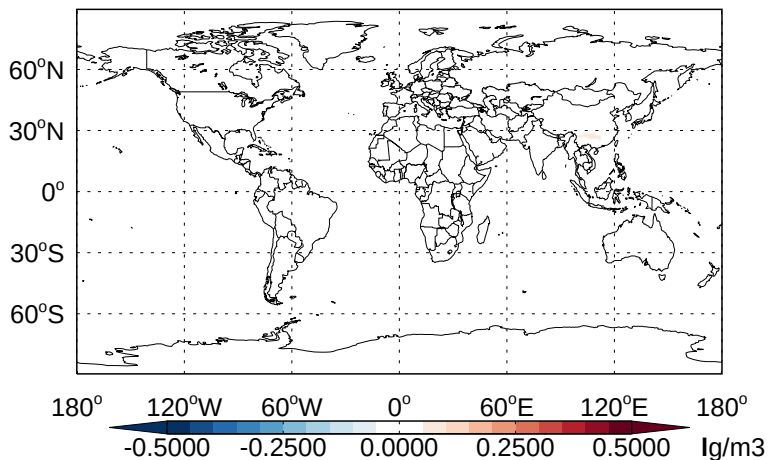
v11-02b-HP - v11-02a NH 3 - Diff @ 500 hPa for Apr
