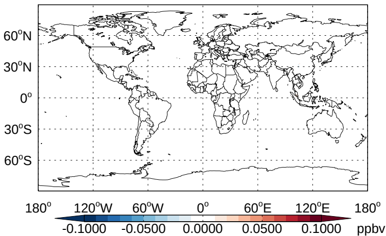
v11-02b-HP - v11-02a ASOA1 - Diff @ Surface for Apr
