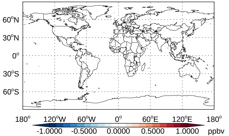
v11-02b-HP - v11-02a HNO 2 - Diff @ 500 hPa for Apr
