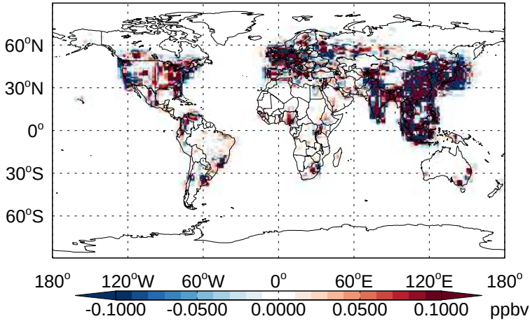
v11-02b-HP - v11-02a XYLE - Diff @ Surface for Apr
