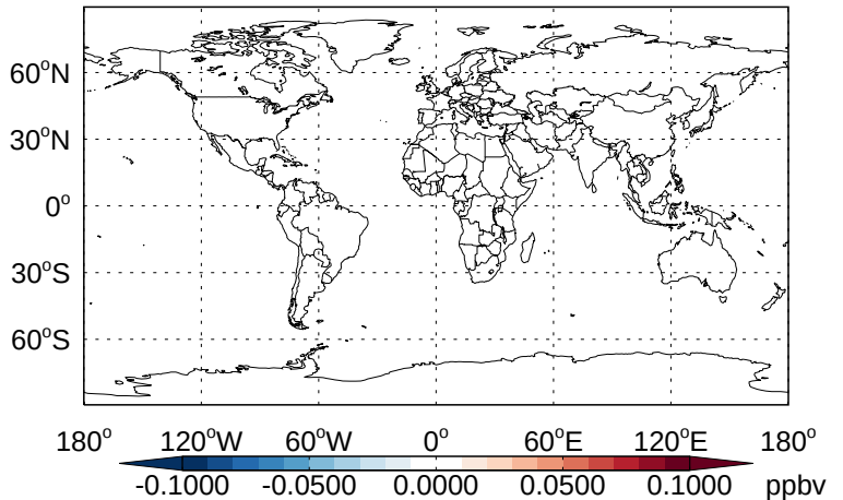
v11-02b-HP - v11-02a CCl4- Diff @ 500 hPa for Apr
