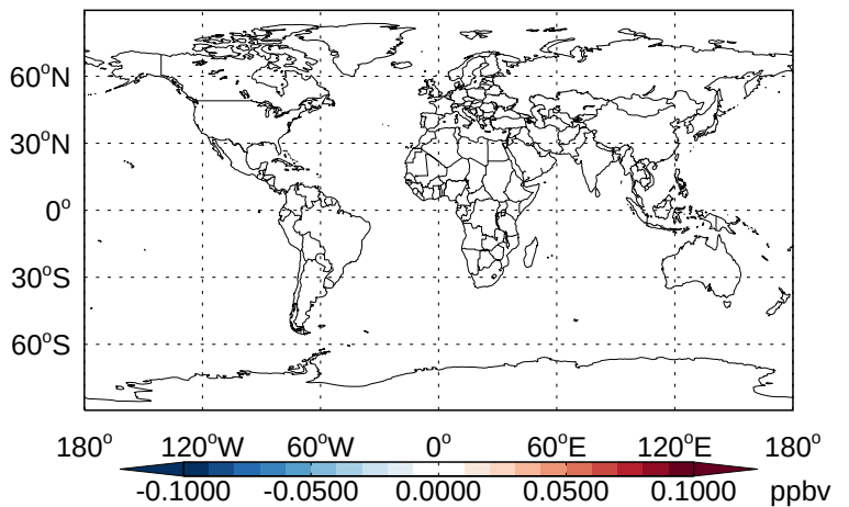
v11-02b-HP - v11-02a H1301- Diff @ 500 hPa for Apr
