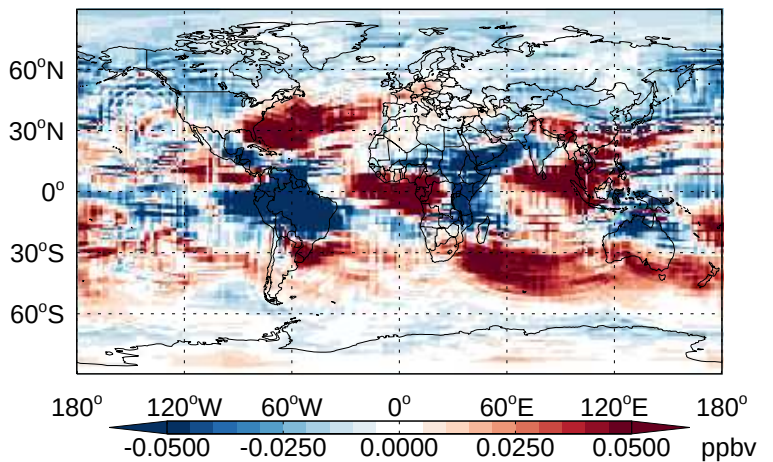
v11-02b-HP - v11-02a MP- Diff @ 500 hPa for Apr
