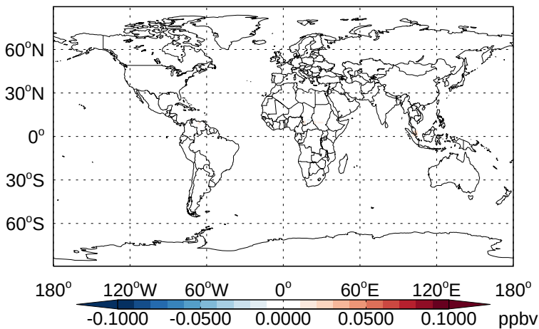
v11-02b-HP - v11-02a ISOG2 - Diff @ Surface for Apr
