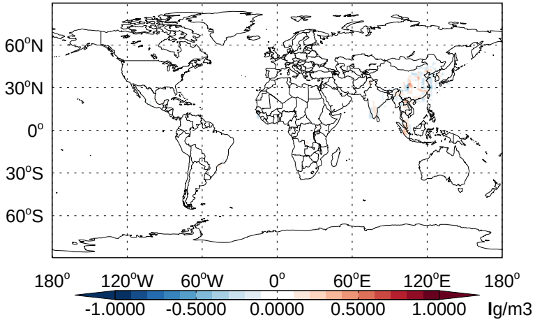
v11-02b-HP - v11-02a BCPI - Diff @ Surface for Apr
