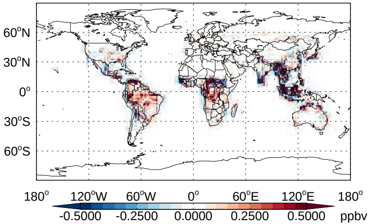
v11-02b-HP - v11-02a CH2O - Diff @ Surface for Apr
