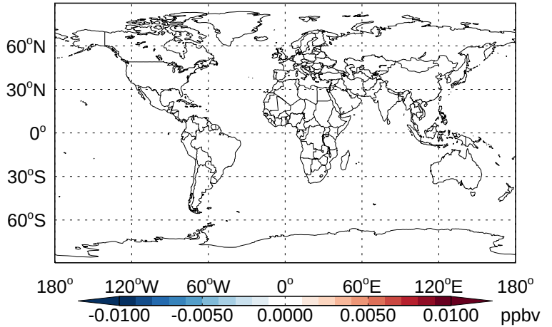
v11-02b-HP - v11-02a HOBr- Diff @ 500 hPa for Apr
