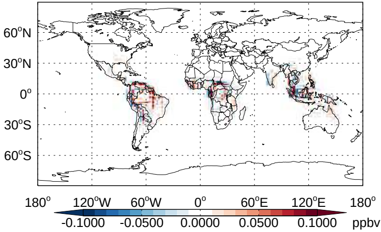
v11-02b-HP - v11-02a TSOG2 - Diff @ Surface for Apr
