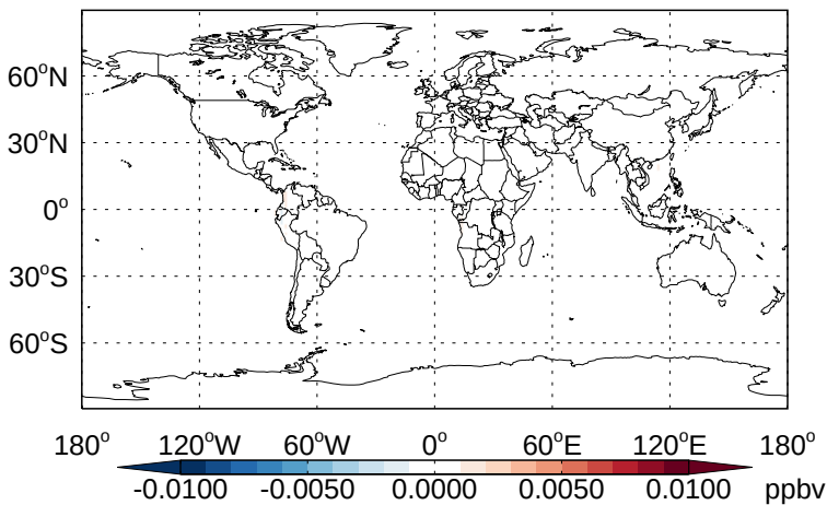
v11-02b-HP - v11-02a CHBr 3 - Diff @ Surface for Apr
