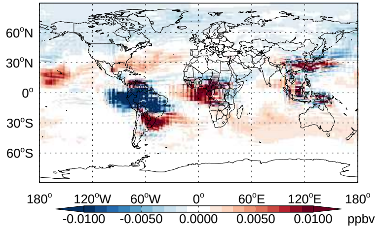
v11-02b-HP - v11-02a MAP- Diff @ 500 hPa for Apr
