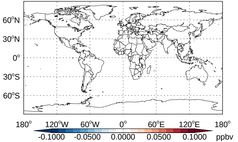
v11-02b-HP - v11-02a HCl- Diff @ 500 hPa for Apr
