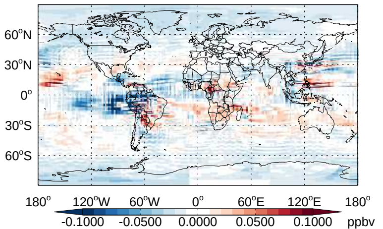
v11-02b-HP - v11-02a EOH- Diff @ 500 hPa for Apr
