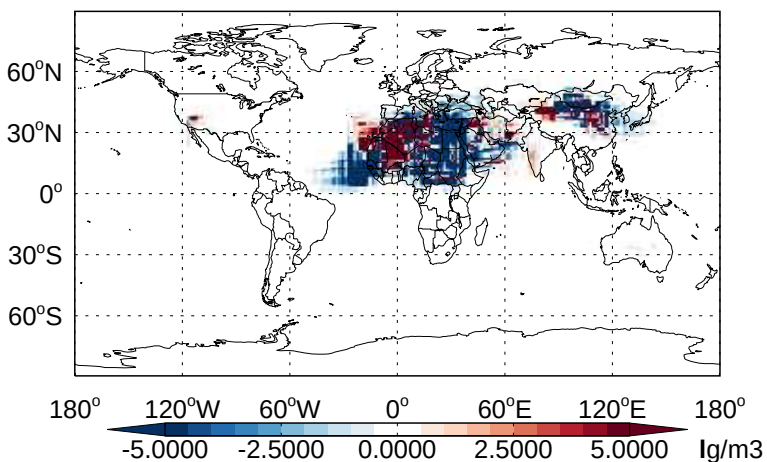
v11-02b-HP - v11-02a DST2 - Diff @ Surface for Apr
