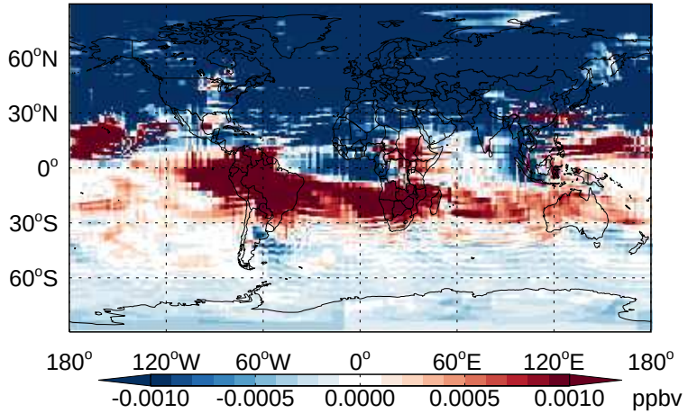
v11-02b-HP - v11-02a PPN- Diff @ 500 hPa for Apr
