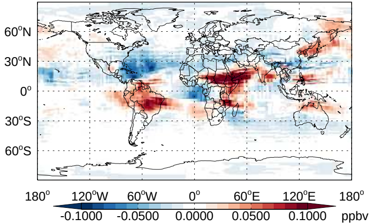
v11-02b-HP - v11-02a HNO 3 - Diff @ 500 hPa for Apr
