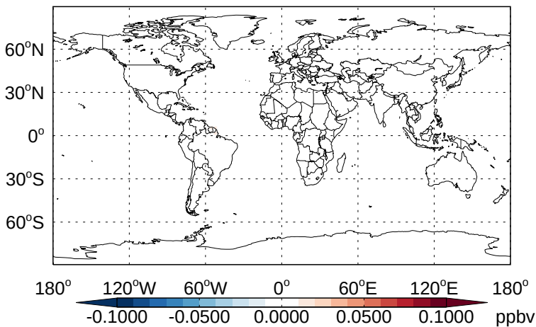
v11-02b-HP - v11-02a TSOG1 - Diff @ Surface for Apr
