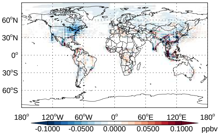
v11-02b-HP - v11-02a PAN - Diff @ Surface for Apr
