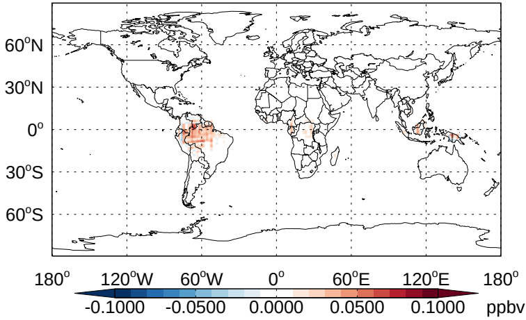
v11-02b-HP - v11-02a LIMO - Diff @ Surface for Apr
