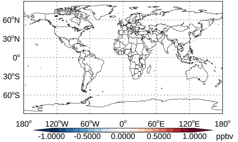
v11-02b-HP - v11-02a NO- Diff @ 500 hPa for Apr
