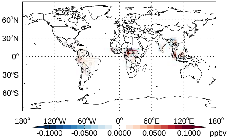
v11-02b-HP - v11-02a ISOA1 - Diff @ Surface for Apr
