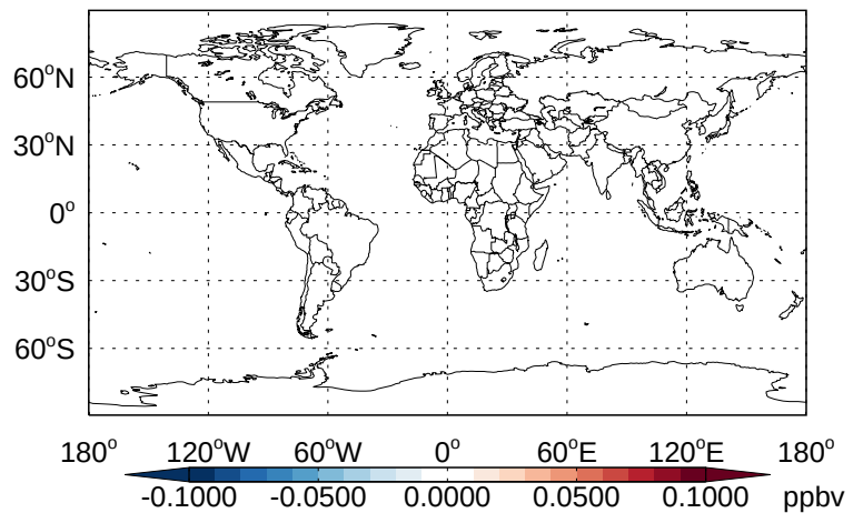
v11-02b-HP - v11-02a TSOA3- Diff @ 500 hPa for Apr
