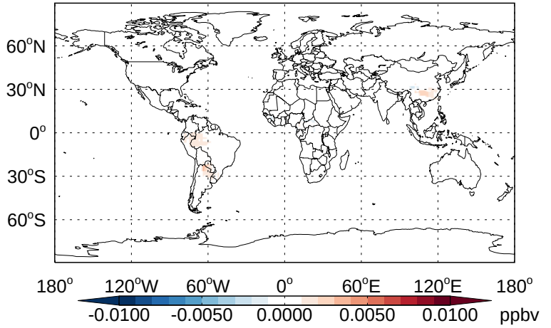
v11-02b-HP - v11-02a MVKN- Diff @ 500 hPa for Apr
