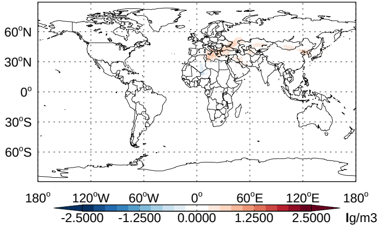
v11-02b-HP - v11-02a DST3- Diff @ 500 hPa for Apr
