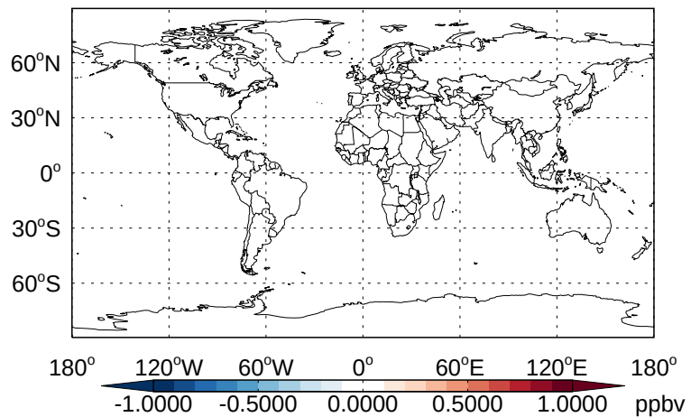
v11-02b-HP - v11-02a NO2- Diff @ 500 hPa for Apr
