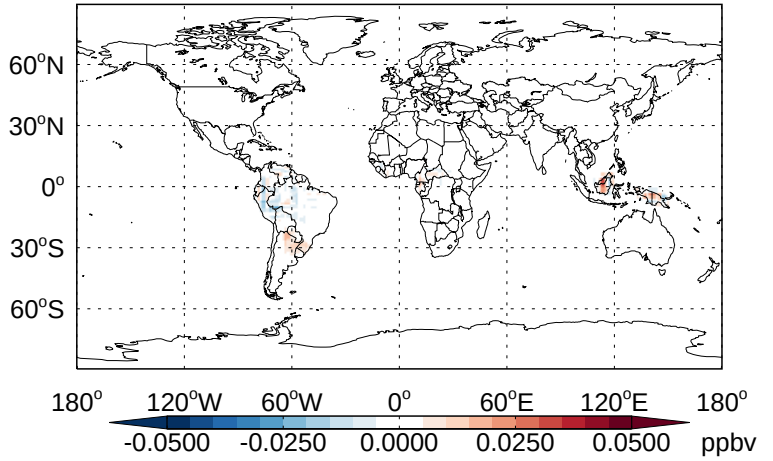
v11-02b-HP - v11-02a MVK- Diff @ 500 hPa for Apr
