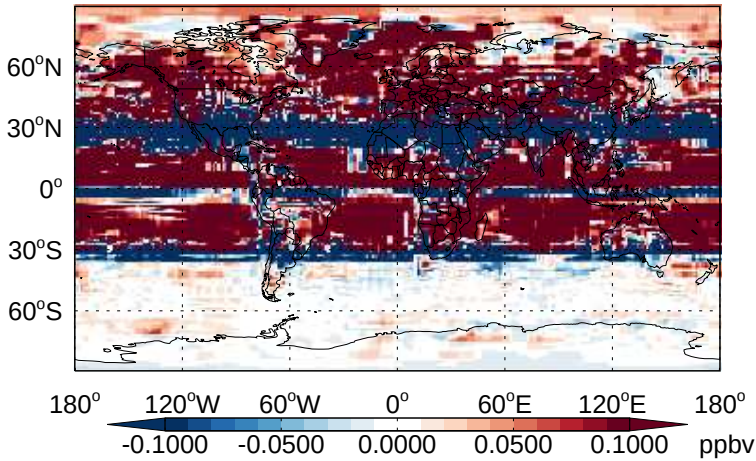
v11-02b-HP - v11-02a CH4 - Diff @ Surface for Apr
