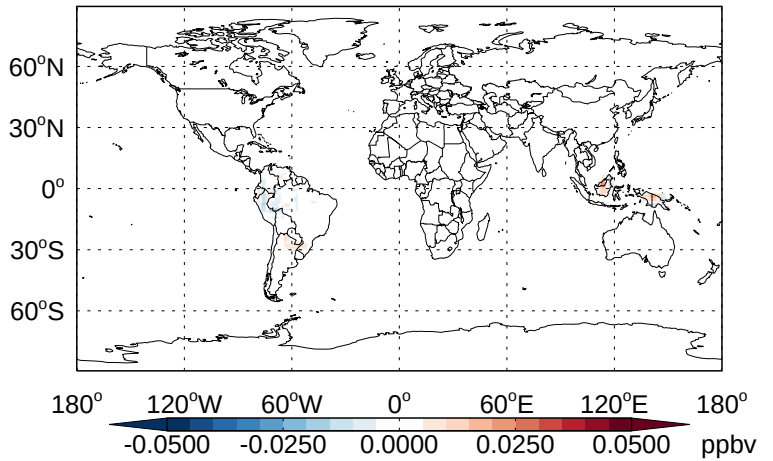
v11-02b-HP - v11-02a MACR- Diff @ 500 hPa for Apr
