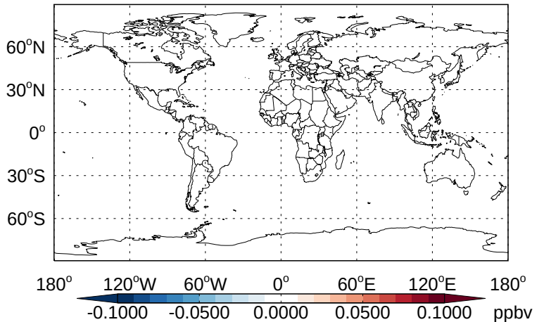
v11-02b-HP - v11-02a ASOA3- Diff @ 500 hPa for Apr
