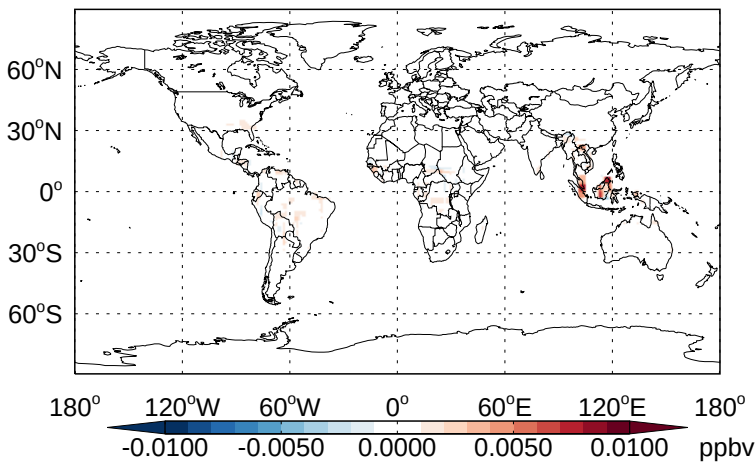
v11-02b-HP - v11-02a MOBA - Diff @ Surface for Apr
