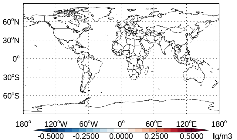
v11-02b-HP - v11-02a SALA- Diff @ 500 hPa for Apr
