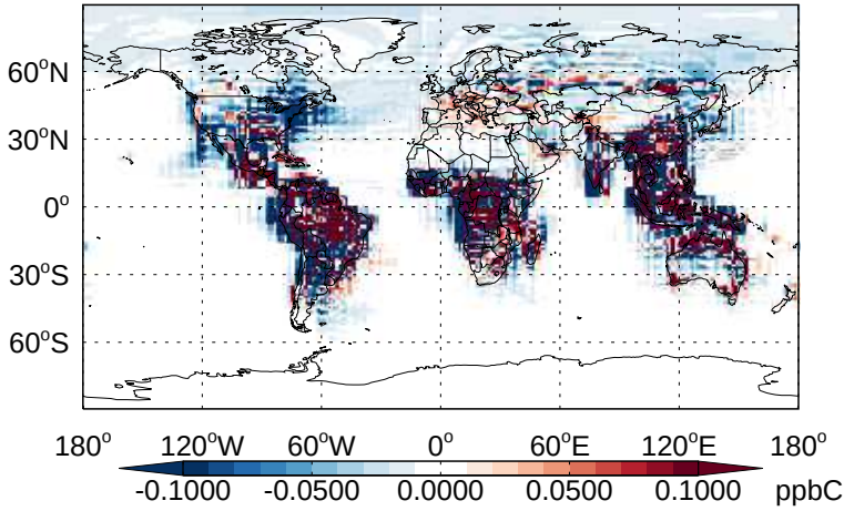
v11-02b-HP - v11-02a MEK - Diff @ Surface for Apr
