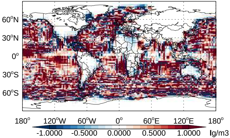
v11-02b-HP - v11-02a SALC - Diff @ Surface for Apr
