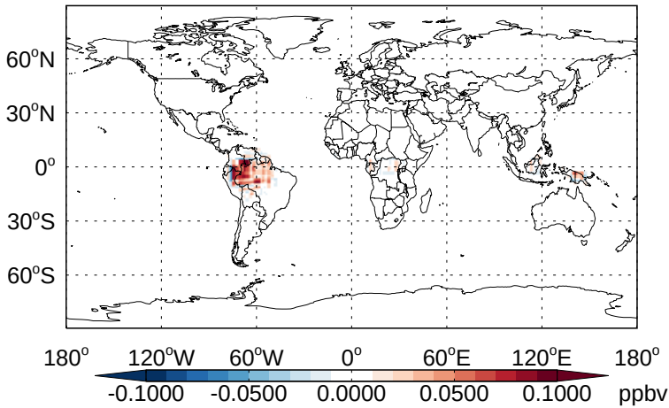
v11-02b-HP - v11-02a MTPO - Diff @ Surface for Apr
