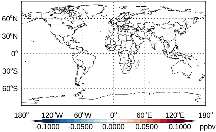
v11-02b-HP - v11-02a ASOG3 - Diff @ Surface for Apr
