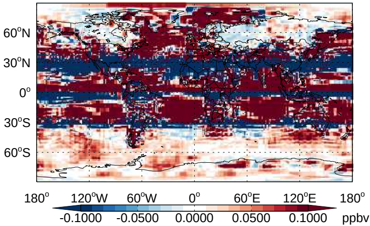
v11-02b-HP - v11-02a CH4 - Diff @ Surface for Jan
