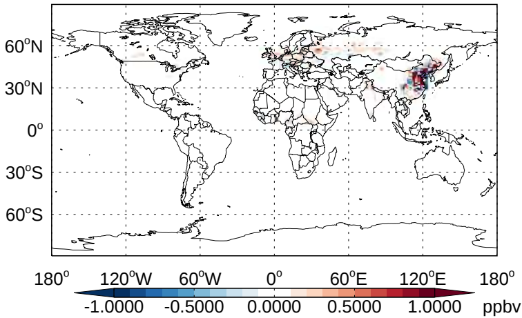
v11-02b-HP - v11-02a HNO 2 - Diff @ Surface for Jan
