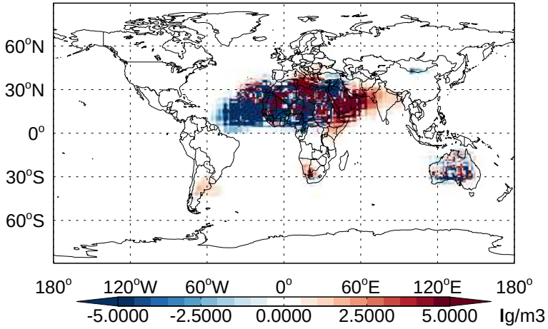
v11-02b-HP - v11-02a DST3 - Diff @ Surface for Jan
