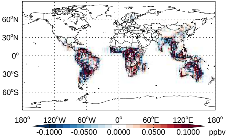
v11-02b-HP - v11-02a HAC - Diff @ Surface for Jan
