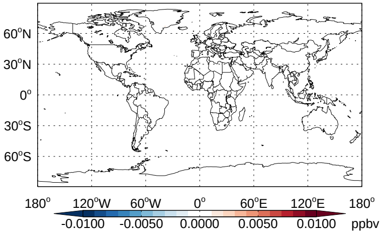
v11-02b-HP - v11-02a Br2 - Diff @ Surface for Jan
