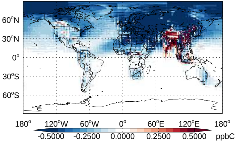
v11-02b-HP - v11-02a C3H8 - Diff @ Surface for Jan
