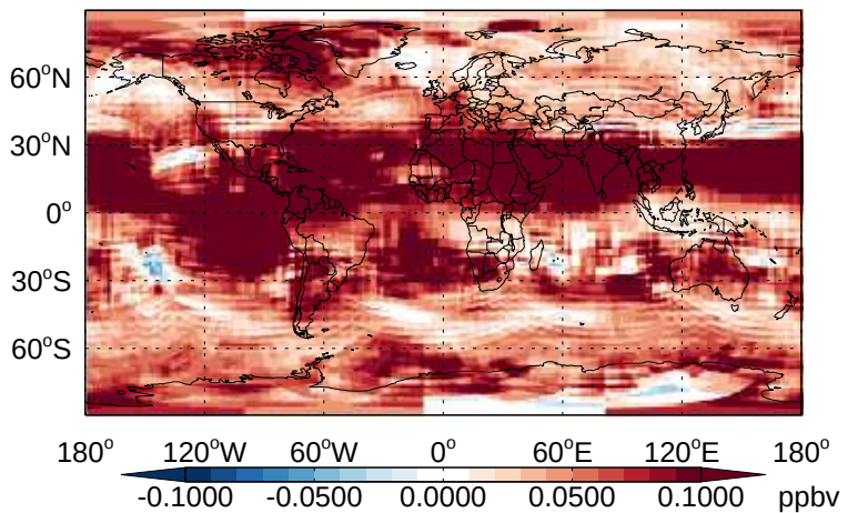
v11-02b-HP - v11-02a N 2 O- Diff @ 500 hPa for Jan
