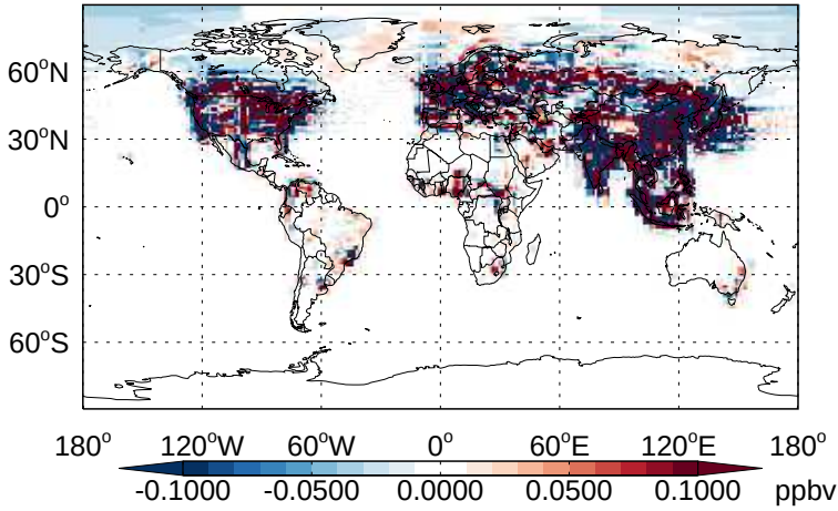
v11-02b-HP - v11-02a XYLE - Diff @ Surface for Jan
