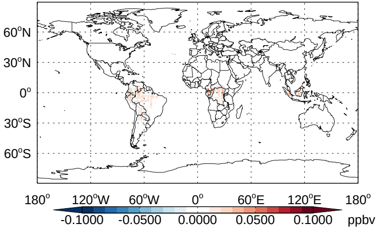
v11-02b-HP - v11-02a TSOA1 - Diff @ Surface for Jan
