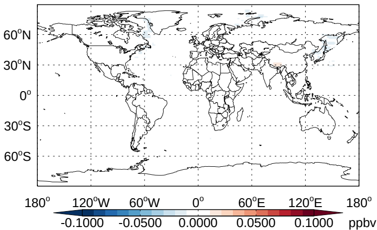
v11-02b-HP - v11-02a N 2 O - Diff @ Surface for Jan
