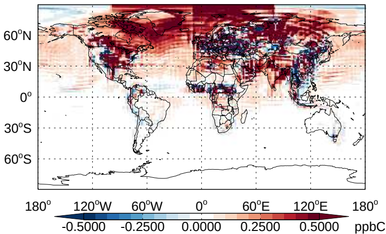
v11-02b-HP - v11-02a C2H6 - Diff @ Surface for Jan
