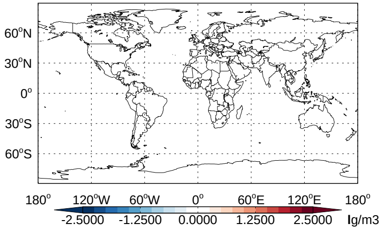
v11-02b-HP - v11-02a DST1- Diff @ 500 hPa for Jan
