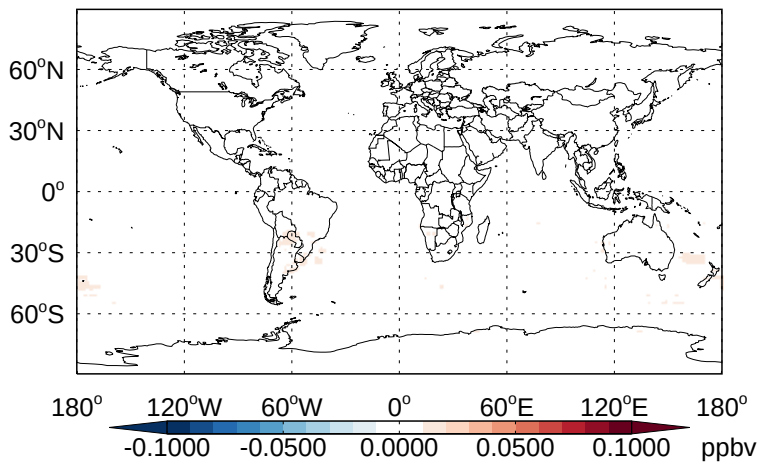
v11-02b-HP - v11-02a CH3Cl- Diff @ 500 hPa for Jan
