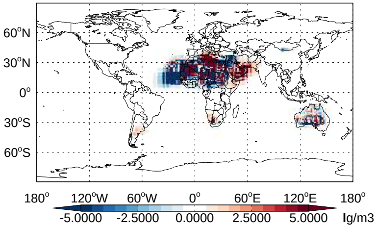
v11-02b-HP - v11-02a DST4 - Diff @ Surface for Jan
