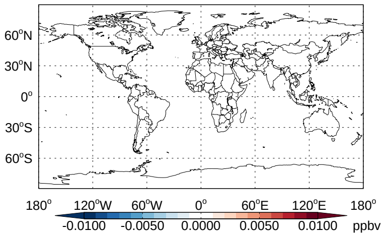
v11-02b-HP - v11-02a HBr- Diff @ 500 hPa for Jan
