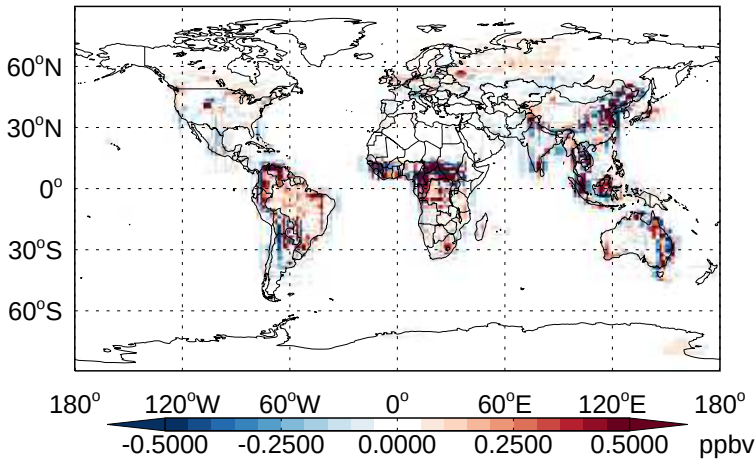
v11-02b-HP - v11-02a CH2O - Diff @ Surface for Jan
