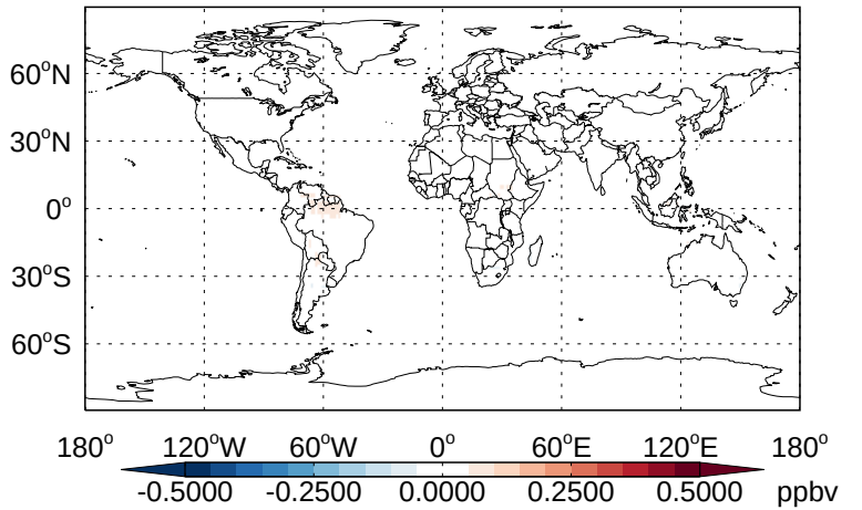
v11-02b-HP - v11-02a CH2O- Diff @ 500 hPa for Jan
