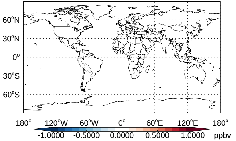
v11-02b-HP - v11-02a NO- Diff @ 500 hPa for Jan
