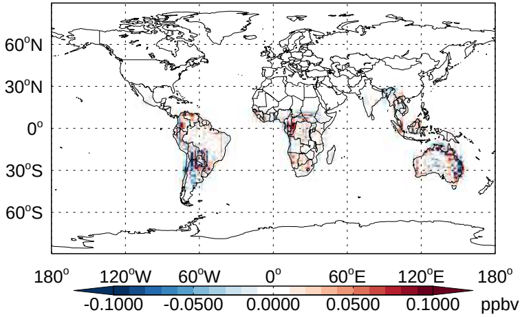
v11-02b-HP - v11-02a ISOG3 - Diff @ Surface for Jan
