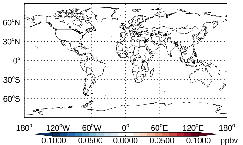
v11-02b-HP - v11-02a BrCl - Diff @ 500 hPa for Jan
