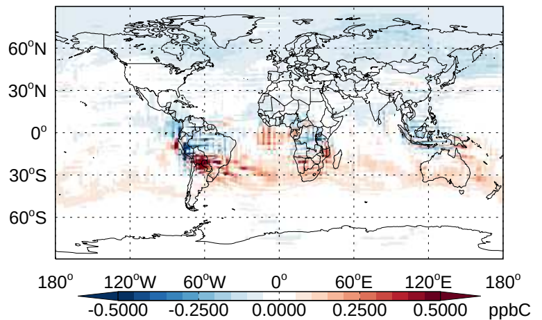
v11-02b-HP - v11-02a ACET- Diff @ 500 hPa for Jan
