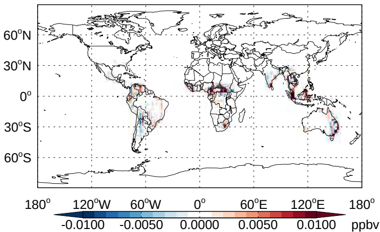
v11-02b-HP - v11-02a PMN - Diff @ Surface for Jan
