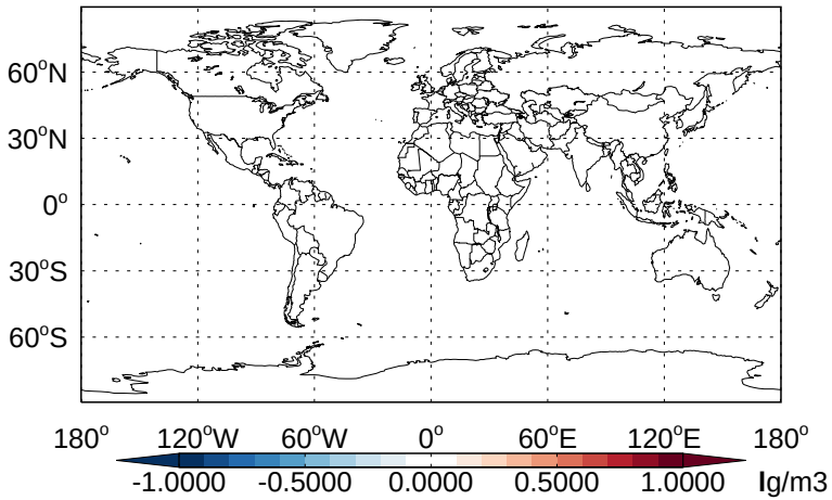
v11-02b-HP - v11-02a MSA - Diff @ Surface for Jan
