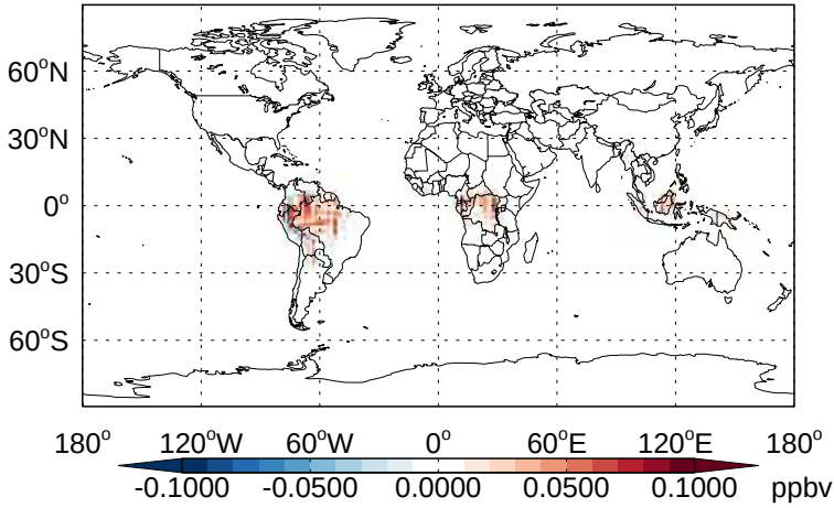
v11-02b-HP - v11-02a TSOA0 - Diff @ Surface for Jan
