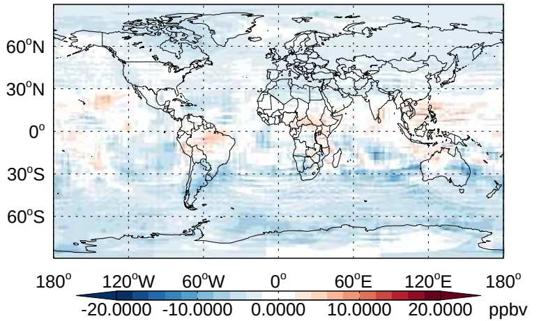
v11-02b-HP - v11-02a O3- Diff @ 500 hPa for Jan
