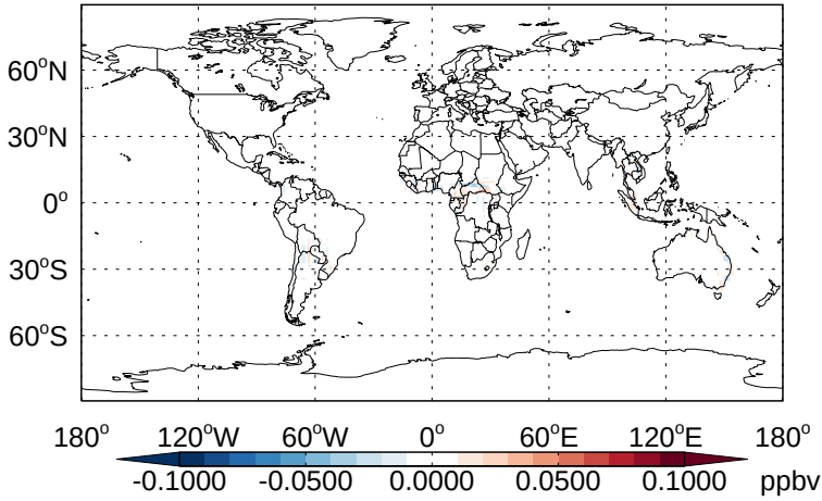
v11-02b-HP - v11-02a PROPNN - Diff @ Surface for Jan
