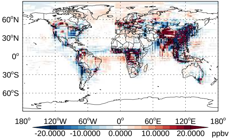
v11-02b-HP - v11-02a CO - Diff @ Surface for Jan
