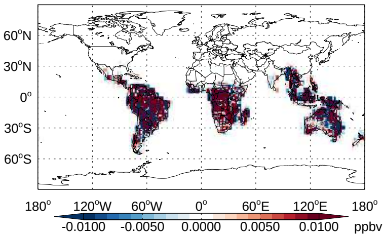
v11-02b-HP - v11-02a RIP - Diff @ Surface for Jan
