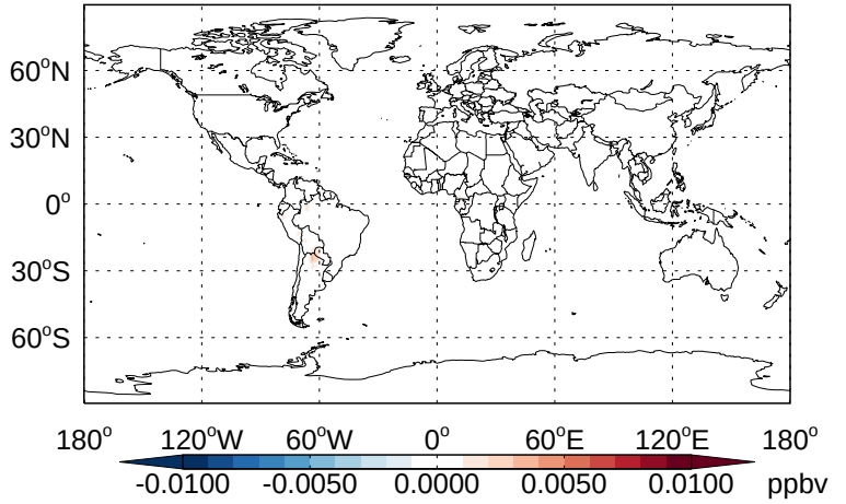
v11-02b-HP - v11-02a MVKN- Diff @ 500 hPa for Jan
