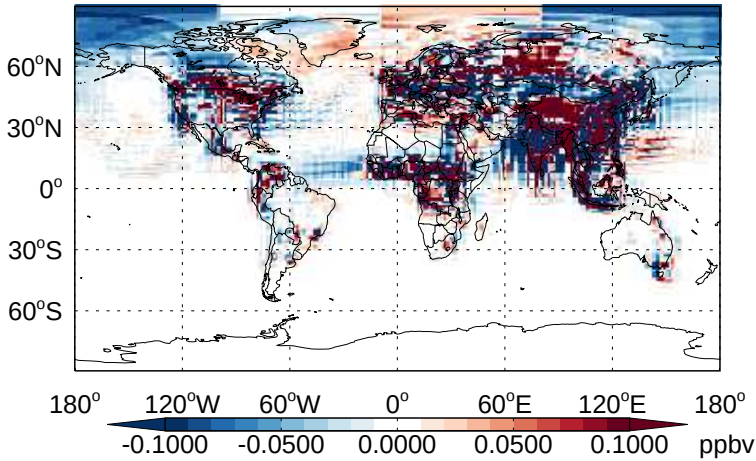
v11-02b-HP - v11-02a BENZ - Diff @ Surface for Jan
