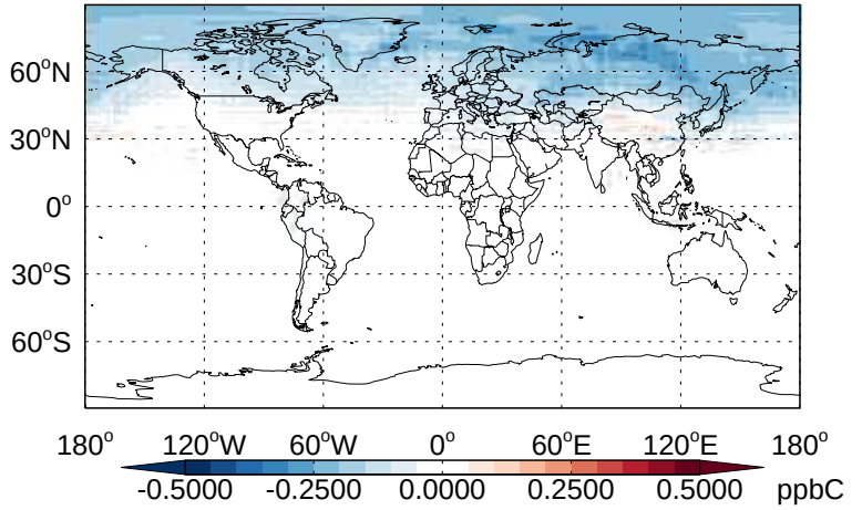
v11-02b-HP - v11-02a C3H8- Diff @ 500 hPa for Jan
