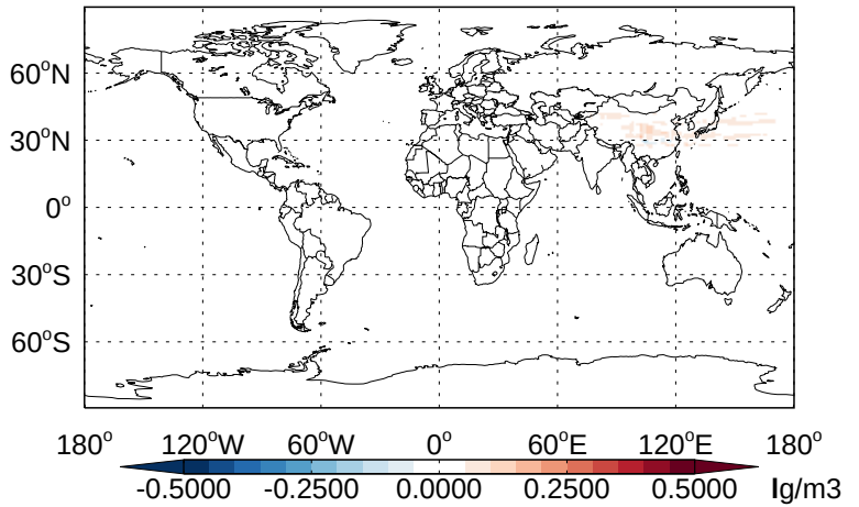
v11-02b-HP - v11-02a NIT- Diff @ 500 hPa for Jan
