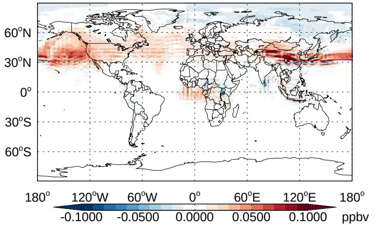
v11-02b-HP - v11-02a BENZ- Diff @ 500 hPa for Jan
