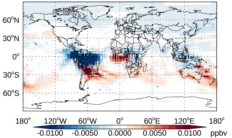
v11-02b-HP - v11-02a MAP- Diff @ 500 hPa for Jan
