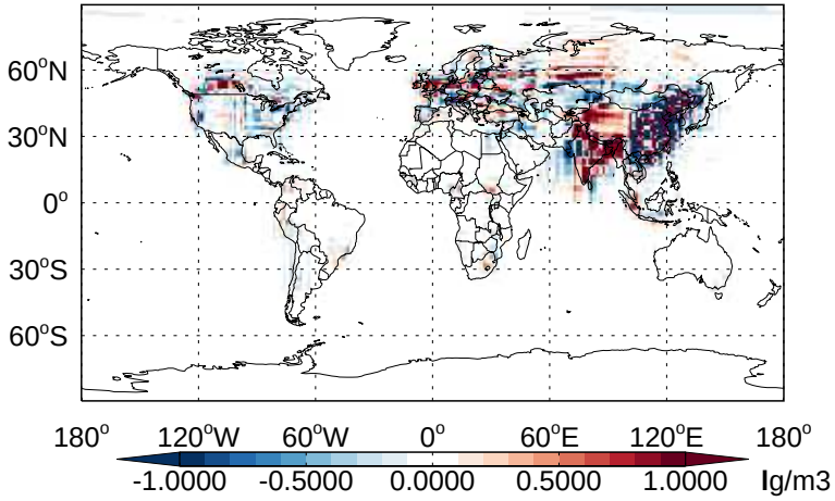
v11-02b-HP - v11-02a NH4 - Diff @ Surface for Jan
