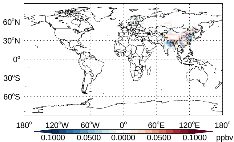
v11-02b-HP - v11-02a MGLY - Diff @ Surface for Jan
