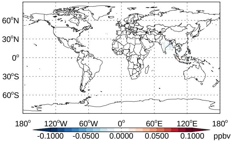
v11-02b-HP - v11-02a ASOAN - Diff @ Surface for Jan
