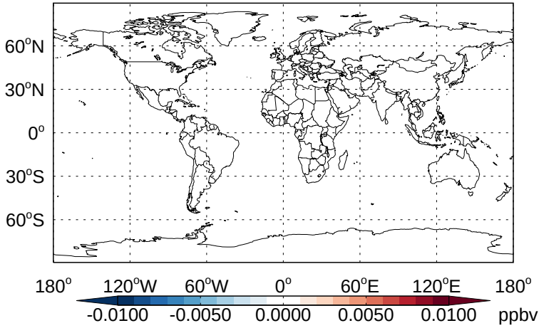
v11-02b-HP - v11-02a BrO - Diff @ Surface for Jan
