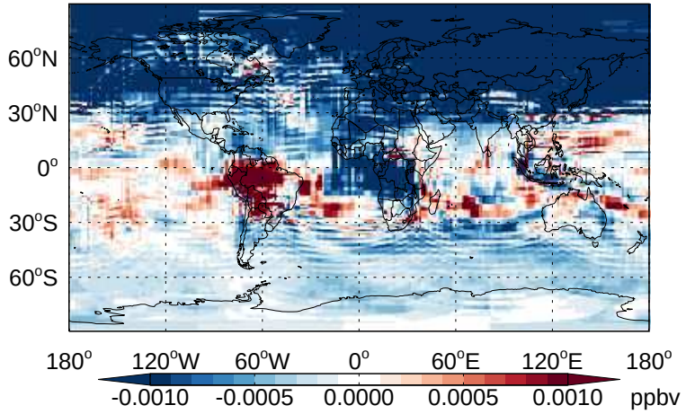
v11-02b-HP - v11-02a PPN- Diff @ 500 hPa for Jan
