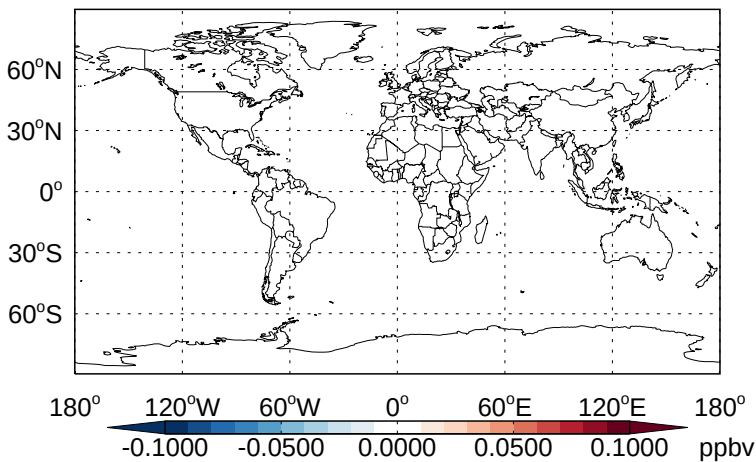
v11-02b-HP - v11-02a ISOG2 - Diff @ Surface for Jan
