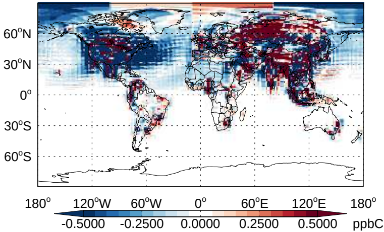
v11-02b-HP - v11-02a ALK4 - Diff @ Surface for Jan
