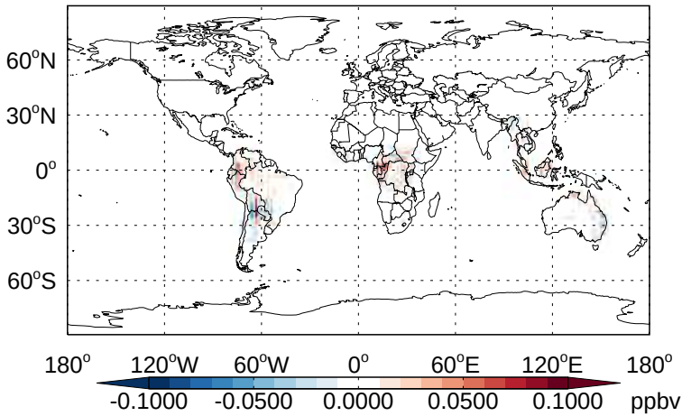
v11-02b-HP - v11-02a ISOA1 - Diff @ Surface for Jan
