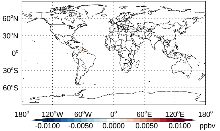
v11-02b-HP - v11-02a NO 3 - Diff @ 500 hPa for Jan
