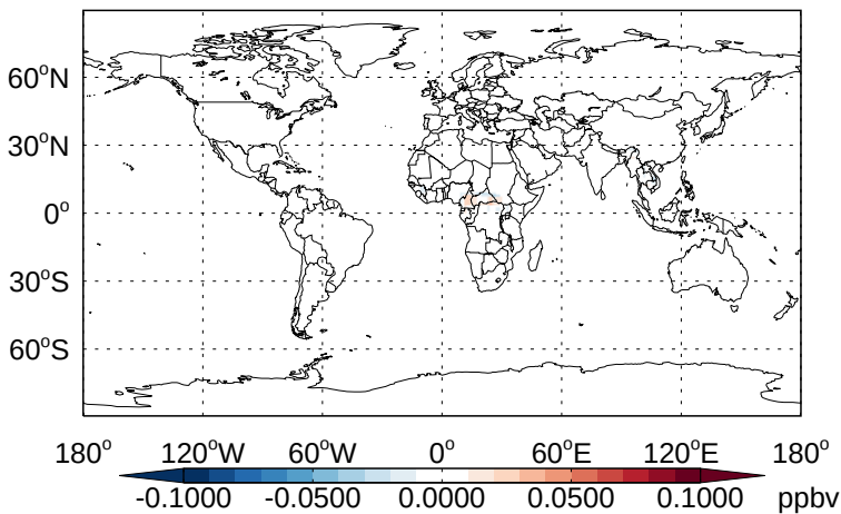
v11-02b-HP - v11-02a ISOA2 - Diff @ Surface for Jan
