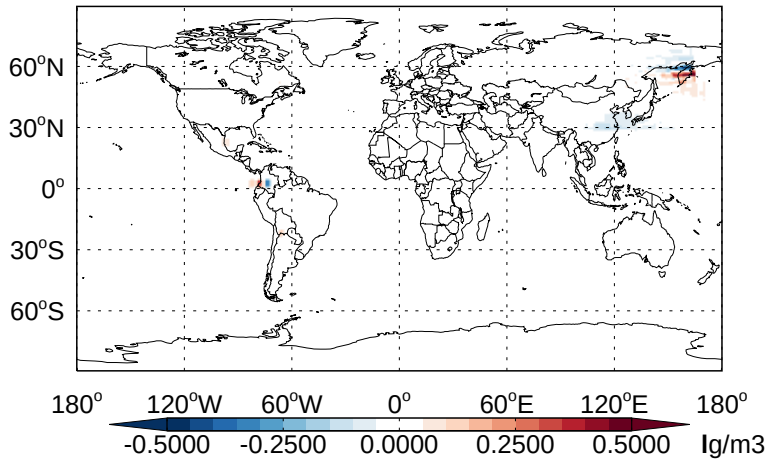
v11-02b-HP - v11-02a SO2- Diff @ 500 hPa for Jan
