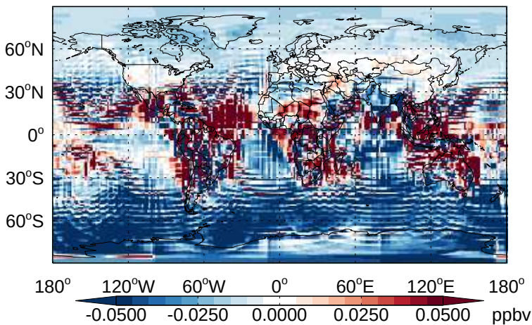
v11-02b-HP - v11-02a MP - Diff @ Surface for Jan
