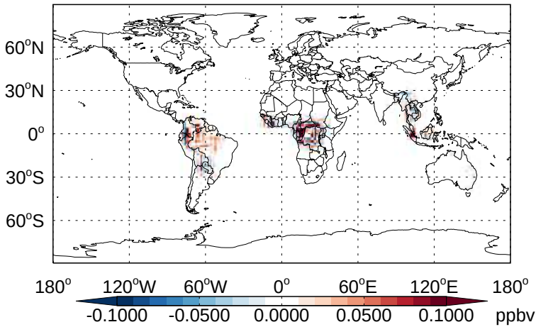
v11-02b-HP - v11-02a TSOA2 - Diff @ Surface for Jan
