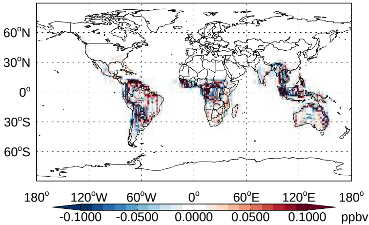
v11-02b-HP - v11-02a TSOG3 - Diff @ Surface for Jan
