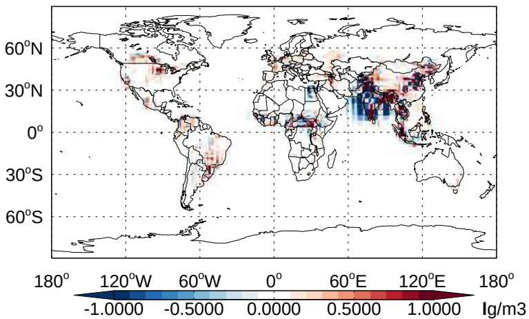
v11-02b-HP - v11-02a NH 3 - Diff @ Surface for Jan
