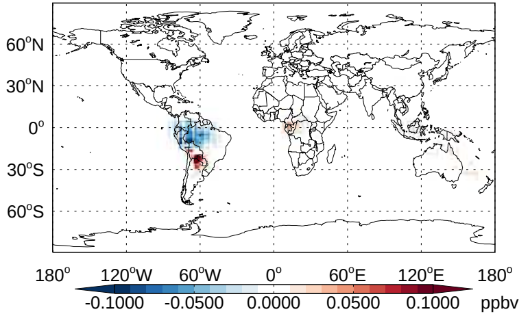
v11-02b-HP - v11-02a HAC- Diff @ 500 hPa for Jan
