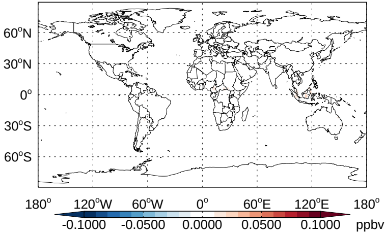
v11-02b-HP - v11-02a ISOPND - Diff @ Surface for Jan
