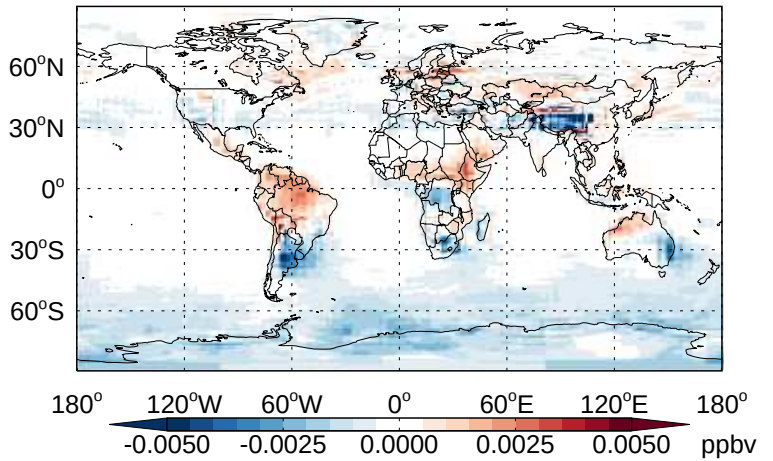
v11-02b-HP - v11-02a HNO4- Diff @ 500 hPa for Jan
