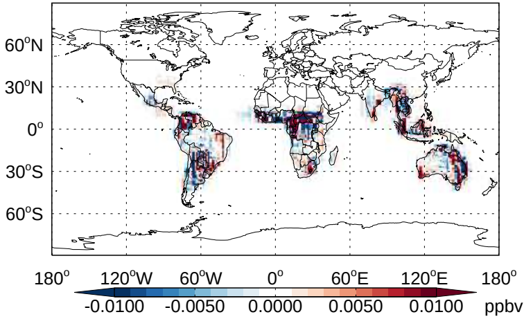
v11-02b-HP - v11-02a MVKN - Diff @ Surface for Jan
