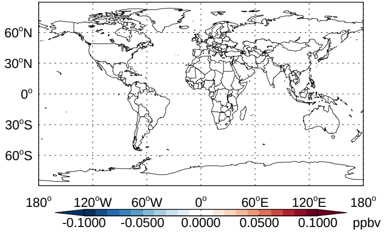
v11-02b-HP - v11-02a HCl- Diff @ 500 hPa for Jan
