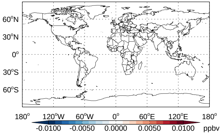
v11-02b-HP - v11-02a CH 3 Br- Diff @ 500 hPa for Jan
