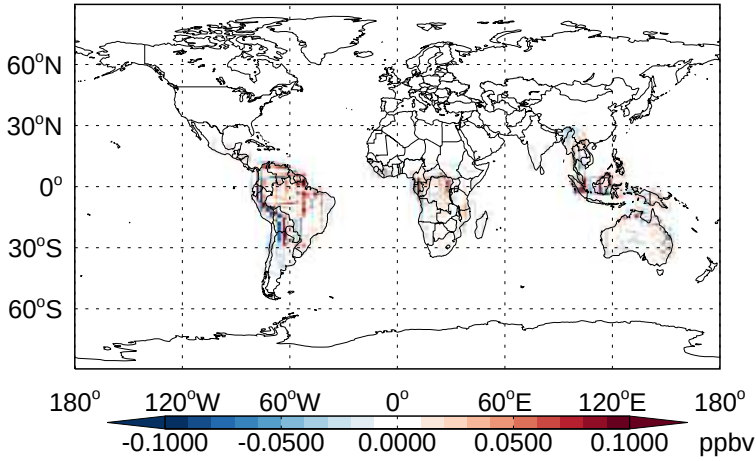
v11-02b-HP - v11-02a TSOG2 - Diff @ Surface for Jan
