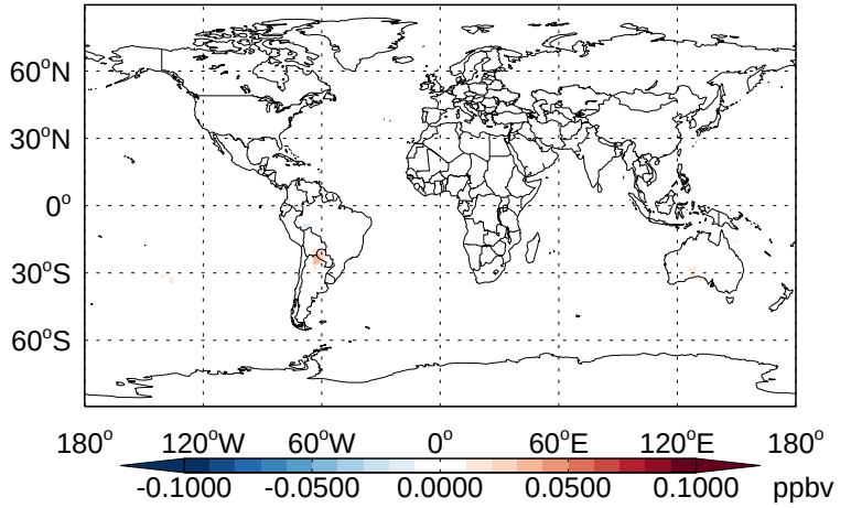
v11-02b-HP - v11-02a ISOG3- Diff @ 500 hPa for Jan
