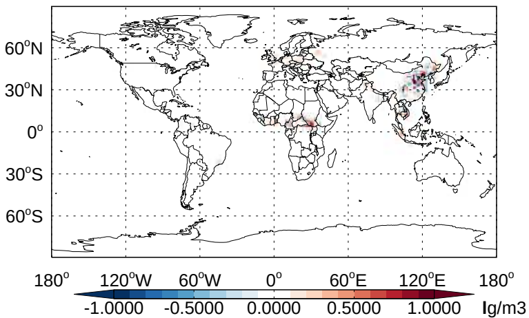
v11-02b-HP - v11-02a BCPO - Diff @ Surface for Jan
