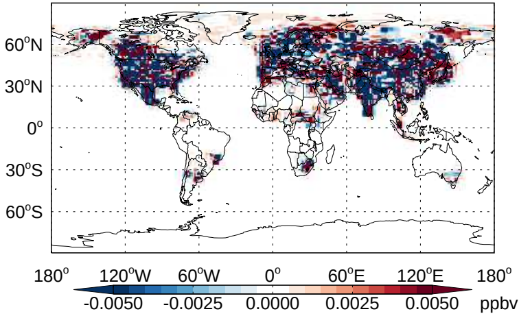
v11-02b-HP - v11-02a N2O5 - Diff @ Surface for Jan
