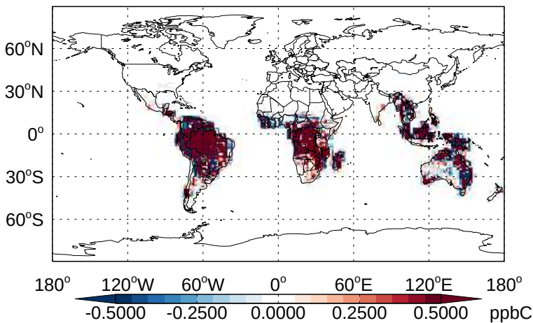
v11-02b-HP - v11-02a ISOP - Diff @ Surface for Jan
