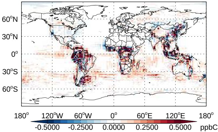
v11-02b-HP - v11-02a ALD2 - Diff @ Surface for Jan
