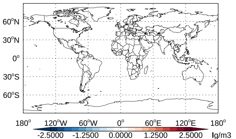
v11-02b-HP - v11-02a DST2- Diff @ 500 hPa for Jan
