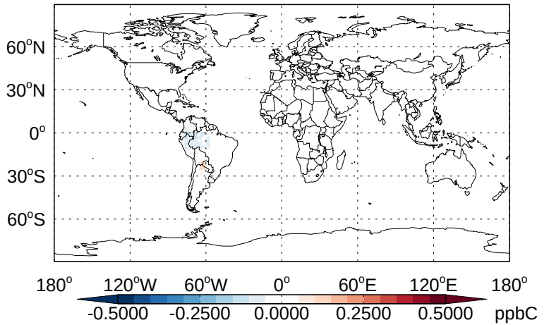
v11-02b-HP - v11-02a ALD2- Diff @ 500 hPa for Jan
