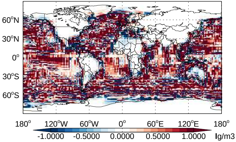
v11-02b-HP - v11-02a SALC - Diff @ Surface for Jan
