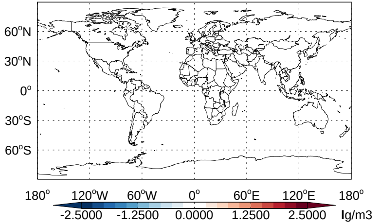
v11-02b-HP - v11-02a DST3- Diff @ 500 hPa for Jan
