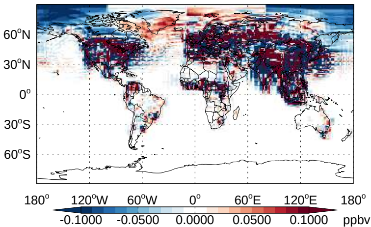
v11-02b-HP - v11-02a TOLU - Diff @ Surface for Jan
