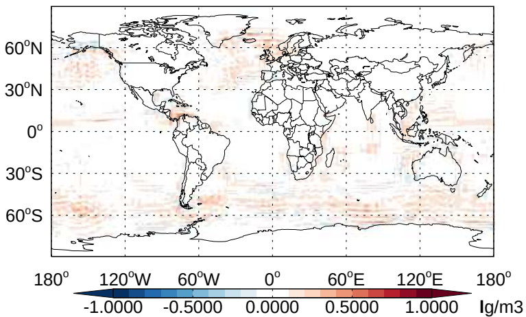
v11-02b-HP - v11-02a SALA - Diff @ Surface for Jan
