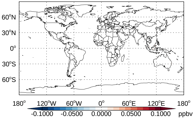
v11-02b-HP - v11-02a ISOPNB - Diff @ Surface for Jan
