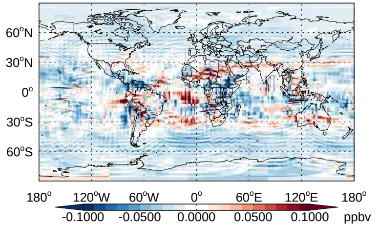
v11-02b-HP - v11-02a H 2 O 2 - Diff @ 500 hPa for Jan
