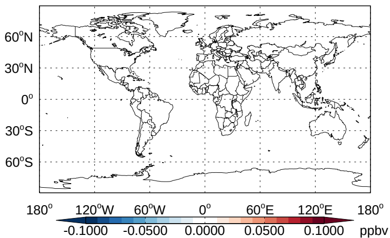
v11-02b-HP - v11-02a MGLY- Diff @ 500 hPa for Jan
