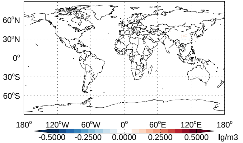
v11-02b-HP - v11-02a NH4- Diff @ 500 hPa for Jan
