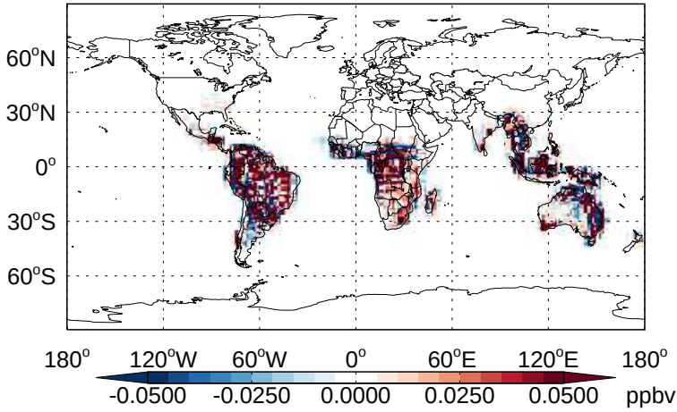
v11-02b-HP - v11-02a MVK - Diff @ Surface for Jan
