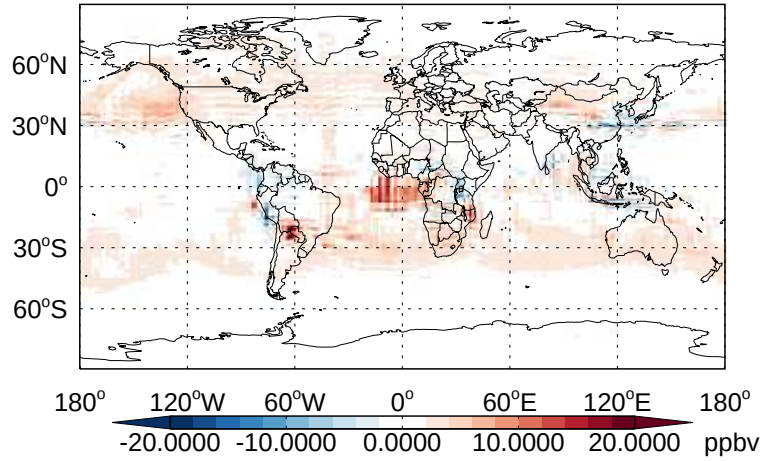
v11-02b-HP - v11-02a CO- Diff @ 500 hPa for Jan
