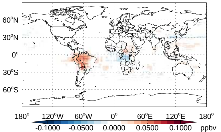
v11-02b-HP - v11-02a PAN- Diff @ 500 hPa for Jan
