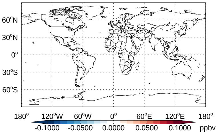
v11-02b-HP - v11-02a CH3Cl - Diff @ Surface for Jan
