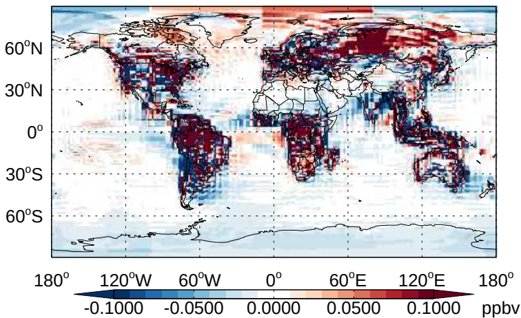
v11-02b-HP - v11-02a EOH - Diff @ Surface for Jan
