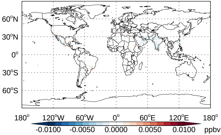
v11-02b-HP - v11-02a NO 3 - Diff @ Surface for Jan
