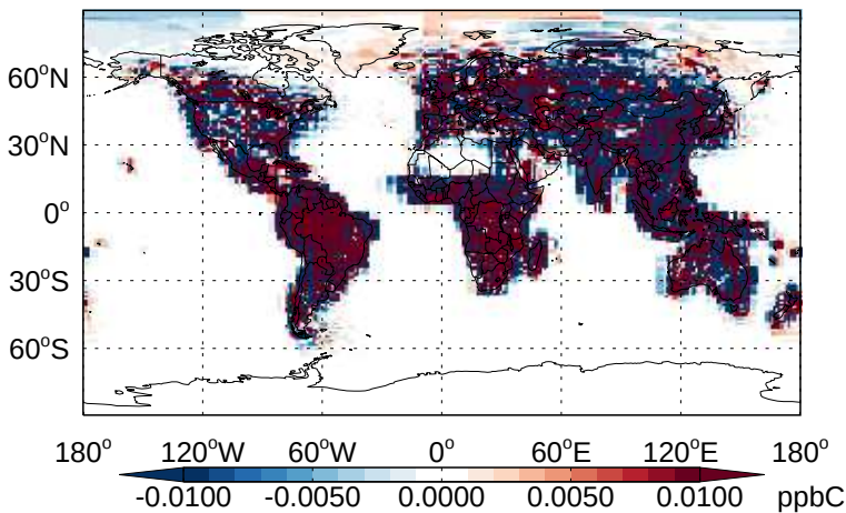
v11-02b-HP - v11-02a PRPE - Diff @ Surface for Jan
