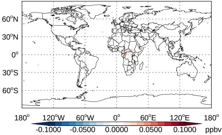
v11-02b-HP - v11-02a ISOA3 - Diff @ Surface for Jan
