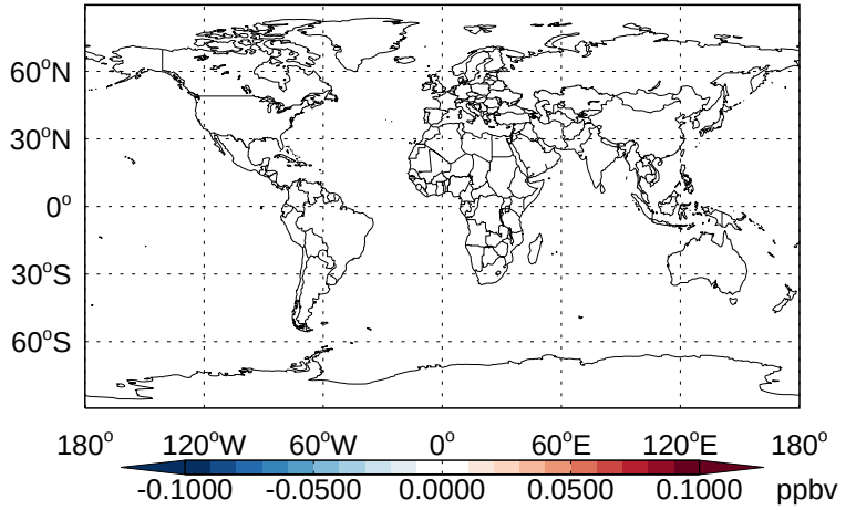
v11-02b-HP - v11-02a HCFC22- Diff @ 500 hPa for Jan
