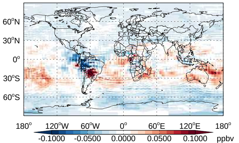
v11-02b-HP - v11-02a EOH- Diff @ 500 hPa for Jan
