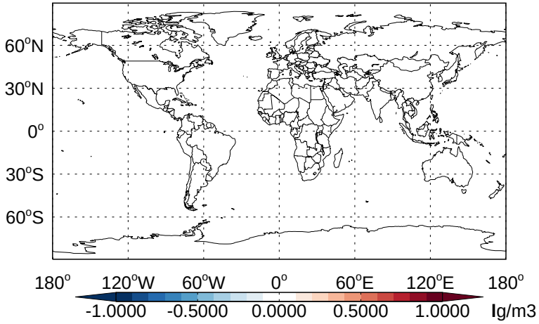
v11-02b-HP - v11-02a SO 4 s - Diff @ Surface for Jan
