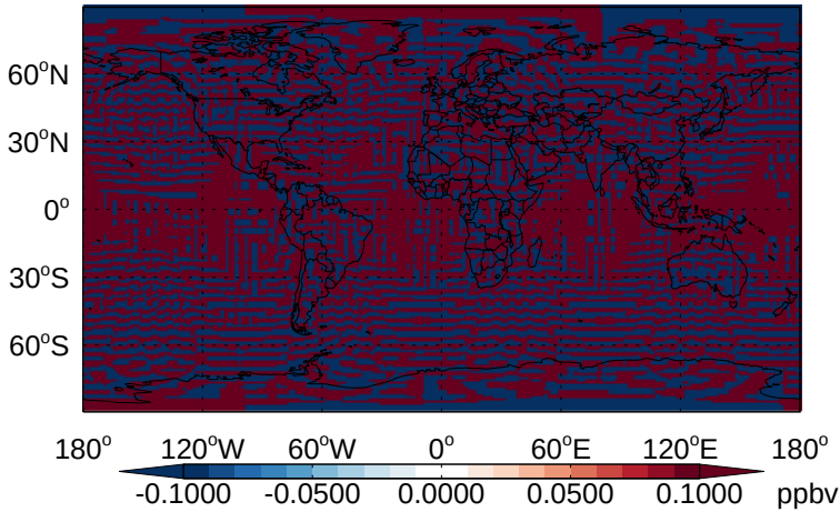
v11-02b-HP - v11-02a H 2 O - Diff @ Surface for Jan
