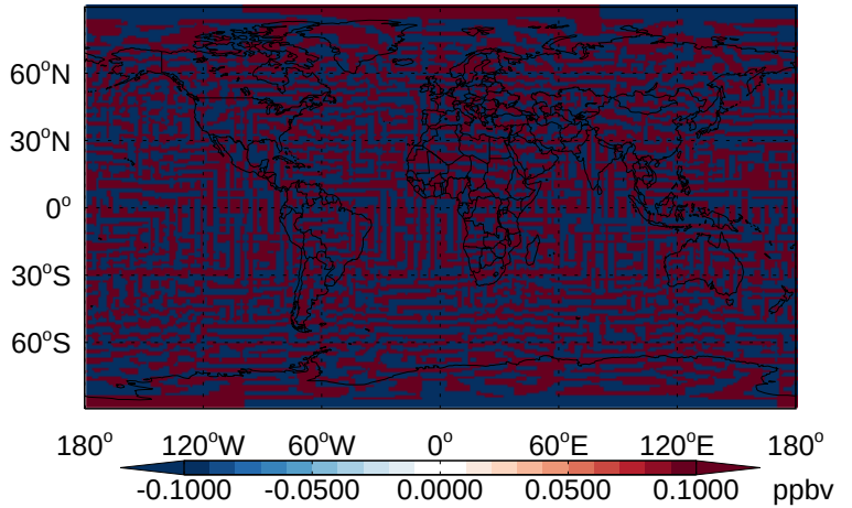
v11-02b-HP - v11-02a H 2 O- Diff @ 500 hPa for Jan
