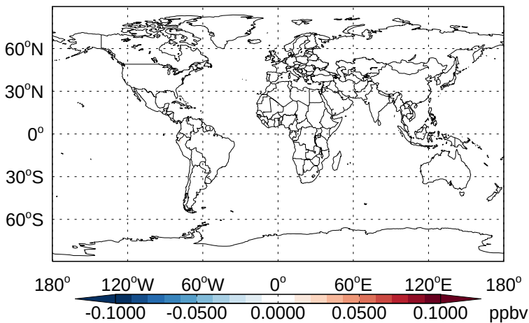
v11-02b-HP - v11-02a TSOG1 - Diff @ Surface for Jan
