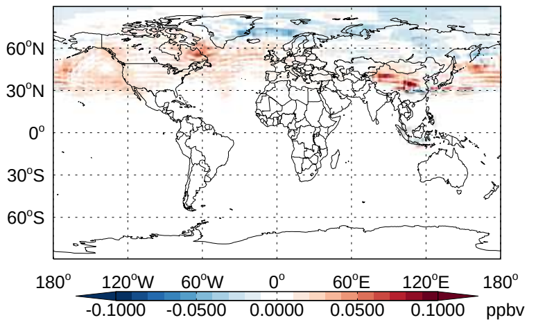
v11-02b-HP - v11-02a TOLU- Diff @ 500 hPa for Jan
