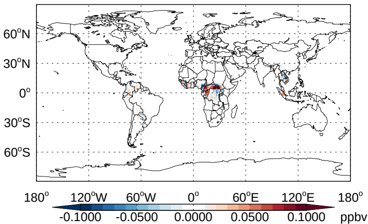
v11-02b-HP - v11-02a TSOA3 - Diff @ Surface for Jan
