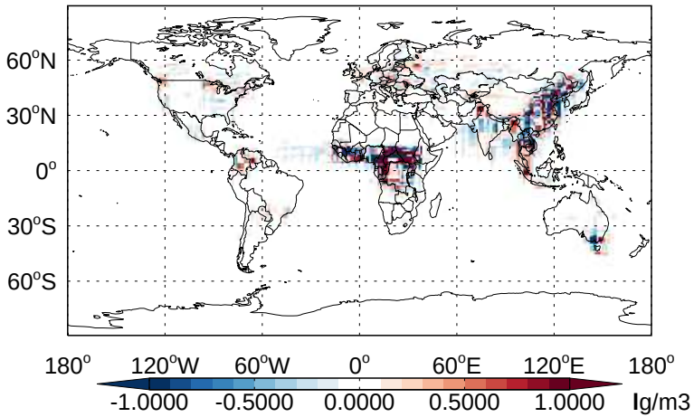
v11-02b-HP - v11-02a OCPI - Diff @ Surface for Jan
