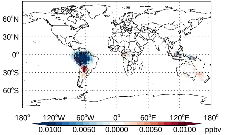
v11-02b-HP - v11-02a IEPOX- Diff @ 500 hPa for Jan
