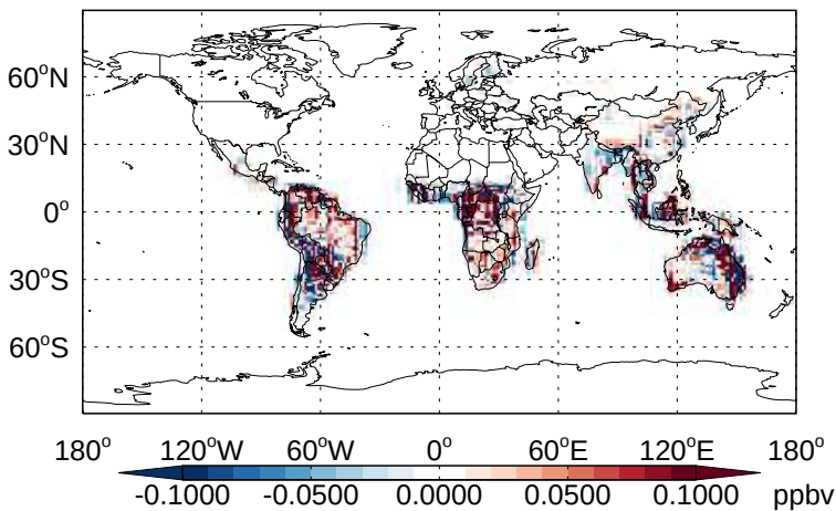
v11-02b-HP - v11-02a GLYC - Diff @ Surface for Jan
