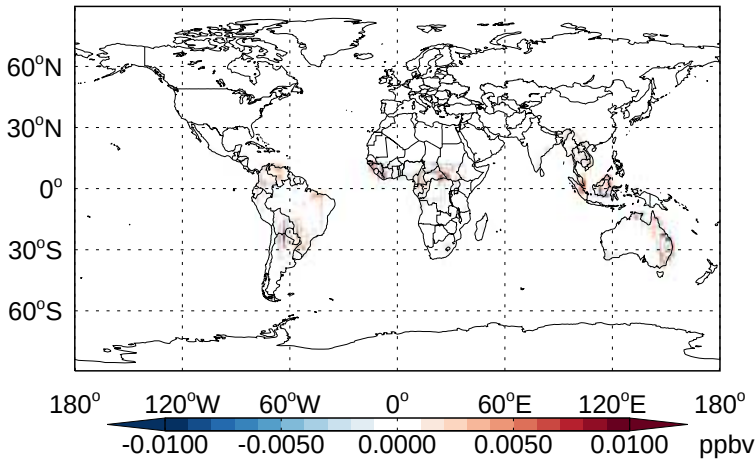
v11-02b-HP - v11-02a MACRN - Diff @ Surface for Jan
