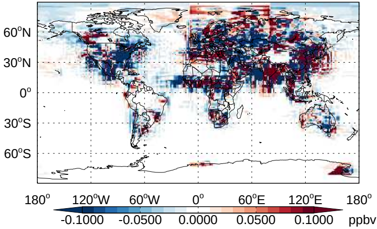
v11-02b-HP - v11-02a HNO 3 - Diff @ Surface for Jan
