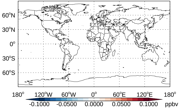
v11-02b-HP - v11-02a ISOG1- Diff @ 500 hPa for Jan
