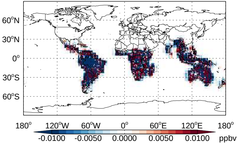
v11-02b-HP - v11-02a IEPOX - Diff @ Surface for Jan
