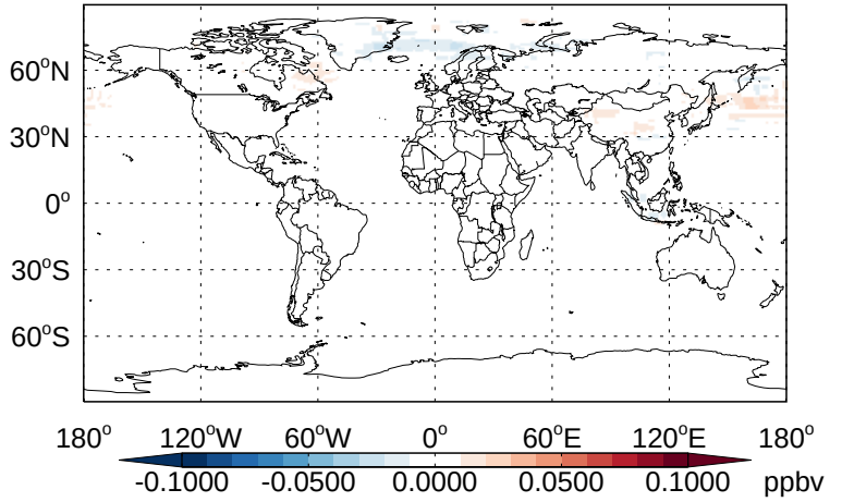
v11-02b-HP - v11-02a XYLE- Diff @ 500 hPa for Jan
