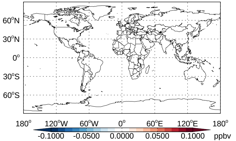
v11-02b-HP - v11-02a ASOG1- Diff @ 500 hPa for Jan
