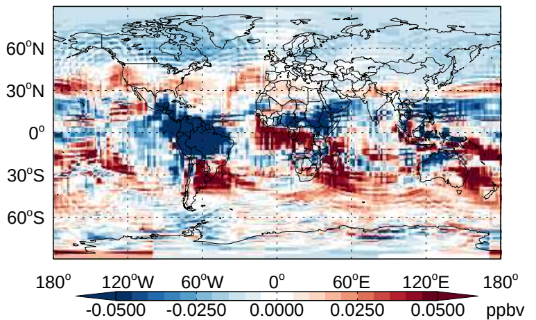
v11-02b-HP - v11-02a MP- Diff @ 500 hPa for Jan
