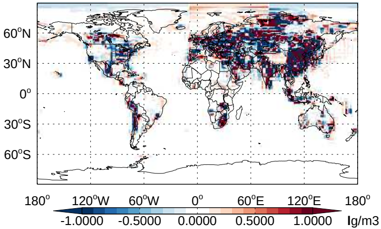
v11-02b-HP - v11-02a SO2 - Diff @ Surface for Jan
