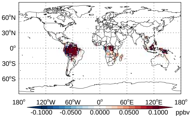
v11-02b-HP - v11-02a MTPA - Diff @ Surface for Jan
