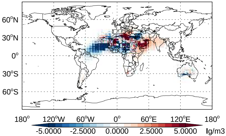
v11-02b-HP - v11-02a DST1 - Diff @ Surface for Jan
