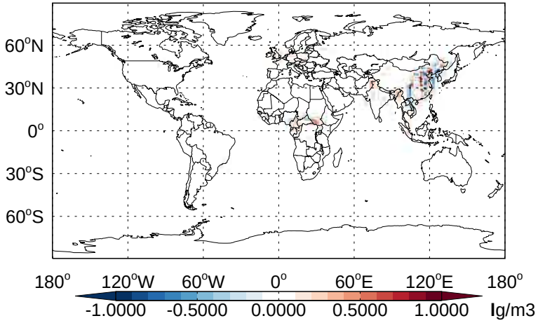
v11-02b-HP - v11-02a BCPI - Diff @ Surface for Jan
