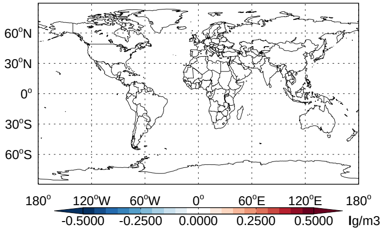
v11-02b-HP - v11-02a OCPI- Diff @ 500 hPa for Jan
