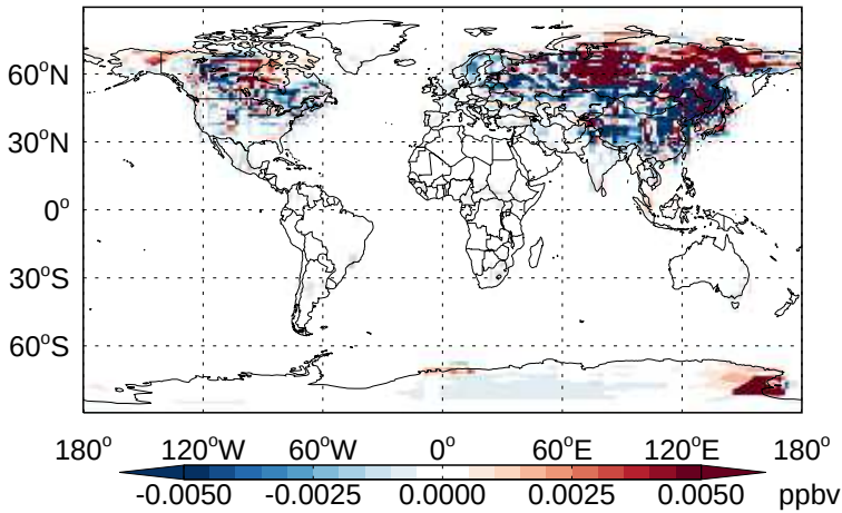
v11-02b-HP - v11-02a HNO4 - Diff @ Surface for Jan
