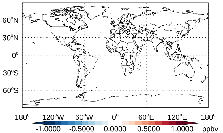
v11-02b-HP - v11-02a NO2- Diff @ 500 hPa for Jan
