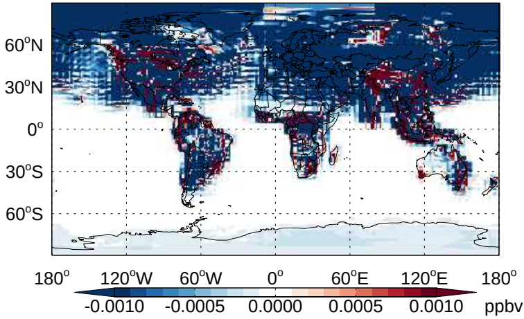
v11-02b-HP - v11-02a PPN - Diff @ Surface for Jan
