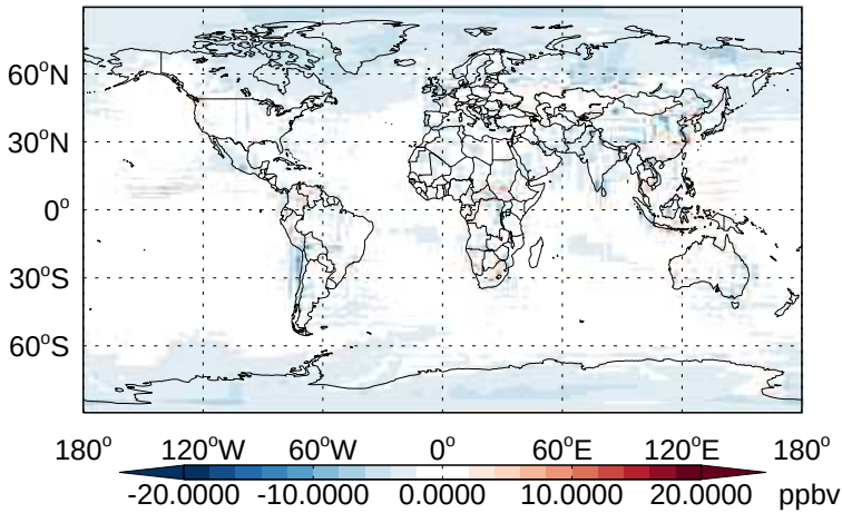
v11-02b-HP - v11-02a O3 - Diff @ Surface for Jan
