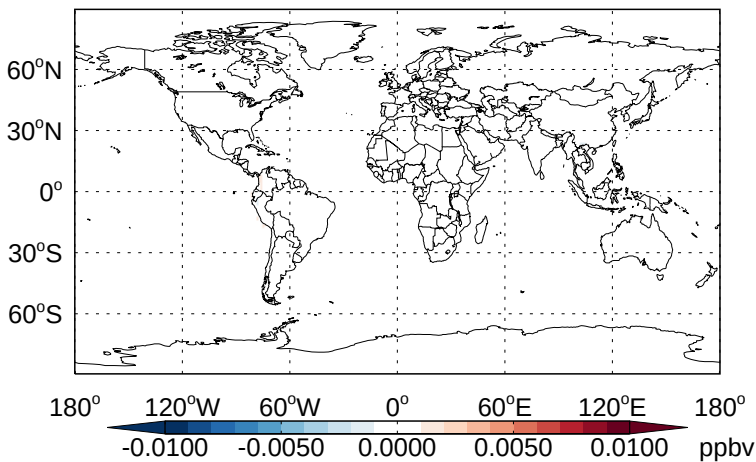
v11-02b-HP - v11-02a CHBr 3 - Diff @ Surface for Jan
