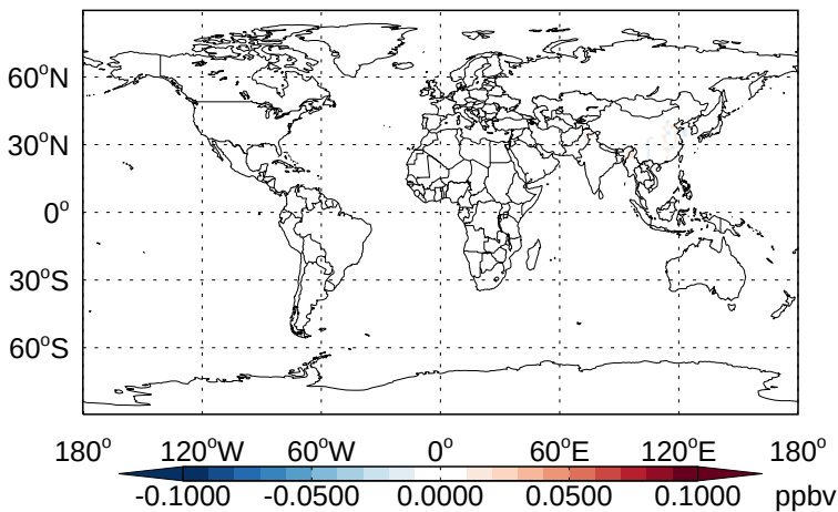
v11-02b-HP - v11-02a ASOA1 - Diff @ Surface for Jan
