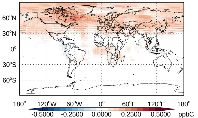
v11-02b-HP - v11-02a C2H6- Diff @ 500 hPa for Jan
