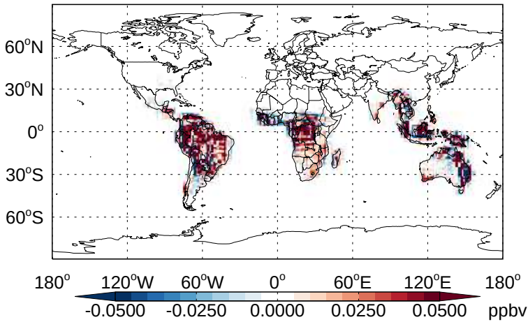
v11-02b-HP - v11-02a MACR - Diff @ Surface for Jan
