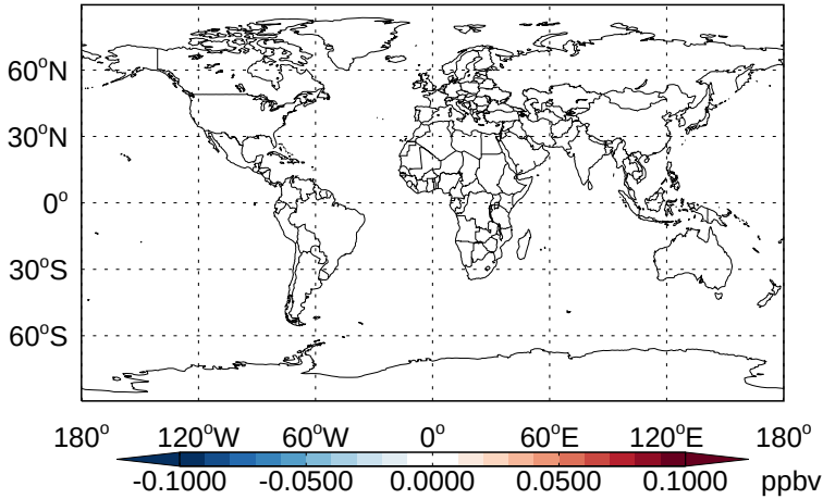
v11-02b-HP - v11-02a CFC11 - Diff @ Surface for Jan
