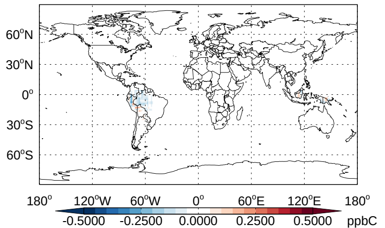
v11-02b-HP - v11-02a ISOP- Diff @ 500 hPa for Jan
