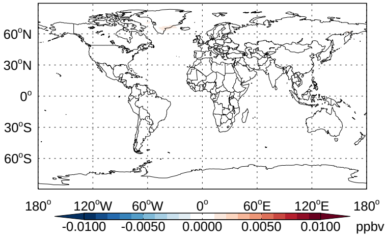
v11-02b-HP - v11-02a HOBr - Diff @ Surface for Jan
