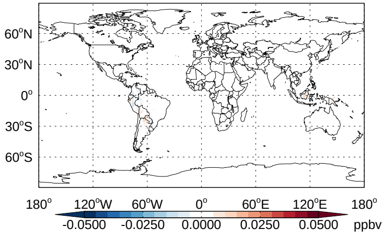
v11-02b-HP - v11-02a MACR- Diff @ 500 hPa for Jan
