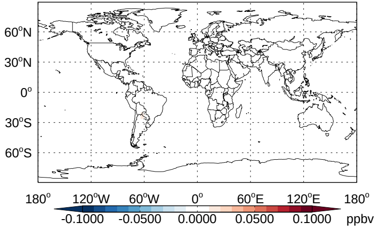
v11-02b-HP - v11-02a TSOG2- Diff @ 500 hPa for Jan
