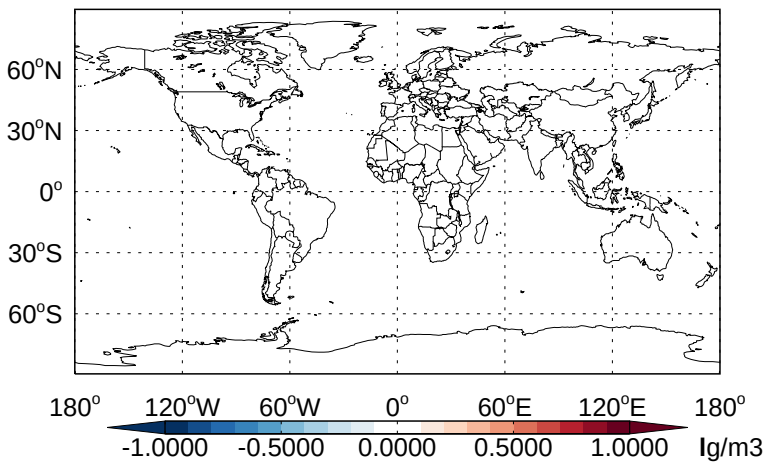
v11-02b-HP - v11-02a NITs - Diff @ Surface for Jan
