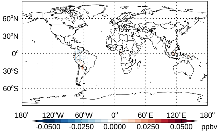
v11-02b-HP - v11-02a MVK- Diff @ 500 hPa for Jan
