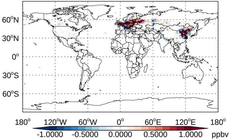
v11-02b-HP - v11-02a NO - Diff @ Surface for Jan
