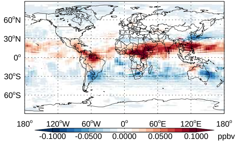
v11-02b-HP - v11-02a HNO 3 - Diff @ 500 hPa for Jan
