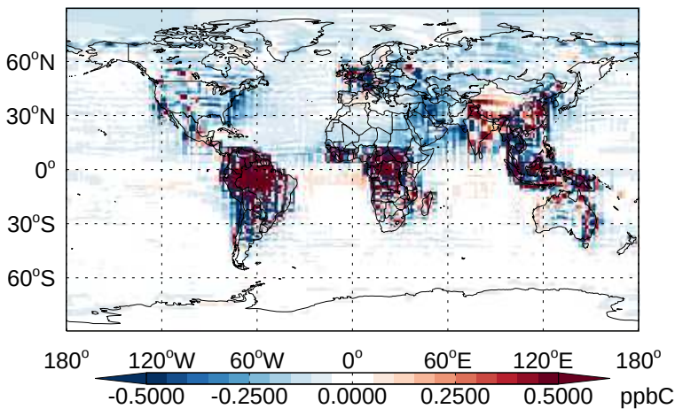
v11-02b-HP - v11-02a ACET - Diff @ Surface for Jan
