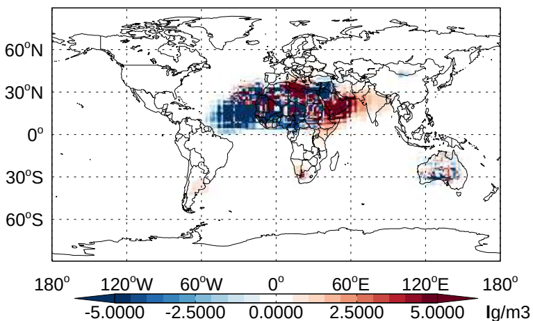
v11-02b-HP - v11-02a DST2 - Diff @ Surface for Jan
