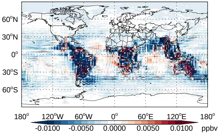
v11-02b-HP - v11-02a MAP - Diff @ Surface for Jan
