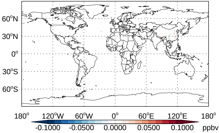
v11-02b-HP - v11-02a ASOA2 - Diff @ Surface for Jan
