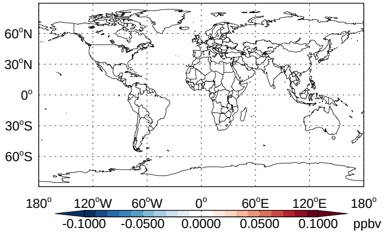
v11-02b-HP - v11-02a HCFC123- Diff @ 500 hPa for Jan
