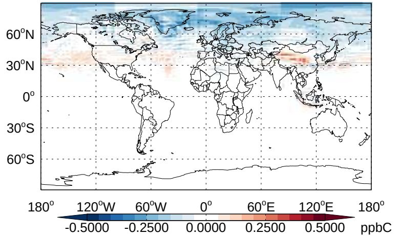
v11-02b-HP - v11-02a ALK4- Diff @ 500 hPa for Jan
