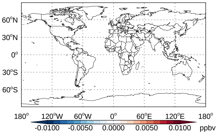
v11-02b-HP - v11-02a HBr - Diff @ Surface for Jan
