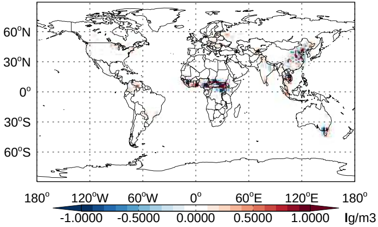
v11-02b-HP - v11-02a OCPO - Diff @ Surface for Jan
