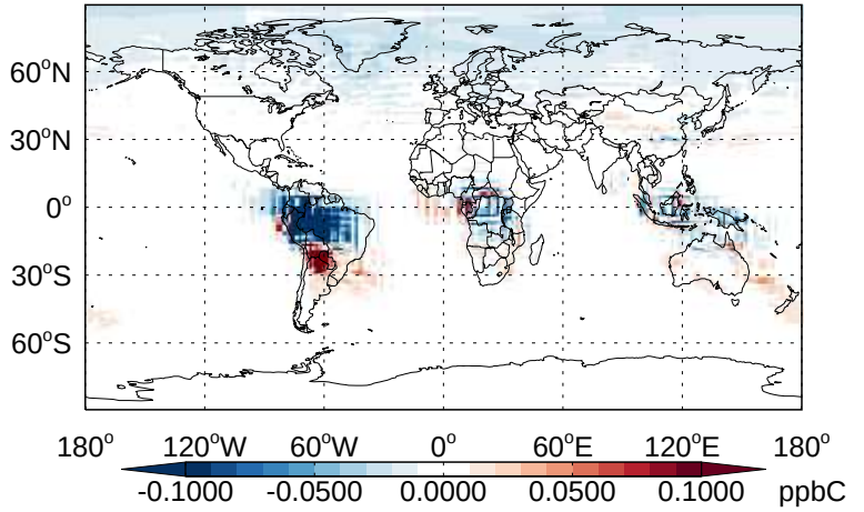
v11-02b-HP - v11-02a MEK- Diff @ 500 hPa for Jan
