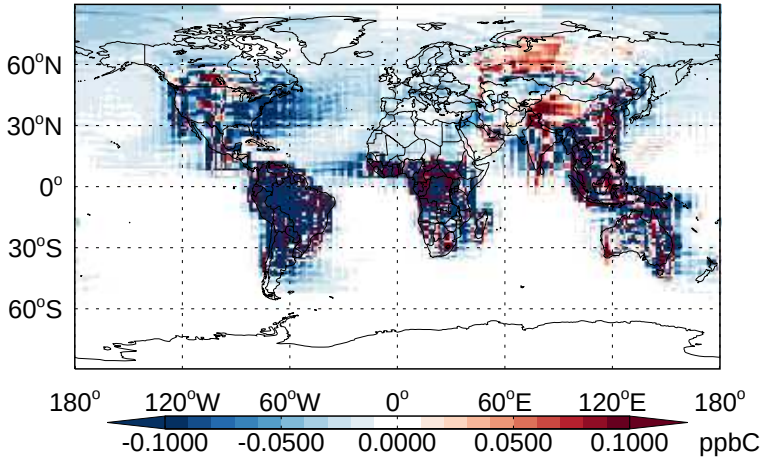
v11-02b-HP - v11-02a MEK - Diff @ Surface for Jan
