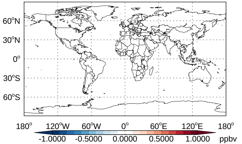
v11-02b-HP - v11-02a HNO 2 - Diff @ 500 hPa for Jan
