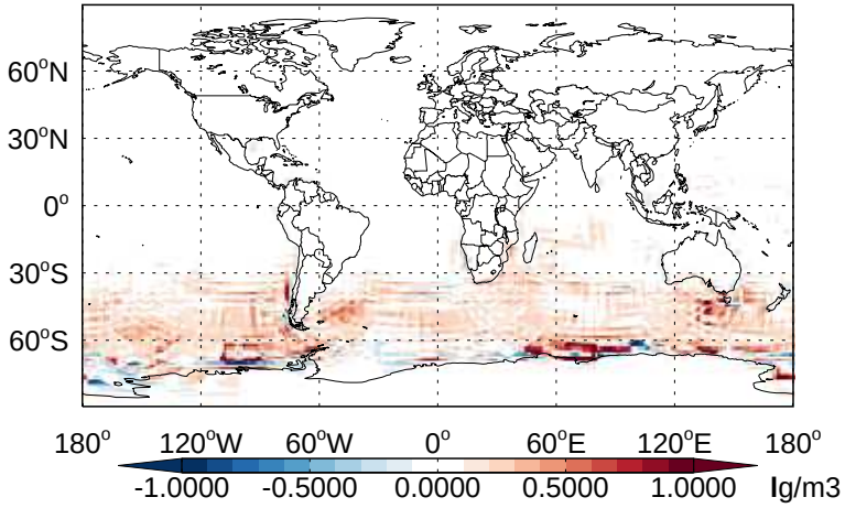
v11-02b-HP - v11-02a DMS - Diff @ Surface for Jan
