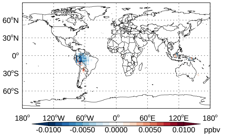
v11-02b-HP - v11-02a RIP- Diff @ 500 hPa for Jan
