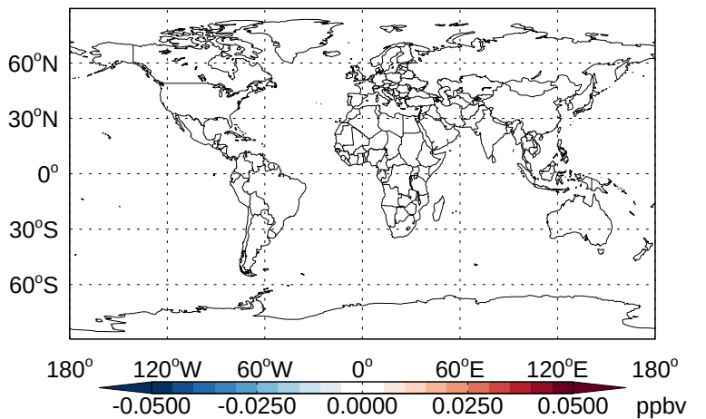
v11-02b-HP - v11-02a RCHO- Diff @ 500 hPa for Jan
