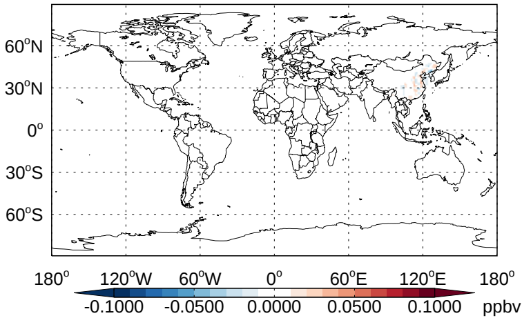
v11-02b-HP - v11-02a ASOA3 - Diff @ Surface for Jan
