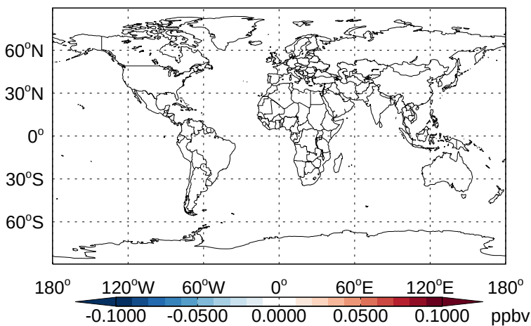
v11-02b-HP - v11-02a BrCl - Diff @ Surface for Jan
