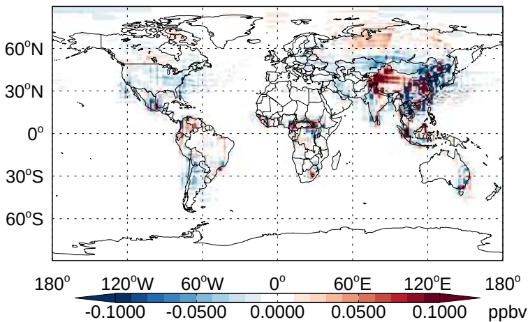
v11-02b-HP - v11-02a PAN - Diff @ Surface for Jan
