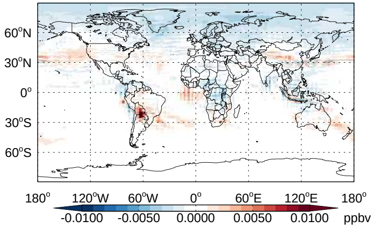
v11-02b-HP - v11-02a R4N2- Diff @ 500 hPa for Jan
