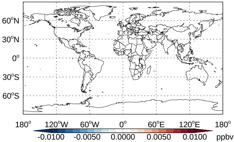
v11-02b-HP - v11-02a CH 3 Br - Diff @ Surface for Jan
