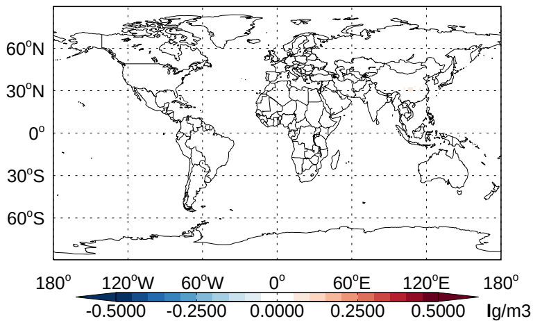
v11-02b-HP - v11-02a NH 3 - Diff @ 500 hPa for Jan
