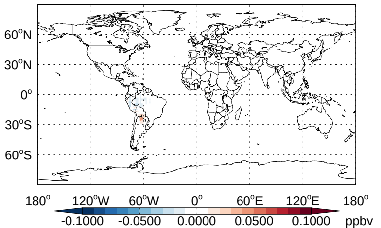
v11-02b-HP - v11-02a GLYC- Diff @ 500 hPa for Jan
