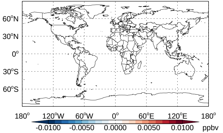
v11-02b-HP - v11-02a CH 2 Br 2 - Diff @ 500 hPa for Jan
