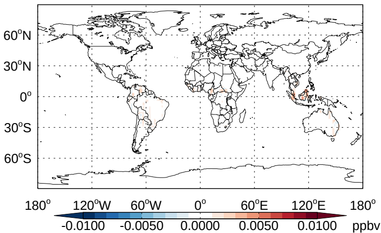
v11-02b-HP - v11-02a MOBA - Diff @ Surface for Jan
