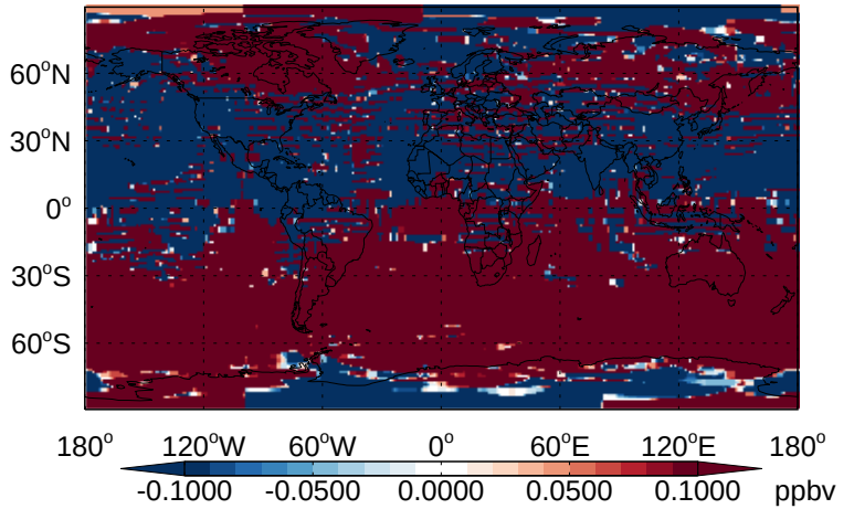
v11-02b-HP - v11-02a CH4- Diff @ 500 hPa for Jan
