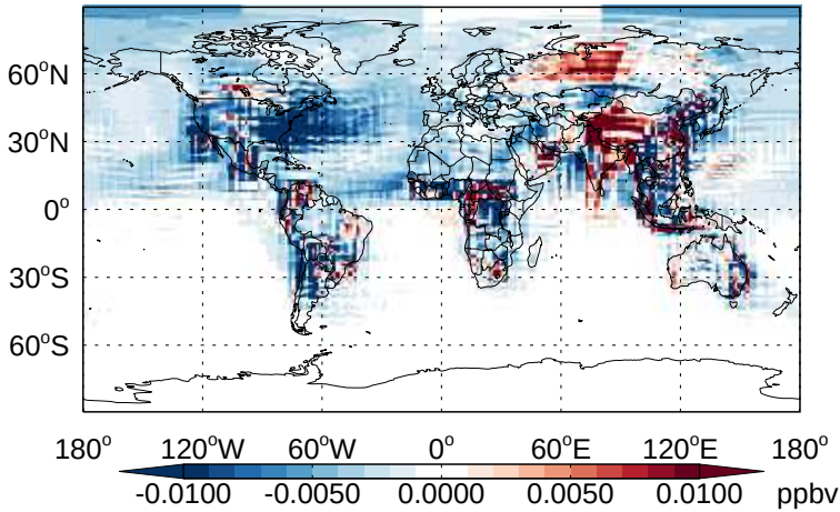
v11-02b-HP - v11-02a R4N2 - Diff @ Surface for Jan
