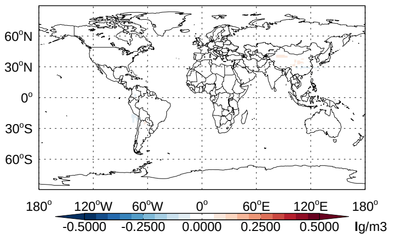
v11-02b-HP - v11-02a SO4- Diff @ 500 hPa for Jan
