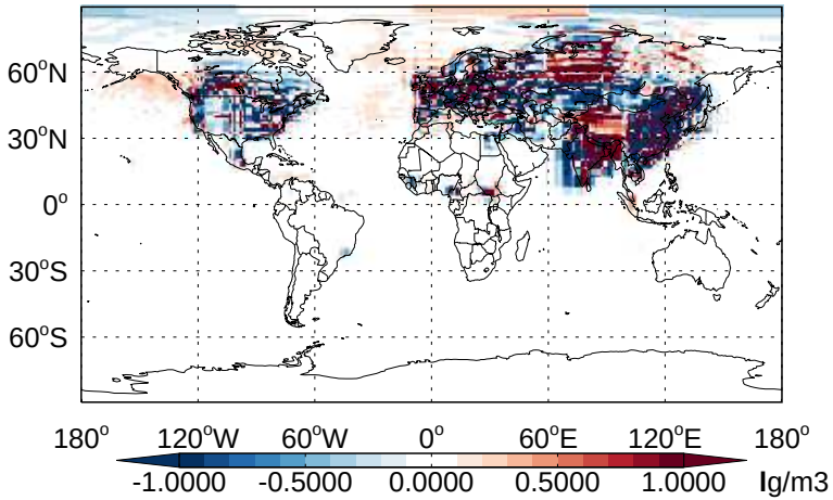
v11-02b-HP - v11-02a NIT - Diff @ Surface for Jan
