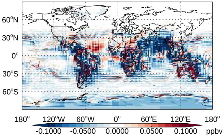
v11-02b-HP - v11-02a H 2 O 2 - Diff @ Surface for Jan
