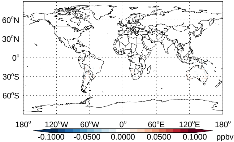
v11-02b-HP - v11-02a ISOG1 - Diff @ Surface for Jan
