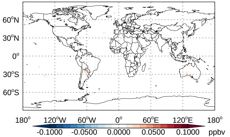
v11-02b-HP - v11-02a TSOG3- Diff @ 500 hPa for Jan
