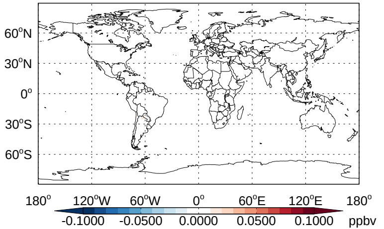
v11-02b-HP - v11-02a ISOA1- Diff @ 500 hPa for Jan
