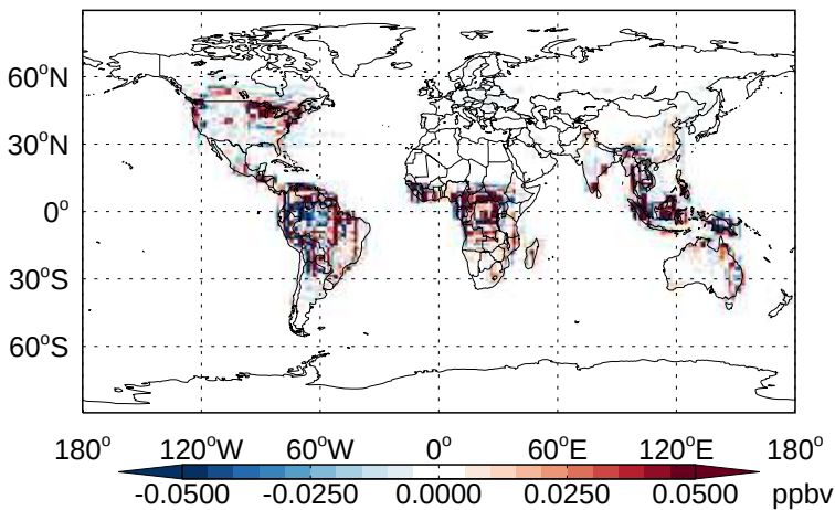
v11-02b-HP - v11-02a RCHO - Diff @ Surface for Jan
