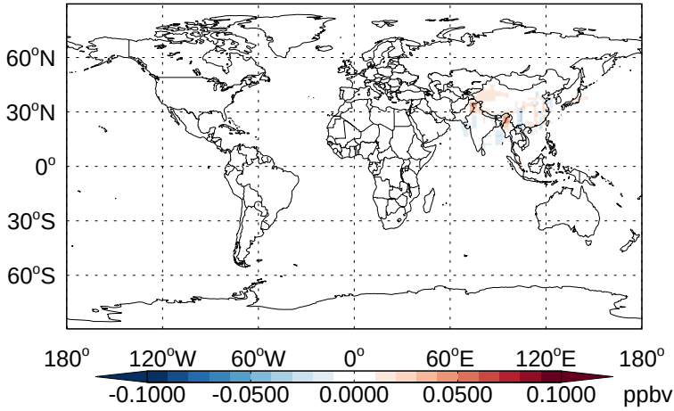
v11-02b-HP - v11-02a ASOG3 - Diff @ Surface for Jan
