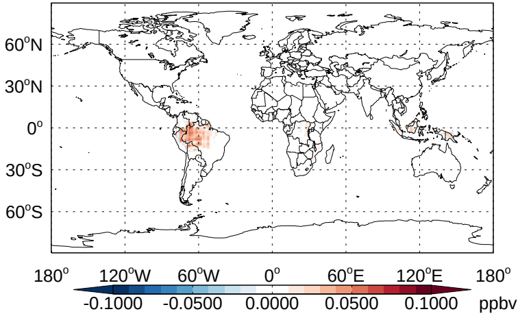
v11-02b-HP - v11-02a LIMO - Diff @ Surface for Jan
