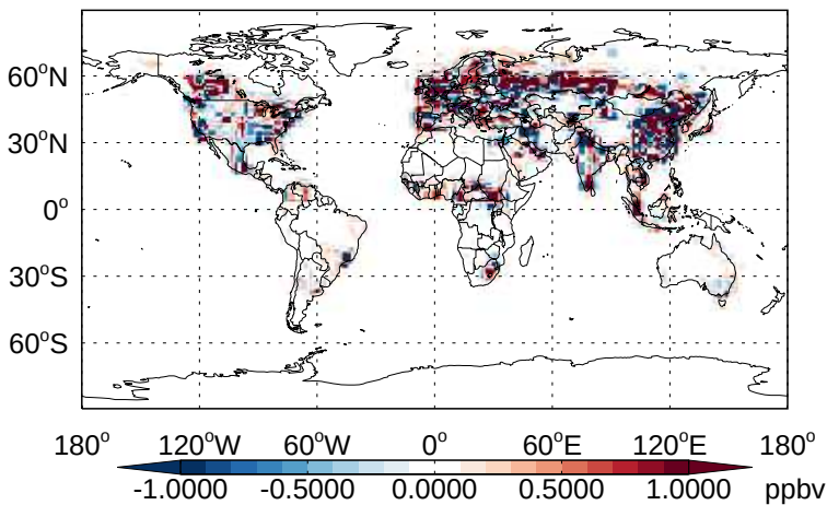
v11-02b-HP - v11-02a NO2 - Diff @ Surface for Jan
