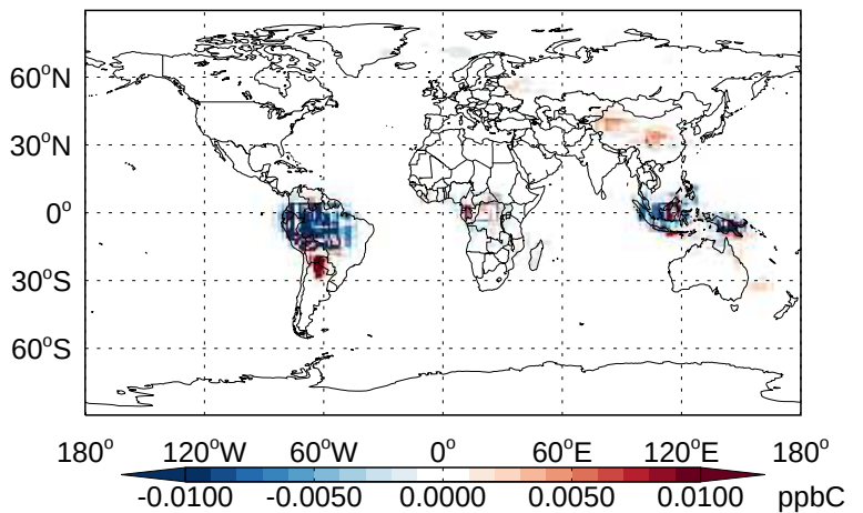
v11-02b-HP - v11-02a PRPE- Diff @ 500 hPa for Jan
