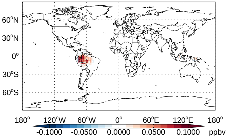
v11-02b-HP - v11-02a MTPO - Diff @ Surface for Jan
