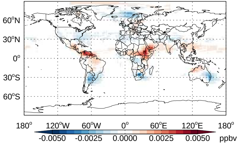
v11-02b-HP - v11-02a N2O5- Diff @ 500 hPa for Jan
