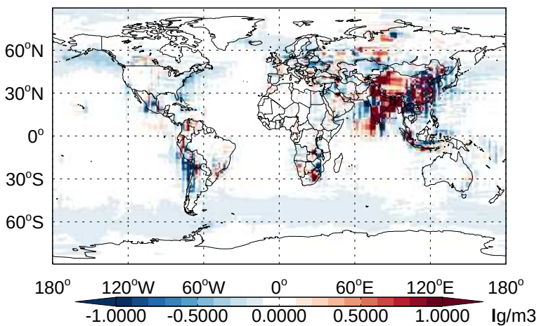
v11-02b-HP - v11-02a SO4 - Diff @ Surface for Jan
