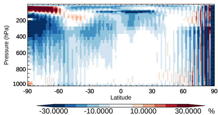
v11-02b-HP / v11-02a CLOO - Zonal mean % diff for Oct
