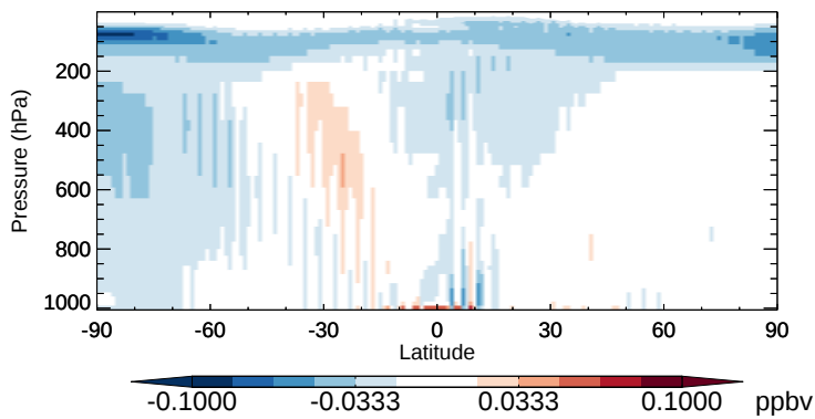
v11-02b-HP - v11-02a EOH - Zonal mean abs diff for Oct
