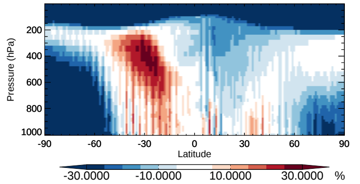
v11-02b-HP / v11-02a ISOG3 - Zonal mean % diff for Oct
