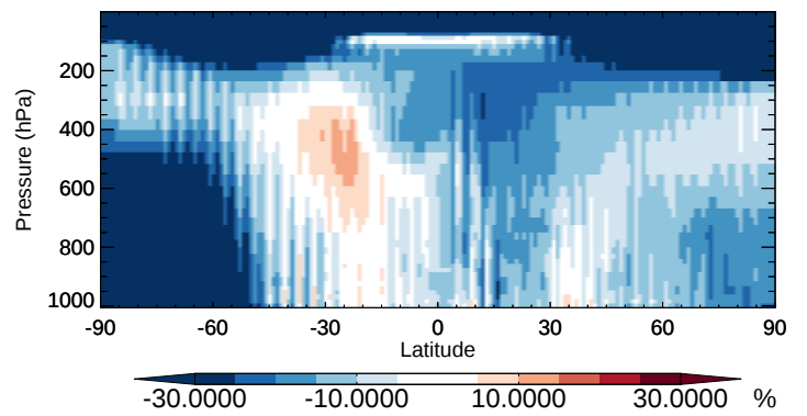
v11-02b-HP / v11-02a ISOG2 - Zonal mean % diff for Oct
