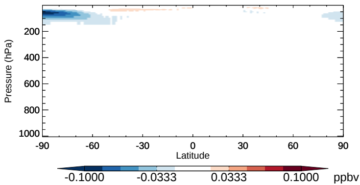
v11-02b-HP - v11-02a CH3Cl - Zonal mean abs diff for Oct
