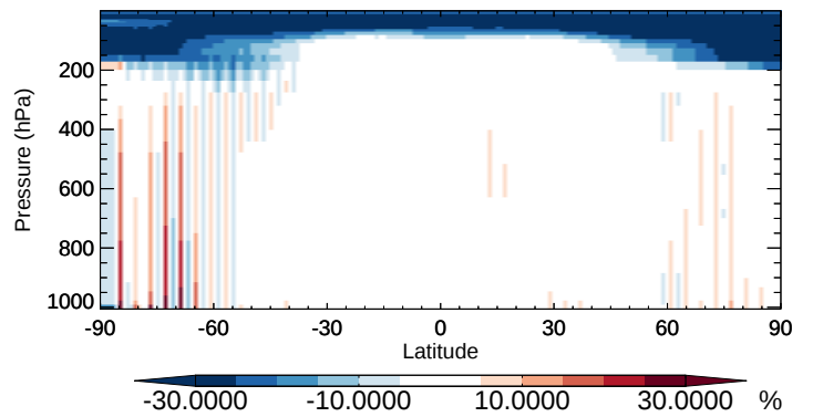
v11-02b-HP / v11-02a H 2 O - Zonal mean % diff for Oct
