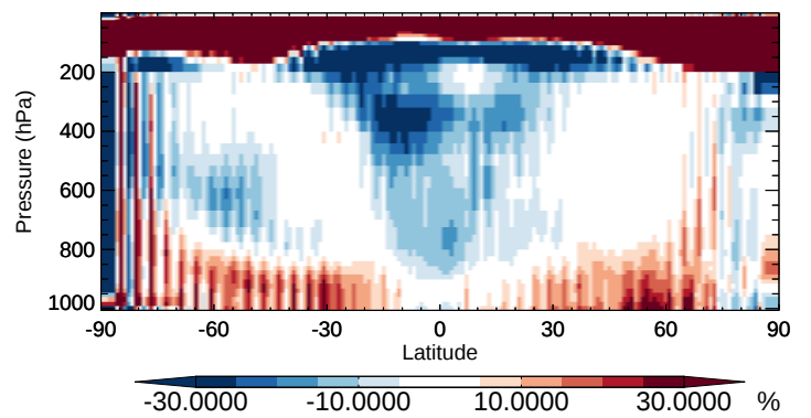
v11-02b-HP / v11-02a Br2 - Zonal mean % diff for Oct
