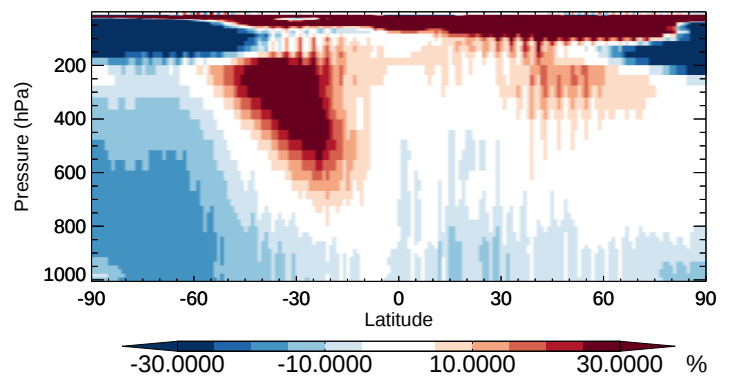
v11-02b-HP / v11-02a R4N2 - Zonal mean % diff for Oct
