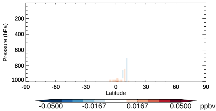
v11-02b-HP - v11-02a MVK - Zonal mean abs diff for Oct
