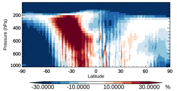
v11-02b-HP / v11-02a TSOA0 - Zonal mean % diff for Oct
