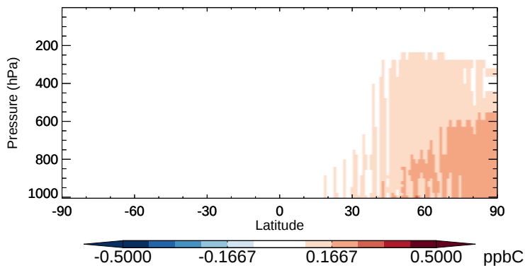
v11-02b-HP - v11-02a C2H6 - Zonal mean abs diff for Oct
