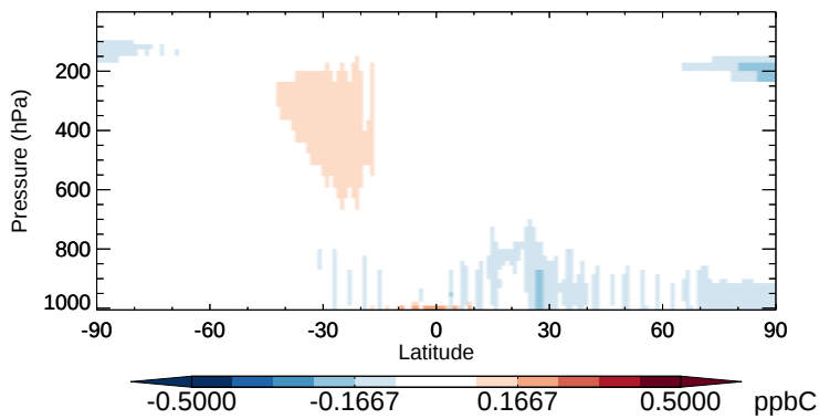
v11-02b-HP - v11-02a ACET - Zonal mean abs diff for Oct
