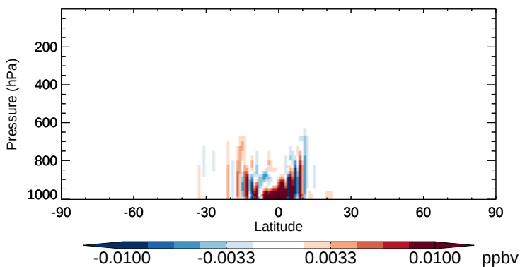
v11-02b-HP - v11-02a RIP - Zonal mean abs diff for Oct
