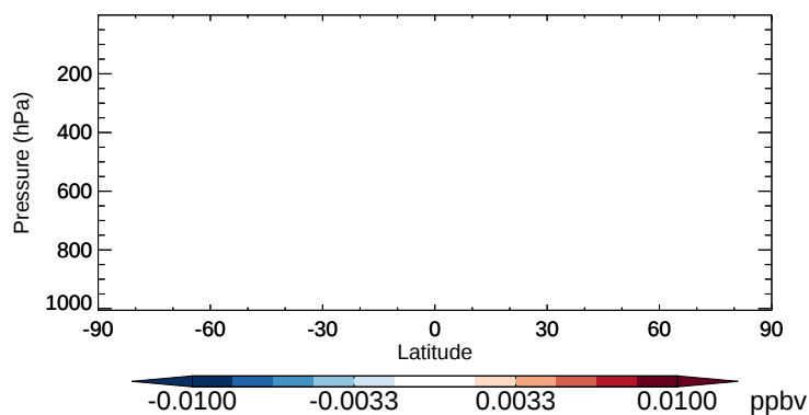
v11-02b-HP - v11-02a CH 2 Br 2 - Zonal mean abs diff for Oct
