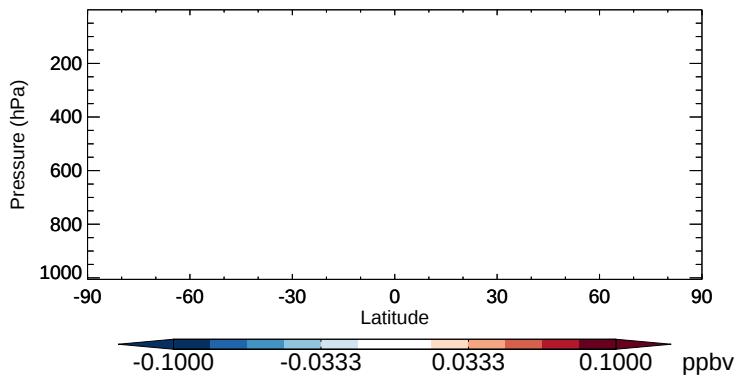
v11-02b-HP - v11-02a ISOG1 - Zonal mean abs diff for Oct
