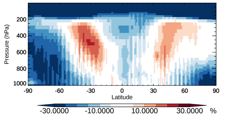
v11-02b-HP / v11-02a ASOAN - Zonal mean % diff for Oct
