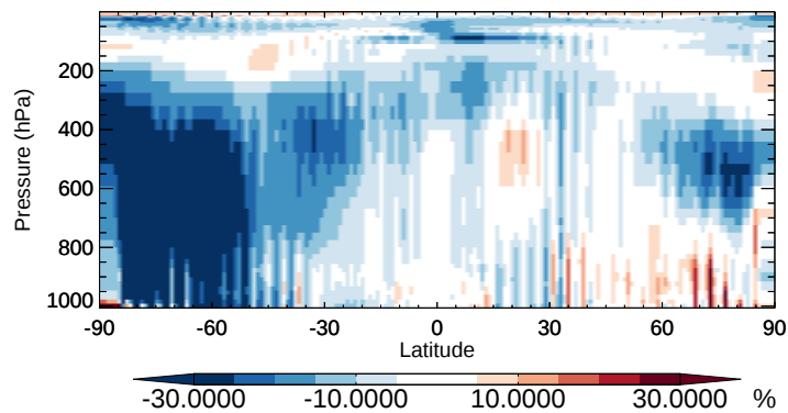
v11-02b-HP / v11-02a MPN - Zonal mean % diff for Oct
