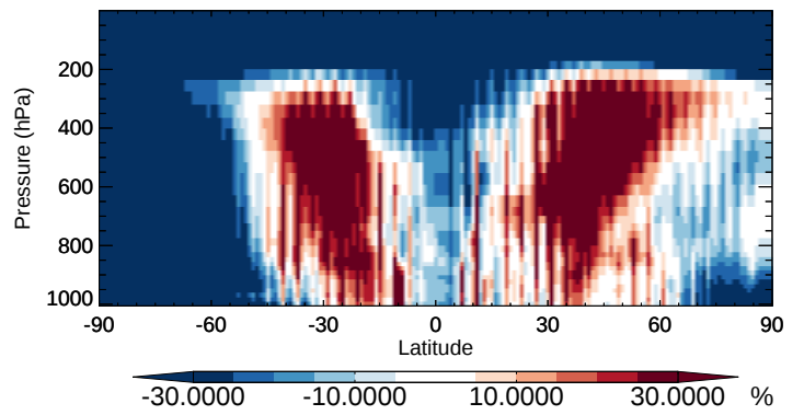
v11-02b-HP / v11-02a ASOA2 - Zonal mean % diff for Oct
