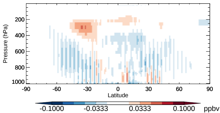
v11-02b-HP - v11-02a H 2 O 2 - Zonal mean abs diff for Oct
