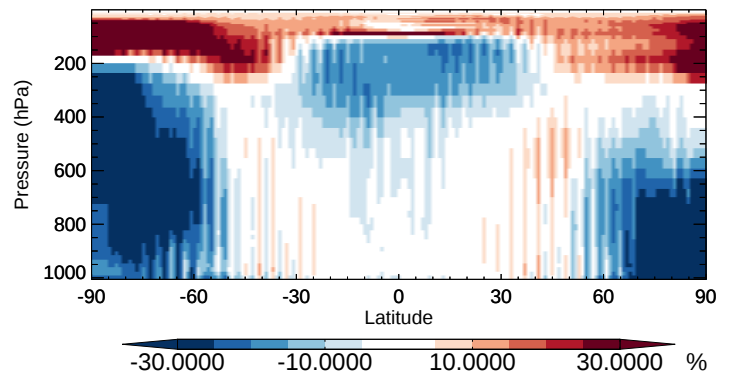
v11-02b-HP / v11-02a HCl - Zonal mean % diff for Oct
