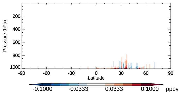
v11-02b-HP - v11-02a TOLU - Zonal mean abs diff for Oct
