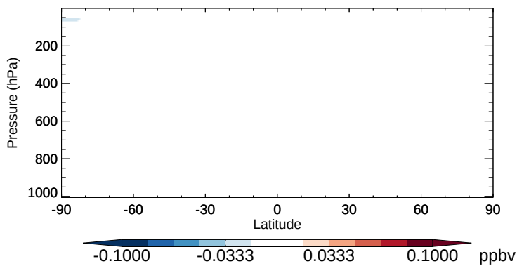
v11-02b-HP - v11-02a CFC113 - Zonal mean abs diff for Oct
