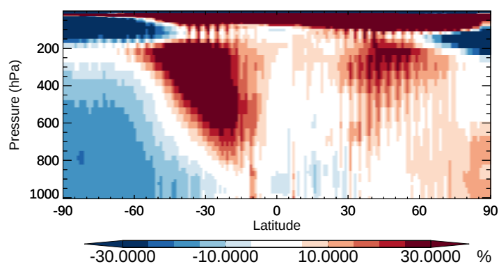
v11-02b-HP / v11-02a BENZ - Zonal mean % diff for Oct
