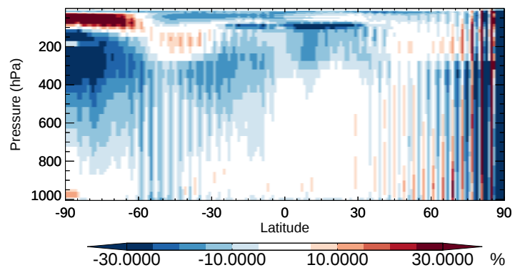
v11-02b-HP / v11-02a Cl - Zonal mean % diff for Oct
