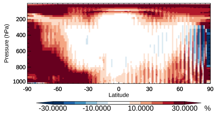
v11-02b-HP / v11-02a HBr - Zonal mean % diff for Oct
