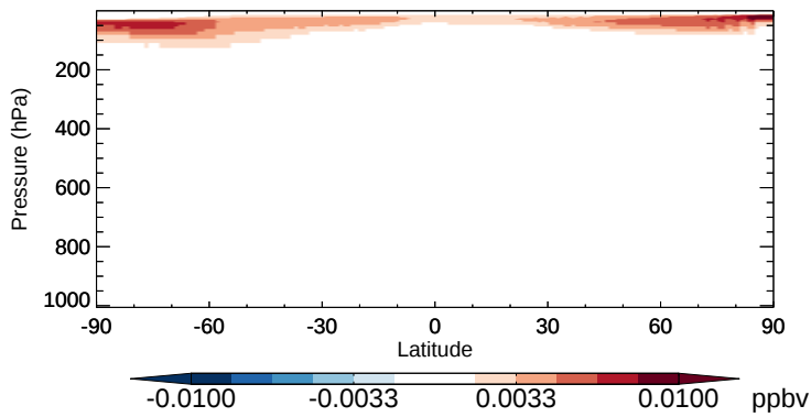
v11-02b-HP - v11-02a BrNO 3 - Zonal mean abs diff for Oct
