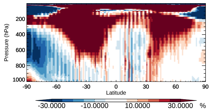
v11-02b-HP / v11-02a HAC - Zonal mean % diff for Oct
