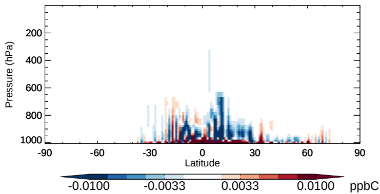
v11-02b-HP - v11-02a PRPE - Zonal mean abs diff for Oct
