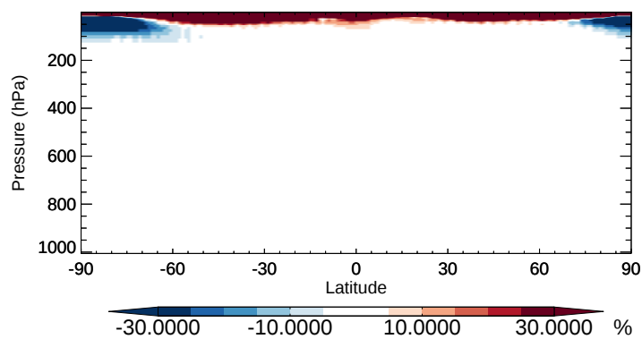
v11-02b-HP / v11-02a CH 3 Br - Zonal mean % diff for Oct
