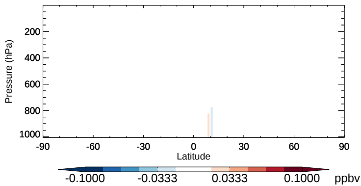
v11-02b-HP - v11-02a GLYC - Zonal mean abs diff for Oct
