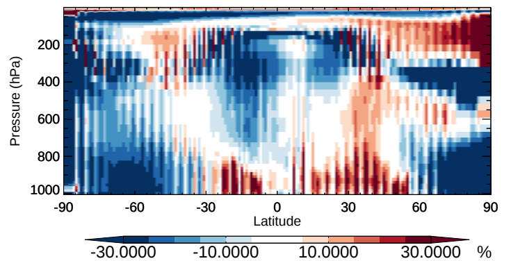
v11-02b-HP / v11-02a BrCl - Zonal mean % diff for Oct
