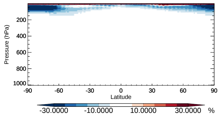
v11-02b-HP / v11-02a CFC113 - Zonal mean % diff for Oct
