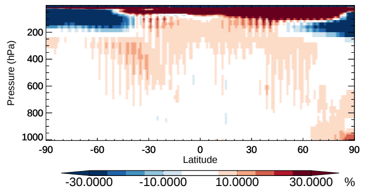
v11-02b-HP / v11-02a CHBr 3 - Zonal mean % diff for Oct
