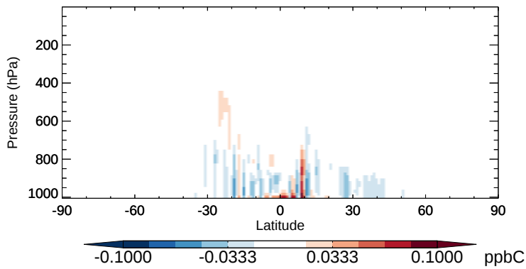
v11-02b-HP - v11-02a MEK - Zonal mean abs diff for Oct
