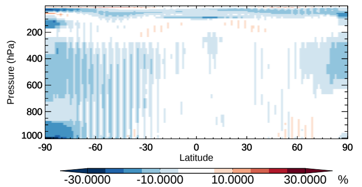
v11-02b-HP / v11-02a CH2O - Zonal mean % diff for Oct
