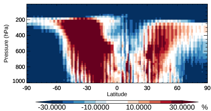
v11-02b-HP / v11-02a ISOA3 - Zonal mean % diff for Oct
