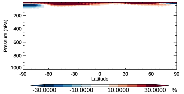
v11-02b-HP / v11-02a CFC12 - Zonal mean % diff for Oct
