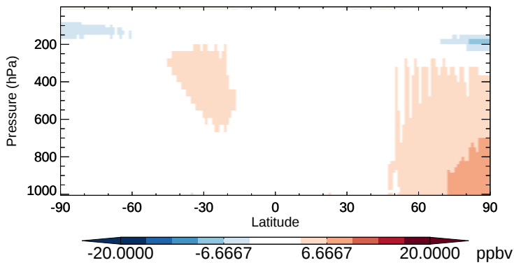
v11-02b-HP - v11-02a CO - Zonal mean abs diff for Oct
