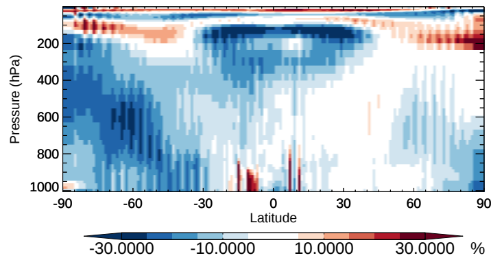
v11-02b-HP / v11-02a HOBr - Zonal mean % diff for Oct
