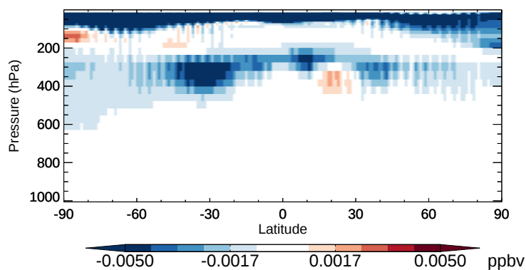
v11-02b-HP - v11-02a HNO4 - Zonal mean abs diff for Oct
