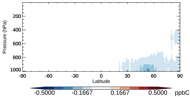
v11-02b-HP - v11-02a C3H8 - Zonal mean abs diff for Oct
