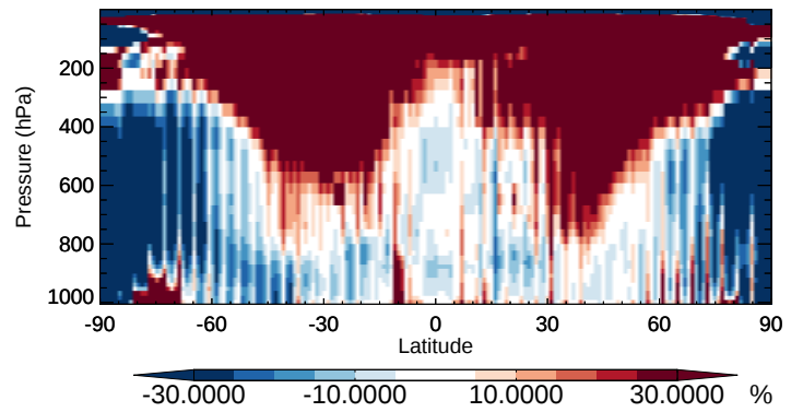
v11-02b-HP / v11-02a BCPO - Zonal mean % diff for Oct
