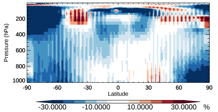
v11-02b-HP / v11-02a HOCl - Zonal mean % diff for Oct
