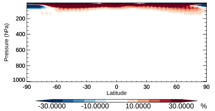
v11-02b-HP / v11-02a CH 3 CCl 3 - Zonal mean % diff for Oct
