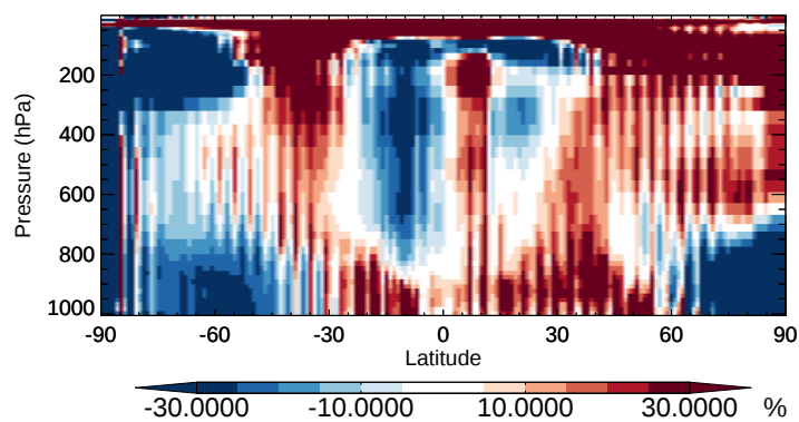
v11-02b-HP / v11-02a OCLO - Zonal mean % diff for Oct
