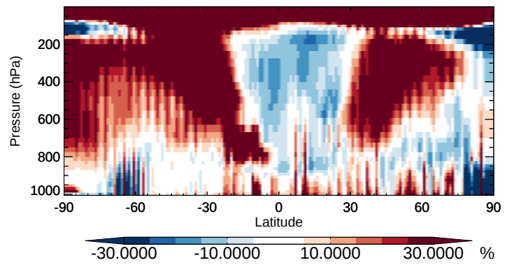
v11-02b-HP / v11-02a SALC - Zonal mean % diff for Oct
