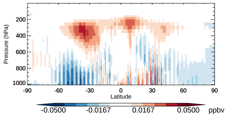
v11-02b-HP - v11-02a MP - Zonal mean abs diff for Oct
