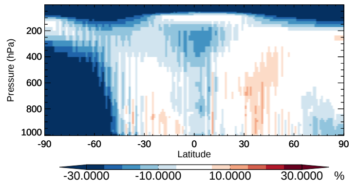
v11-02b-HP / v11-02a ASOG3 - Zonal mean % diff for Oct
