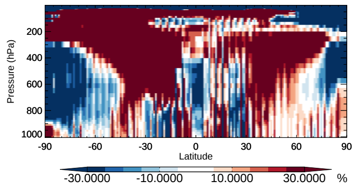
v11-02b-HP / v11-02a PMN - Zonal mean % diff for Oct
