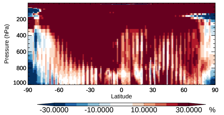
v11-02b-HP / v11-02a DMS - Zonal mean % diff for Oct
