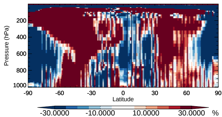
v11-02b-HP / v11-02a MOBA - Zonal mean % diff for Oct
