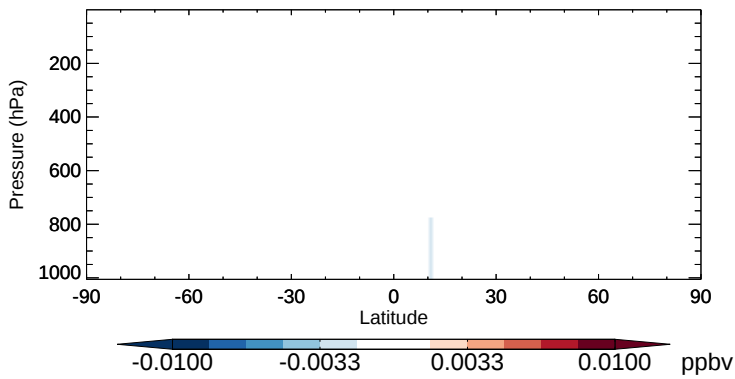
v11-02b-HP - v11-02a MVKN - Zonal mean abs diff for Oct
