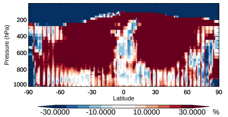
v11-02b-HP / v11-02a NH 3 - Zonal mean % diff for Oct
