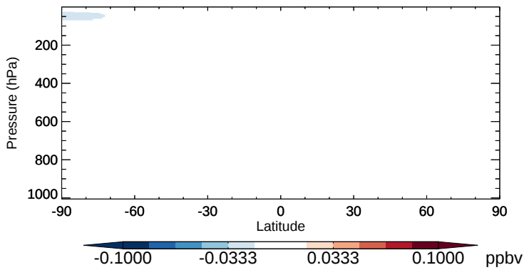
v11-02b-HP - v11-02a HCFC22 - Zonal mean abs diff for Oct
