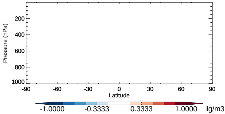
v11-02b-HP - v11-02a BCPI - Zonal mean abs diff for Oct
