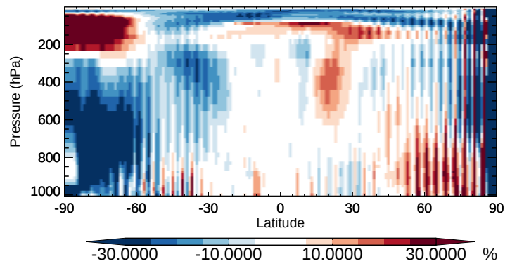
v11-02b-HP / v11-02a NO - Zonal mean % diff for Oct
