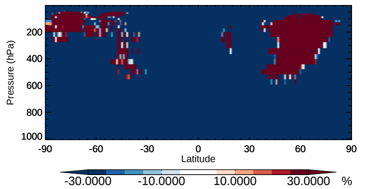
v11-02b-HP / v11-02a ClNO2 - Zonal mean % diff for Oct
