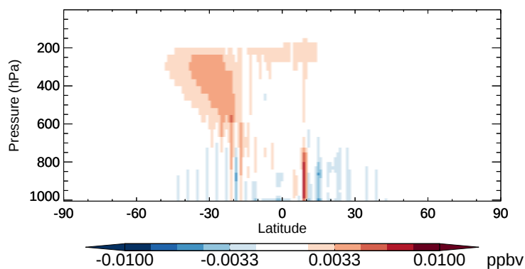
v11-02b-HP - v11-02a MAP - Zonal mean abs diff for Oct
