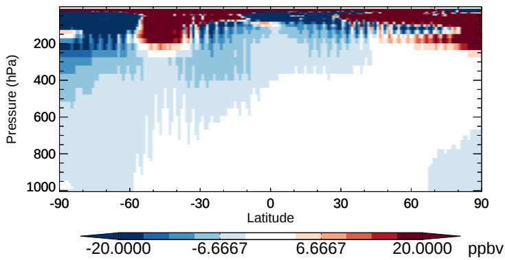
v11-02b-HP - v11-02a O3 - Zonal mean abs diff for Oct
