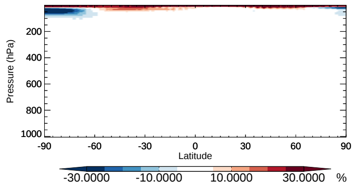
v11-02b-HP / v11-02a N 2 O - Zonal mean % diff for Oct
