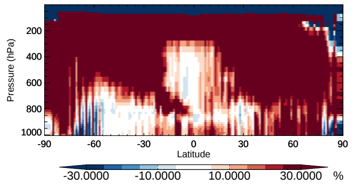
v11-02b-HP / v11-02a SO 4 s - Zonal mean % diff for Oct
