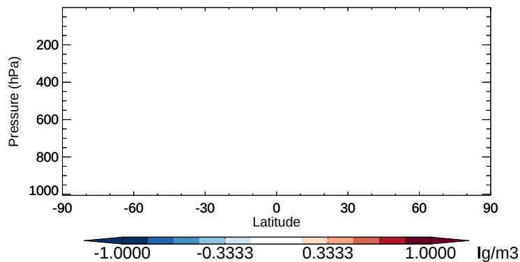
v11-02b-HP - v11-02a NITs - Zonal mean abs diff for Oct
