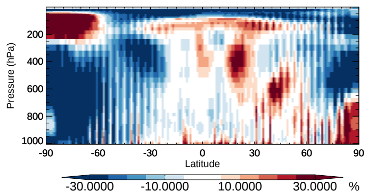
v11-02b-HP / v11-02a HNO 2 - Zonal mean % diff for Oct
