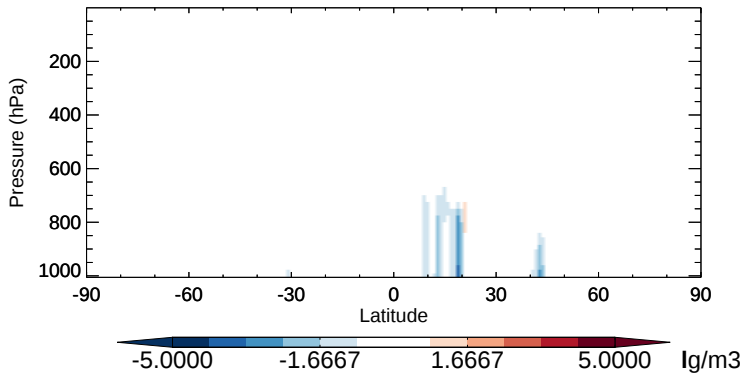
v11-02b-HP - v11-02a DST3 - Zonal mean abs diff for Oct
