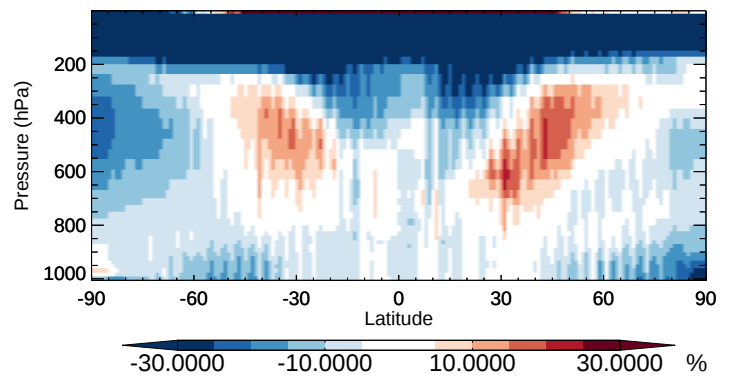
v11-02b-HP / v11-02a SO 4 - Zonal mean % diff for Oct
