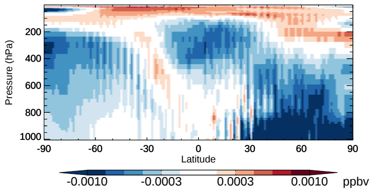
v11-02b-HP - v11-02a PPN - Zonal mean abs diff for Oct
