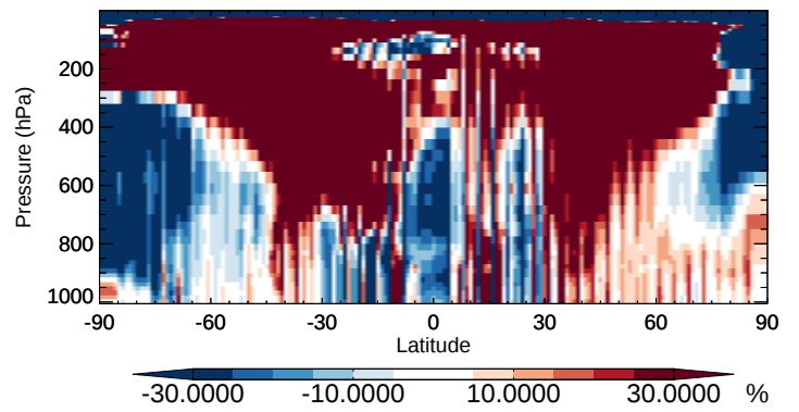
v11-02b-HP / v11-02a MVK - Zonal mean % diff for Oct
