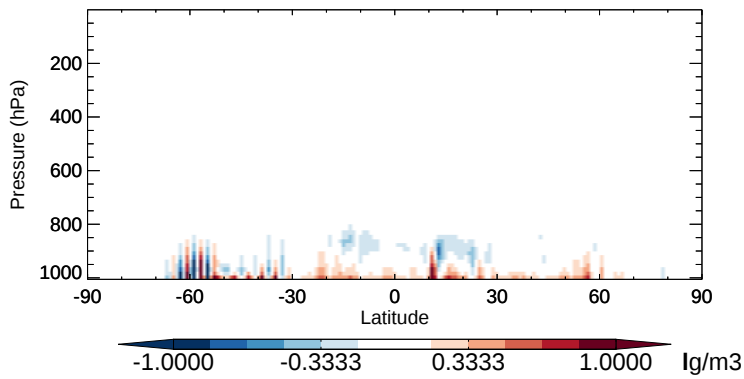
v11-02b-HP - v11-02a SALC - Zonal mean abs diff for Oct
