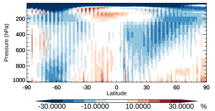
v11-02b-HP / v11-02a TSOG0 - Zonal mean % diff for Oct
