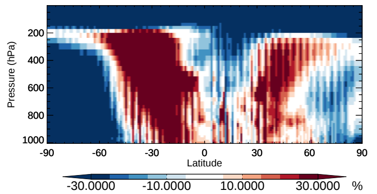
v11-02b-HP / v11-02a TSOA3 - Zonal mean % diff for Oct
