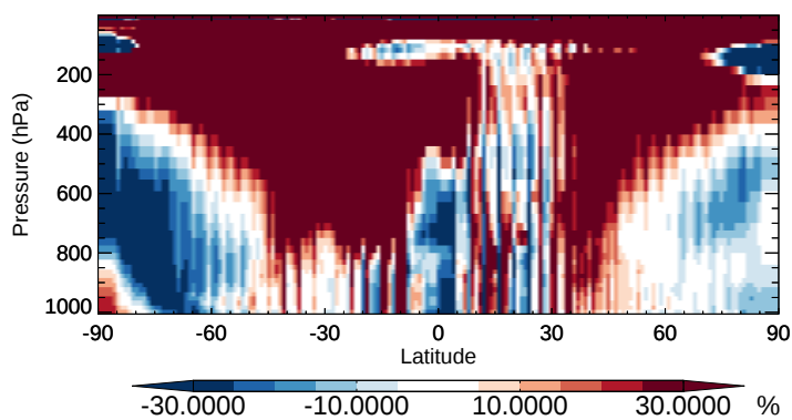
v11-02b-HP / v11-02a IEPOX - Zonal mean % diff for Oct
