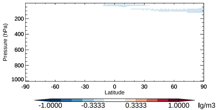
v11-02b-HP - v11-02a SO 4 - Zonal mean abs diff for Oct
