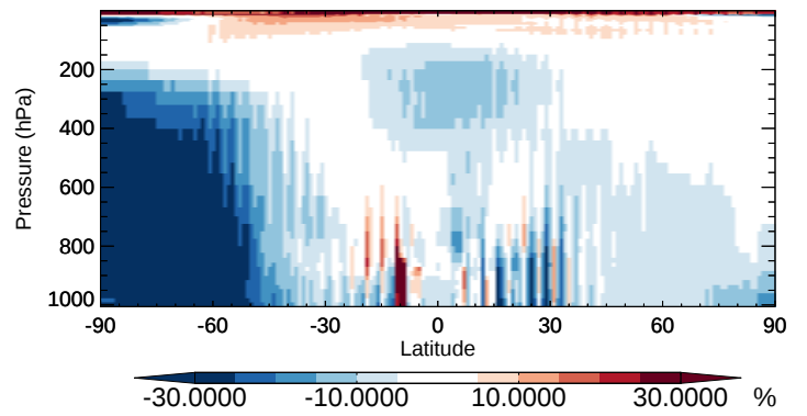
v11-02b-HP / v11-02a PPN - Zonal mean % diff for Oct
