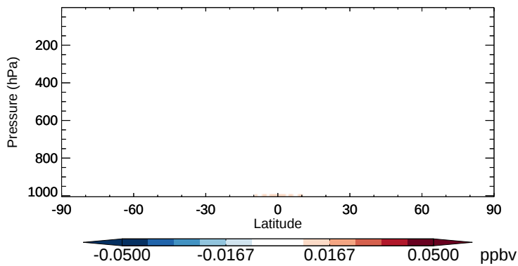
v11-02b-HP - v11-02a RCHO - Zonal mean abs diff for Oct
