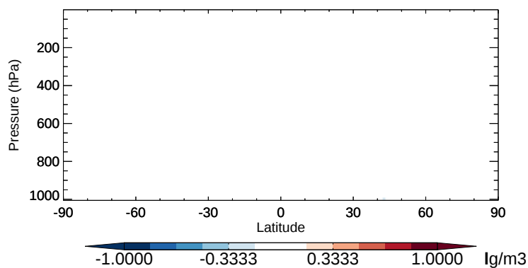
v11-02b-HP - v11-02a NH4 - Zonal mean abs diff for Oct
