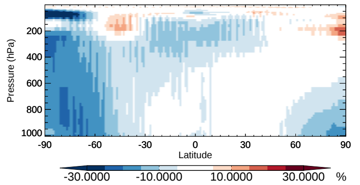
v11-02b-HP / v11-02a O3 - Zonal mean % diff for Oct
