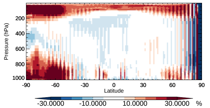
v11-02b-HP / v11-02a Br - Zonal mean % diff for Oct
