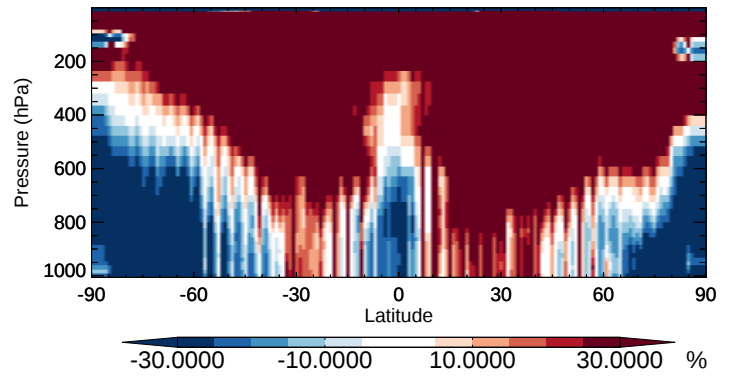
v11-02b-HP / v11-02a DST3 - Zonal mean % diff for Oct
