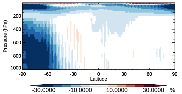
v11-02b-HP / v11-02a EOH - Zonal mean % diff for Oct
