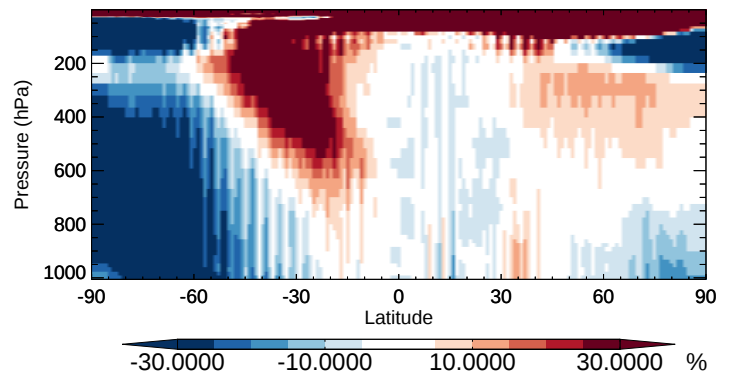
v11-02b-HP / v11-02a PROPNN - Zonal mean % diff for Oct
