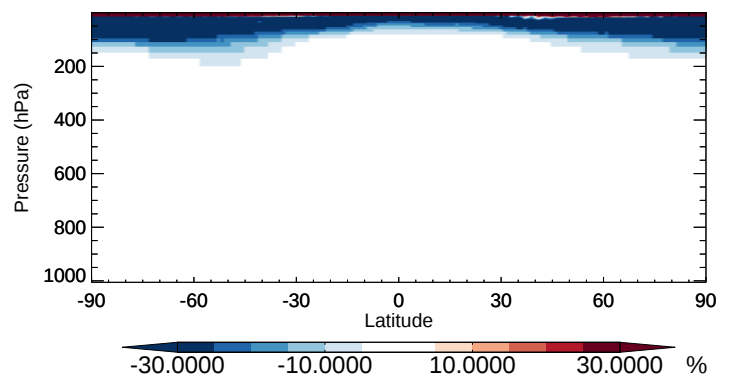
v11-02b-HP / v11-02a HCFC141b - Zonal mean % diff for Oct
