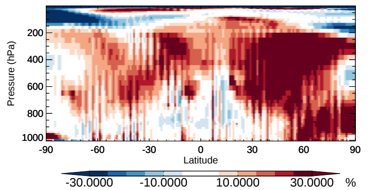
v11-02b-HP / v11-02a SO 2 - Zonal mean % diff for Oct
