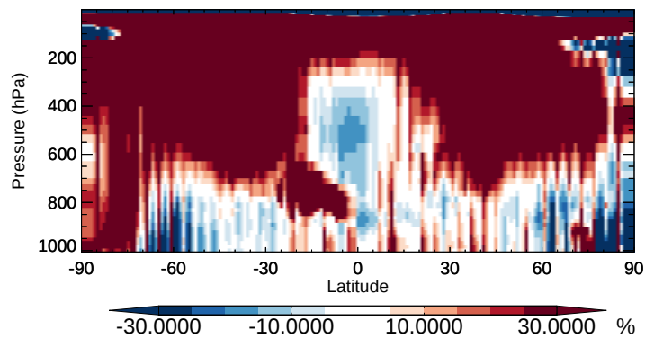
v11-02b-HP / v11-02a NITs - Zonal mean % diff for Oct
