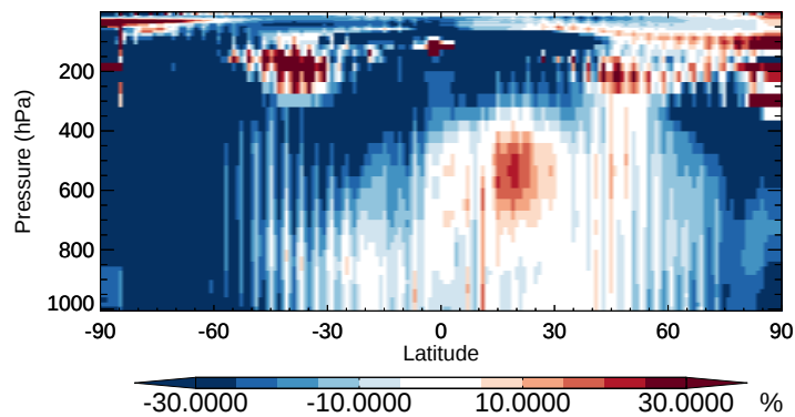
v11-02b-HP / v11-02a Cl2 - Zonal mean % diff for Oct
