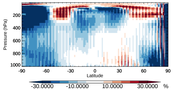
v11-02b-HP / v11-02a ClO - Zonal mean % diff for Oct
