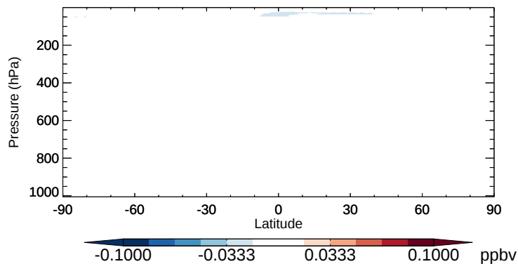
v11-02b-HP - v11-02a MPN - Zonal mean abs diff for Oct
