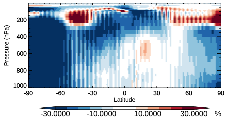
v11-02b-HP / v11-02a ClNO3 - Zonal mean % diff for Oct
