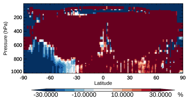
v11-02b-HP / v11-02a NIT - Zonal mean % diff for Oct
