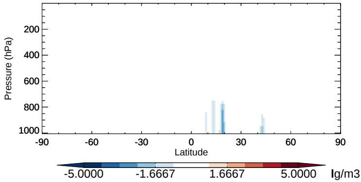
v11-02b-HP - v11-02a DST4 - Zonal mean abs diff for Oct
