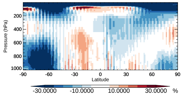
v11-02b-HP / v11-02a ISOG1 - Zonal mean % diff for Oct
