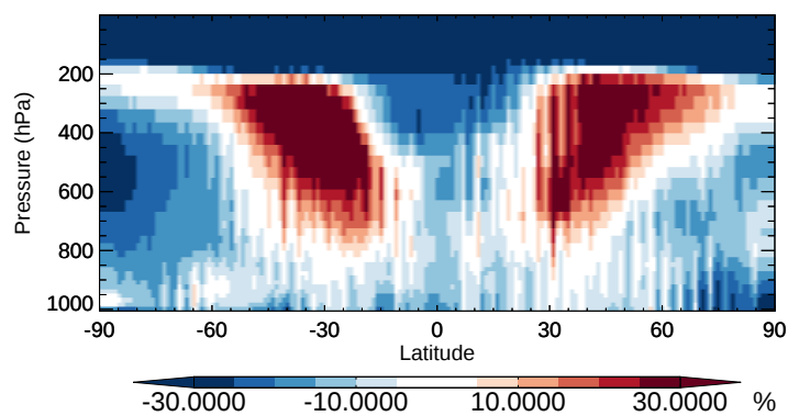
v11-02b-HP / v11-02a NH4 - Zonal mean % diff for Oct
