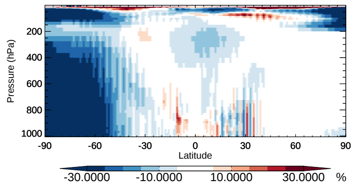
v11-02b-HP / v11-02a PAN - Zonal mean % diff for Oct
