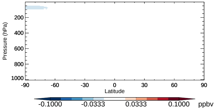
v11-02b-HP - v11-02a CFC11 - Zonal mean abs diff for Oct
