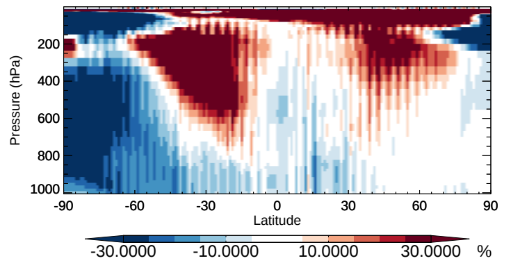
v11-02b-HP / v11-02a MEK - Zonal mean % diff for Oct
