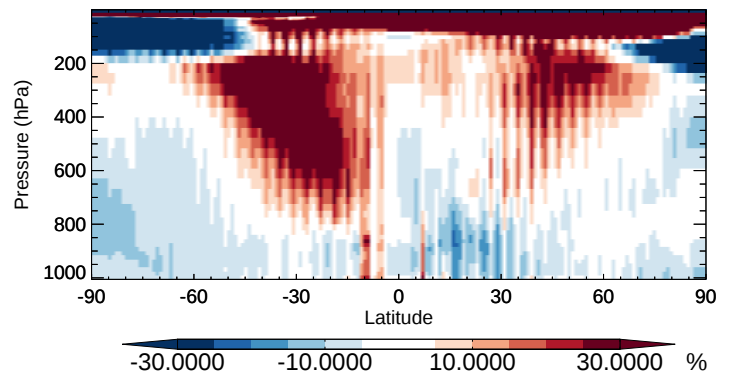
v11-02b-HP / v11-02a ALK4 - Zonal mean % diff for Oct
