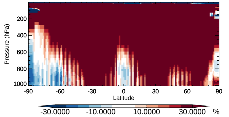
v11-02b-HP / v11-02a DST4 - Zonal mean % diff for Oct
