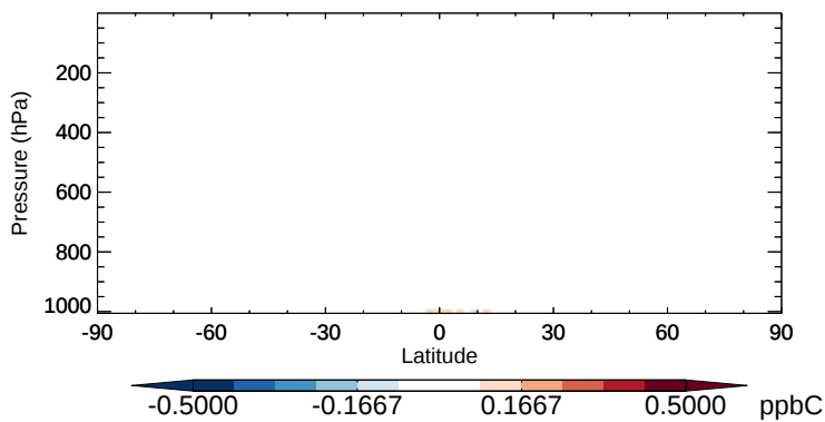
v11-02b-HP - v11-02a ALD2 - Zonal mean abs diff for Oct
