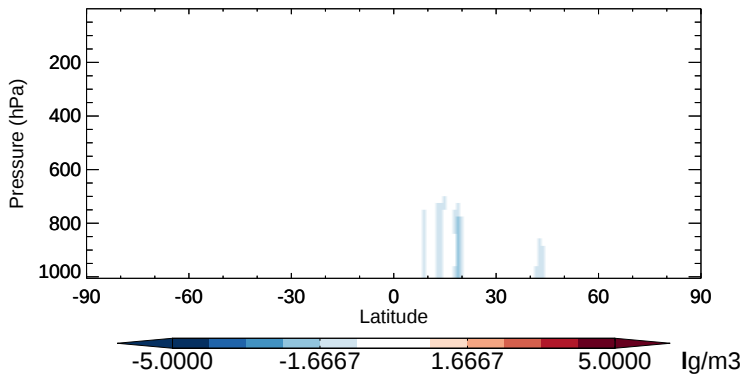
v11-02b-HP - v11-02a DST2 - Zonal mean abs diff for Oct
