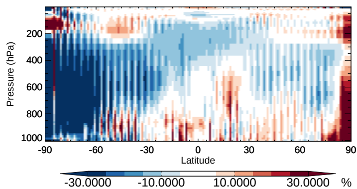
v11-02b-HP / v11-02a NO 3 - Zonal mean % diff for Oct
