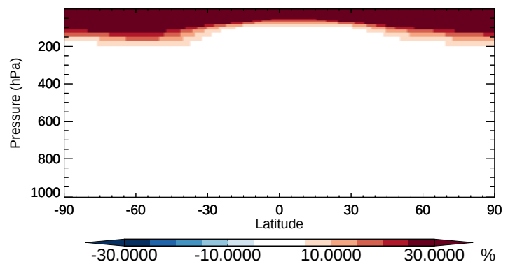
v11-02b-HP / v11-02a CFC114 - Zonal mean % diff for Oct
