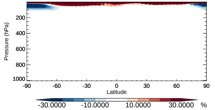
v11-02b-HP / v11-02a CFC11 - Zonal mean % diff for Oct
