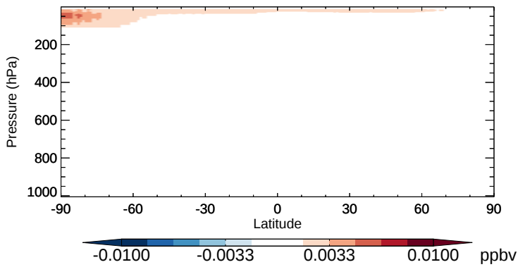
v11-02b-HP - v11-02a BrO - Zonal mean abs diff for Oct
