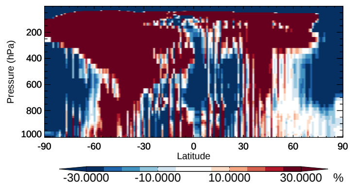
v11-02b-HP / v11-02a RIP - Zonal mean % diff for Oct
