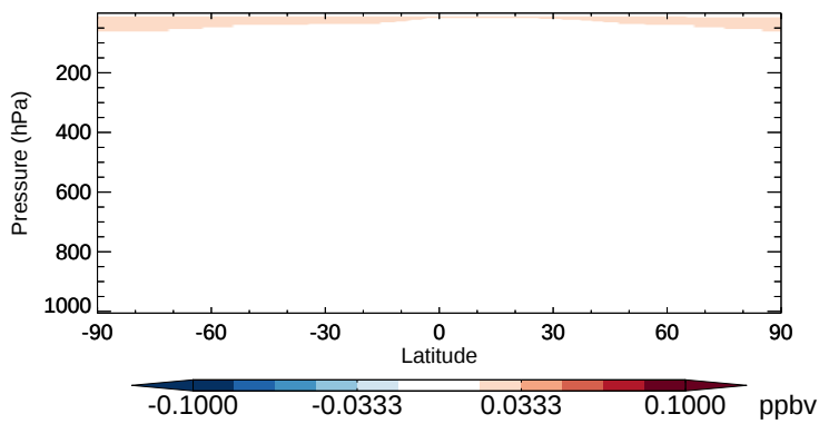
v11-02b-HP - v11-02a CFC115 - Zonal mean abs diff for Oct
