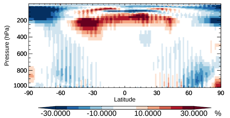
v11-02b-HP / v11-02a H 2 O 2 - Zonal mean % diff for Oct
