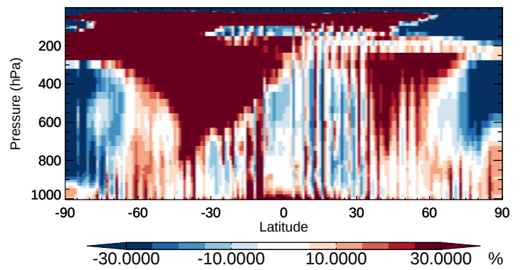
v11-02b-HP / v11-02a PRPE - Zonal mean % diff for Oct
