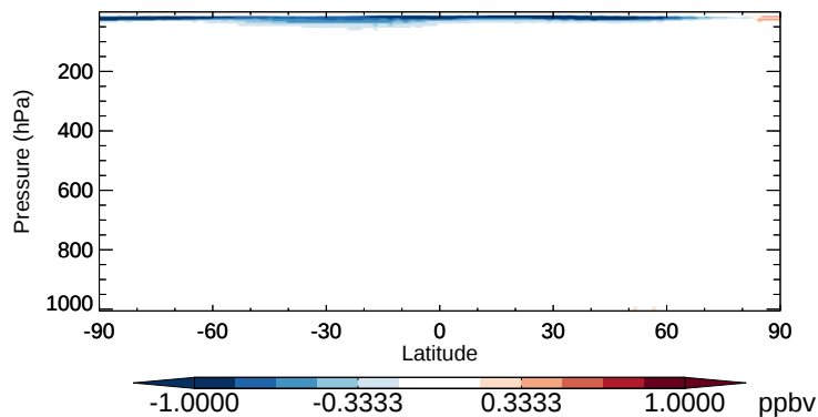
v11-02b-HP - v11-02a NO2 - Zonal mean abs diff for Oct
