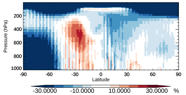
v11-02b-HP / v11-02a TSOG2 - Zonal mean % diff for Oct
