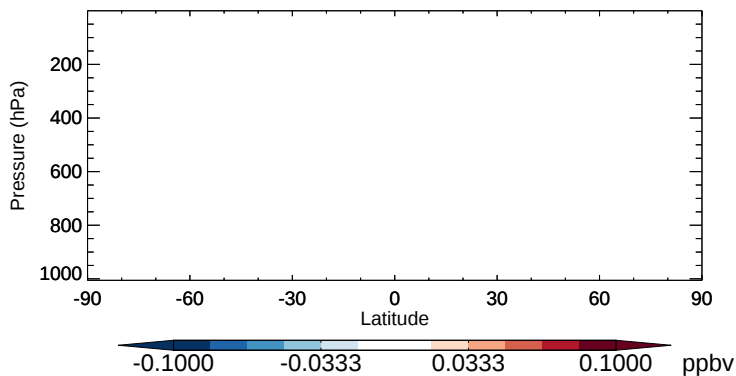
v11-02b-HP - v11-02a BrCl - Zonal mean abs diff for Oct
