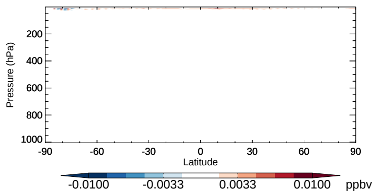
v11-02b-HP - v11-02a NO 3 - Zonal mean abs diff for Oct
