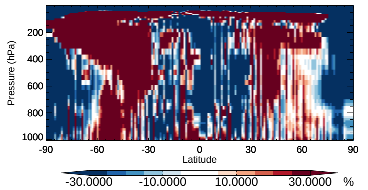
v11-02b-HP / v11-02a ISOP - Zonal mean % diff for Oct
