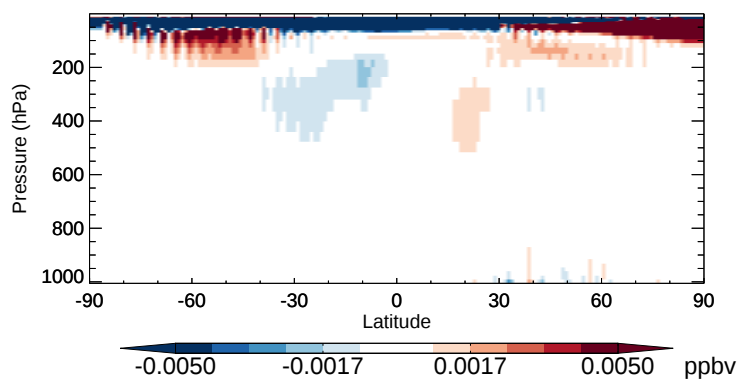
v11-02b-HP - v11-02a N2O5 - Zonal mean abs diff for Oct
