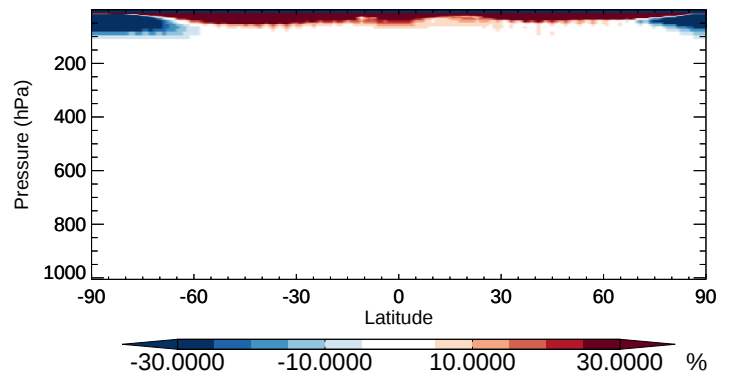
v11-02b-HP / v11-02a H2402 - Zonal mean % diff for Oct
