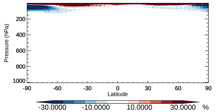
v11-02b-HP / v11-02a H1301 - Zonal mean % diff for Oct
