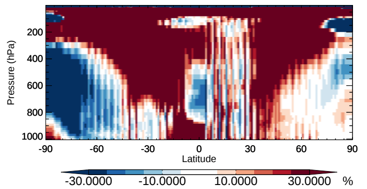
v11-02b-HP / v11-02a GLYC - Zonal mean % diff for Oct
