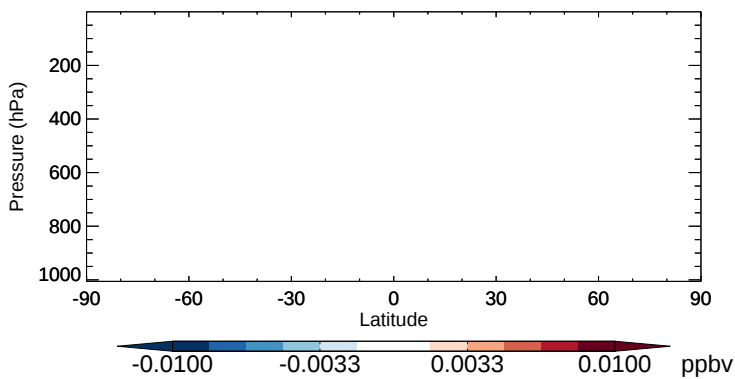
v11-02b-HP - v11-02a MACRN - Zonal mean abs diff for Oct
