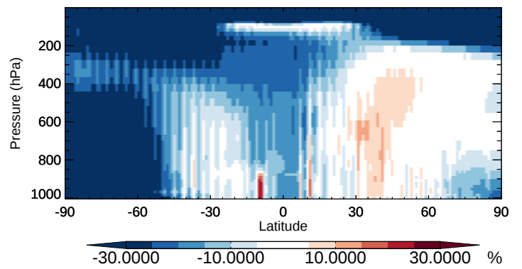
v11-02b-HP / v11-02a ASOG2 - Zonal mean % diff for Oct
