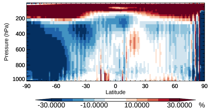
v11-02b-HP / v11-02a BrNO 3 - Zonal mean % diff for Oct
