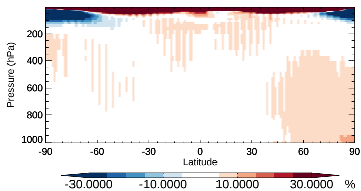
v11-02b-HP / v11-02a CH 2 Br 2 - Zonal mean % diff for Oct
