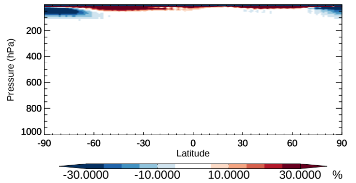
v11-02b-HP / v11-02a OCS - Zonal mean % diff for Oct
