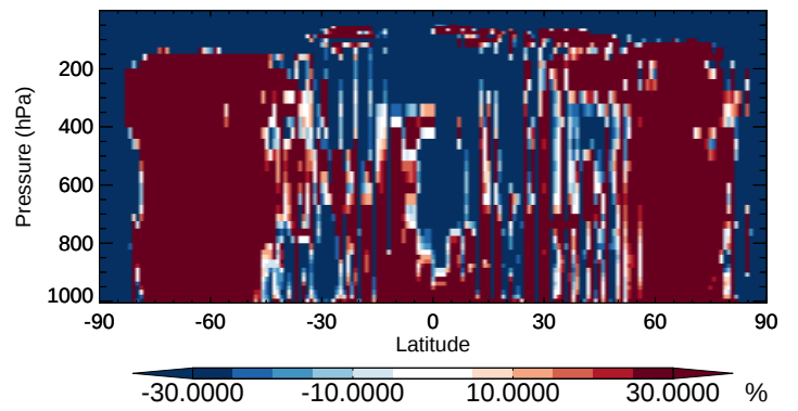
v11-02b-HP / v11-02a LIMO - Zonal mean % diff for Oct
