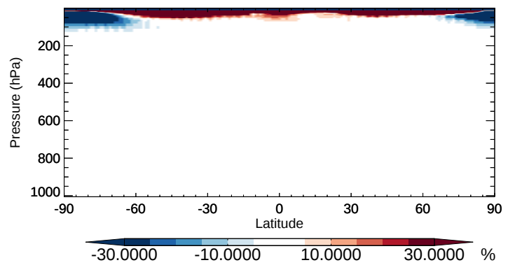
v11-02b-HP / v11-02a H1211 - Zonal mean % diff for Oct
