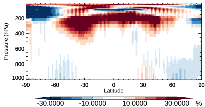
v11-02b-HP / v11-02a MP - Zonal mean % diff for Oct
