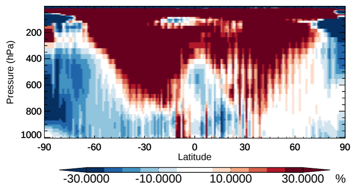
v11-02b-HP / v11-02a TOLU - Zonal mean % diff for Oct
