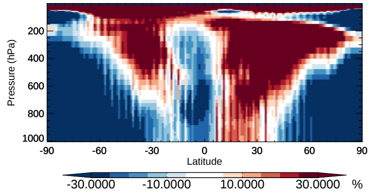
v11-02b-HP / v11-02a DST1 - Zonal mean % diff for Oct
