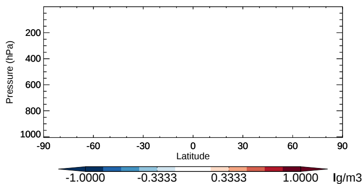
v11-02b-HP - v11-02a NIT - Zonal mean abs diff for Oct
