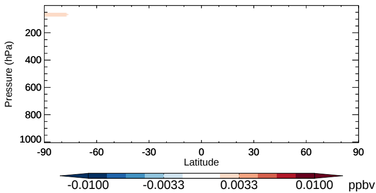
v11-02b-HP - v11-02a HBr - Zonal mean abs diff for Oct
