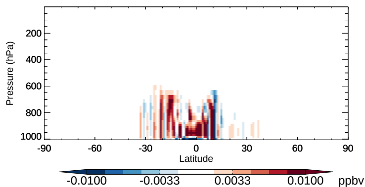
v11-02b-HP - v11-02a IEPOX - Zonal mean abs diff for Oct
