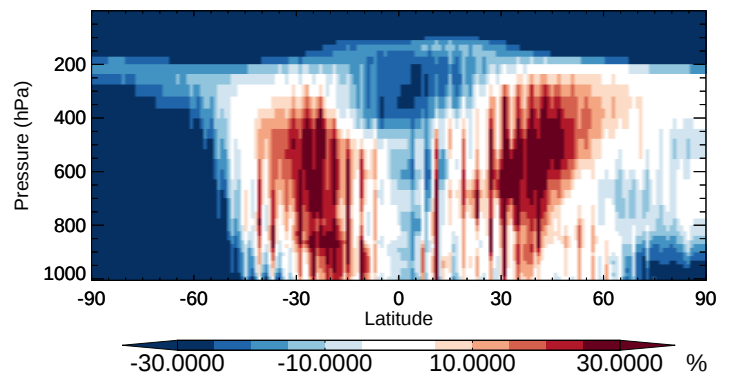
v11-02b-HP / v11-02a ASOA1 - Zonal mean % diff for Oct
