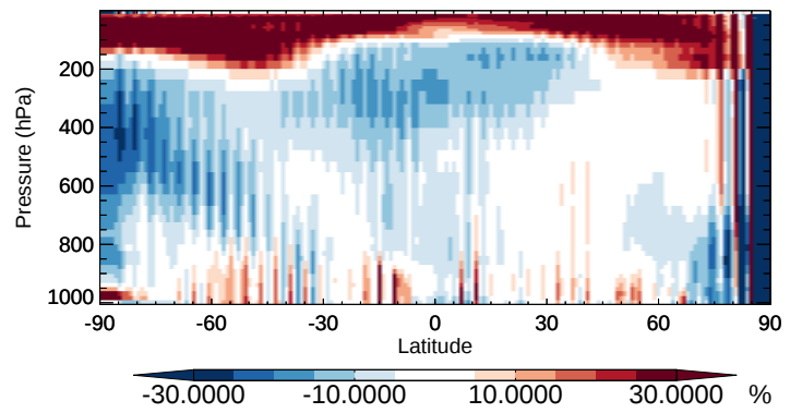
v11-02b-HP / v11-02a BrO - Zonal mean % diff for Oct
