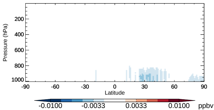
v11-02b-HP - v11-02a R4N2 - Zonal mean abs diff for Oct
