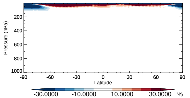
v11-02b-HP / v11-02a CCl4 - Zonal mean % diff for Oct
