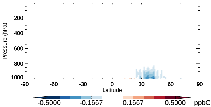
v11-02b-HP - v11-02a ALK4 - Zonal mean abs diff for Oct
