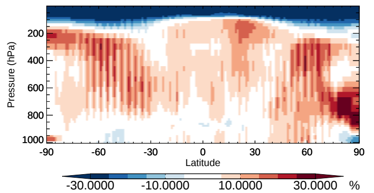
v11-02b-HP / v11-02a MSA - Zonal mean % diff for Oct
