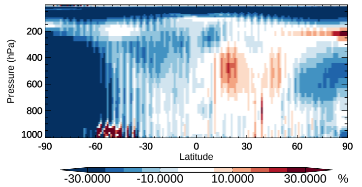
v11-02b-HP / v11-02a HNO 3 - Zonal mean % diff for Oct
