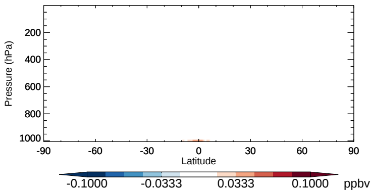
v11-02b-HP - v11-02a MTPA - Zonal mean abs diff for Oct
