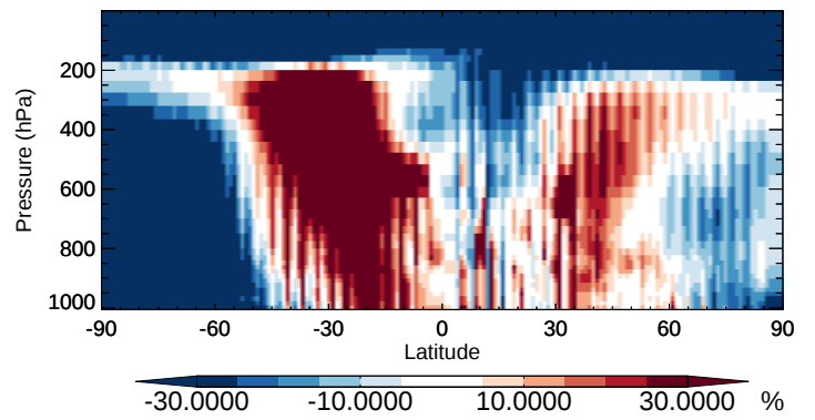
v11-02b-HP / v11-02a TSOA2 - Zonal mean % diff for Oct
