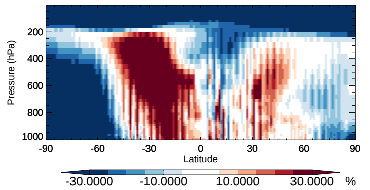
v11-02b-HP / v11-02a TSOA1 - Zonal mean % diff for Oct
