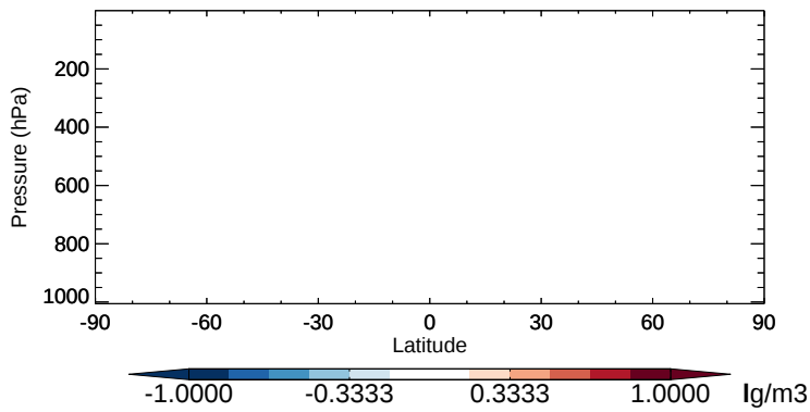
v11-02b-HP - v11-02a SO 4 s - Zonal mean abs diff for Oct
