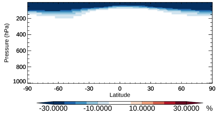
v11-02b-HP / v11-02a HCFC142b - Zonal mean % diff for Oct
