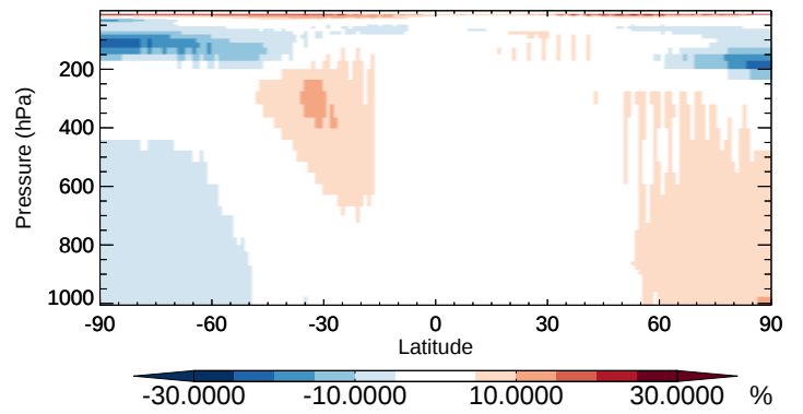
v11-02b-HP / v11-02a CO - Zonal mean % diff for Oct
