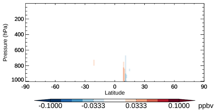
v11-02b-HP - v11-02a HAC - Zonal mean abs diff for Oct
