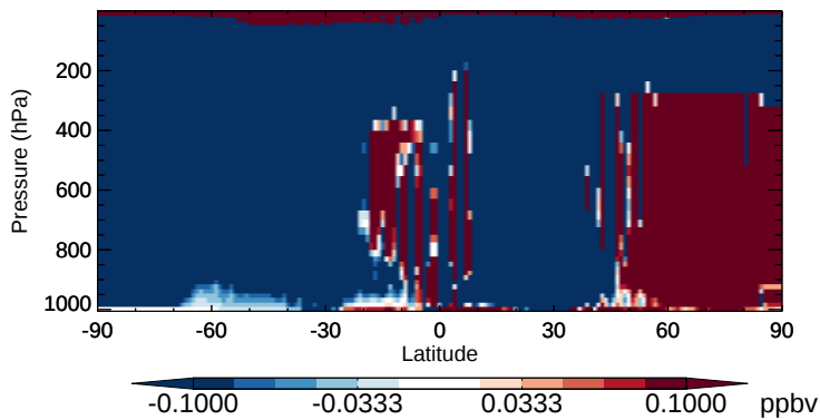
v11-02b-HP - v11-02a CH4 - Zonal mean abs diff for Oct
