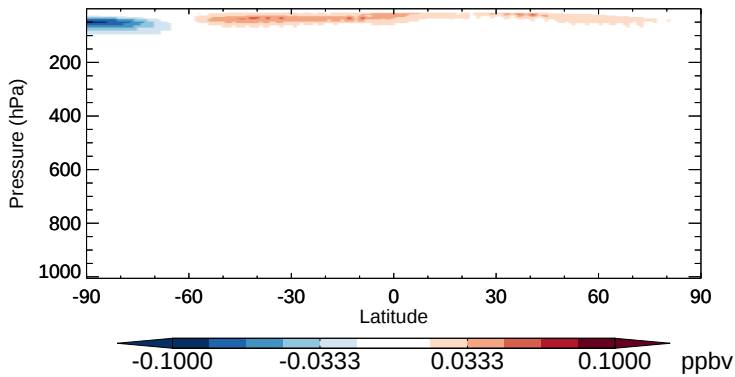
v11-02b-HP - v11-02a CFC12 - Zonal mean abs diff for Oct
