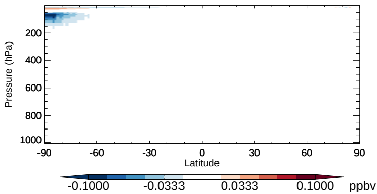
v11-02b-HP - v11-02a ClO - Zonal mean abs diff for Oct
