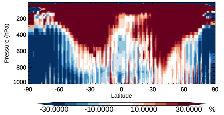
v11-02b-HP / v11-02a OCPO - Zonal mean % diff for Oct
