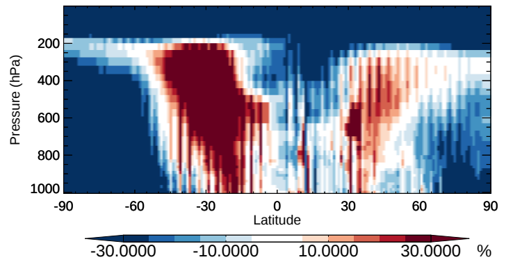
v11-02b-HP / v11-02a ISOA2 - Zonal mean % diff for Oct
