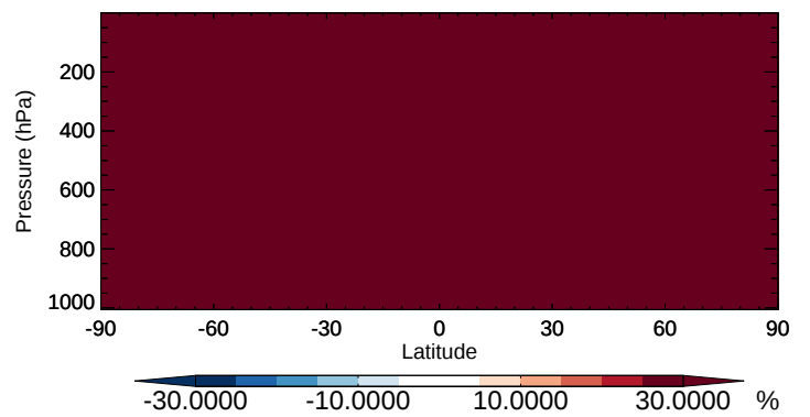
v11-02b-HP / v11-02a HCFC123 - Zonal mean % diff for Oct
