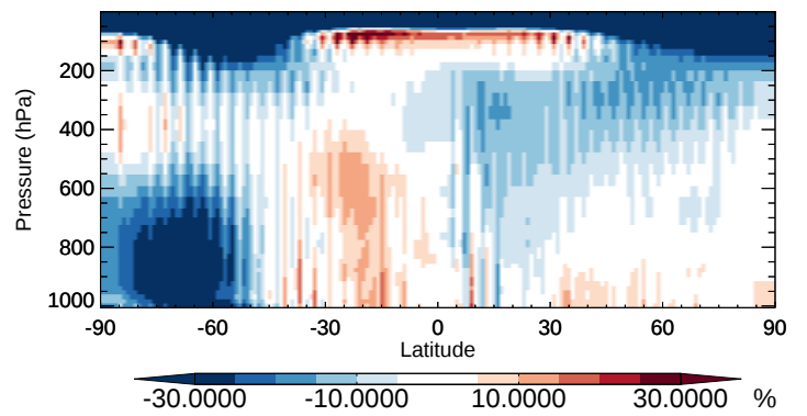
v11-02b-HP / v11-02a TSOG1 - Zonal mean % diff for Oct
