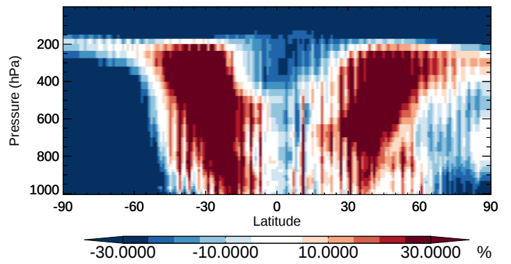
v11-02b-HP / v11-02a ASOA3 - Zonal mean % diff for Oct
