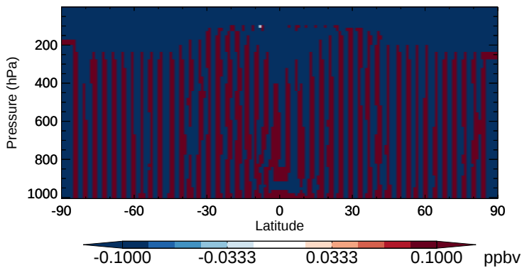
v11-02b-HP - v11-02a H 2 O - Zonal mean abs diff for Oct
