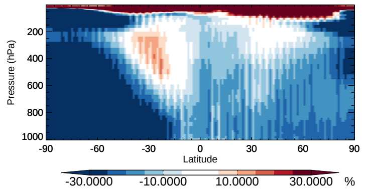
v11-02b-HP / v11-02a C3H8 - Zonal mean % diff for Oct
