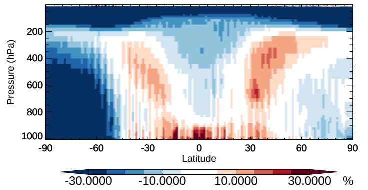
v11-02b-HP / v11-02a MGLY - Zonal mean % diff for Oct
