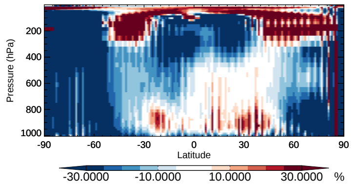
v11-02b-HP / v11-02a Cl 2 O 2 - Zonal mean % diff for Oct
