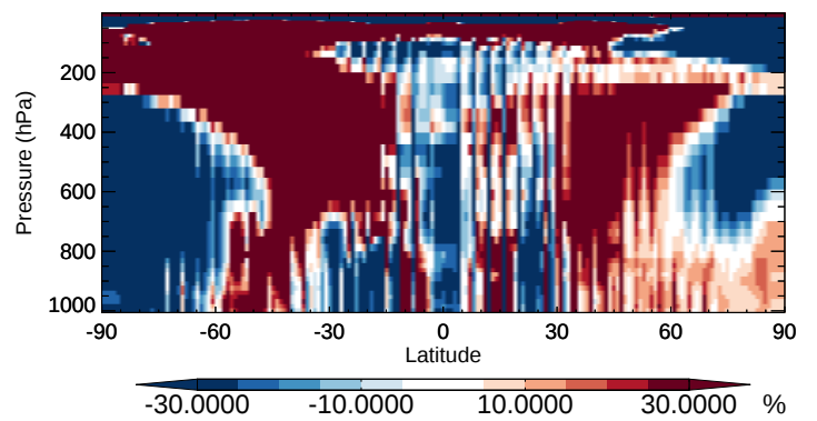
v11-02b-HP / v11-02a MACRN - Zonal mean % diff for Oct
