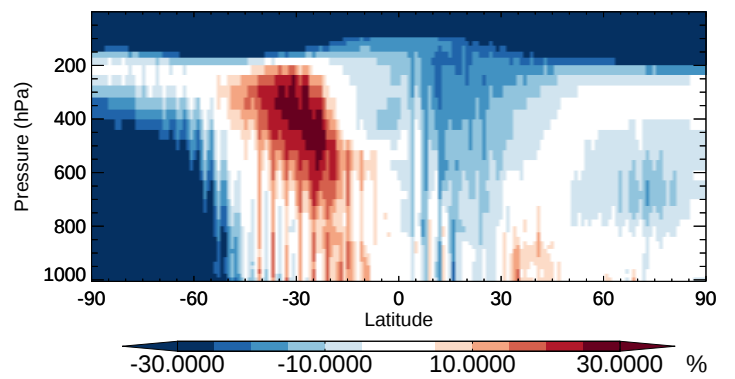
v11-02b-HP / v11-02a TSOG3 - Zonal mean % diff for Oct
