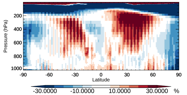
v11-02b-HP / v11-02a SALA - Zonal mean % diff for Oct
