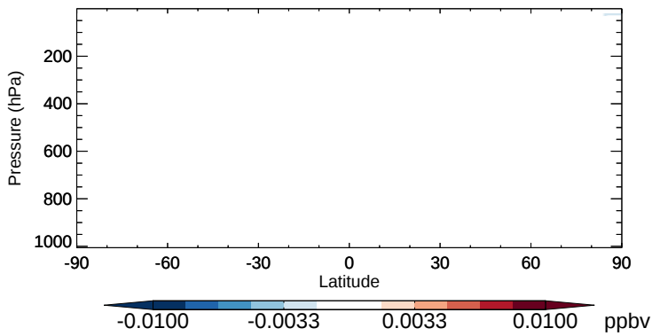
v11-02b-HP - v11-02a HOBr - Zonal mean abs diff for Oct
