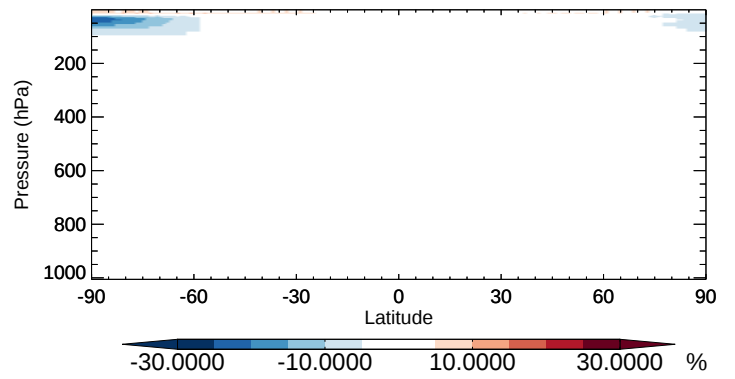
v11-02b-HP / v11-02a HCFC22 - Zonal mean % diff for Oct
