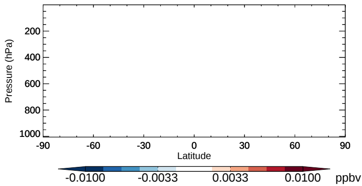
v11-02b-HP - v11-02a BrNO 2 - Zonal mean abs diff for Oct
