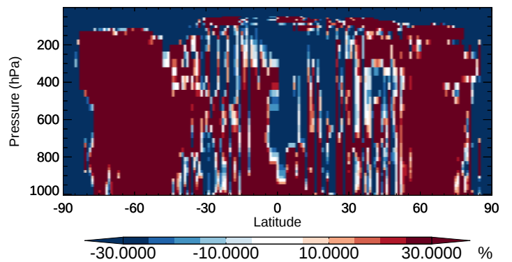
v11-02b-HP / v11-02a MTPA - Zonal mean % diff for Oct
