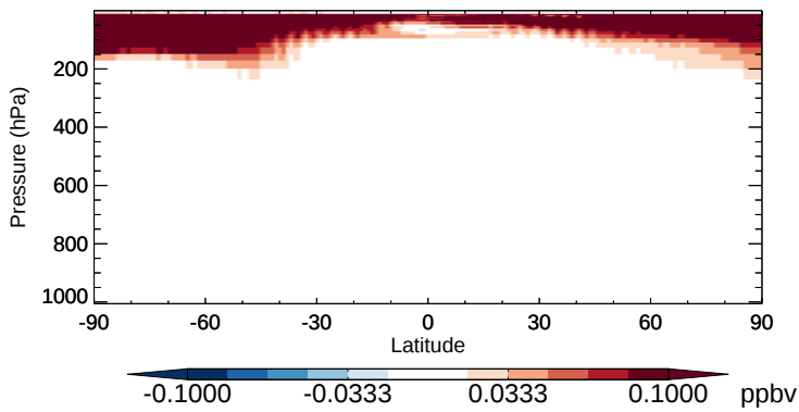
v11-02b-HP - v11-02a HCl - Zonal mean abs diff for Oct
