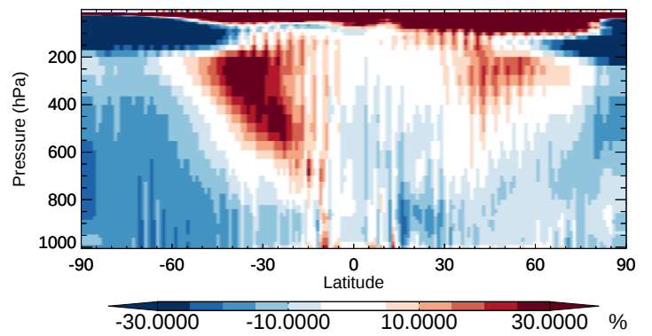
v11-02b-HP / v11-02a RCHO - Zonal mean % diff for Oct
