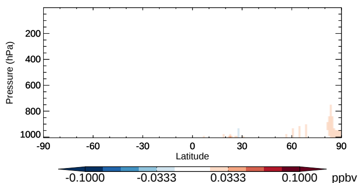
v11-02b-HP - v11-02a BENZ - Zonal mean abs diff for Oct
