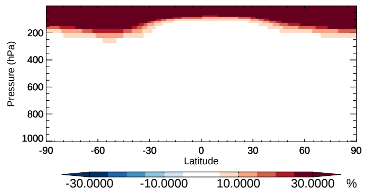
v11-02b-HP / v11-02a CFC115 - Zonal mean % diff for Oct
