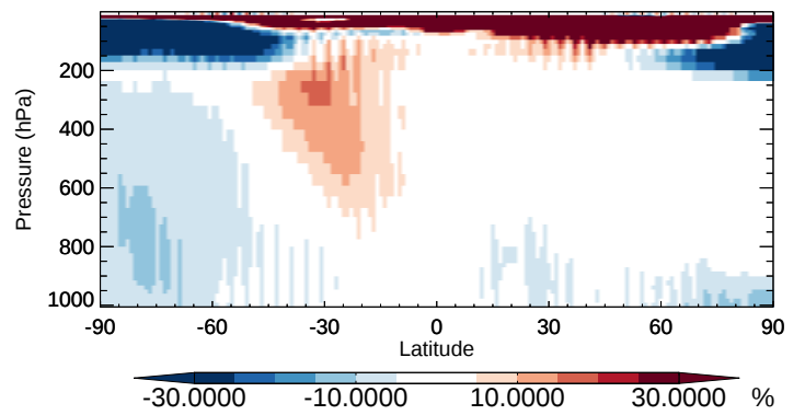
v11-02b-HP / v11-02a ACET - Zonal mean % diff for Oct
