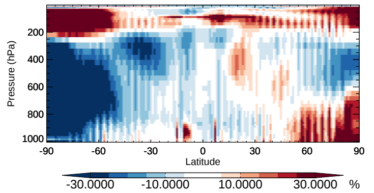
v11-02b-HP / v11-02a BrNO 2 - Zonal mean % diff for Oct
