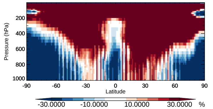
v11-02b-HP / v11-02a DST2 - Zonal mean % diff for Oct
