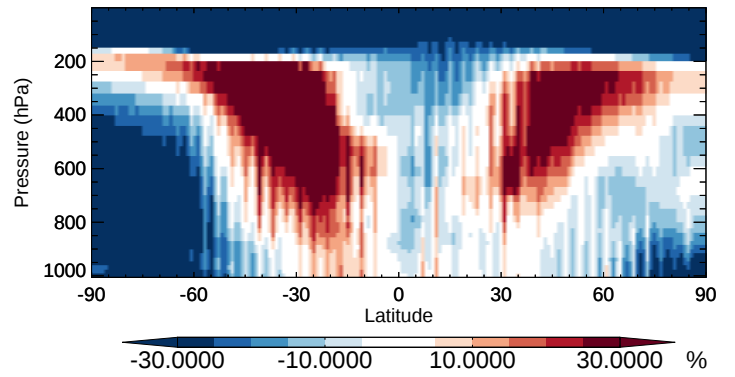
v11-02b-HP / v11-02a BCPI - Zonal mean % diff for Oct
