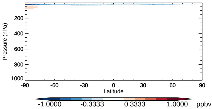
v11-02b-HP - v11-02a NO - Zonal mean abs diff for Oct
