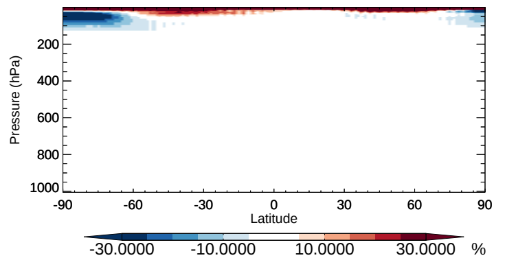
v11-02b-HP / v11-02a CH3Cl - Zonal mean % diff for Oct
