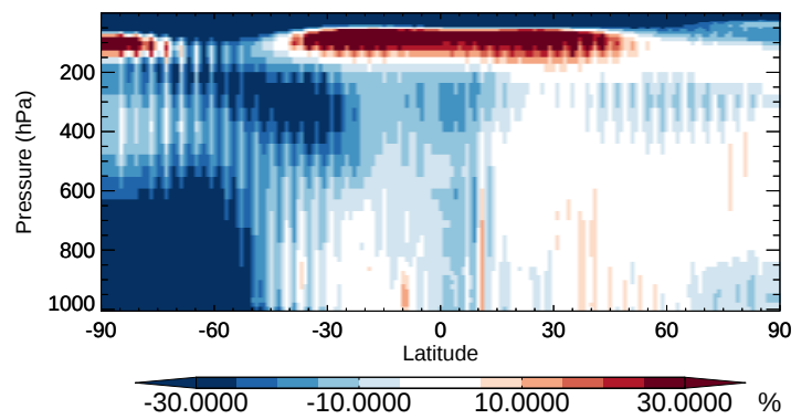
v11-02b-HP / v11-02a ASOG1 - Zonal mean % diff for Oct
