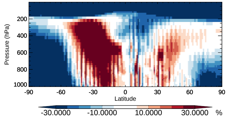
v11-02b-HP / v11-02a ISOA1 - Zonal mean % diff for Oct
