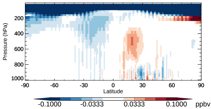
v11-02b-HP - v11-02a HNO 3 - Zonal mean abs diff for Oct
