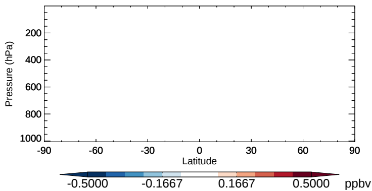
v11-02b-HP - v11-02a CH2O - Zonal mean abs diff for Oct
