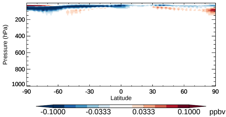
v11-02b-HP - v11-02a ClNO3 - Zonal mean abs diff for Oct
