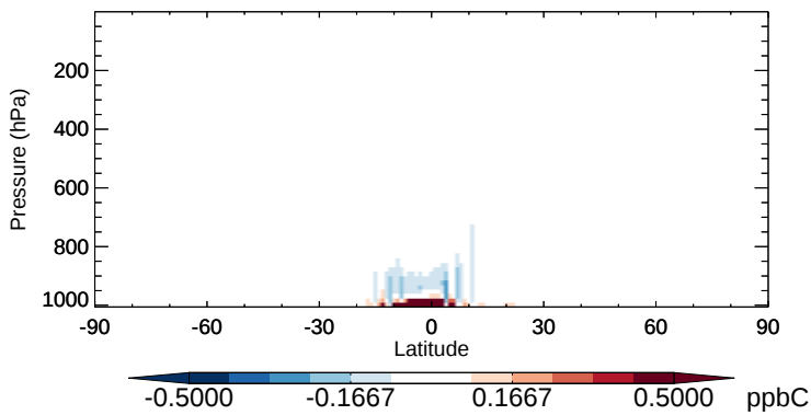
v11-02b-HP - v11-02a ISOP - Zonal mean abs diff for Oct
