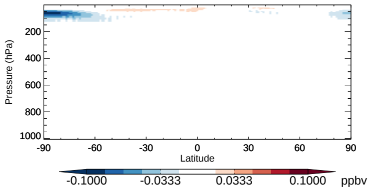
v11-02b-HP - v11-02a OCS - Zonal mean abs diff for Oct
