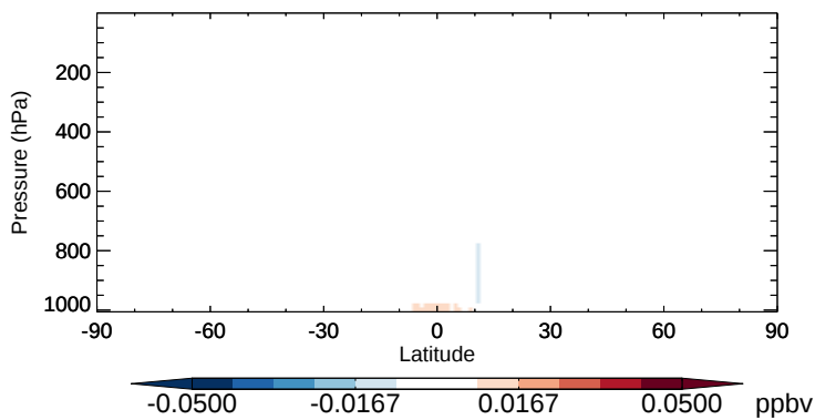
v11-02b-HP - v11-02a MACR - Zonal mean abs diff for Oct
