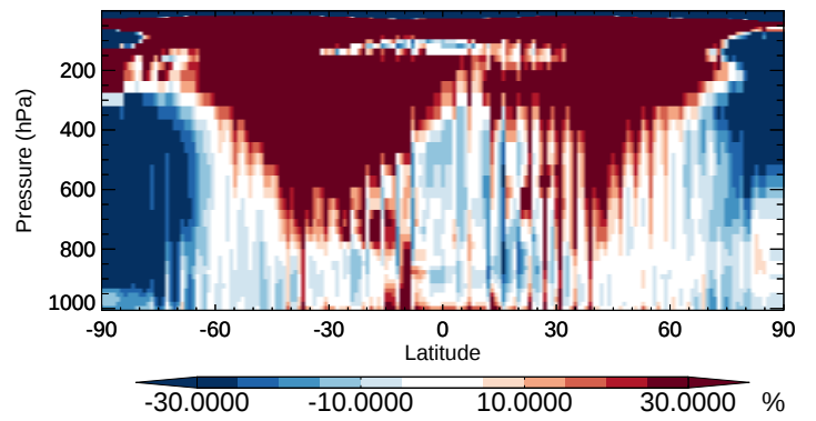
v11-02b-HP / v11-02a XYLE - Zonal mean % diff for Oct
