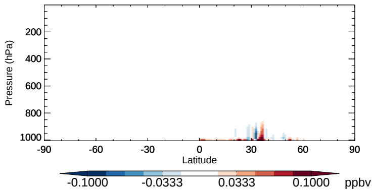
v11-02b-HP - v11-02a XYLE - Zonal mean abs diff for Oct
