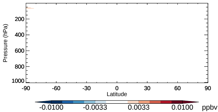
v11-02b-HP - v11-02a Br - Zonal mean abs diff for Oct
