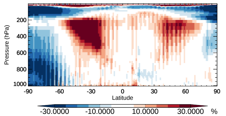
v11-02b-HP / v11-02a ALD2 - Zonal mean % diff for Oct
