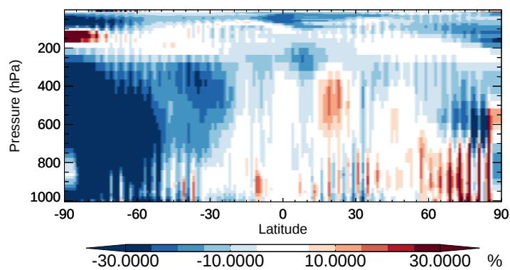
v11-02b-HP / v11-02a HNO4 - Zonal mean % diff for Oct
