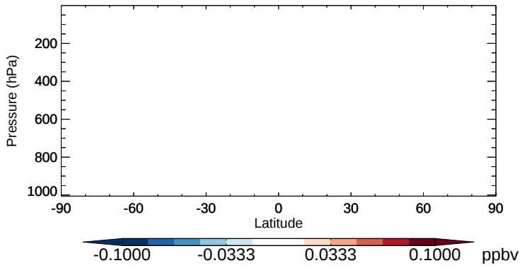
v11-02b-HP - v11-02a HCFC142b - Zonal mean abs diff for Oct
