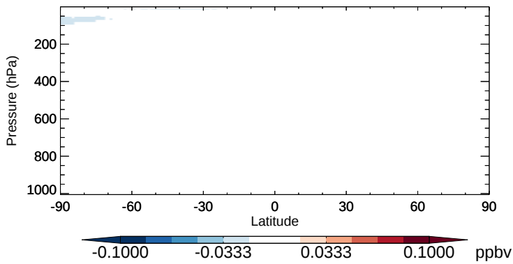
v11-02b-HP - v11-02a HOCl - Zonal mean abs diff for Oct
