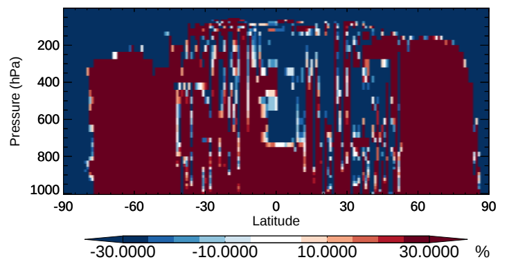
v11-02b-HP / v11-02a MTPO - Zonal mean % diff for Oct
