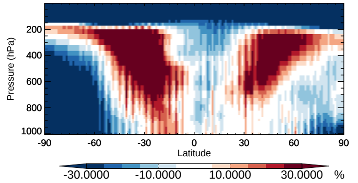
v11-02b-HP / v11-02a OCPI - Zonal mean % diff for Oct
