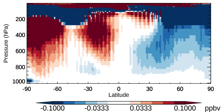
v11-02b-HP - v11-02a N 2 O - Zonal mean abs diff for Oct
