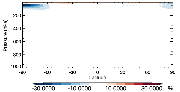
v11-02b-HP / v11-02a CH4 - Zonal mean % diff for Oct
