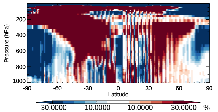
v11-02b-HP / v11-02a MACR - Zonal mean % diff for Oct
