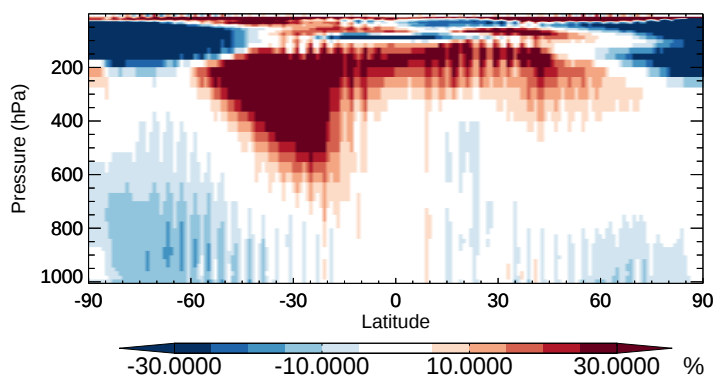
v11-02b-HP / v11-02a MAP - Zonal mean % diff for Oct
