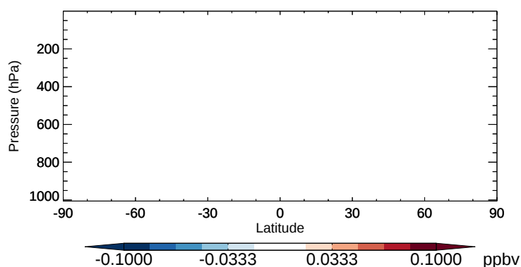
v11-02b-HP - v11-02a ISOPNB - Zonal mean abs diff for Oct
