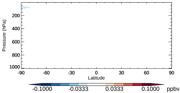
v11-02b-HP - v11-02a Cl 2 O 2 - Zonal mean abs diff for Oct
