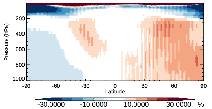
v11-02b-HP / v11-02a C2H6 - Zonal mean % diff for Oct
