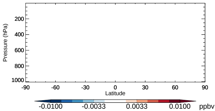
v11-02b-HP - v11-02a PMN - Zonal mean abs diff for Oct
