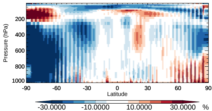
v11-02b-HP / v11-02a NO2 - Zonal mean % diff for Oct
