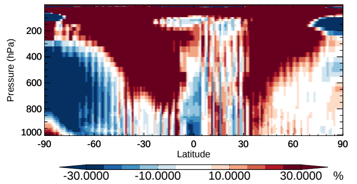
v11-02b-HP / v11-02a MVKN - Zonal mean % diff for Oct
