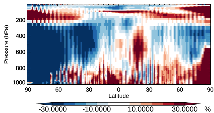
v11-02b-HP / v11-02a N2O5 - Zonal mean % diff for Oct
