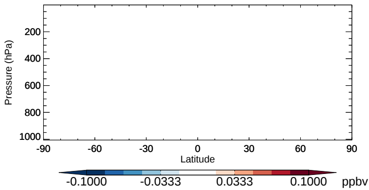
v11-02b-HP - v11-02a ASOAN - Zonal mean abs diff for Oct
