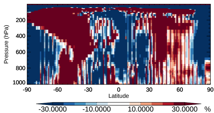
v11-02b-HP / v11-02a ISOPND - Zonal mean % diff for Oct
