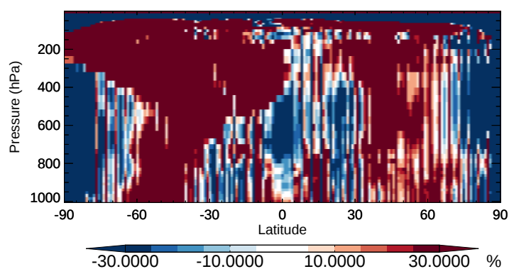
v11-02b-HP / v11-02a ISOPNB - Zonal mean % diff for Oct
