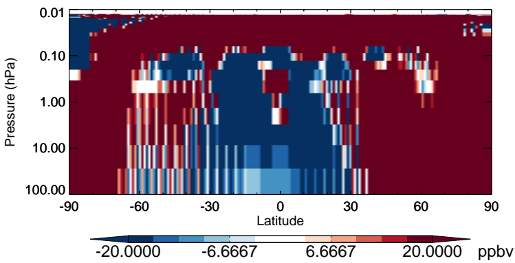
v11-02b-HP - v11-02a O3 - Strat zonal mean abs diff for Apr
