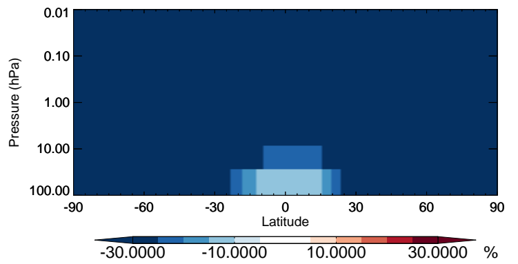
v11-02b-HP / v11-02a ASOAN - Strat zonal mean % diff for Apr
