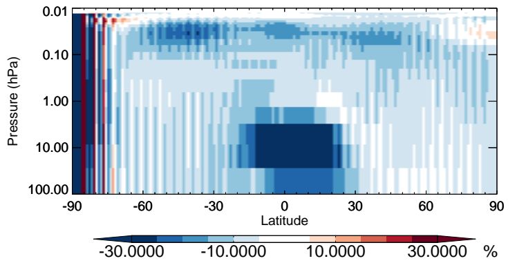
v11-02b-HP / v11-02a ClOO - Strat zonal mean % diff for Apr
