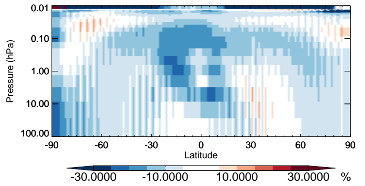
v11-02b-HP / v11-02a HNO4 - Strat zonal mean % diff for Apr
