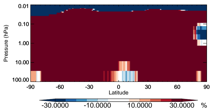
v11-02b-HP / v11-02a TOLU - Strat zonal mean % diff for Apr
