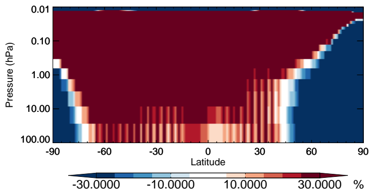
v11-02b-HP / v11-02a ALK4 - Strat zonal mean % diff for Apr
