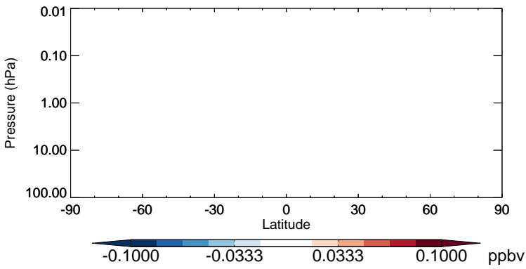
v11-02b-HP - v11-02a CCl4 - Strat zonal mean abs diff for Apr
