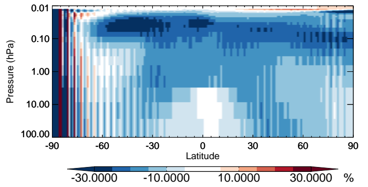
v11-02b-HP / v11-02a NO - Strat zonal mean % diff for Apr
