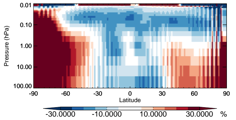
v11-02b-HP / v11-02a N2O5 - Strat zonal mean % diff for Apr
