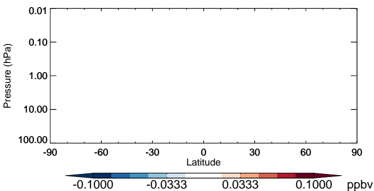
v11-02b-HP - v11-02a ISOA2 - Strat zonal mean abs diff for Apr
