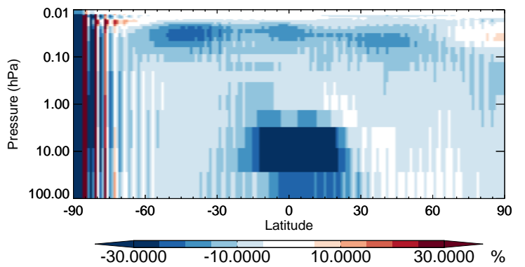
v11-02b-HP / v11-02a Cl - Strat zonal mean % diff for Apr
