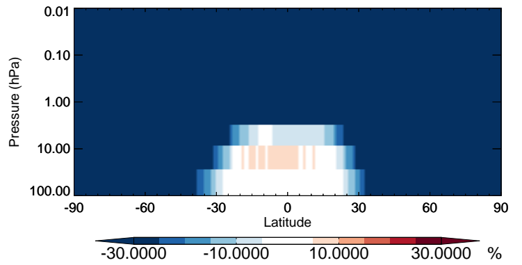
v11-02b-HP / v11-02a ISO3 - Strat zonal mean % diff for Apr
