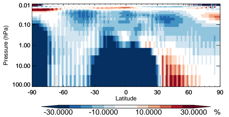
v11-02b-HP / v11-02a Cl2 - Strat zonal mean % diff for Apr
