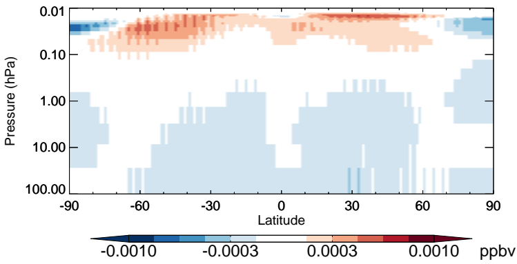
v11-02b-HP - v11-02a PPN - Strat zonal mean abs diff for Apr
