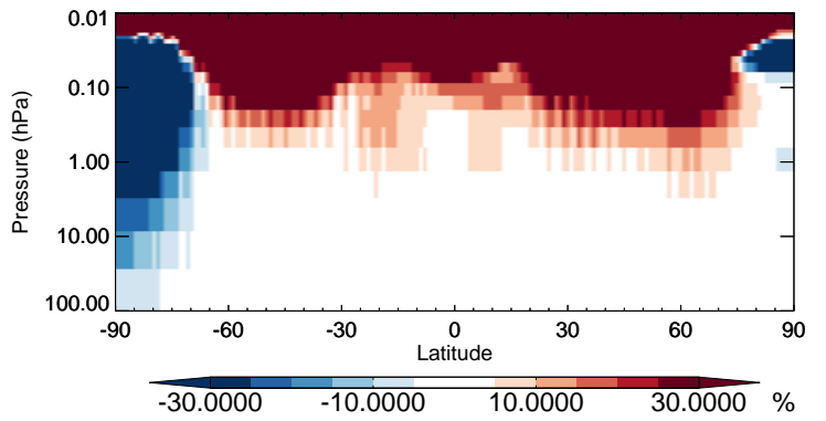
v11-02b-HP / v11-02a CH 3 Br - Strat zonal mean % diff for Apr
