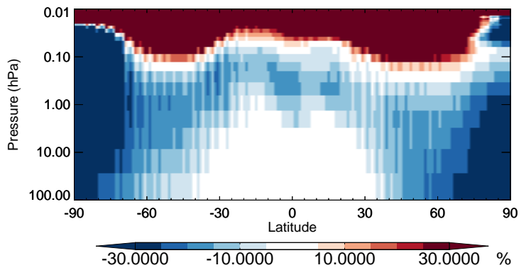
v11-02b-HP / v11-02a C2H6 - Strat zonal mean % diff for Apr
