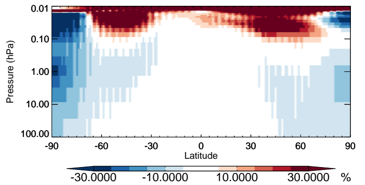
v11-02b-HP / v11-02a CH3Cl - Strat zonal mean % diff for Apr
