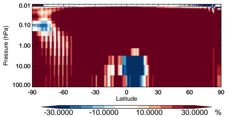
v11-02b-HP / v11-02a OCIO - Strat zonal mean % diff for Apr
