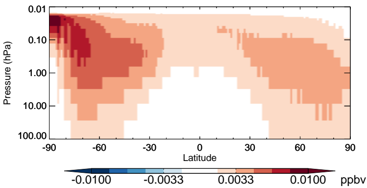
v11-02b-HP - v11-02a BrNO 3 - Strat zonal mean abs diff for Apr
