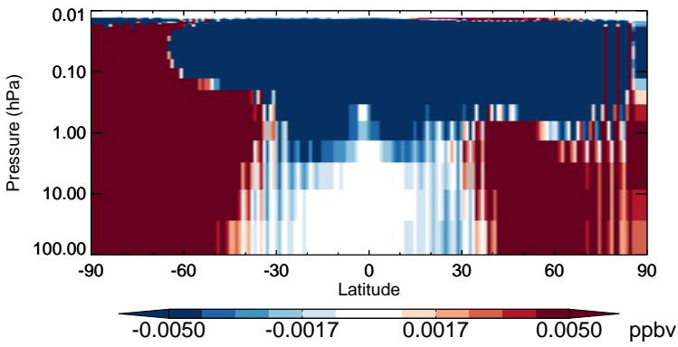
v11-02b-HP - v11-02a N2O5 - Strat zonal mean abs diff for Apr
