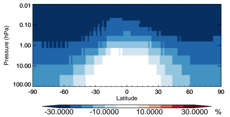
v11-02b-HP / v11-02a MSA - Strat zonal mean % diff for Apr
