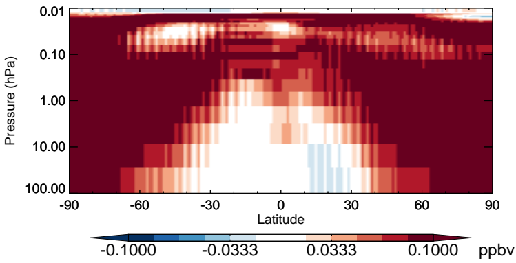
v11-02b-HP - v11-02a HCl - Strat zonal mean abs diff for Apr
