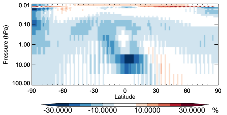
v11-02b-HP / v11-02a MPN - Strat zonal mean % diff for Apr
