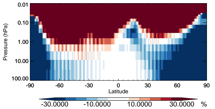
v11-02b-HP / v11-02a C3H8 - Strat zonal mean % diff for Apr
