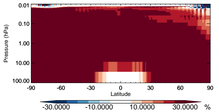
v11-02b-HP / v11-02a BrNO 3 - Strat zonal mean % diff for Apr
