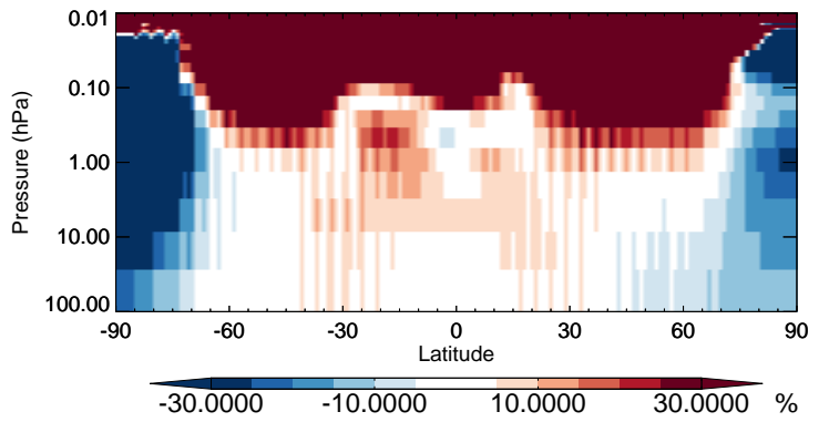
v11-02b-HP / v11-02a CH 2 Br 2 - Strat zonal mean % diff for Apr
