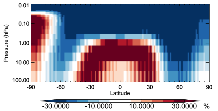
v11-02b-HP / v11-02a ISOG1 - Strat zonal mean % diff for Apr
