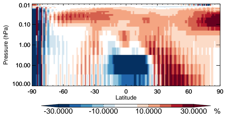
v11-02b-HP / v11-02a ClO - Strat zonal mean % diff for Apr
