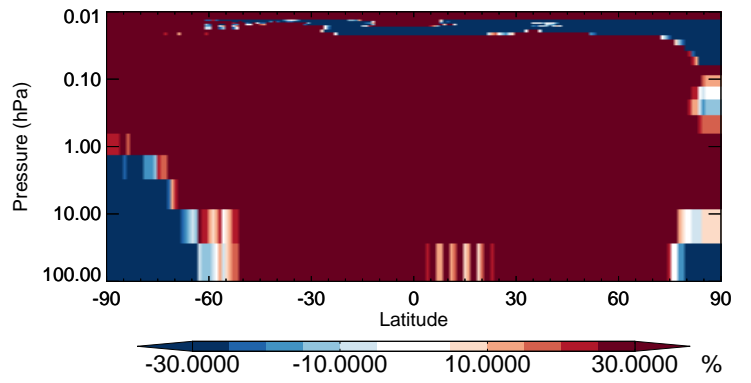
v11-02b-HP / v11-02a IEPOX - Strat zonal mean % diff for Apr
