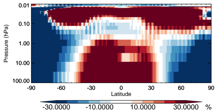
v11-02b-HP / v11-02a MAP - Strat zonal mean % diff for Apr
