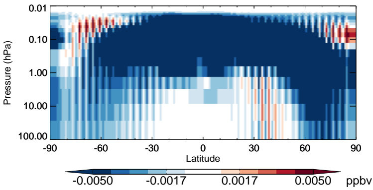
v11-02b-HP - v11-02a HNO4 - Strat zonal mean abs diff for Apr
