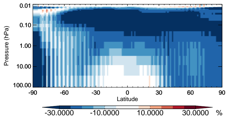
v11-02b-HP / v11-02a HNO 2 - Strat zonal mean % diff for Apr
