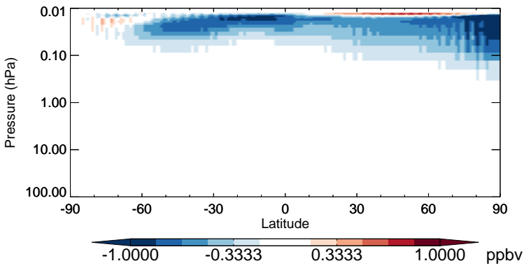
v11-02b-HP - v11-02a NO - Strat zonal mean abs diff for Apr
