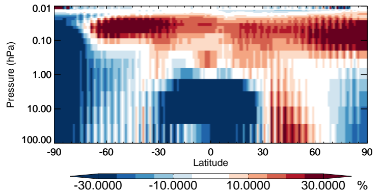
v11-02b-HP / v11-02a HOCl - Strat zonal mean % diff for Apr
