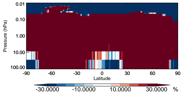
v11-02b-HP / v11-02a XYLE - Strat zonal mean % diff for Apr
