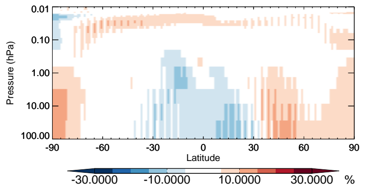
v11-02b-HP / v11-02a O3 - Strat zonal mean % diff for Apr
