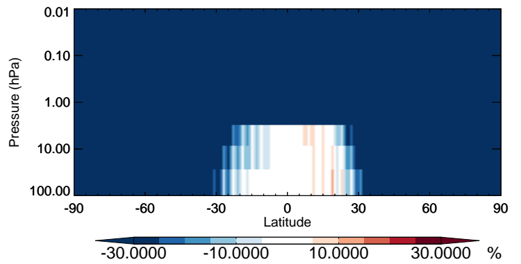
v11-02b-HP / v11-02a ASOG2 - Strat zonal mean % diff for Apr
