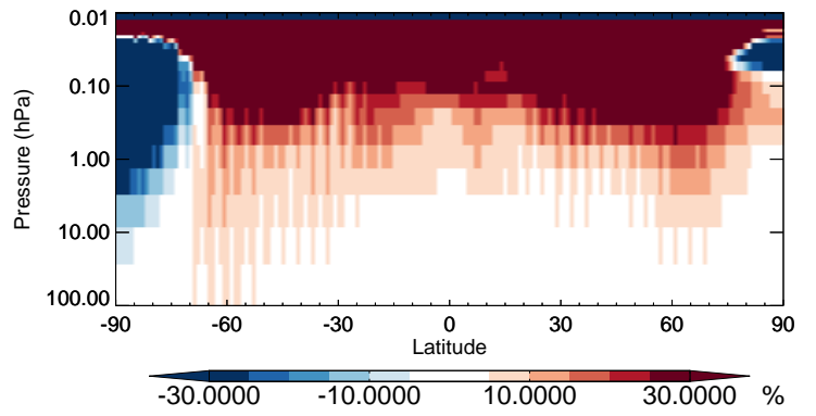
v11-02b-HP / v11-02a CCl4 - Strat zonal mean % diff for Apr
