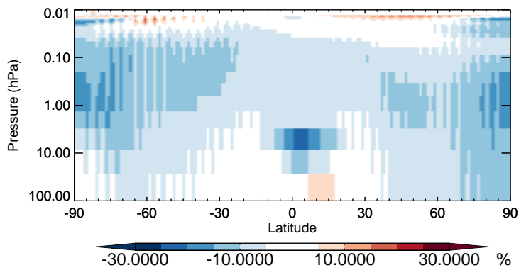
v11-02b-HP / v11-02a CH2O - Strat zonal mean % diff for Apr
