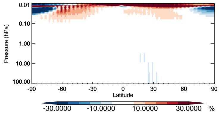
v11-02b-HP / v11-02a PPN - Strat zonal mean % diff for Apr
