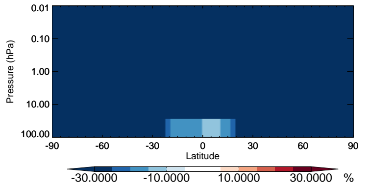
v11-02b-HP / v11-02a TSOA0 - Strat zonal mean % diff for Apr
