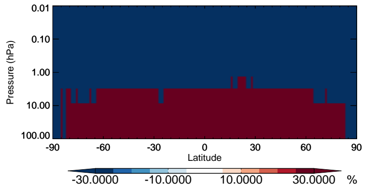
v11-02b-HP / v11-02a SO 4 s - Strat zonal mean % diff for Apr
