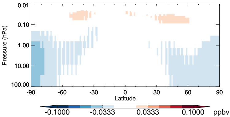
v11-02b-HP - v11-02a CH3Cl - Strat zonal mean abs diff for Apr
