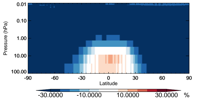
v11-02b-HP / v11-02a ASOG3 - Strat zonal mean % diff for Apr
