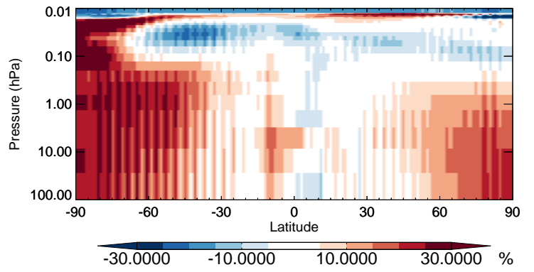
v11-02b-HP / v11-02a BrNO 2 - Strat zonal mean % diff for Apr
