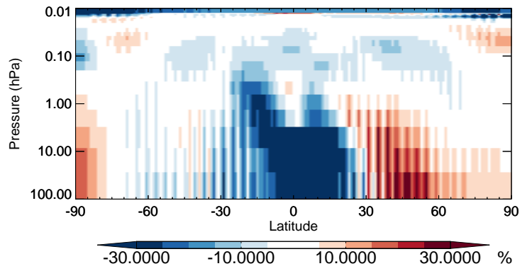
v11-02b-HP / v11-02a ClNO3 - Strat zonal mean % diff for Apr
