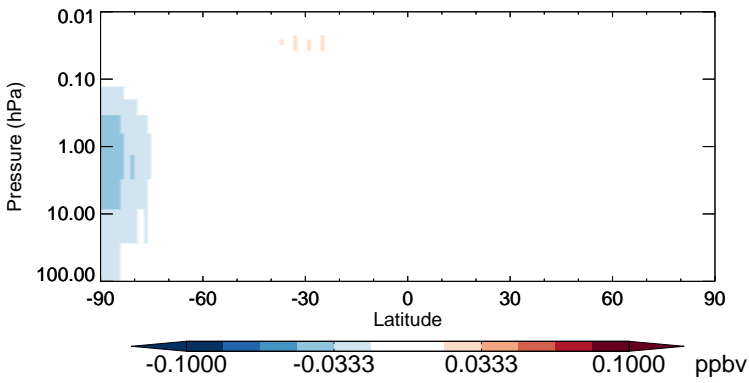
v11-02b-HP - v11-02a HOCl - Strat zonal mean abs diff for Apr
