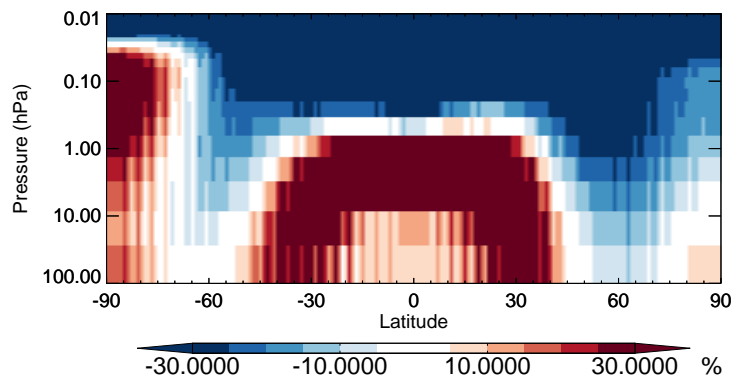
v11-02b-HP / v11-02a ASOG1 - Strat zonal mean % diff for Apr
