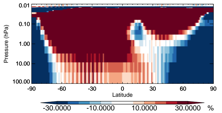
v11-02b-HP / v11-02a R4N2 - Strat zonal mean % diff for Apr
