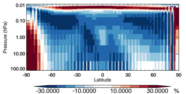
v11-02b-HP / v11-02a BrCl - Strat zonal mean % diff for Apr
