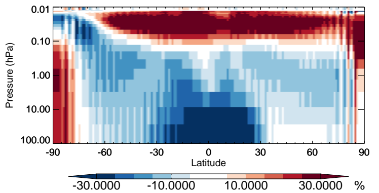
v11-02b-HP / v11-02a HOBr - Strat zonal mean % diff for Apr
