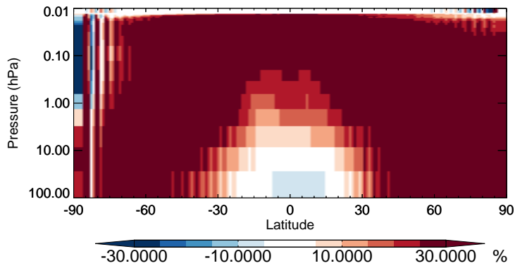
v11-02b-HP / v11-02a BrO - Strat zonal mean % diff for Apr
