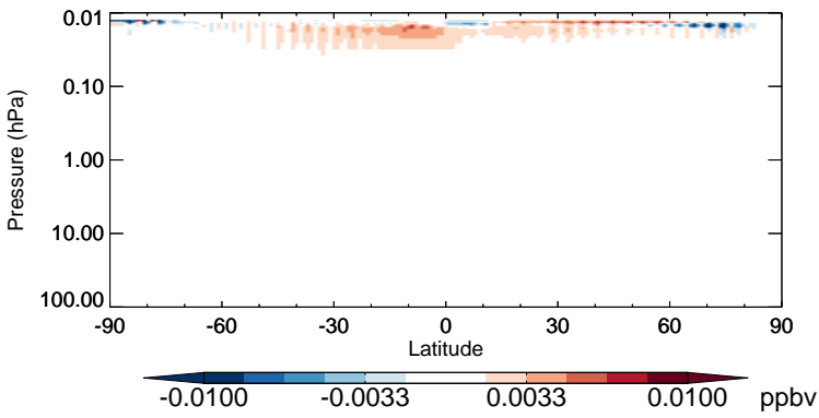
v11-02b-HP - v11-02a NO 3 - Strat zonal mean abs diff for Apr
