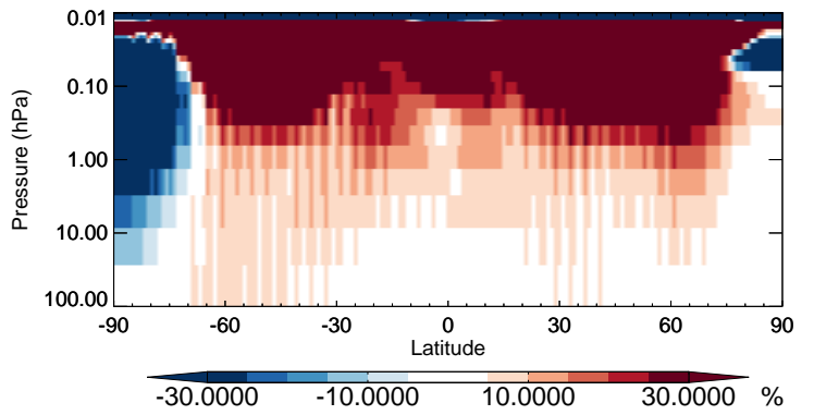
v11-02b-HP / v11-02a H2402 - Strat zonal mean % diff for Apr
