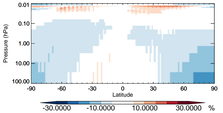
v11-02b-HP / v11-02a CO - Strat zonal mean % diff for Apr
