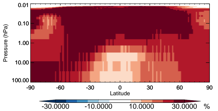
v11-02b-HP / v11-02a HBr - Strat zonal mean % diff for Apr
