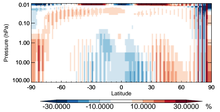
v11-02b-HP / v11-02a NO 3 - Strat zonal mean % diff for Apr
