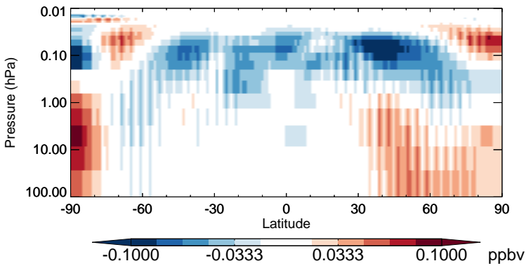
v11-02b-HP - v11-02a ClNO3 - Strat zonal mean abs diff for Apr
