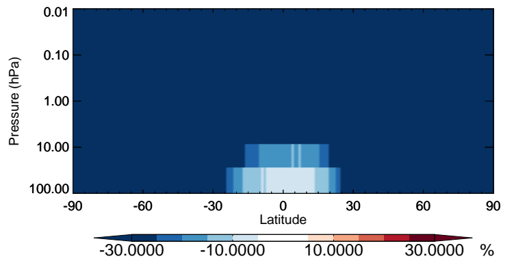
v11-02b-HP / v11-02a ASOA1 - Strat zonal mean % diff for Apr
