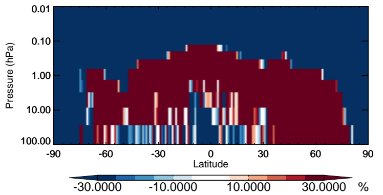
v11-02b-HP / v11-02a ISOP - Strat zonal mean % diff for Apr
