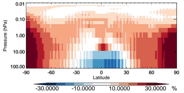
v11-02b-HP / v11-02a HCl - Strat zonal mean % diff for Apr
