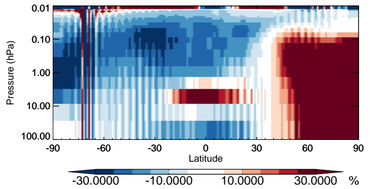
v11-02b-HP / v11-02a N2O5 - Strat zonal mean % diff for Jan
