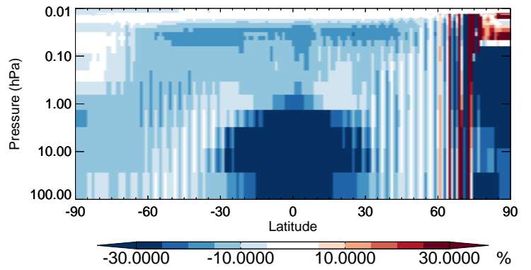
v11-02b-HP / v11-02a ClOO - Strat zonal mean % diff for Jan
