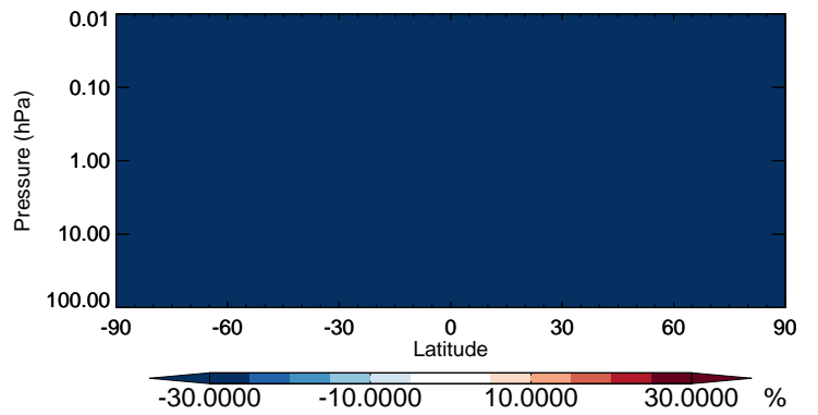
v11-02b-HP / v11-02a ISOA2 - Strat zonal mean % diff for Jan
