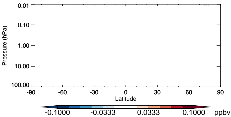
v11-02b-HP - v11-02a Cl - Strat zonal mean abs diff for Jan
