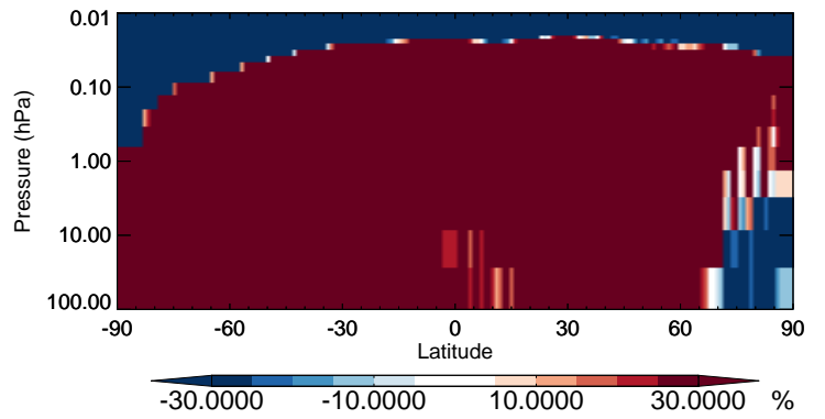
v11-02b-HP / v11-02a OCPO - Strat zonal mean % diff for Jan
