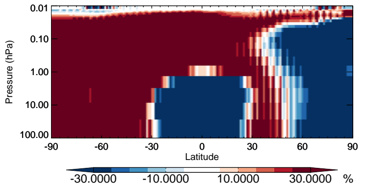
v11-02b-HP / v11-02a Cl 2 O 2 - Strat zonal mean % diff for Jan
