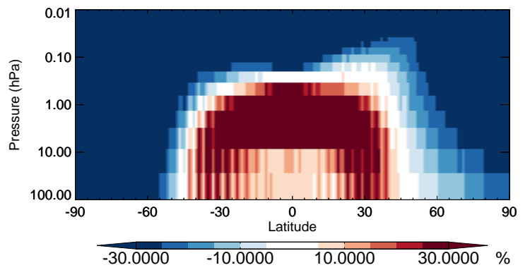
v11-02b-HP / v11-02a ASOG1 - Strat zonal mean % diff for Jan
