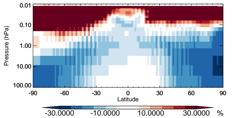
v11-02b-HP / v11-02a EOH - Strat zonal mean % diff for Jan
