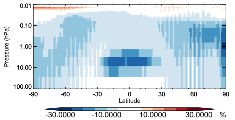
v11-02b-HP / v11-02a CH2O - Strat zonal mean % diff for Jan
