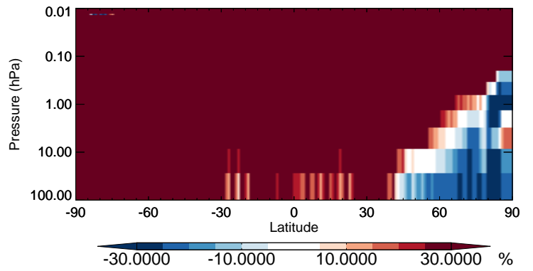
v11-02b-HP / v11-02a IEPOX - Strat zonal mean % diff for Jan
