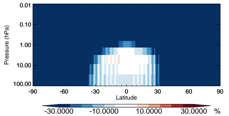
v11-02b-HP / v11-02a ISOG2 - Strat zonal mean % diff for Jan
