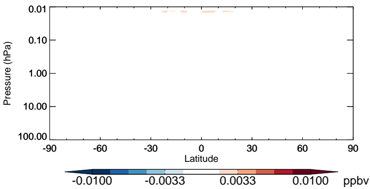
v11-02b-HP - v11-02a HOBr - Strat zonal mean abs diff for Jan
