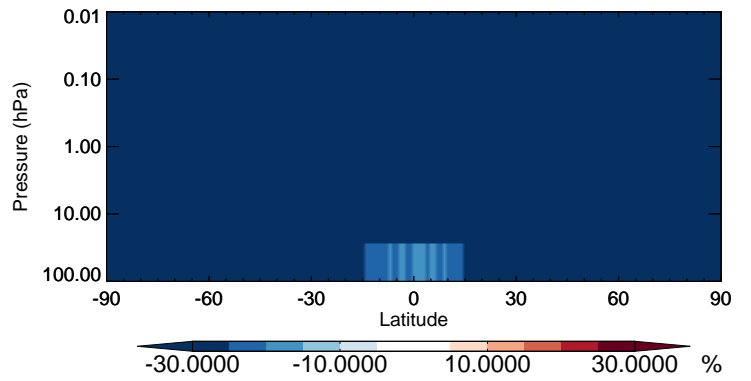
v11-02b-HP / v11-02a ISOA3 - Strat zonal mean % diff for Jan
