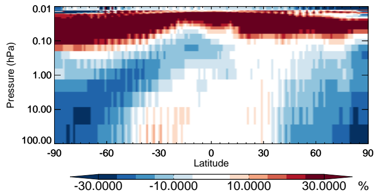
v11-02b-HP / v11-02a PAN - Strat zonal mean % diff for Jan
