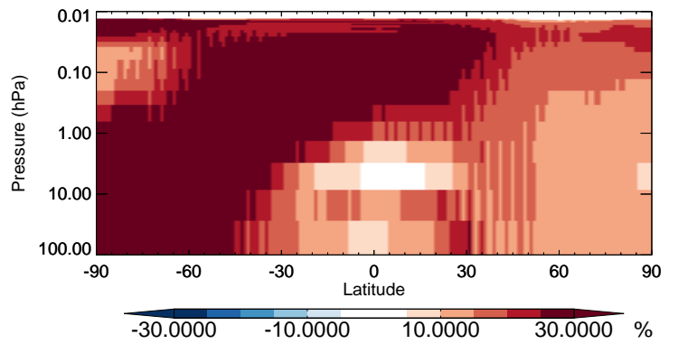
v11-02b-HP / v11-02a HBr - Strat zonal mean % diff for Jan
