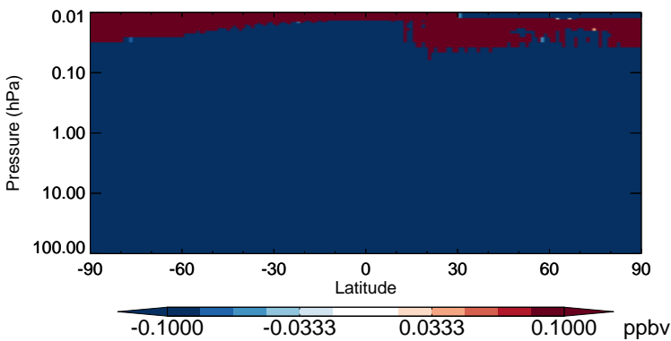
v11-02b-HP - v11-02a CH4 - Strat zonal mean abs diff for Jan
