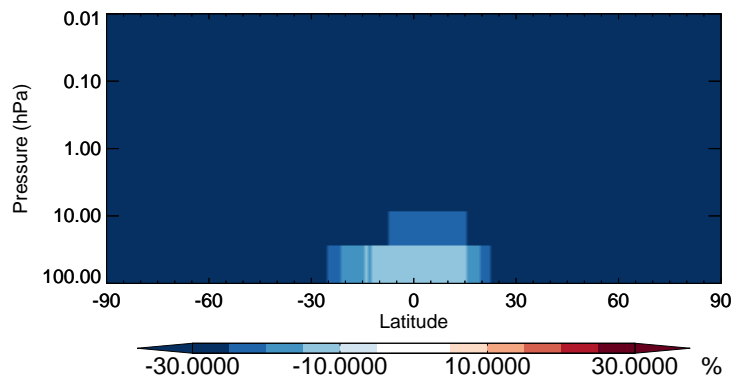
v11-02b-HP / v11-02a ISOA1 - Strat zonal mean % diff for Jan
