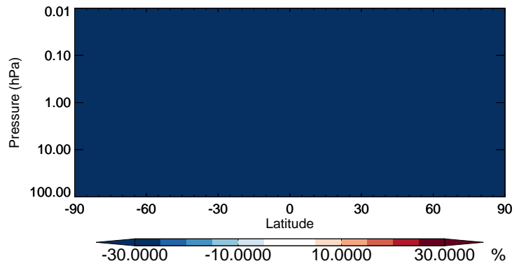
v11-02b-HP / v11-02a NH4 - Strat zonal mean % diff for Jan
