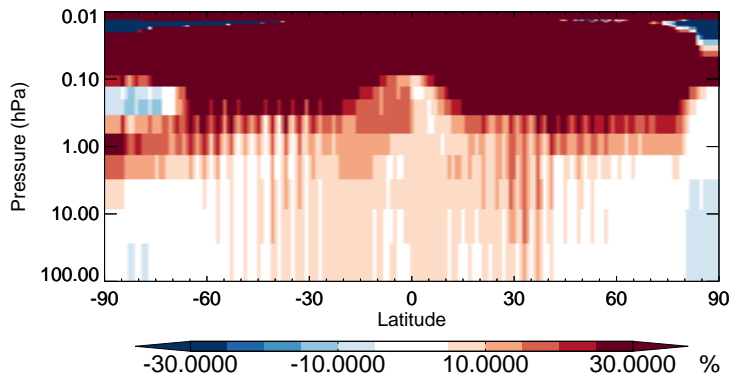
v11-02b-HP / v11-02a CH 2 Br 2 - Strat zonal mean % diff for Jan
