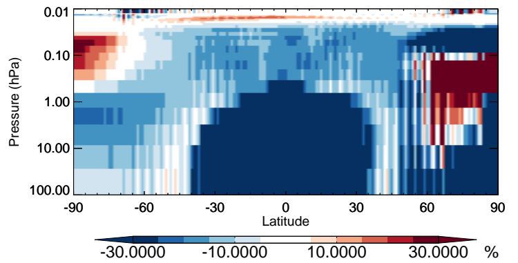
v11-02b-HP / v11-02a Cl2 - Strat zonal mean % diff for Jan
