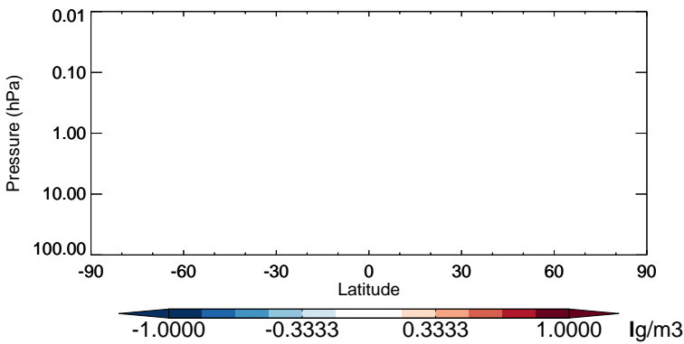
v11-02b-HP - v11-02a NITs - Strat zonal mean abs diff for Jan
