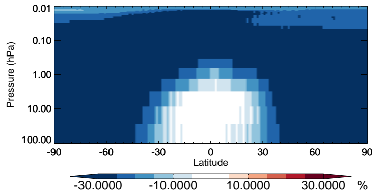
v11-02b-HP / v11-02a ASOG3 - Strat zonal mean % diff for Jan
