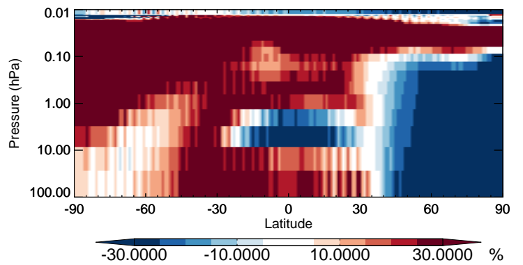
v11-02b-HP / v11-02a MAP - Strat zonal mean % diff for Jan
