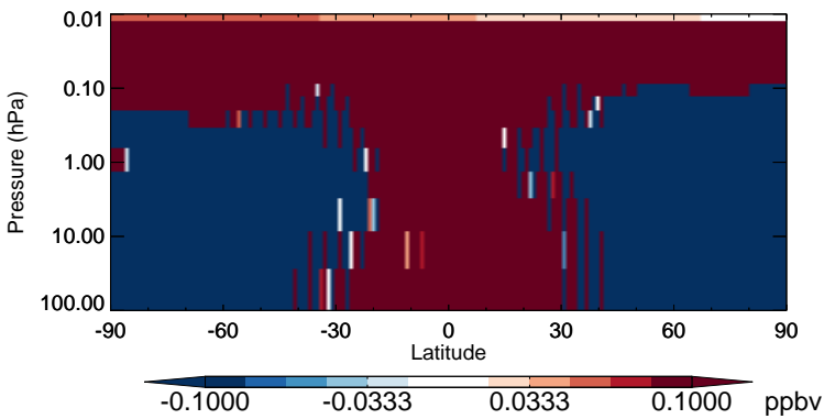
v11-02b-HP - v11-02a N 2 O - Strat zonal mean abs diff for Jan
