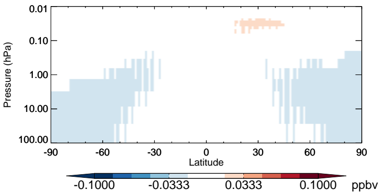
v11-02b-HP - v11-02a CH3Cl - Strat zonal mean abs diff for Jan
