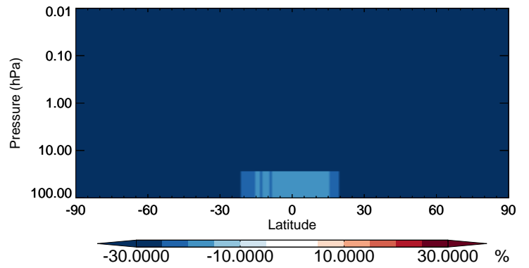
v11-02b-HP / v11-02a TSOA1 - Strat zonal mean % diff for Jan
