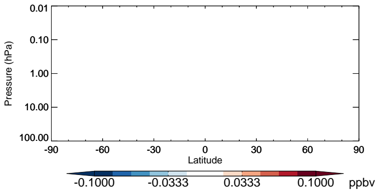
v11-02b-HP - v11-02a MGLY - Strat zonal mean abs diff for Jan
