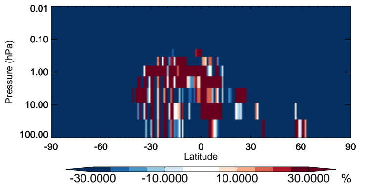
v11-02b-HP / v11-02a MTPA - Strat zonal mean % diff for Jan
