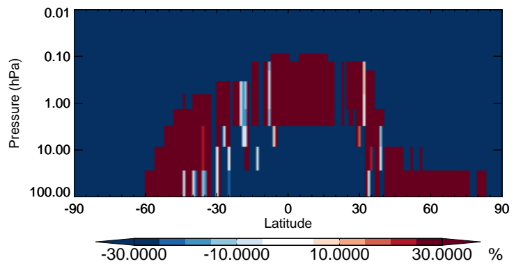
v11-02b-HP / v11-02a NIT - Strat zonal mean % diff for Jan
