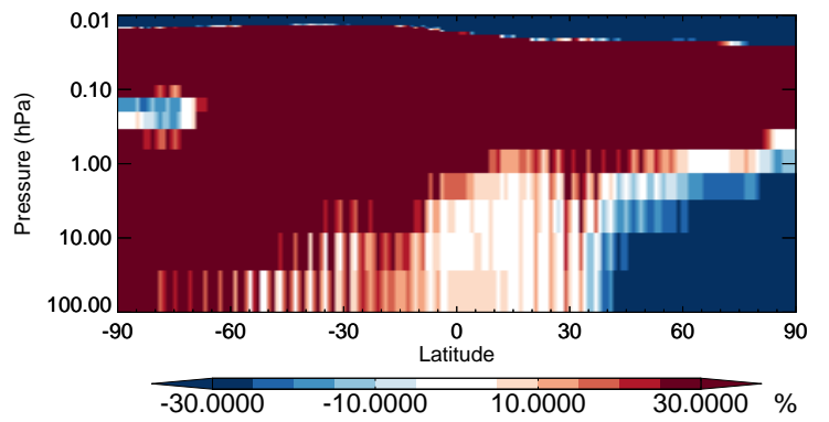
v11-02b-HP / v11-02a BENZ - Strat zonal mean % diff for Jan
