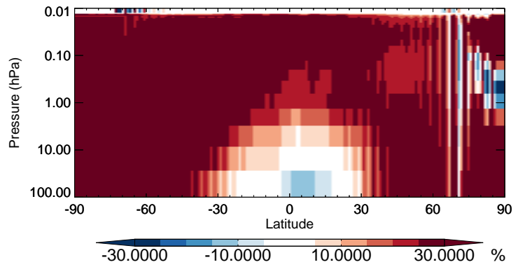
v11-02b-HP / v11-02a BrO - Strat zonal mean % diff for Jan
