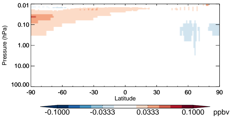
v11-02b-HP - v11-02a ClO - Strat zonal mean abs diff for Jan
