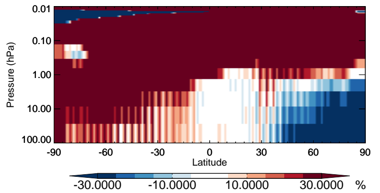
v11-02b-HP / v11-02a CHBr 3 - Strat zonal mean % diff for Jan
