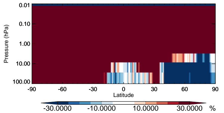
v11-02b-HP / v11-02a PMN - Strat zonal mean % diff for Jan
