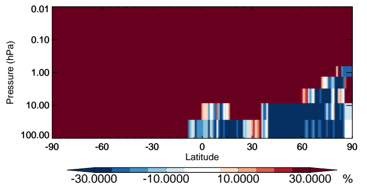
v11-02b-HP / v11-02a MACRN - Strat zonal mean % diff for Jan
