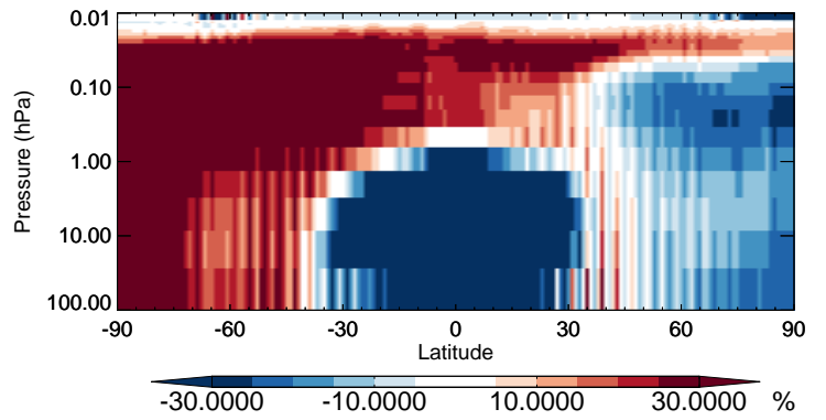
v11-02b-HP / v11-02a HOCl - Strat zonal mean % diff for Jan
