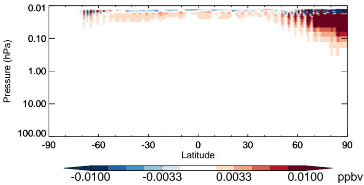
v11-02b-HP - v11-02a NO 3 - Strat zonal mean abs diff for Jan
