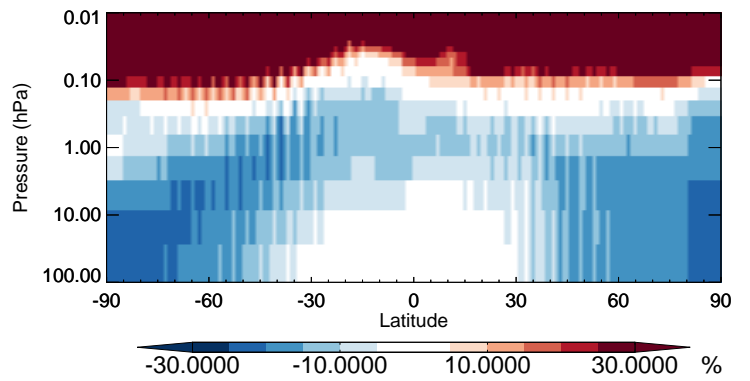
v11-02b-HP / v11-02a C2H6 - Strat zonal mean % diff for Jan
