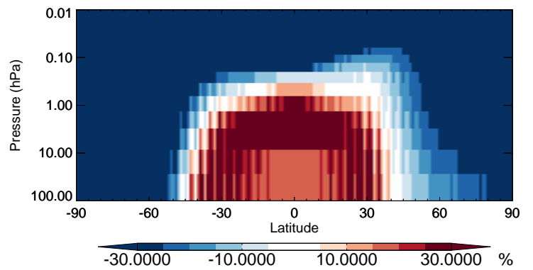
v11-02b-HP / v11-02a ISOG1 - Strat zonal mean % diff for Jan
