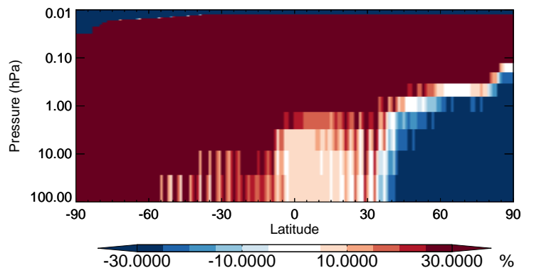
v11-02b-HP / v11-02a ALK4 - Strat zonal mean % diff for Jan
