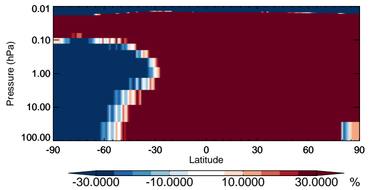
v11-02b-HP / v11-02a DST2 - Strat zonal mean % diff for Jan
