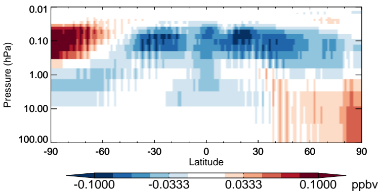
v11-02b-HP - v11-02a ClNO3 - Strat zonal mean abs diff for Jan
