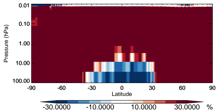
v11-02b-HP / v11-02a Br2 - Strat zonal mean % diff for Jan
