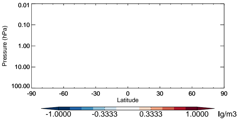
v11-02b-HP - v11-02a NH4 - Strat zonal mean abs diff for Jan
