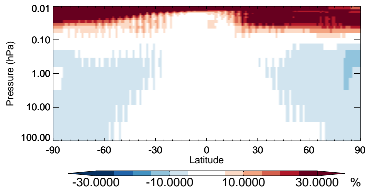
v11-02b-HP / v11-02a CH3Cl - Strat zonal mean % diff for Jan
