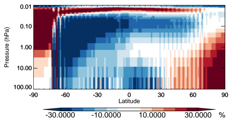
v11-02b-HP / v11-02a BrCl - Strat zonal mean % diff for Jan
