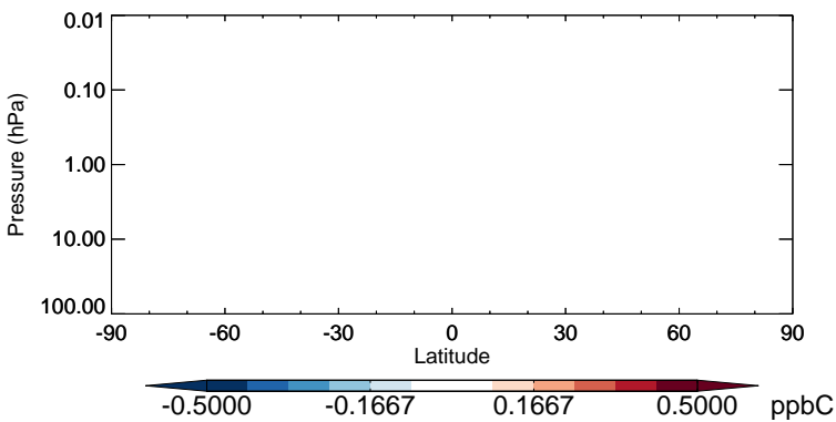
v11-02b-HP - v11-02a ALD2 - Strat zonal mean abs diff for Jan
