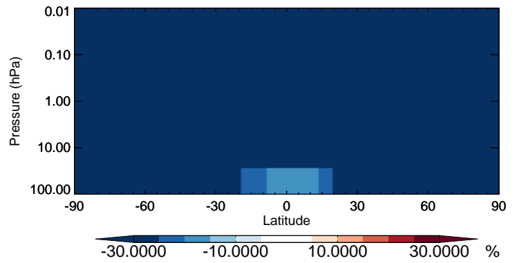
v11-02b-HP / v11-02a TSOA0 - Strat zonal mean % diff for Jan
