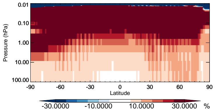
v11-02b-HP / v11-02a H2402 - Strat zonal mean % diff for Jan
