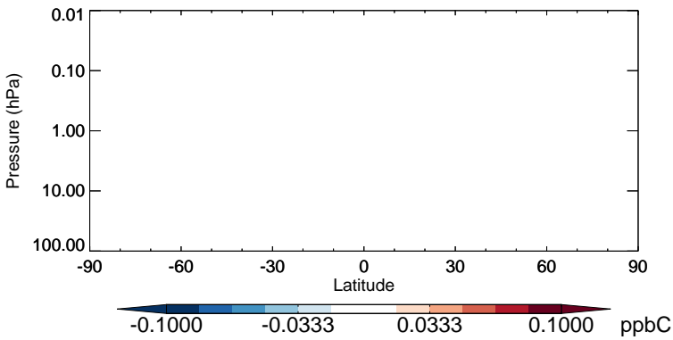
v11-02b-HP - v11-02a MEK - Strat zonal mean abs diff for Jan
