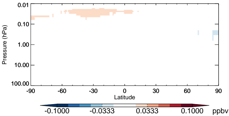
v11-02b-HP - v11-02a HOCl - Strat zonal mean abs diff for Jan
