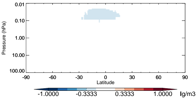
v11-02b-HP - v11-02a SO 4 - Strat zonal mean abs diff for Jan
