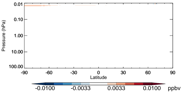
v11-02b-HP - v11-02a Br - Strat zonal mean abs diff for Jan
