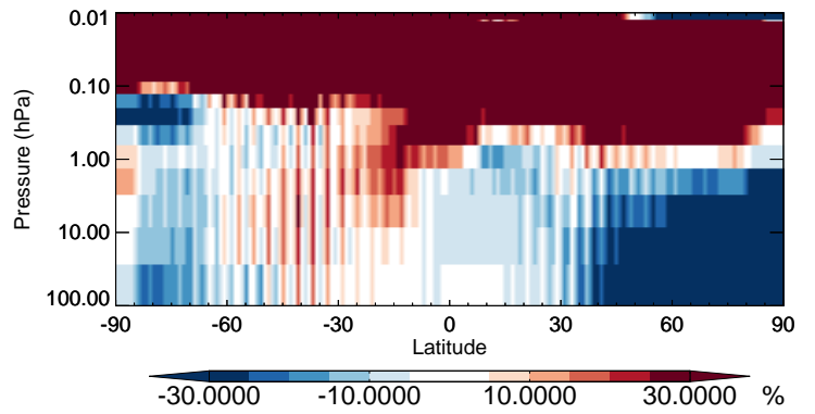
v11-02b-HP / v11-02a C3H8 - Strat zonal mean % diff for Jan
