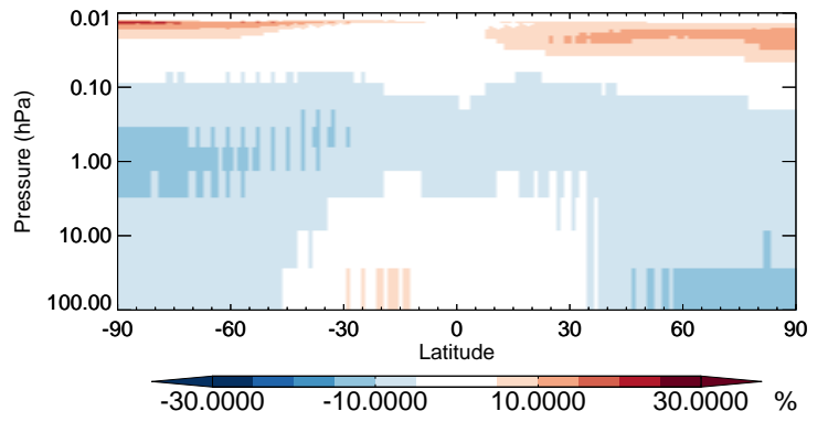
v11-02b-HP / v11-02a CO - Strat zonal mean % diff for Jan
