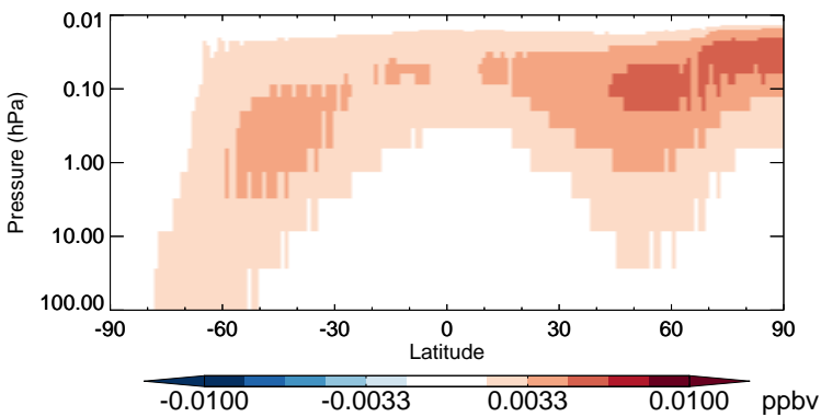
v11-02b-HP - v11-02a BrNO 3 - Strat zonal mean abs diff for Jan
