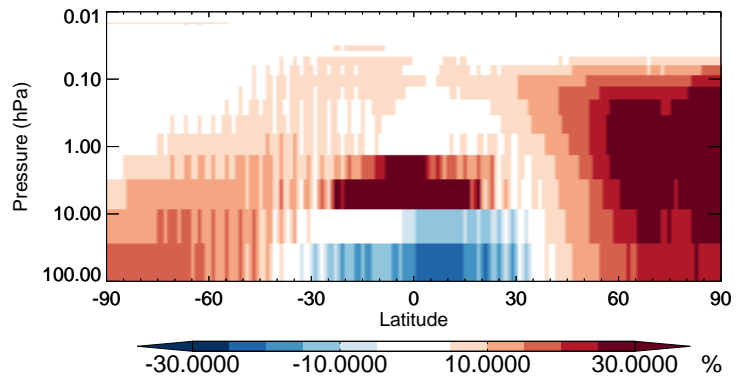
v11-02b-HP / v11-02a HCl - Strat zonal mean % diff for Jan
