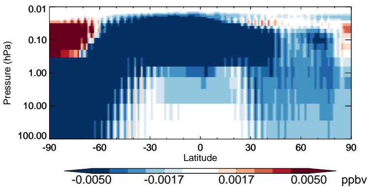
v11-02b-HP - v11-02a HNO4 - Strat zonal mean abs diff for Jan
