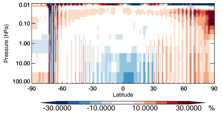
v11-02b-HP / v11-02a NO 3 - Strat zonal mean % diff for Jan
