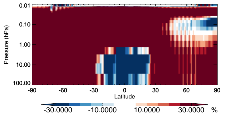
v11-02b-HP / v11-02a OCIO - Strat zonal mean % diff for Jan
