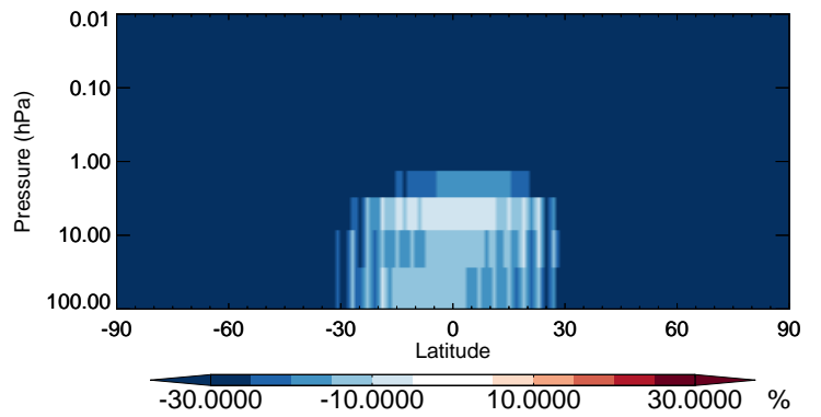
v11-02b-HP / v11-02a ASOG2 - Strat zonal mean % diff for Jan
