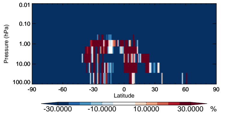
v11-02b-HP / v11-02a LIMO - Strat zonal mean % diff for Jan
