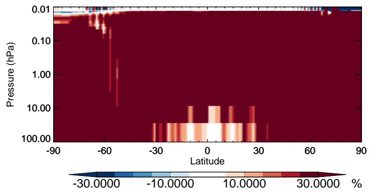
v11-02b-HP / v11-02a Br2 - Strat zonal mean % diff for Jul
