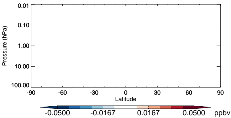
v11-02b-HP - v11-02a MACR - Strat zonal mean abs diff for Jul
