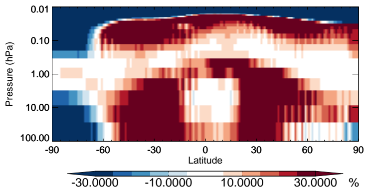
v11-02b-HP / v11-02a SO 2 - Strat zonal mean % diff for Jul
