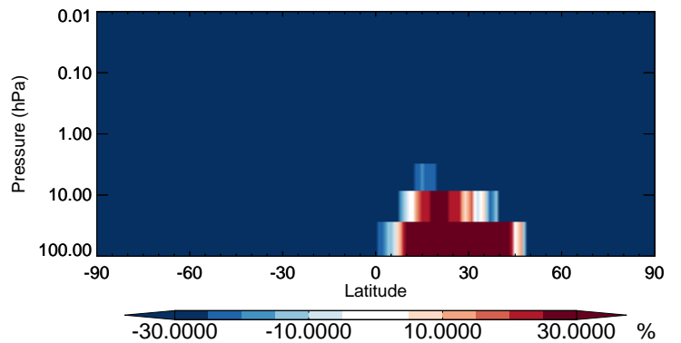
v11-02b-HP / v11-02a NH 3 - Strat zonal mean % diff for Jul
