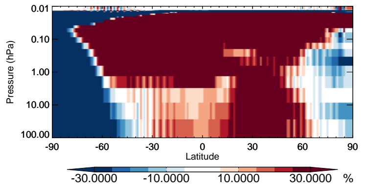
v11-02b-HP / v11-02a RCHO - Strat zonal mean % diff for Jul
