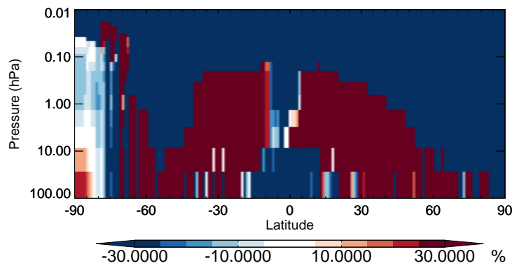
v11-02b-HP / v11-02a NIT - Strat zonal mean % diff for Jul
