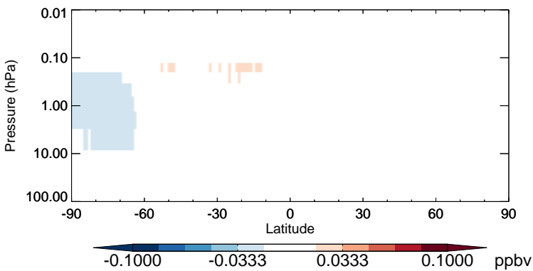
v11-02b-HP - v11-02a CFC11 - Strat zonal mean abs diff for Jul
