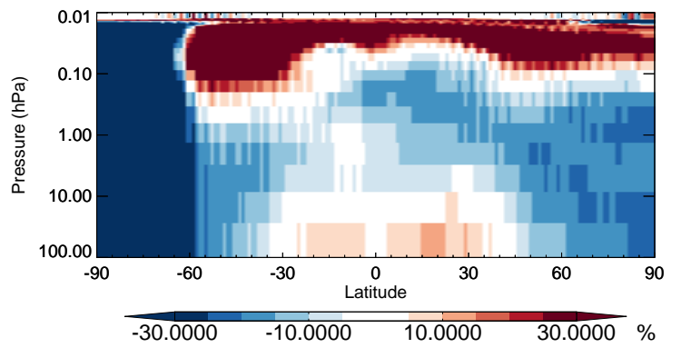
v11-02b-HP / v11-02a ALD2 - Strat zonal mean % diff for Jul
