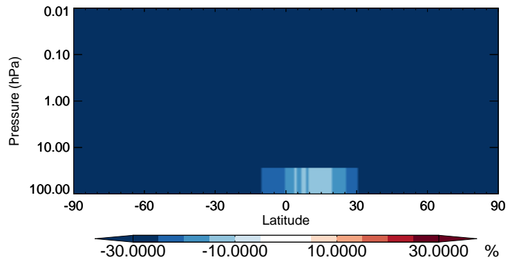
v11-02b-HP / v11-02a BCPI - Strat zonal mean % diff for Jul
