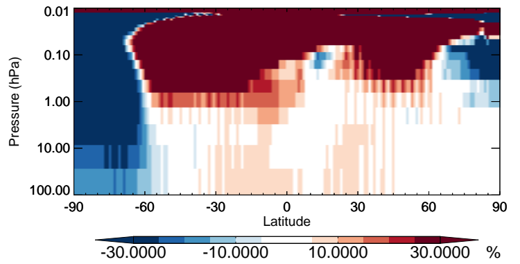
v11-02b-HP / v11-02a CH 2 Br 2 - Strat zonal mean % diff for Jul
