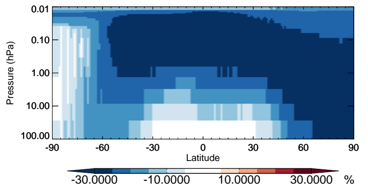
v11-02b-HP / v11-02a H 2 O - Strat zonal mean % diff for Jul
