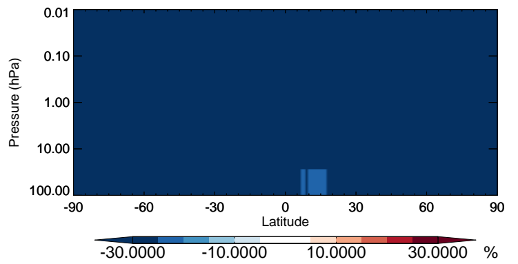
v11-02b-HP / v11-02a ASOA3 - Strat zonal mean % diff for Jul
