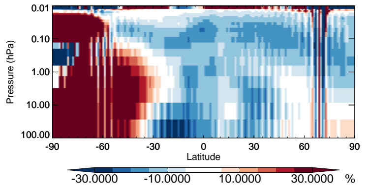
v11-02b-HP / v11-02a N2O5 - Strat zonal mean % diff for Jul
