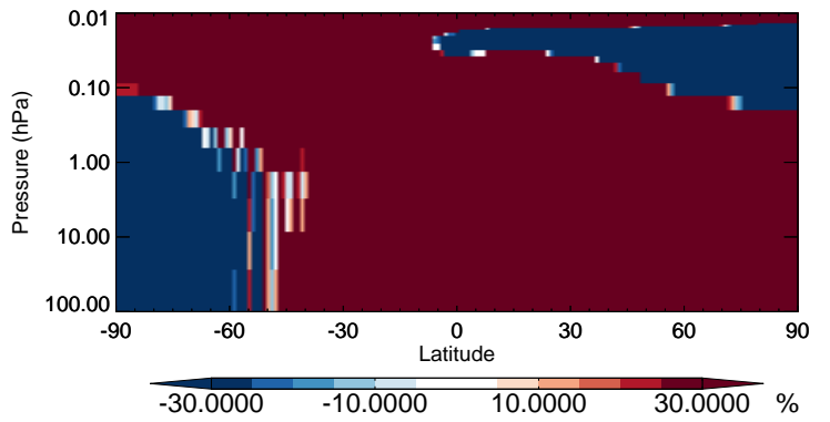
v11-02b-HP / v11-02a DMS - Strat zonal mean % diff for Jul
