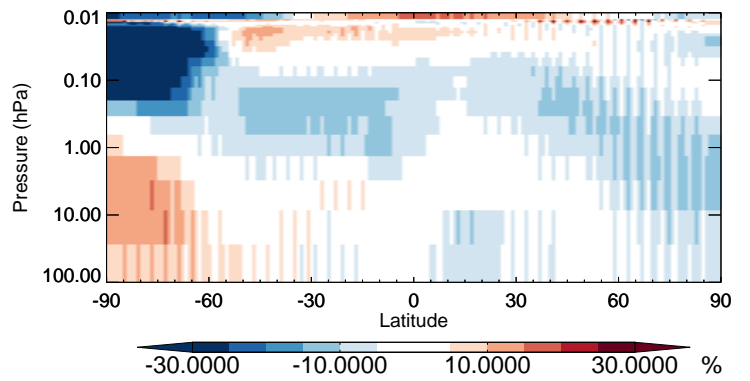
v11-02b-HP / v11-02a MPN - Strat zonal mean % diff for Jul
