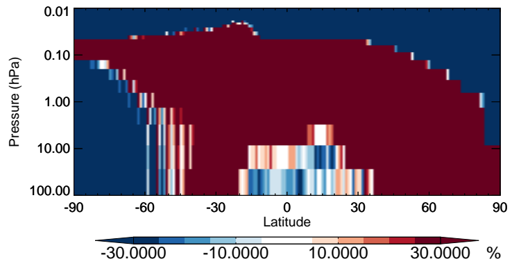
v11-02b-HP / v11-02a XYLE - Strat zonal mean % diff for Jul
