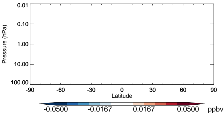
v11-02b-HP - v11-02a MP - Strat zonal mean abs diff for Jul
