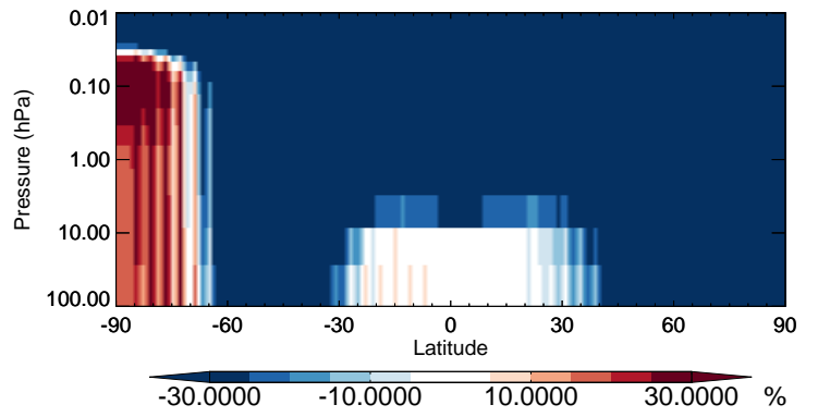
v11-02b-HP / v11-02a TSOG2 - Strat zonal mean % diff for Jul
