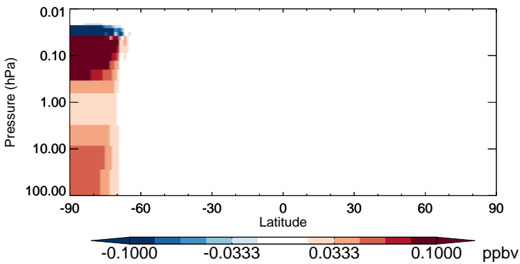
v11-02b-HP - v11-02a Cl2 - Strat zonal mean abs diff for Jul
