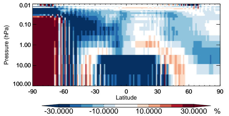
v11-02b-HP / v11-02a Cl2 - Strat zonal mean % diff for Jul
