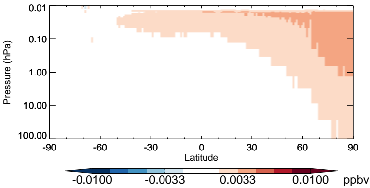
v11-02b-HP - v11-02a BrO - Strat zonal mean abs diff for Jul
