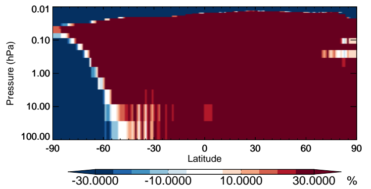
v11-02b-HP / v11-02a BENZ - Strat zonal mean % diff for Jul
