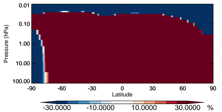
v11-02b-HP / v11-02a DST4 - Strat zonal mean % diff for Jul
