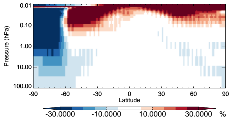
v11-02b-HP / v11-02a CH3Cl - Strat zonal mean % diff for Jul
