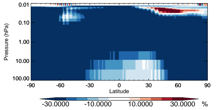
v11-02b-HP / v11-02a MGLY - Strat zonal mean % diff for Jul
