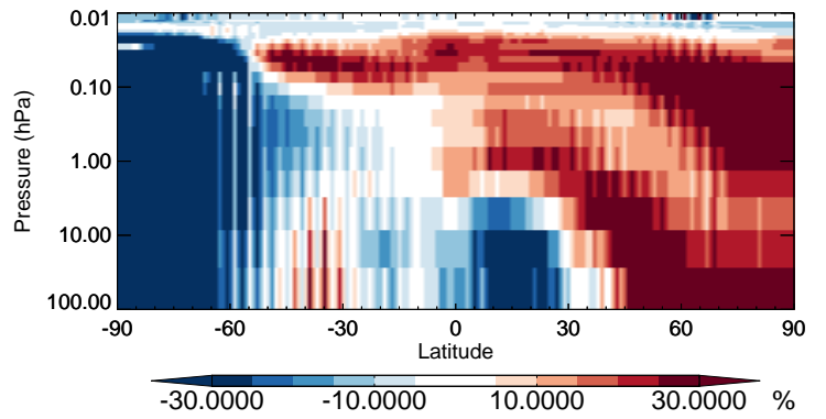
v11-02b-HP / v11-02a HOCl - Strat zonal mean % diff for Jul
