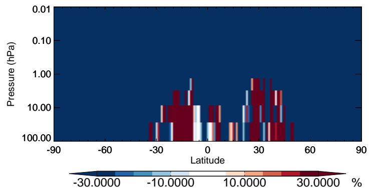
v11-02b-HP / v11-02a MTPO - Strat zonal mean % diff for Jul
