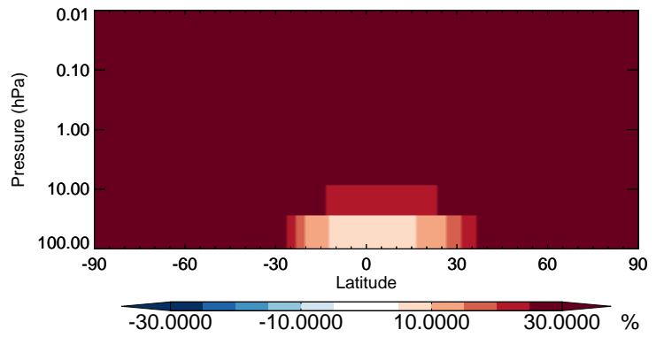
v11-02b-HP / v11-02a CFC115 - Strat zonal mean % diff for Jul
