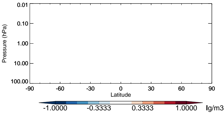
v11-02b-HP - v11-02a SO 4 s - Strat zonal mean abs diff for Jul
