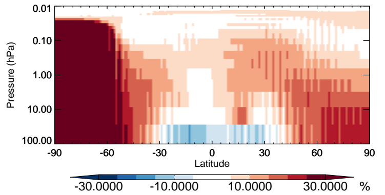
v11-02b-HP / v11-02a HCl - Strat zonal mean % diff for Jul
