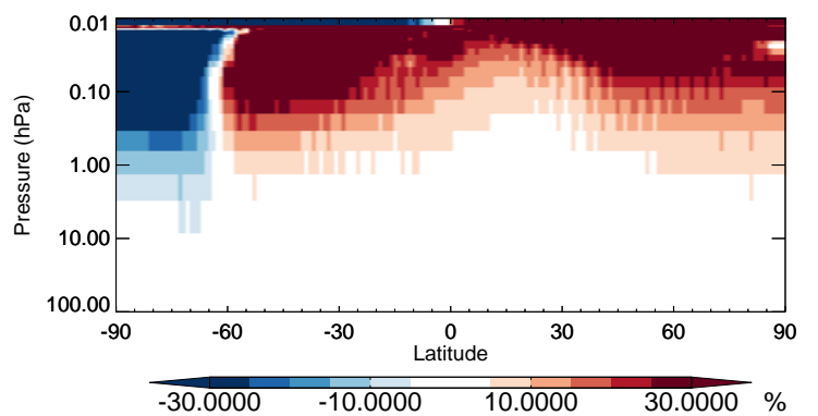
v11-02b-HP / v11-02a CFC12 - Strat zonal mean % diff for Jul
