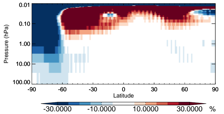
v11-02b-HP / v11-02a OCS - Strat zonal mean % diff for Jul
