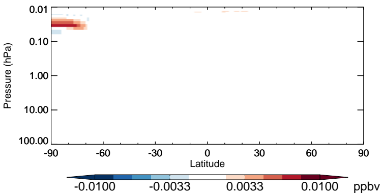
v11-02b-HP - v11-02a HOBr - Strat zonal mean abs diff for Jul
