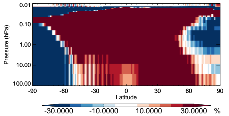
v11-02b-HP / v11-02a MEK - Strat zonal mean % diff for Jul
