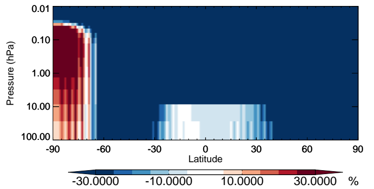
v11-02b-HP / v11-02a ISOG2 - Strat zonal mean % diff for Jul
