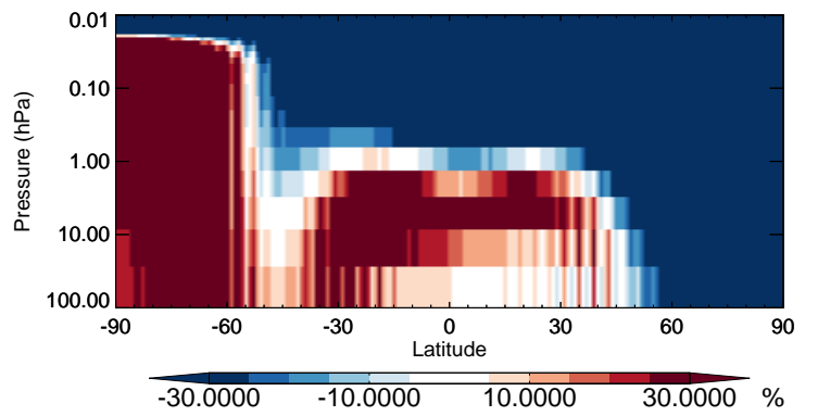
v11-02b-HP / v11-02a ISOG1 - Strat zonal mean % diff for Jul
