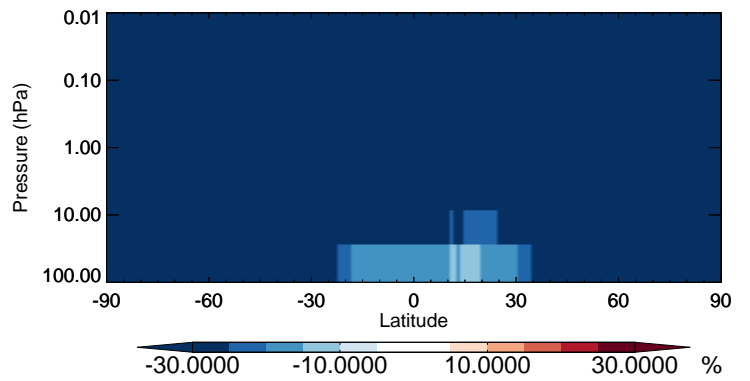
v11-02b-HP / v11-02a ASOA1 - Strat zonal mean % diff for Jul
