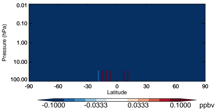
v11-02b-HP - v11-02a H 2 O - Strat zonal mean abs diff for Jul
