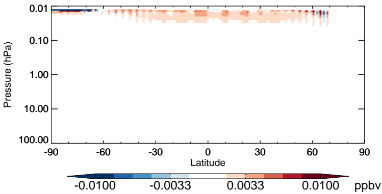
v11-02b-HP - v11-02a NO 3 - Strat zonal mean abs diff for Jul
