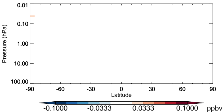
v11-02b-HP - v11-02a ClNO2 - Strat zonal mean abs diff for Jul
