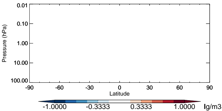
v11-02b-HP - v11-02a SO 2 - Strat zonal mean abs diff for Jul
