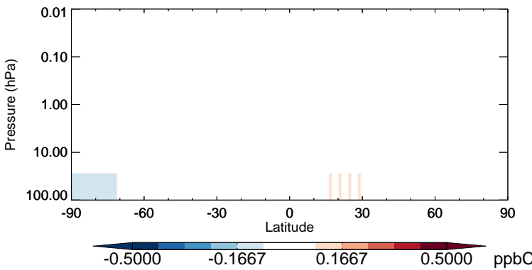
v11-02b-HP - v11-02a ACET - Strat zonal mean abs diff for Jul
