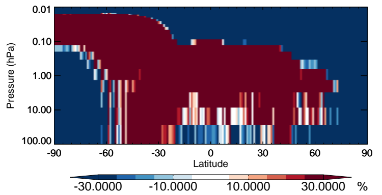
v11-02b-HP / v11-02a MACR - Strat zonal mean % diff for Jul
