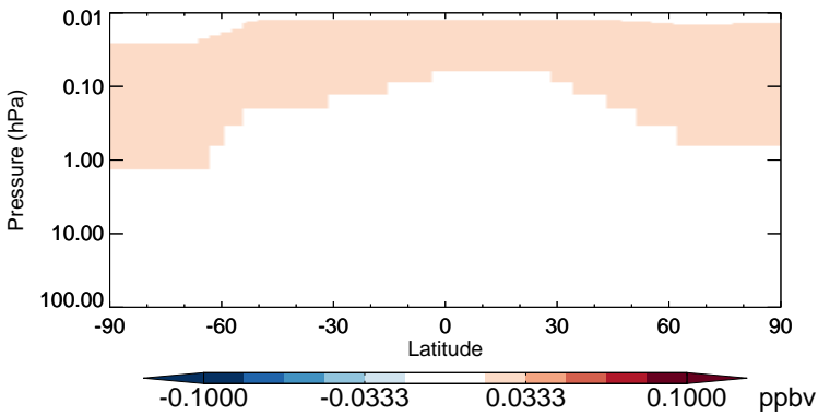
v11-02b-HP - v11-02a CFC115 - Strat zonal mean abs diff for Jul
