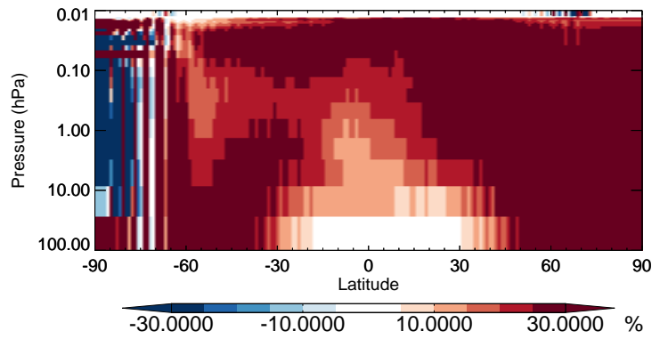
v11-02b-HP / v11-02a BrO - Strat zonal mean % diff for Jul
