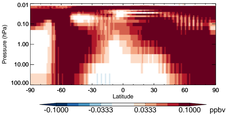
v11-02b-HP - v11-02a HCl - Strat zonal mean abs diff for Jul
