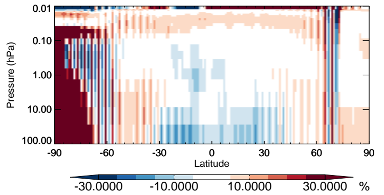
v11-02b-HP / v11-02a NO 3 - Strat zonal mean % diff for Jul
