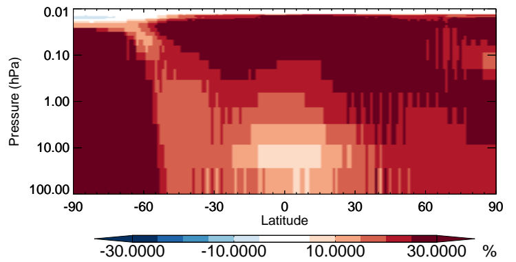
v11-02b-HP / v11-02a HBr - Strat zonal mean % diff for Jul
