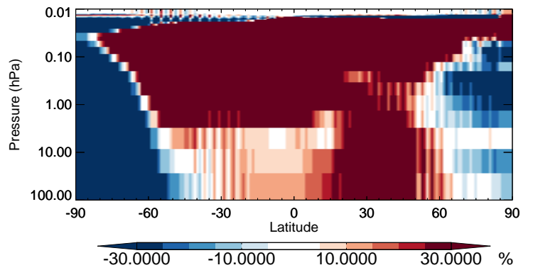
v11-02b-HP / v11-02a ACET - Strat zonal mean % diff for Jul
