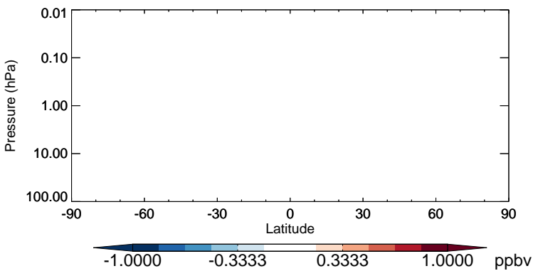
v11-02b-HP - v11-02a HNO 2 - Strat zonal mean abs diff for Jul
