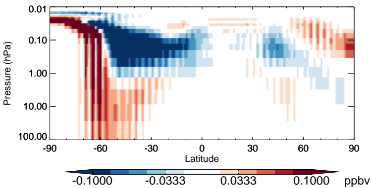
v11-02b-HP - v11-02a ClNO3 - Strat zonal mean abs diff for Jul
