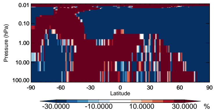
v11-02b-HP / v11-02a MOBA - Strat zonal mean % diff for Jul
