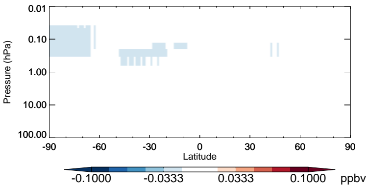
v11-02b-HP - v11-02a MPN - Strat zonal mean abs diff for Jul
