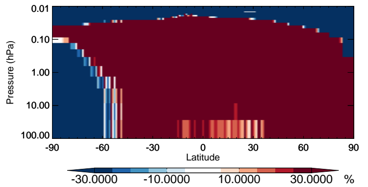
v11-02b-HP / v11-02a TOLU - Strat zonal mean % diff for Jul
