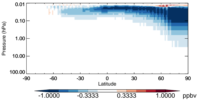
v11-02b-HP - v11-02a NO - Strat zonal mean abs diff for Jul
