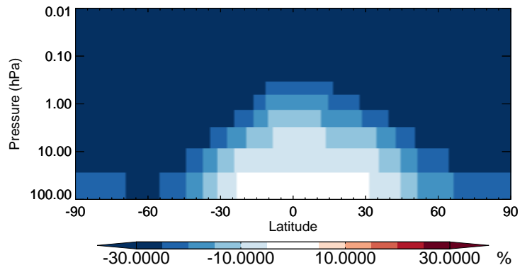
v11-02b-HP / v11-02a HCFC142b - Strat zonal mean % diff for Jul
