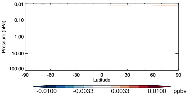
v11-02b-HP - v11-02a Br - Strat zonal mean abs diff for Jul
