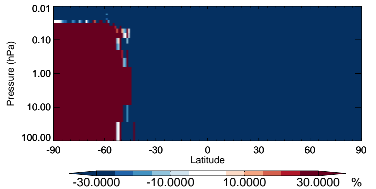
v11-02b-HP / v11-02a ClNO2 - Strat zonal mean % diff for Jul
