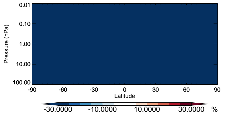
v11-02b-HP / v11-02a TSOA0 - Strat zonal mean % diff for Jul
