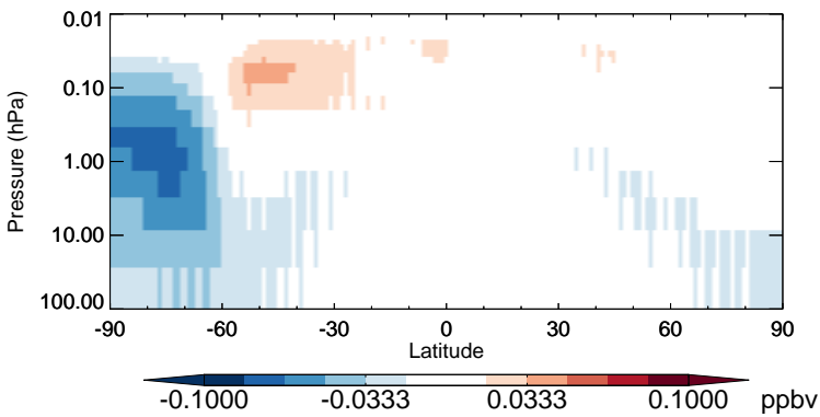
v11-02b-HP - v11-02a CH3Cl - Strat zonal mean abs diff for Jul
