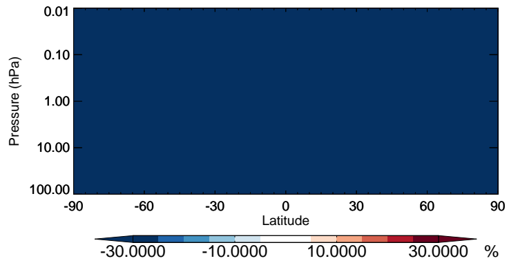
v11-02b-HP / v11-02a ISOA3 - Strat zonal mean % diff for Jul
