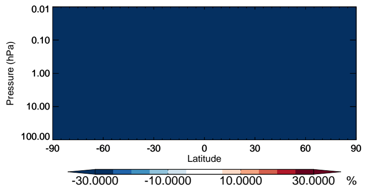
v11-02b-HP / v11-02a TSOA2 - Strat zonal mean % diff for Jul
