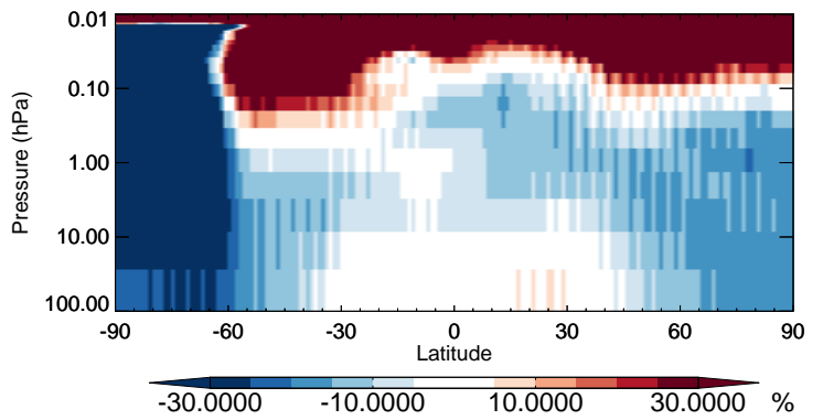
v11-02b-HP / v11-02a C2H6 - Strat zonal mean % diff for Jul
