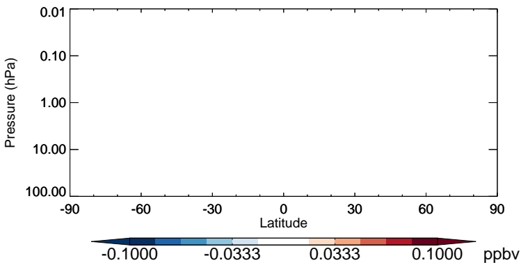
v11-02b-HP - v11-02a PAN - Strat zonal mean abs diff for Jul
