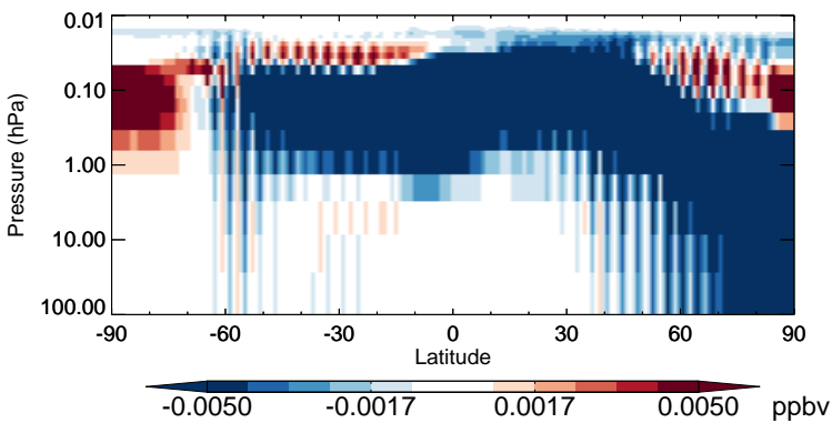
v11-02b-HP - v11-02a HNO4 - Strat zonal mean abs diff for Jul
