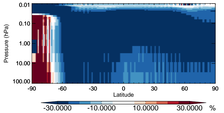
v11-02b-HP / v11-02a HNO 3 - Strat zonal mean % diff for Jul
