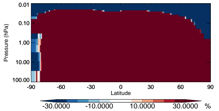
v11-02b-HP / v11-02a OCPO - Strat zonal mean % diff for Jul
