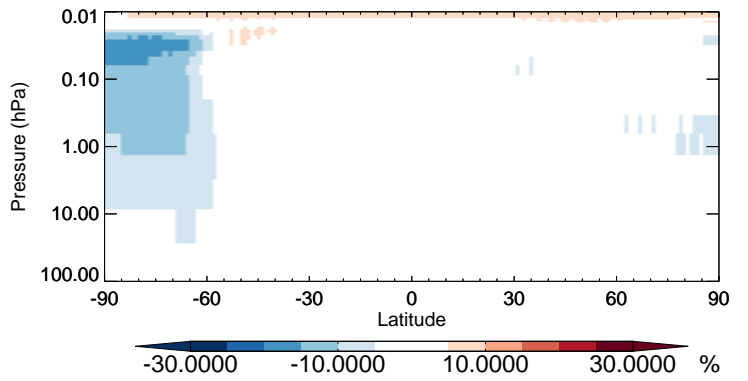
v11-02b-HP / v11-02a HCFC22 - Strat zonal mean % diff for Jul
