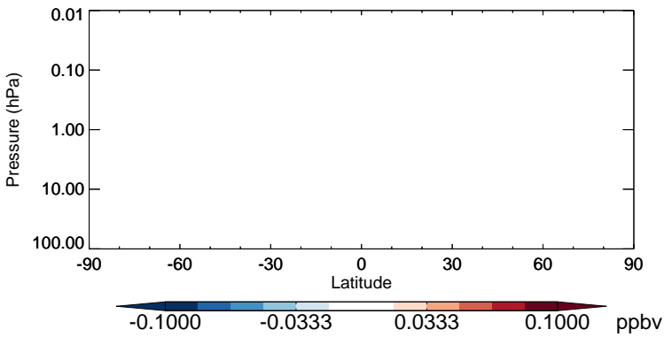
v11-02b-HP - v11-02a H1211 - Strat zonal mean abs diff for Jul
