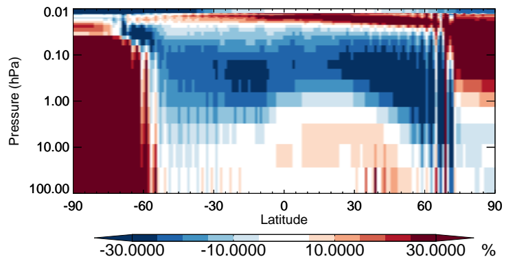
v11-02b-HP / v11-02a BrCl - Strat zonal mean % diff for Jul
