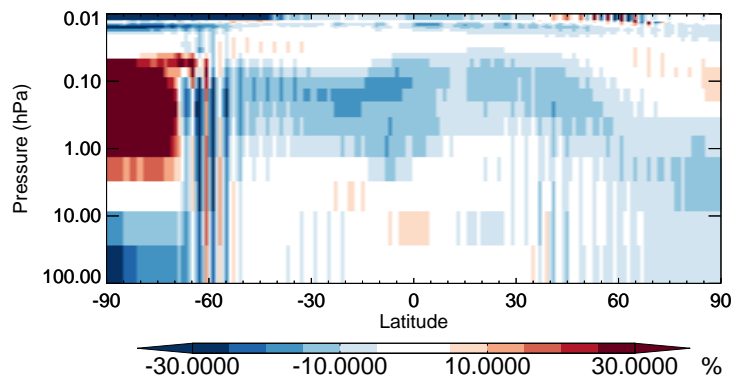
v11-02b-HP / v11-02a HNO4 - Strat zonal mean % diff for Jul
