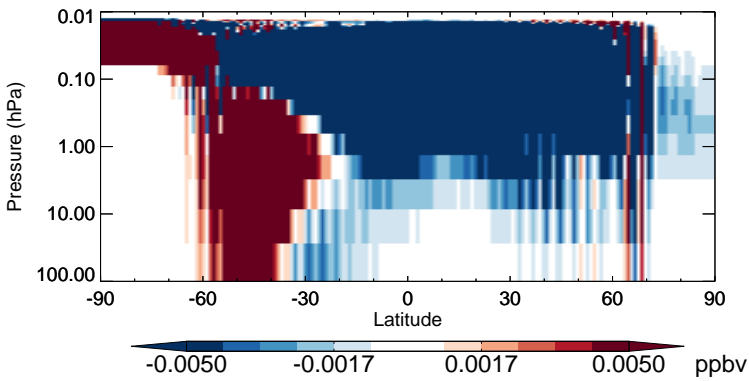
v11-02b-HP - v11-02a N2O5 - Strat zonal mean abs diff for Jul
