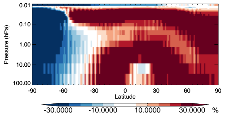
v11-02b-HP / v11-02a MP - Strat zonal mean % diff for Jul
