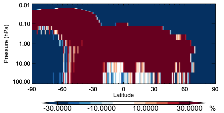
v11-02b-HP / v11-02a PMN - Strat zonal mean % diff for Jul
