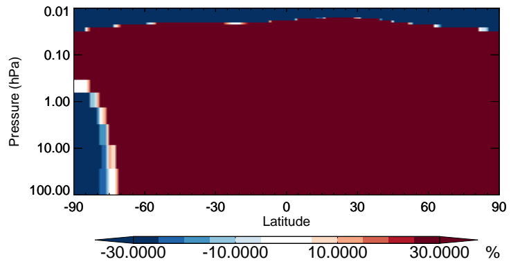
v11-02b-HP / v11-02a DST3 - Strat zonal mean % diff for Jul
