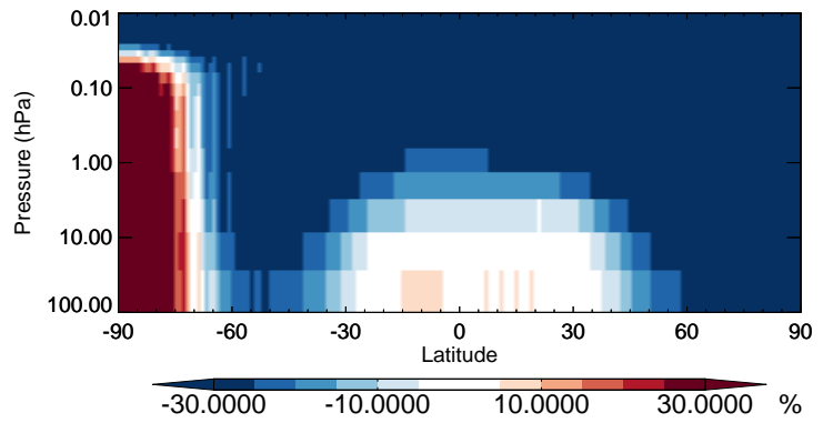
v11-02b-HP / v11-02a ASOG3 - Strat zonal mean % diff for Jul
