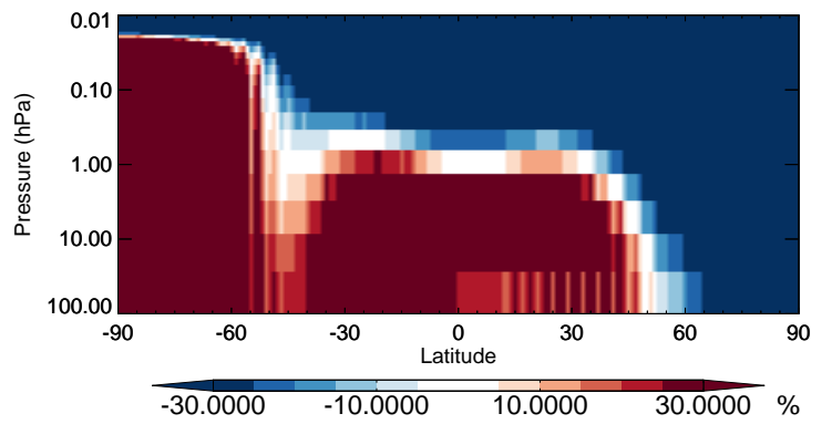
v11-02b-HP / v11-02a ASOG1 - Strat zonal mean % diff for Jul
