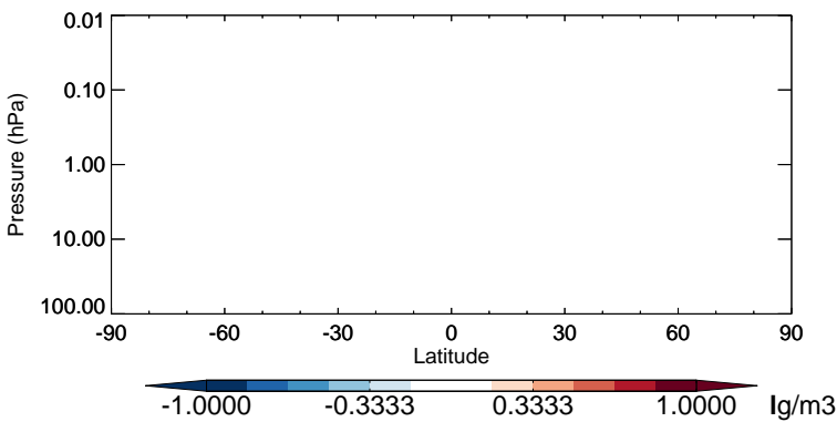
v11-02b-HP - v11-02a MSA - Strat zonal mean abs diff for Jul
