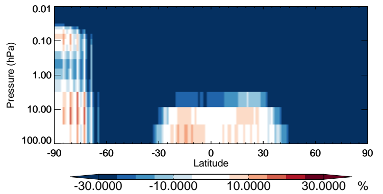
v11-02b-HP / v11-02a ASOG2 - Strat zonal mean % diff for Jul
