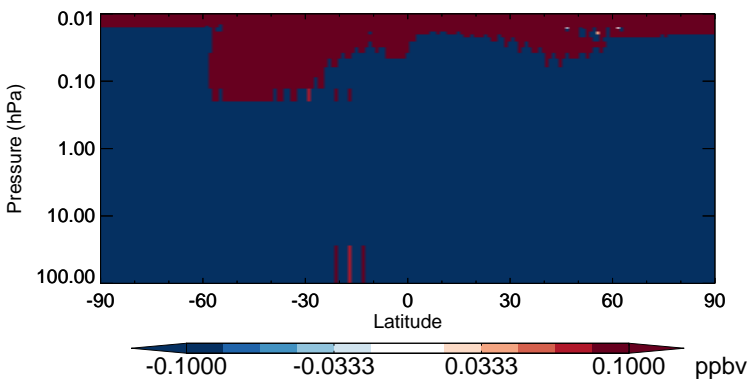
v11-02b-HP - v11-02a CH4 - Strat zonal mean abs diff for Jul
