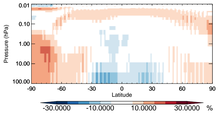
v11-02b-HP / v11-02a O3 - Strat zonal mean % diff for Jul
