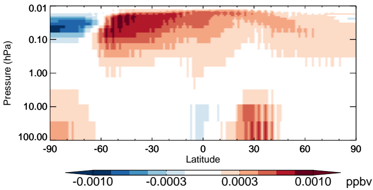
v11-02b-HP - v11-02a PPN - Strat zonal mean abs diff for Jul
