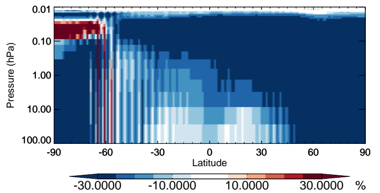
v11-02b-HP / v11-02a HNO 2 - Strat zonal mean % diff for Jul
