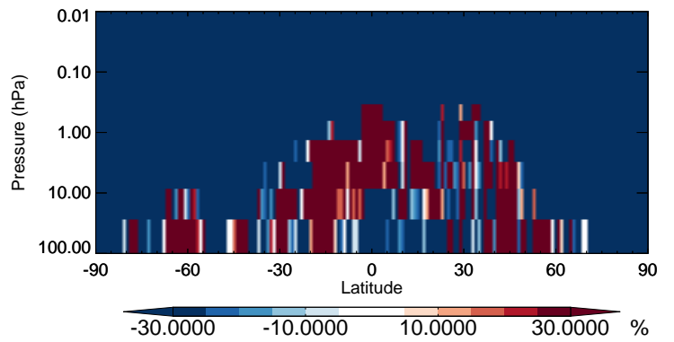
v11-02b-HP / v11-02a MTPA - Strat zonal mean % diff for Jul
