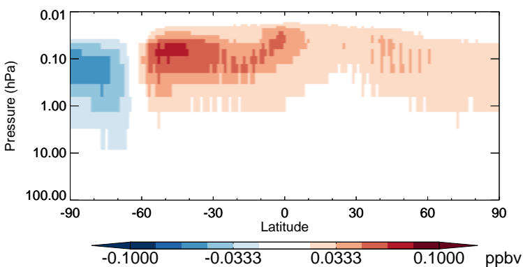
v11-02b-HP - v11-02a CFC12 - Strat zonal mean abs diff for Jul
