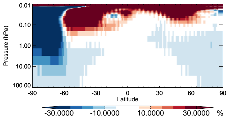
v11-02b-HP / v11-02a H1301 - Strat zonal mean % diff for Jul
