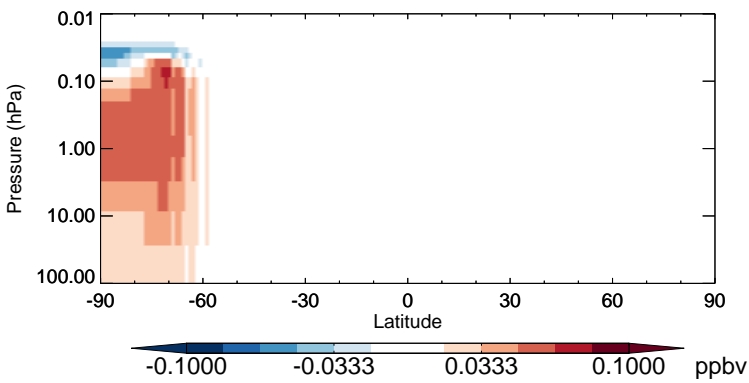
v11-02b-HP - v11-02a OCIO - Strat zonal mean abs diff for Jul
