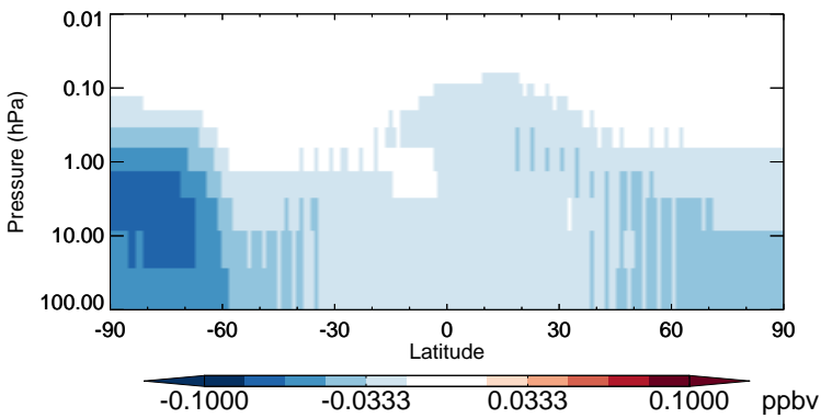
v11-02b-HP - v11-02a EOH - Strat zonal mean abs diff for Jul
