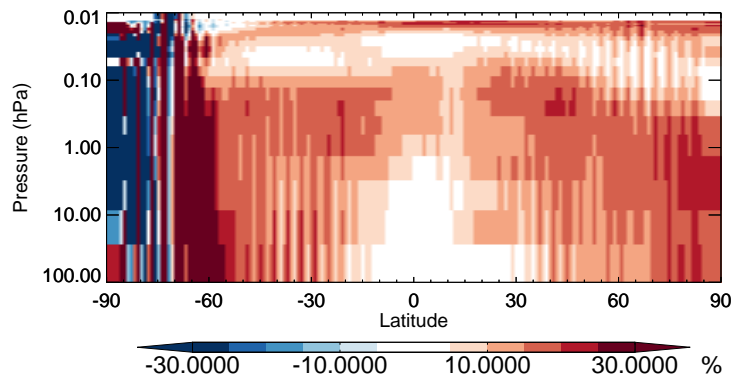
v11-02b-HP / v11-02a Br - Strat zonal mean % diff for Jul
