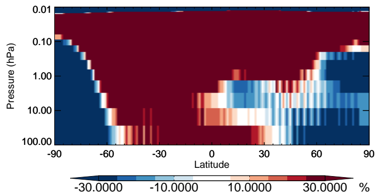
v11-02b-HP / v11-02a DST1 - Strat zonal mean % diff for Jul
