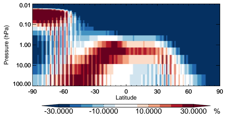
v11-02b-HP / v11-02a TSOG0 - Strat zonal mean % diff for Jul
