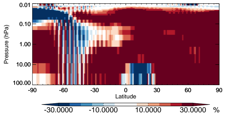
v11-02b-HP / v11-02a Cl 2 O 2 - Strat zonal mean % diff for Jul
