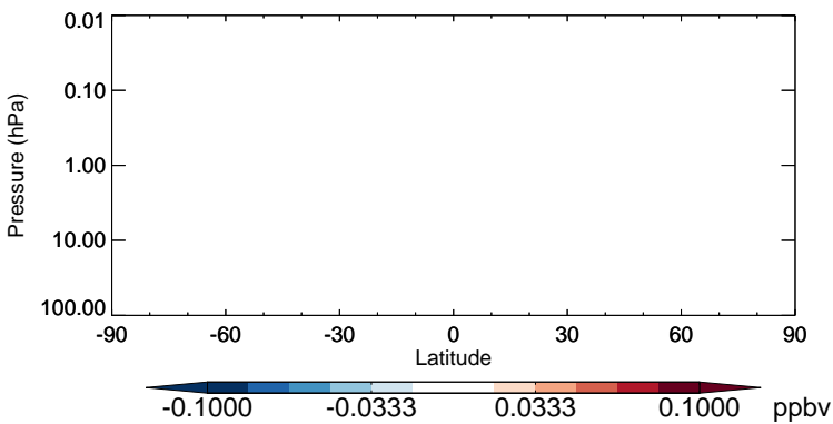
v11-02b-HP - v11-02a H 2 O 2 - Strat zonal mean abs diff for Jul
