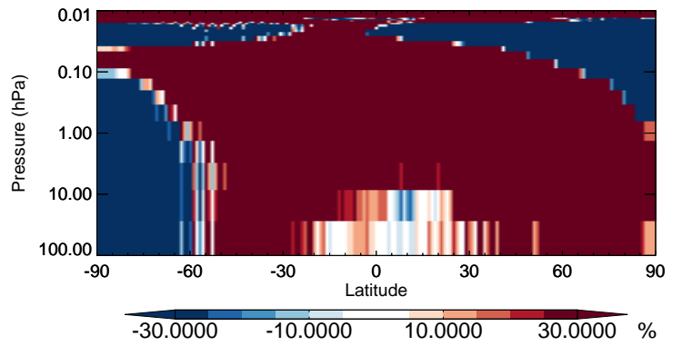
v11-02b-HP / v11-02a MVKN - Strat zonal mean % diff for Jul
