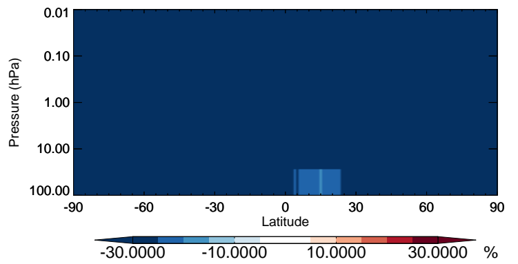
v11-02b-HP / v11-02a OCPI - Strat zonal mean % diff for Jul
