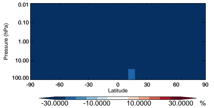
v11-02b-HP / v11-02a ASOA2 - Strat zonal mean % diff for Jul
