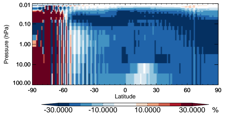
v11-02b-HP / v11-02a NO - Strat zonal mean % diff for Jul
