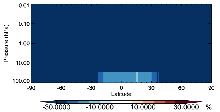
v11-02b-HP / v11-02a ASOAN - Strat zonal mean % diff for Jul
