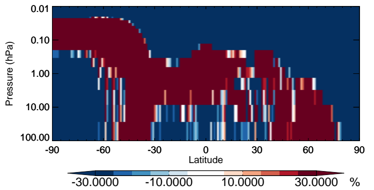
v11-02b-HP / v11-02a ISOP - Strat zonal mean % diff for Jul
