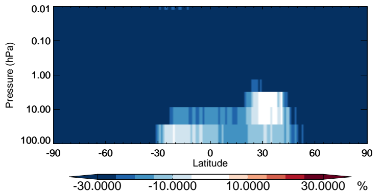
v11-02b-HP / v11-02a SO 4 - Strat zonal mean % diff for Jul
