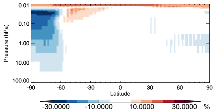
v11-02b-HP / v11-02a CH4 - Strat zonal mean % diff for Jul
