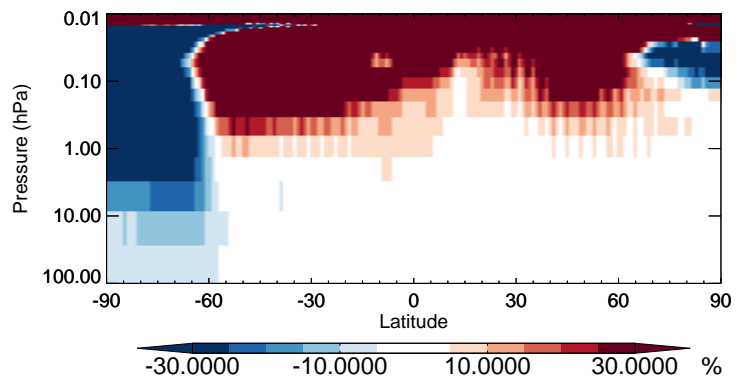
v11-02b-HP / v11-02a CH 3 Br - Strat zonal mean % diff for Jul
