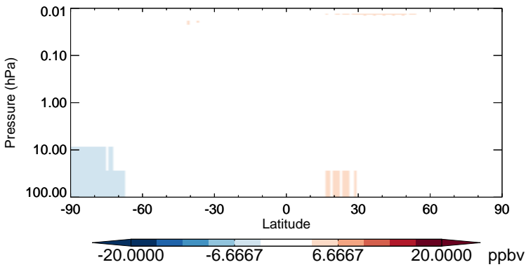
v11-02b-HP - v11-02a CO - Strat zonal mean abs diff for Jul
