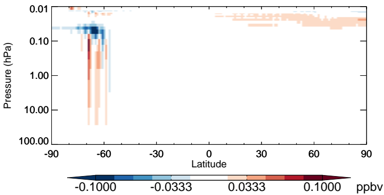
v11-02b-HP - v11-02a ClO - Strat zonal mean abs diff for Jul
