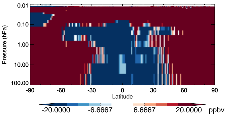
v11-02b-HP - v11-02a O3 - Strat zonal mean abs diff for Jul
