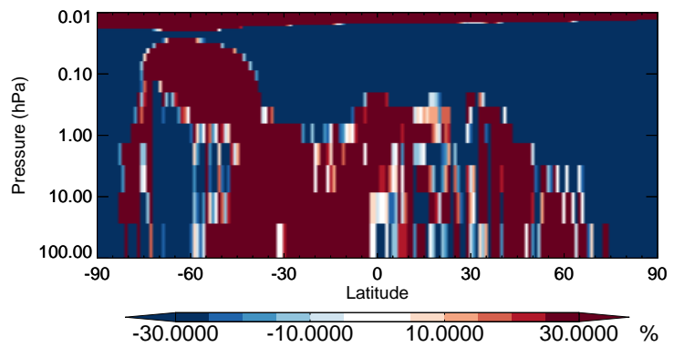
v11-02b-HP / v11-02a ISOPNB - Strat zonal mean % diff for Jul
