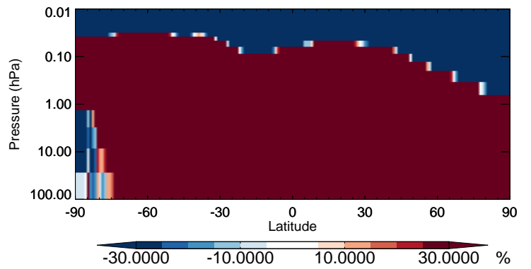
v11-02b-HP / v11-02a NITs - Strat zonal mean % diff for Jul
