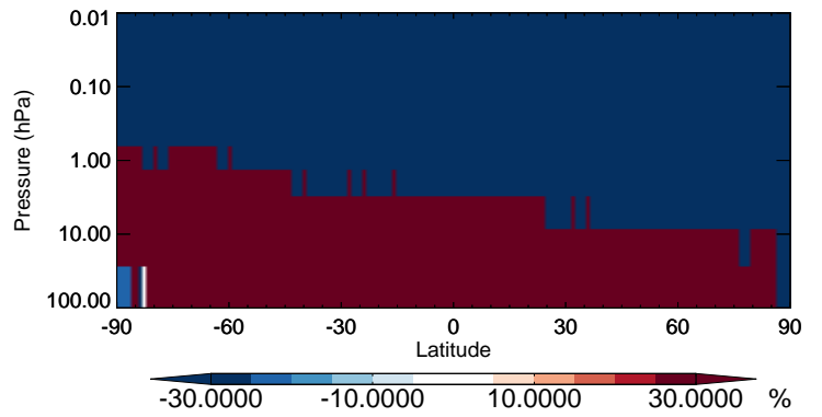
v11-02b-HP / v11-02a SO 4 s - Strat zonal mean % diff for Jul
