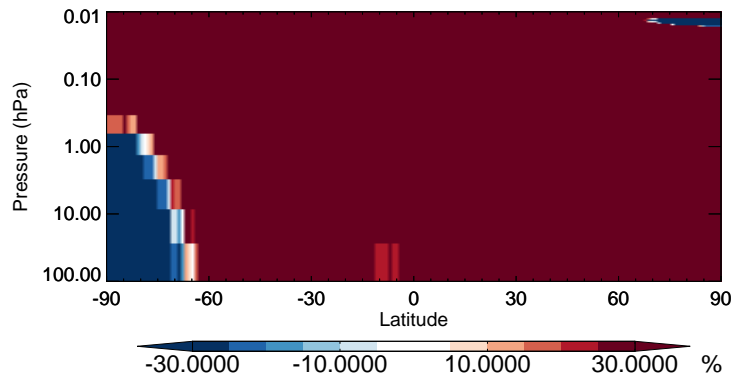
v11-02b-HP / v11-02a SALC - Strat zonal mean % diff for Jul
