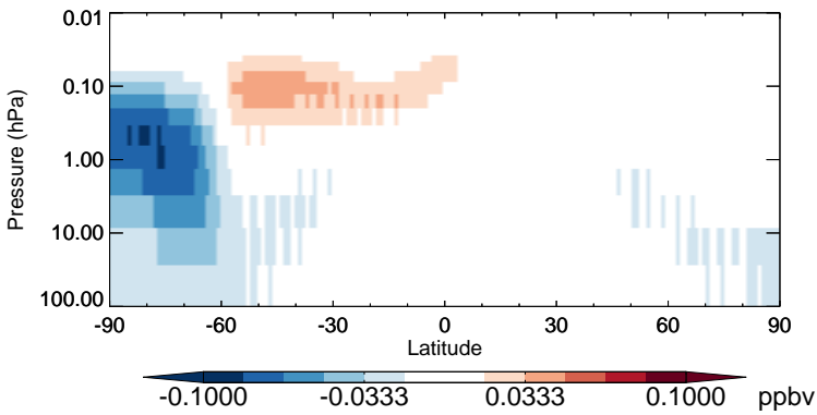
v11-02b-HP - v11-02a OCS - Strat zonal mean abs diff for Jul
