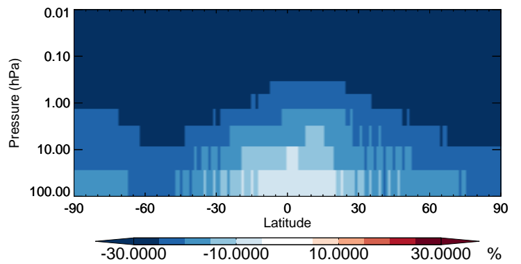
v11-02b-HP / v11-02a MSA - Strat zonal mean % diff for Jul
