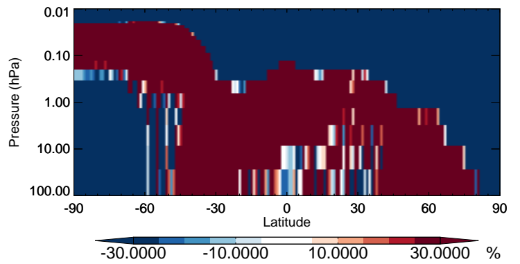
v11-02b-HP / v11-02a RIP - Strat zonal mean % diff for Jul
