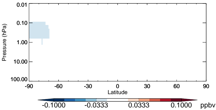
v11-02b-HP - v11-02a HCFC22 - Strat zonal mean abs diff for Jul
