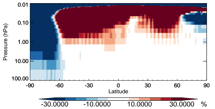
v11-02b-HP / v11-02a H1211 - Strat zonal mean % diff for Jul
