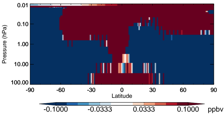
v11-02b-HP - v11-02a N 2 O - Strat zonal mean abs diff for Jul
