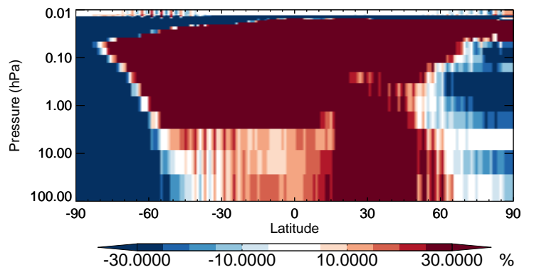
v11-02b-HP / v11-02a R4N2 - Strat zonal mean % diff for Jul
