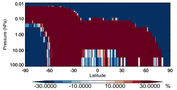
v11-02b-HP / v11-02a MVK - Strat zonal mean % diff for Jul
