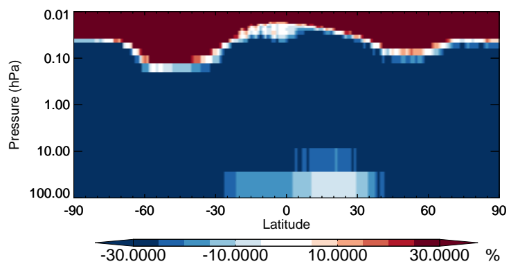
v11-02b-HP / v11-02a SALA - Strat zonal mean % diff for Jul
