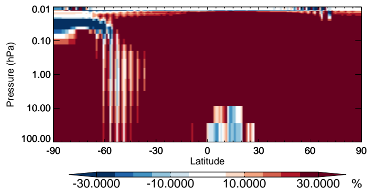
v11-02b-HP / v11-02a OCIO - Strat zonal mean % diff for Jul
