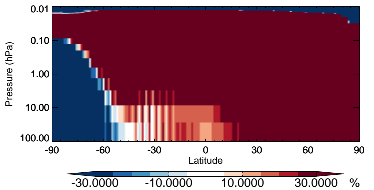
v11-02b-HP / v11-02a ALK4 - Strat zonal mean % diff for Jul
