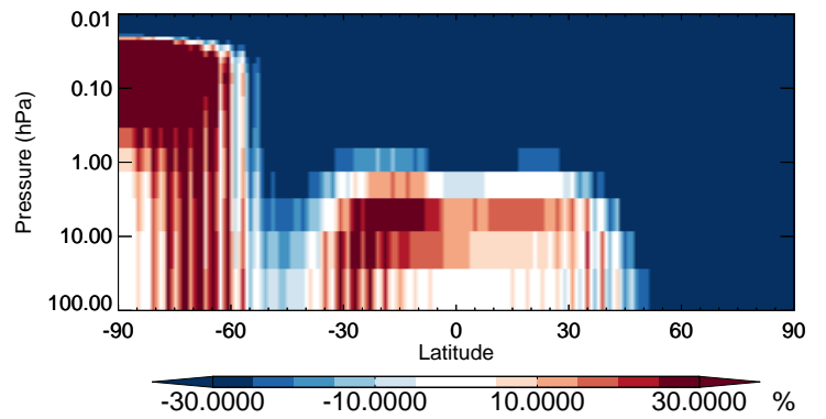
v11-02b-HP / v11-02a TSOG1 - Strat zonal mean % diff for Jul
