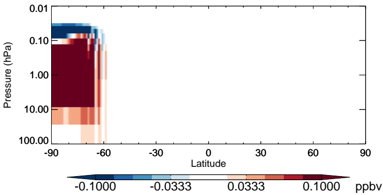
v11-02b-HP - v11-02a Cl 2 O 2 - Strat zonal mean abs diff for Jul
