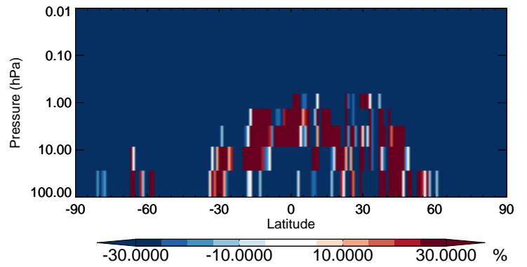
v11-02b-HP / v11-02a LIMO - Strat zonal mean % diff for Jul
