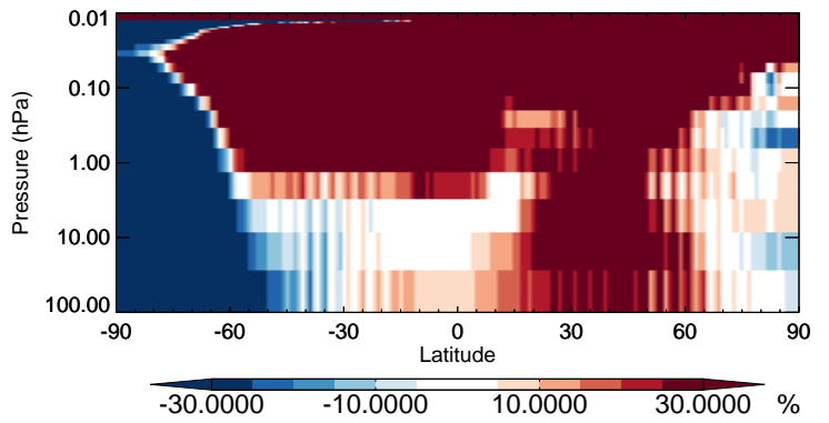
v11-02b-HP / v11-02a C3H8 - Strat zonal mean % diff for Jul
