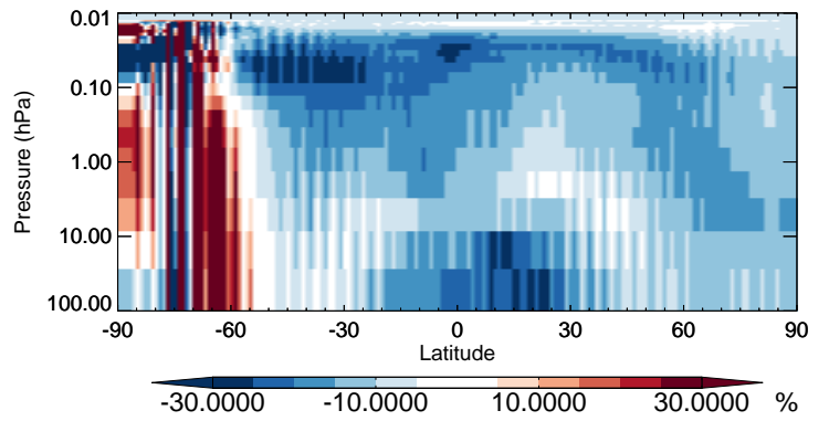
v11-02b-HP / v11-02a ClOO - Strat zonal mean % diff for Jul
