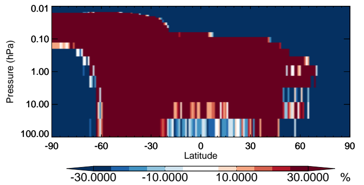
v11-02b-HP / v11-02a PRPE - Strat zonal mean % diff for Jul
