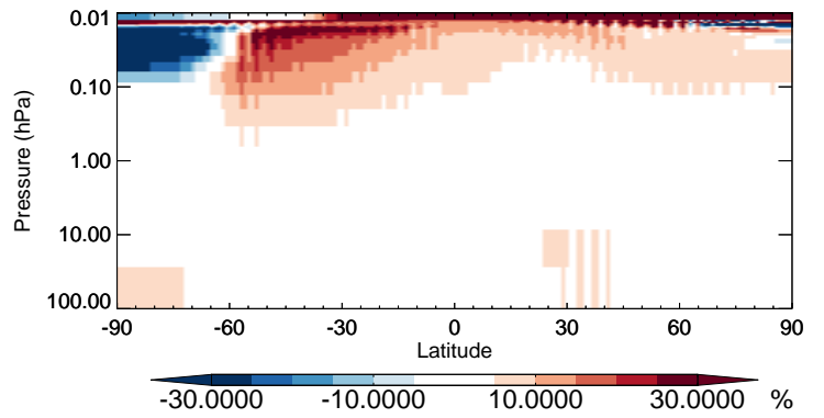
v11-02b-HP / v11-02a PPN - Strat zonal mean % diff for Jul
