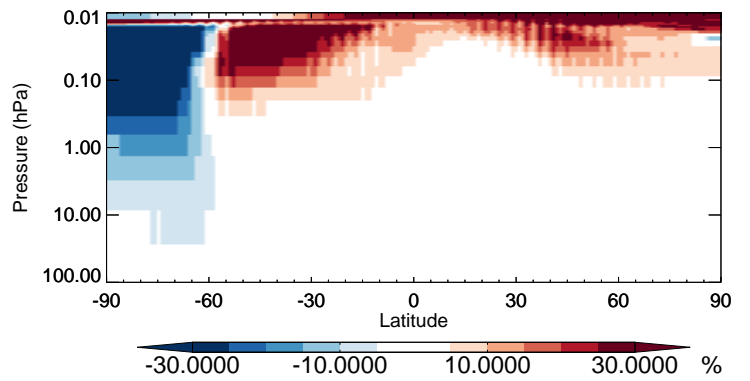
v11-02b-HP / v11-02a N 2 O - Strat zonal mean % diff for Jul
