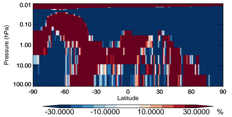
v11-02b-HP / v11-02a ISOPND - Strat zonal mean % diff for Jul
