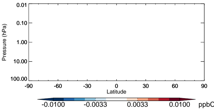
v11-02b-HP - v11-02a PRPE - Strat zonal mean abs diff for Jul
