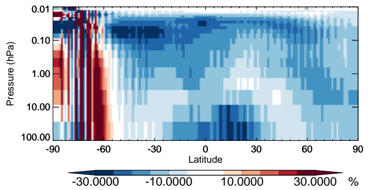
v11-02b-HP / v11-02a Cl - Strat zonal mean % diff for Jul
