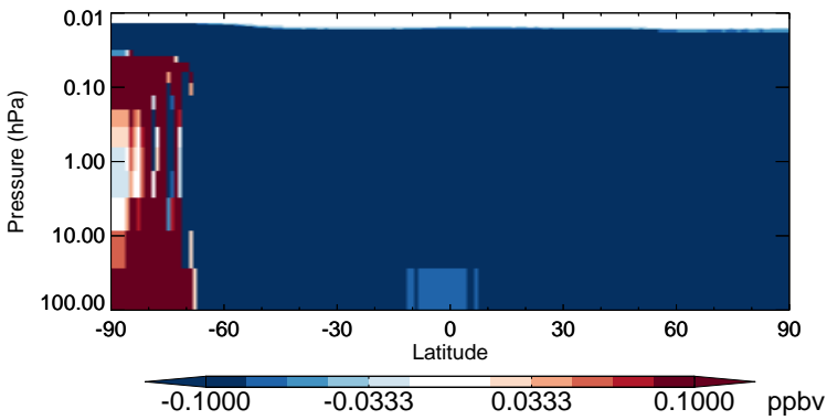
v11-02b-HP - v11-02a HNO 3 - Strat zonal mean abs diff for Jul
