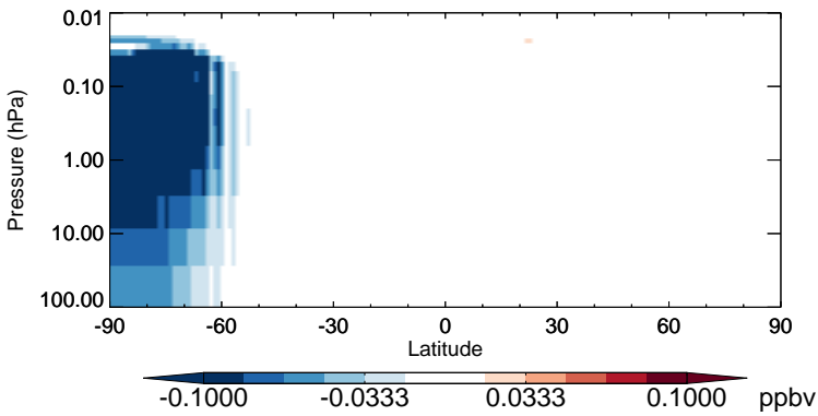
v11-02b-HP - v11-02a HOCl - Strat zonal mean abs diff for Jul
