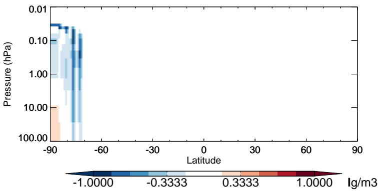
v11-02b-HP - v11-02a NIT - Strat zonal mean abs diff for Jul
