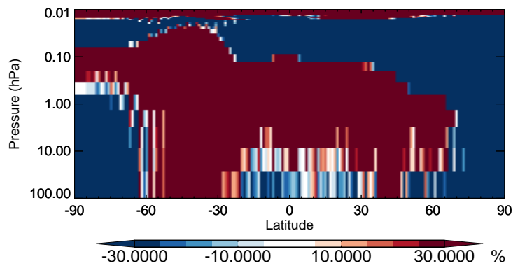
v11-02b-HP / v11-02a MACRN - Strat zonal mean % diff for Jul
