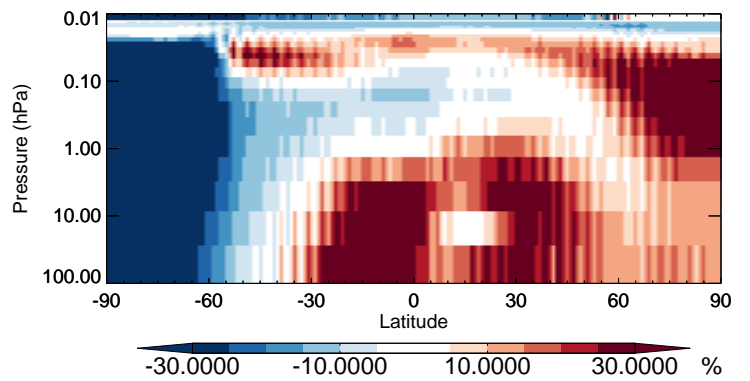
v11-02b-HP / v11-02a H 2 O 2 - Strat zonal mean % diff for Jul
