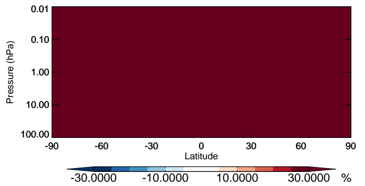
v11-02b-HP / v11-02a HCFC123 - Strat zonal mean % diff for Jul
