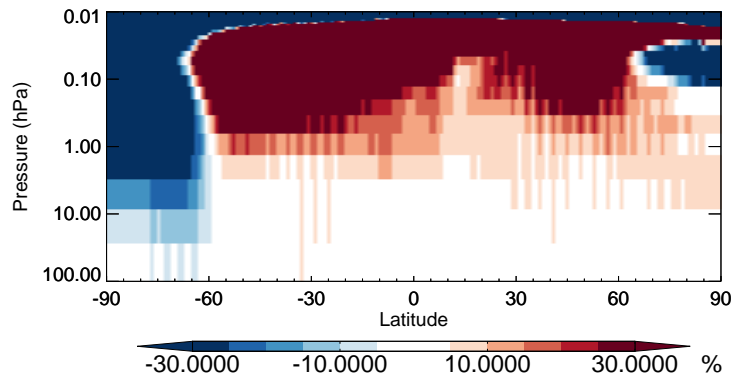
v11-02b-HP / v11-02a H2402 - Strat zonal mean % diff for Jul
