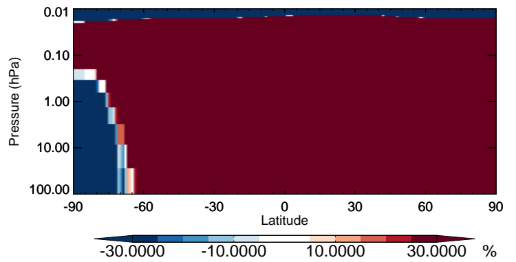
v11-02b-HP / v11-02a DST2 - Strat zonal mean % diff for Jul
