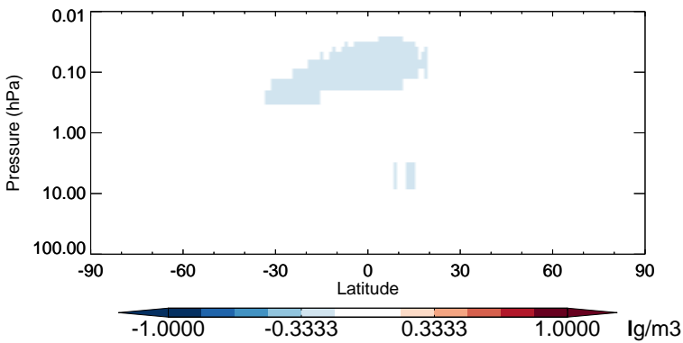
v11-02b-HP - v11-02a SO 4 - Strat zonal mean abs diff for Jul
