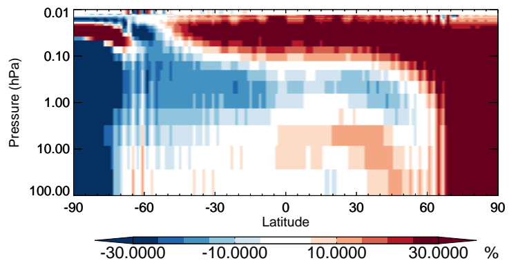
v11-02b-HP / v11-02a HOBr - Strat zonal mean % diff for Jul
