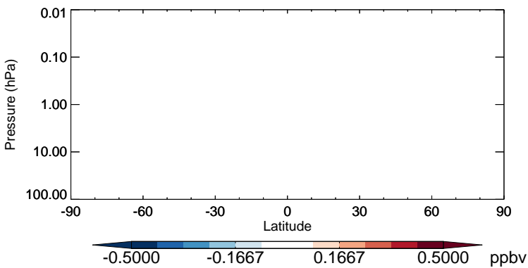
v11-02b-HP - v11-02a CH2O - Strat zonal mean abs diff for Jul
