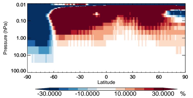
v11-02b-HP / v11-02a CCl4 - Strat zonal mean % diff for Jul
