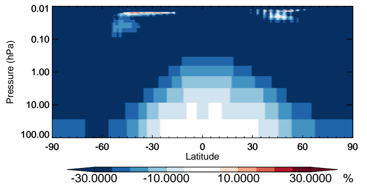
v11-02b-HP / v11-02a HCFC141b - Strat zonal mean % diff for Jul
