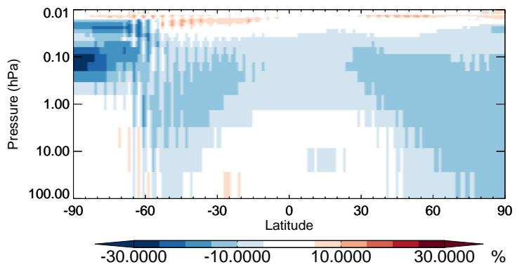
v11-02b-HP / v11-02a CH2O - Strat zonal mean % diff for Jul
