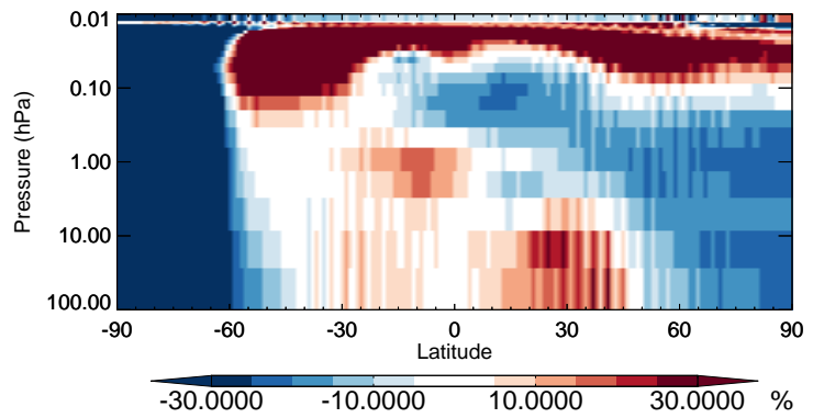
v11-02b-HP / v11-02a PAN - Strat zonal mean % diff for Jul
