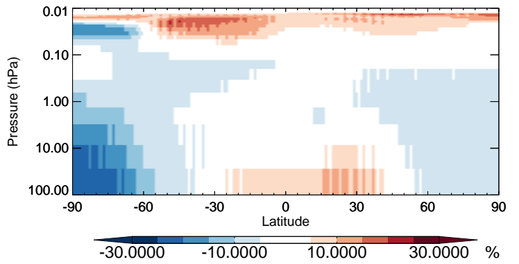
v11-02b-HP / v11-02a CO - Strat zonal mean % diff for Jul
