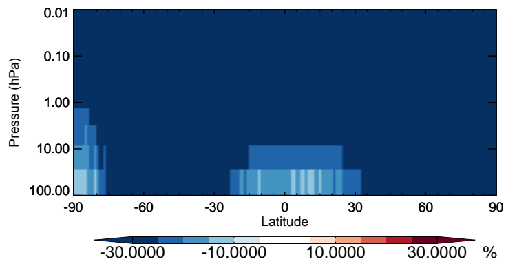
v11-02b-HP / v11-02a TSOG3 - Strat zonal mean % diff for Jul
