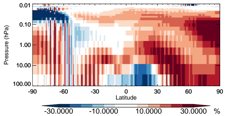
v11-02b-HP / v11-02a ClO - Strat zonal mean % diff for Jul
