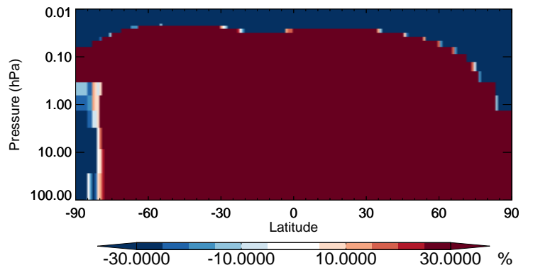
v11-02b-HP / v11-02a BCPO - Strat zonal mean % diff for Jul
