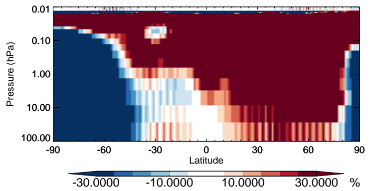
v11-02b-HP / v11-02a R4N2 - Strat zonal mean % diff for Oct
