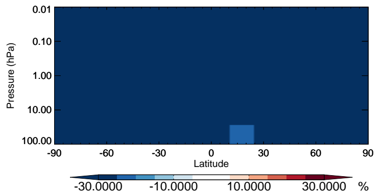
v11-02b-HP / v11-02a ASOAN - Strat zonal mean % diff for Oct
