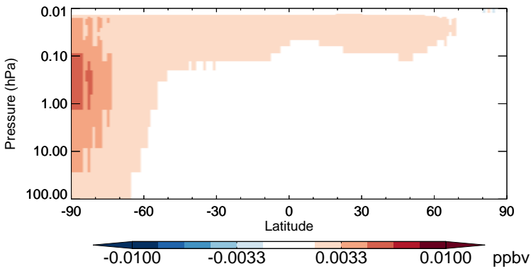
v11-02b-HP - v11-02a BrO - Strat zonal mean abs diff for Oct
