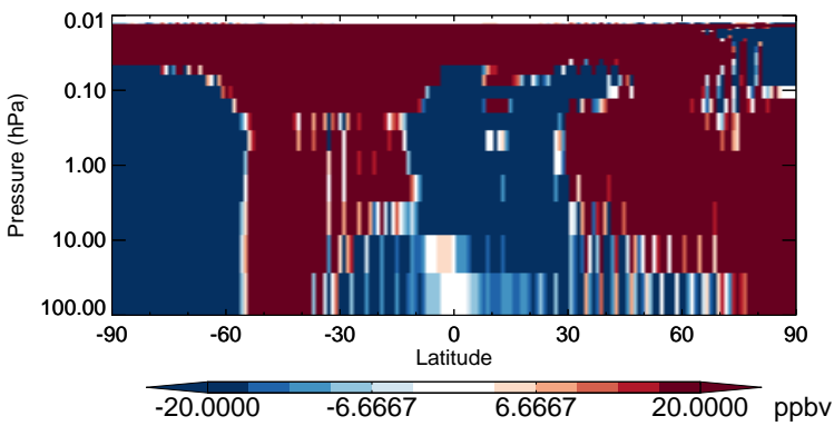
v11-02b-HP - v11-02a O3 - Strat zonal mean abs diff for Oct
