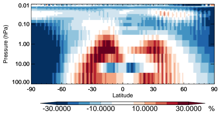
v11-02b-HP / v11-02a H 2 O 2 - Strat zonal mean % diff for Oct
