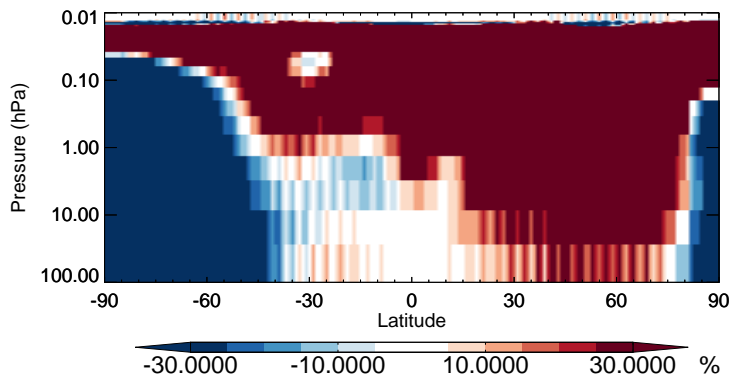
v11-02b-HP / v11-02a ACET - Strat zonal mean % diff for Oct
