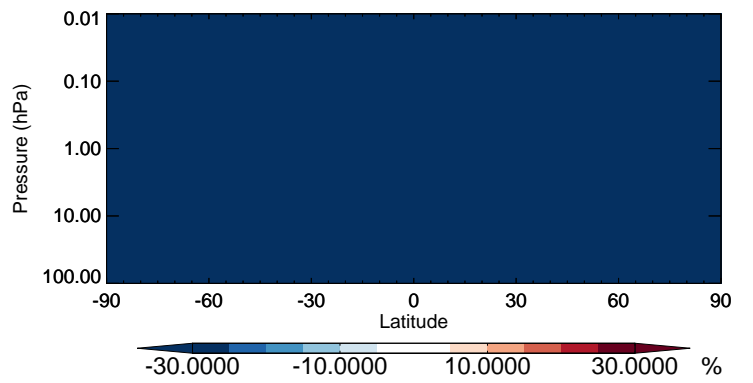
v11-02b-HP / v11-02a ISOA1 - Strat zonal mean % diff for Oct
