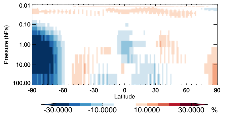
v11-02b-HP / v11-02a O3 - Strat zonal mean % diff for Oct
