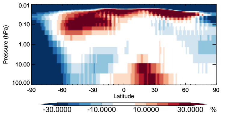
v11-02b-HP / v11-02a SO2 - Strat zonal mean % diff for Oct
