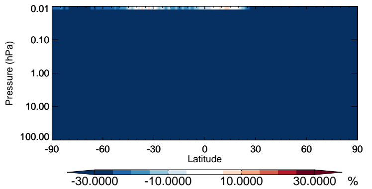
v11-02b-HP / v11-02a SO4 - Strat zonal mean % diff for Oct
