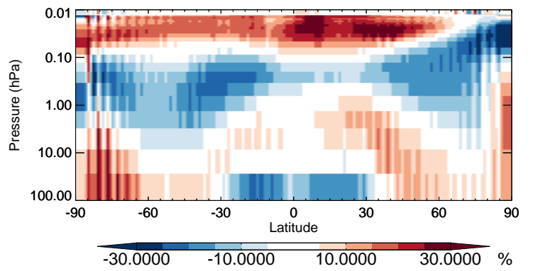
v11-02b-HP / v11-02a HOBr - Strat zonal mean % diff for Oct
