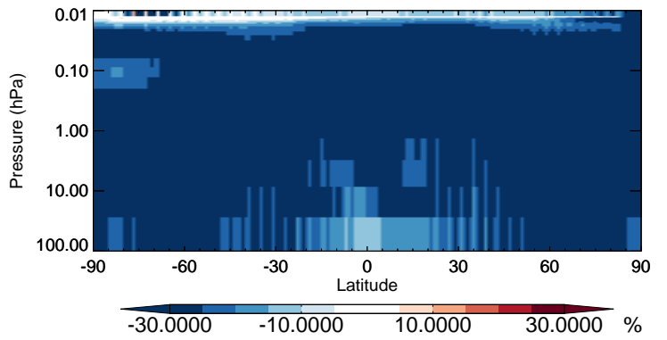
v11-02b-HP / v11-02a HNO 3 - Strat zonal mean % diff for Oct
