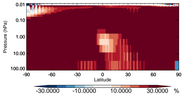
v11-02b-HP / v11-02a BrNO 3 - Strat zonal mean % diff for Oct
