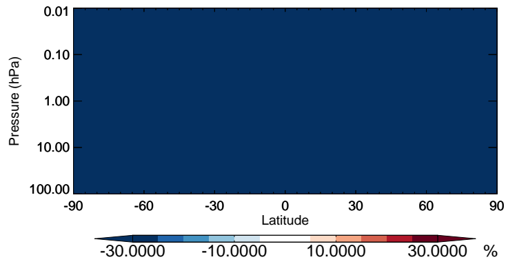
v11-02b-HP / v11-02a TSOA0 - Strat zonal mean % diff for Oct
