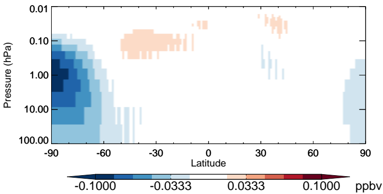
v11-02b-HP - v11-02a CH3Cl - Strat zonal mean abs diff for Oct
