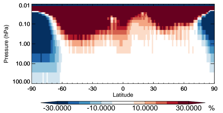
v11-02b-HP / v11-02a CCl4 - Strat zonal mean % diff for Oct
