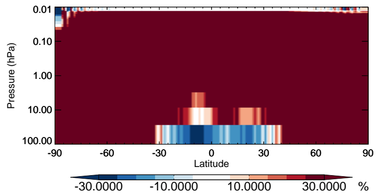
v11-02b-HP / v11-02a Br2 - Strat zonal mean % diff for Oct
