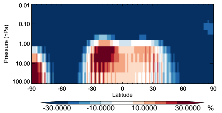
v11-02b-HP / v11-02a ISOG1 - Strat zonal mean % diff for Oct
