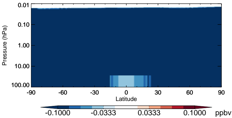
v11-02b-HP - v11-02a HNO 3 - Strat zonal mean abs diff for Oct
