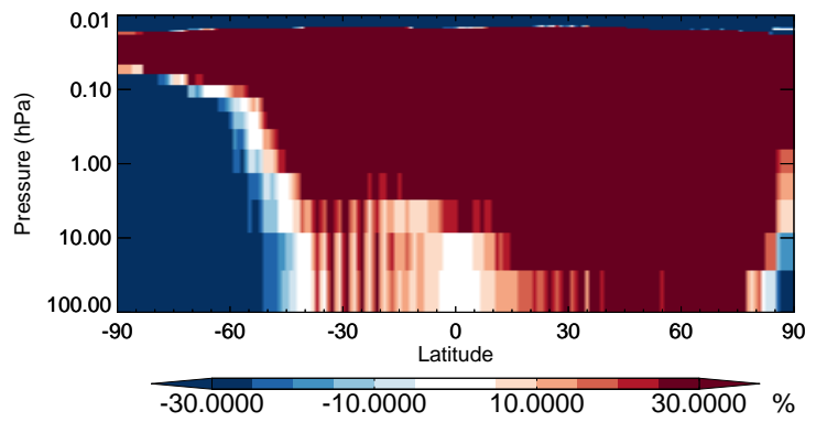
v11-02b-HP / v11-02a BENZ - Strat zonal mean % diff for Oct
