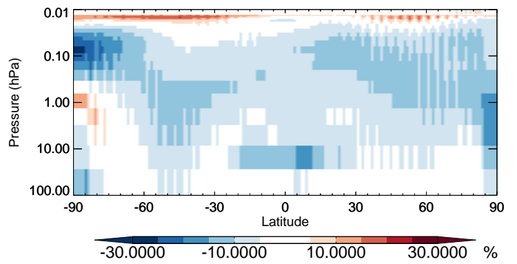
v11-02b-HP / v11-02a CH2O - Strat zonal mean % diff for Oct
