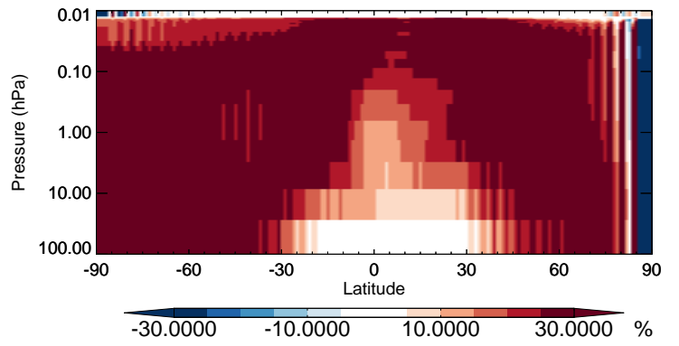
v11-02b-HP / v11-02a BrO - Strat zonal mean % diff for Oct
