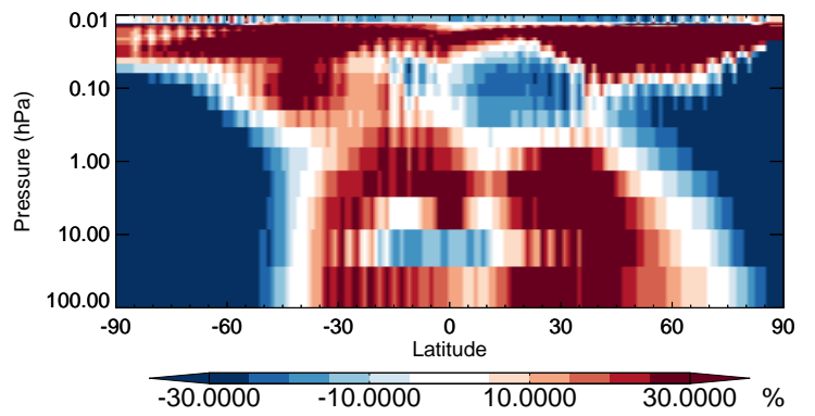
v11-02b-HP / v11-02a MAP - Strat zonal mean % diff for Oct
