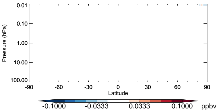
v11-02b-HP - v11-02a Cl - Strat zonal mean abs diff for Oct
