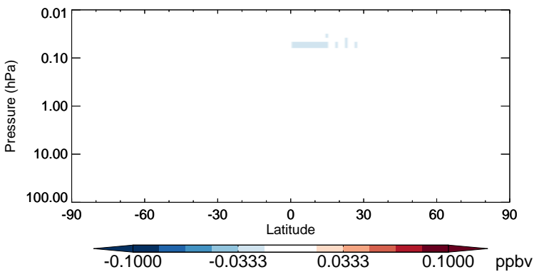
v11-02b-HP - v11-02a H 2 O 2 - Strat zonal mean abs diff for Oct
