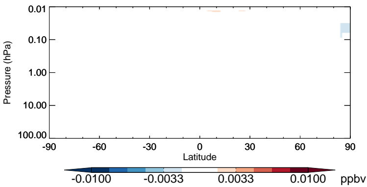
v11-02b-HP - v11-02a HOBr - Strat zonal mean abs diff for Oct
