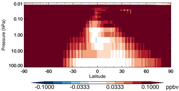
v11-02b-HP - v11-02a HCl - Strat zonal mean abs diff for Oct
