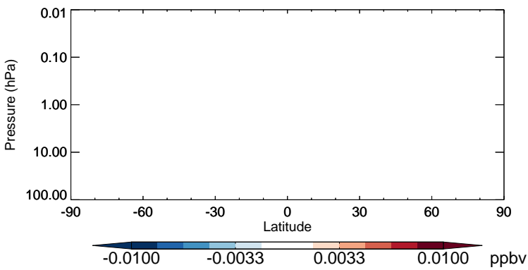
v11-02b-HP - v11-02a CH 3 Br - Strat zonal mean abs diff for Oct
