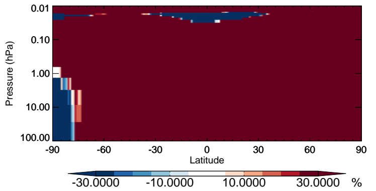
v11-02b-HP / v11-02a DMS - Strat zonal mean % diff for Oct
