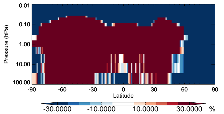
v11-02b-HP / v11-02a MACR - Strat zonal mean % diff for Oct
