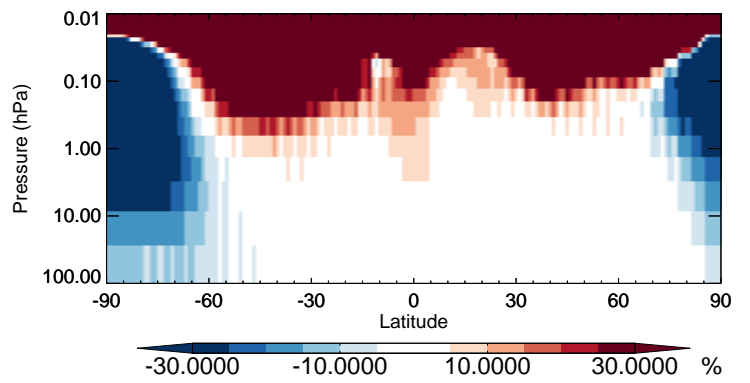
v11-02b-HP / v11-02a CH 3 Br - Strat zonal mean % diff for Oct
