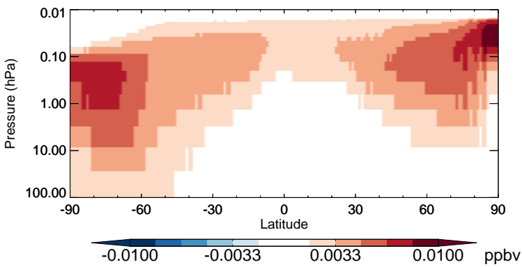
v11-02b-HP - v11-02a BrNO 3 - Strat zonal mean abs diff for Oct
