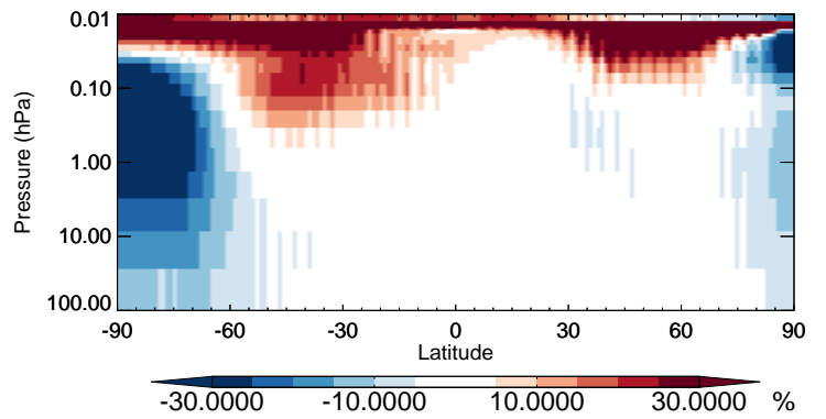
v11-02b-HP / v11-02a CH3Cl - Strat zonal mean % diff for Oct
