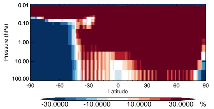
v11-02b-HP / v11-02a ALK4 - Strat zonal mean % diff for Oct
