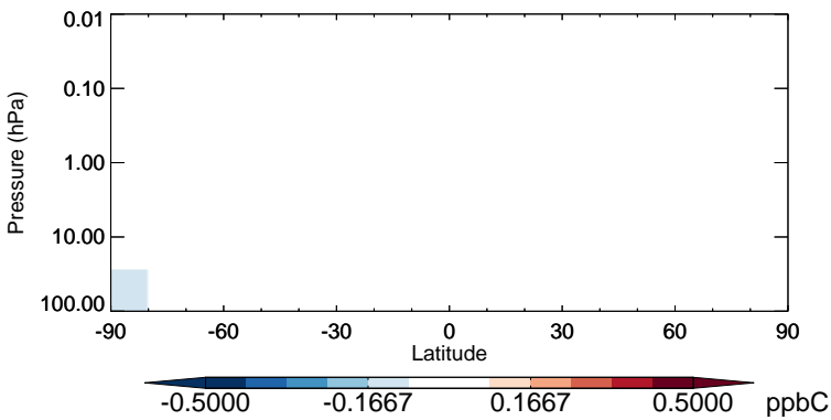
v11-02b-HP - v11-02a ACET - Strat zonal mean abs diff for Oct
