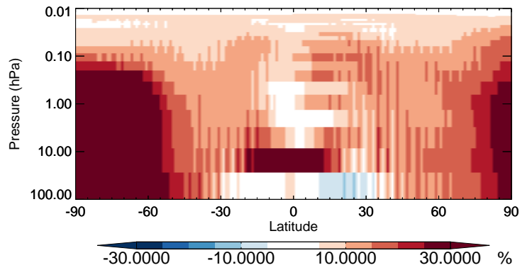
v11-02b-HP / v11-02a HCl - Strat zonal mean % diff for Oct
