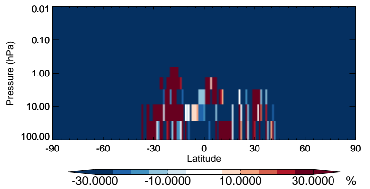
v11-02b-HP / v11-02a MTPO - Strat zonal mean % diff for Oct
