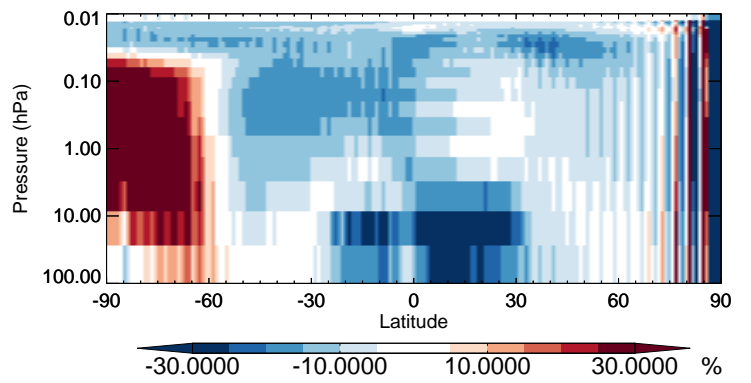
v11-02b-HP / v11-02a Cl - Strat zonal mean % diff for Oct
