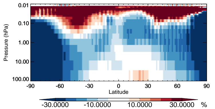
v11-02b-HP / v11-02a ALD2 - Strat zonal mean % diff for Oct
