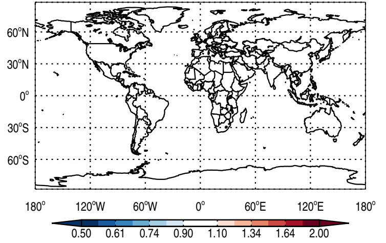
Ratio @ 500 hPa for PASV
