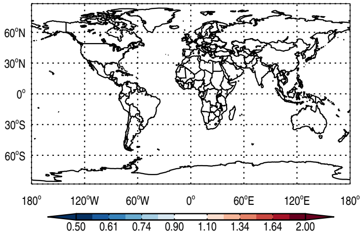
Ratio @ Surface for Rn
