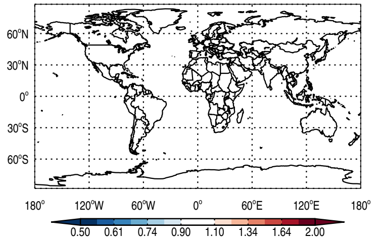
Ratio @ 500 hPa for Pb
