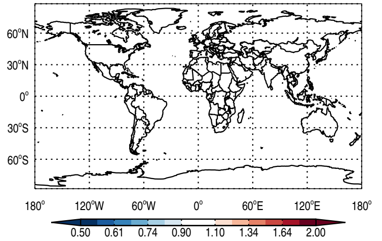
Ratio @ 500 hPa for Rn
