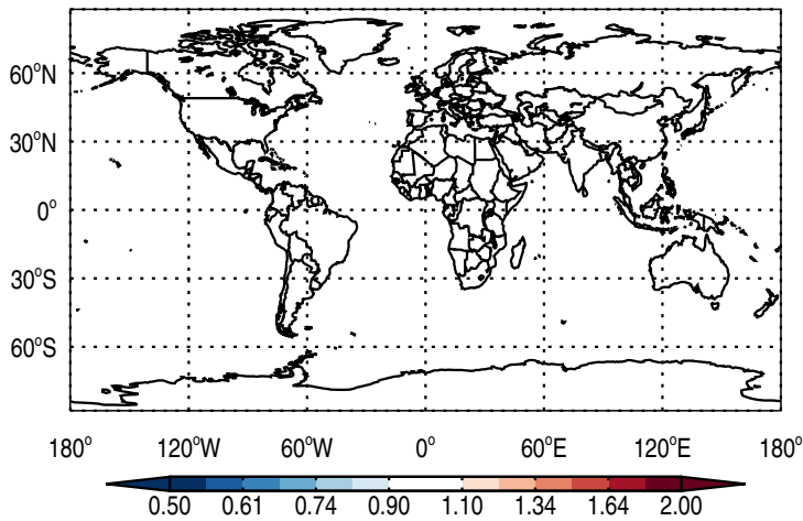
Ratio @ Surface for Pb
