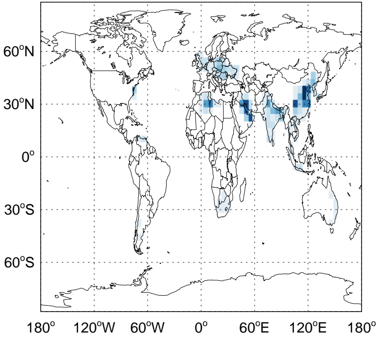
C3H8 column anth+biof emissions for Jan
