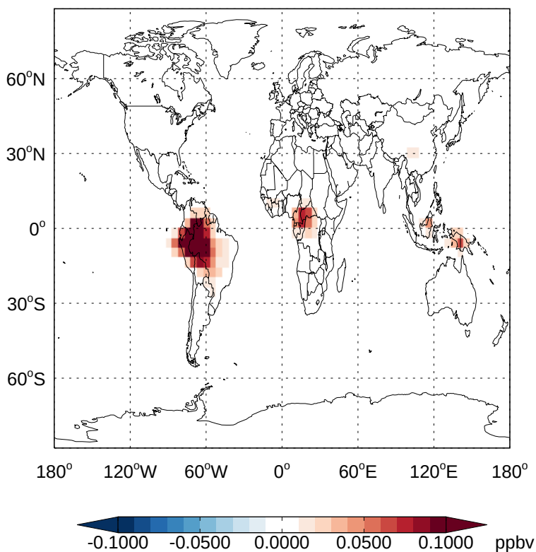
v11-02d - v11-02a IEPOXA- Diff @ 500 hPa for Apr
