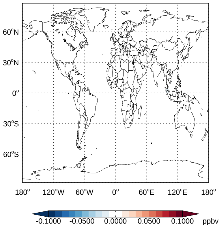
v11-02d - v11-02a MONITS - Diff @ Surface for Apr
