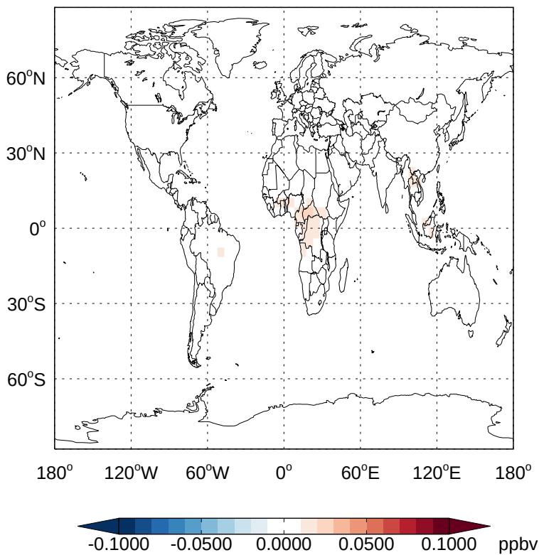
v11-02d - v11-02a LVOCOA - Diff @ Surface for Apr
