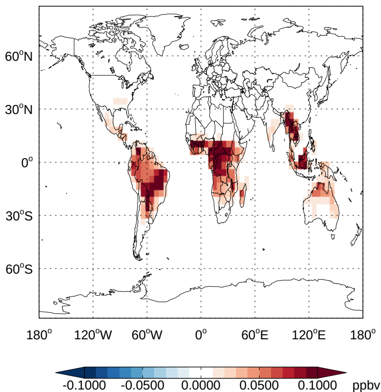
v11-02d - v11-02a IEPOXB - Diff @ Surface for Apr
