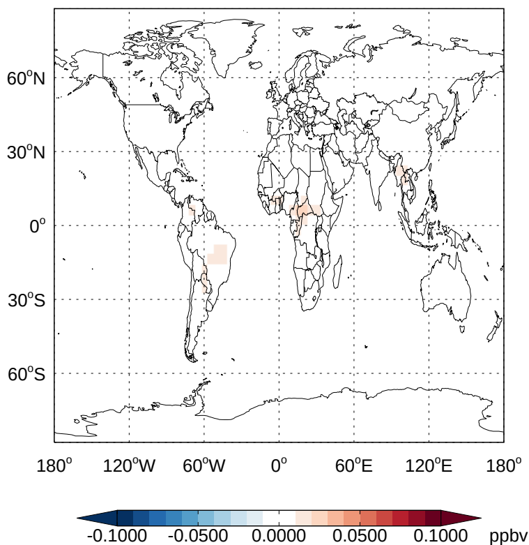
v11-02d - v11-02a IEPOXD - Diff @ Surface for Apr
