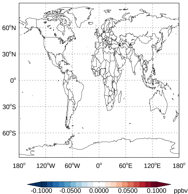
v11-02d - v11-02a MONITU - Diff @ Surface for Apr
