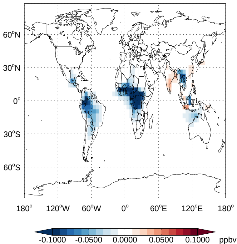
v11-02d - v11-02a SOAGX - Diff @ Surface for Apr
