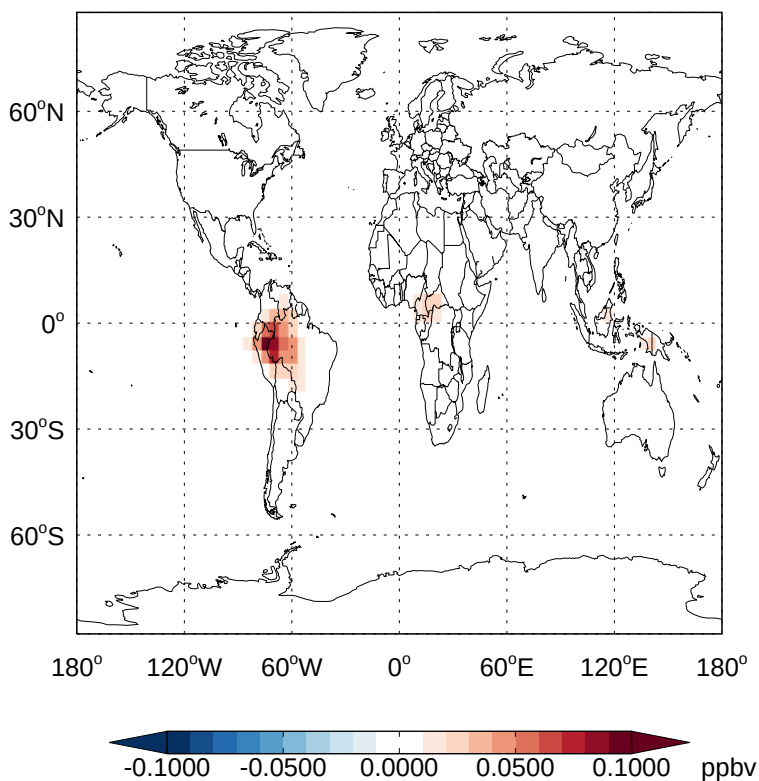
v11-02d - v11-02a IEPOXB- Diff @ 500 hPa for Apr
