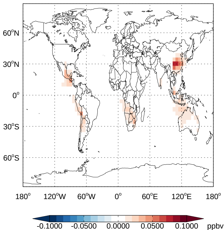
v11-02d - v11-02a SOAME - Diff @ Surface for Apr
