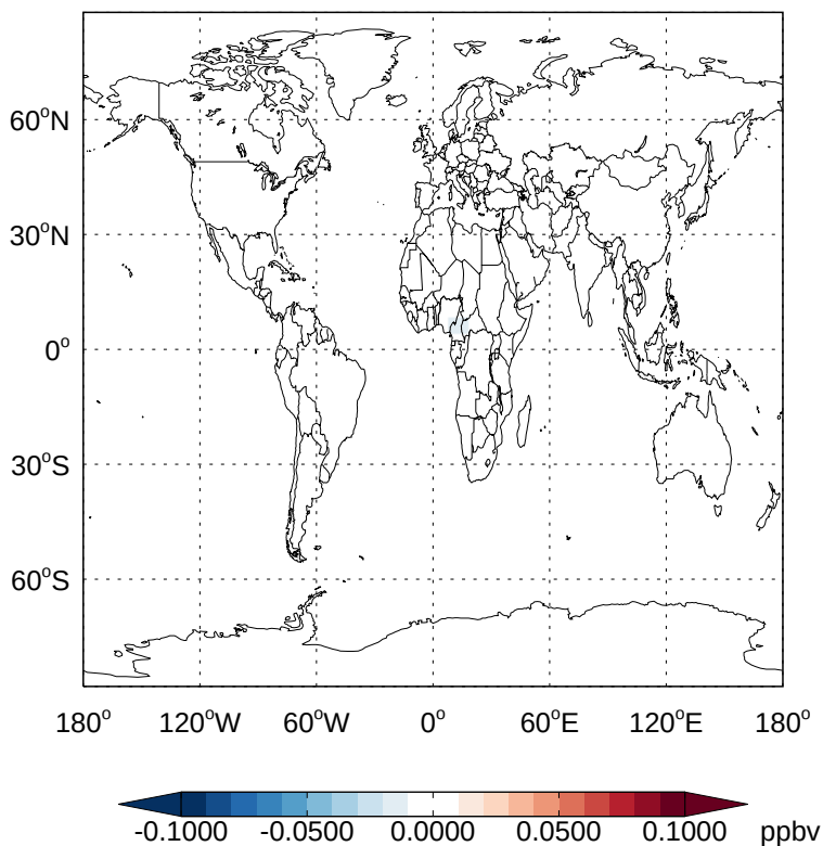
v11-02d - v11-02a SOAGX- Diff @ 500 hPa for Apr
