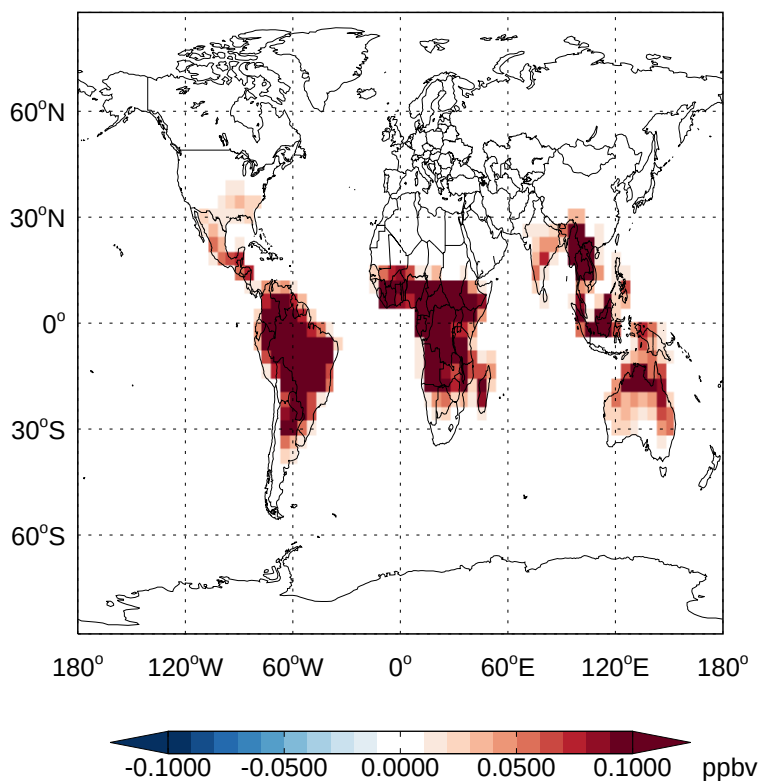
v11-02d - v11-02a IEPOXA - Diff @ Surface for Apr
