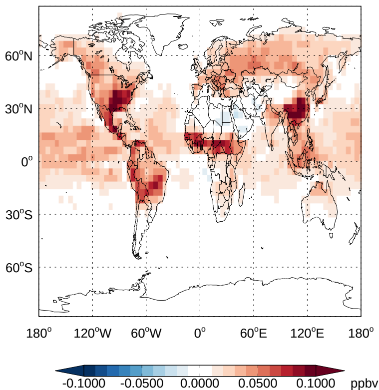
v11-02d - v11-02a CH4 - Diff @ Surface for Jul
