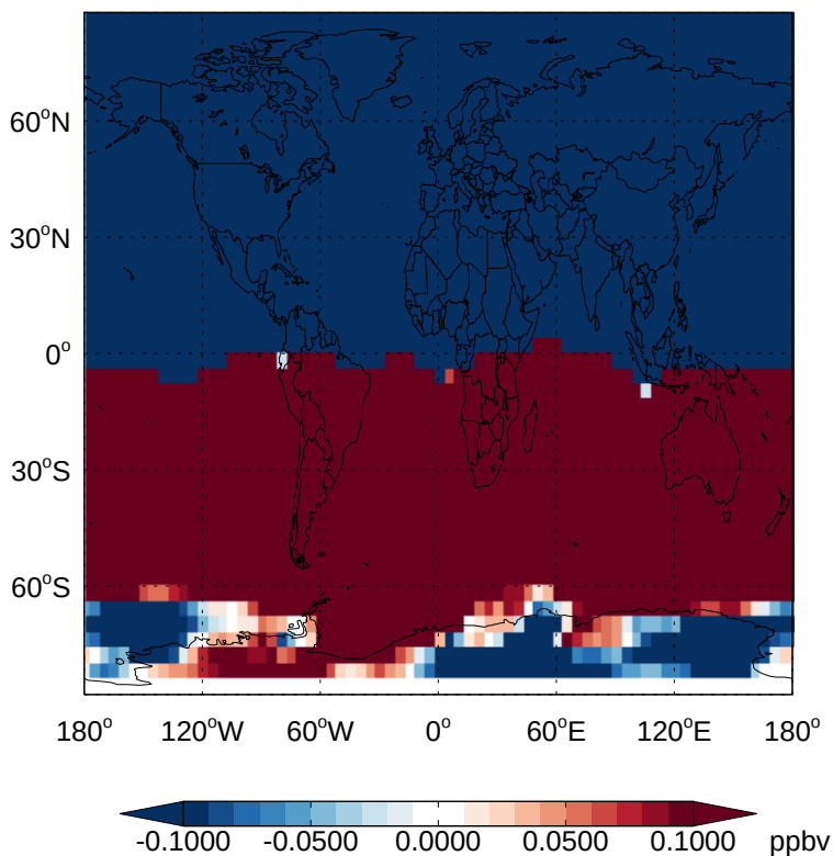
v11-02d - v11-02a CH4- Diff @ 500 hPa for Jul
