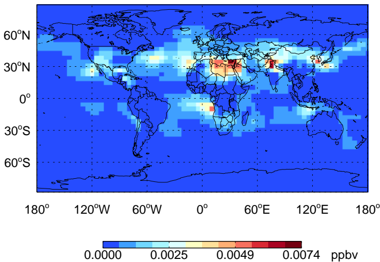
HOCl - Species map @ surface for Jul
