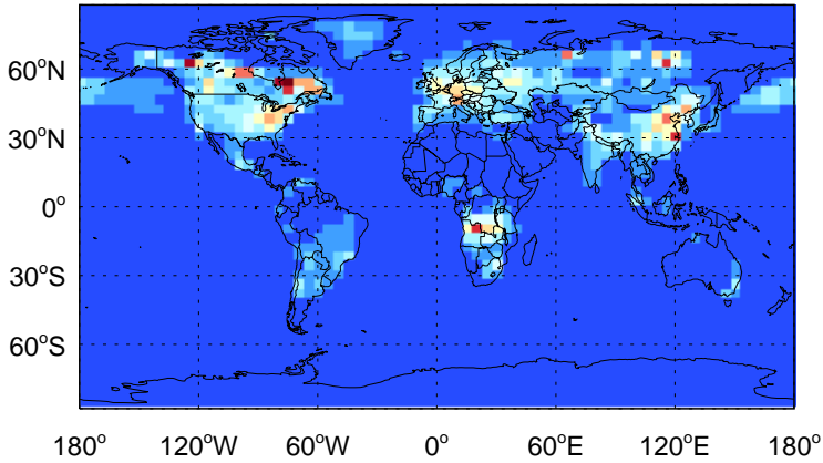
HNO 4 - Species map @ surface for Jul
