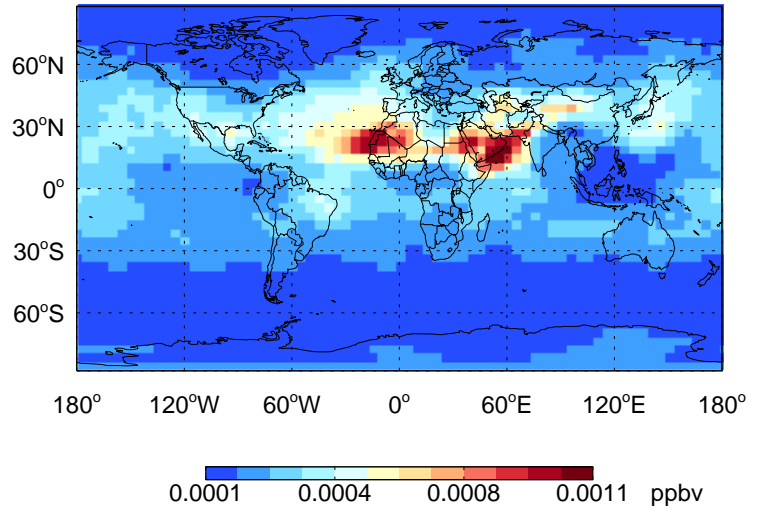
HOCl - Species map @ 500 hPa for Jul
