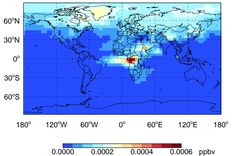
ASOA1 - Species map @ 500 hPa for Jul
