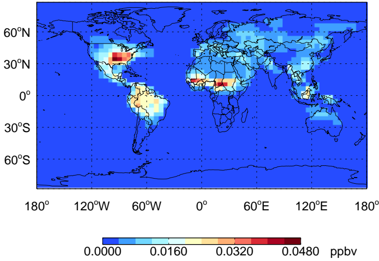
ISO-G1 - Species map @ surface for Jul
