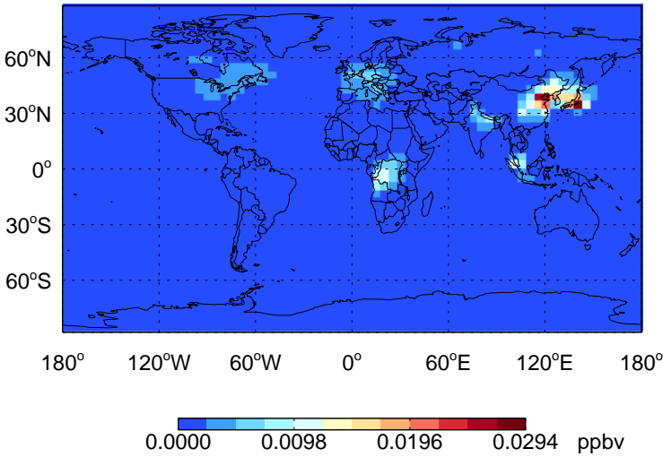
ASOA1 - Species map @ surface for Jul
