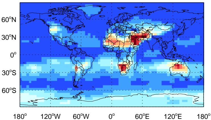
ISO2 - Species map @ surface for Jul
