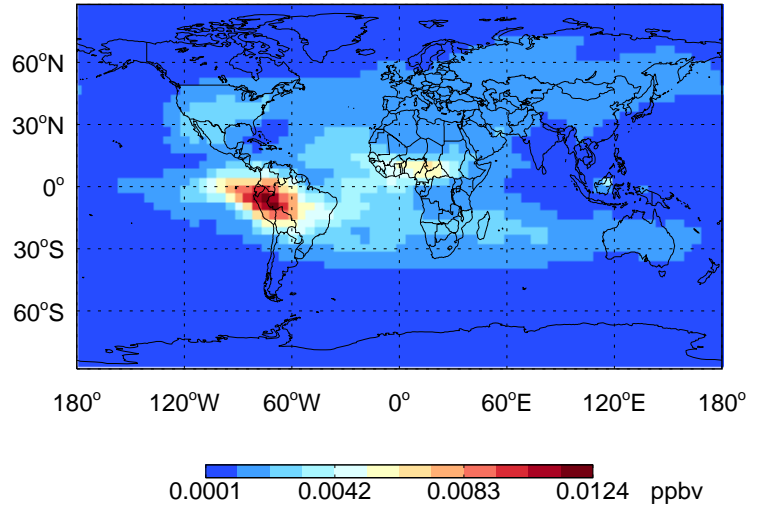
ISO-G1 - Species map @ 500 hPa for Jul
