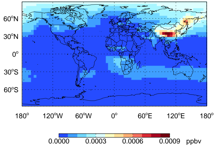
ASOA1 - Species map @ 500 hPa for Oct
