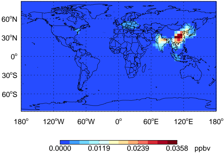
ASOA1 - Species map @ surface for Oct
