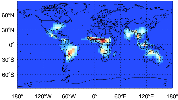
PROPNN - Species map @ surface for Oct
