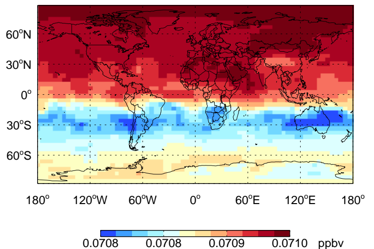
CCI4 - Species map @ 500 hPa for Oct
