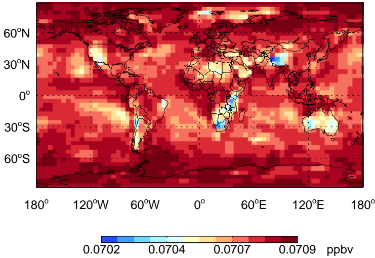
CCI4 - Species map @ surface for Oct
