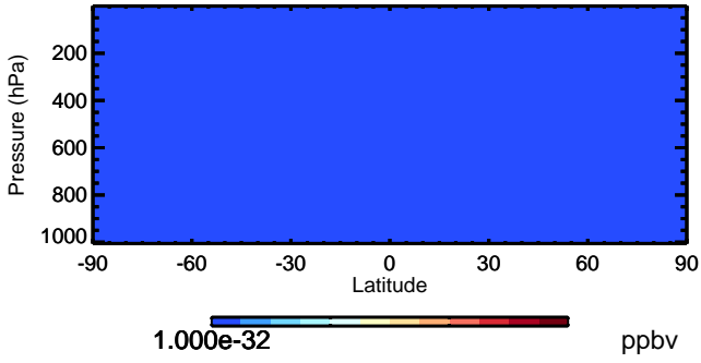
v11-02a SOAME - Species Zonal Mean for Oct
