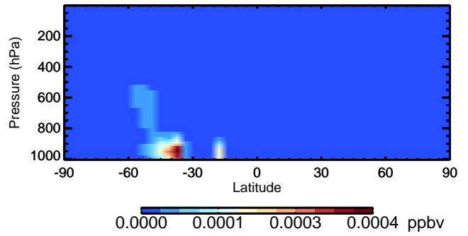
v11-02c HPALD - Species Curtain @ -180.000 for Oct
