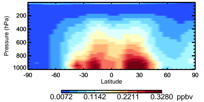
v11-02c CH2O - Species Curtain @ -180.000 for Oct
