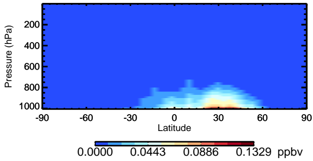
v11-02c SOAP - Species Zonal Mean for Oct
