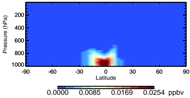
v11-02c RIPB - Species Zonal Mean for Oct
