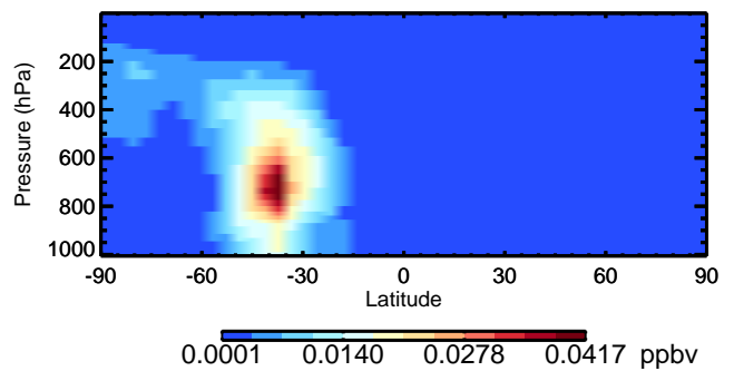
v11-02d SOAIE - Species Curtain @ -180.000 for Oct
