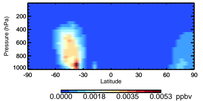
v11-02d GLYC - Species Curtain @ -180.000 for Oct
