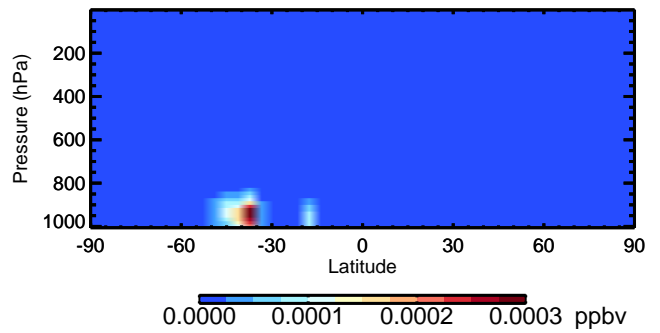
v11-02d RIPB - Species Curtain @ -180.000 for Oct
