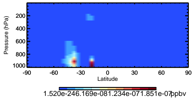
v11-02d LVOC - Species Curtain @ -180.000 for Oct
