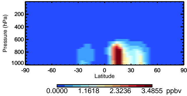
v11-02a DST1 - Species Zonal Mean for Oct
