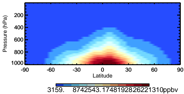
v11-02d H2O - Species Zonal Mean for Oct
