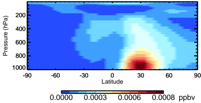
ASOG1 - Species Zonal Mean for Oct
