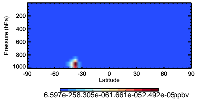
v11-02c MACRN - Species Curtain @ -180.000 for Oct
