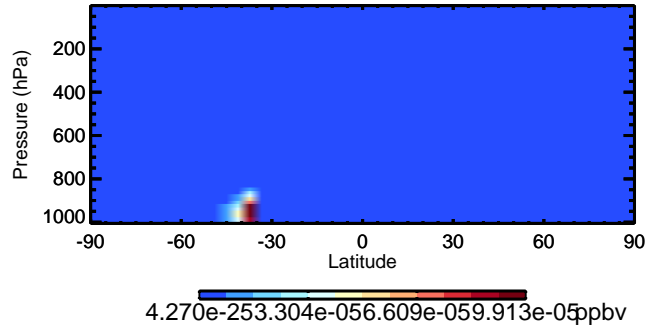
v11-02a ISOPNB - Species Curtain @ -180.000 for Oct
