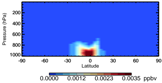
v11-02c RIPD - Species Zonal Mean for Oct
