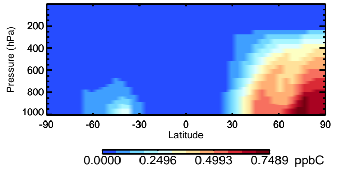
v11-02c ALK4 - Species Curtain @ -180.000 for Oct
