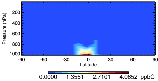
v11-02c ISOP - Species Zonal Mean for Oct
