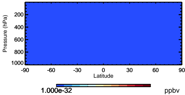
v11-02a SOAIE - Species Zonal Mean for Oct
