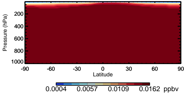
CFC114 - Species Zonal Mean for Oct
