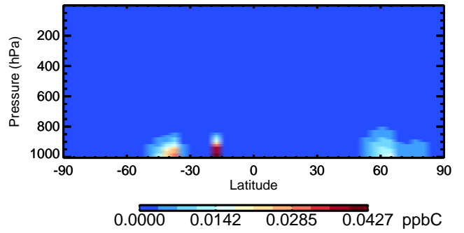
v11-02c PRPE - Species Curtain @ -180.000 for Oct
