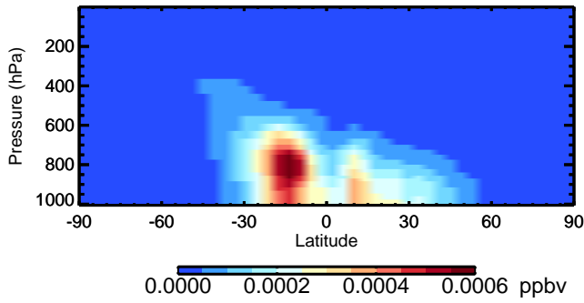
v11-02c ISN10A - Species Zonal Mean for Oct
