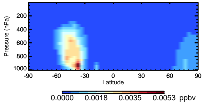
v11-02c GLYC - Species Curtain @ -180.000 for Oct
