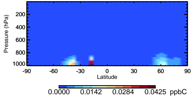
v11-02a PRPE - Species Curtain @ -180.000 for Oct
