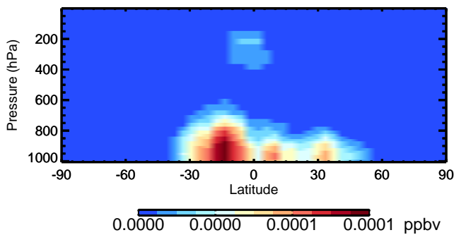
v11-02d MACRN - Species Zonal Mean for Oct
