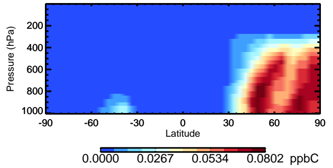
v11-02c TOLU - Species Curtain @ -180.000 for Oct
