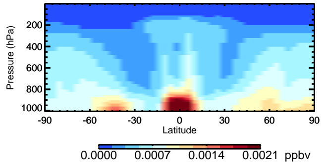
v11-02a CHBr3 - Species Curtain @ -180.000 for Oct
