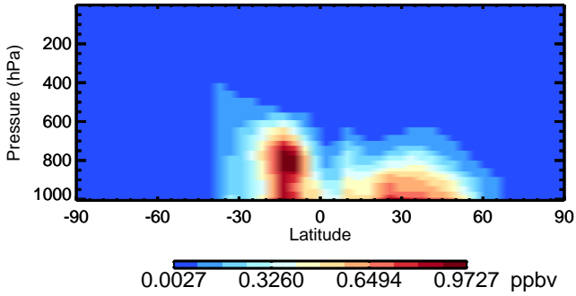
v11-02a OCPI - Species Zonal Mean for Oct
