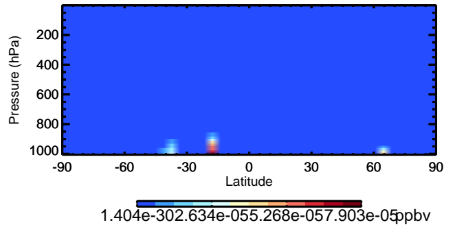
v11-02c LIMO - Species Curtain @ -180.000 for Oct
