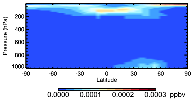
BrNO 2 - Species Zonal Mean for Oct
