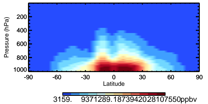
v11-02d H2O - Species Curtain @ -180.000 for Oct
