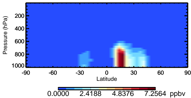
v11-02d DST2 - Species Zonal Mean for Oct
