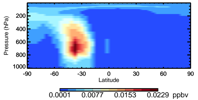
v11-02c SOAIE - Species Curtain @ -180.000 for Oct
