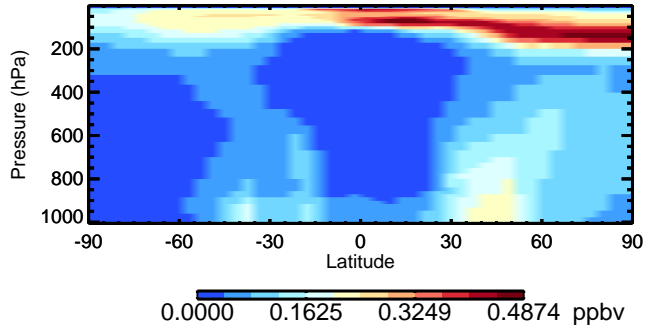
v11-02a SO4 - Species Curtain @ -180.000 for Oct
