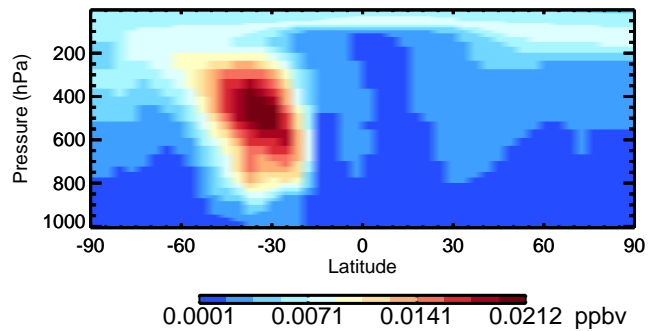
v11-02d ISO3 - Species Curtain @ -180.000 for Oct
