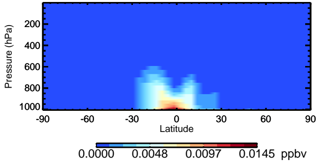
v11-02a TSOA1 - Species Zonal Mean for Oct
