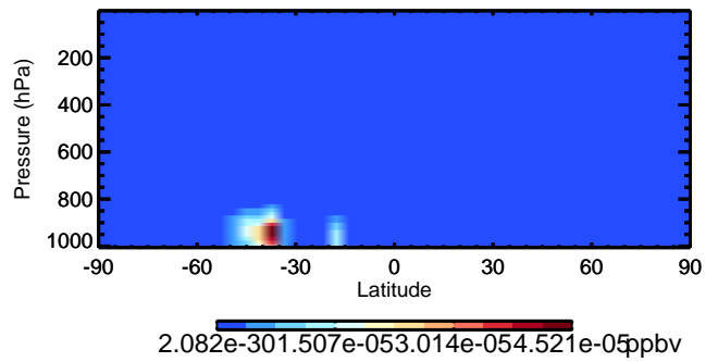
v11-02d RIPD - Species Curtain @ -180.000 for Oct
