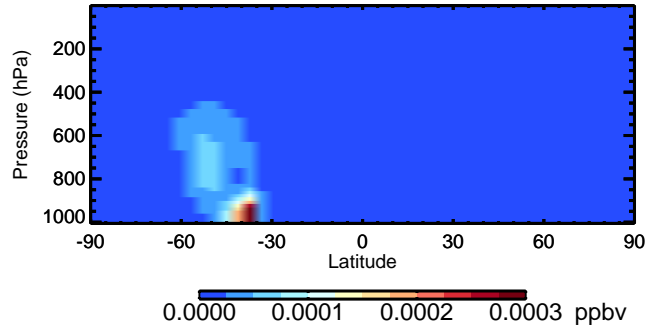
v11-02a NPMN - Species Curtain @ -180.000 for Oct
