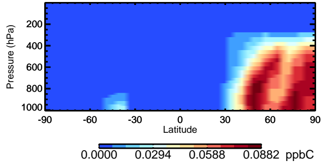
v11-02a TOLU - Species Curtain @ -180.000 for Oct
