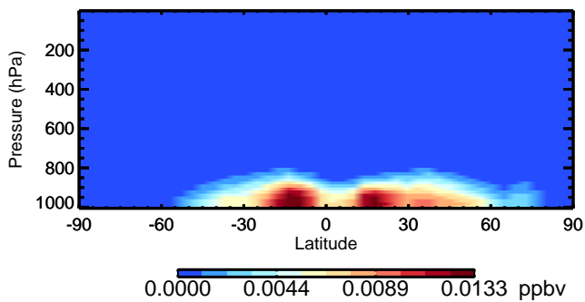
v11-02d NITs - Species Zonal Mean for Oct
