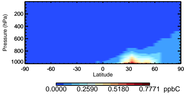
v11-02a TOLU - Species Zonal Mean for Oct
