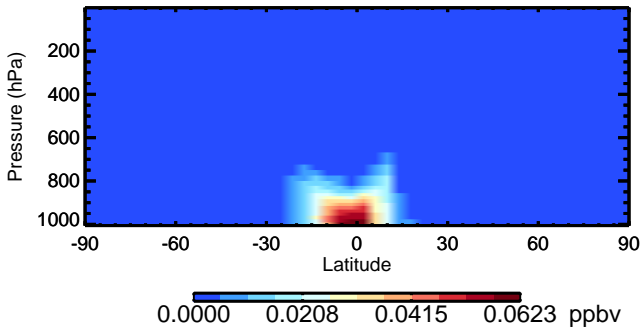
v11-02c HPALD - Species Zonal Mean for Oct
