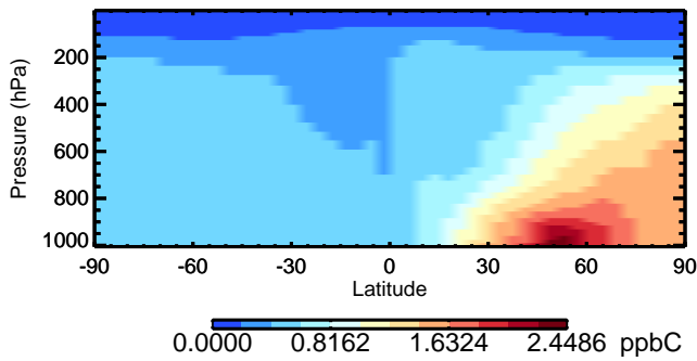
v11-02c C2H6 - Species Zonal Mean for Oct
