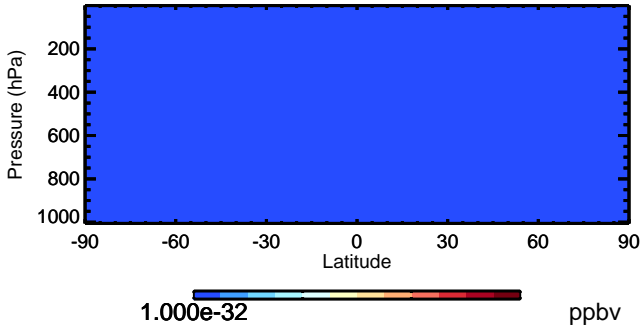
v11-02a HONIT - Species Zonal Mean for Oct
