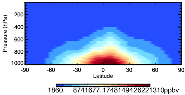
v11-02c H2O - Species Zonal Mean for Oct
