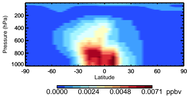
v11-02d ISO G1 - Species Zonal Mean for Oct
