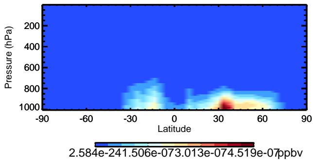
v11-02d NPMN - Species Zonal Mean for Oct
