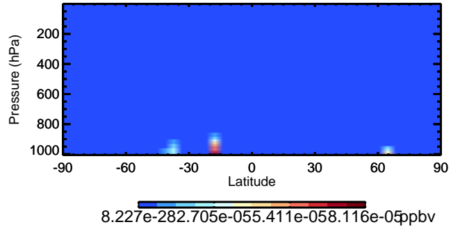
v11-02a LIMO - Species Curtain @ -180.000 for Oct
