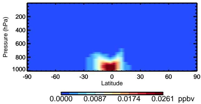
v11-02d RIPB - Species Zonal Mean for Oct
