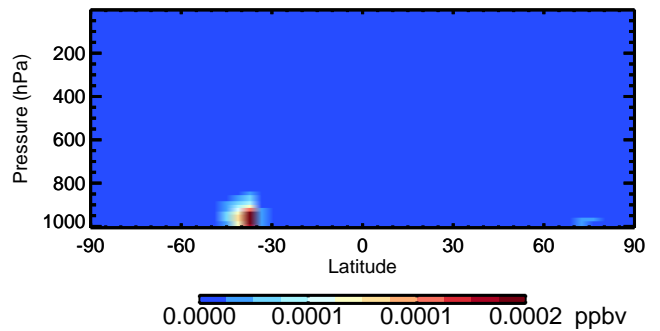
v11-02d ISN1 - Species Curtain @ -180.000 for Oct
