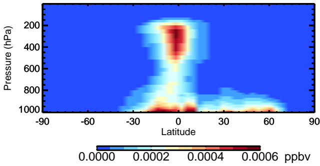
v11-02c HONIT - Species Zonal Mean for Oct
