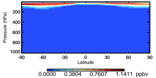
CINO3 - Species Curtain @ -180.000 for Oct
