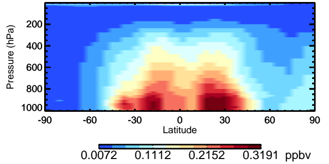
v11-02a CH2O - Species Curtain @ -180.000 for Oct
