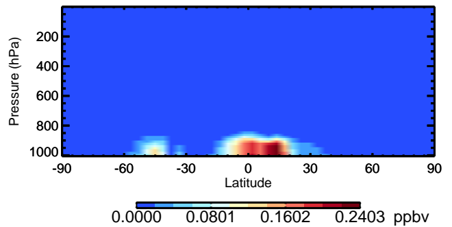
v11-02d NH3 - Species Curtain @ -180.000 for Oct
