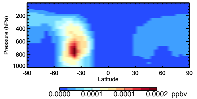
v11-02d ISN10A - Species Curtain @ -180.000 for Oct
