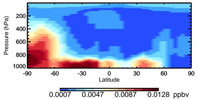
v11-02d MSA - Species Curtain @ -180.000 for Oct
