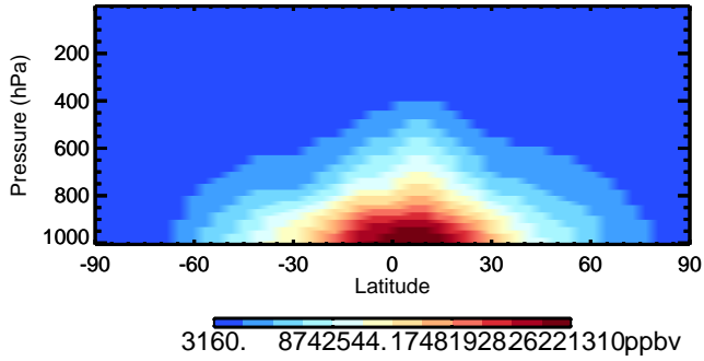
v11-02a H2O - Species Zonal Mean for Oct
