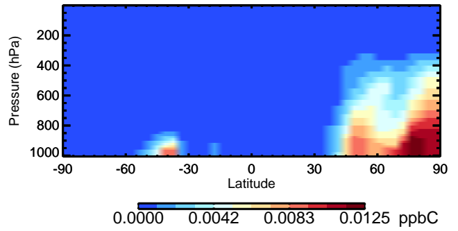
v11-02c XYLE - Species Curtain @ -180.000 for Oct
