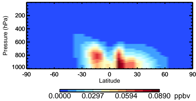
v11-02c INDIOL - Species Zonal Mean for Oct
