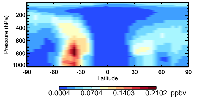
v11-02c OCPI - Species Curtain @ -180.000 for Oct
