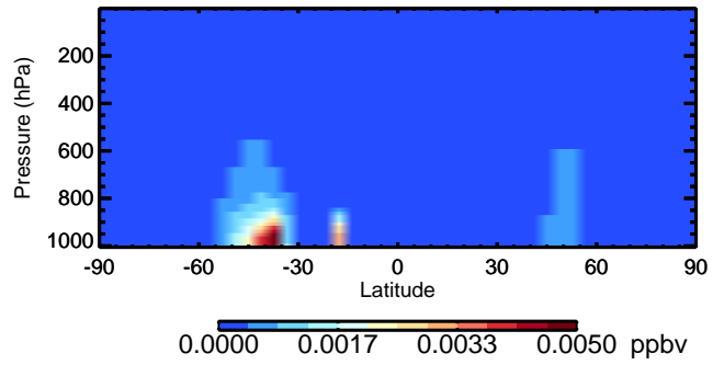
v11-02c SOAP - Species Curtain @ -180.000 for Oct
