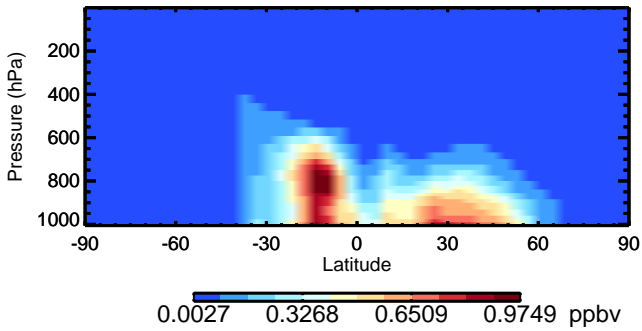
v11-02c OCPI - Species Zonal Mean for Oct
