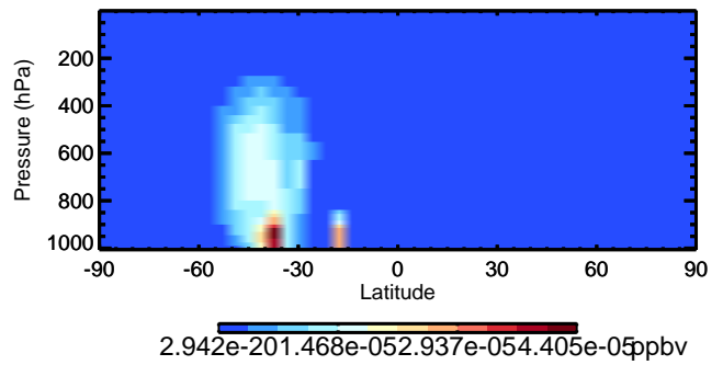
v11-02d HCOOH - Species Curtain @ -180.000 for Oct
