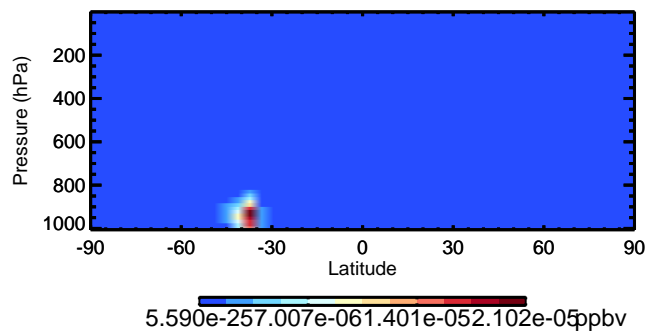
v11-02d MACRN - Species Curtain @ -180.000 for Oct
