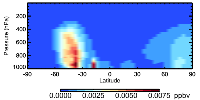
v11-02d HAC - Species Curtain @ -180.000 for Oct
