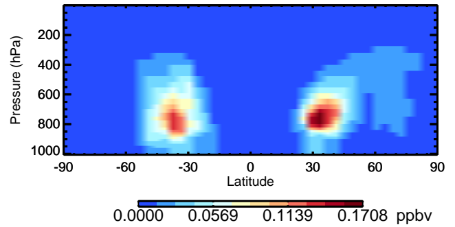
v11-02c DST2 - Species Curtain @ -180.000 for Oct
