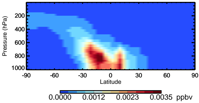
v11-02c SOAME - Species Zonal Mean for Oct
