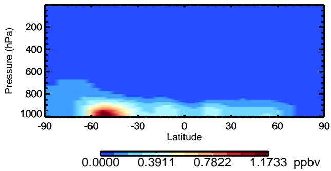
v11-02c SALA - Species Zonal Mean for Oct
