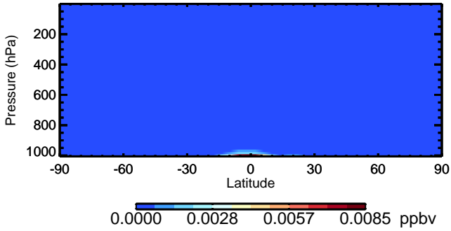
v11-02a LIMO - Species Zonal Mean for Oct
