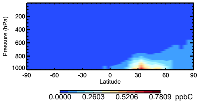
v11-02d TOLU - Species Zonal Mean for Oct
