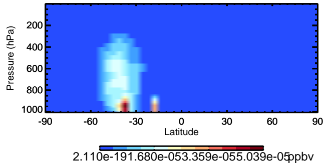
v11-02c HCOOH - Species Curtain @ -180.000 for Oct
