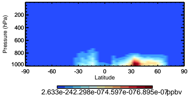
v11-02c NPMN - Species Zonal Mean for Oct
