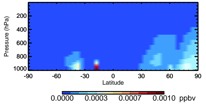
v11-02c GLYX - Species Curtain @ -180.000 for Oct
