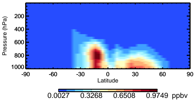
v11-02d OCPI - Species Zonal Mean for Oct
