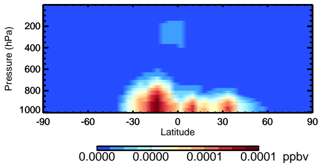
v11-02c MACRN - Species Zonal Mean for Oct
