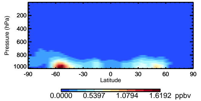
v11-02a SALA - Species Curtain @ -180.000 for Oct
