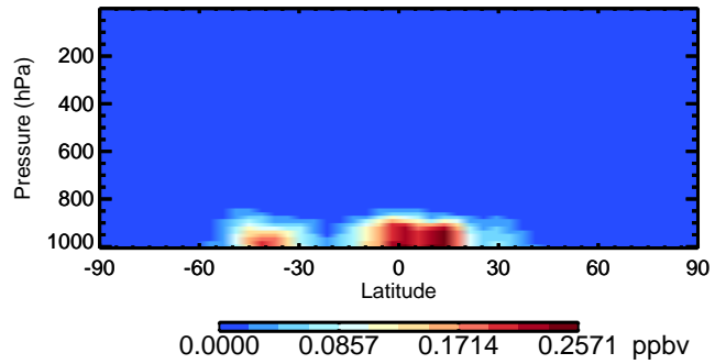
v11-02c NH3 - Species Curtain @ -180.000 for Oct
