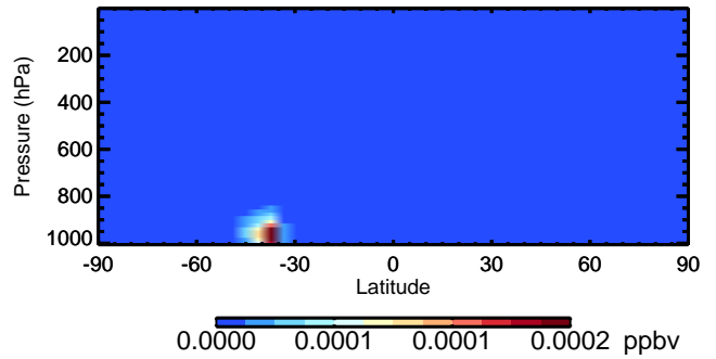
v11-02c ISN1 - Species Curtain @ -180.000 for Oct
