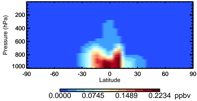
v11-02a HAC - Species Zonal Mean for Oct
