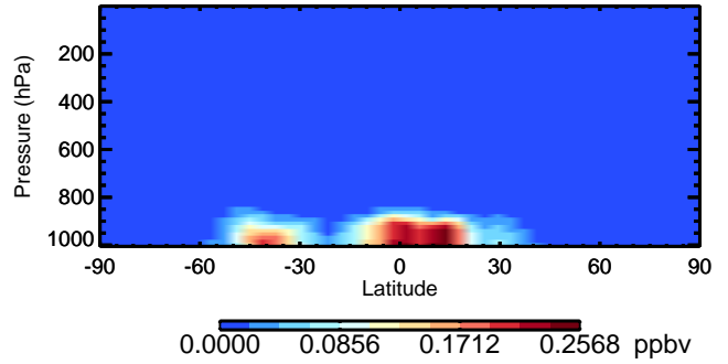
v11-02a NH3 - Species Curtain @ -180.000 for Oct
