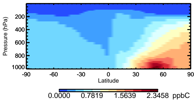
v11-02d C2H6 - Species Zonal Mean for Oct
