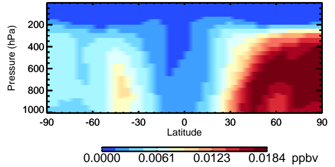
v11-02a R4N2 - Species Curtain @ -180.000 for Oct
