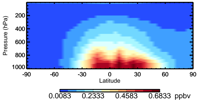
v11-02c CH2O - Species Zonal Mean for Oct
