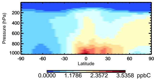
ACET - Species Zonal Mean for Oct
