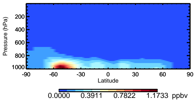
v11-02d SALA - Species Zonal Mean for Oct
