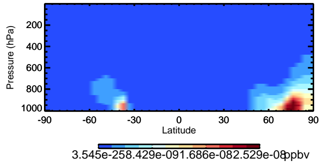
v11-02c NPMN - Species Curtain @ -180.000 for Oct
