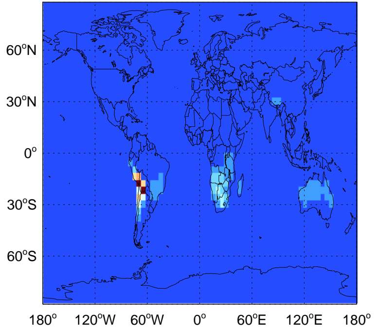
JCH3Cl - J-Value @ 500 hPa for Jan
