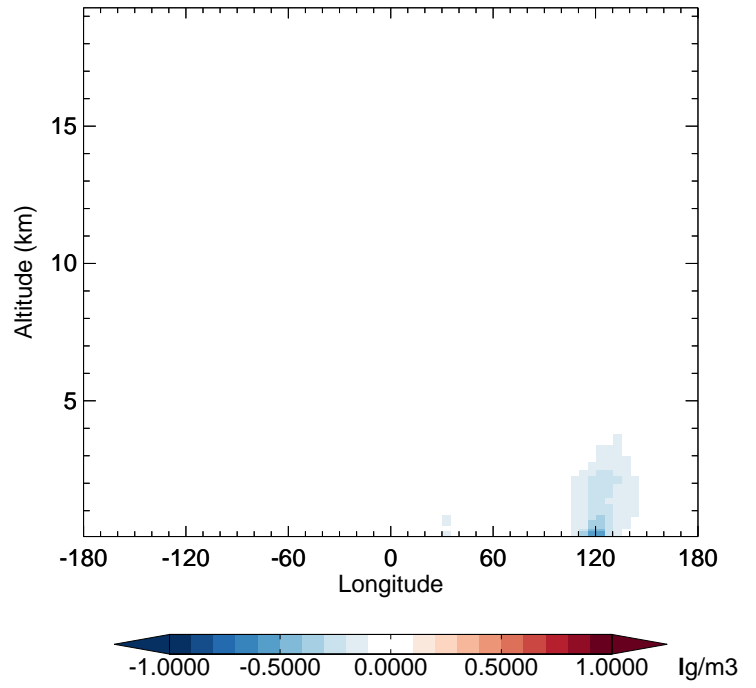
v11-02d - v11-02c NIT - Diff along 42N for Apr
