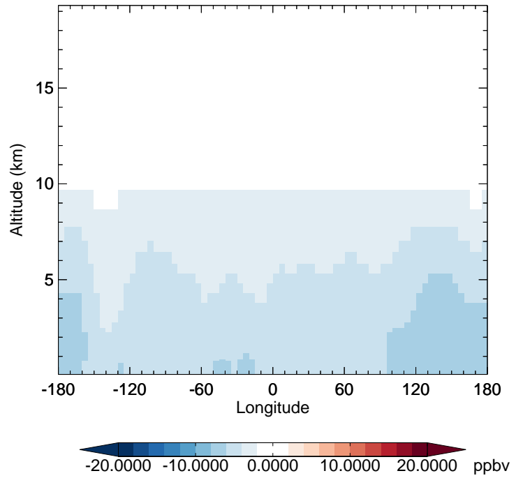
v11-02d - v11-02a CO - Diff along 42N for Apr
