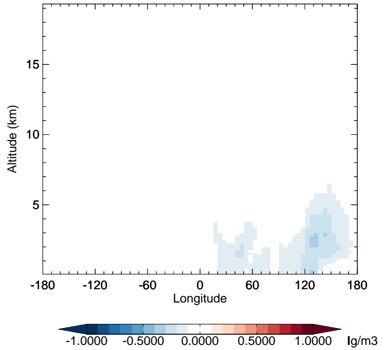
v11-02d - v11-02a SO 2 - Diff along 42N for Apr
