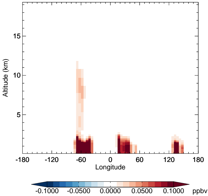
v11-02d - v11-02a RIPA - Diff along 15S for Apr
