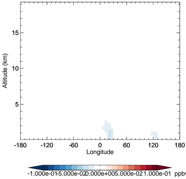
v11-02d - v11-02c SOAME - Diff along 15S for Apr
