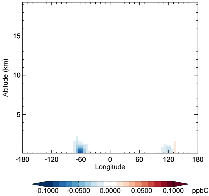
v11-02d - v11-02c MEK - Diff along 15S for Apr
