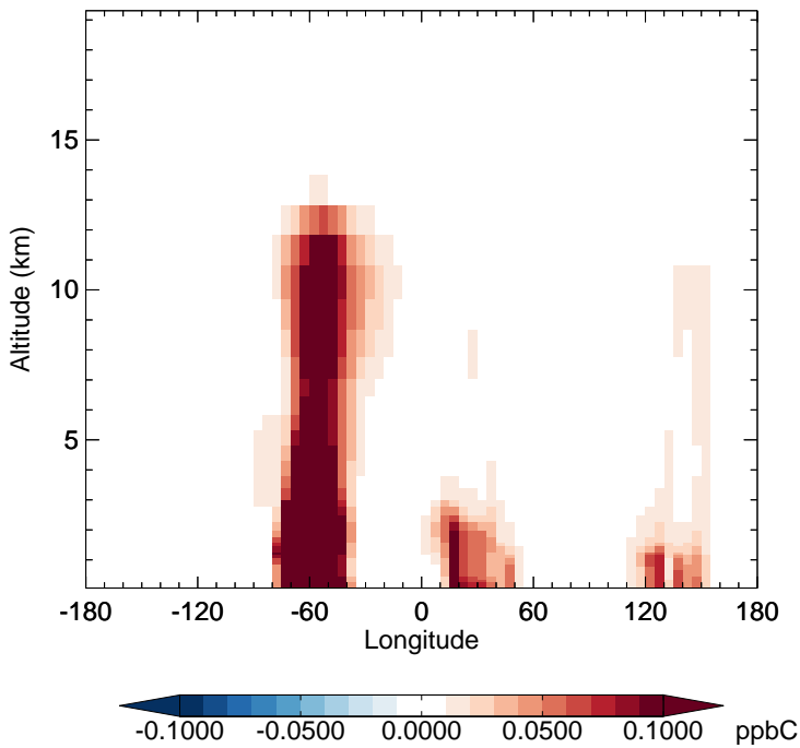
v11-02d - v11-02a MEK - Diff along 15S for Apr
