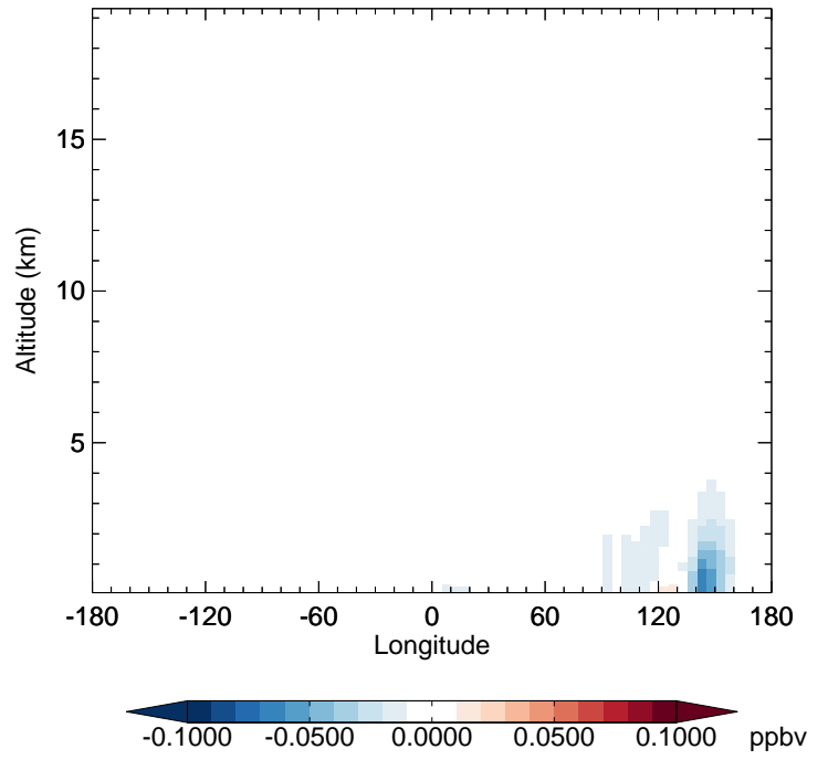
v11-02d - v11-02c XYLE - Diff along 42N for Apr
