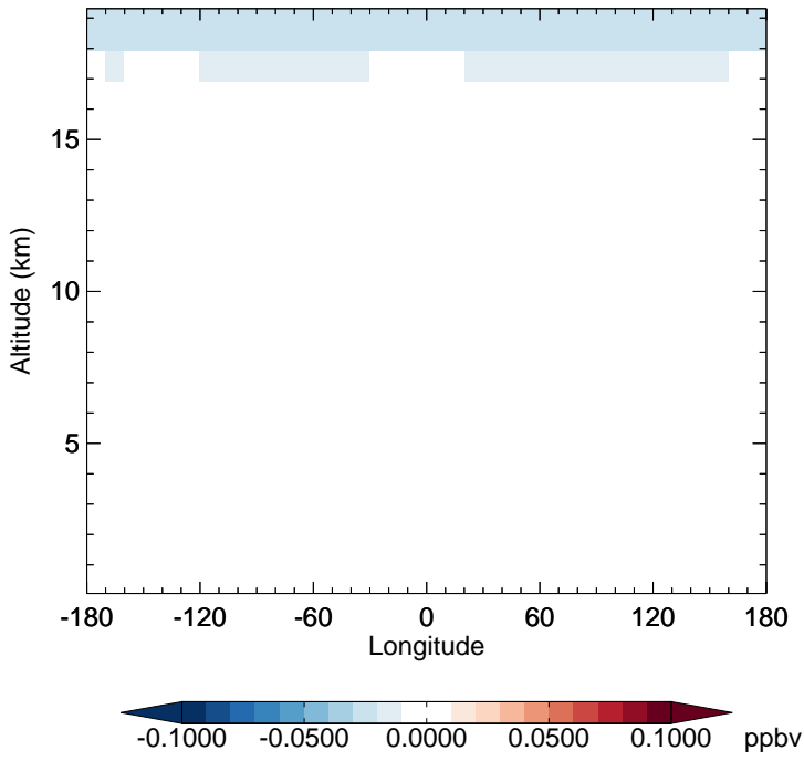
v11-02d - v11-02c PAN - Diff along 15S for Apr
