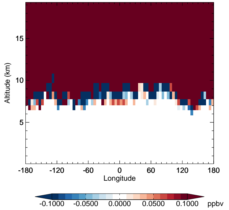
v11-02d - v11-02c H2O - Diff along 42N for Apr
