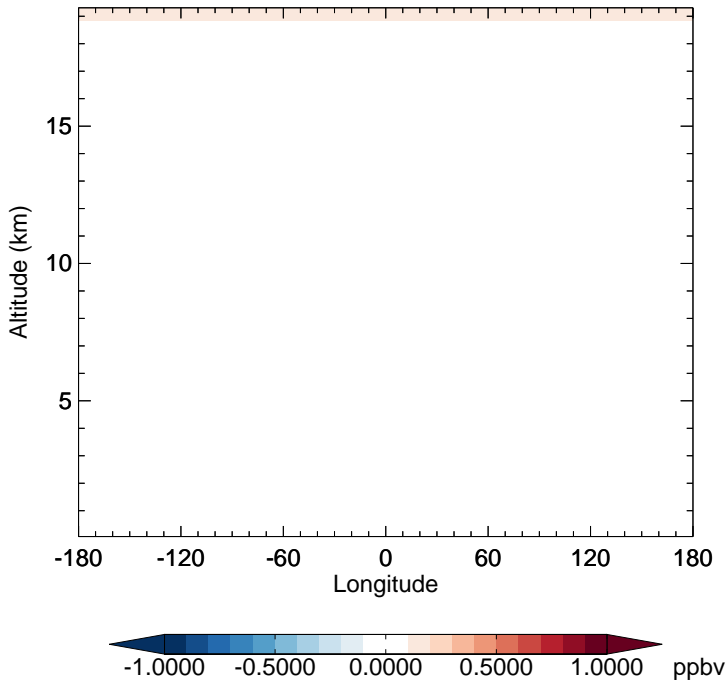
v11-02d - v11-02a NO 2 - Diff along 15S for Apr
