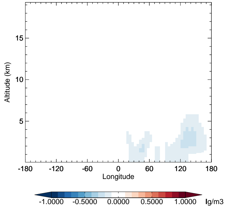
v11-02d - v11-02c SO 2 - Diff along 42N for Apr
