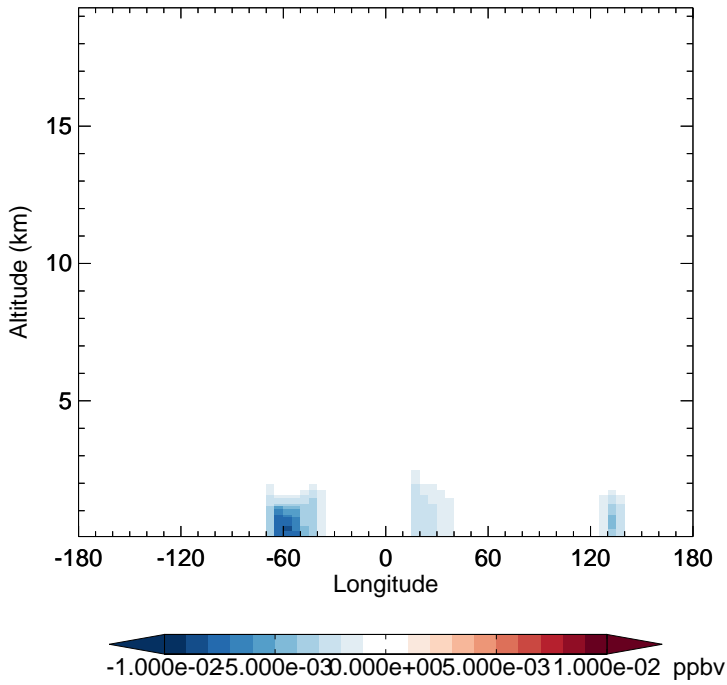
v11-02d - v11-02a MACRN - Diff along 15S for Apr
