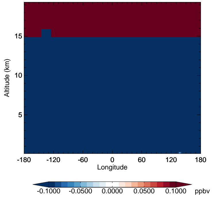
v11-02d - v11-02c CH4 - Diff along 42N for Apr
