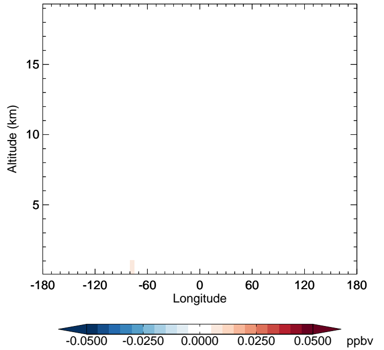
v11-02d - v11-02a MVK - Diff along 42N for Apr
