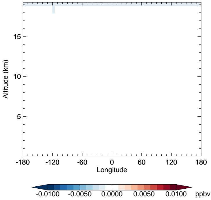
v11-02d - v11-02c BrNO3 - Diff along 15S for Apr
