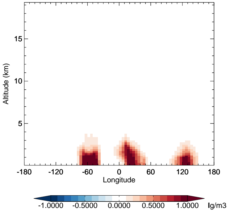
v11-02d - v11-02a SOAS - Diff along 15S for Apr
