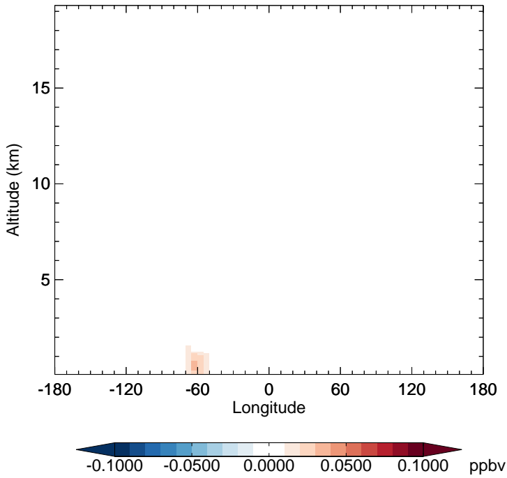
v11-02d - v11-02a RIPD - Diff along 15S for Apr
