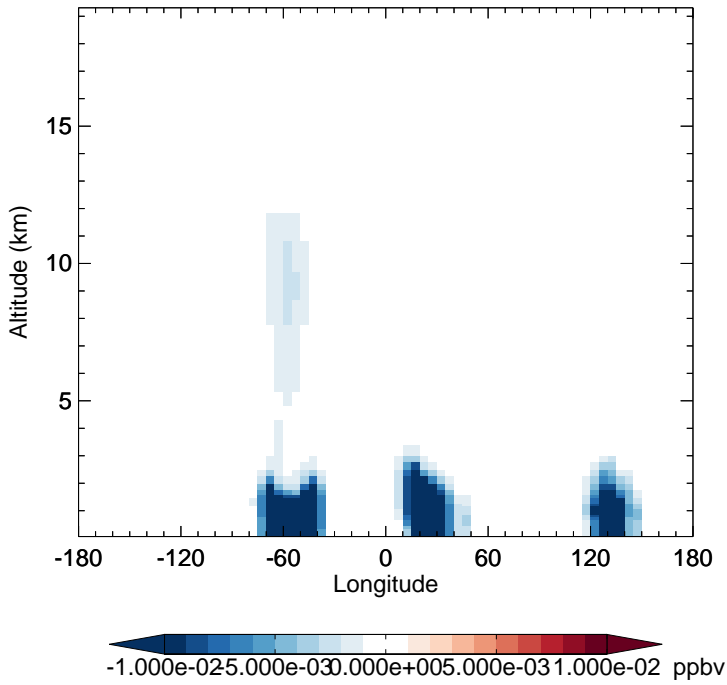
v11-02d - v11-02a MVKN - Diff along 15S for Apr
