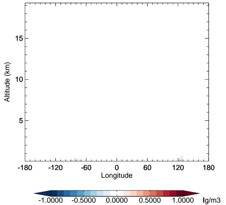
v11-02d - v11-02a NH4 - Diff along 42N for Apr
