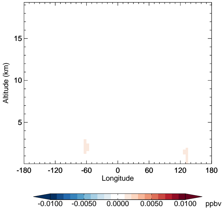
v11-02d - v11-02c R4N2 - Diff along 15S for Apr
