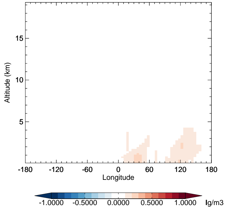
v11-02d - v11-02c SO4 - Diff along 42N for Apr
