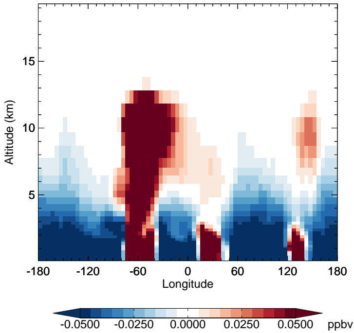
v11-02d - v11-02a MP - Diff along 15S for Apr
