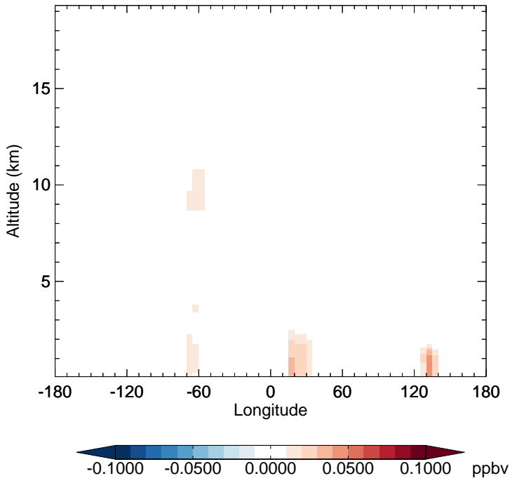
v11-02d - v11-02c IEPOXB - Diff along 15S for Apr
