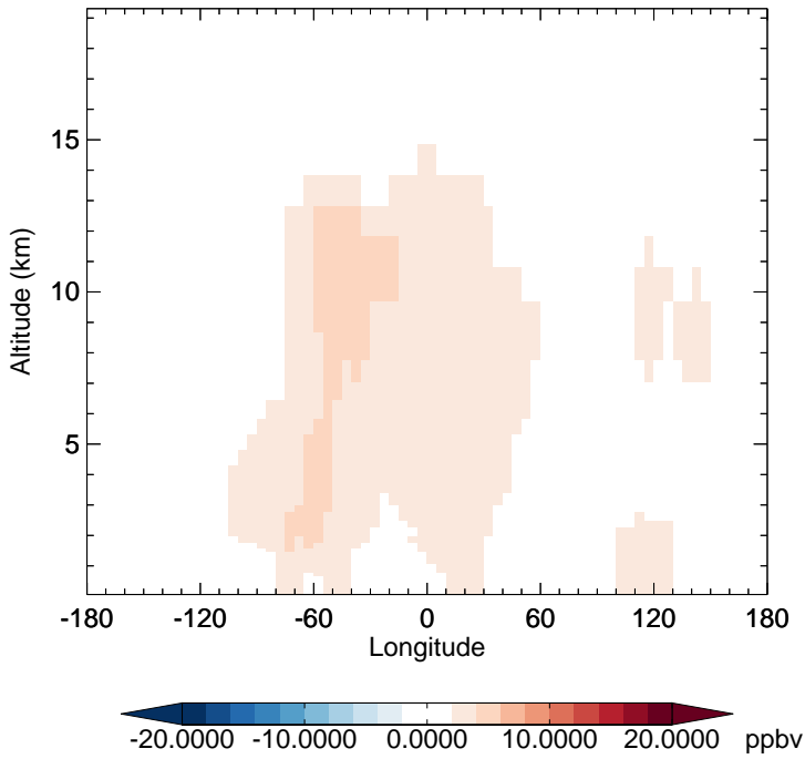
v11-02d - v11-02a CO - Diff along 15S for Apr
