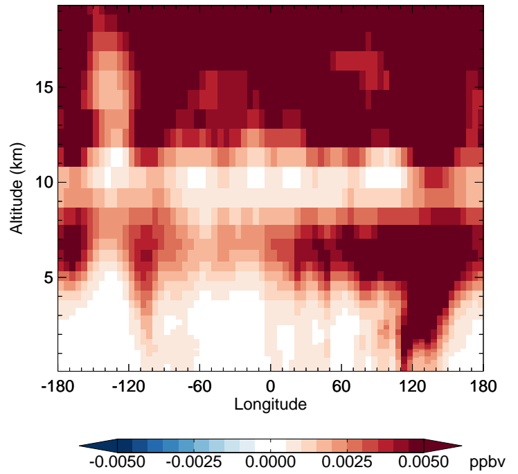
v11-02d - v11-02a HNO 4 - Diff along 42N for Apr
