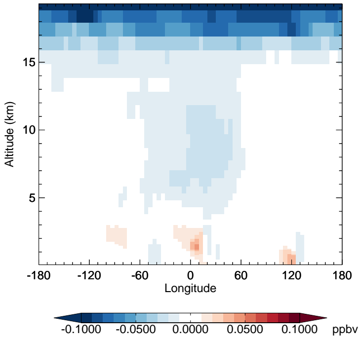
v11-02d - v11-02a HNO 3 - Diff along 15S for Apr
