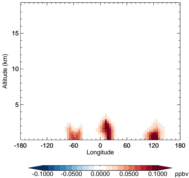
v11-02d - v11-02a INDIOL - Diff along 15S for Apr
