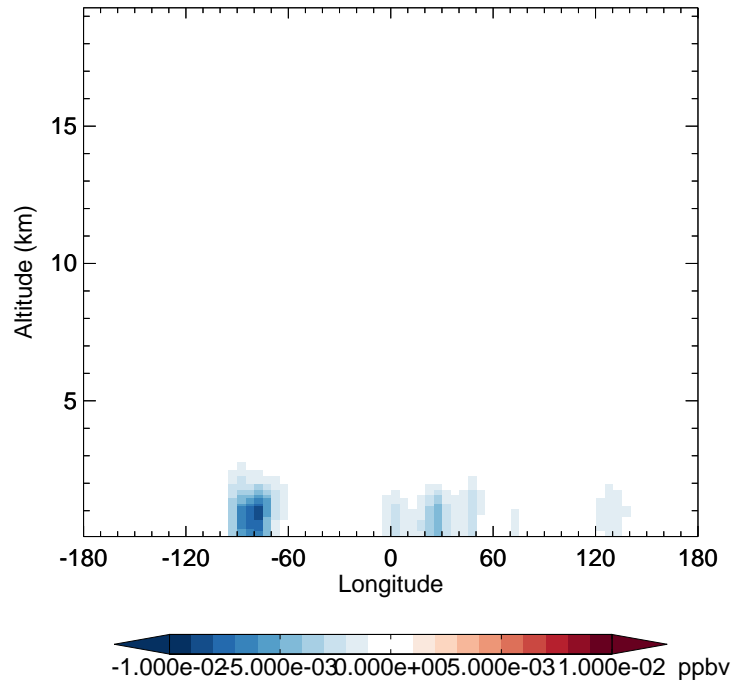
v11-02d - v11-02a MVKN - Diff along 42N for Apr
