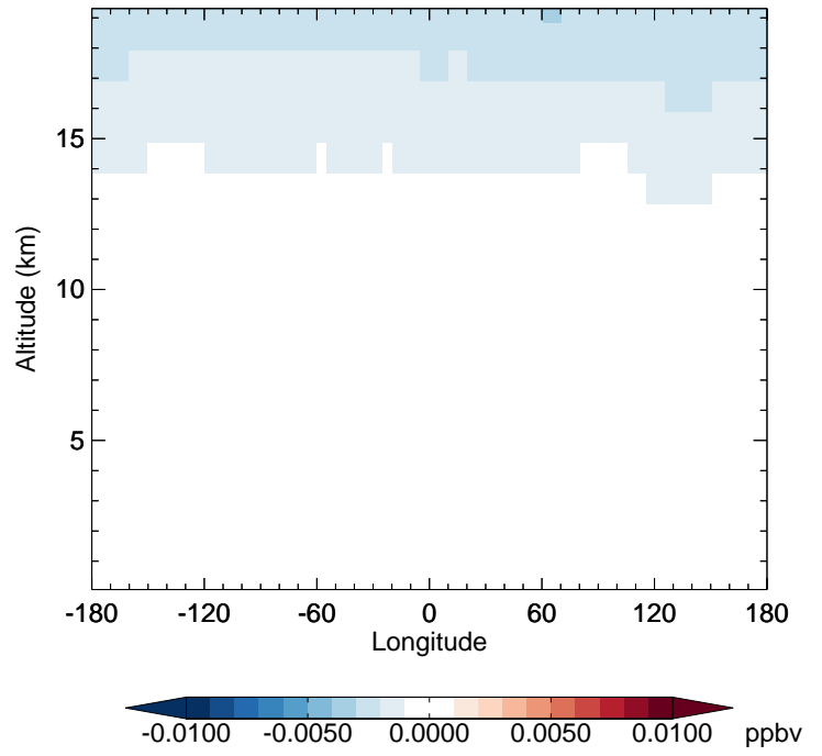
v11-02d - v11-02c BrNO3 - Diff along 42N for Apr
