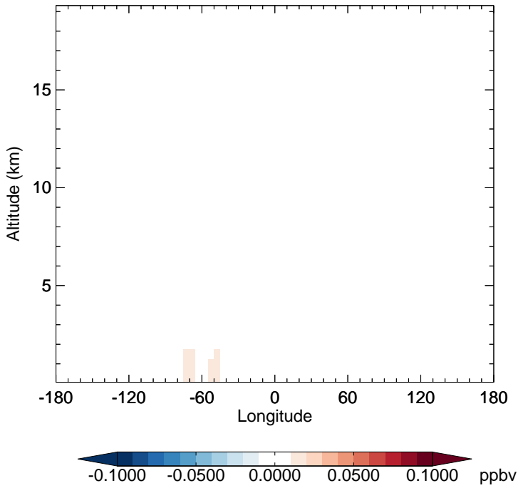
v11-02d - v11-02a TOLU - Diff along 15S for Apr
