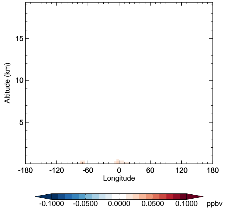
v11-02d - v11-02a CINO2 - Diff along 42N for Apr
