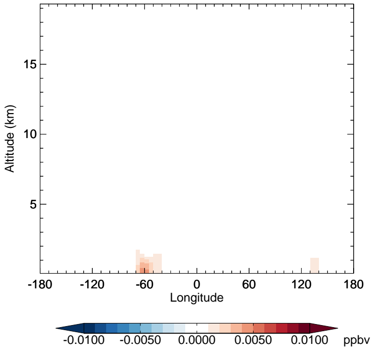
v11-02d - v11-02a MOBA - Diff along 15S for Apr
