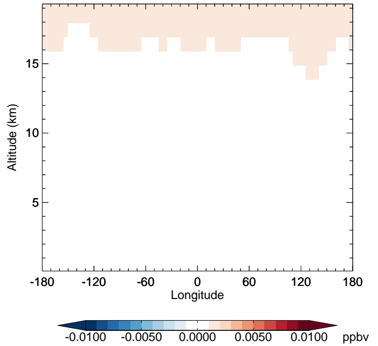
v11-02d - v11-02a BrNO3 - Diff along 42N for Apr
