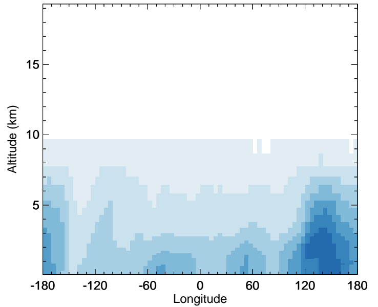
v11-02d - v11-02a BENZ - Diff along 42N for Apr
