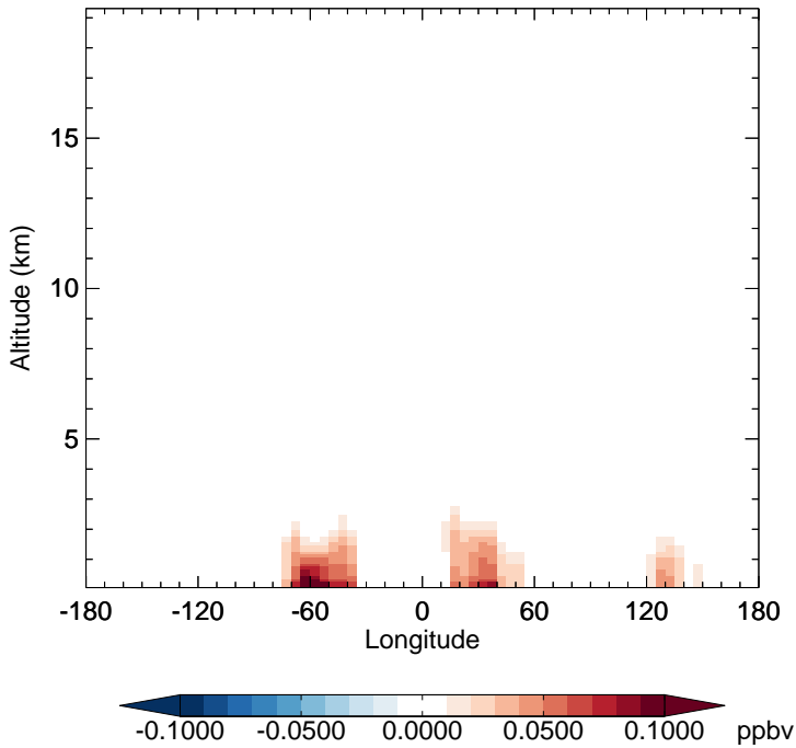
v11-02d - v11-02a SOAP - Diff along 15S for Apr
