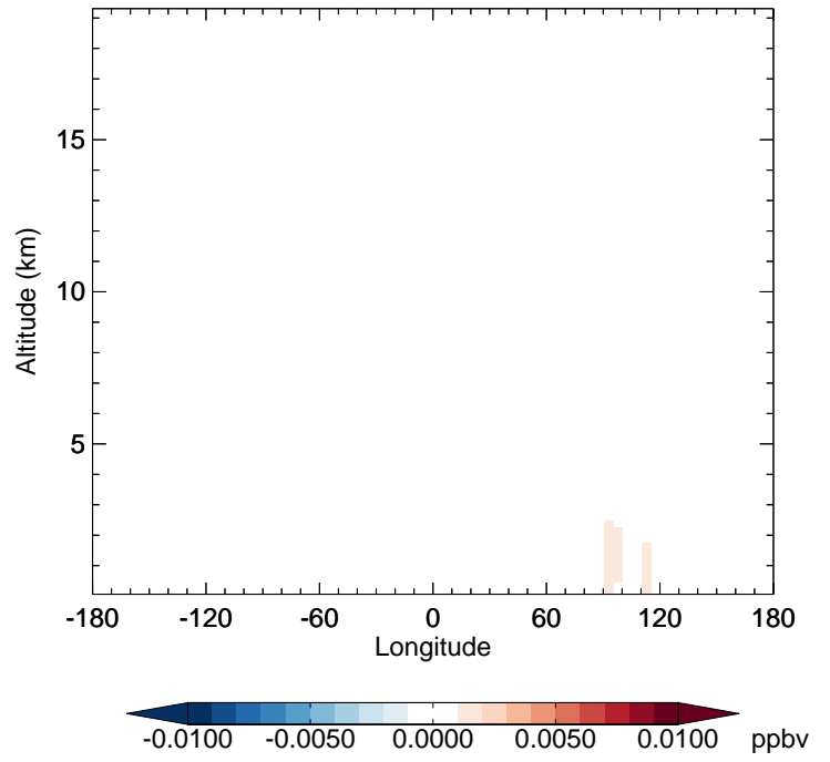
v11-02d - v11-02c R4N2 - Diff along 42N for Apr
