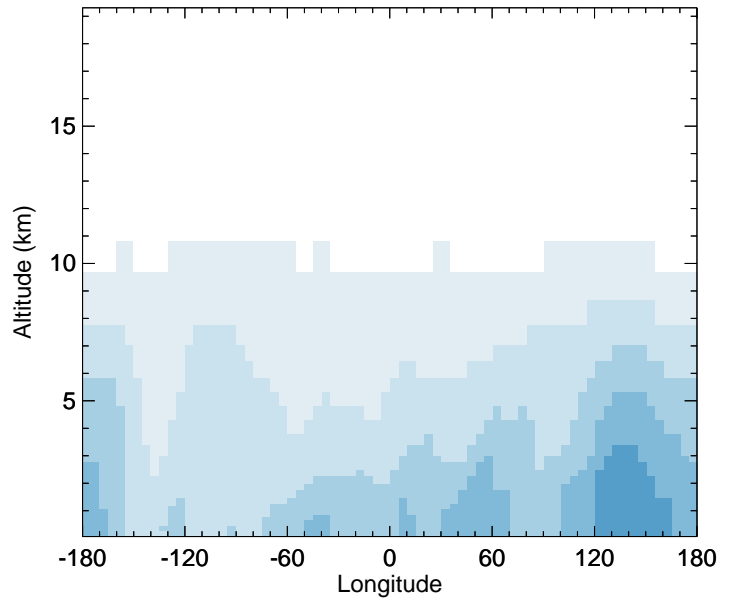
v11-02d - v11-02a C3H8 - Diff along 42N for Apr
