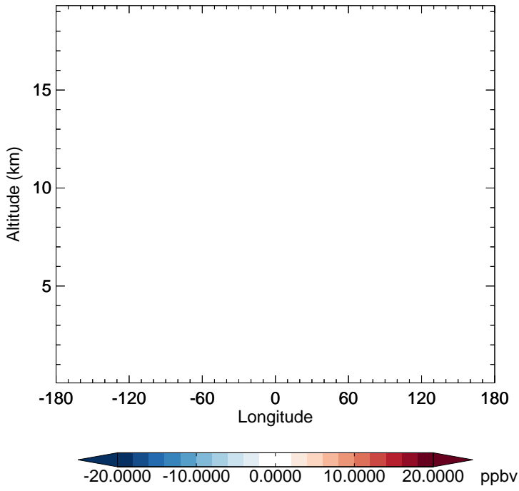
v11-02d - v11-02c CO - Diff along 15S for Apr
