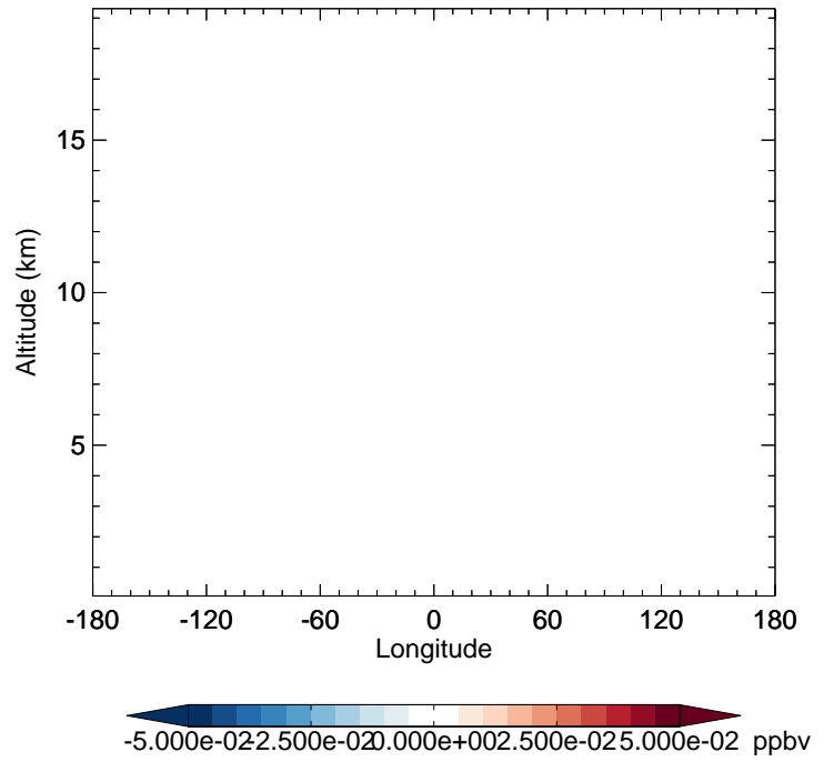
v11-02d - v11-02c MVK - Diff along 42N for Apr
