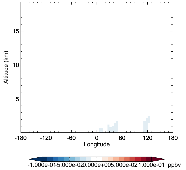
v11-02d - v11-02c EOH - Diff along 42N for Apr
