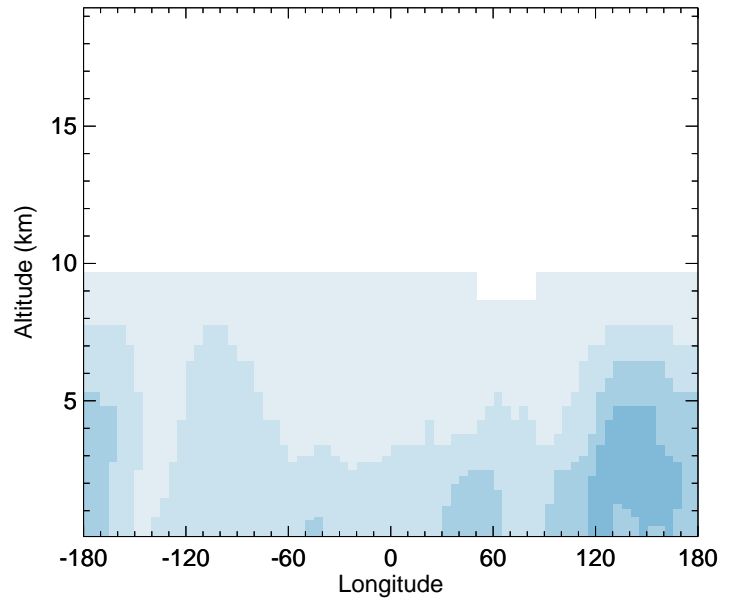
v11-02d - v11-02c BENZ - Diff along 42N for Apr
