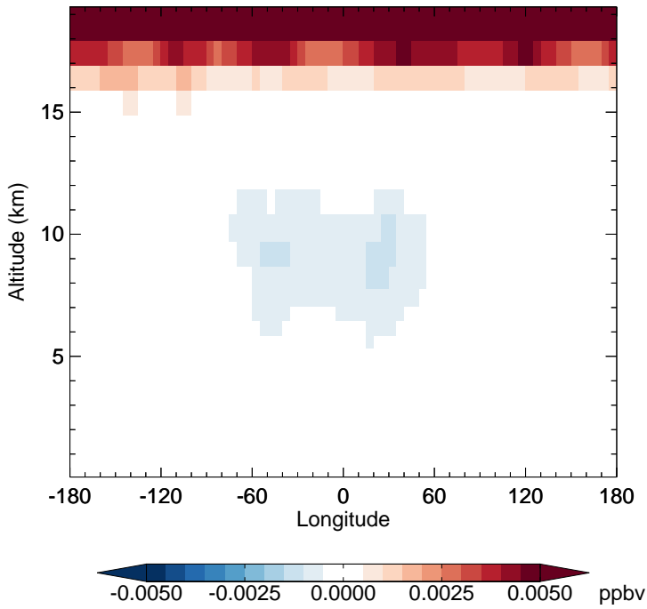
v11-02d - v11-02a N2O5 - Diff along 15S for Apr
