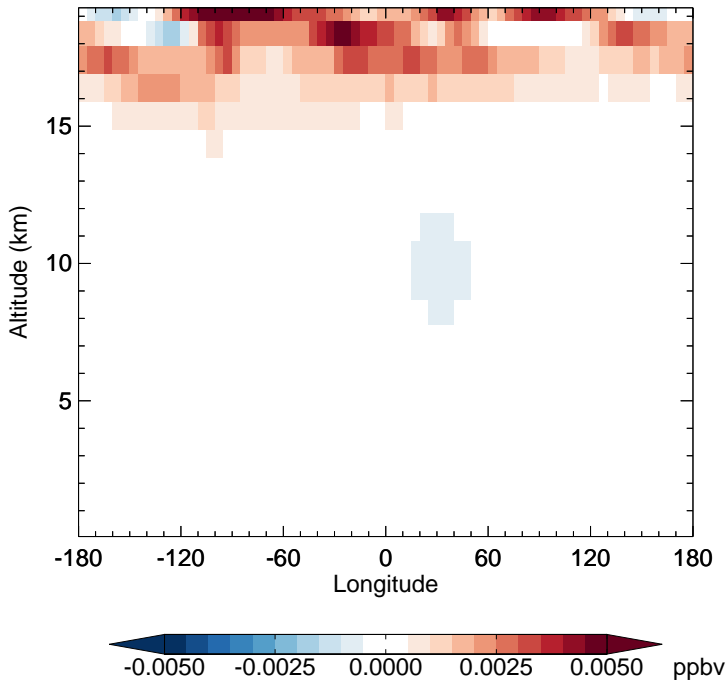
v11-02d - v11-02c N2O5 - Diff along 15S for Apr
