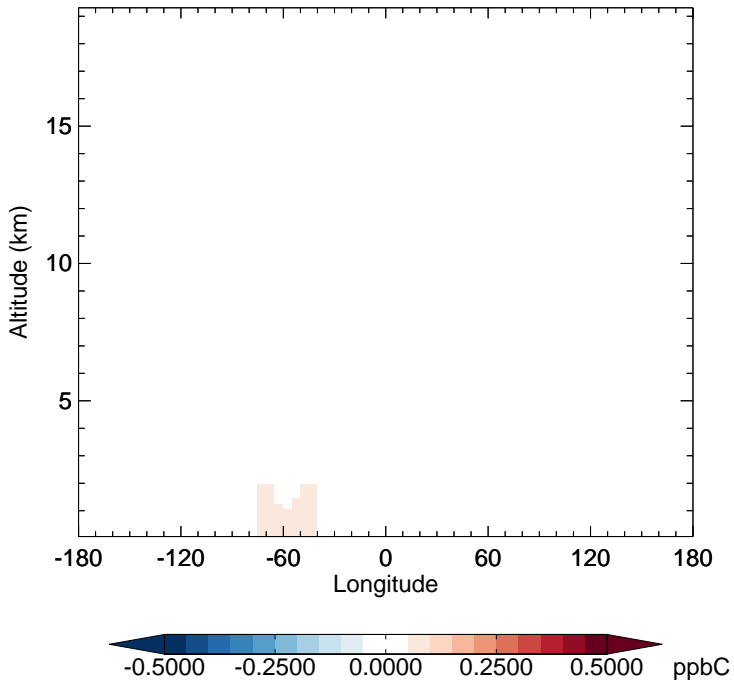
v11-02d - v11-02a ALK4 - Diff along 15S for Apr
