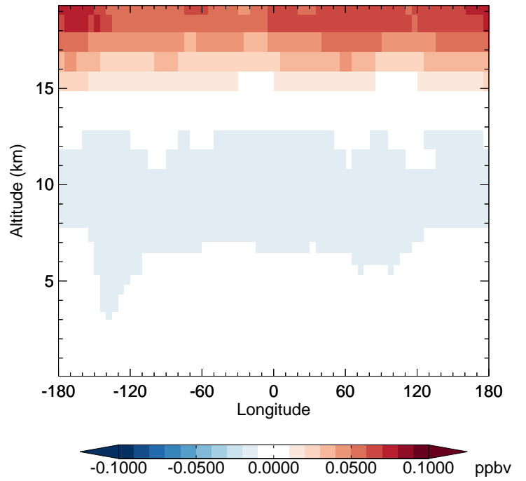
v11-02d - v11-02c OCS - Diff along 42N for Apr
