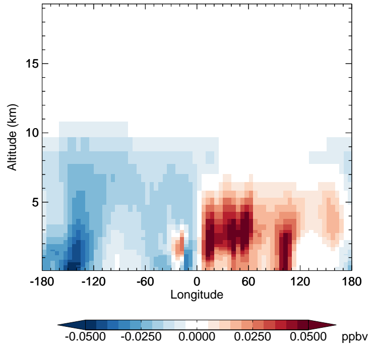
v11-02d - v11-02c MP - Diff along 42N for Apr
