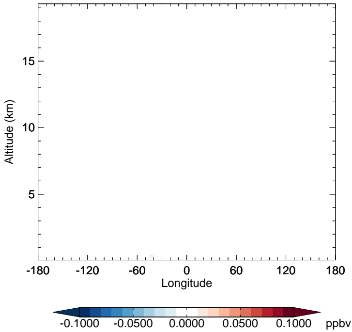
v11-02d - v11-02a ISOPNB - Diff along 15S for Apr
