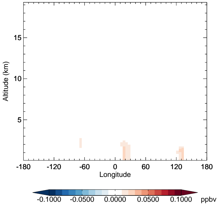
v11-02d - v11-02c HC187 - Diff along 15S for Apr
