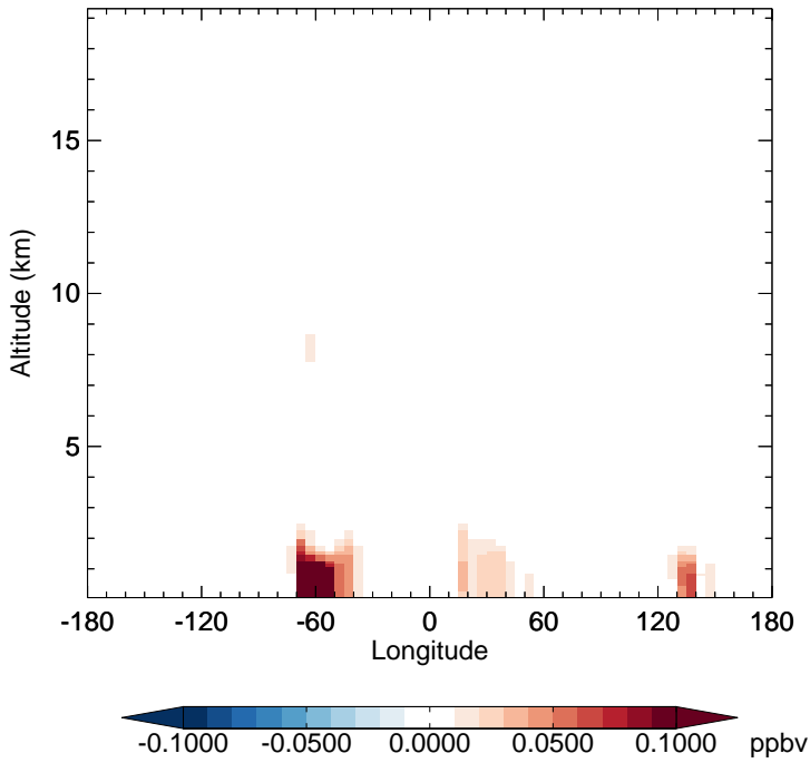
v11-02d - v11-02a RIPB - Diff along 15S for Apr
