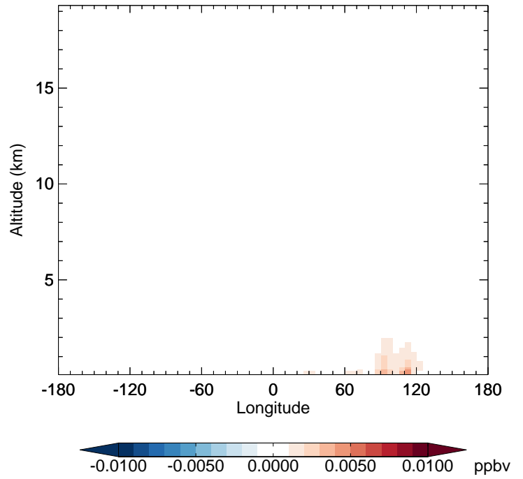
v11-02d - v11-02c NO3 - Diff along 42N for Apr
