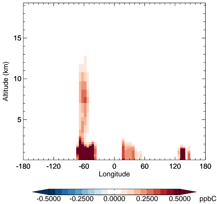
v11-02d - v11-02a ISOP - Diff along 15S for Apr
