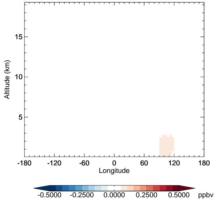
v11-02d - v11-02c CH 2 O - Diff along 42N for Apr
