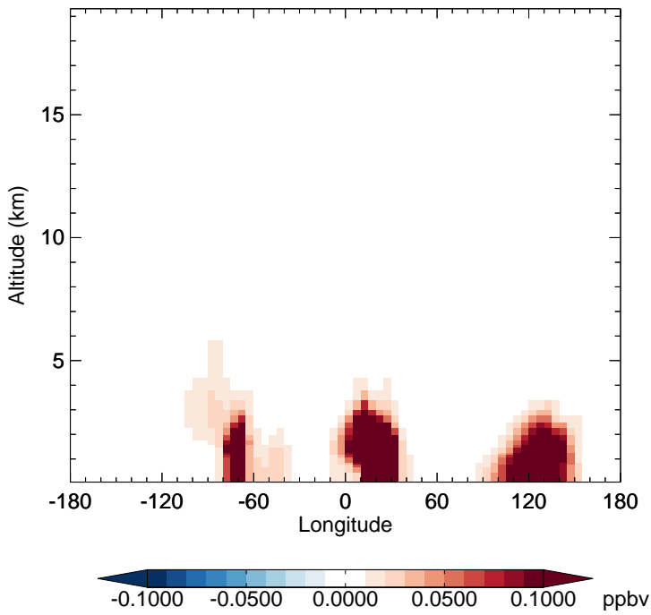
v11-02d - v11-02a SOAIE - Diff along 15S for Apr
