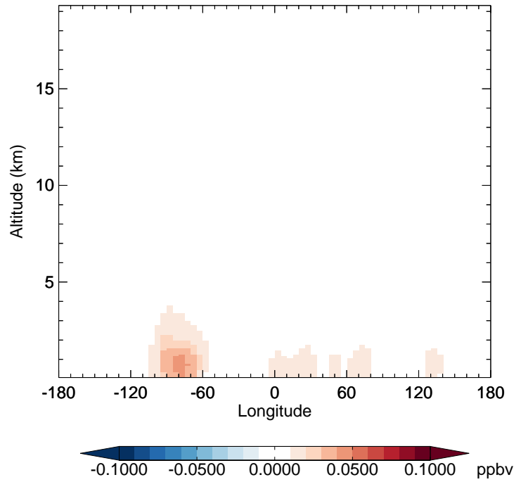
v11-02d - v11-02a IONITA - Diff along 42N for Apr
