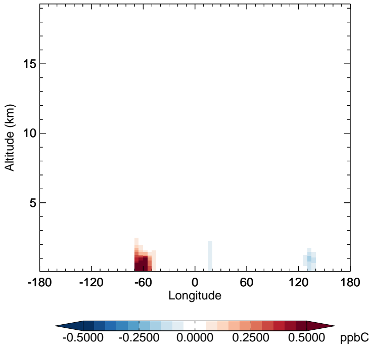
v11-02d - v11-02c ISOP - Diff along 15S for Apr
