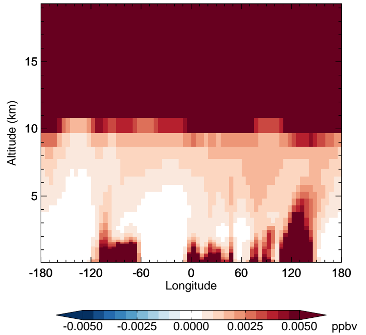
v11-02d - v11-02a N2O5 - Diff along 42N for Apr
