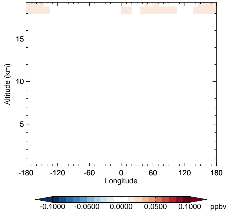
v11-02d - v11-02c CFC113 - Diff along 42N for Apr
