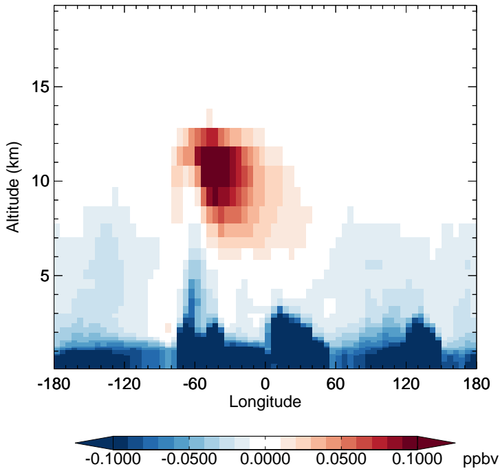
v11-02d - v11-02a H2O2 - Diff along 15S for Apr
