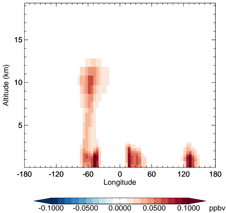
v11-02d - v11-02a HC187 - Diff along 15S for Apr
