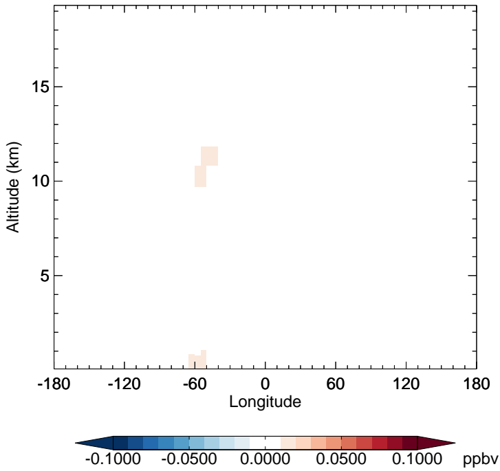
v11-02d - v11-02a TSOA2 - Diff along 15S for Apr
