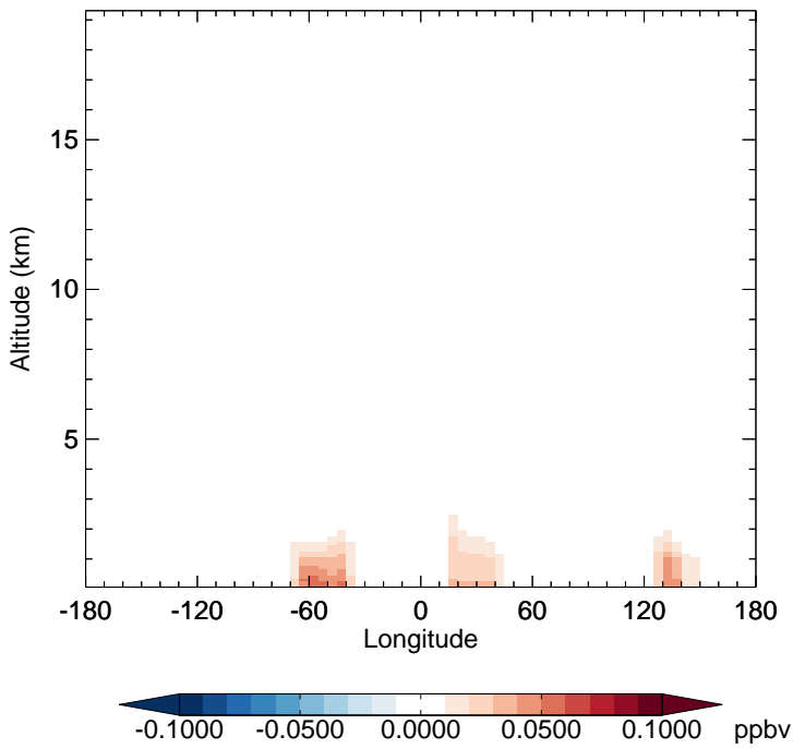
v11-02d - v11-02a GLYX - Diff along 15S for Apr
