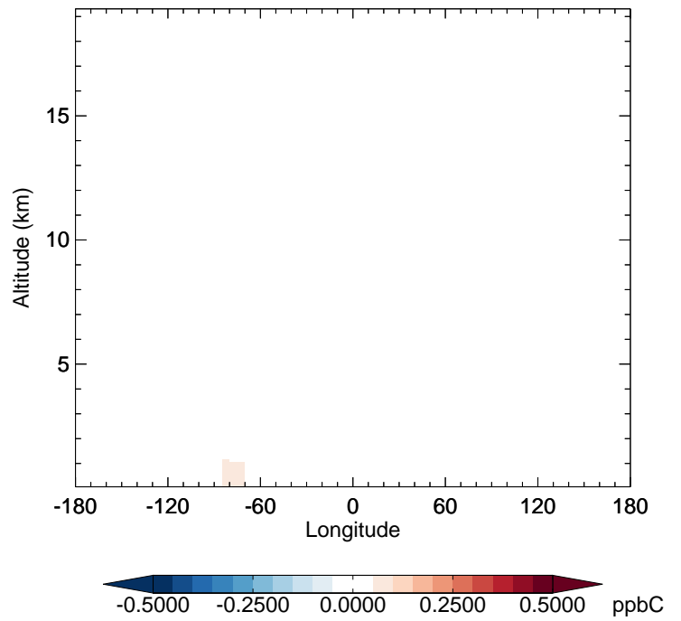
v11-02d - v11-02a ALD2 - Diff along 42N for Apr
