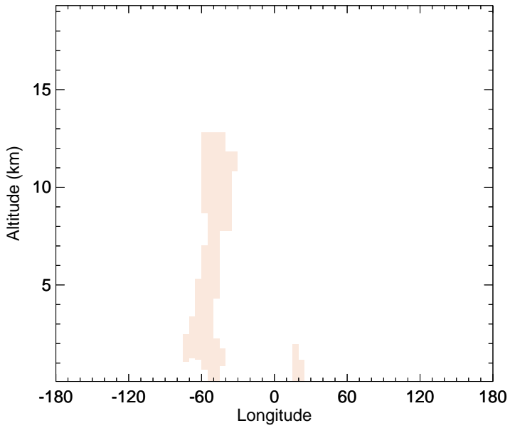
v11-02d - v11-02a ACET - Diff along 15S for Apr
