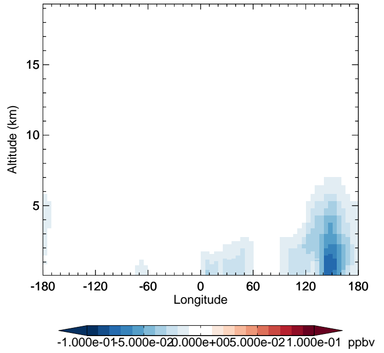
v11-02d - v11-02c TOLU - Diff along 42N for Apr
