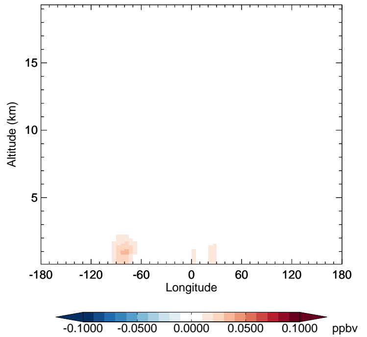
v11-02d - v11-02a IMAE - Diff along 42N for Apr
