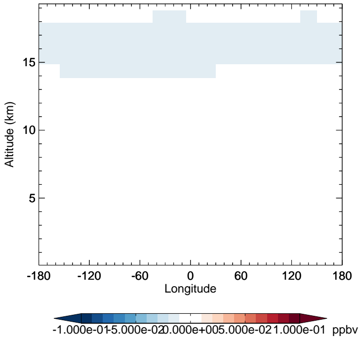
v11-02d - v11-02c HCFC22 - Diff along 15S for Apr
