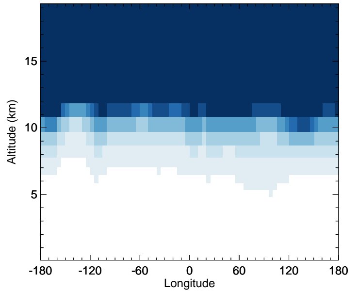
v11-02d - v11-02a HCl - Diff along 42N for Apr
