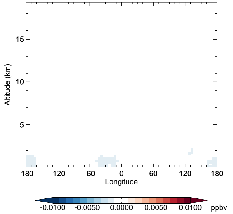
v11-02d - v11-02c HOBr - Diff along 42N for Apr
