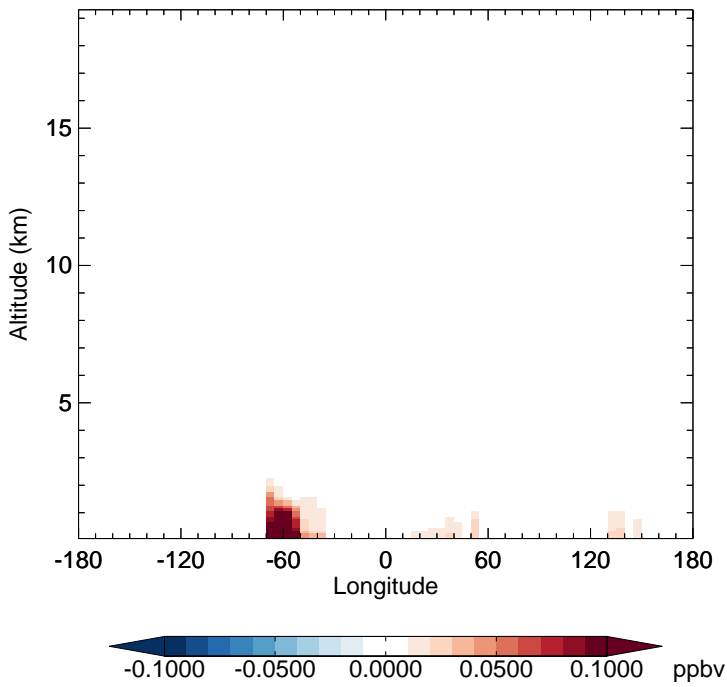
v11-02d - v11-02a MTPA - Diff along 15S for Apr
