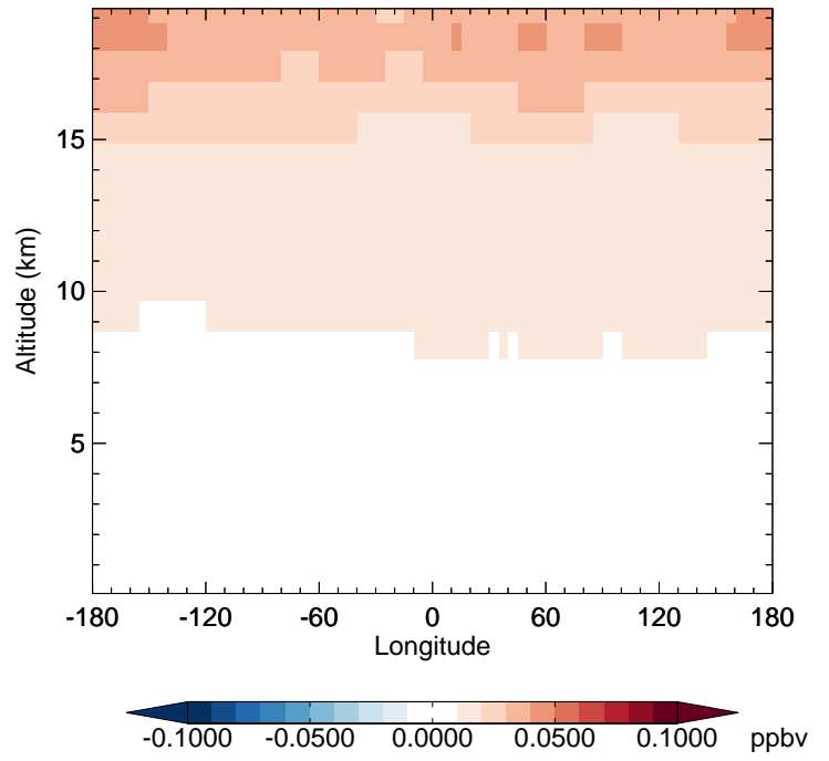
v11-02d - v11-02c CFC11 - Diff along 42N for Apr
