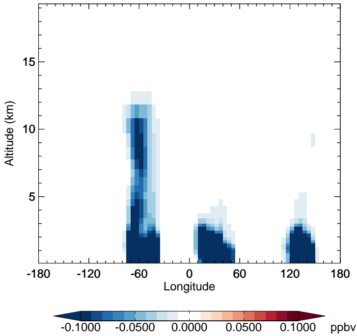
v11-02d - v11-02a HAC - Diff along 15S for Apr
