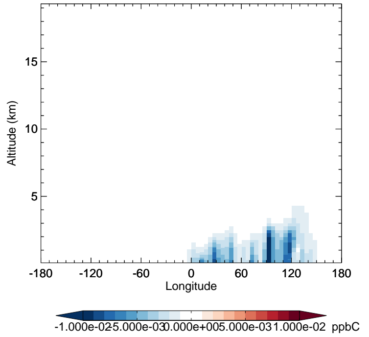
v11-02d - v11-02c PRPE - Diff along 42N for Apr
