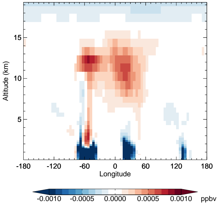
v11-02d - v11-02a PPN - Diff along 15S for Apr
