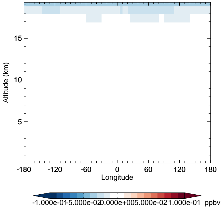
v11-02d - v11-02a N2O - Diff along 15S for Apr
