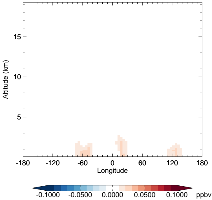
v11-02d - v11-02a SOAGX - Diff along 15S for Apr
