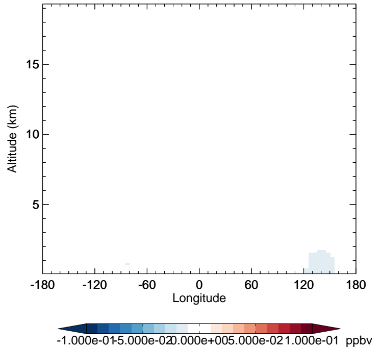
v11-02d - v11-02c SOAGX - Diff along 42N for Apr
