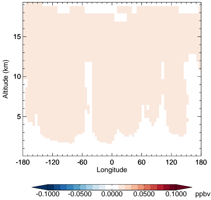
v11-02d - v11-02c CFC12 - Diff along 15S for Apr
