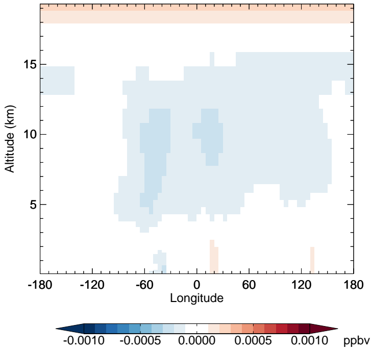
v11-02d - v11-02c PPN - Diff along 15S for Apr
