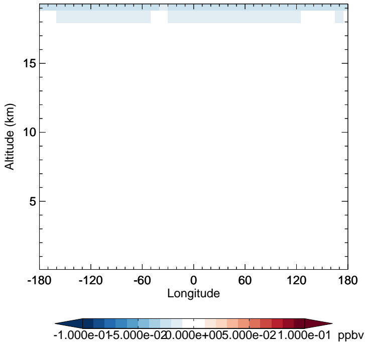
v11-02d - v11-02a CINO3 - Diff along 15S for Apr
