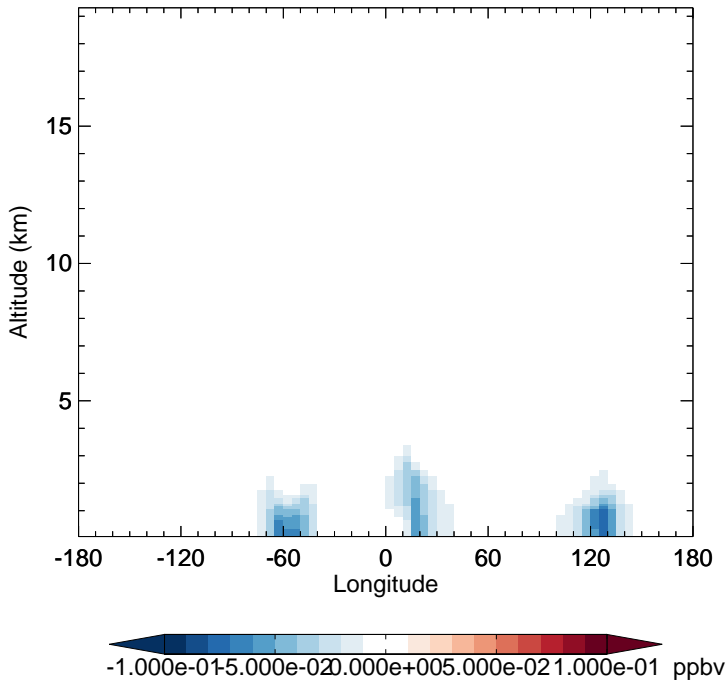
v11-02d - v11-02c SOAGX - Diff along 15S for Apr
