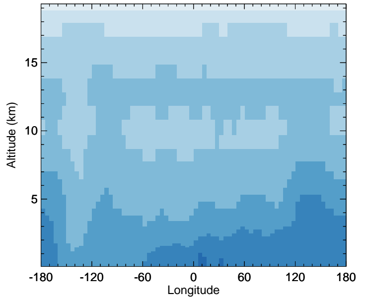
v11-02d - v11-02c C2H6 - Diff along 42N for Apr
