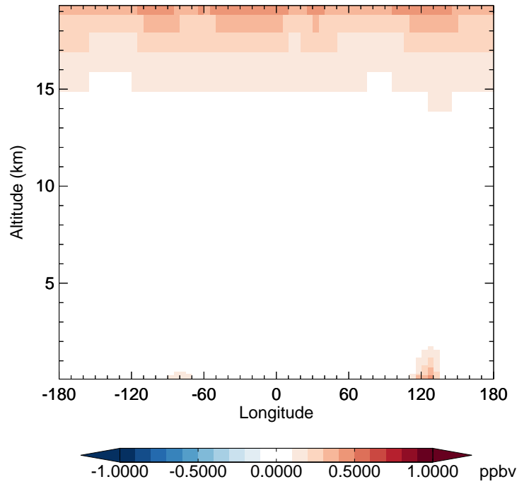
v11-02d - v11-02a NO 2 - Diff along 42N for Apr
