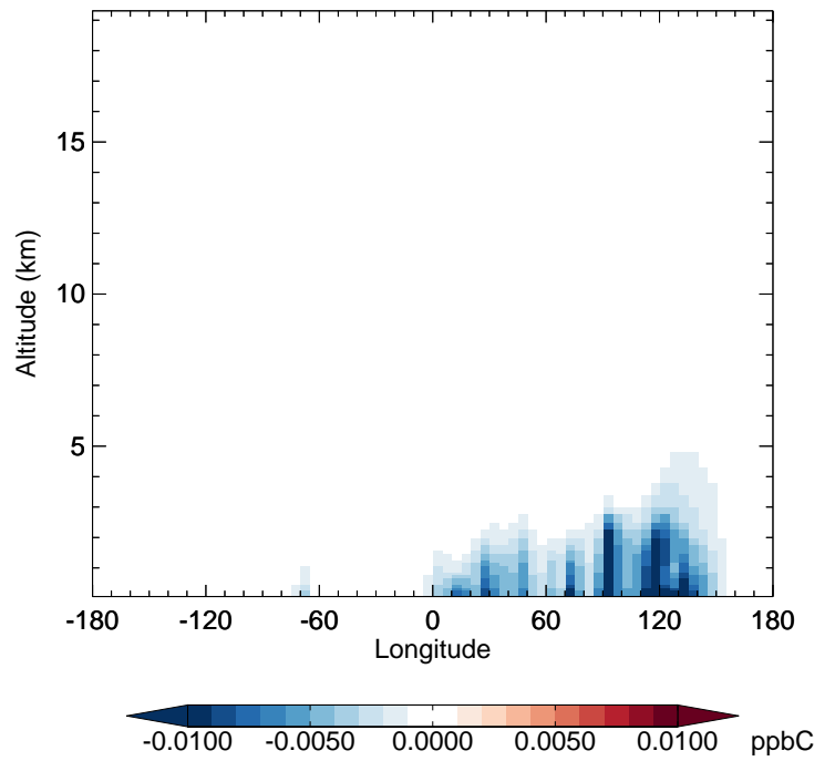
v11-02d - v11-02a PRPE - Diff along 42N for Apr
