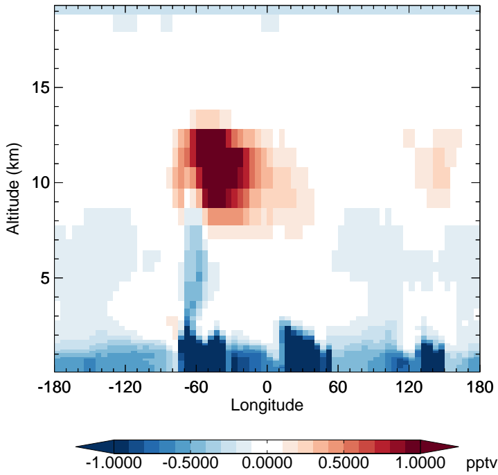
v11-02d - v11-02a HO2 - Diff along 15S for Apr
