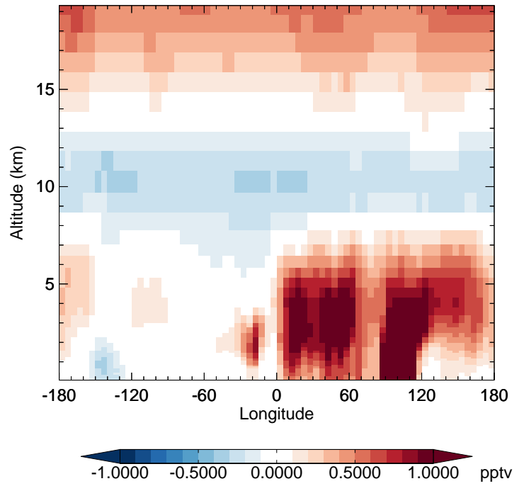
v11-02d - v11-02c HO2 - Diff along 42N for Apr
