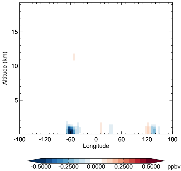
v11-02d - v11-02a CH 2 O - Diff along 15S for Apr
