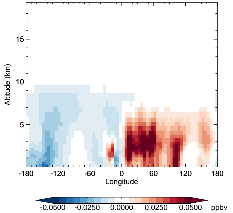
v11-02d - v11-02a MP - Diff along 42N for Apr
