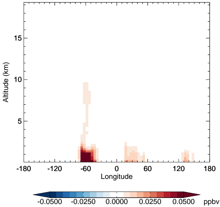
v11-02d - v11-02a RCHO - Diff along 15S for Apr
