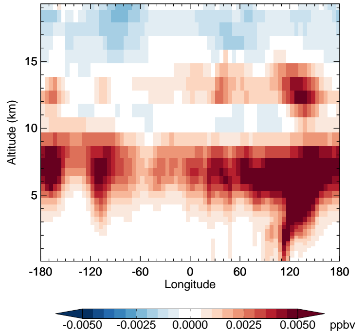
v11-02d - v11-02c HNO 4 - Diff along 42N for Apr
