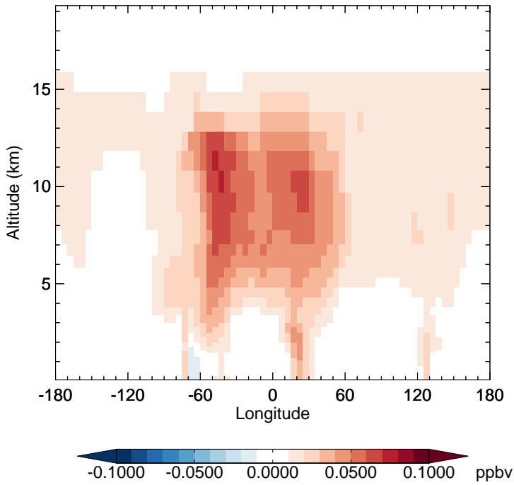
v11-02d - v11-02a PAN - Diff along 15S for Apr
