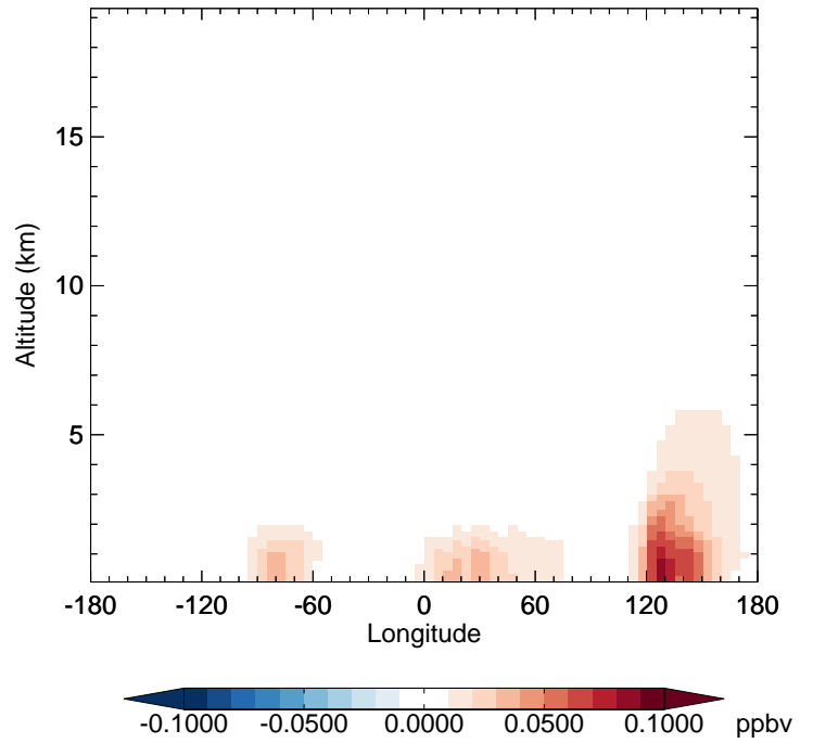
v11-02d - v11-02a SOAGX - Diff along 42N for Apr
