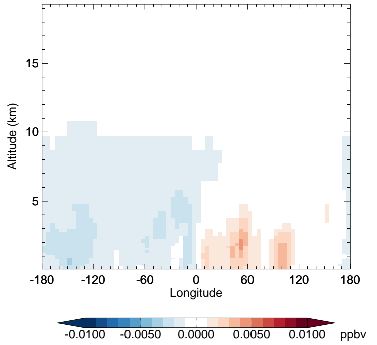
v11-02d - v11-02c MAP - Diff along 42N for Apr
