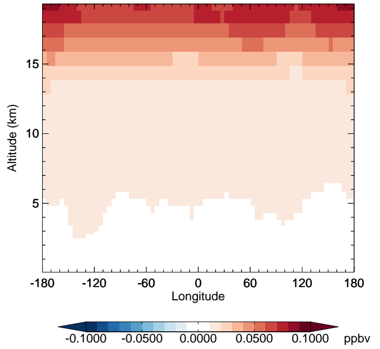
v11-02d - v11-02c CFC12 - Diff along 42N for Apr
