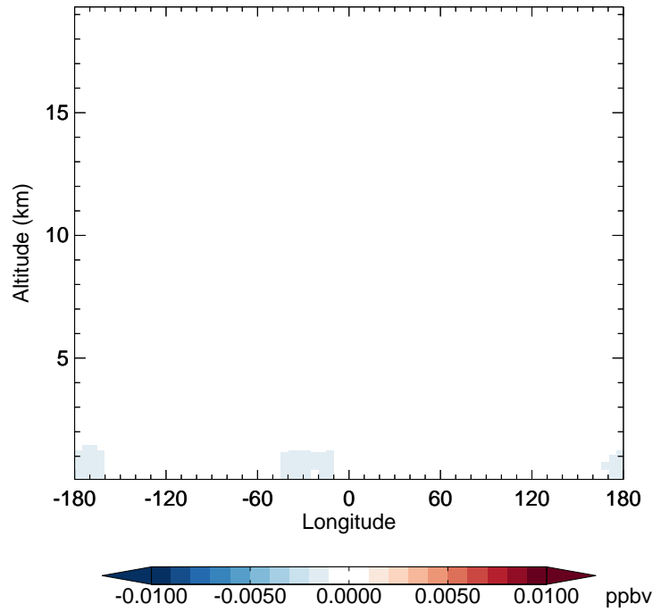
v11-02d - v11-02a HOBr - Diff along 42N for Apr
