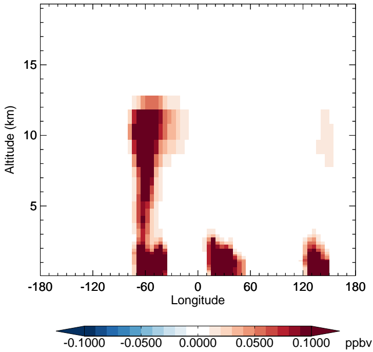
v11-02d - v11-02a IEPOXA - Diff along 15S for Apr
