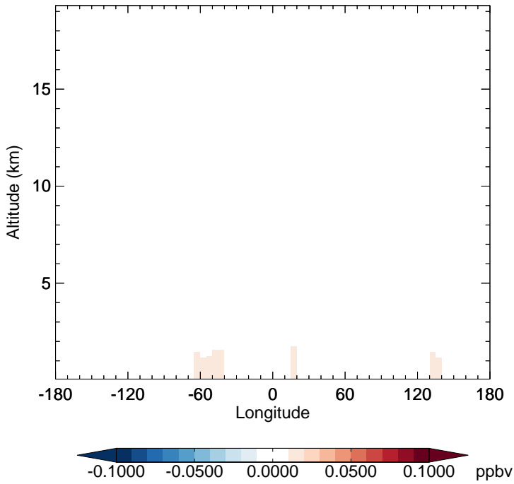
v11-02d - v11-02a IEPOXD - Diff along 15S for Apr
