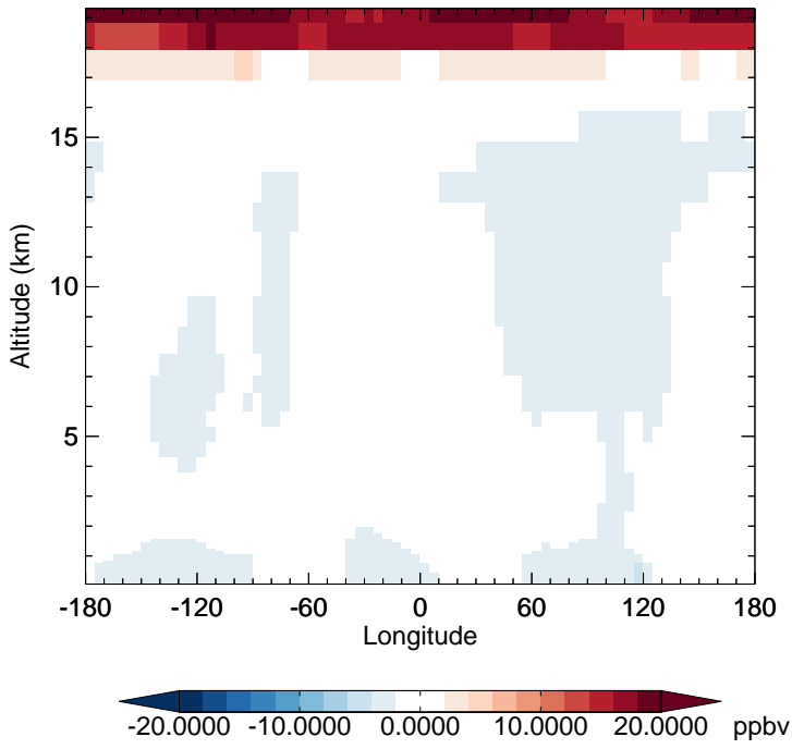
v11-02d - v11-02c O3 - Diff along 15S for Apr
