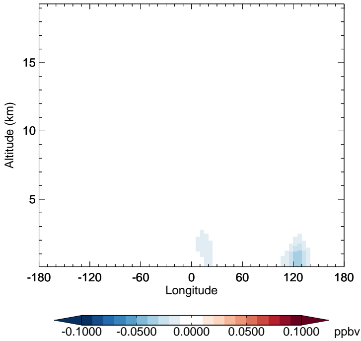
v11-02d - v11-02c INDIOL - Diff along 15S for Apr
