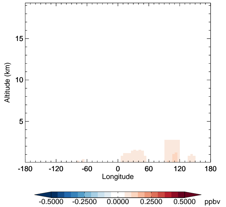
v11-02d - v11-02a CH 2 O - Diff along 42N for Apr
