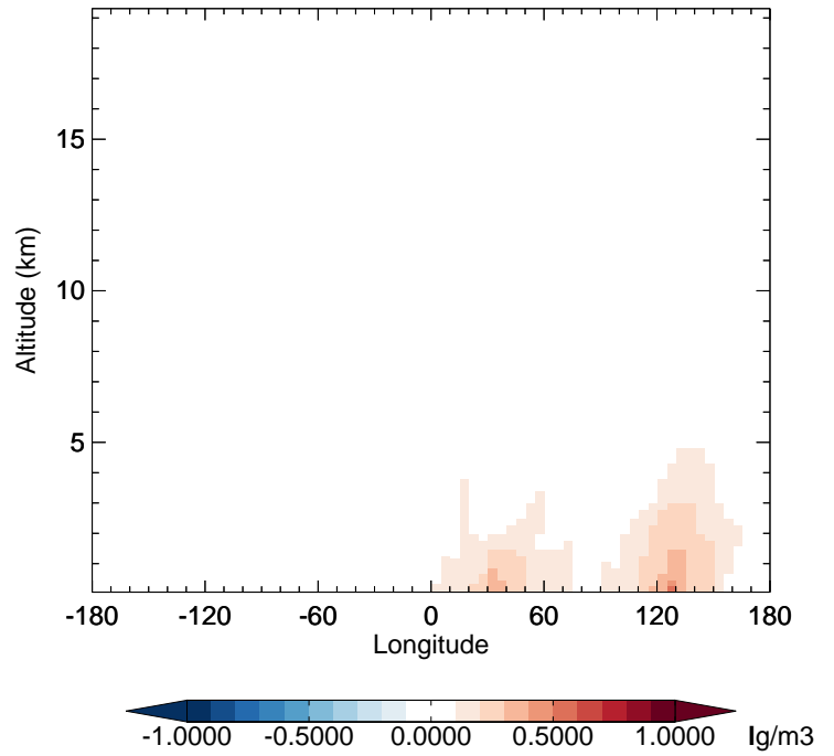
v11-02d - v11-02a SO4 - Diff along 42N for Apr
