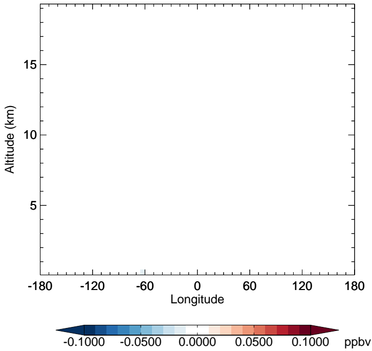
v11-02d - v11-02a ISOA1 - Diff along 15S for Apr
