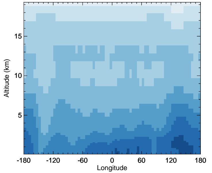
v11-02d - v11-02a C2H6 - Diff along 42N for Apr
