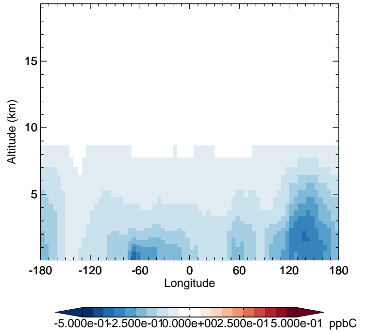
v11-02d - v11-02a ALK4 - Diff along 42N for Apr
