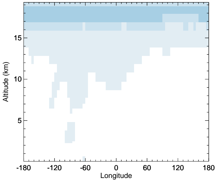
v11-02d - v11-02a C2H6 - Diff along 15S for Apr
