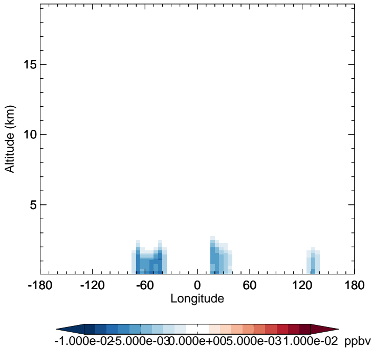
v11-02d - v11-02a NPMN - Diff along 15S for Apr
