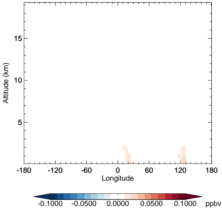
v11-02d - v11-02a TSOG3 - Diff along 15S for Apr
