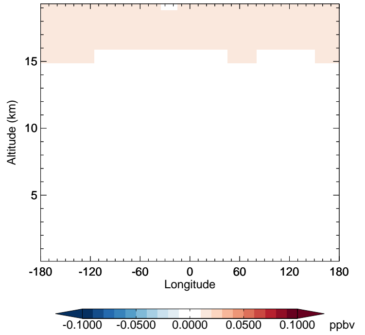
v11-02d - v11-02c CCI4 - Diff along 42N for Apr
