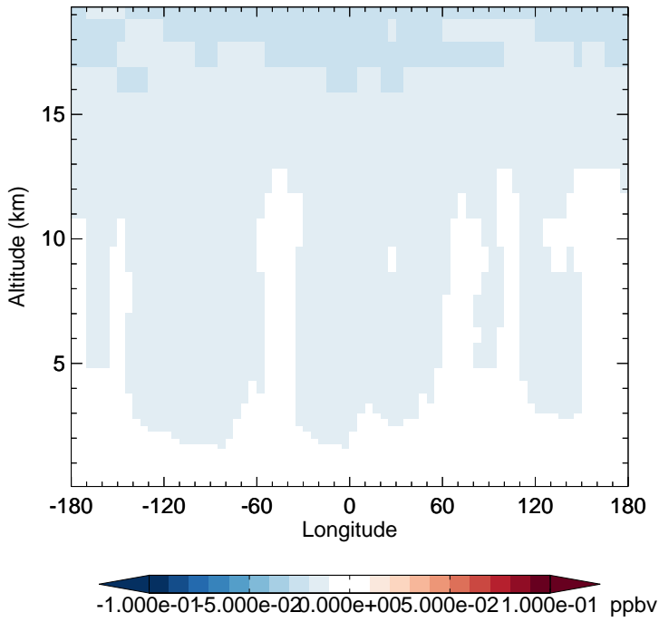
v11-02d - v11-02c OCS - Diff along 15S for Apr
