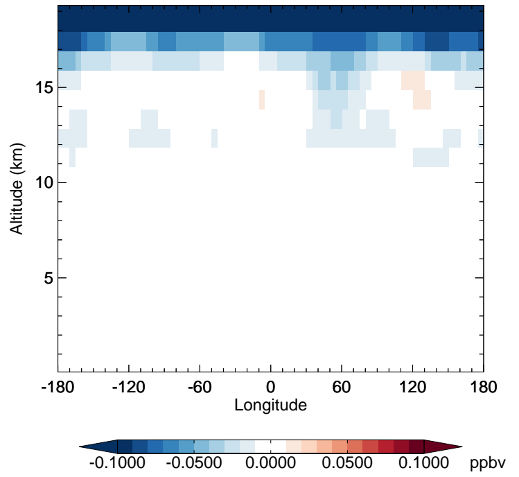
v11-02d - v11-02c CINO3 - Diff along 42N for Apr
