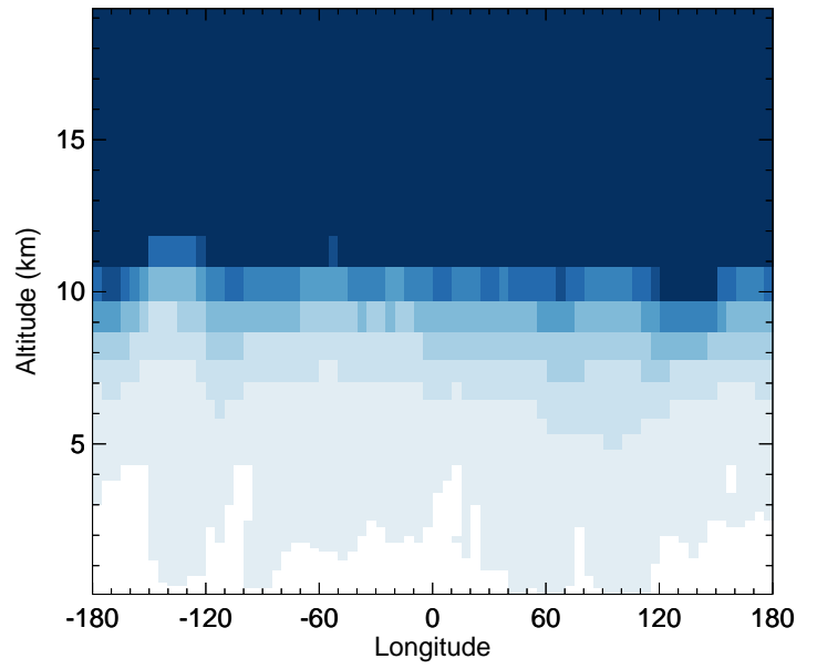
v11-02d - v11-02c HCl - Diff along 42N for Apr
