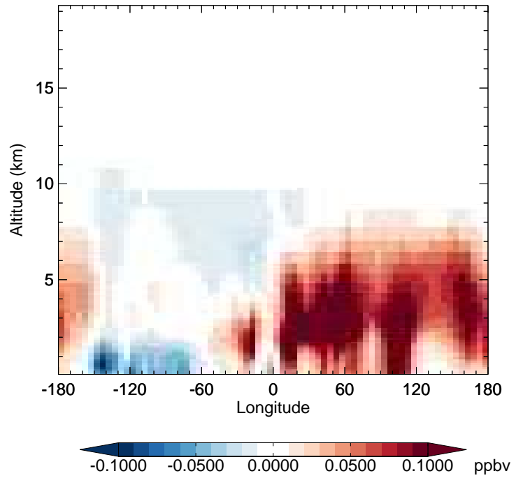
v11-02d - v11-02a H2O2 - Diff along 42N for Apr
