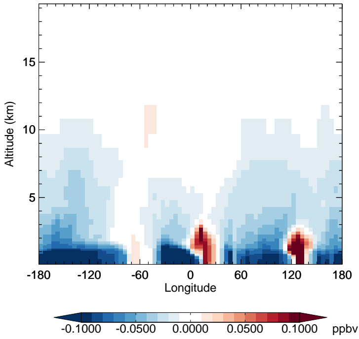
v11-02d - v11-02c H2O2 - Diff along 15S for Apr
