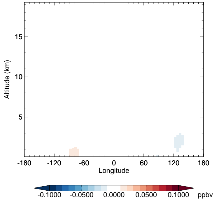
v11-02d - v11-02a MGLY - Diff along 42N for Apr
