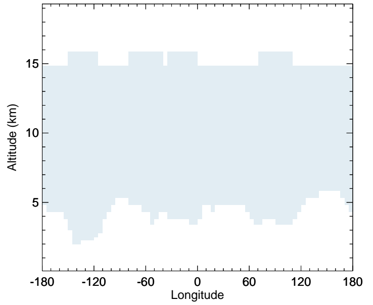
v11-02d - v11-02c HCFC141b - Diff along 42N for Apr
