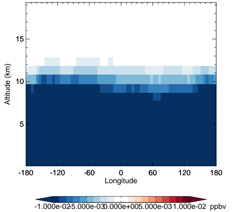
v11-02d - v11-02a R4N2 - Diff along 42N for Apr
