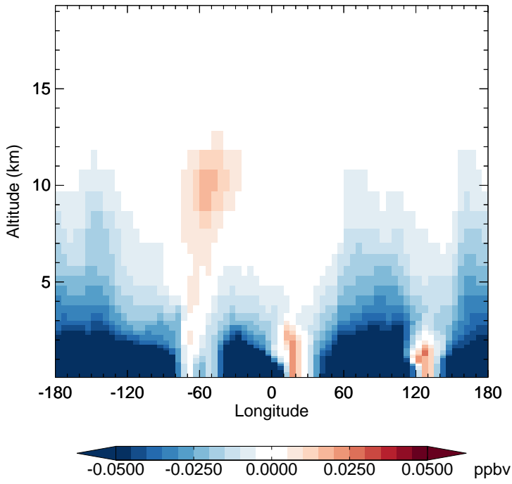
v11-02d - v11-02c MP - Diff along 15S for Apr
