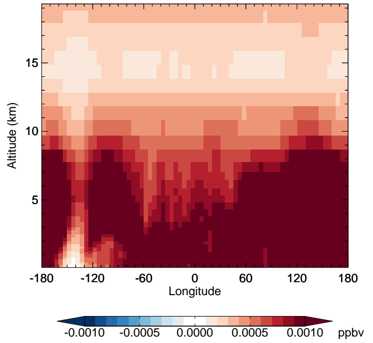
v11-02d - v11-02c PPN - Diff along 42N for Apr
