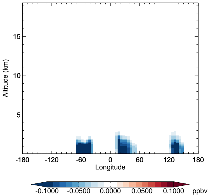
v11-02d - v11-02a GLYC - Diff along 15S for Apr
