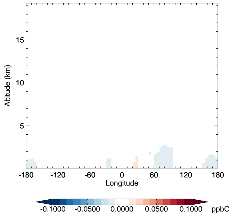
v11-02d - v11-02a MEK - Diff along 42N for Apr
