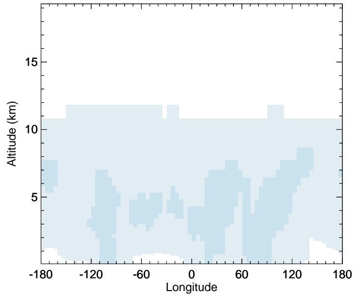
v11-02d - v11-02a ACET - Diff along 42N for Apr
