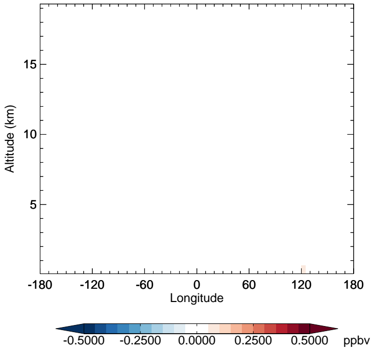
v11-02d - v11-02c CH 2 O - Diff along 15S for Apr
