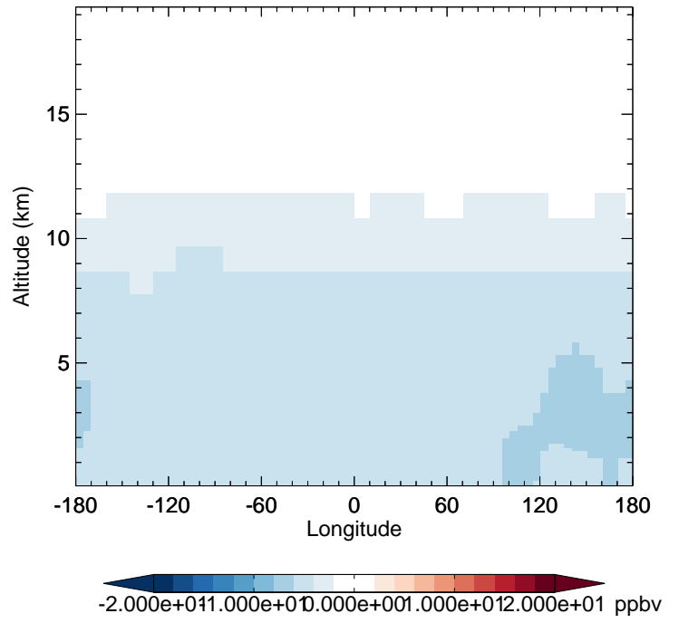
v11-02d - v11-02c CO - Diff along 42N for Apr
