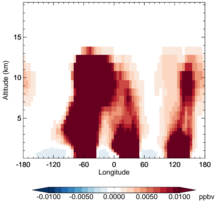
v11-02d - v11-02a MAP - Diff along 15S for Apr
