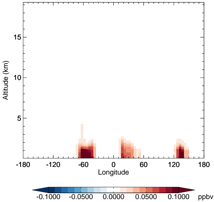
v11-02d - v11-02a MGLY - Diff along 15S for Apr
