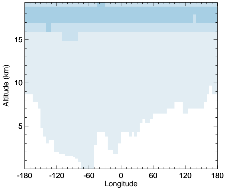
v11-02d - v11-02c C2H6 - Diff along 15S for Apr
