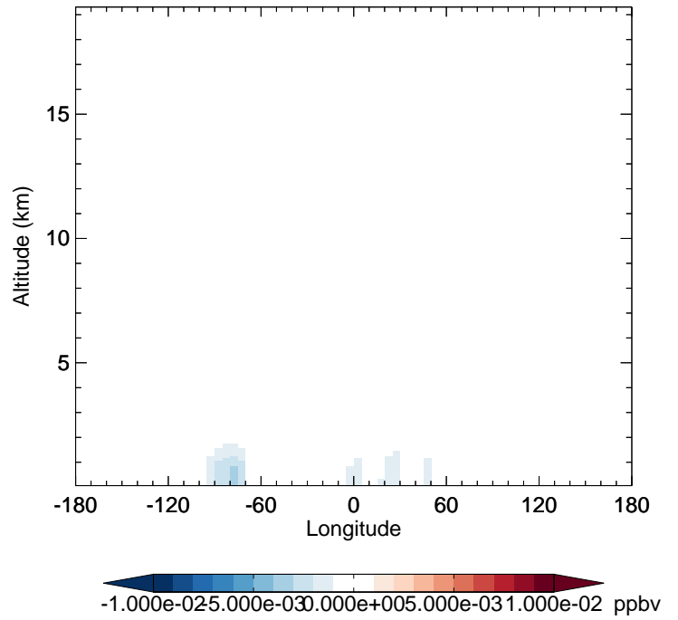
v11-02d - v11-02a NPMN - Diff along 42N for Apr
