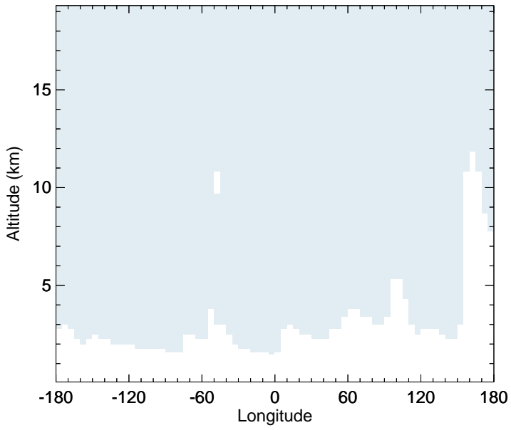
v11-02d - v11-02c HCFC141b - Diff along 15S for Apr
