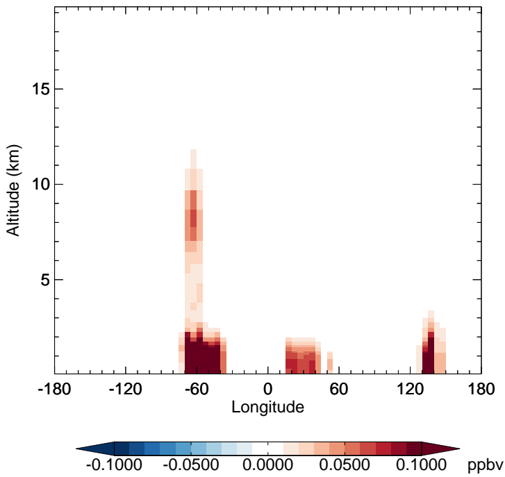
v11-02d - v11-02a RIPA - Diff along 15S for Jan
