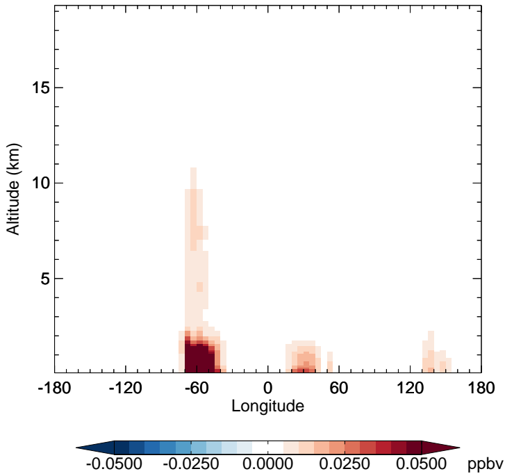
v11-02d - v11-02a RCHO - Diff along 15S for Jan
