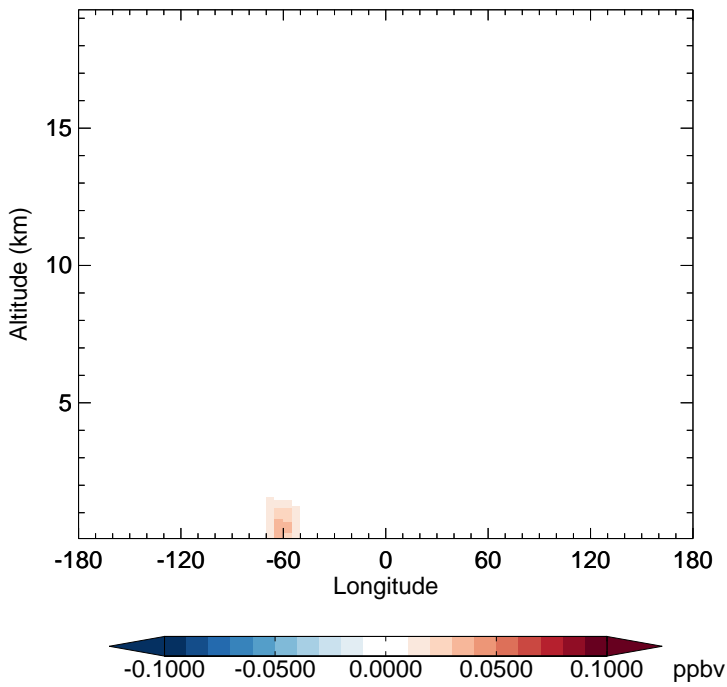
v11-02d - v11-02a RIPD - Diff along 15S for Jan
