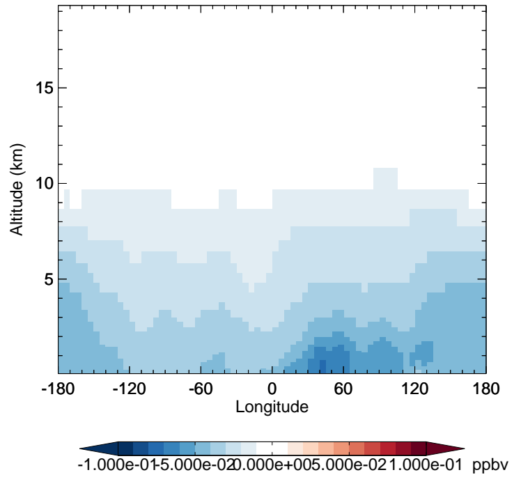
v11-02d - v11-02a BENZ - Diff along 42N for Jan
