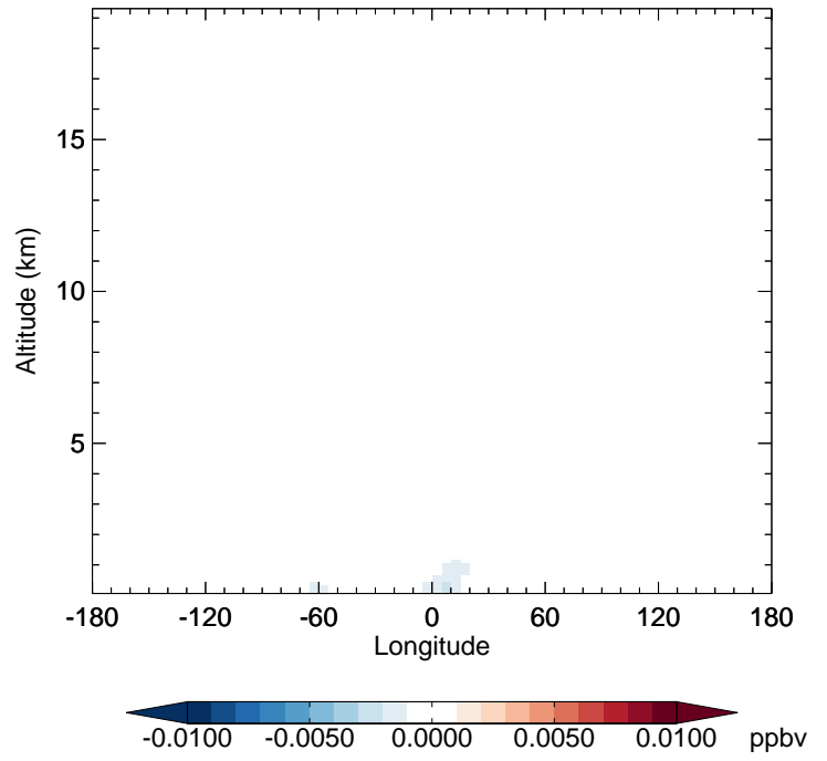
v11-02d - v11-02c NO3 - Diff along 42N for Jan
