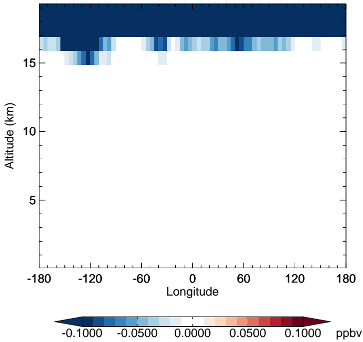
v11-02d - v11-02a H2O - Diff along 15S for Jan
