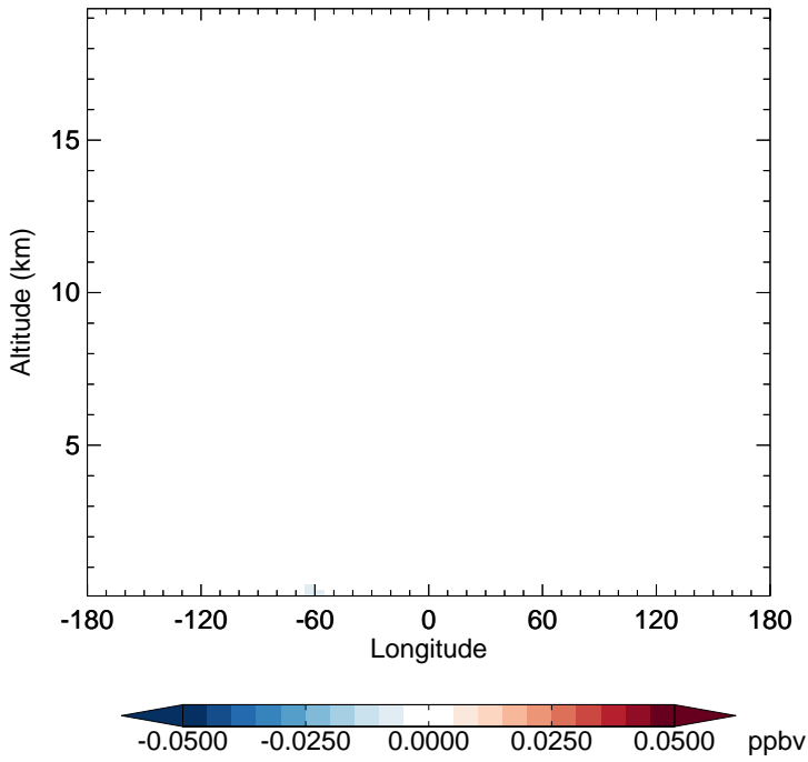
v11-02d - v11-02c RCHO - Diff along 15S for Jan
