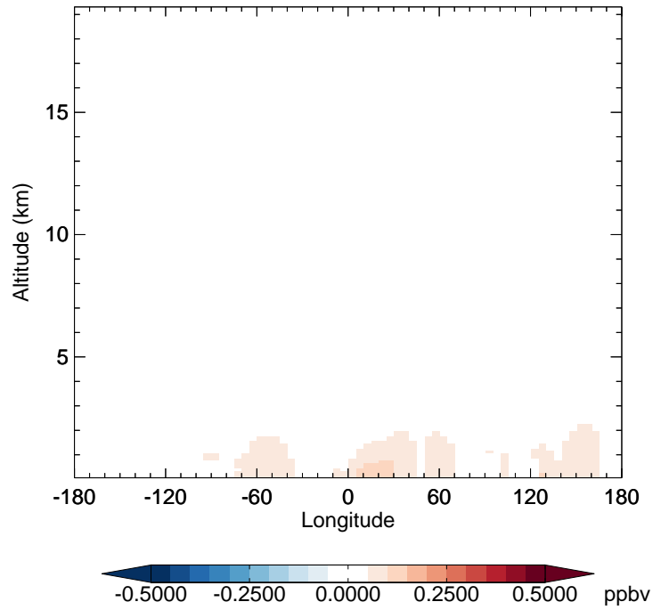
v11-02d - v11-02a CH 2 O - Diff along 42N for Jan
