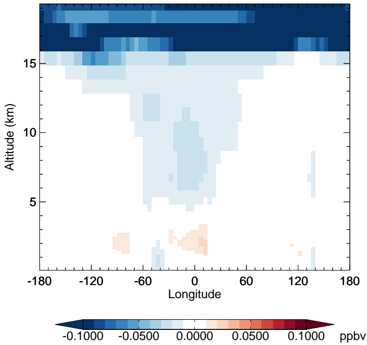
v11-02d - v11-02a HNO 3 - Diff along 15S for Jan
