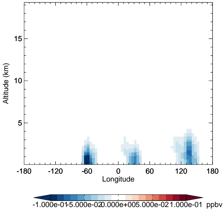
v11-02d - v11-02c SOAGX - Diff along 15S for Jan
