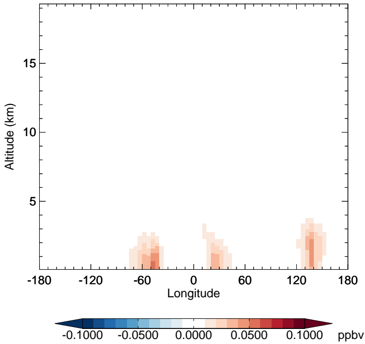
v11-02d - v11-02a IONITA - Diff along 15S for Jan
