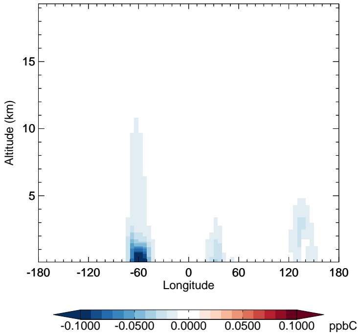
v11-02d - v11-02c MEK - Diff along 15S for Jan
