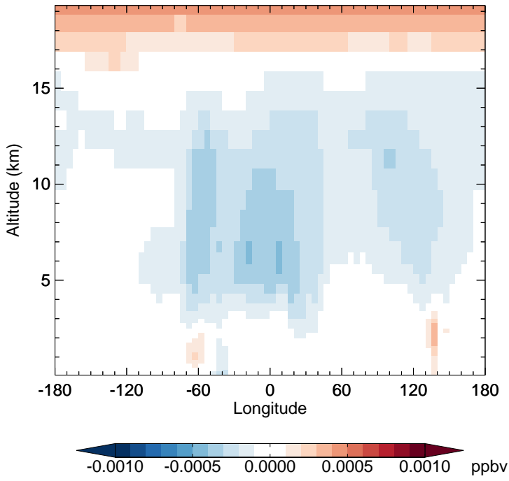
v11-02d - v11-02c PPN - Diff along 15S for Jan
