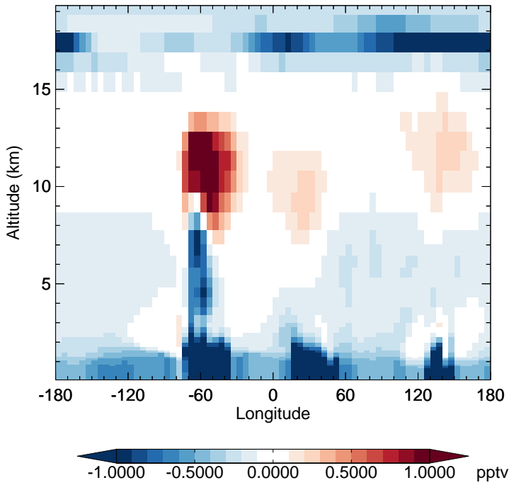
v11-02d - v11-02a HO2 - Diff along 15S for Jan
