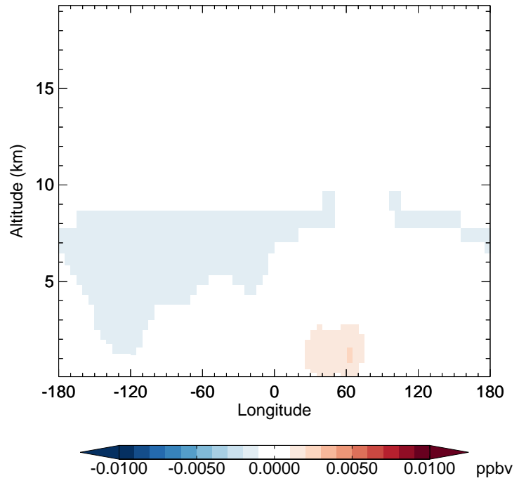
v11-02d - v11-02c MAP - Diff along 42N for Jan
