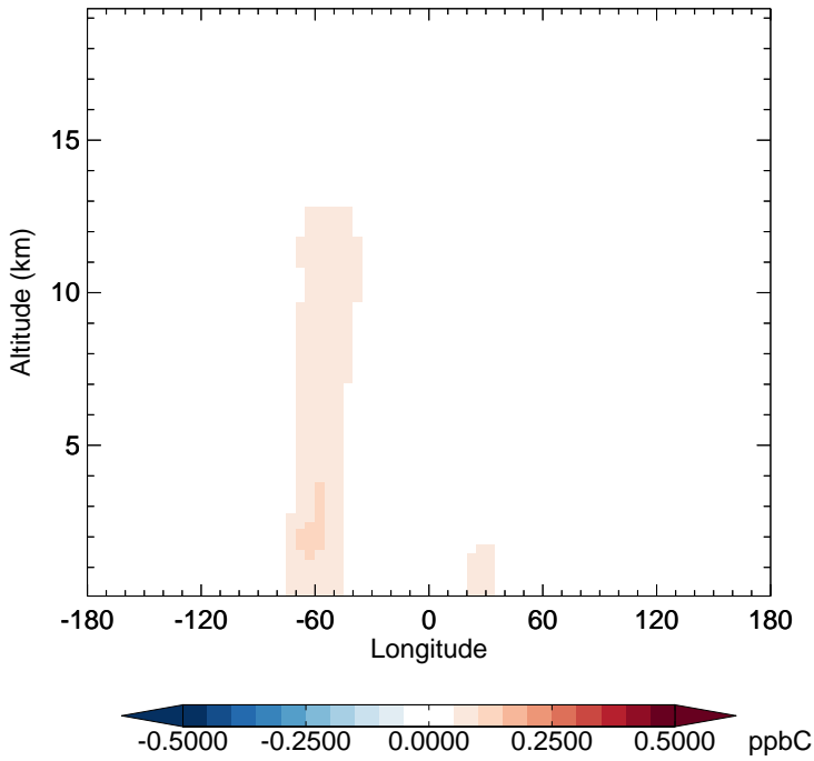
v11-02d - v11-02a ACET - Diff along 15S for Jan
