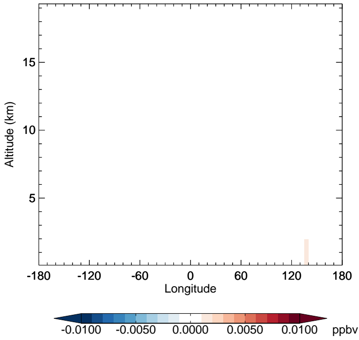
v11-02d - v11-02c MVKN - Diff along 15S for Jan
