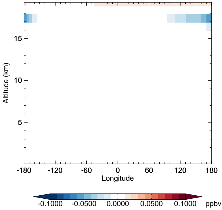
v11-02d - v11-02c CINO3 - Diff along 15S for Jan
