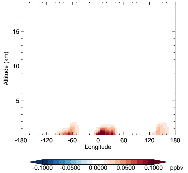
v11-02d - v11-02c CINO2 - Diff along 42N for Jan
