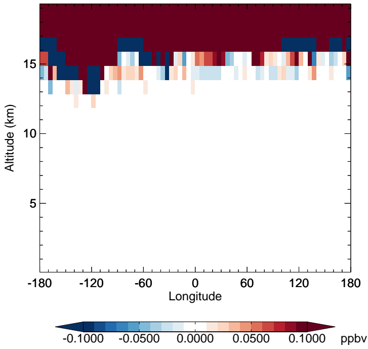
v11-02d - v11-02c H2O - Diff along 15S for Jan
