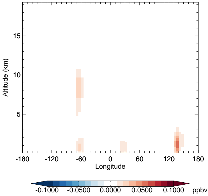
v11-02d - v11-02c IEPOXB - Diff along 15S for Jan
