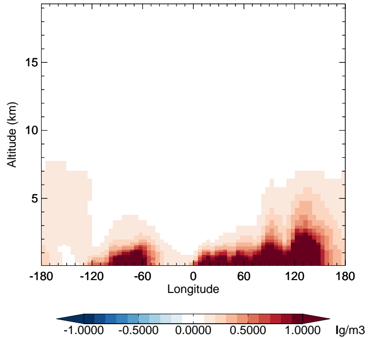
v11-02d - v11-02a SOAS - Diff along 42N for Jan
