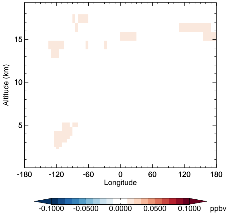
v11-02d - v11-02c CFC12 - Diff along 15S for Jan
