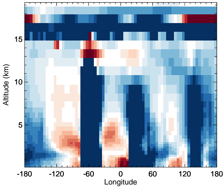
v11-02d - v11-02a OH - Diff along 15S for Jan
