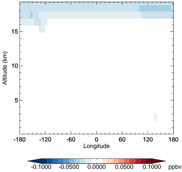
v11-02d - v11-02c PAN - Diff along 15S for Jan
