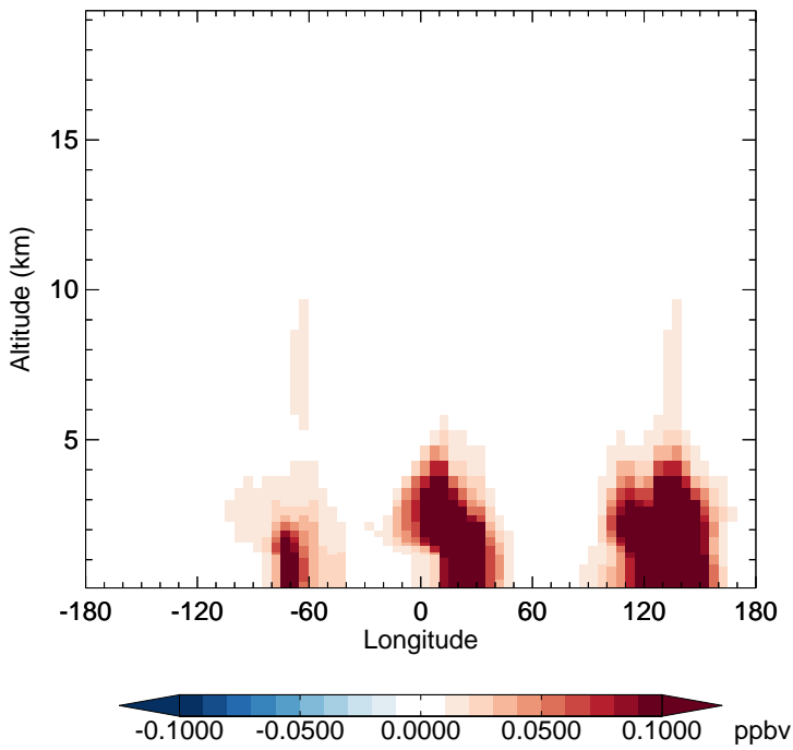
v11-02d - v11-02a SOAIE - Diff along 15S for Jan
