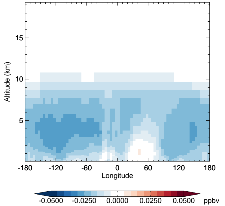
v11-02d - v11-02a MP - Diff along 42N for Jan
