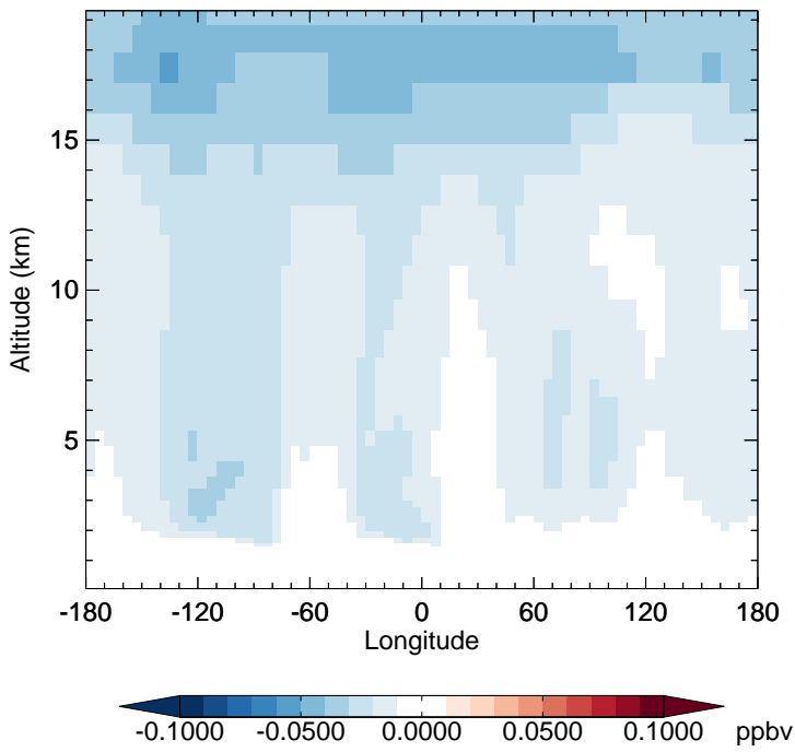
v11-02d - v11-02c CH3Cl - Diff along 15S for Jan
