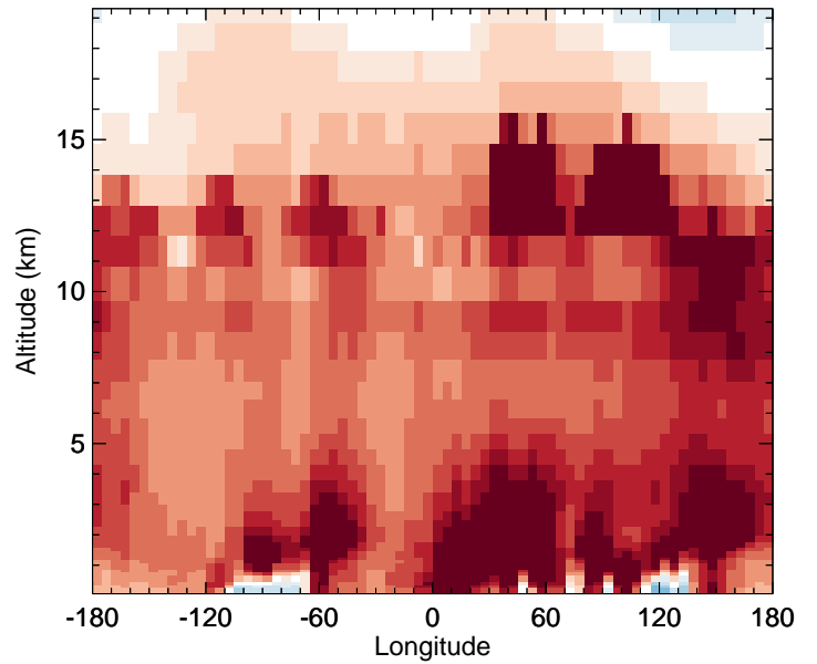
v11-02d - v11-02a OH - Diff along 42N for Jan
