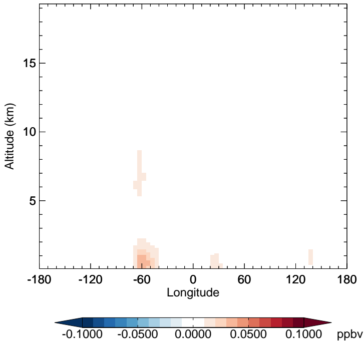
v11-02d - v11-02a TSOG2 - Diff along 15S for Jan
