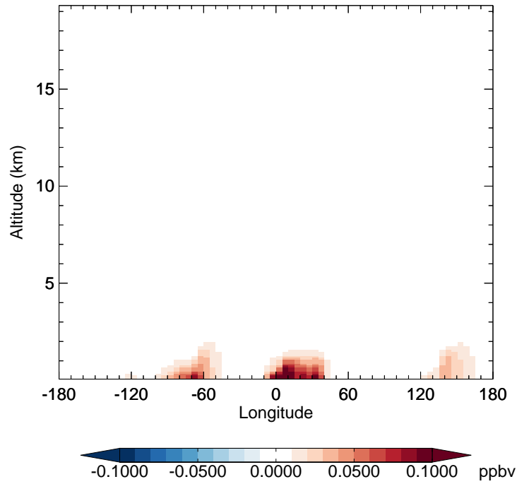
v11-02d - v11-02a CINO2 - Diff along 42N for Jan
