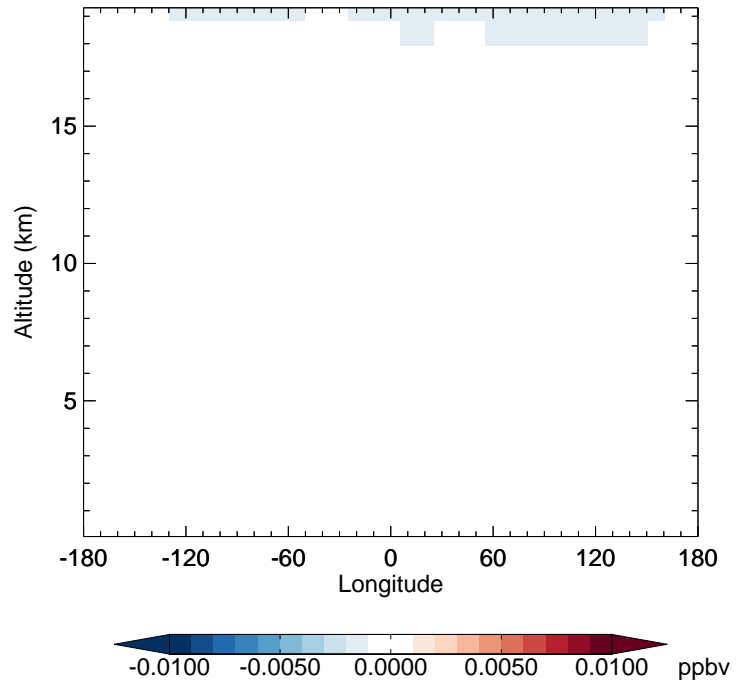
v11-02d - v11-02a BrO - Diff along 42N for Jan
