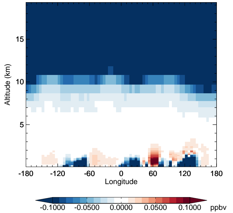
v11-02d - v11-02a HNO 3 - Diff along 42N for Jan
