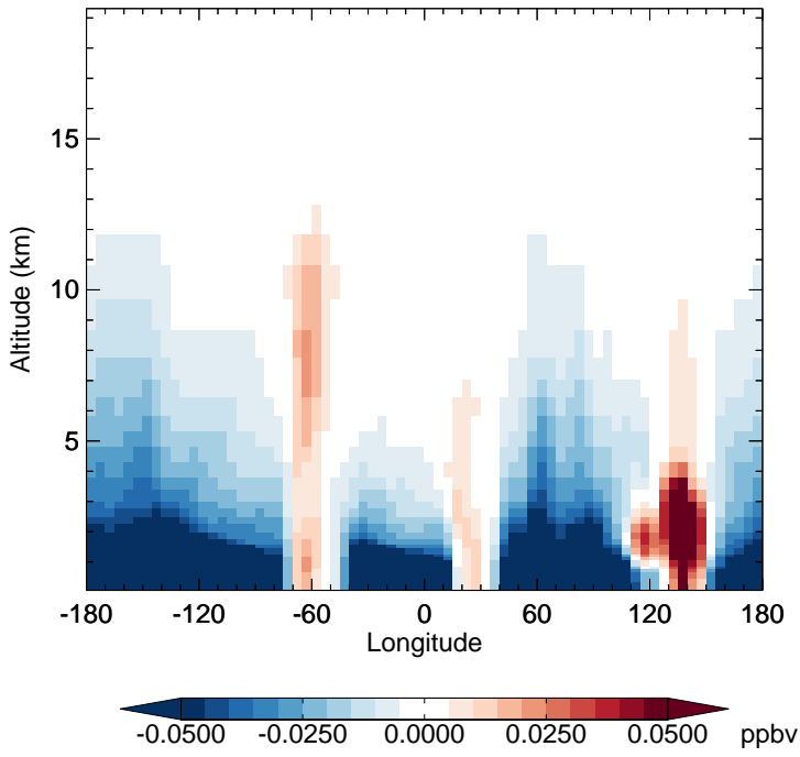
v11-02d - v11-02c MP - Diff along 15S for Jan
