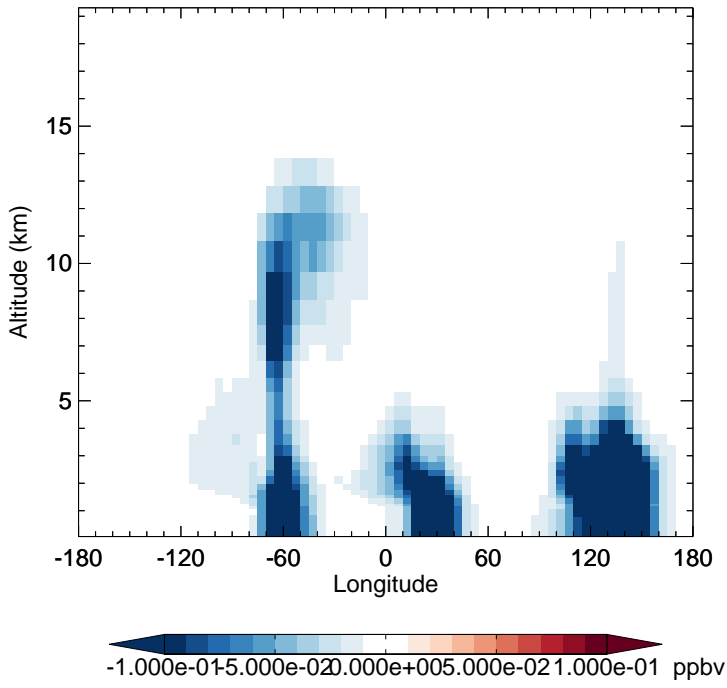
v11-02d - v11-02c SOAIE - Diff along 15S for Jan
