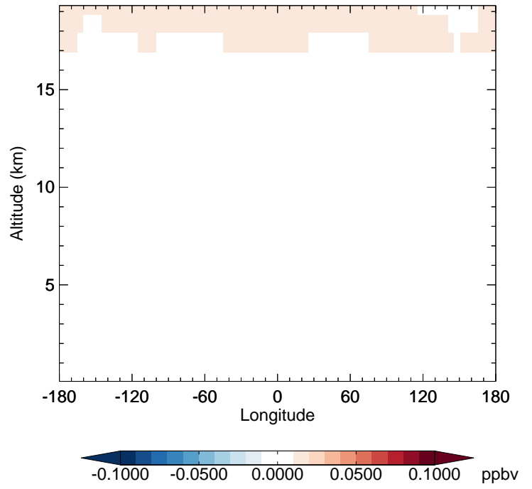
v11-02d - v11-02c CCI4 - Diff along 42N for Jan
