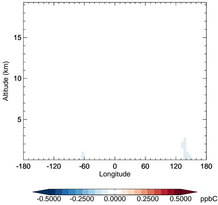
v11-02d - v11-02c ALD2 - Diff along 15S for Jan
