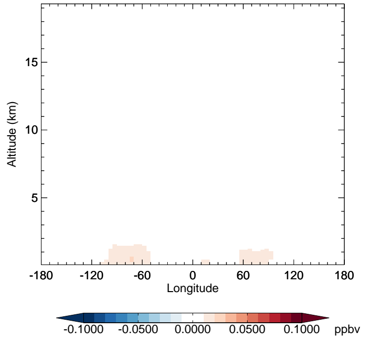
v11-02d - v11-02a IONITA - Diff along 42N for Jan
