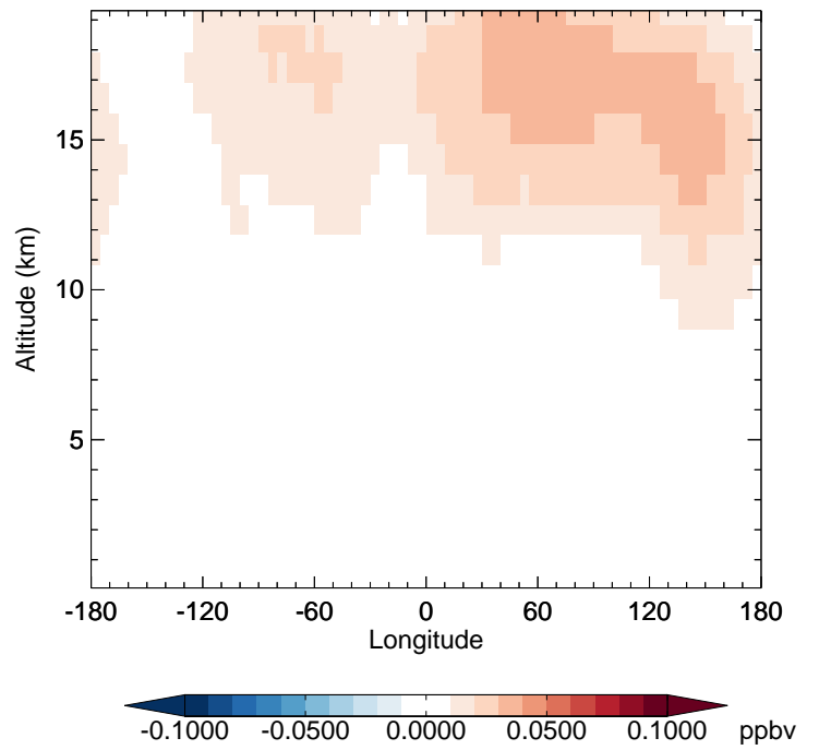
v11-02d - v11-02a MPN - Diff along 42N for Jan
