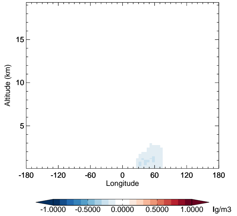
v11-02d - v11-02c SO 2 - Diff along 42N for Jan
