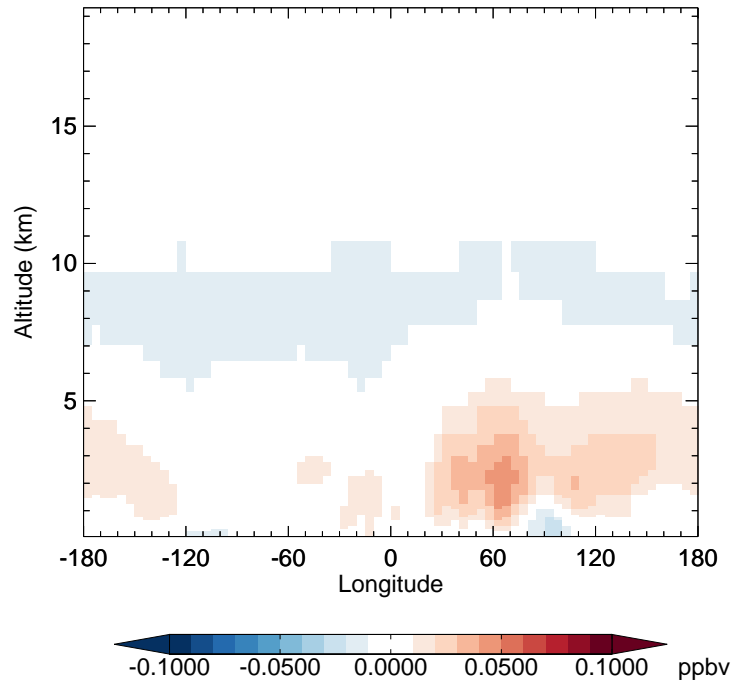
v11-02d - v11-02a H2O2 - Diff along 42N for Jan
