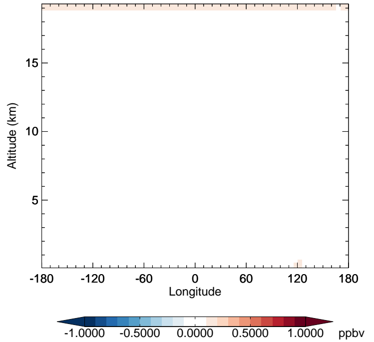
v11-02d - v11-02a NO - Diff along 42N for Jan
