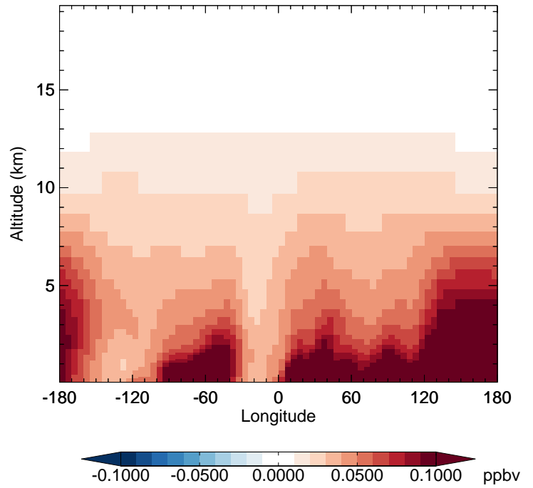
v11-02d - v11-02a PAN - Diff along 42N for Jan
