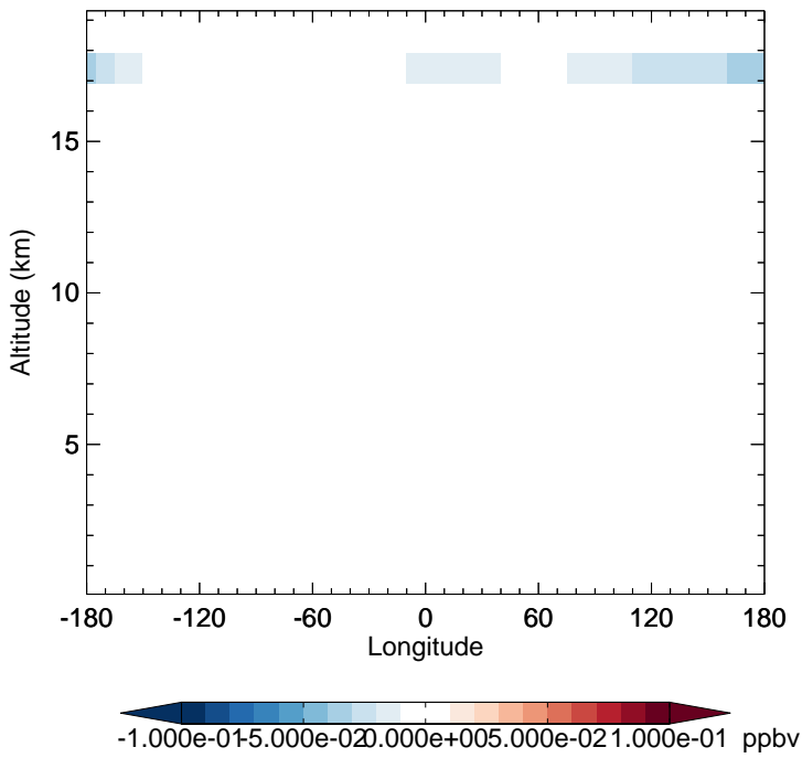
v11-02d - v11-02a ClO - Diff along 15S for Jan
