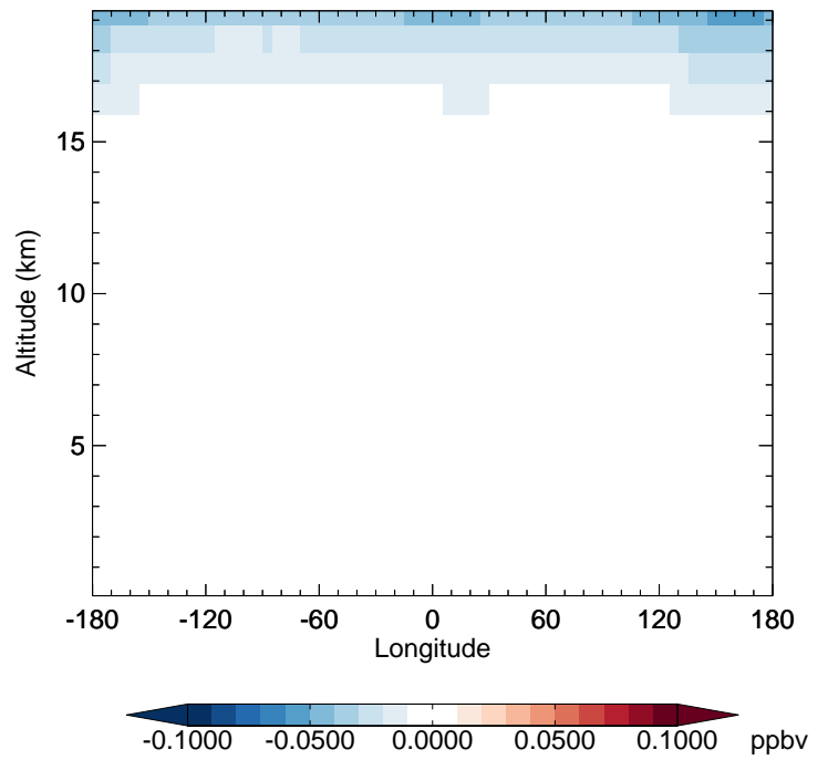
v11-02d - v11-02a N2O - Diff along 42N for Jan
