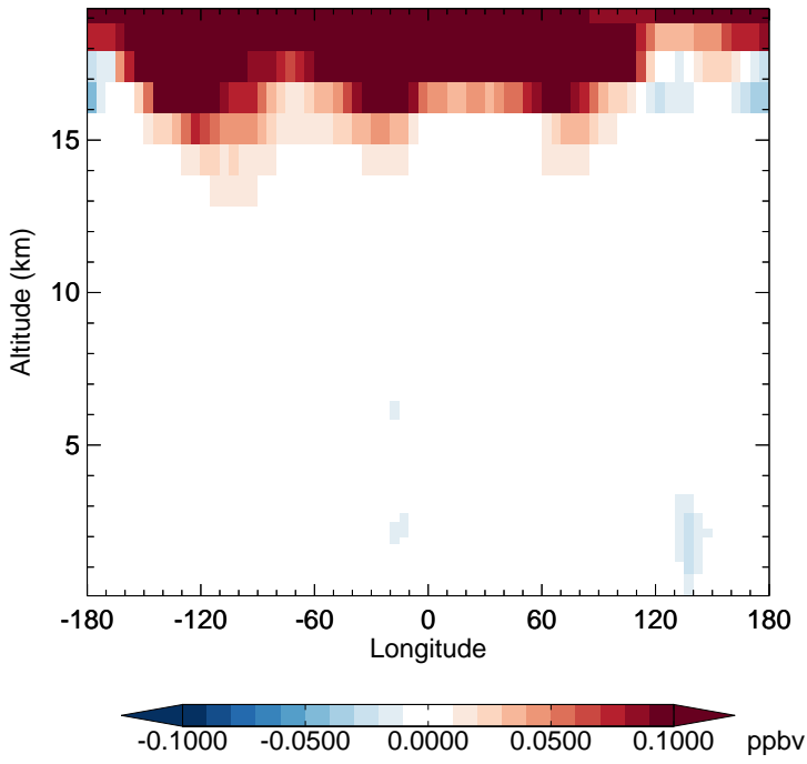
v11-02d - v11-02c HNO 3 - Diff along 15S for Jan
