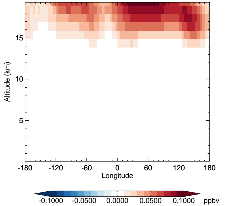
v11-02d - v11-02a CINO3 - Diff along 42N for Jan
