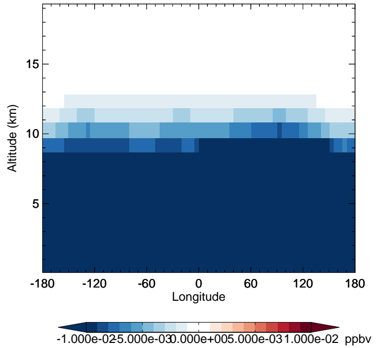
v11-02d - v11-02a R4N2 - Diff along 42N for Jan
