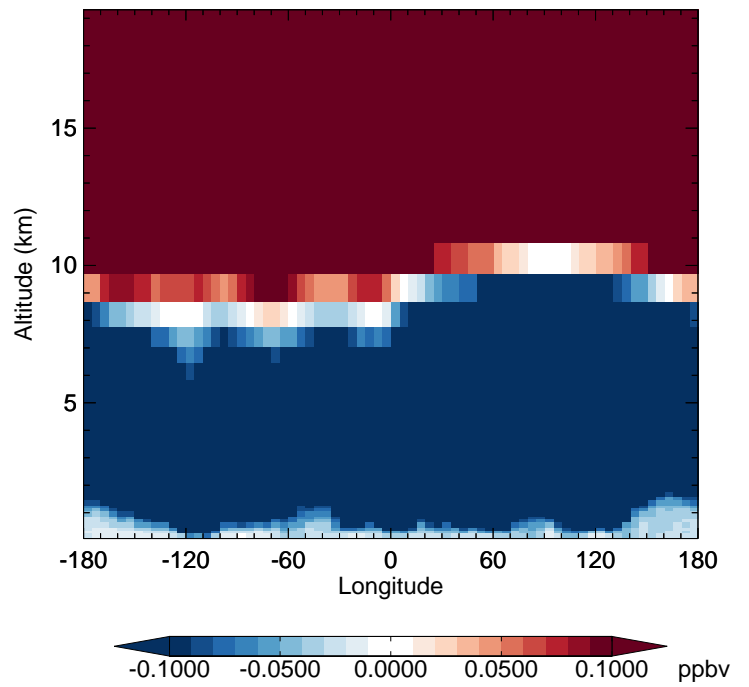
v11-02d - v11-02a CH4 - Diff along 42N for Jan
