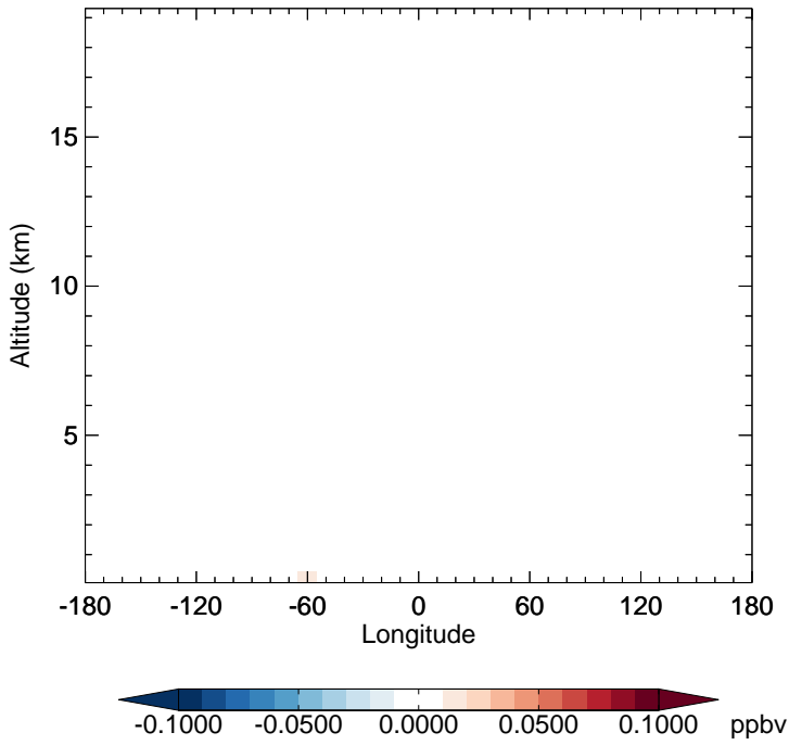
v11-02d - v11-02c GLYX - Diff along 15S for Jan
