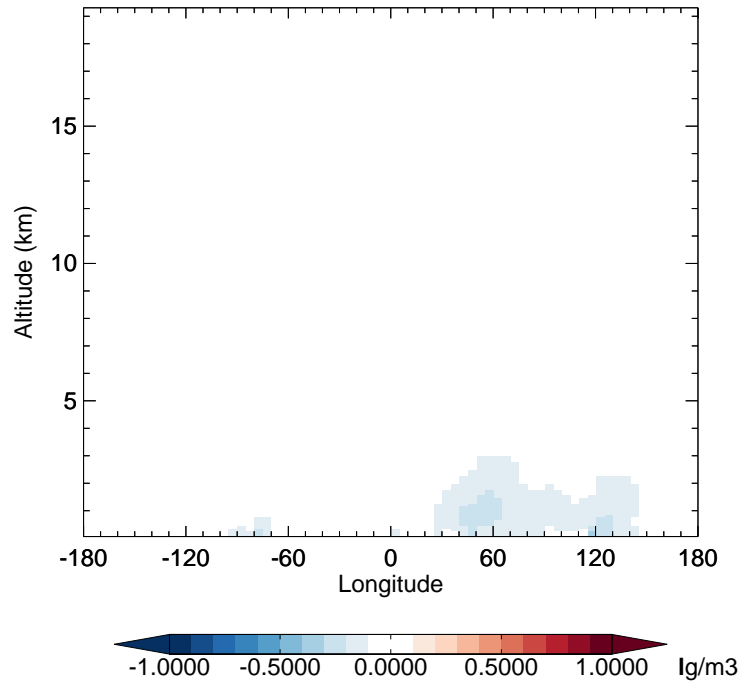
v11-02d - v11-02a SO 2 - Diff along 42N for Jan
