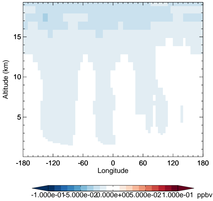
v11-02d - v11-02c OCS - Diff along 15S for Jan
