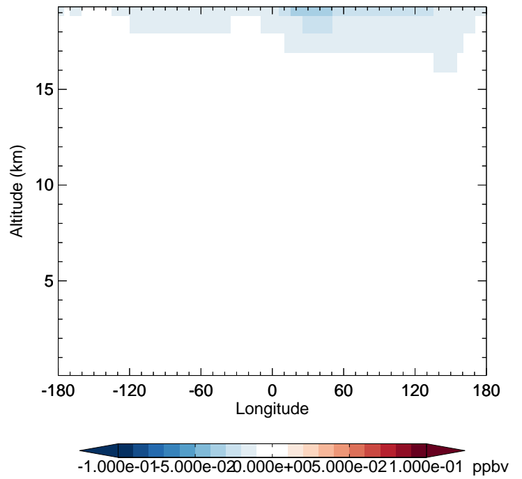
v11-02d - v11-02a ClO - Diff along 42N for Jan
