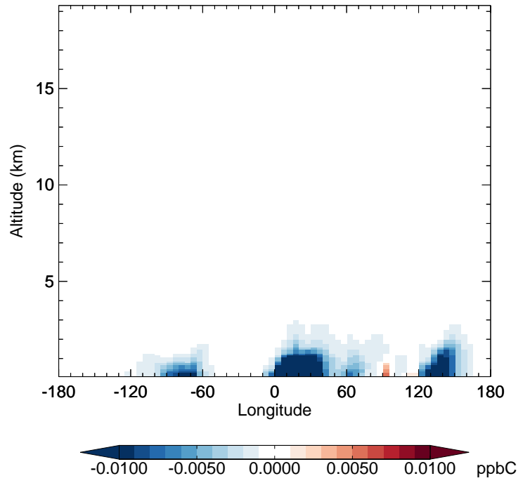
v11-02d - v11-02c PRPE - Diff along 42N for Jan
