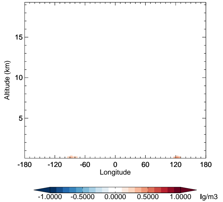
v11-02d - v11-02a NH3 - Diff along 42N for Jan
