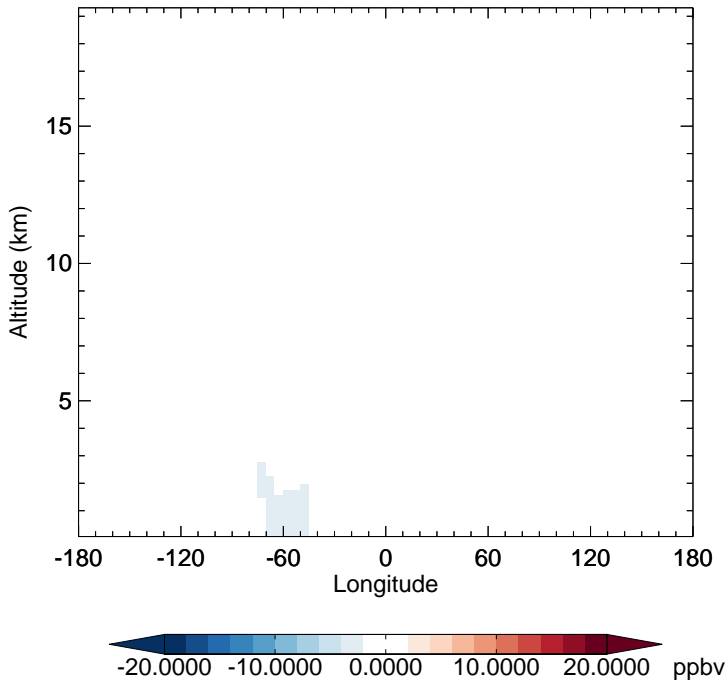
v11-02d - v11-02c CO - Diff along 15S for Jan
