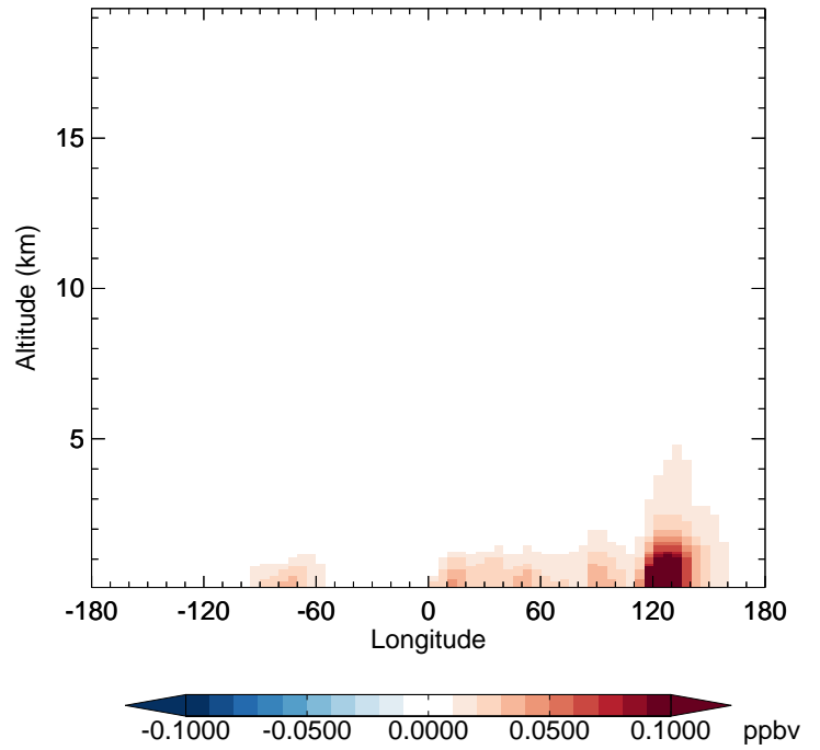
v11-02d - v11-02a SOAGX - Diff along 42N for Jan
