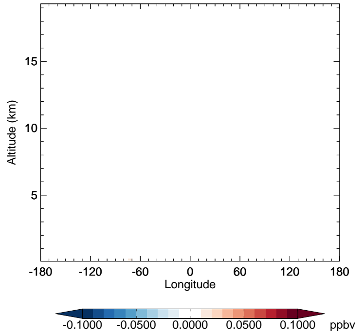
v11-02d - v11-02c INDIOL - Diff along 42N for Jan
