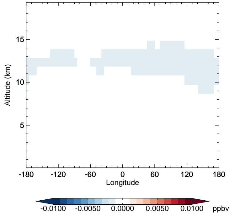
v11-02d - v11-02c HBr - Diff along 42N for Jan
