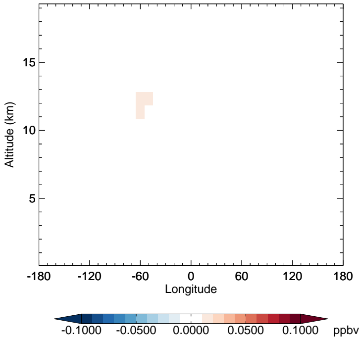
v11-02d - v11-02a ISOA3 - Diff along 15S for Jan
