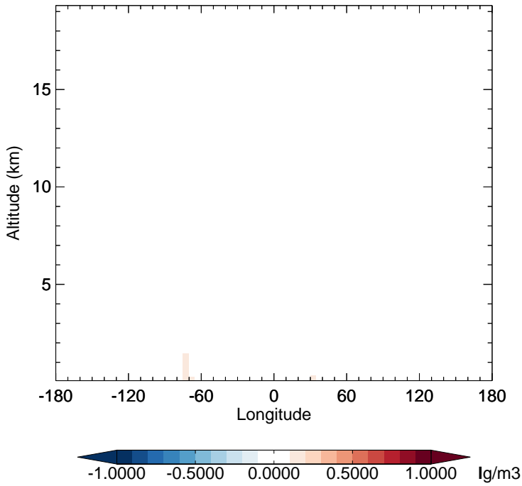
v11-02d - v11-02a SO 2 - Diff along 15S for Jan
