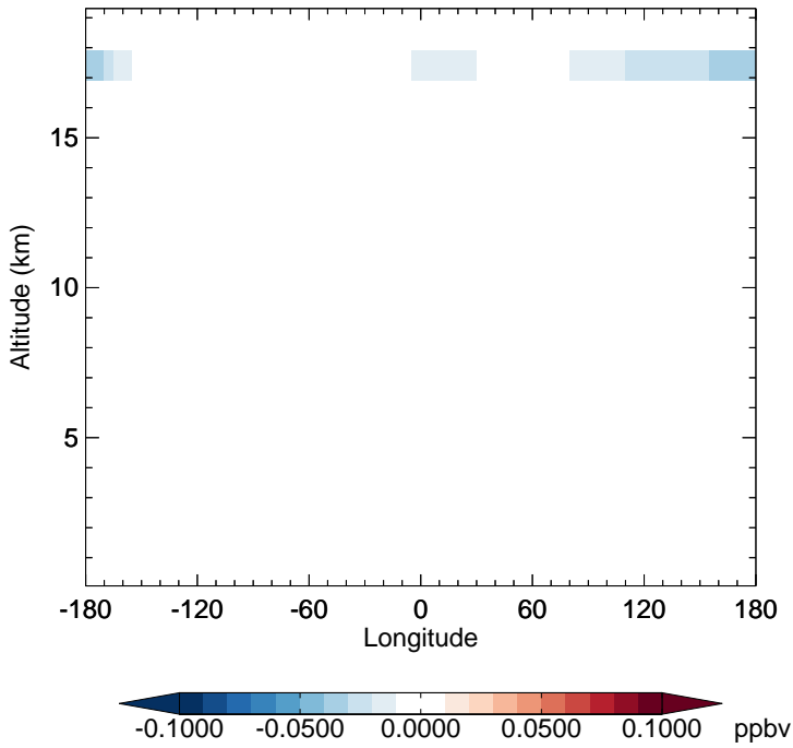
v11-02d - v11-02a HOCl - Diff along 15S for Jan
