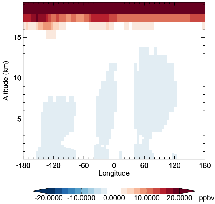
v11-02d - v11-02c O3 - Diff along 15S for Jan
