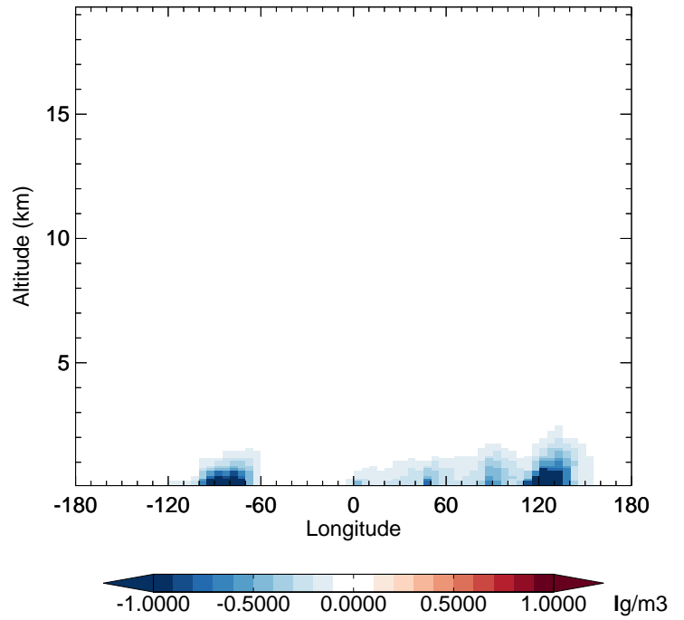
v11-02d - v11-02a NIT - Diff along 42N for Jan
