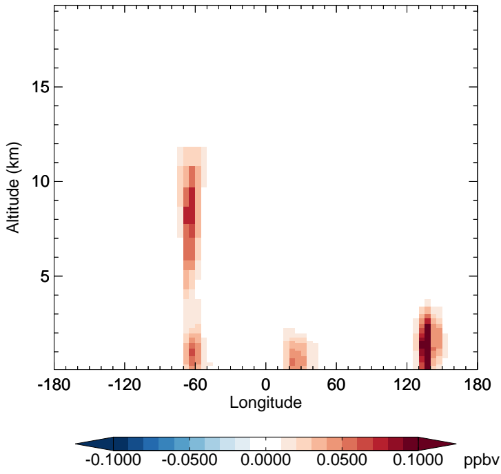
v11-02d - v11-02c IEPOXA - Diff along 15S for Jan
