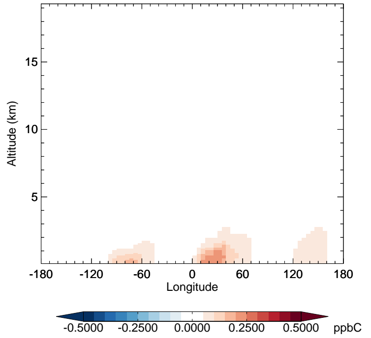
v11-02d - v11-02c ACET - Diff along 42N for Jan
