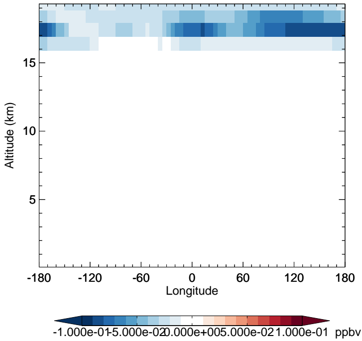
v11-02d - v11-02a CINO3 - Diff along 15S for Jan
