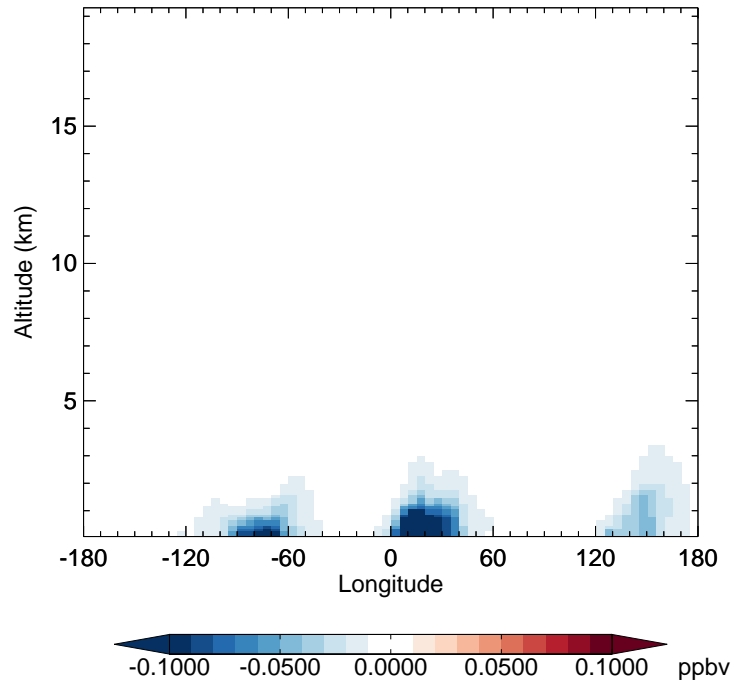
v11-02d - v11-02c XYLE - Diff along 42N for Jan
