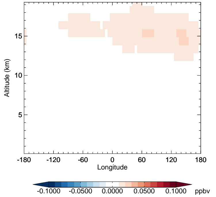
v11-02d - v11-02c MPN - Diff along 42N for Jan
