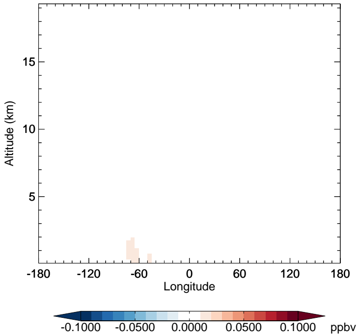
v11-02d - v11-02a TOLU - Diff along 15S for Jan
