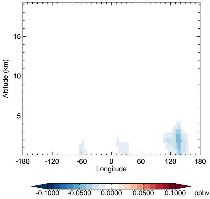
v11-02d - v11-02c INDIOL - Diff along 15S for Jan
