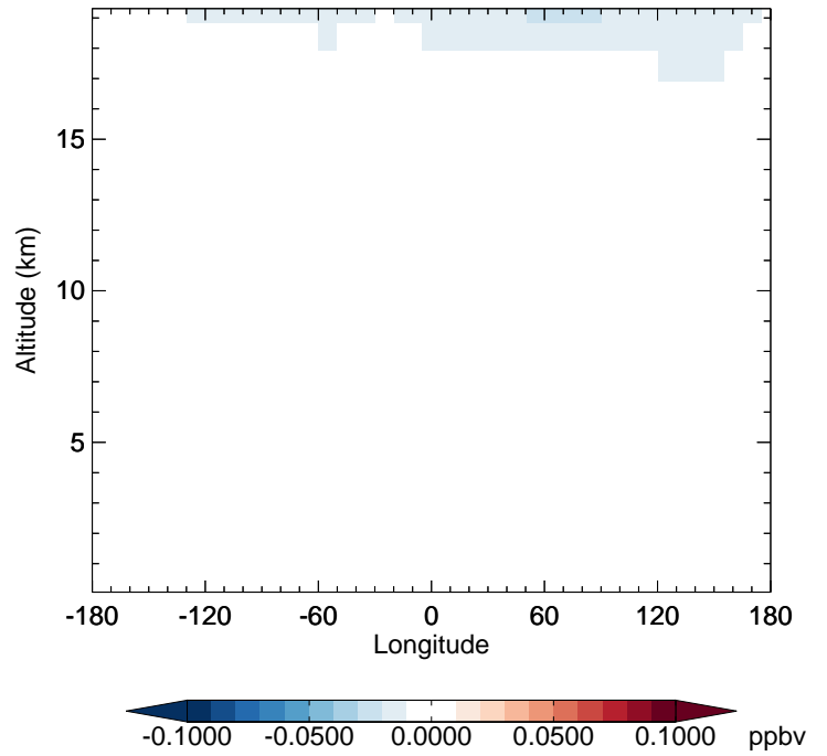
v11-02d - v11-02a HOCl - Diff along 42N for Jan
