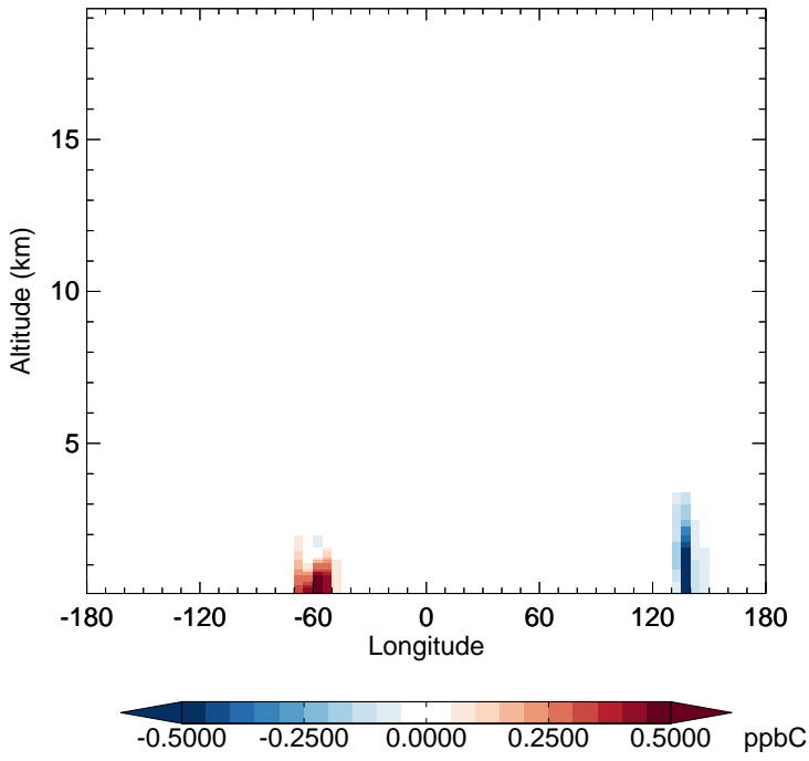
v11-02d - v11-02c ISOP - Diff along 15S for Jan
