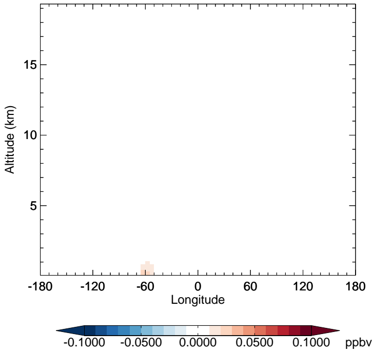
v11-02d - v11-02c MTPA - Diff along 15S for Jan
