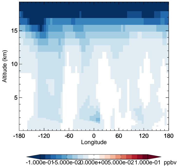
v11-02d - v11-02c HCl - Diff along 15S for Jan
