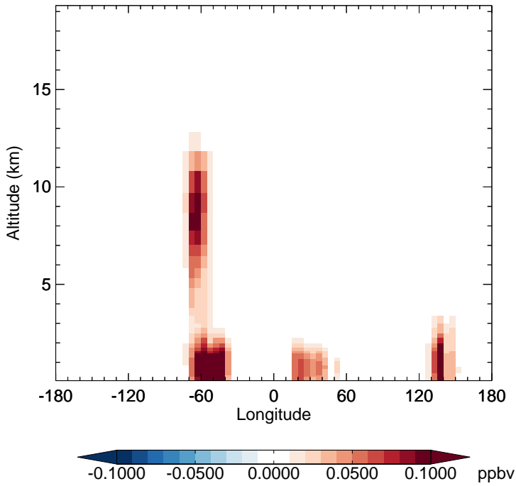
v11-02d - v11-02a IEPOXB - Diff along 15S for Jan
