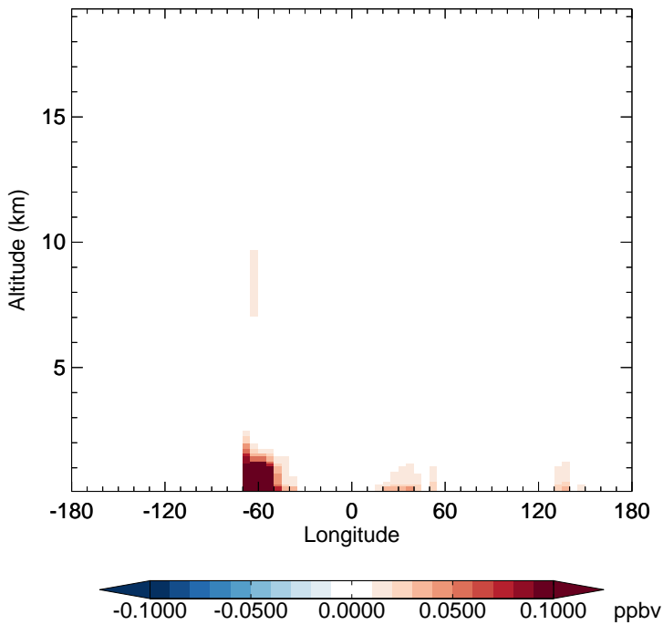
v11-02d - v11-02a MTPA - Diff along 15S for Jan
