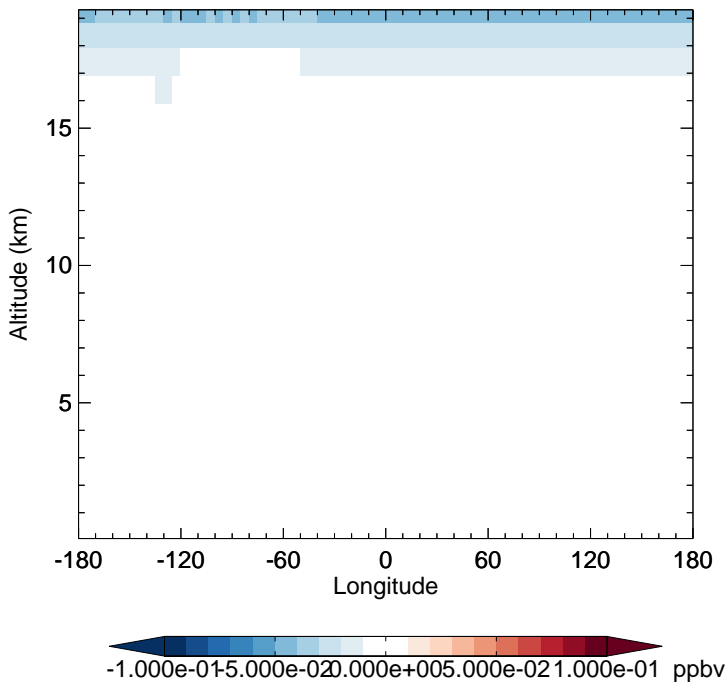
v11-02d - v11-02a N2O - Diff along 15S for Jan
