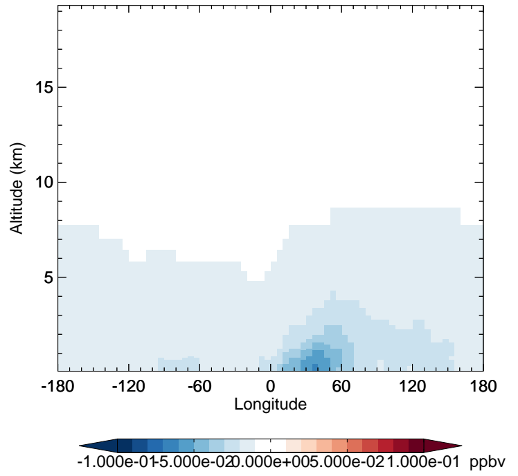
v11-02d - v11-02c BENZ - Diff along 42N for Jan
