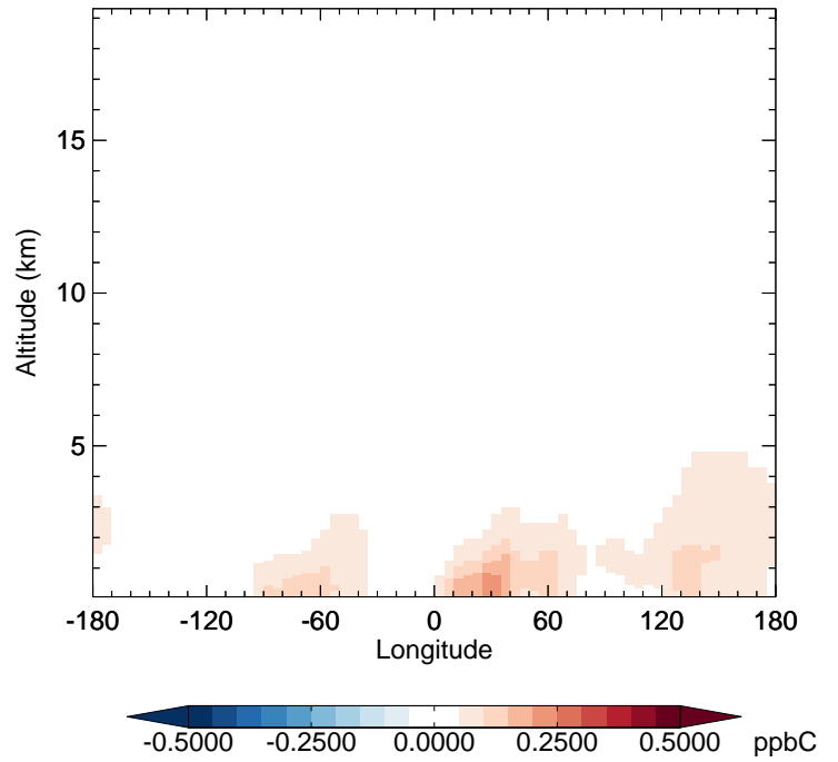
v11-02d - v11-02a ACET - Diff along 42N for Jan
