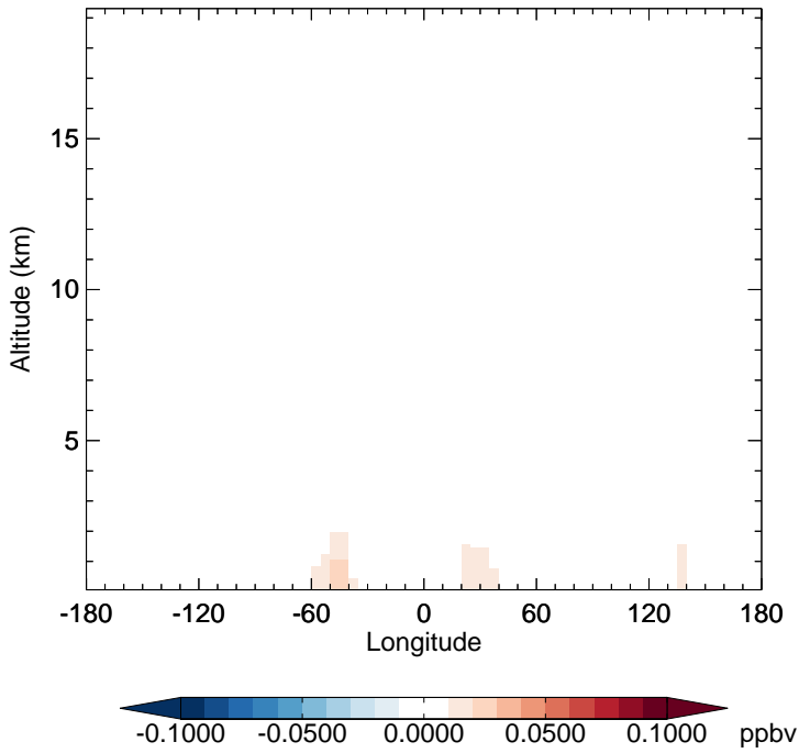
v11-02d - v11-02a MONITA - Diff along 15S for Jan
