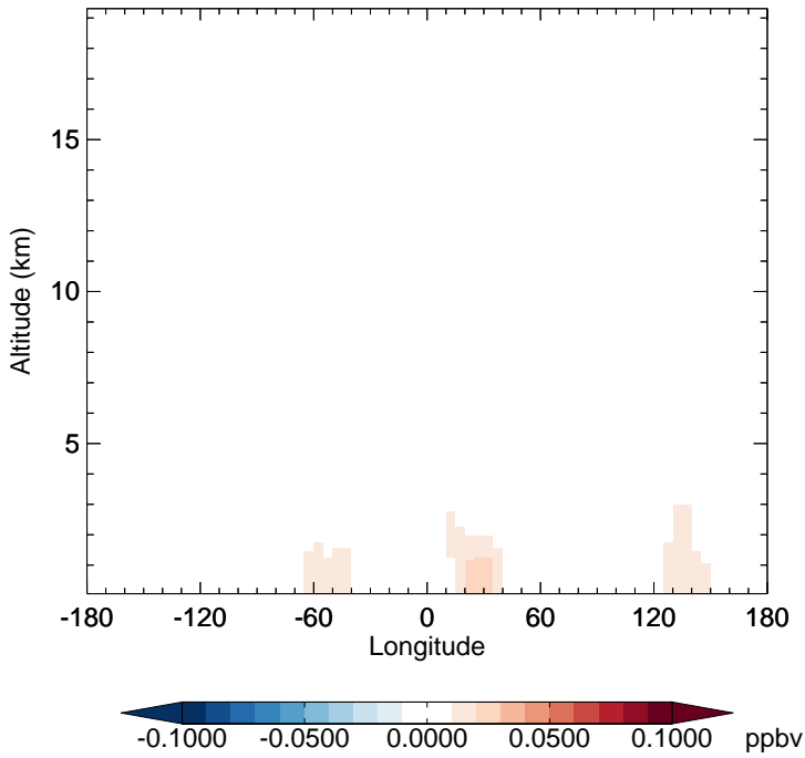
v11-02d - v11-02a SOAGX - Diff along 15S for Jan
