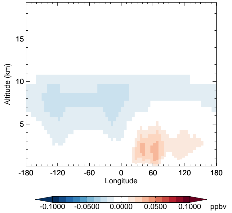
v11-02d - v11-02c H2O2 - Diff along 42N for Jan
