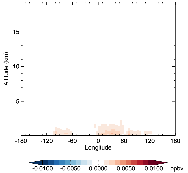
v11-02d - v11-02a NO3 - Diff along 42N for Jan
