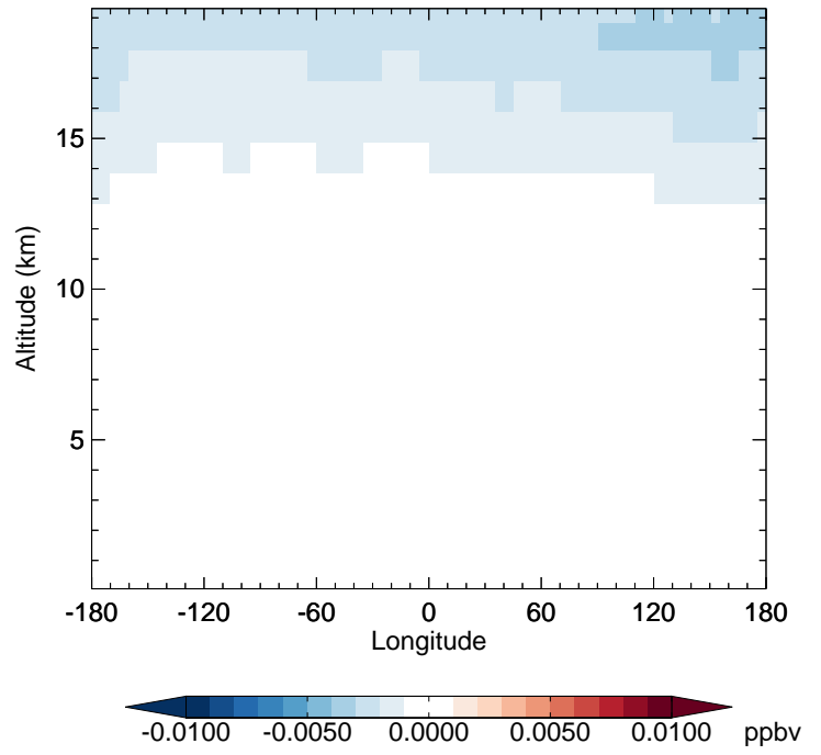
v11-02d - v11-02c BrNO3 - Diff along 42N for Jan
