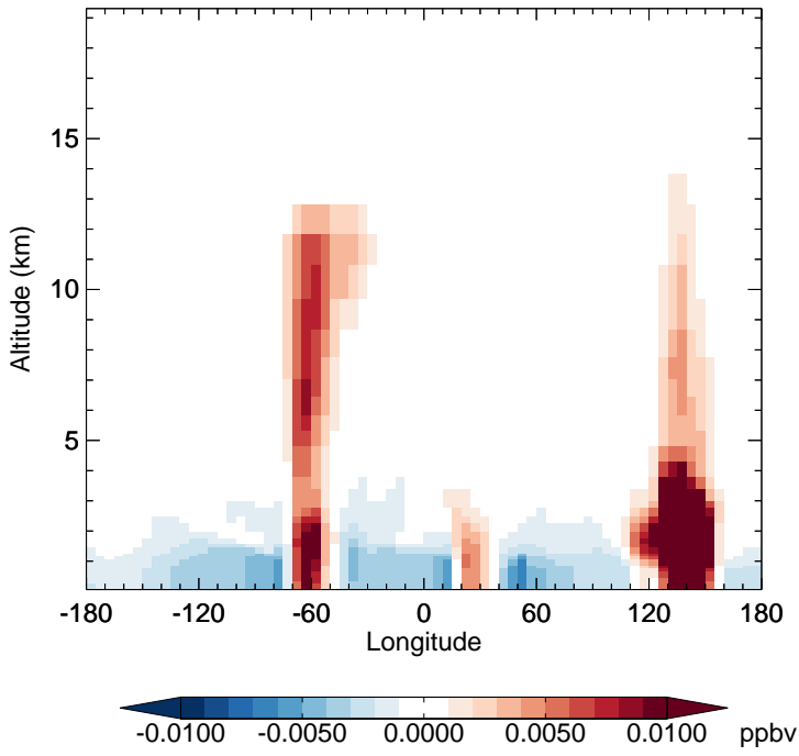
v11-02d - v11-02c MAP - Diff along 15S for Jan
