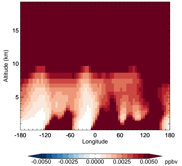
v11-02d - v11-02a N2O5 - Diff along 42N for Jan
