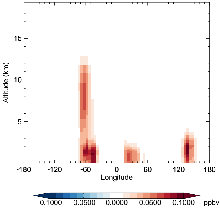
v11-02d - v11-02a HC187 - Diff along 15S for Jan
