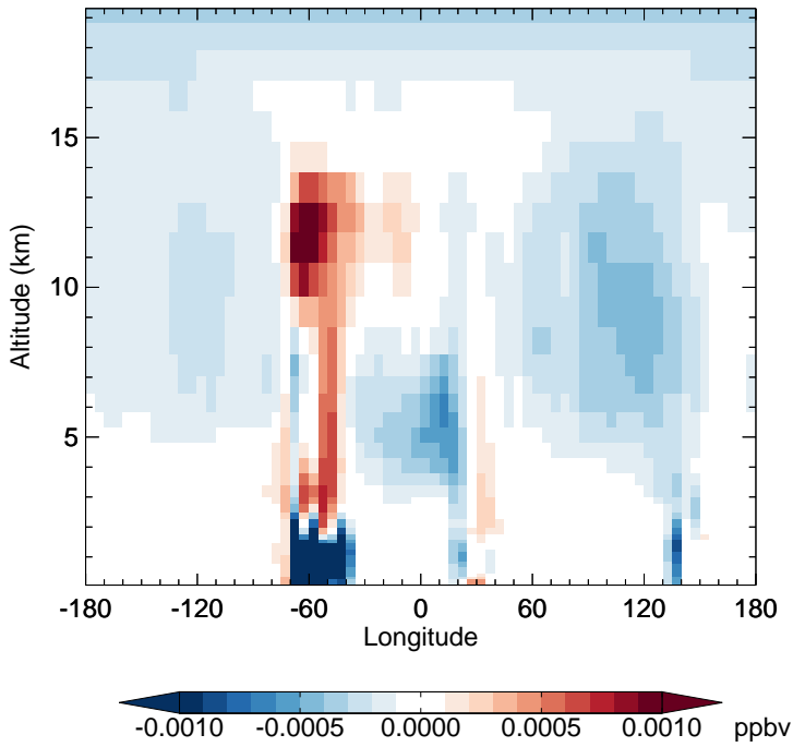
v11-02d - v11-02a PPN - Diff along 15S for Jan
