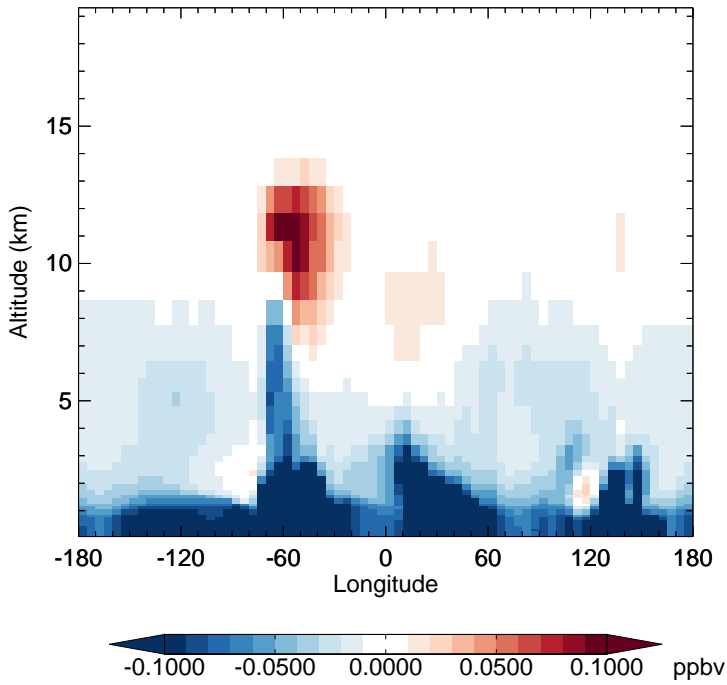
v11-02d - v11-02a H2O2 - Diff along 15S for Jan
