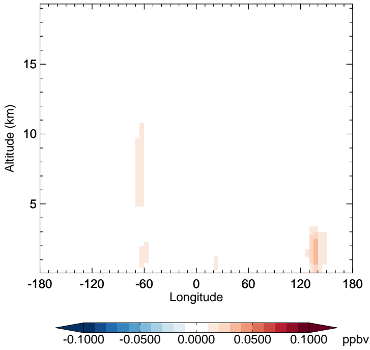
v11-02d - v11-02c HC187 - Diff along 15S for Jan
