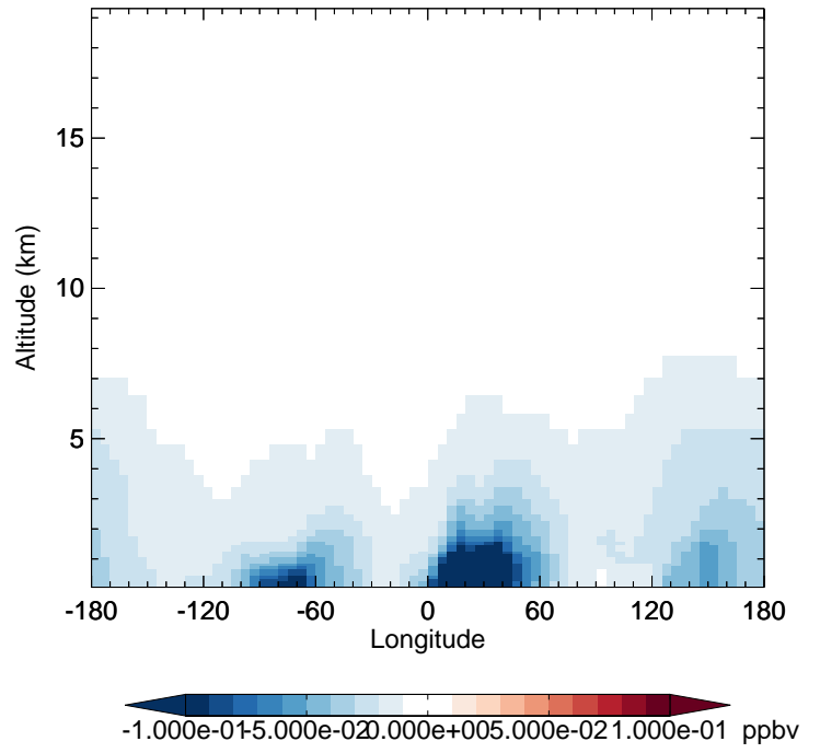
v11-02d - v11-02c TOLU - Diff along 42N for Jan
