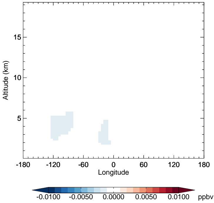
v11-02d - v11-02c HBr - Diff along 15S for Jan
