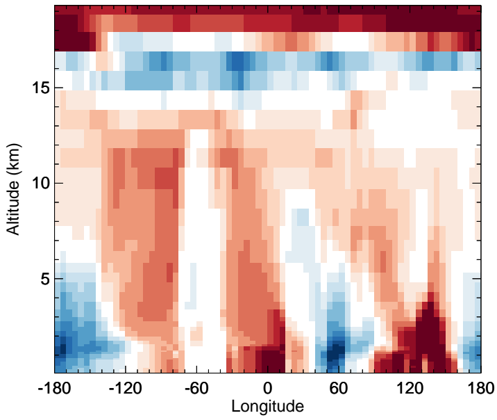
v11-02d - v11-02c OH - Diff along 15S for Jan
