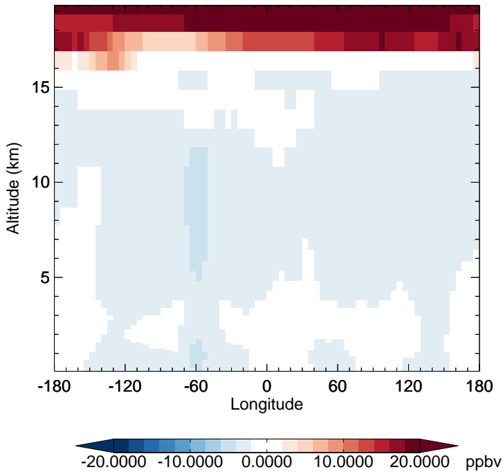
v11-02d - v11-02a O3 - Diff along 15S for Jan
