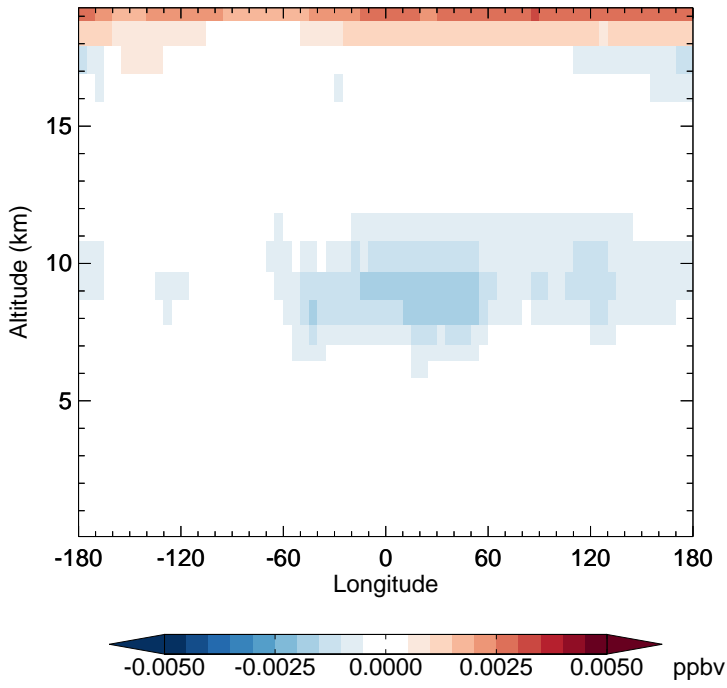
v11-02d - v11-02c HNO 4 - Diff along 15S for Jan
