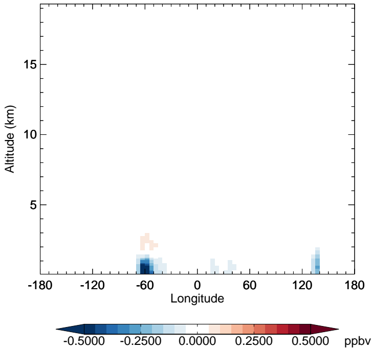
v11-02d - v11-02a CH 2 O - Diff along 15S for Jan
