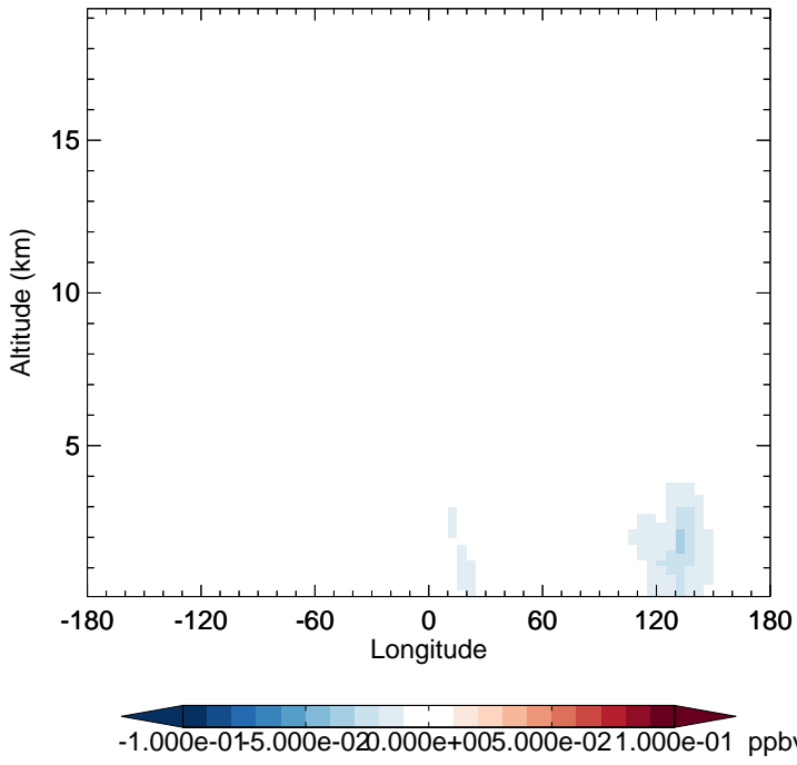
v11-02d - v11-02c SOAME - Diff along 15S for Jan
