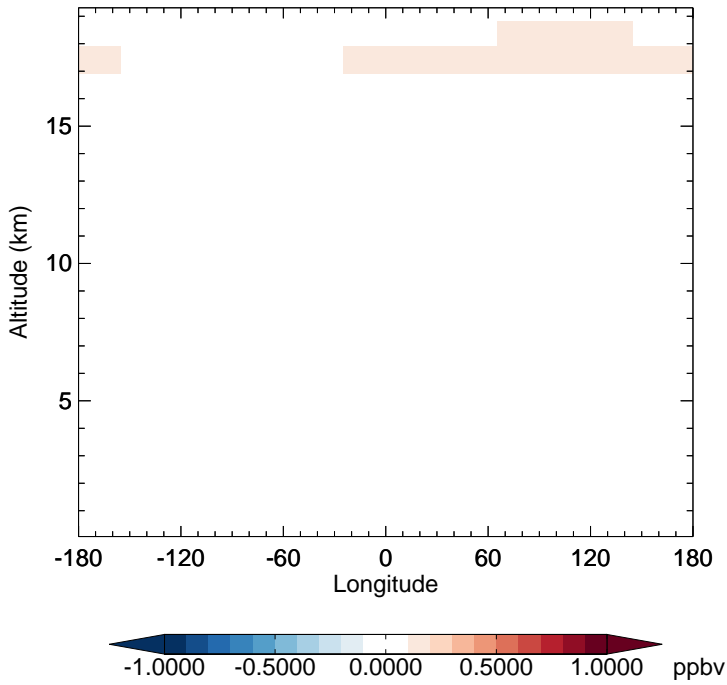
v11-02d - v11-02a NO - Diff along 15S for Jan
