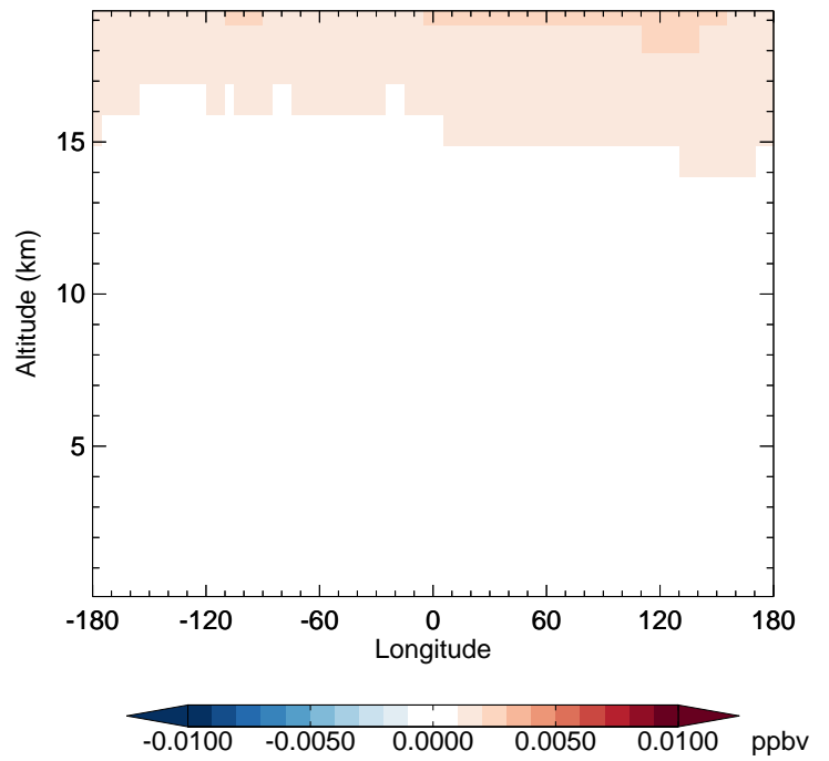
v11-02d - v11-02a BrNO3 - Diff along 42N for Jan
