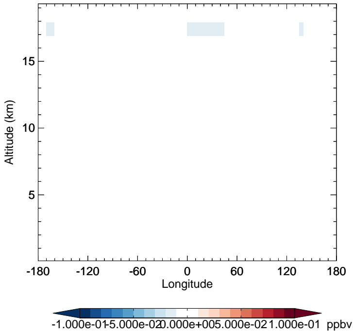
v11-02d - v11-02a Cl2 - Diff along 15S for Jan
