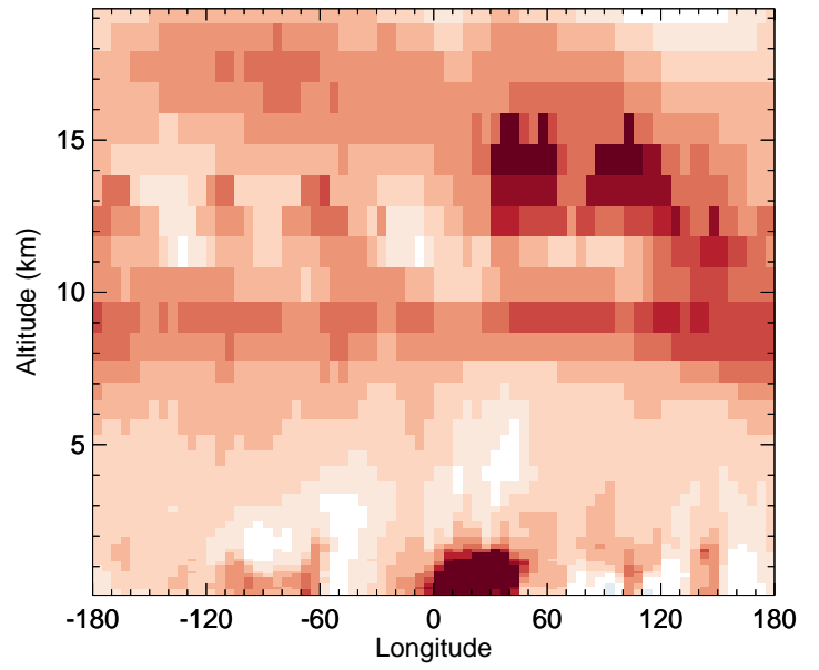
v11-02d - v11-02c OH - Diff along 42N for Jan
