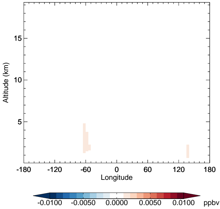
v11-02d - v11-02c R4N2 - Diff along 15S for Jan
