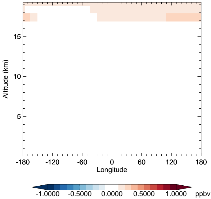
v11-02d - v11-02a NO 2 - Diff along 15S for Jan
