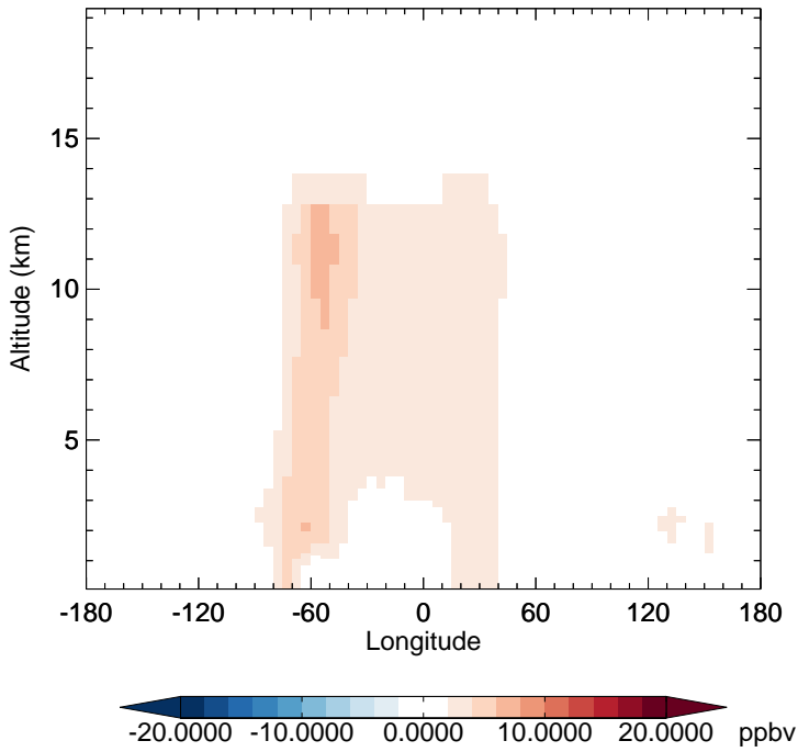
v11-02d - v11-02a CO - Diff along 15S for Jan
