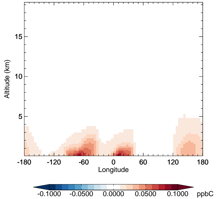
v11-02d - v11-02a MEK - Diff along 42N for Jan
