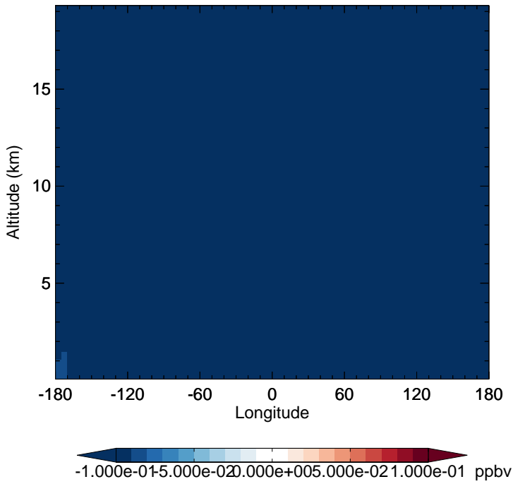
v11-02d - v11-02a EOH - Diff along 15S for Jan
