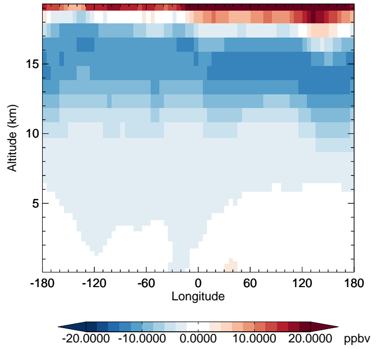
v11-02d - v11-02c O3 - Diff along 42N for Jan
