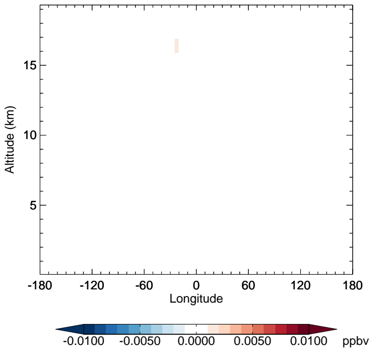
v11-02d - v11-02a BrNO3 - Diff along 15S for Jan
