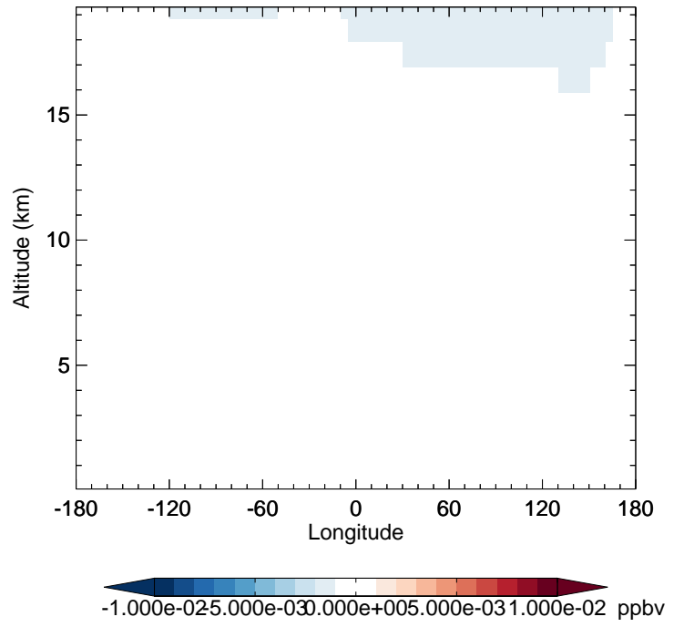
v11-02d - v11-02c BrO - Diff along 42N for Jan
