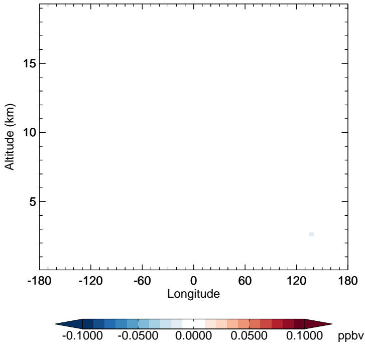
v11-02d - v11-02c GLYC - Diff along 15S for Jan
