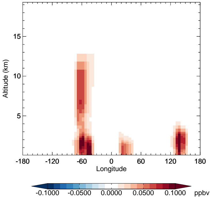
v11-02d - v11-02a IMAE - Diff along 15S for Jan
