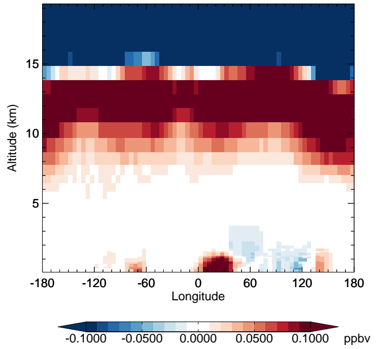
v11-02d - v11-02c HNO 3 - Diff along 42N for Jan
