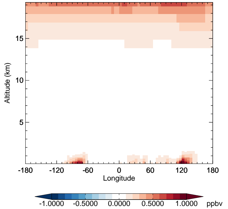
v11-02d - v11-02a NO 2 - Diff along 42N for Jan
