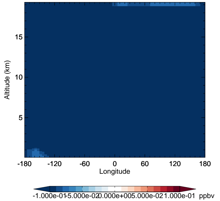
v11-02d - v11-02a EOH - Diff along 42N for Jan
