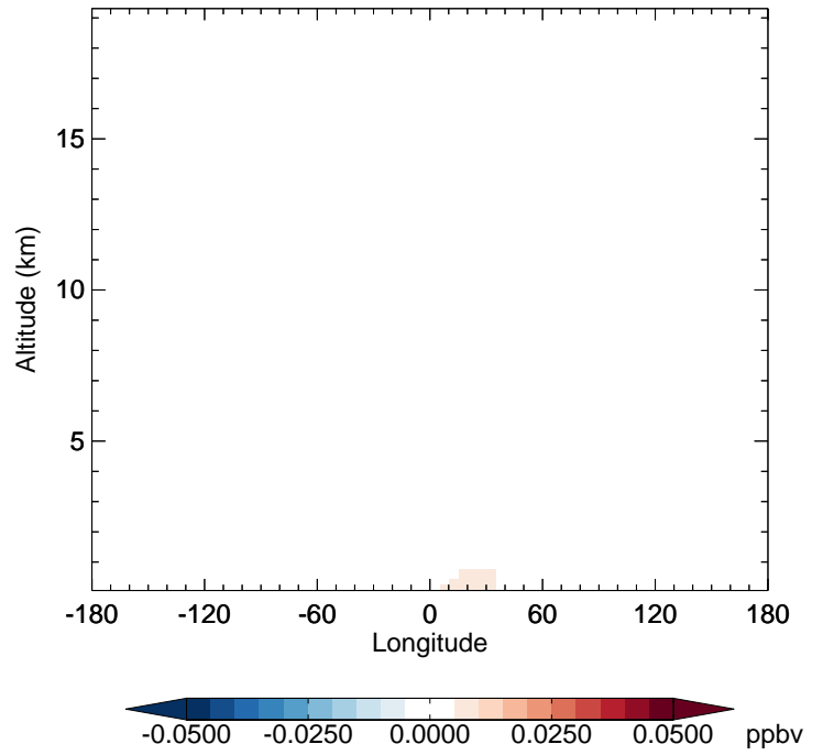
v11-02d - v11-02c RCHO - Diff along 42N for Jan
