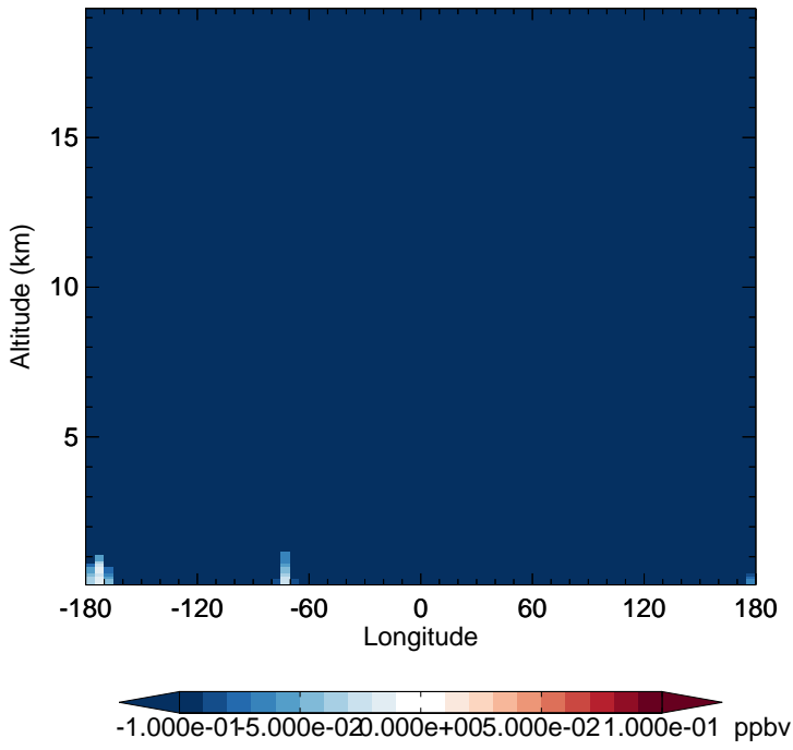
v11-02d - v11-02c CH4 - Diff along 15S for Jan
