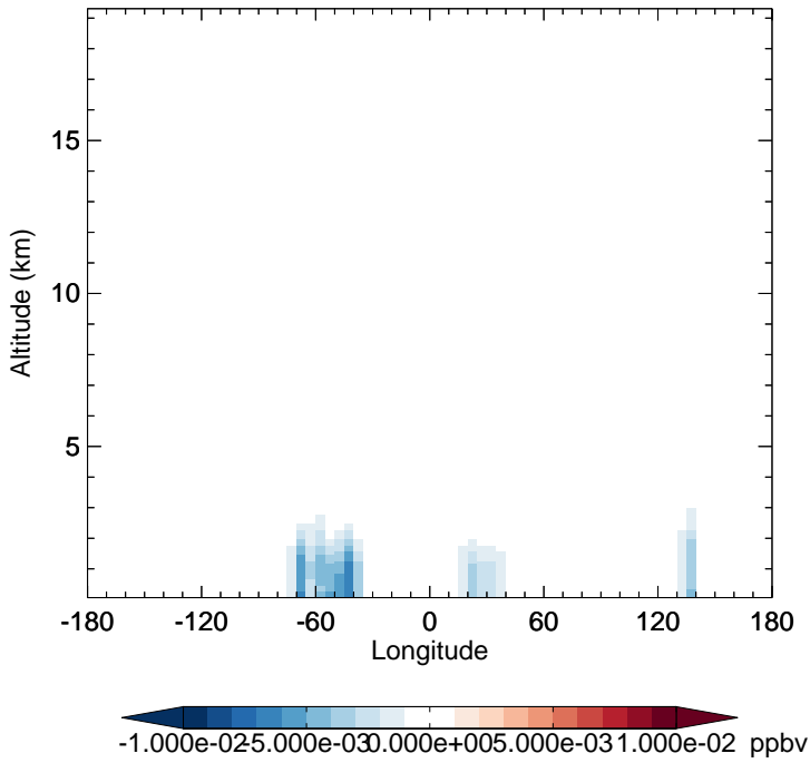
v11-02d - v11-02a NPMN - Diff along 15S for Jan
