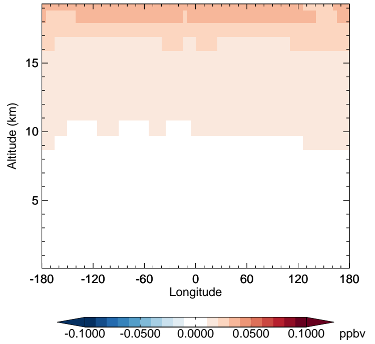
v11-02d - v11-02c CFC11 - Diff along 42N for Jan
