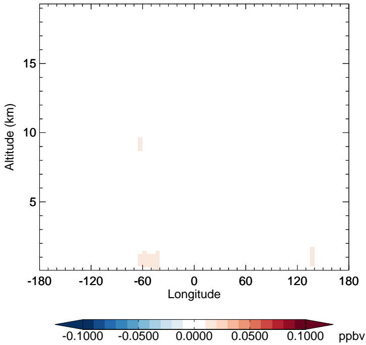
v11-02d - v11-02a IEPOXD - Diff along 15S for Jan
