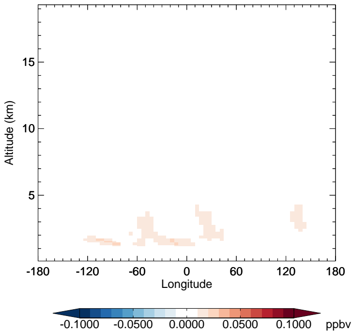
v11-02d - v11-02a CH3Cl - Diff along 15S for Jan
