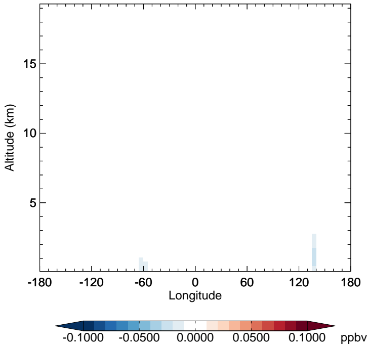
v11-02d - v11-02c HPALD - Diff along 15S for Jan
