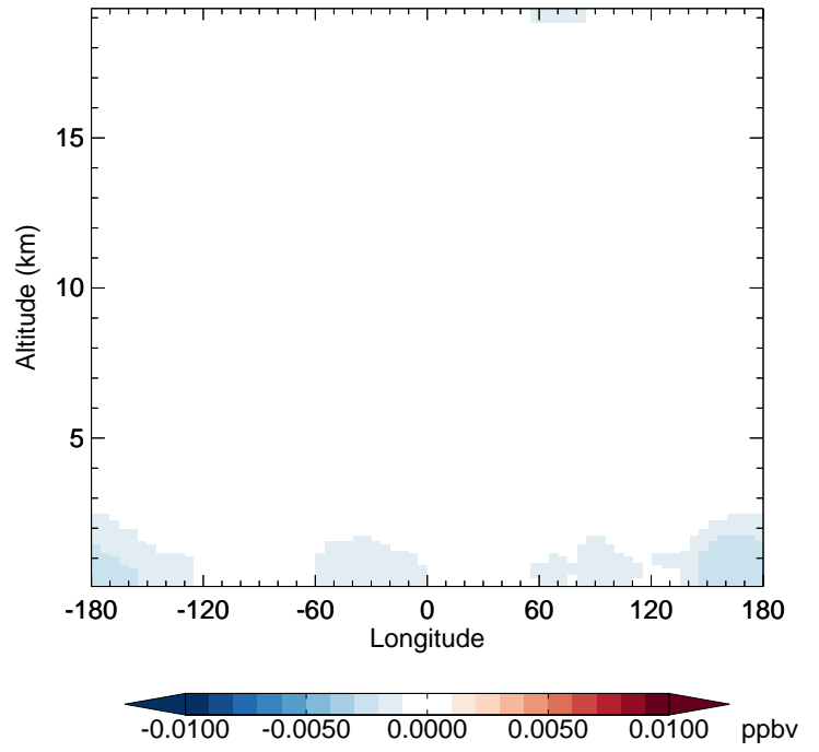
v11-02d - v11-02c HOBr - Diff along 42N for Jan
