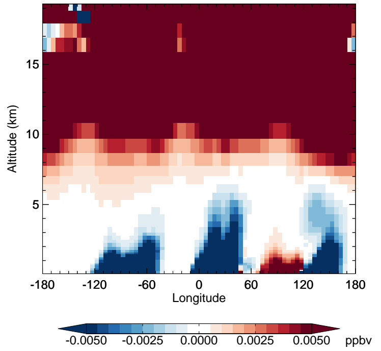
v11-02d - v11-02c N2O5 - Diff along 42N for Jan
