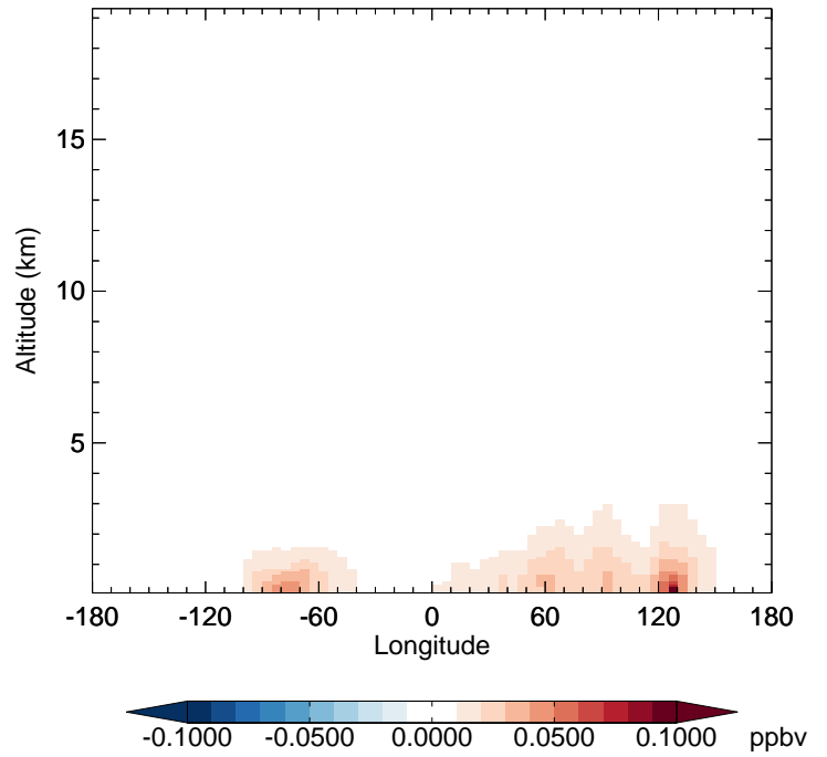
v11-02d - v11-02a INDIOL - Diff along 42N for Jan
