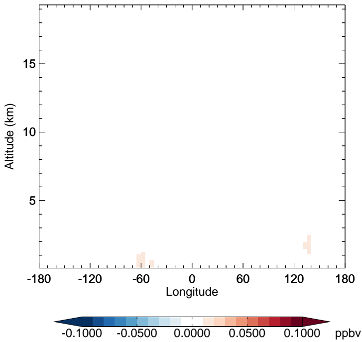
v11-02d - v11-02a LVOCOA - Diff along 15S for Jan
