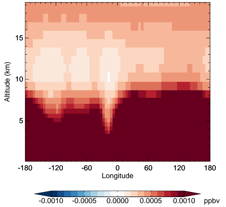
v11-02d - v11-02c PPN - Diff along 42N for Jan
