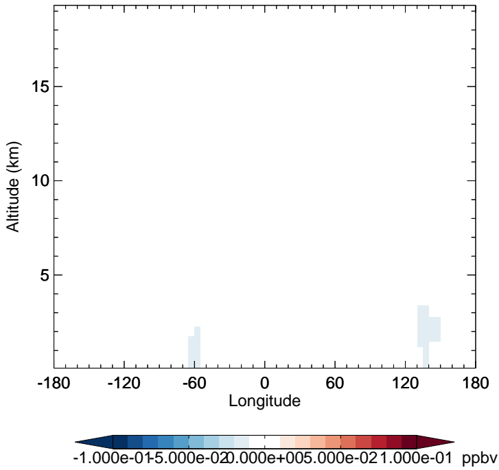
v11-02d - v11-02a PROPNN - Diff along 15S for Jan
