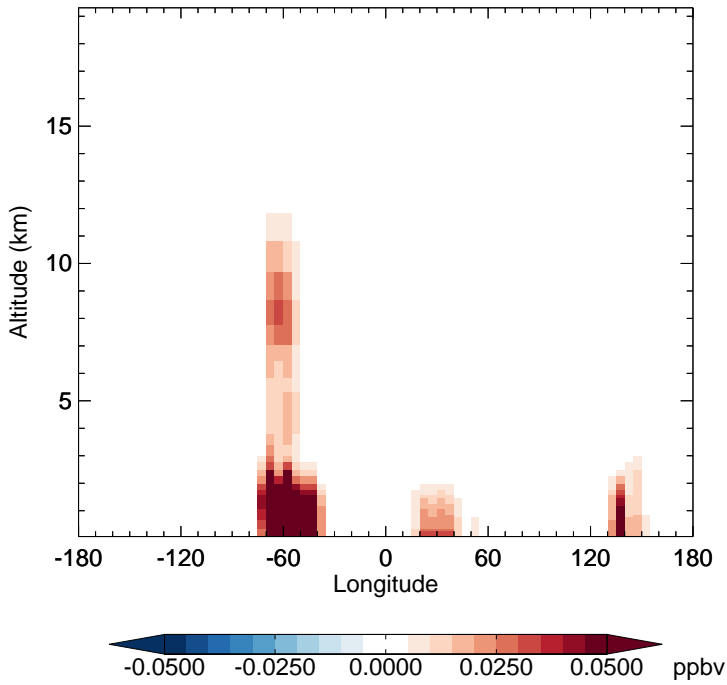
v11-02d - v11-02a MACR - Diff along 15S for Jan
