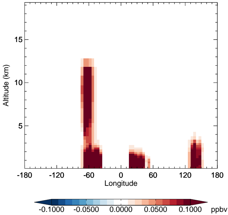
v11-02d - v11-02a IEPOXA - Diff along 15S for Jan
