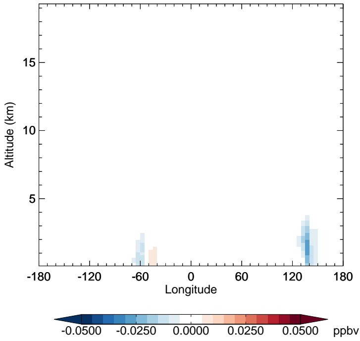
v11-02d - v11-02c MVK - Diff along 15S for Jan
