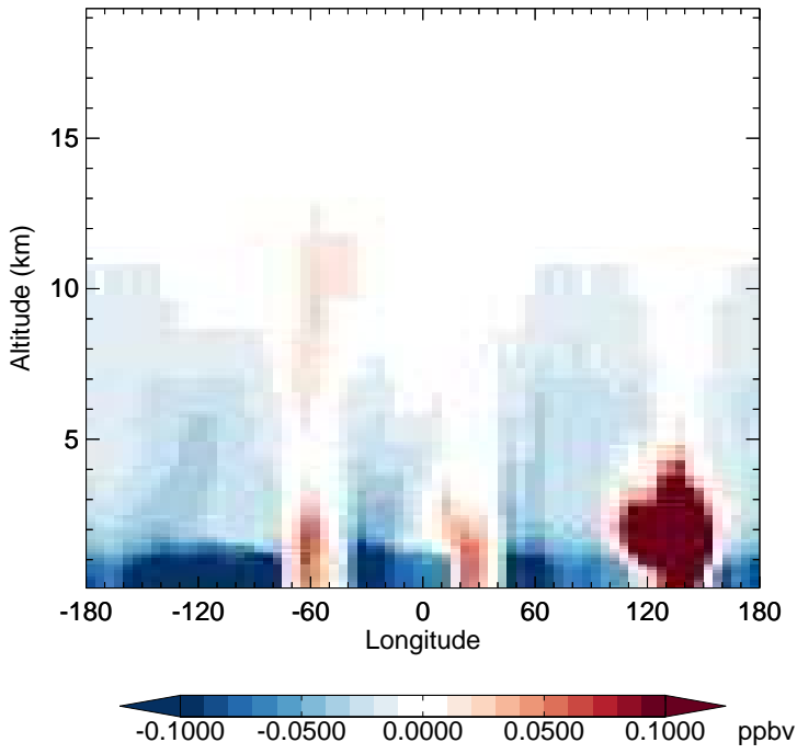
v11-02d - v11-02c H2O2 - Diff along 15S for Jan
