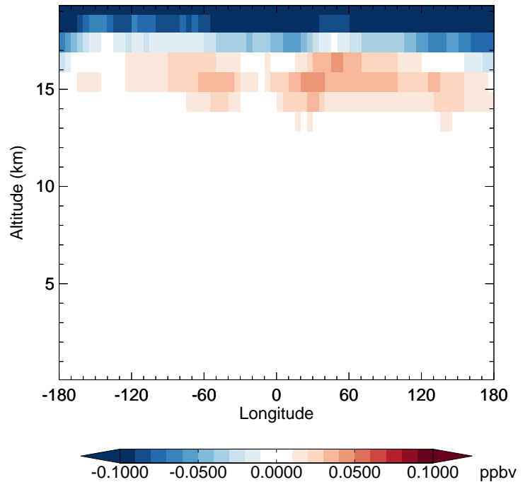
v11-02d - v11-02c CINO3 - Diff along 42N for Jan
