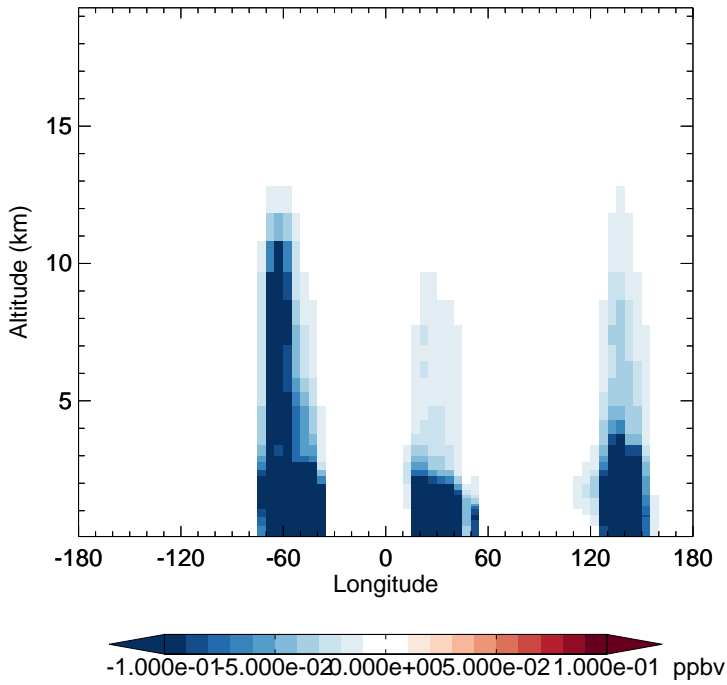
v11-02d - v11-02a HAC - Diff along 15S for Jan
