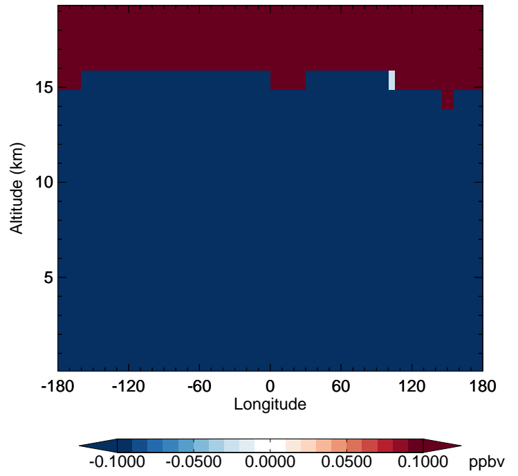
v11-02d - v11-02c CH4 - Diff along 42N for Jan
