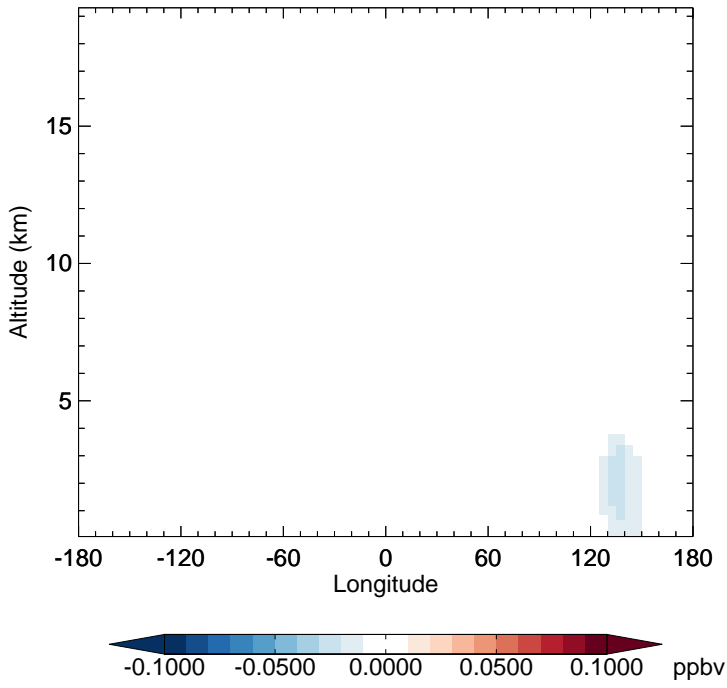
v11-02d - v11-02c EOH - Diff along 15S for Jan
