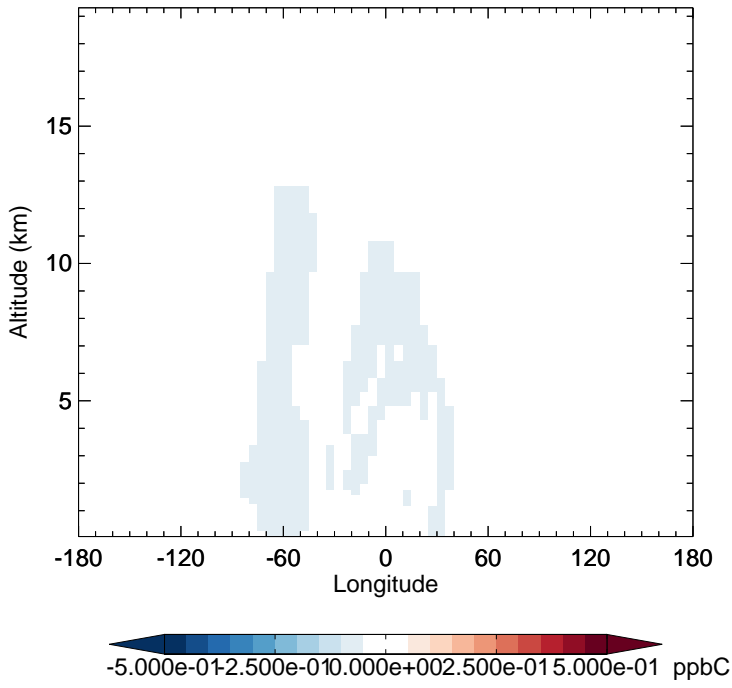
v11-02d - v11-02c ACET - Diff along 15S for Jan
