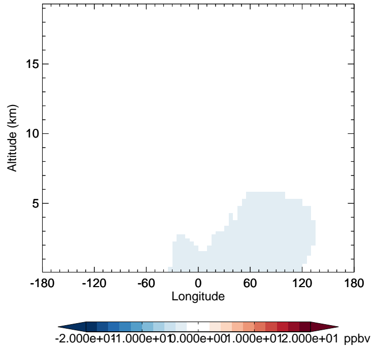
v11-02d - v11-02c CO - Diff along 42N for Jan
