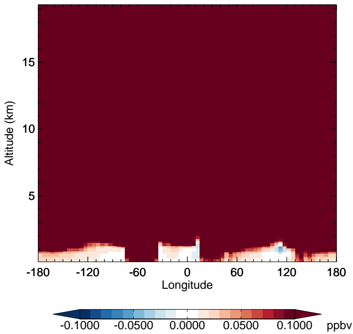
v11-02d - v11-02a CH4 - Diff along 15S for Jan
