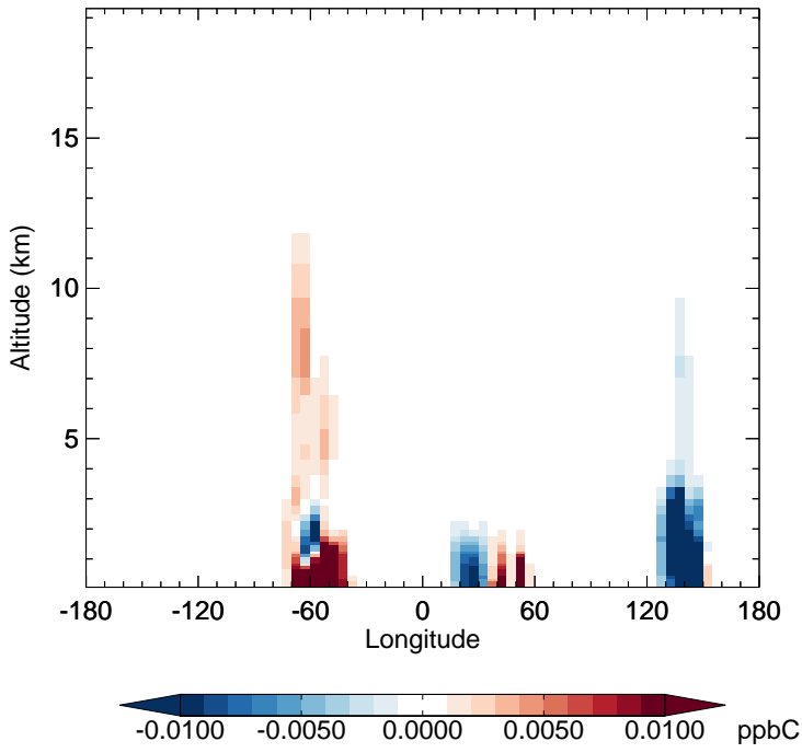
v11-02d - v11-02c PRPE - Diff along 15S for Jan
