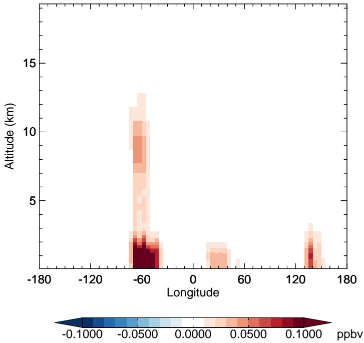
v11-02d - v11-02a IPMN - Diff along 15S for Jan
