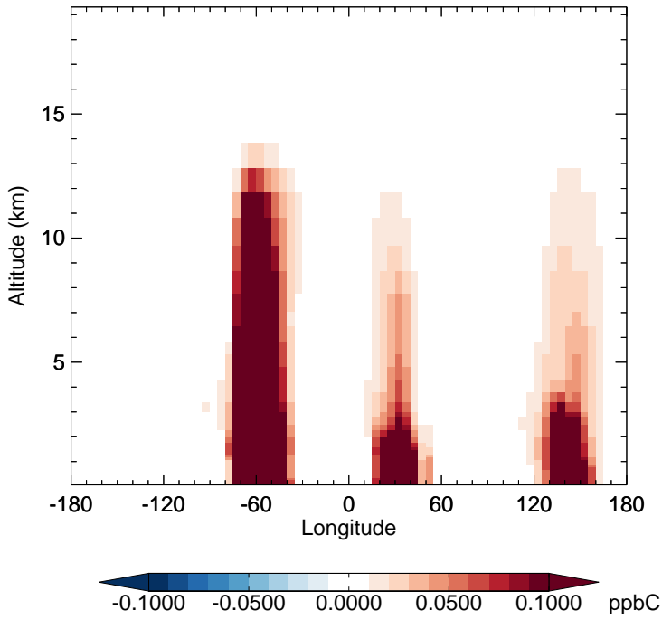
v11-02d - v11-02a MEK - Diff along 15S for Jan
