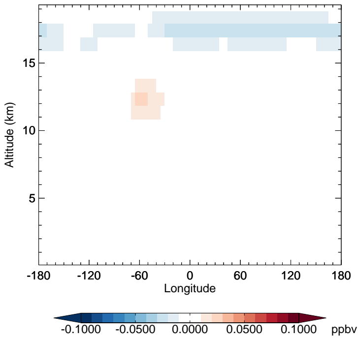
v11-02d - v11-02a MPN - Diff along 15S for Jan
