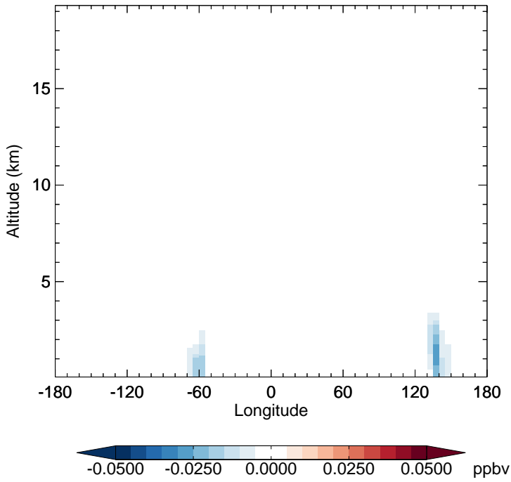
v11-02d - v11-02c MACR - Diff along 15S for Jan
