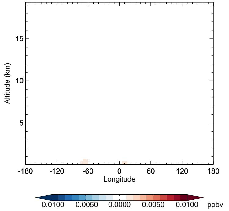
v11-02d - v11-02c R4N2 - Diff along 42N for Jan
