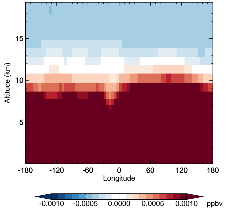
v11-02d - v11-02a PPN - Diff along 42N for Jan
