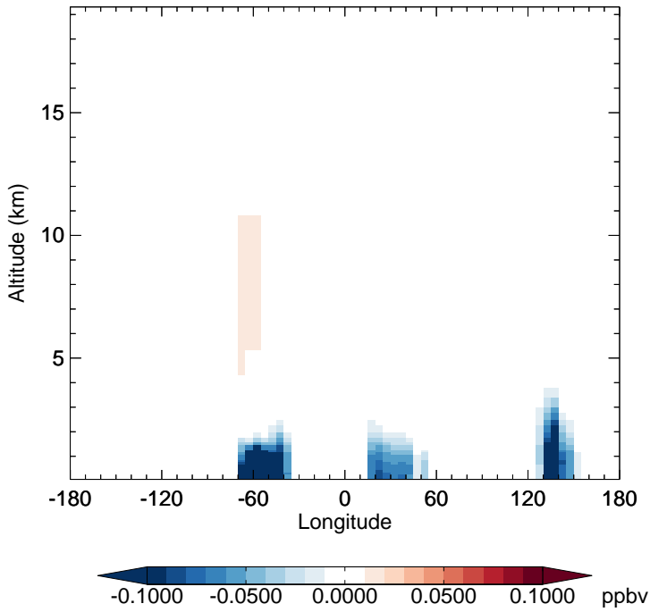
v11-02d - v11-02a GLYC - Diff along 15S for Jan
