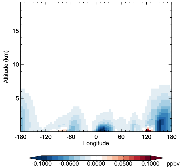
v11-02d - v11-02a XYLE - Diff along 42N for Jan
