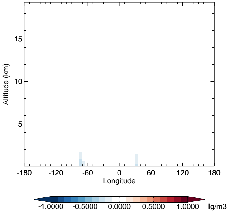
v11-02d - v11-02a SO4 - Diff along 15S for Jan
