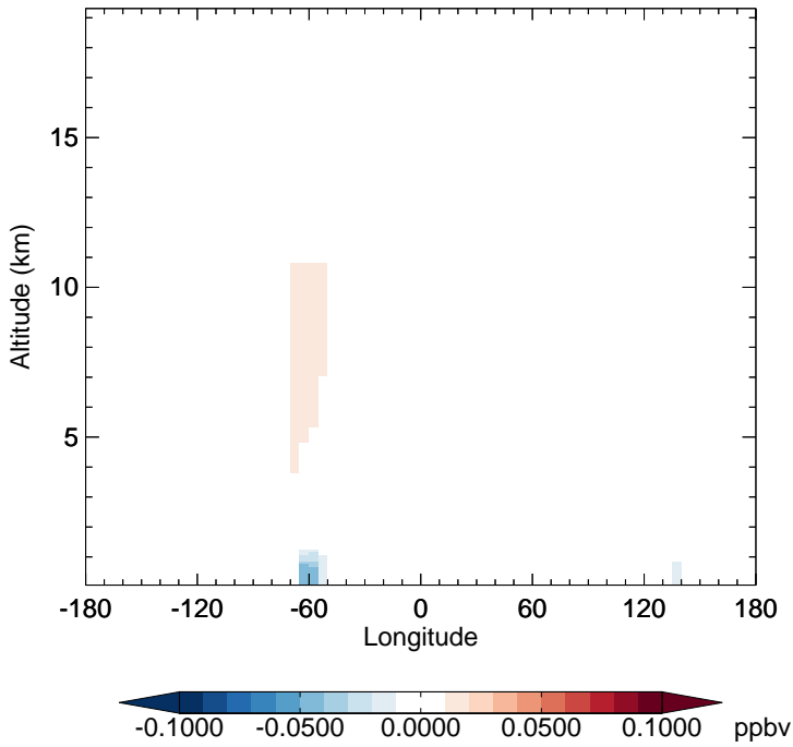
v11-02d - v11-02a ISO3 - Diff along 15S for Jan
