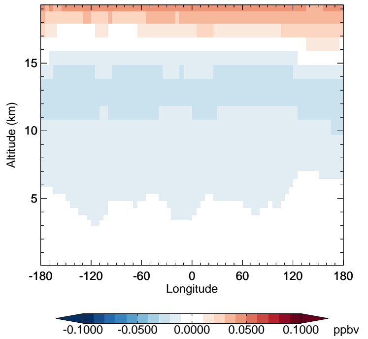
v11-02d - v11-02c CH3Cl - Diff along 42N for Jan
