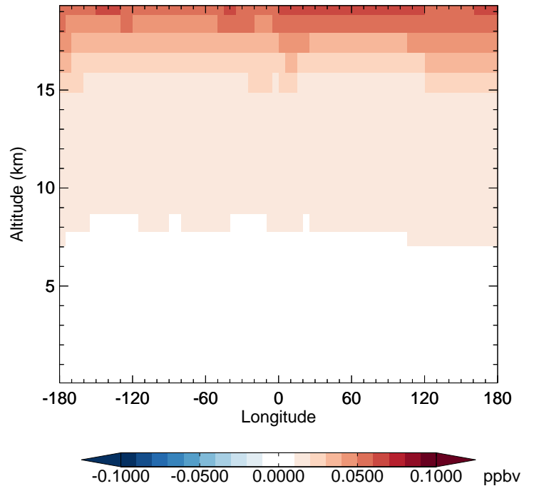
v11-02d - v11-02c CFC12 - Diff along 42N for Jan
