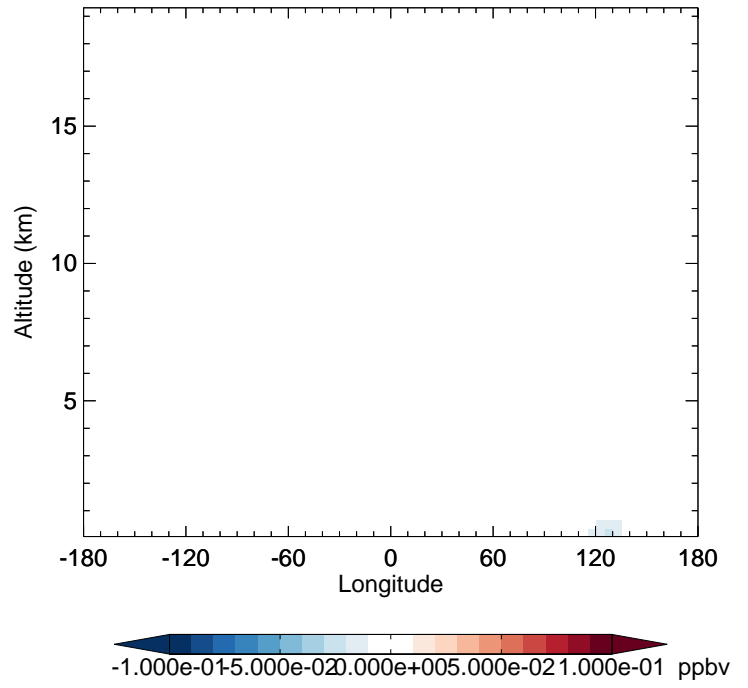
v11-02d - v11-02c SOAGX - Diff along 42N for Jan
