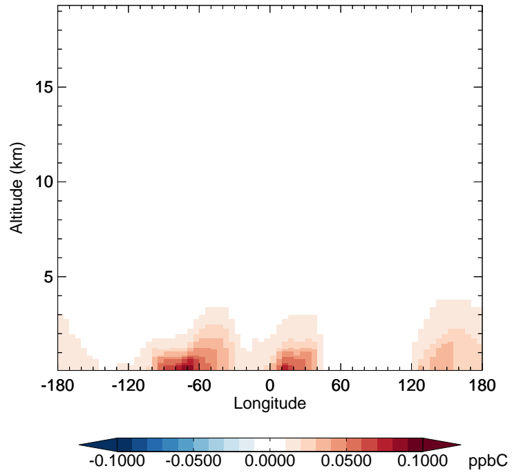
v11-02d - v11-02c MEK - Diff along 42N for Jan
