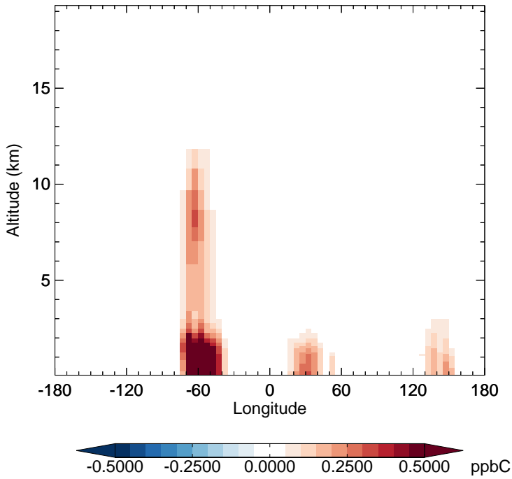
v11-02d - v11-02a ALD2 - Diff along 15S for Jan
