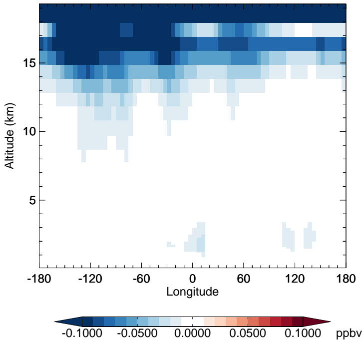
v11-02d - v11-02a HCl - Diff along 15S for Jan
