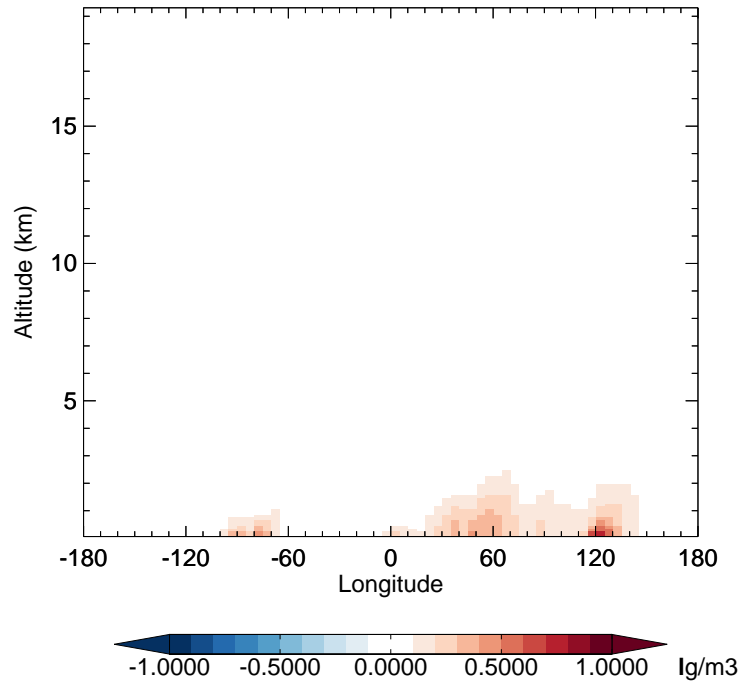
v11-02d - v11-02a SO4 - Diff along 42N for Jan
