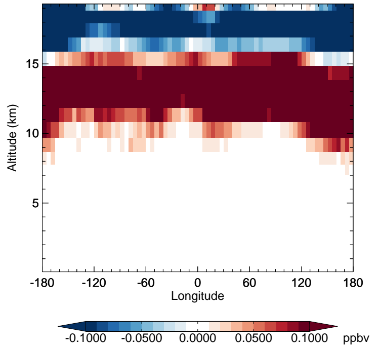
v11-02d - v11-02a H2O - Diff along 42N for Jan
