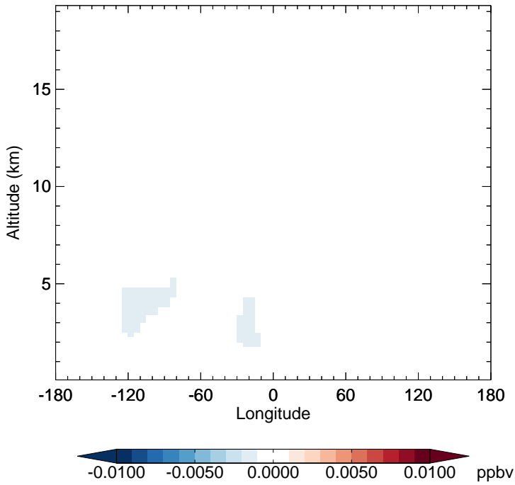
v11-02d - v11-02a HBr - Diff along 15S for Jan
