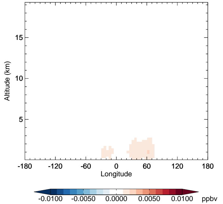
v11-02d - v11-02a MAP - Diff along 42N for Jan
