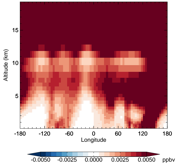
v11-02d - v11-02a HNO 4 - Diff along 42N for Jan
