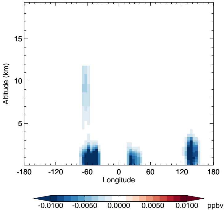
v11-02d - v11-02a MVKN - Diff along 15S for Jan
