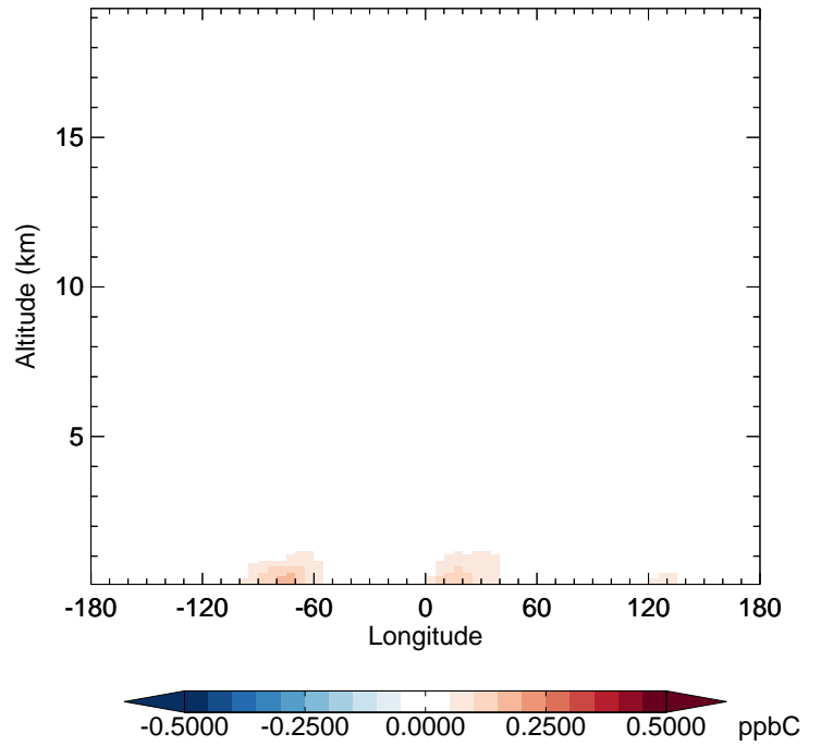
v11-02d - v11-02a ALD2 - Diff along 42N for Jan
