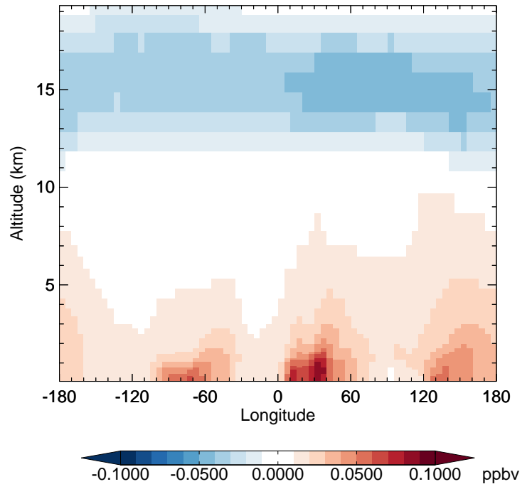
v11-02d - v11-02c PAN - Diff along 42N for Jan
