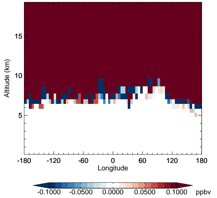
v11-02d - v11-02c H2O - Diff along 42N for Jan
