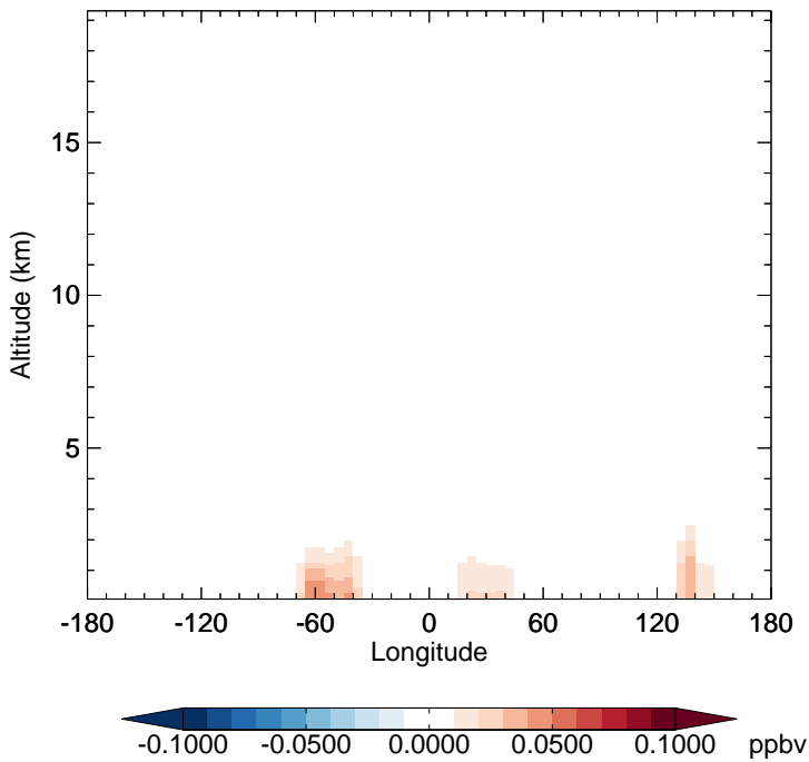
v11-02d - v11-02a GLYX - Diff along 15S for Jan
