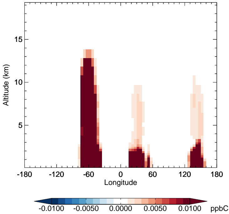
v11-02d - v11-02a PRPE - Diff along 15S for Jan
