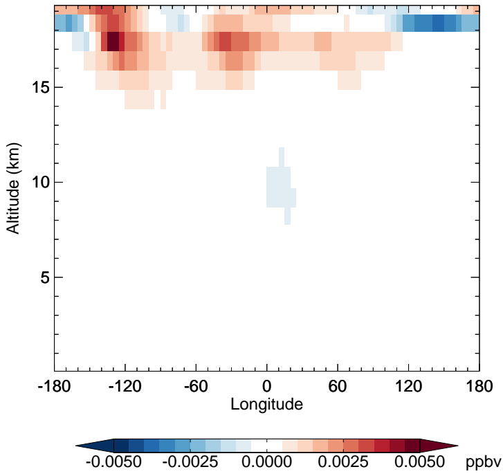
v11-02d - v11-02c N2O5 - Diff along 15S for Jan
