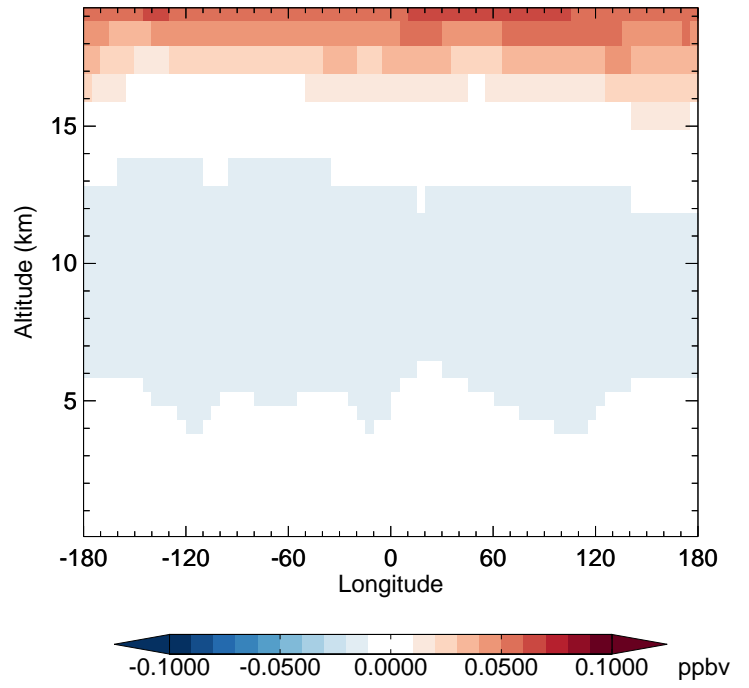
v11-02d - v11-02c OCS - Diff along 42N for Jan
