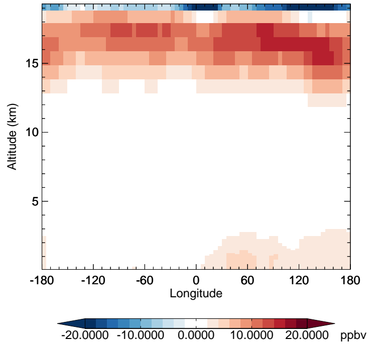
v11-02d - v11-02a O3 - Diff along 42N for Jan
