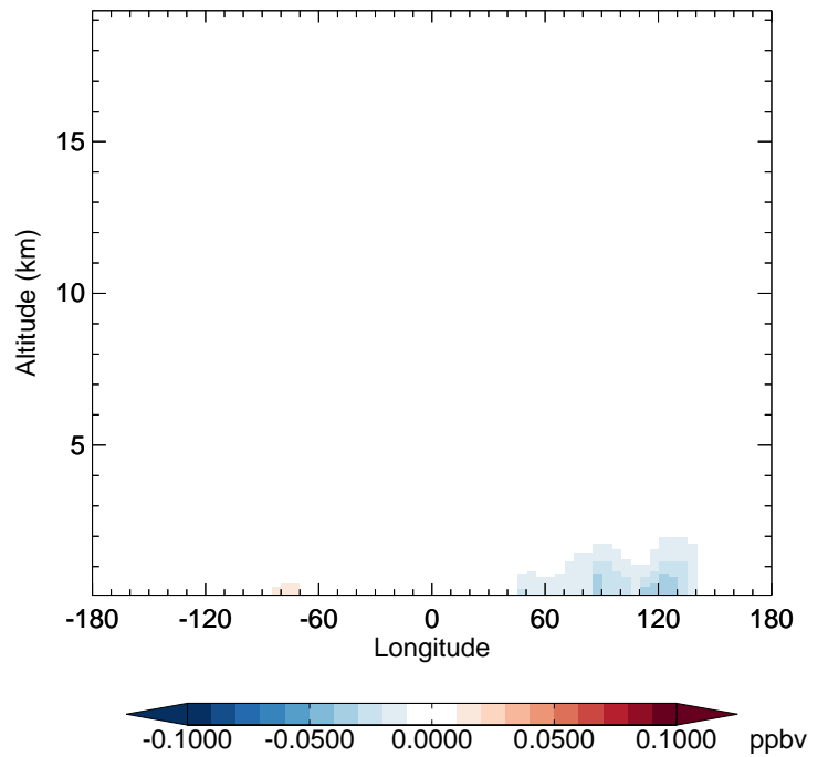
v11-02d - v11-02a MGLY - Diff along 42N for Jan
