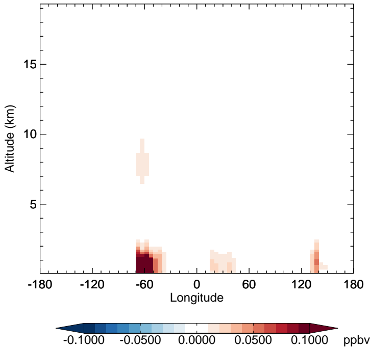
v11-02d - v11-02a RIPB - Diff along 15S for Jan
