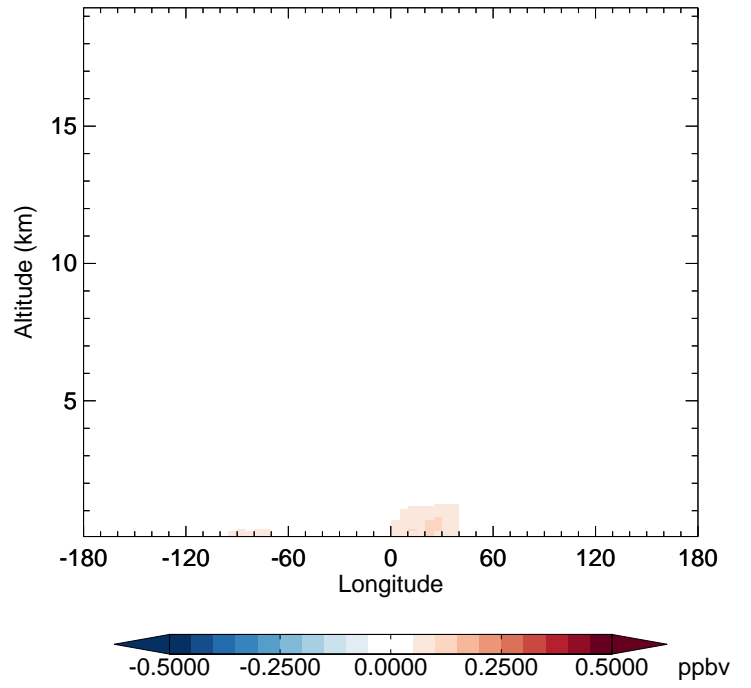
v11-02d - v11-02c CH 2 O - Diff along 42N for Jan
