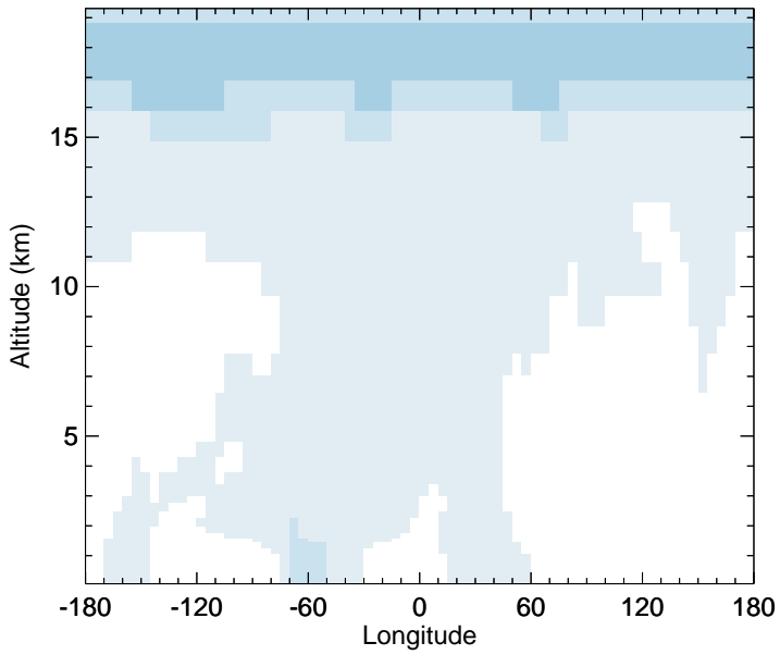
v11-02d - v11-02c C2H6 - Diff along 15S for Jan
