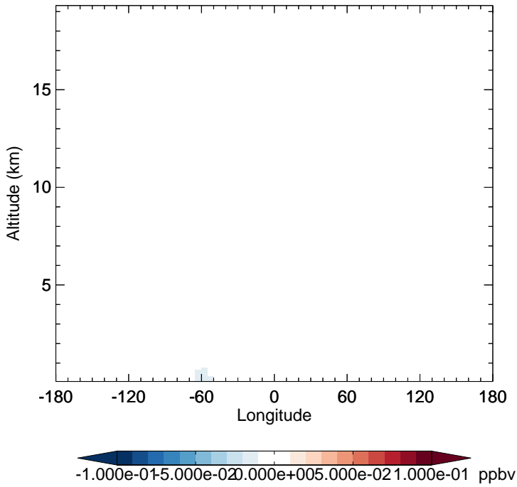
v11-02d - v11-02a ISOPND - Diff along 15S for Jan
