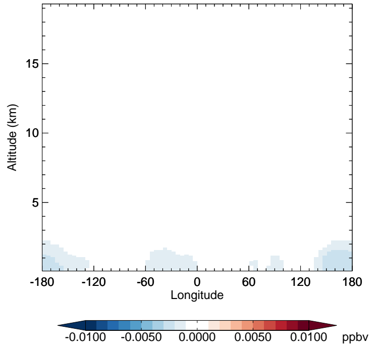
v11-02d - v11-02a HOBr - Diff along 42N for Jan
