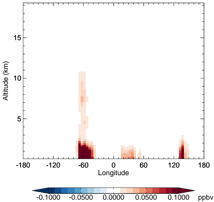
v11-02d - v11-02a HPALD - Diff along 15S for Jan
