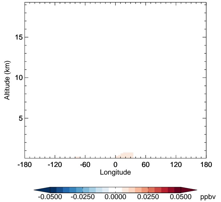
v11-02d - v11-02a RCHO - Diff along 42N for Jan
