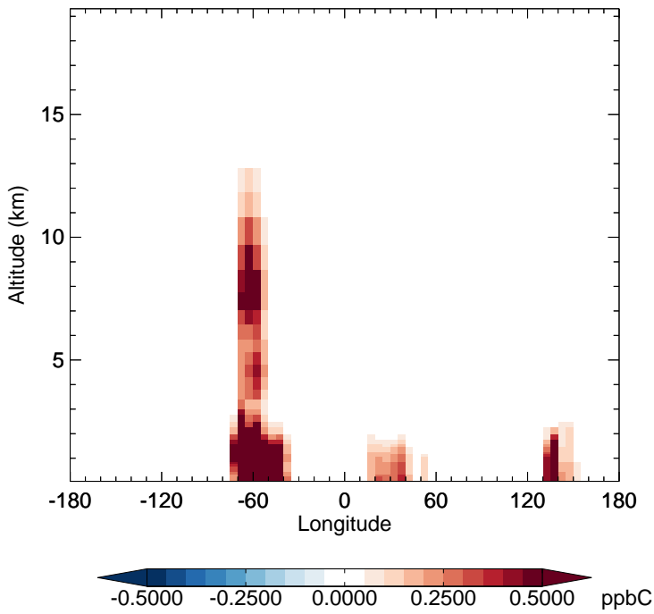
v11-02d - v11-02a ISOP - Diff along 15S for Jan
