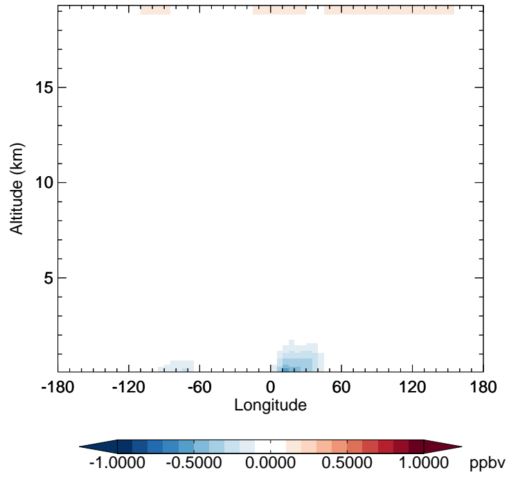
v11-02d - v11-02c NO 2 - Diff along 42N for Jan
