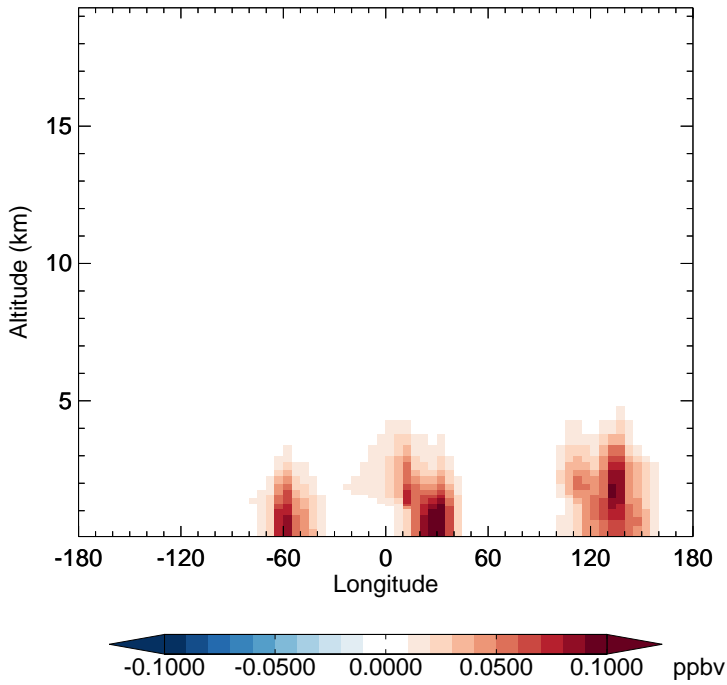
v11-02d - v11-02a INDIOL - Diff along 15S for Jan
