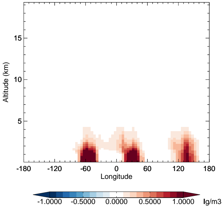
v11-02d - v11-02a SOAS - Diff along 15S for Jan
