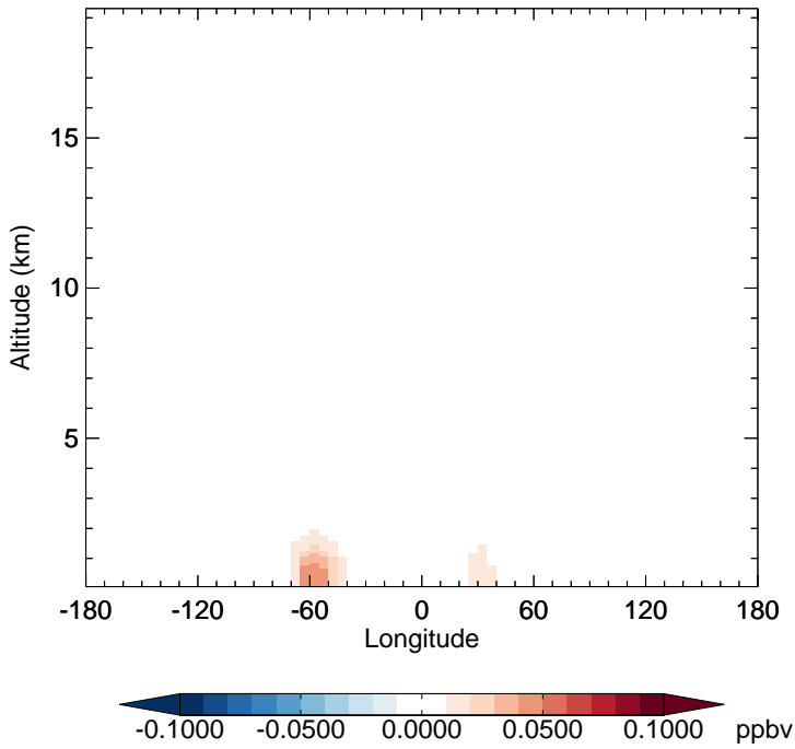
v11-02d - v11-02a TSOA0 - Diff along 15S for Jan
