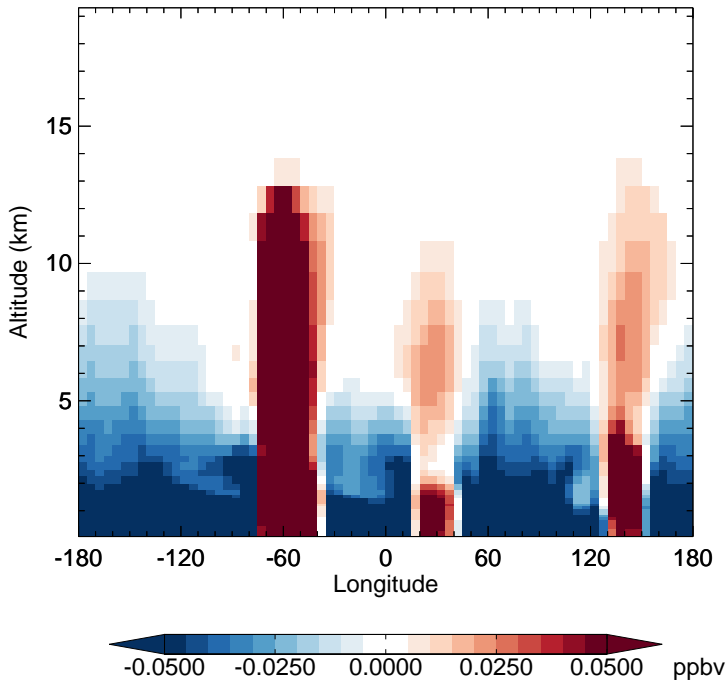
v11-02d - v11-02a MP - Diff along 15S for Jan
