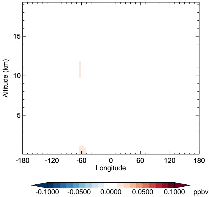
v11-02d - v11-02a TSOA2 - Diff along 15S for Jan
