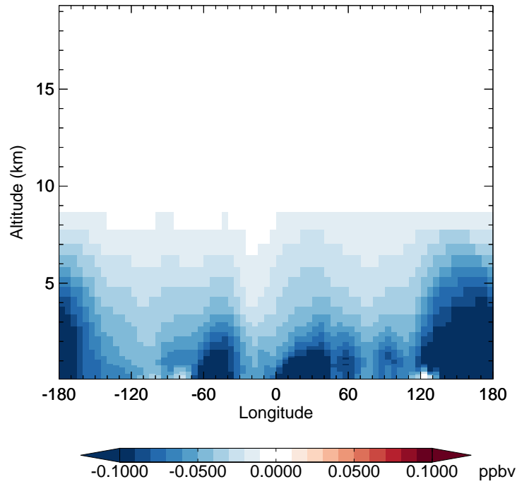
v11-02d - v11-02a TOLU - Diff along 42N for Jan
