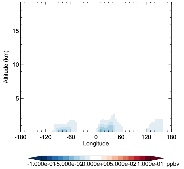
v11-02d - v11-02c EOH - Diff along 42N for Jan
