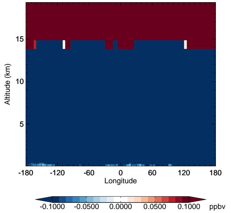
v11-02d - v11-02c N2O - Diff along 42N for Jan
