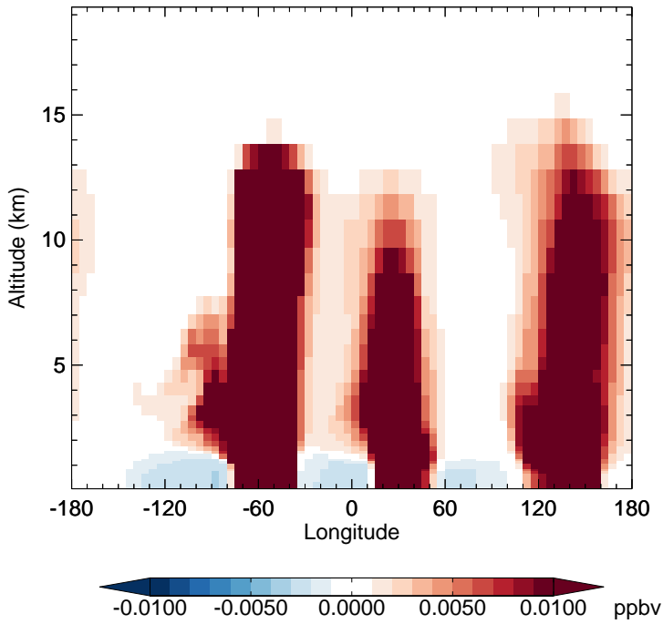
v11-02d - v11-02a MAP - Diff along 15S for Jan
