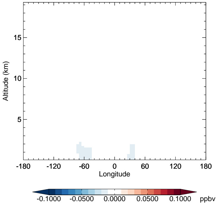
v11-02d - v11-02c BENZ - Diff along 15S for Jan
