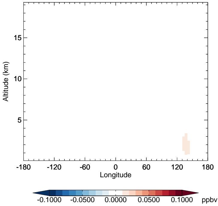
v11-02d - v11-02c IONITA - Diff along 15S for Jan
