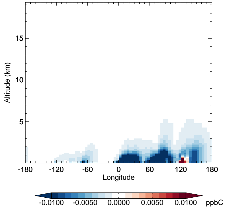
v11-02d - v11-02a PRPE - Diff along 42N for Jan
