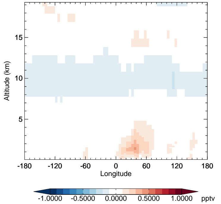
v11-02d - v11-02c HO2 - Diff along 42N for Jan
