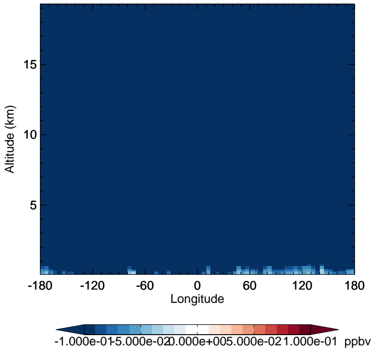
v11-02d - v11-02c N2O - Diff along 15S for Jan
