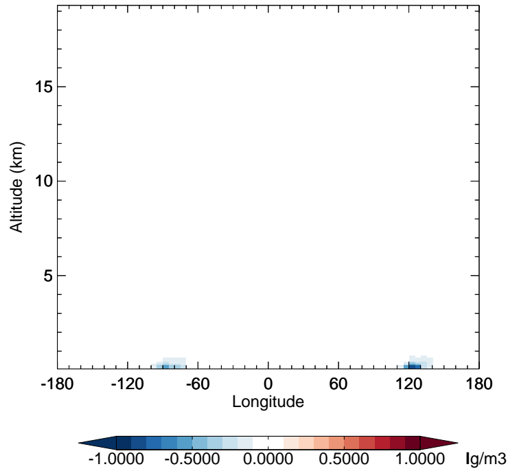
v11-02d - v11-02a NH4 - Diff along 42N for Jan
