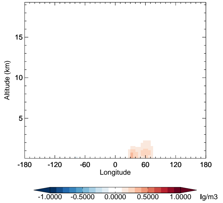
v11-02d - v11-02c SO4 - Diff along 42N for Jan
