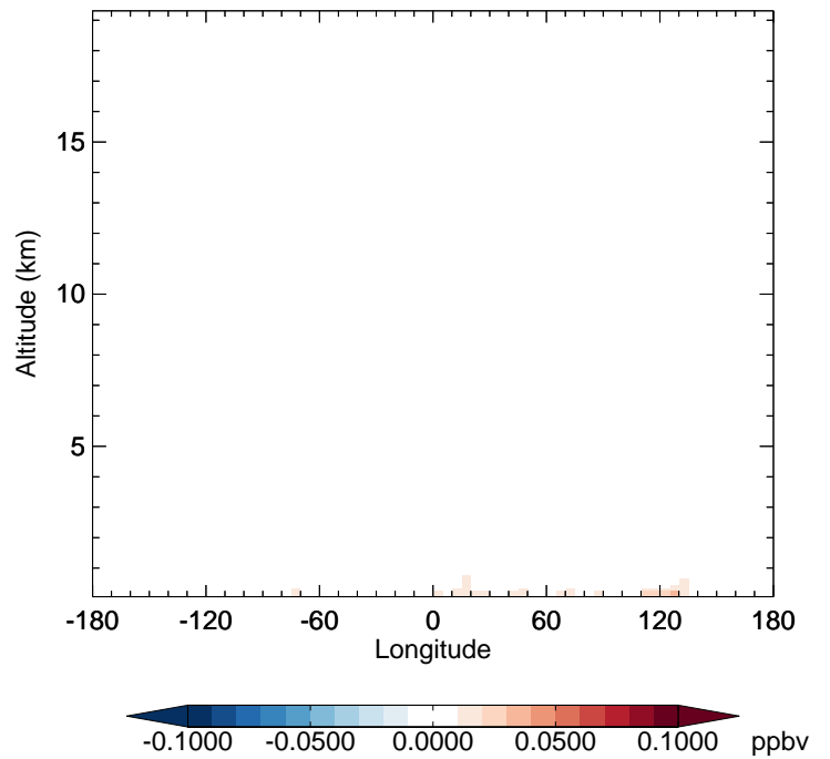
v11-02d - v11-02a GLYX - Diff along 42N for Jan
