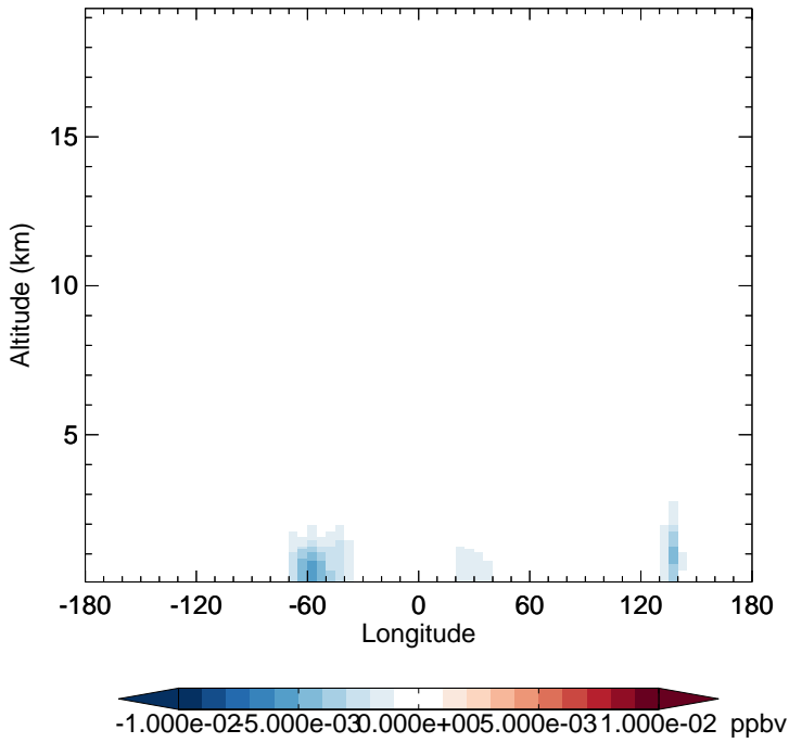
v11-02d - v11-02a MACRN - Diff along 15S for Jan
