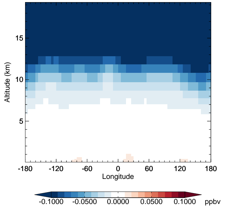
v11-02d - v11-02a HCl - Diff along 42N for Jan
