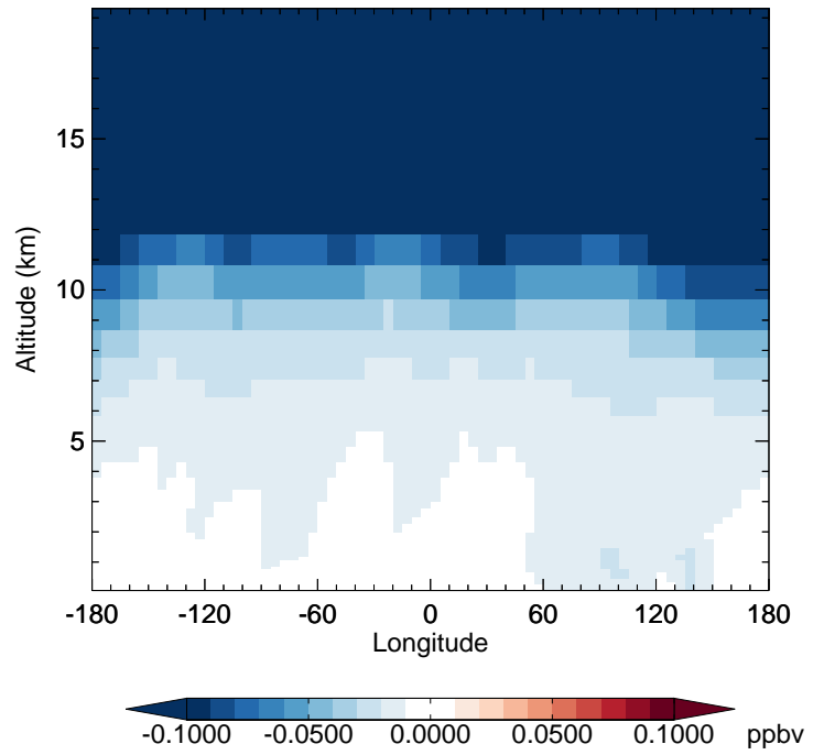
v11-02d - v11-02c HCl - Diff along 42N for Jan
