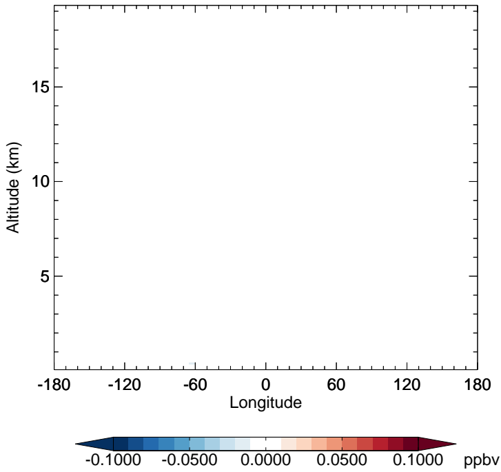
v11-02d - v11-02a ISOG1 - Diff along 15S for Jan
